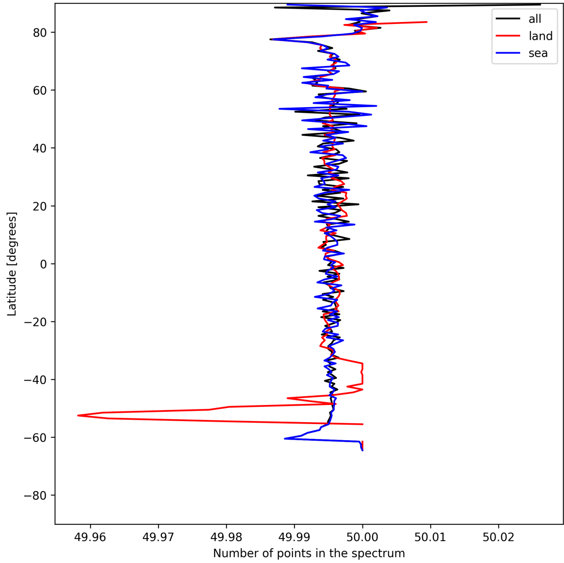
Figure 25: Zonal average of “Number of points in the spectrum” for 2025-06-28 to 2025-06-29.
