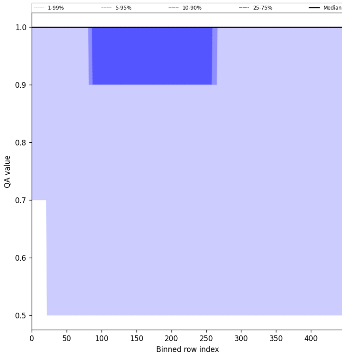
Figure 44: Along track statistics of “QA value” for 2025-06-28 to 2025-06-29
