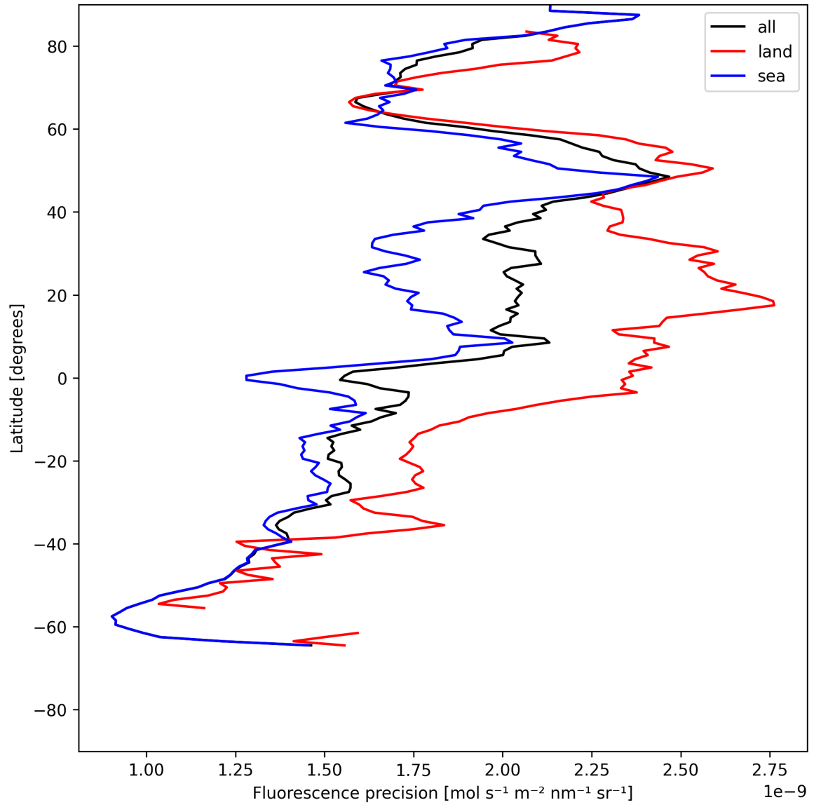
Figure 22: Zonal average of “Fluorescence precision” for 2025-06-28 to 2025-06-29.
