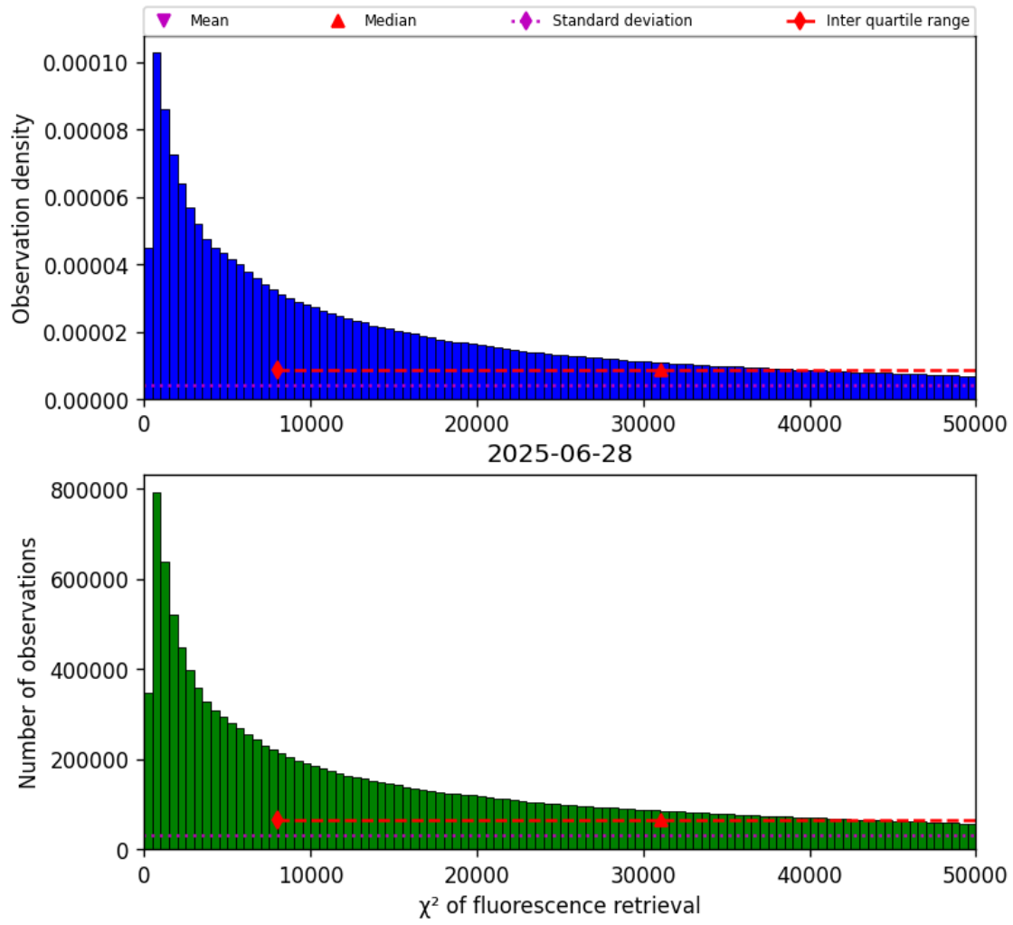
Figure 40: Histogram of “ \chi^2 of fluorescence retrieval” for 2025-06-28 to 2025-06-29
