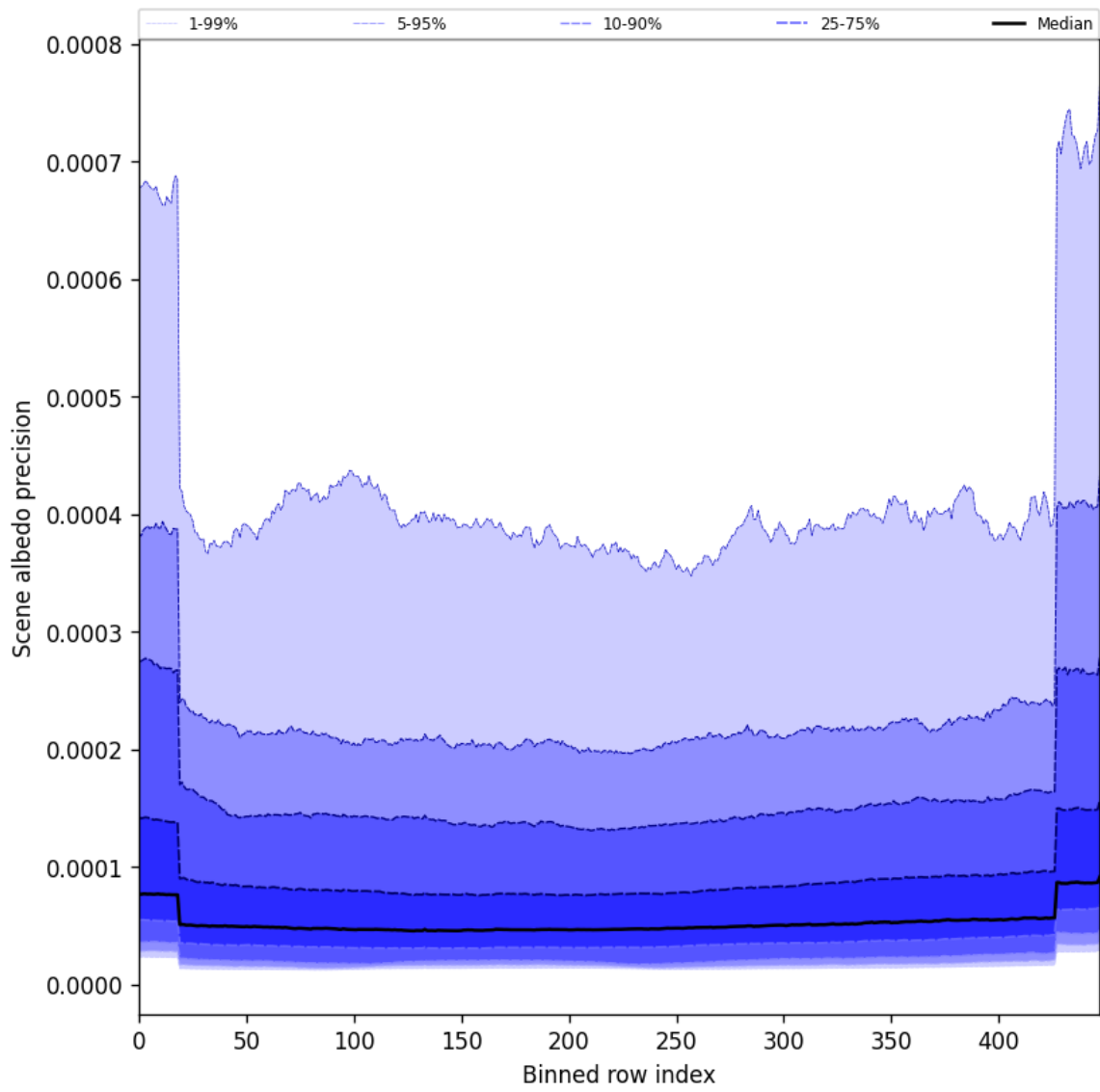
Figure 50: Along track statistics of “Scene albedo precision” for 2025-06-28 to 2025-06-29
