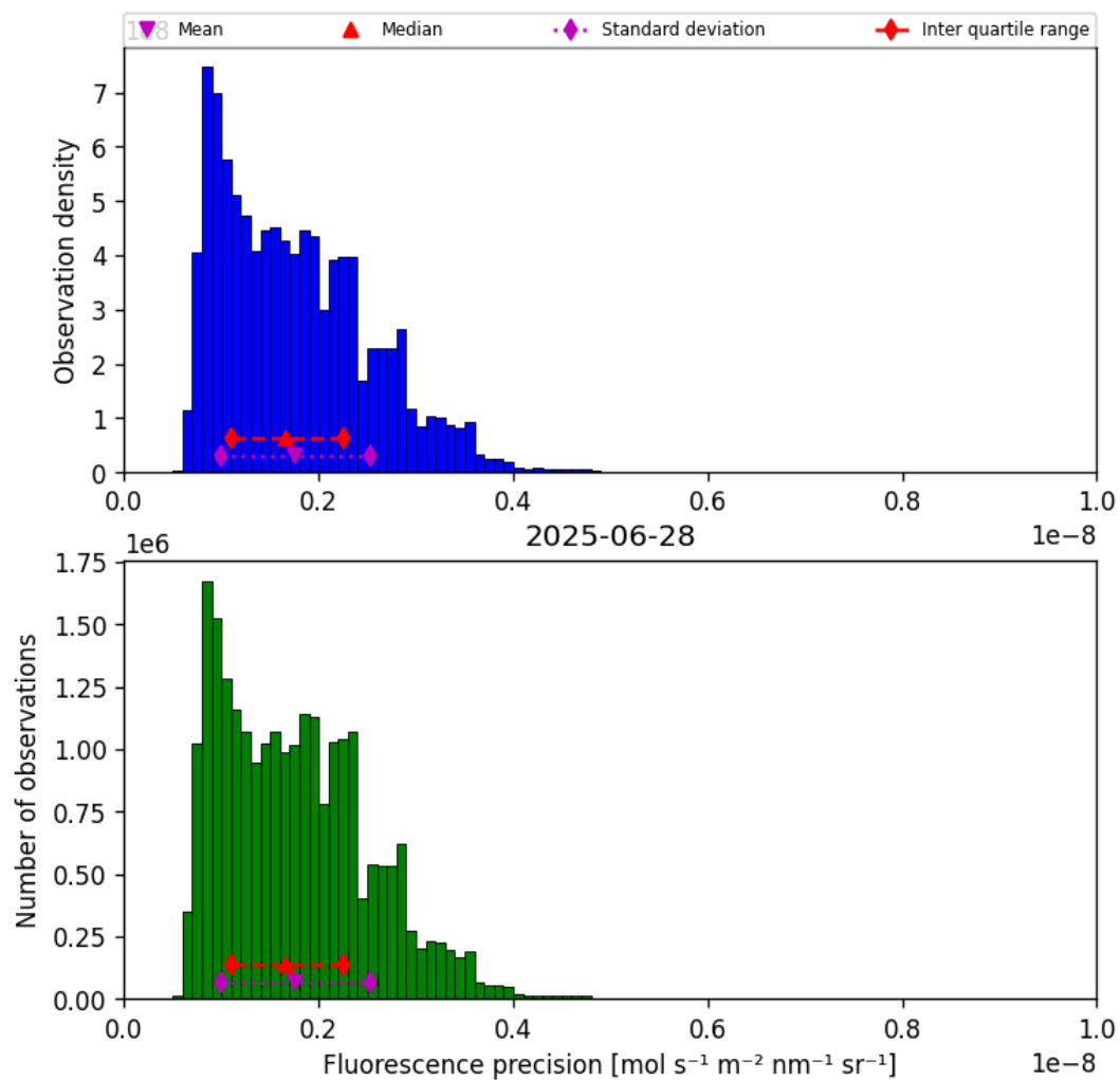
Figure 39: Histogram of “Fluorescence precision” for 2025-06-28 to 2025-06-29
