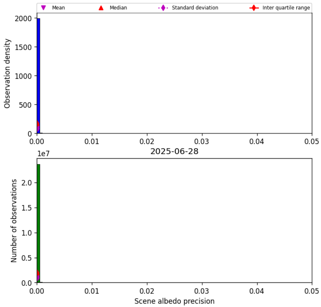
Figure 33: Histogram of “Scene albedo precision” for 2025-06-28 to 2025-06-29
