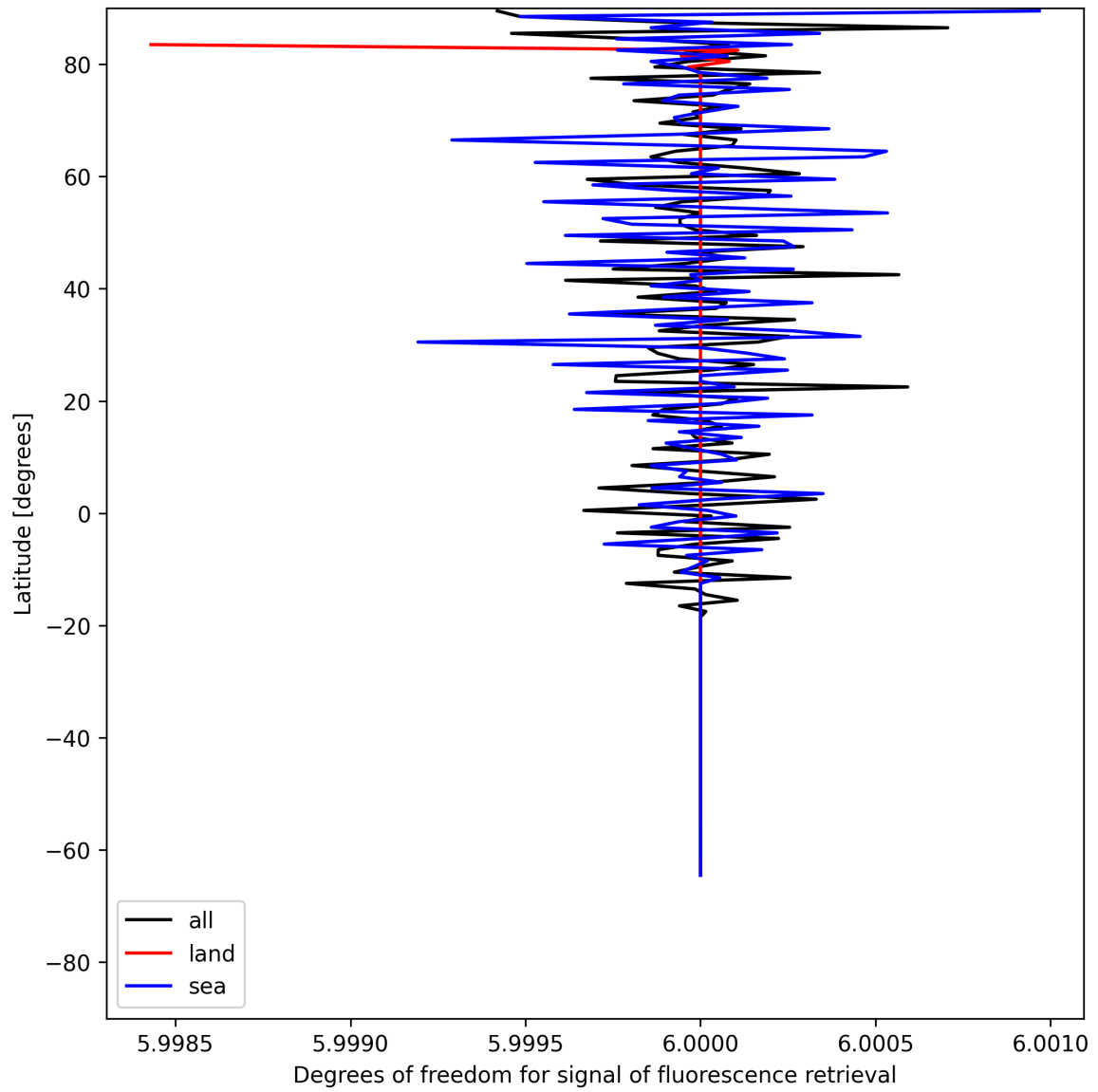
Figure 24: Zonal average of “Degrees of freedom for signal of fluorescence retrieval” for 2025-06-28 to 2025-06-29.
