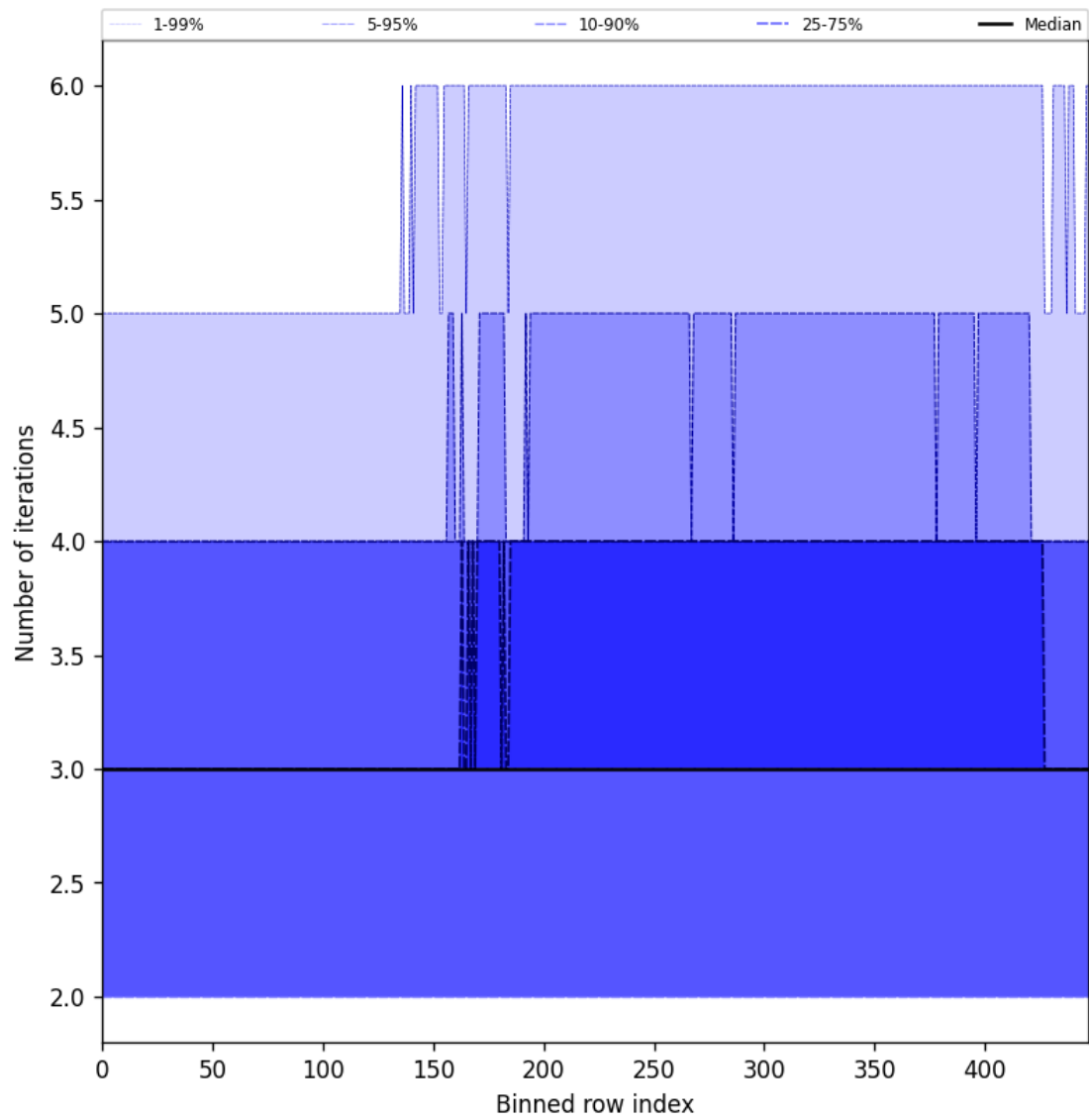
Figure 54: Along track statistics of “Number of iterations” for 2025-06-28 to 2025-06-29
