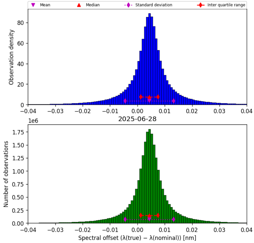
Figure 43: Histogram of “Spectral offset ( \lambda_{\text{true}} - \lambda_{\text{nominal}} )” for 2025-06-28 to 2025-06-29
