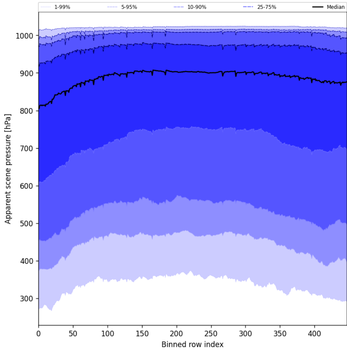
Figure 51: Along track statistics of “Apparent scene pressure” for 2025-06-28 to 2025-06-29
