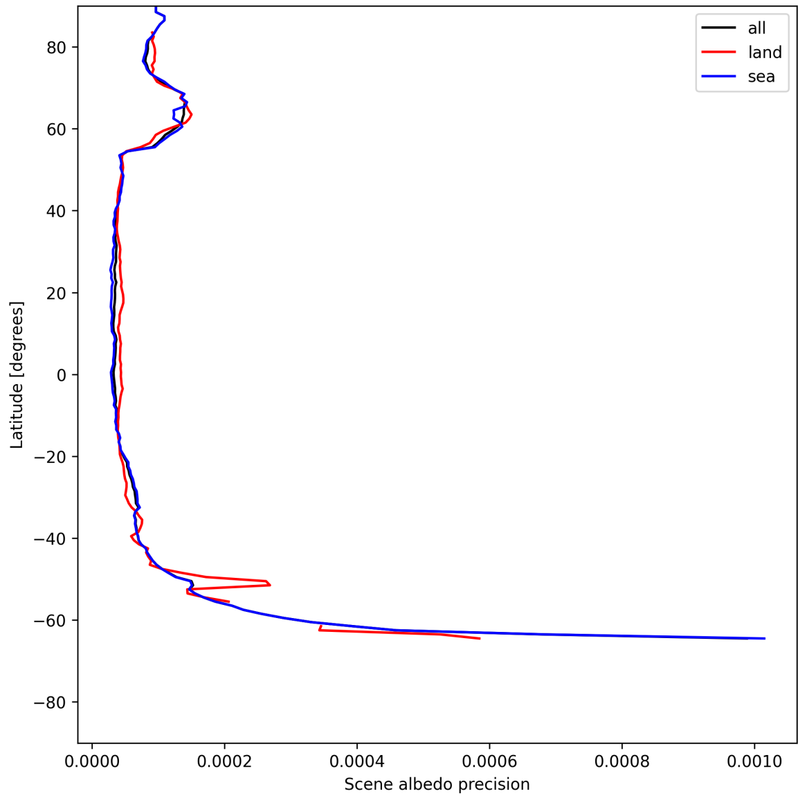
Figure 16: Zonal average of “Scene albedo precision” for 2025-06-28 to 2025-06-29.
