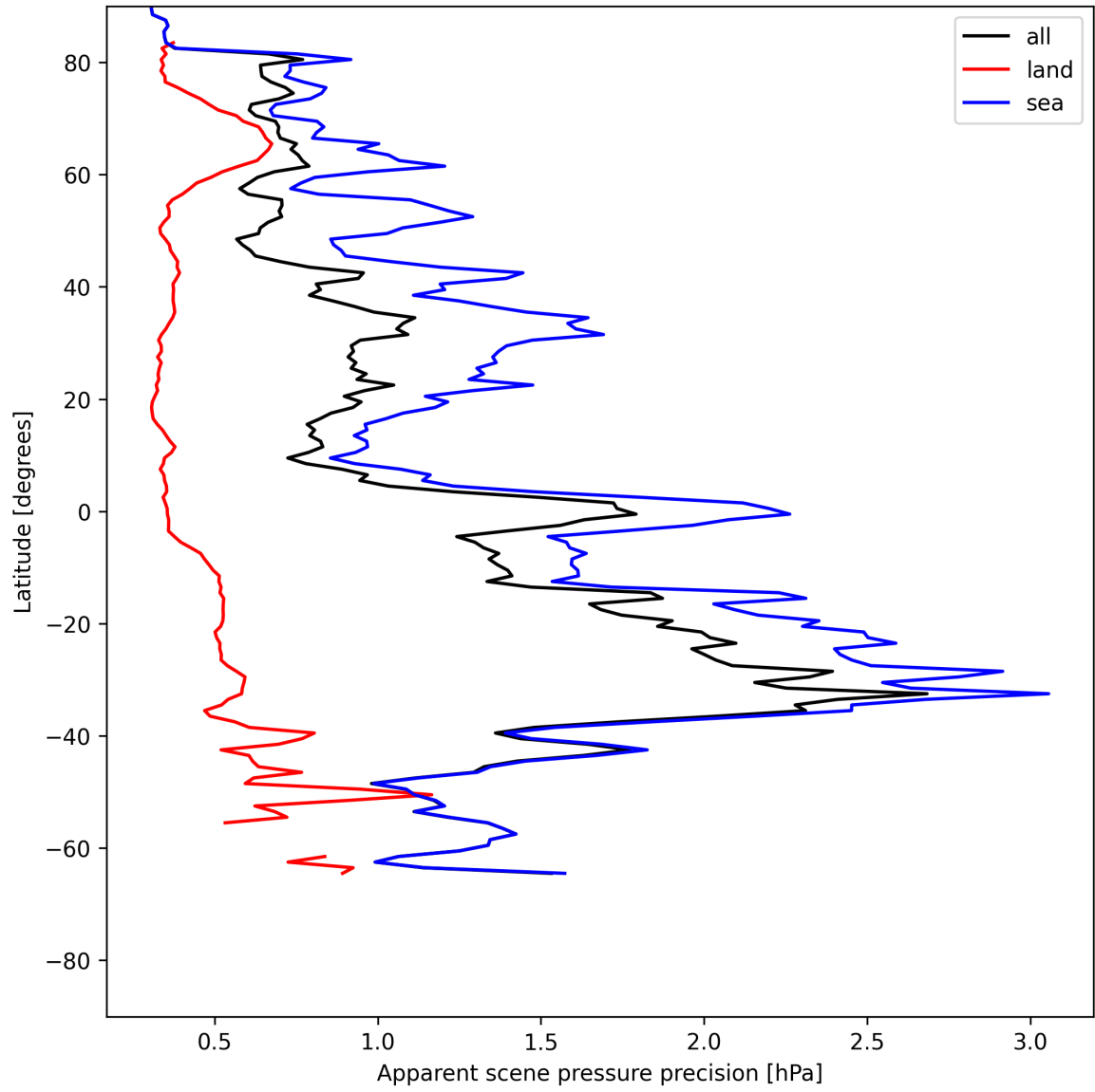
Figure 18: Zonal average of “Apparent scene pressure precision” for 2025-06-28 to 2025-06-29.
