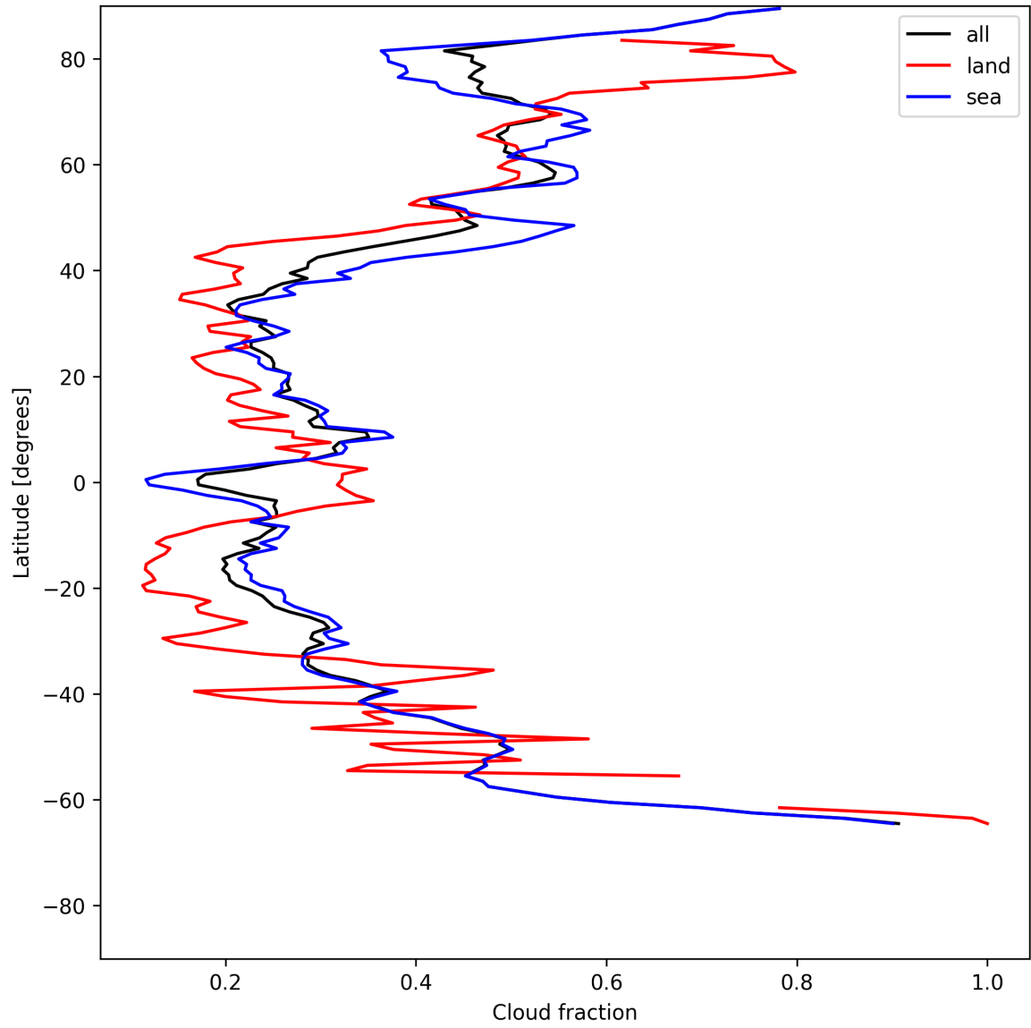
Figure 13: Zonal average of “Cloud fraction” for 2025-06-28 to 2025-06-29.
