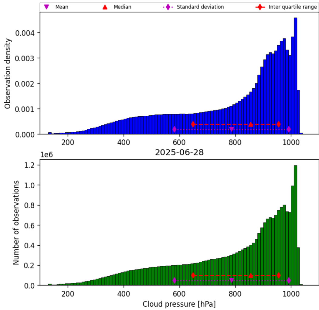
Figure 28: Histogram of “Cloud pressure” for 2025-06-28 to 2025-06-29
