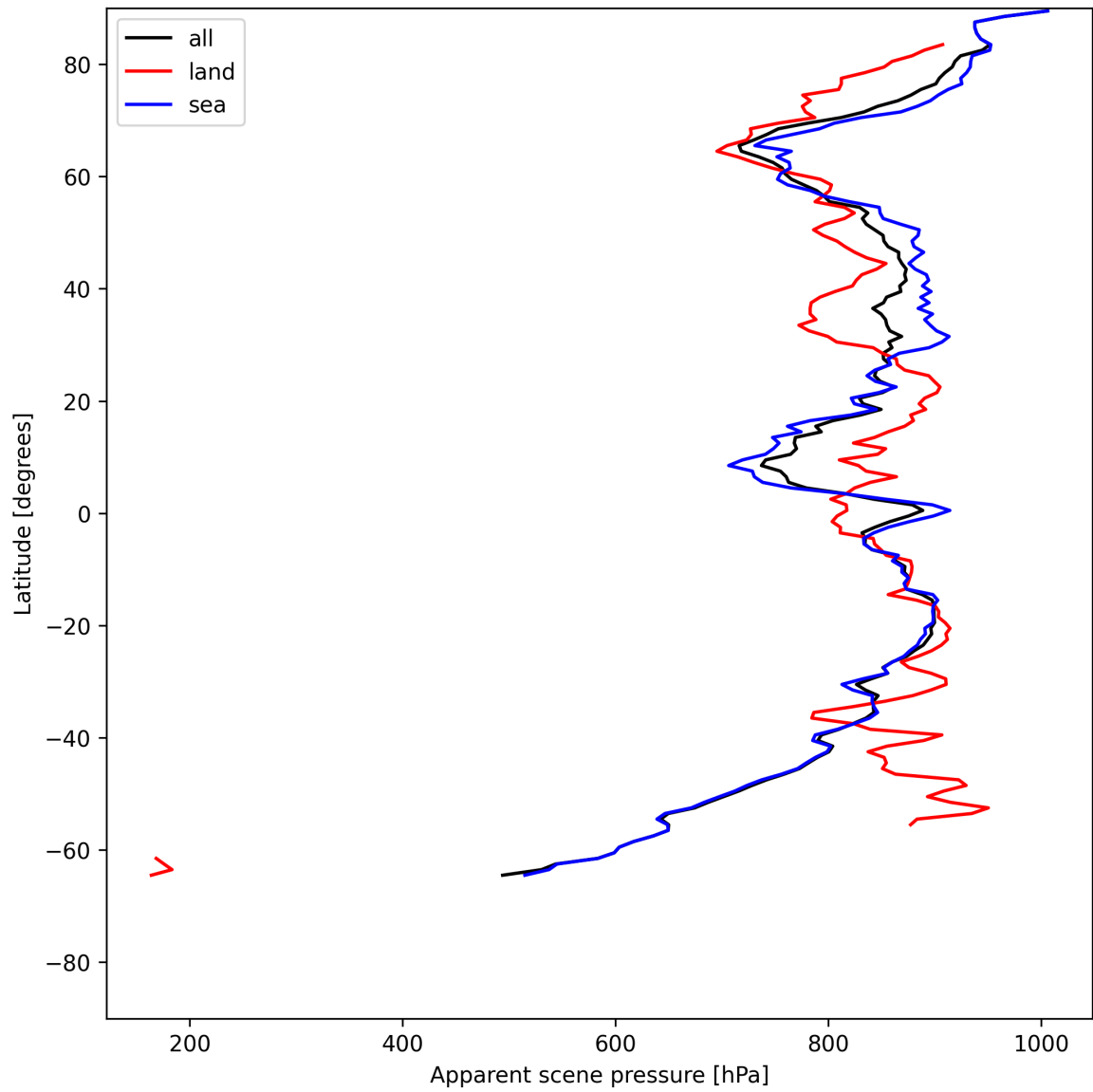
Figure 17: Zonal average of “Apparent scene pressure” for 2025-06-28 to 2025-06-29.
