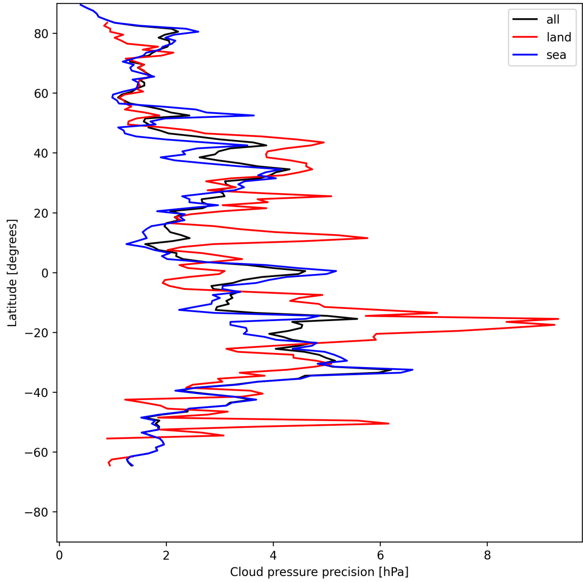
Figure 12: Zonal average of “Cloud pressure precision” for 2025-06-28 to 2025-06-29.
