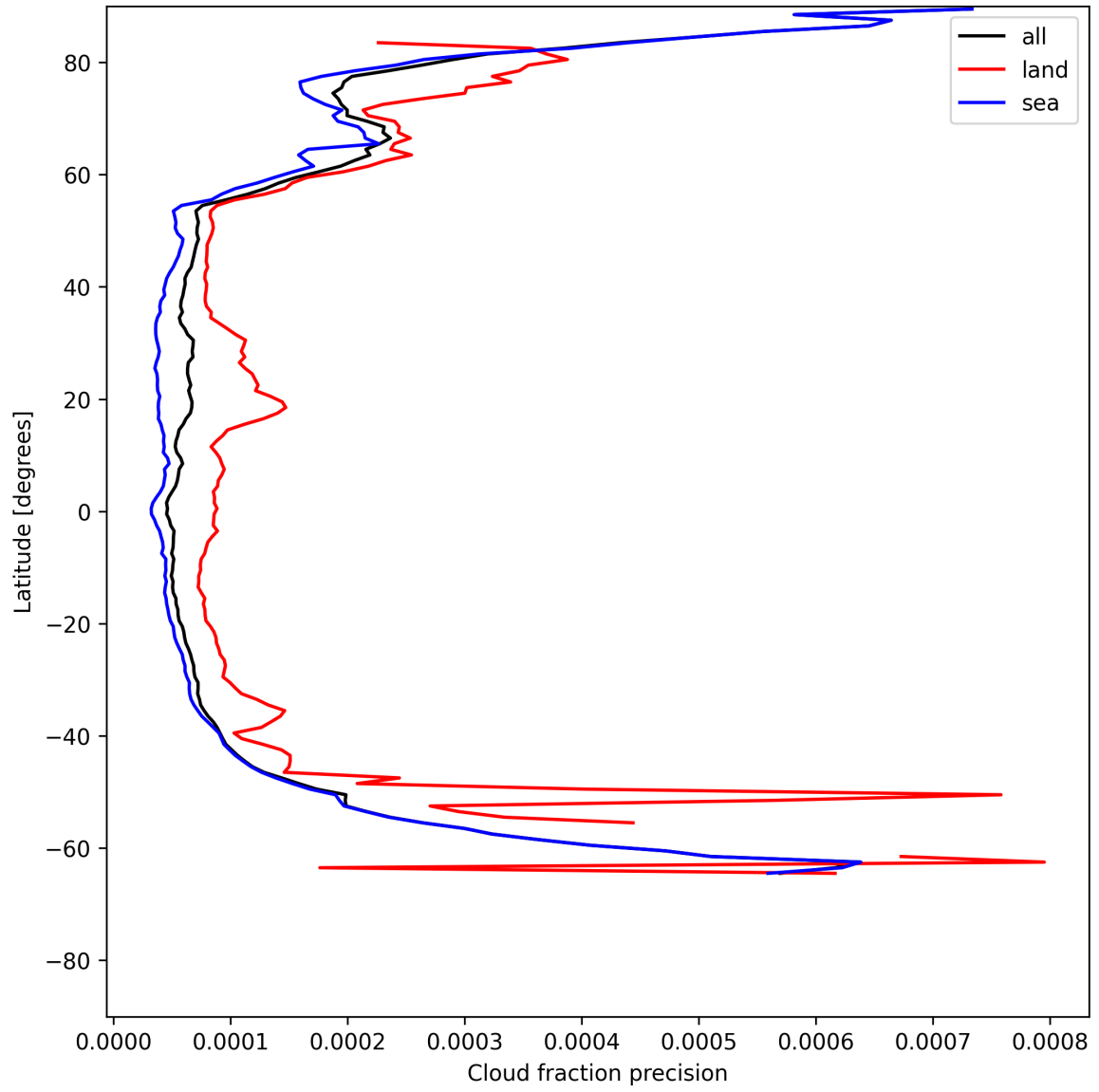
Figure 14: Zonal average of “Cloud fraction precision” for 2025-06-28 to 2025-06-29.
