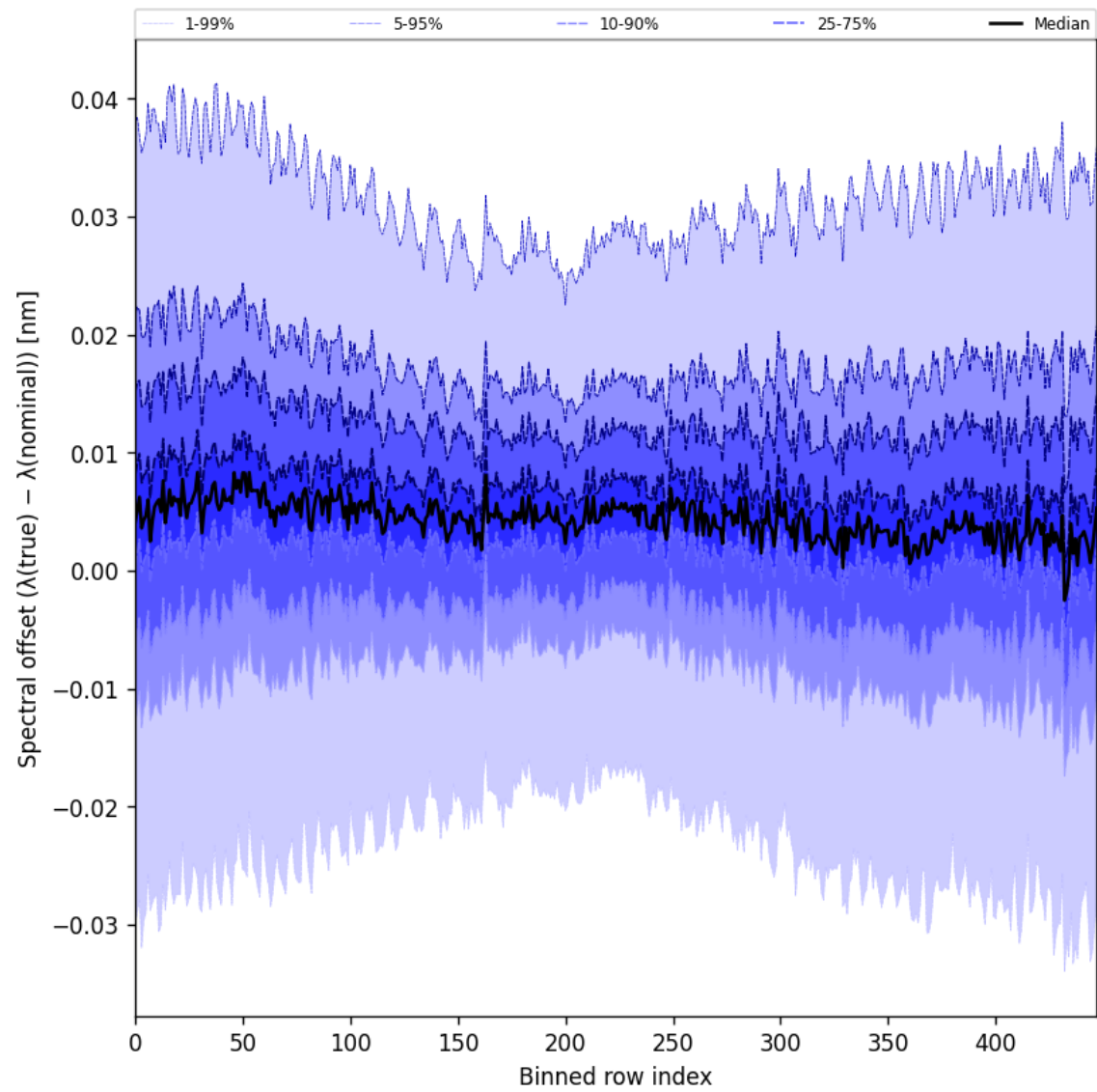
Figure 60: Along track statistics of “Spectral offset ( \lambda_{\text{true}} - \lambda_{\text{nominal}} )” for 2025-06-28 to 2025-06-29
