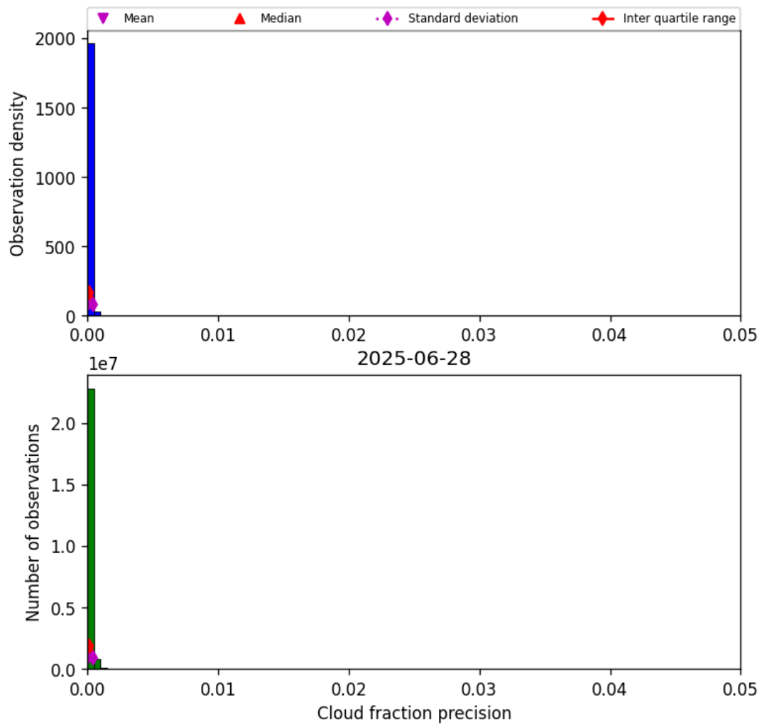
Figure 31: Histogram of “Cloud fraction precision” for 2025-06-28 to 2025-06-29
