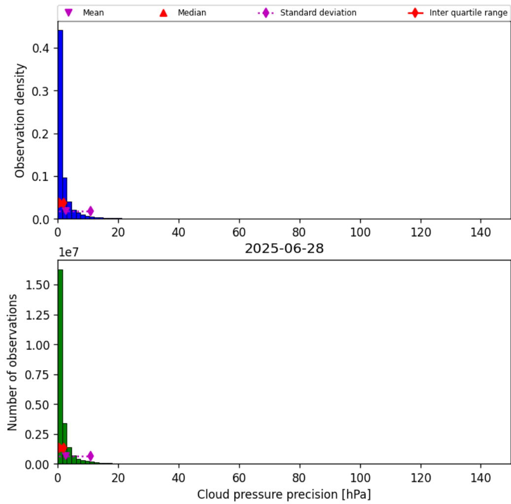
Figure 29: Histogram of “Cloud pressure precision” for 2025-06-28 to 2025-06-29
