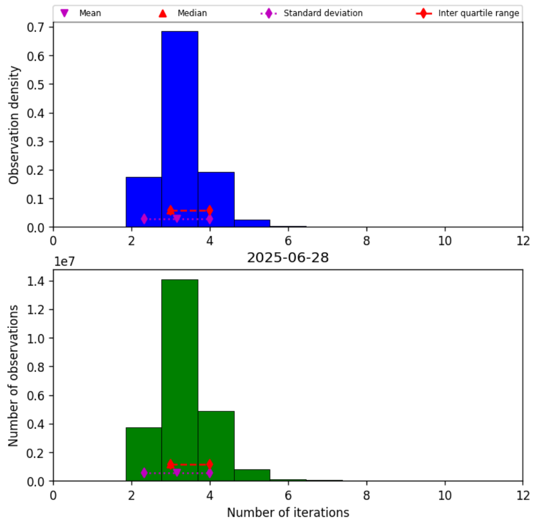
Figure 37: Histogram of “Number of iterations” for 2025-06-28 to 2025-06-29
