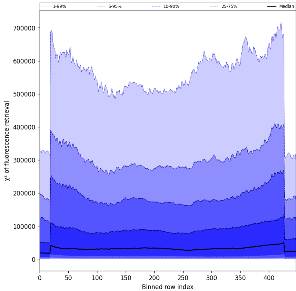
Figure 57: Along track statistics of “ \chi^2 of fluorescence retrieval” for 2025-06-28 to 2025-06-29
