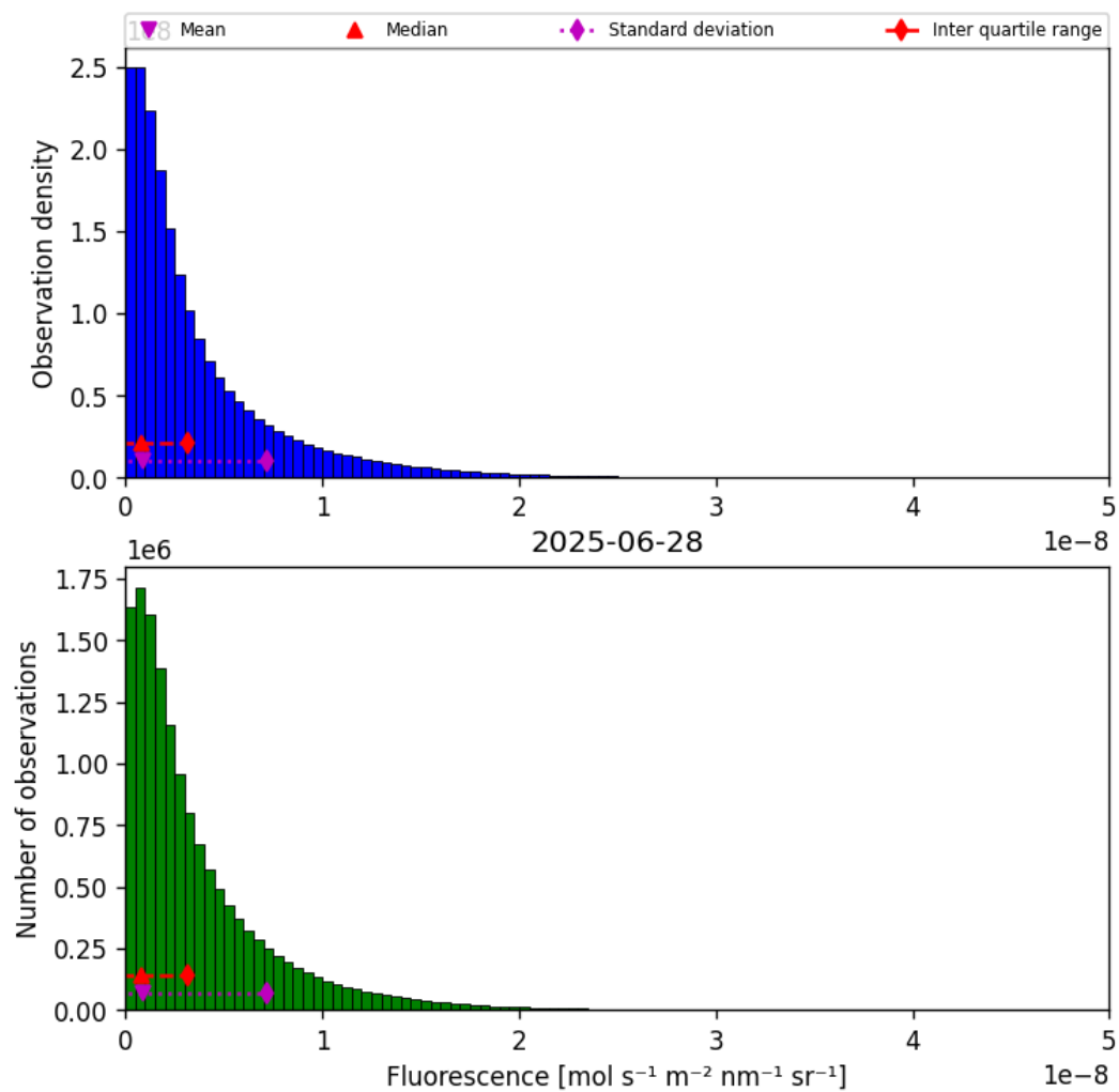
Figure 38: Histogram of “Fluorescence” for 2025-06-28 to 2025-06-29
