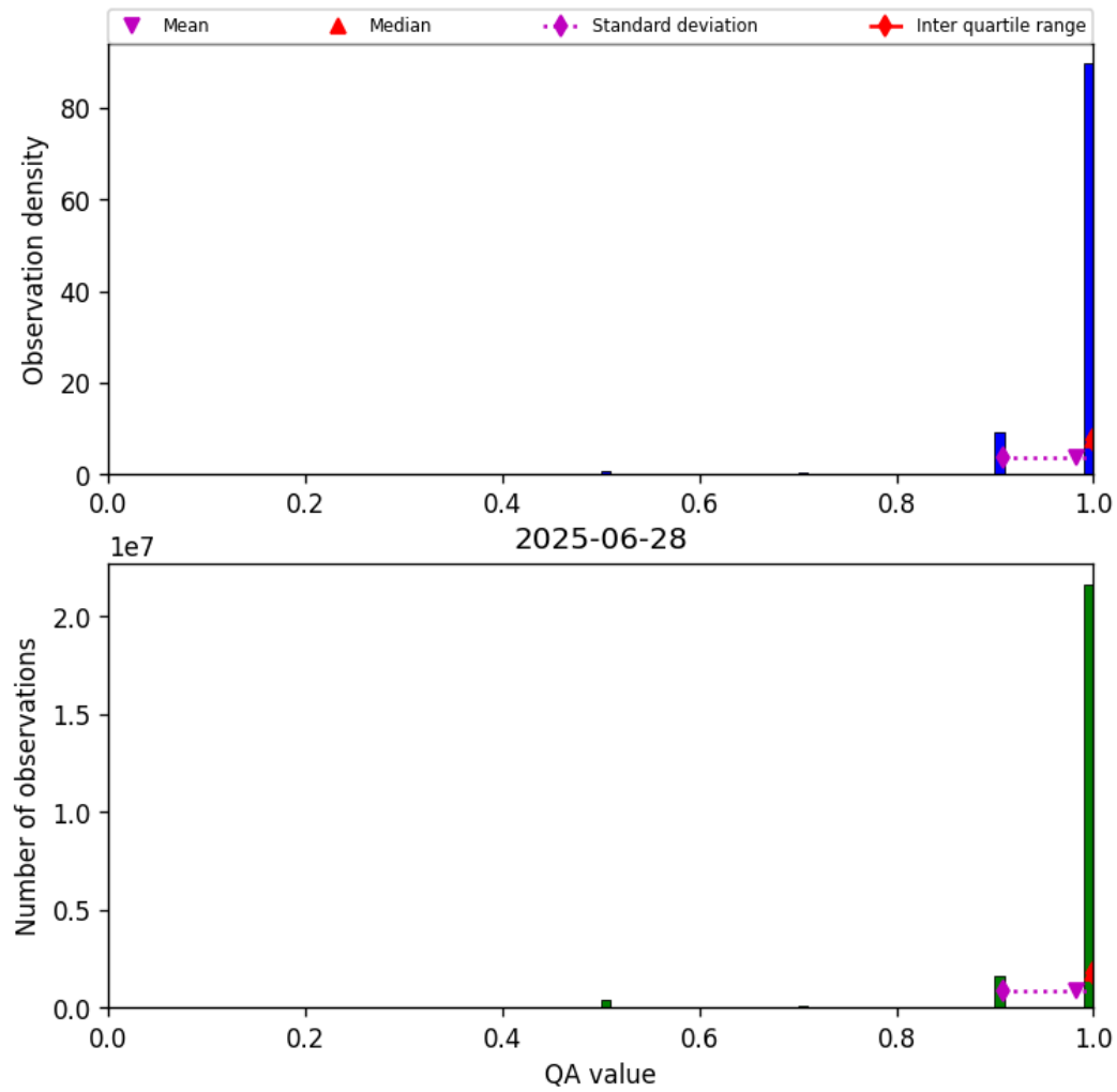
Figure 27: Histogram of “QA value” for 2025-06-28 to 2025-06-29
