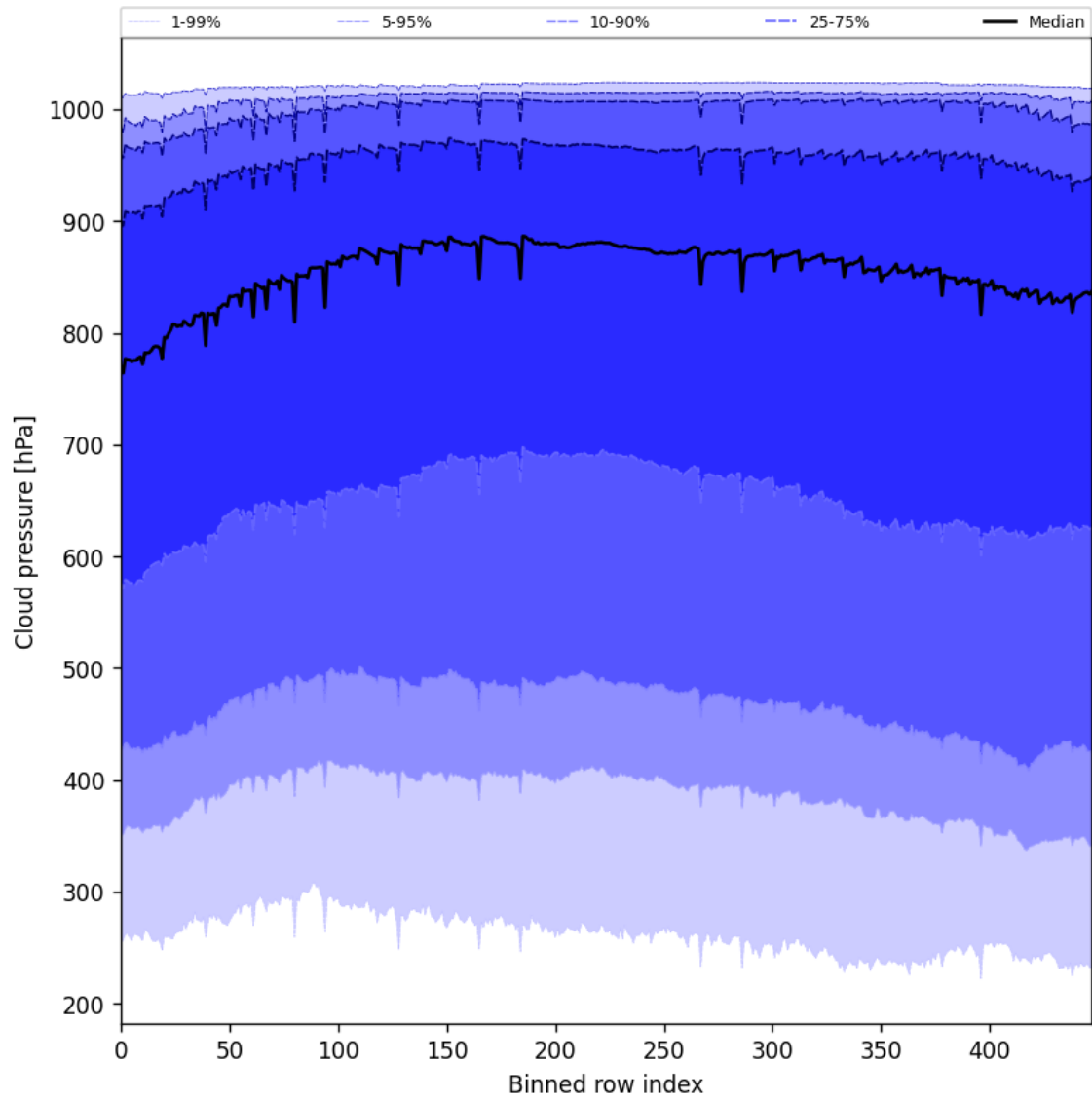
Figure 45: Along track statistics of “Cloud pressure” for 2025-06-28 to 2025-06-29
