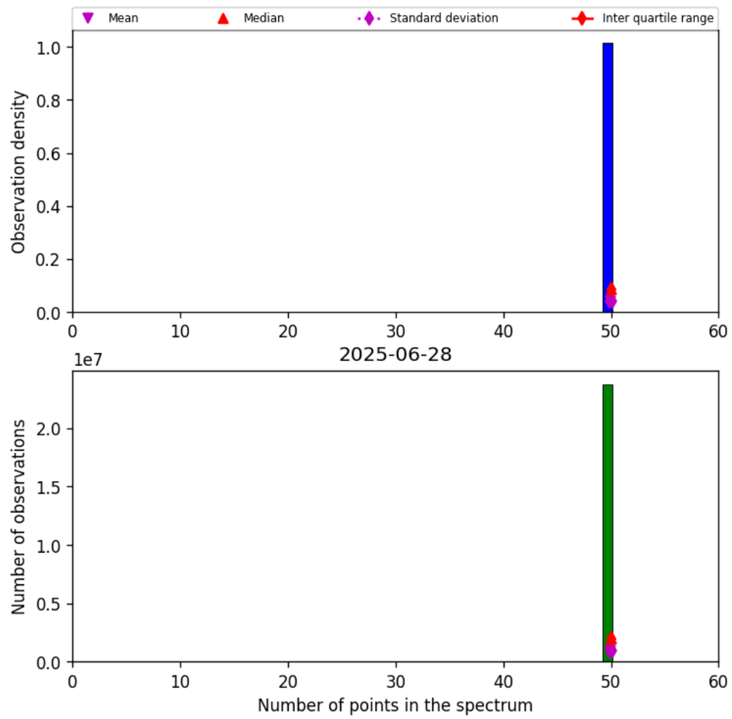
Figure 42: Histogram of "Number of points in the spectrum" for 2025-06-28 to 2025-06-29
