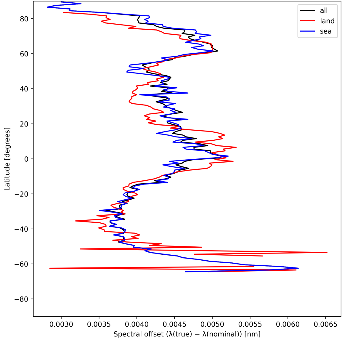
Figure 26: Zonal average of “Spectral offset ( \lambda_{\text{true}} - \lambda_{\text{nominal}} )” for 2025-06-28 to 2025-06-29.
