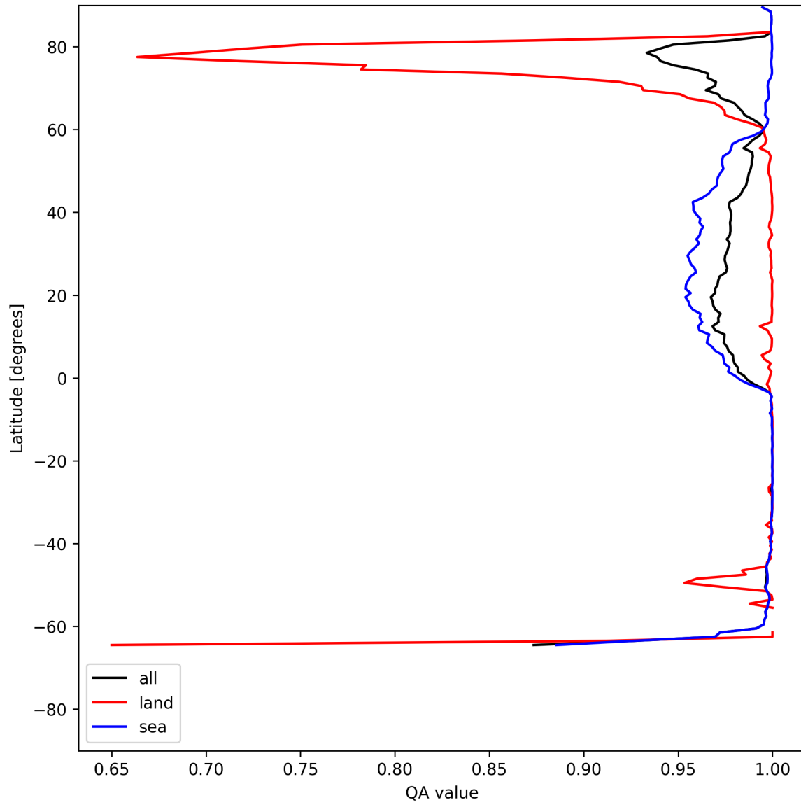
Figure 10: Zonal average of “QA value” for 2025-06-28 to 2025-06-29.
