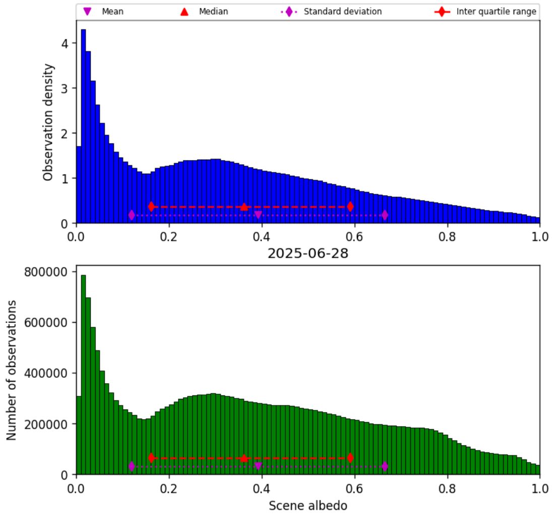
Figure 32: Histogram of “Scene albedo” for 2025-06-28 to 2025-06-29
