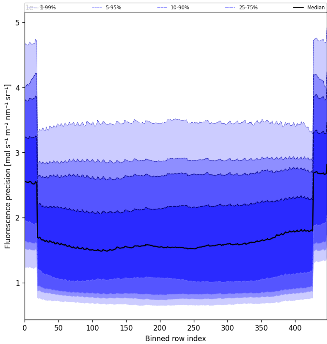
Figure 56: Along track statistics of “Fluorescence precision” for 2025-06-28 to 2025-06-29
