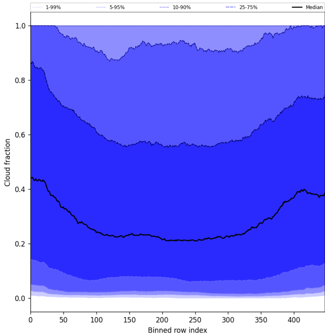
Figure 47: Along track statistics of “Cloud fraction” for 2025-06-28 to 2025-06-29
