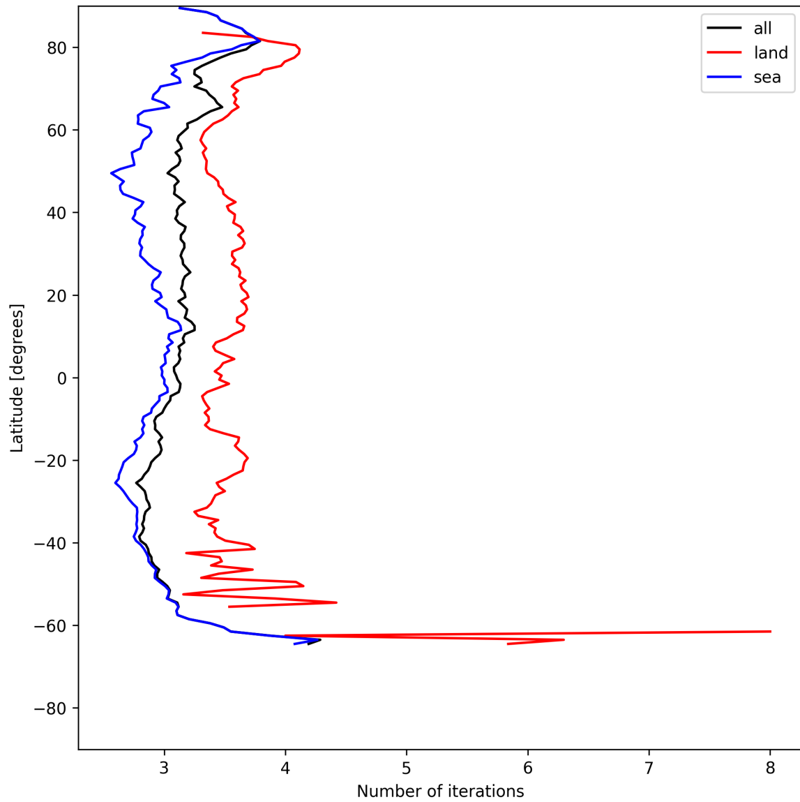
Figure 20: Zonal average of “Number of iterations” for 2025-06-28 to 2025-06-29.
