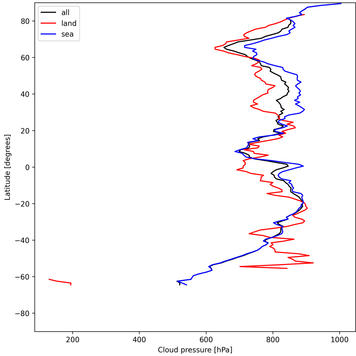
Figure 11: Zonal average of “Cloud pressure” for 2025-06-28 to 2025-06-29.
