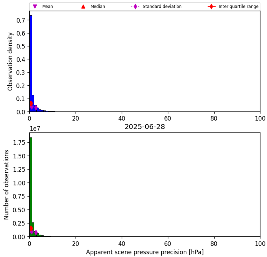
Figure 35: Histogram of “Apparent scene pressure precision” for 2025-06-28 to 2025-06-29
