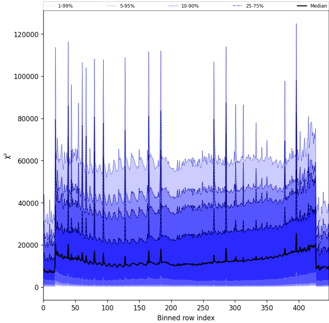
Figure 53: Along track statistics of “ \chi^2 ” for 2025-06-28 to 2025-06-29
