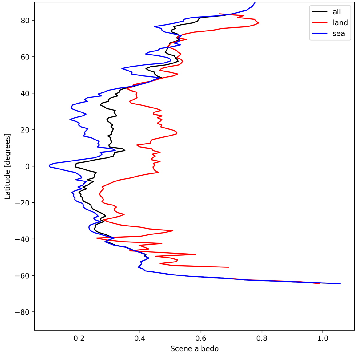
Figure 15: Zonal average of “Scene albedo” for 2025-06-28 to 2025-06-29.
