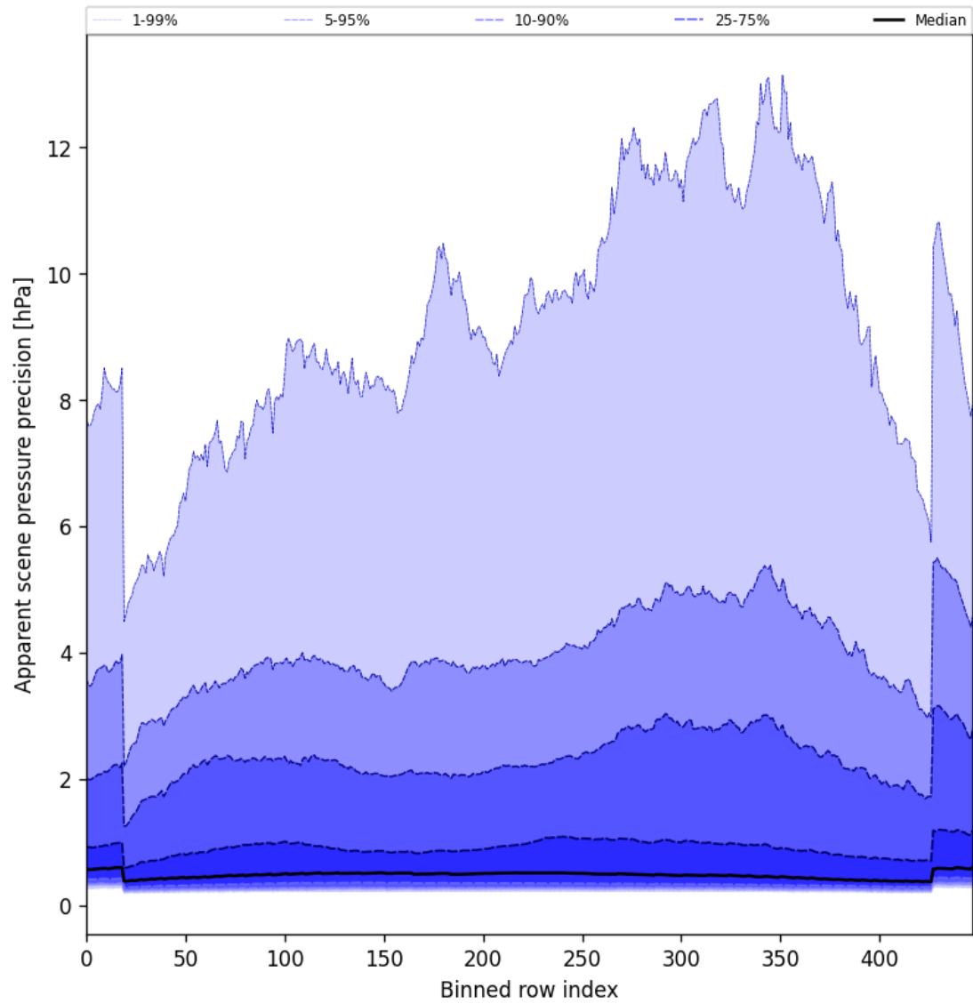
Figure 52: Along track statistics of “Apparent scene pressure precision” for 2025-06-28 to 2025-06-29
