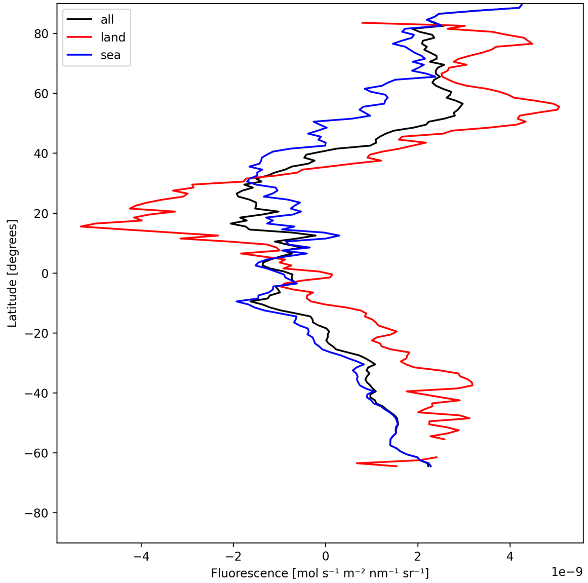
Figure 21: Zonal average of “Fluorescence” for 2025-06-28 to 2025-06-29.
