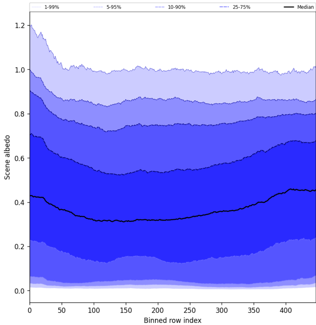
Figure 49: Along track statistics of “Scene albedo” for 2025-06-28 to 2025-06-29
