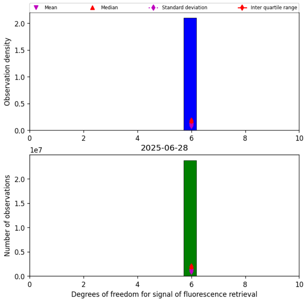
Figure 41: Histogram of “Degrees of freedom for signal of fluorescence retrieval” for 2025-06-28 to 2025-06-29
