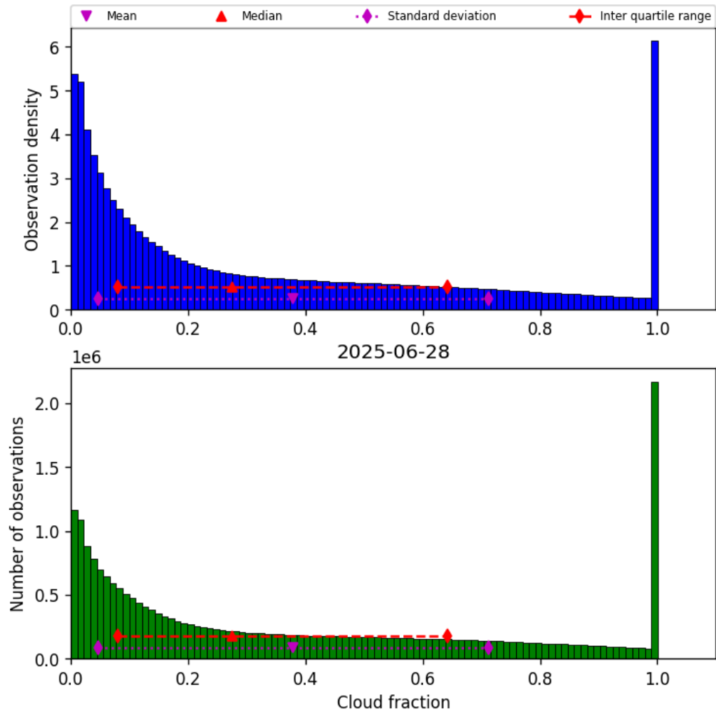
Figure 30: Histogram of “Cloud fraction” for 2025-06-28 to 2025-06-29
