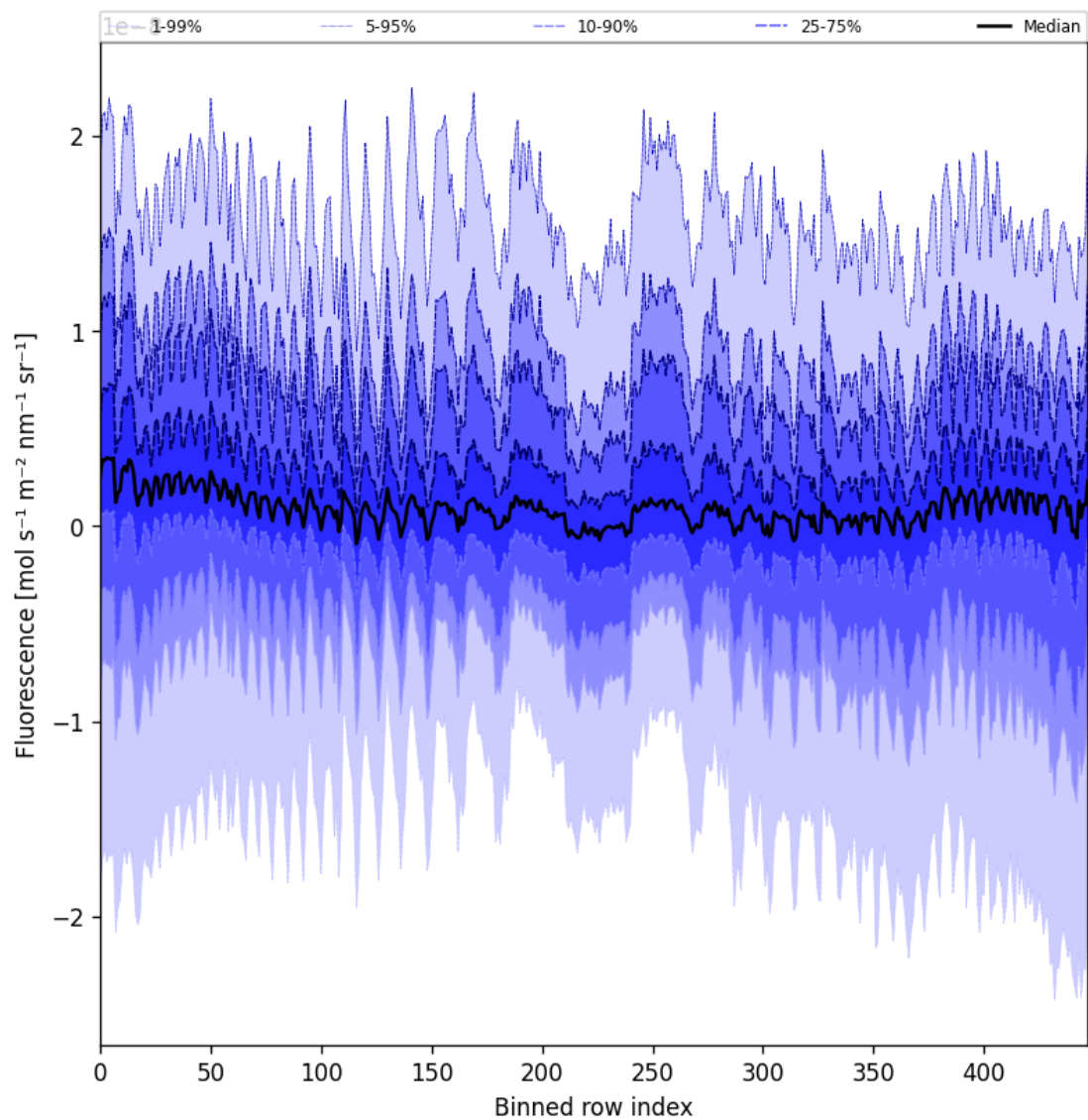
Figure 55: Along track statistics of “Fluorescence” for 2025-06-28 to 2025-06-29
