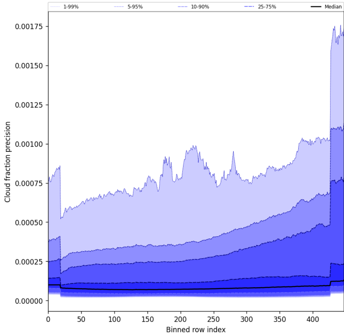
Figure 48: Along track statistics of “Cloud fraction precision” for 2025-06-28 to 2025-06-29
