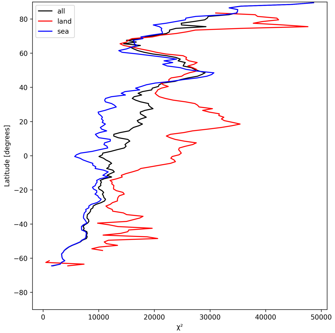
Figure 19: Zonal average of “ \chi^2 ” for 2025-06-28 to 2025-06-29.
