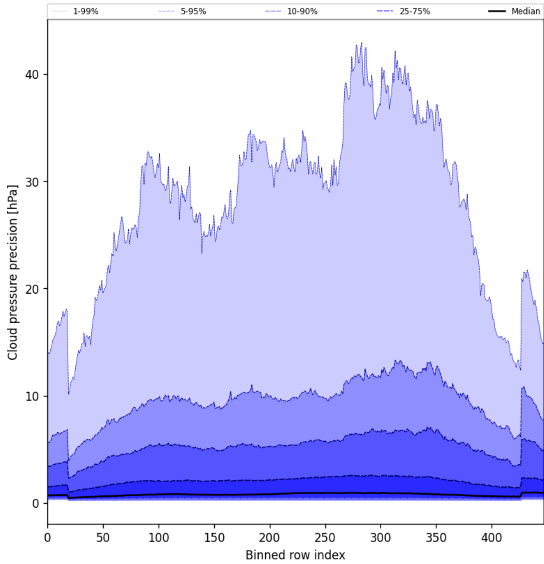
Figure 46: Along track statistics of “Cloud pressure precision” for 2025-06-28 to 2025-06-29
