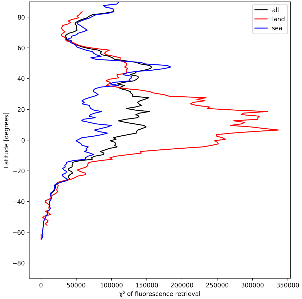
Figure 23: Zonal average of “ \chi^2 of fluorescence retrieval” for 2025-06-28 to 2025-06-29.
