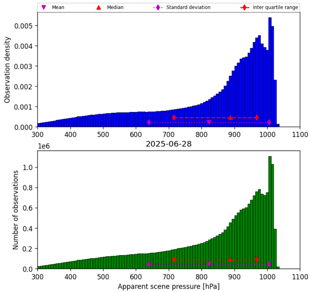
Figure 34: Histogram of “Apparent scene pressure” for 2025-06-28 to 2025-06-29
