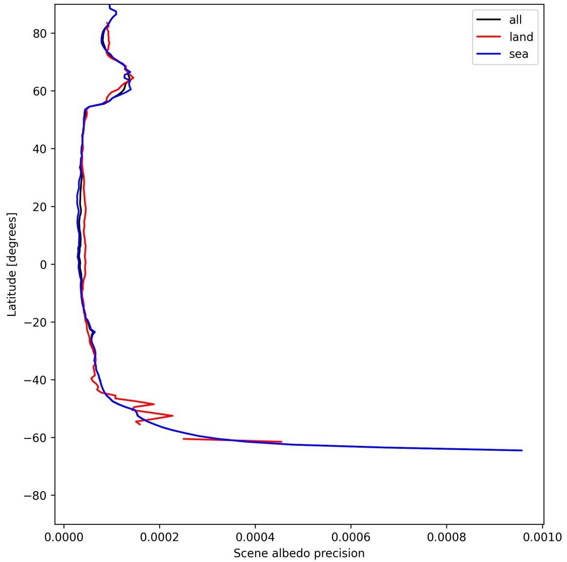
Figure 16: Zonal average of “Scene albedo precision” for 2025-06-29 to 2025-06-30.
