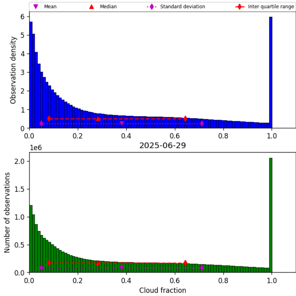
Figure 30: Histogram of “Cloud fraction” for 2025-06-29 to 2025-06-30
