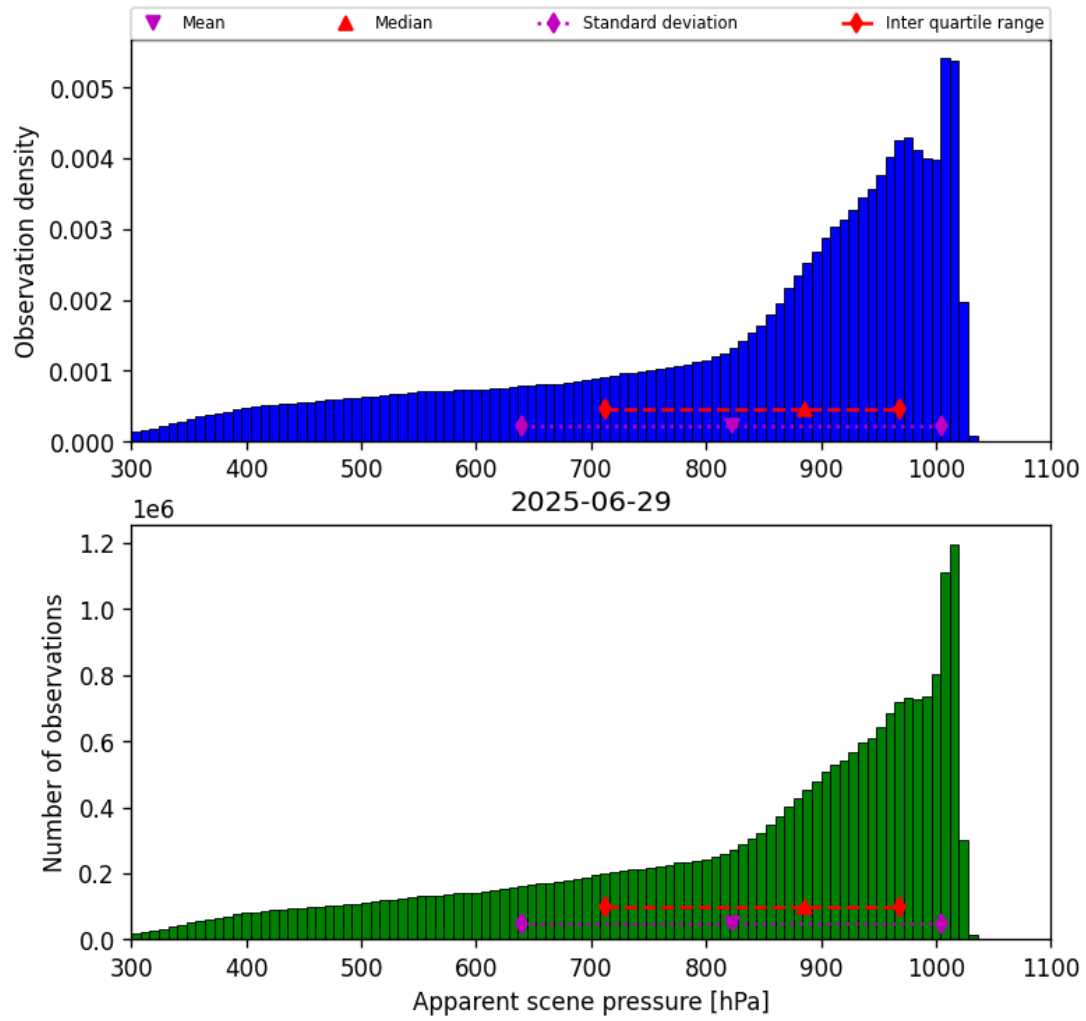
Figure 34: Histogram of “Apparent scene pressure” for 2025-06-29 to 2025-06-30
