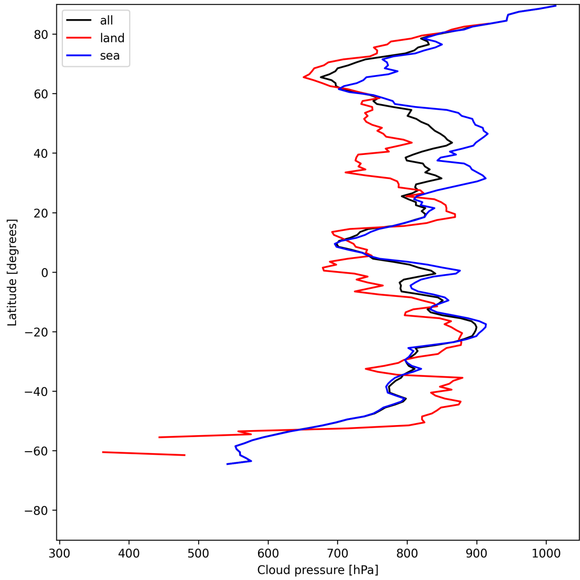
Figure 11: Zonal average of “Cloud pressure” for 2025-06-29 to 2025-06-30.
