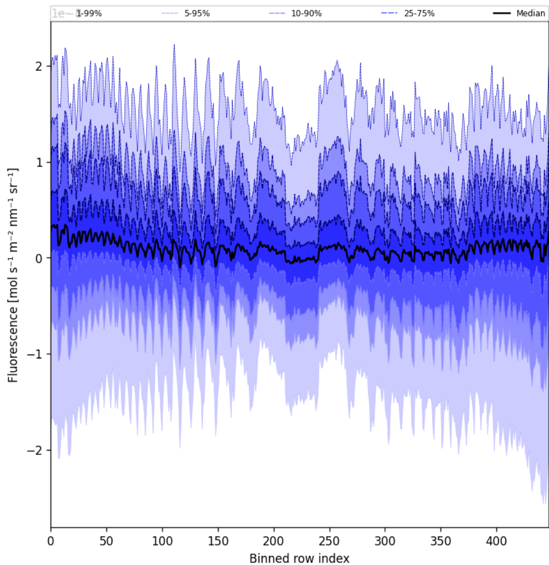
Figure 55: Along track statistics of "Fluorescence" for 2025-06-29 to 2025-06-30
