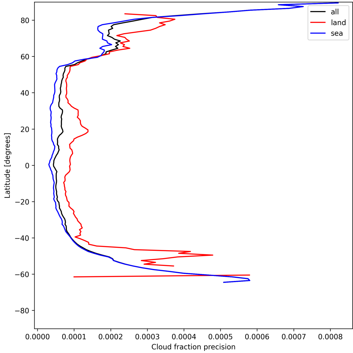
Figure 14: Zonal average of “Cloud fraction precision” for 2025-06-29 to 2025-06-30.
