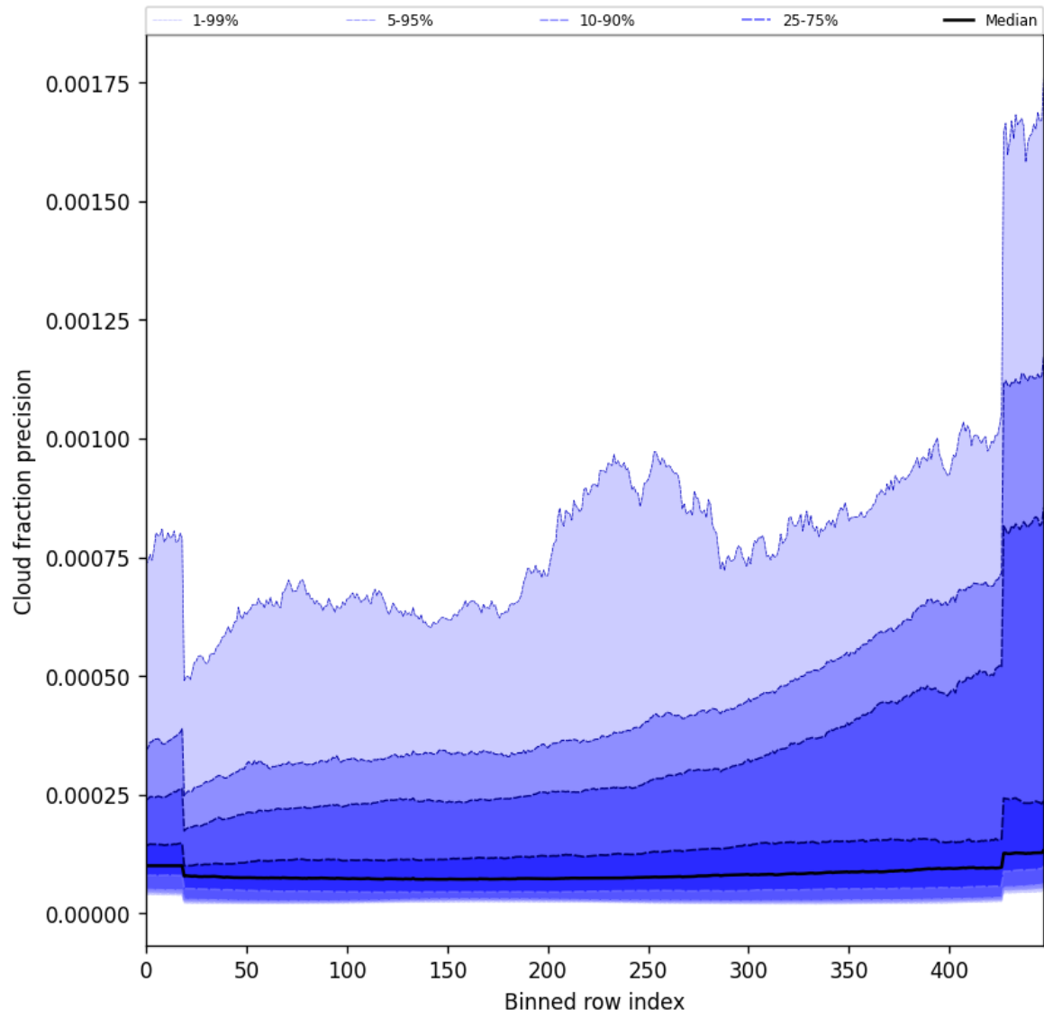
Figure 48: Along track statistics of “Cloud fraction precision” for 2025-06-29 to 2025-06-30
