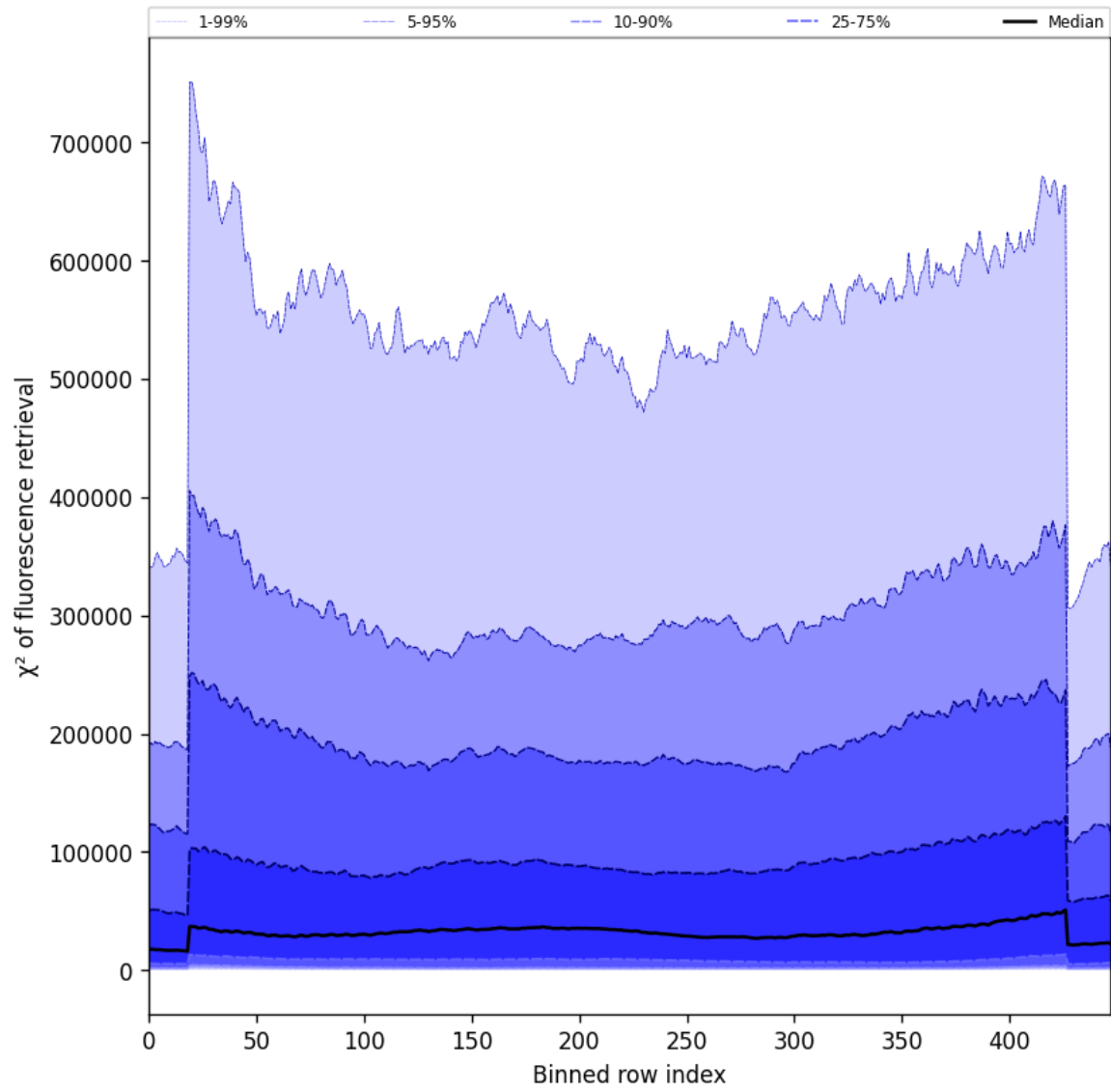
Figure 57: Along track statistics of “ \chi^2 of fluorescence retrieval” for 2025-06-29 to 2025-06-30
