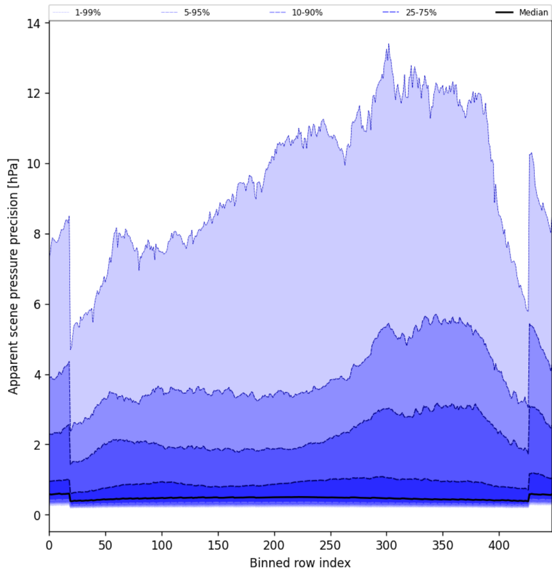
Figure 52: Along track statistics of “Apparent scene pressure precision” for 2025-06-29 to 2025-06-30
