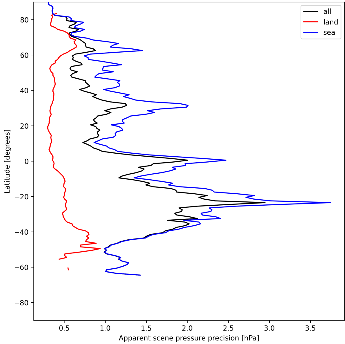
Figure 18: Zonal average of “Apparent scene pressure precision” for 2025-06-29 to 2025-06-30.
