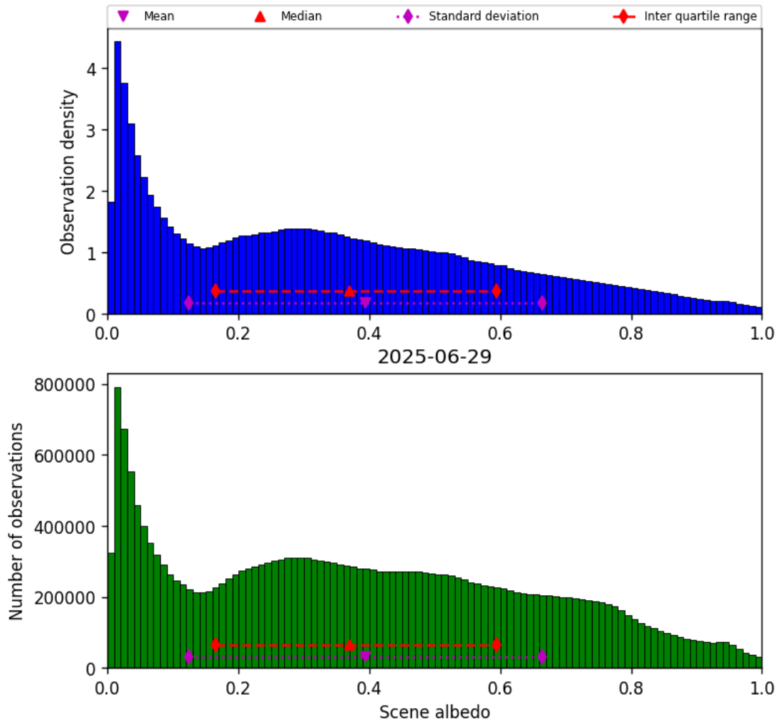
Figure 32: Histogram of “Scene albedo” for 2025-06-29 to 2025-06-30
