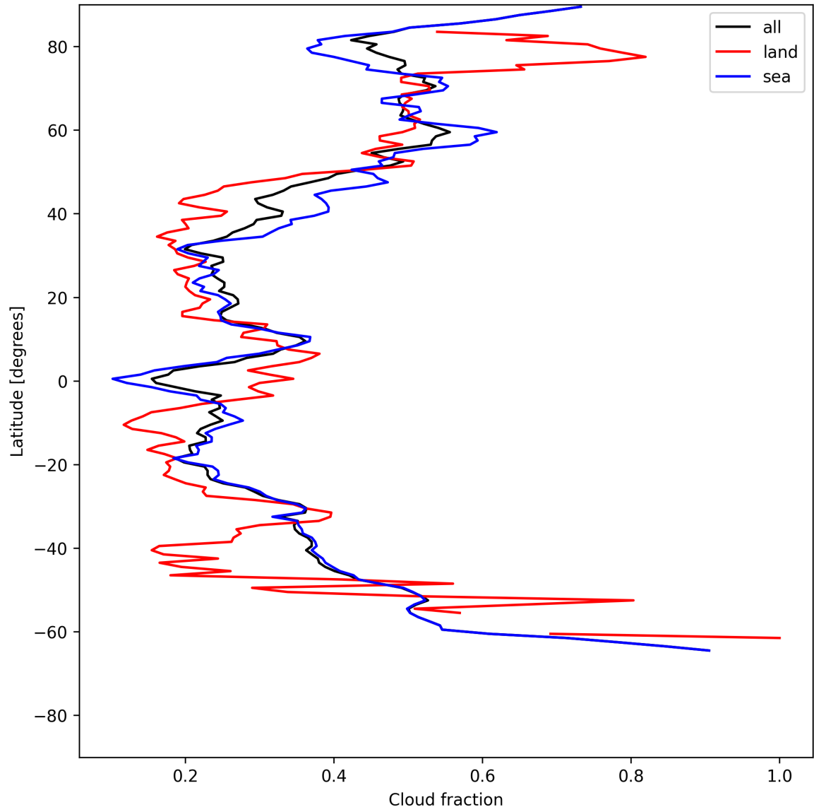
Figure 13: Zonal average of “Cloud fraction” for 2025-06-29 to 2025-06-30.
