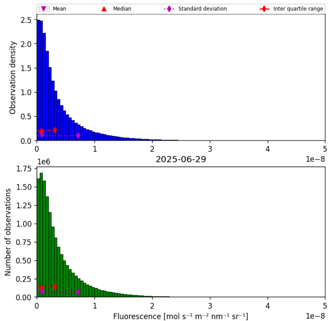
Figure 38: Histogram of “Fluorescence” for 2025-06-29 to 2025-06-30
