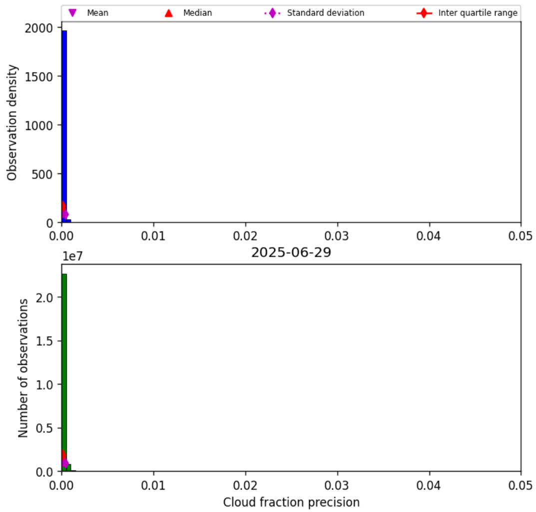
Figure 31: Histogram of “Cloud fraction precision” for 2025-06-29 to 2025-06-30
