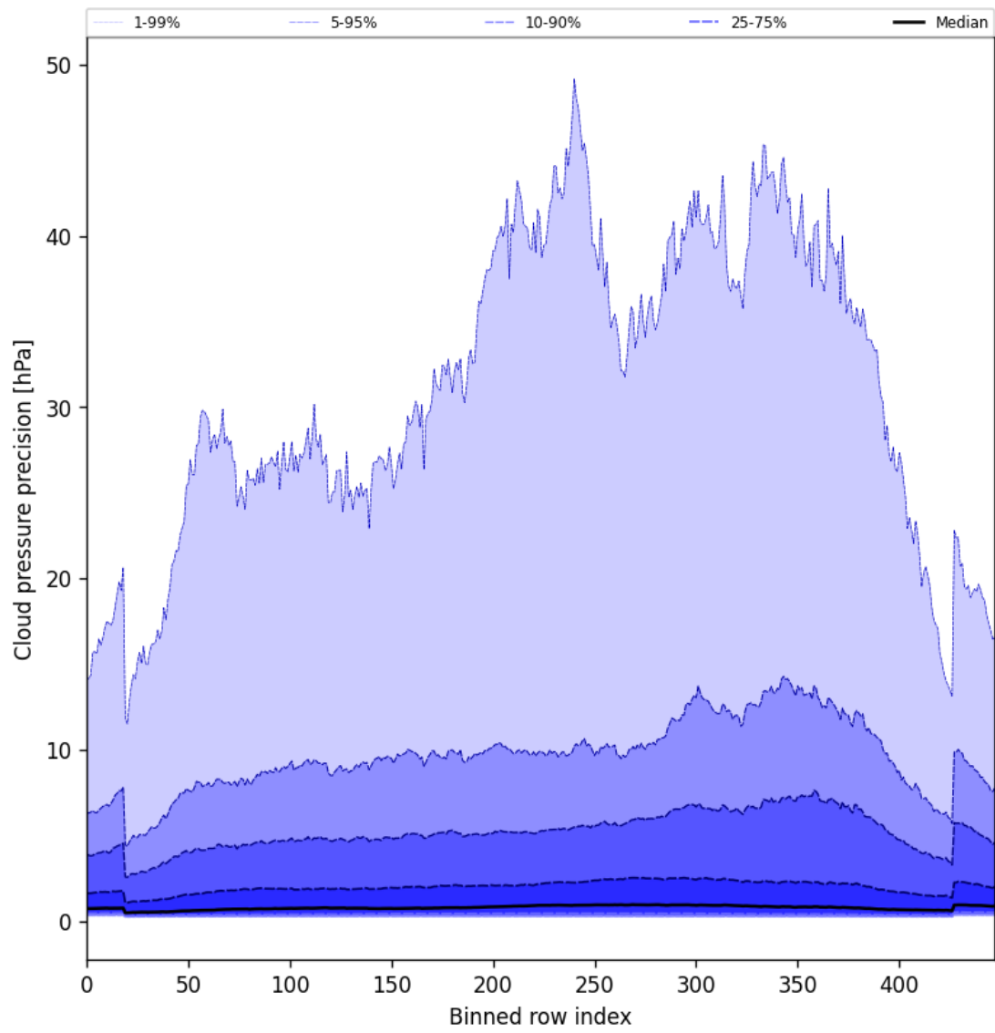
Figure 46: Along track statistics of “Cloud pressure precision” for 2025-06-29 to 2025-06-30
