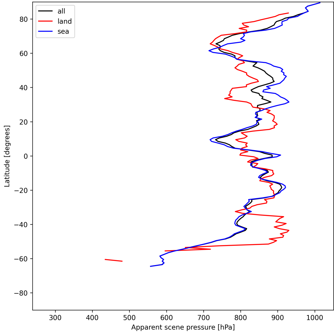
Figure 17: Zonal average of “Apparent scene pressure” for 2025-06-29 to 2025-06-30.
