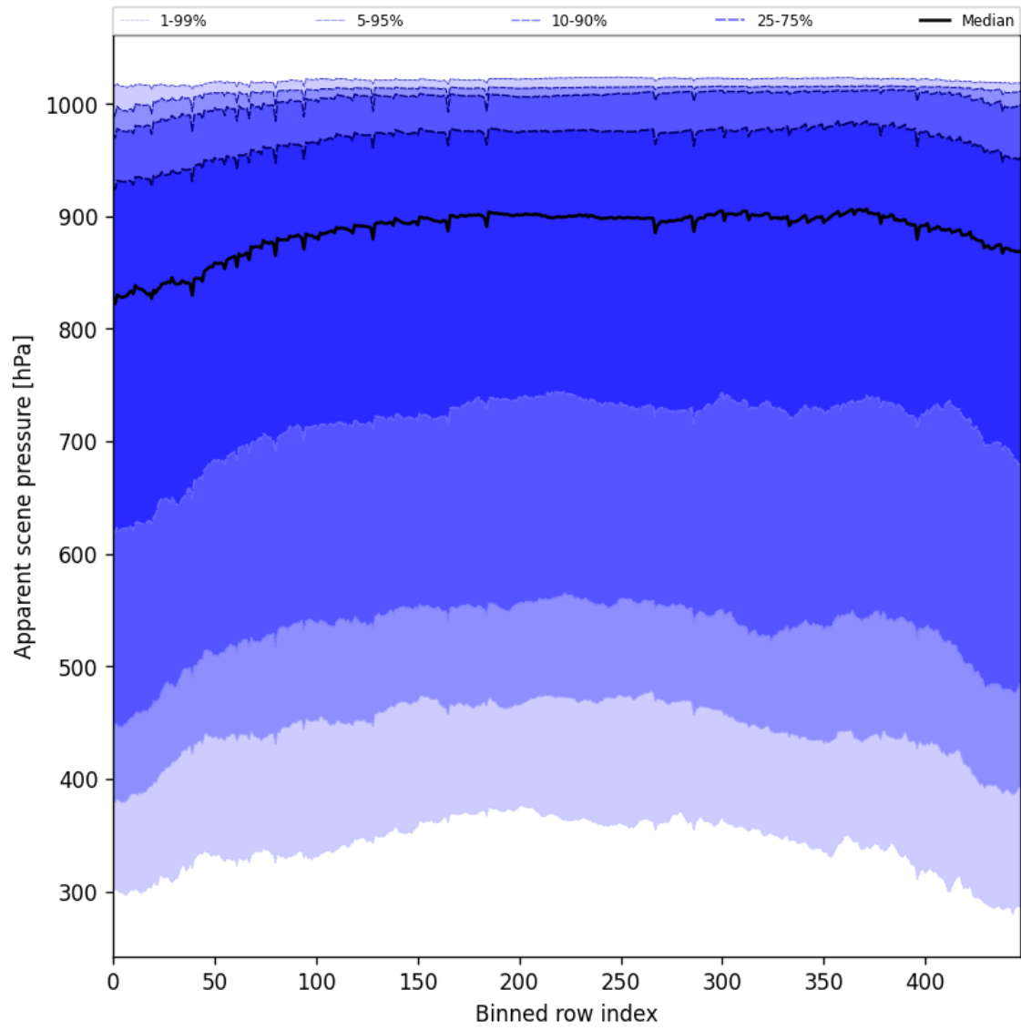
Figure 51: Along track statistics of “Apparent scene pressure” for 2025-06-29 to 2025-06-30
