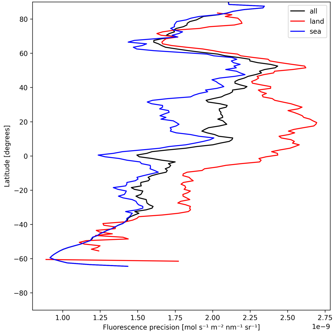
Figure 22: Zonal average of “Fluorescence precision” for 2025-06-29 to 2025-06-30.
