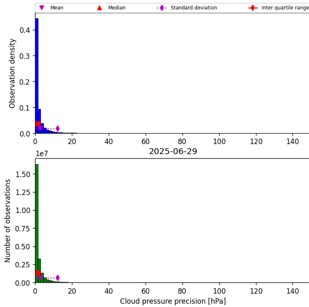
Figure 29: Histogram of “Cloud pressure precision” for 2025-06-29 to 2025-06-30
