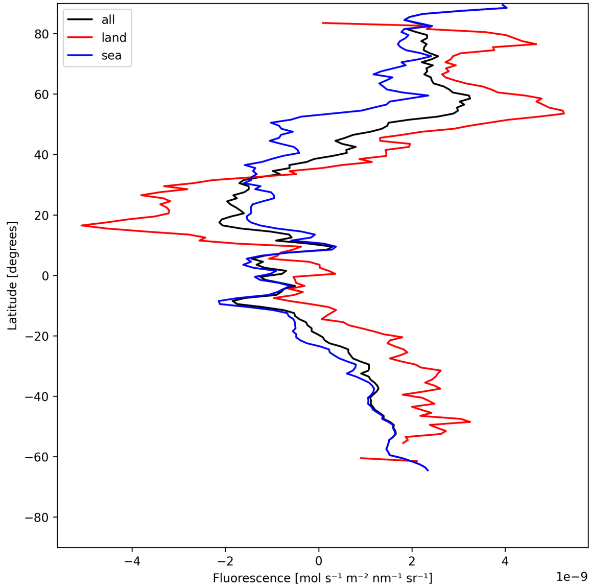
Figure 21: Zonal average of “Fluorescence” for 2025-06-29 to 2025-06-30.
