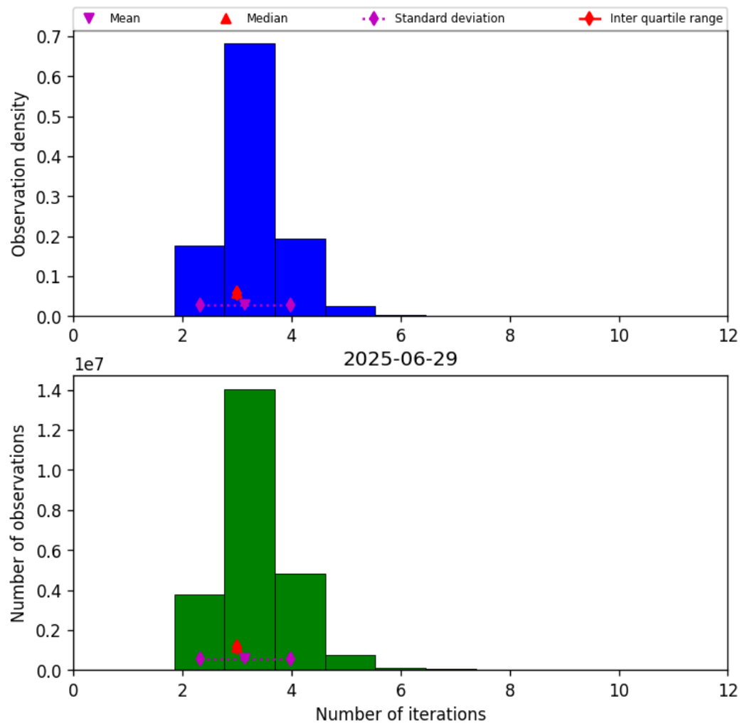
Figure 37: Histogram of “Number of iterations” for 2025-06-29 to 2025-06-30
