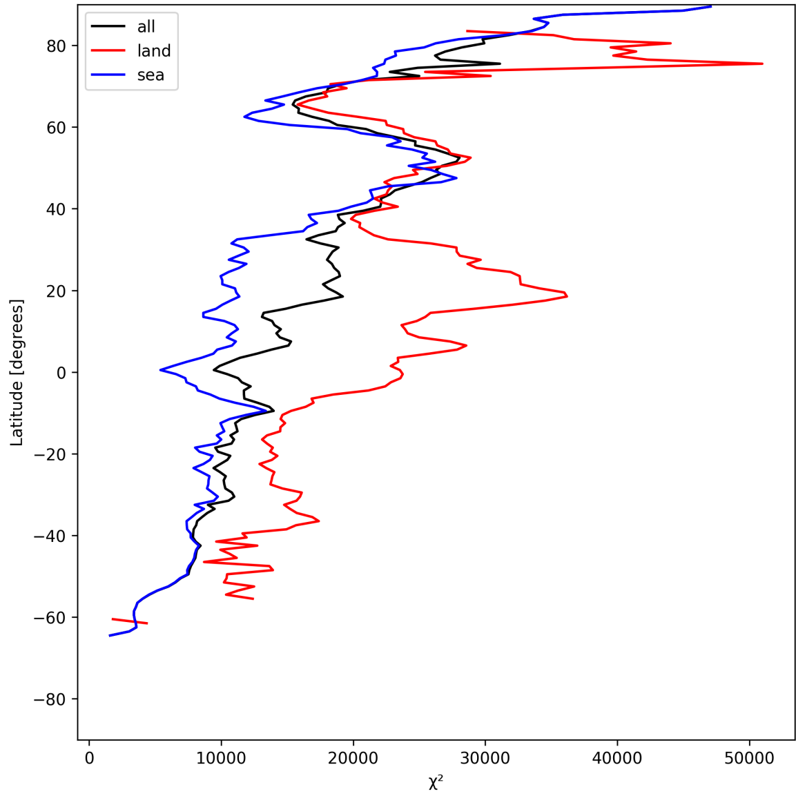
Figure 19: Zonal average of “ \chi^2 ” for 2025-06-29 to 2025-06-30.
