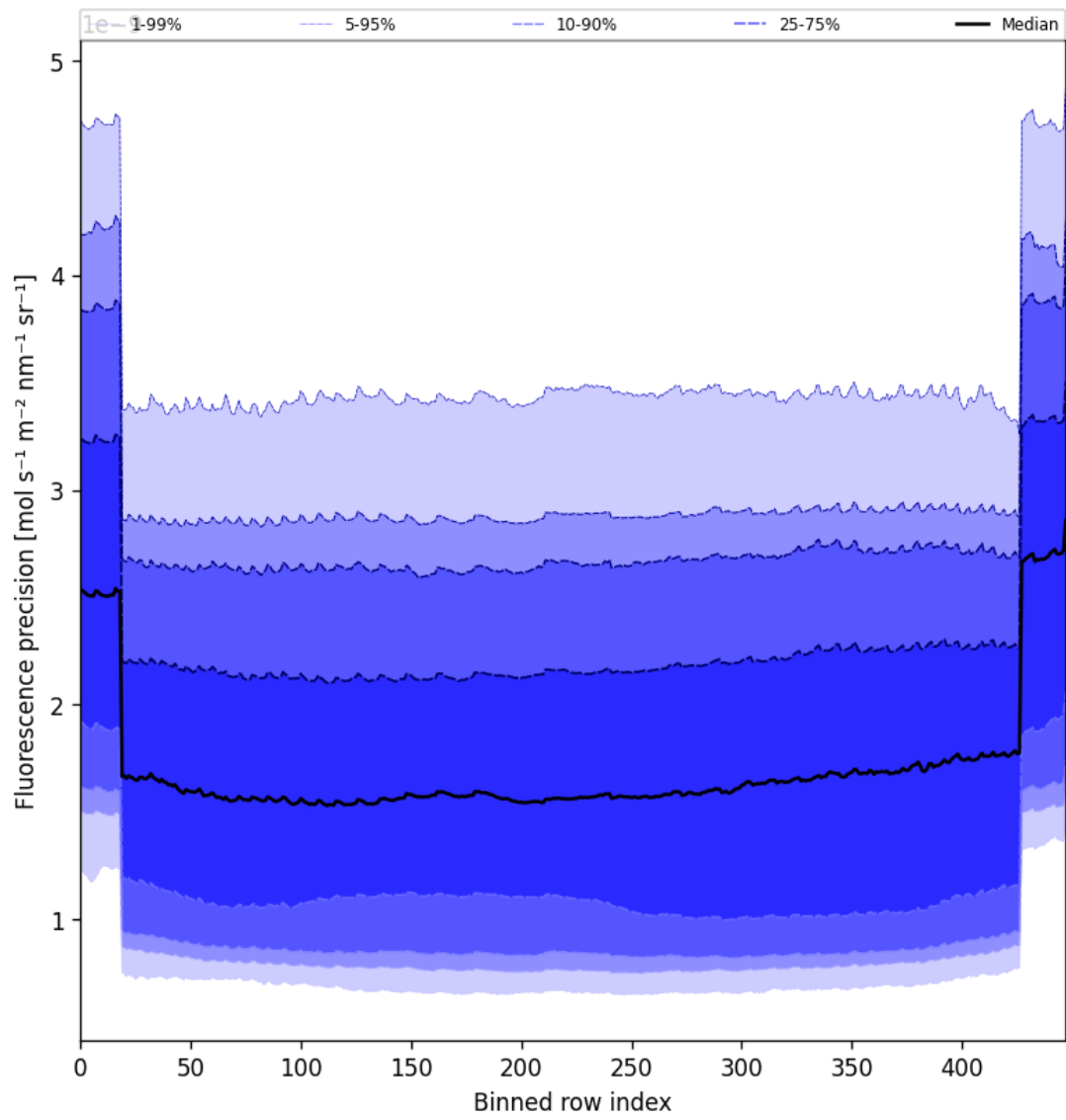
Figure 56: Along track statistics of “Fluorescence precision” for 2025-06-29 to 2025-06-30
