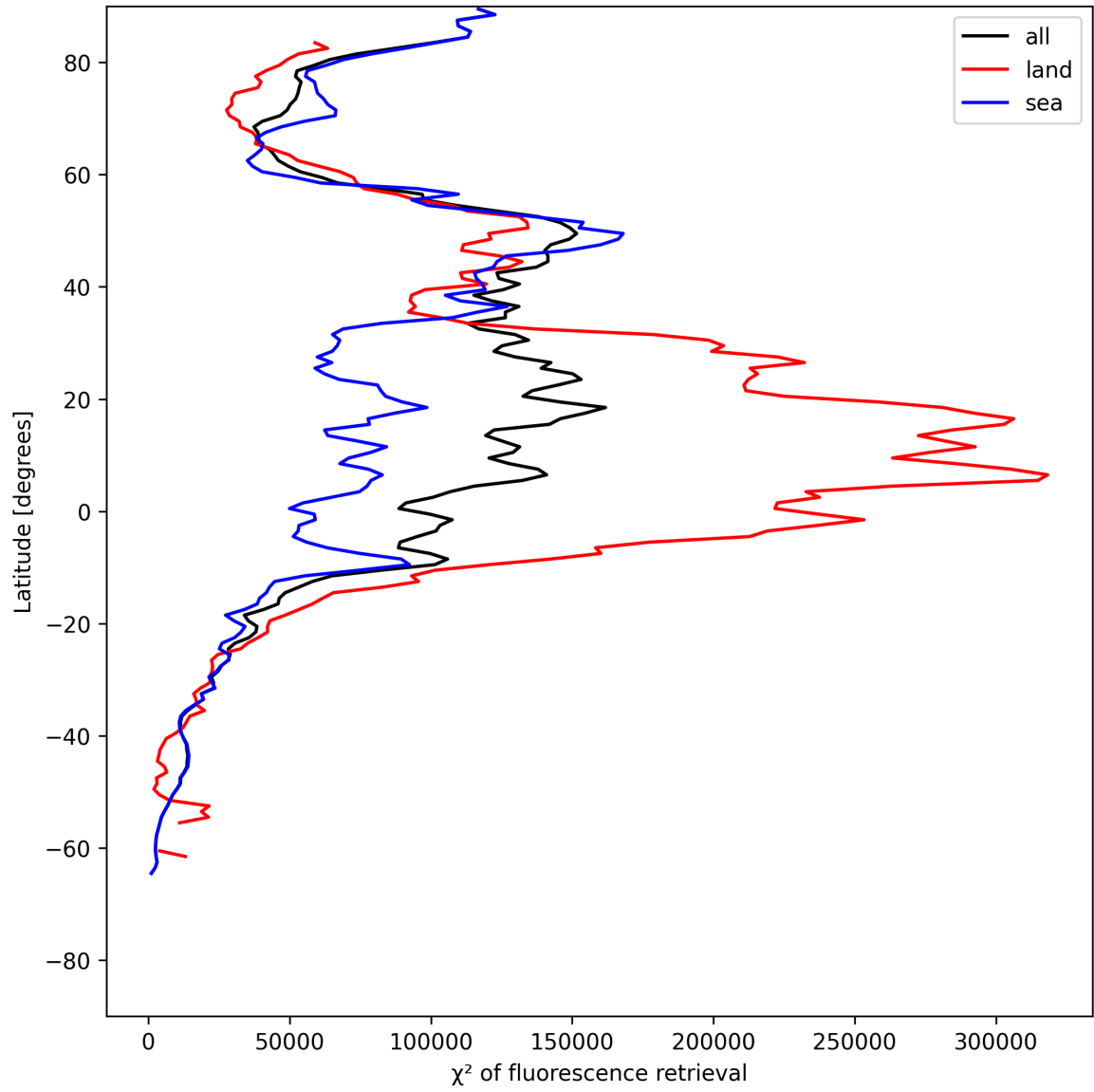
Figure 23: Zonal average of “ \chi^2 of fluorescence retrieval” for 2025-06-29 to 2025-06-30.
