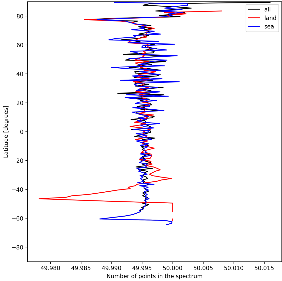
Figure 25: Zonal average of “Number of points in the spectrum” for 2025-06-29 to 2025-06-30.
