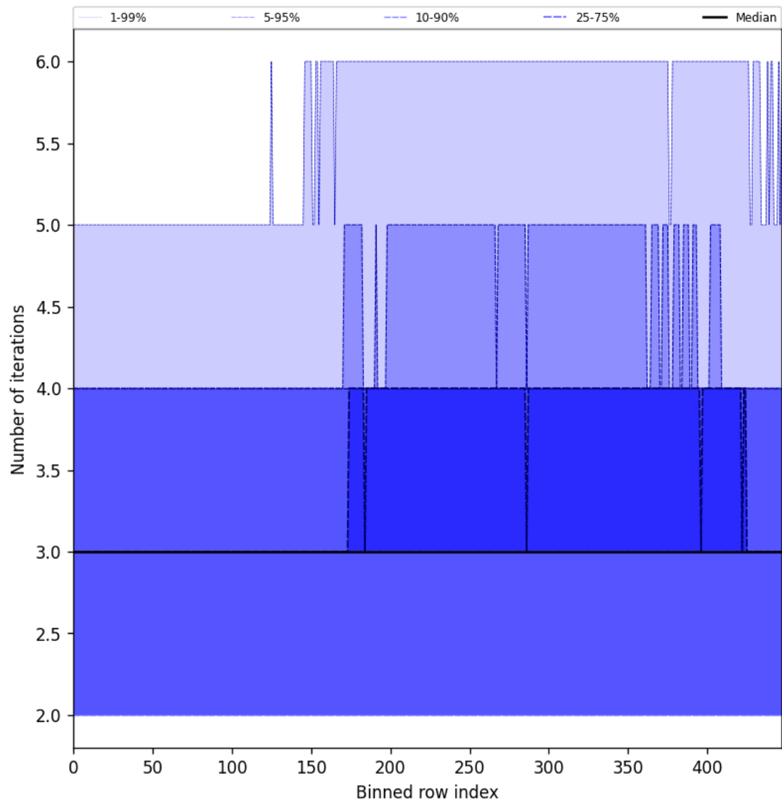
Figure 54: Along track statistics of “Number of iterations” for 2025-06-29 to 2025-06-30
