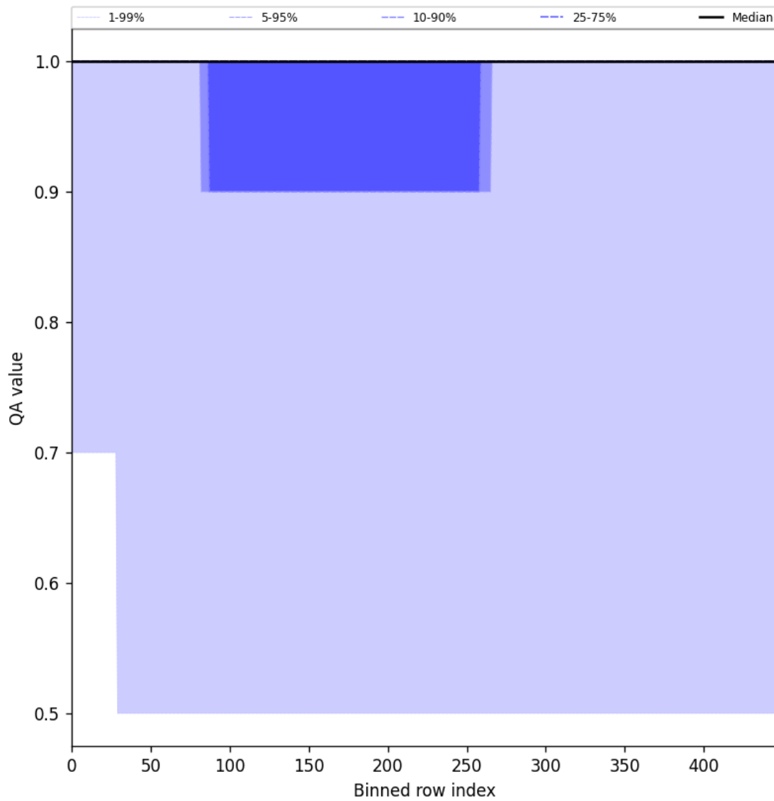
Figure 44: Along track statistics of “QA value” for 2025-06-29 to 2025-06-30
