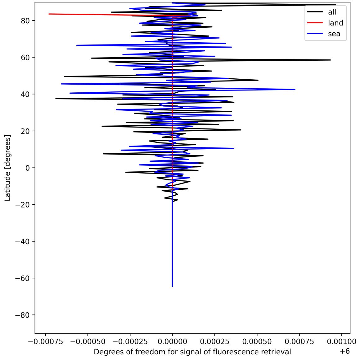
Figure 24: Zonal average of “Degrees of freedom for signal of fluorescence retrieval” for 2025-06-29 to 2025-06-30.
