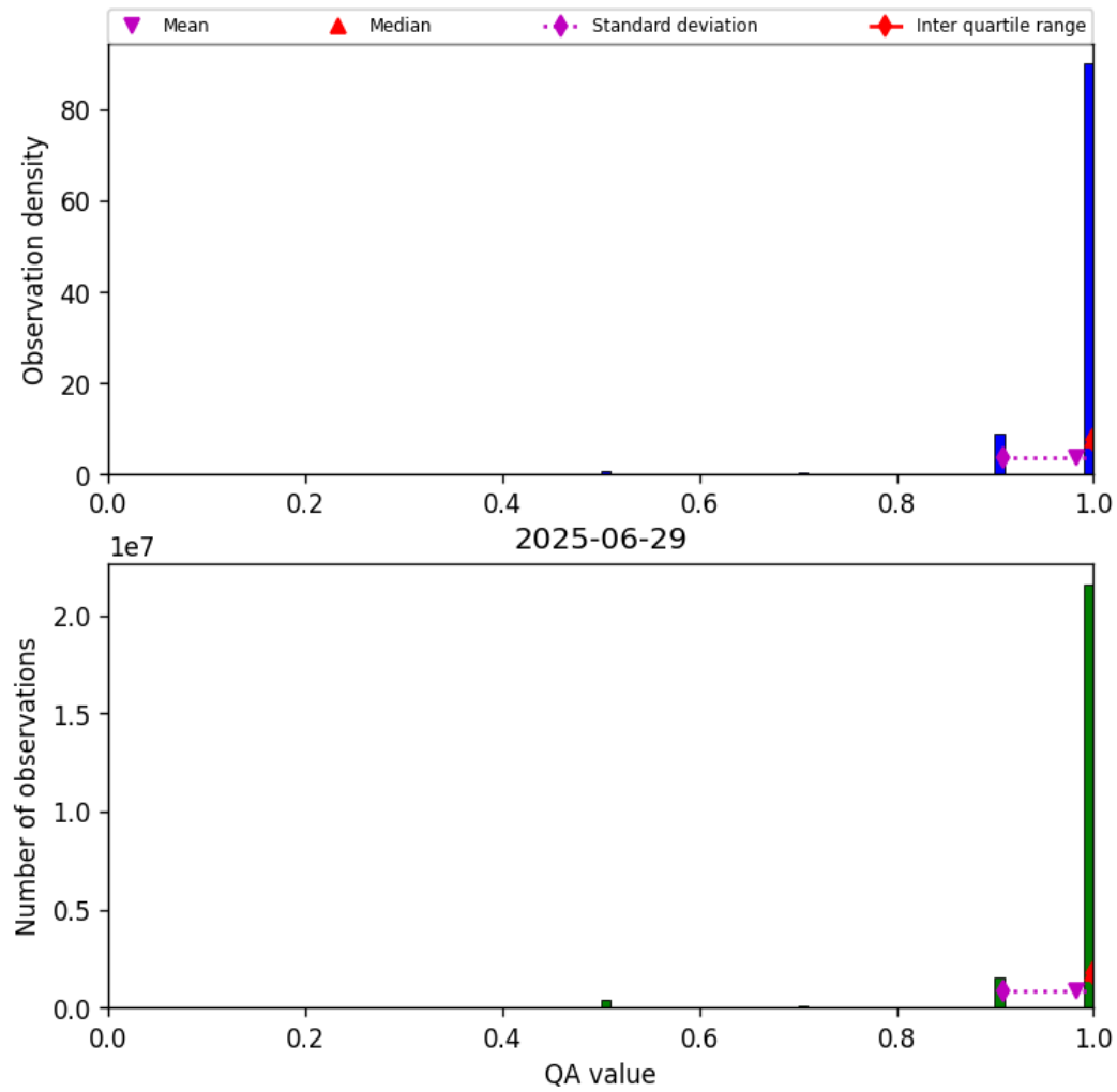
Figure 27: Histogram of “QA value” for 2025-06-29 to 2025-06-30
