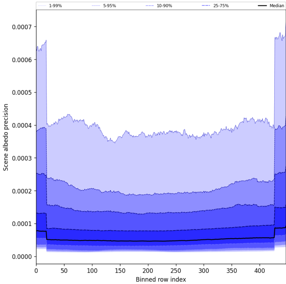
Figure 50: Along track statistics of “Scene albedo precision” for 2025-06-29 to 2025-06-30
