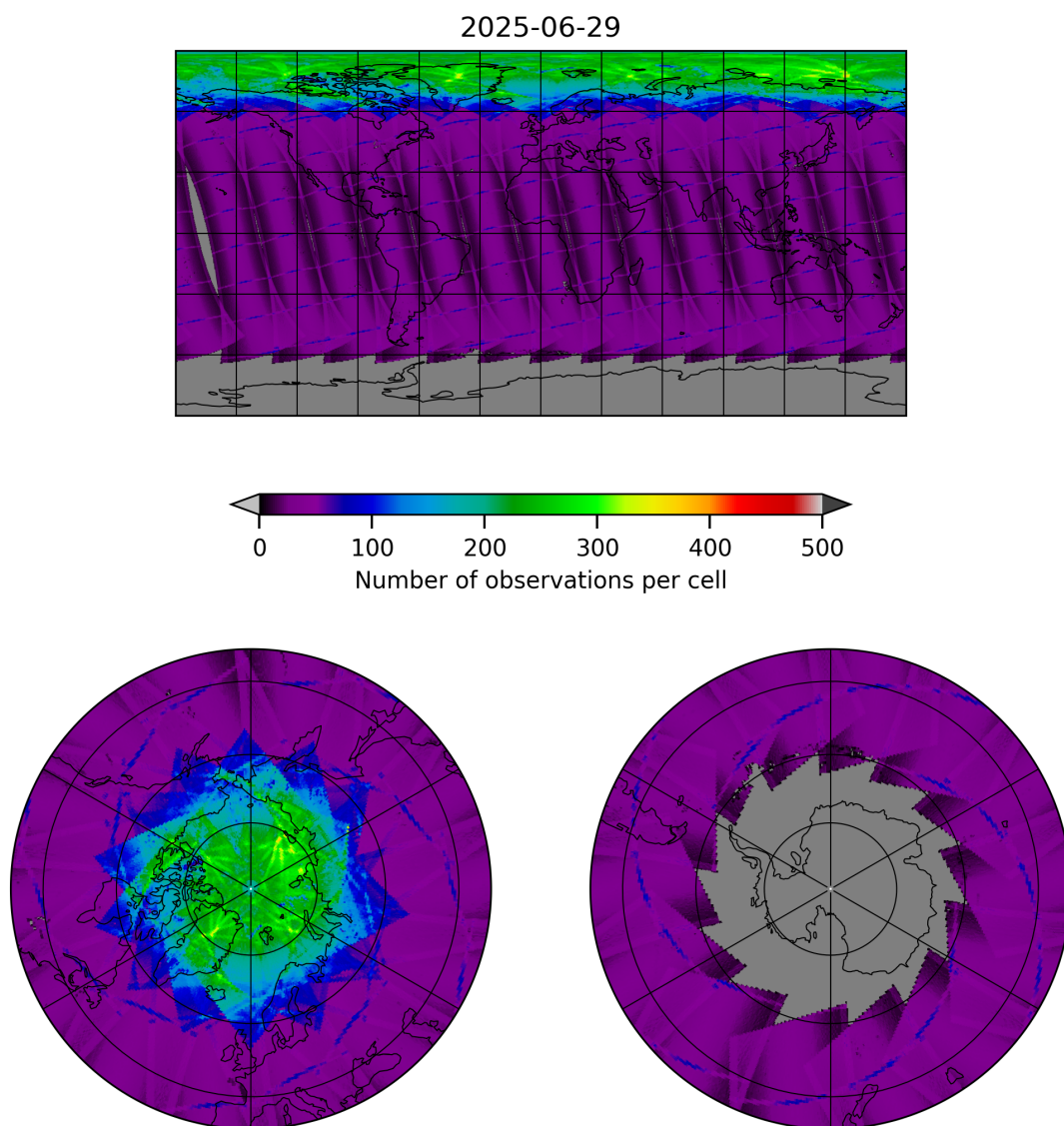
Figure 9: Map of the number of observations for 2025-06-29 to 2025-06-30
