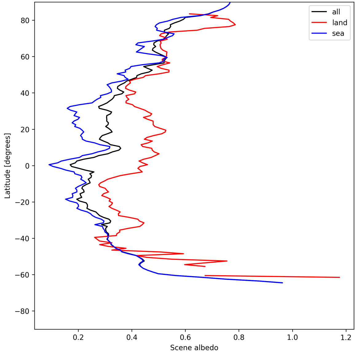
Figure 15: Zonal average of “Scene albedo” for 2025-06-29 to 2025-06-30.
