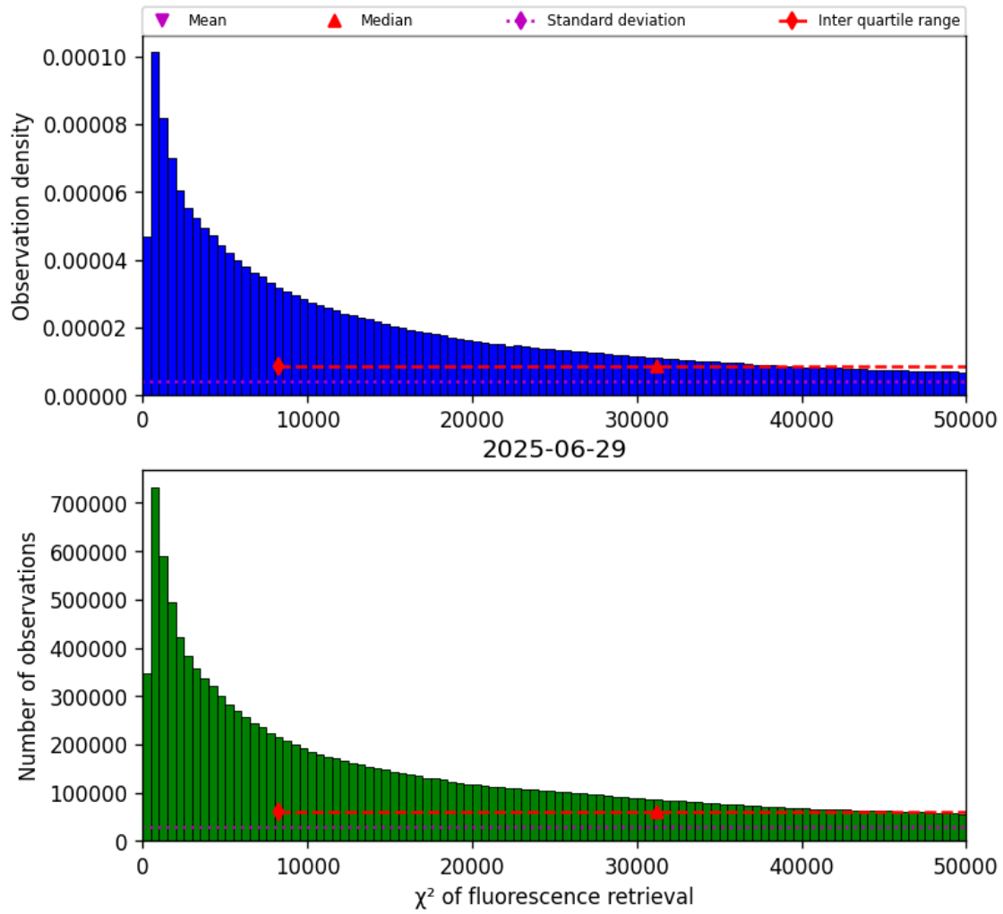
Figure 40: Histogram of “ \chi^2 of fluorescence retrieval” for 2025-06-29 to 2025-06-30
