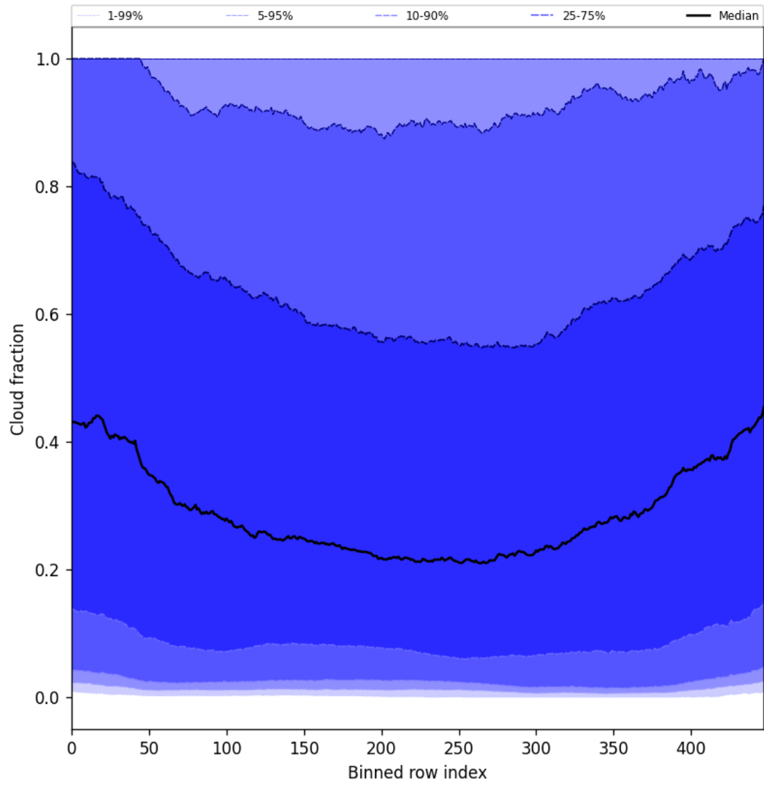
Figure 47: Along track statistics of “Cloud fraction” for 2025-06-29 to 2025-06-30
