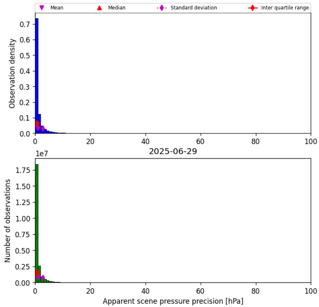
Figure 35: Histogram of “Apparent scene pressure precision” for 2025-06-29 to 2025-06-30
