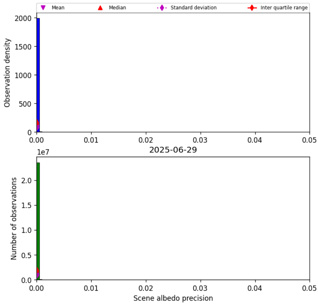
Figure 33: Histogram of “Scene albedo precision” for 2025-06-29 to 2025-06-30
