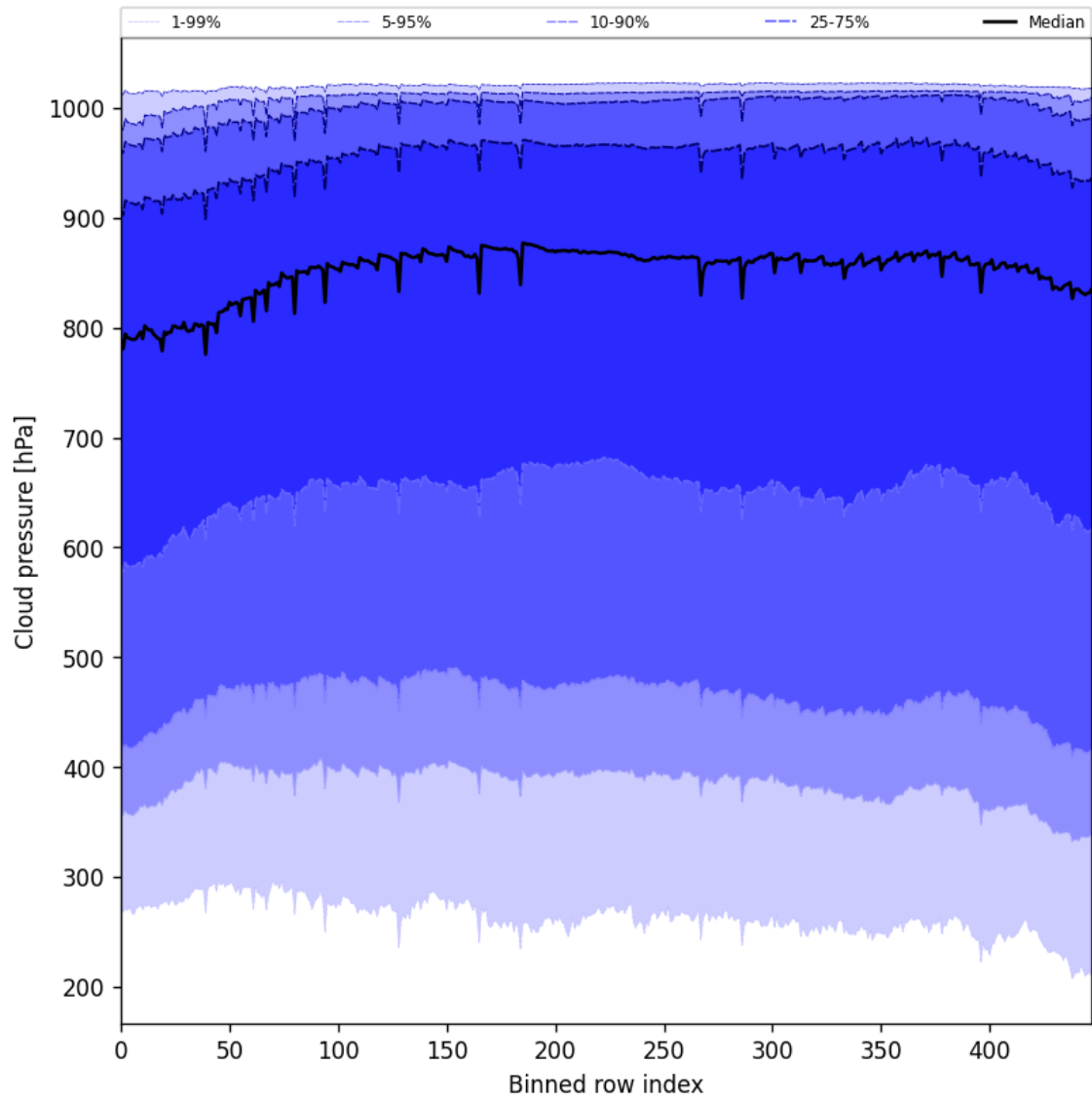
Figure 45: Along track statistics of “Cloud pressure” for 2025-06-29 to 2025-06-30
