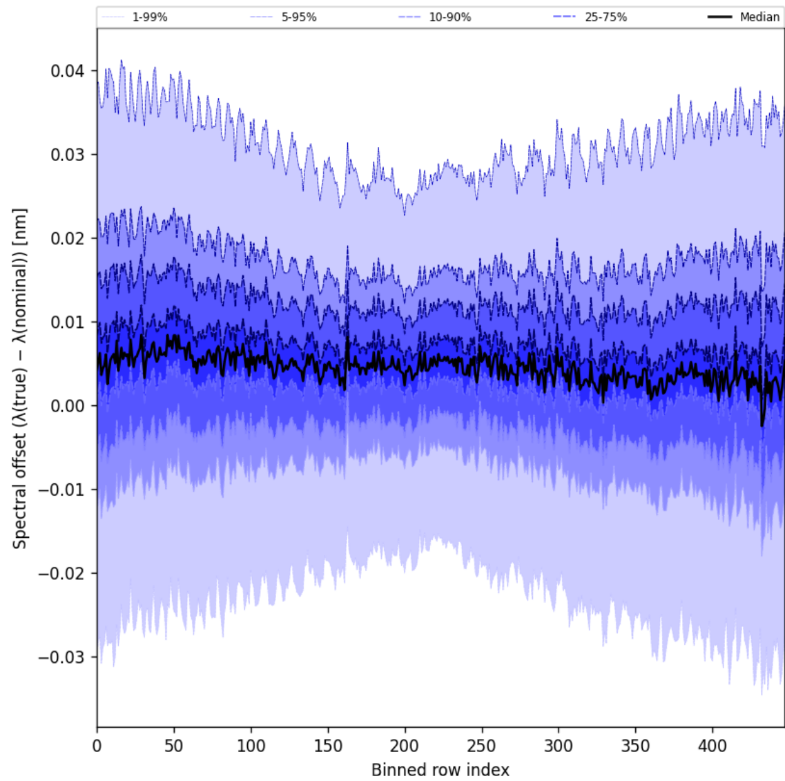
Figure 60: Along track statistics of “Spectral offset ( \lambda_{\text{true}} - \lambda_{\text{nominal}} )” for 2025-06-29 to 2025-06-30
