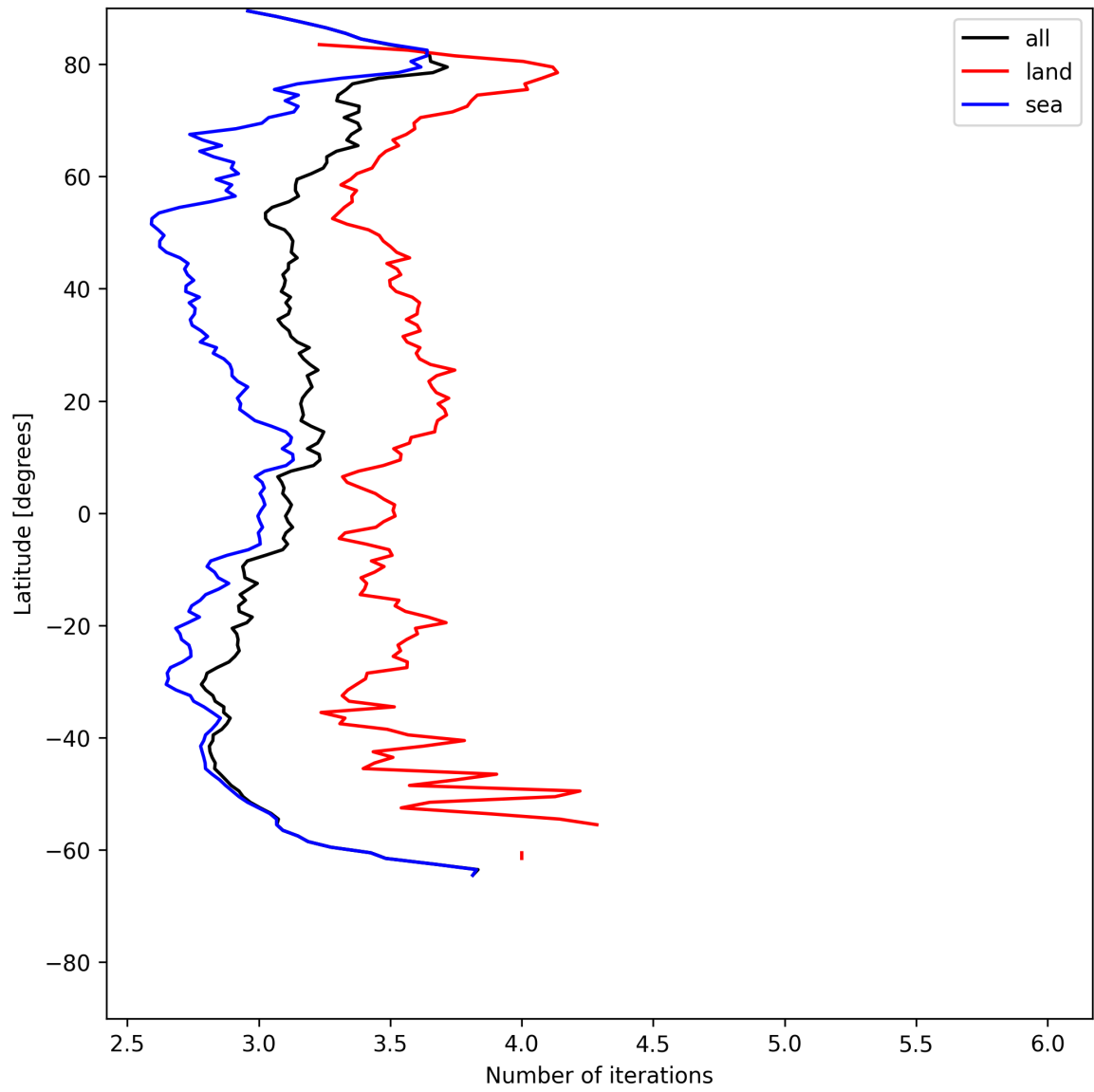
Figure 20: Zonal average of “Number of iterations” for 2025-06-29 to 2025-06-30.
