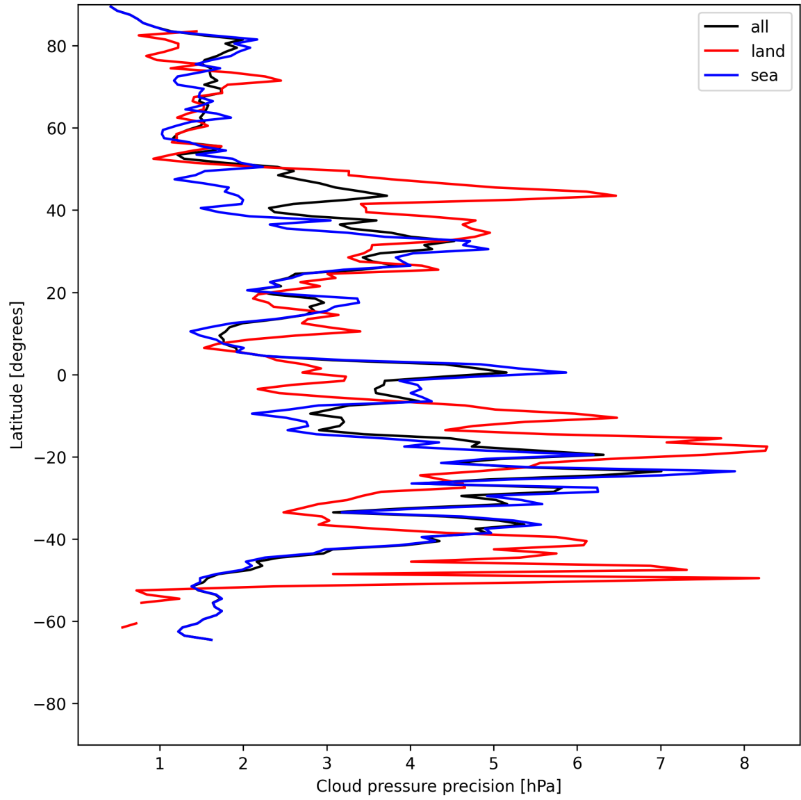
Figure 12: Zonal average of “Cloud pressure precision” for 2025-06-29 to 2025-06-30.
