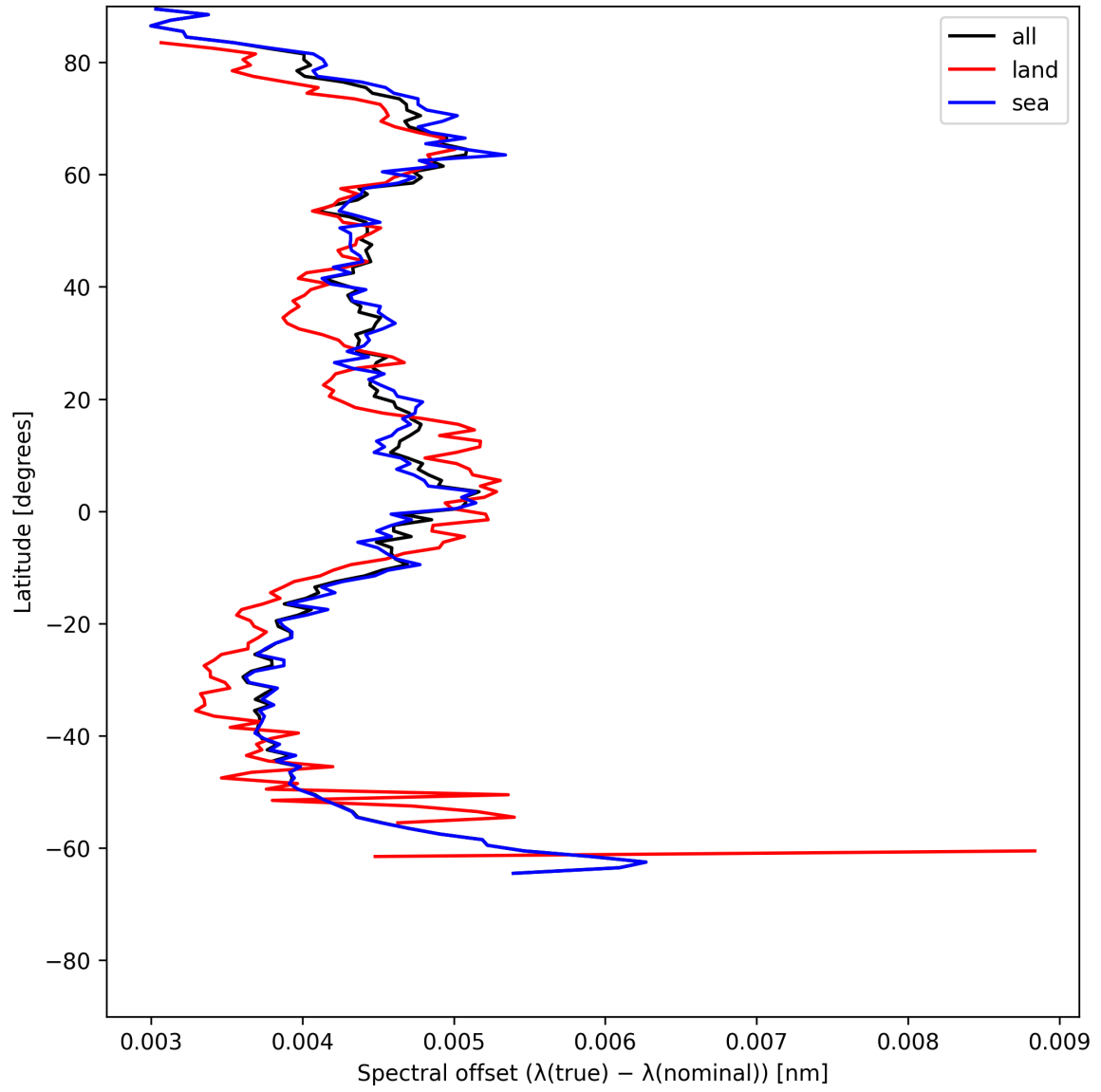
Figure 26: Zonal average of “Spectral offset ( \lambda_{\text{true}} - \lambda_{\text{nominal}} )” for 2025-06-29 to 2025-06-30.
