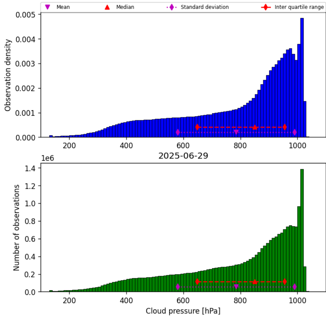
Figure 28: Histogram of “Cloud pressure” for 2025-06-29 to 2025-06-30
