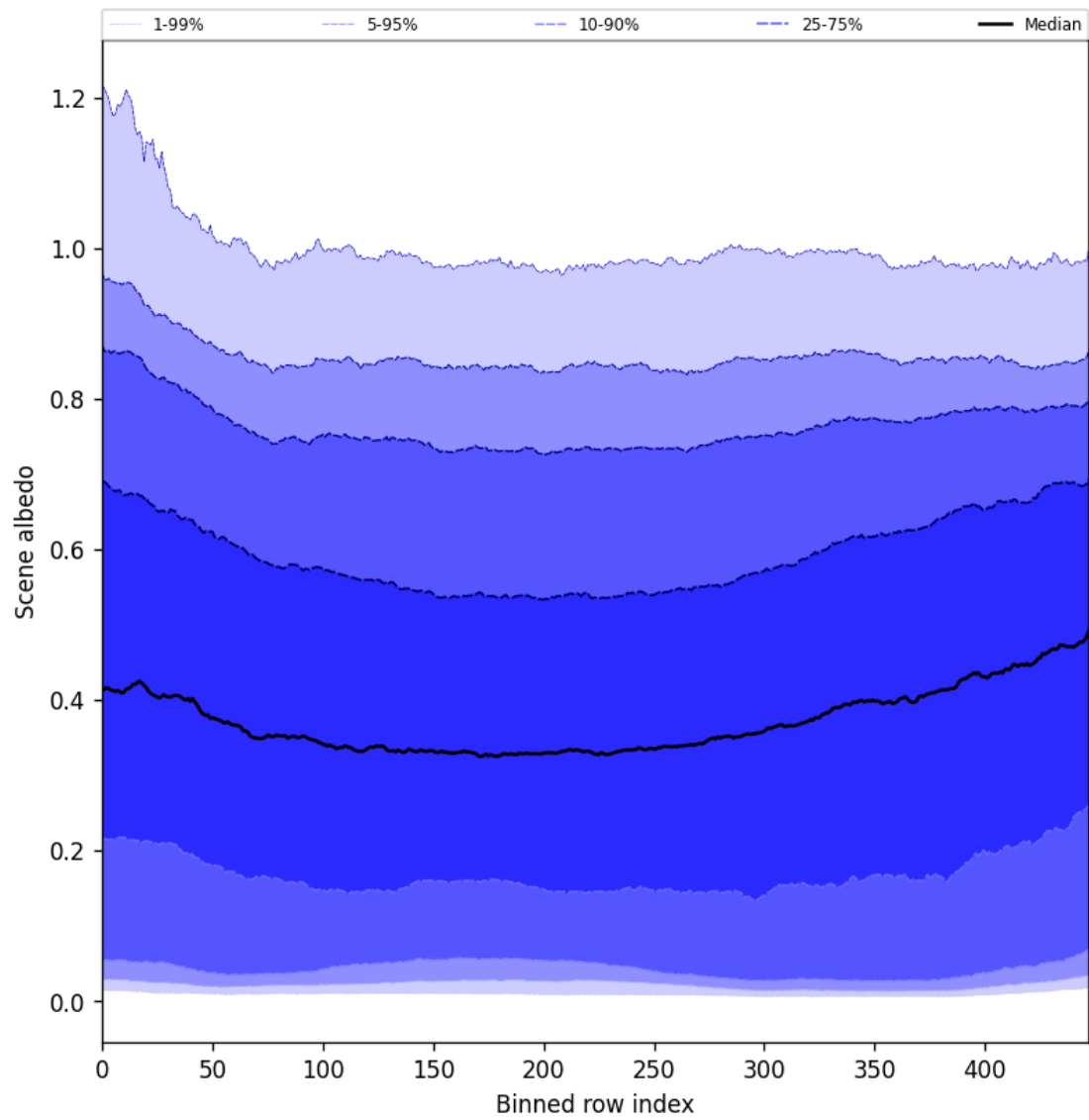
Figure 49: Along track statistics of “Scene albedo” for 2025-06-29 to 2025-06-30
