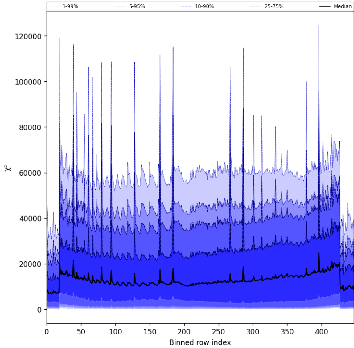
Figure 53: Along track statistics of “ \chi^2 ” for 2025-06-29 to 2025-06-30
