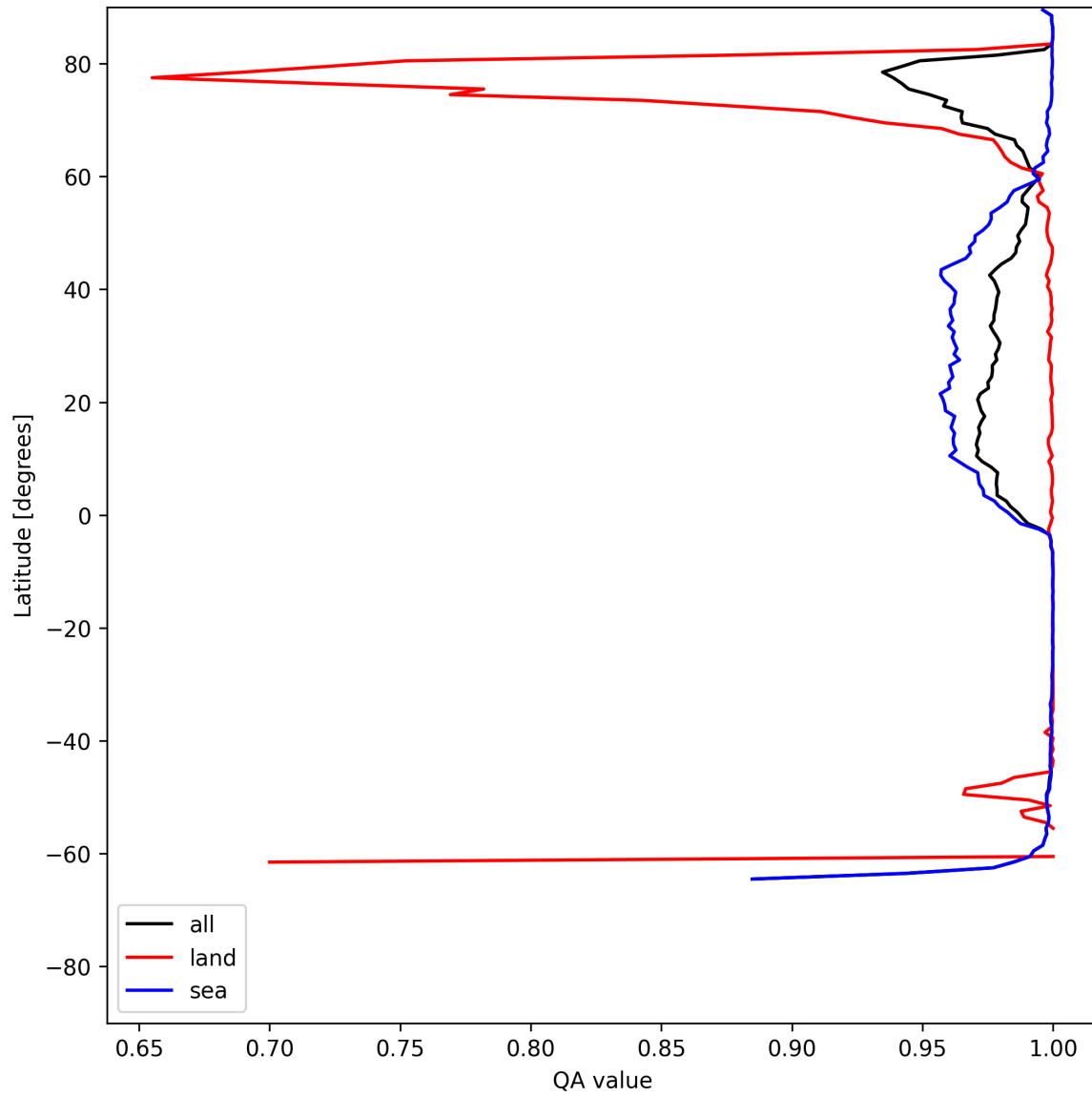
Figure 10: Zonal average of “QA value” for 2025-06-29 to 2025-06-30.
