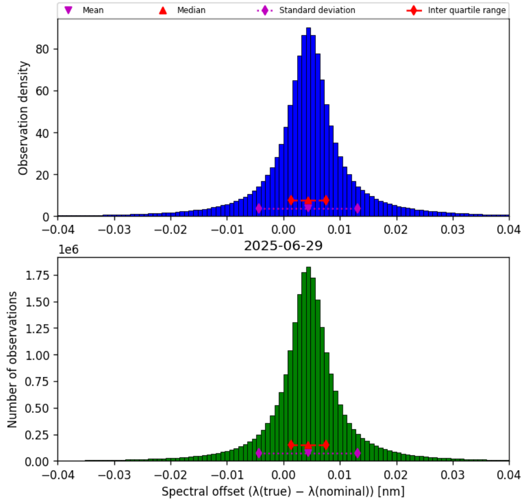
Figure 43: Histogram of “Spectral offset ( \lambda_{\text{true}} - \lambda_{\text{nominal}} )” for 2025-06-29 to 2025-06-30
