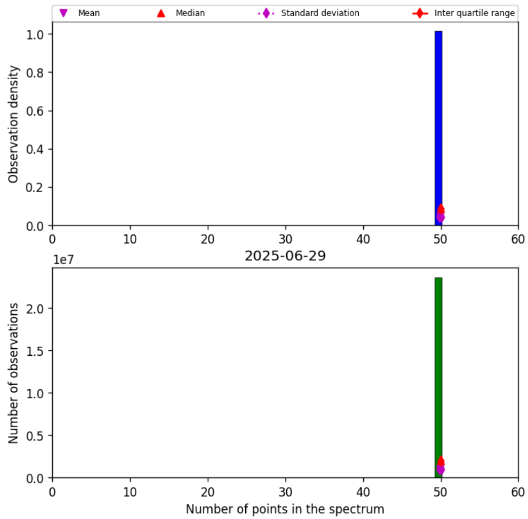
Figure 42: Histogram of “Number of points in the spectrum” for 2025-06-29 to 2025-06-30
