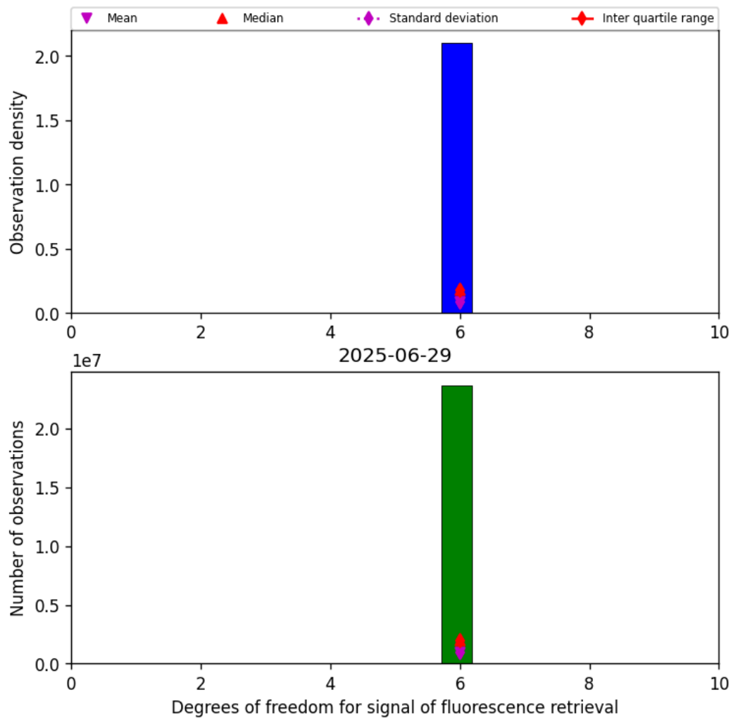
Figure 41: Histogram of “Degrees of freedom for signal of fluorescence retrieval” for 2025-06-29 to 2025-06-30
