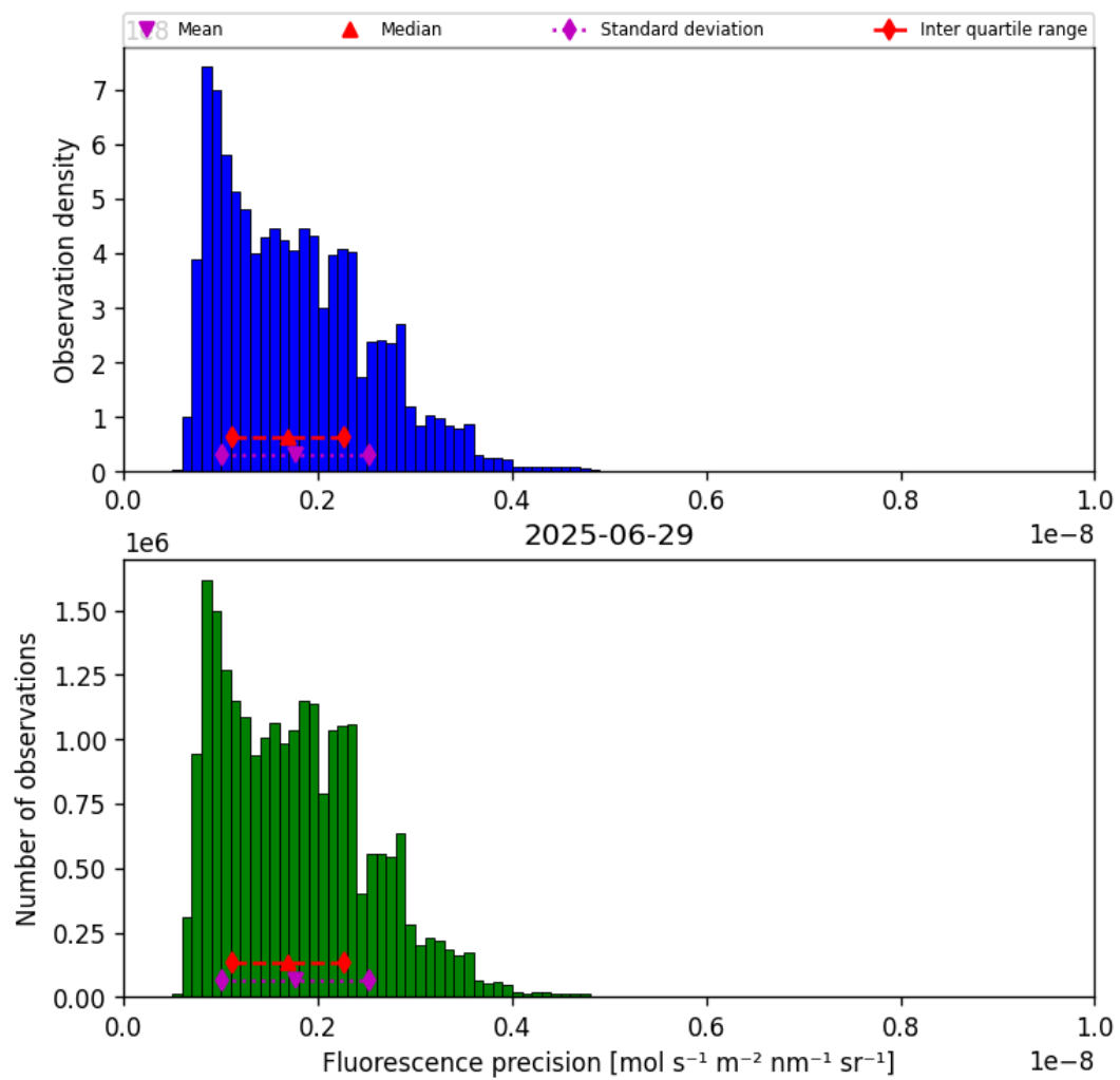
Figure 39: Histogram of “Fluorescence precision” for 2025-06-29 to 2025-06-30
