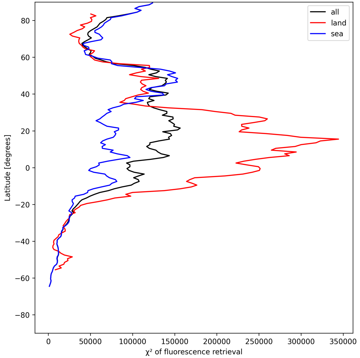
Figure 23: Zonal average of “ \chi^2 of fluorescence retrieval” for 2025-06-30 to 2025-06-30.
