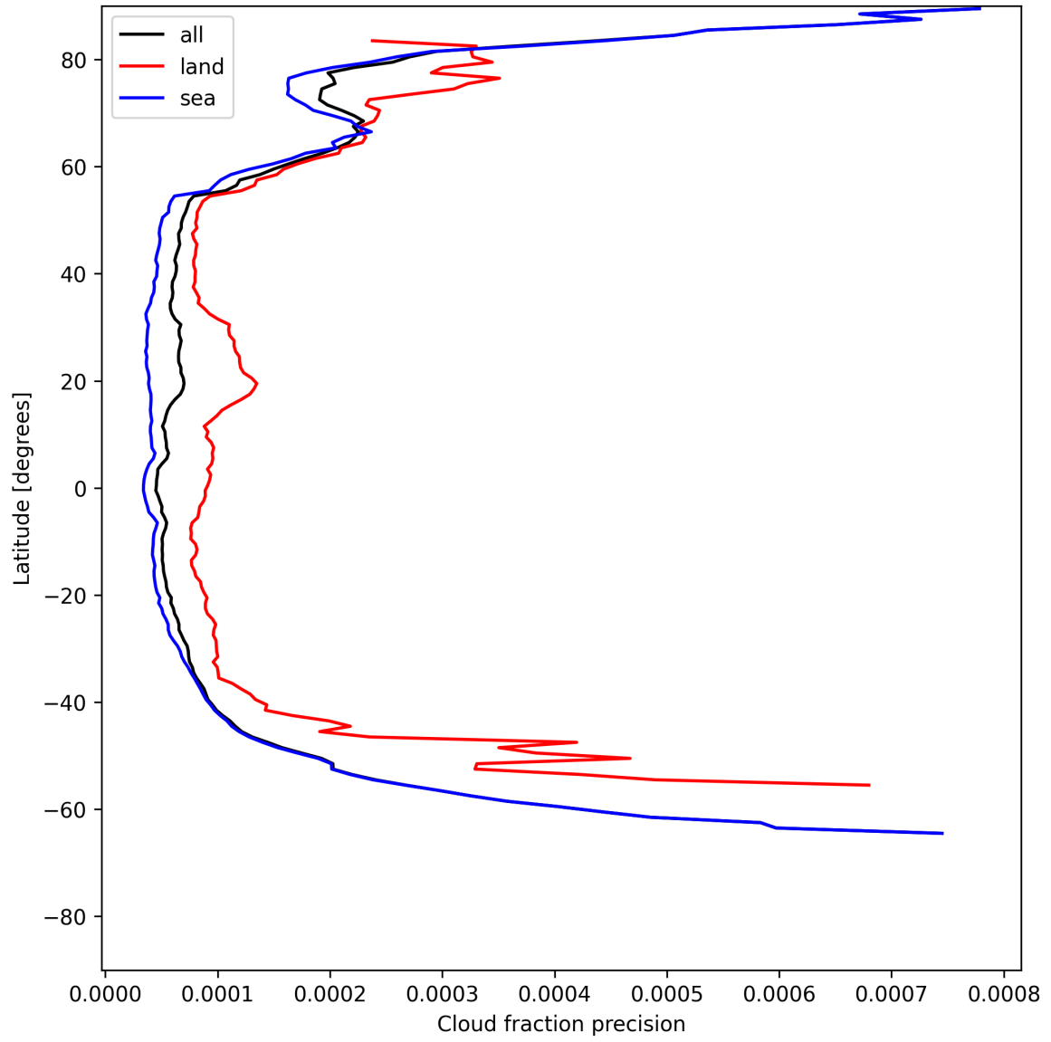
Figure 14: Zonal average of “Cloud fraction precision” for 2025-06-30 to 2025-06-30.
