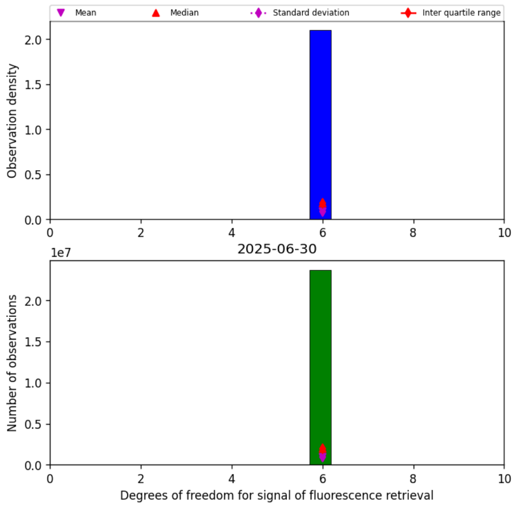
Figure 41: Histogram of “Degrees of freedom for signal of fluorescence retrieval” for 2025-06-30 to 2025-06-30
