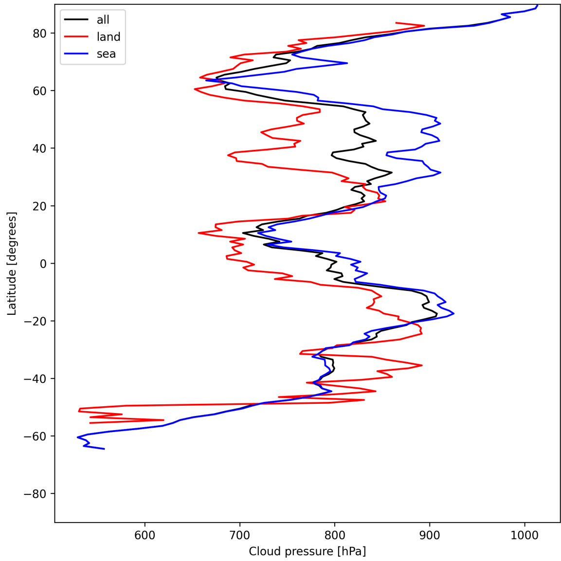
Figure 11: Zonal average of “Cloud pressure” for 2025-06-30 to 2025-06-30.
