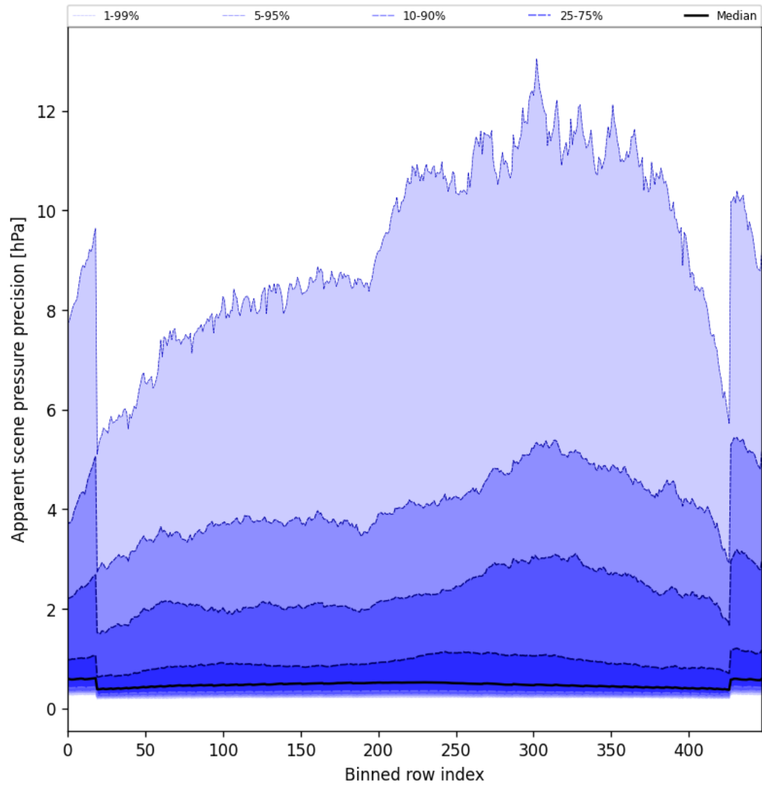
Figure 52: Along track statistics of “Apparent scene pressure precision” for 2025-06-30 to 2025-06-30
