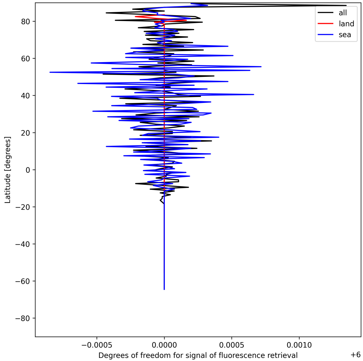
Figure 24: Zonal average of “Degrees of freedom for signal of fluorescence retrieval” for 2025-06-30 to 2025-06-30.
