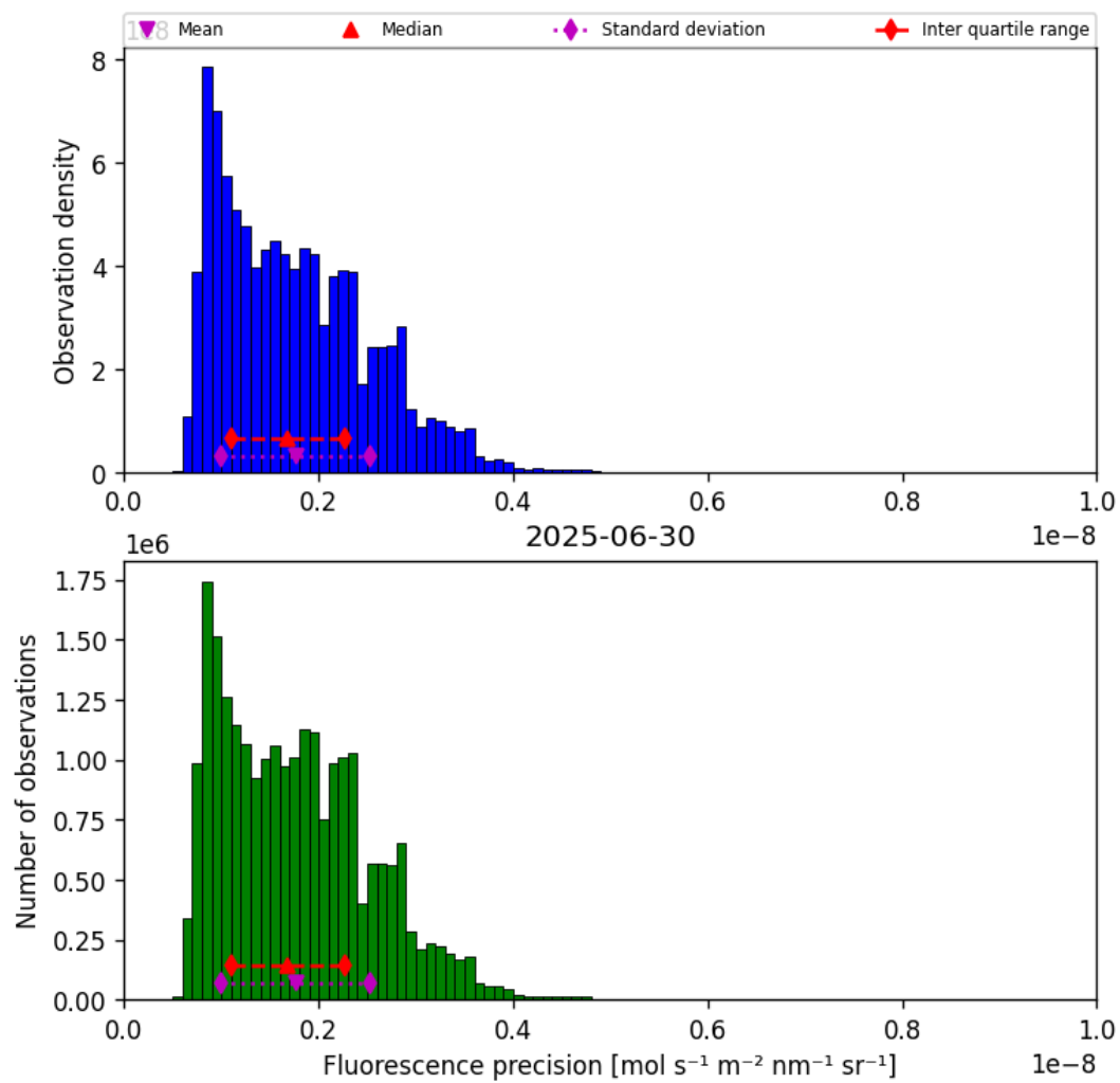
Figure 39: Histogram of “Fluorescence precision” for 2025-06-30 to 2025-06-30
