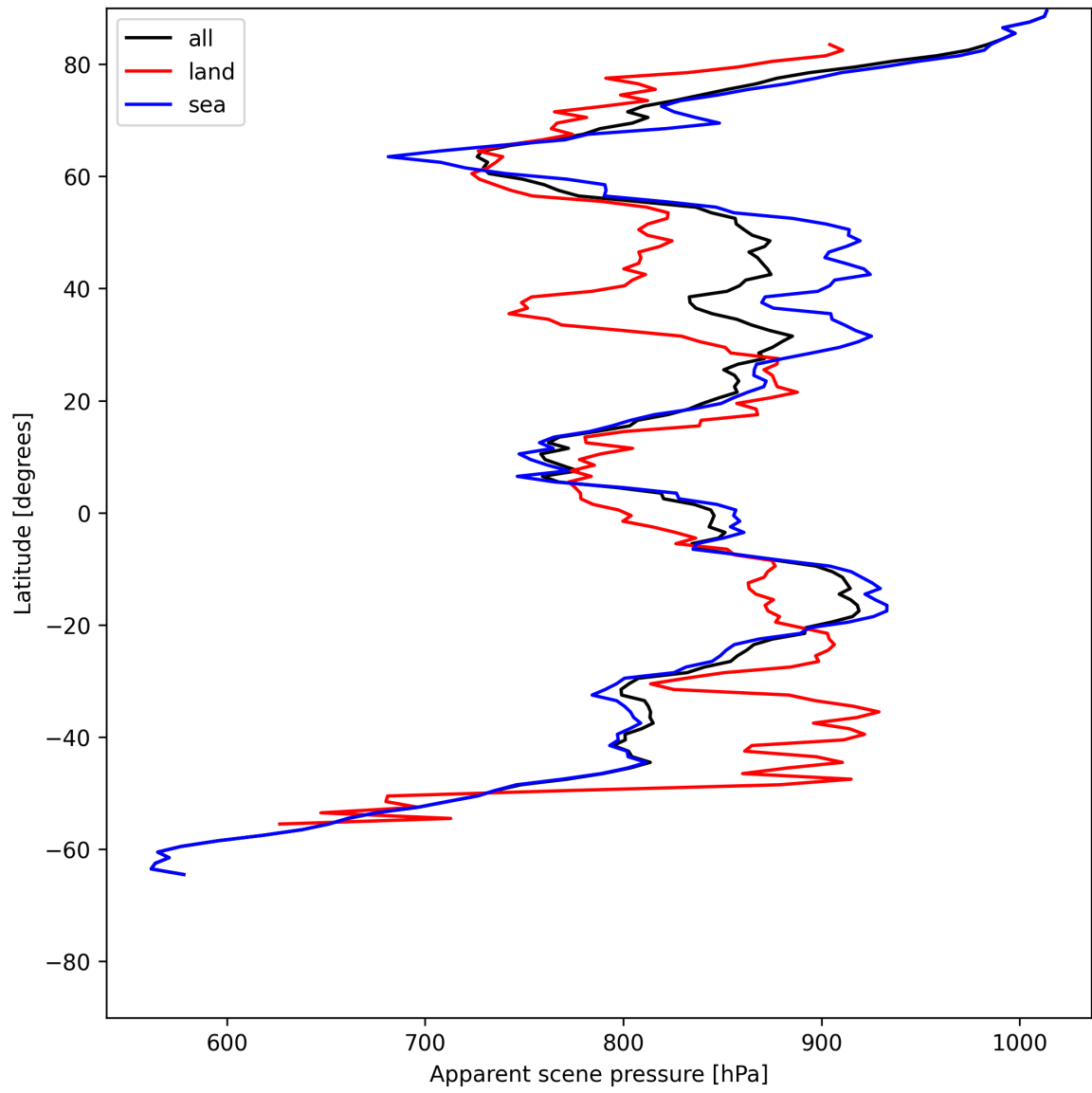
Figure 17: Zonal average of “Apparent scene pressure” for 2025-06-30 to 2025-06-30.
