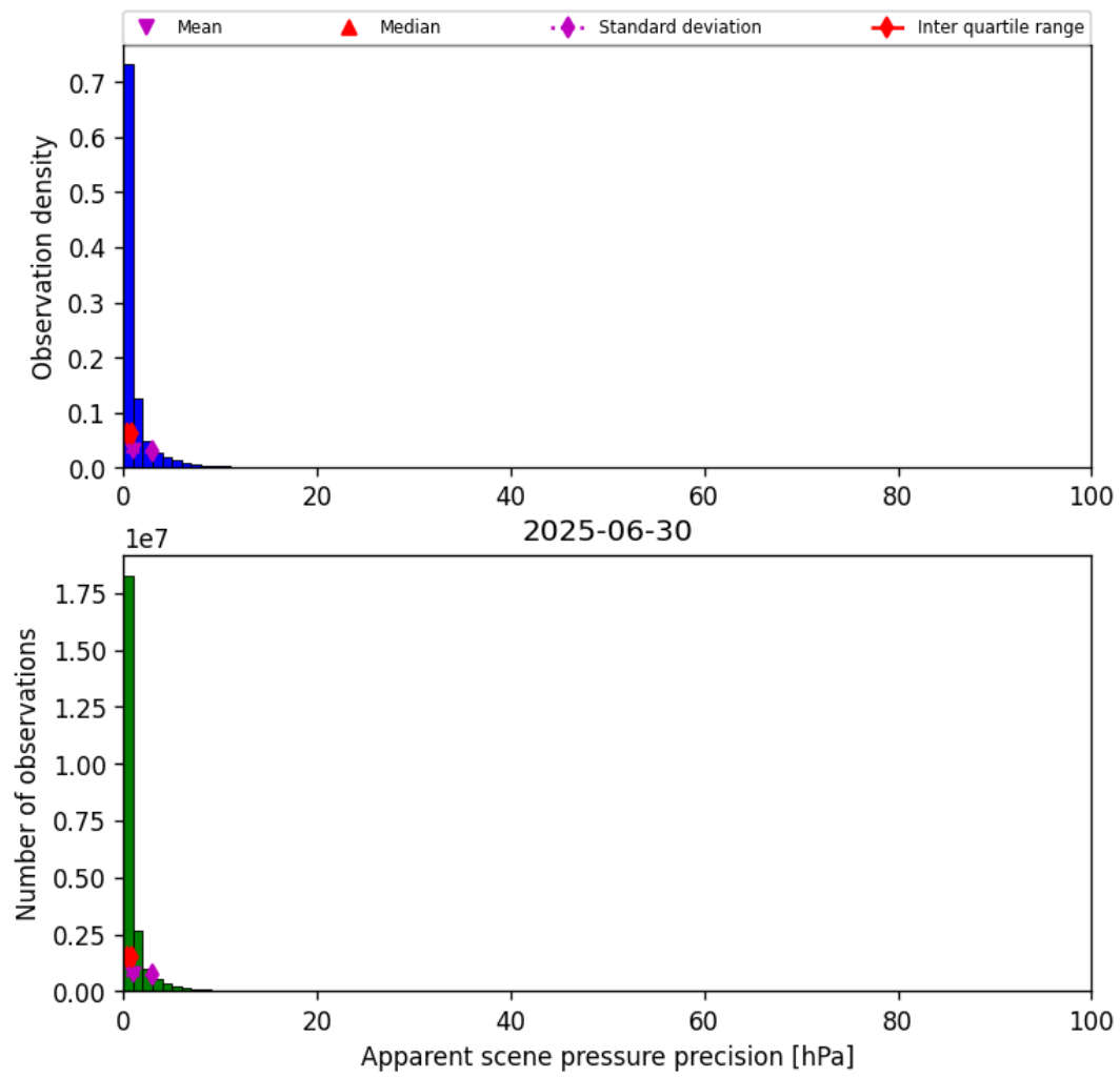
Figure 35: Histogram of “Apparent scene pressure precision” for 2025-06-30 to 2025-06-30
