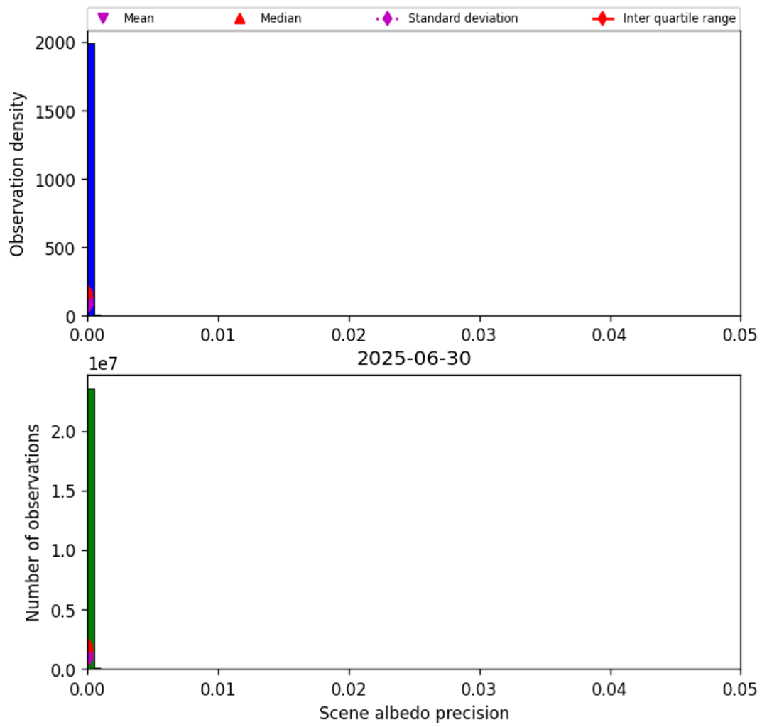
Figure 33: Histogram of “Scene albedo precision” for 2025-06-30 to 2025-06-30
