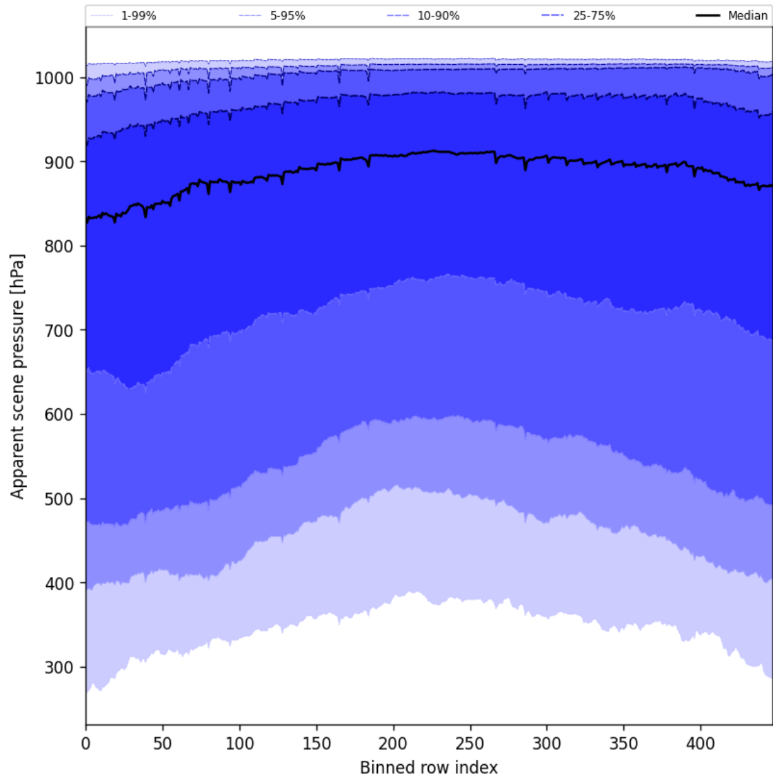
Figure 51: Along track statistics of “Apparent scene pressure” for 2025-06-30 to 2025-06-30
