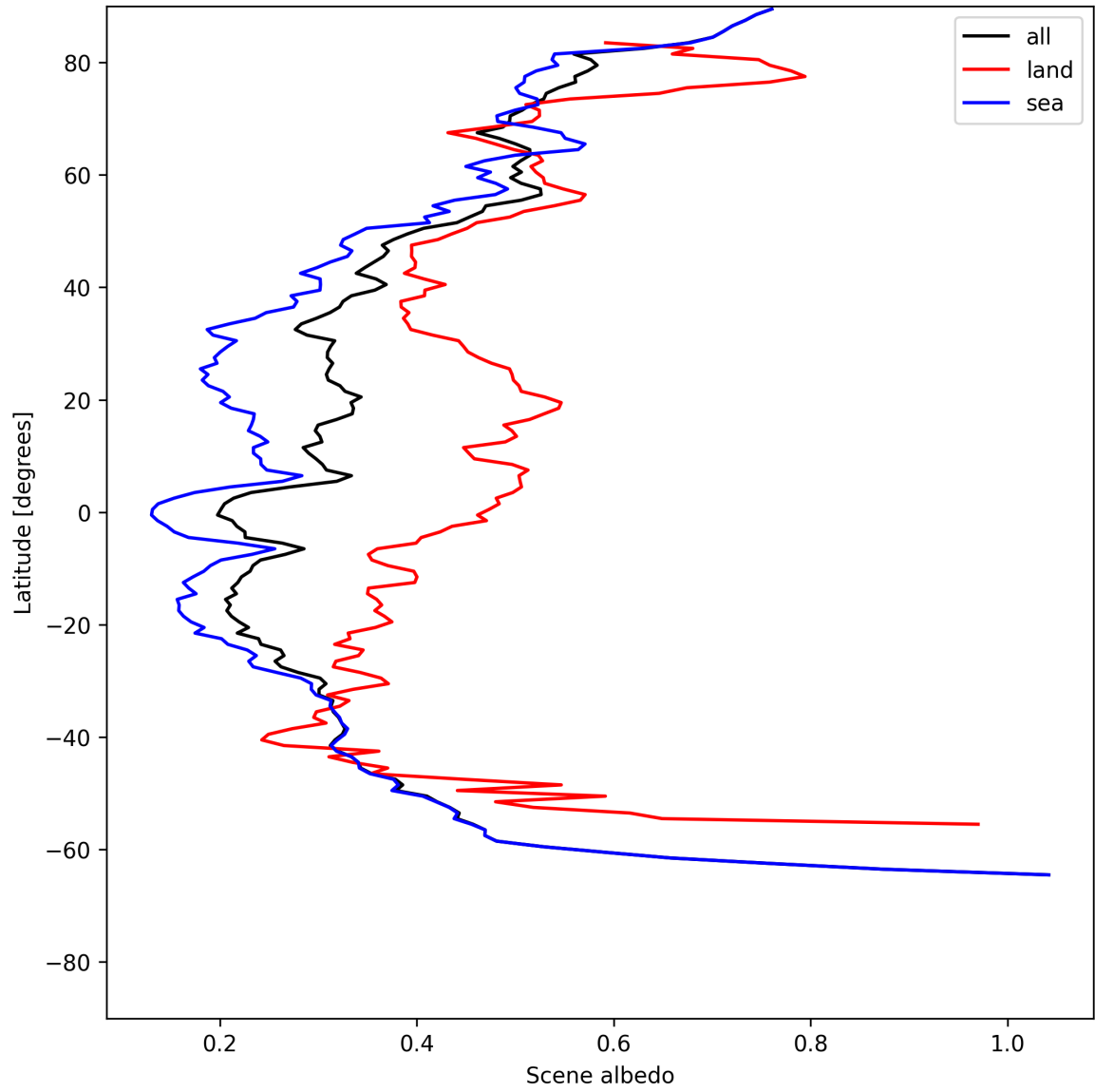
Figure 15: Zonal average of “Scene albedo” for 2025-06-30 to 2025-06-30.
