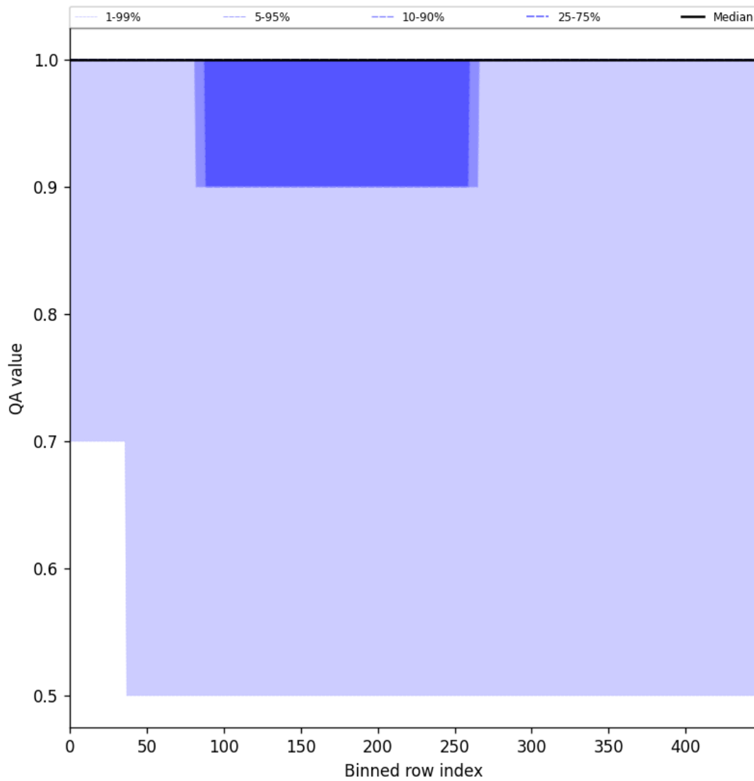
Figure 44: Along track statistics of “QA value” for 2025-06-30 to 2025-06-30
