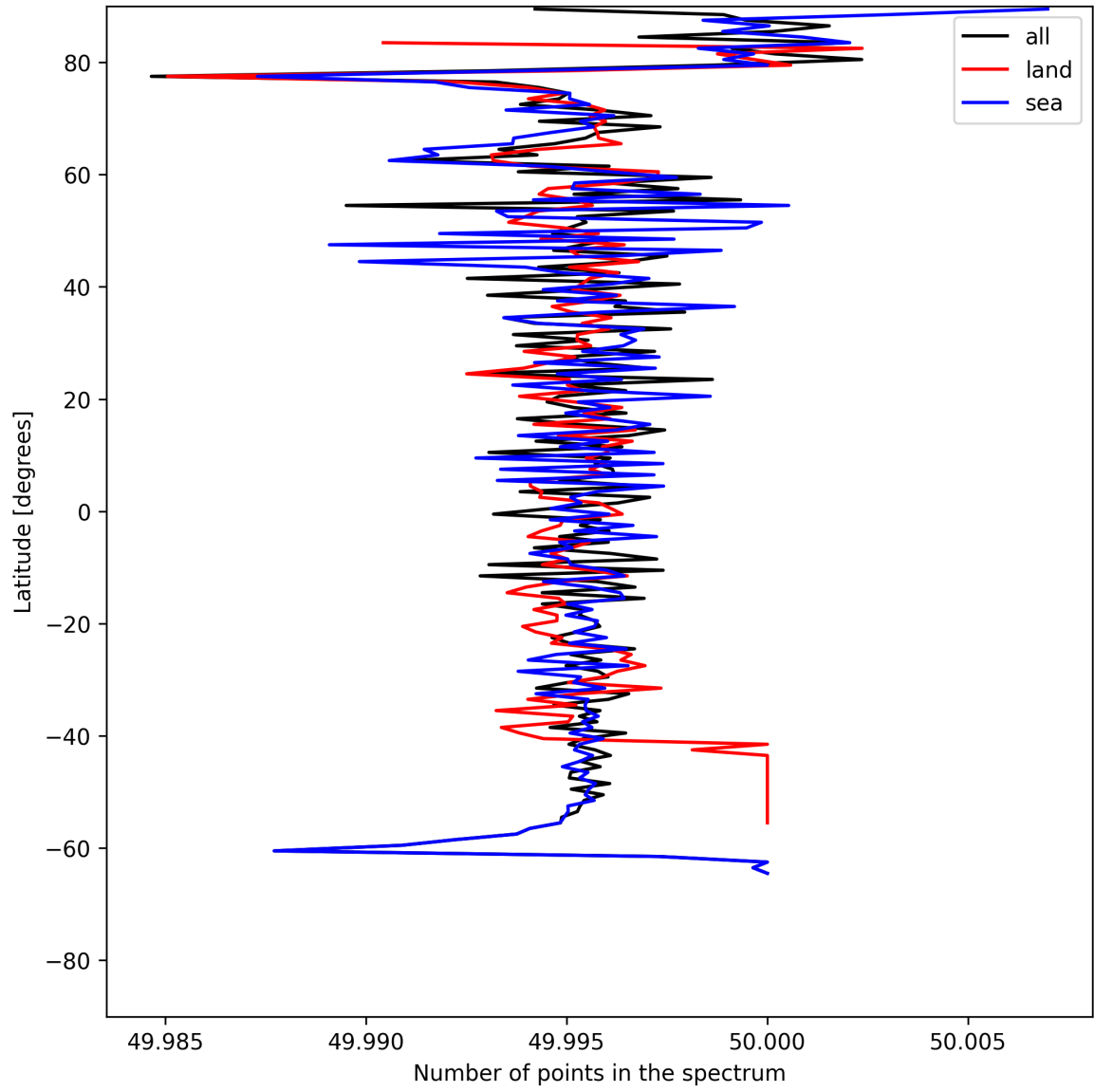
Figure 25: Zonal average of “Number of points in the spectrum” for 2025-06-30 to 2025-06-30.
