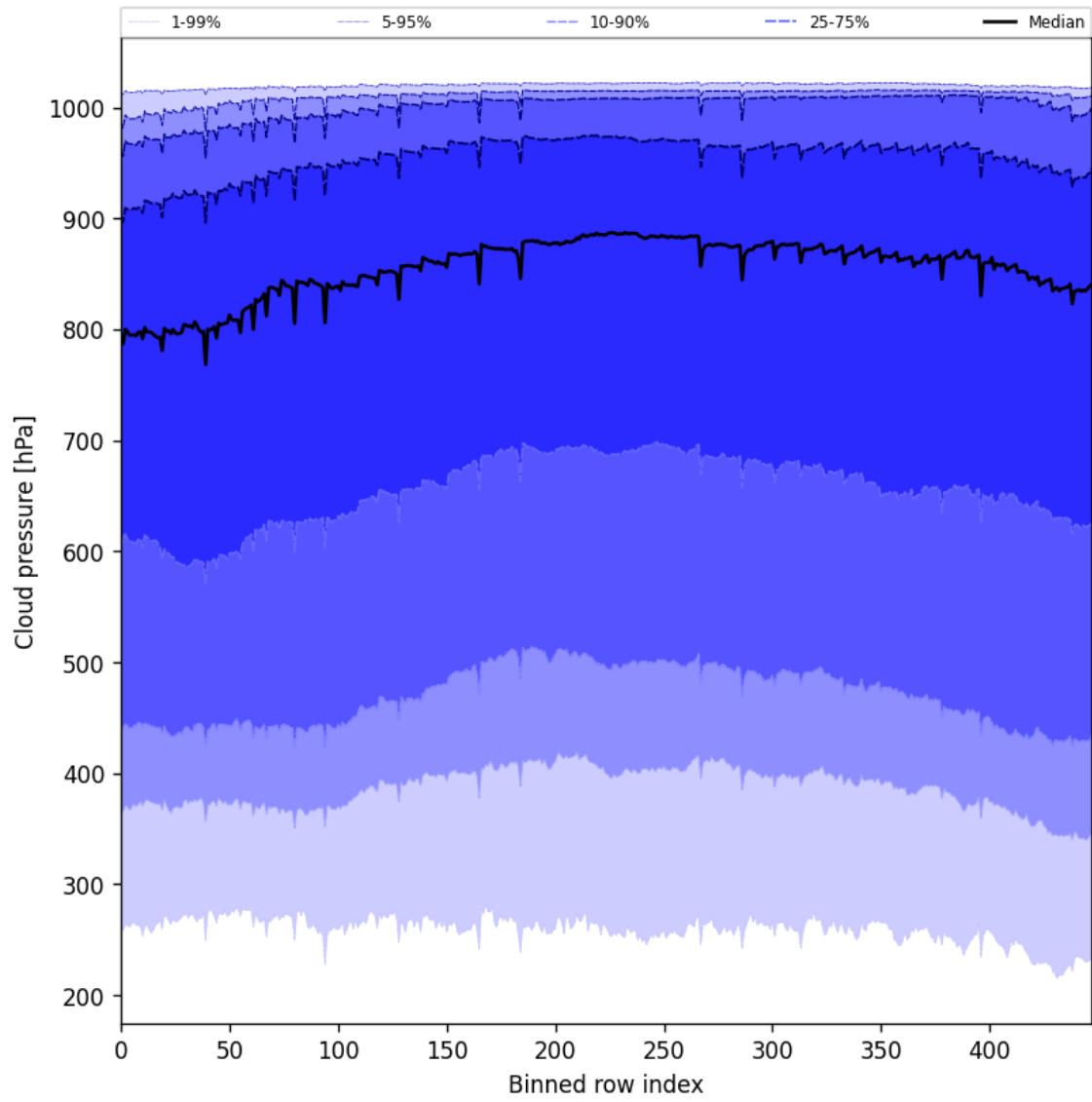
Figure 45: Along track statistics of “Cloud pressure” for 2025-06-30 to 2025-06-30
