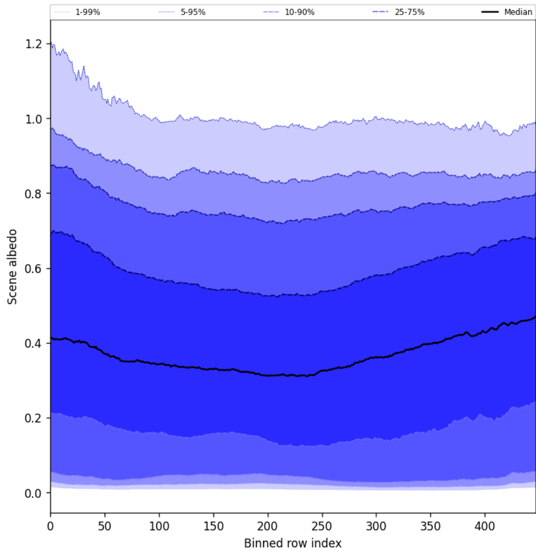
Figure 49: Along track statistics of “Scene albedo” for 2025-06-30 to 2025-06-30
