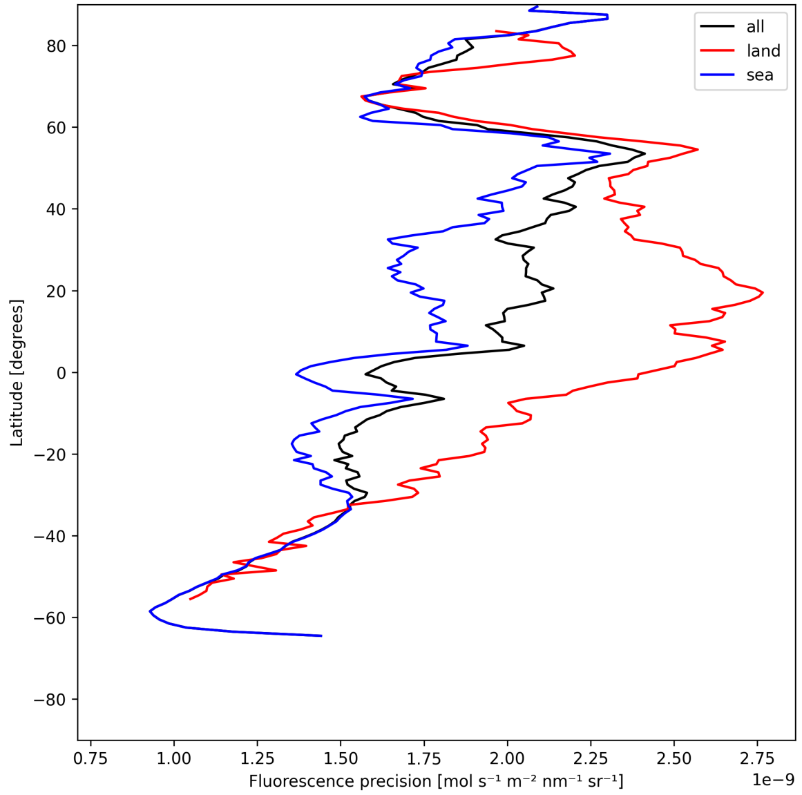
Figure 22: Zonal average of “Fluorescence precision” for 2025-06-30 to 2025-06-30.
