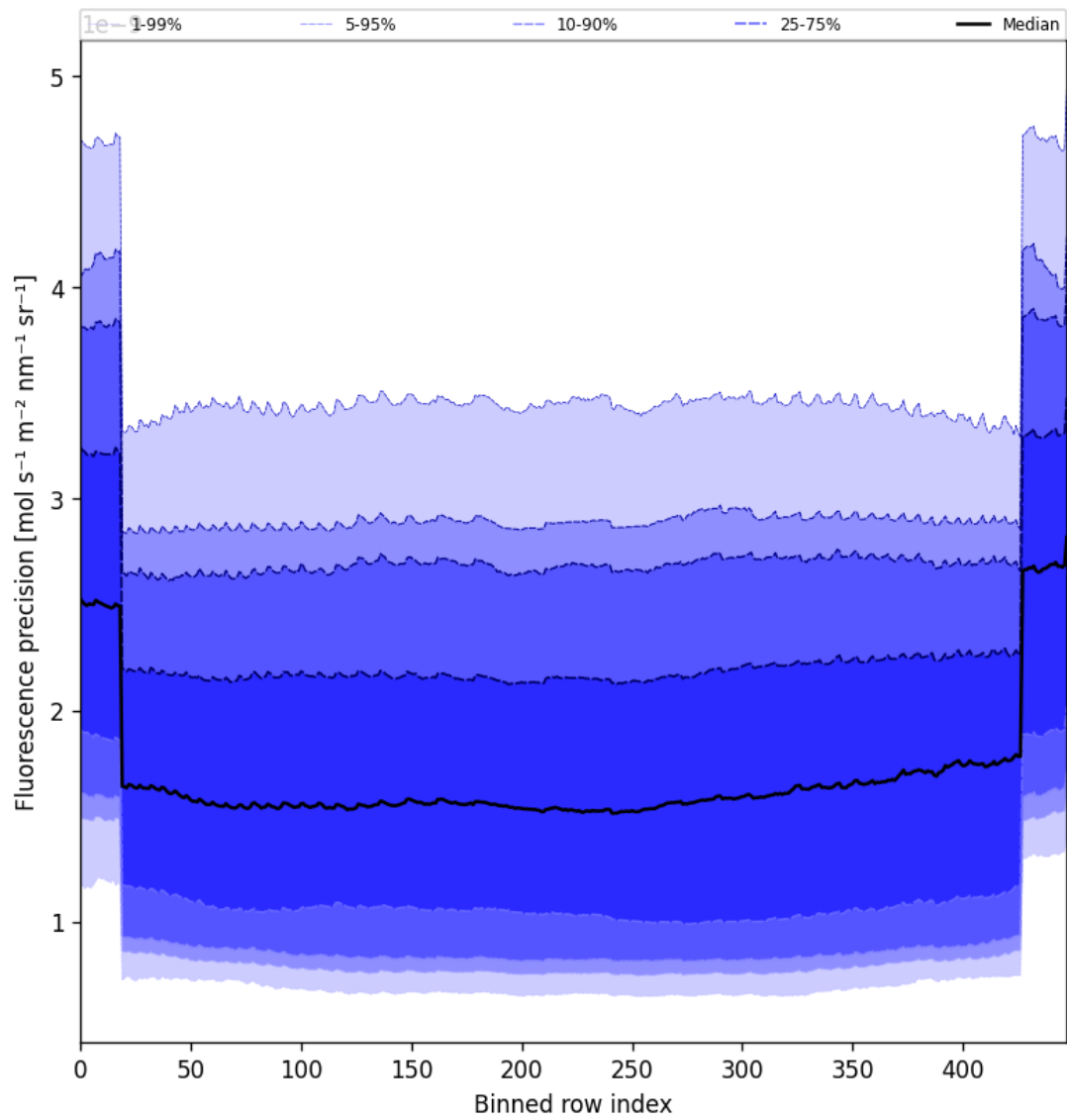
Figure 56: Along track statistics of “Fluorescence precision” for 2025-06-30 to 2025-06-30
