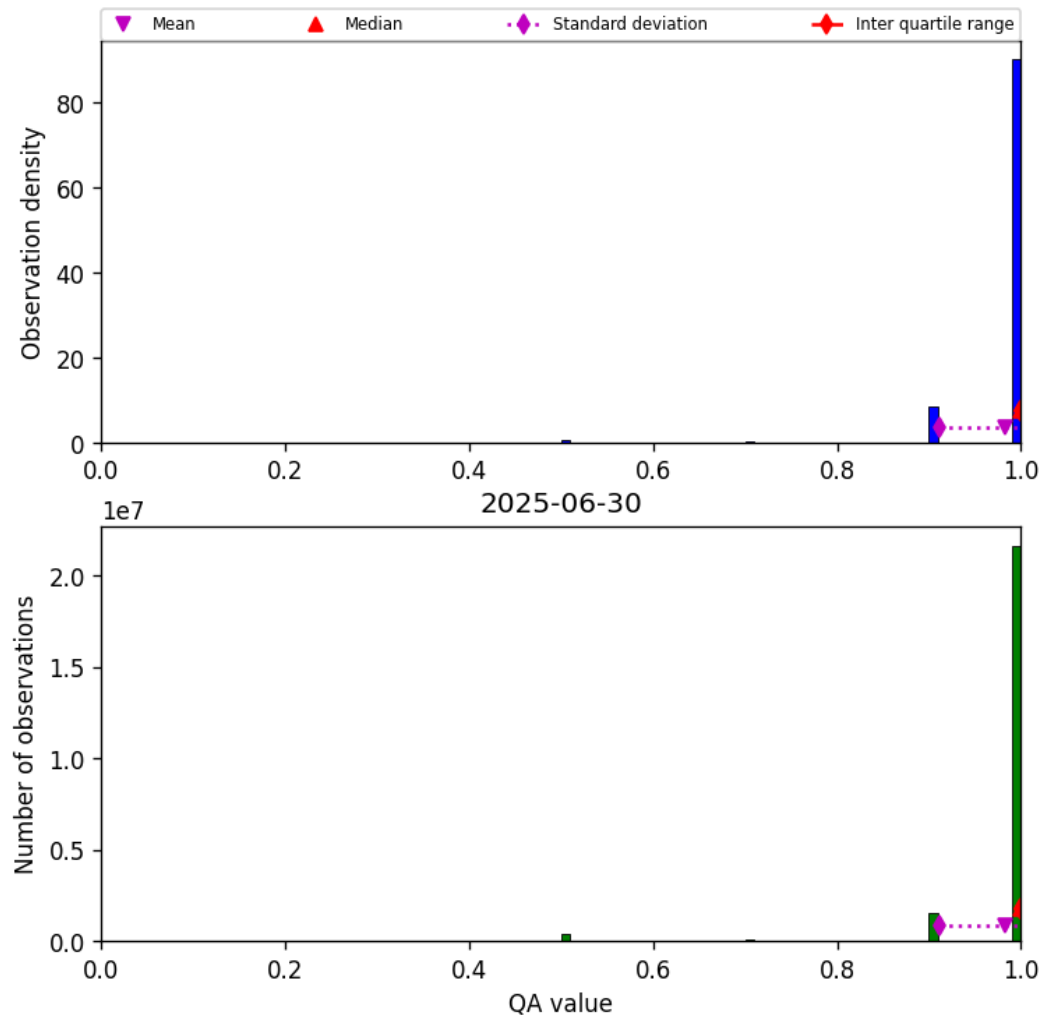
Figure 27: Histogram of “QA value” for 2025-06-30 to 2025-06-30
