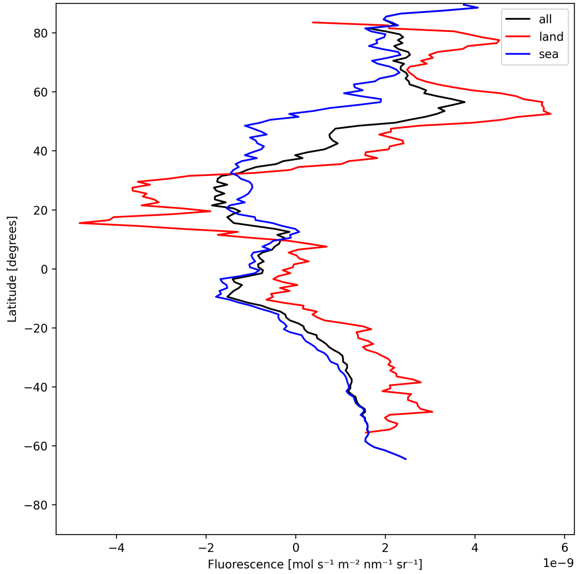
Figure 21: Zonal average of “Fluorescence” for 2025-06-30 to 2025-06-30.
