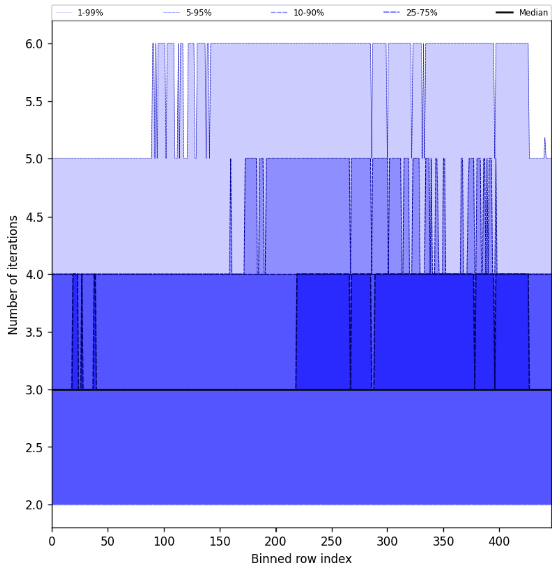
Figure 54: Along track statistics of “Number of iterations” for 2025-06-30 to 2025-06-30
