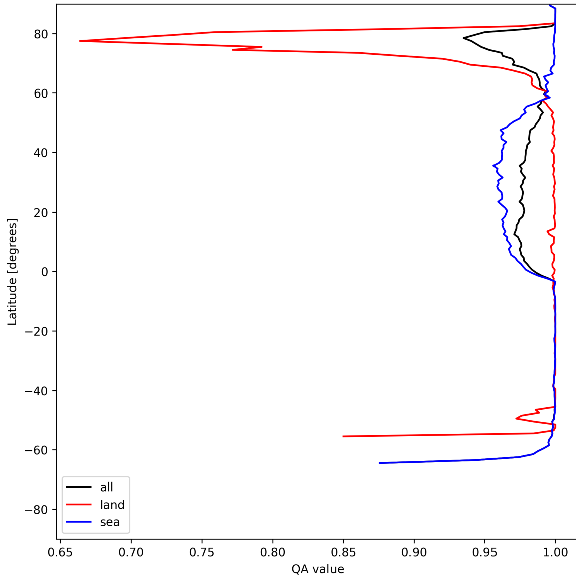
Figure 10: Zonal average of “QA value” for 2025-06-30 to 2025-06-30.
