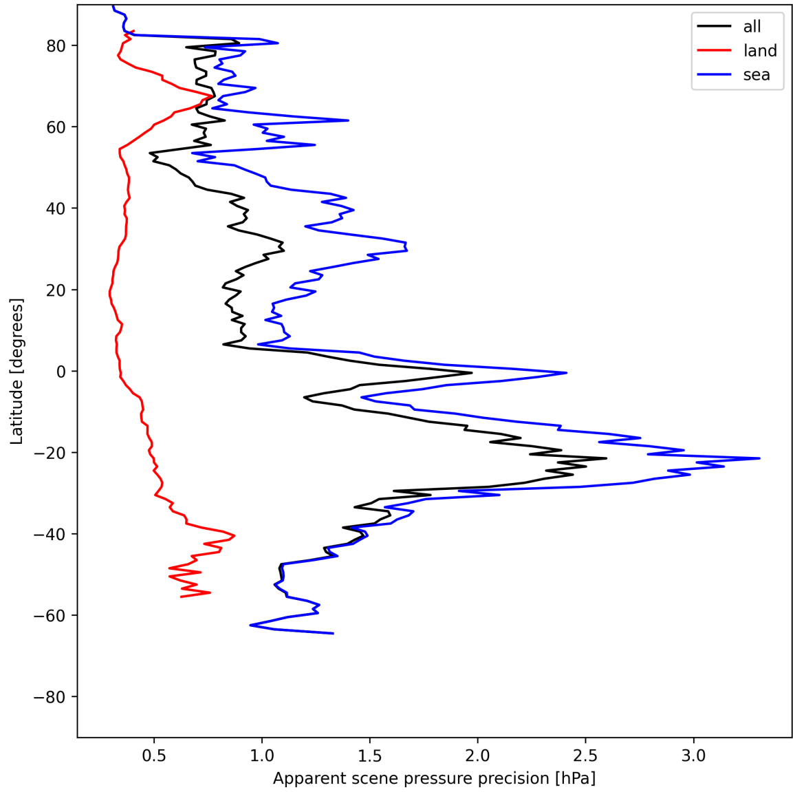
Figure 18: Zonal average of “Apparent scene pressure precision” for 2025-06-30 to 2025-06-30.
