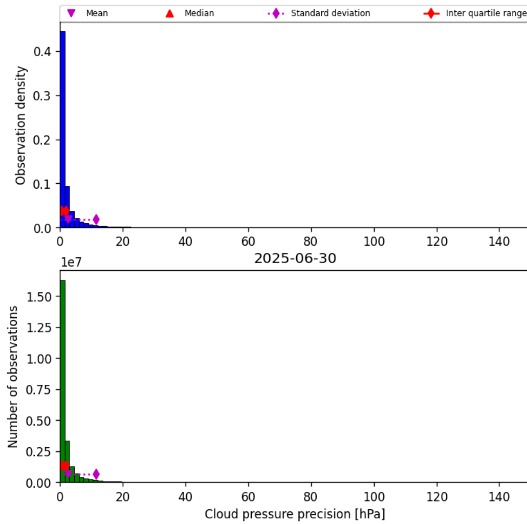
Figure 29: Histogram of “Cloud pressure precision” for 2025-06-30 to 2025-06-30
