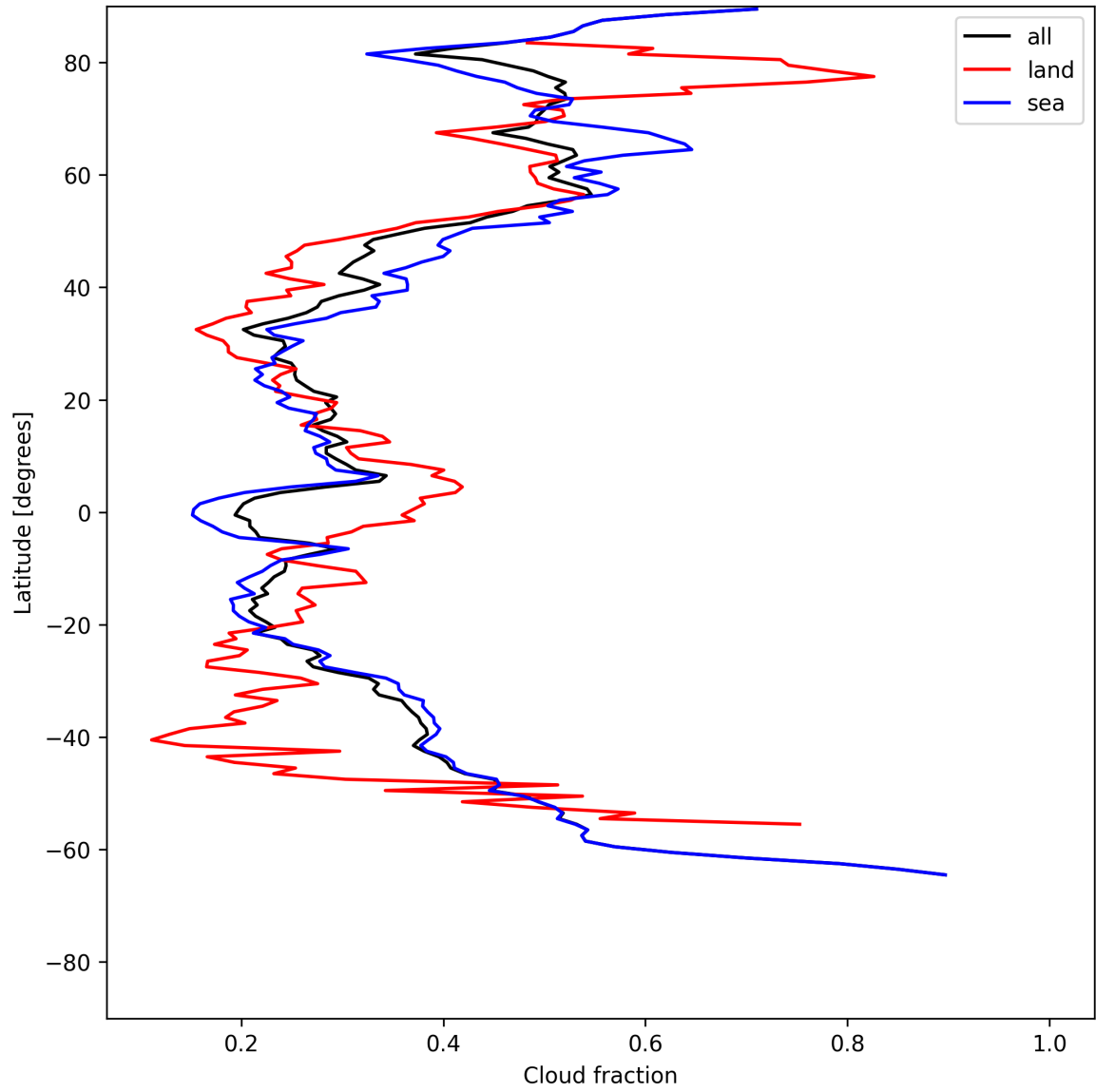
Figure 13: Zonal average of “Cloud fraction” for 2025-06-30 to 2025-06-30.
