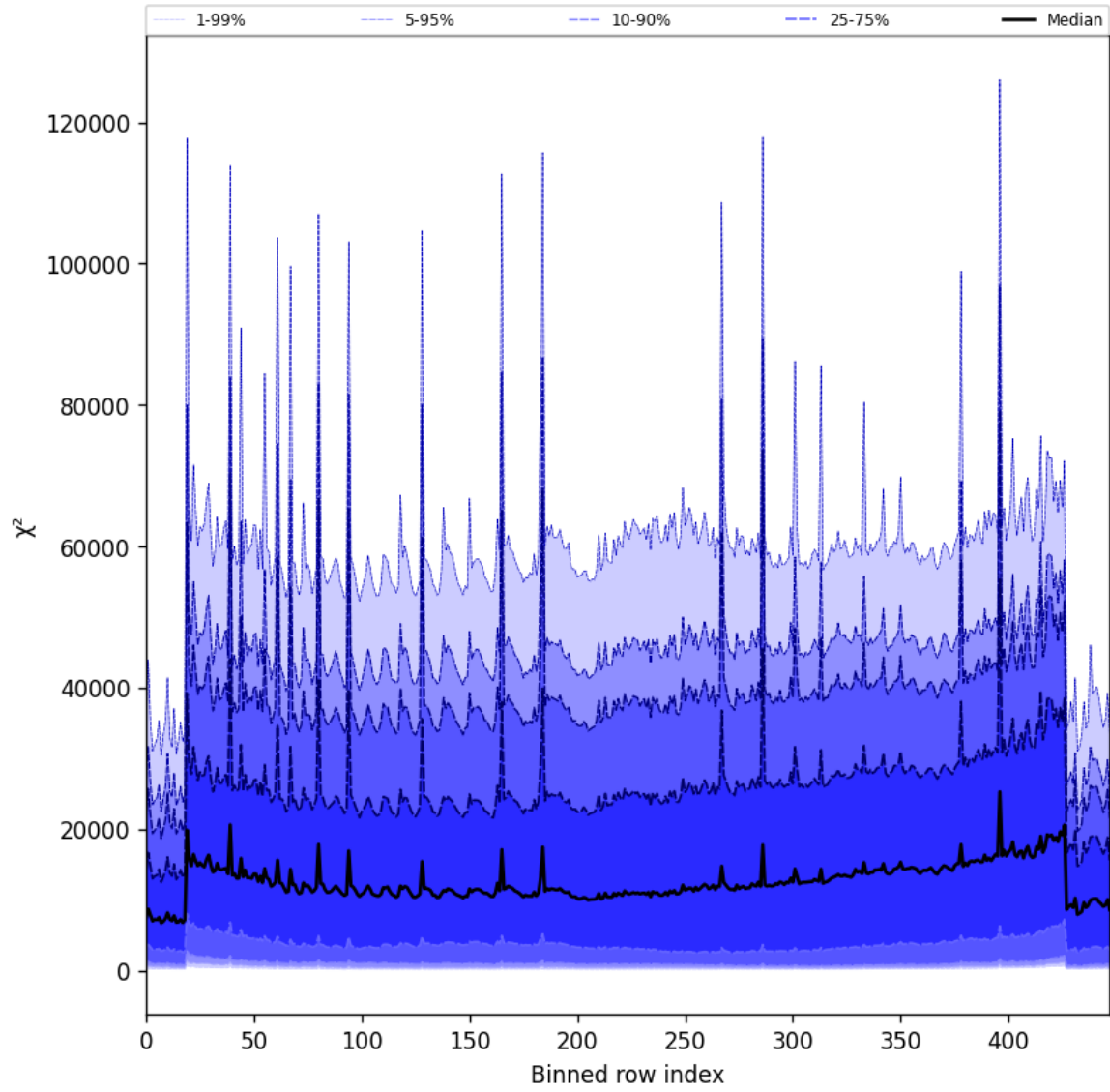
Figure 53: Along track statistics of “ \chi^2 ” for 2025-06-30 to 2025-06-30
