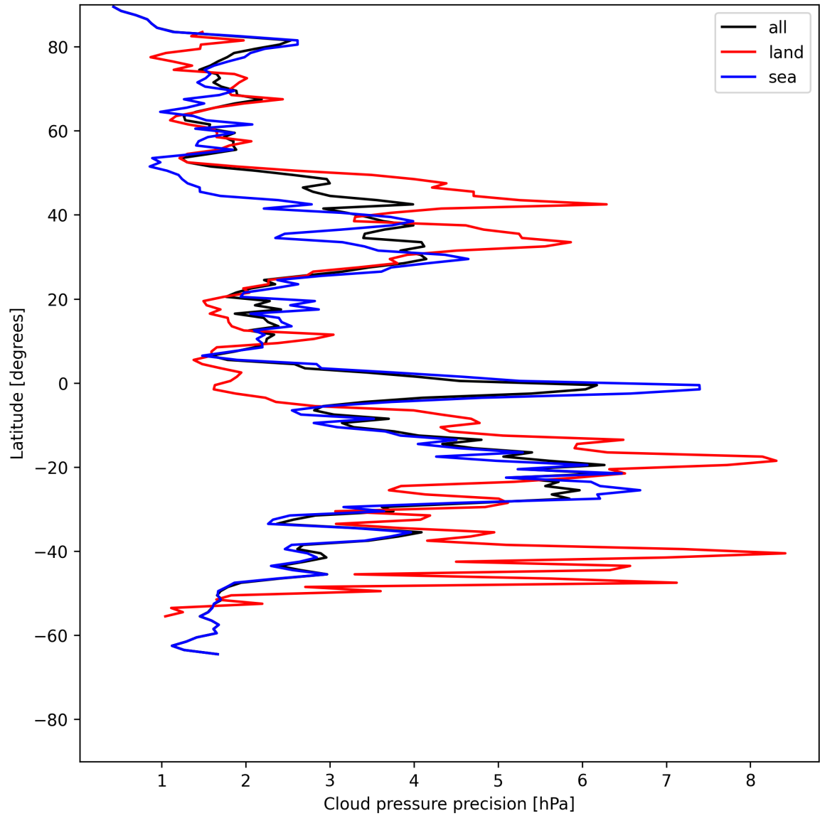
Figure 12: Zonal average of “Cloud pressure precision” for 2025-06-30 to 2025-06-30.
