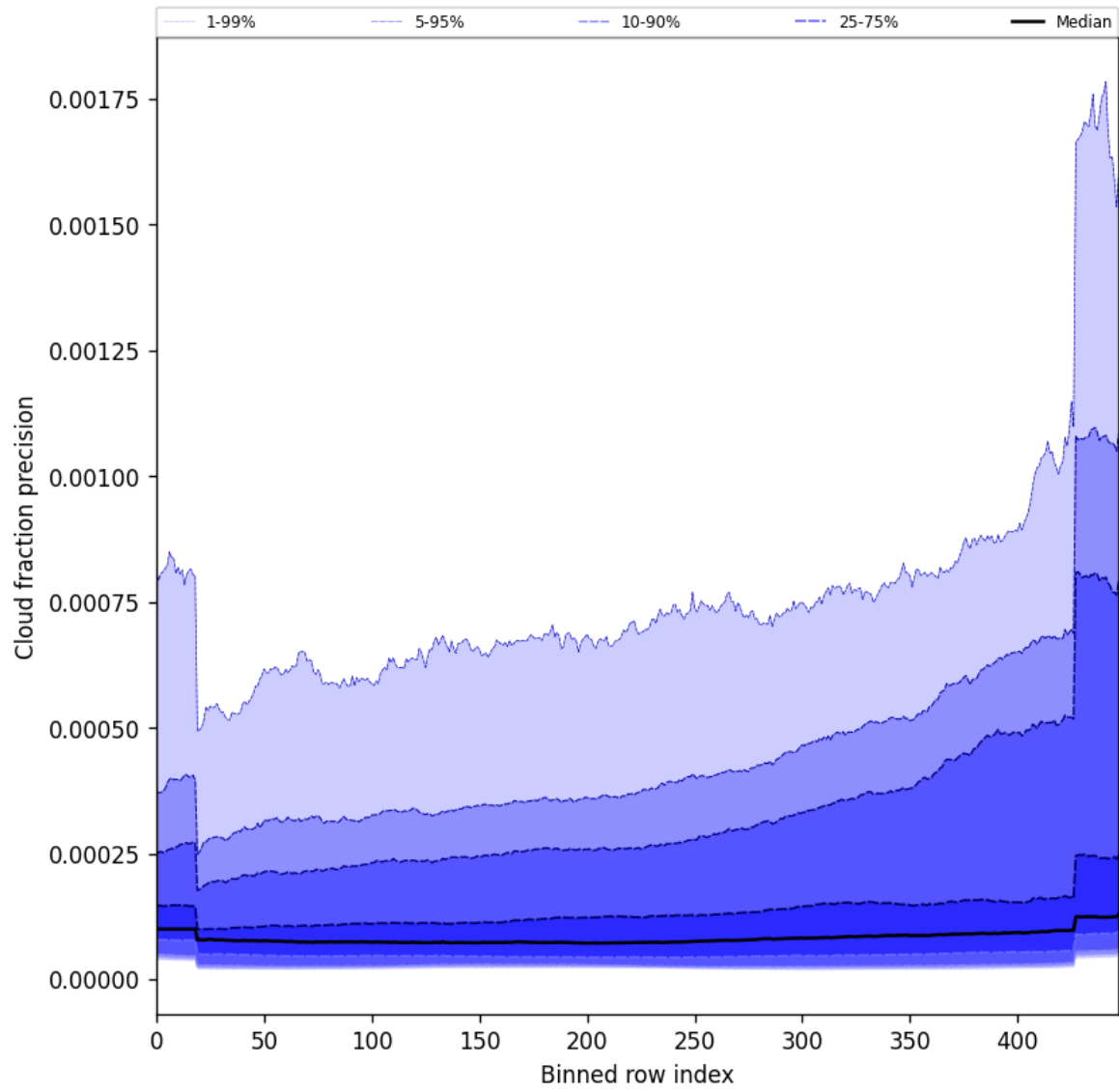
Figure 48: Along track statistics of “Cloud fraction precision” for 2025-06-30 to 2025-06-30
