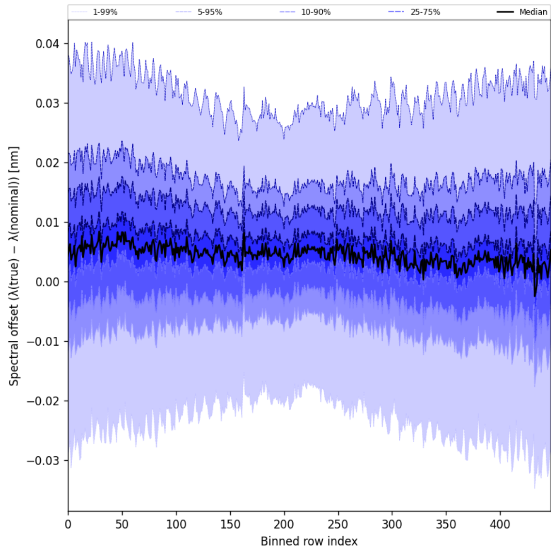
Figure 60: Along track statistics of “Spectral offset ( \lambda_{\text{true}} - \lambda_{\text{nominal}} )” for 2025-06-30 to 2025-06-30
