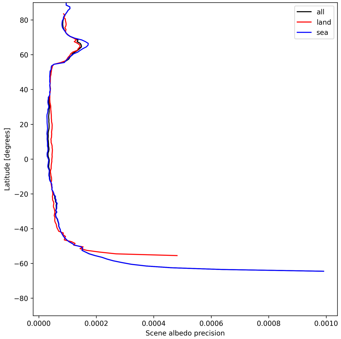
Figure 16: Zonal average of “Scene albedo precision” for 2025-06-30 to 2025-06-30.
