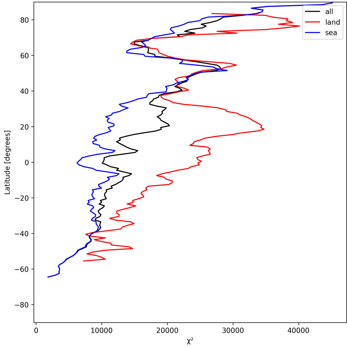
Figure 19: Zonal average of “ \chi^2 ” for 2025-06-30 to 2025-06-30.
