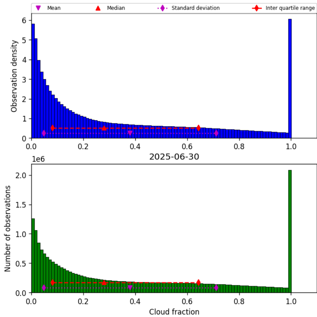
Figure 30: Histogram of “Cloud fraction” for 2025-06-30 to 2025-06-30
