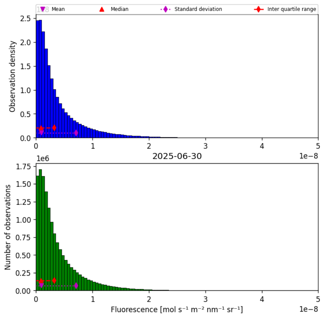
Figure 38: Histogram of “Fluorescence” for 2025-06-30 to 2025-06-30
