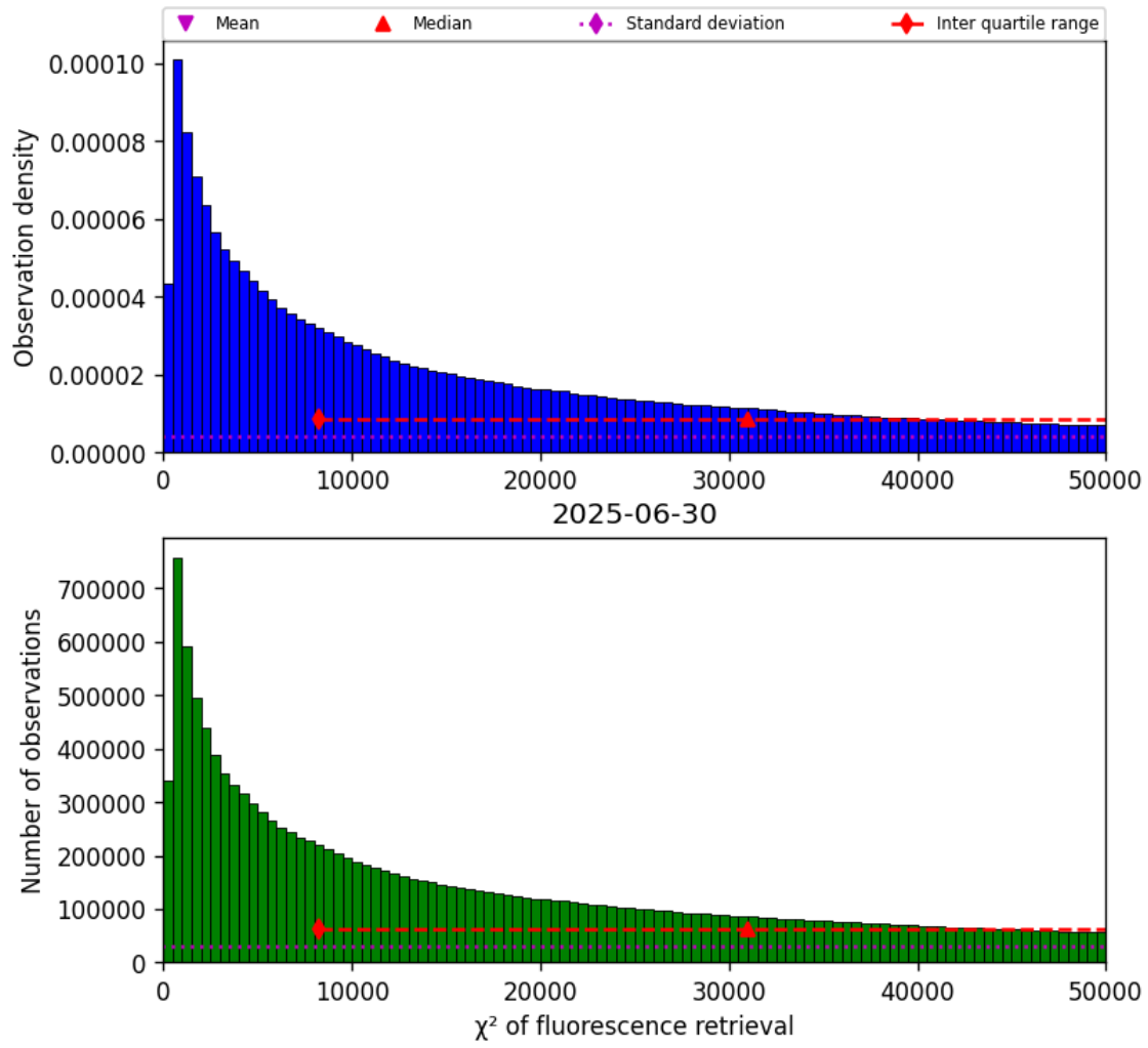
Figure 40: Histogram of “ \chi^2 of fluorescence retrieval” for 2025-06-30 to 2025-06-30
