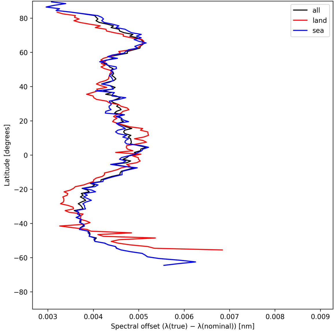
Figure 26: Zonal average of “Spectral offset ( \lambda_{\text{true}} - \lambda_{\text{nominal}} )” for 2025-06-30 to 2025-06-30.
