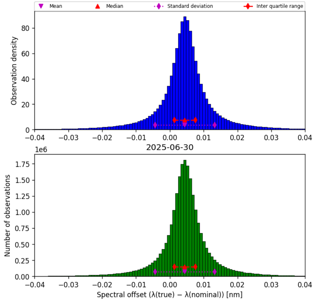
Figure 43: Histogram of “Spectral offset ( \lambda_{\text{true}} - \lambda_{\text{nominal}} )” for 2025-06-30 to 2025-06-30
