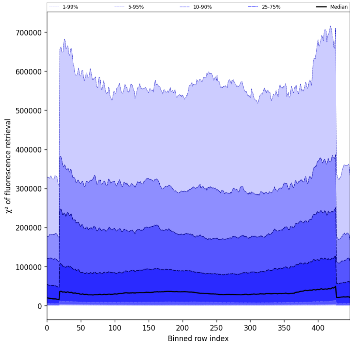
Figure 57: Along track statistics of “ \chi^2 of fluorescence retrieval” for 2025-06-30 to 2025-06-30
