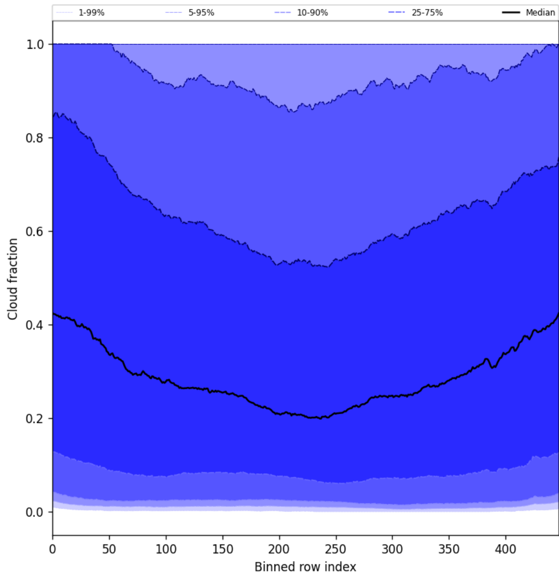
Figure 47: Along track statistics of “Cloud fraction” for 2025-06-30 to 2025-06-30
