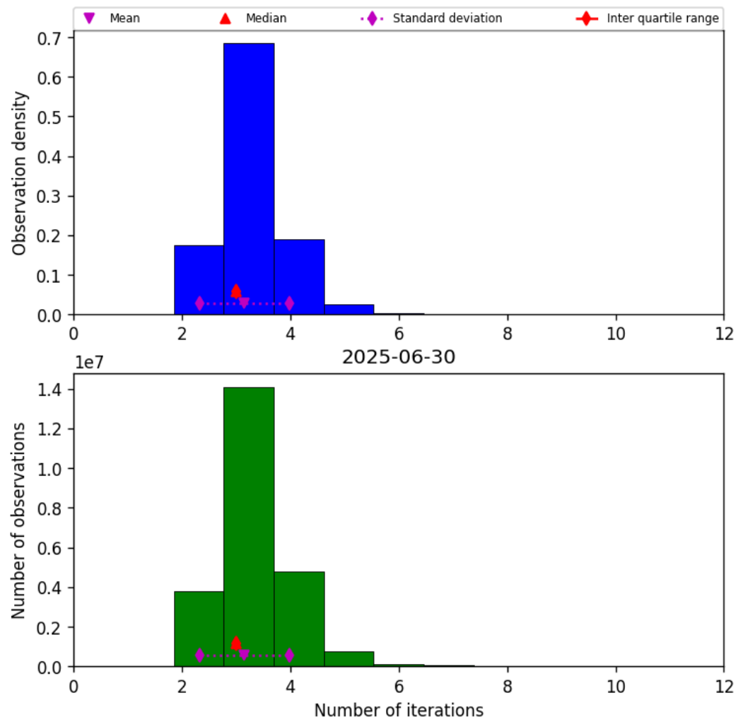
Figure 37: Histogram of “Number of iterations” for 2025-06-30 to 2025-06-30
