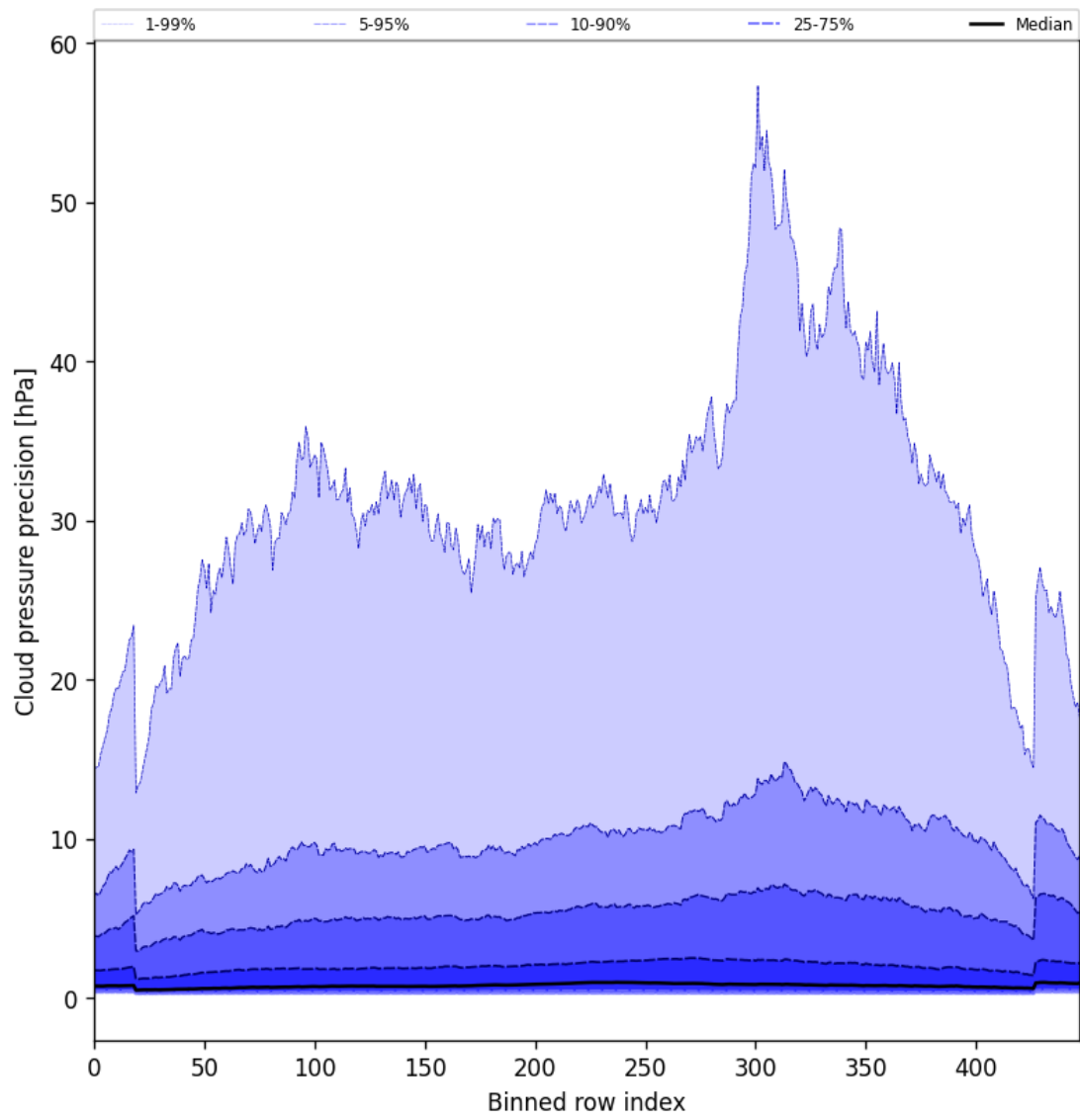
Figure 46: Along track statistics of “Cloud pressure precision” for 2025-06-30 to 2025-06-30
