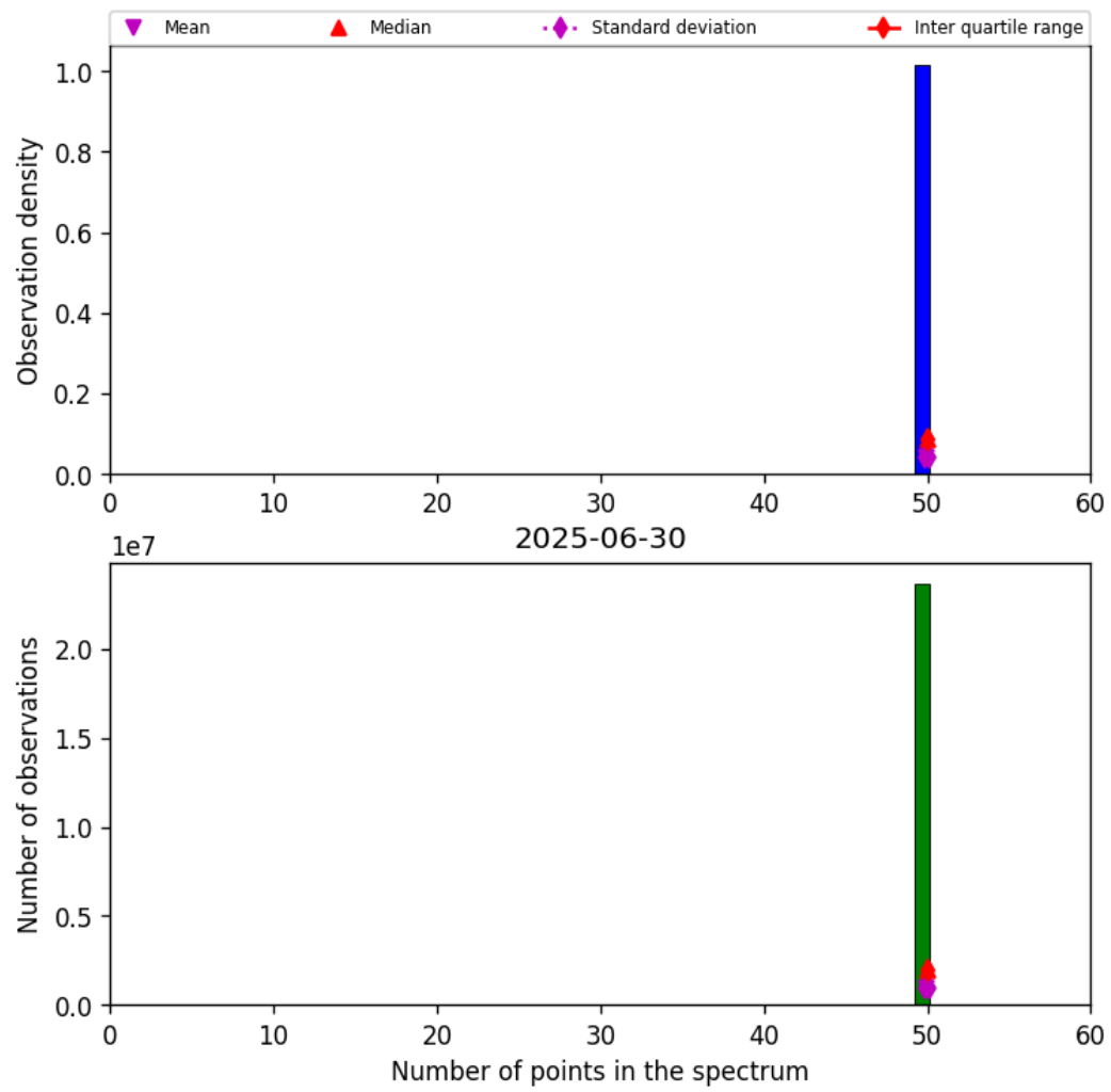
Figure 42: Histogram of "Number of points in the spectrum" for 2025-06-30 to 2025-06-30
