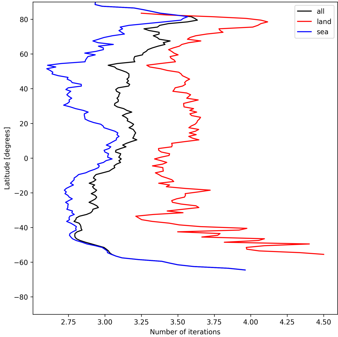
Figure 20: Zonal average of “Number of iterations” for 2025-06-30 to 2025-06-30.
