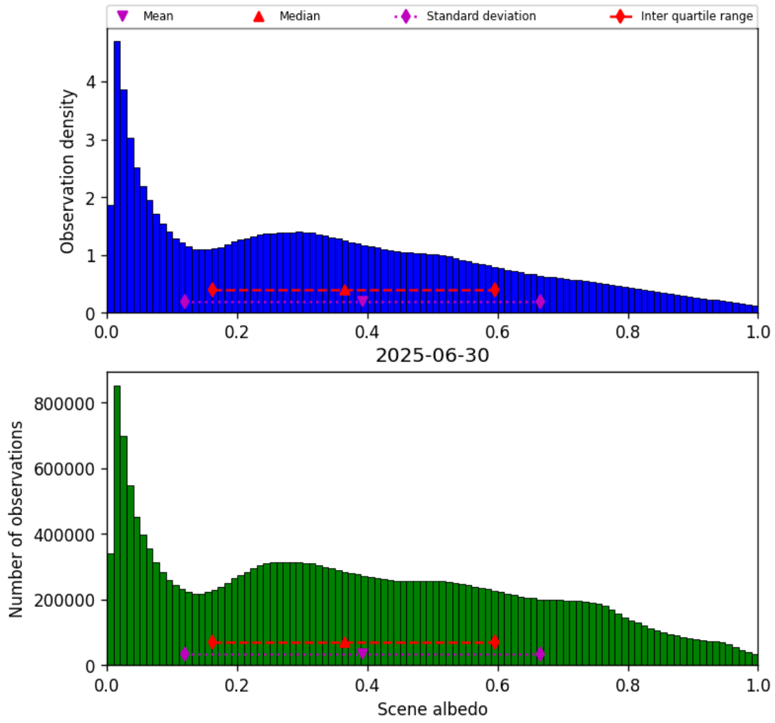
Figure 32: Histogram of “Scene albedo” for 2025-06-30 to 2025-06-30
