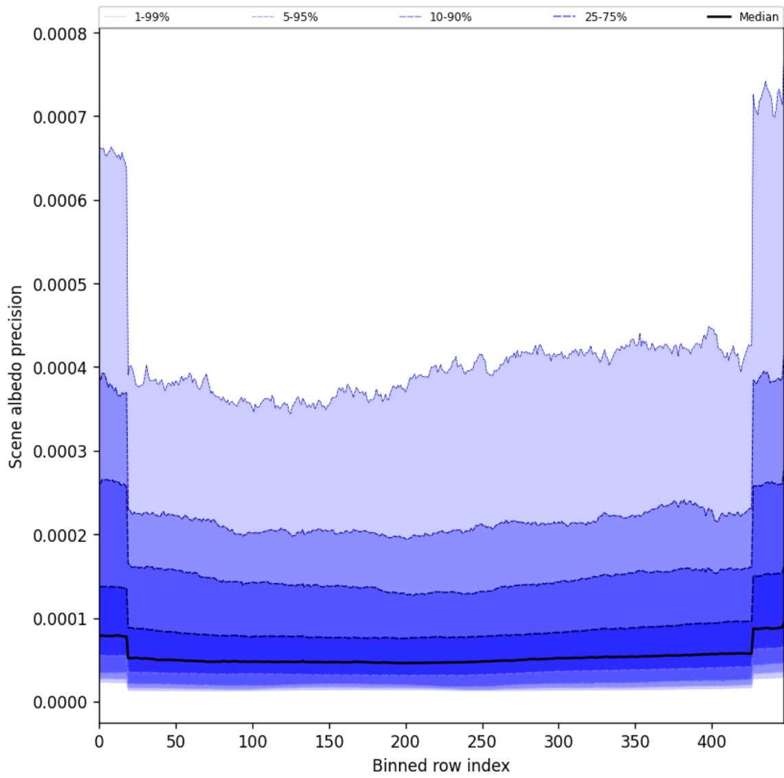
Figure 50: Along track statistics of “Scene albedo precision” for 2025-06-30 to 2025-06-30
