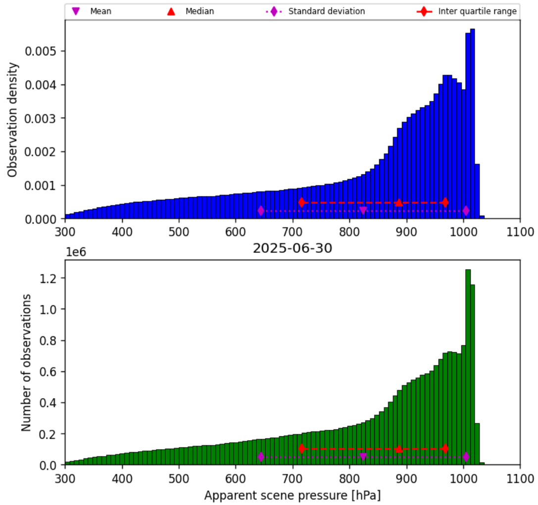
Figure 34: Histogram of “Apparent scene pressure” for 2025-06-30 to 2025-06-30
