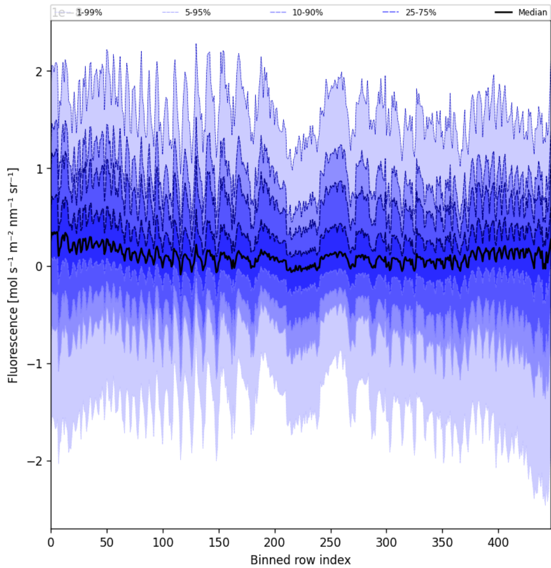
Figure 55: Along track statistics of “Fluorescence” for 2025-06-30 to 2025-06-30
