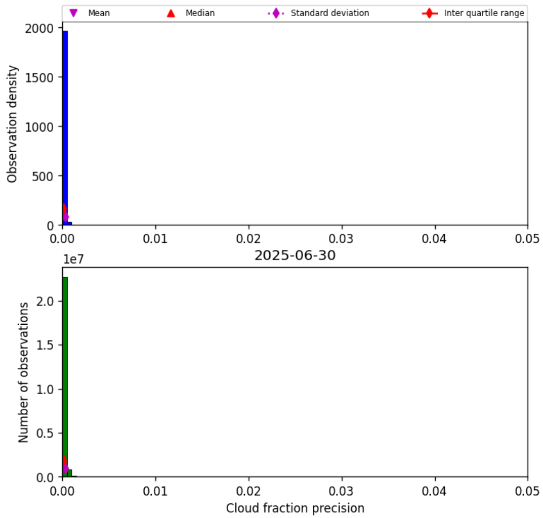
Figure 31: Histogram of “Cloud fraction precision” for 2025-06-30 to 2025-06-30
