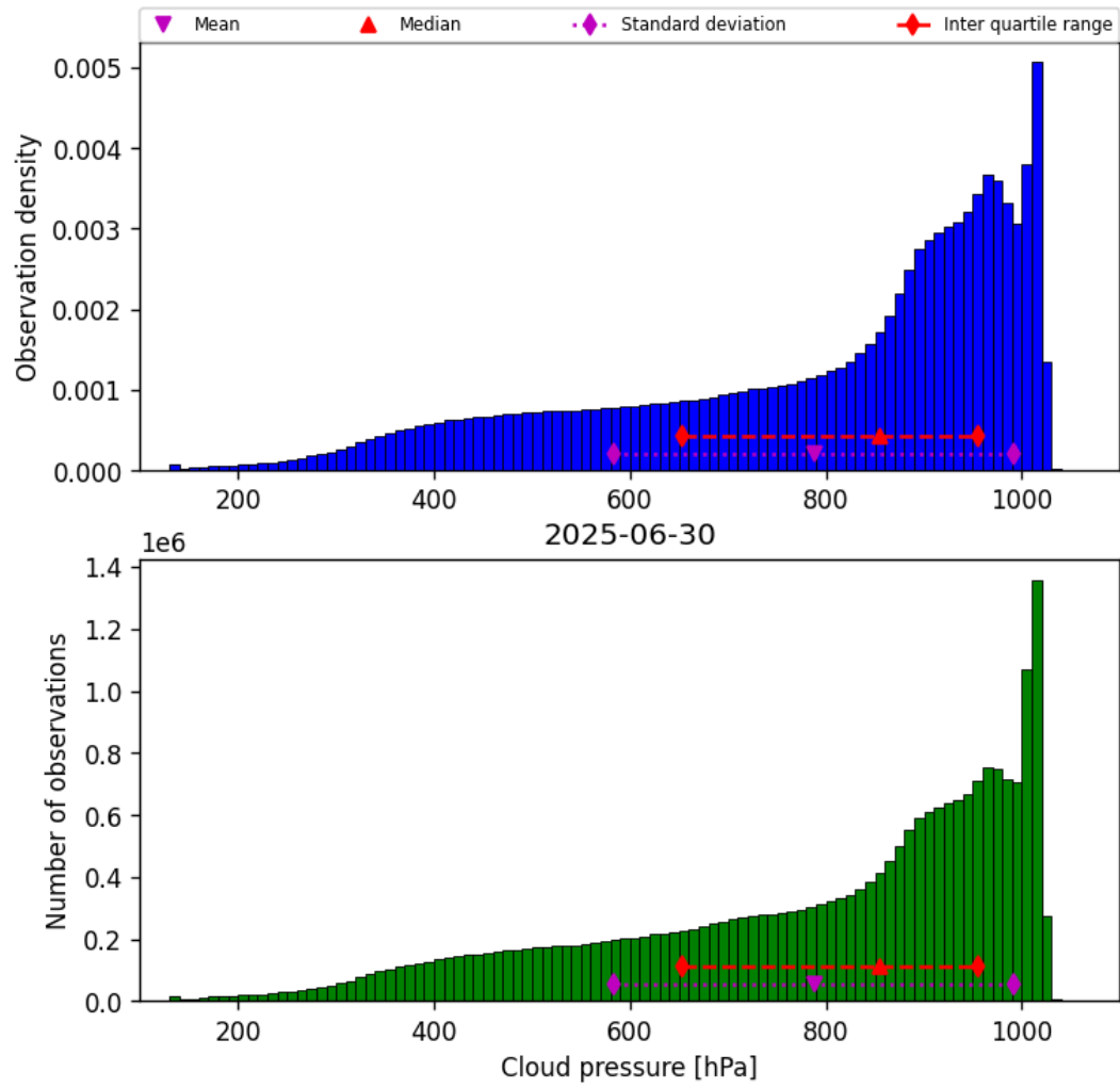
Figure 28: Histogram of “Cloud pressure” for 2025-06-30 to 2025-06-30
