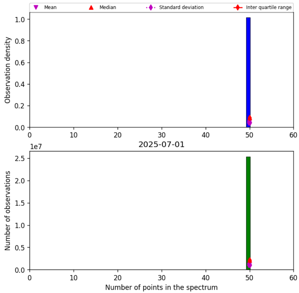
Figure 42: Histogram of “Number of points in the spectrum” for 2025-07-01 to 2025-07-02
