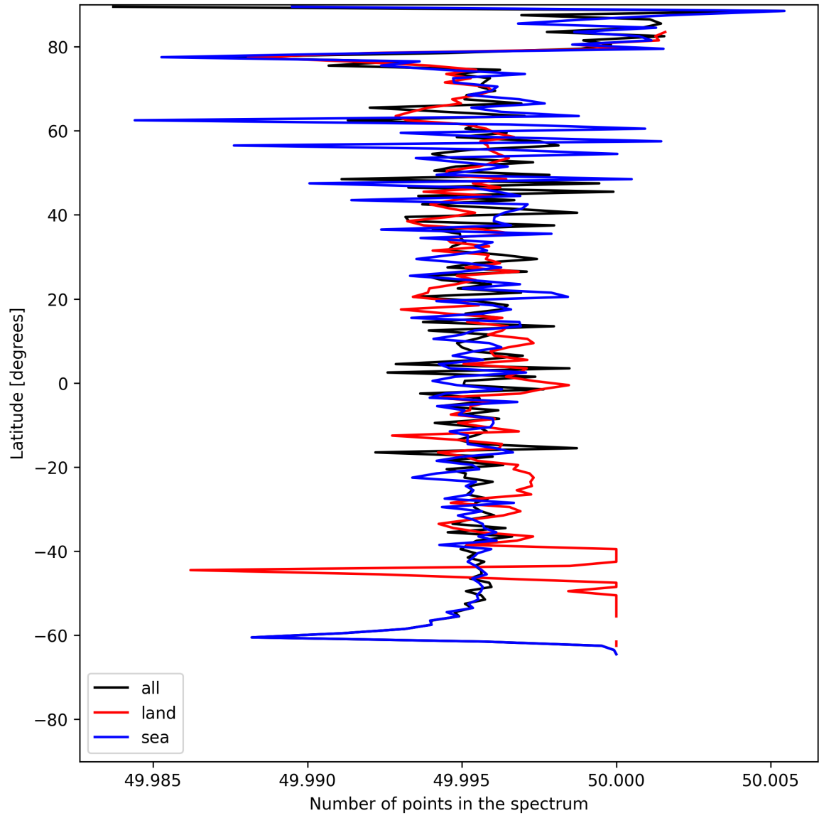
Figure 25: Zonal average of “Number of points in the spectrum” for 2025-07-01 to 2025-07-02.
