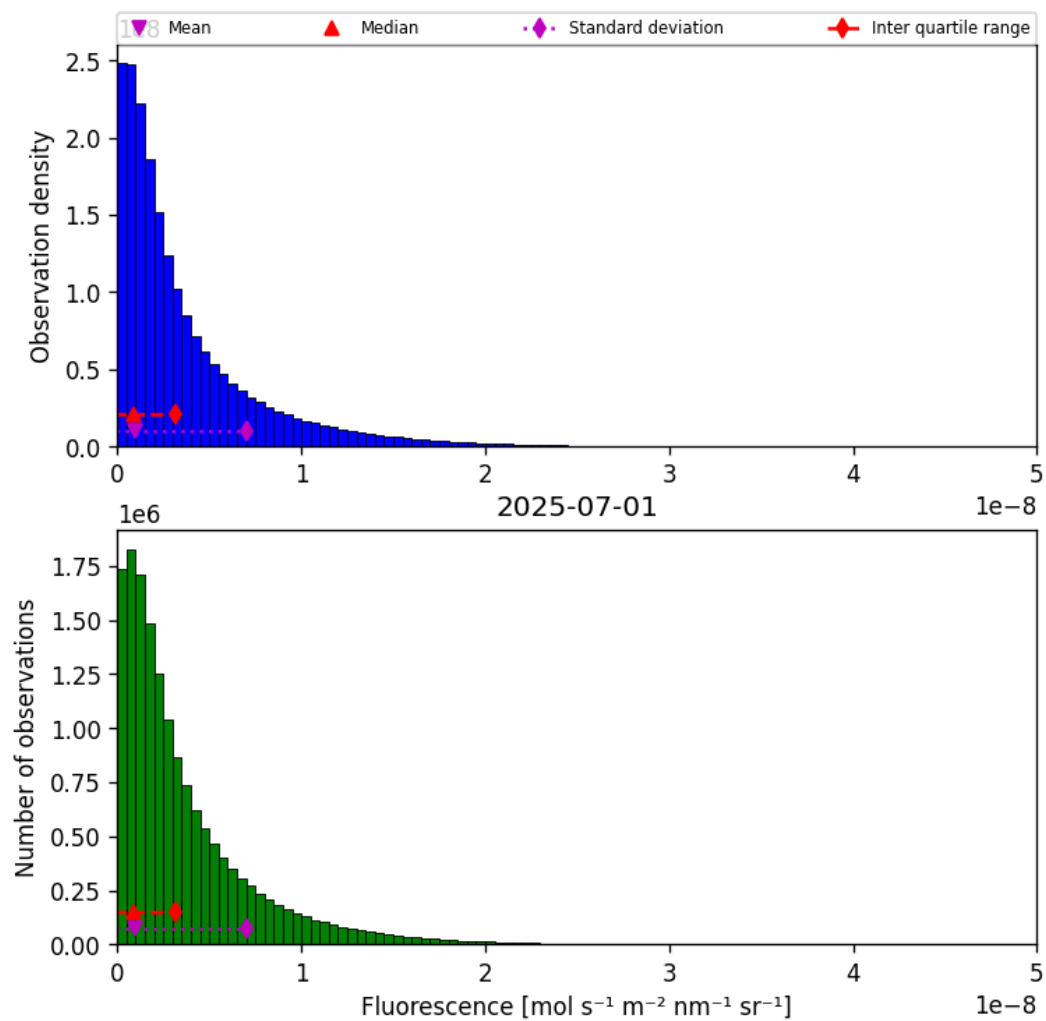
Figure 38: Histogram of “Fluorescence” for 2025-07-01 to 2025-07-02
