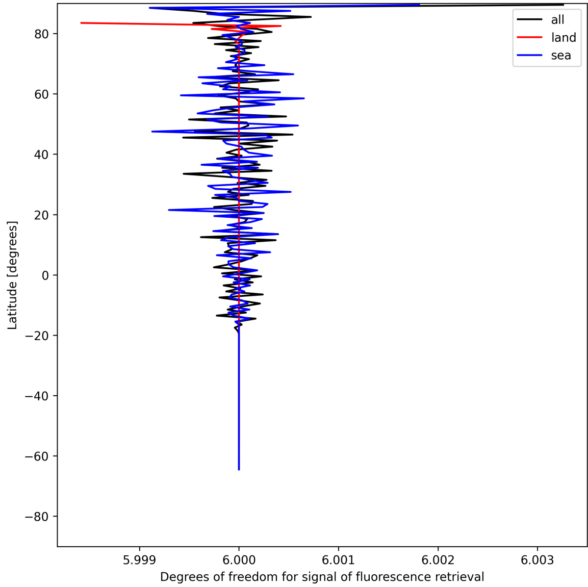
Figure 24: Zonal average of “Degrees of freedom for signal of fluorescence retrieval” for 2025-07-01 to 2025-07-02.
