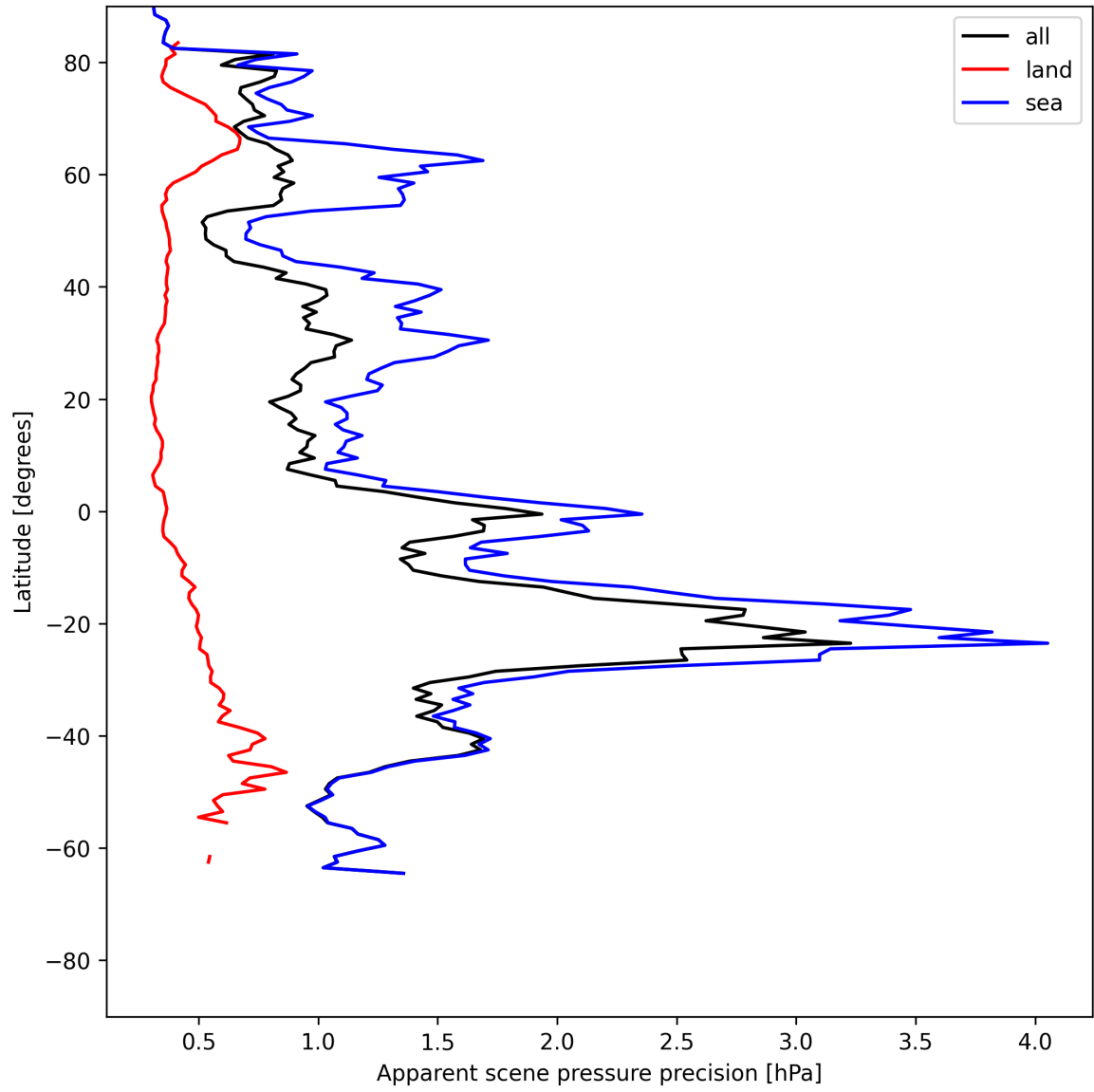
Figure 18: Zonal average of “Apparent scene pressure precision” for 2025-07-01 to 2025-07-02.
