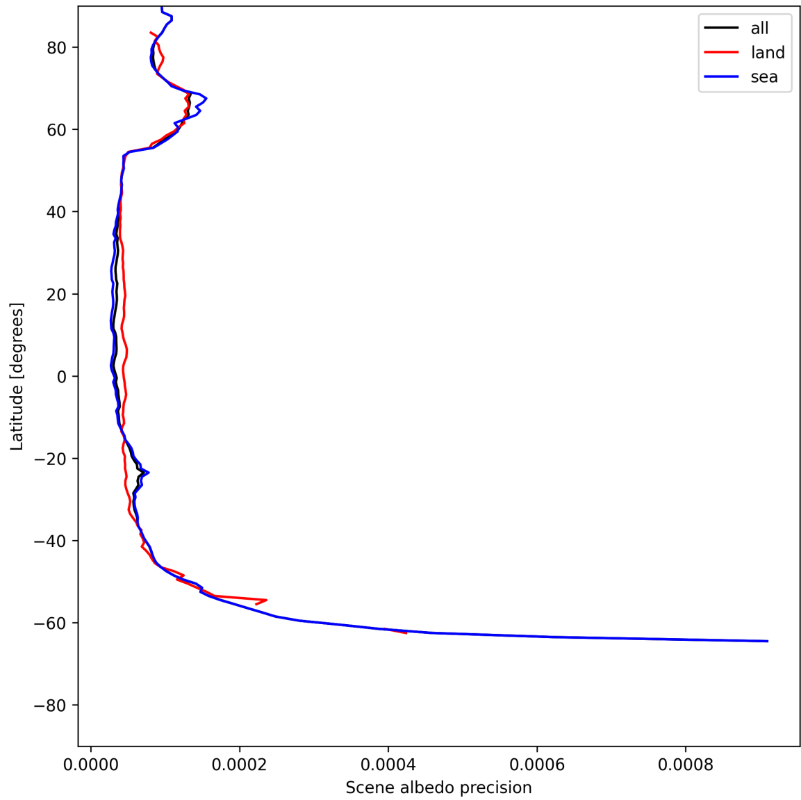
Figure 16: Zonal average of “Scene albedo precision” for 2025-07-01 to 2025-07-02.
