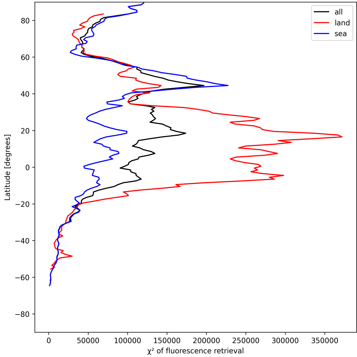
Figure 23: Zonal average of “ \chi^2 of fluorescence retrieval” for 2025-07-01 to 2025-07-02.
