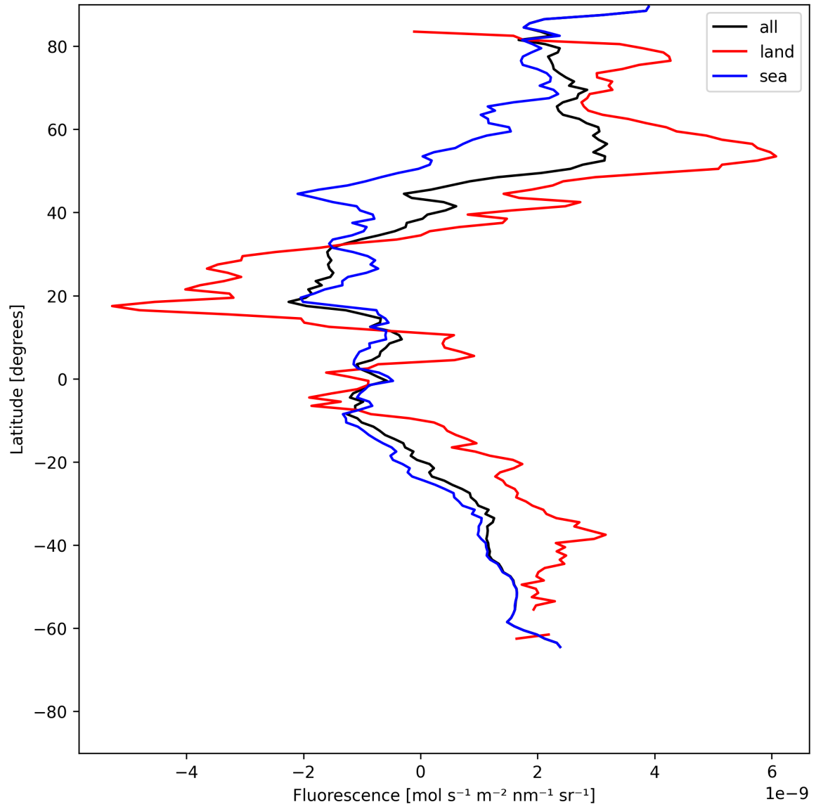
Figure 21: Zonal average of “Fluorescence” for 2025-07-01 to 2025-07-02.
