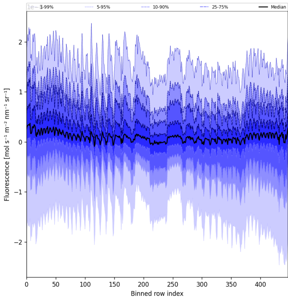
Figure 55: Along track statistics of “Fluorescence” for 2025-07-01 to 2025-07-02
