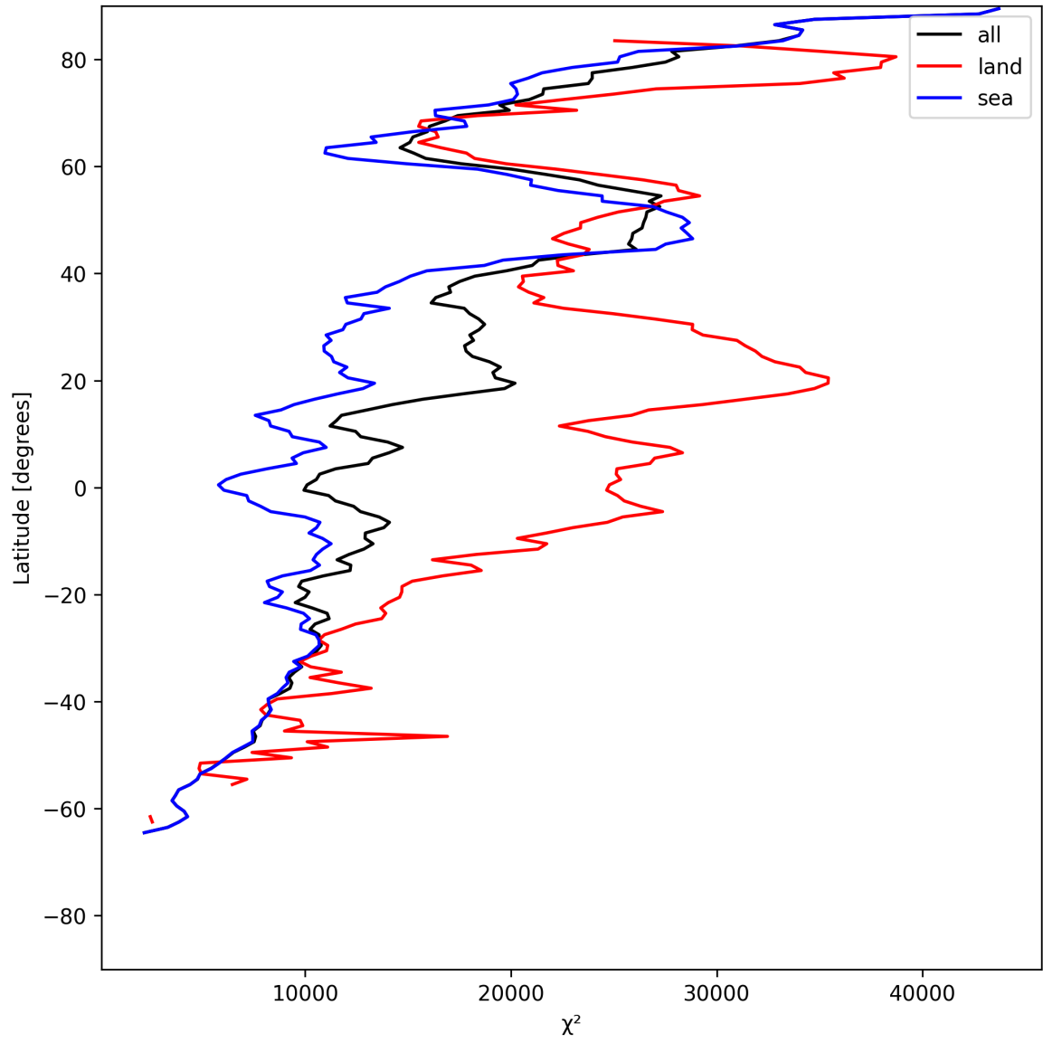
Figure 19: Zonal average of “ \chi^2 ” for 2025-07-01 to 2025-07-02.
