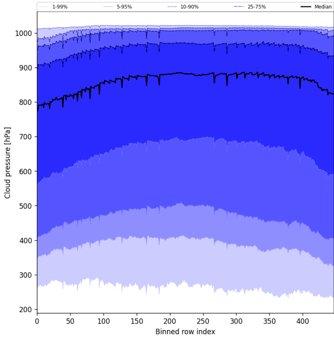
Figure 45: Along track statistics of “Cloud pressure” for 2025-07-01 to 2025-07-02
