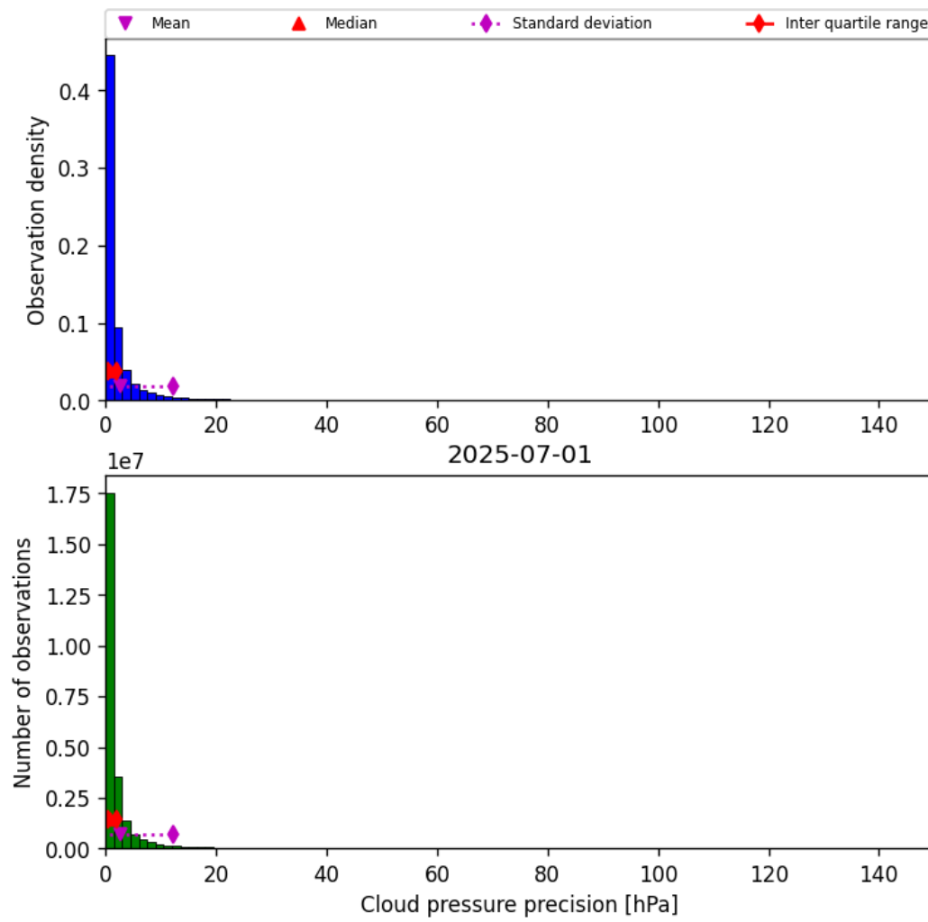
Figure 29: Histogram of “Cloud pressure precision” for 2025-07-01 to 2025-07-02
