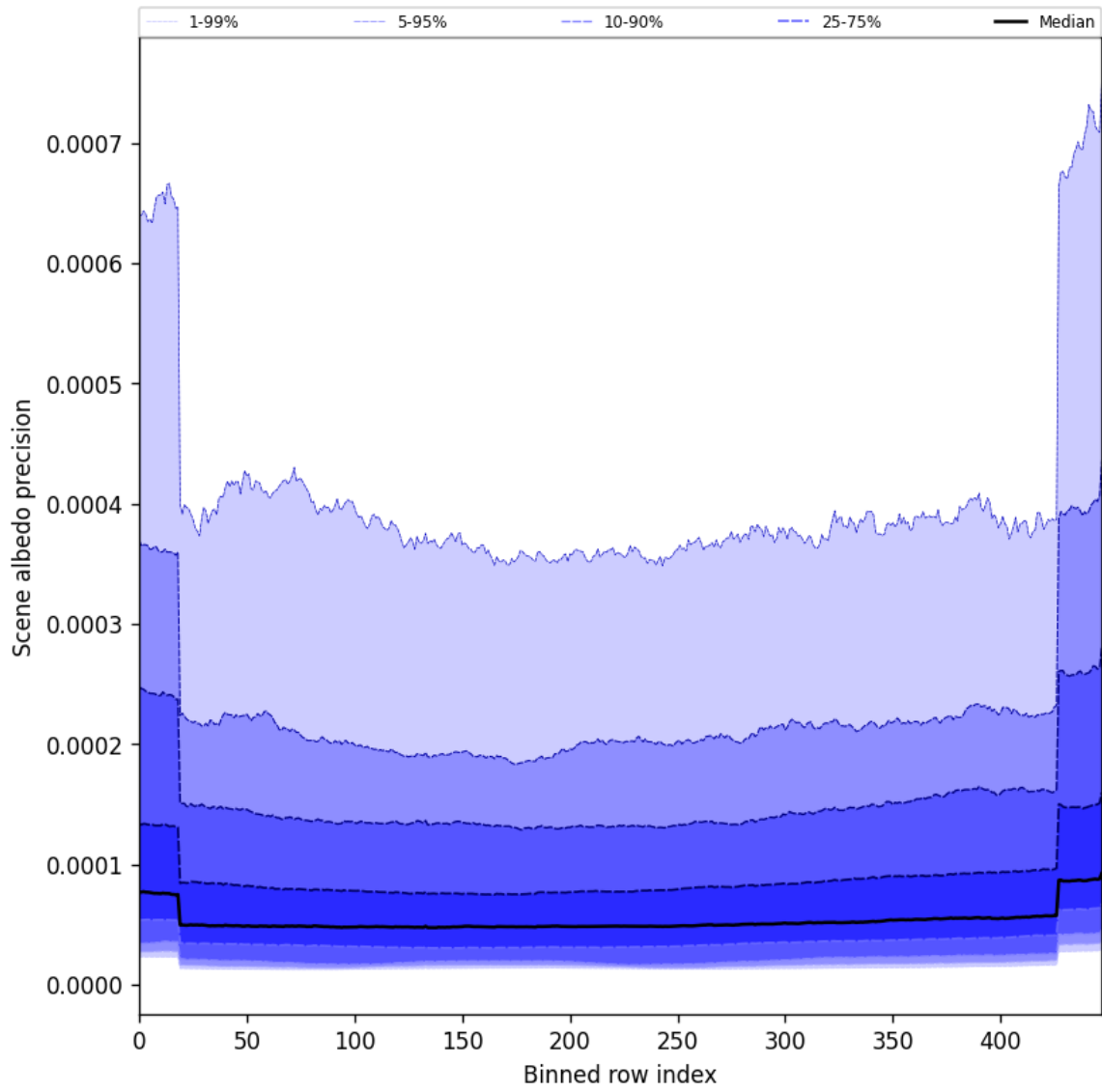
Figure 50: Along track statistics of “Scene albedo precision” for 2025-07-01 to 2025-07-02
