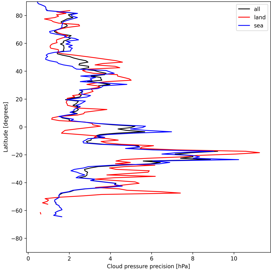
Figure 12: Zonal average of “Cloud pressure precision” for 2025-07-01 to 2025-07-02.
