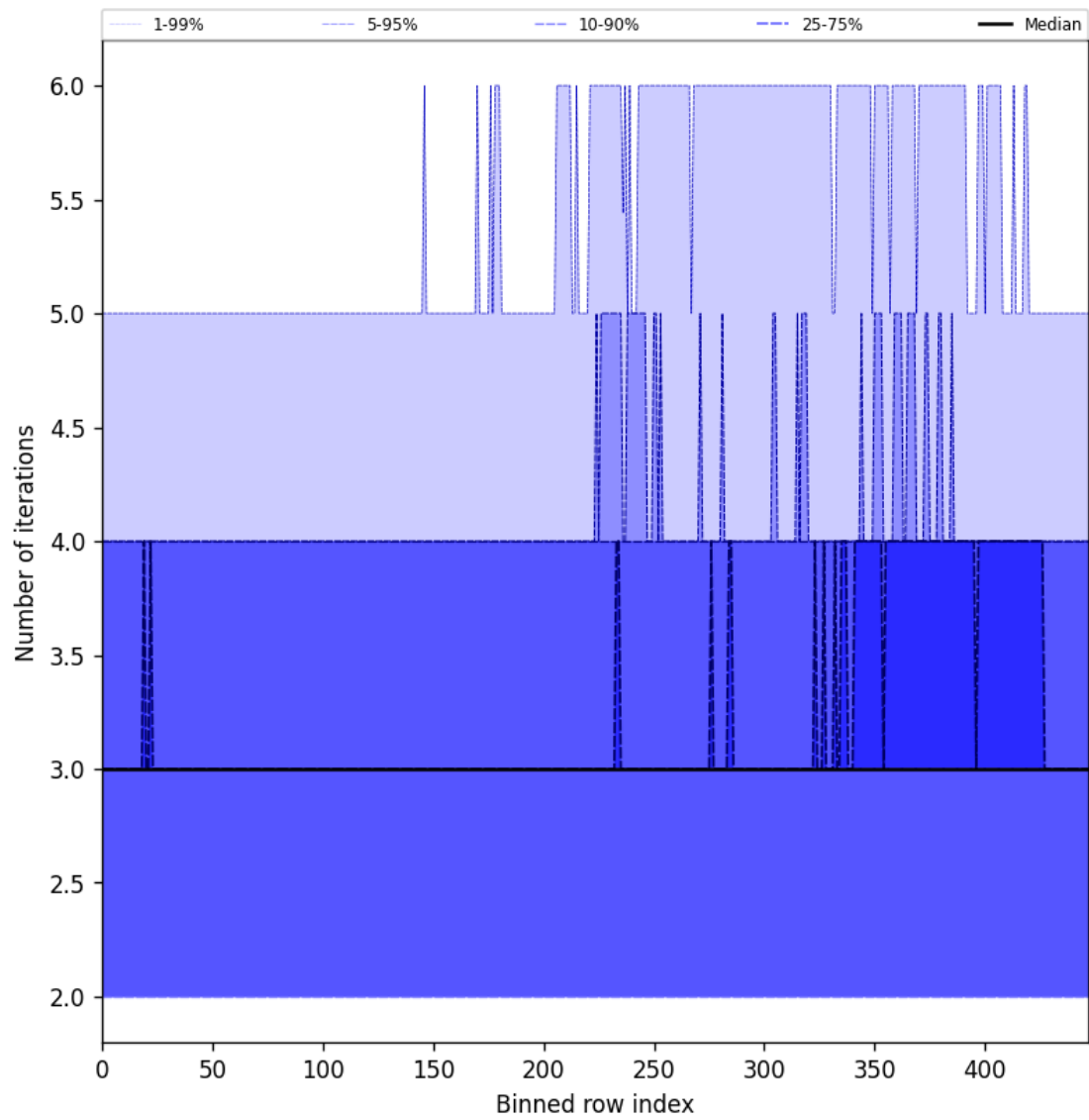
Figure 54: Along track statistics of “Number of iterations” for 2025-07-01 to 2025-07-02
