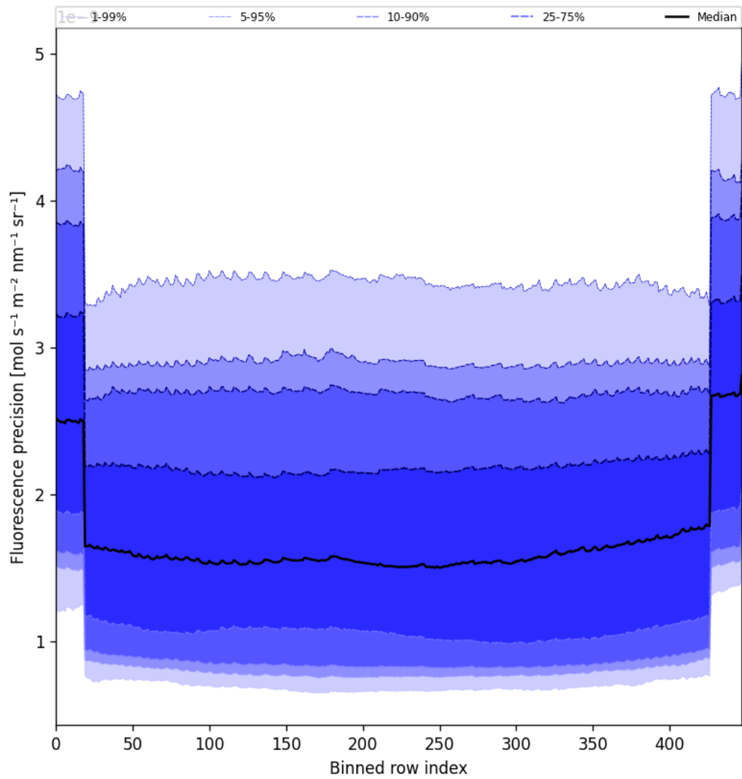
Figure 56: Along track statistics of “Fluorescence precision” for 2025-07-01 to 2025-07-02
