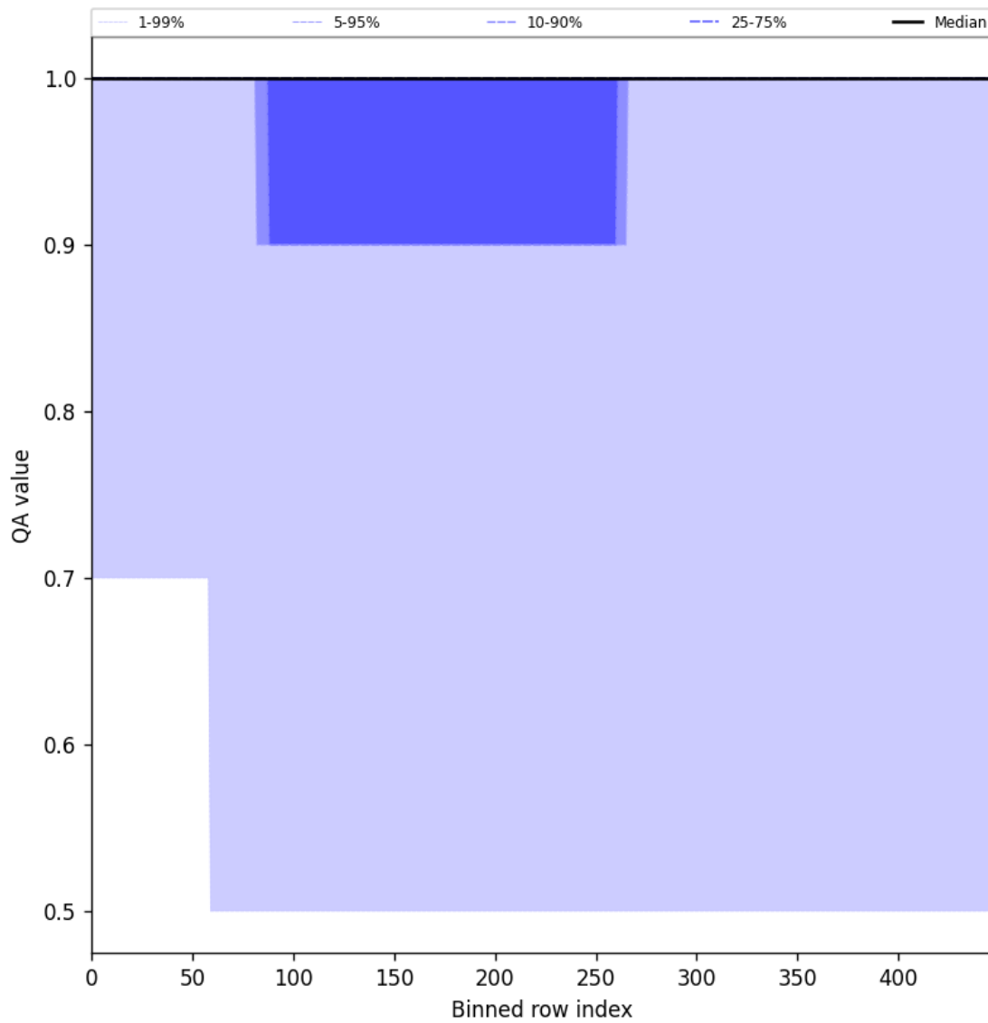
Figure 44: Along track statistics of “QA value” for 2025-07-01 to 2025-07-02
