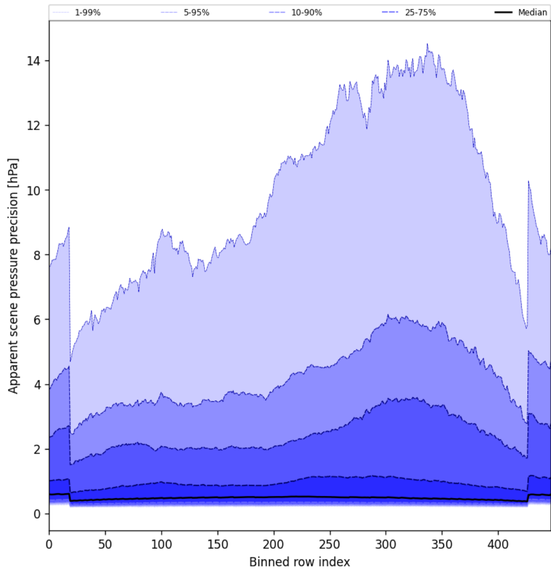
Figure 52: Along track statistics of “Apparent scene pressure precision” for 2025-07-01 to 2025-07-02
