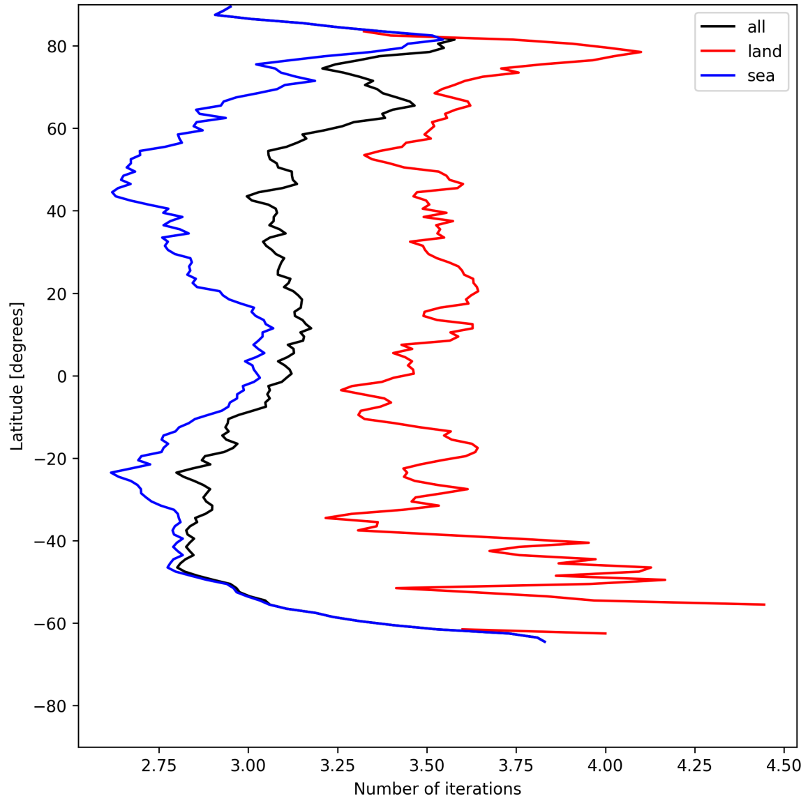
Figure 20: Zonal average of “Number of iterations” for 2025-07-01 to 2025-07-02.
