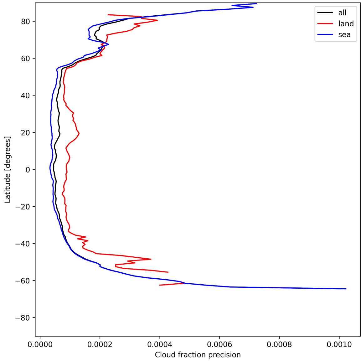
Figure 14: Zonal average of “Cloud fraction precision” for 2025-07-01 to 2025-07-02.
