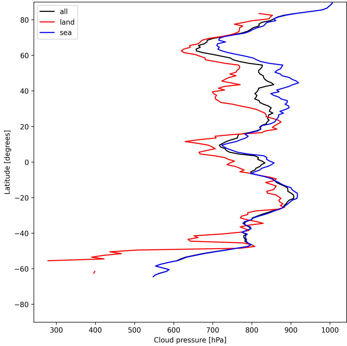
Figure 11: Zonal average of “Cloud pressure” for 2025-07-01 to 2025-07-02.
