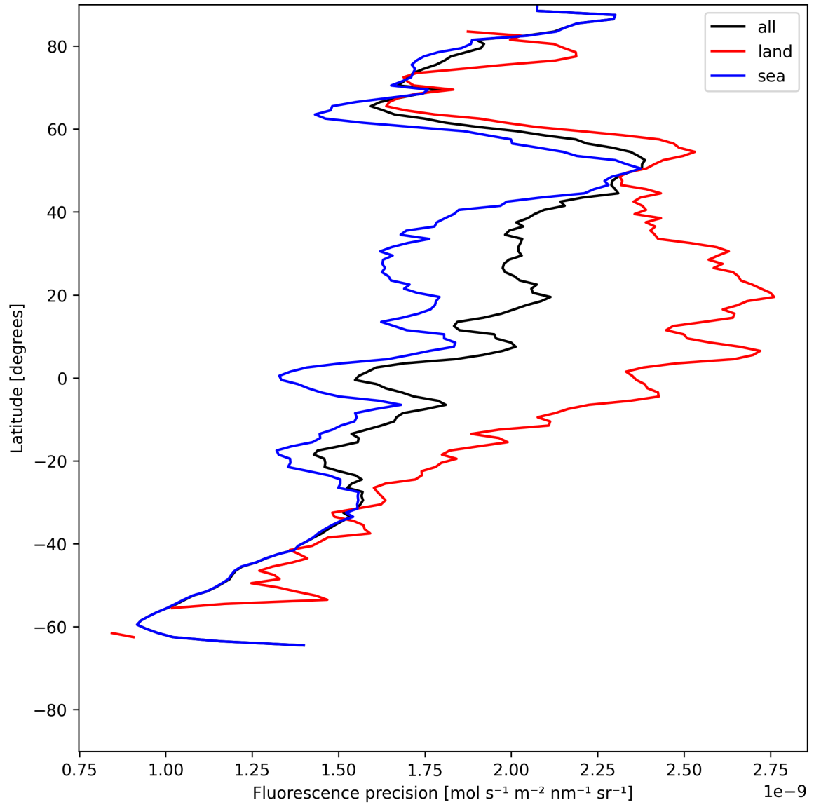
Figure 22: Zonal average of “Fluorescence precision” for 2025-07-01 to 2025-07-02.
