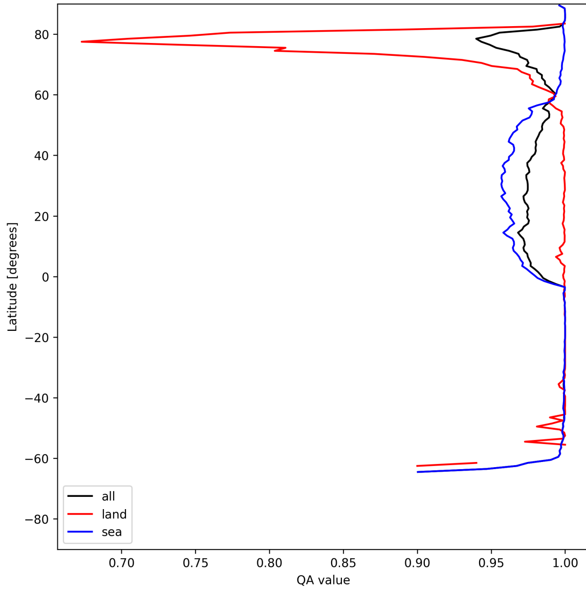
Figure 10: Zonal average of “QA value” for 2025-07-01 to 2025-07-02.
