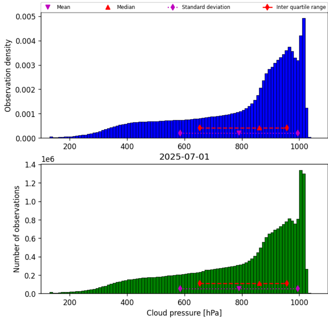
Figure 28: Histogram of “Cloud pressure” for 2025-07-01 to 2025-07-02
