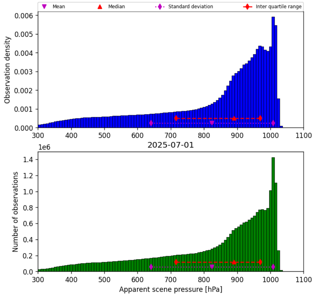
Figure 34: Histogram of “Apparent scene pressure” for 2025-07-01 to 2025-07-02
