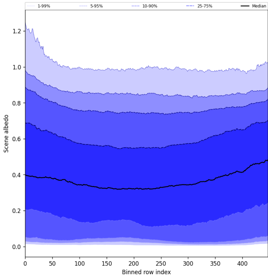
Figure 49: Along track statistics of “Scene albedo” for 2025-07-01 to 2025-07-02
