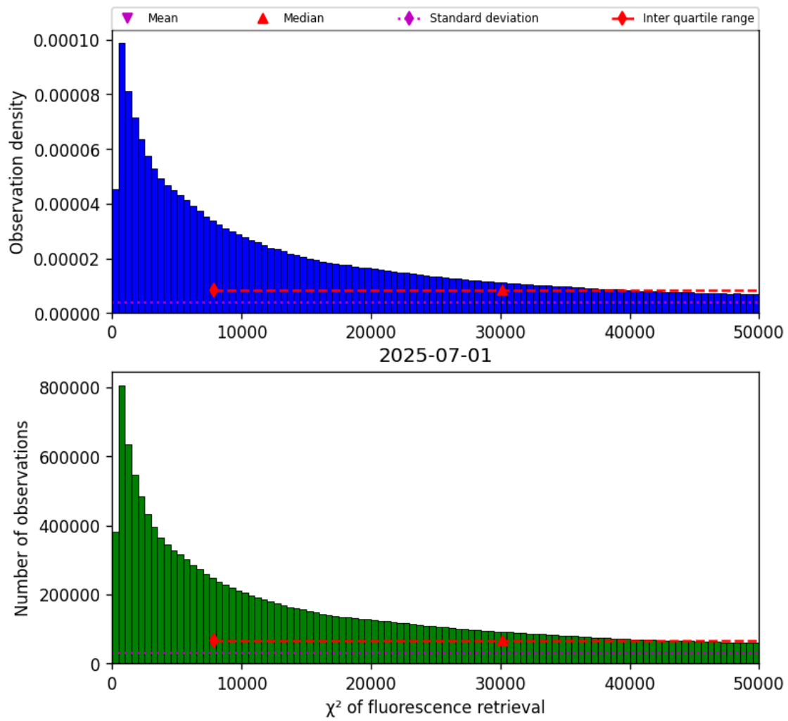
Figure 40: Histogram of “ \chi^2 of fluorescence retrieval” for 2025-07-01 to 2025-07-02
