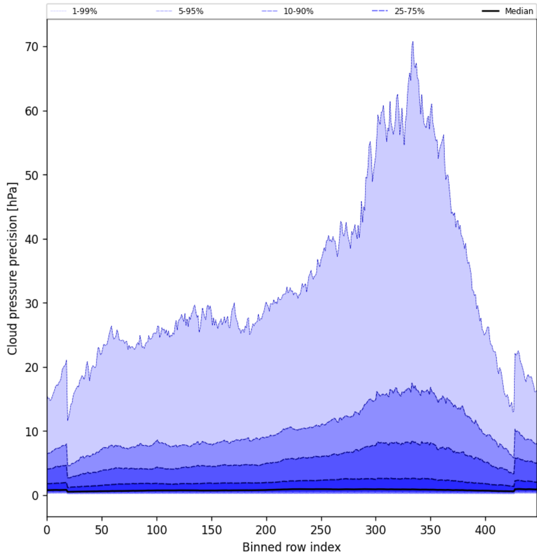
Figure 46: Along track statistics of “Cloud pressure precision” for 2025-07-01 to 2025-07-02
