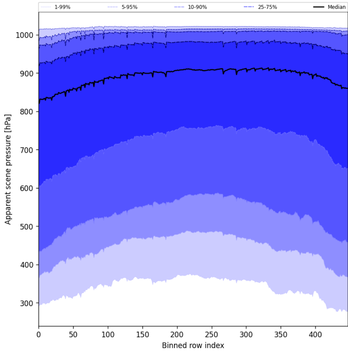
Figure 51: Along track statistics of “Apparent scene pressure” for 2025-07-01 to 2025-07-02
