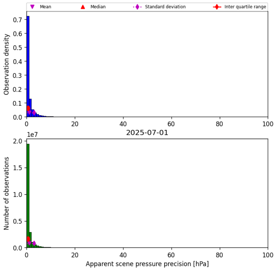
Figure 35: Histogram of “Apparent scene pressure precision” for 2025-07-01 to 2025-07-02
