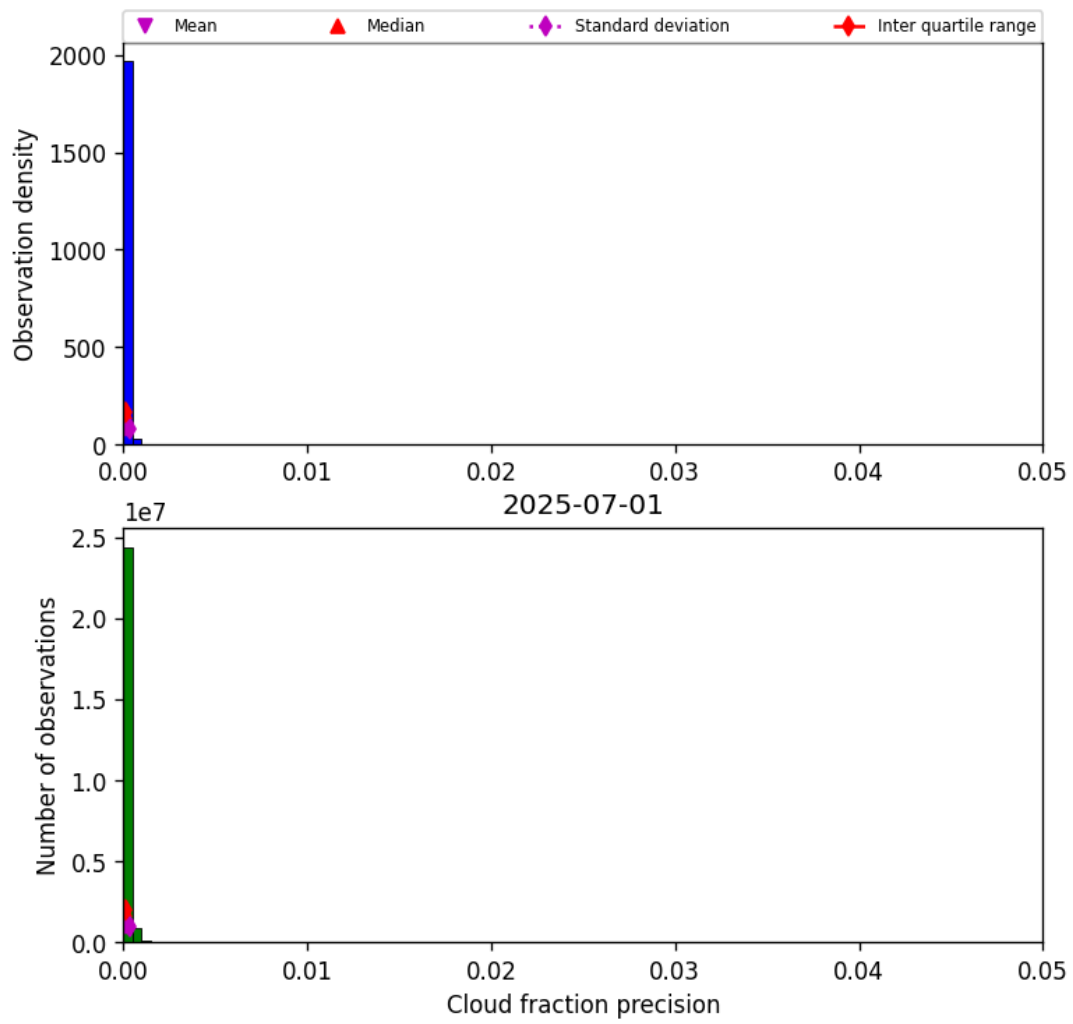
Figure 31: Histogram of “Cloud fraction precision” for 2025-07-01 to 2025-07-02
