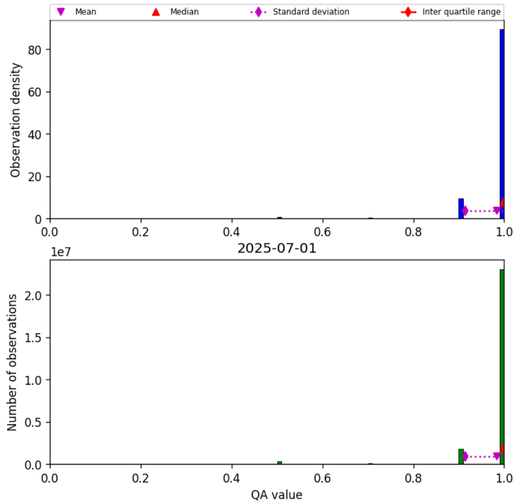
Figure 27: Histogram of “QA value” for 2025-07-01 to 2025-07-02
