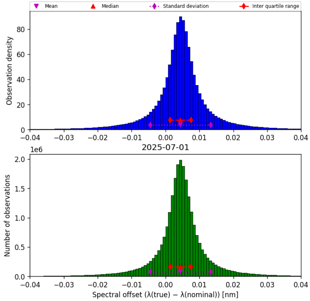
Figure 43: Histogram of “Spectral offset ( \lambda_{\text{true}} - \lambda_{\text{nominal}} )” for 2025-07-01 to 2025-07-02
