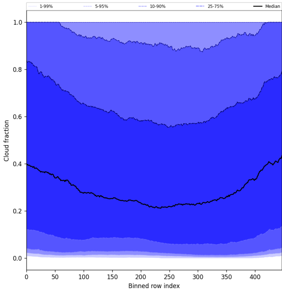
Figure 47: Along track statistics of “Cloud fraction” for 2025-07-01 to 2025-07-02
