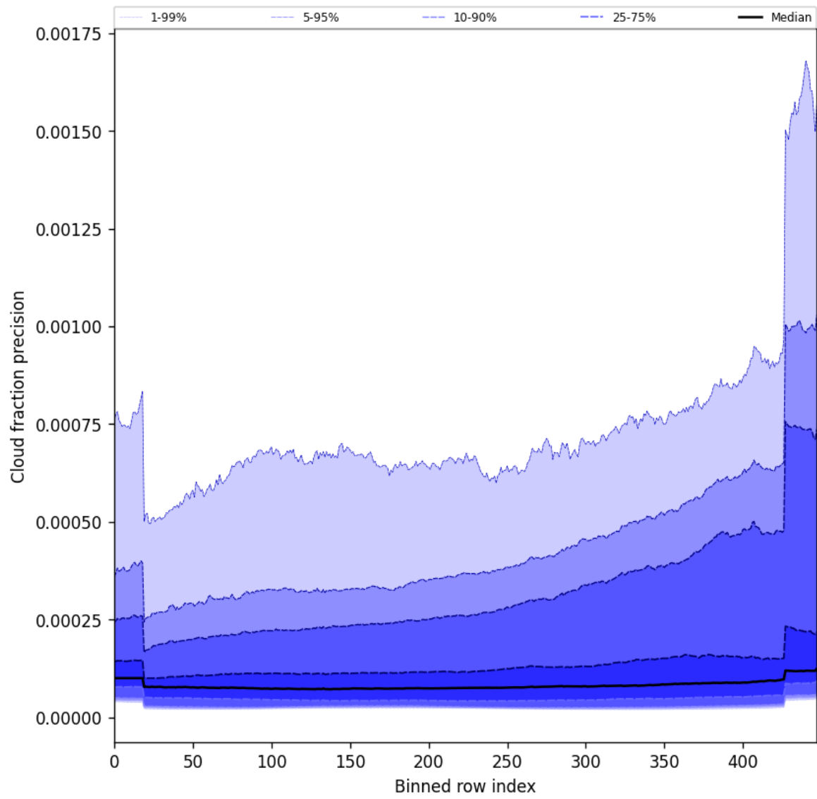
Figure 48: Along track statistics of “Cloud fraction precision” for 2025-07-01 to 2025-07-02
