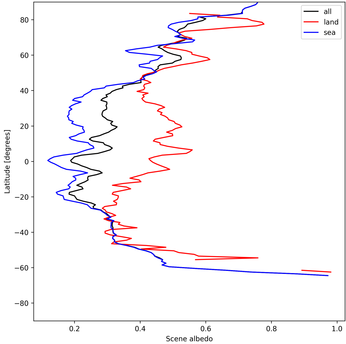
Figure 15: Zonal average of “Scene albedo” for 2025-07-01 to 2025-07-02.
