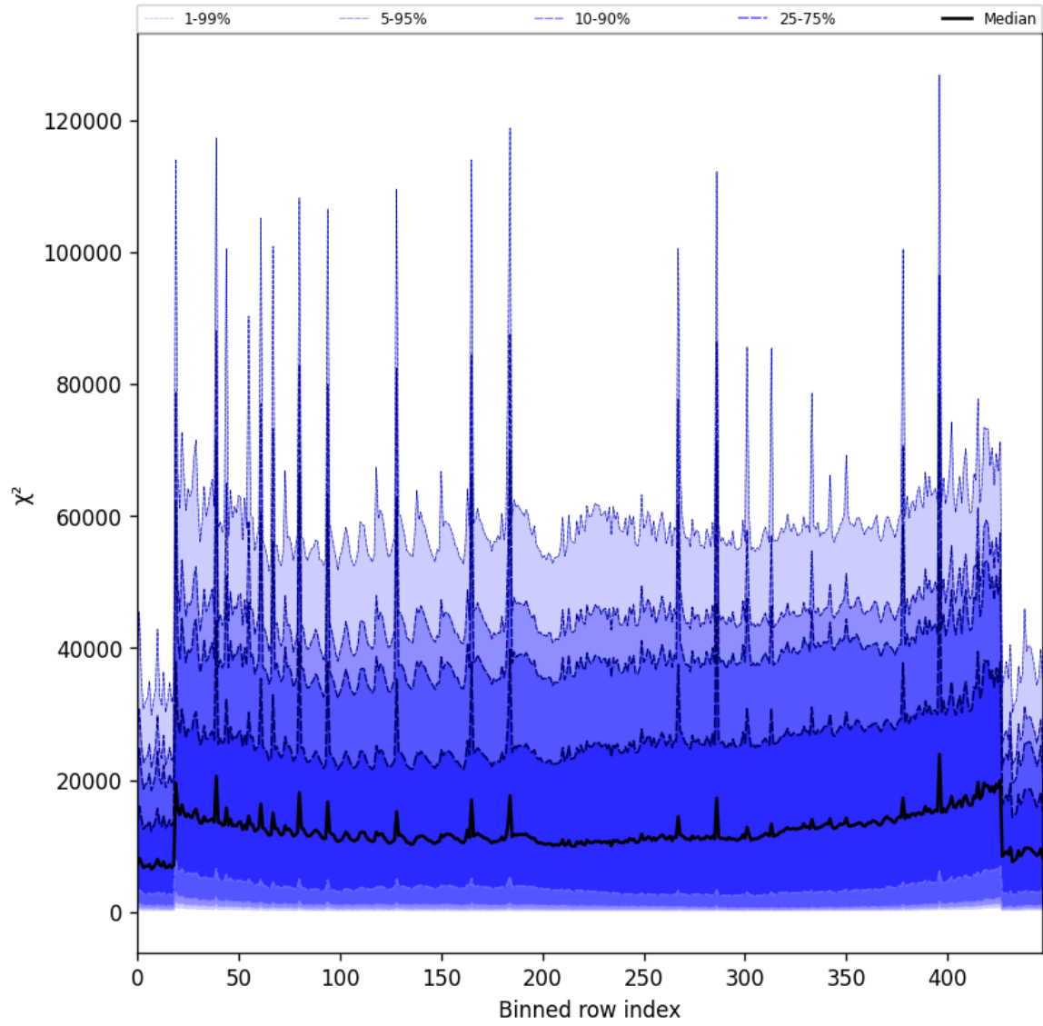
Figure 53: Along track statistics of “ \chi^2 ” for 2025-07-01 to 2025-07-02
