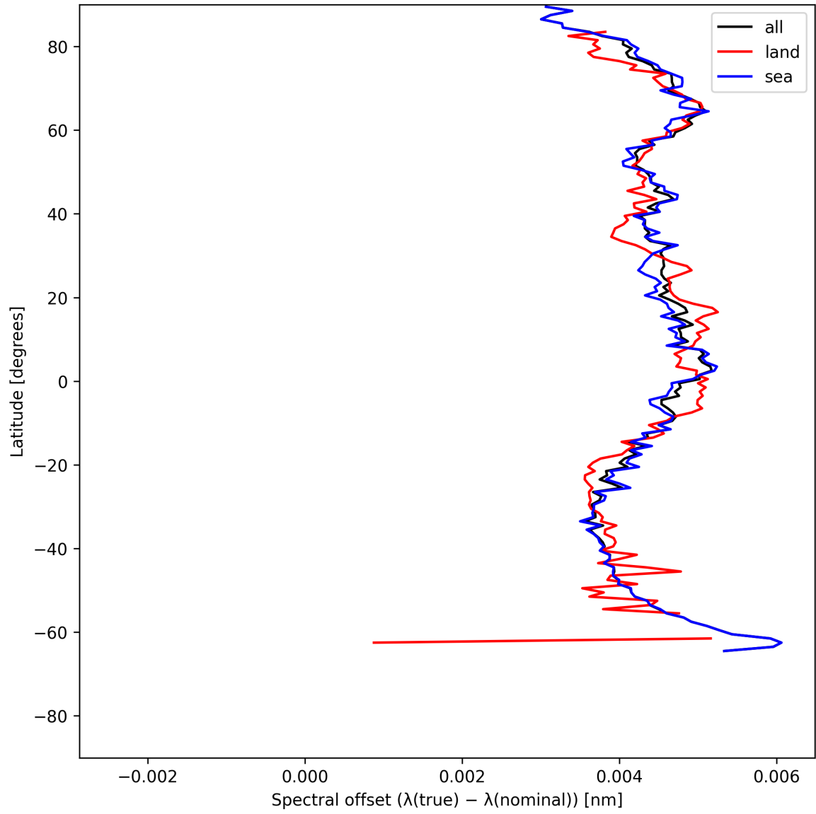
Figure 26: Zonal average of “Spectral offset ( \lambda_{\text{true}} - \lambda_{\text{nominal}} )” for 2025-07-01 to 2025-07-02.
