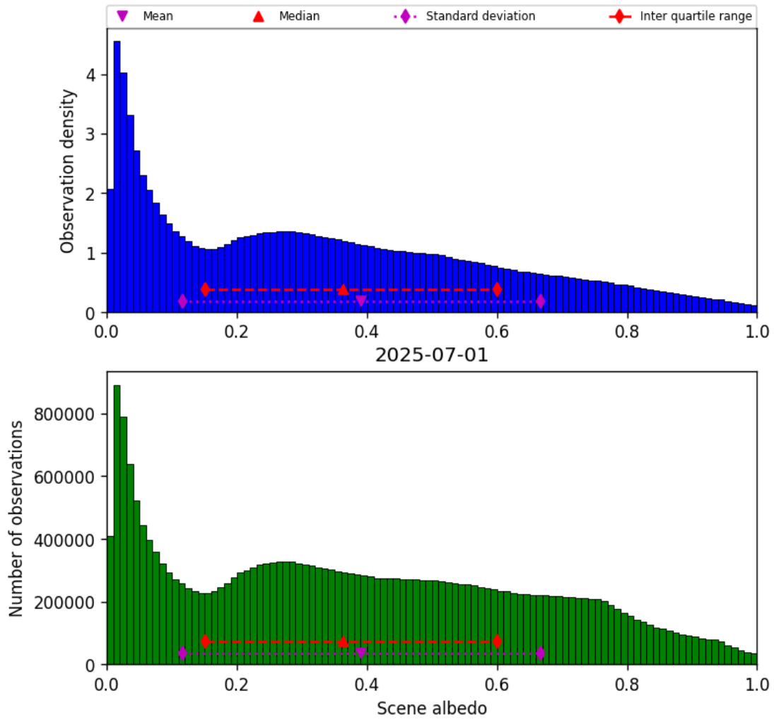
Figure 32: Histogram of “Scene albedo” for 2025-07-01 to 2025-07-02
