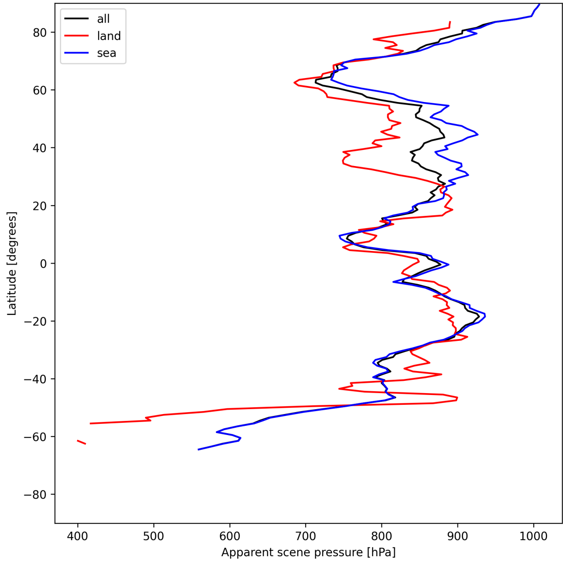
Figure 17: Zonal average of “Apparent scene pressure” for 2025-07-01 to 2025-07-02.
