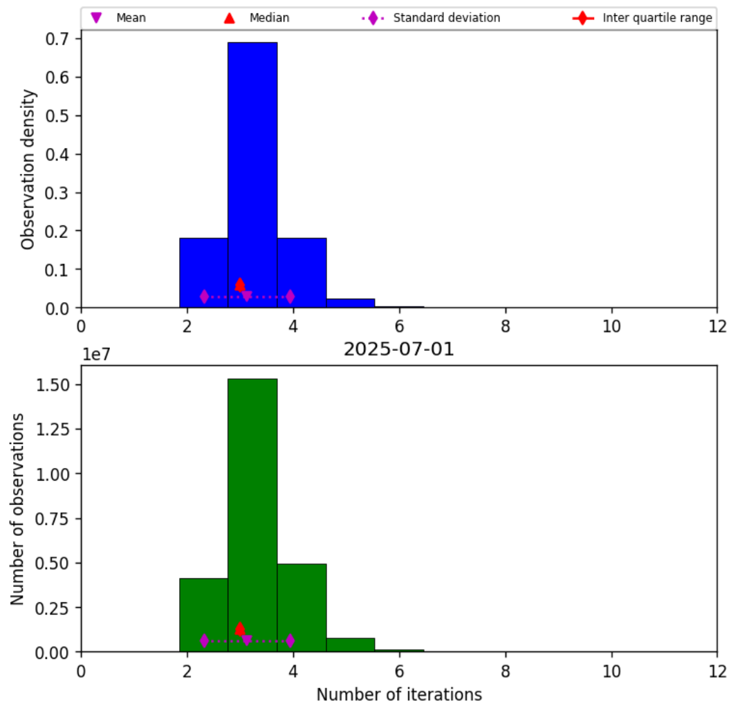
Figure 37: Histogram of “Number of iterations” for 2025-07-01 to 2025-07-02
