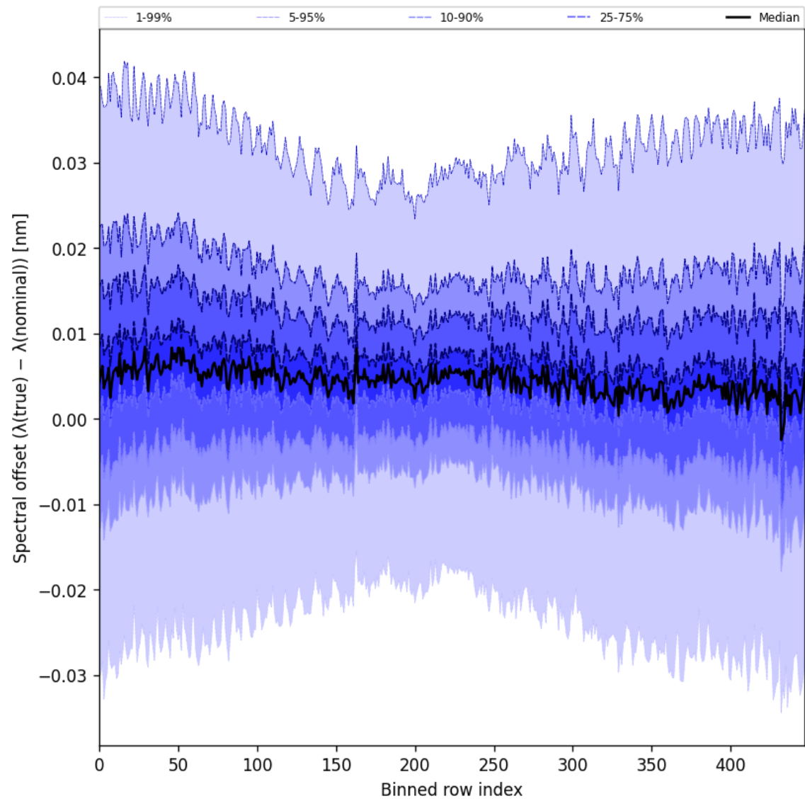
Figure 60: Along track statistics of “Spectral offset ( \lambda_{\text{true}} - \lambda_{\text{nominal}} )” for 2025-07-01 to 2025-07-02
