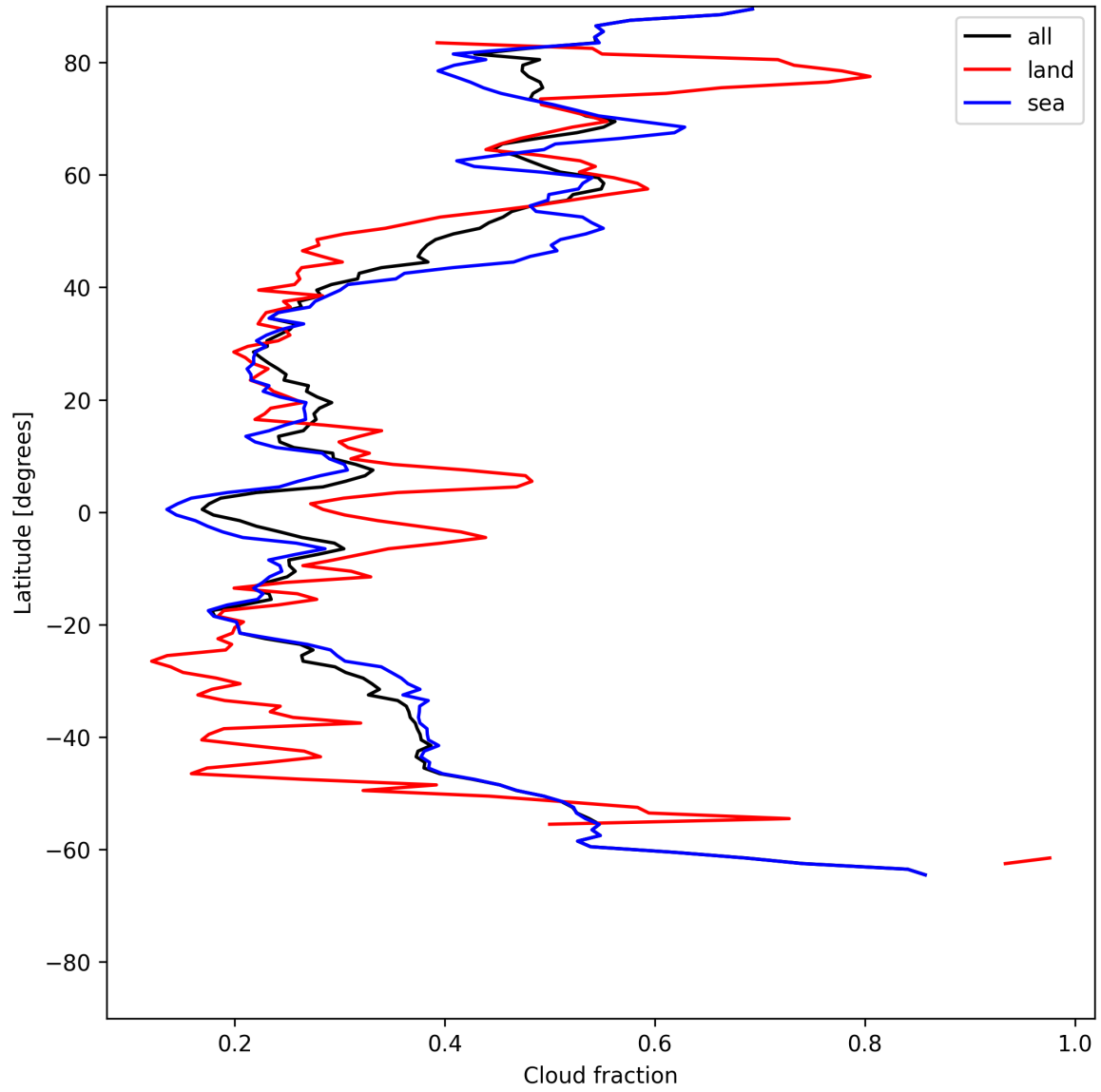
Figure 13: Zonal average of “Cloud fraction” for 2025-07-01 to 2025-07-02.
