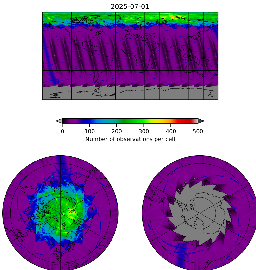
Figure 9: Map of the number of observations for 2025-07-01 to 2025-07-02
