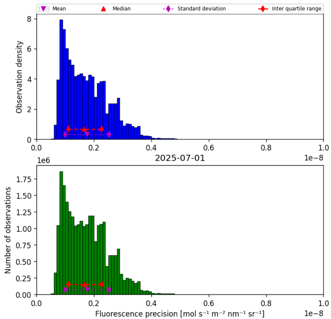
Figure 39: Histogram of “Fluorescence precision” for 2025-07-01 to 2025-07-02
