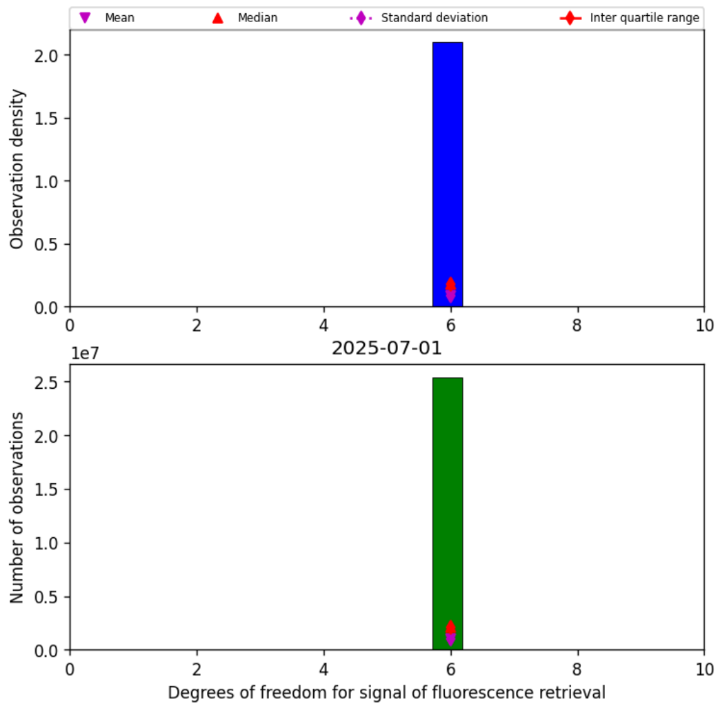
Figure 41: Histogram of “Degrees of freedom for signal of fluorescence retrieval” for 2025-07-01 to 2025-07-02
