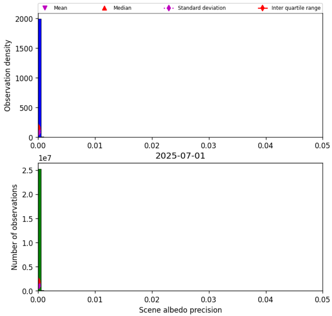
Figure 33: Histogram of “Scene albedo precision” for 2025-07-01 to 2025-07-02
