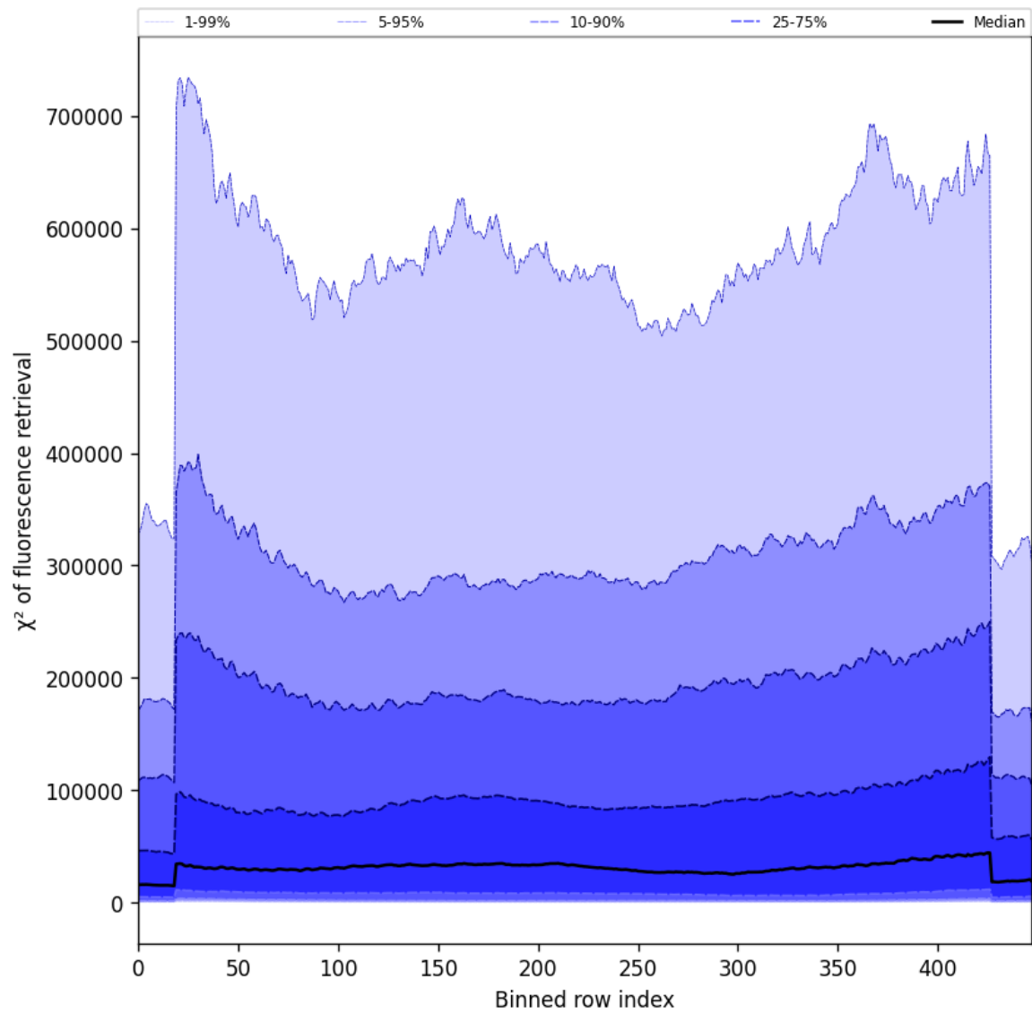
Figure 57: Along track statistics of “ \chi^2 of fluorescence retrieval” for 2025-07-01 to 2025-07-02
