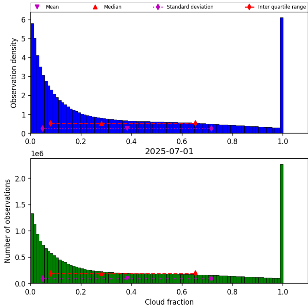
Figure 30: Histogram of “Cloud fraction” for 2025-07-01 to 2025-07-02
