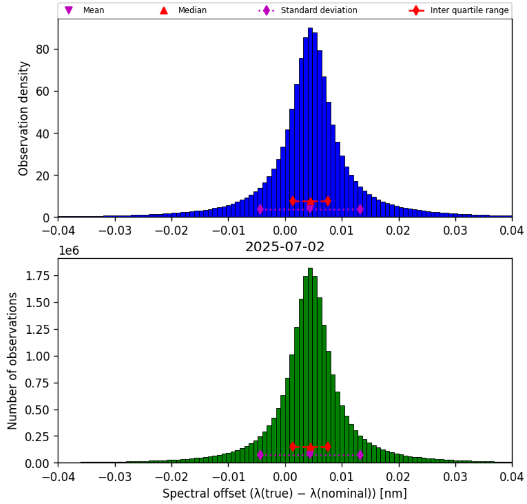
Figure 43: Histogram of “Spectral offset ( \lambda_{\text{true}} - \lambda_{\text{nominal}} )” for 2025-07-02 to 2025-07-03
