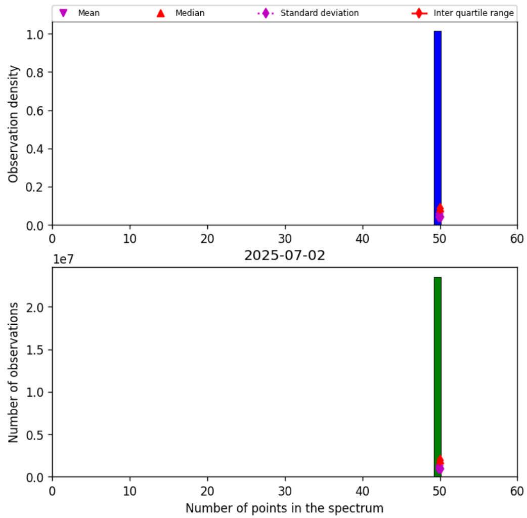
Figure 42: Histogram of “Number of points in the spectrum” for 2025-07-02 to 2025-07-03
