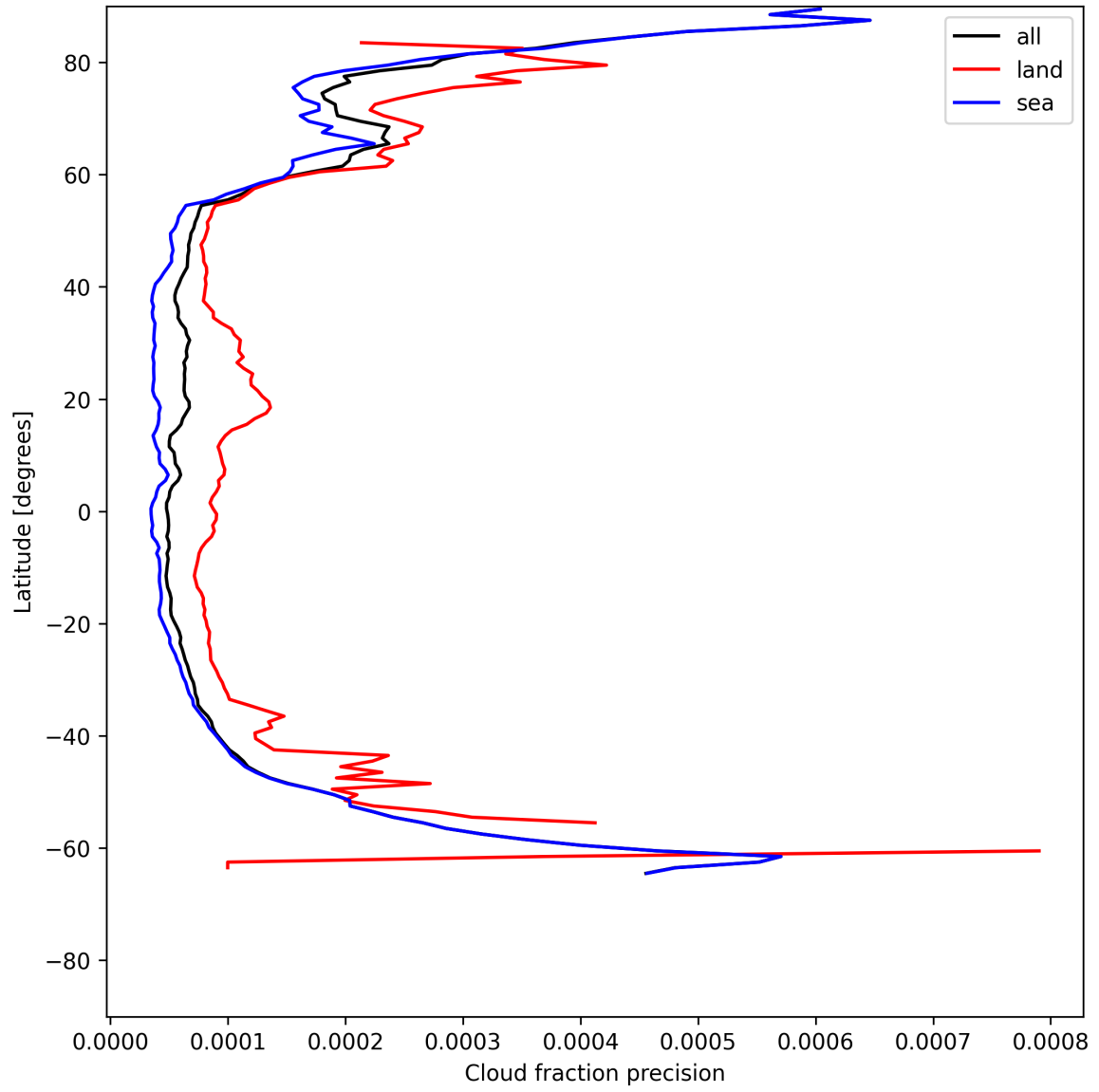
Figure 14: Zonal average of “Cloud fraction precision” for 2025-07-02 to 2025-07-03.
