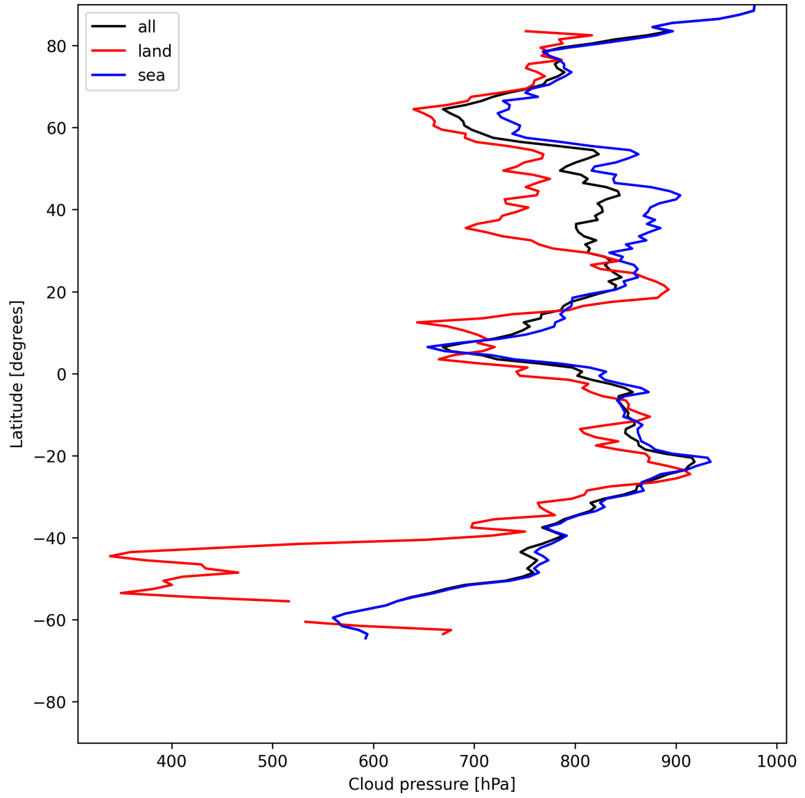
Figure 11: Zonal average of “Cloud pressure” for 2025-07-02 to 2025-07-03.
