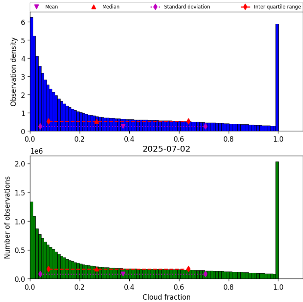
Figure 30: Histogram of “Cloud fraction” for 2025-07-02 to 2025-07-03
