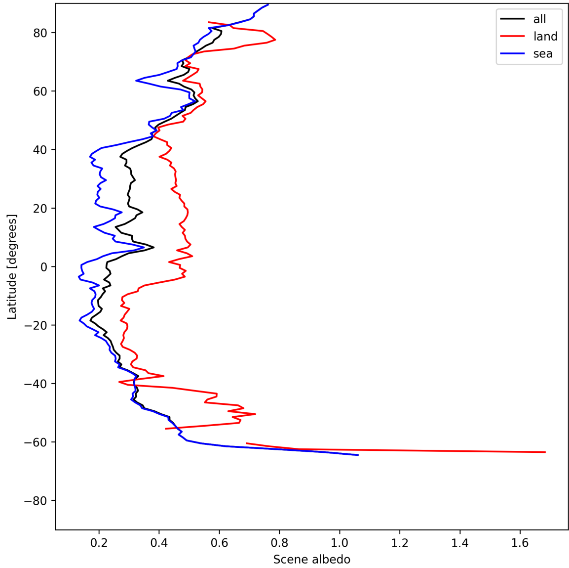
Figure 15: Zonal average of “Scene albedo” for 2025-07-02 to 2025-07-03.
