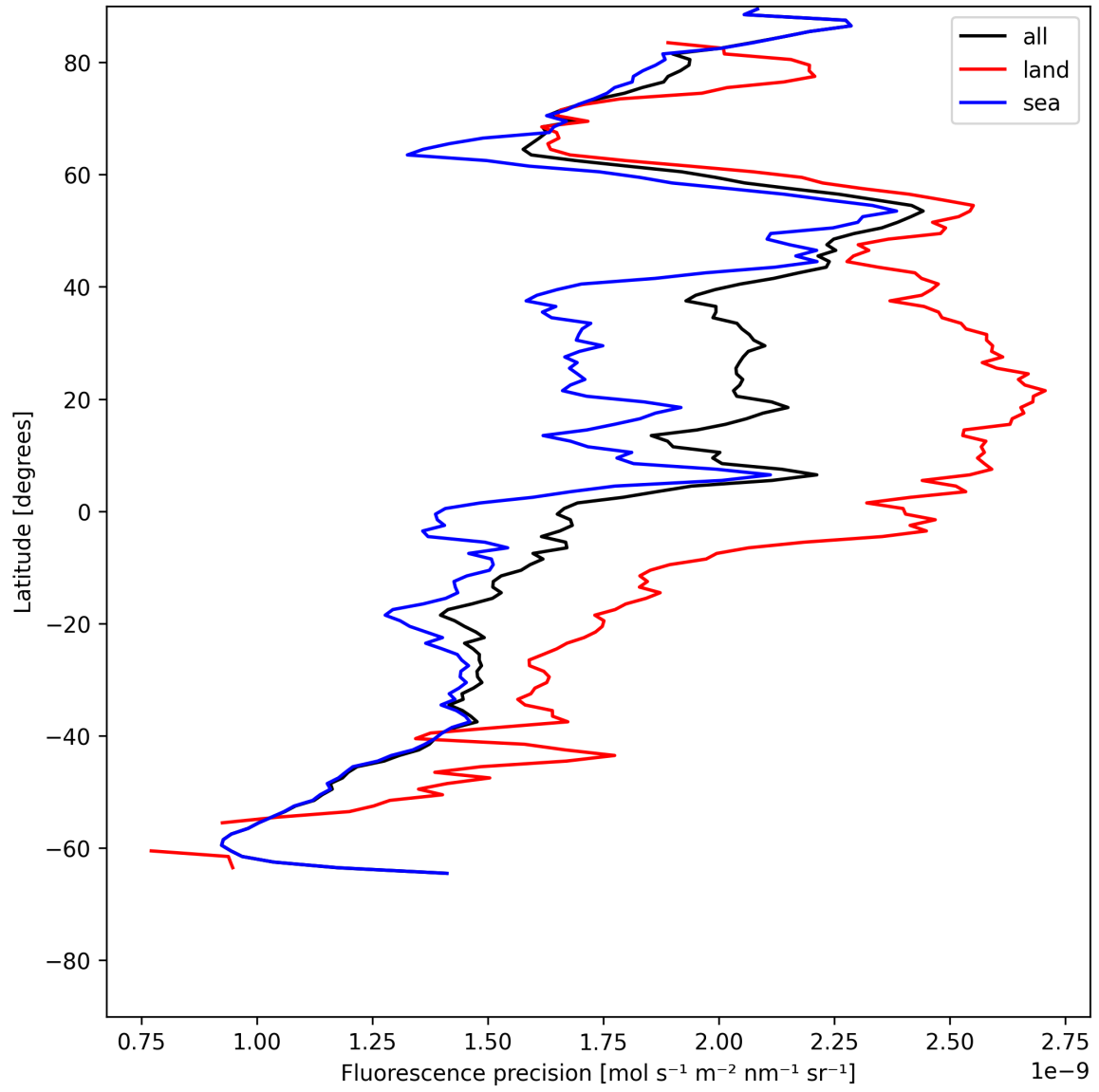
Figure 22: Zonal average of “Fluorescence precision” for 2025-07-02 to 2025-07-03.
