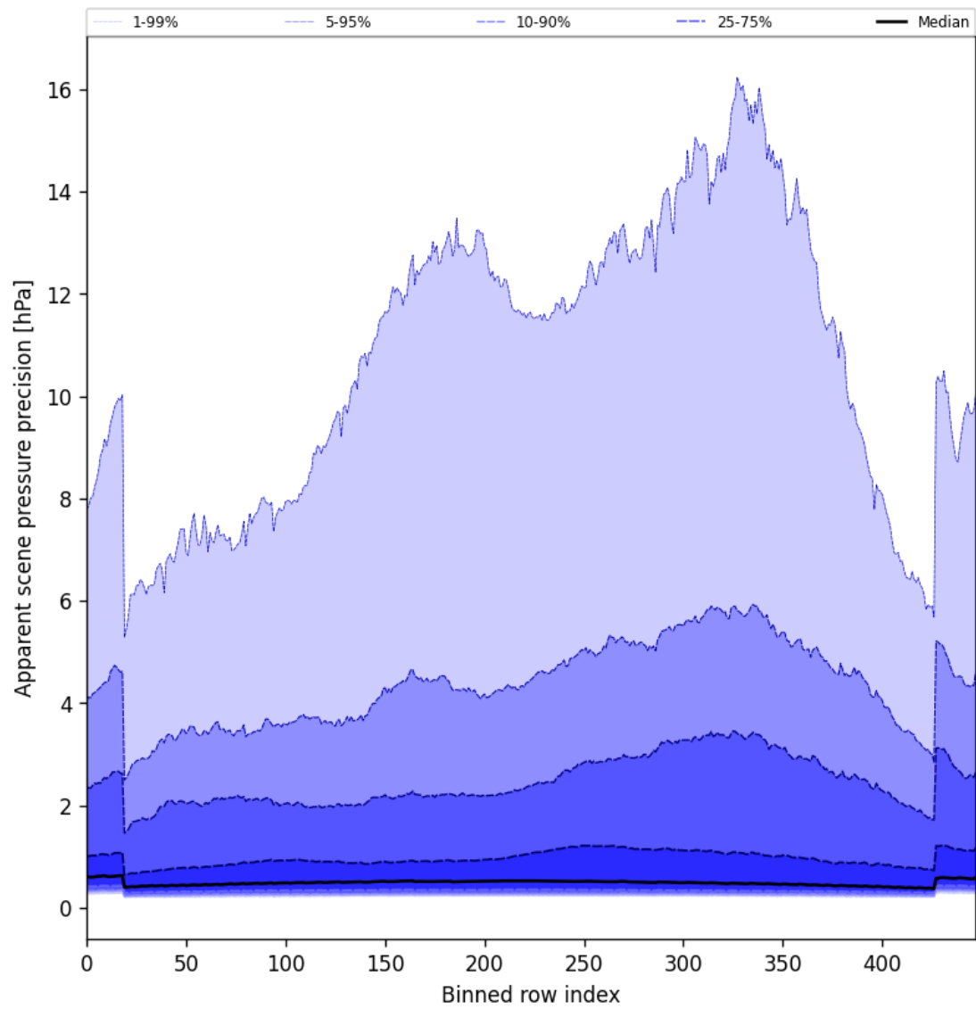
Figure 52: Along track statistics of “Apparent scene pressure precision” for 2025-07-02 to 2025-07-03
