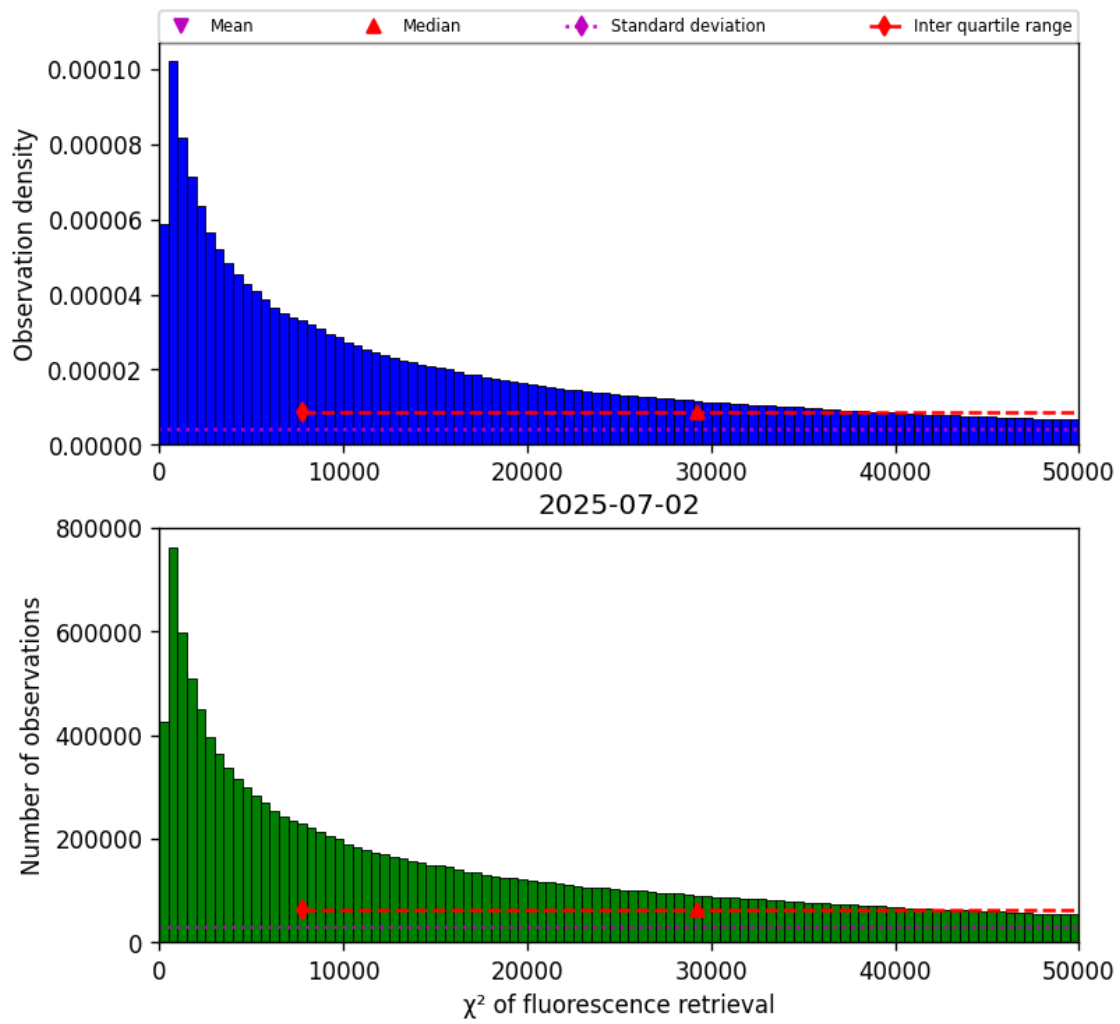
Figure 40: Histogram of “ \chi^2 of fluorescence retrieval” for 2025-07-02 to 2025-07-03
