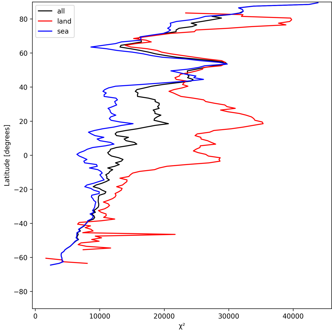
Figure 19: Zonal average of “ \chi^2 ” for 2025-07-02 to 2025-07-03.
