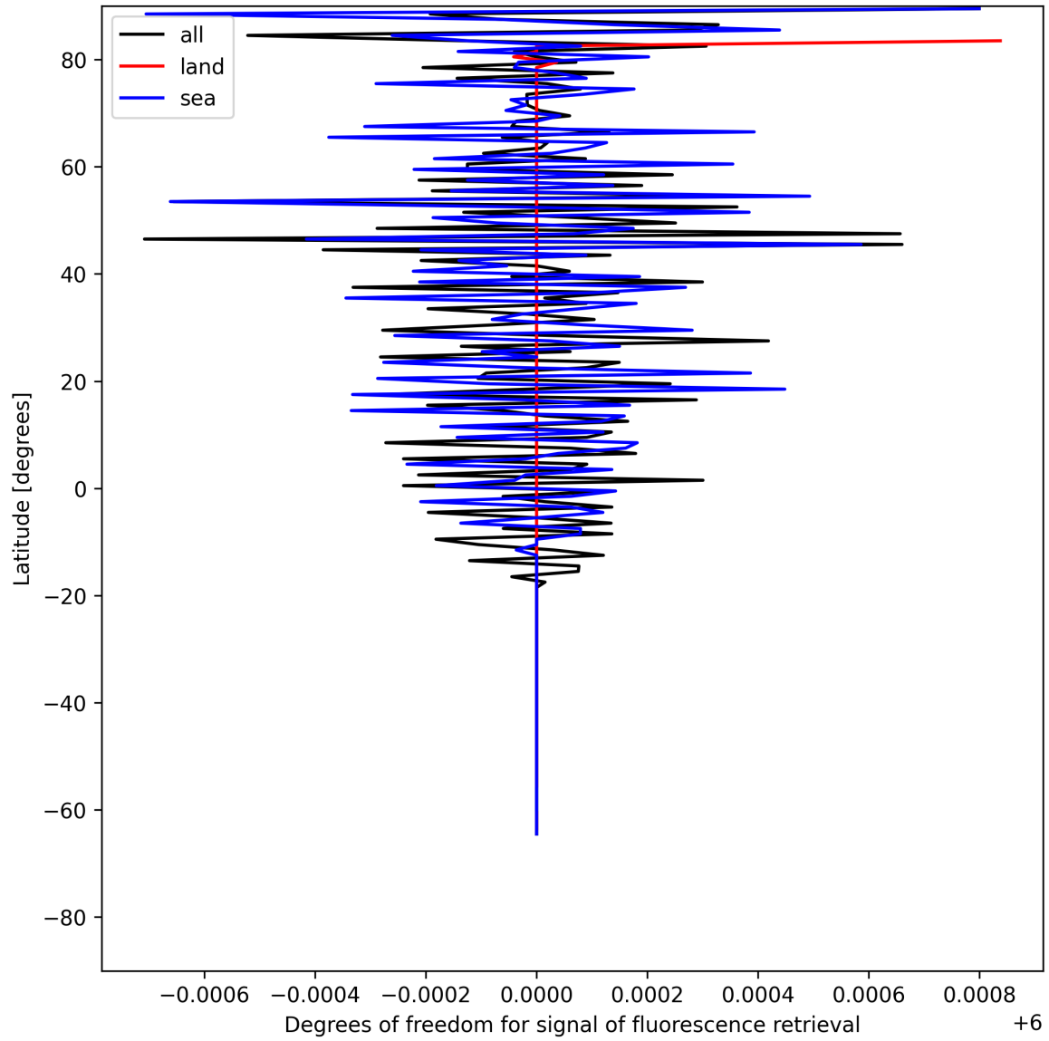
Figure 24: Zonal average of “Degrees of freedom for signal of fluorescence retrieval” for 2025-07-02 to 2025-07-03.
