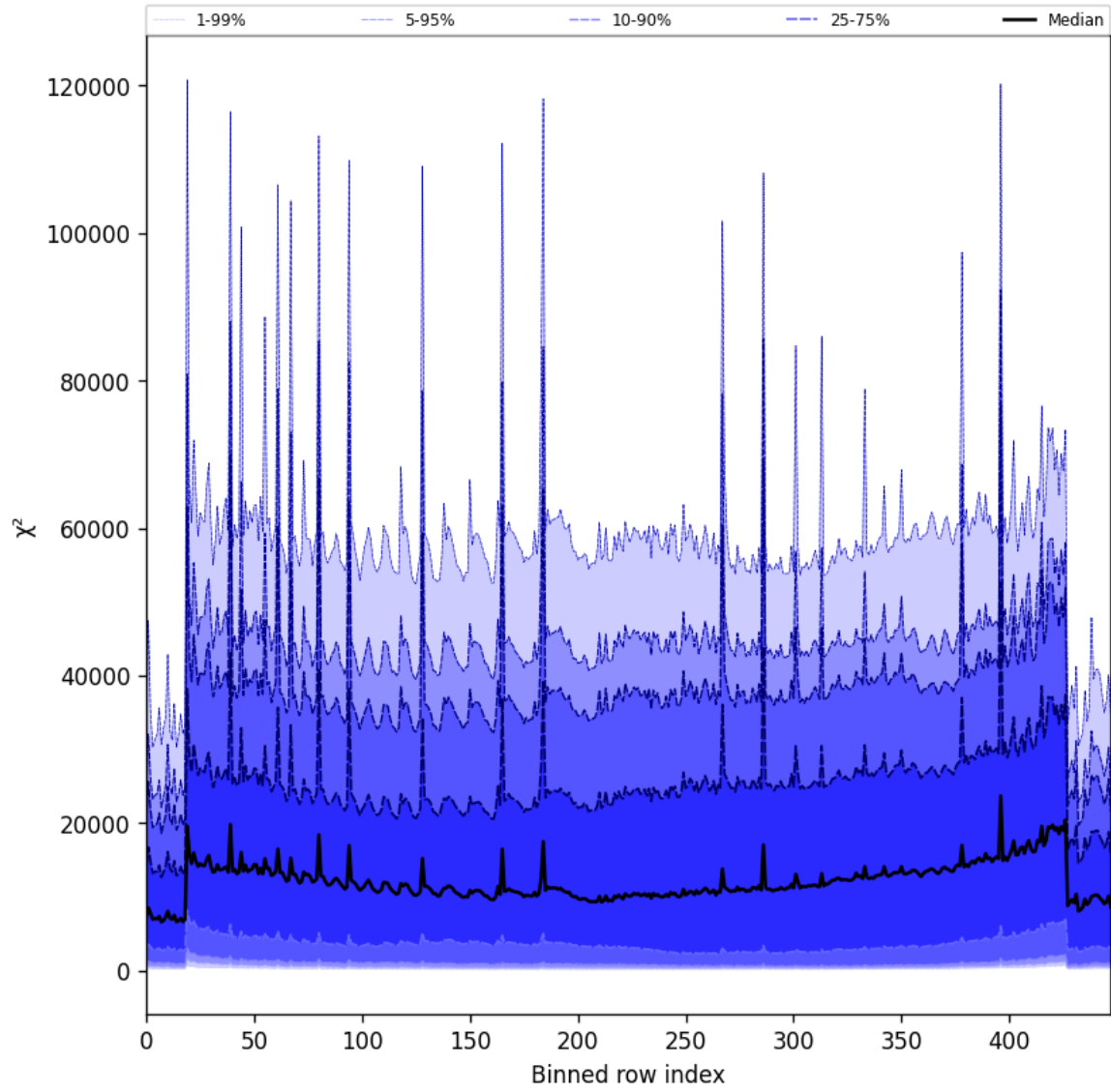
Figure 53: Along track statistics of “ \chi^2 ” for 2025-07-02 to 2025-07-03
