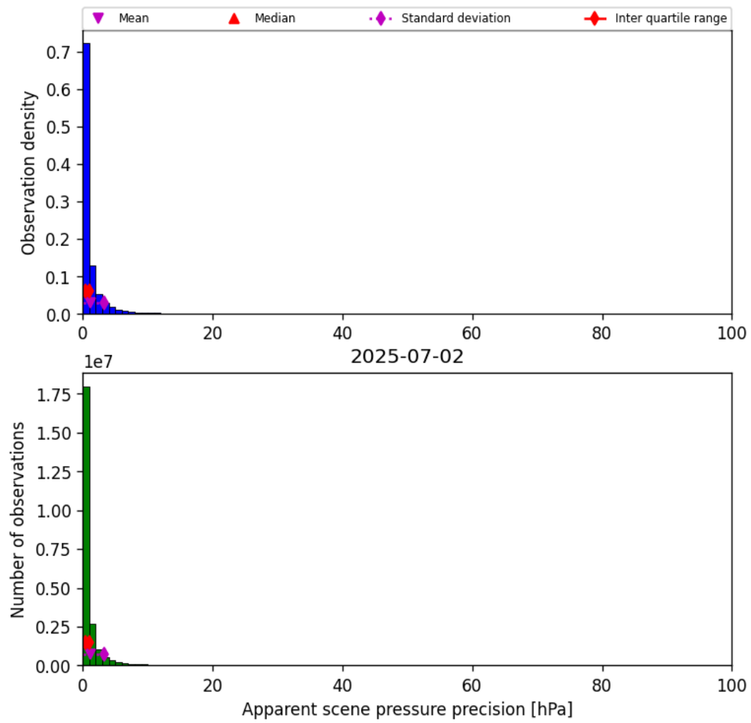
Figure 35: Histogram of “Apparent scene pressure precision” for 2025-07-02 to 2025-07-03
