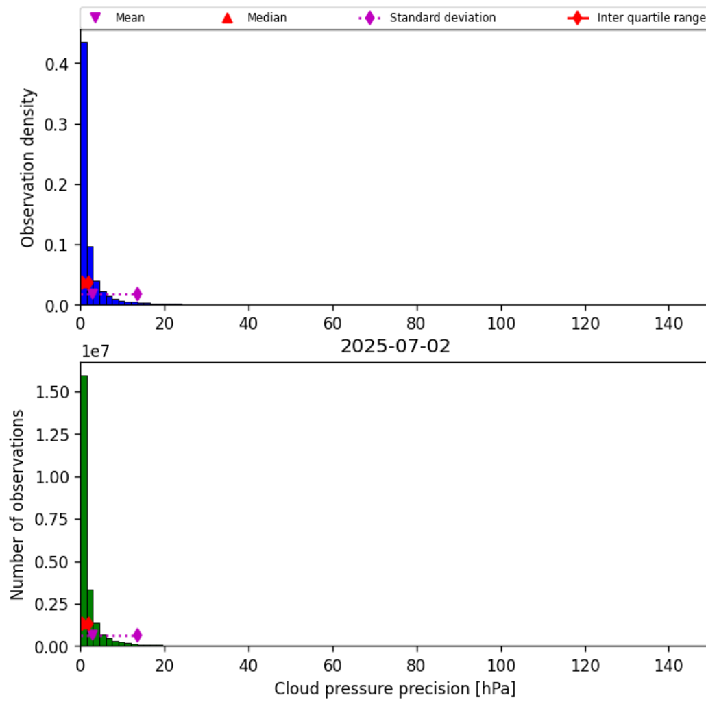
Figure 29: Histogram of “Cloud pressure precision” for 2025-07-02 to 2025-07-03
