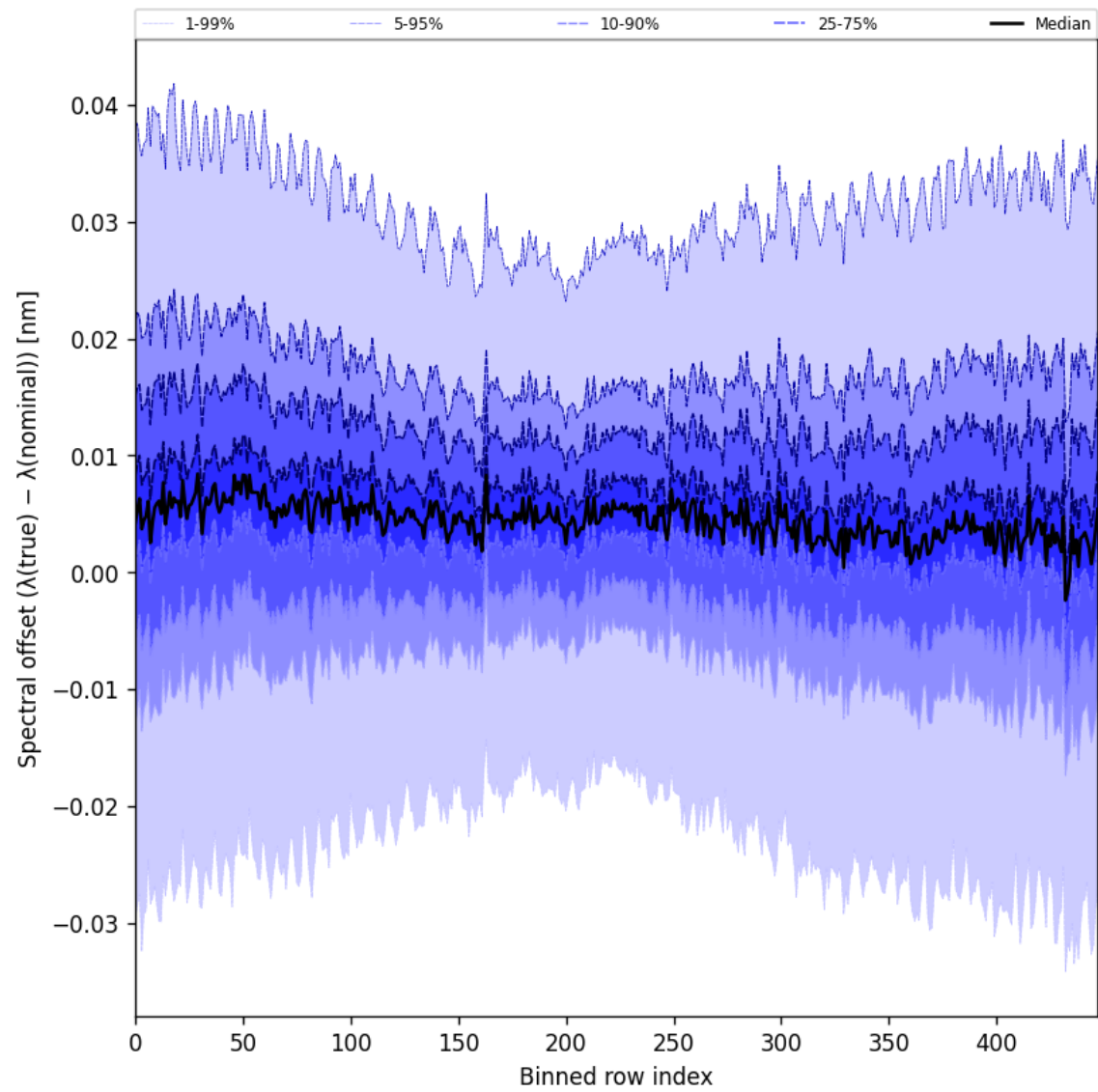
Figure 60: Along track statistics of “Spectral offset ( \lambda_{\text{true}} - \lambda_{\text{nominal}} )” for 2025-07-02 to 2025-07-03
