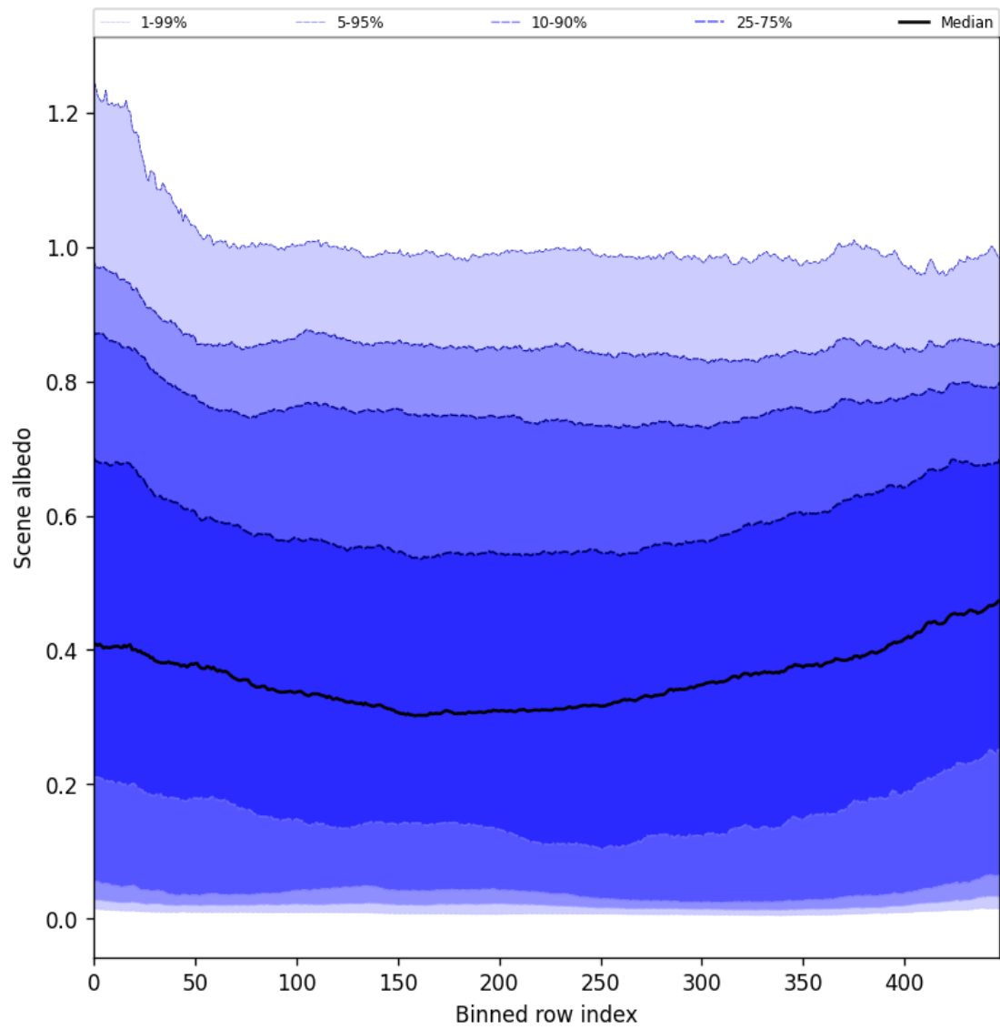
Figure 49: Along track statistics of “Scene albedo” for 2025-07-02 to 2025-07-03
