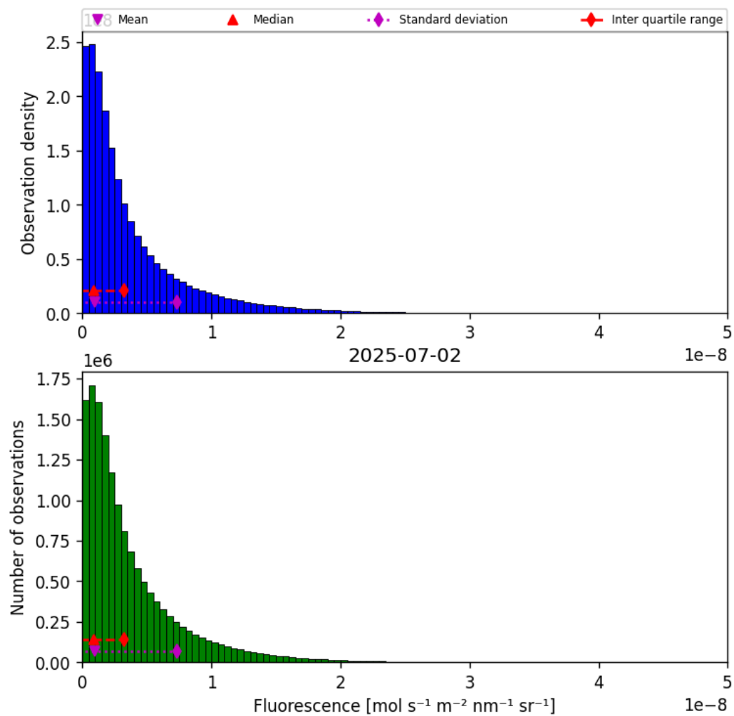
Figure 38: Histogram of “Fluorescence” for 2025-07-02 to 2025-07-03
