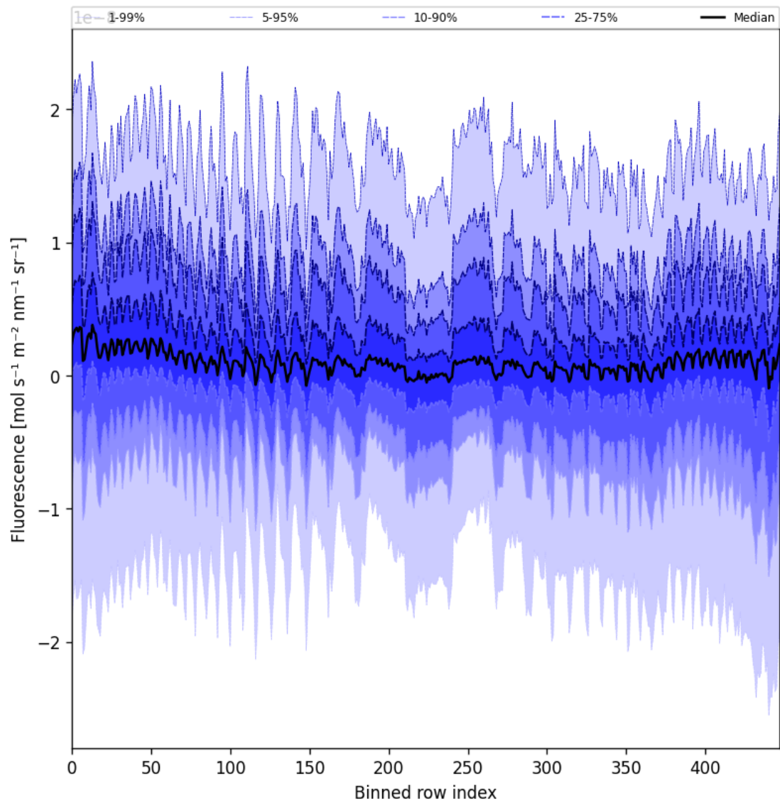
Figure 55: Along track statistics of “Fluorescence” for 2025-07-02 to 2025-07-03
