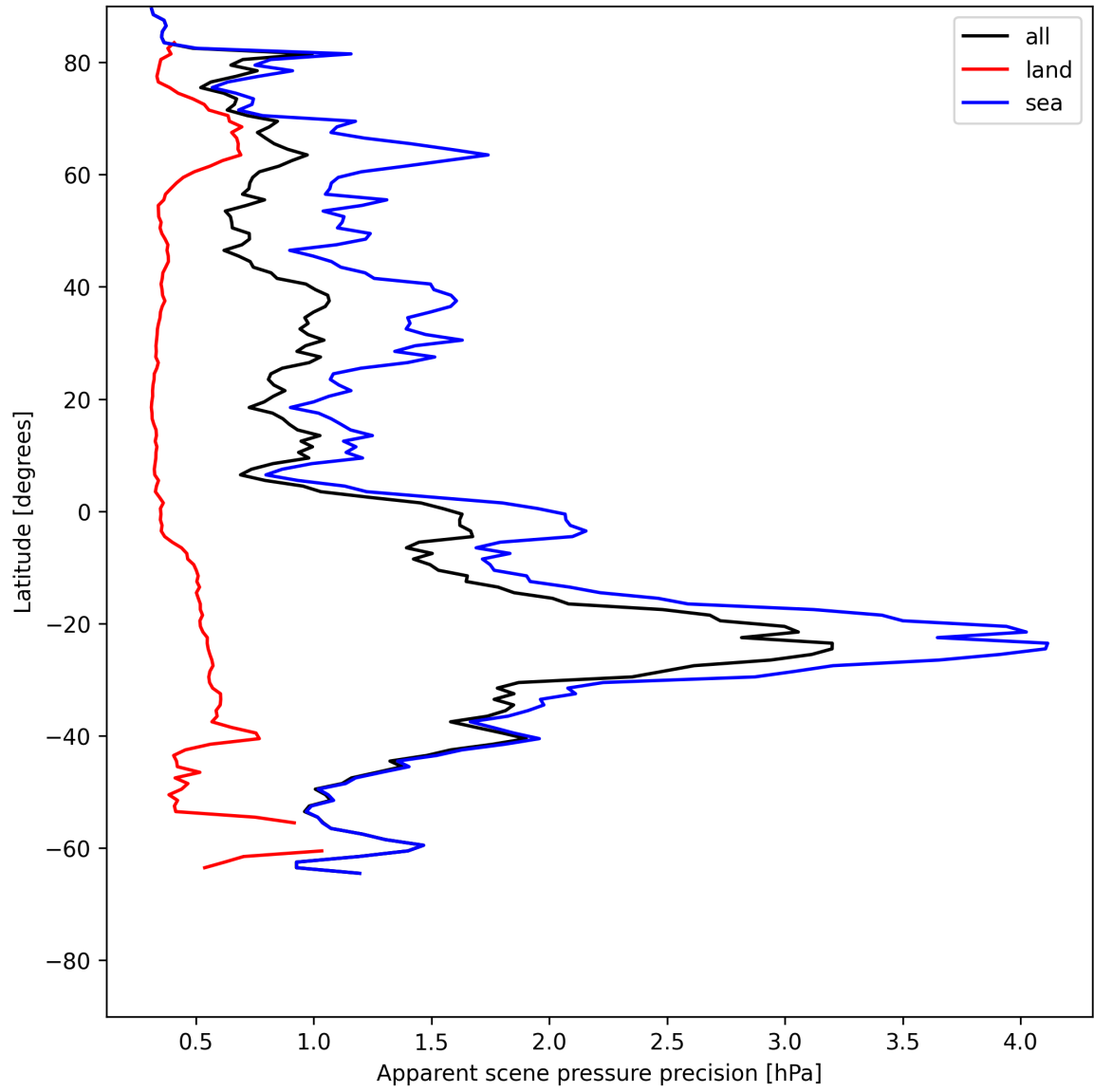
Figure 18: Zonal average of “Apparent scene pressure precision” for 2025-07-02 to 2025-07-03.
