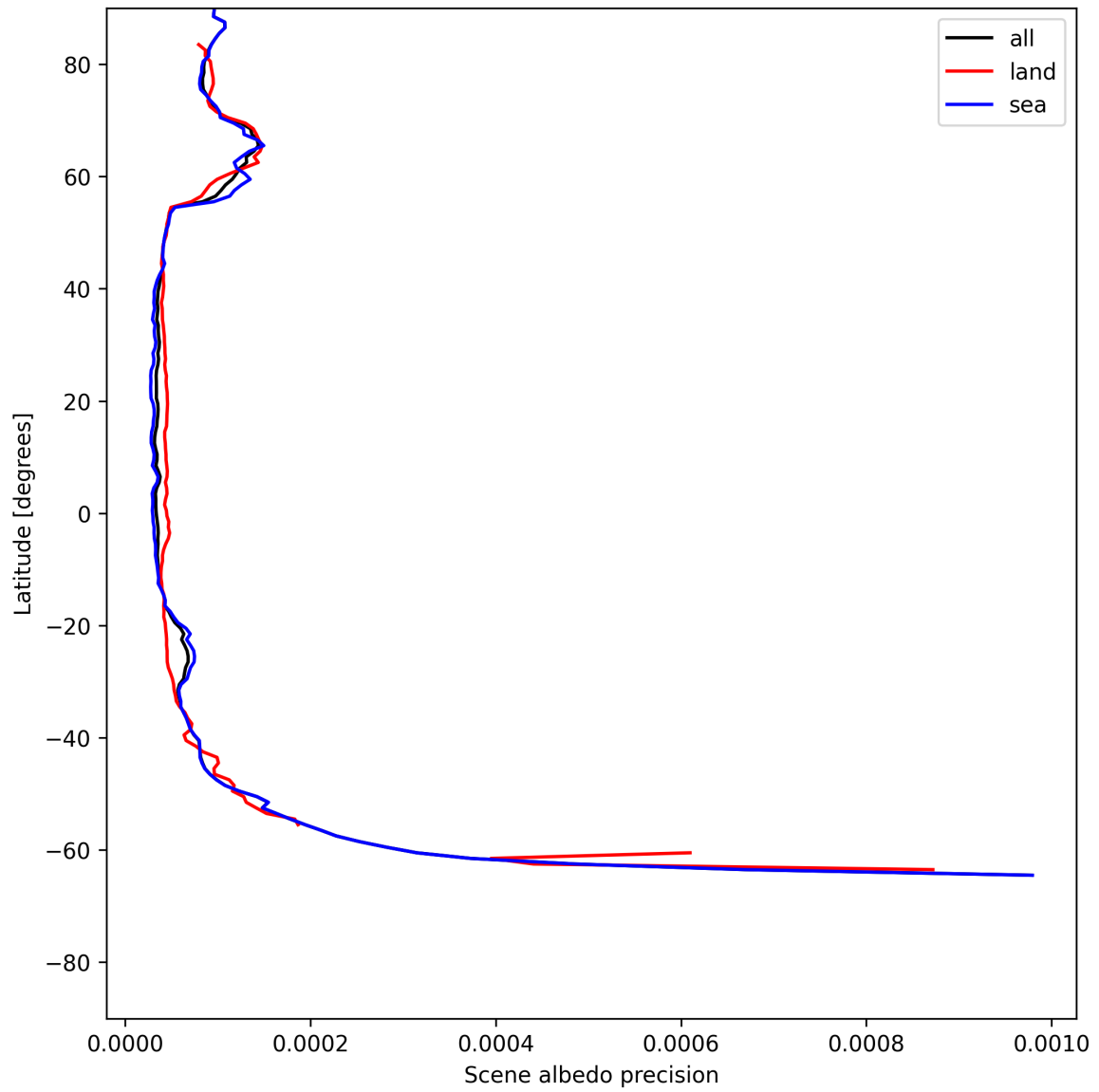
Figure 16: Zonal average of “Scene albedo precision” for 2025-07-02 to 2025-07-03.
