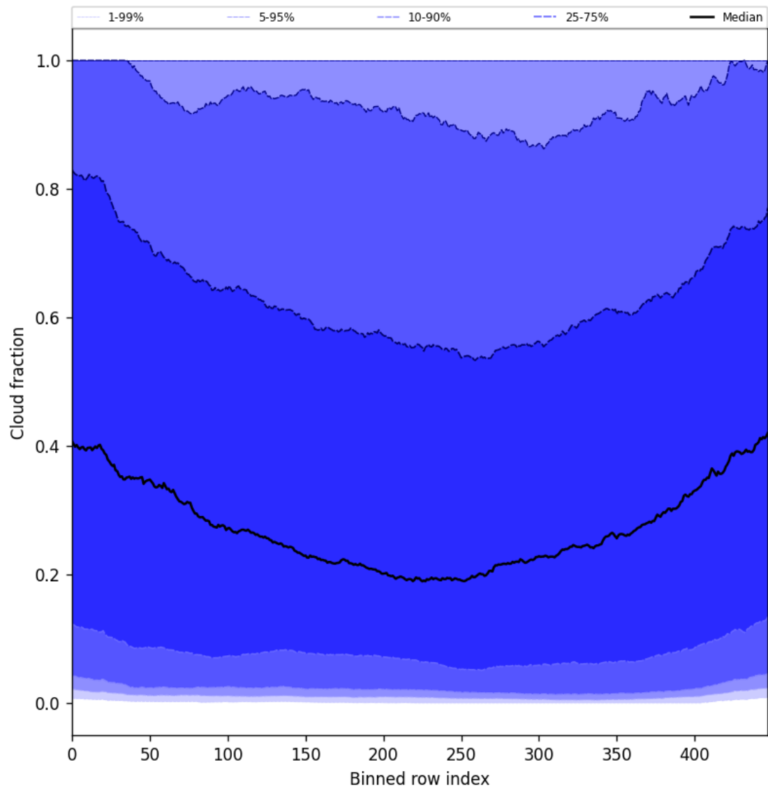
Figure 47: Along track statistics of “Cloud fraction” for 2025-07-02 to 2025-07-03
