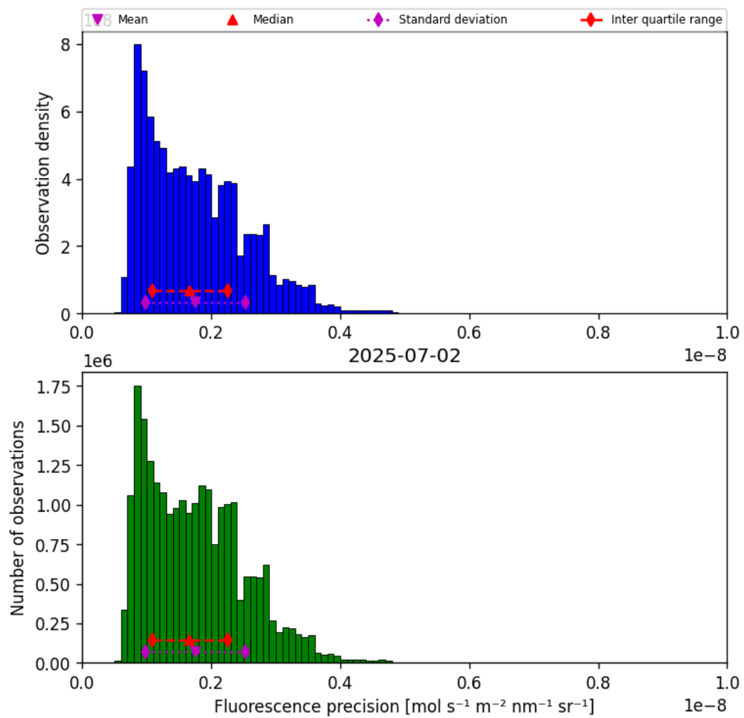
Figure 39: Histogram of “Fluorescence precision” for 2025-07-02 to 2025-07-03
