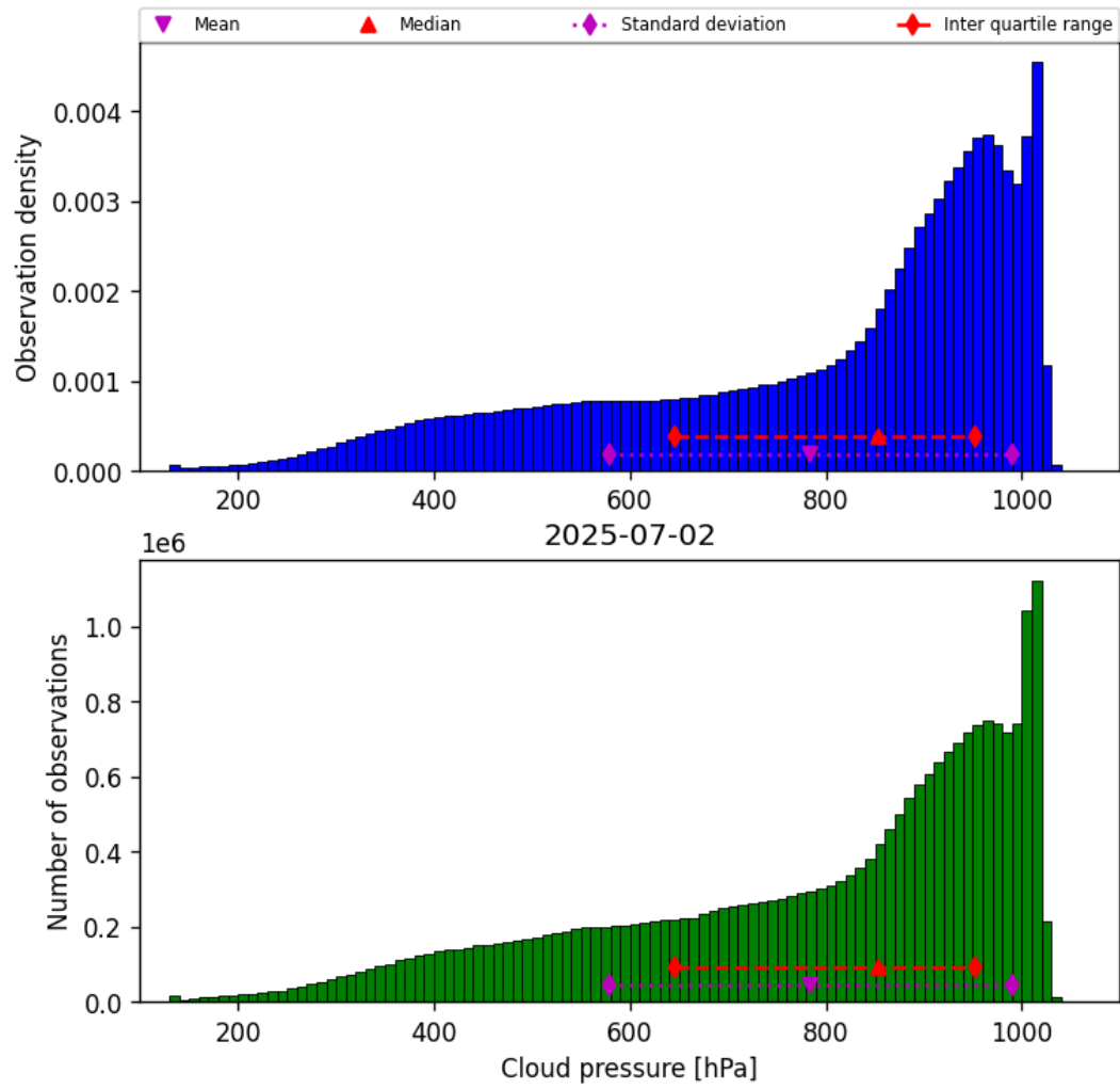
Figure 28: Histogram of “Cloud pressure” for 2025-07-02 to 2025-07-03
