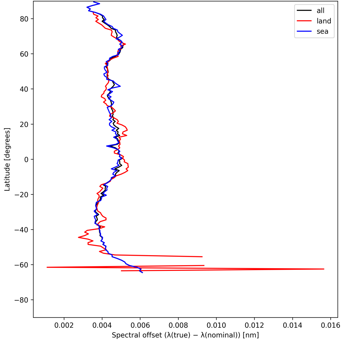
Figure 26: Zonal average of “Spectral offset ( \lambda_{\text{true}} - \lambda_{\text{nominal}} )” for 2025-07-02 to 2025-07-03.
