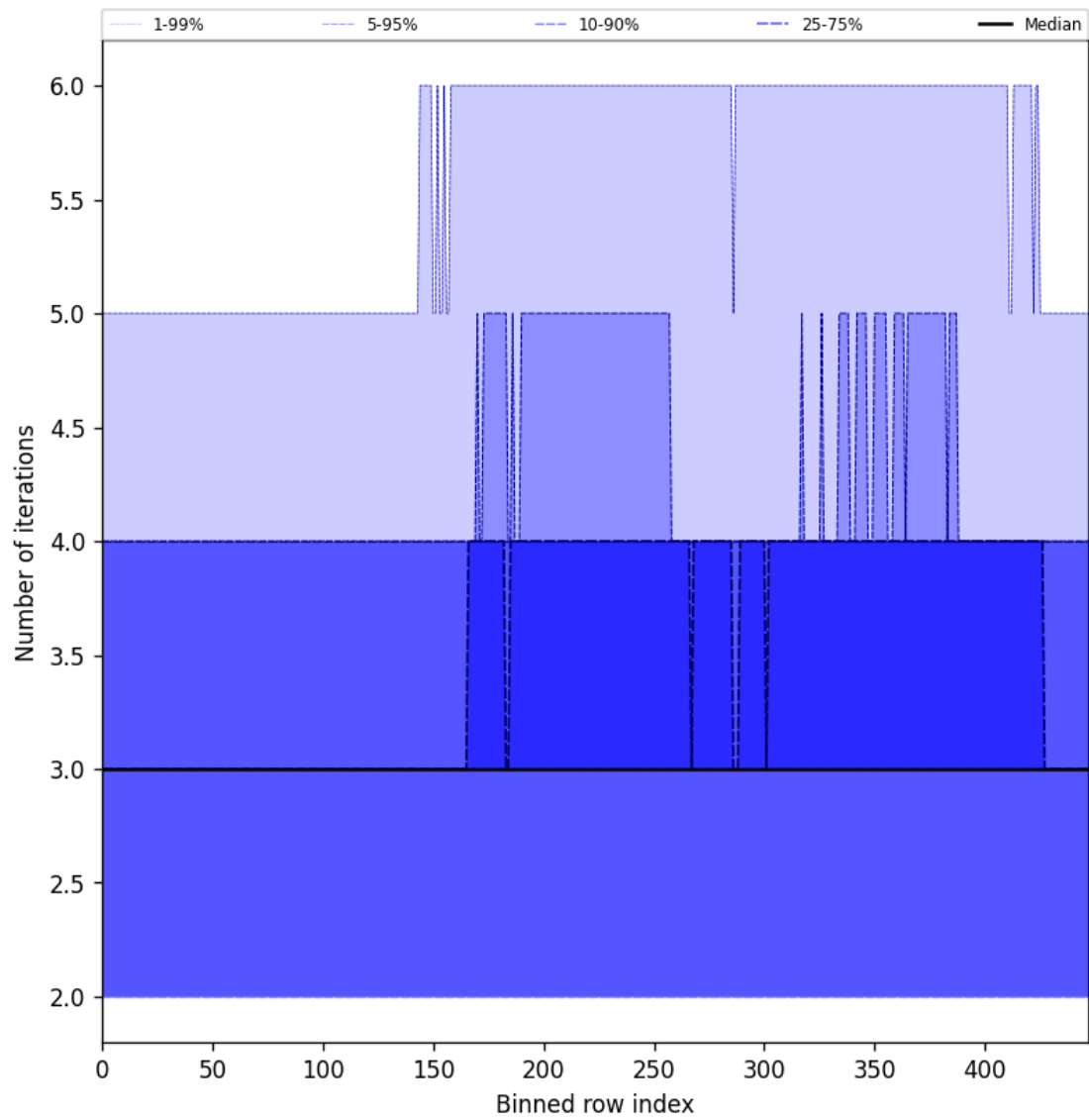
Figure 54: Along track statistics of “Number of iterations” for 2025-07-02 to 2025-07-03
