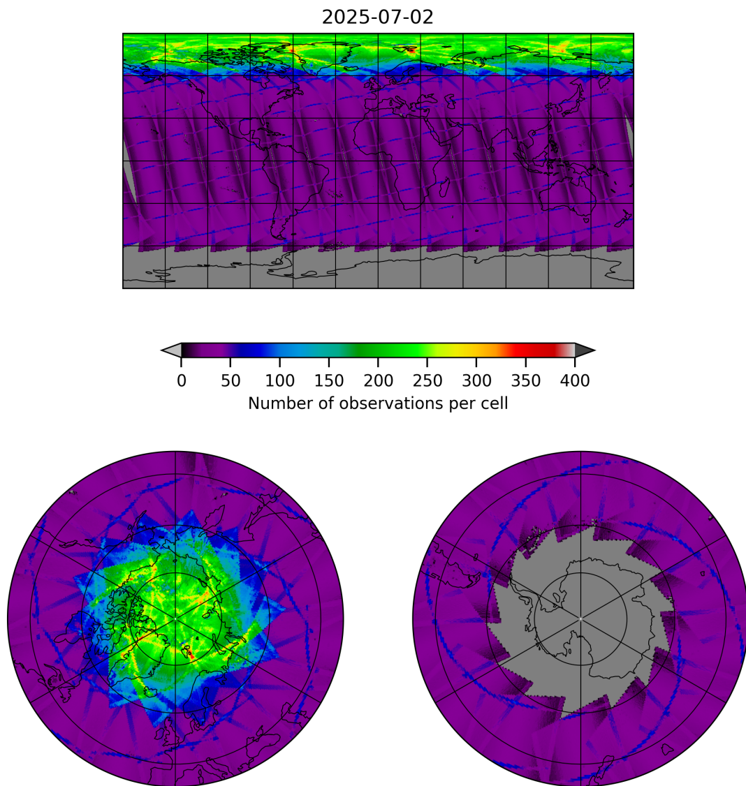
Figure 9: Map of the number of observations for 2025-07-02 to 2025-07-03
