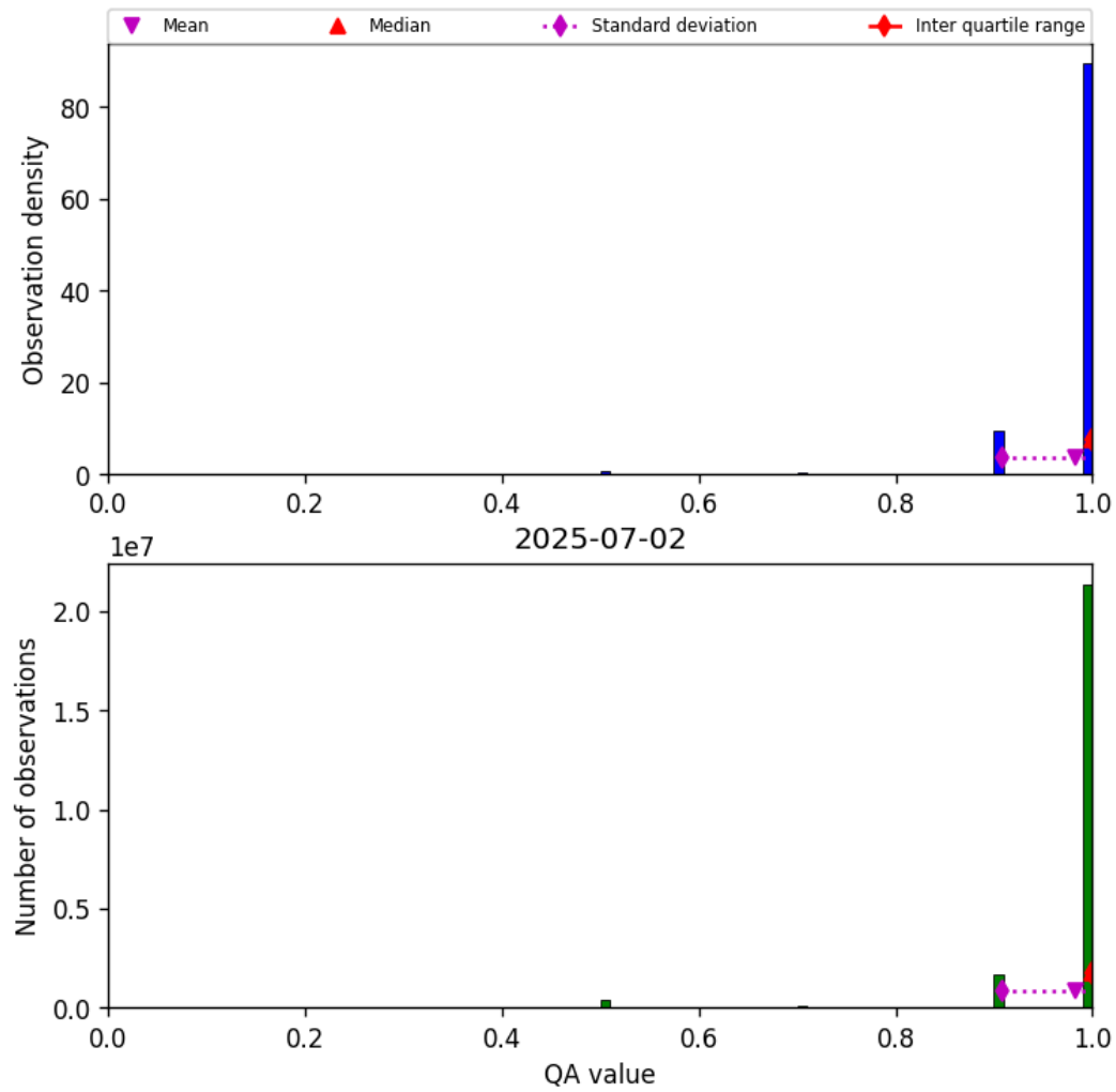
Figure 27: Histogram of “QA value” for 2025-07-02 to 2025-07-03
