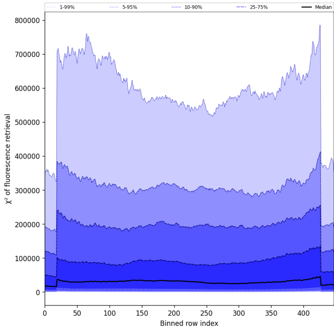
Figure 57: Along track statistics of “ \chi^2 of fluorescence retrieval” for 2025-07-02 to 2025-07-03
