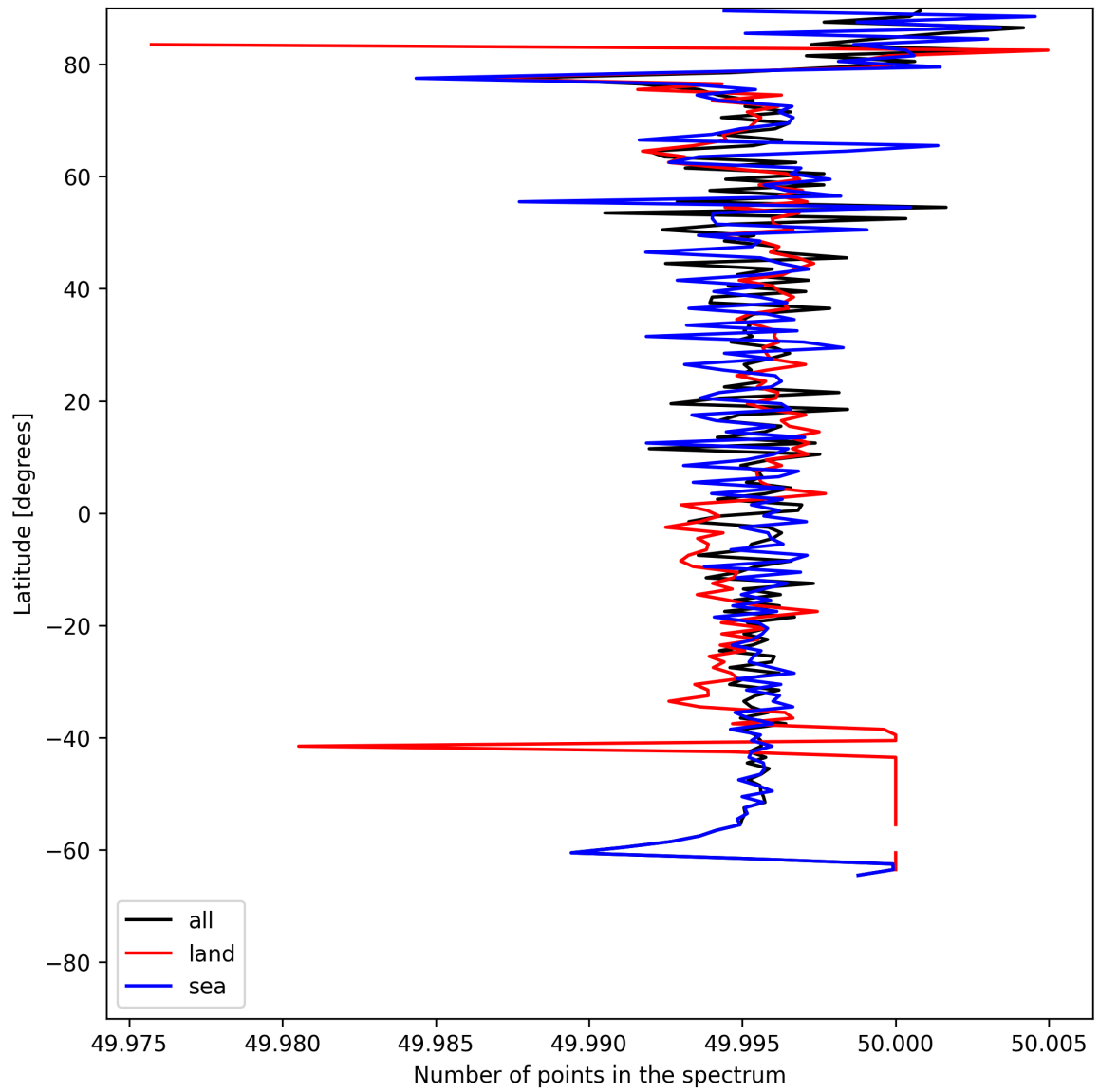
Figure 25: Zonal average of “Number of points in the spectrum” for 2025-07-02 to 2025-07-03.
