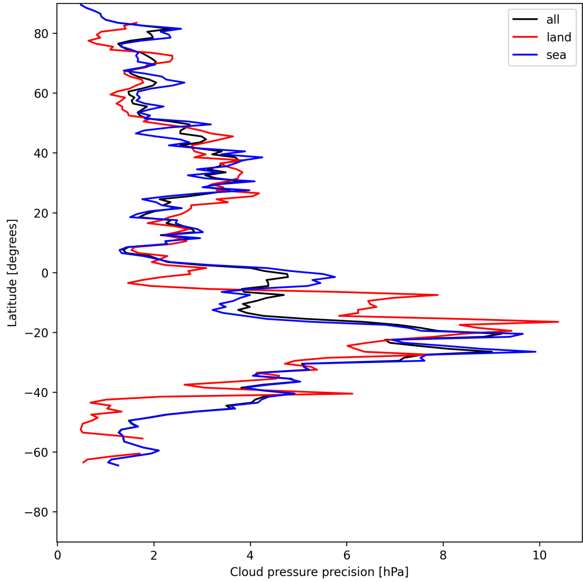
Figure 12: Zonal average of “Cloud pressure precision” for 2025-07-02 to 2025-07-03.
