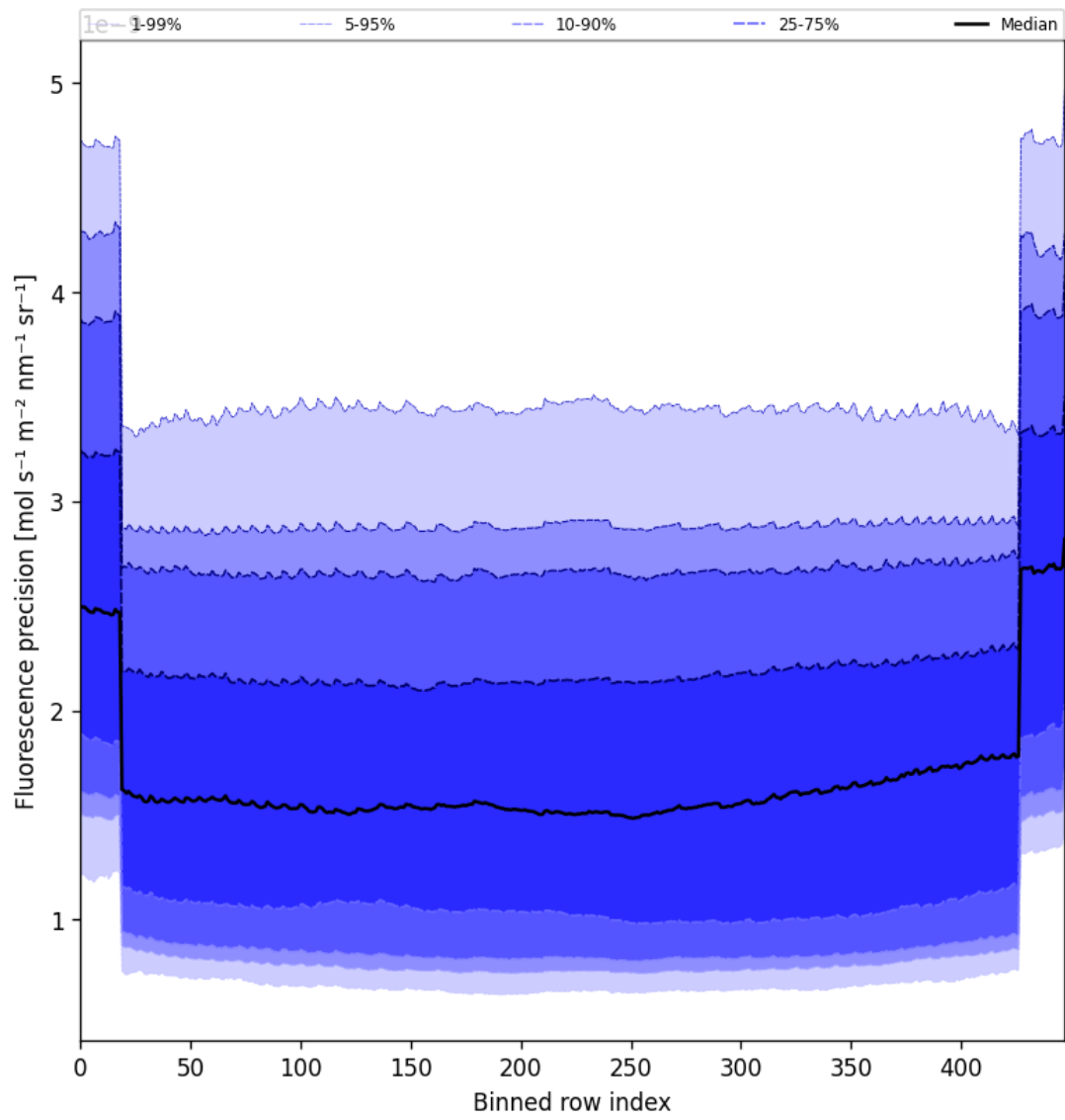
Figure 56: Along track statistics of “Fluorescence precision” for 2025-07-02 to 2025-07-03
