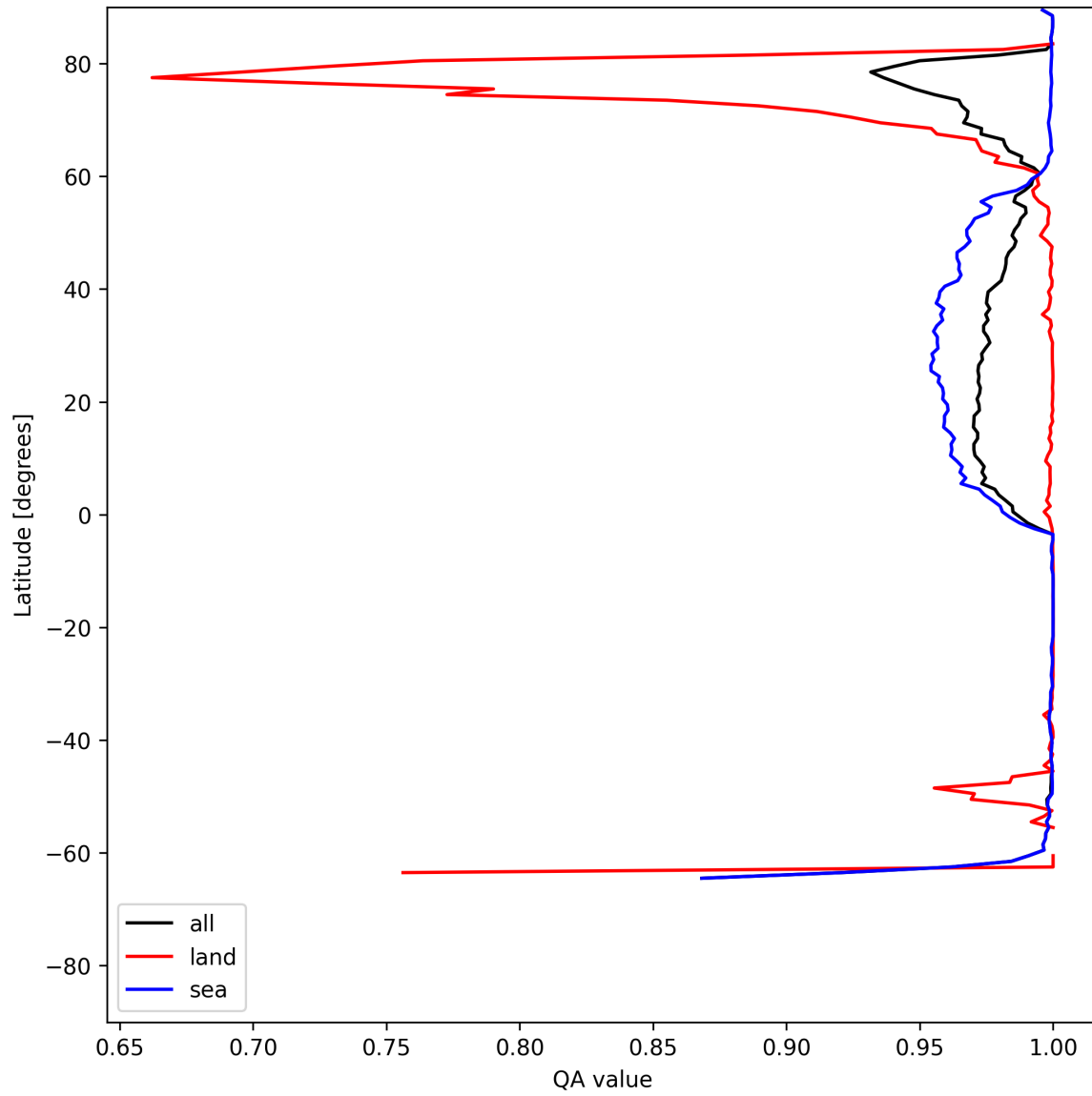
Figure 10: Zonal average of “QA value” for 2025-07-02 to 2025-07-03.
