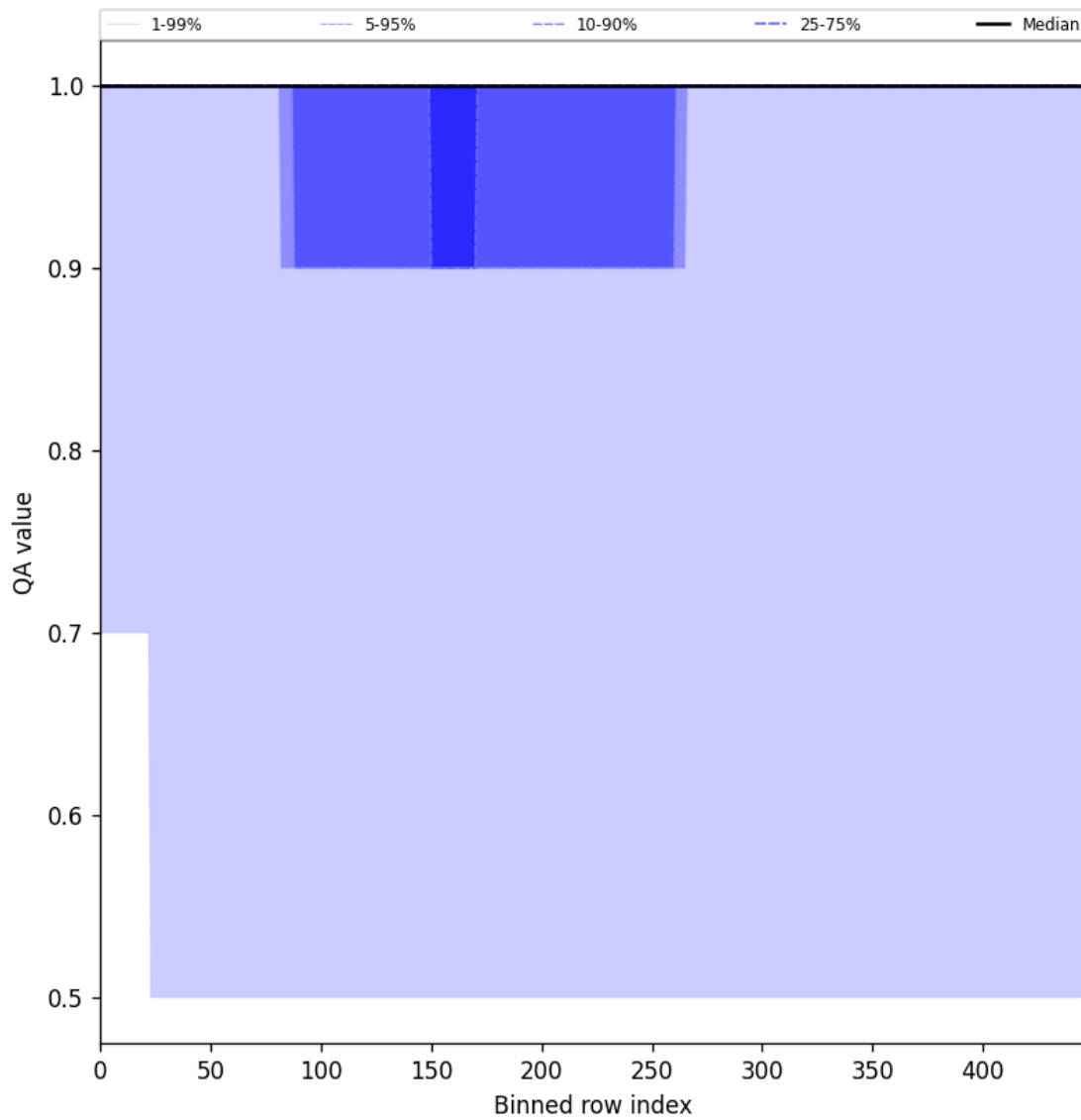
Figure 44: Along track statistics of “QA value” for 2025-07-02 to 2025-07-03
