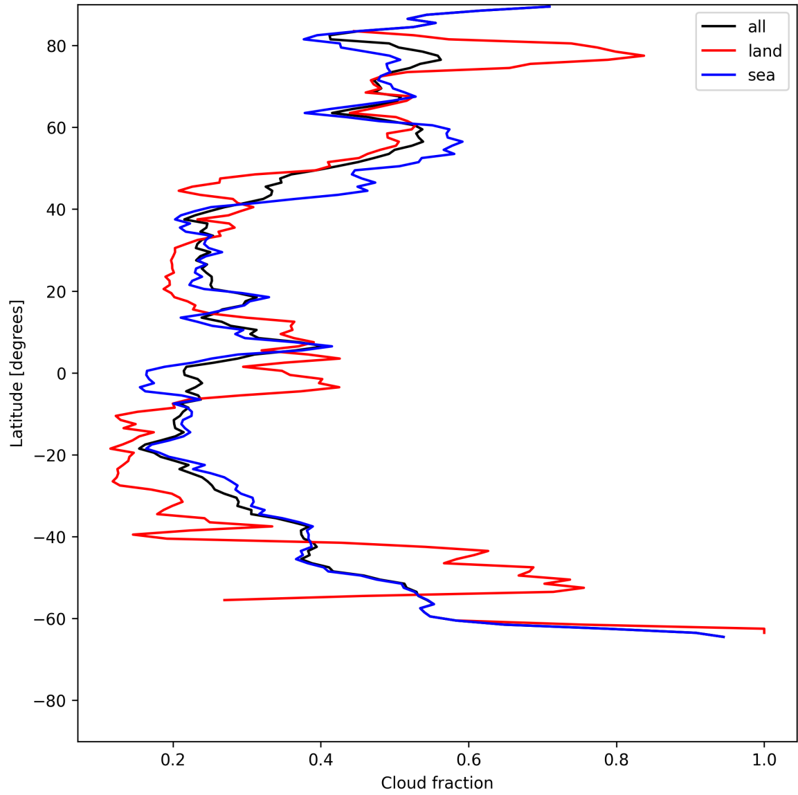
Figure 13: Zonal average of “Cloud fraction” for 2025-07-02 to 2025-07-03.
