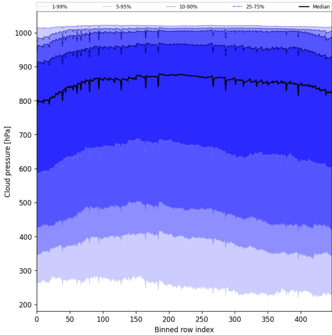
Figure 45: Along track statistics of “Cloud pressure” for 2025-07-02 to 2025-07-03
