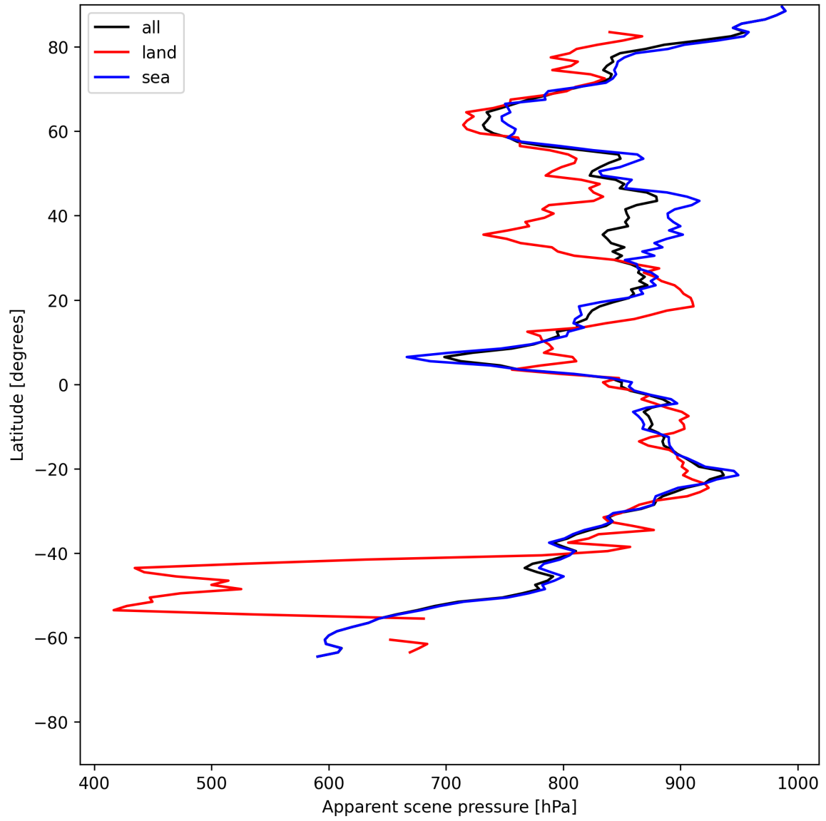
Figure 17: Zonal average of “Apparent scene pressure” for 2025-07-02 to 2025-07-03.
