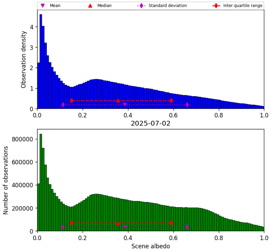
Figure 32: Histogram of “Scene albedo” for 2025-07-02 to 2025-07-03
