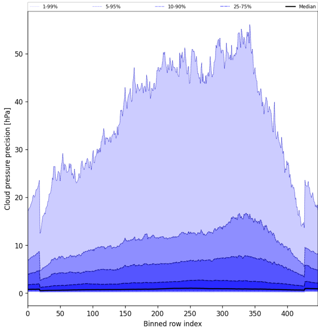
Figure 46: Along track statistics of “Cloud pressure precision” for 2025-07-02 to 2025-07-03
