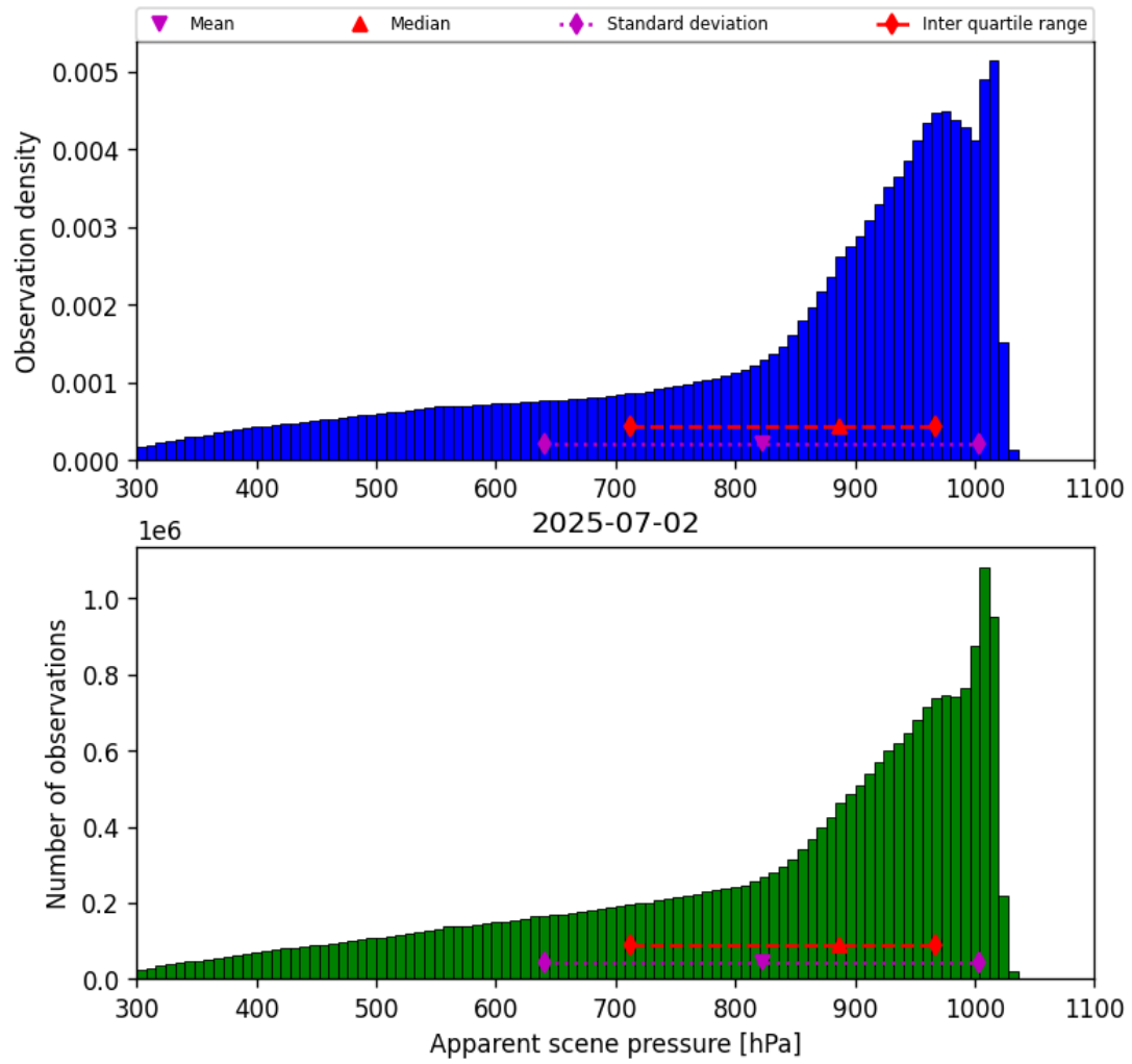
Figure 34: Histogram of “Apparent scene pressure” for 2025-07-02 to 2025-07-03
