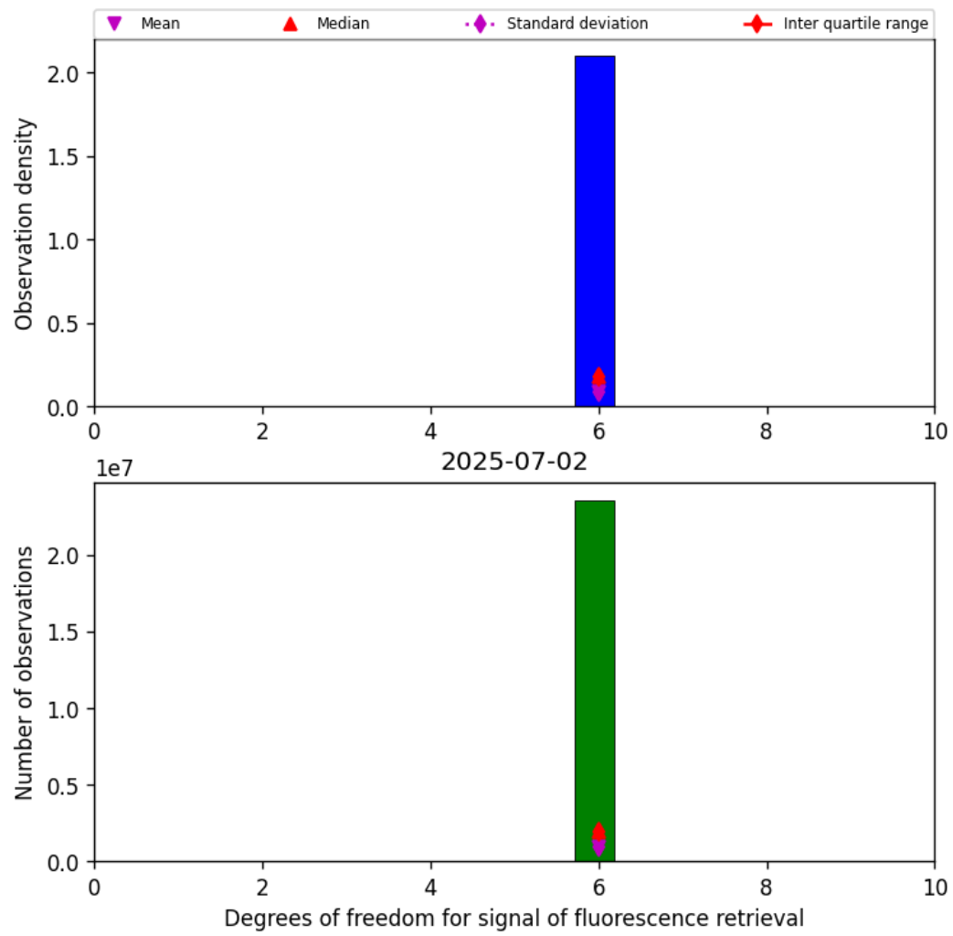
Figure 41: Histogram of “Degrees of freedom for signal of fluorescence retrieval” for 2025-07-02 to 2025-07-03
