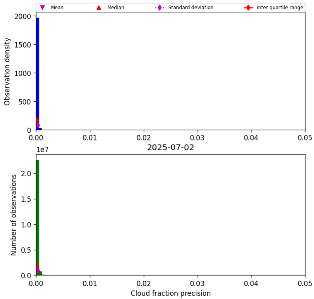
Figure 31: Histogram of “Cloud fraction precision” for 2025-07-02 to 2025-07-03
