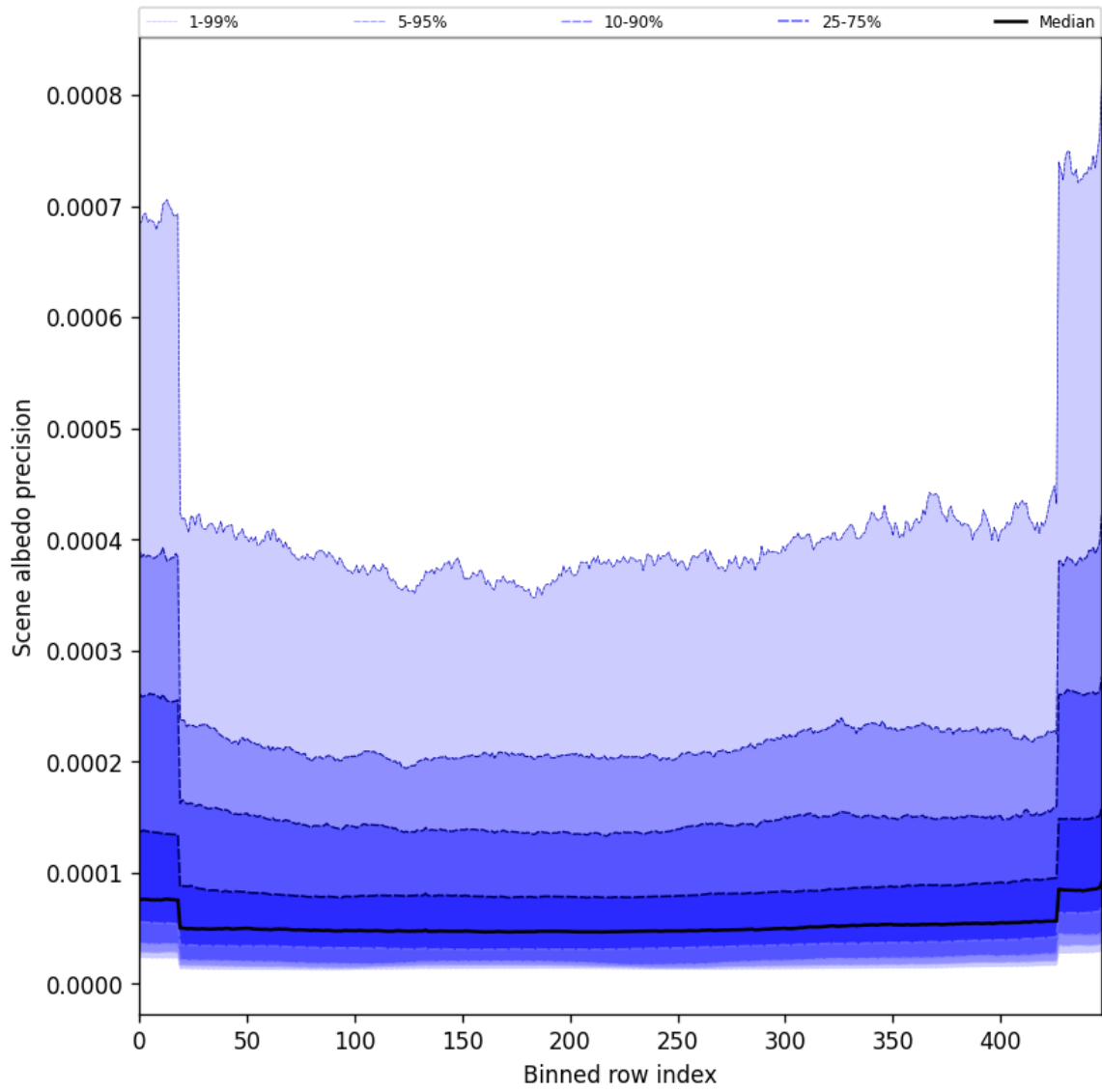
Figure 50: Along track statistics of “Scene albedo precision” for 2025-07-02 to 2025-07-03
