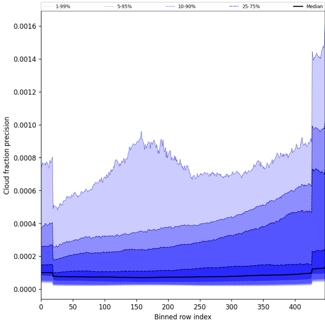
Figure 48: Along track statistics of “Cloud fraction precision” for 2025-07-02 to 2025-07-03
