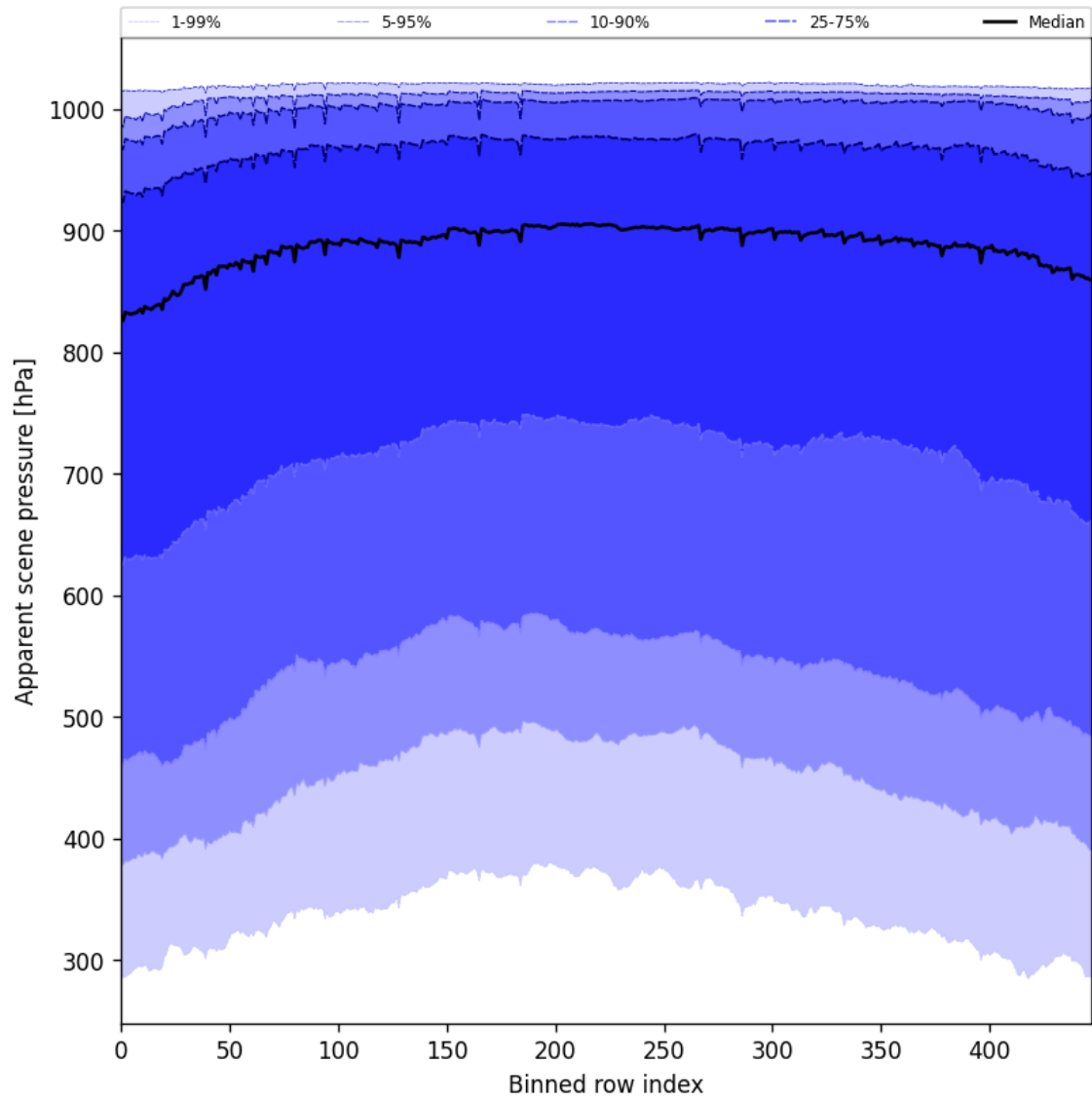
Figure 51: Along track statistics of “Apparent scene pressure” for 2025-07-02 to 2025-07-03
