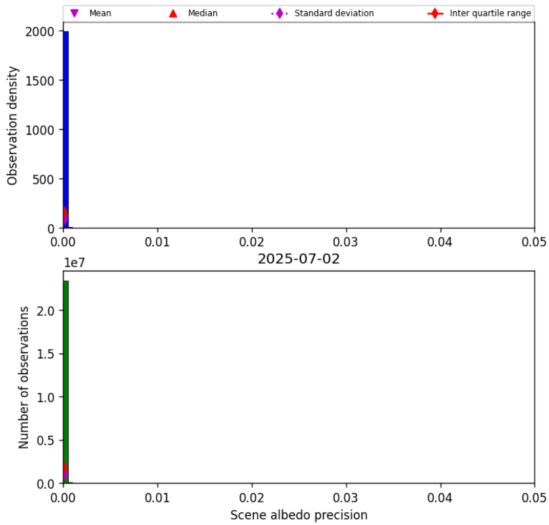
Figure 33: Histogram of “Scene albedo precision” for 2025-07-02 to 2025-07-03
