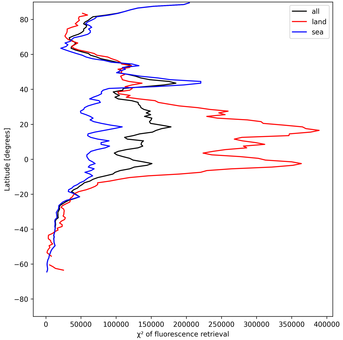
Figure 23: Zonal average of “ \chi^2 of fluorescence retrieval” for 2025-07-02 to 2025-07-03.
