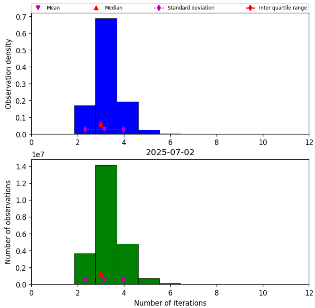
Figure 37: Histogram of “Number of iterations” for 2025-07-02 to 2025-07-03
