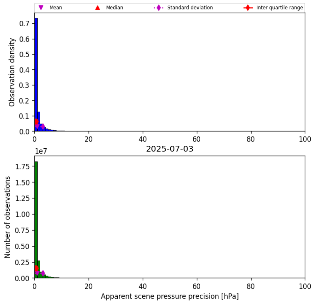
Figure 35: Histogram of “Apparent scene pressure precision” for 2025-07-03 to 2025-07-04
