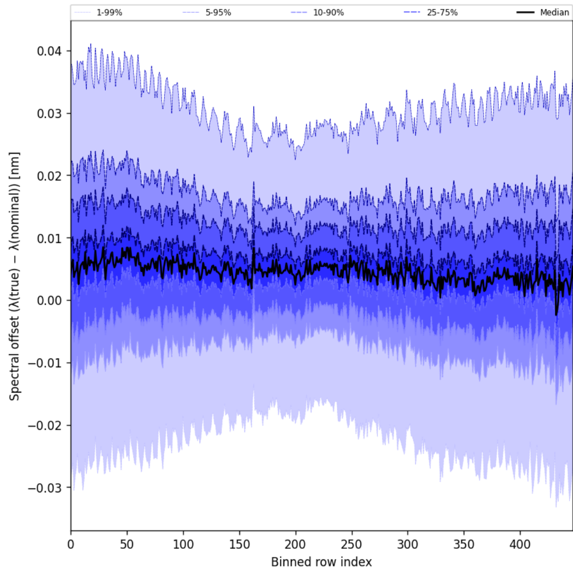
Figure 60: Along track statistics of “Spectral offset ( \lambda_{\text{true}} - \lambda_{\text{nominal}} )” for 2025-07-03 to 2025-07-04
