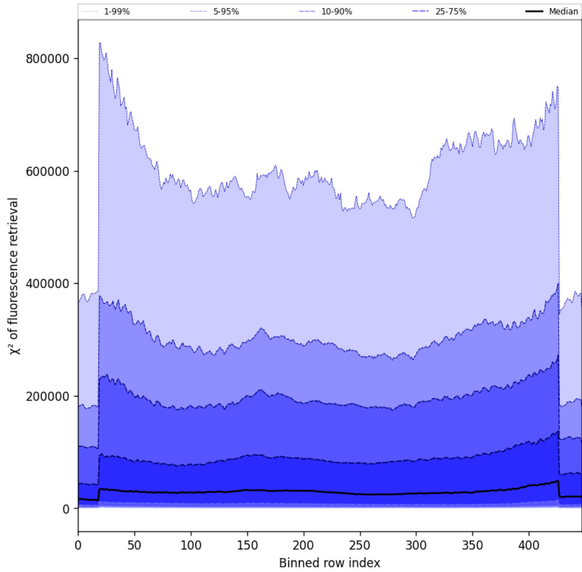
Figure 57: Along track statistics of “ \chi^2 of fluorescence retrieval” for 2025-07-03 to 2025-07-04
