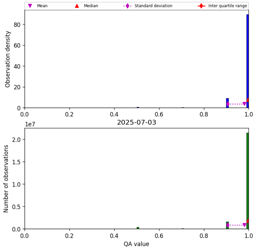
Figure 27: Histogram of “QA value” for 2025-07-03 to 2025-07-04
