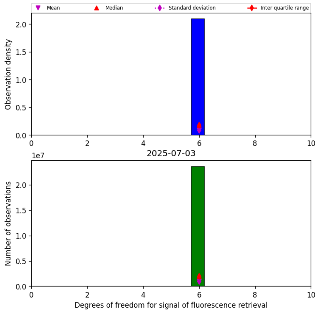
Figure 41: Histogram of “Degrees of freedom for signal of fluorescence retrieval” for 2025-07-03 to 2025-07-04
