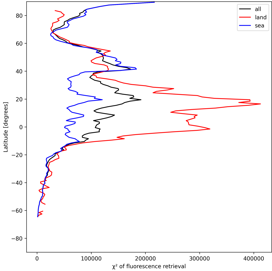
Figure 23: Zonal average of “ \chi^2 of fluorescence retrieval” for 2025-07-03 to 2025-07-04.
