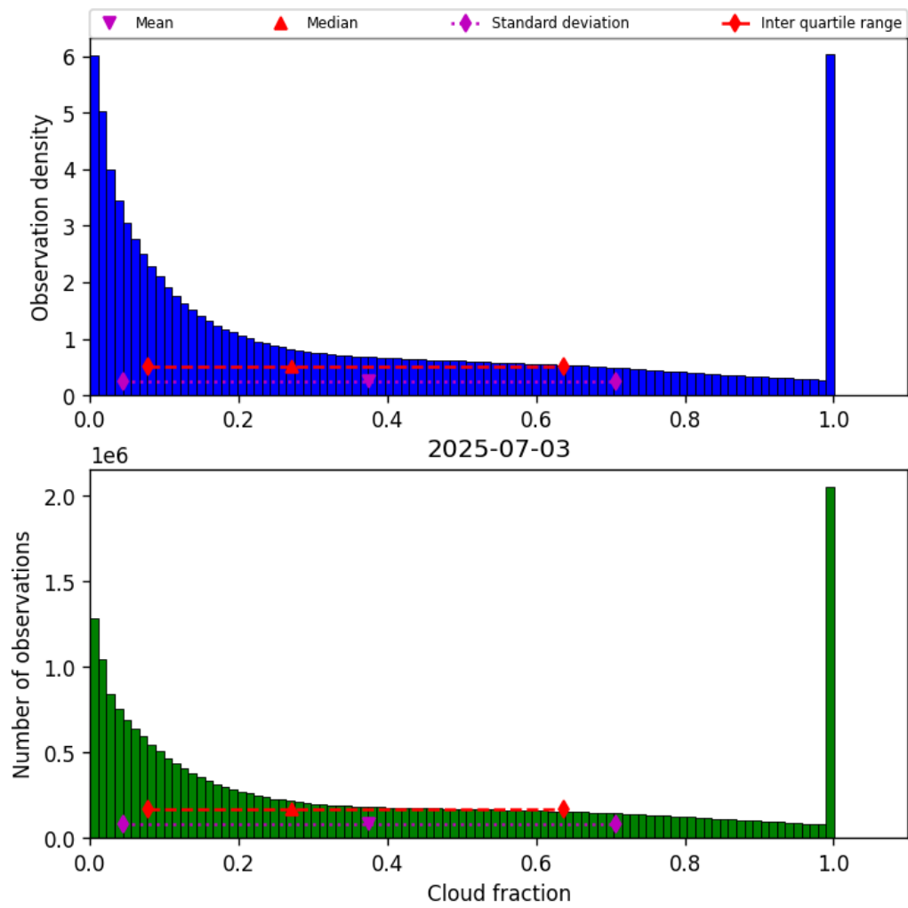
Figure 30: Histogram of “Cloud fraction” for 2025-07-03 to 2025-07-04
