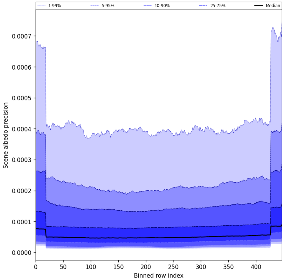
Figure 50: Along track statistics of “Scene albedo precision” for 2025-07-03 to 2025-07-04
