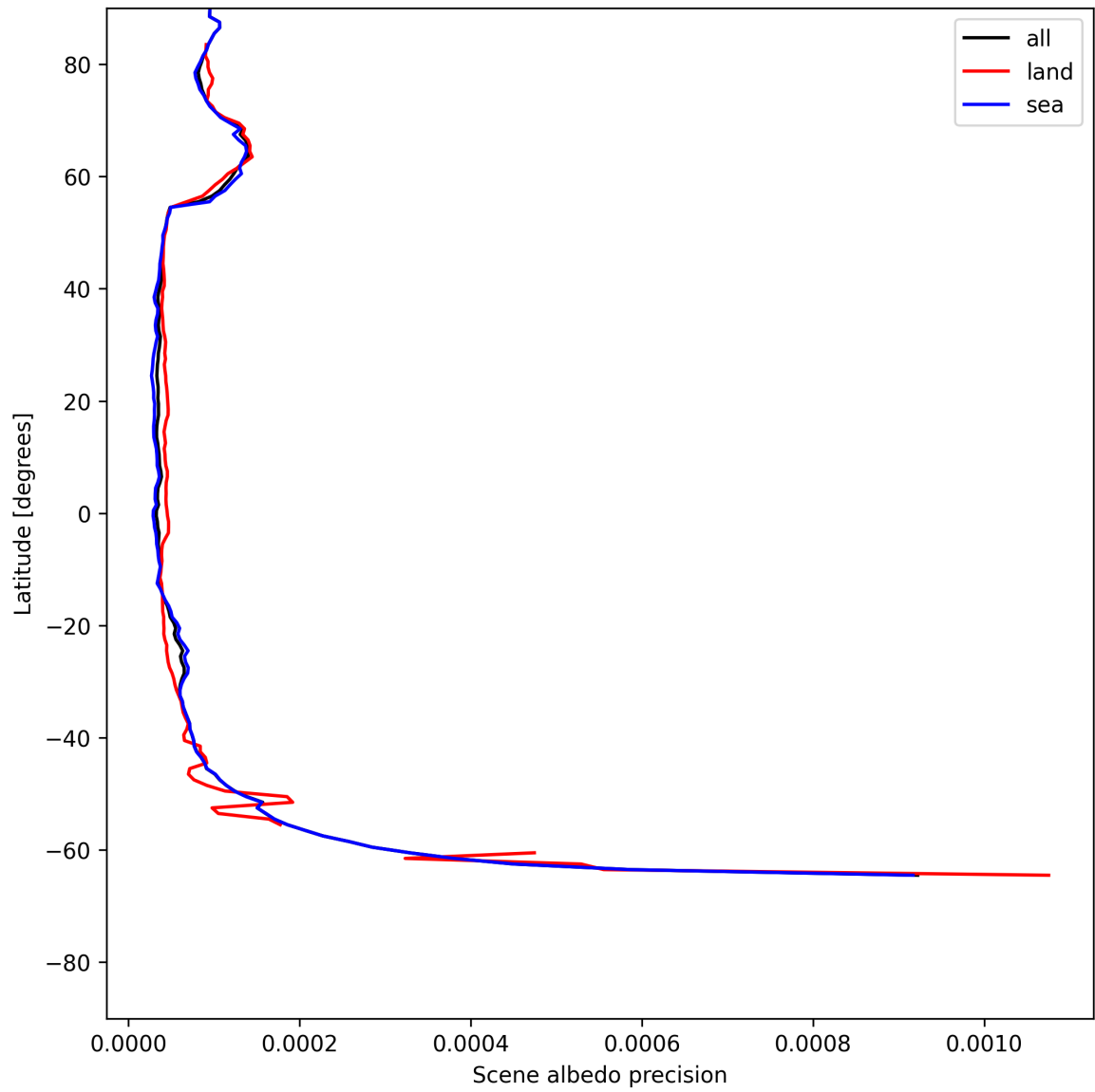
Figure 16: Zonal average of “Scene albedo precision” for 2025-07-03 to 2025-07-04.
