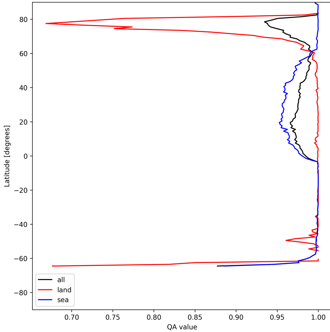
Figure 10: Zonal average of “QA value” for 2025-07-03 to 2025-07-04.
