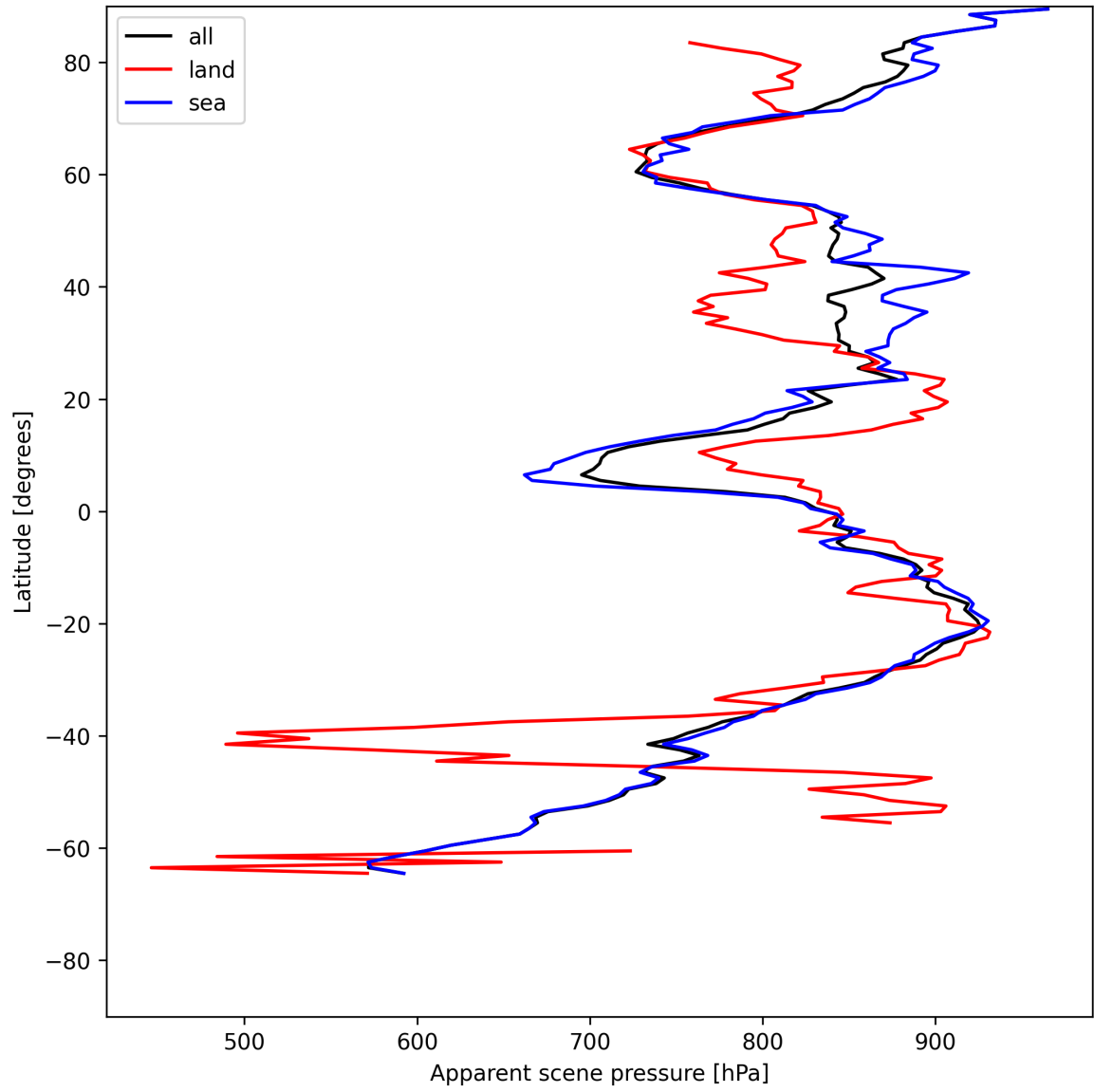
Figure 17: Zonal average of “Apparent scene pressure” for 2025-07-03 to 2025-07-04.
