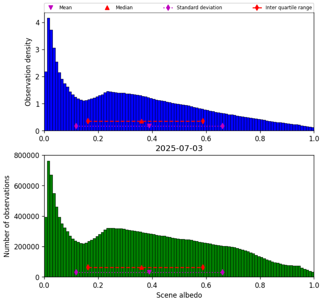
Figure 32: Histogram of “Scene albedo” for 2025-07-03 to 2025-07-04
