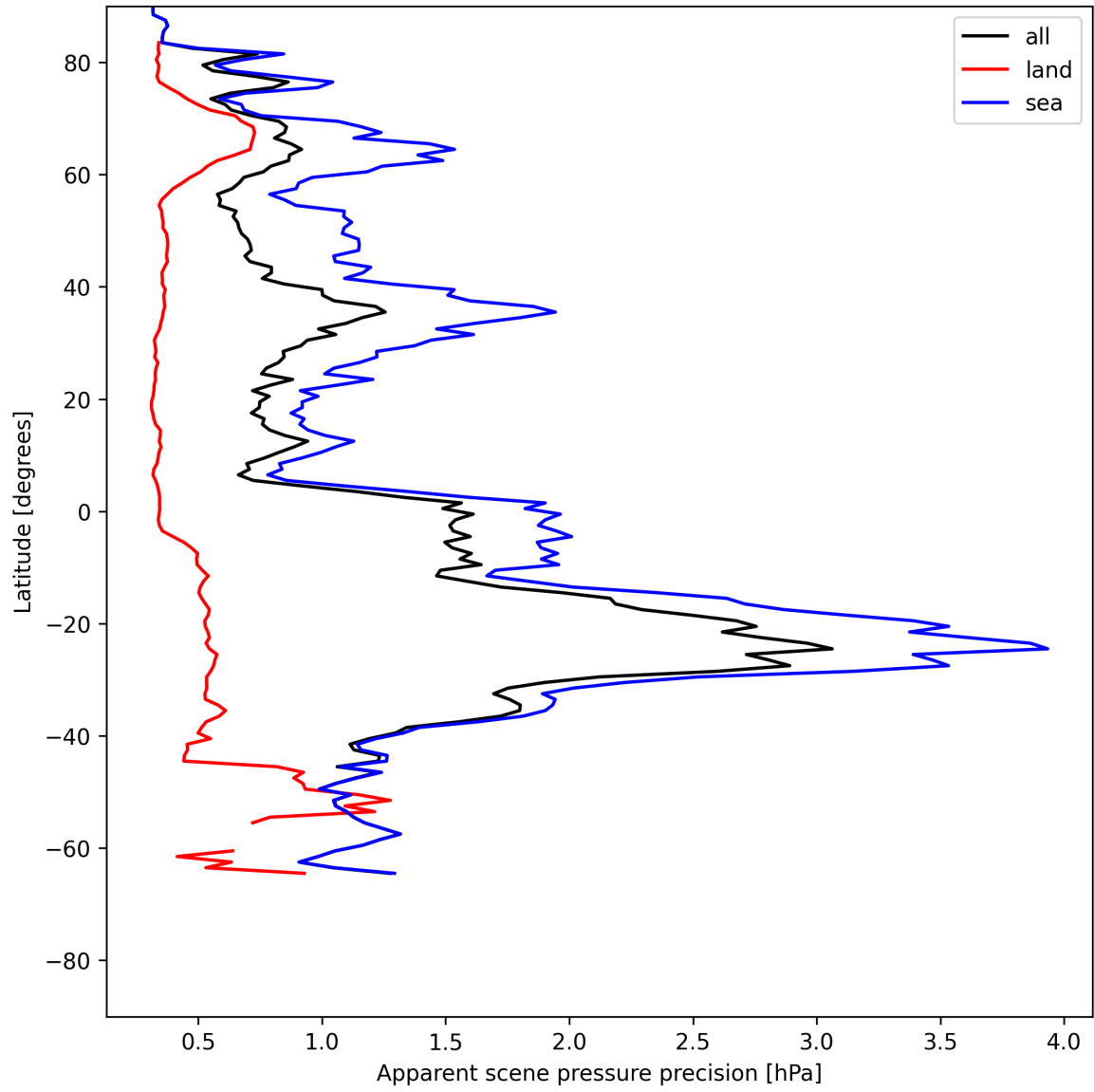
Figure 18: Zonal average of “Apparent scene pressure precision” for 2025-07-03 to 2025-07-04.
