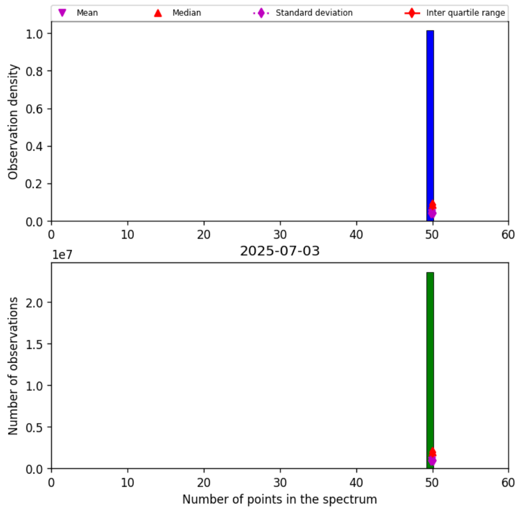
Figure 42: Histogram of “Number of points in the spectrum” for 2025-07-03 to 2025-07-04
