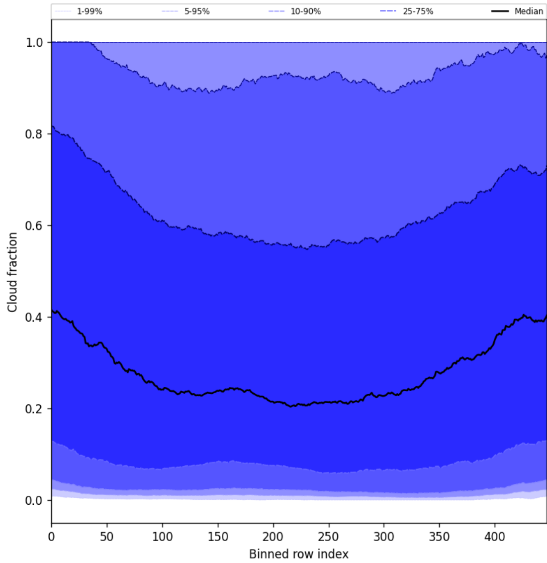
Figure 47: Along track statistics of “Cloud fraction” for 2025-07-03 to 2025-07-04
