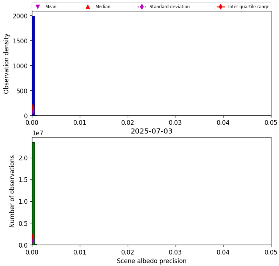
Figure 33: Histogram of “Scene albedo precision” for 2025-07-03 to 2025-07-04
