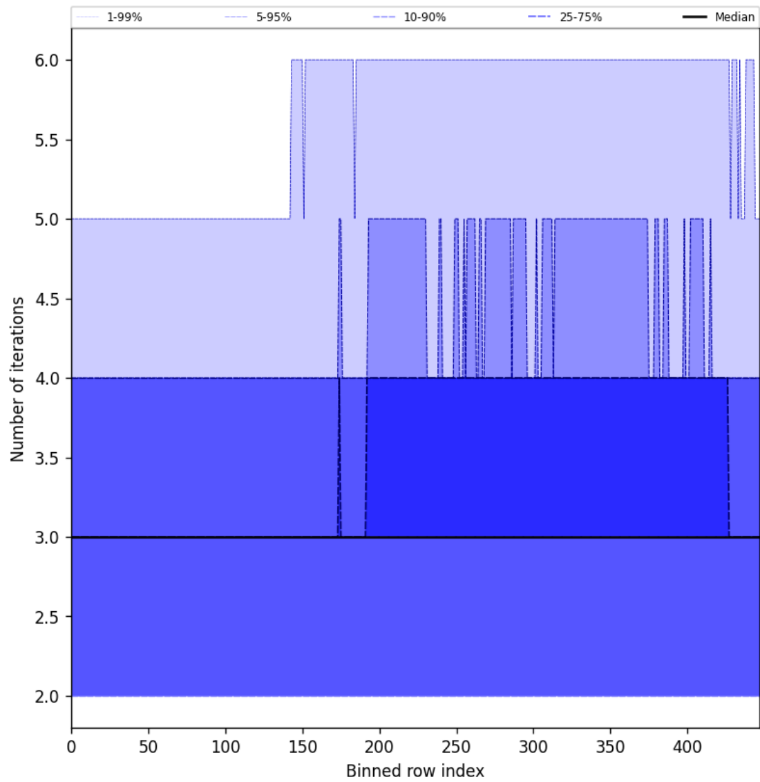
Figure 54: Along track statistics of “Number of iterations” for 2025-07-03 to 2025-07-04
