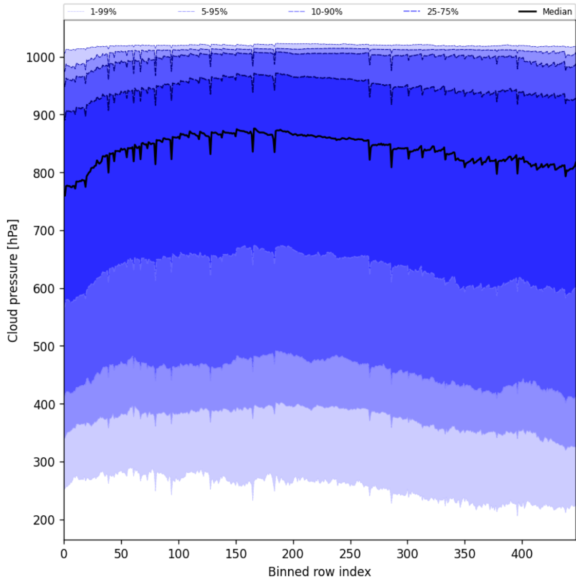
Figure 45: Along track statistics of “Cloud pressure” for 2025-07-03 to 2025-07-04
