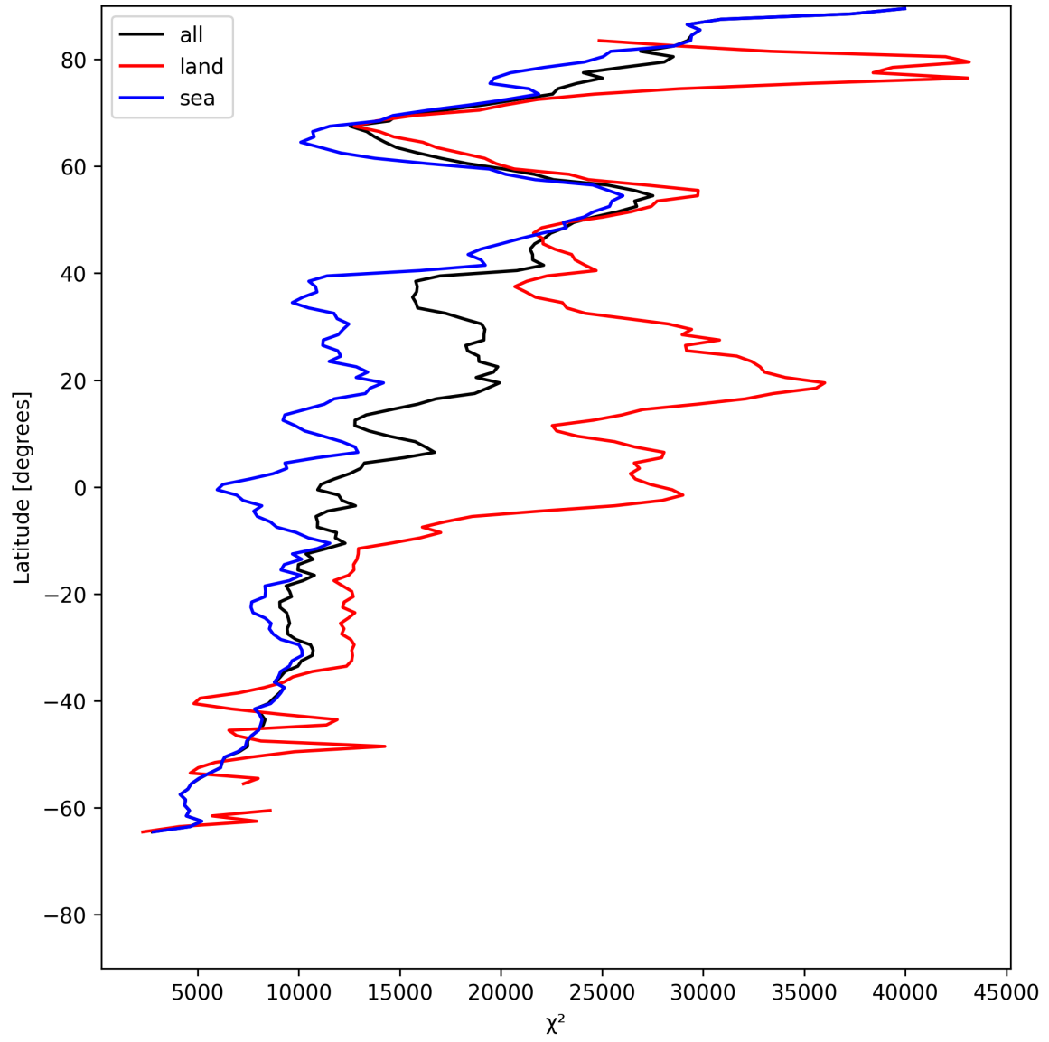
Figure 19: Zonal average of “ \chi^2 ” for 2025-07-03 to 2025-07-04.
