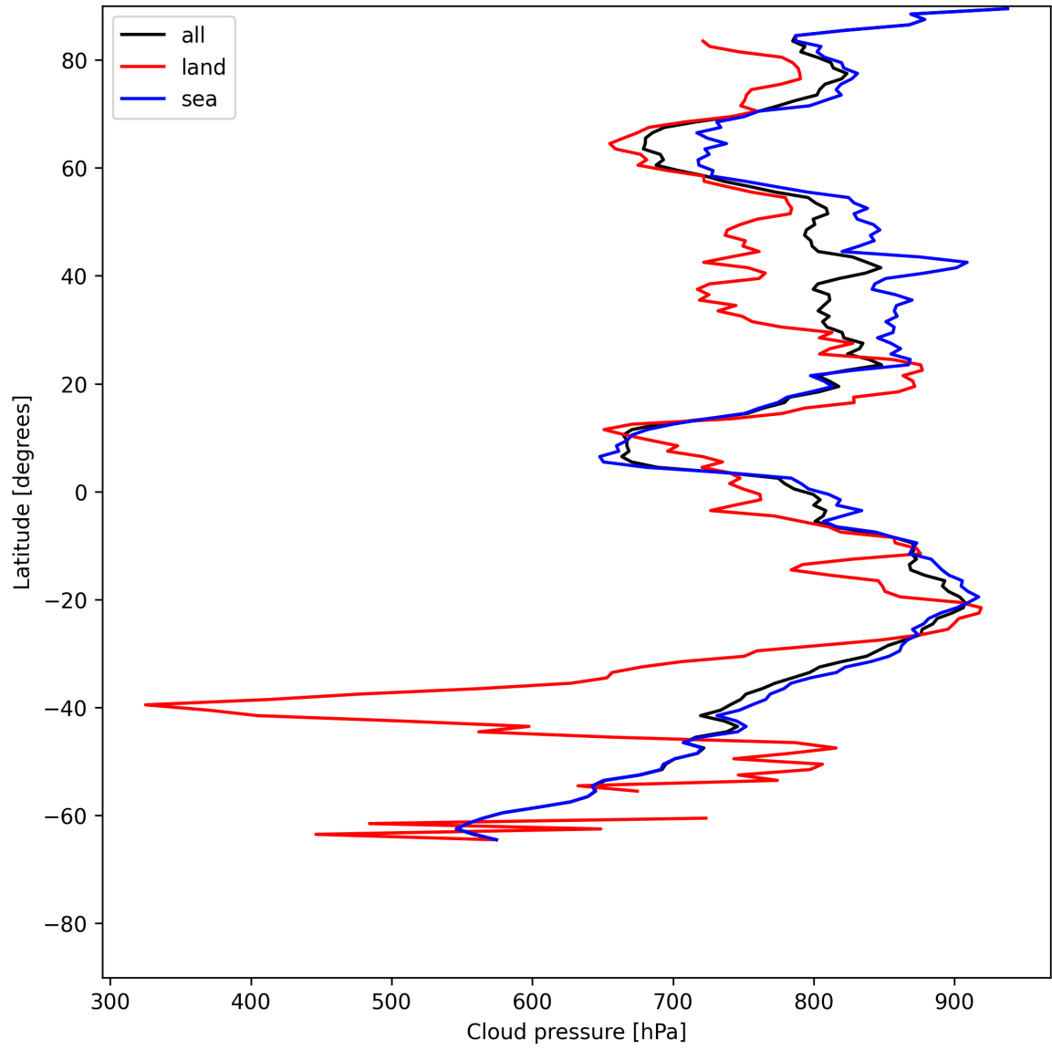
Figure 11: Zonal average of “Cloud pressure” for 2025-07-03 to 2025-07-04.
