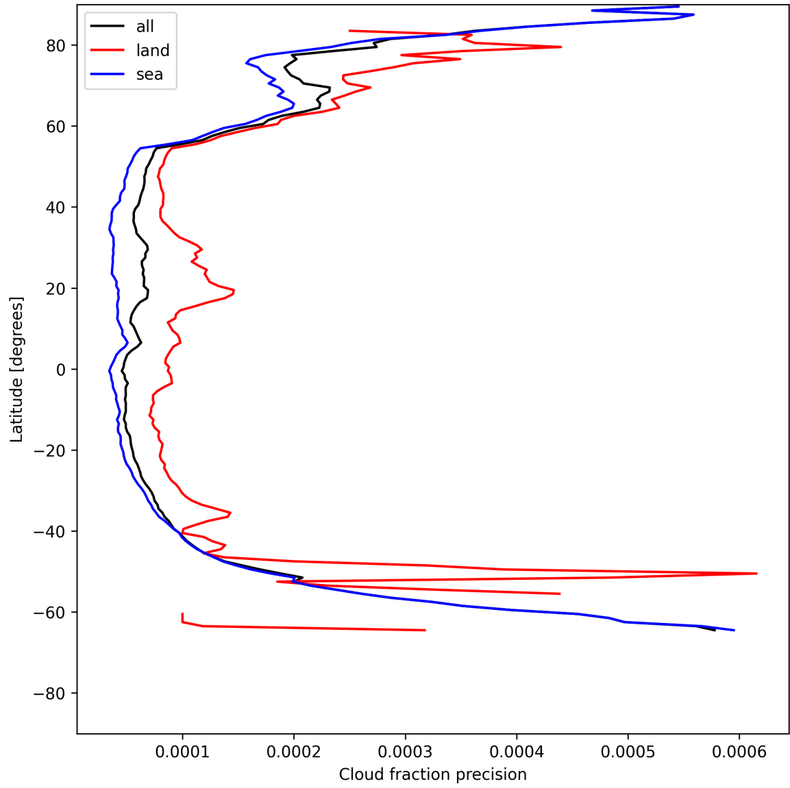
Figure 14: Zonal average of “Cloud fraction precision” for 2025-07-03 to 2025-07-04.
