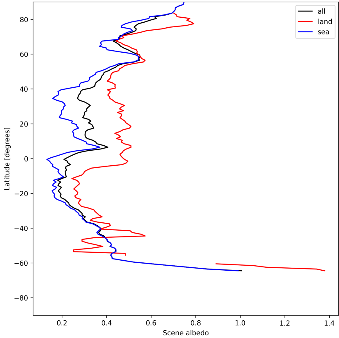
Figure 15: Zonal average of “Scene albedo” for 2025-07-03 to 2025-07-04.
