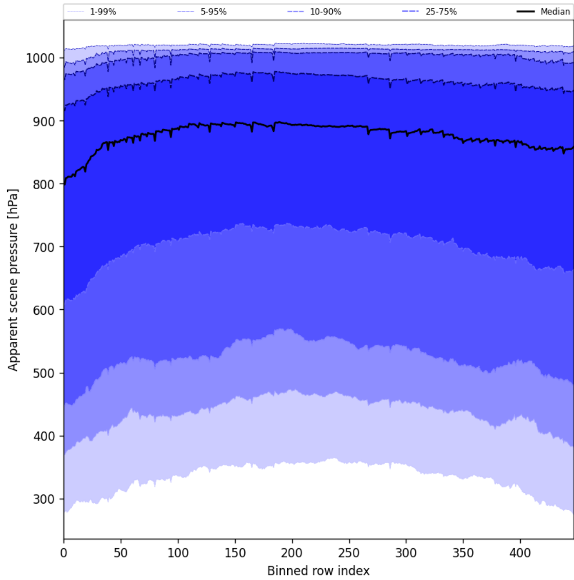
Figure 51: Along track statistics of “Apparent scene pressure” for 2025-07-03 to 2025-07-04
