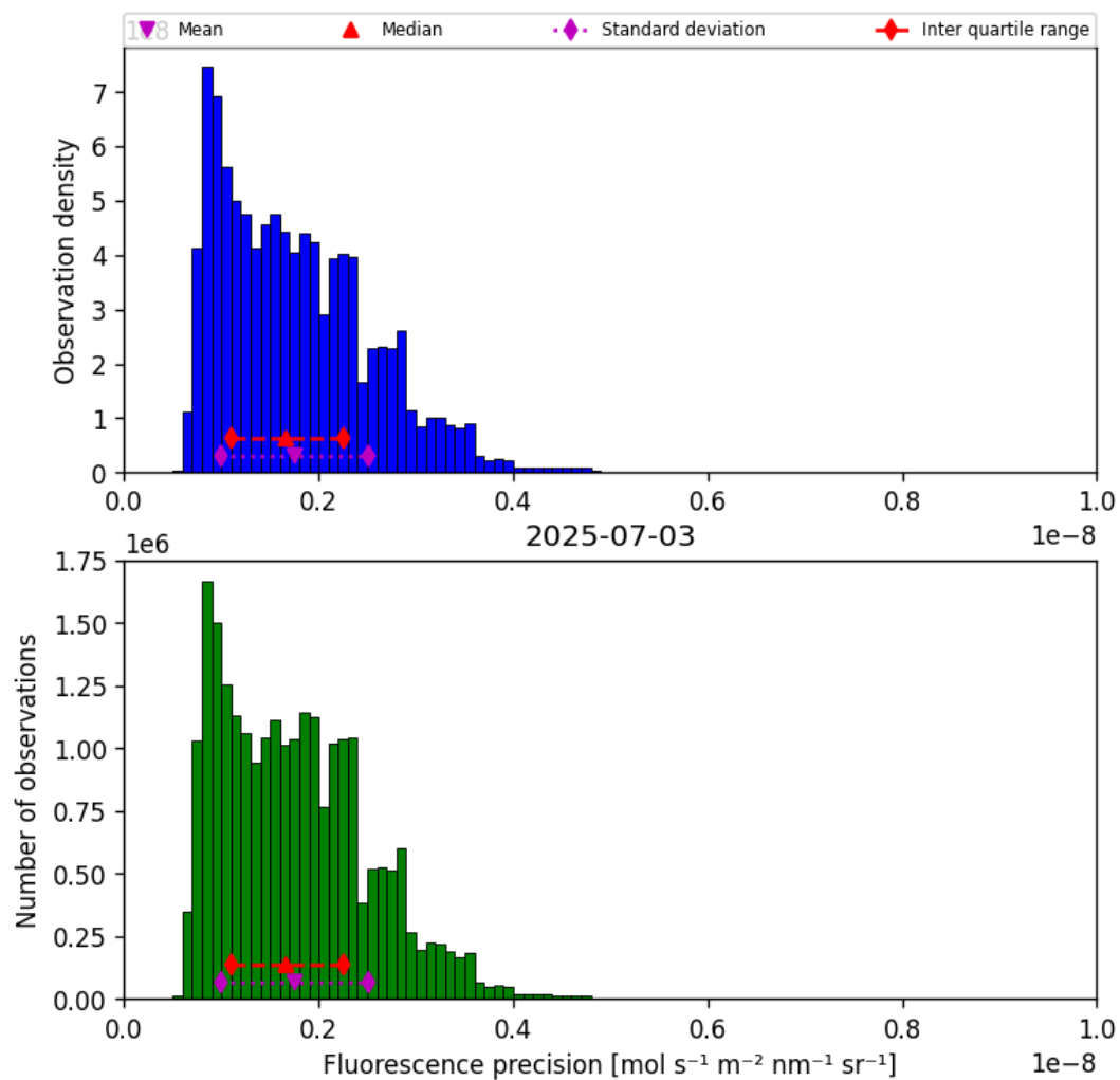
Figure 39: Histogram of “Fluorescence precision” for 2025-07-03 to 2025-07-04
