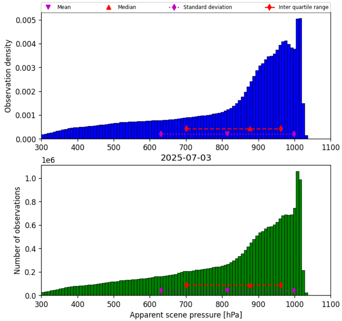
Figure 34: Histogram of “Apparent scene pressure” for 2025-07-03 to 2025-07-04
