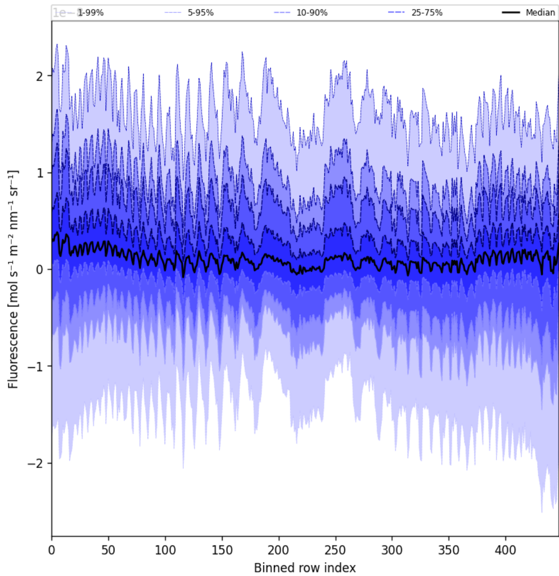
Figure 55: Along track statistics of “Fluorescence” for 2025-07-03 to 2025-07-04
