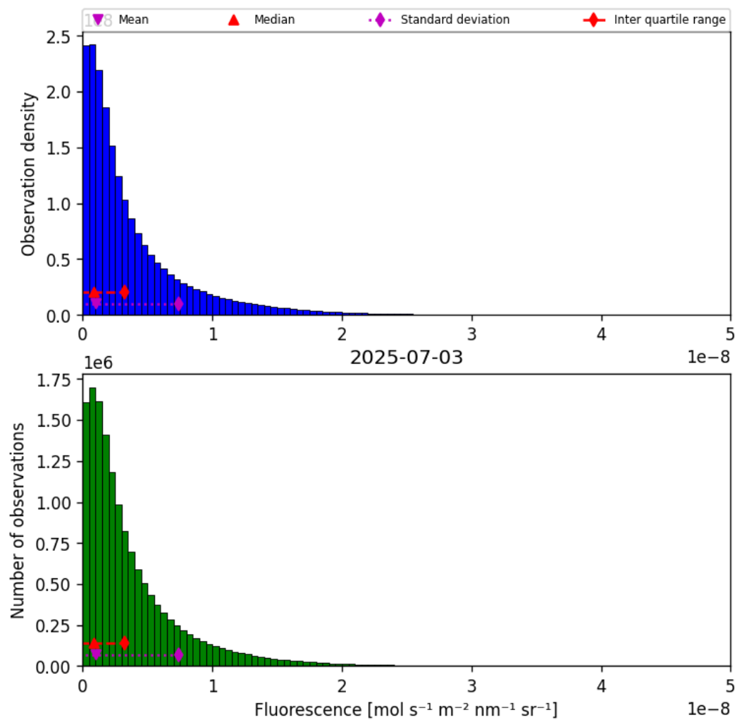
Figure 38: Histogram of “Fluorescence” for 2025-07-03 to 2025-07-04
