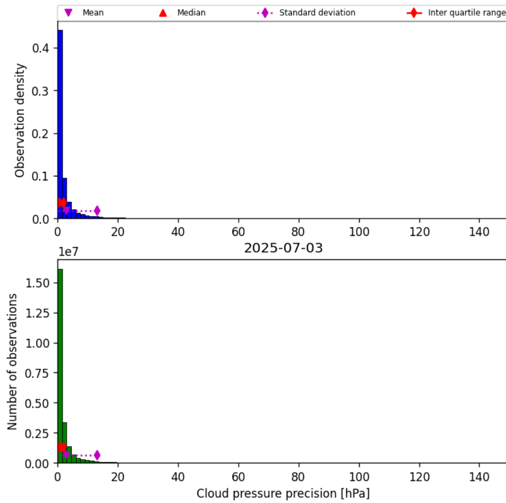
Figure 29: Histogram of “Cloud pressure precision” for 2025-07-03 to 2025-07-04
