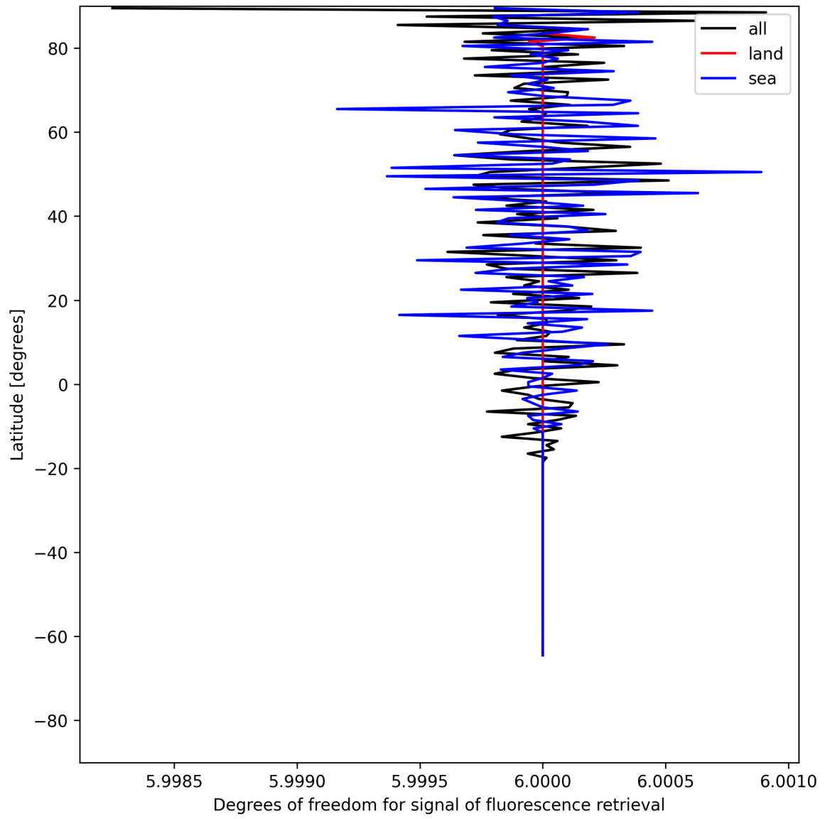
Figure 24: Zonal average of “Degrees of freedom for signal of fluorescence retrieval” for 2025-07-03 to 2025-07-04.
