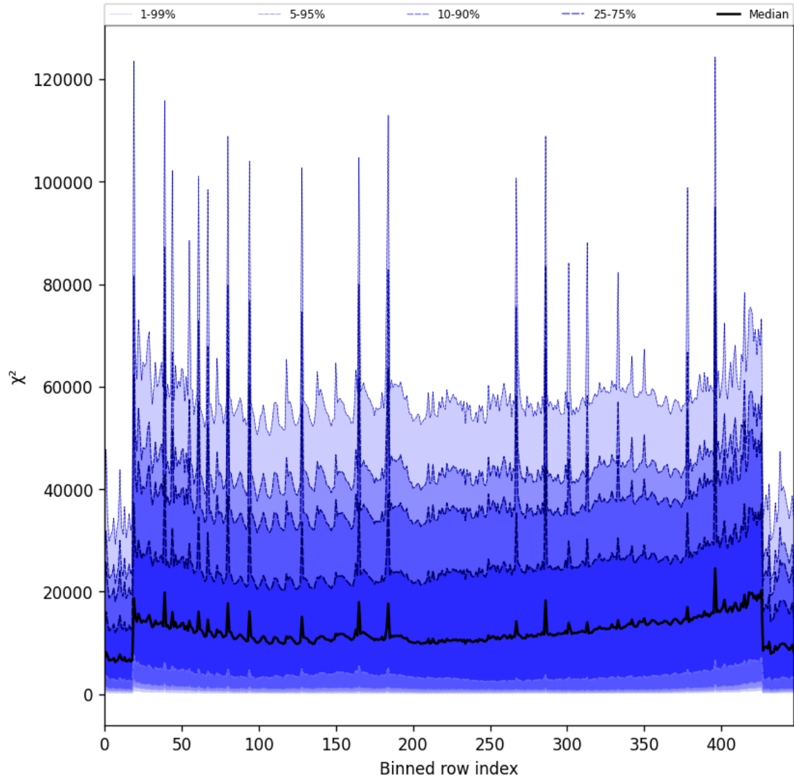
Figure 53: Along track statistics of “ \chi^2 ” for 2025-07-03 to 2025-07-04
