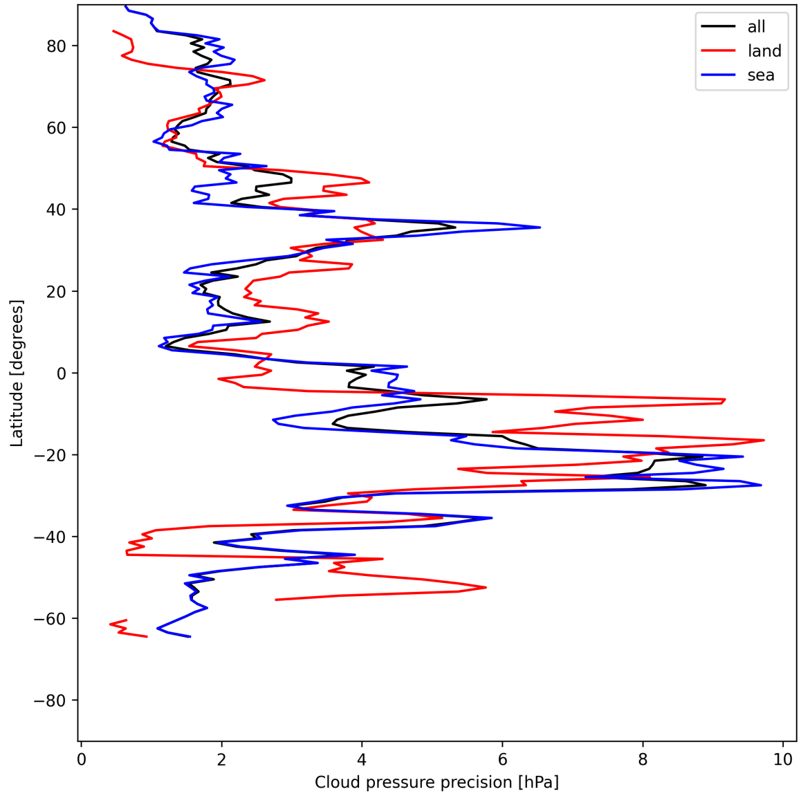
Figure 12: Zonal average of "Cloud pressure precision" for 2025-07-03 to 2025-07-04.
