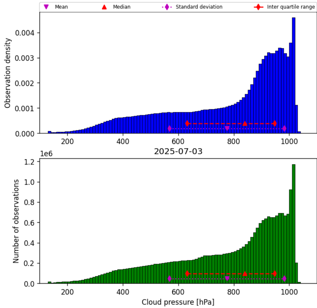
Figure 28: Histogram of “Cloud pressure” for 2025-07-03 to 2025-07-04
