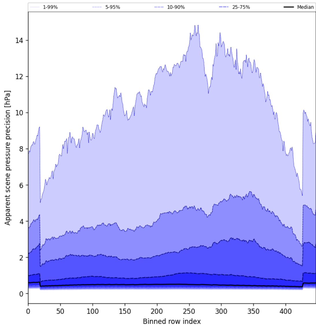
Figure 52: Along track statistics of “Apparent scene pressure precision” for 2025-07-03 to 2025-07-04
