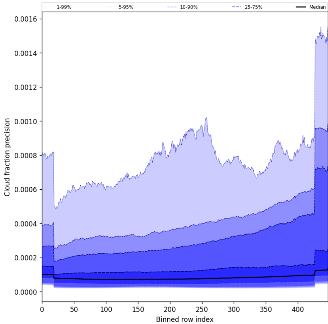
Figure 48: Along track statistics of “Cloud fraction precision” for 2025-07-03 to 2025-07-04
