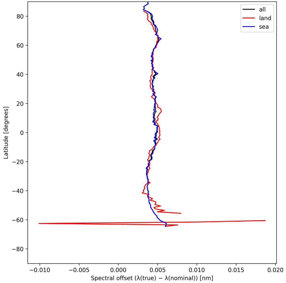
Figure 26: Zonal average of “Spectral offset ( \lambda_{\text{true}} - \lambda_{\text{nominal}} )” for 2025-07-03 to 2025-07-04.
