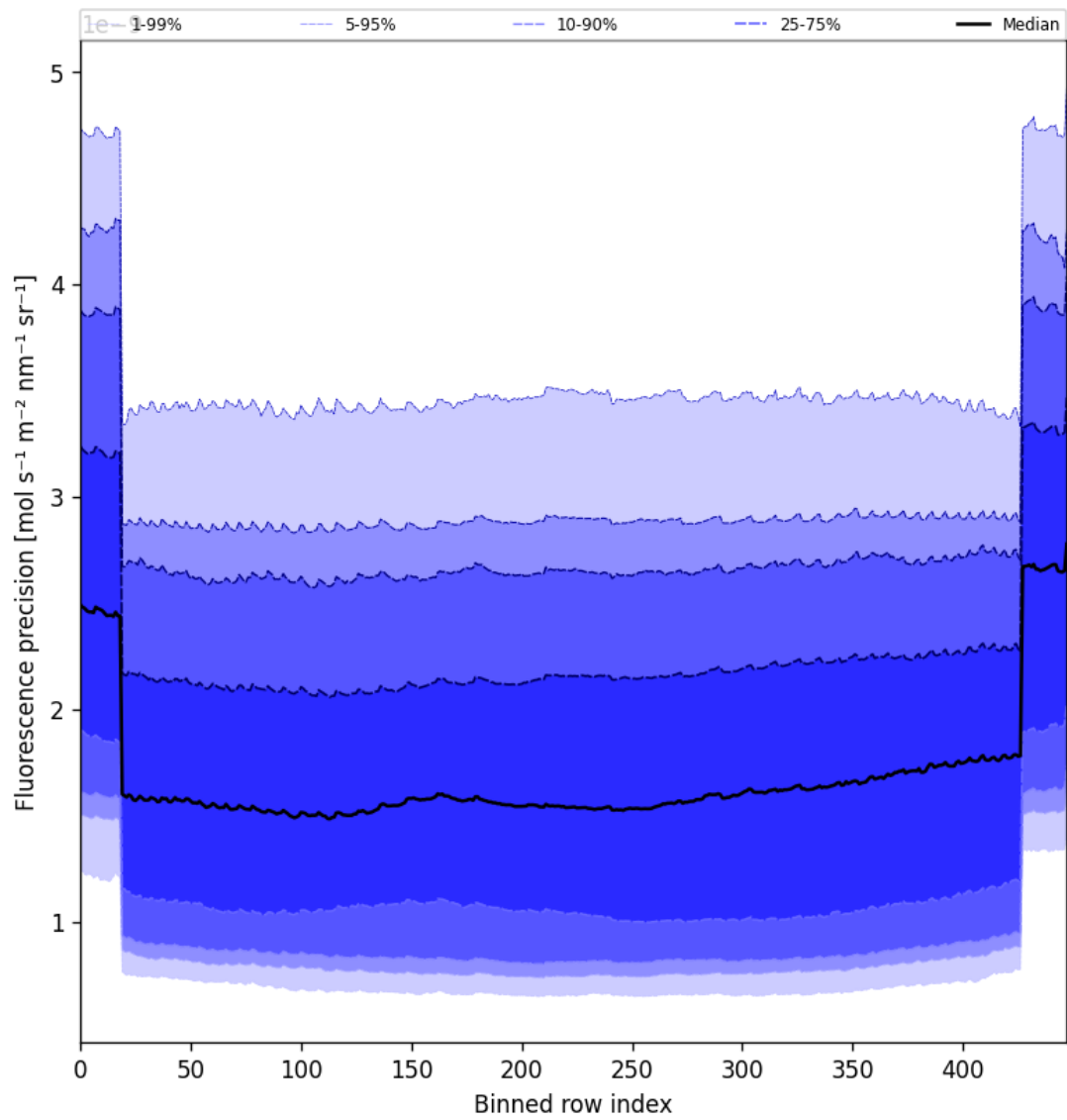
Figure 56: Along track statistics of “Fluorescence precision” for 2025-07-03 to 2025-07-04
