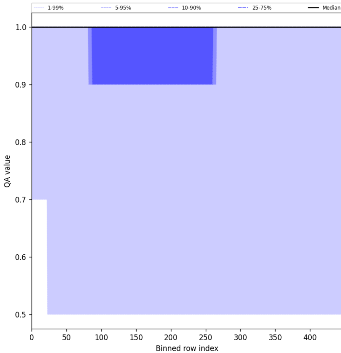
Figure 44: Along track statistics of “QA value” for 2025-07-03 to 2025-07-04
