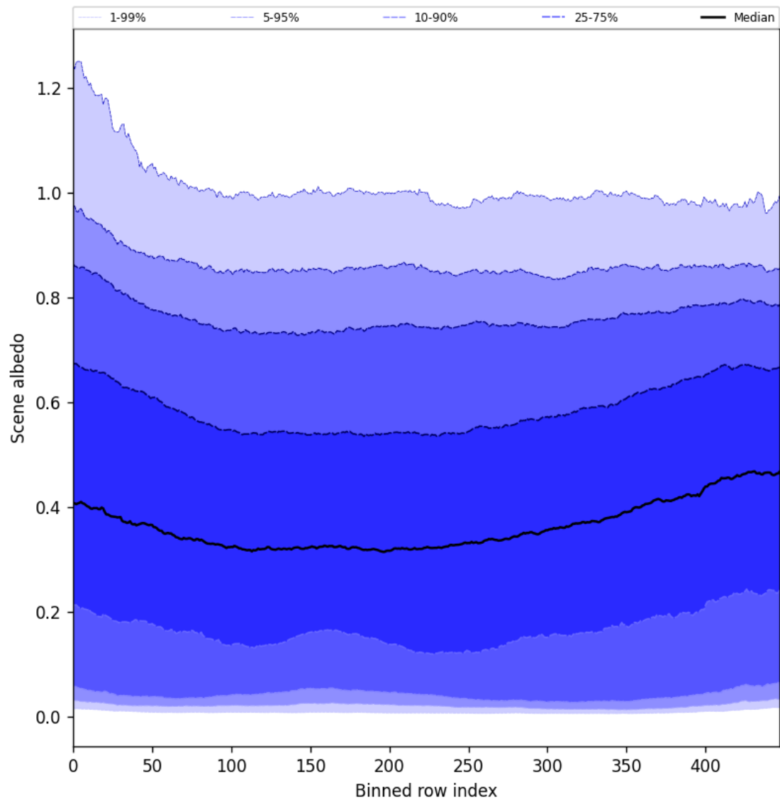
Figure 49: Along track statistics of “Scene albedo” for 2025-07-03 to 2025-07-04
