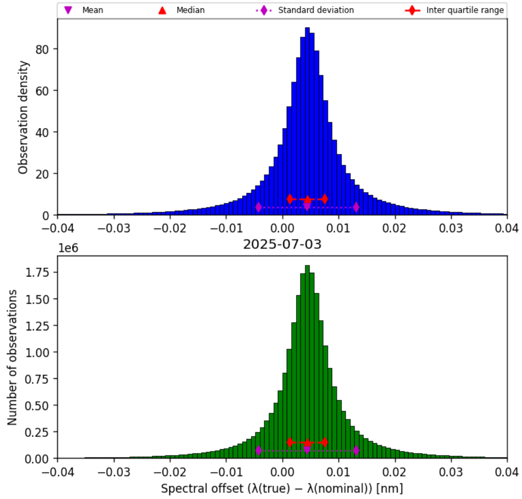
Figure 43: Histogram of “Spectral offset ( \lambda_{\text{true}} - \lambda_{\text{nominal}} )” for 2025-07-03 to 2025-07-04
