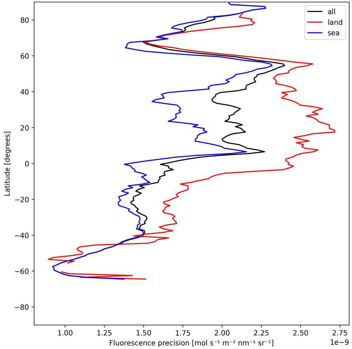
Figure 22: Zonal average of “Fluorescence precision” for 2025-07-03 to 2025-07-04.
