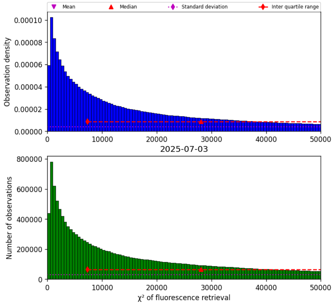
Figure 40: Histogram of “ \chi^2 of fluorescence retrieval” for 2025-07-03 to 2025-07-04
