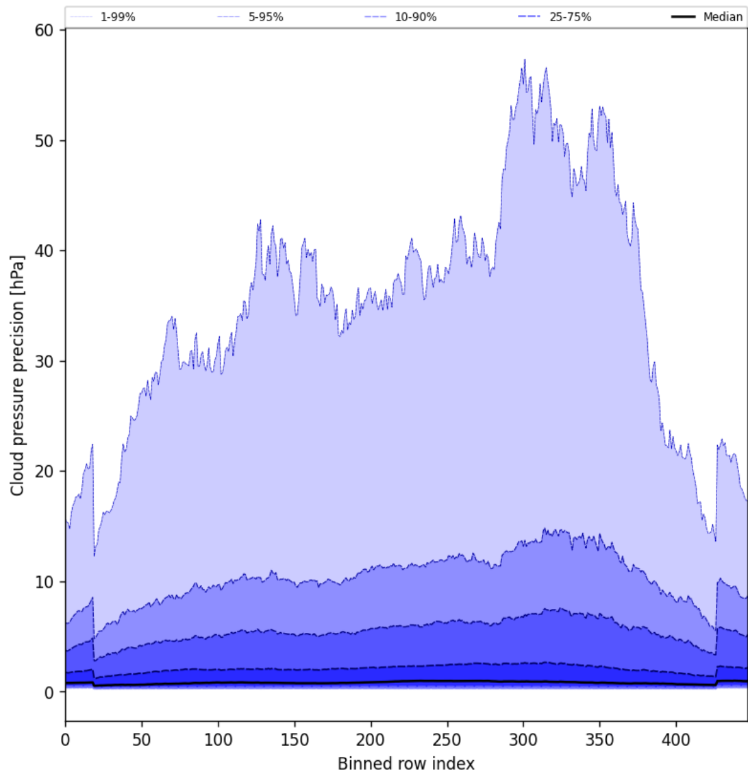
Figure 46: Along track statistics of “Cloud pressure precision” for 2025-07-03 to 2025-07-04
