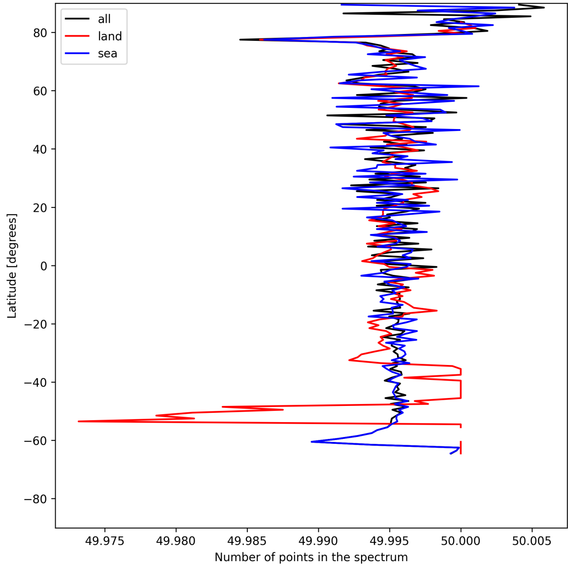
Figure 25: Zonal average of “Number of points in the spectrum” for 2025-07-03 to 2025-07-04.
