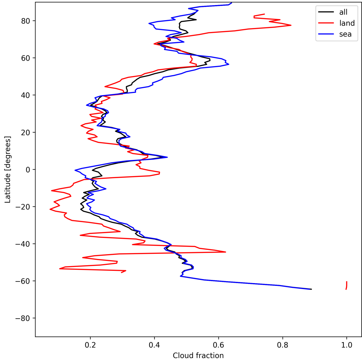
Figure 13: Zonal average of “Cloud fraction” for 2025-07-03 to 2025-07-04.
