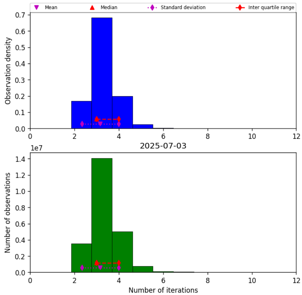
Figure 37: Histogram of “Number of iterations” for 2025-07-03 to 2025-07-04
