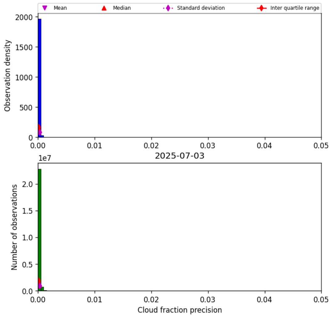
Figure 31: Histogram of “Cloud fraction precision” for 2025-07-03 to 2025-07-04
