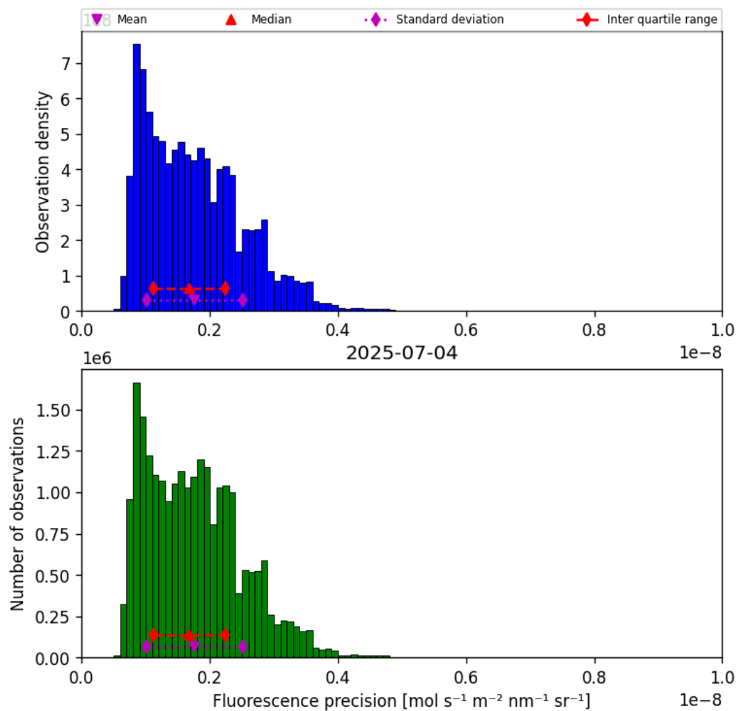
Figure 39: Histogram of “Fluorescence precision” for 2025-07-04 to 2025-07-05
