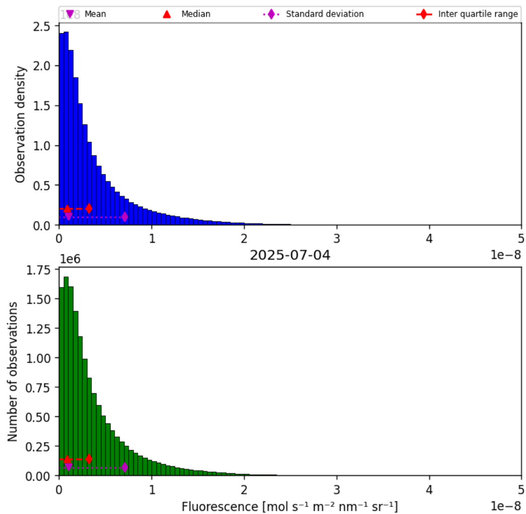
Figure 38: Histogram of “Fluorescence” for 2025-07-04 to 2025-07-05
