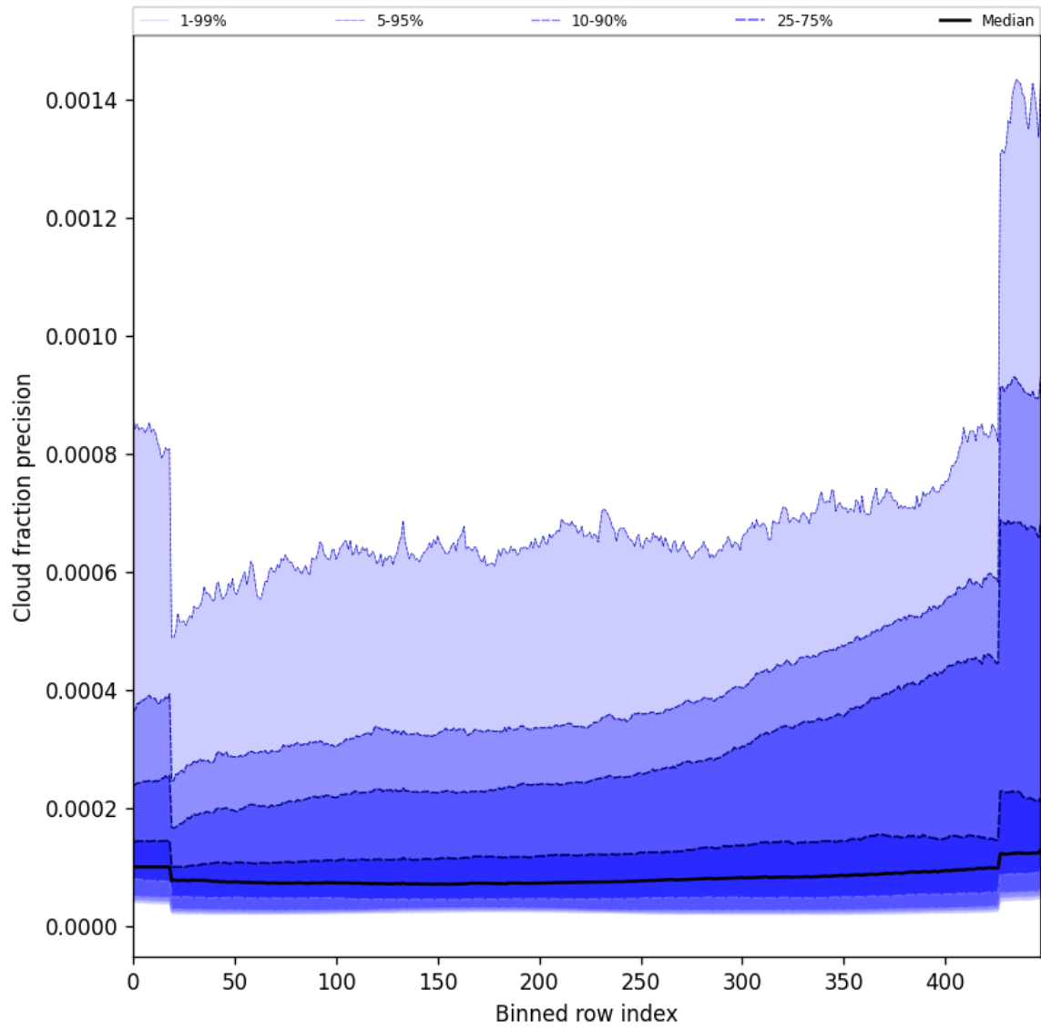
Figure 48: Along track statistics of “Cloud fraction precision” for 2025-07-04 to 2025-07-05
