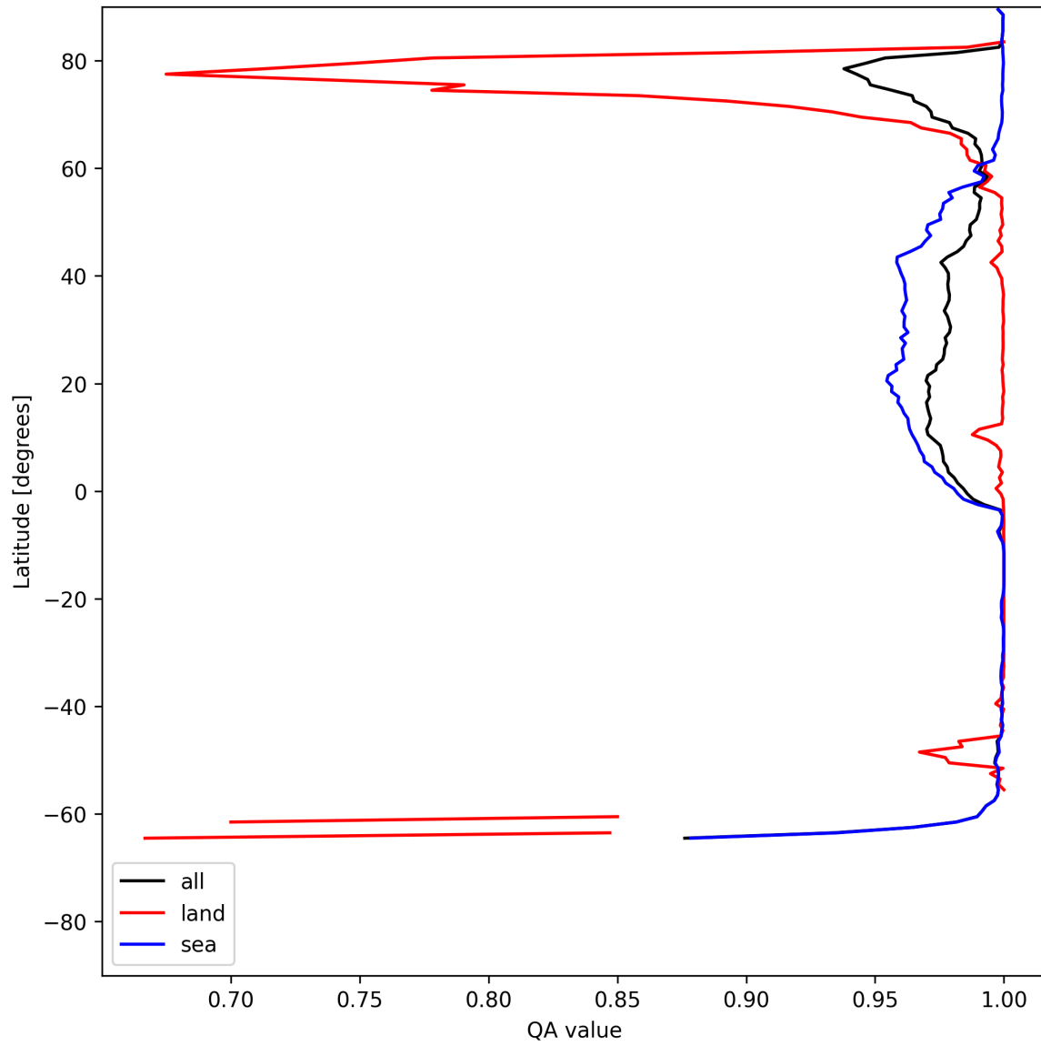
Figure 10: Zonal average of “QA value” for 2025-07-04 to 2025-07-05.
