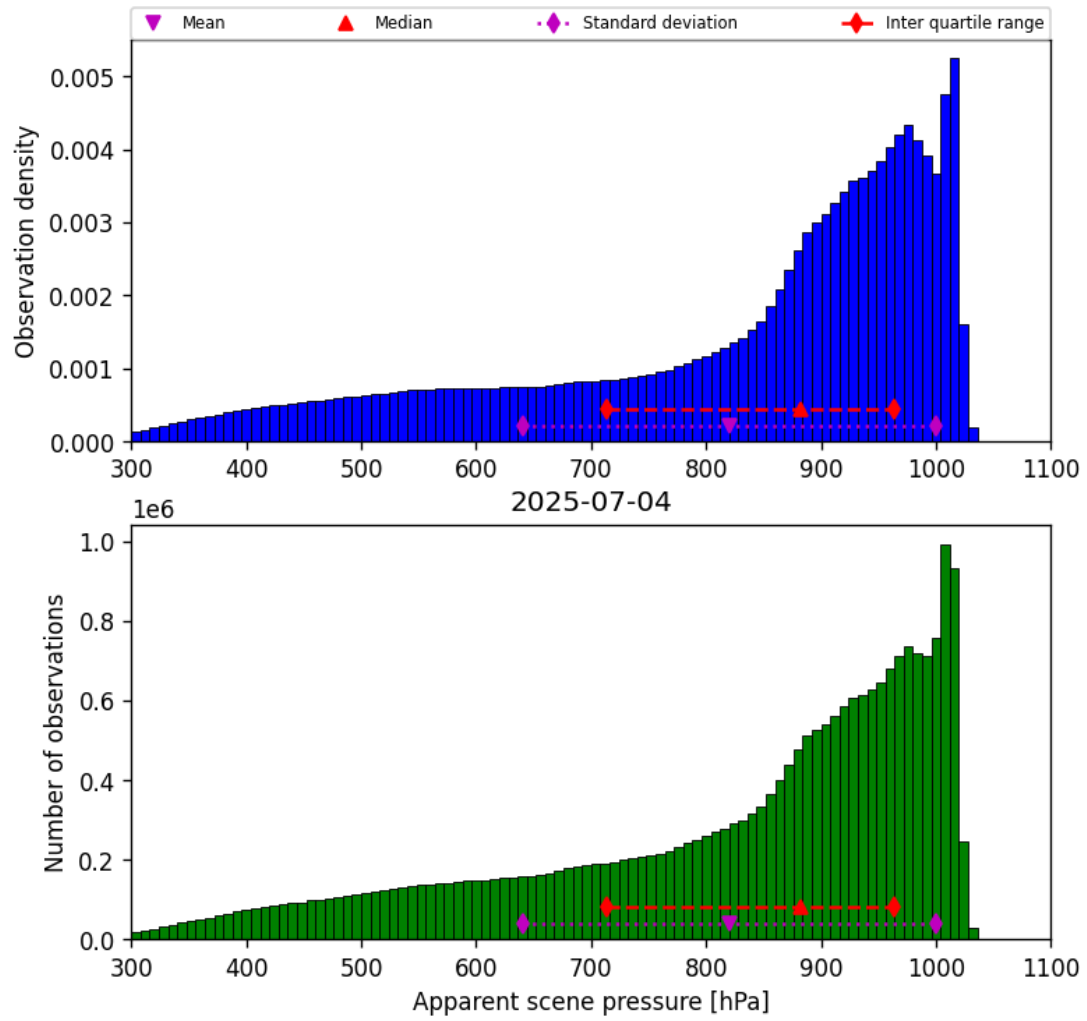
Figure 34: Histogram of “Apparent scene pressure” for 2025-07-04 to 2025-07-05
