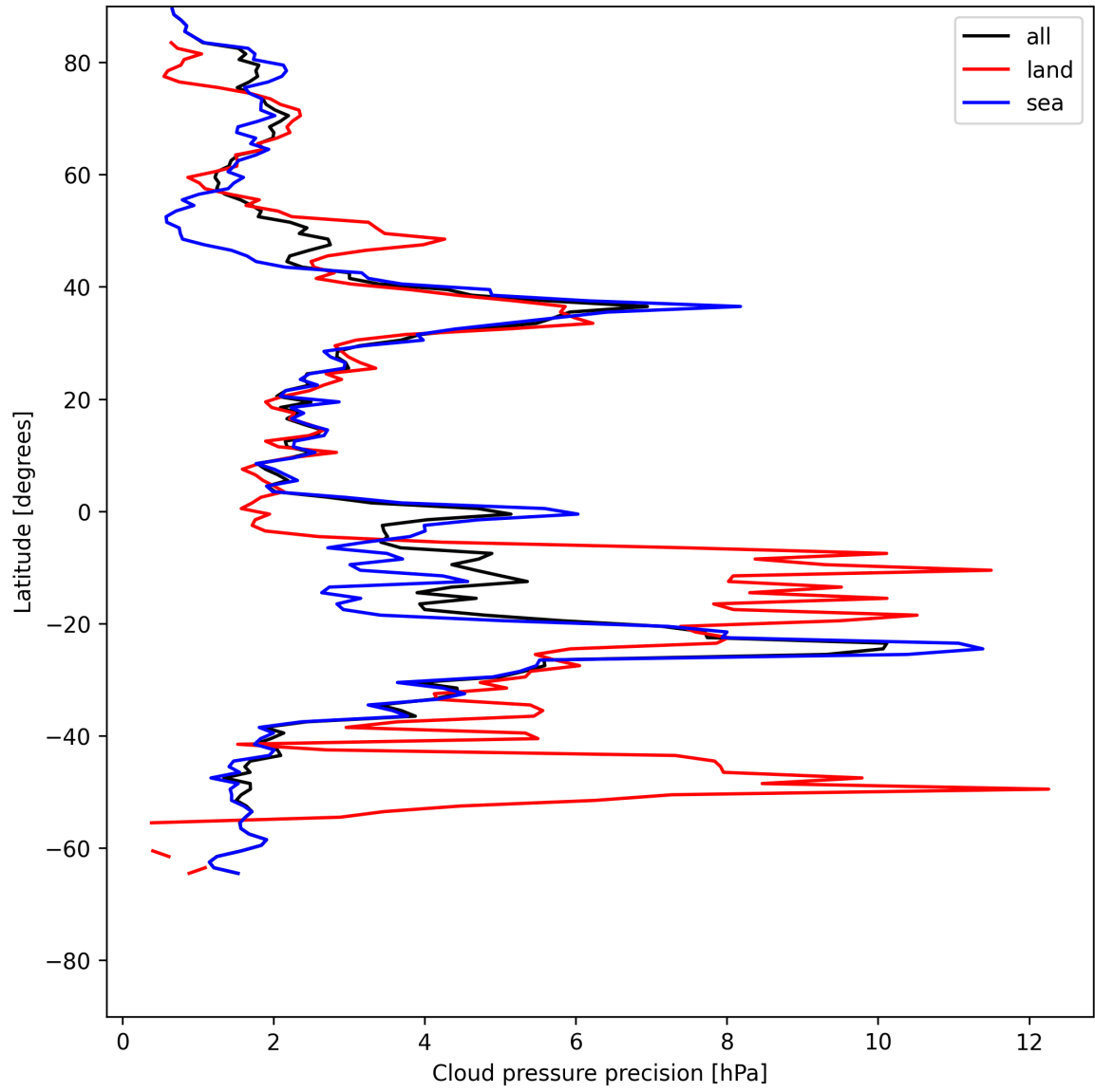
Figure 12: Zonal average of “Cloud pressure precision” for 2025-07-04 to 2025-07-05.
