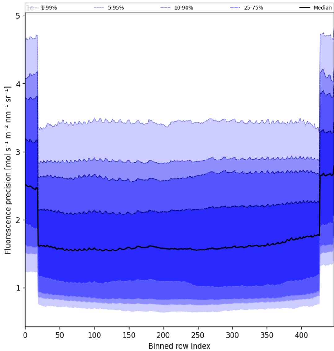
Figure 56: Along track statistics of “Fluorescence precision” for 2025-07-04 to 2025-07-05
