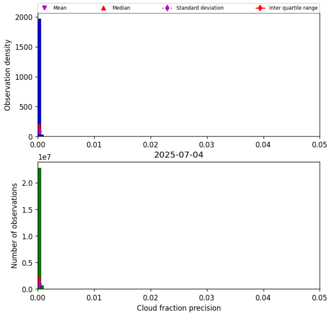
Figure 31: Histogram of “Cloud fraction precision” for 2025-07-04 to 2025-07-05
