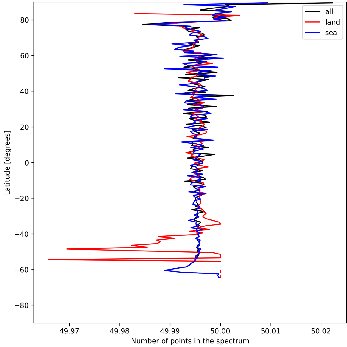
Figure 25: Zonal average of “Number of points in the spectrum” for 2025-07-04 to 2025-07-05.
