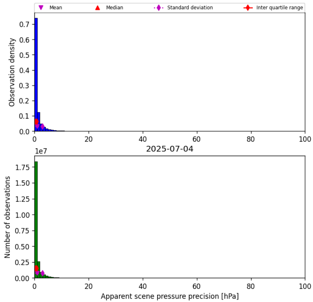
Figure 35: Histogram of “Apparent scene pressure precision” for 2025-07-04 to 2025-07-05
