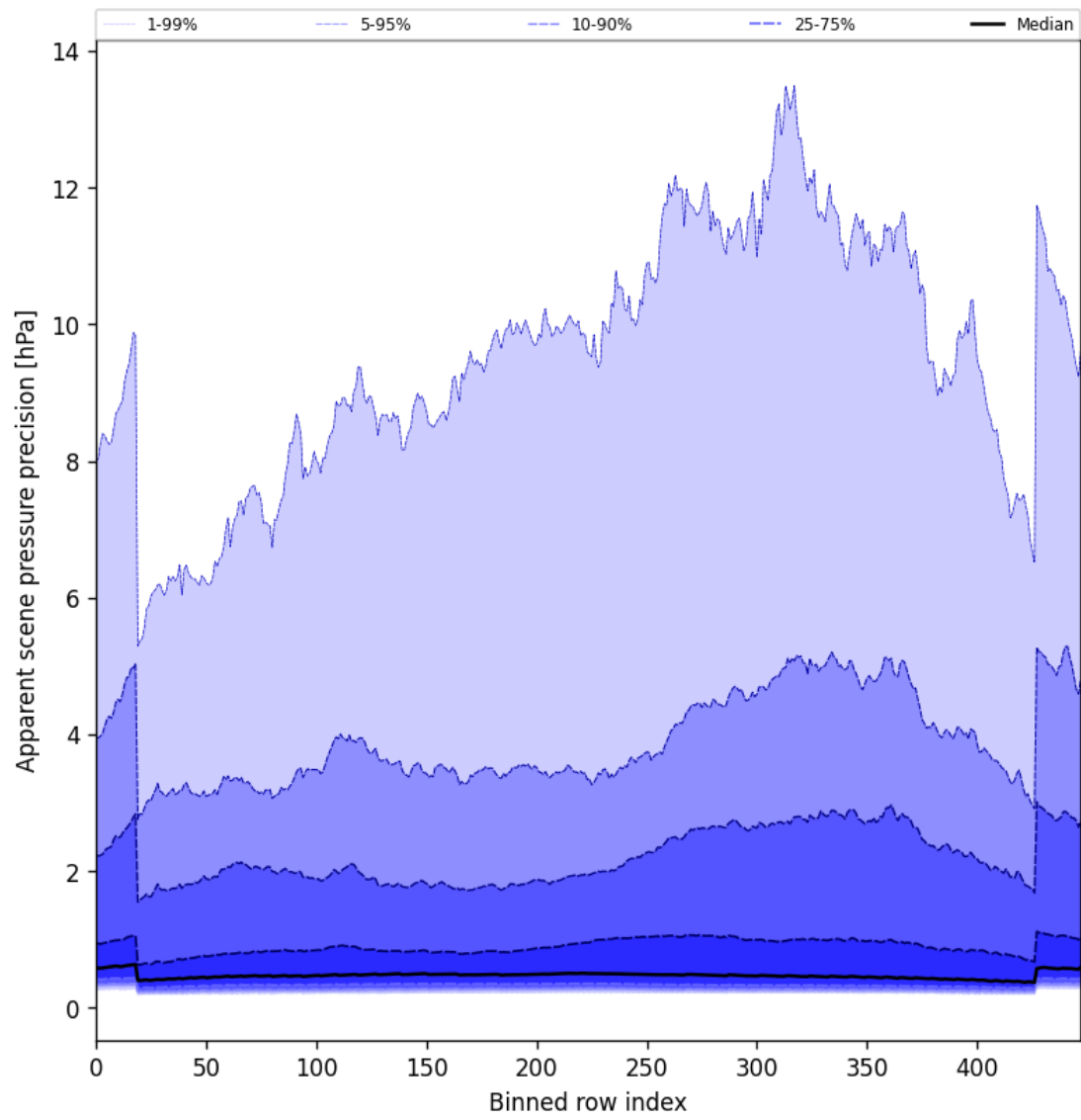
Figure 52: Along track statistics of “Apparent scene pressure precision” for 2025-07-04 to 2025-07-05
