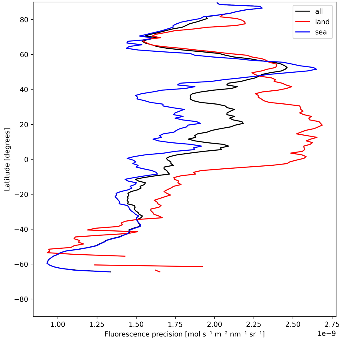
Figure 22: Zonal average of “Fluorescence precision” for 2025-07-04 to 2025-07-05.
