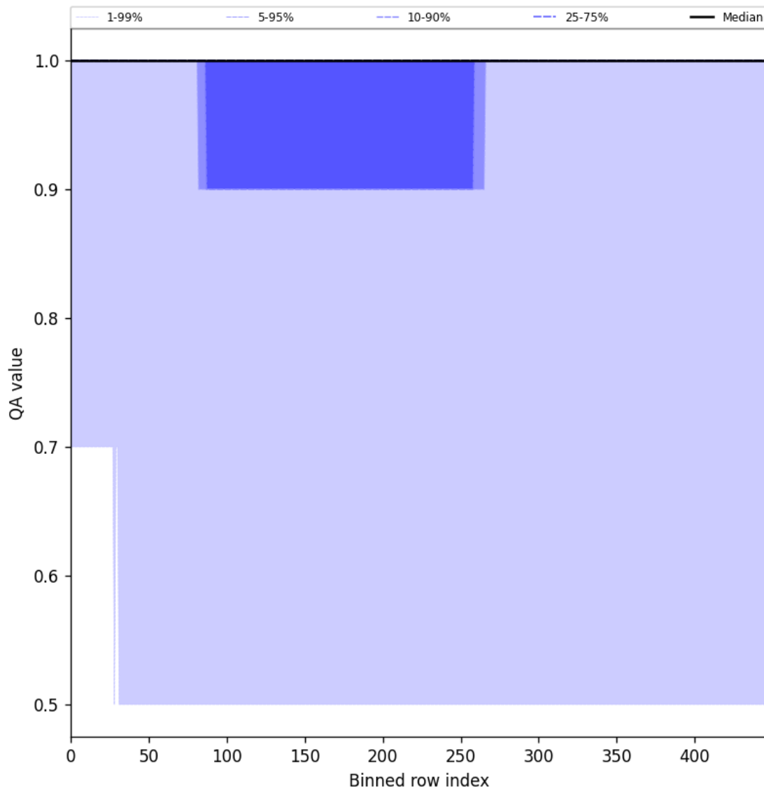
Figure 44: Along track statistics of “QA value” for 2025-07-04 to 2025-07-05
