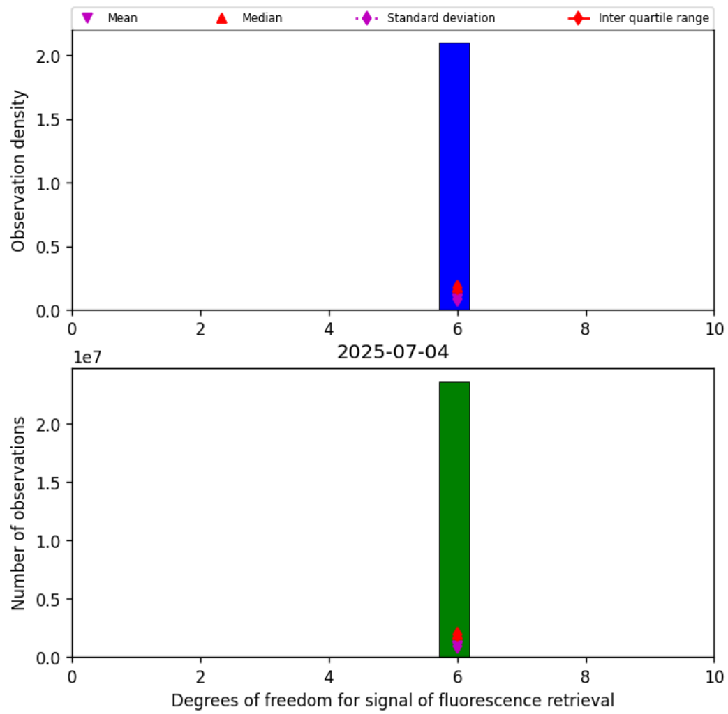
Figure 41: Histogram of “Degrees of freedom for signal of fluorescence retrieval” for 2025-07-04 to 2025-07-05
