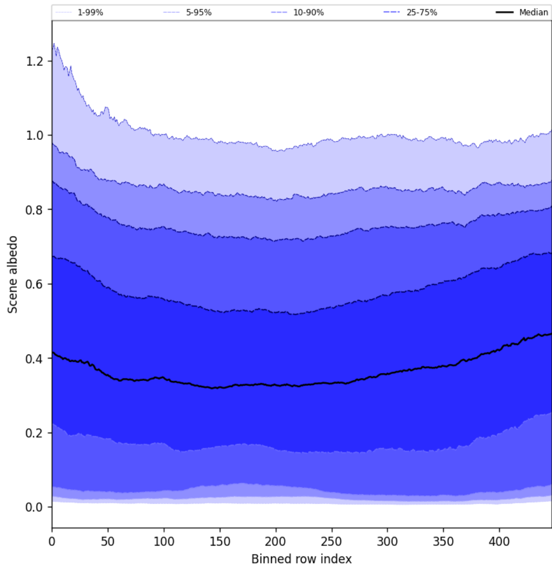
Figure 49: Along track statistics of “Scene albedo” for 2025-07-04 to 2025-07-05
