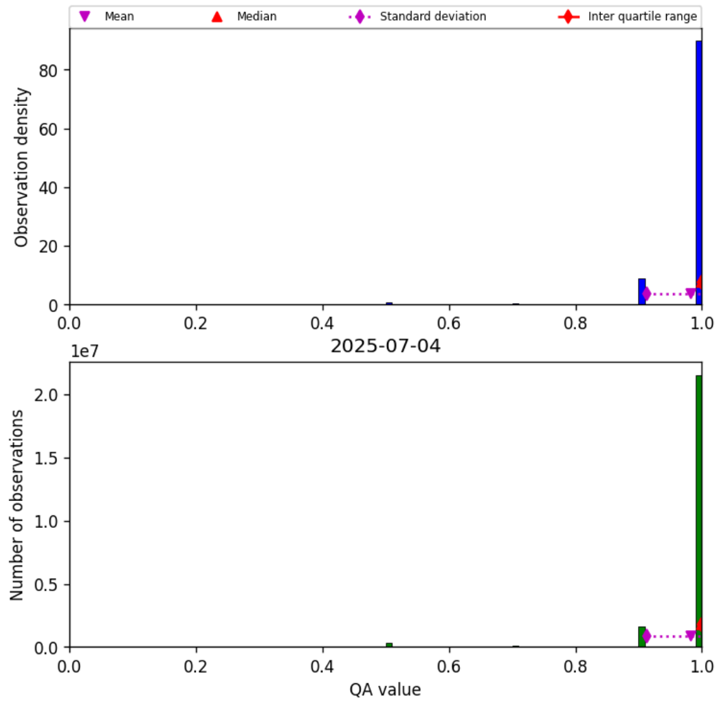
Figure 27: Histogram of “QA value” for 2025-07-04 to 2025-07-05
