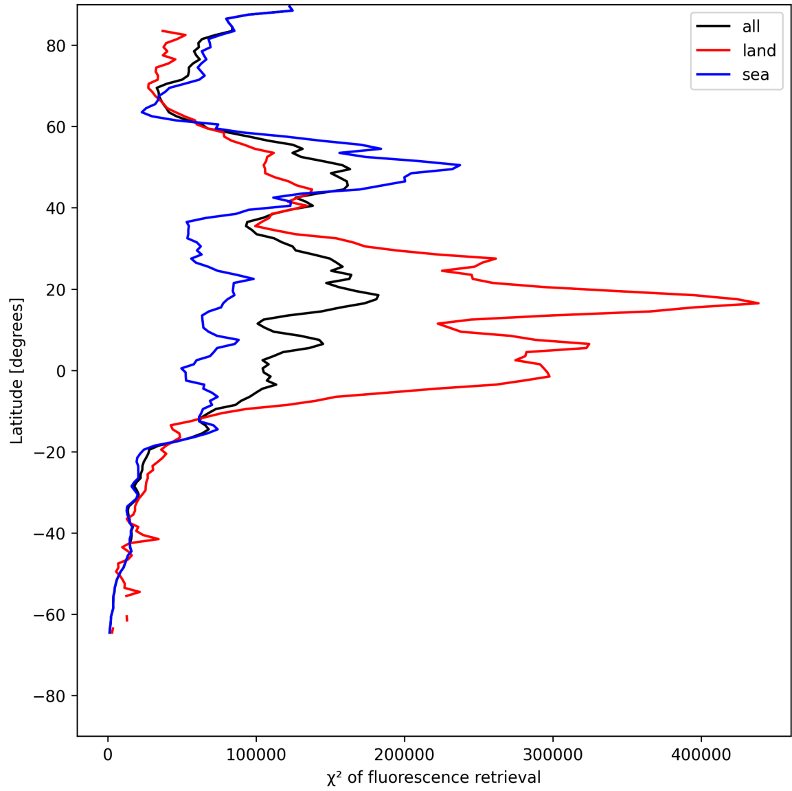
Figure 23: Zonal average of “ \chi^2 of fluorescence retrieval” for 2025-07-04 to 2025-07-05.
