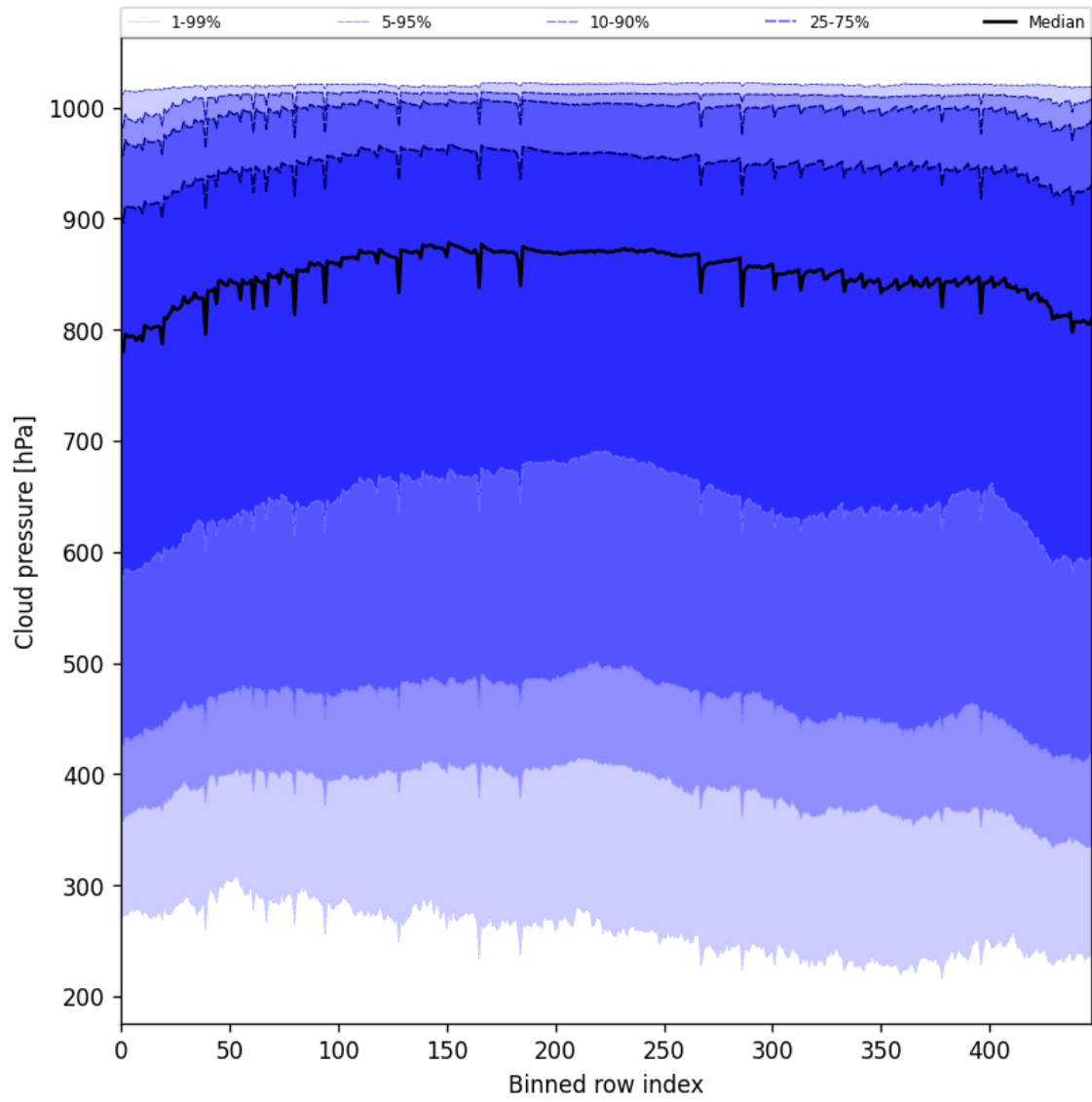
Figure 45: Along track statistics of “Cloud pressure” for 2025-07-04 to 2025-07-05
