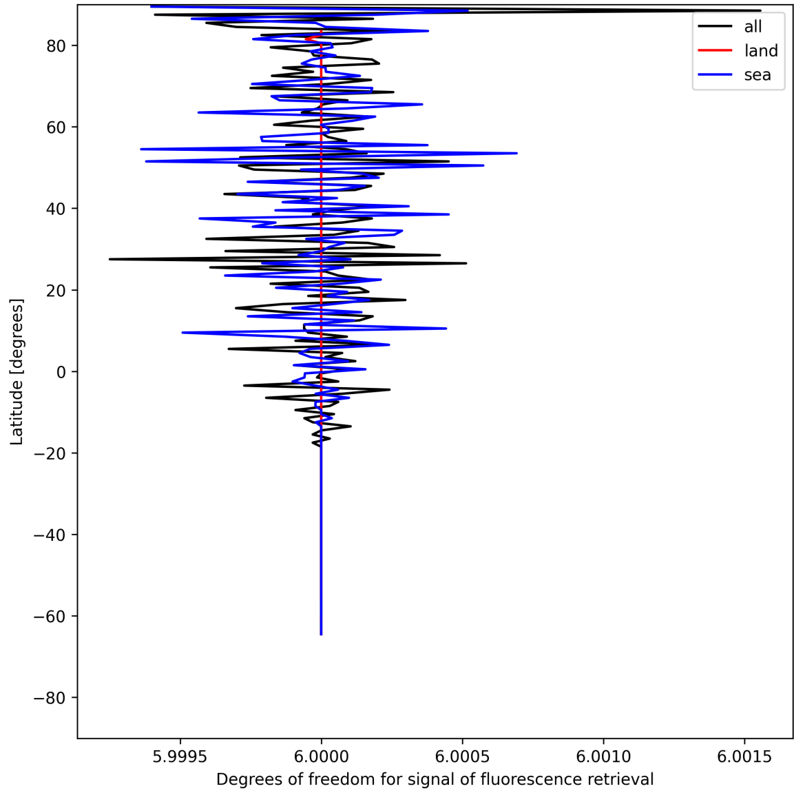
Figure 24: Zonal average of “Degrees of freedom for signal of fluorescence retrieval” for 2025-07-04 to 2025-07-05.
