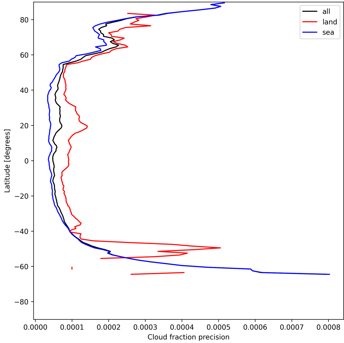
Figure 14: Zonal average of “Cloud fraction precision” for 2025-07-04 to 2025-07-05.
