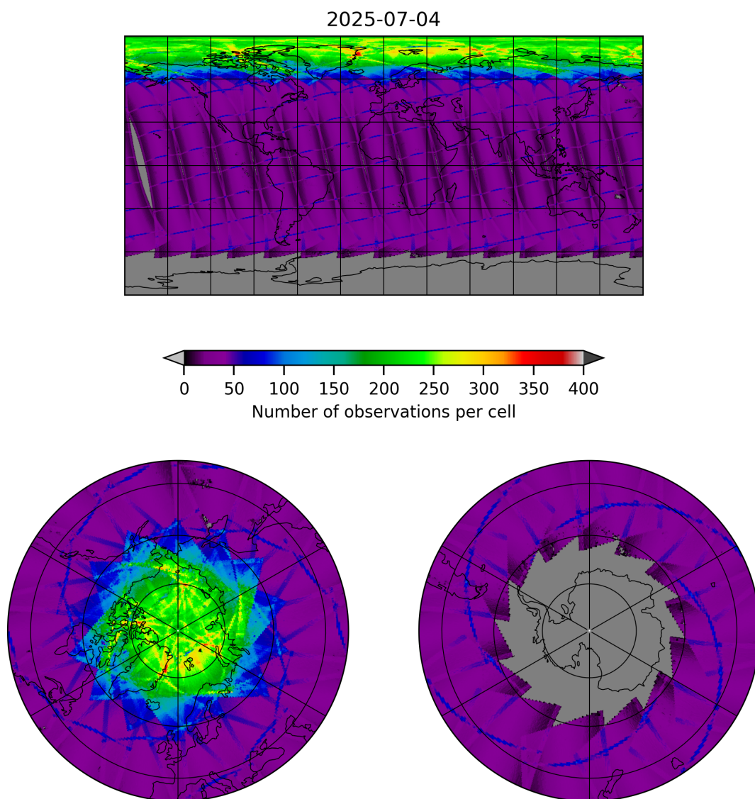
Figure 9: Map of the number of observations for 2025-07-04 to 2025-07-05
