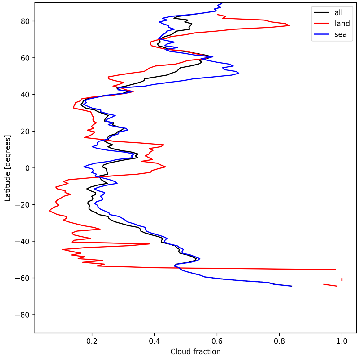
Figure 13: Zonal average of “Cloud fraction” for 2025-07-04 to 2025-07-05.
