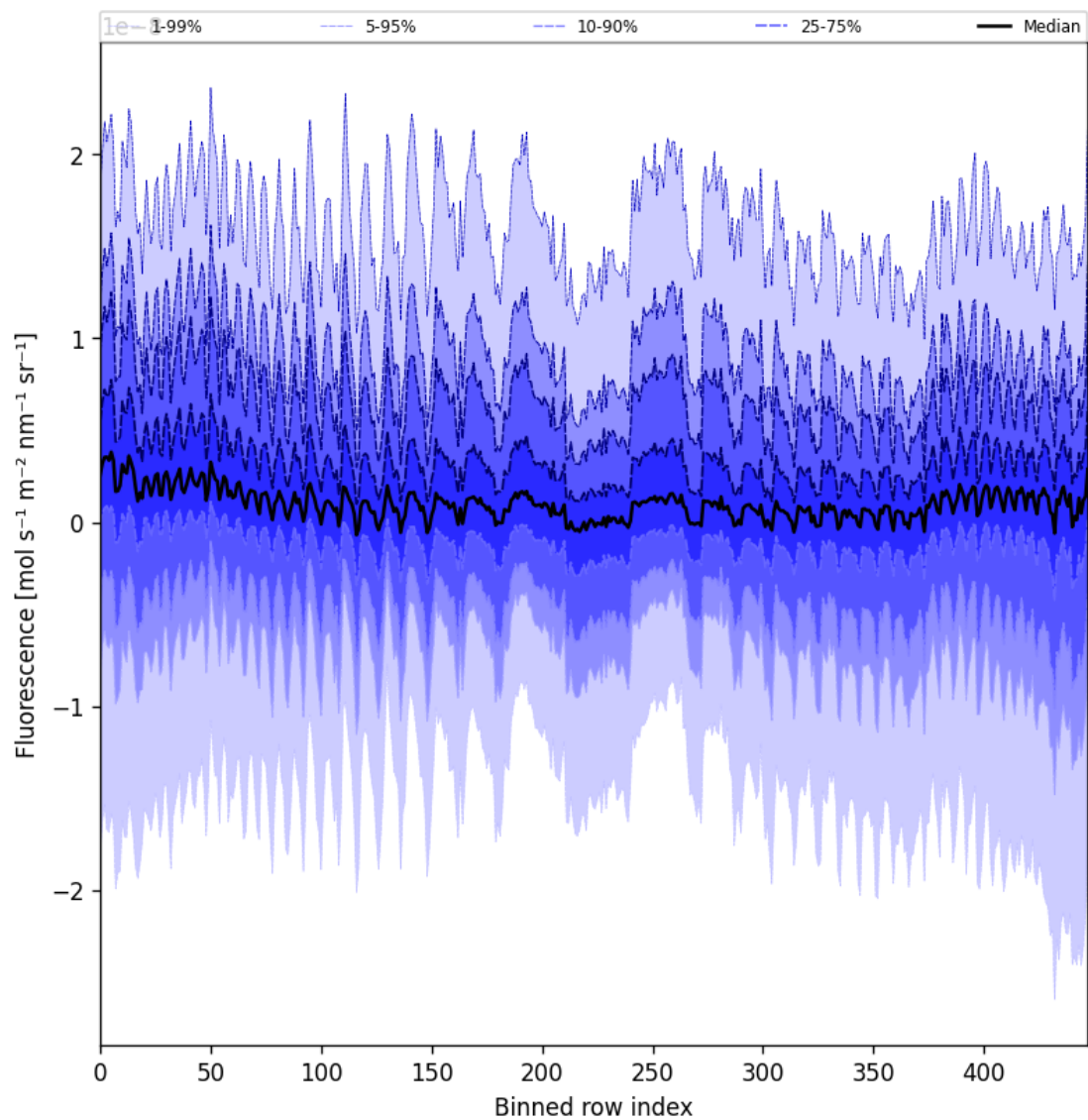
Figure 55: Along track statistics of “Fluorescence” for 2025-07-04 to 2025-07-05
