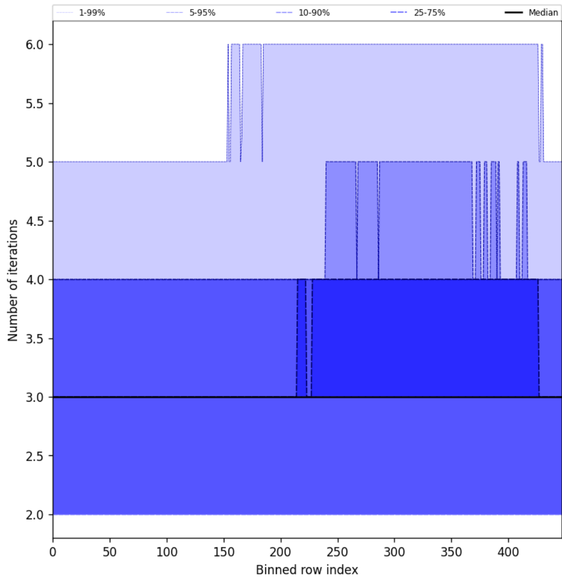
Figure 54: Along track statistics of “Number of iterations” for 2025-07-04 to 2025-07-05
