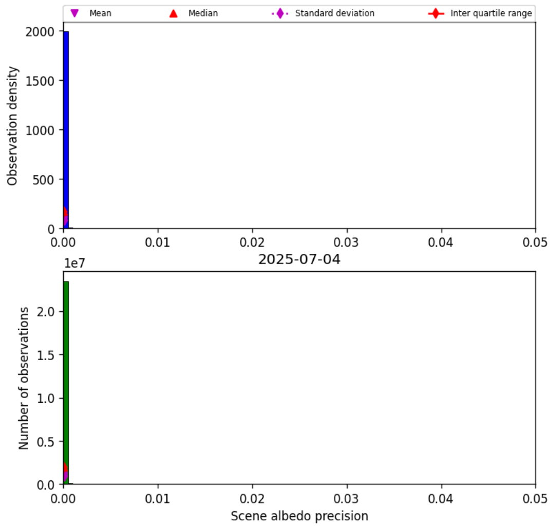
Figure 33: Histogram of “Scene albedo precision” for 2025-07-04 to 2025-07-05
