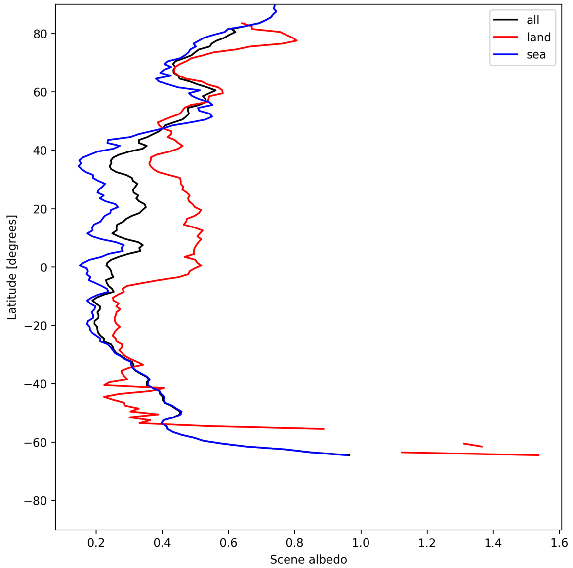
Figure 15: Zonal average of “Scene albedo” for 2025-07-04 to 2025-07-05.
