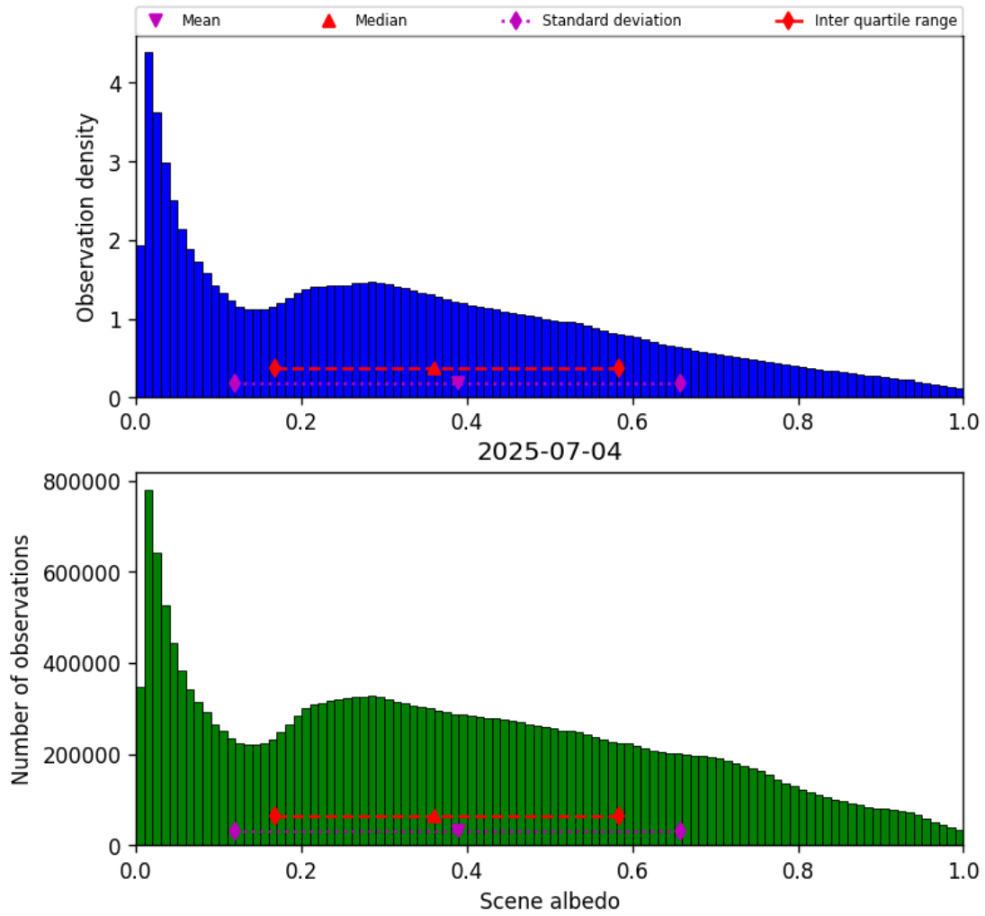
Figure 32: Histogram of “Scene albedo” for 2025-07-04 to 2025-07-05
