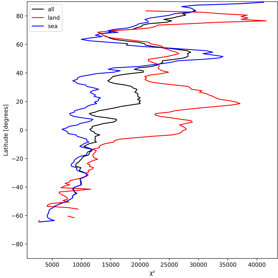
Figure 19: Zonal average of “ \chi^2 ” for 2025-07-04 to 2025-07-05.
