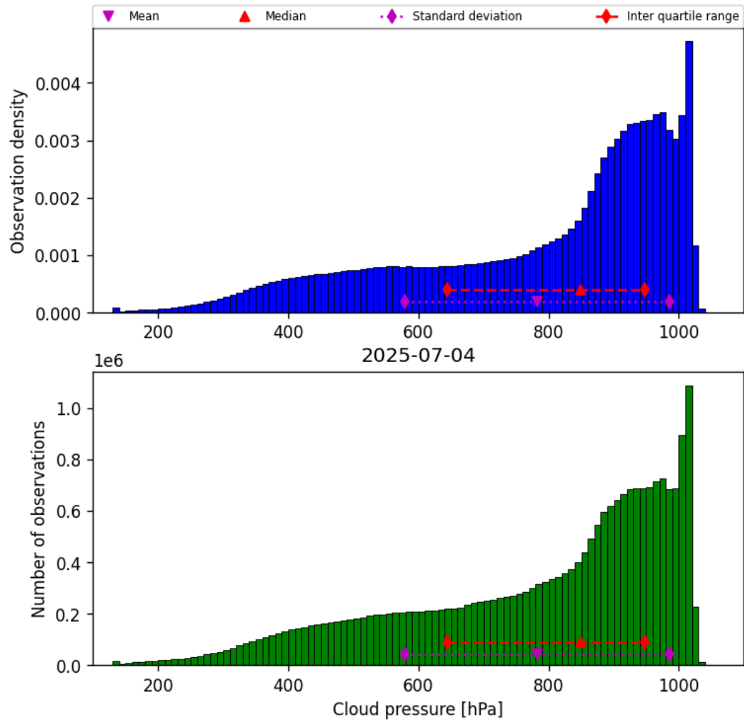
Figure 28: Histogram of “Cloud pressure” for 2025-07-04 to 2025-07-05
