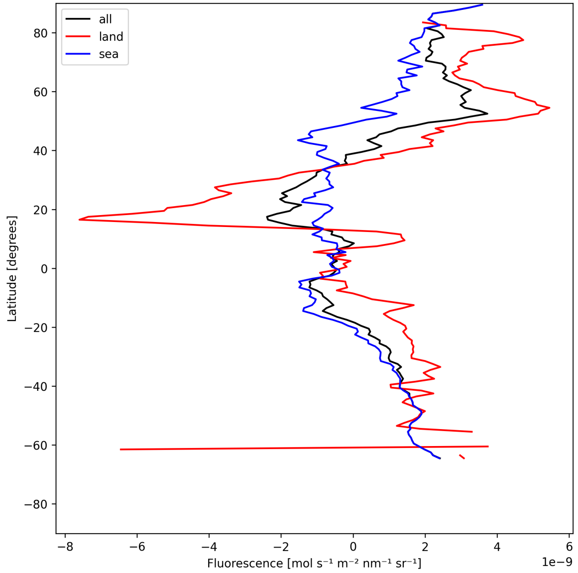
Figure 21: Zonal average of “Fluorescence” for 2025-07-04 to 2025-07-05.
