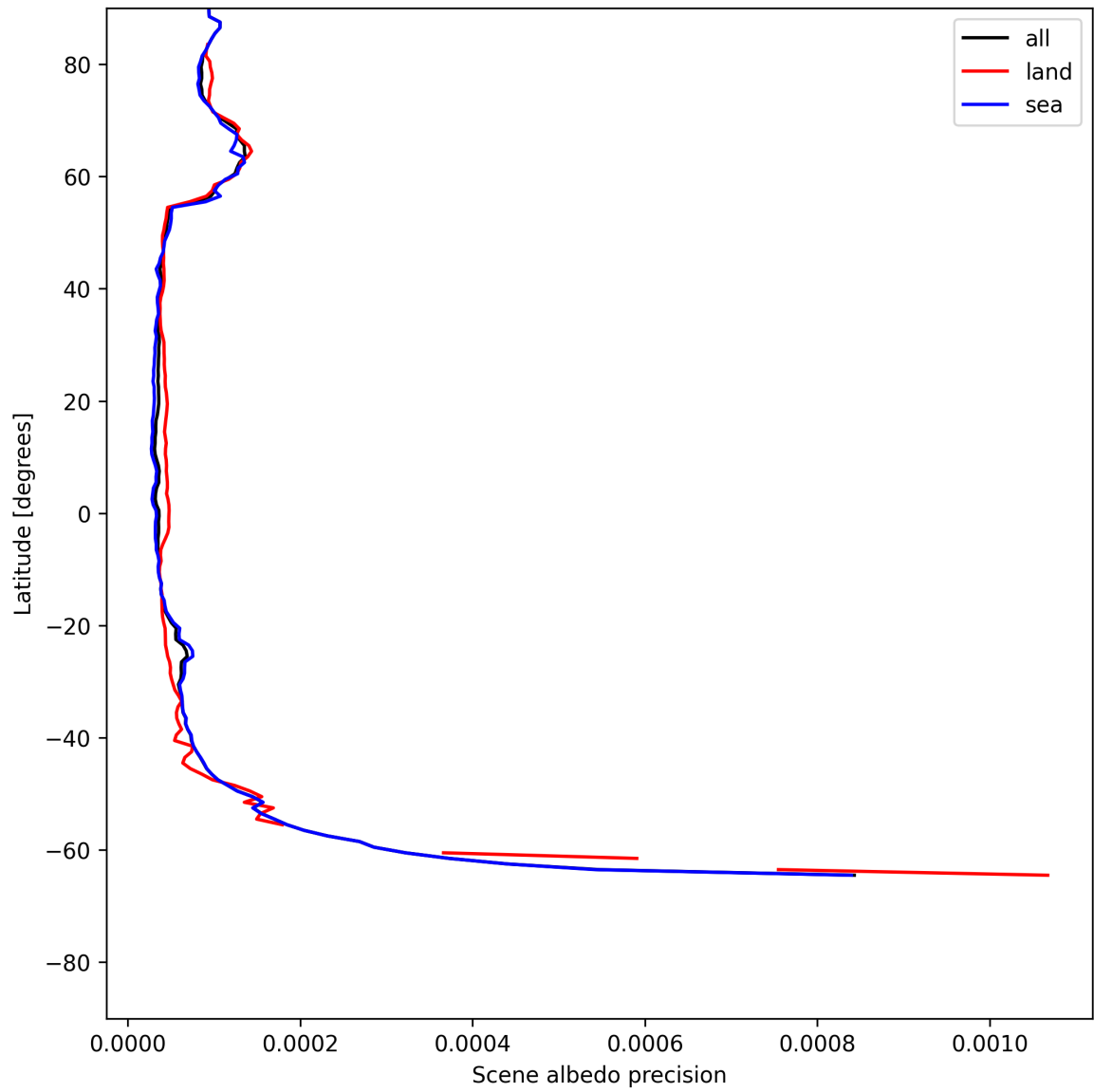
Figure 16: Zonal average of “Scene albedo precision” for 2025-07-04 to 2025-07-05.
