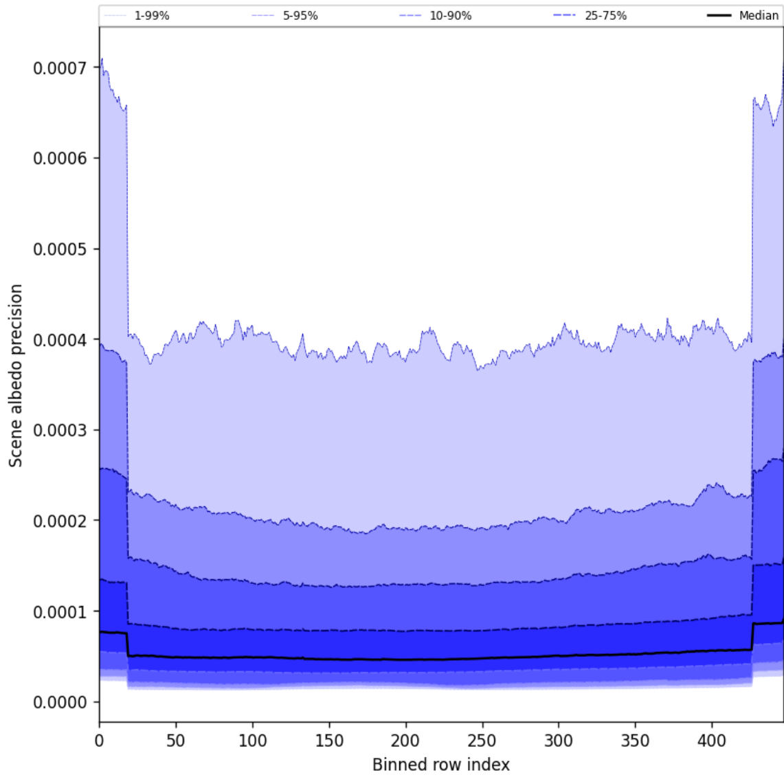
Figure 50: Along track statistics of “Scene albedo precision” for 2025-07-04 to 2025-07-05
