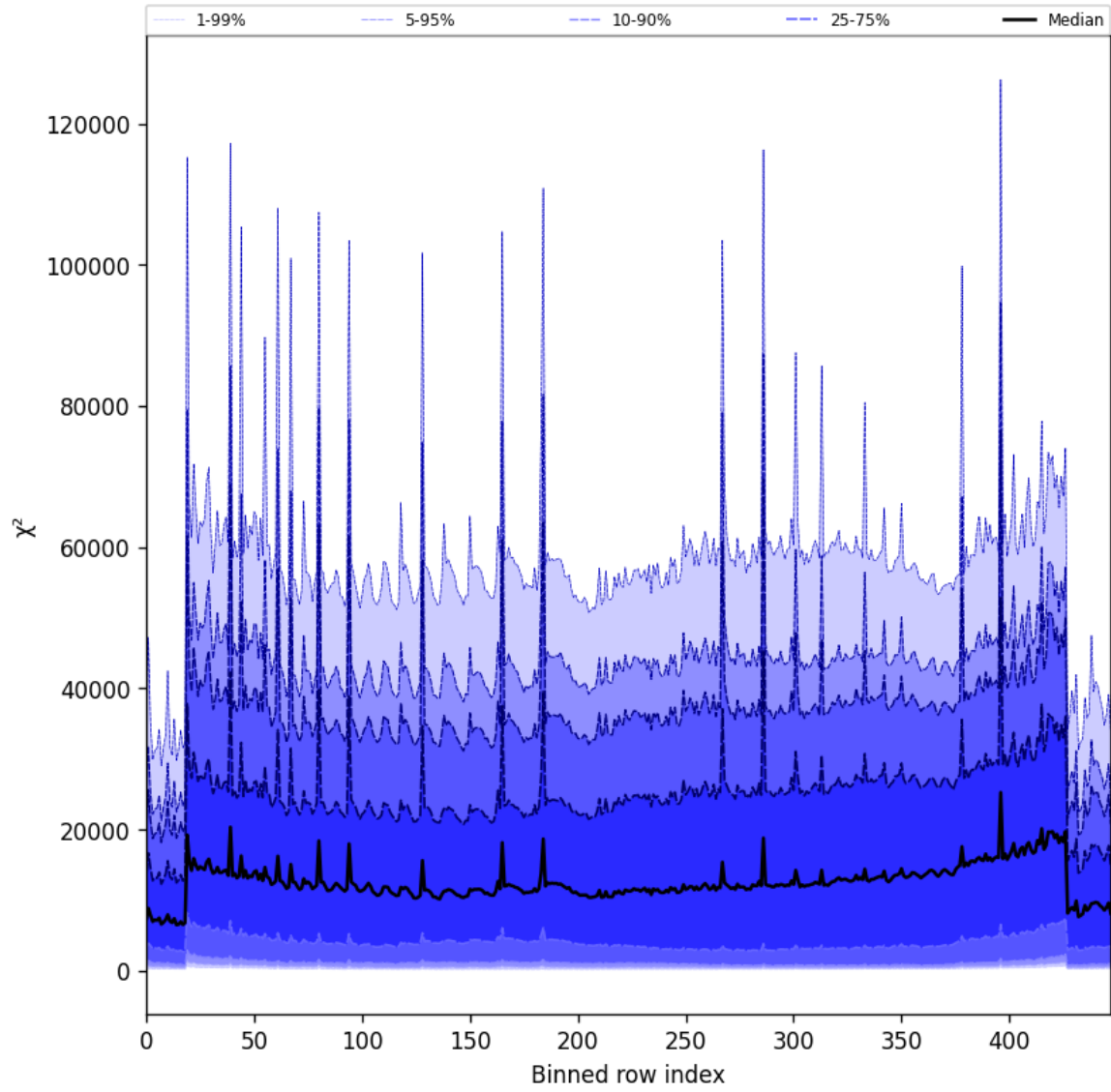
Figure 53: Along track statistics of “ \chi^2 ” for 2025-07-04 to 2025-07-05
