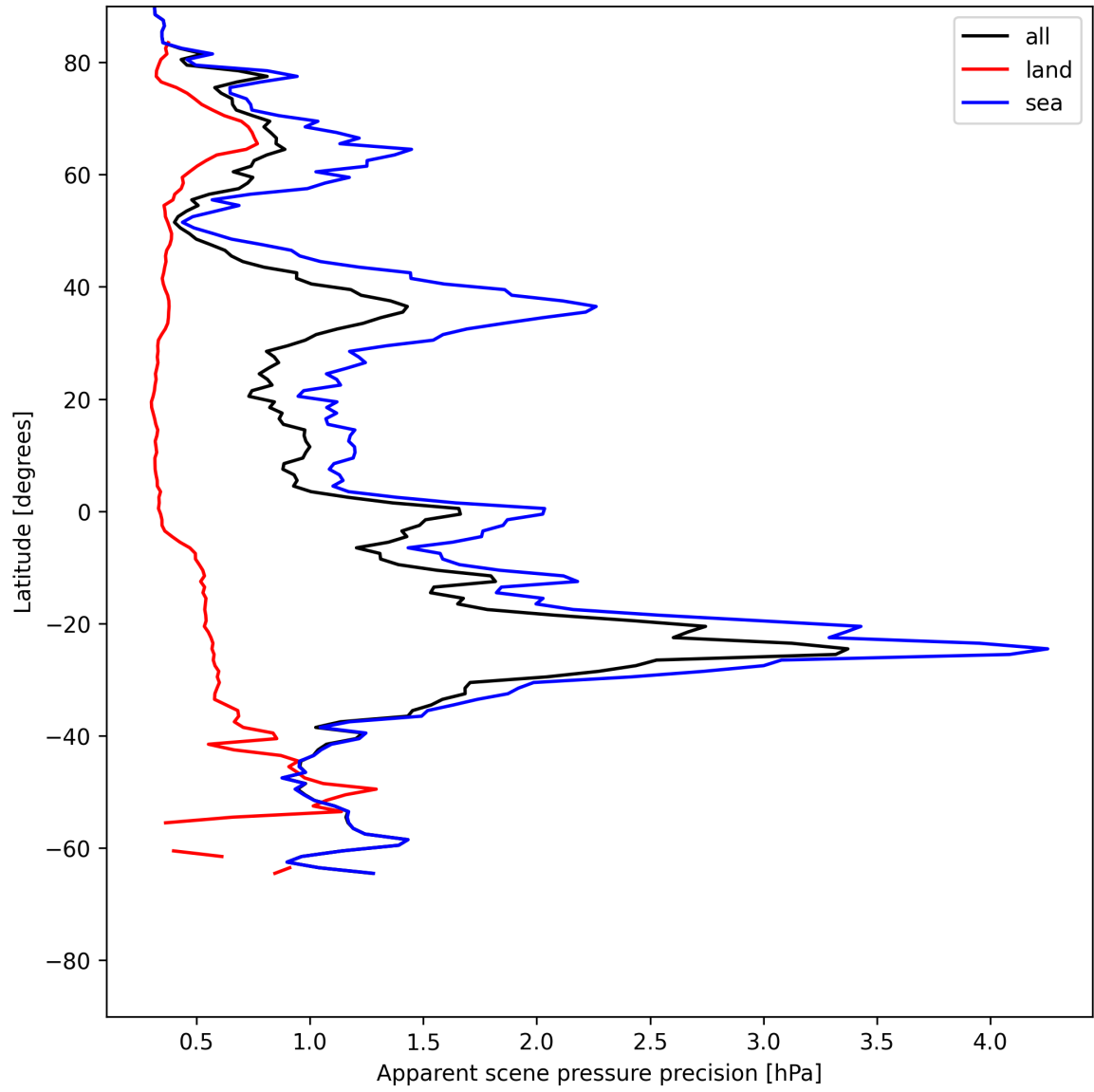
Figure 18: Zonal average of “Apparent scene pressure precision” for 2025-07-04 to 2025-07-05.
