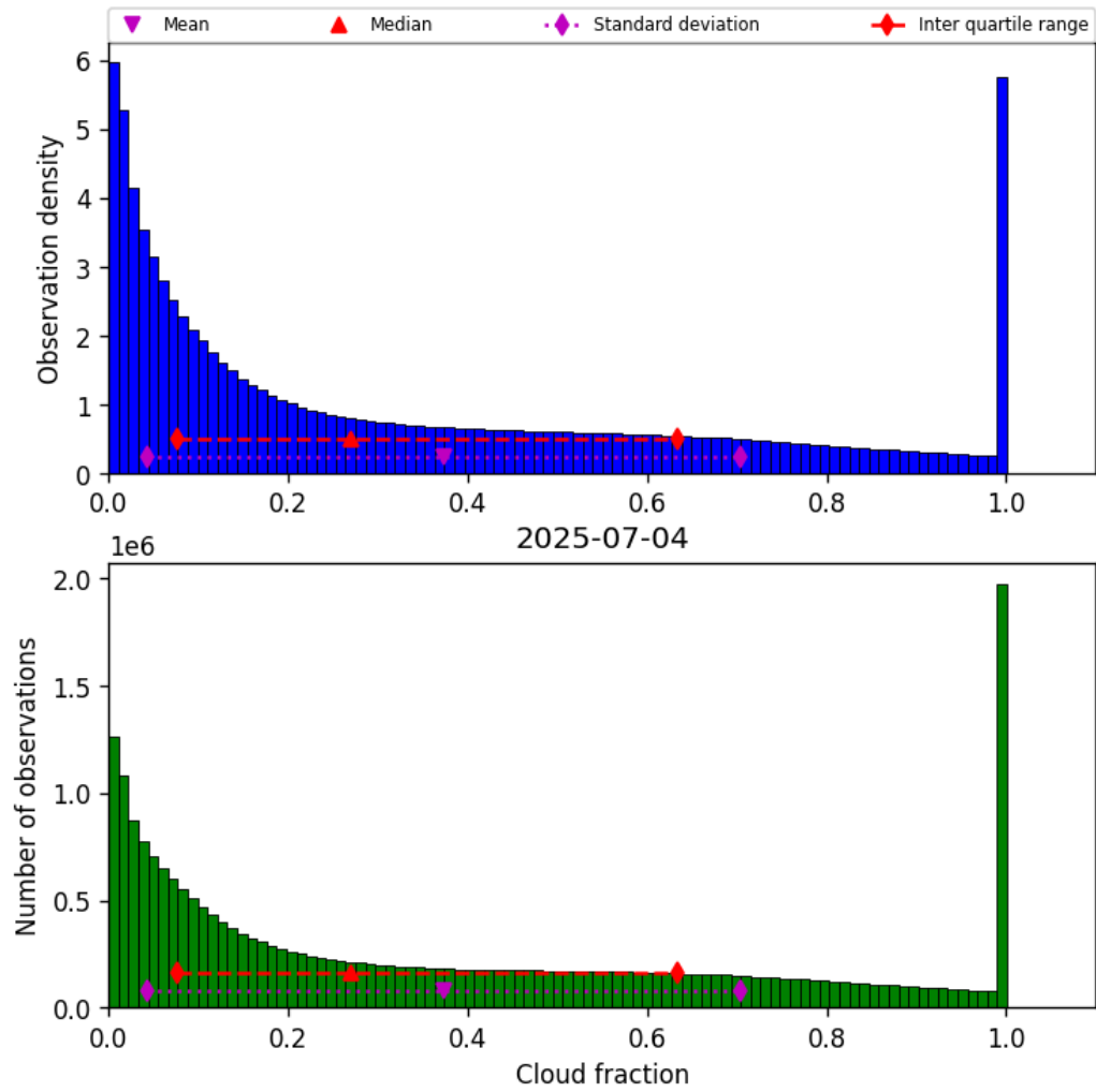
Figure 30: Histogram of “Cloud fraction” for 2025-07-04 to 2025-07-05
