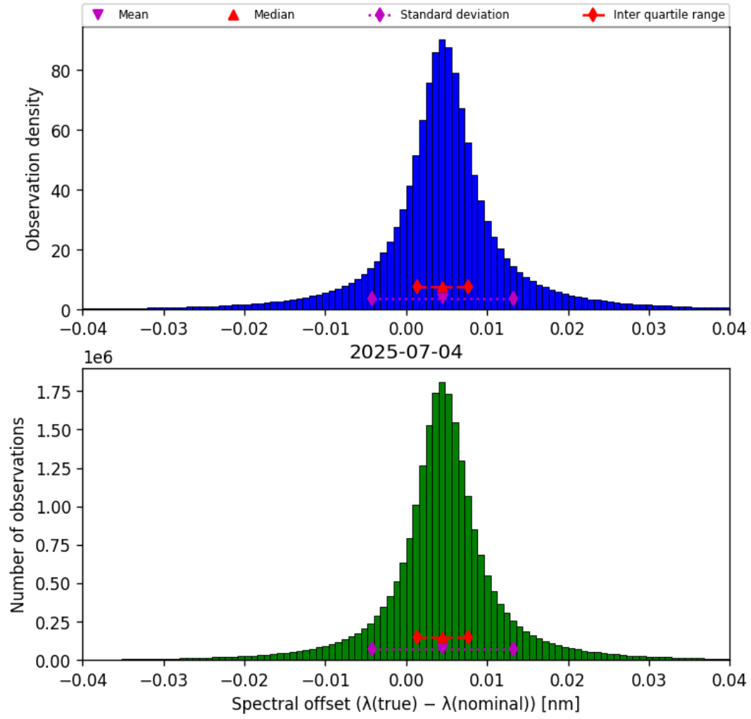
Figure 43: Histogram of “Spectral offset ( \lambda_{\text{true}} - \lambda_{\text{nominal}} )” for 2025-07-04 to 2025-07-05
