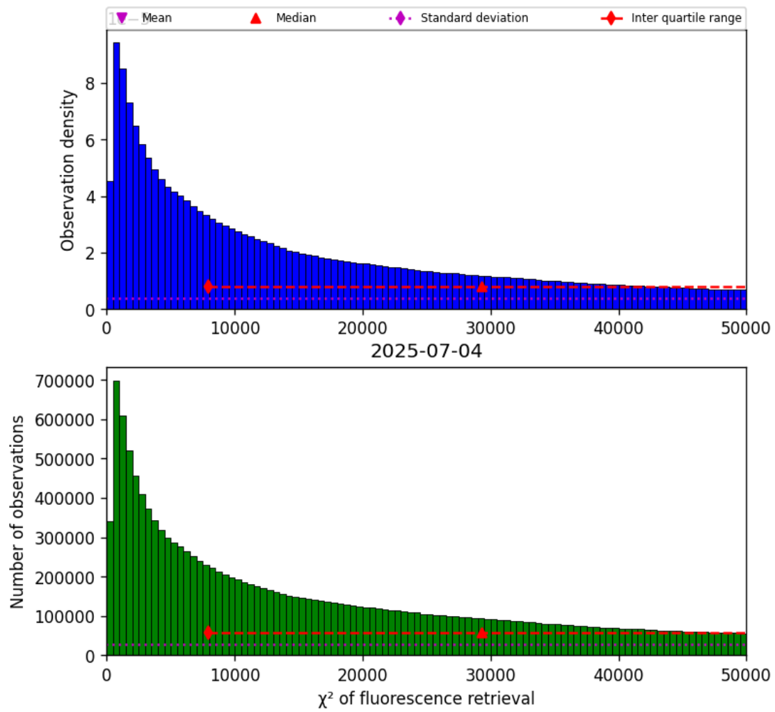
Figure 40: Histogram of “ \chi^2 of fluorescence retrieval” for 2025-07-04 to 2025-07-05
