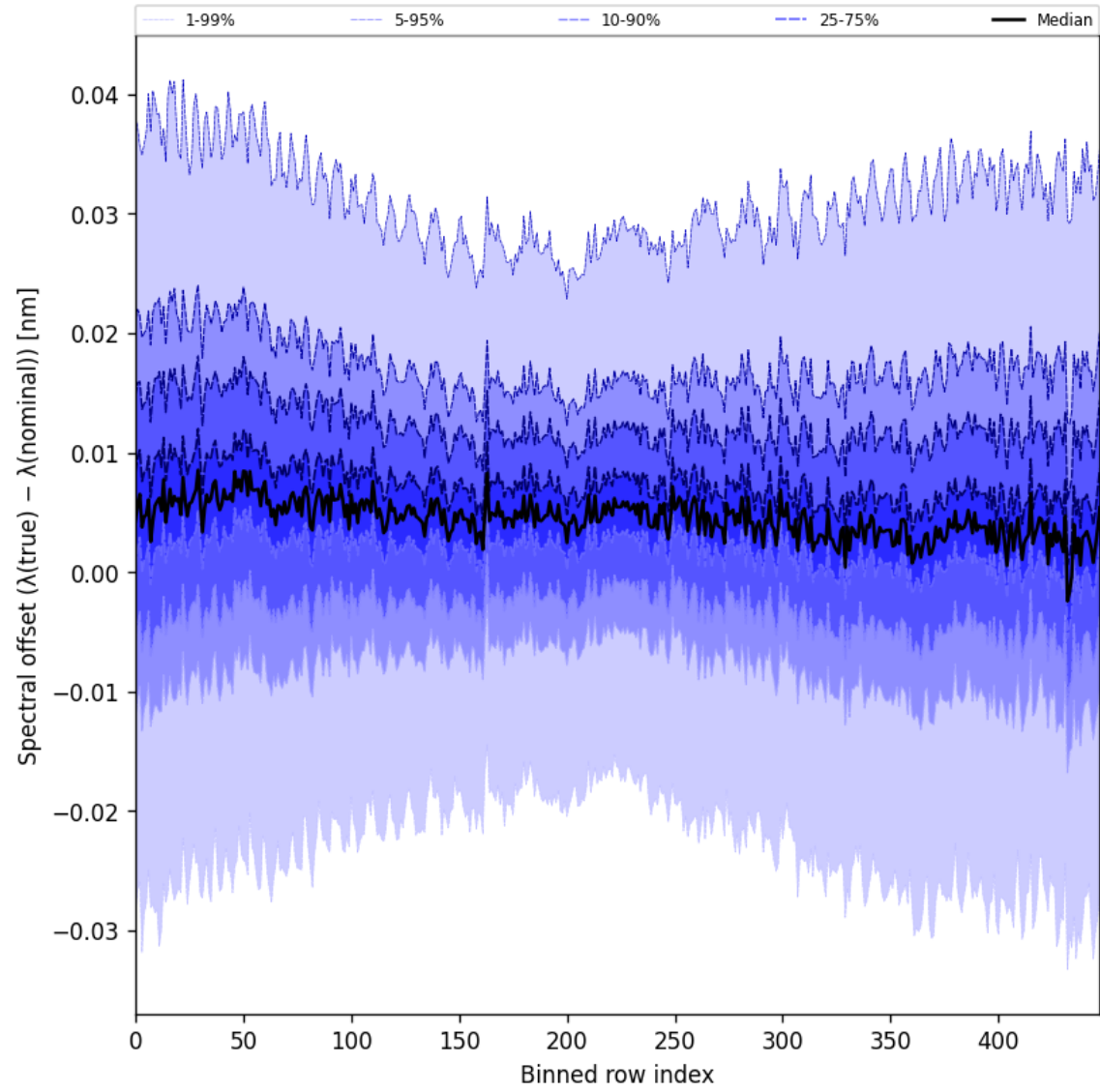
Figure 60: Along track statistics of “Spectral offset ( \lambda_{\text{true}} - \lambda_{\text{nominal}} )” for 2025-07-04 to 2025-07-05
