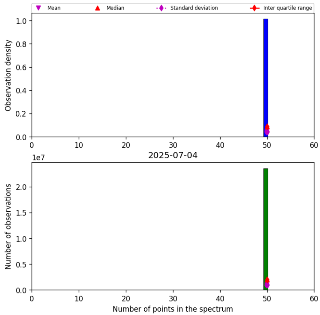
Figure 42: Histogram of “Number of points in the spectrum” for 2025-07-04 to 2025-07-05
