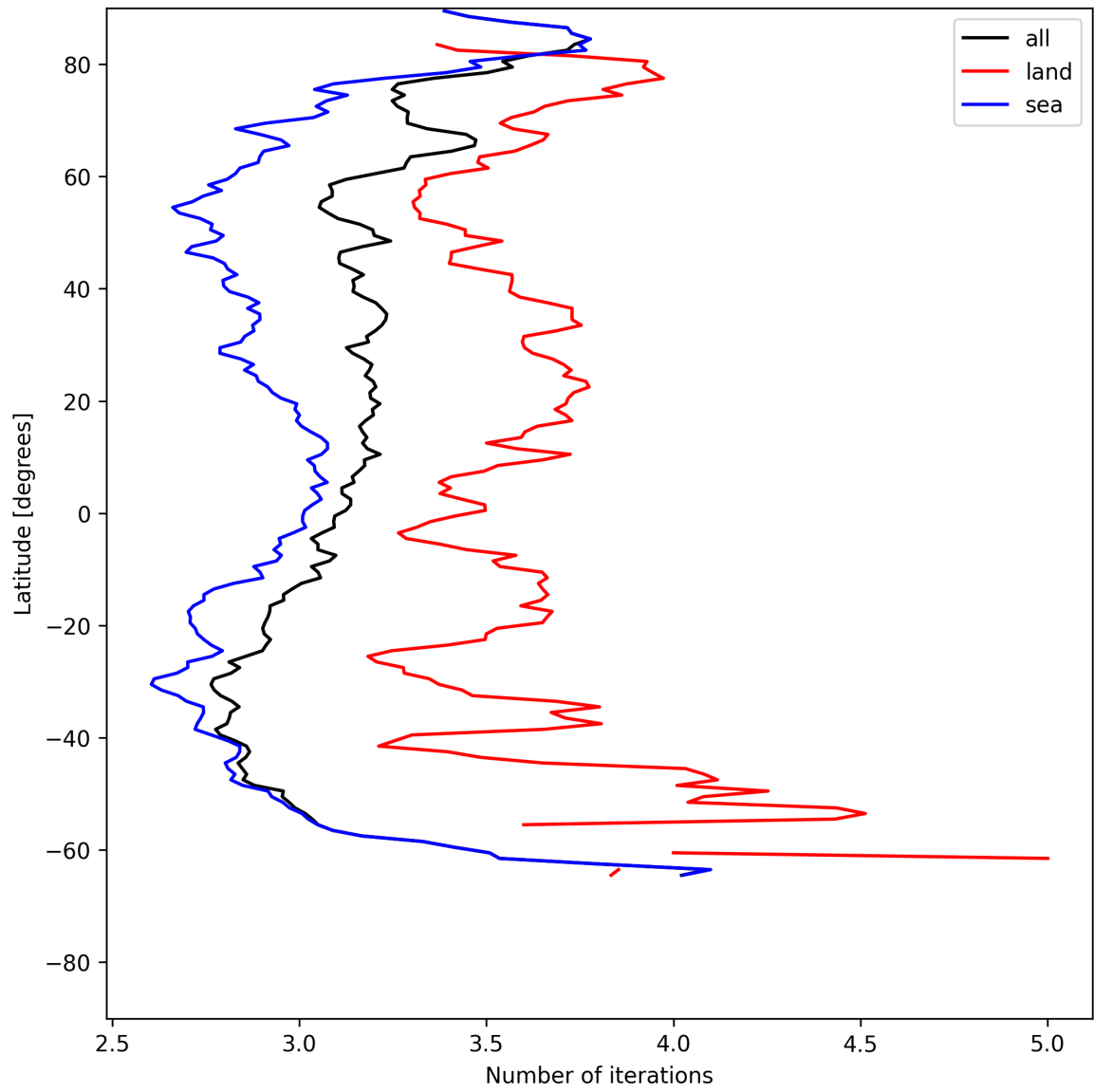
Figure 20: Zonal average of “Number of iterations” for 2025-07-04 to 2025-07-05.
