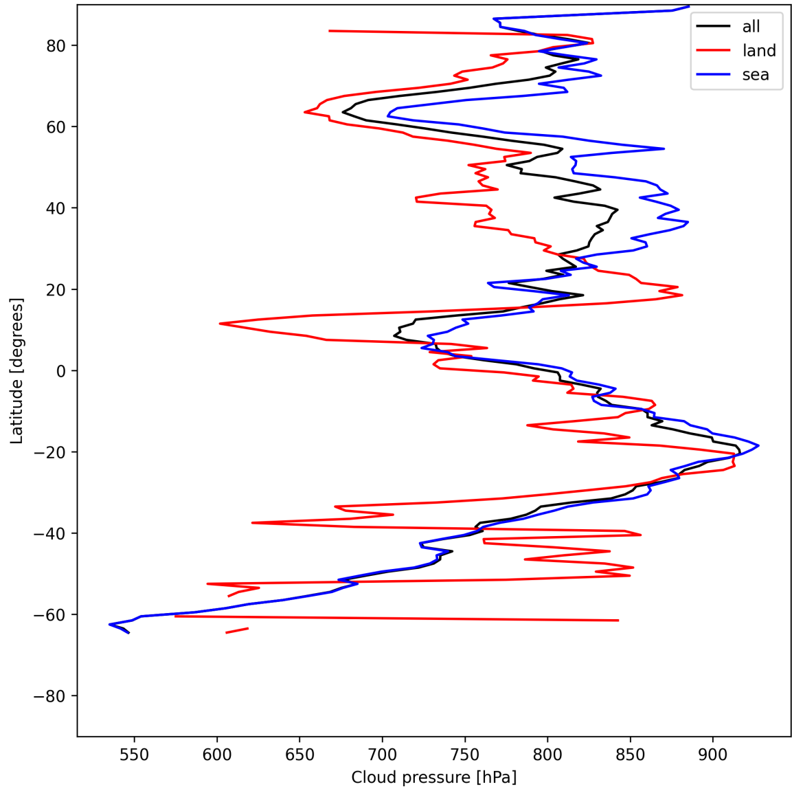
Figure 11: Zonal average of “Cloud pressure” for 2025-07-04 to 2025-07-05.
