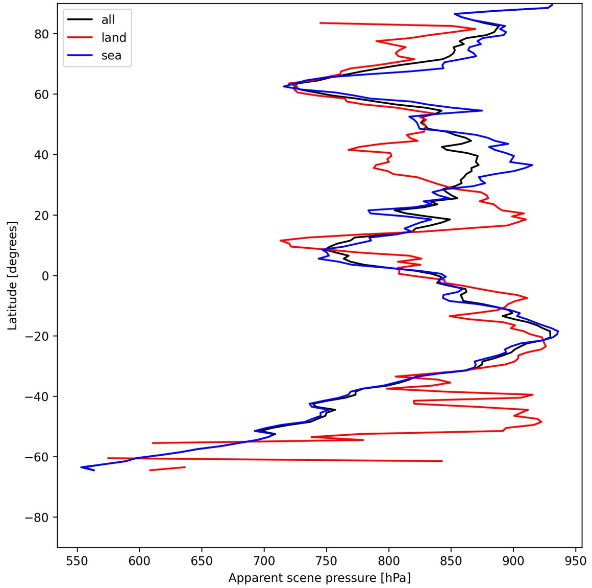
Figure 17: Zonal average of “Apparent scene pressure” for 2025-07-04 to 2025-07-05.
