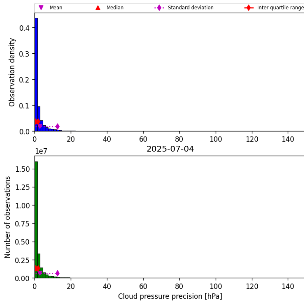
Figure 29: Histogram of “Cloud pressure precision” for 2025-07-04 to 2025-07-05
