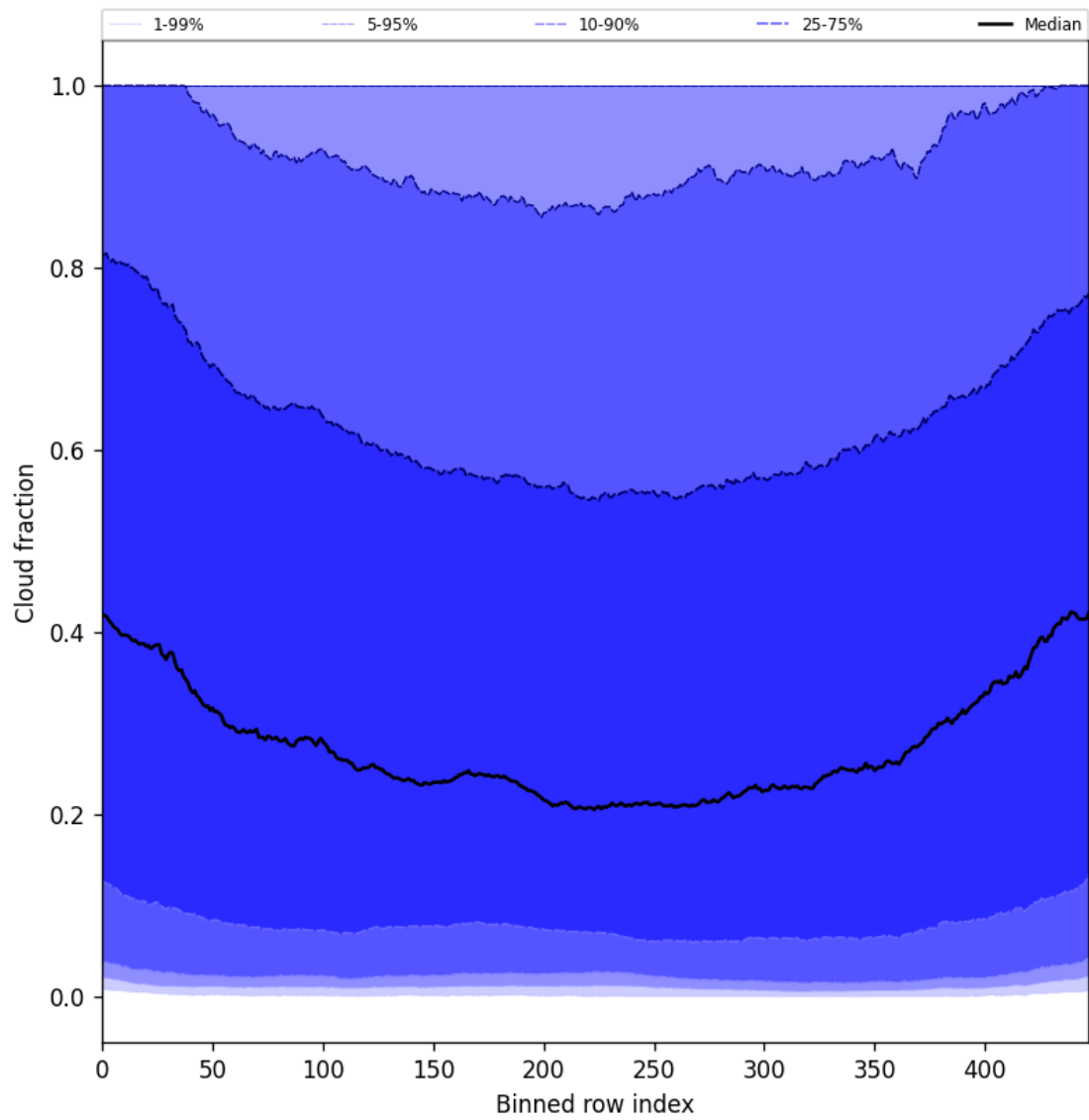
Figure 47: Along track statistics of “Cloud fraction” for 2025-07-04 to 2025-07-05
