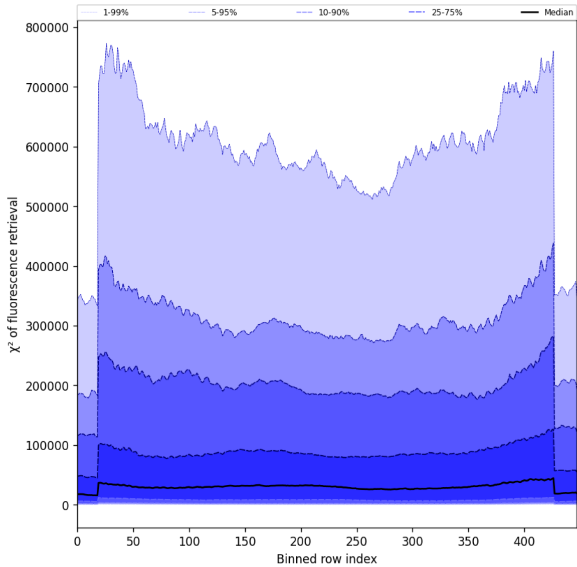
Figure 57: Along track statistics of “ \chi^2 of fluorescence retrieval” for 2025-07-04 to 2025-07-05
