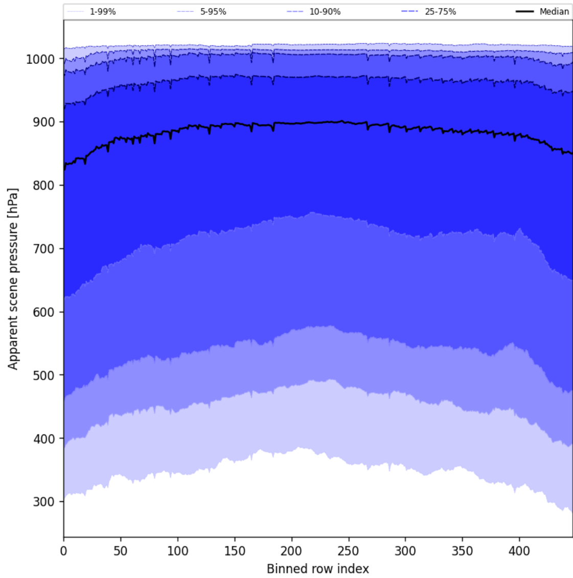
Figure 51: Along track statistics of “Apparent scene pressure” for 2025-07-04 to 2025-07-05
