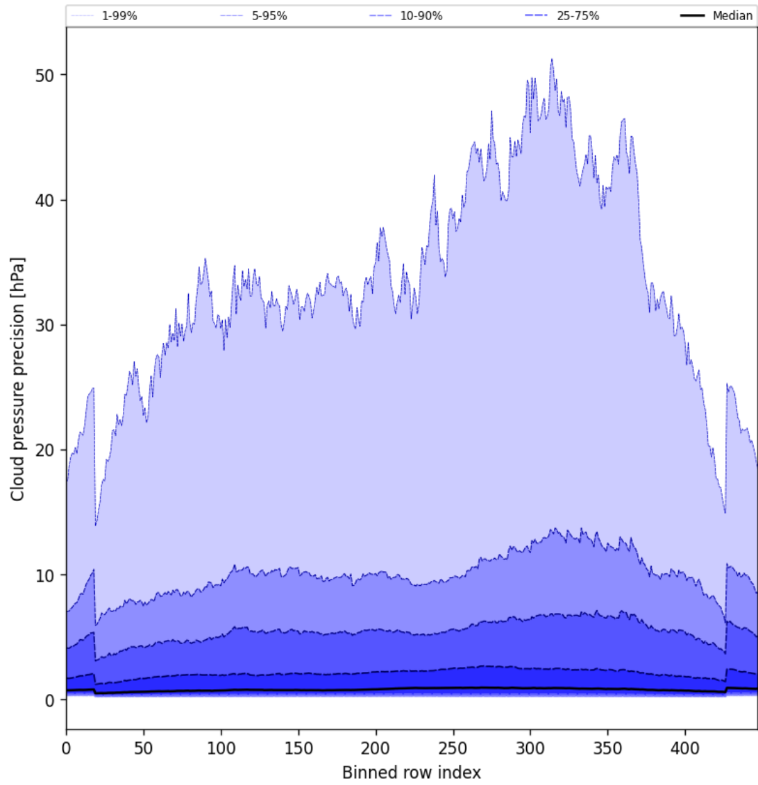
Figure 46: Along track statistics of “Cloud pressure precision” for 2025-07-04 to 2025-07-05
