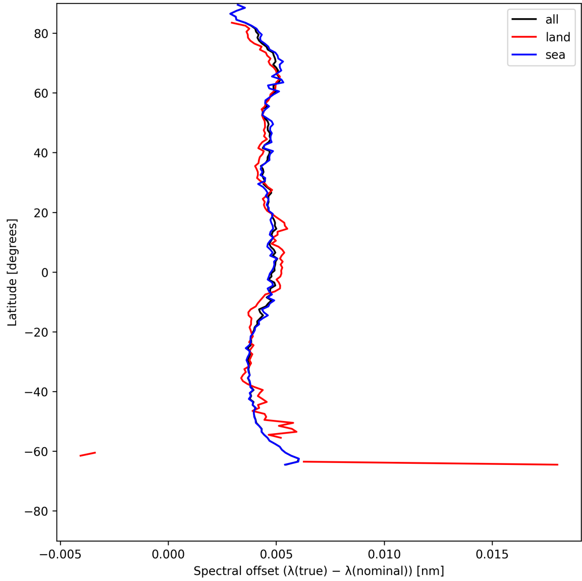
Figure 26: Zonal average of “Spectral offset ( \lambda_{\text{true}} - \lambda_{\text{nominal}} )” for 2025-07-04 to 2025-07-05.
