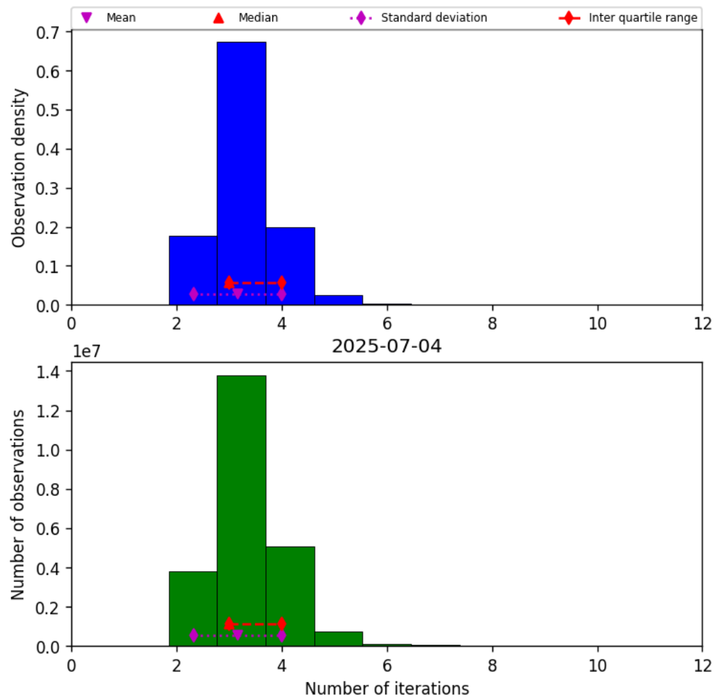
Figure 37: Histogram of “Number of iterations” for 2025-07-04 to 2025-07-05
