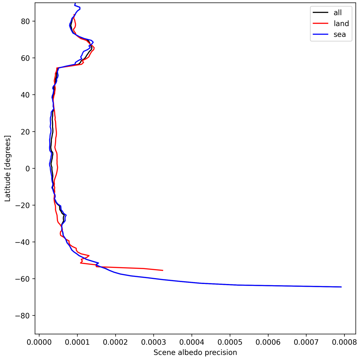
Figure 16: Zonal average of “Scene albedo precision” for 2025-07-05 to 2025-07-06.
