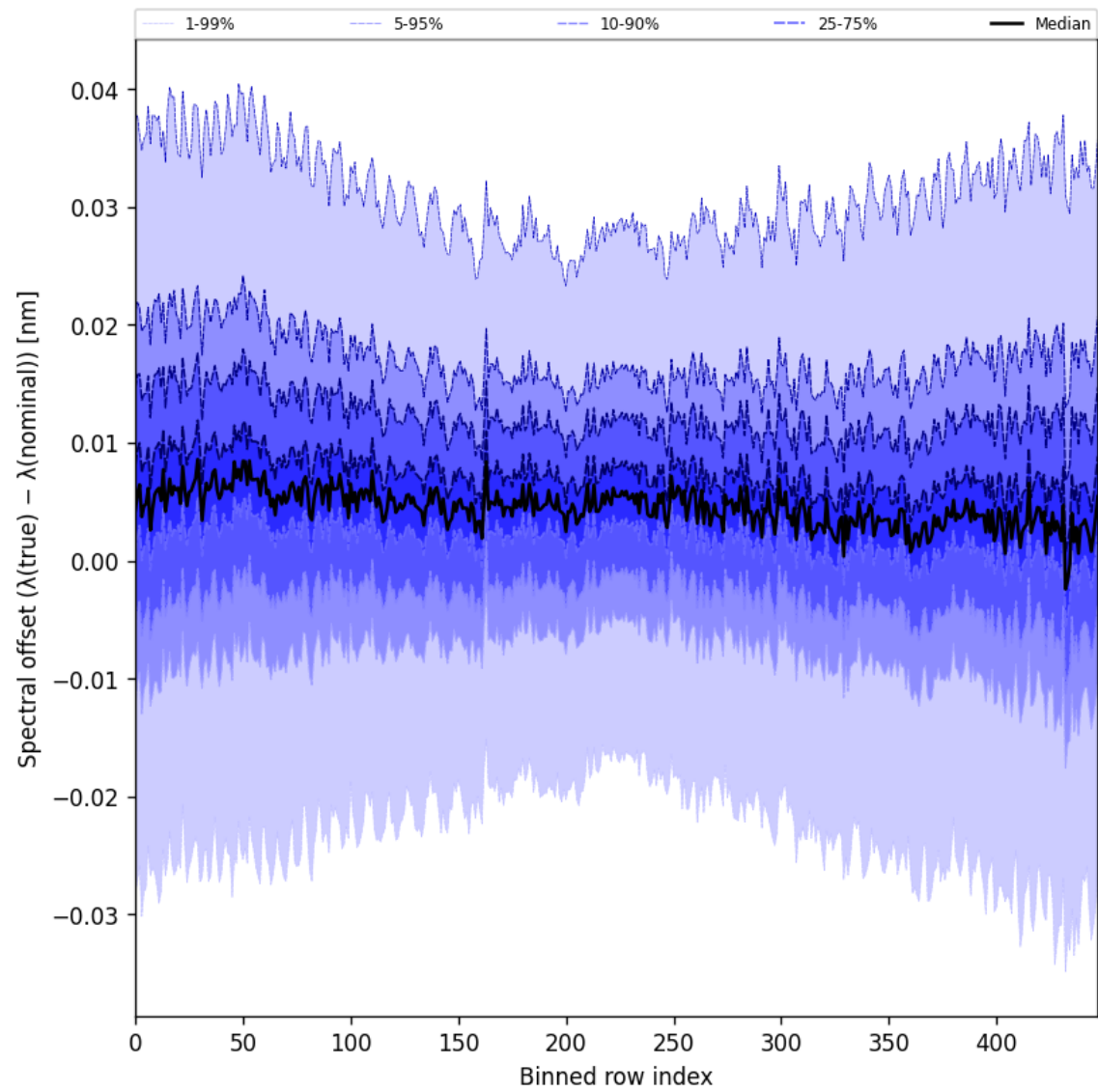
Figure 60: Along track statistics of “Spectral offset ( \lambda_{\text{true}} - \lambda_{\text{nominal}} )” for 2025-07-05 to 2025-07-06
