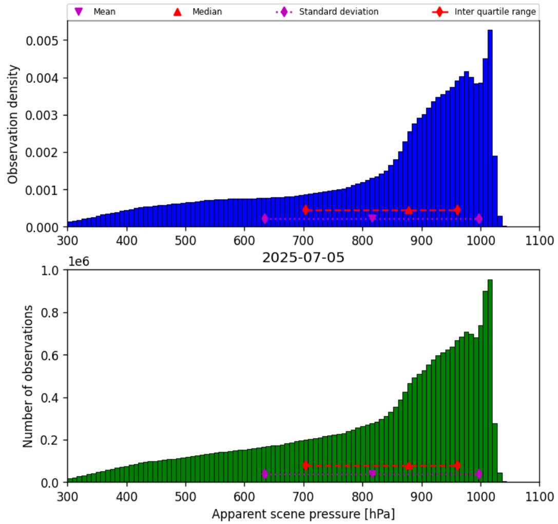
Figure 34: Histogram of “Apparent scene pressure” for 2025-07-05 to 2025-07-06
