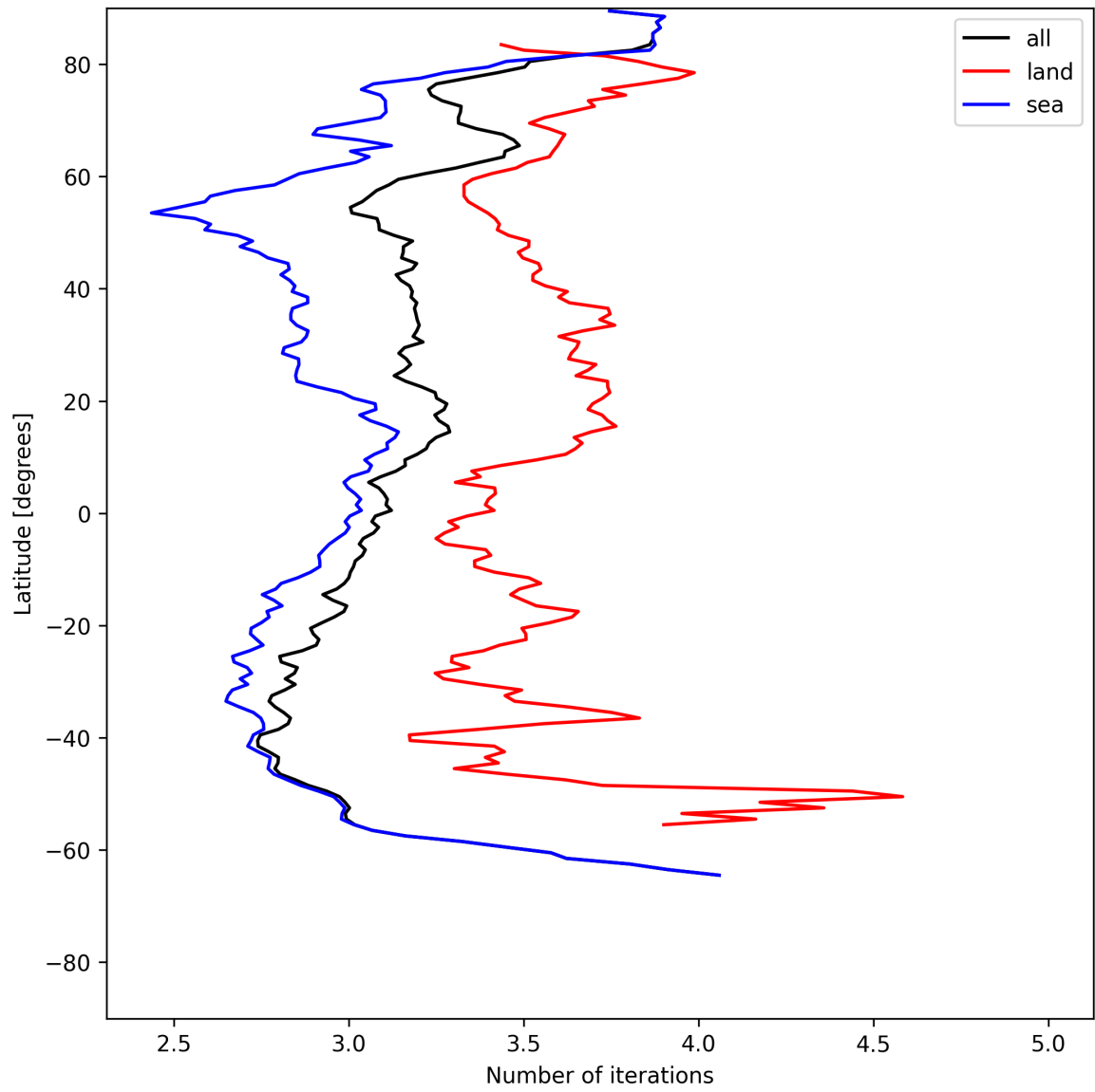
Figure 20: Zonal average of “Number of iterations” for 2025-07-05 to 2025-07-06.
