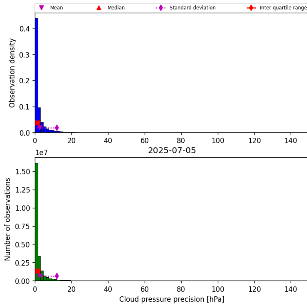
Figure 29: Histogram of “Cloud pressure precision” for 2025-07-05 to 2025-07-06
