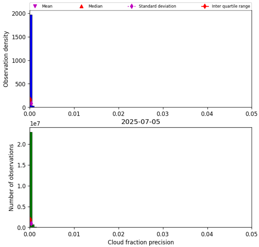
Figure 31: Histogram of “Cloud fraction precision” for 2025-07-05 to 2025-07-06
