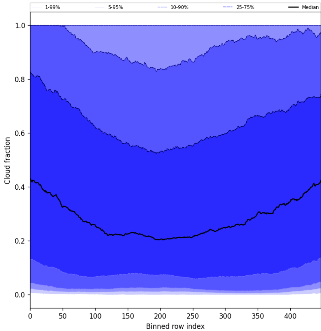
Figure 47: Along track statistics of “Cloud fraction” for 2025-07-05 to 2025-07-06
