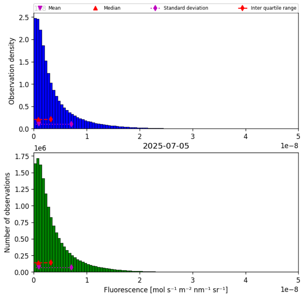
Figure 38: Histogram of “Fluorescence” for 2025-07-05 to 2025-07-06
