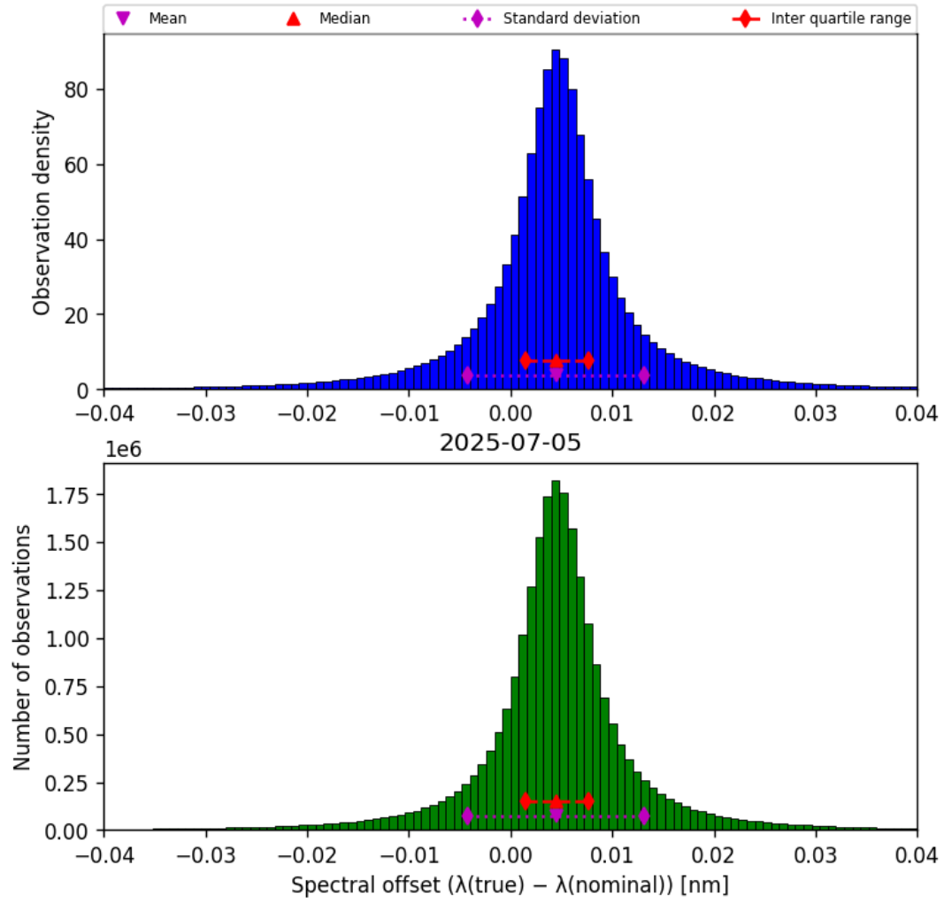
Figure 43: Histogram of “Spectral offset ( \lambda_{\text{true}} - \lambda_{\text{nominal}} )” for 2025-07-05 to 2025-07-06
