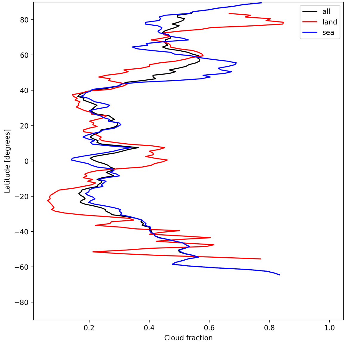
Figure 13: Zonal average of “Cloud fraction” for 2025-07-05 to 2025-07-06.
