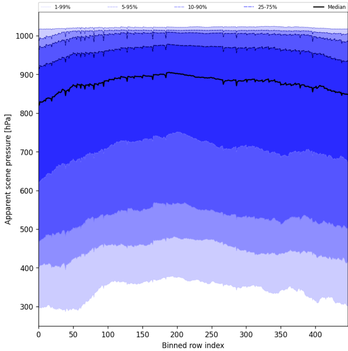
Figure 51: Along track statistics of “Apparent scene pressure” for 2025-07-05 to 2025-07-06
