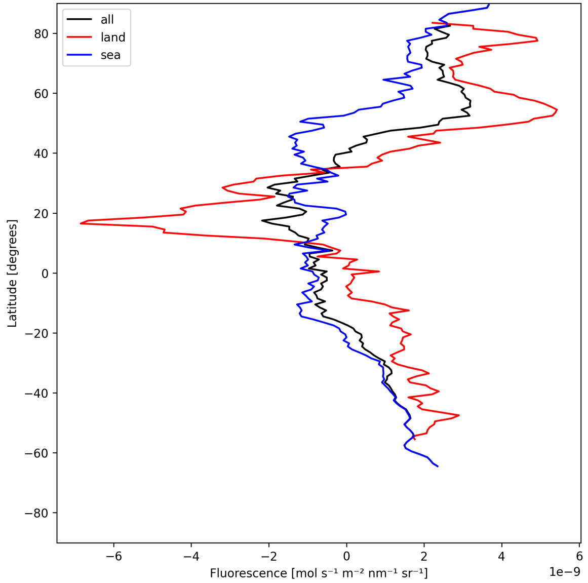
Figure 21: Zonal average of “Fluorescence” for 2025-07-05 to 2025-07-06.
