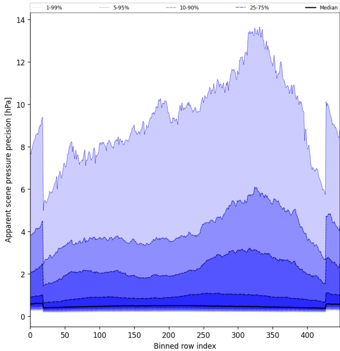
Figure 52: Along track statistics of “Apparent scene pressure precision” for 2025-07-05 to 2025-07-06
