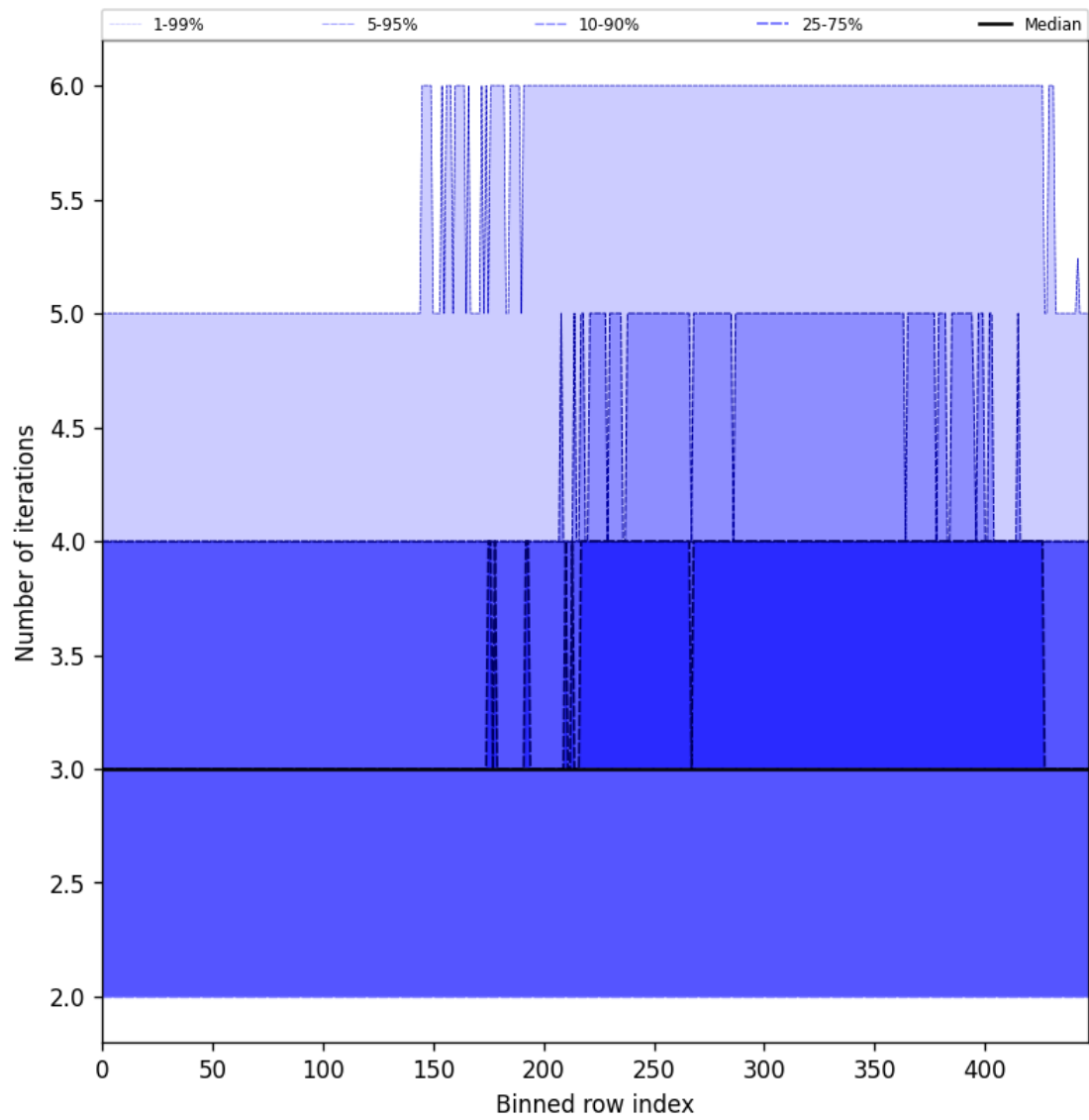
Figure 54: Along track statistics of “Number of iterations” for 2025-07-05 to 2025-07-06
