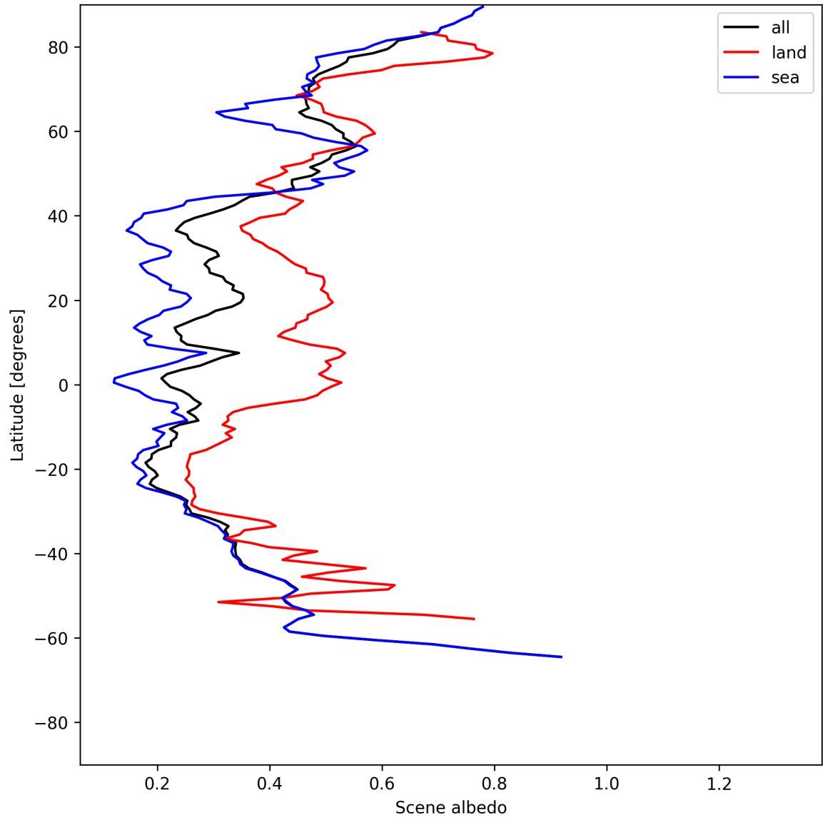
Figure 15: Zonal average of “Scene albedo” for 2025-07-05 to 2025-07-06.
