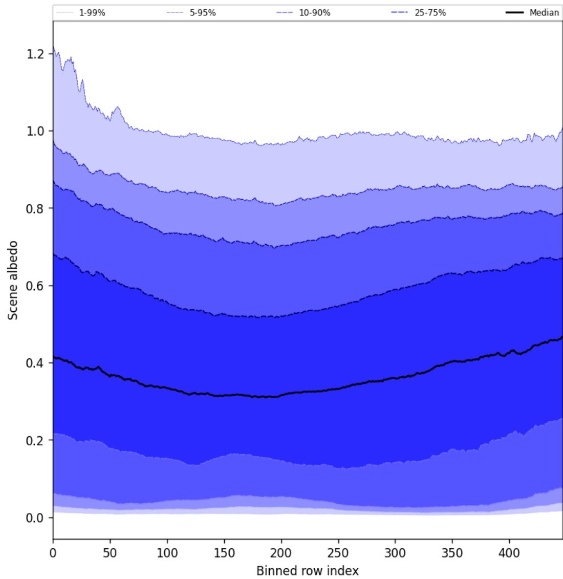
Figure 49: Along track statistics of “Scene albedo” for 2025-07-05 to 2025-07-06
