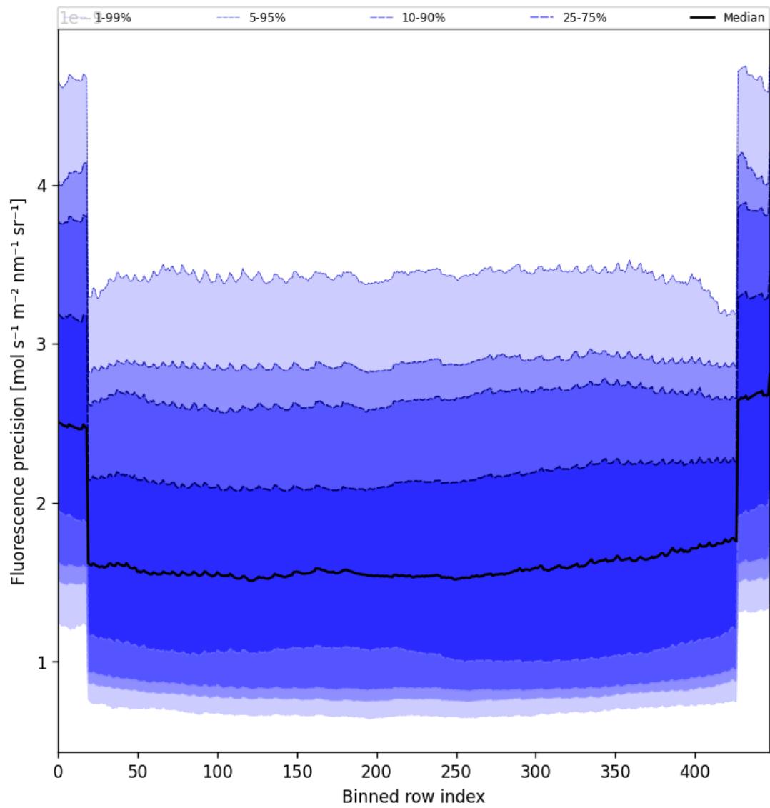
Figure 56: Along track statistics of “Fluorescence precision” for 2025-07-05 to 2025-07-06
