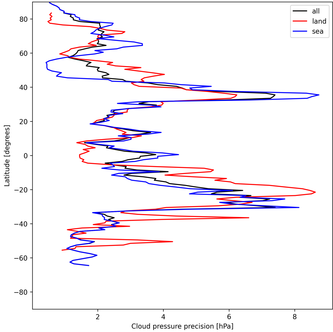
Figure 12: Zonal average of "Cloud pressure precision" for 2025-07-05 to 2025-07-06.
