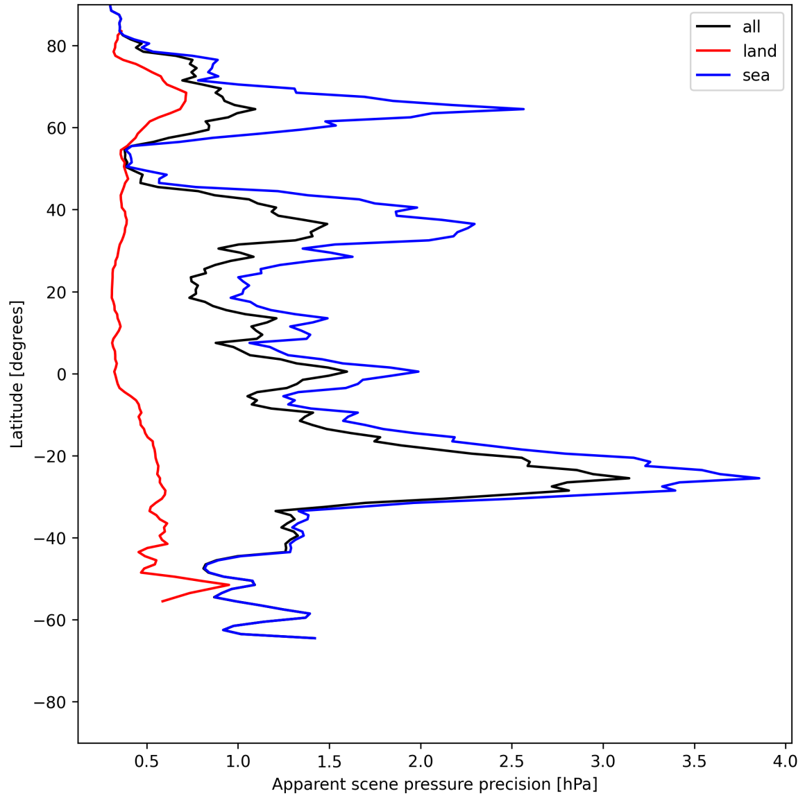
Figure 18: Zonal average of “Apparent scene pressure precision” for 2025-07-05 to 2025-07-06.
