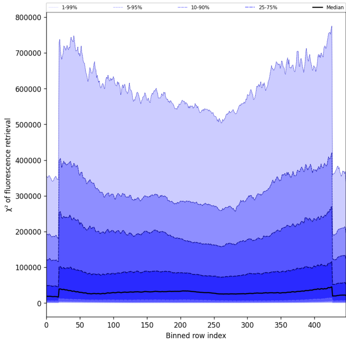
Figure 57: Along track statistics of “ \chi^2 of fluorescence retrieval” for 2025-07-05 to 2025-07-06
