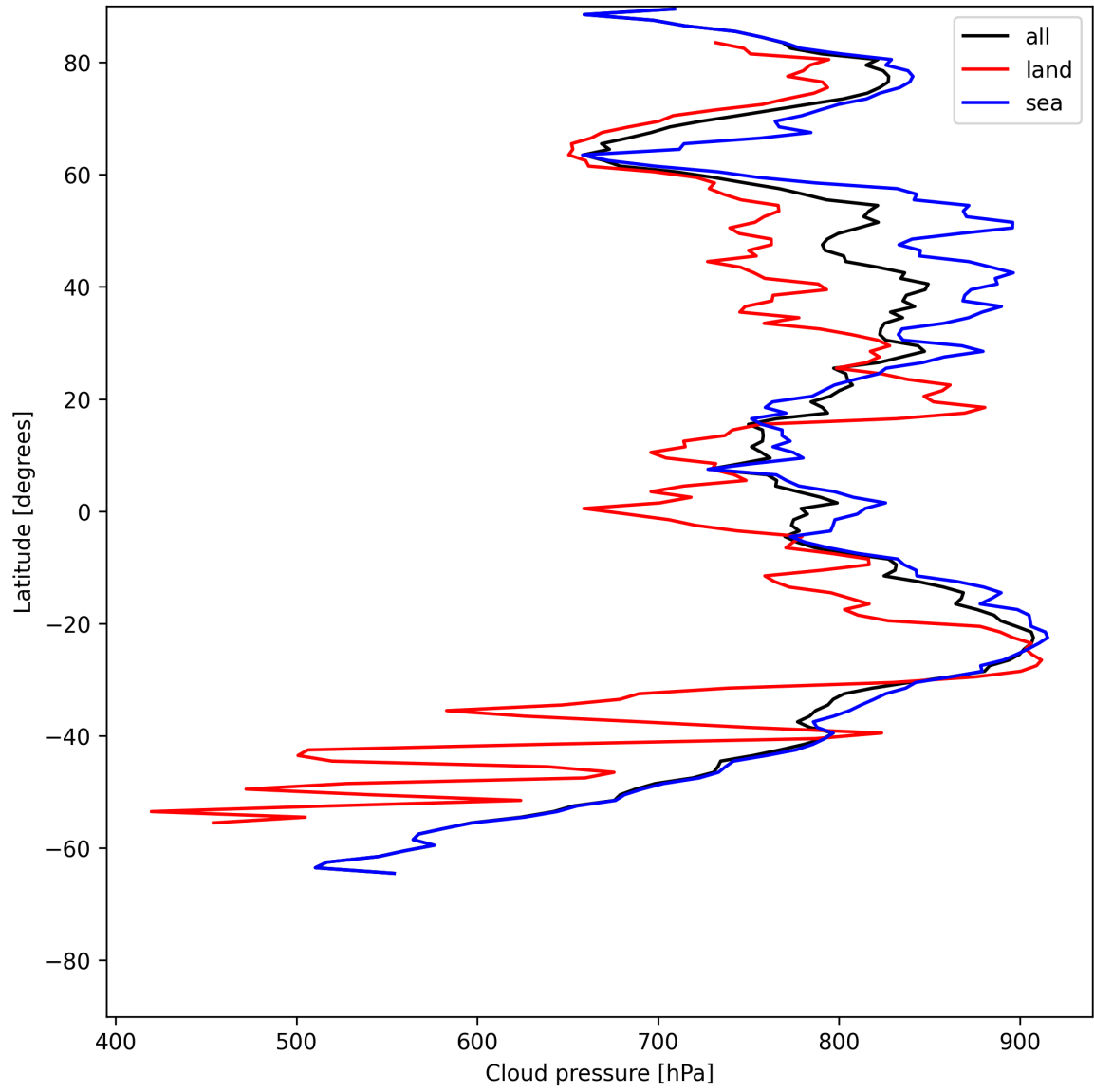
Figure 11: Zonal average of “Cloud pressure” for 2025-07-05 to 2025-07-06.
