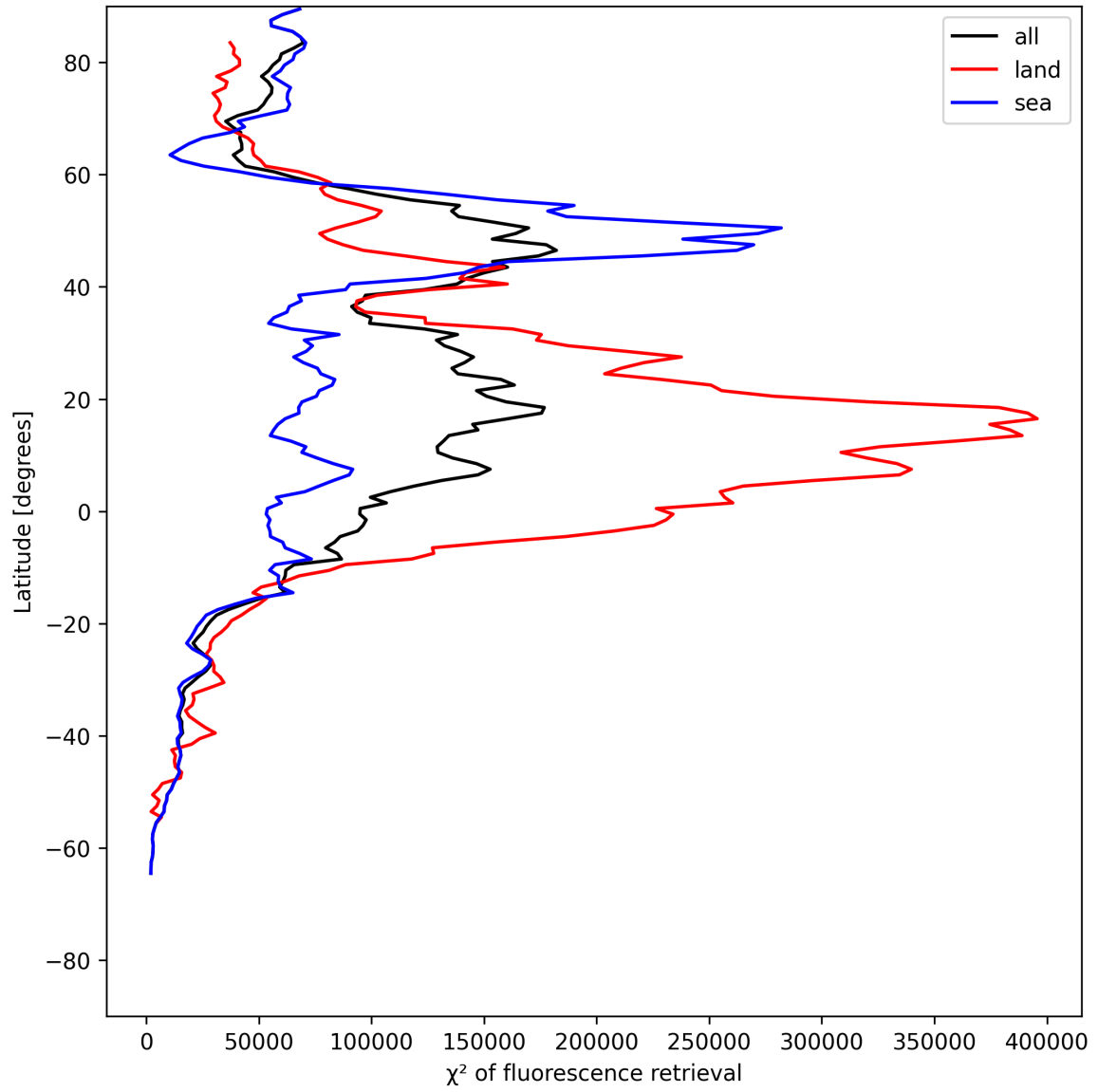
Figure 23: Zonal average of “ \chi^2 of fluorescence retrieval” for 2025-07-05 to 2025-07-06.
