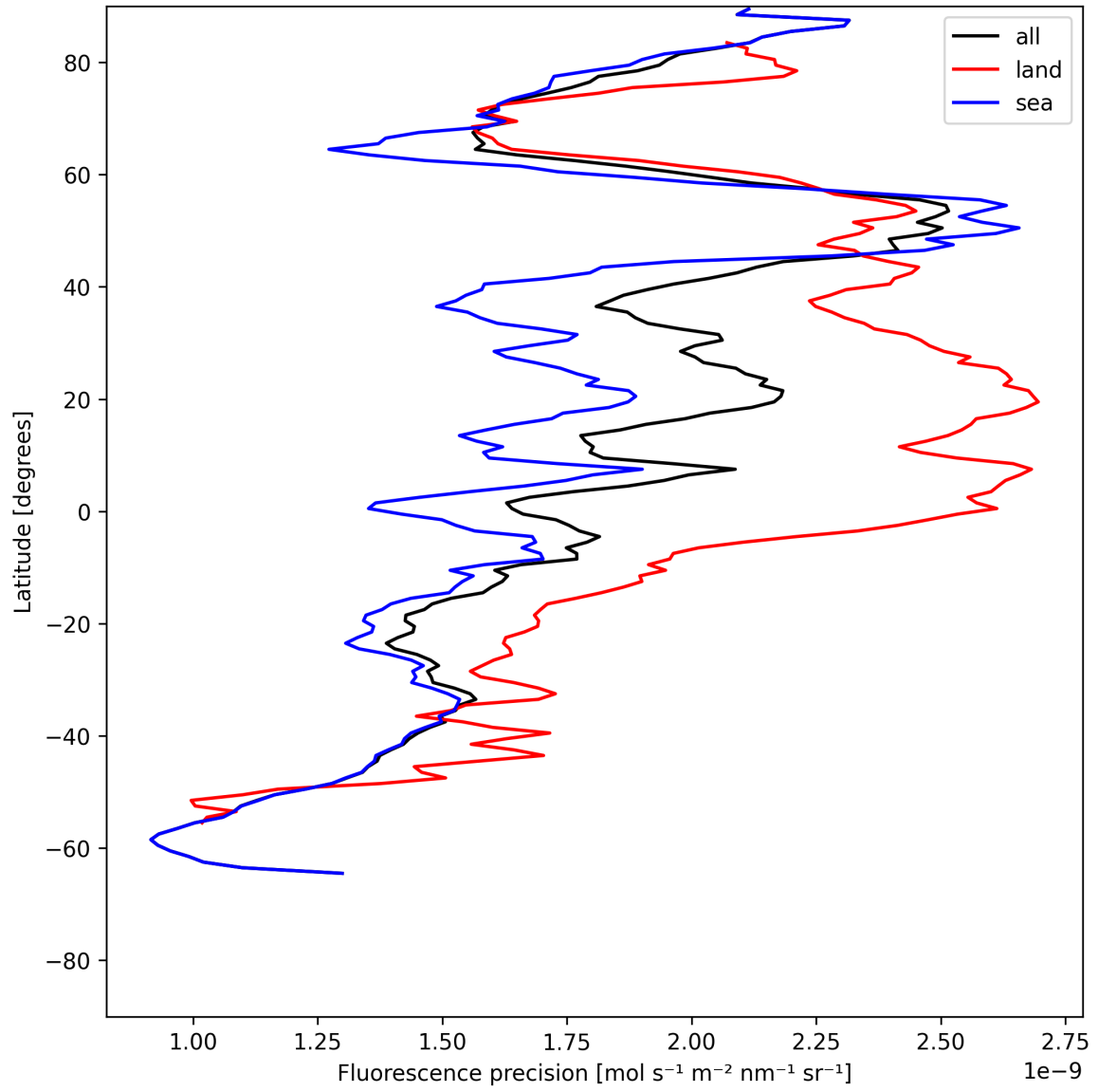
Figure 22: Zonal average of "Fluorescence precision" for 2025-07-05 to 2025-07-06.
