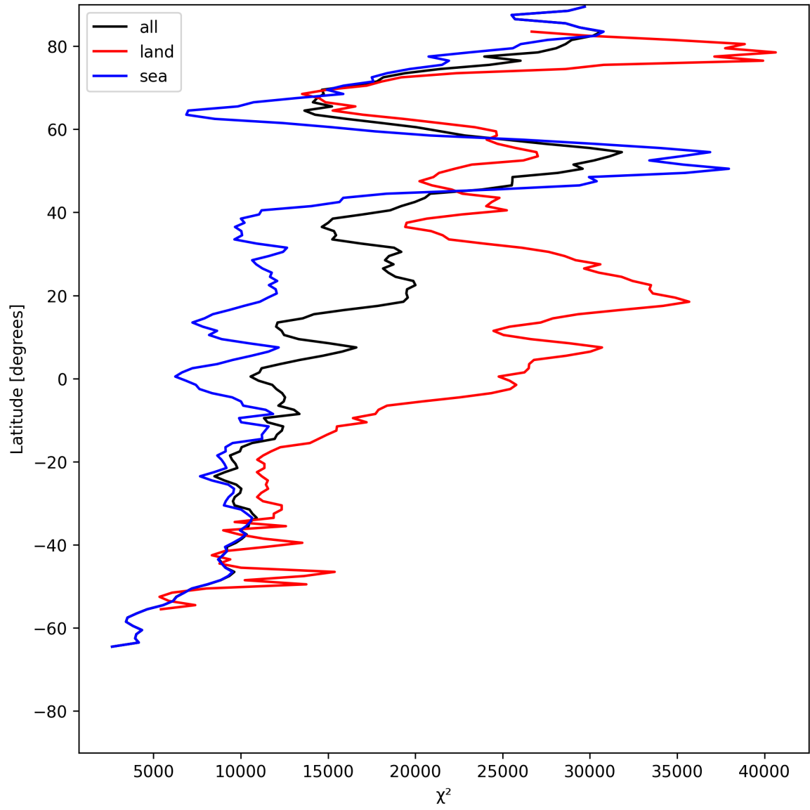
Figure 19: Zonal average of “ \chi^2 ” for 2025-07-05 to 2025-07-06.
