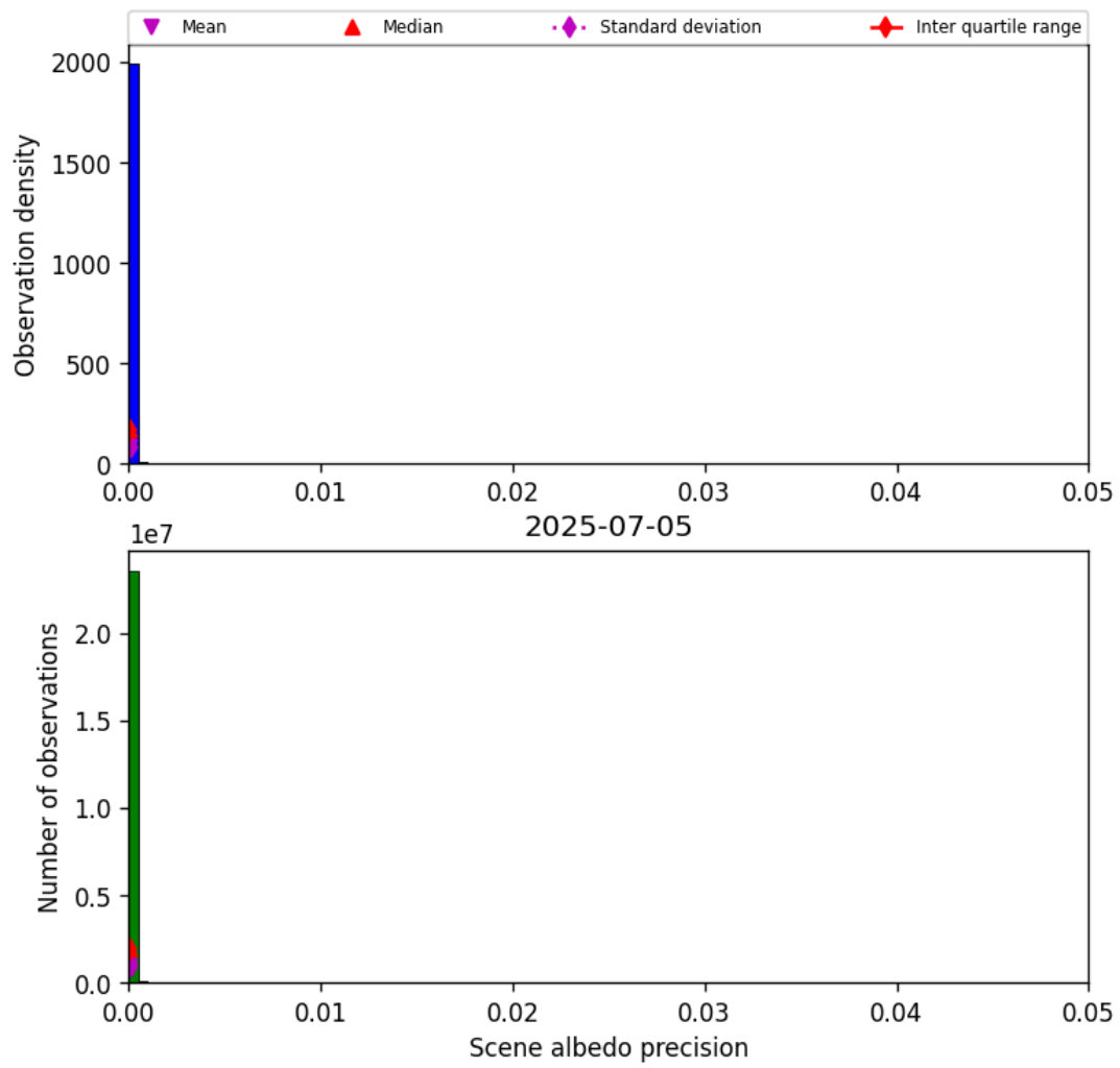
Figure 33: Histogram of “Scene albedo precision” for 2025-07-05 to 2025-07-06
