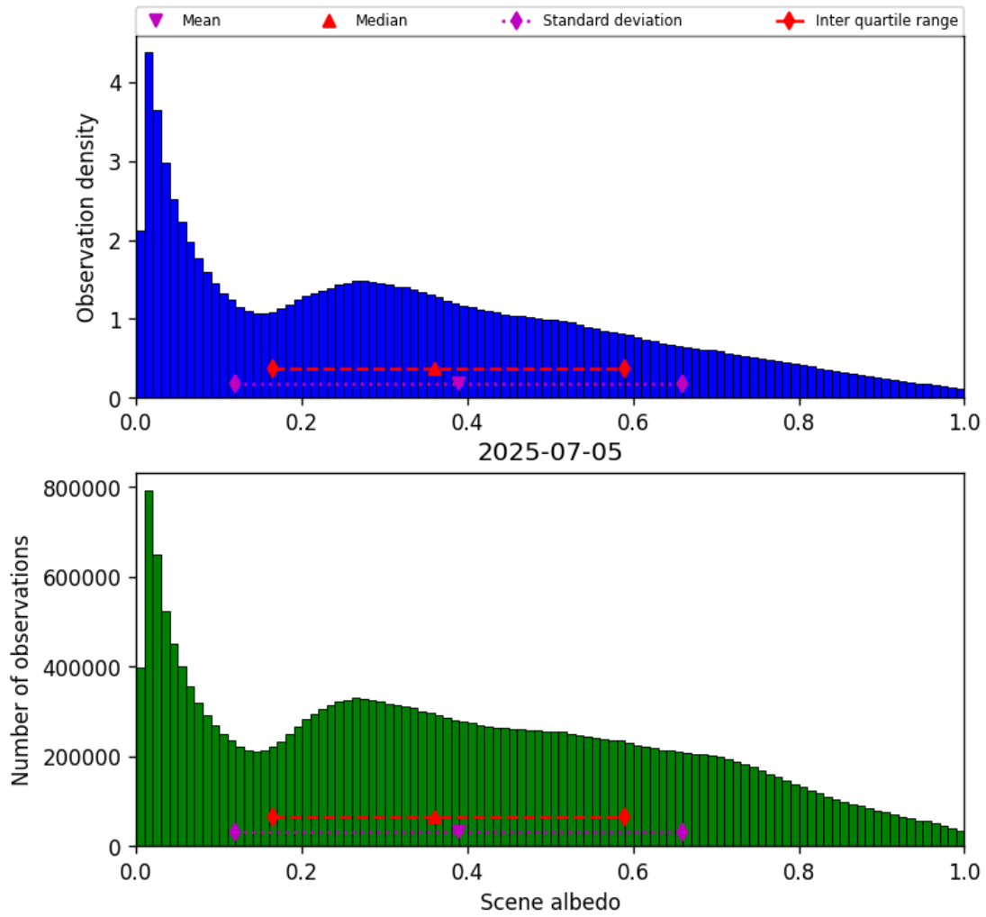
Figure 32: Histogram of “Scene albedo” for 2025-07-05 to 2025-07-06
