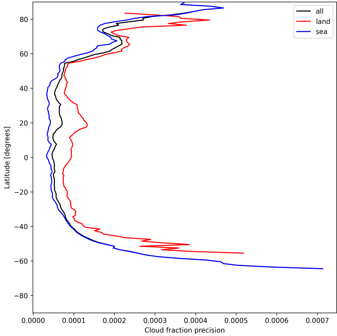
Figure 14: Zonal average of “Cloud fraction precision” for 2025-07-05 to 2025-07-06.
