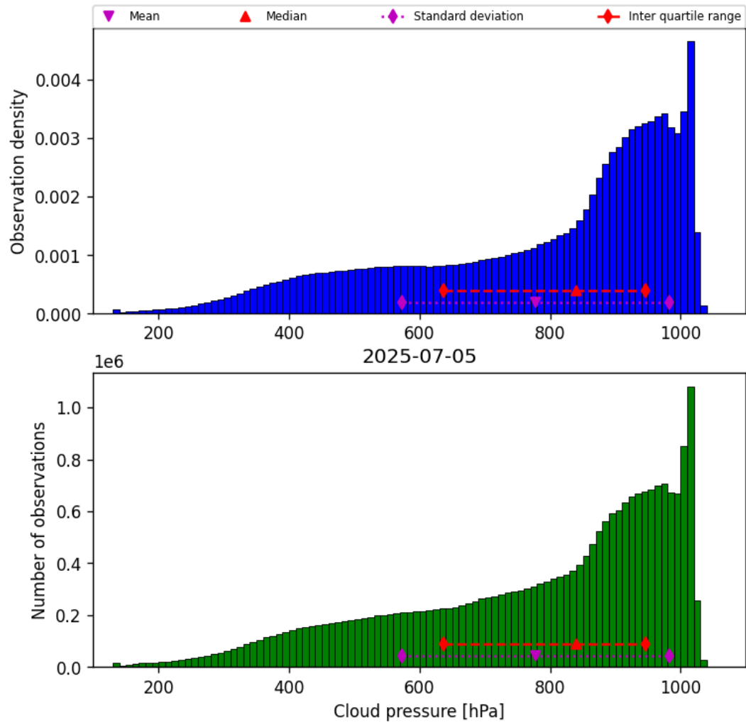
Figure 28: Histogram of “Cloud pressure” for 2025-07-05 to 2025-07-06
