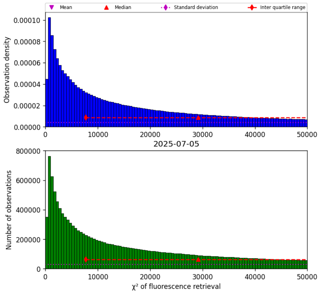
Figure 40: Histogram of “ \chi^2 of fluorescence retrieval” for 2025-07-05 to 2025-07-06
