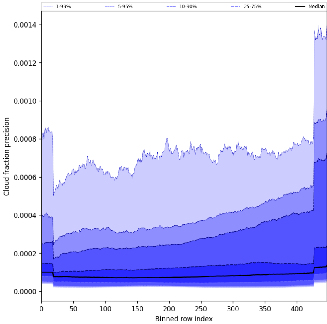
Figure 48: Along track statistics of “Cloud fraction precision” for 2025-07-05 to 2025-07-06
