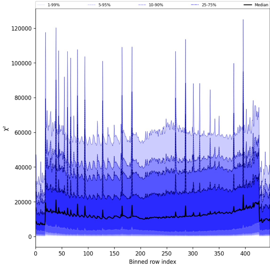
Figure 53: Along track statistics of “ \chi^2 ” for 2025-07-05 to 2025-07-06
