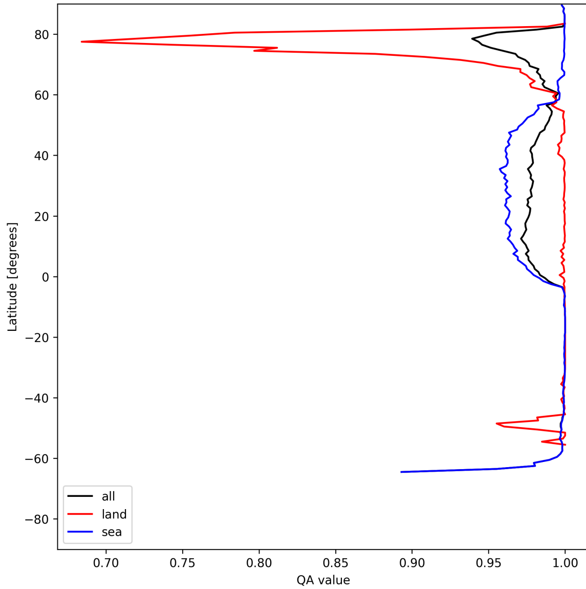
Figure 10: Zonal average of “QA value” for 2025-07-05 to 2025-07-06.
