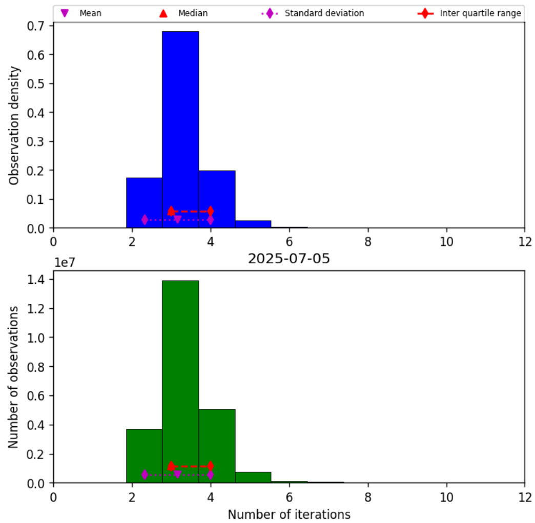
Figure 37: Histogram of “Number of iterations” for 2025-07-05 to 2025-07-06
