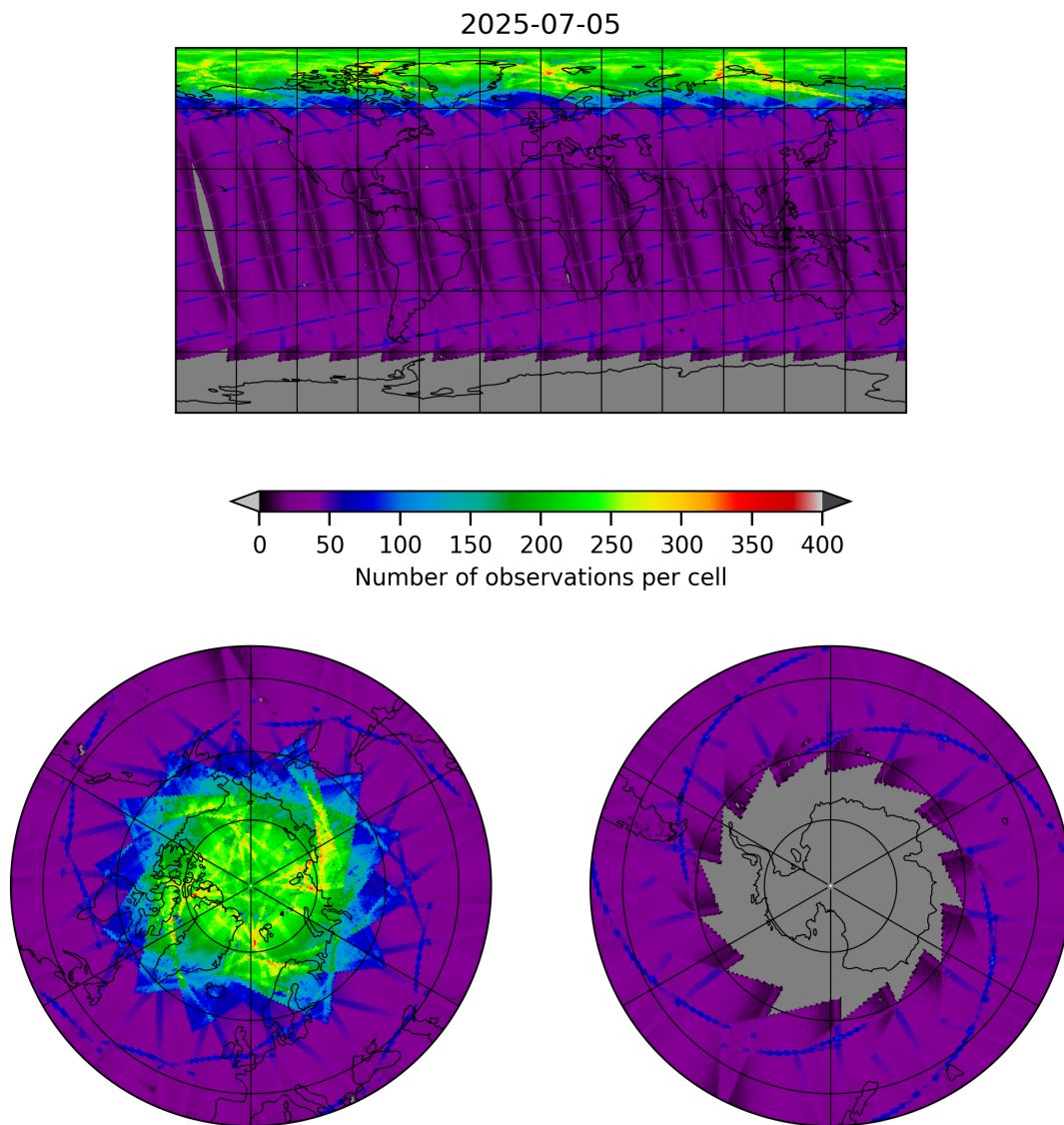
Figure 9: Map of the number of observations for 2025-07-05 to 2025-07-06
