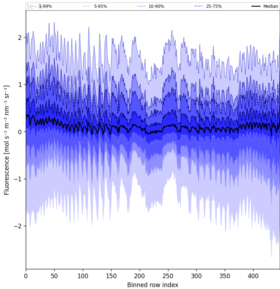
Figure 55: Along track statistics of “Fluorescence” for 2025-07-05 to 2025-07-06
