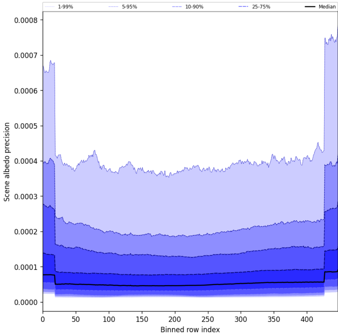
Figure 50: Along track statistics of “Scene albedo precision” for 2025-07-05 to 2025-07-06
