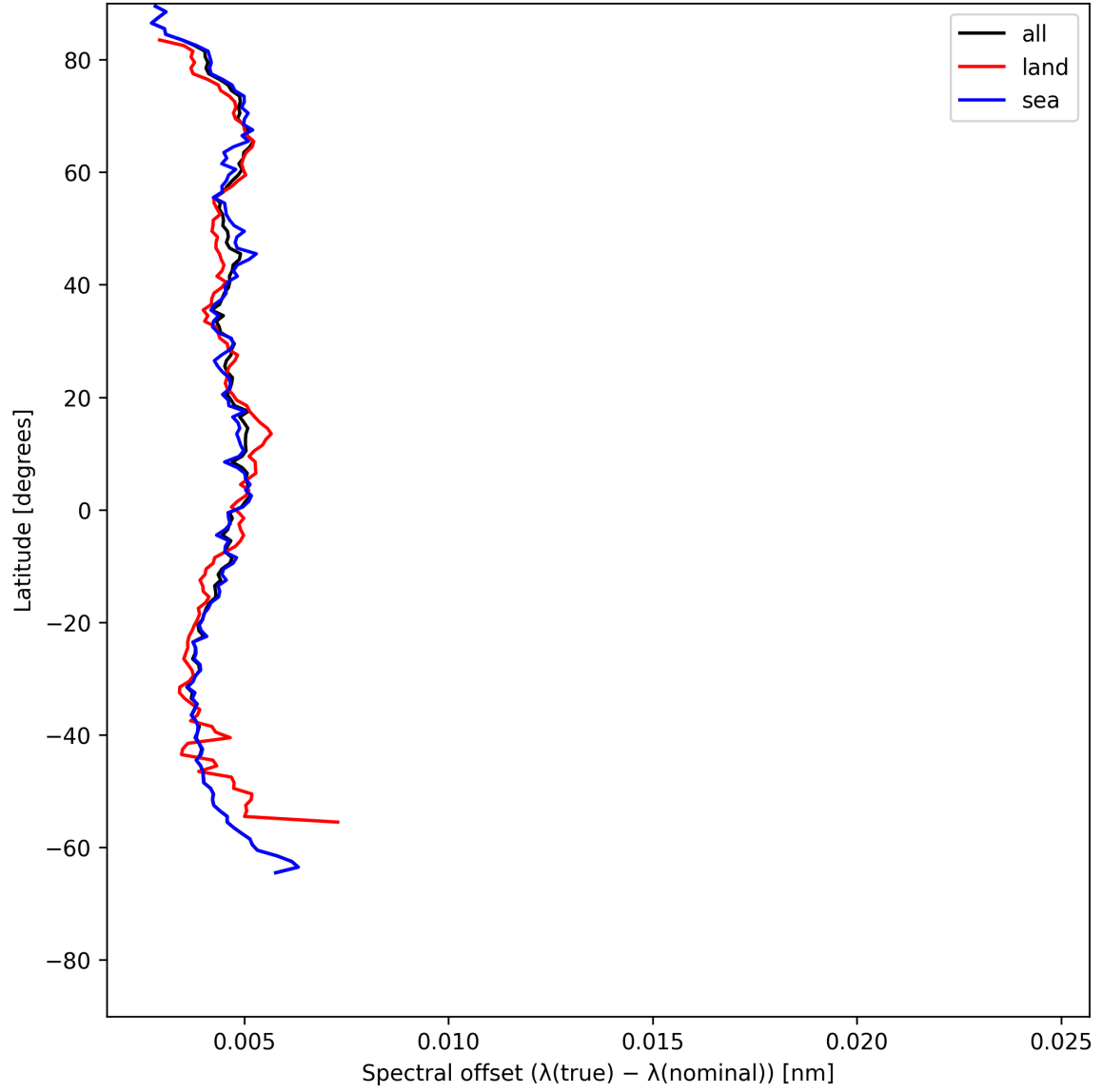
Figure 26: Zonal average of “Spectral offset ( \lambda_{\text{true}} - \lambda_{\text{nominal}} )” for 2025-07-05 to 2025-07-06.
