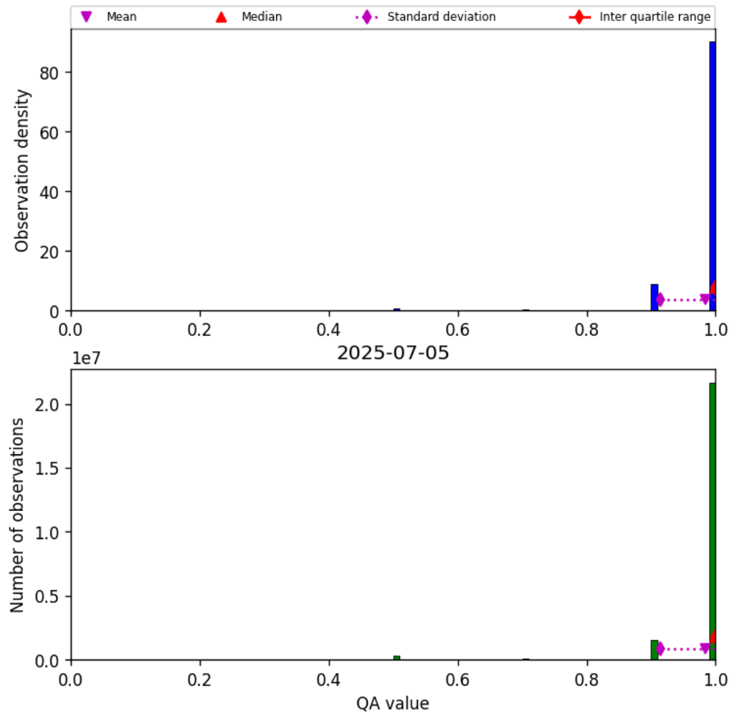
Figure 27: Histogram of “QA value” for 2025-07-05 to 2025-07-06
