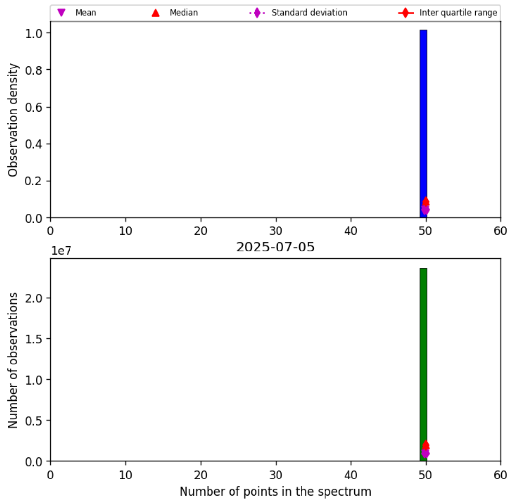
Figure 42: Histogram of "Number of points in the spectrum" for 2025-07-05 to 2025-07-06
