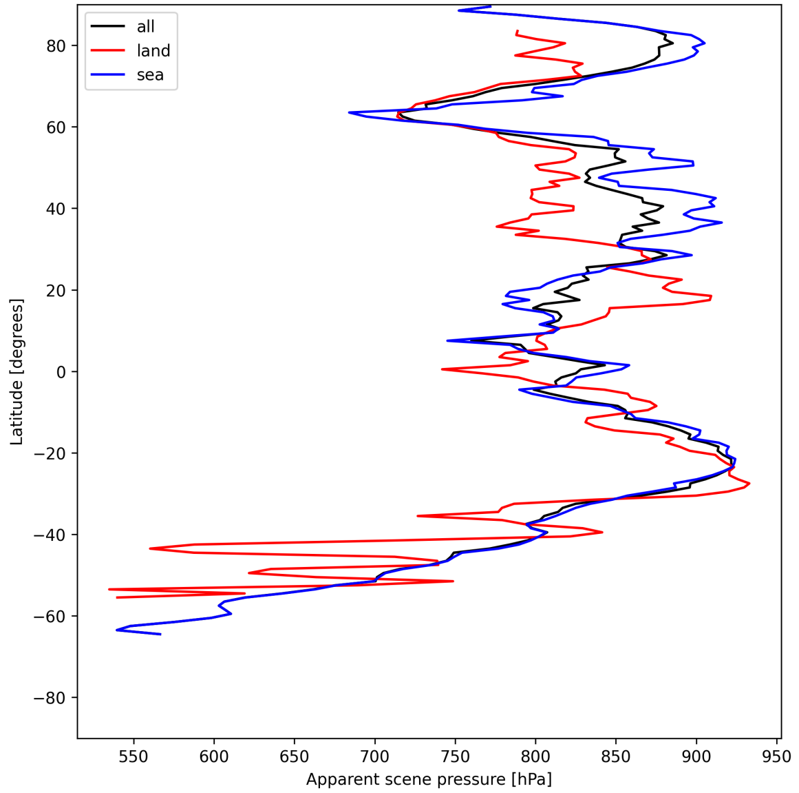
Figure 17: Zonal average of “Apparent scene pressure” for 2025-07-05 to 2025-07-06.
