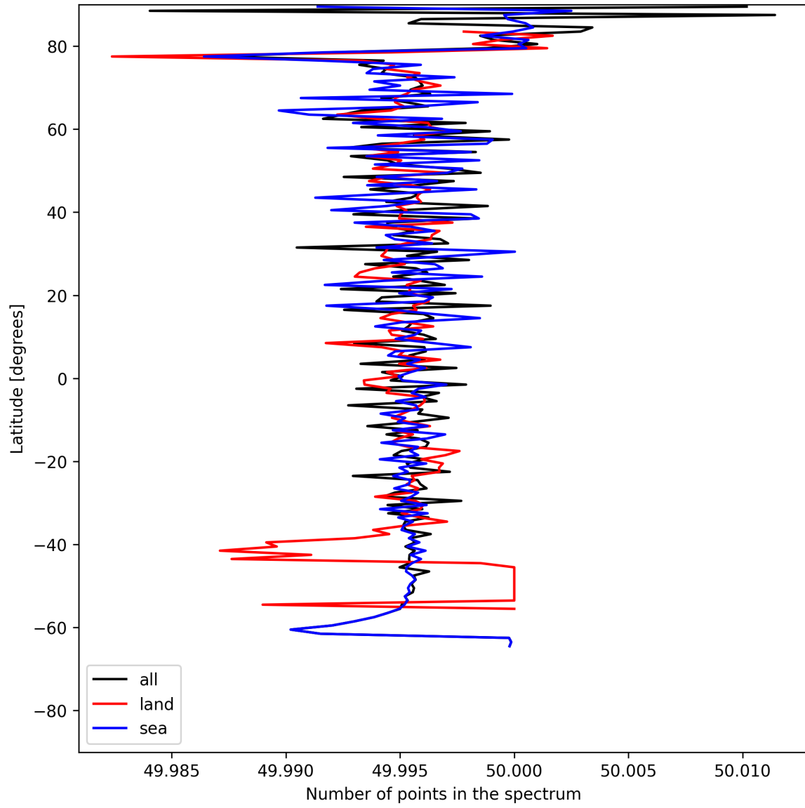
Figure 25: Zonal average of “Number of points in the spectrum” for 2025-07-05 to 2025-07-06.
