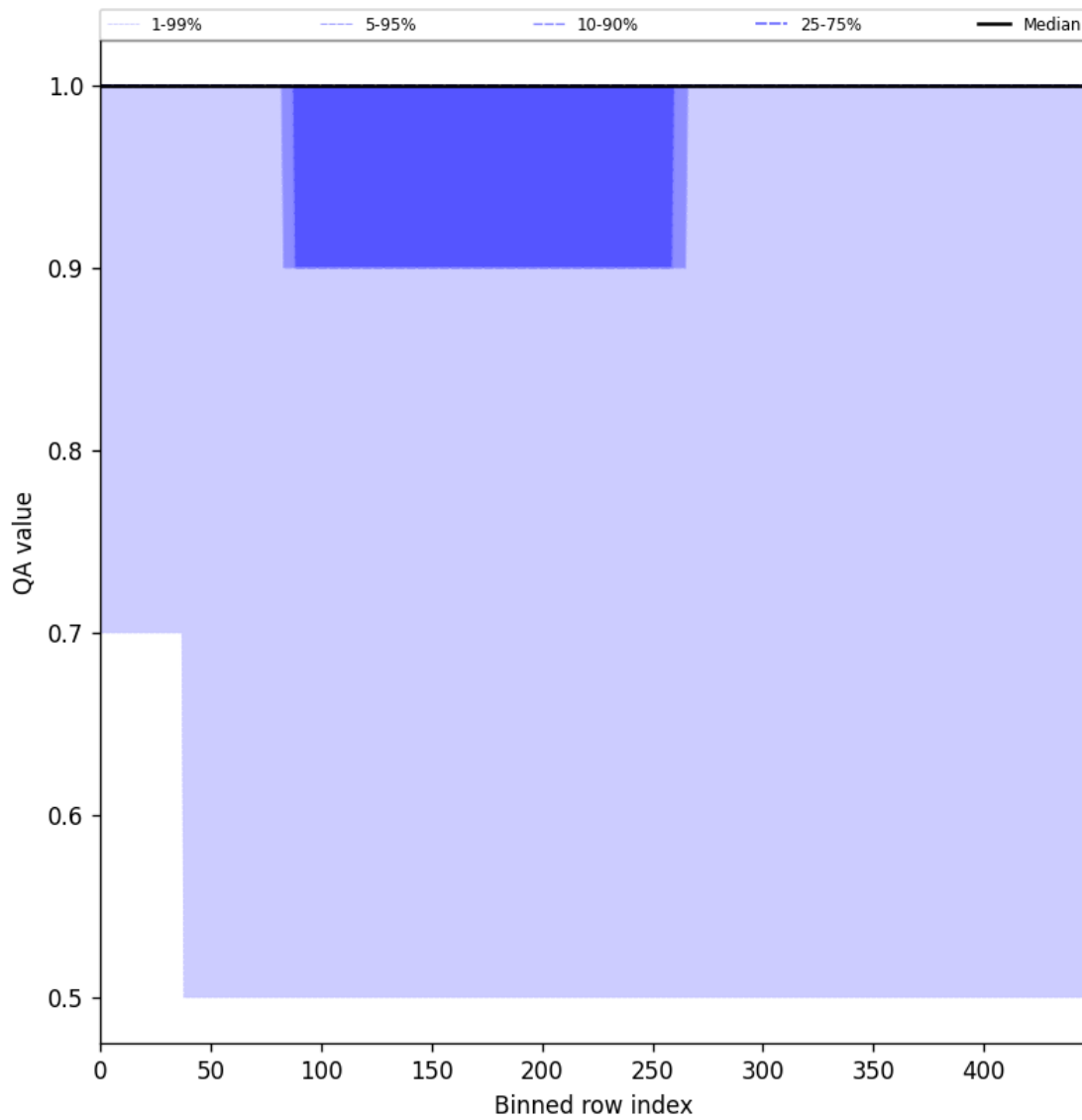
Figure 44: Along track statistics of “QA value” for 2025-07-05 to 2025-07-06
