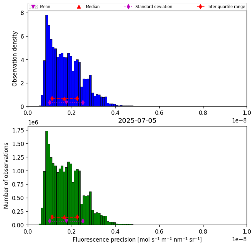
Figure 39: Histogram of “Fluorescence precision” for 2025-07-05 to 2025-07-06
