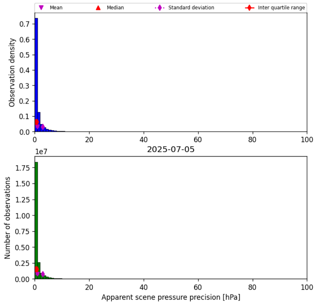
Figure 35: Histogram of “Apparent scene pressure precision” for 2025-07-05 to 2025-07-06
