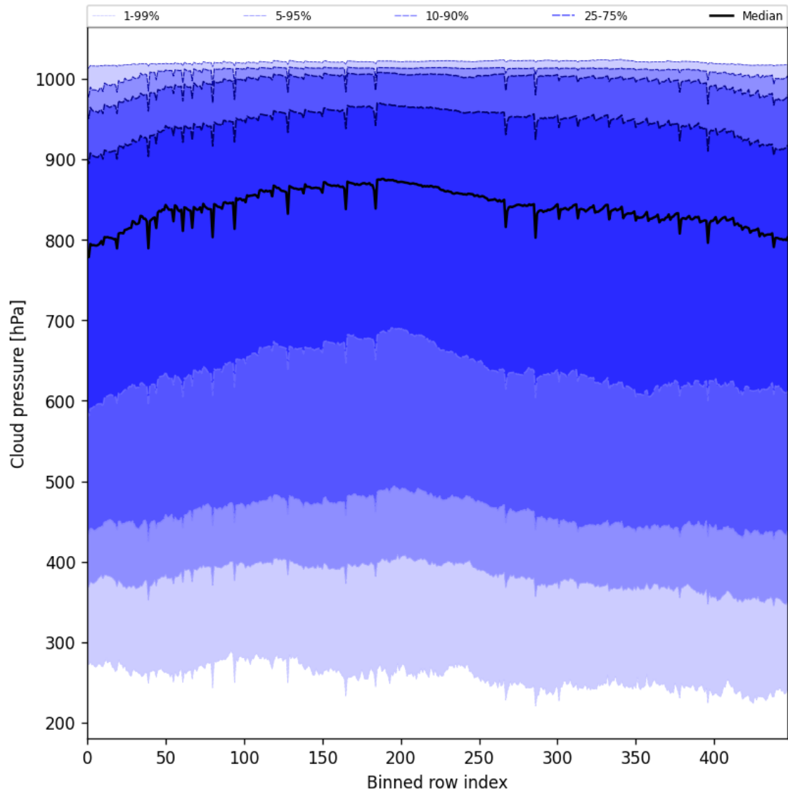
Figure 45: Along track statistics of “Cloud pressure” for 2025-07-05 to 2025-07-06
