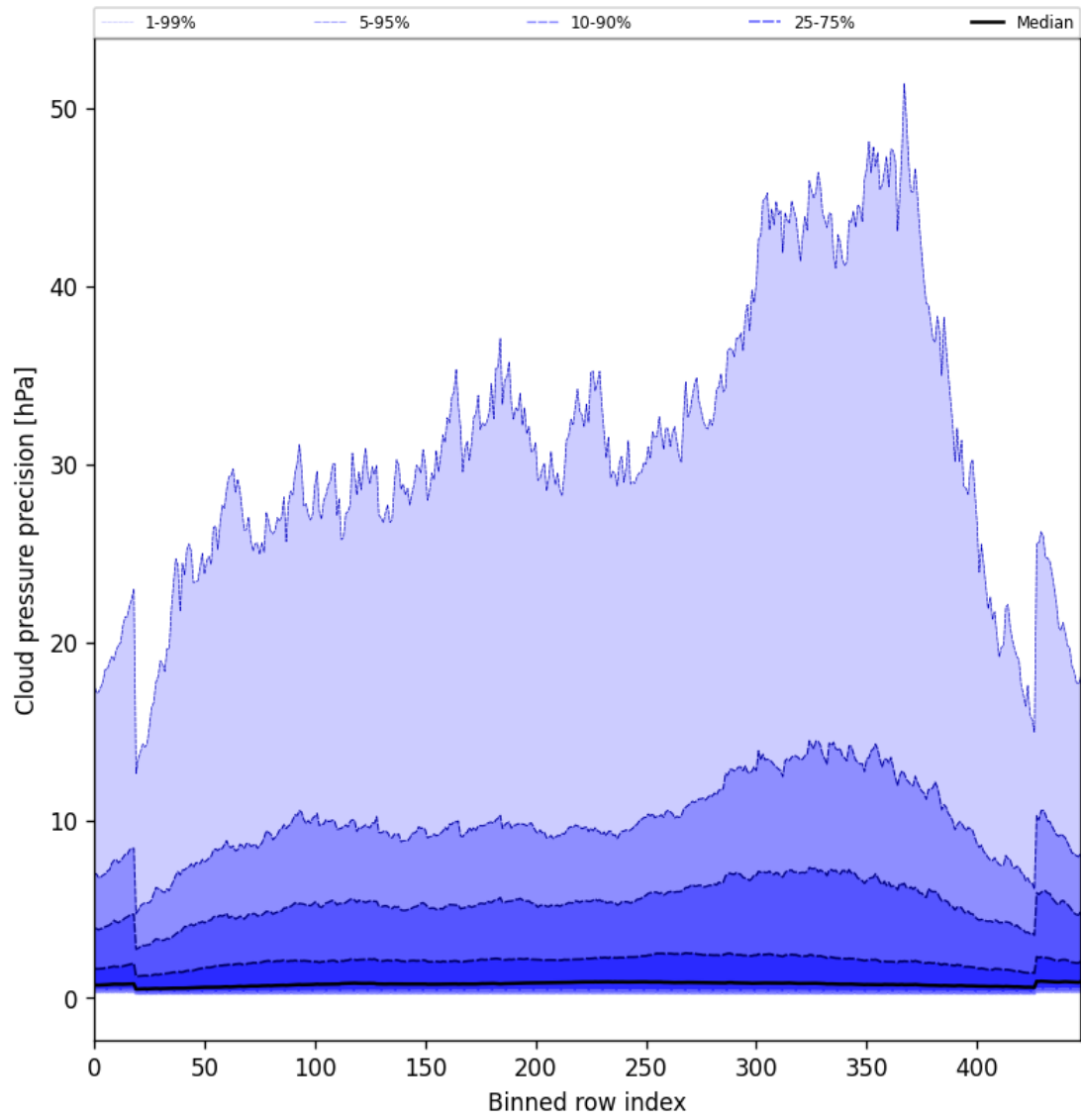
Figure 46: Along track statistics of “Cloud pressure precision” for 2025-07-05 to 2025-07-06
