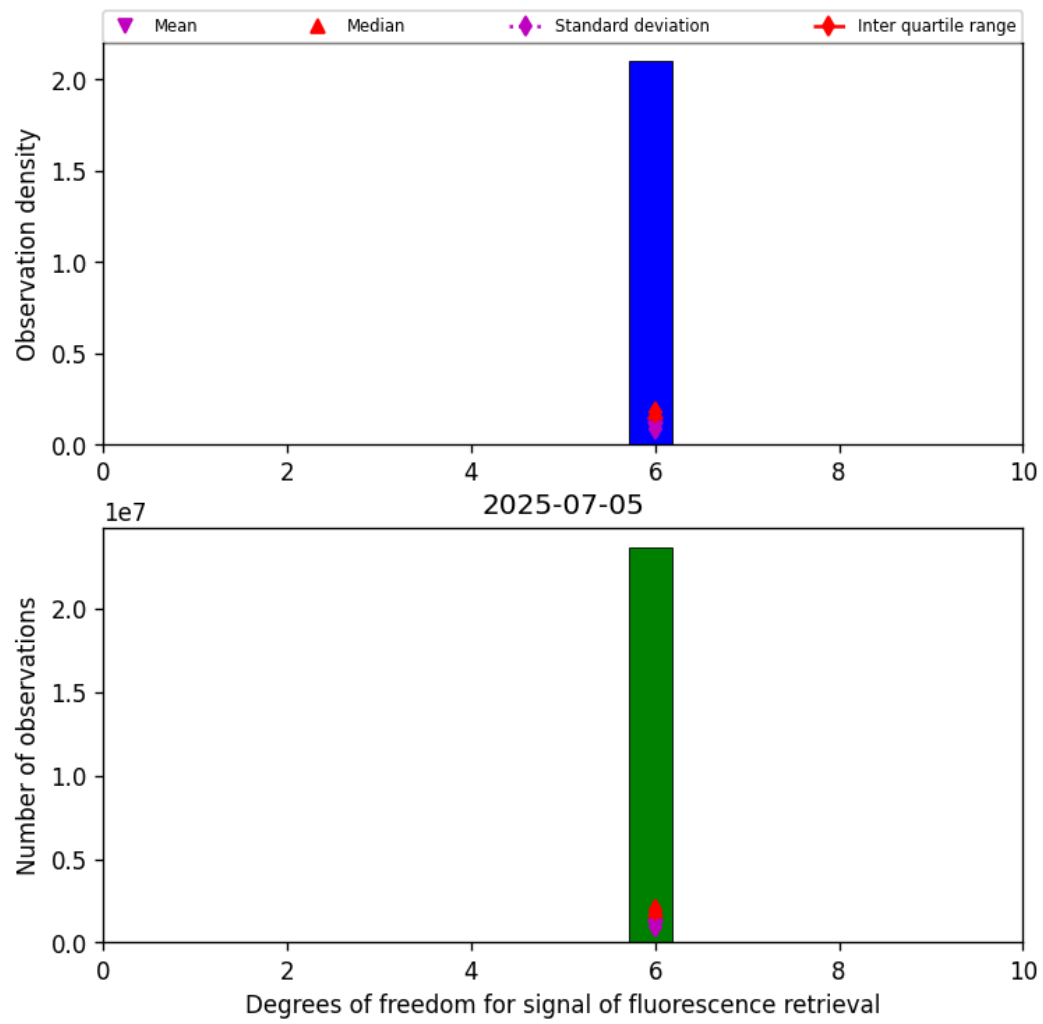
Figure 41: Histogram of “Degrees of freedom for signal of fluorescence retrieval” for 2025-07-05 to 2025-07-06
