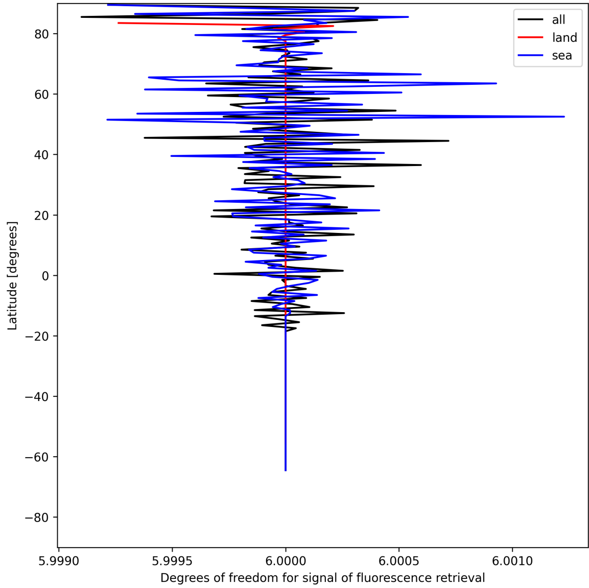
Figure 24: Zonal average of “Degrees of freedom for signal of fluorescence retrieval” for 2025-07-05 to 2025-07-06.
