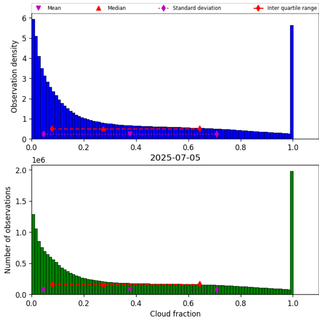
Figure 30: Histogram of “Cloud fraction” for 2025-07-05 to 2025-07-06
