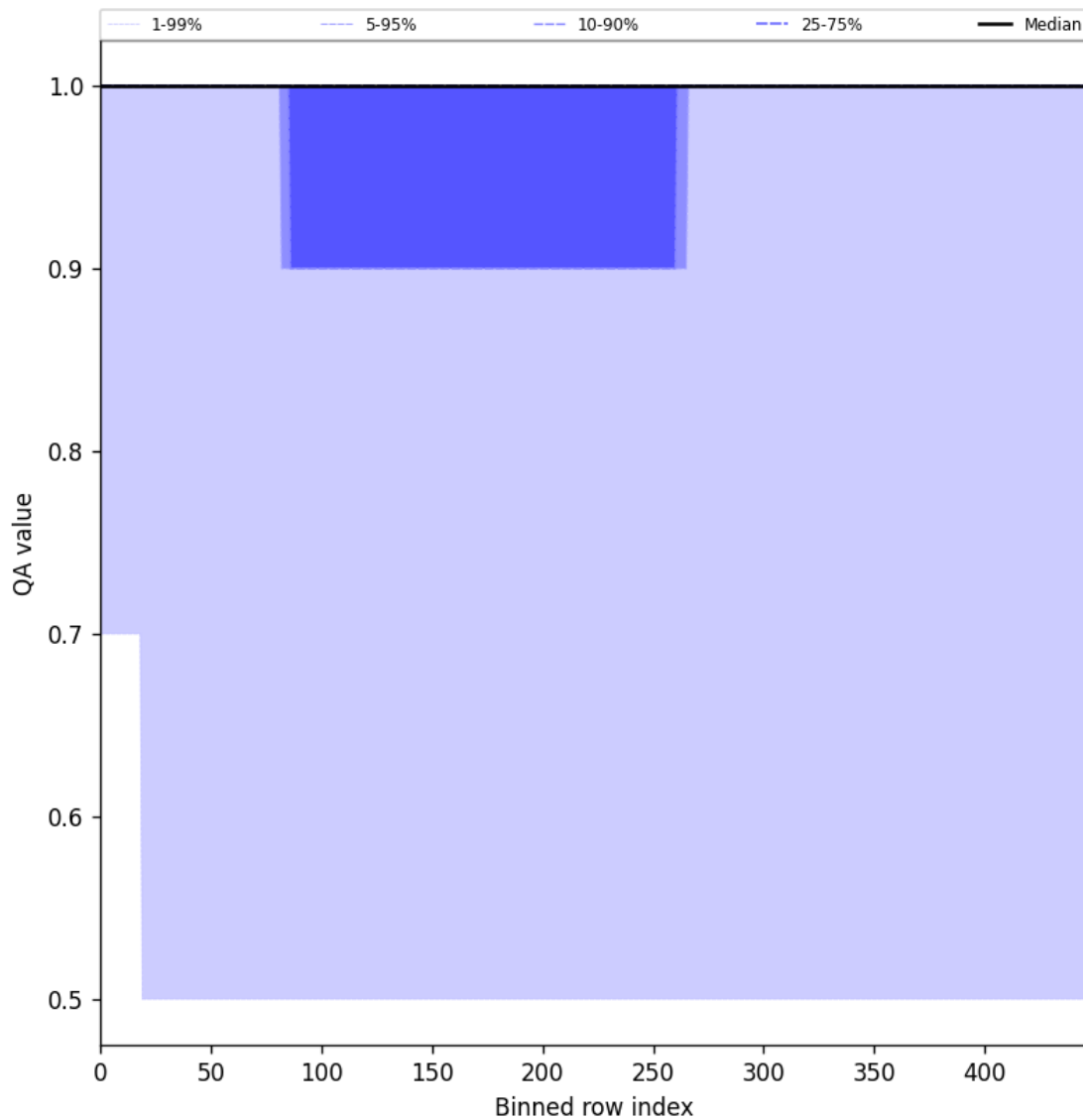
Figure 44: Along track statistics of “QA value” for 2025-07-08 to 2025-07-09
