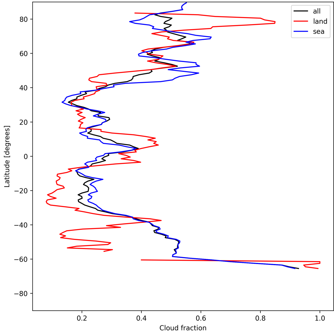
Figure 13: Zonal average of “Cloud fraction” for 2025-07-08 to 2025-07-09.
