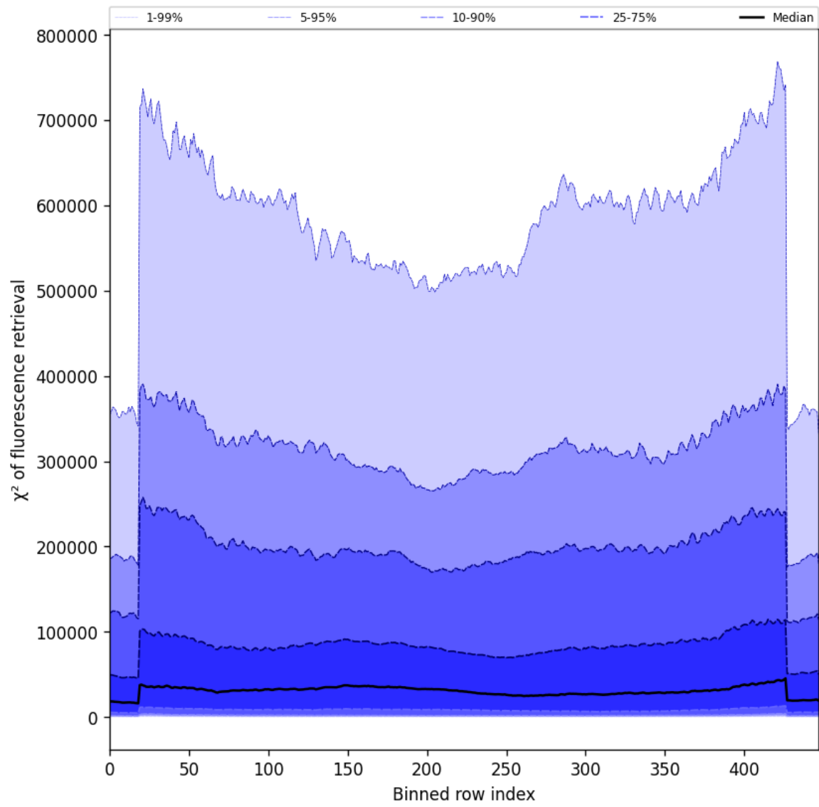
Figure 57: Along track statistics of “ \chi^2 of fluorescence retrieval” for 2025-07-08 to 2025-07-09
