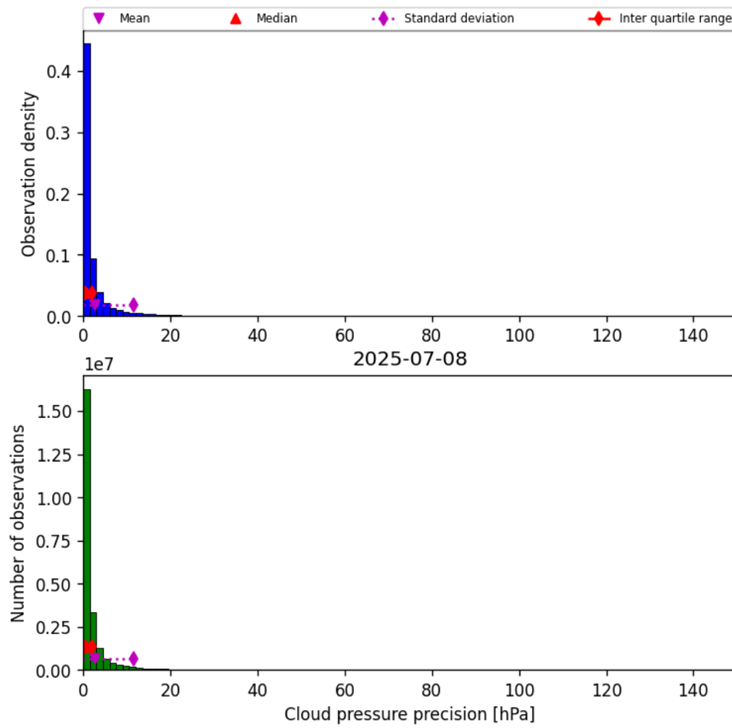
Figure 29: Histogram of “Cloud pressure precision” for 2025-07-08 to 2025-07-09
