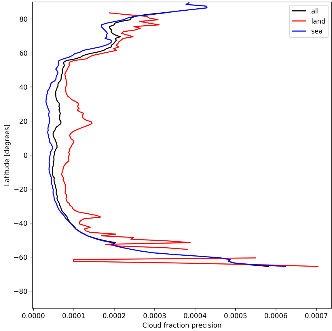
Figure 14: Zonal average of “Cloud fraction precision” for 2025-07-08 to 2025-07-09.
