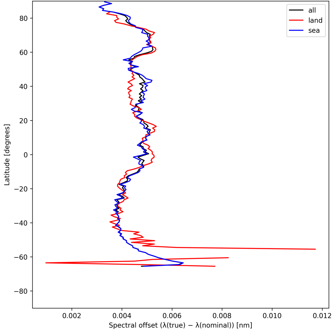
Figure 26: Zonal average of “Spectral offset ( \lambda_{\text{true}} - \lambda_{\text{nominal}} )” for 2025-07-08 to 2025-07-09.
