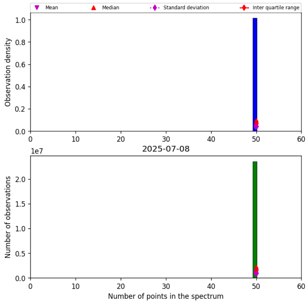
Figure 42: Histogram of “Number of points in the spectrum” for 2025-07-08 to 2025-07-09
