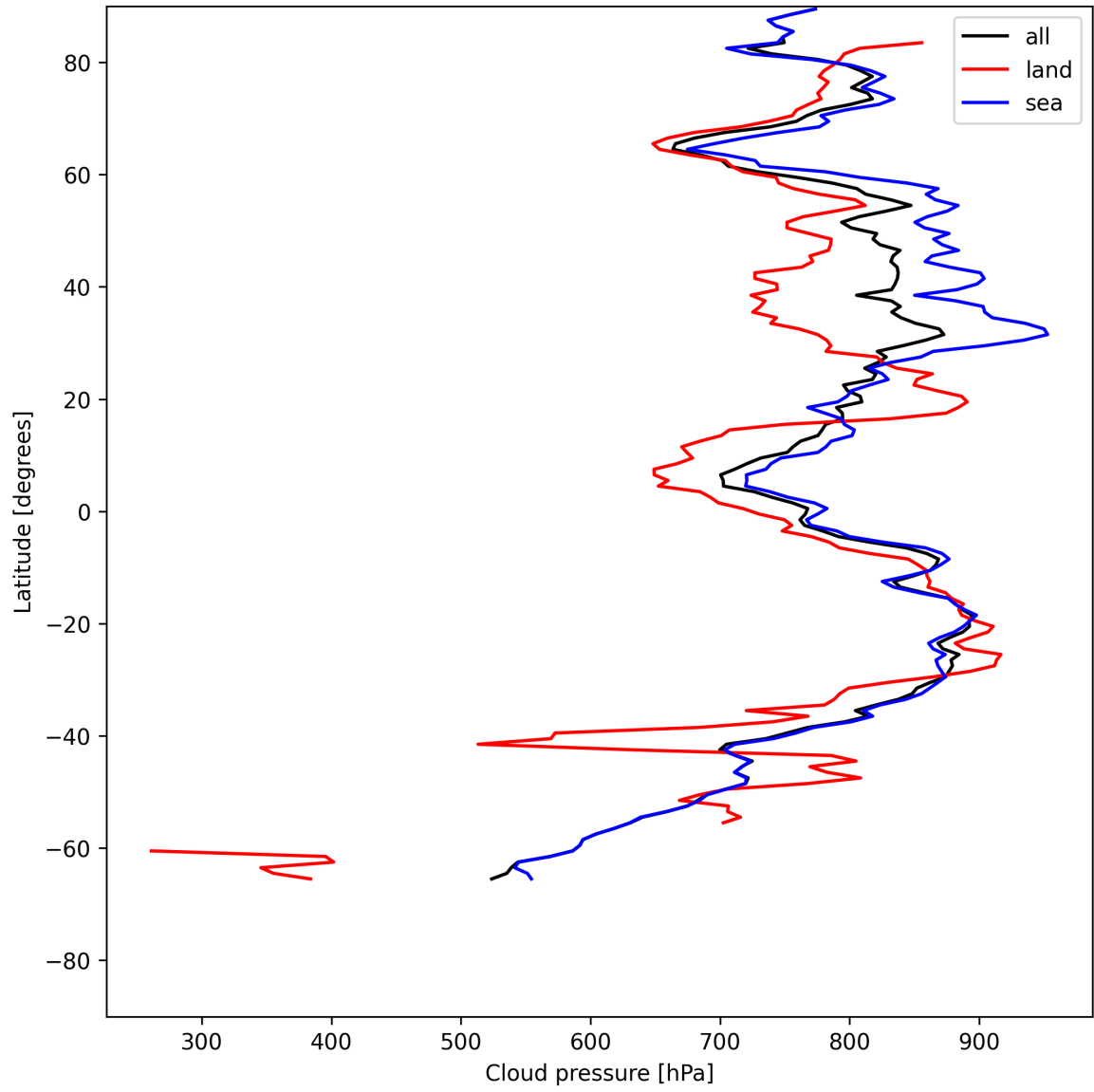
Figure 11: Zonal average of “Cloud pressure” for 2025-07-08 to 2025-07-09.
