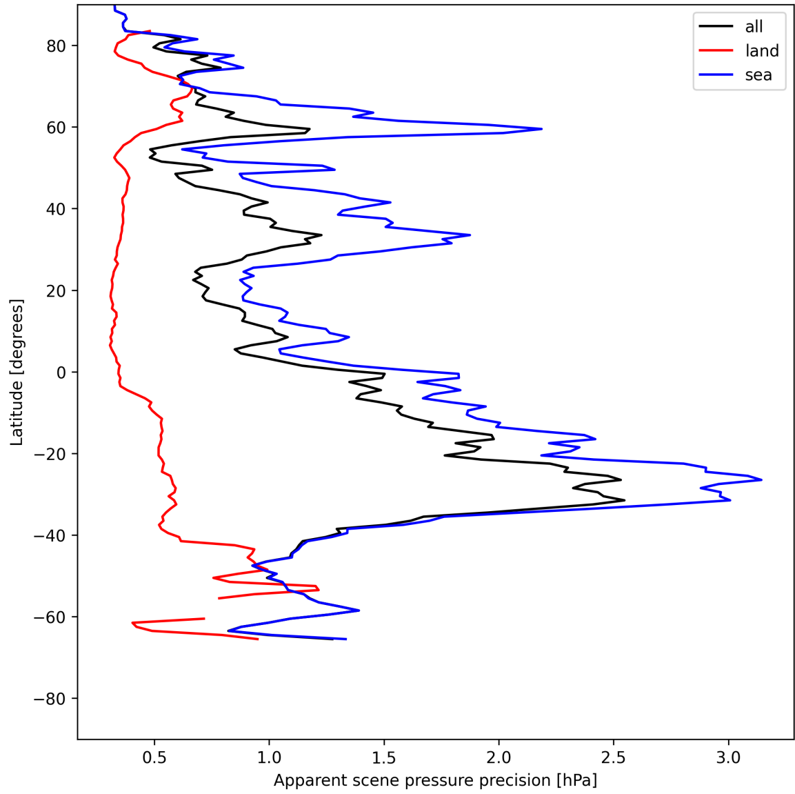
Figure 18: Zonal average of “Apparent scene pressure precision” for 2025-07-08 to 2025-07-09.
