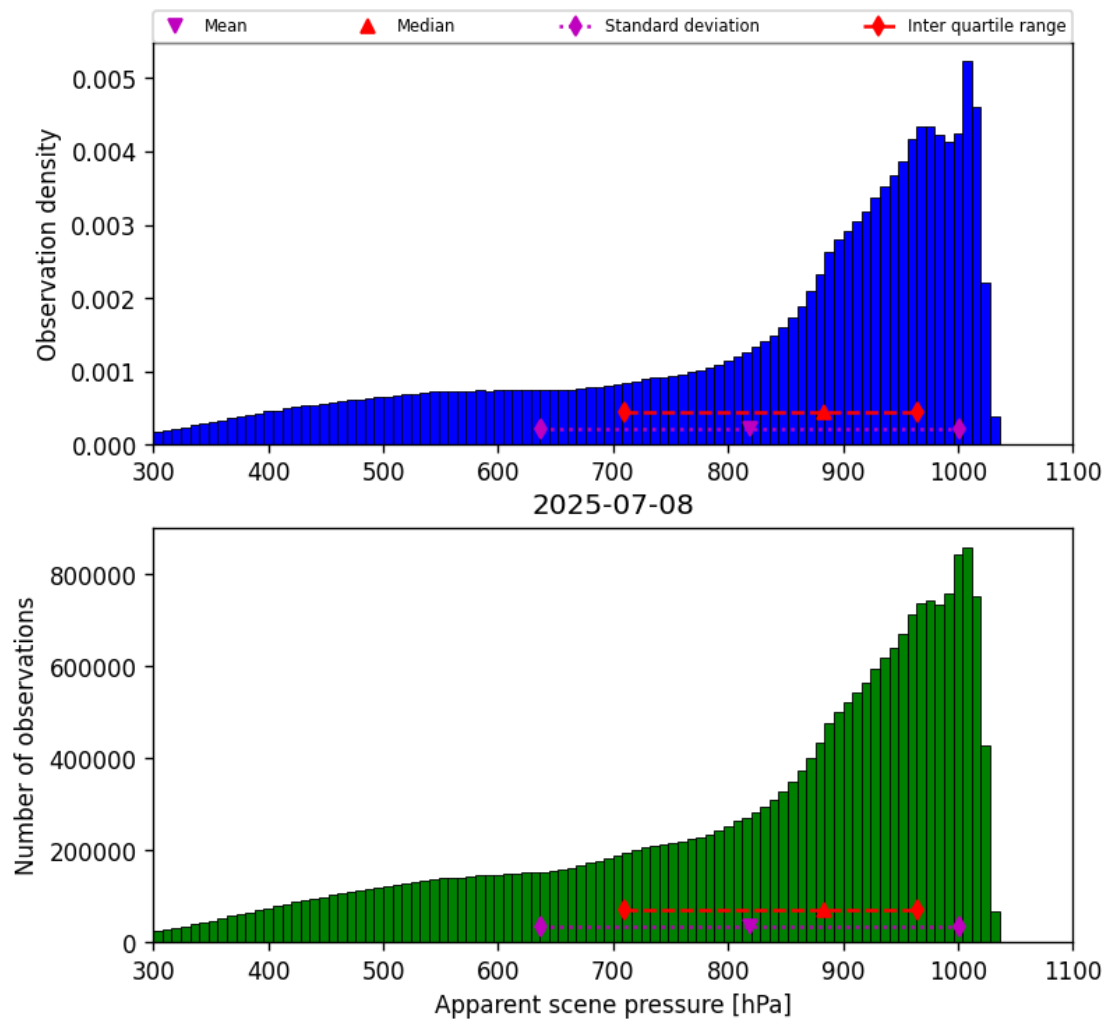
Figure 34: Histogram of “Apparent scene pressure” for 2025-07-08 to 2025-07-09
