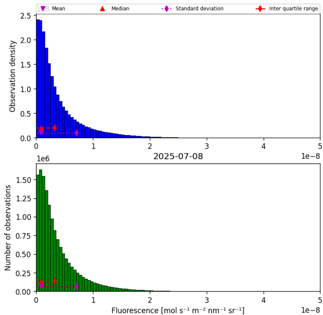
Figure 38: Histogram of “Fluorescence” for 2025-07-08 to 2025-07-09
