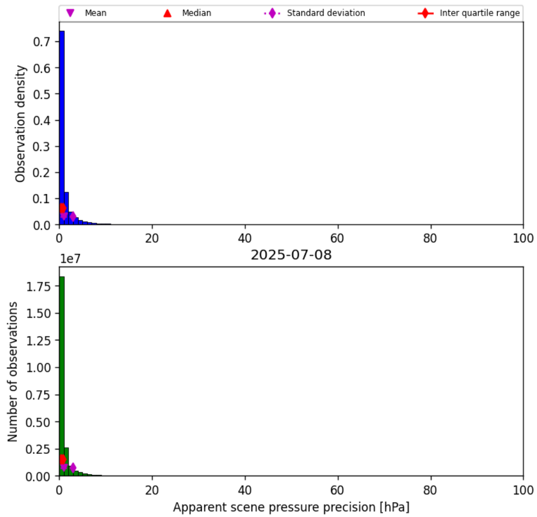
Figure 35: Histogram of “Apparent scene pressure precision” for 2025-07-08 to 2025-07-09
