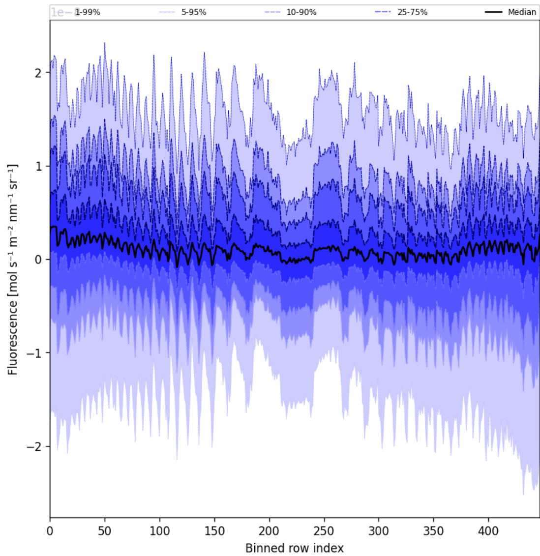
Figure 55: Along track statistics of “Fluorescence” for 2025-07-08 to 2025-07-09
