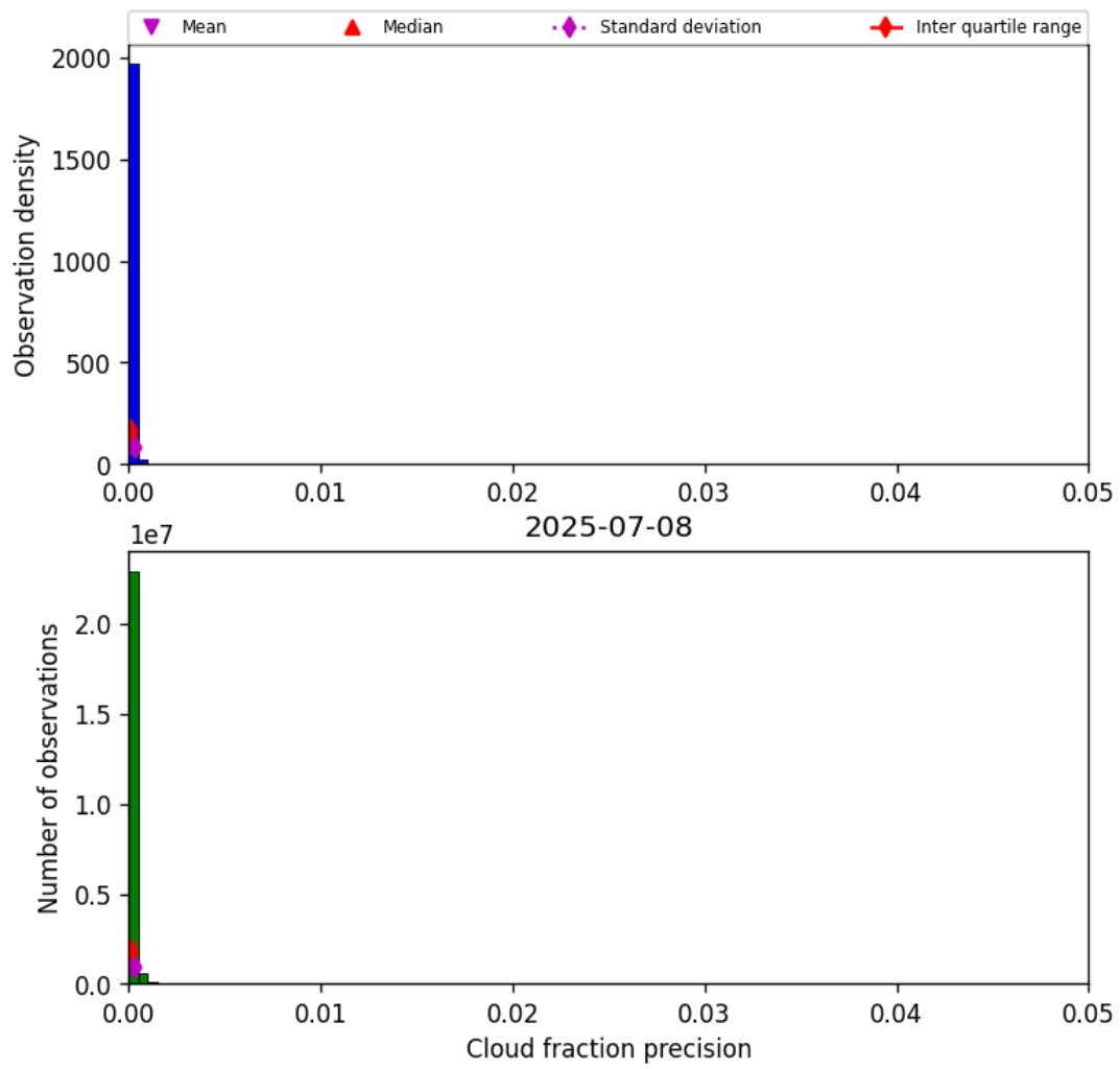
Figure 31: Histogram of “Cloud fraction precision” for 2025-07-08 to 2025-07-09
