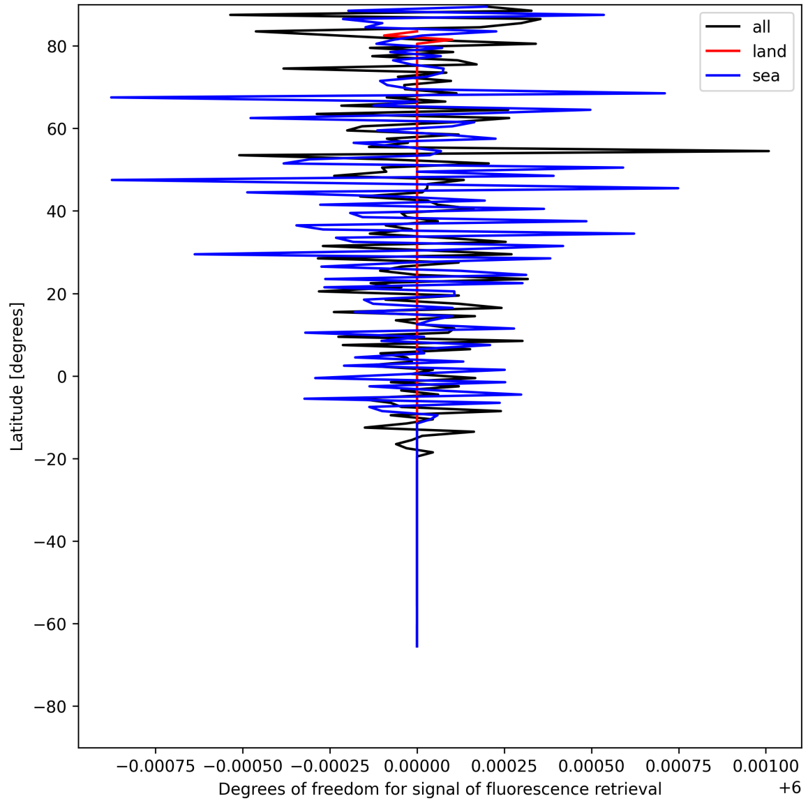
Figure 24: Zonal average of “Degrees of freedom for signal of fluorescence retrieval” for 2025-07-08 to 2025-07-09.
