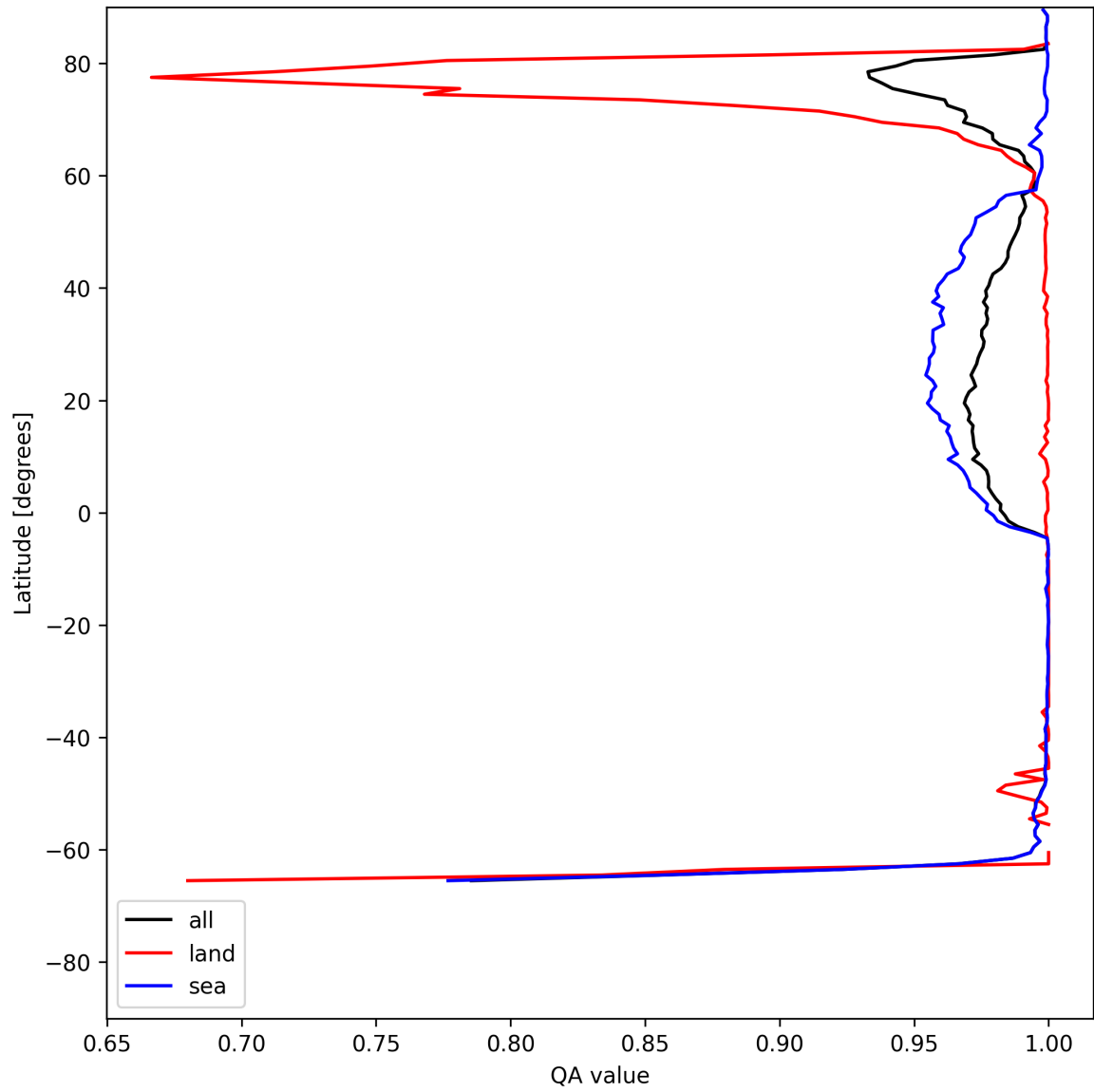
Figure 10: Zonal average of “QA value” for 2025-07-08 to 2025-07-09.
