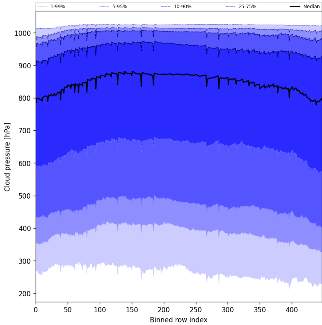
Figure 45: Along track statistics of “Cloud pressure” for 2025-07-08 to 2025-07-09
