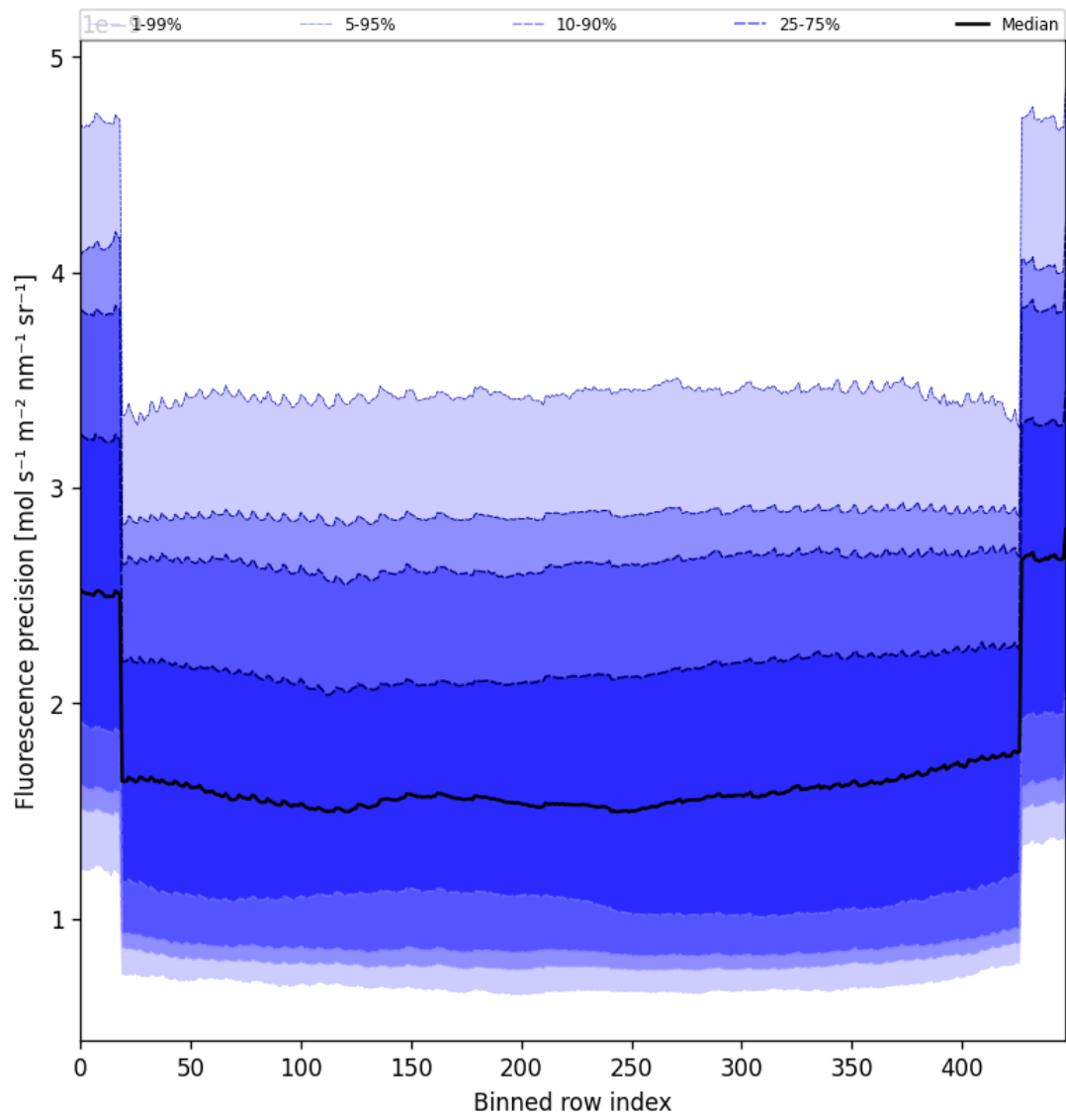
Figure 56: Along track statistics of “Fluorescence precision” for 2025-07-08 to 2025-07-09
