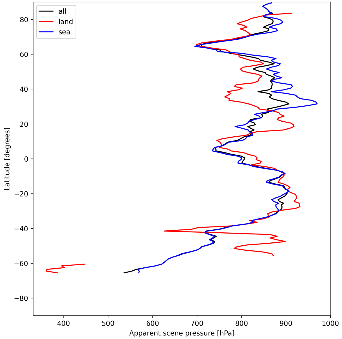
Figure 17: Zonal average of “Apparent scene pressure” for 2025-07-08 to 2025-07-09.
