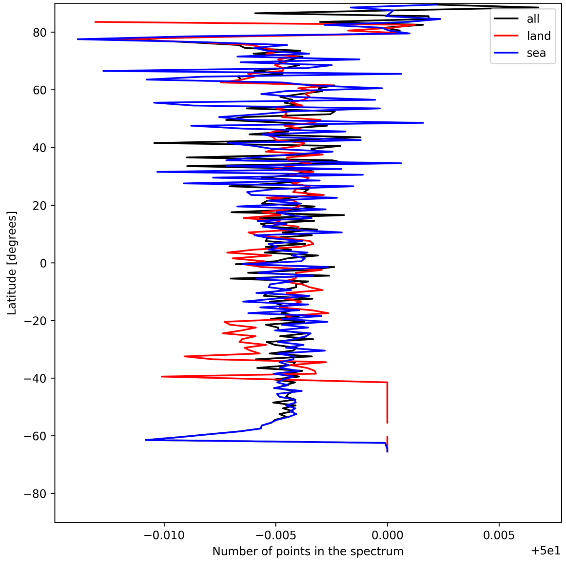
Figure 25: Zonal average of “Number of points in the spectrum” for 2025-07-08 to 2025-07-09.
