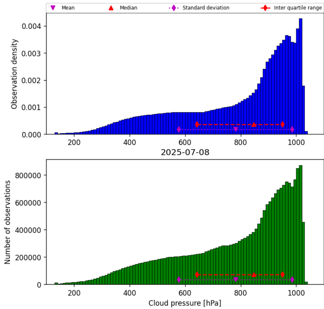
Figure 28: Histogram of “Cloud pressure” for 2025-07-08 to 2025-07-09
