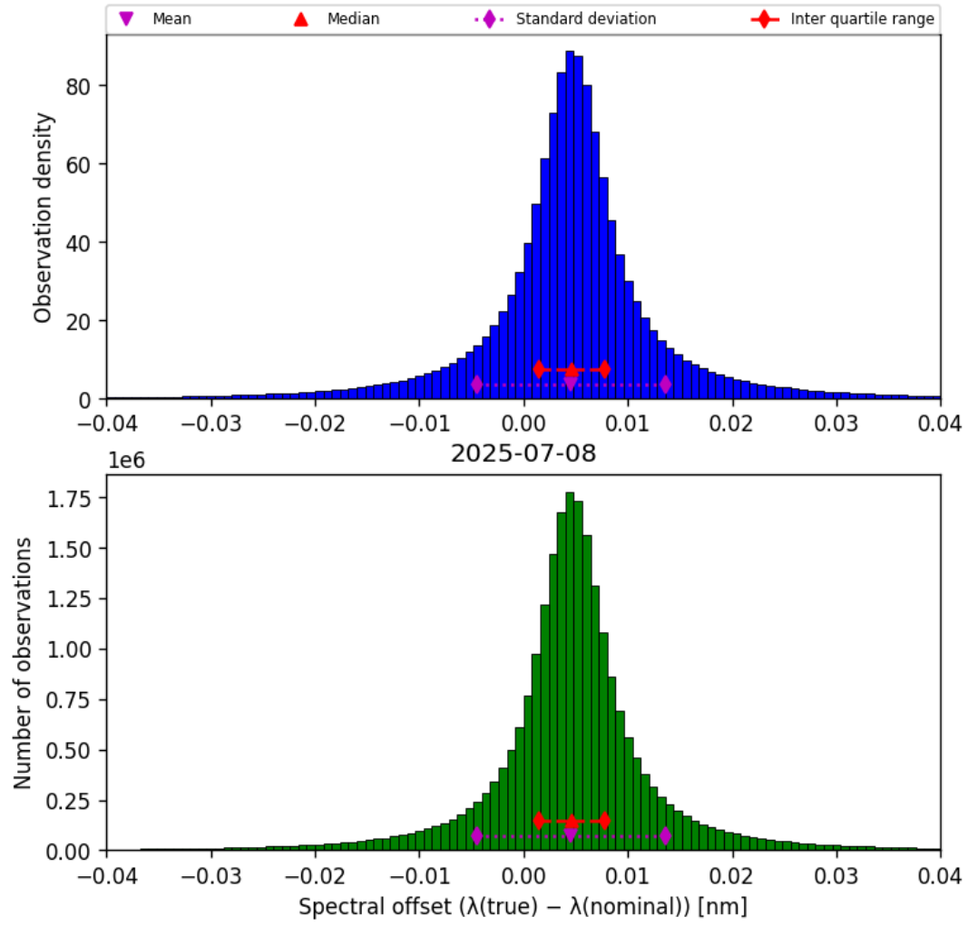
Figure 43: Histogram of “Spectral offset ( \lambda_{\text{true}} - \lambda_{\text{nominal}} )” for 2025-07-08 to 2025-07-09
