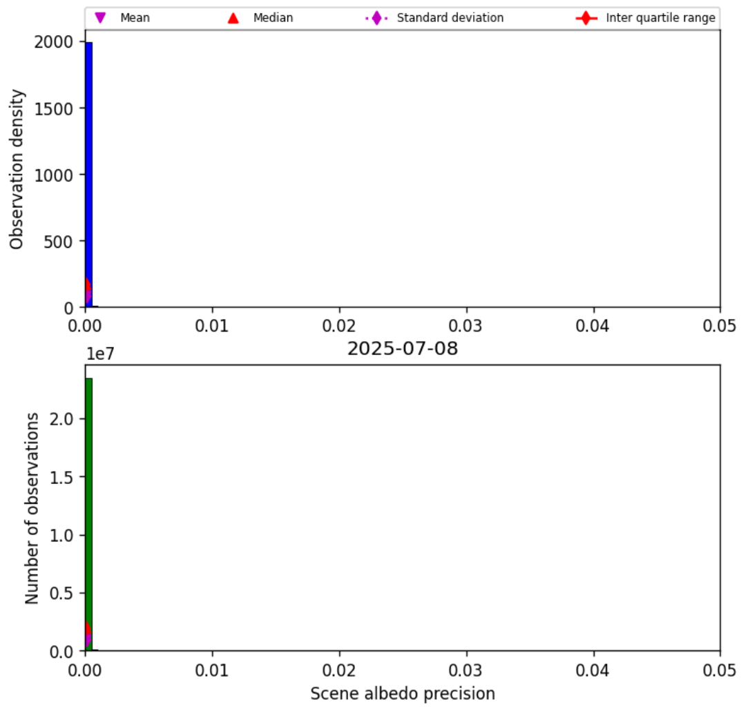
Figure 33: Histogram of “Scene albedo precision” for 2025-07-08 to 2025-07-09
