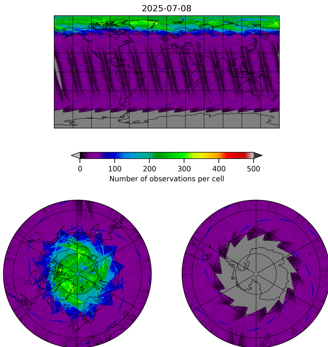
Figure 9: Map of the number of observations for 2025-07-08 to 2025-07-09
