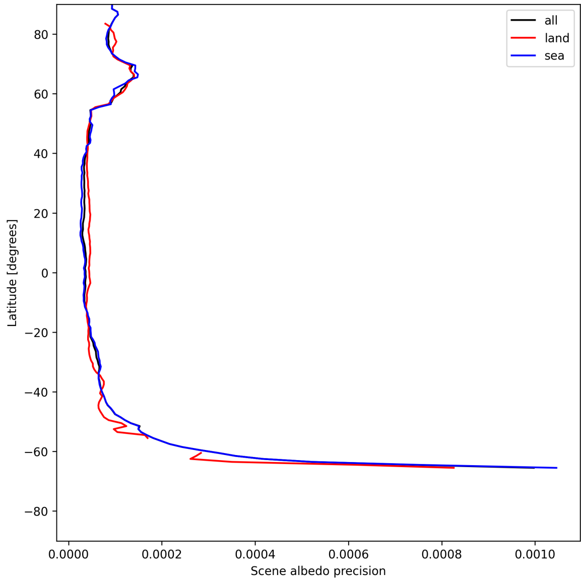
Figure 16: Zonal average of “Scene albedo precision” for 2025-07-08 to 2025-07-09.
