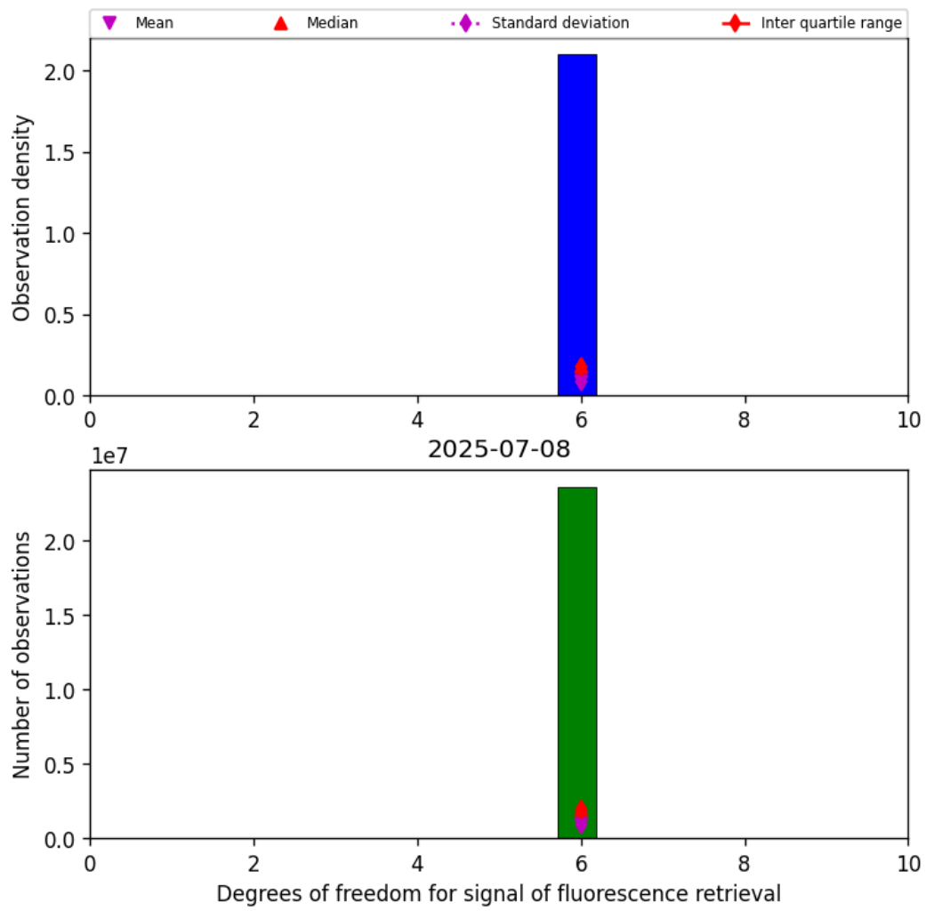
Figure 41: Histogram of “Degrees of freedom for signal of fluorescence retrieval” for 2025-07-08 to 2025-07-09
