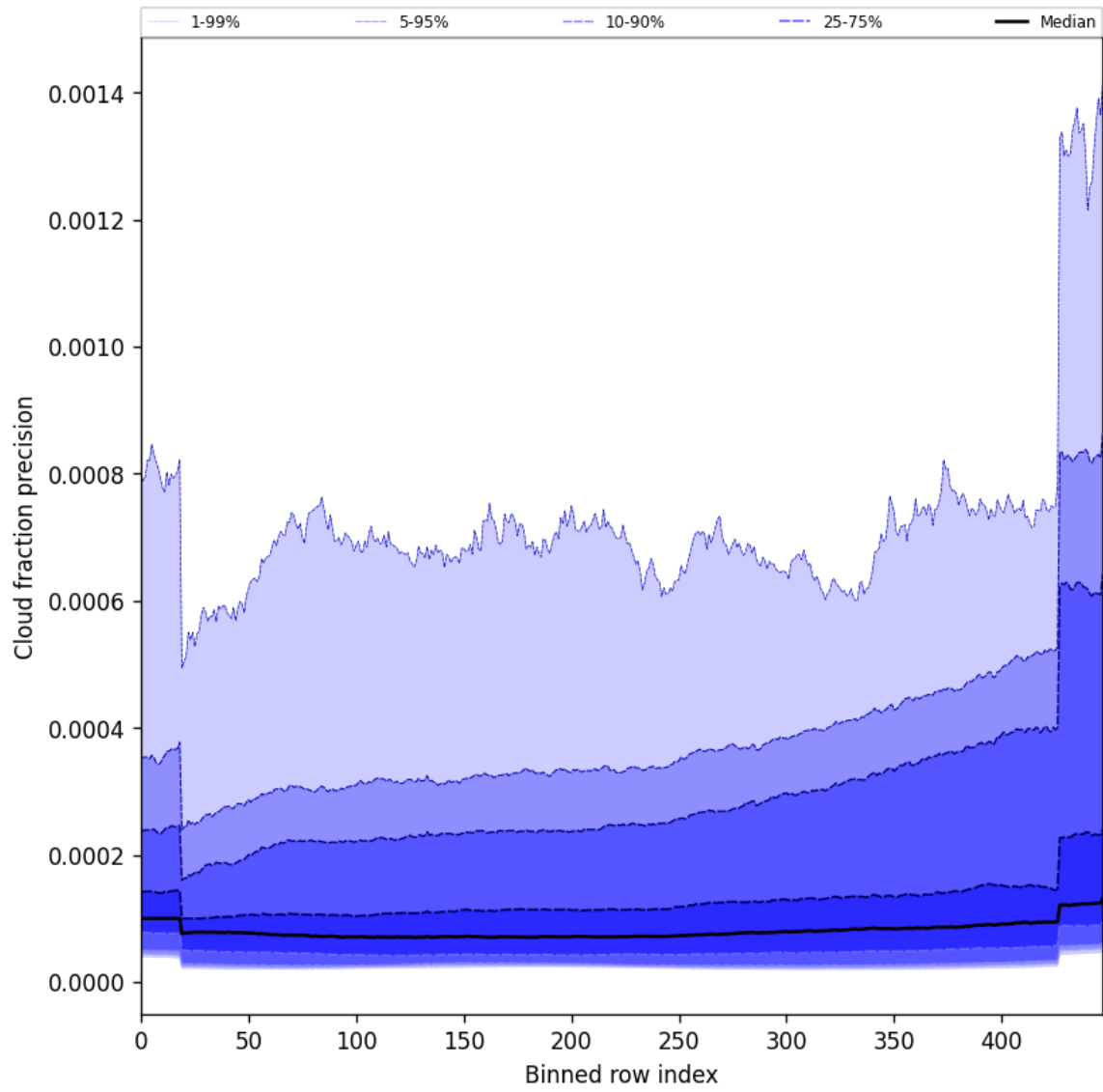
Figure 48: Along track statistics of “Cloud fraction precision” for 2025-07-08 to 2025-07-09
