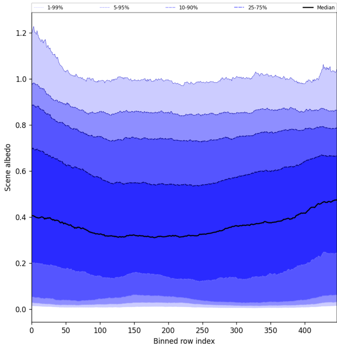
Figure 49: Along track statistics of “Scene albedo” for 2025-07-08 to 2025-07-09
