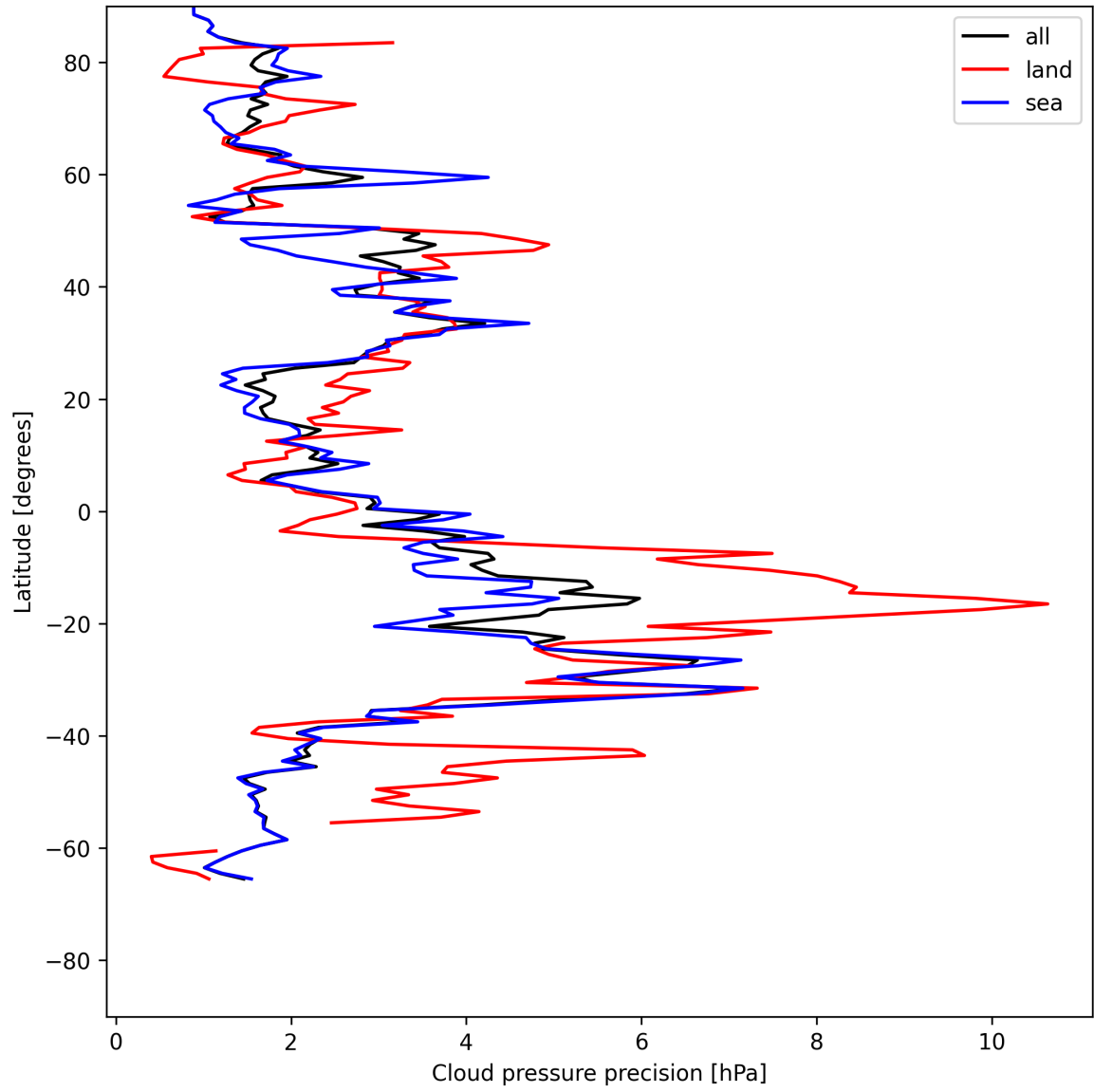
Figure 12: Zonal average of “Cloud pressure precision” for 2025-07-08 to 2025-07-09.
