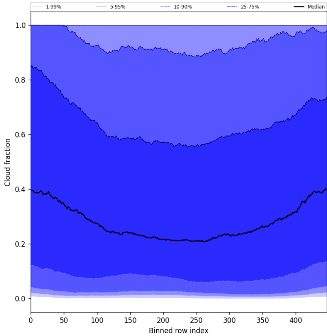
Figure 47: Along track statistics of “Cloud fraction” for 2025-07-08 to 2025-07-09
