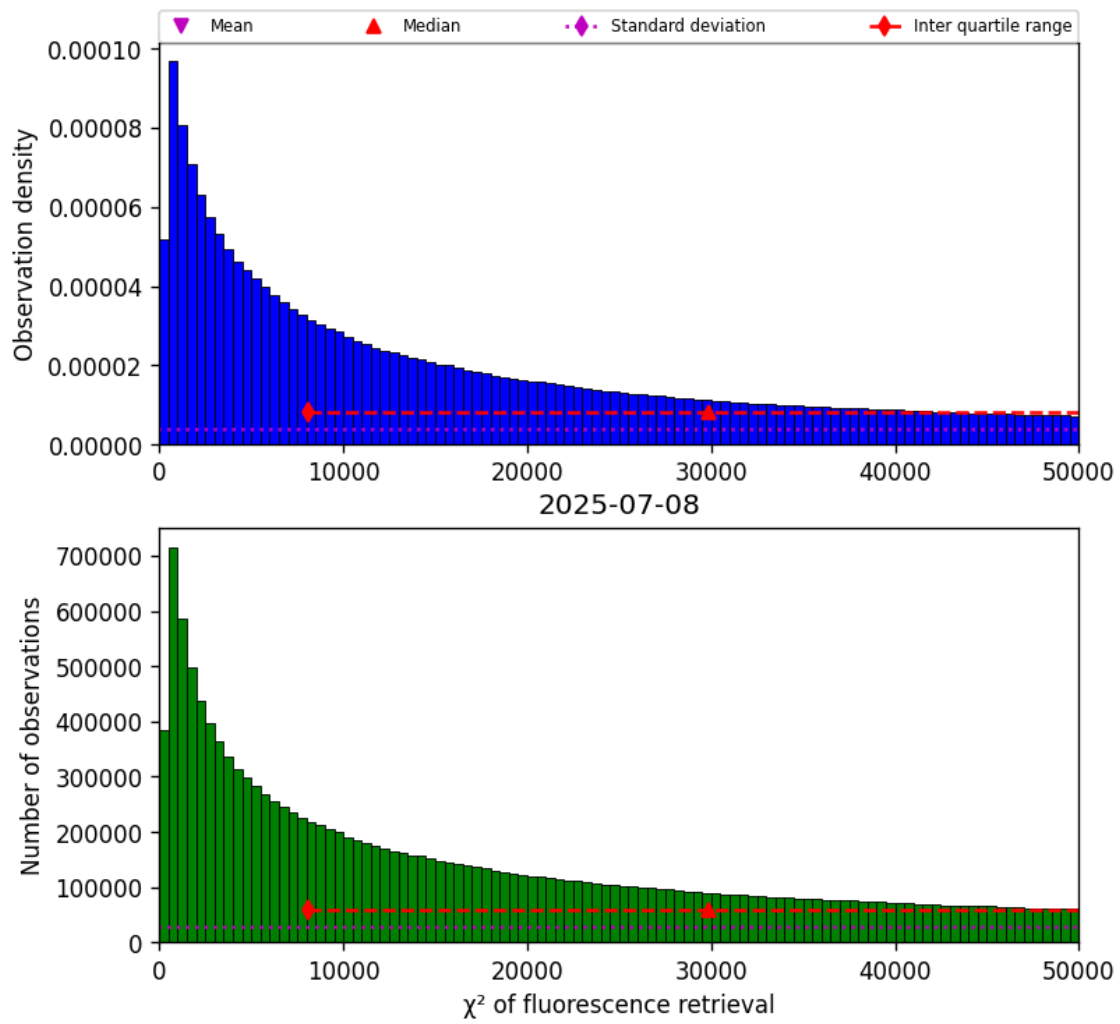
Figure 40: Histogram of “ \chi^2 of fluorescence retrieval” for 2025-07-08 to 2025-07-09
