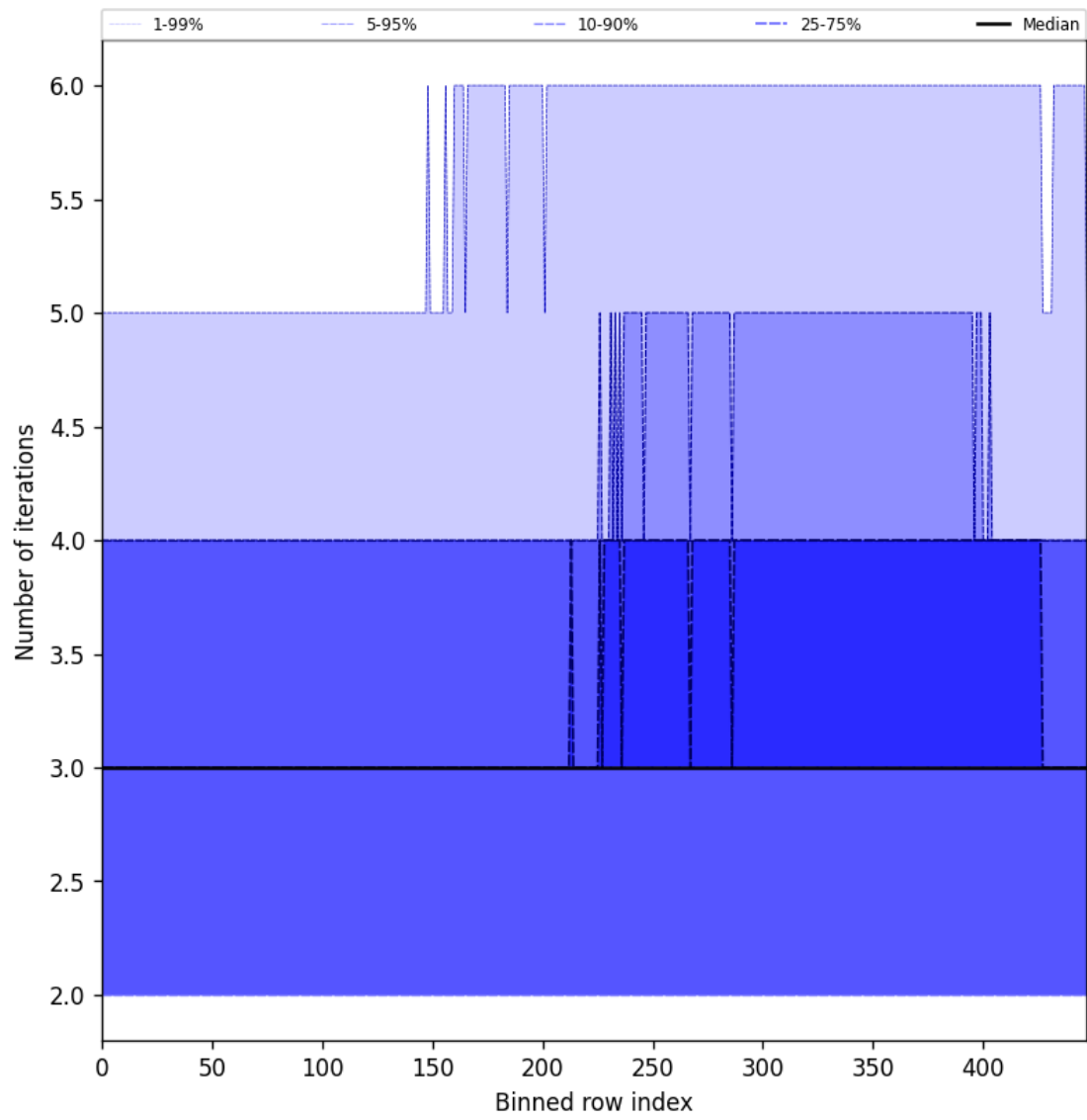
Figure 54: Along track statistics of “Number of iterations” for 2025-07-08 to 2025-07-09
