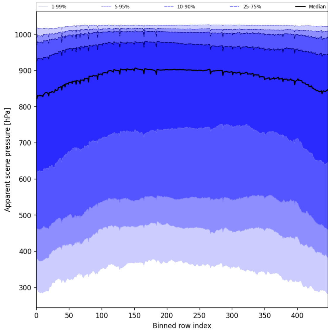
Figure 51: Along track statistics of “Apparent scene pressure” for 2025-07-08 to 2025-07-09
