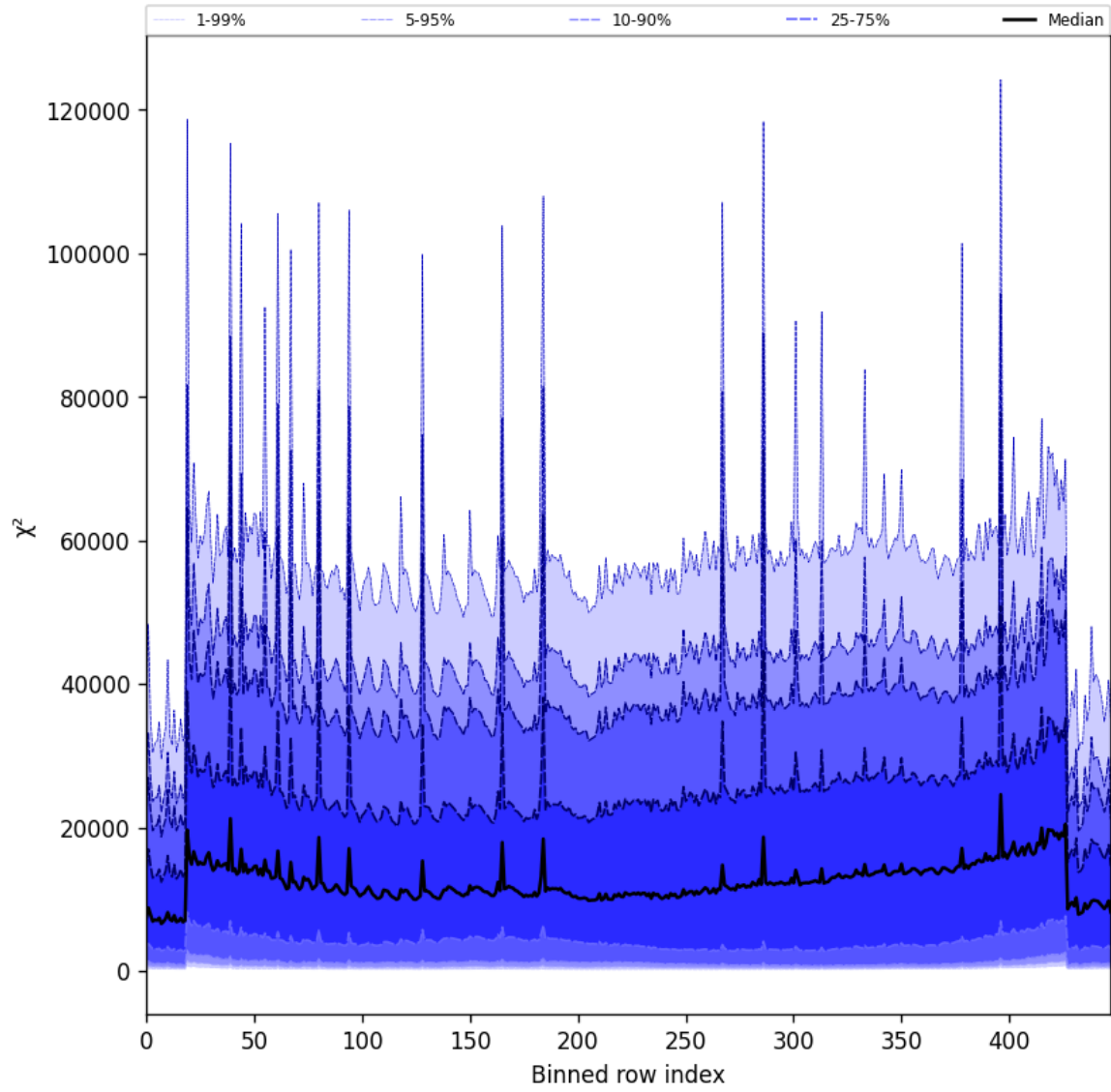
Figure 53: Along track statistics of “ \chi^2 ” for 2025-07-08 to 2025-07-09
