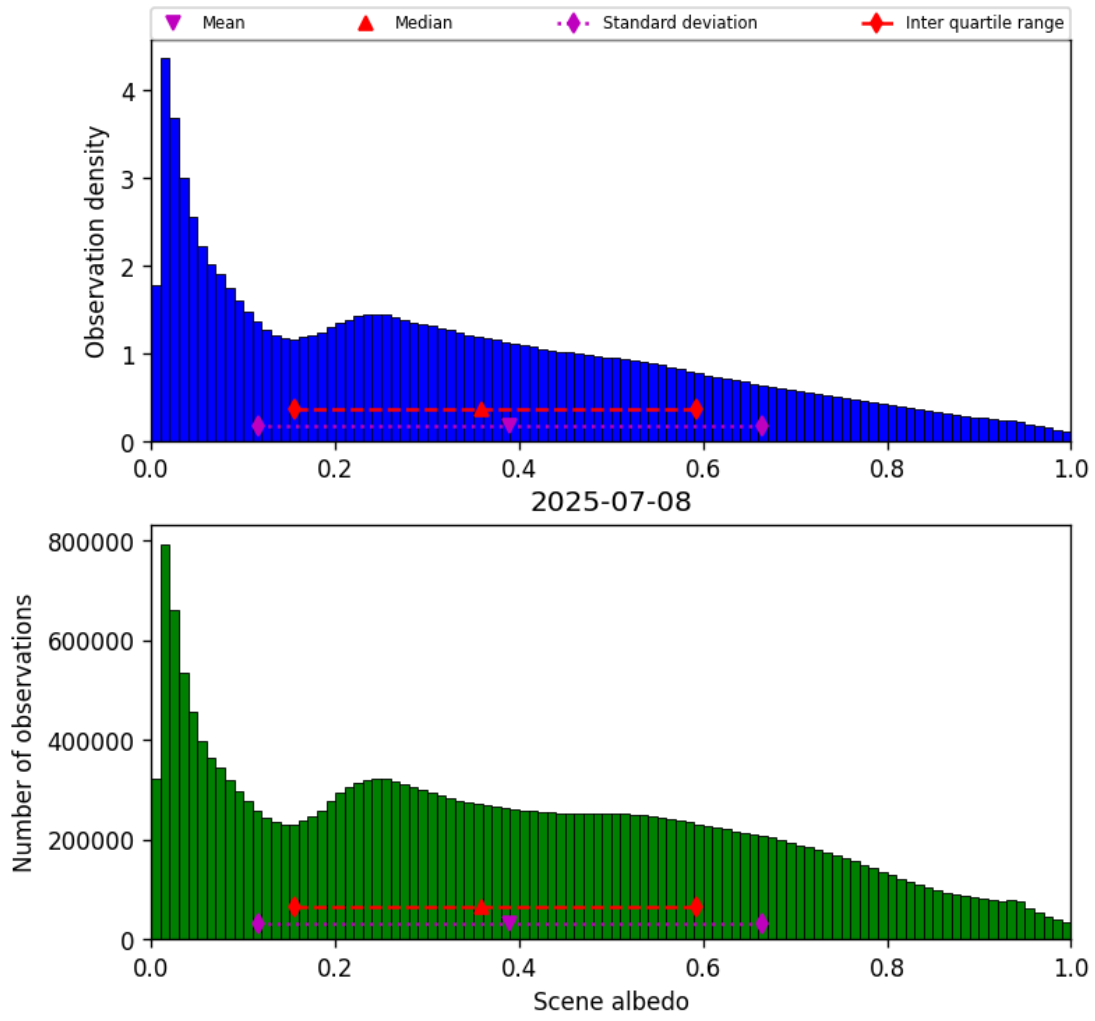
Figure 32: Histogram of “Scene albedo” for 2025-07-08 to 2025-07-09
