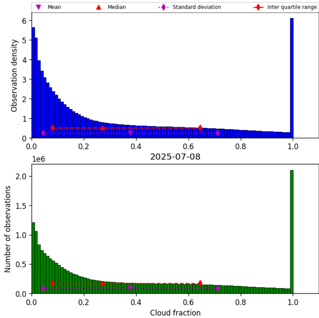
Figure 30: Histogram of “Cloud fraction” for 2025-07-08 to 2025-07-09
