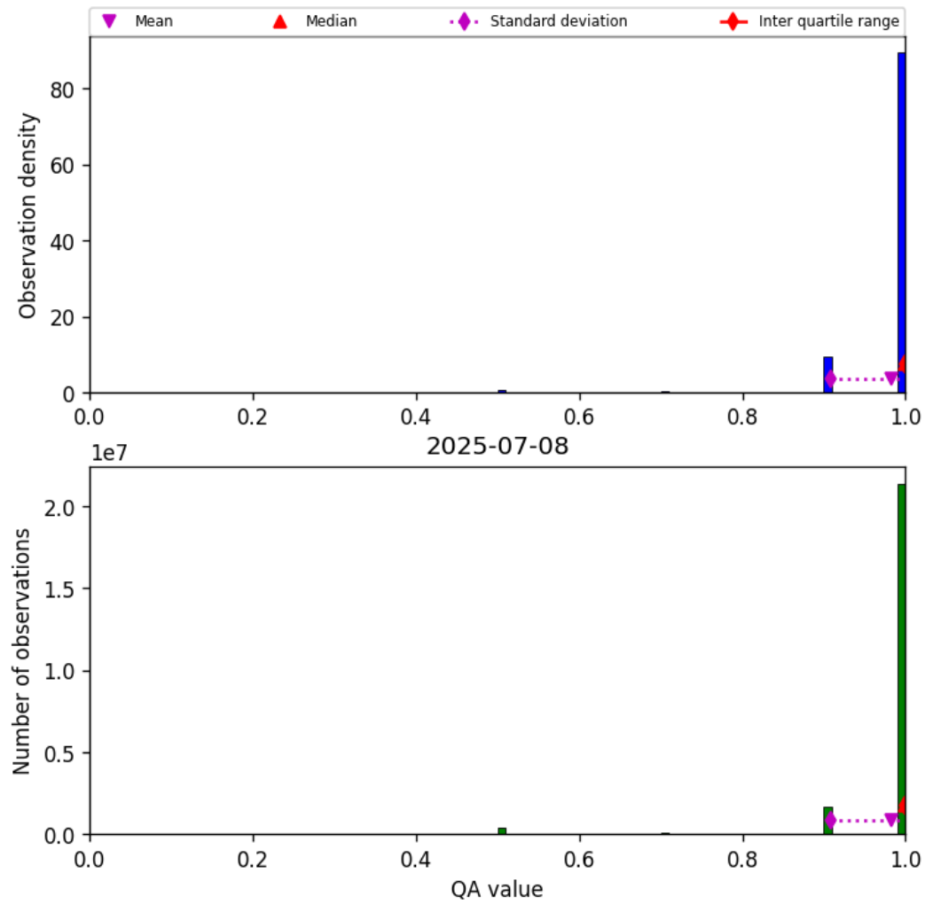
Figure 27: Histogram of “QA value” for 2025-07-08 to 2025-07-09
