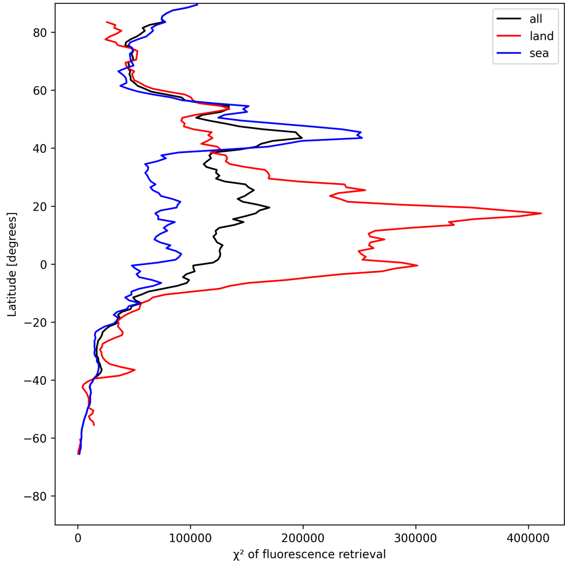
Figure 23: Zonal average of “ \chi^2 of fluorescence retrieval” for 2025-07-08 to 2025-07-09.
