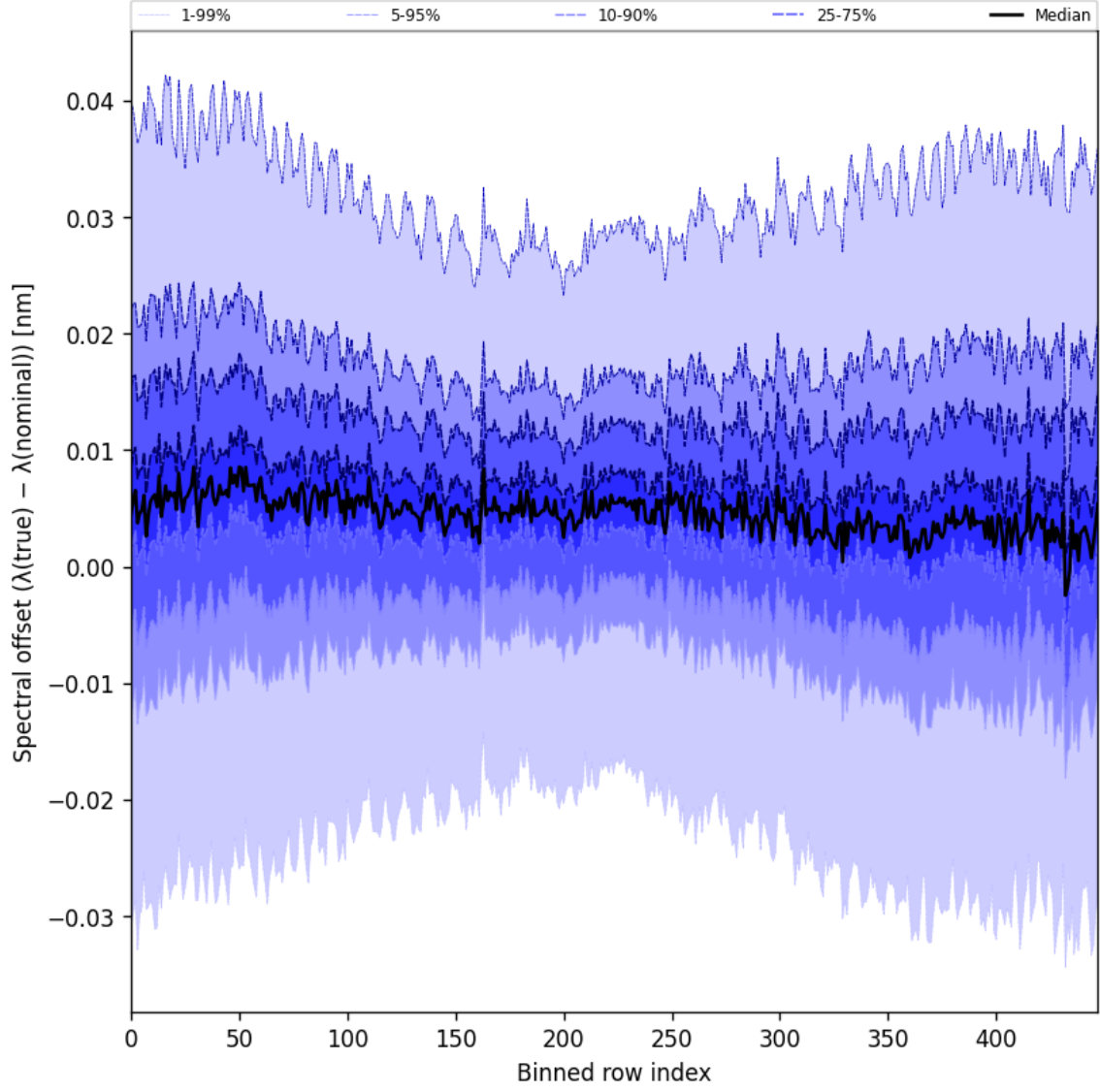
Figure 60: Along track statistics of “Spectral offset ( \lambda_{\text{true}} - \lambda_{\text{nominal}} )” for 2025-07-08 to 2025-07-09
