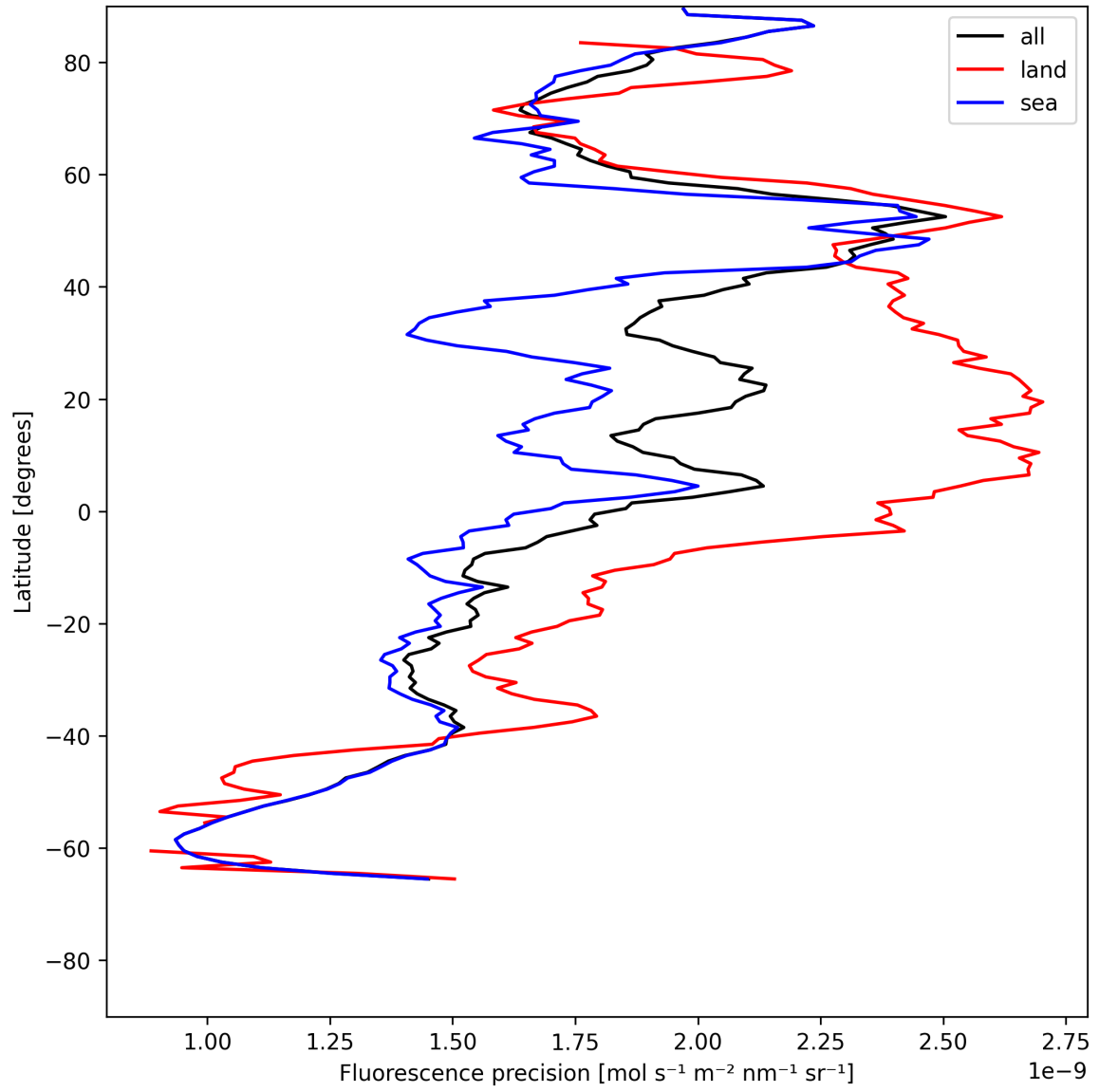
Figure 22: Zonal average of “Fluorescence precision” for 2025-07-08 to 2025-07-09.
