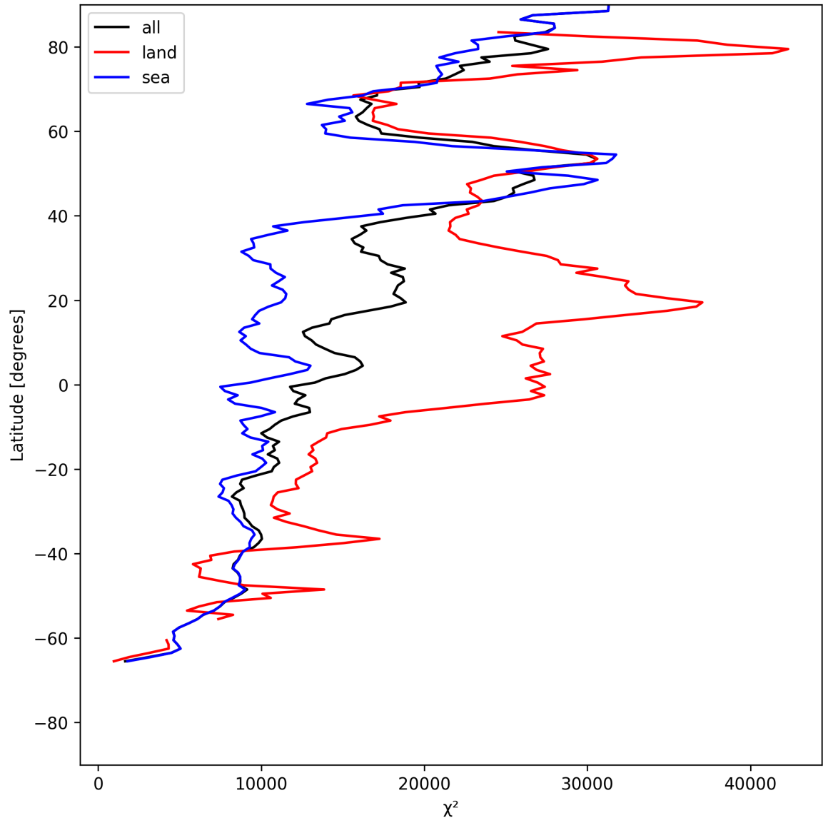
Figure 19: Zonal average of “ \chi^2 ” for 2025-07-08 to 2025-07-09.
