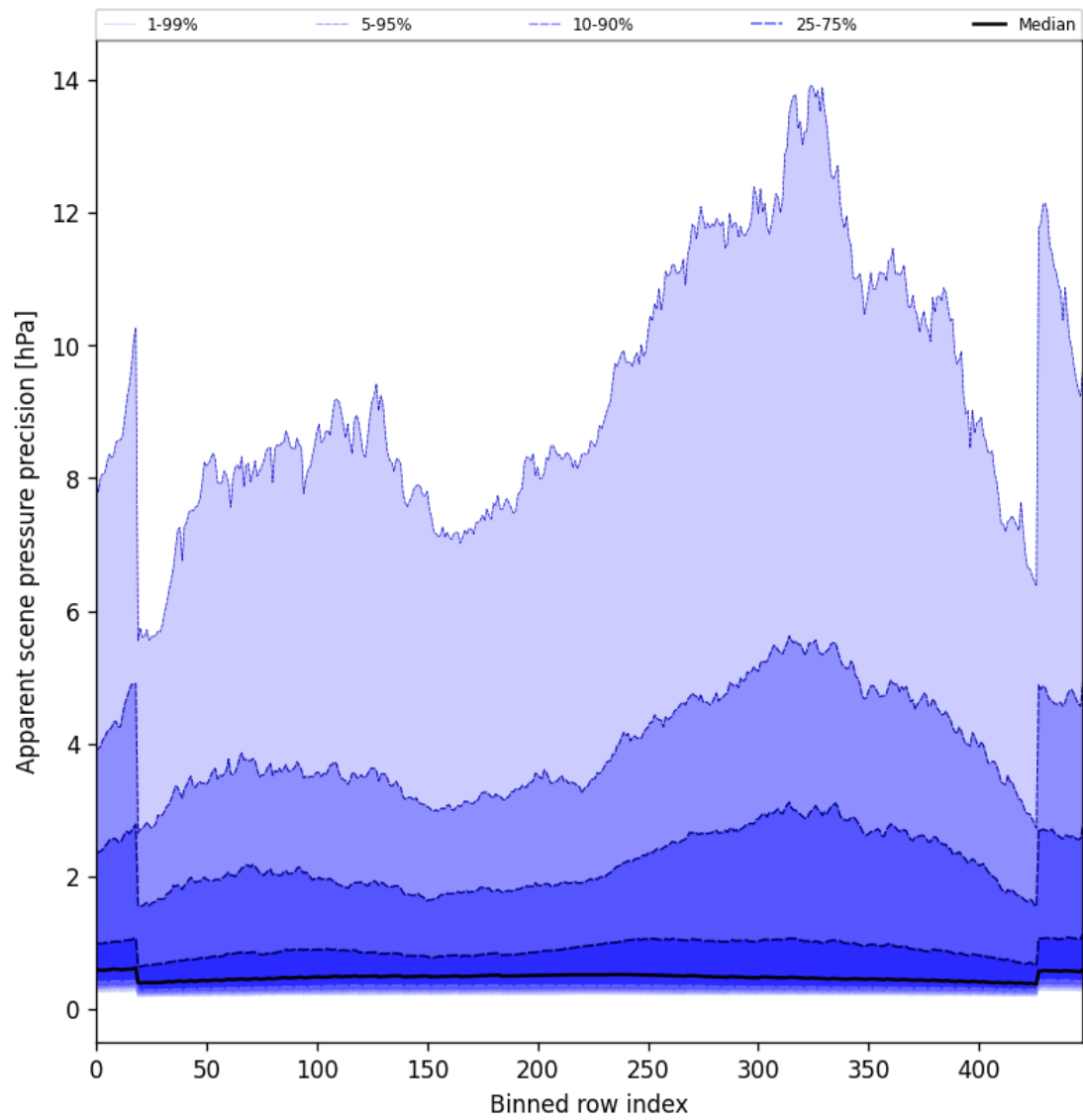
Figure 52: Along track statistics of “Apparent scene pressure precision” for 2025-07-08 to 2025-07-09
