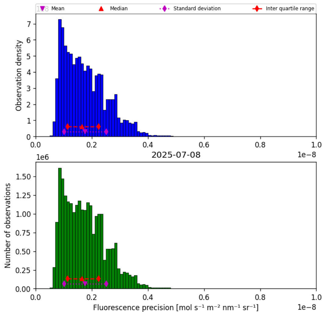
Figure 39: Histogram of “Fluorescence precision” for 2025-07-08 to 2025-07-09
