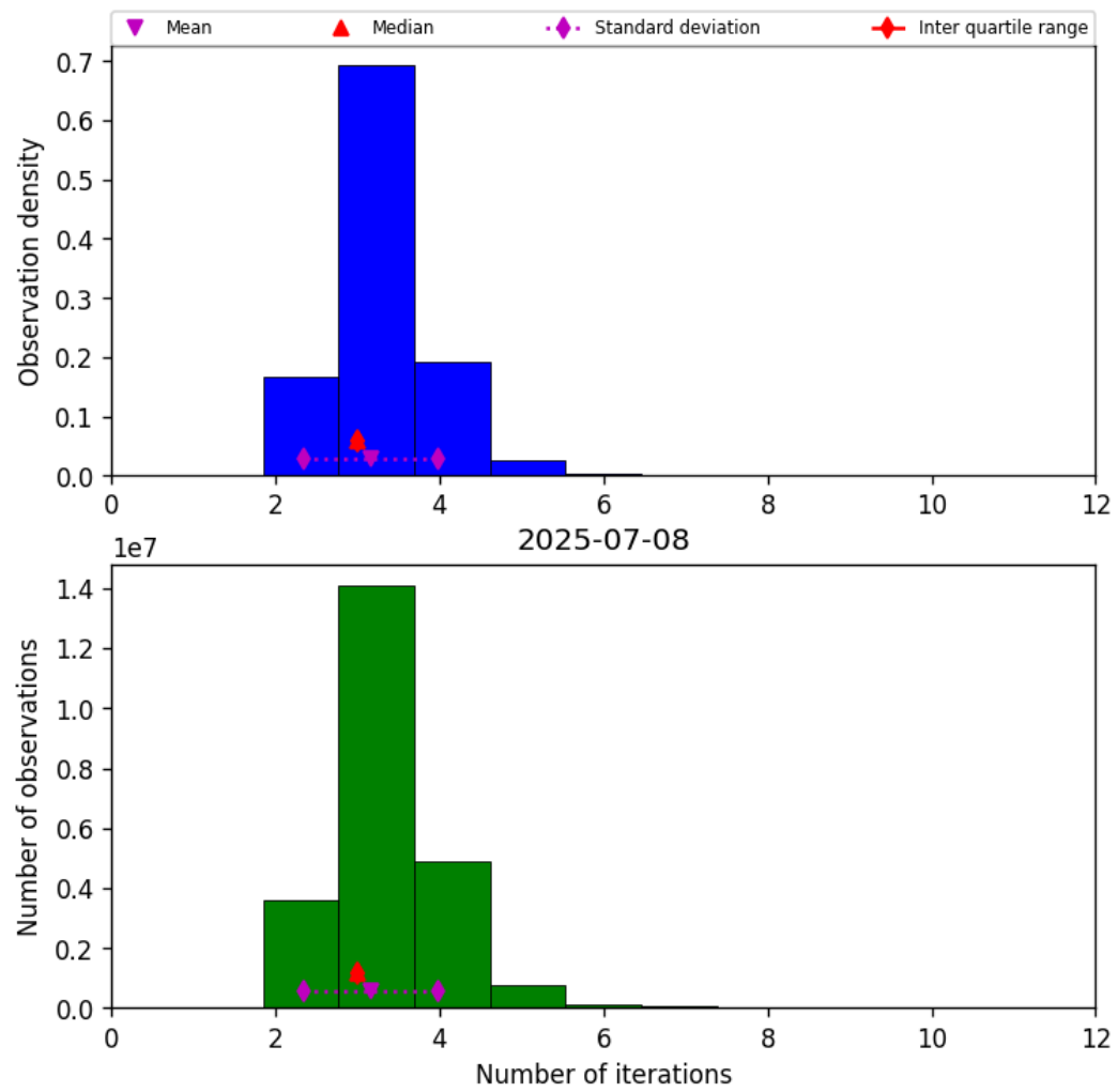
Figure 37: Histogram of “Number of iterations” for 2025-07-08 to 2025-07-09
