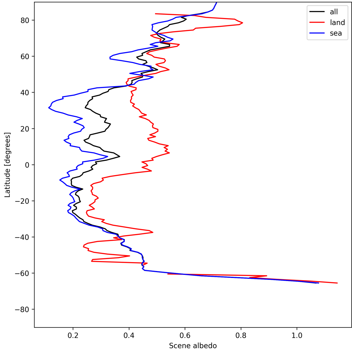
Figure 15: Zonal average of “Scene albedo” for 2025-07-08 to 2025-07-09.
