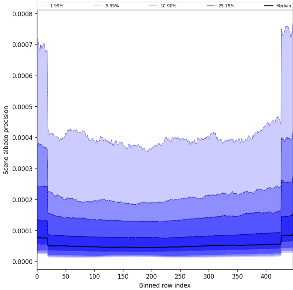
Figure 50: Along track statistics of “Scene albedo precision” for 2025-07-08 to 2025-07-09
