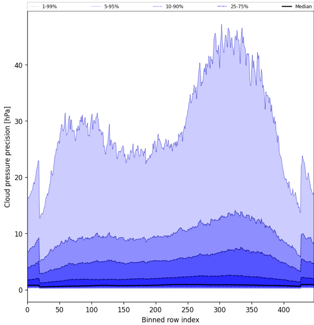
Figure 46: Along track statistics of “Cloud pressure precision” for 2025-07-08 to 2025-07-09
