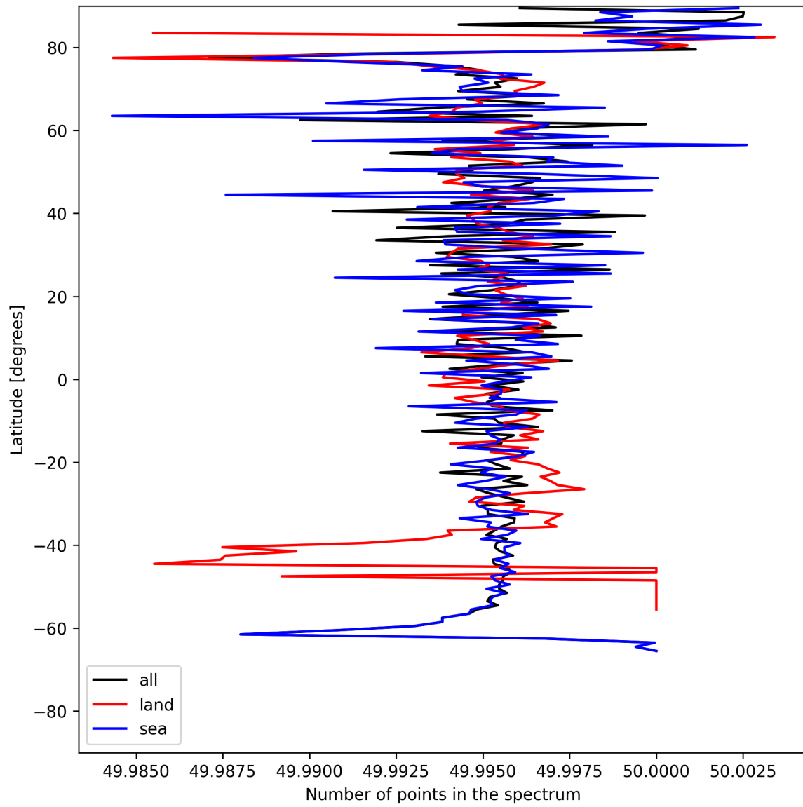
Figure 25: Zonal average of “Number of points in the spectrum” for 2025-07-10 to 2025-07-11.
