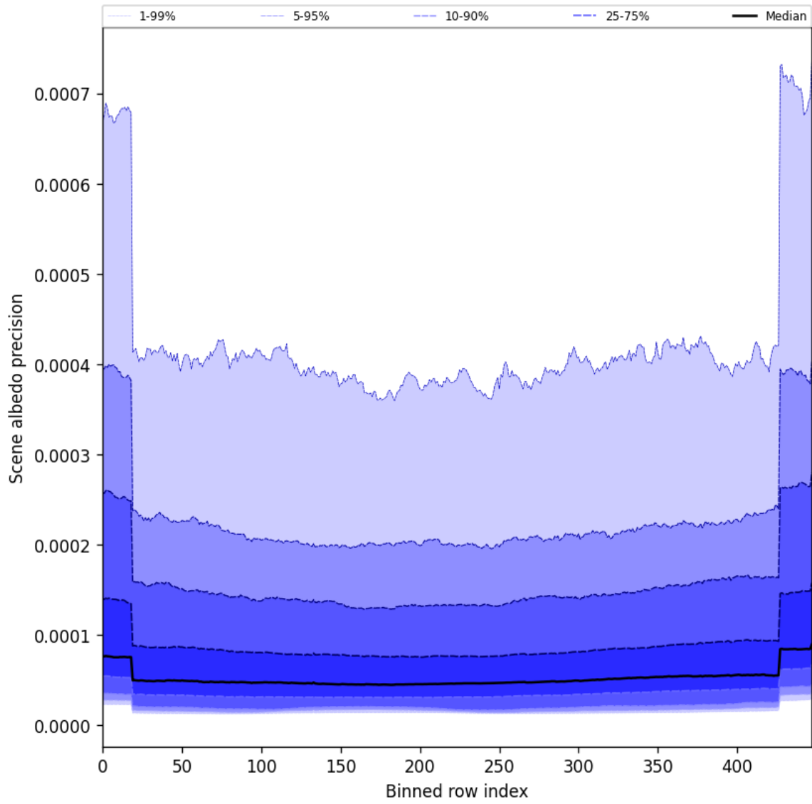
Figure 50: Along track statistics of “Scene albedo precision” for 2025-07-10 to 2025-07-11
