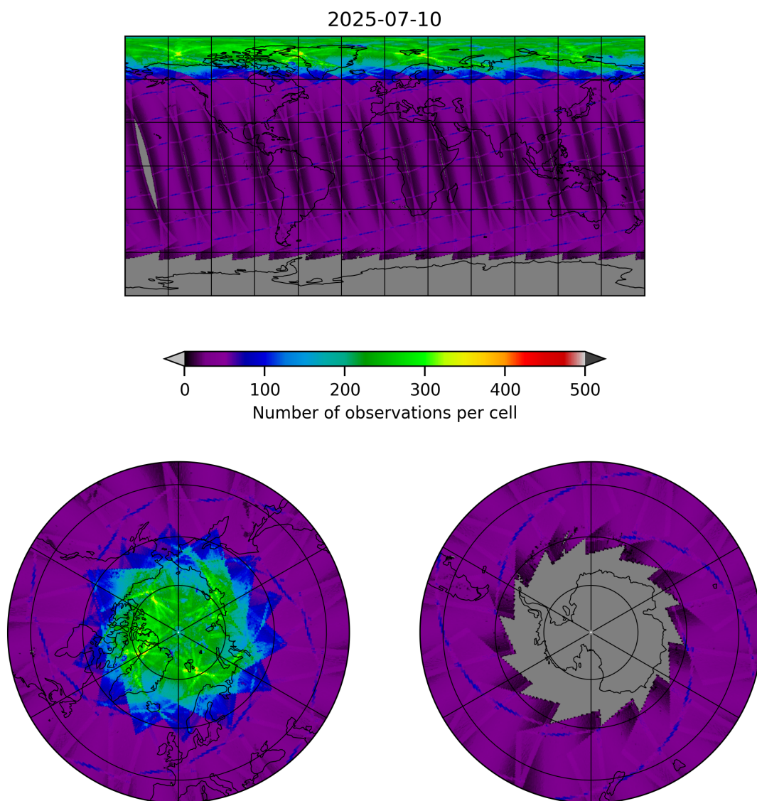
Figure 9: Map of the number of observations for 2025-07-10 to 2025-07-11
