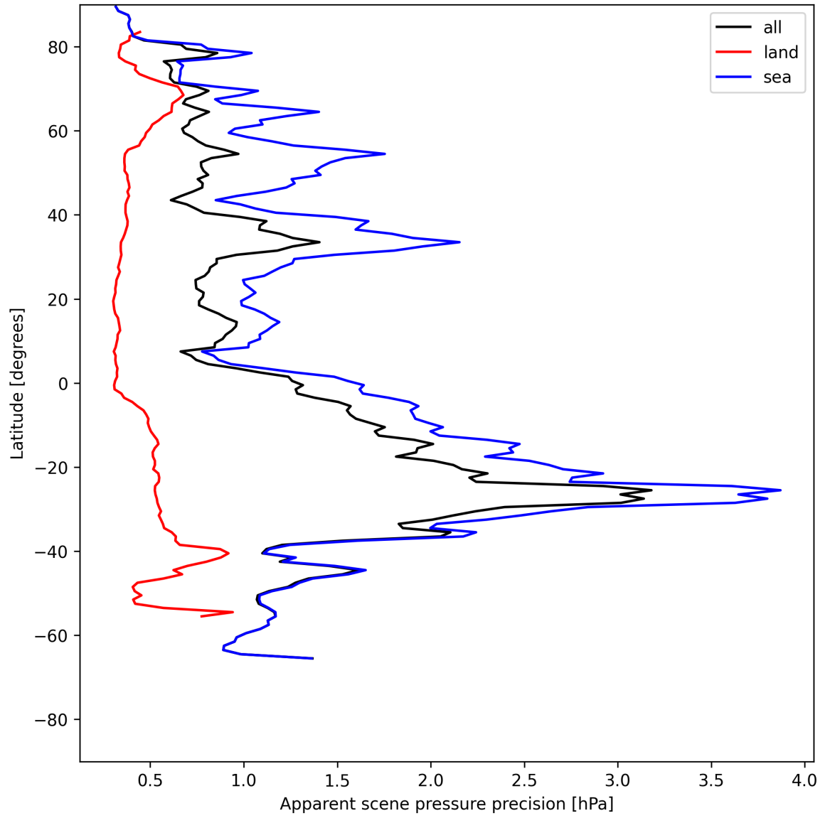
Figure 18: Zonal average of “Apparent scene pressure precision” for 2025-07-10 to 2025-07-11.
