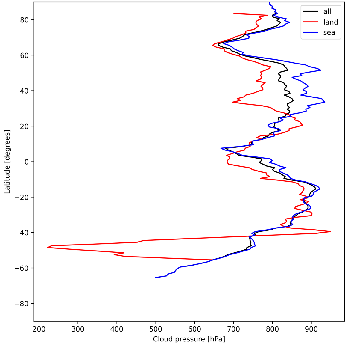
Figure 11: Zonal average of “Cloud pressure” for 2025-07-10 to 2025-07-11.
