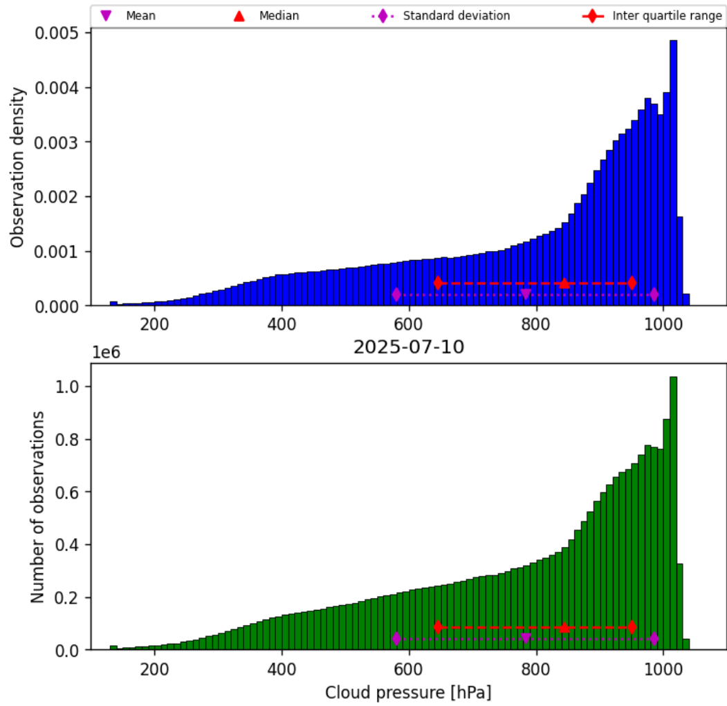
Figure 28: Histogram of “Cloud pressure” for 2025-07-10 to 2025-07-11
