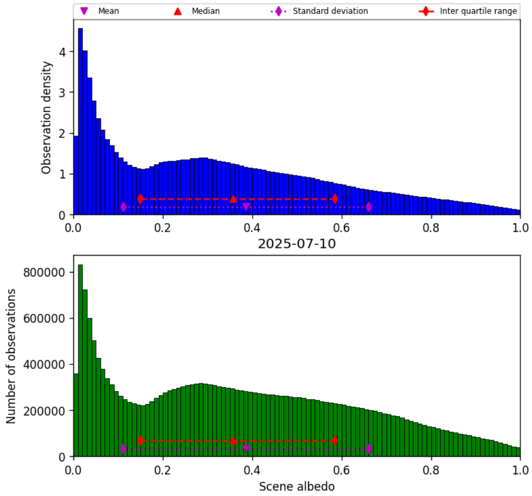
Figure 32: Histogram of “Scene albedo” for 2025-07-10 to 2025-07-11
