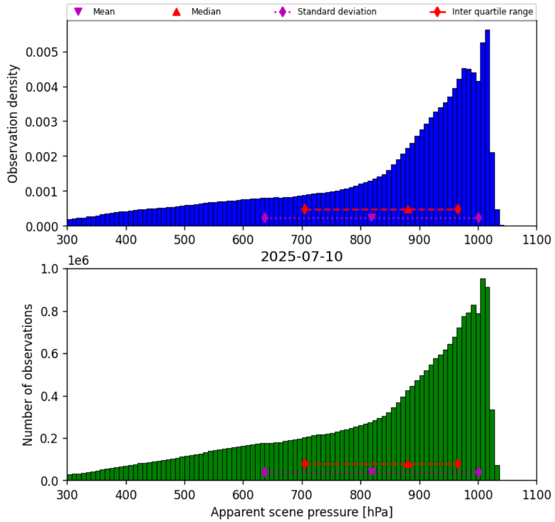
Figure 34: Histogram of “Apparent scene pressure” for 2025-07-10 to 2025-07-11
