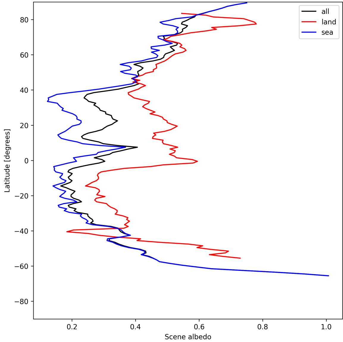
Figure 15: Zonal average of “Scene albedo” for 2025-07-10 to 2025-07-11.
