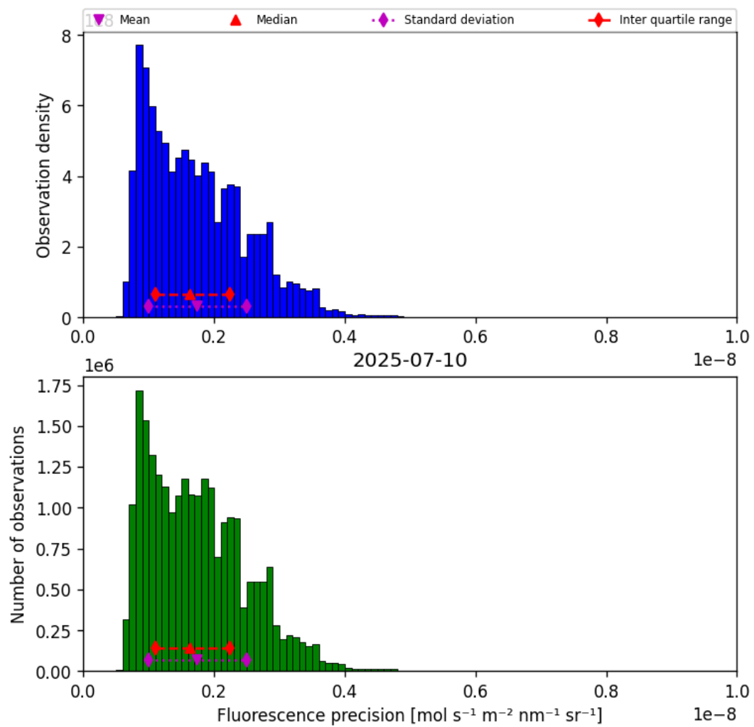
Figure 39: Histogram of “Fluorescence precision” for 2025-07-10 to 2025-07-11
