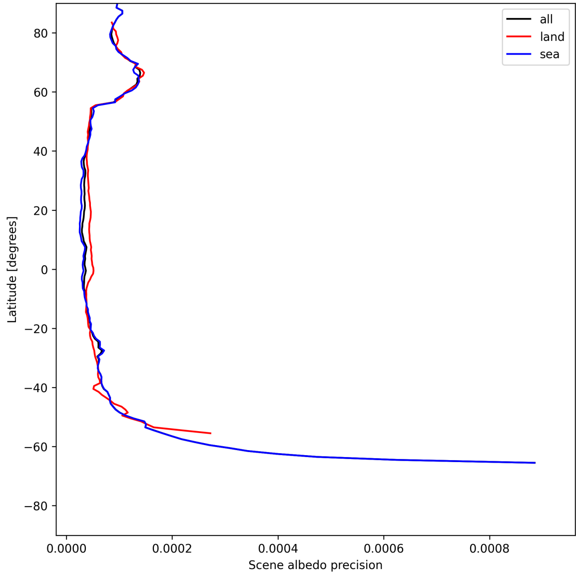
Figure 16: Zonal average of “Scene albedo precision” for 2025-07-10 to 2025-07-11.
