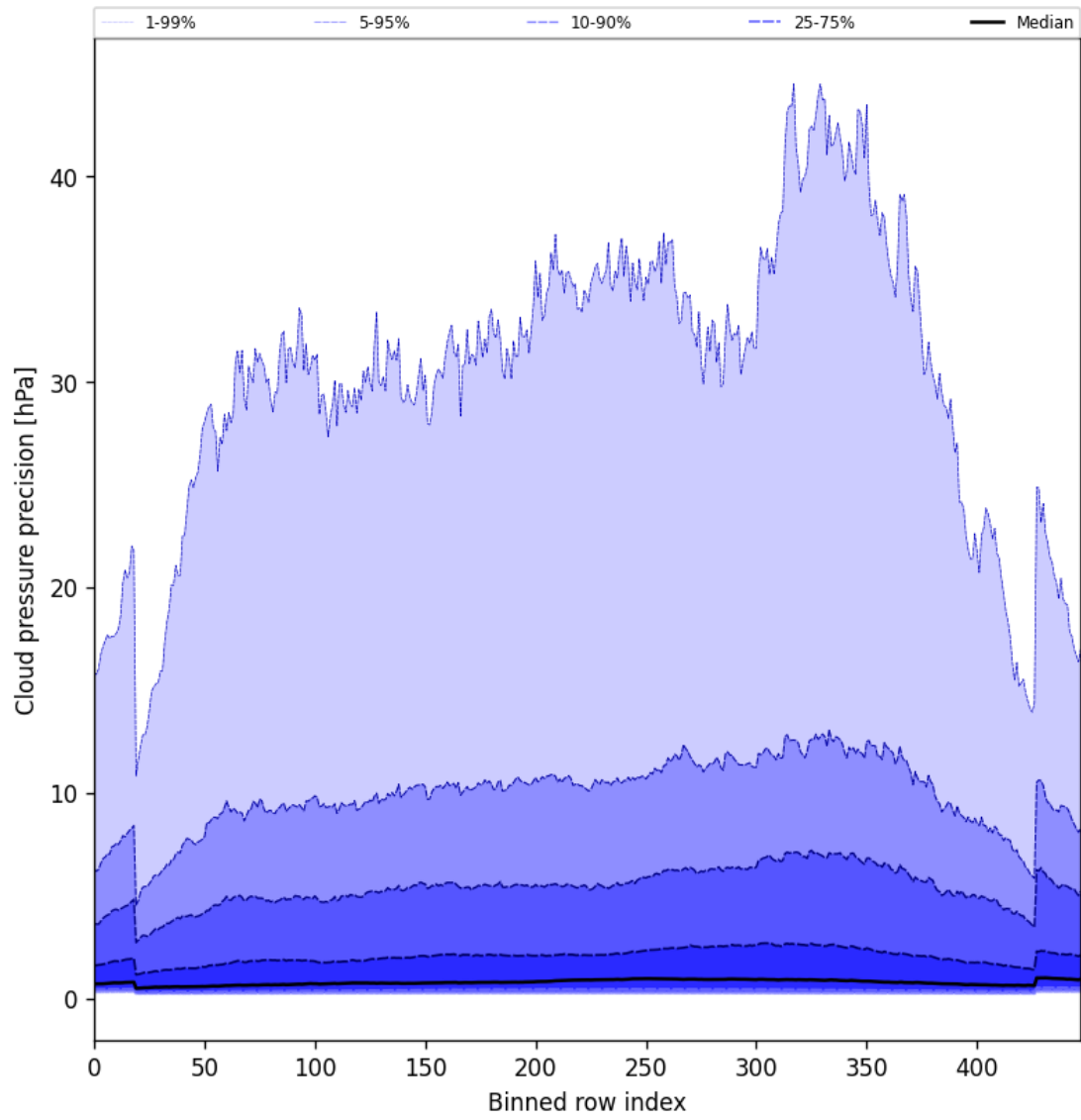
Figure 46: Along track statistics of “Cloud pressure precision” for 2025-07-10 to 2025-07-11
