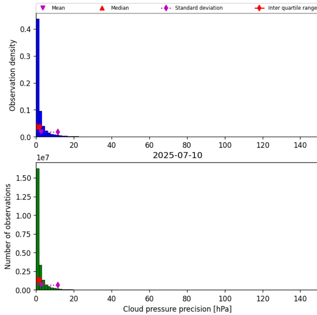
Figure 29: Histogram of "Cloud pressure precision" for 2025-07-10 to 2025-07-11
