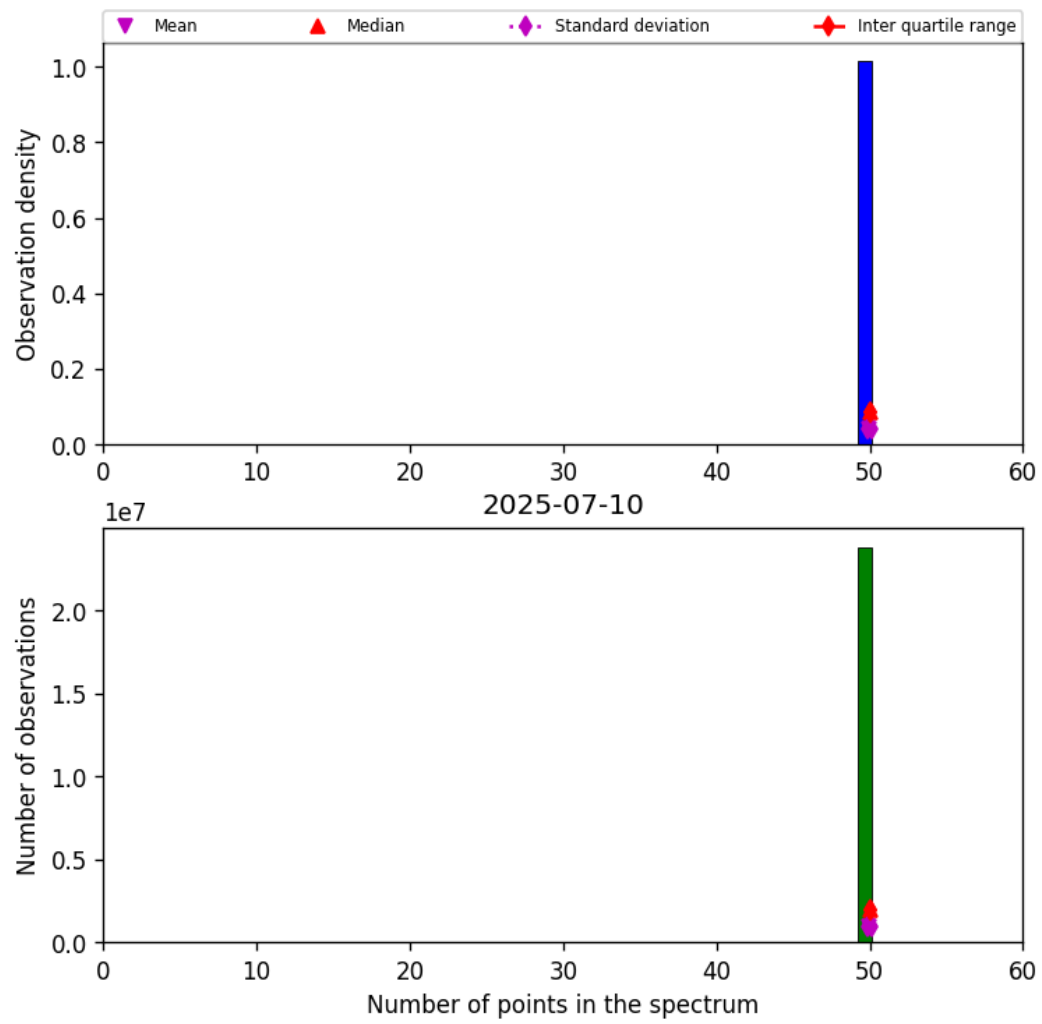
Figure 42: Histogram of “Number of points in the spectrum” for 2025-07-10 to 2025-07-11
