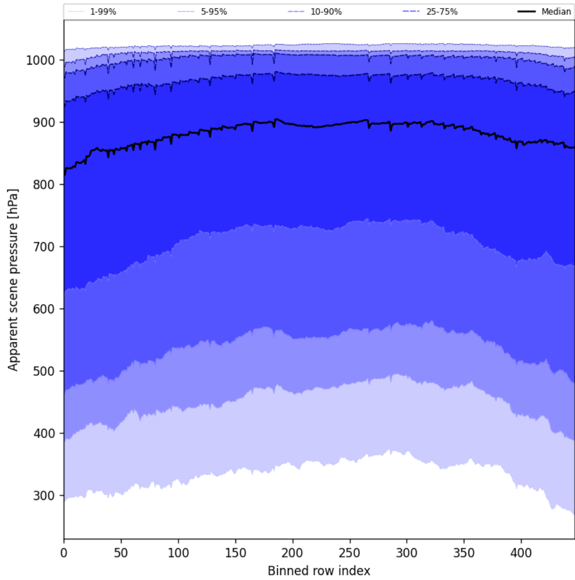
Figure 51: Along track statistics of “Apparent scene pressure” for 2025-07-10 to 2025-07-11
