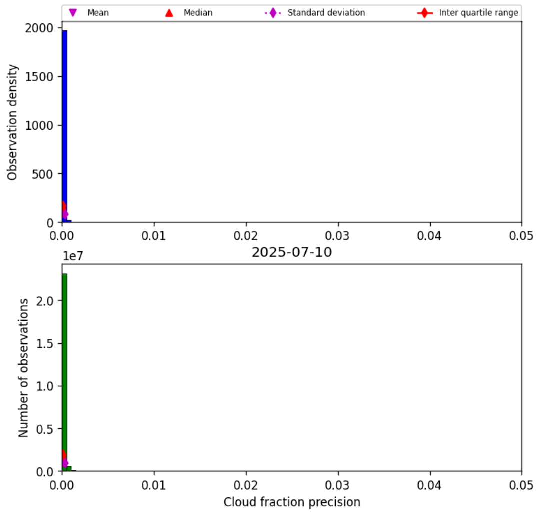
Figure 31: Histogram of “Cloud fraction precision” for 2025-07-10 to 2025-07-11
