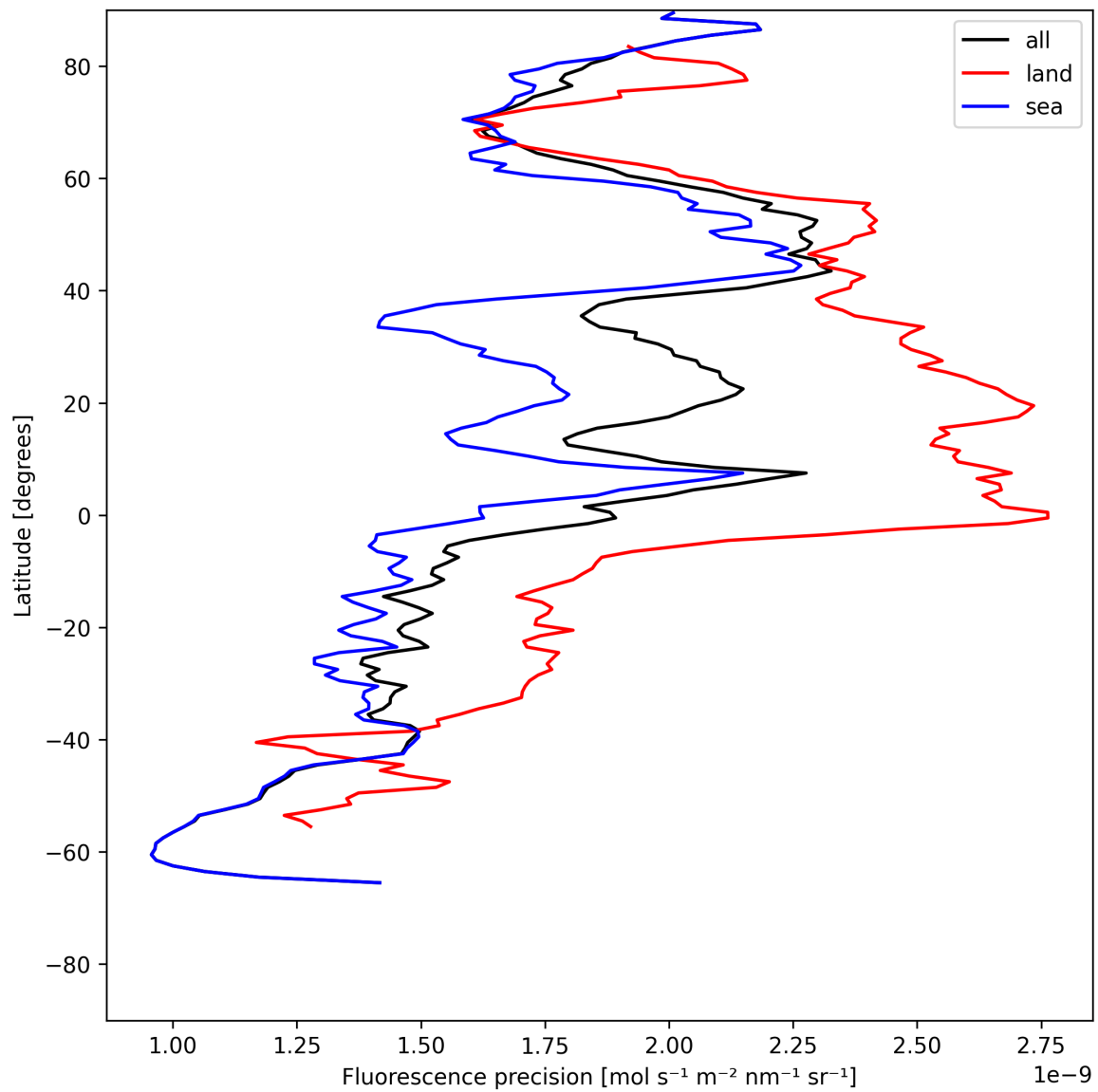
Figure 22: Zonal average of “Fluorescence precision” for 2025-07-10 to 2025-07-11.
