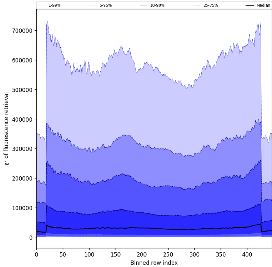
Figure 57: Along track statistics of “ \chi^2 of fluorescence retrieval” for 2025-07-10 to 2025-07-11
