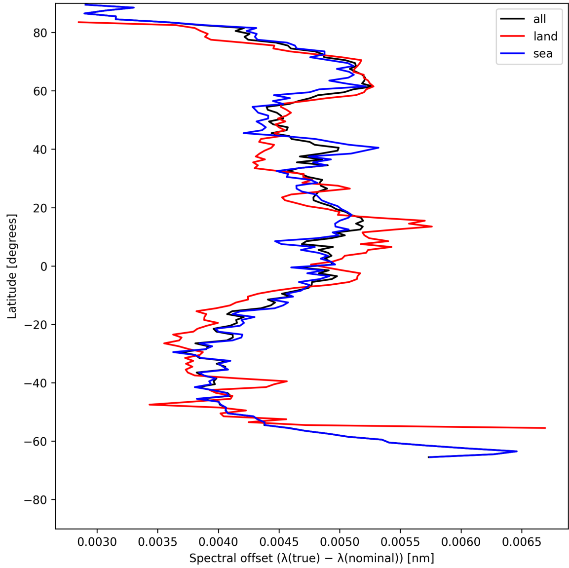
Figure 26: Zonal average of “Spectral offset ( \lambda_{\text{true}} - \lambda_{\text{nominal}} )” for 2025-07-10 to 2025-07-11.
