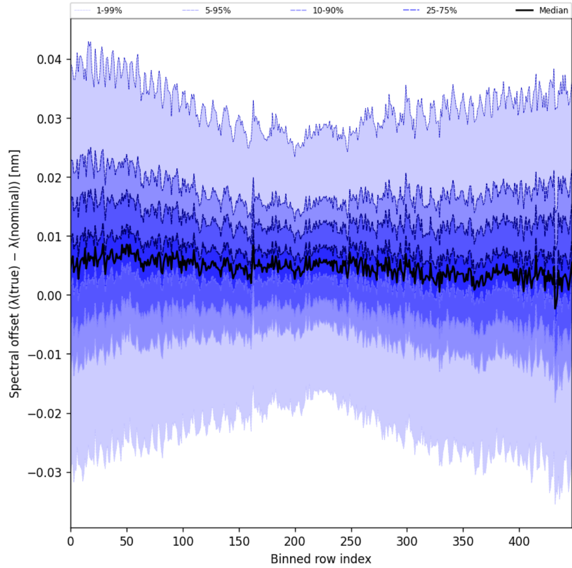
Figure 60: Along track statistics of “Spectral offset ( \lambda_{\text{true}} - \lambda_{\text{nominal}} )” for 2025-07-10 to 2025-07-11
