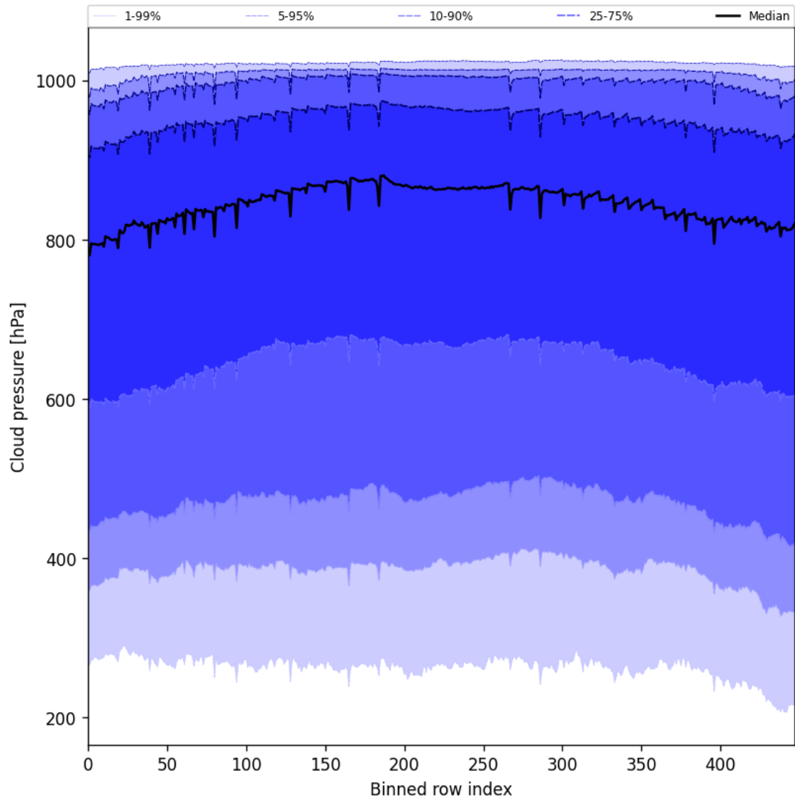
Figure 45: Along track statistics of “Cloud pressure” for 2025-07-10 to 2025-07-11
