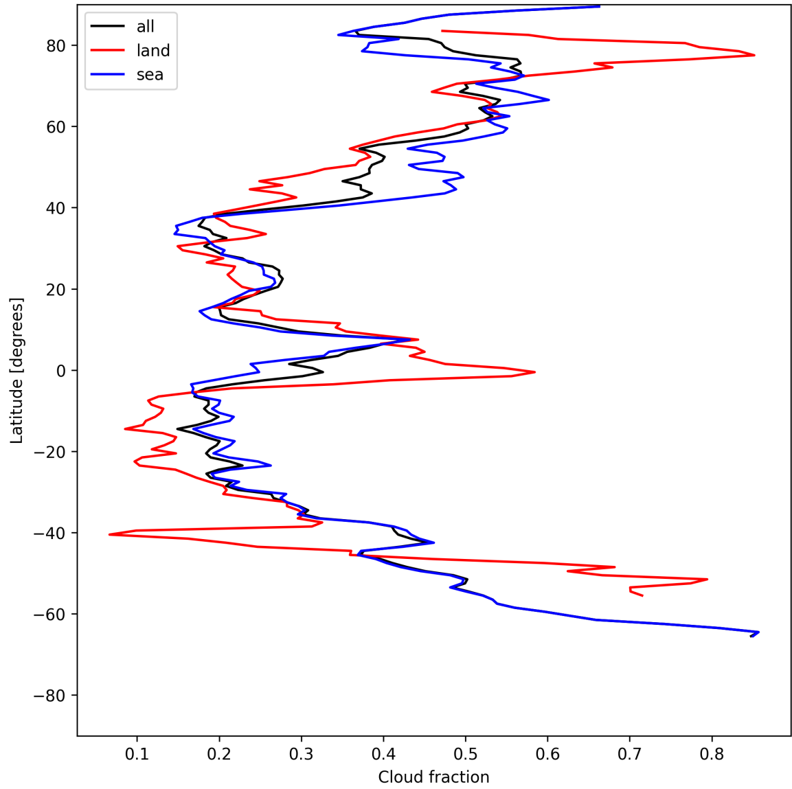
Figure 13: Zonal average of “Cloud fraction” for 2025-07-10 to 2025-07-11.
