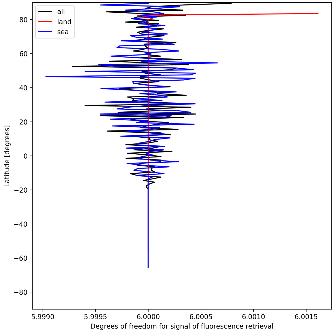
Figure 24: Zonal average of “Degrees of freedom for signal of fluorescence retrieval” for 2025-07-10 to 2025-07-11.
