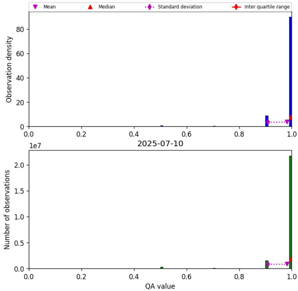
Figure 27: Histogram of “QA value” for 2025-07-10 to 2025-07-11
