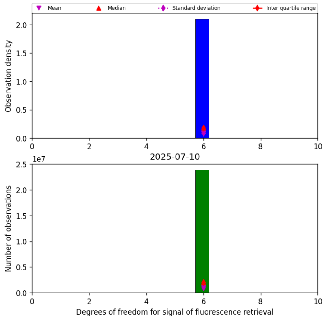
Figure 41: Histogram of “Degrees of freedom for signal of fluorescence retrieval” for 2025-07-10 to 2025-07-11
