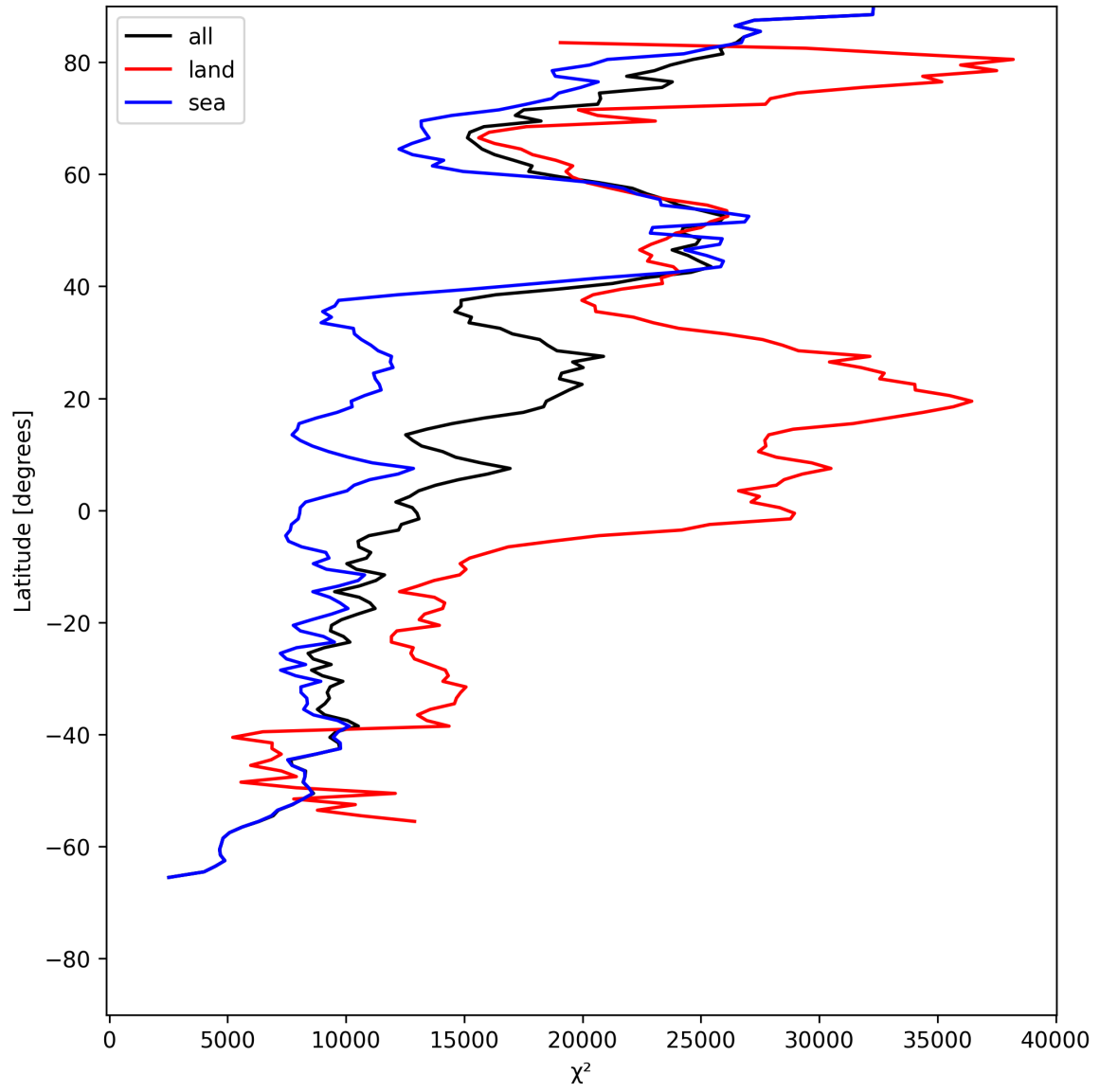
Figure 19: Zonal average of “ \chi^2 ” for 2025-07-10 to 2025-07-11.
