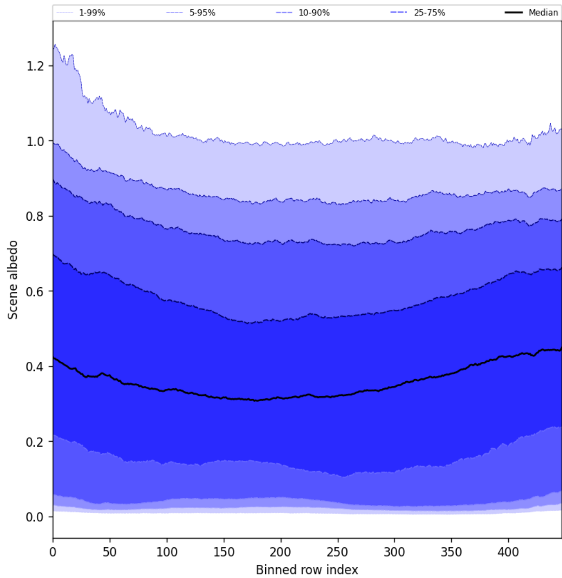
Figure 49: Along track statistics of “Scene albedo” for 2025-07-10 to 2025-07-11
