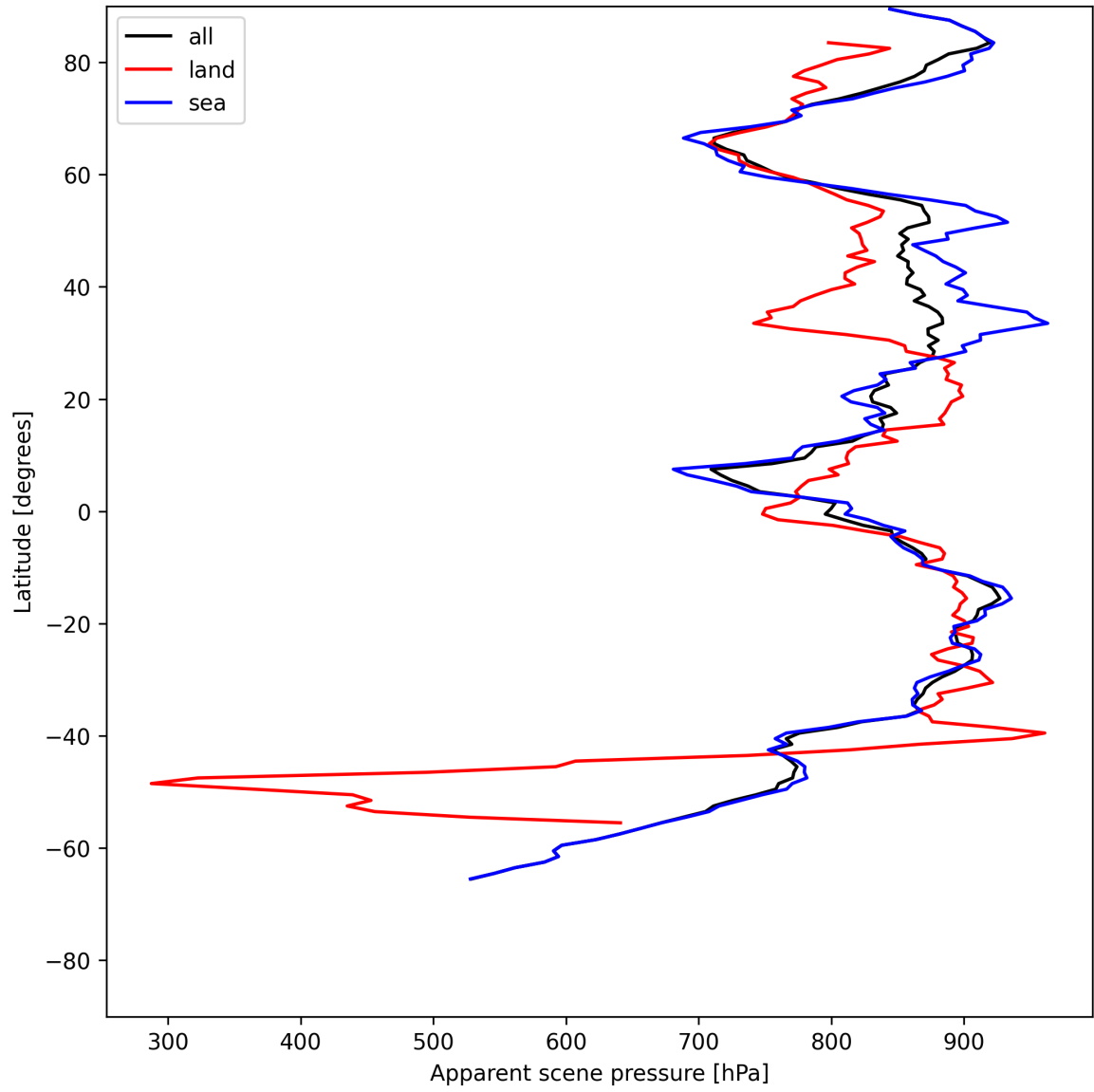
Figure 17: Zonal average of “Apparent scene pressure” for 2025-07-10 to 2025-07-11.
