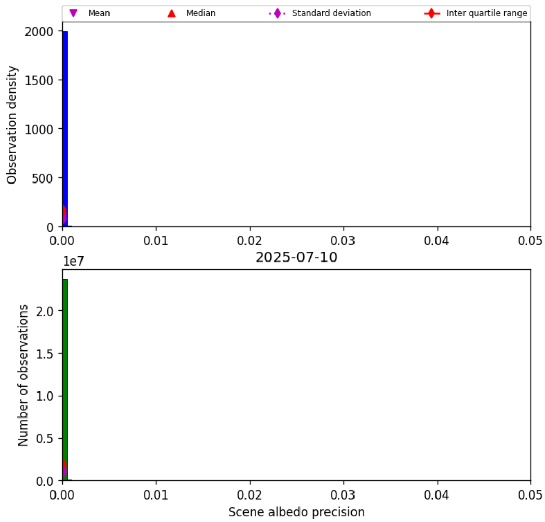
Figure 33: Histogram of “Scene albedo precision” for 2025-07-10 to 2025-07-11
