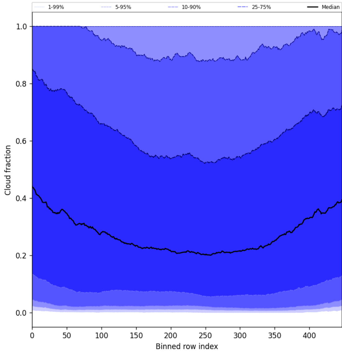
Figure 47: Along track statistics of “Cloud fraction” for 2025-07-10 to 2025-07-11
