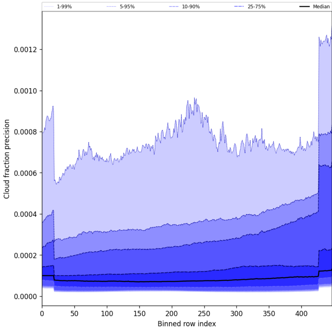
Figure 48: Along track statistics of “Cloud fraction precision” for 2025-07-10 to 2025-07-11
