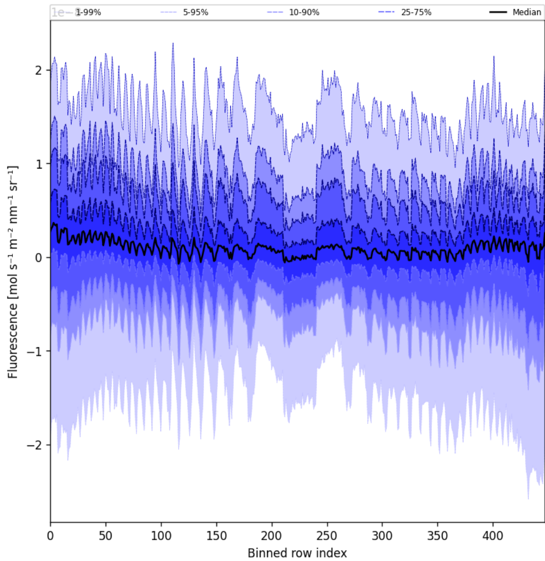
Figure 55: Along track statistics of “Fluorescence” for 2025-07-10 to 2025-07-11
