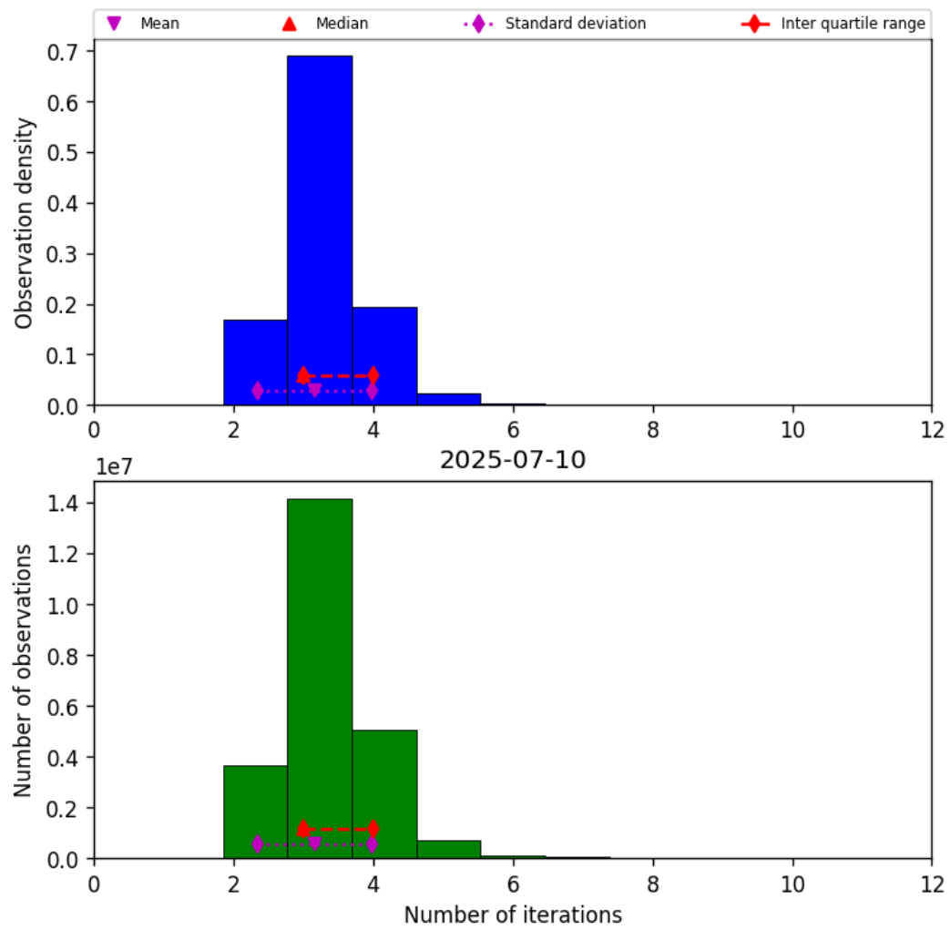
Figure 37: Histogram of “Number of iterations” for 2025-07-10 to 2025-07-11
