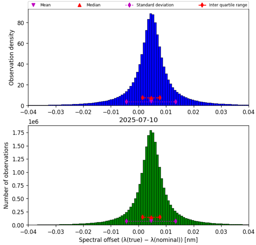
Figure 43: Histogram of “Spectral offset ( \lambda_{\text{true}} - \lambda_{\text{nominal}} )” for 2025-07-10 to 2025-07-11
