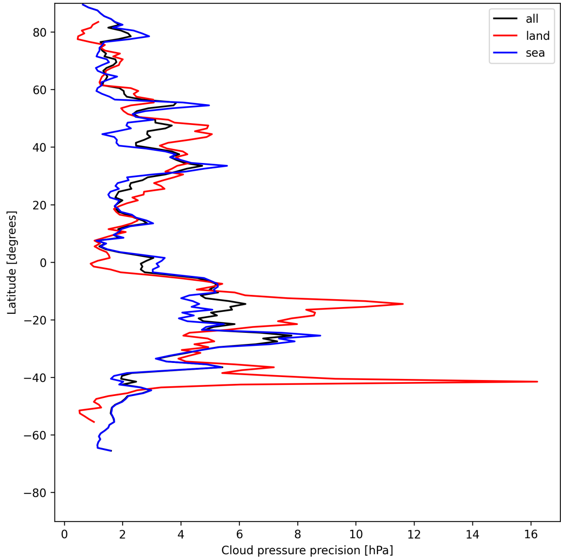
Figure 12: Zonal average of “Cloud pressure precision” for 2025-07-10 to 2025-07-11.
