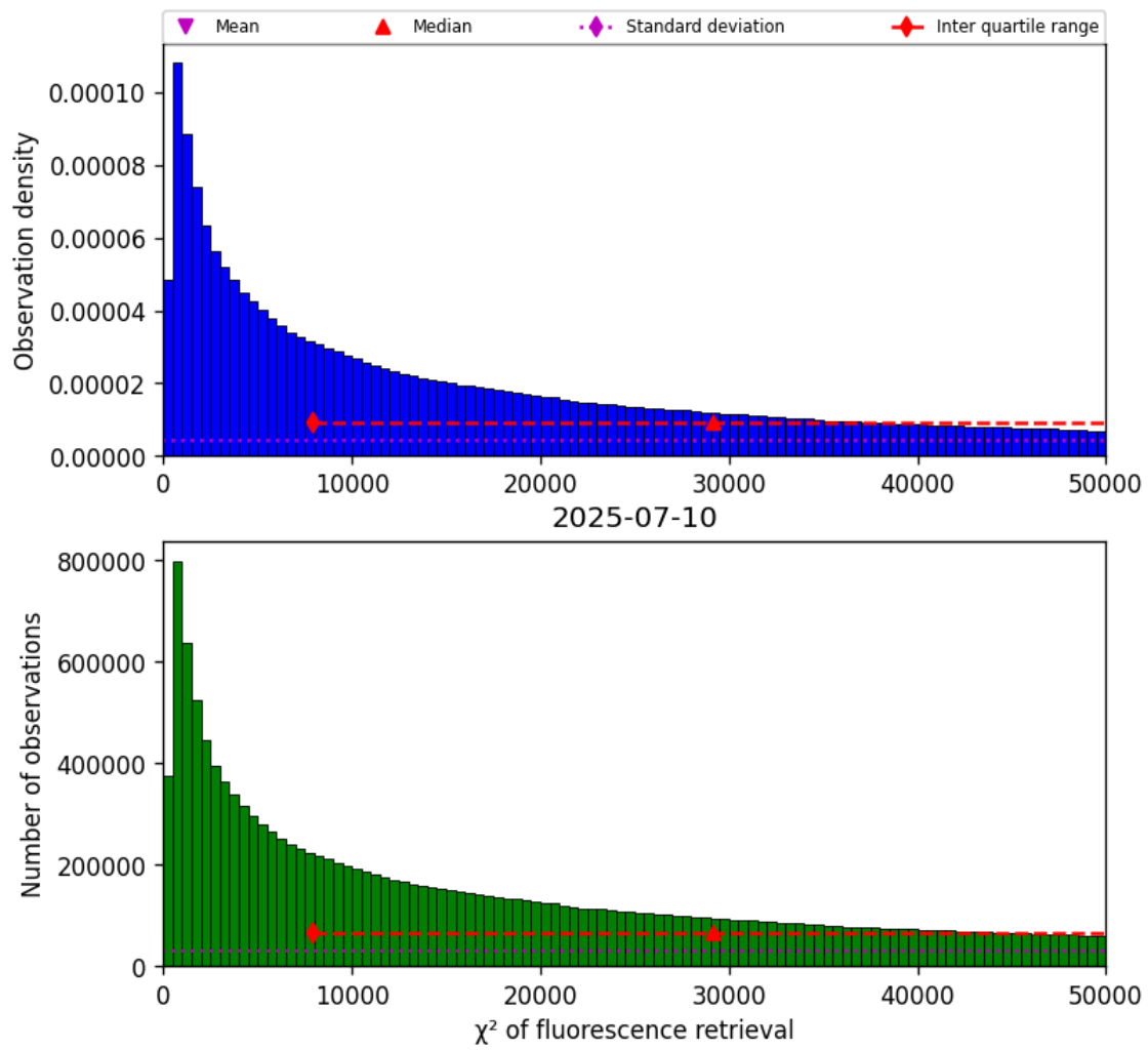
Figure 40: Histogram of “ \chi^2 of fluorescence retrieval” for 2025-07-10 to 2025-07-11
