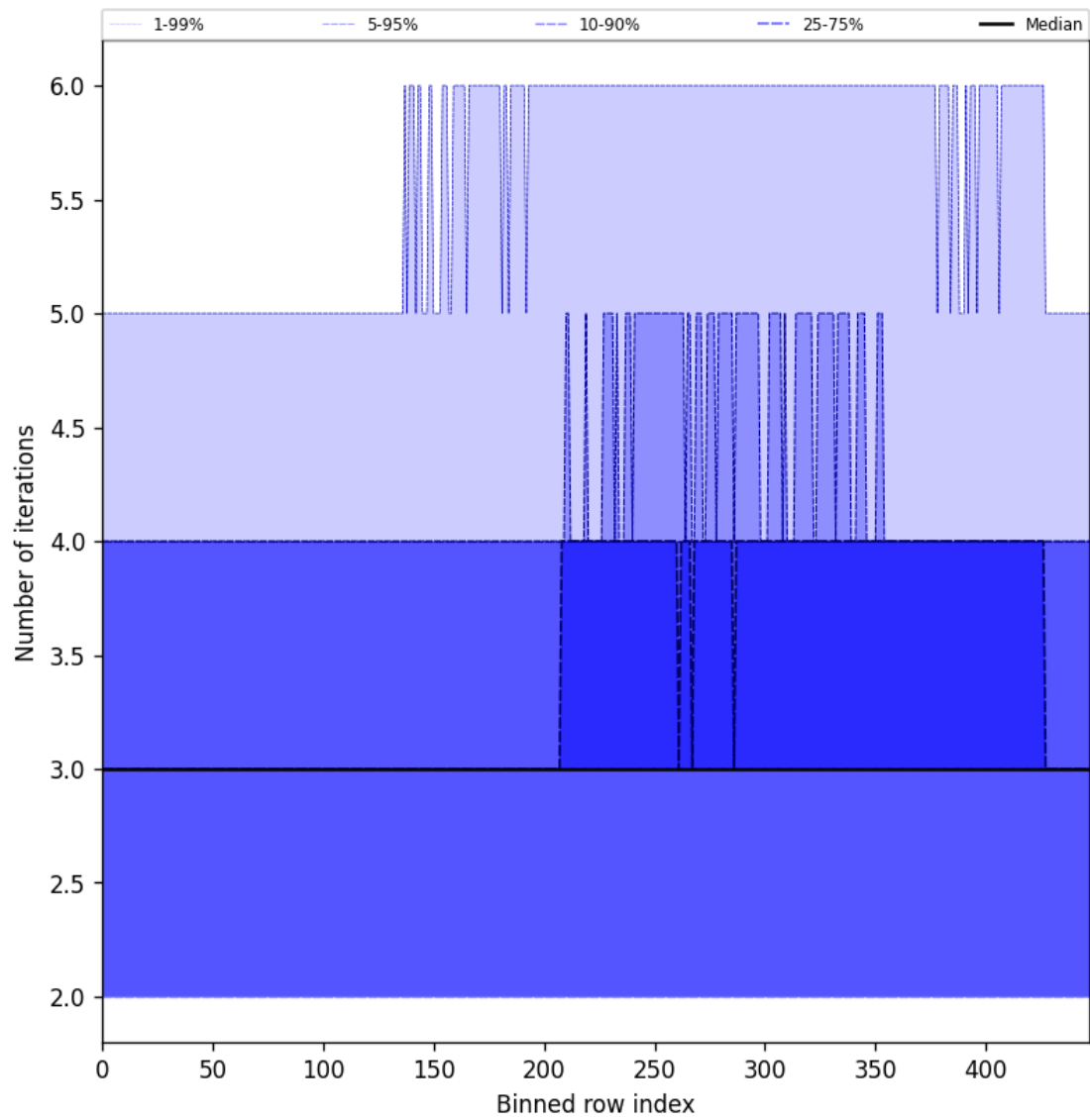
Figure 54: Along track statistics of “Number of iterations” for 2025-07-10 to 2025-07-11
