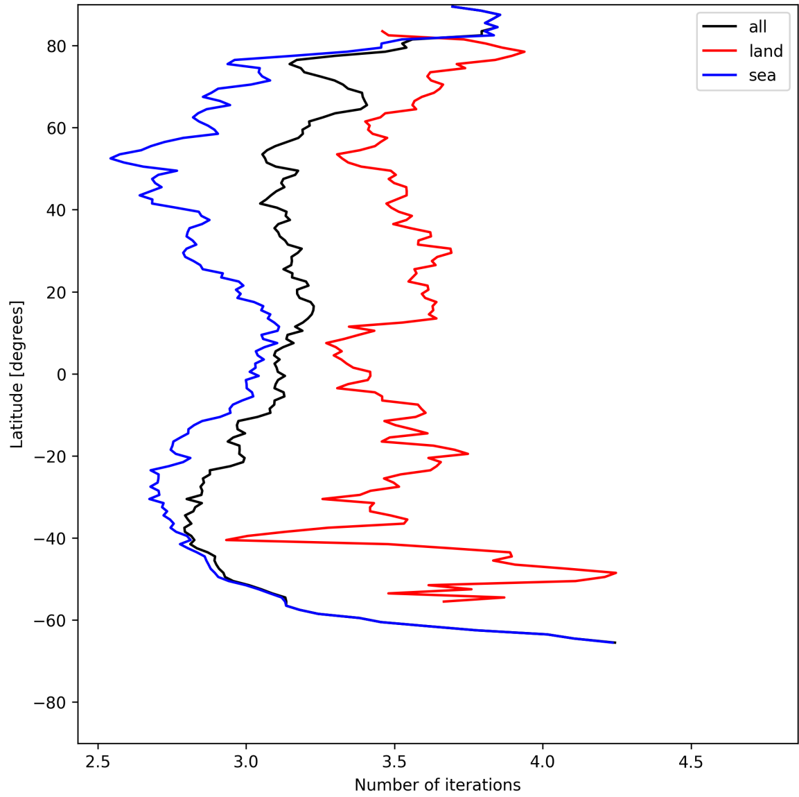
Figure 20: Zonal average of “Number of iterations” for 2025-07-10 to 2025-07-11.
