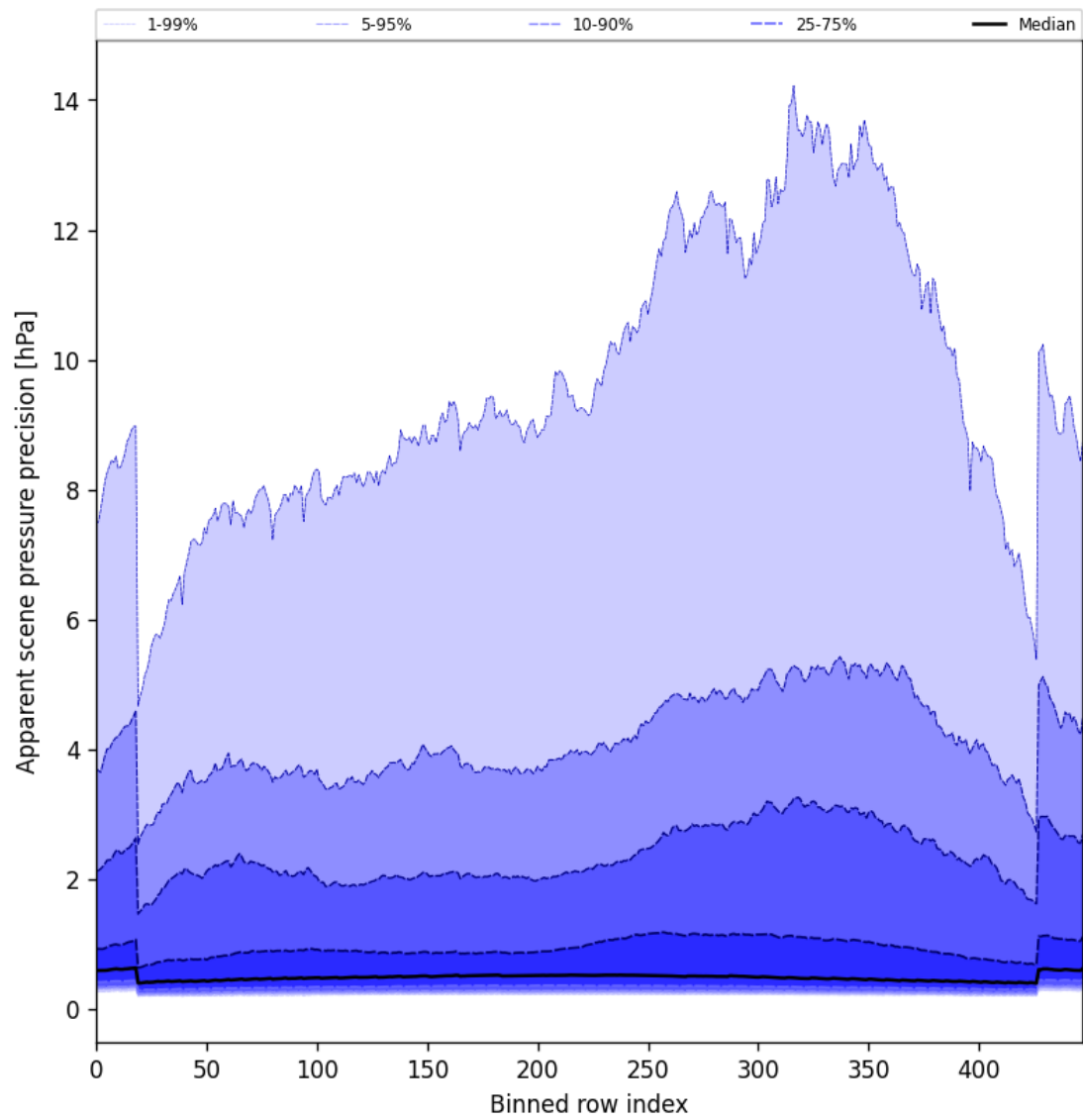
Figure 52: Along track statistics of “Apparent scene pressure precision” for 2025-07-10 to 2025-07-11
