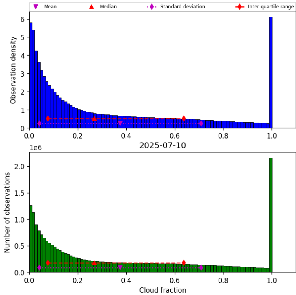
Figure 30: Histogram of “Cloud fraction” for 2025-07-10 to 2025-07-11
