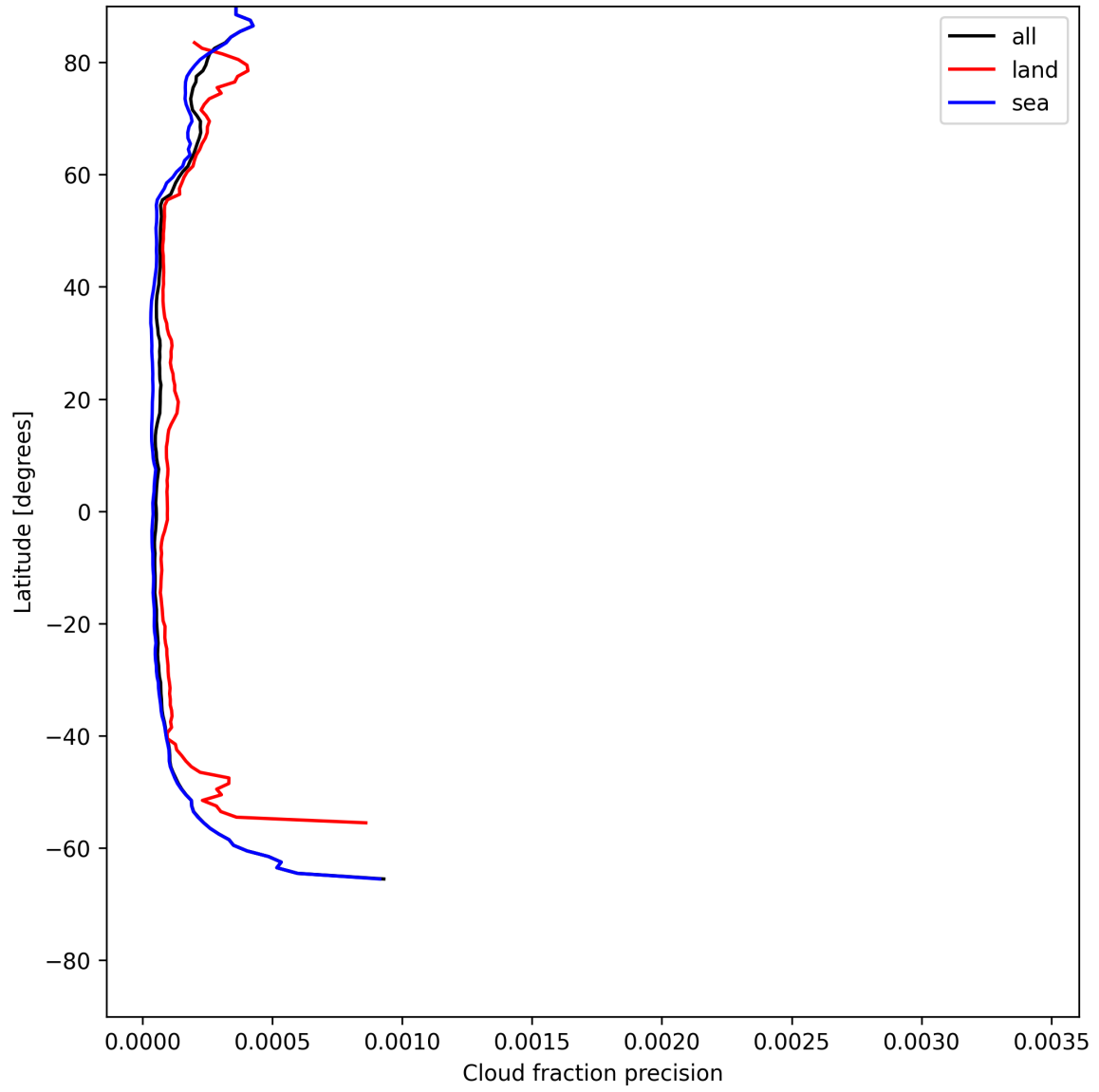
Figure 14: Zonal average of “Cloud fraction precision” for 2025-07-10 to 2025-07-11.
