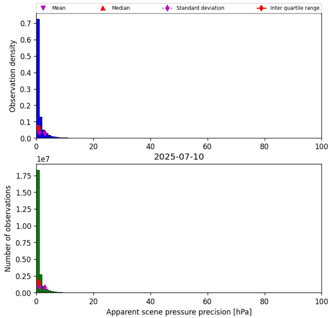
Figure 35: Histogram of “Apparent scene pressure precision” for 2025-07-10 to 2025-07-11
