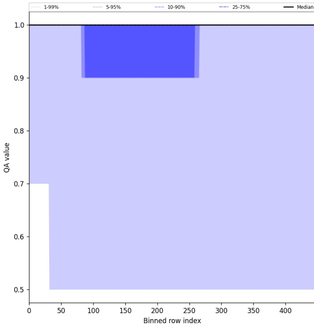
Figure 44: Along track statistics of “QA value” for 2025-07-10 to 2025-07-11
