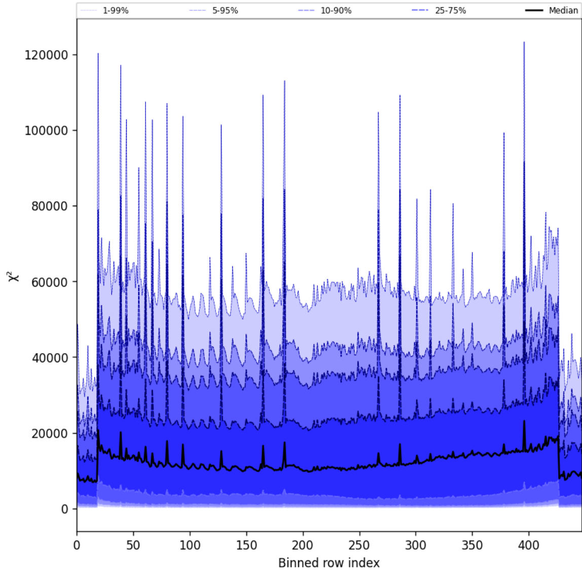
Figure 53: Along track statistics of “ \chi^2 ” for 2025-07-10 to 2025-07-11
