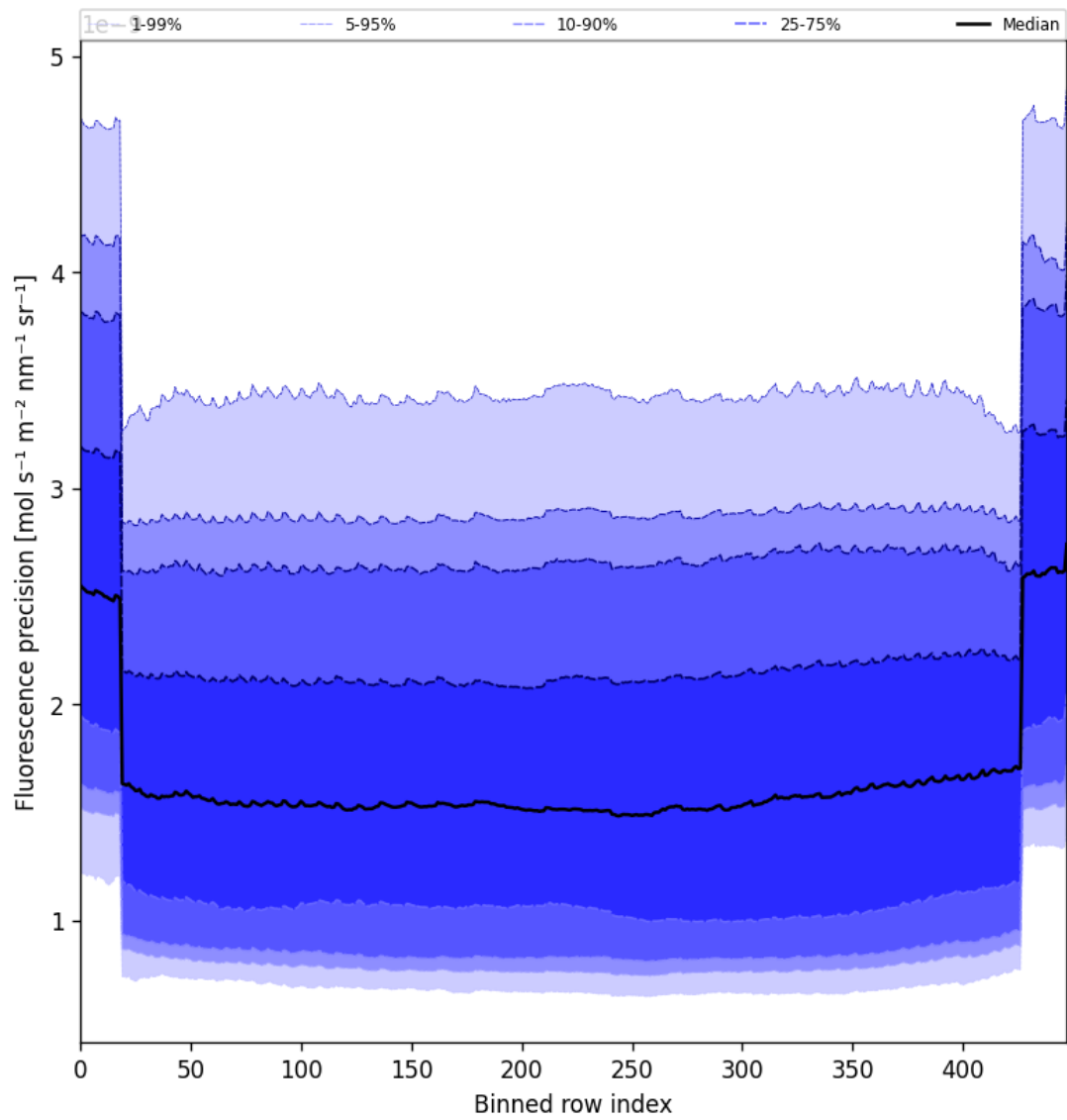
Figure 56: Along track statistics of “Fluorescence precision” for 2025-07-10 to 2025-07-11
