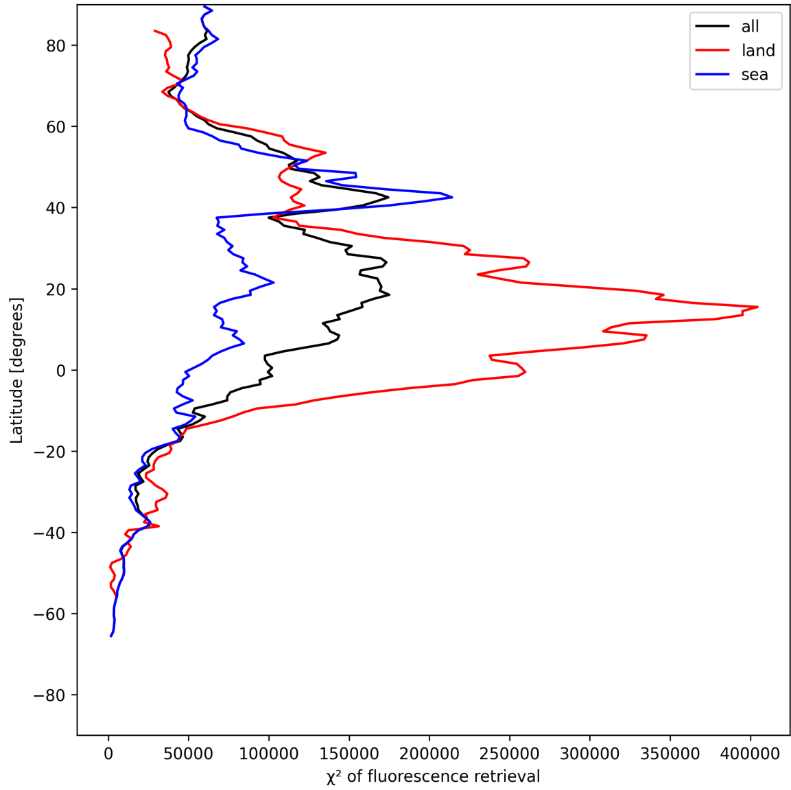
Figure 23: Zonal average of “ \chi^2 of fluorescence retrieval” for 2025-07-10 to 2025-07-11.
