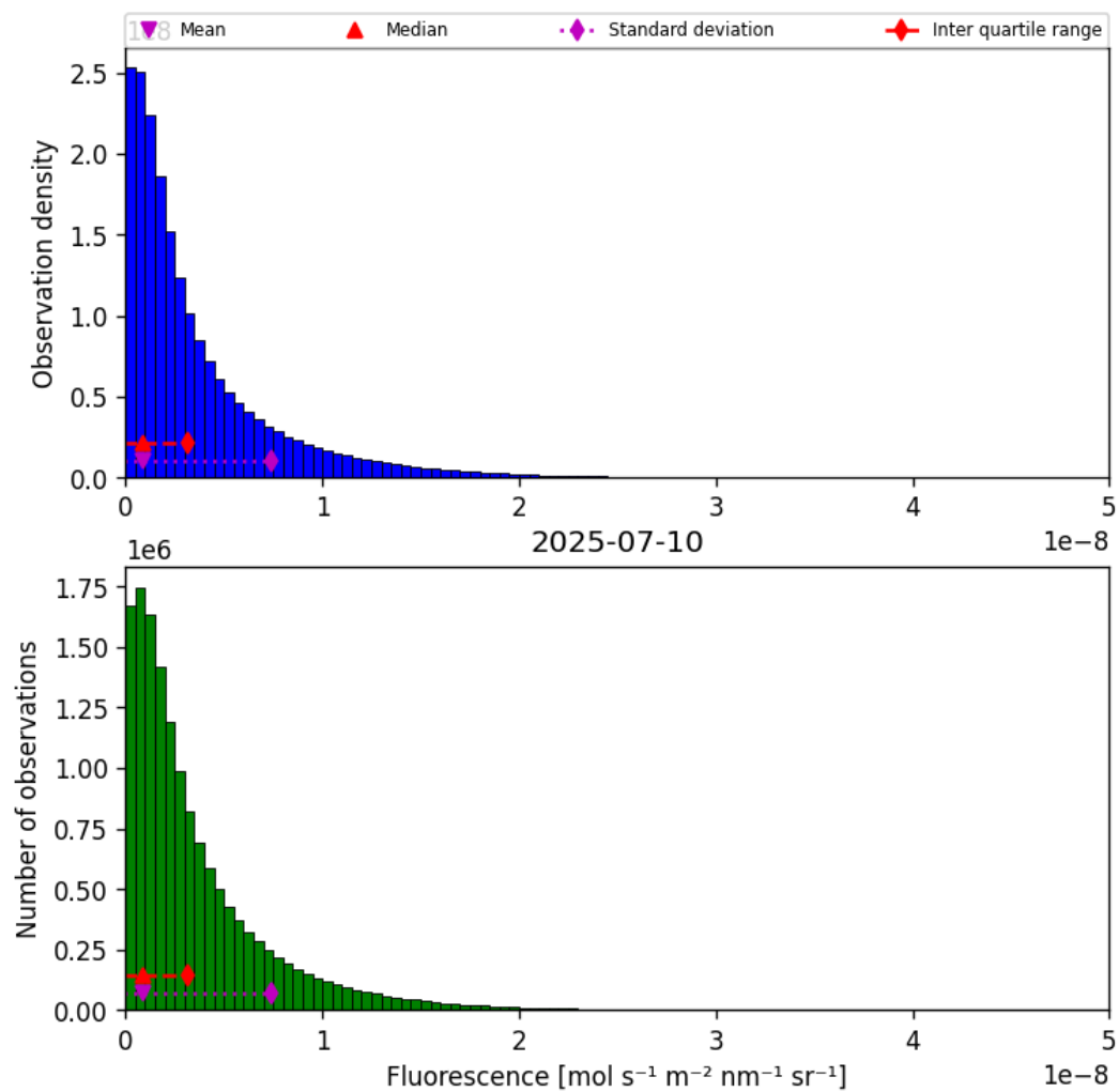
Figure 38: Histogram of “Fluorescence” for 2025-07-10 to 2025-07-11
