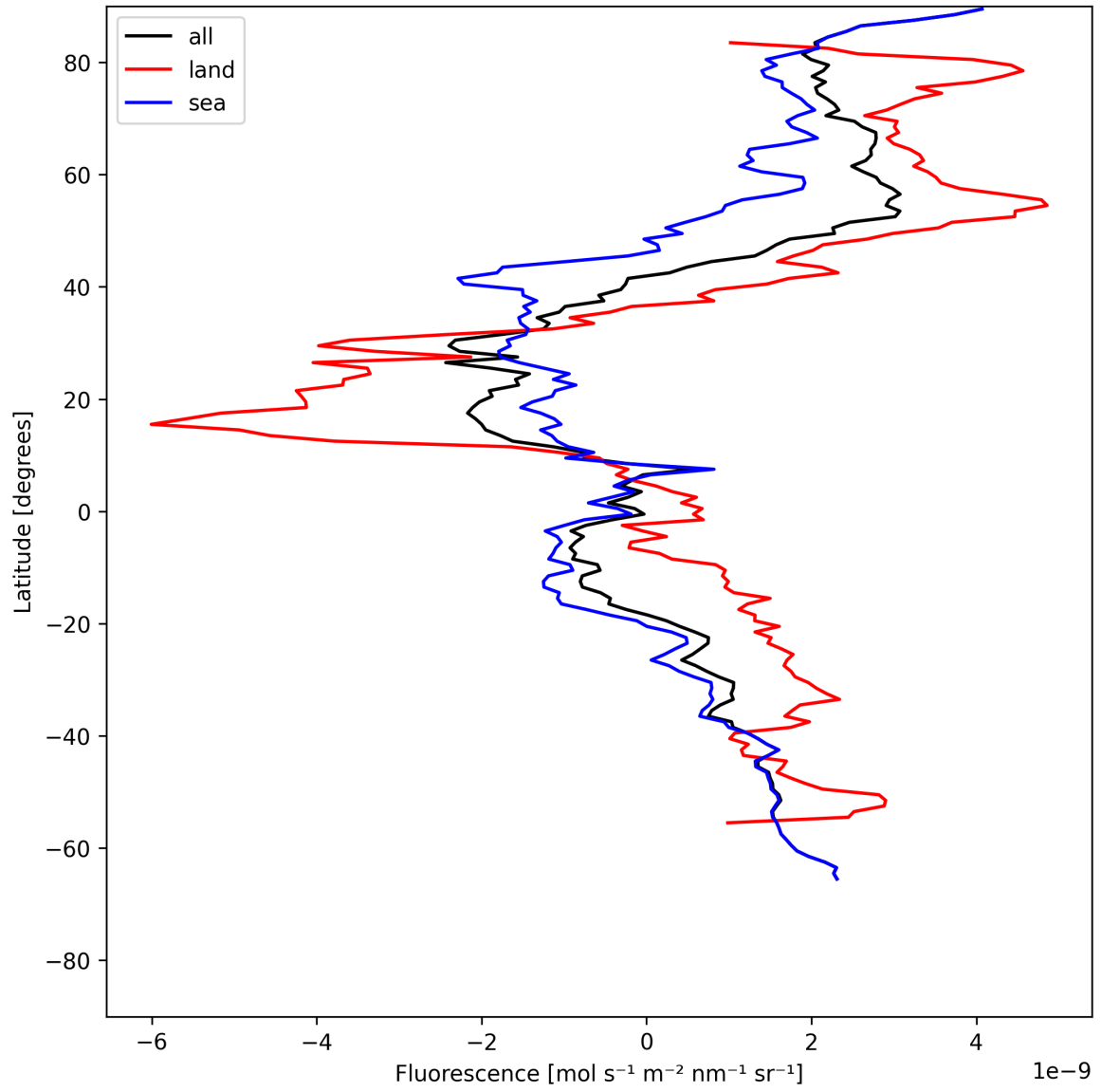
Figure 21: Zonal average of “Fluorescence” for 2025-07-10 to 2025-07-11.
