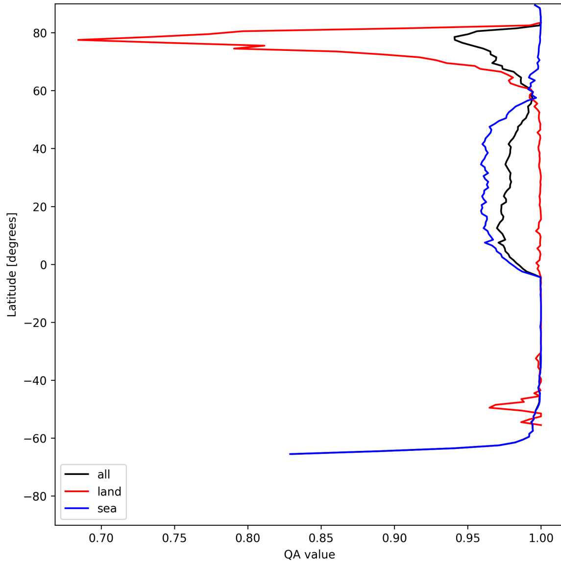
Figure 10: Zonal average of “QA value” for 2025-07-10 to 2025-07-11.
