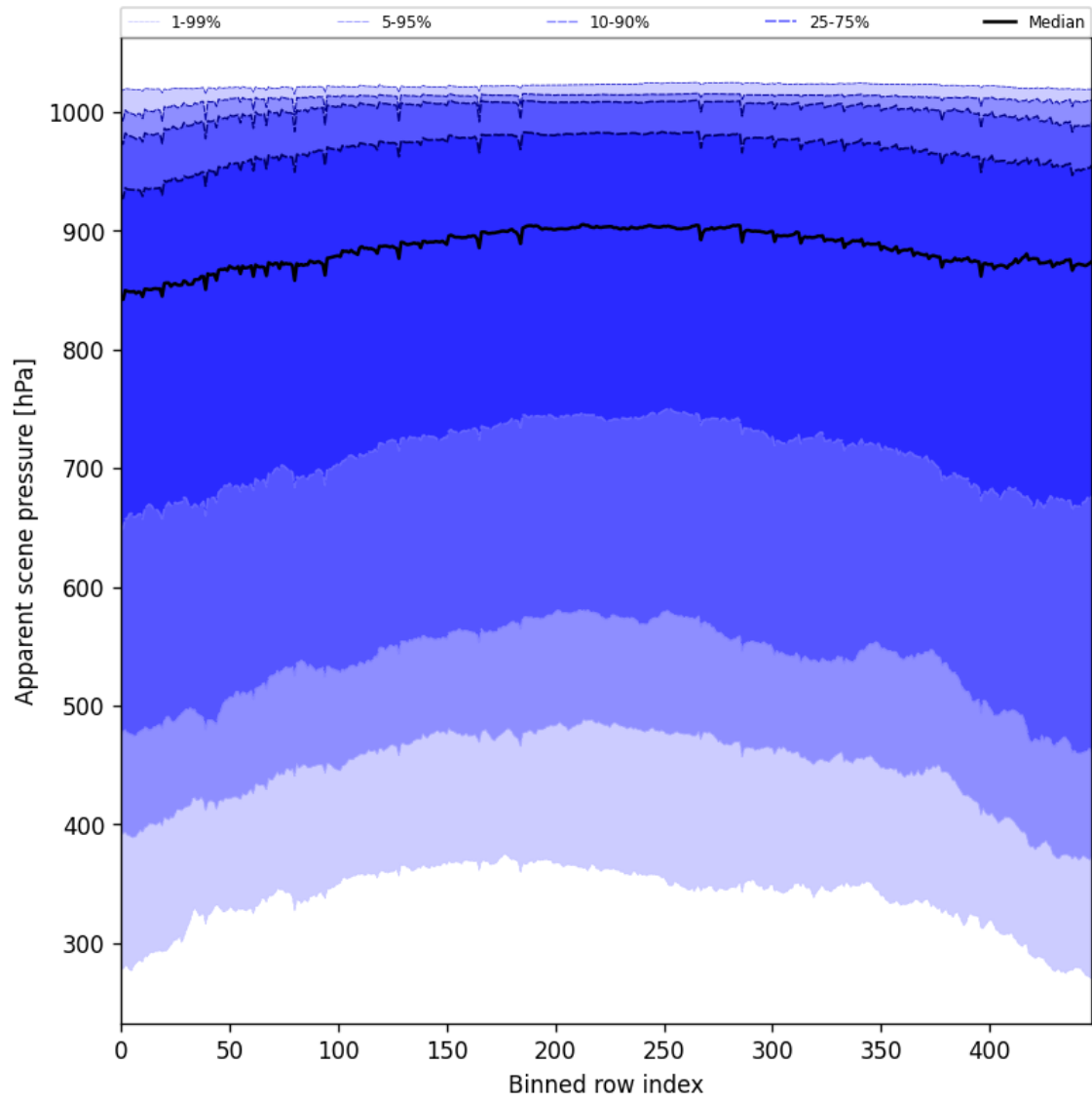
Figure 51: Along track statistics of “Apparent scene pressure” for 2025-07-11 to 2025-07-11
