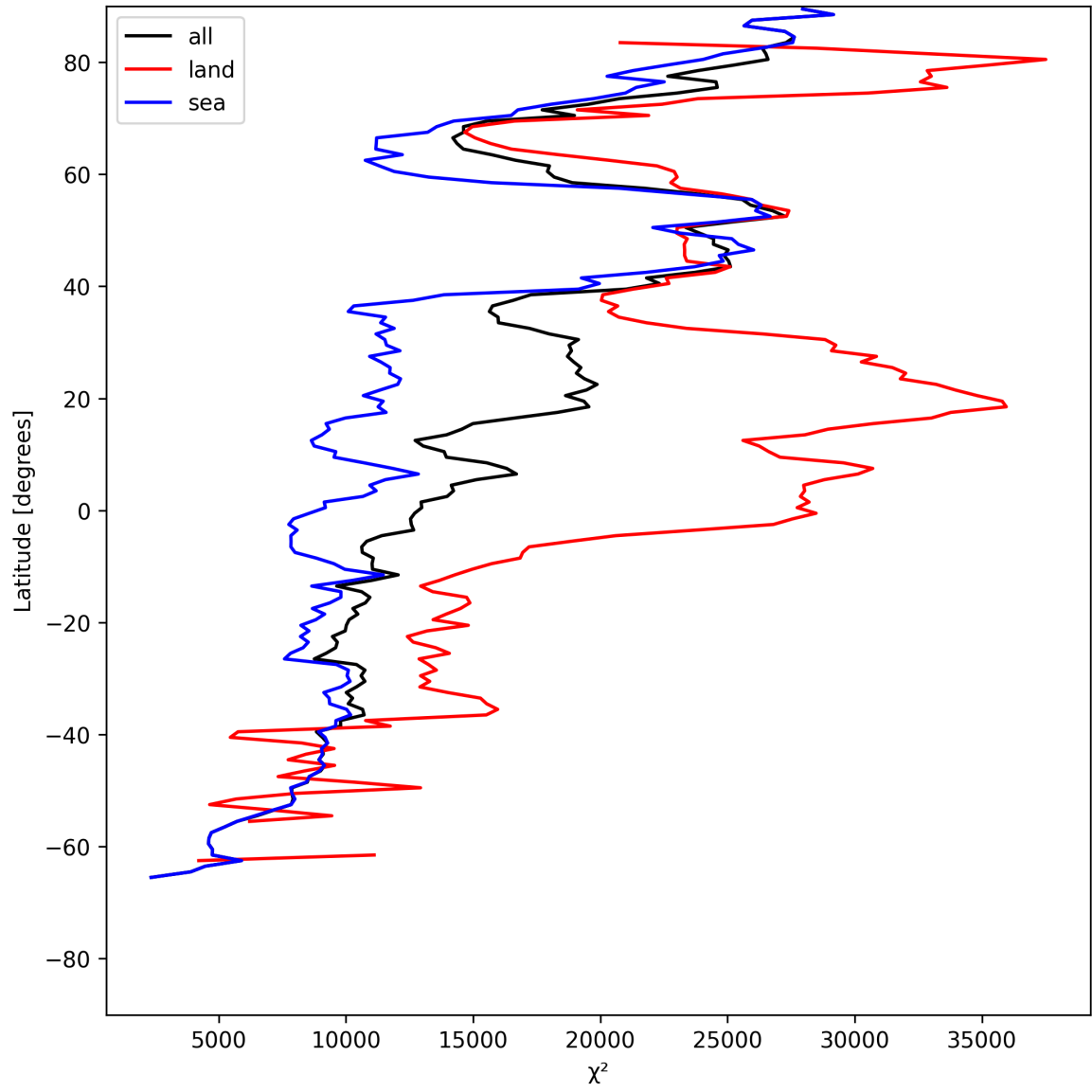
Figure 19: Zonal average of “ \chi^2 ” for 2025-07-11 to 2025-07-11.
