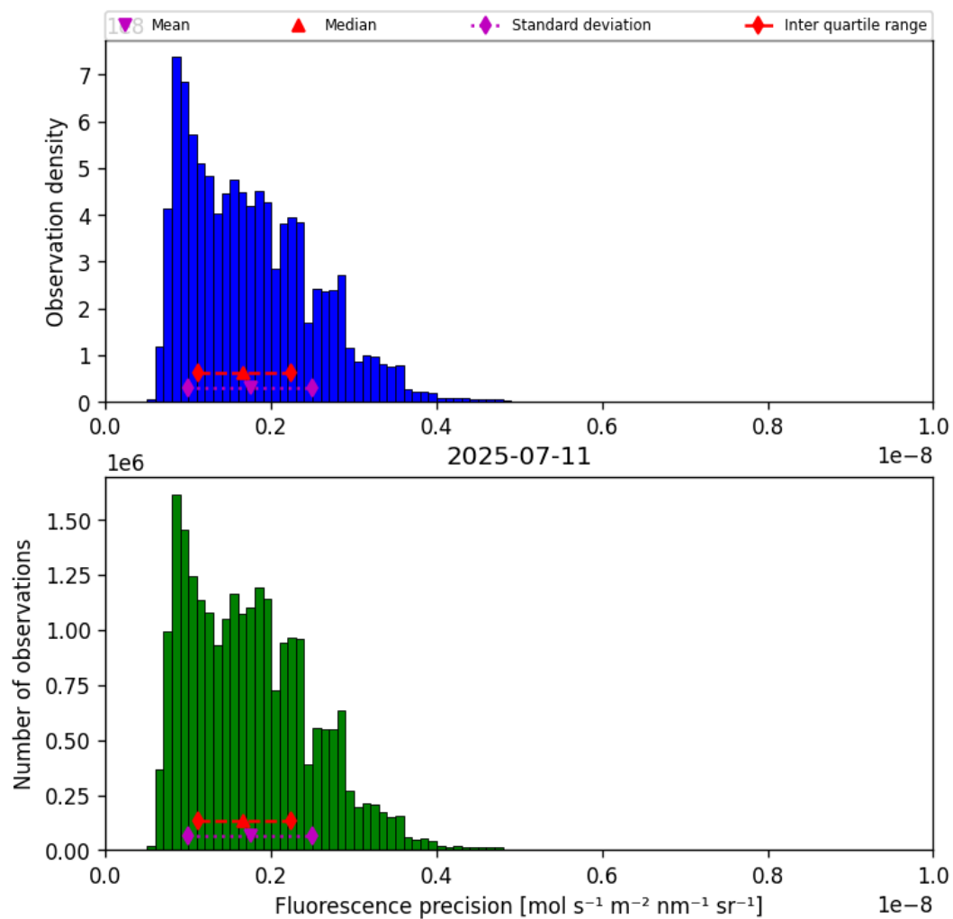
Figure 39: Histogram of “Fluorescence precision” for 2025-07-11 to 2025-07-11
