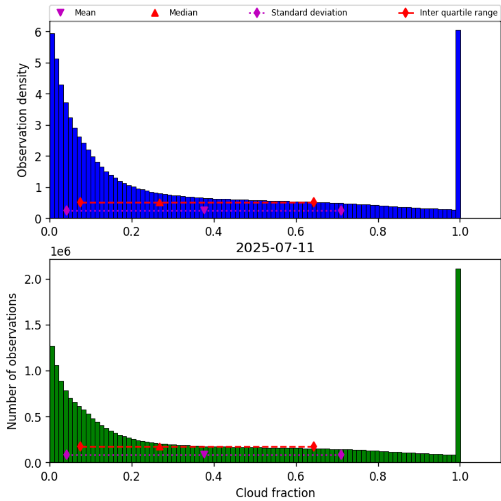
Figure 30: Histogram of “Cloud fraction” for 2025-07-11 to 2025-07-11
