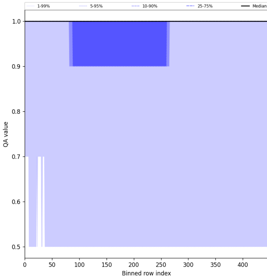
Figure 44: Along track statistics of “QA value” for 2025-07-11 to 2025-07-11
