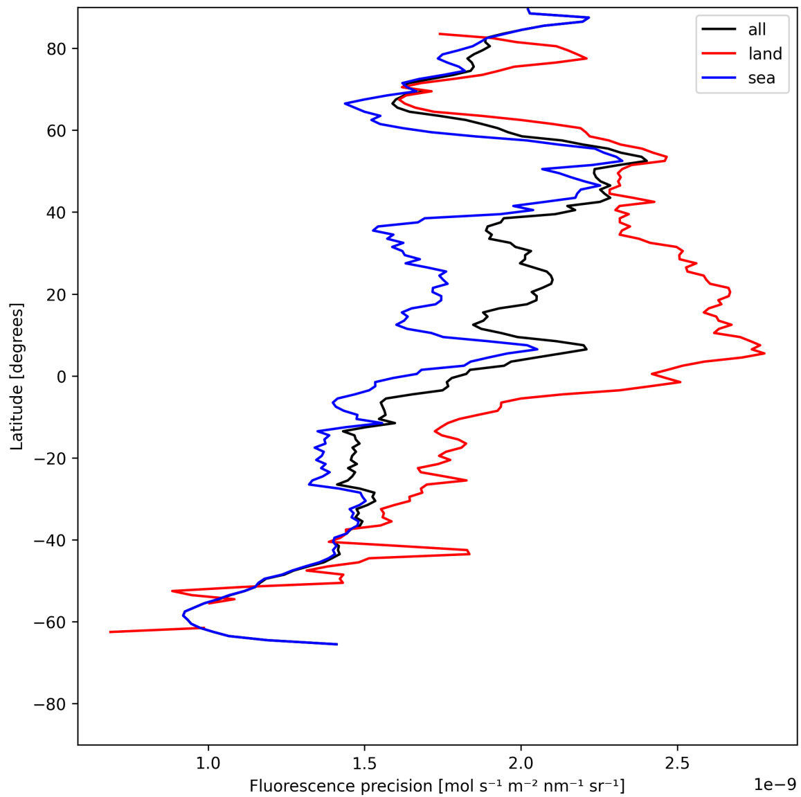
Figure 22: Zonal average of “Fluorescence precision” for 2025-07-11 to 2025-07-11.
