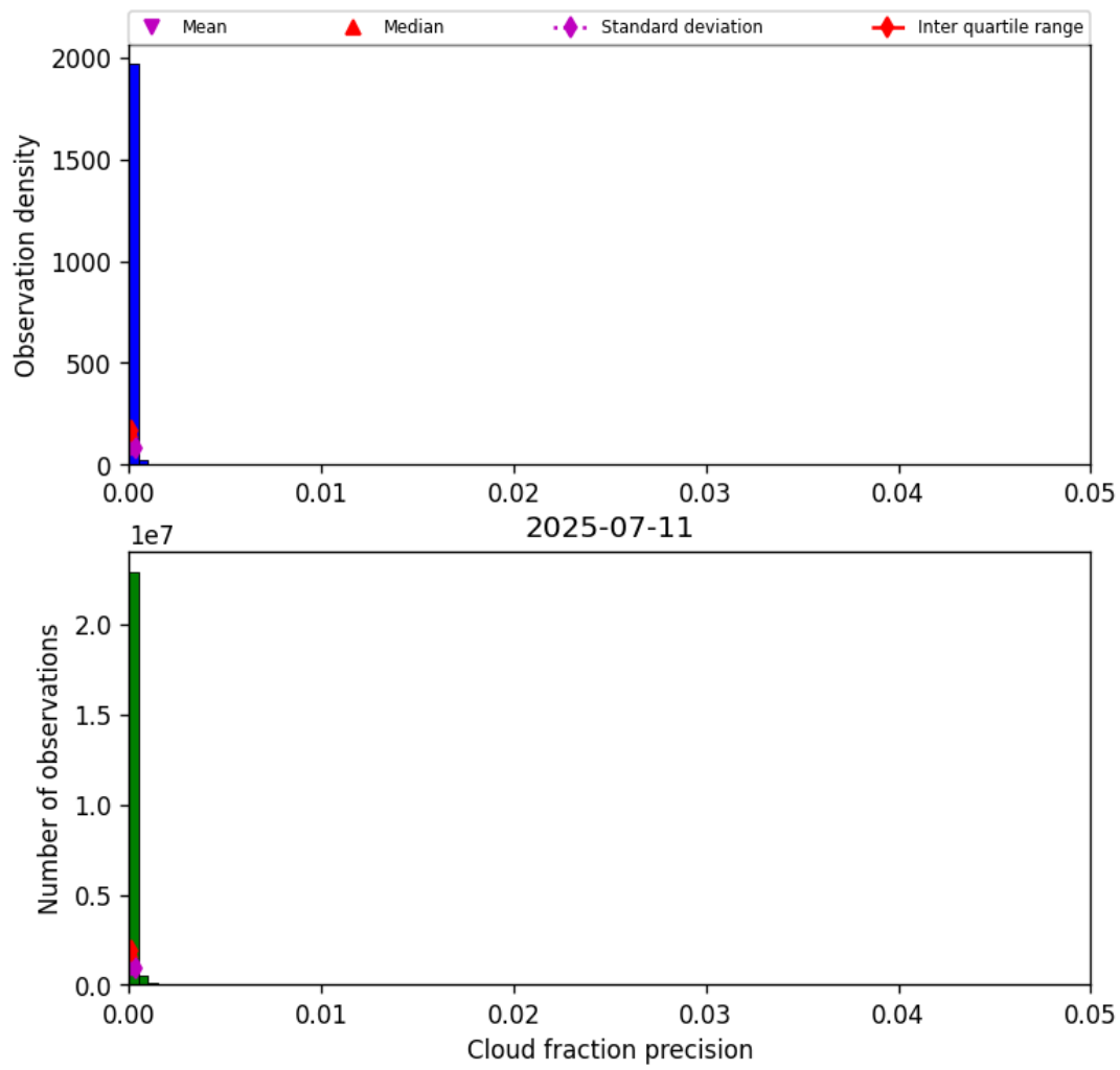
Figure 31: Histogram of “Cloud fraction precision” for 2025-07-11 to 2025-07-11
