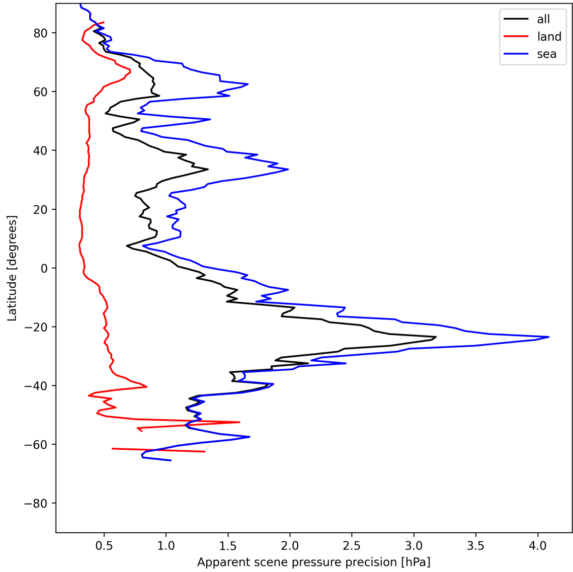
Figure 18: Zonal average of “Apparent scene pressure precision” for 2025-07-11 to 2025-07-11.
