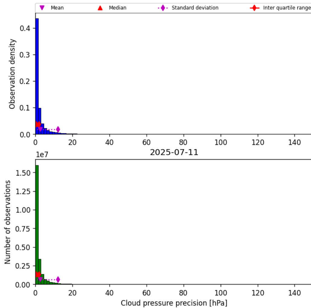
Figure 29: Histogram of “Cloud pressure precision” for 2025-07-11 to 2025-07-11
