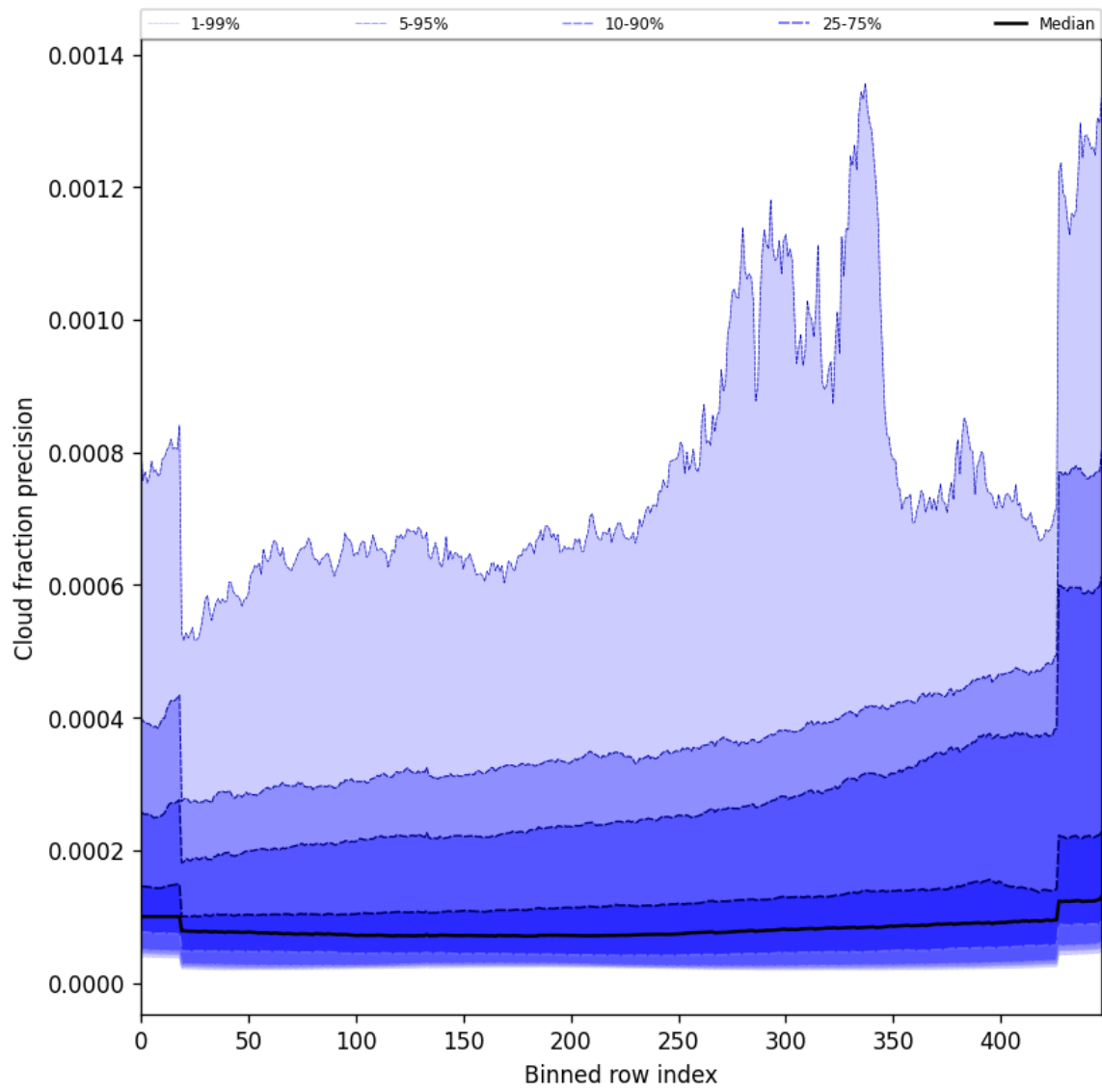
Figure 48: Along track statistics of “Cloud fraction precision” for 2025-07-11 to 2025-07-11
