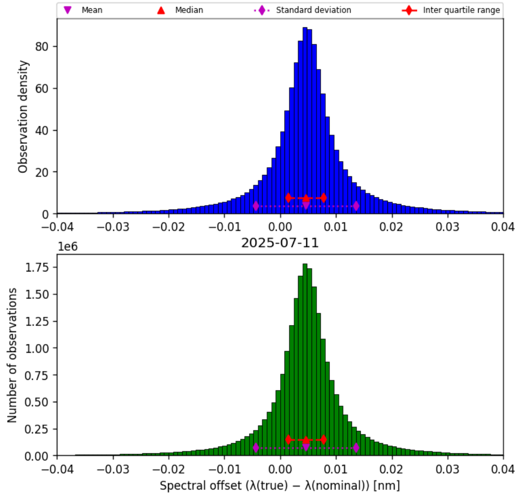
Figure 43: Histogram of “Spectral offset ( \lambda_{\text{true}} - \lambda_{\text{nominal}} )” for 2025-07-11 to 2025-07-11
