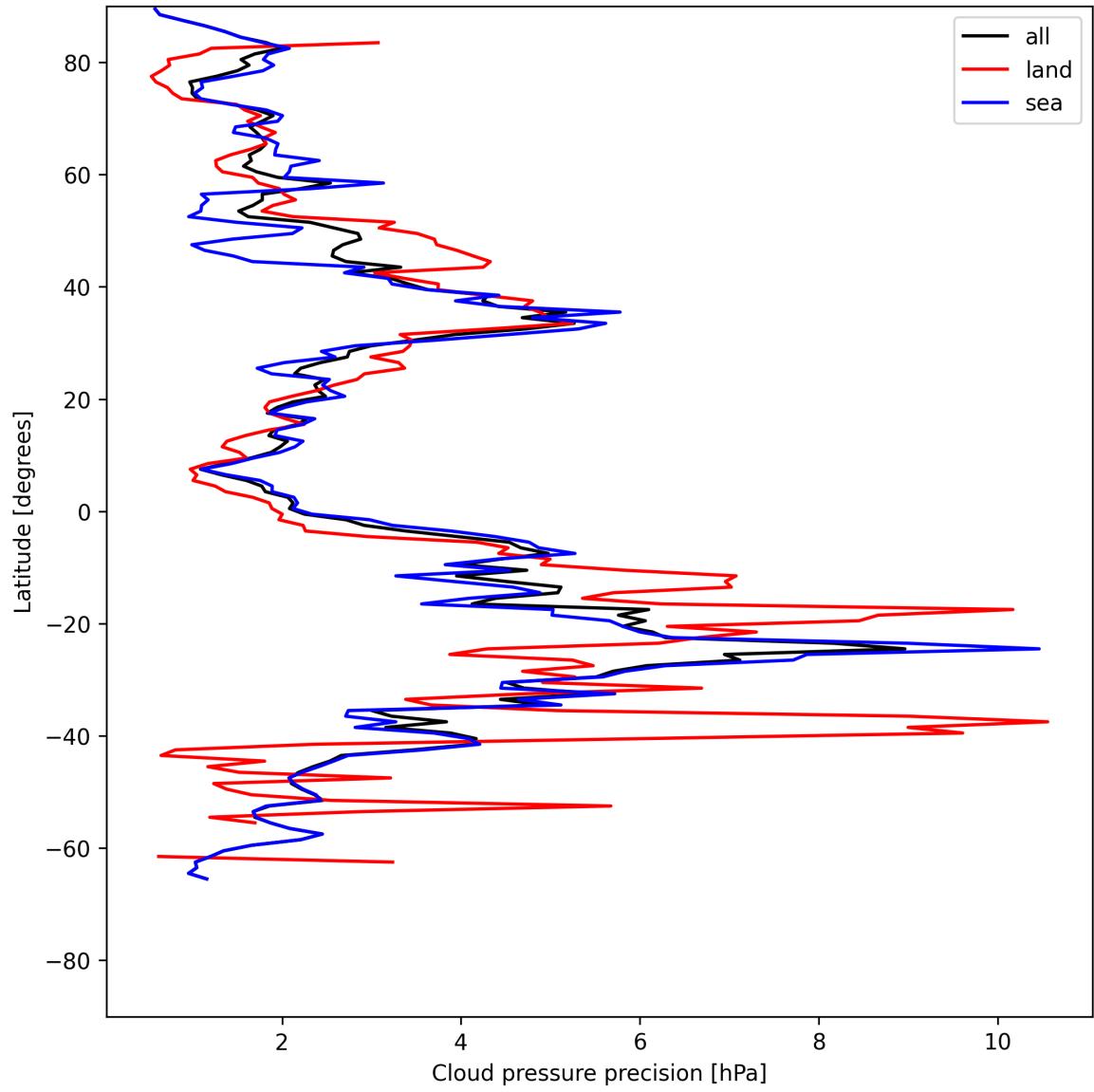
Figure 12: Zonal average of “Cloud pressure precision” for 2025-07-11 to 2025-07-11.
