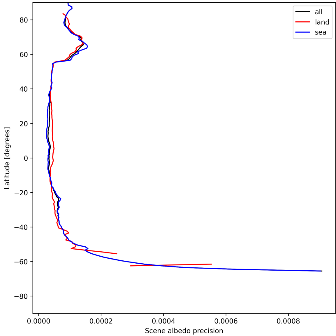
Figure 16: Zonal average of “Scene albedo precision” for 2025-07-11 to 2025-07-11.
