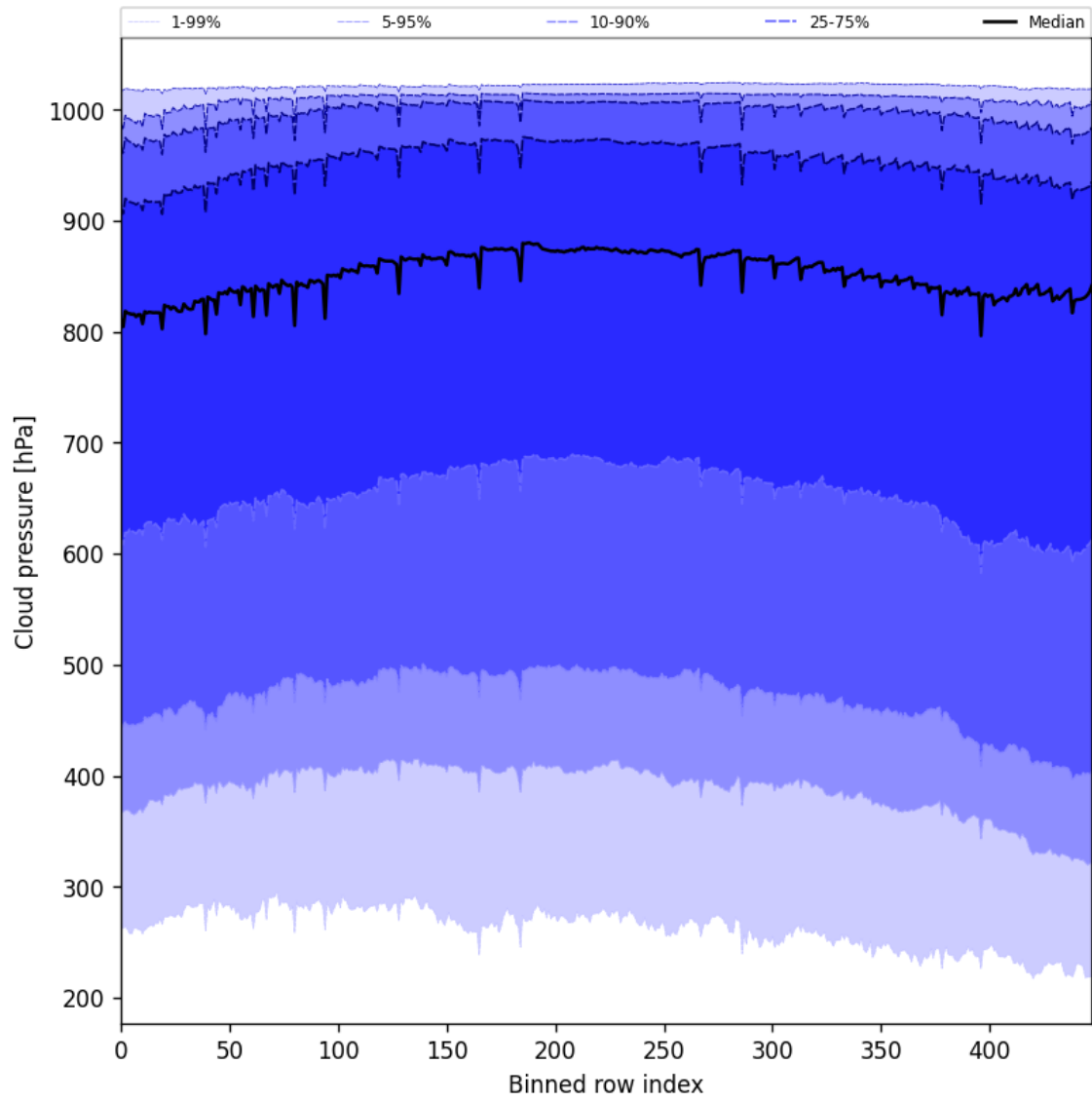
Figure 45: Along track statistics of “Cloud pressure” for 2025-07-11 to 2025-07-11
