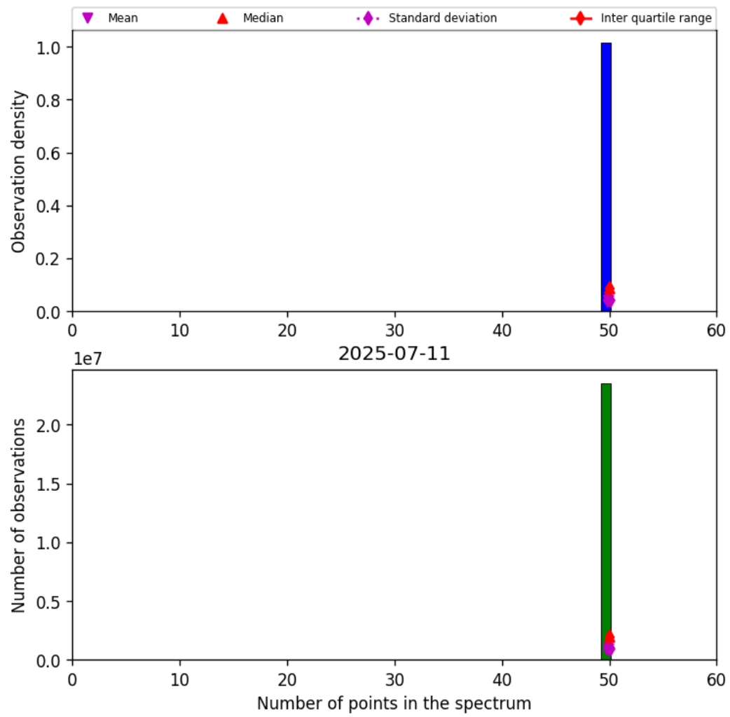
Figure 42: Histogram of "Number of points in the spectrum" for 2025-07-11 to 2025-07-11
