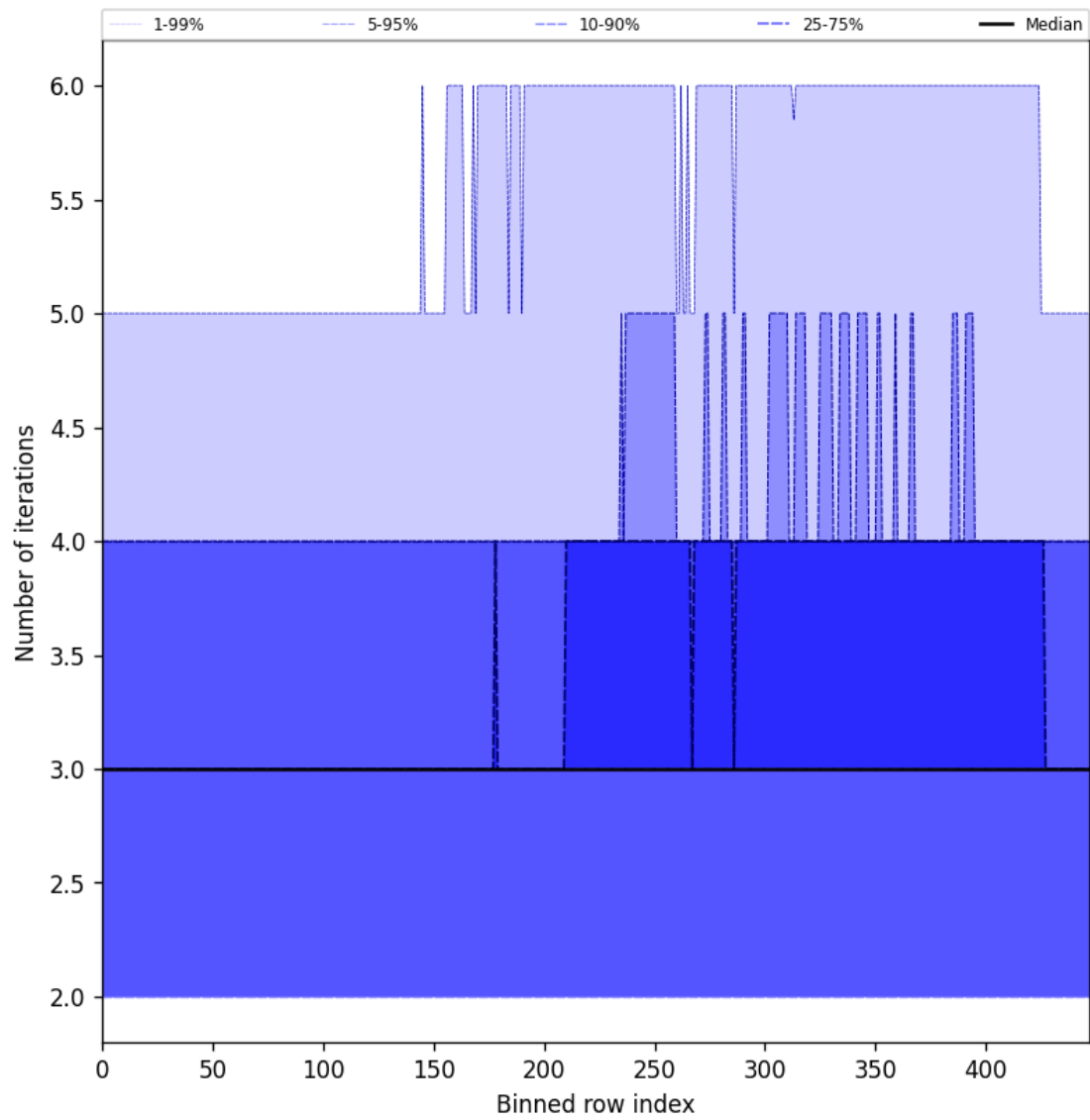
Figure 54: Along track statistics of “Number of iterations” for 2025-07-11 to 2025-07-11
