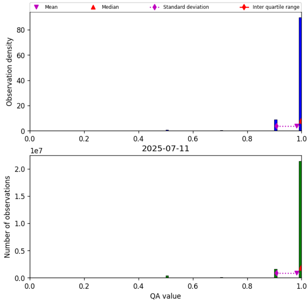
Figure 27: Histogram of “QA value” for 2025-07-11 to 2025-07-11
