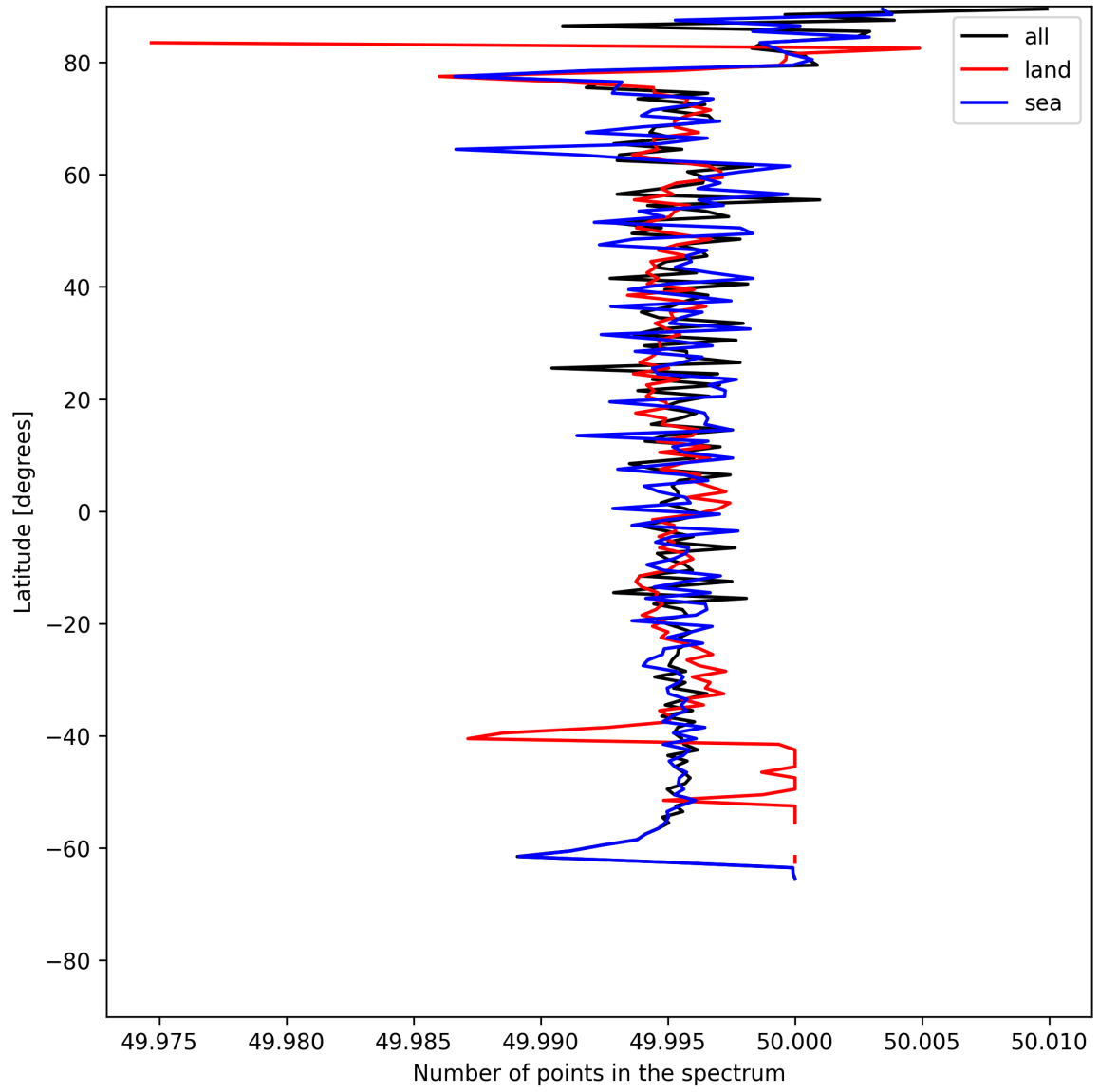
Figure 25: Zonal average of “Number of points in the spectrum” for 2025-07-11 to 2025-07-11.
