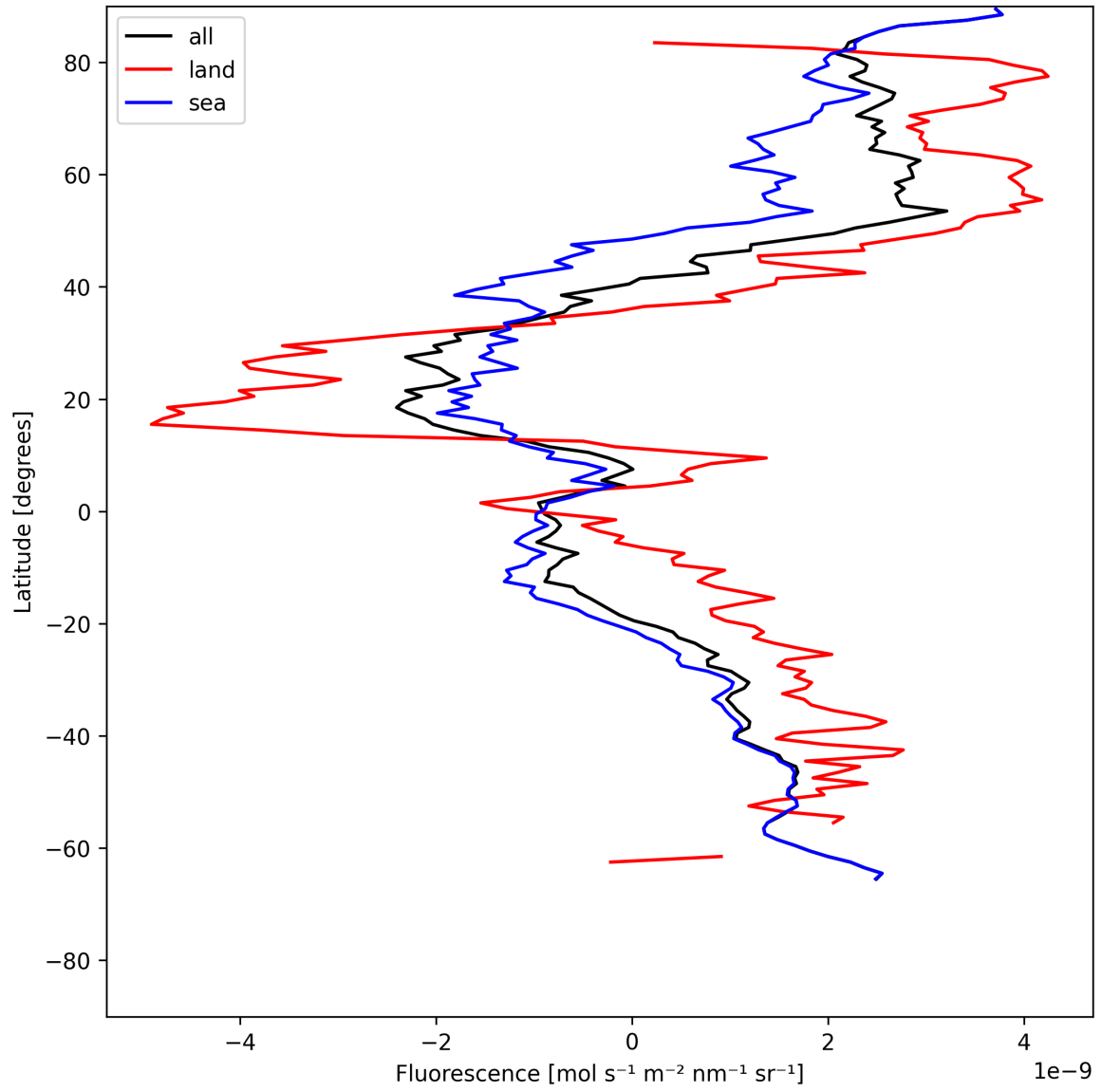
Figure 21: Zonal average of “Fluorescence” for 2025-07-11 to 2025-07-11.
