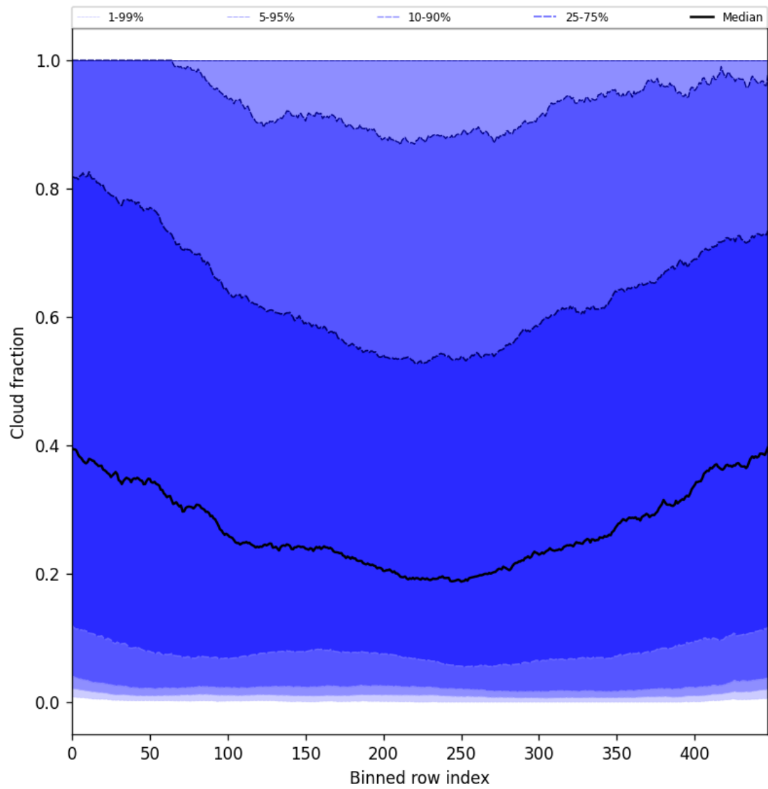
Figure 47: Along track statistics of “Cloud fraction” for 2025-07-11 to 2025-07-11
