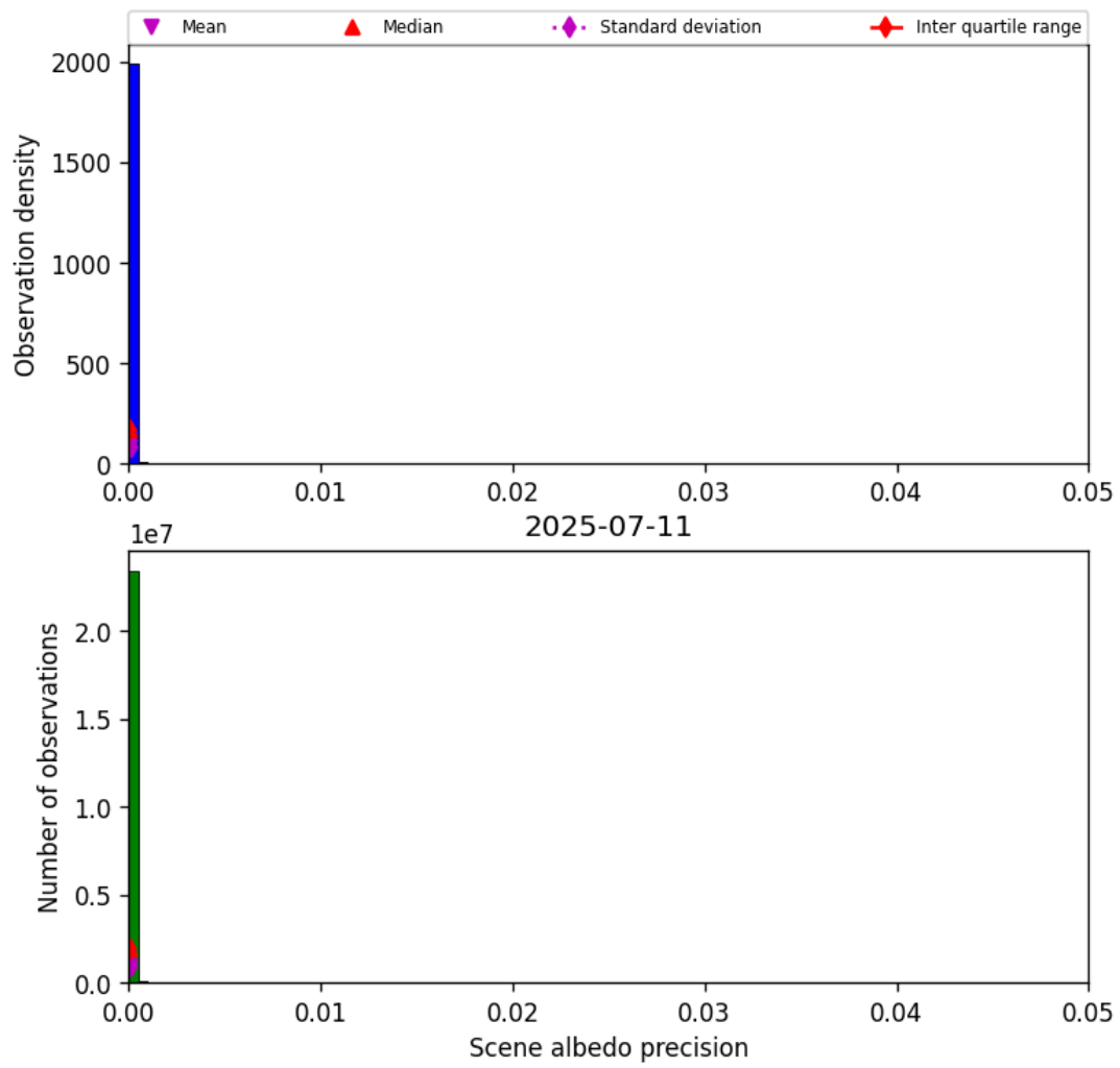
Figure 33: Histogram of “Scene albedo precision” for 2025-07-11 to 2025-07-11
