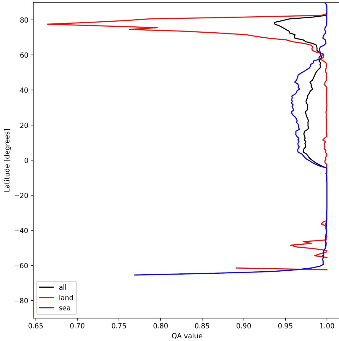
Figure 10: Zonal average of “QA value” for 2025-07-11 to 2025-07-11.
