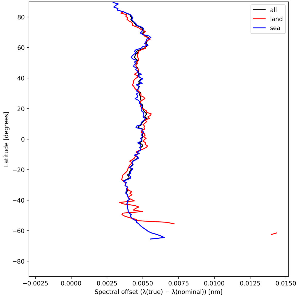
Figure 26: Zonal average of “Spectral offset ( \lambda_{\text{true}} - \lambda_{\text{nominal}} )” for 2025-07-11 to 2025-07-11.
