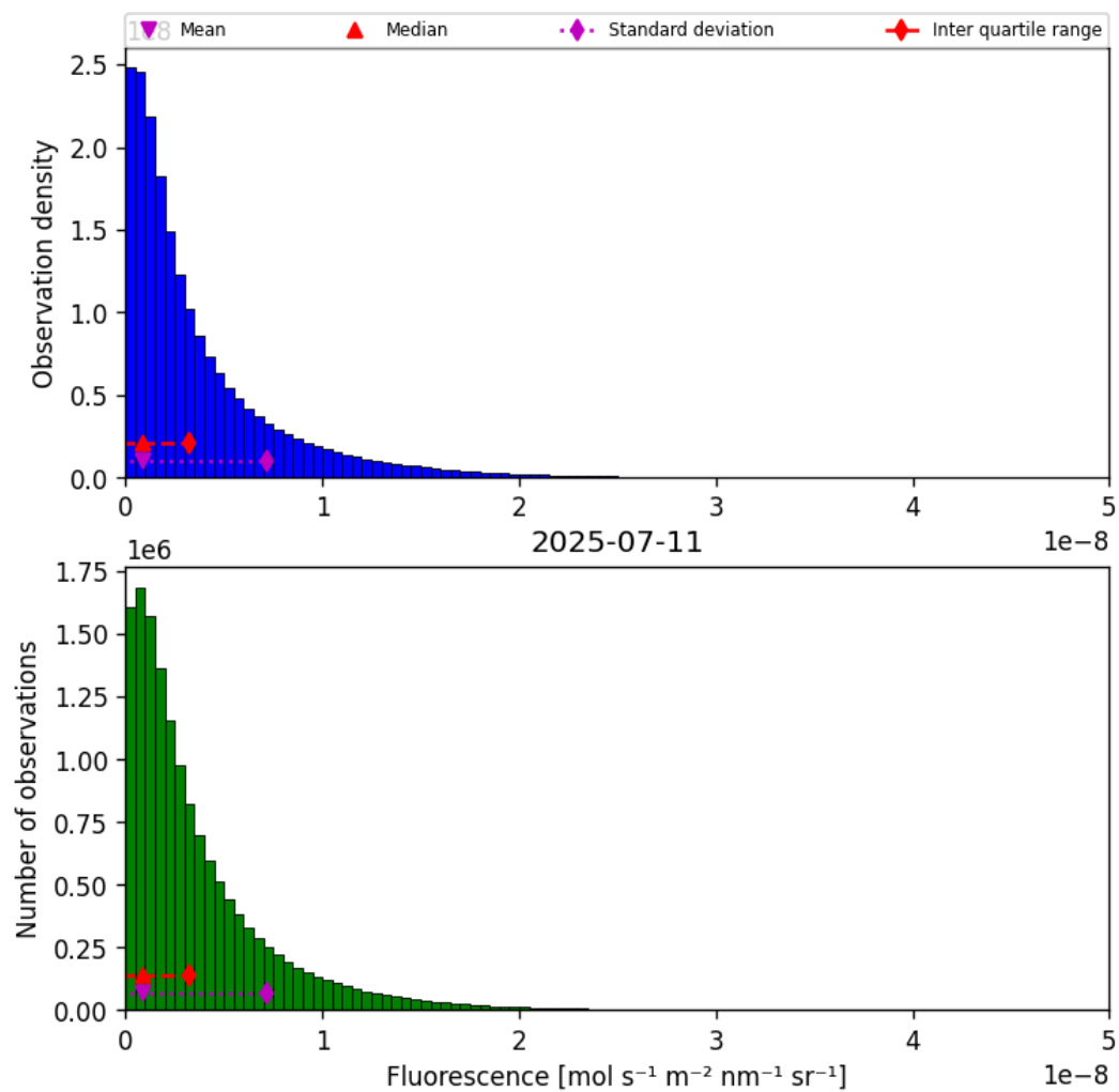
Figure 38: Histogram of “Fluorescence” for 2025-07-11 to 2025-07-11
