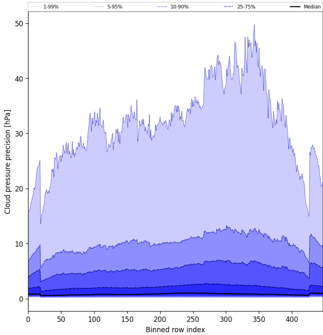
Figure 46: Along track statistics of “Cloud pressure precision” for 2025-07-11 to 2025-07-11
