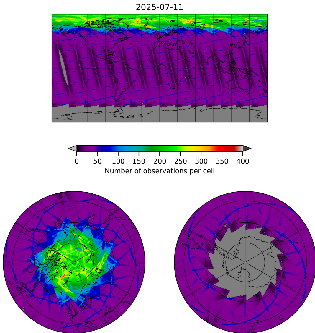
Figure 9: Map of the number of observations for 2025-07-11 to 2025-07-11
