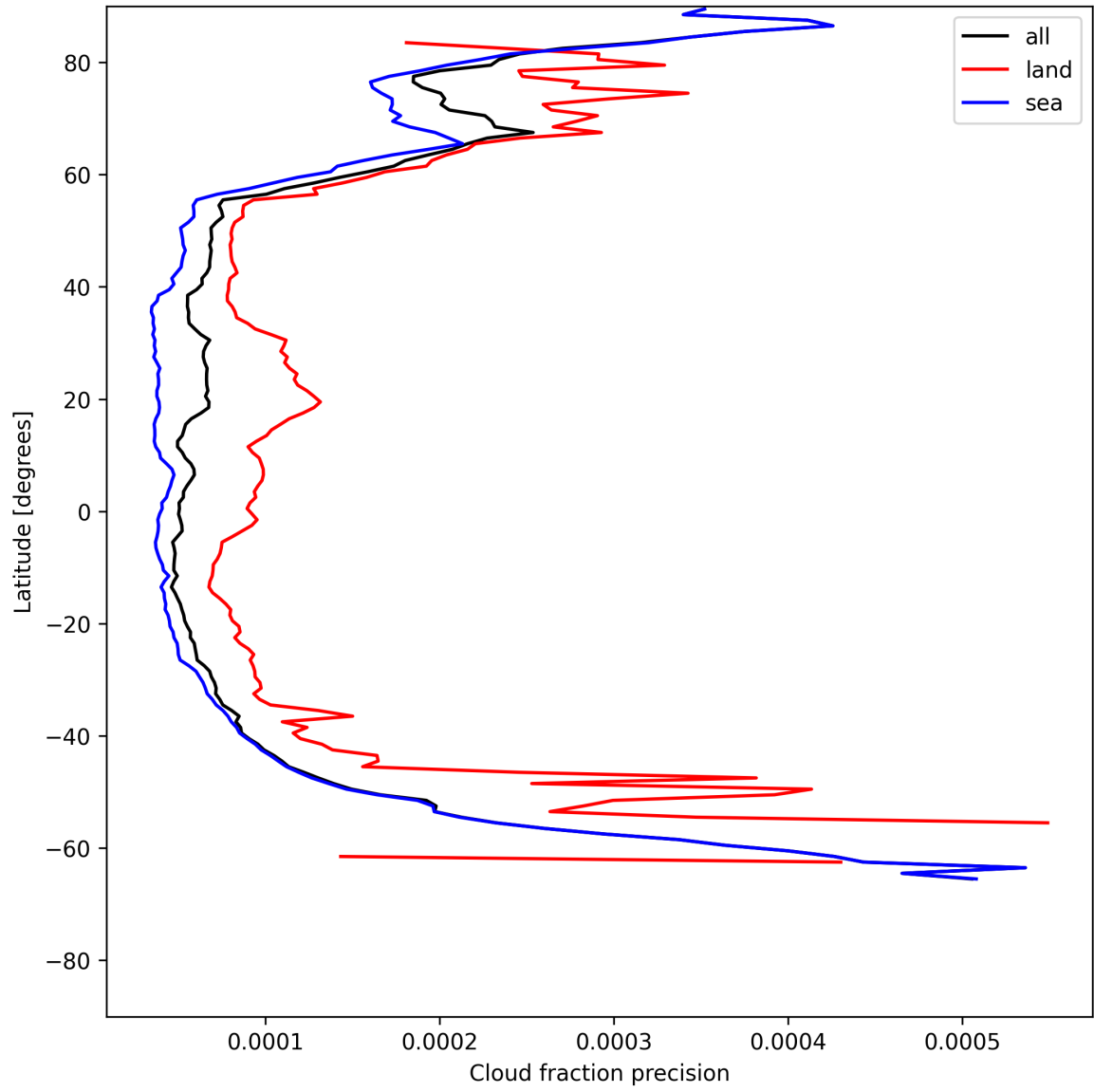
Figure 14: Zonal average of “Cloud fraction precision” for 2025-07-11 to 2025-07-11.
