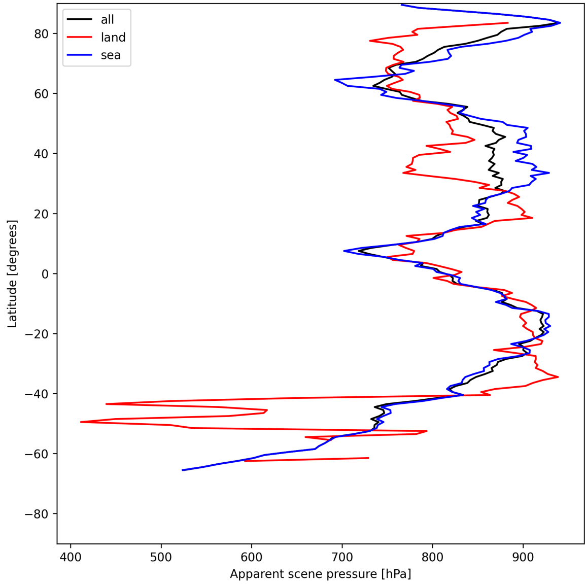
Figure 17: Zonal average of “Apparent scene pressure” for 2025-07-11 to 2025-07-11.
