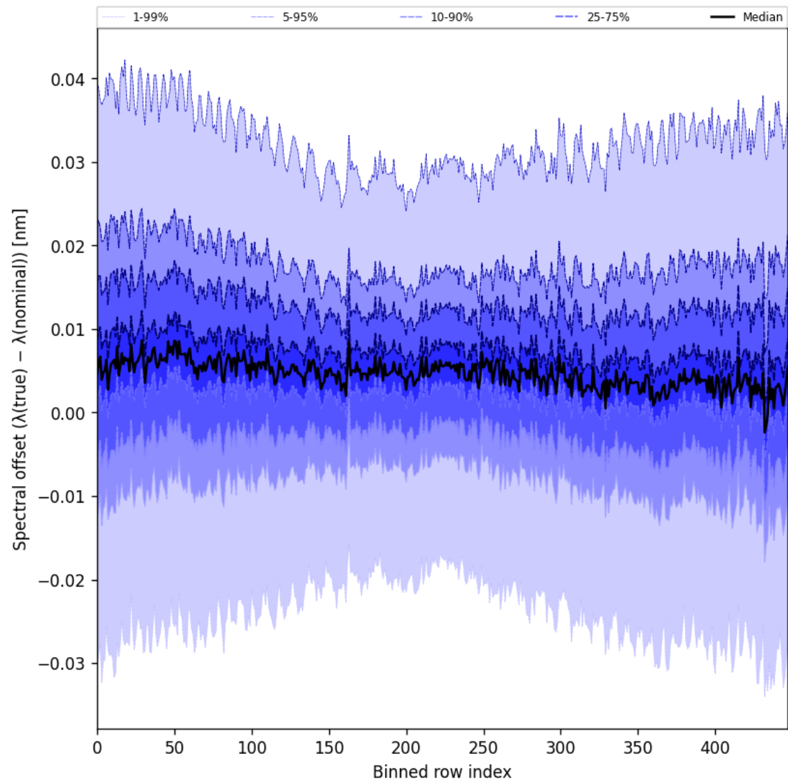
Figure 60: Along track statistics of “Spectral offset ( \lambda_{\text{true}} - \lambda_{\text{nominal}} )” for 2025-07-11 to 2025-07-11
