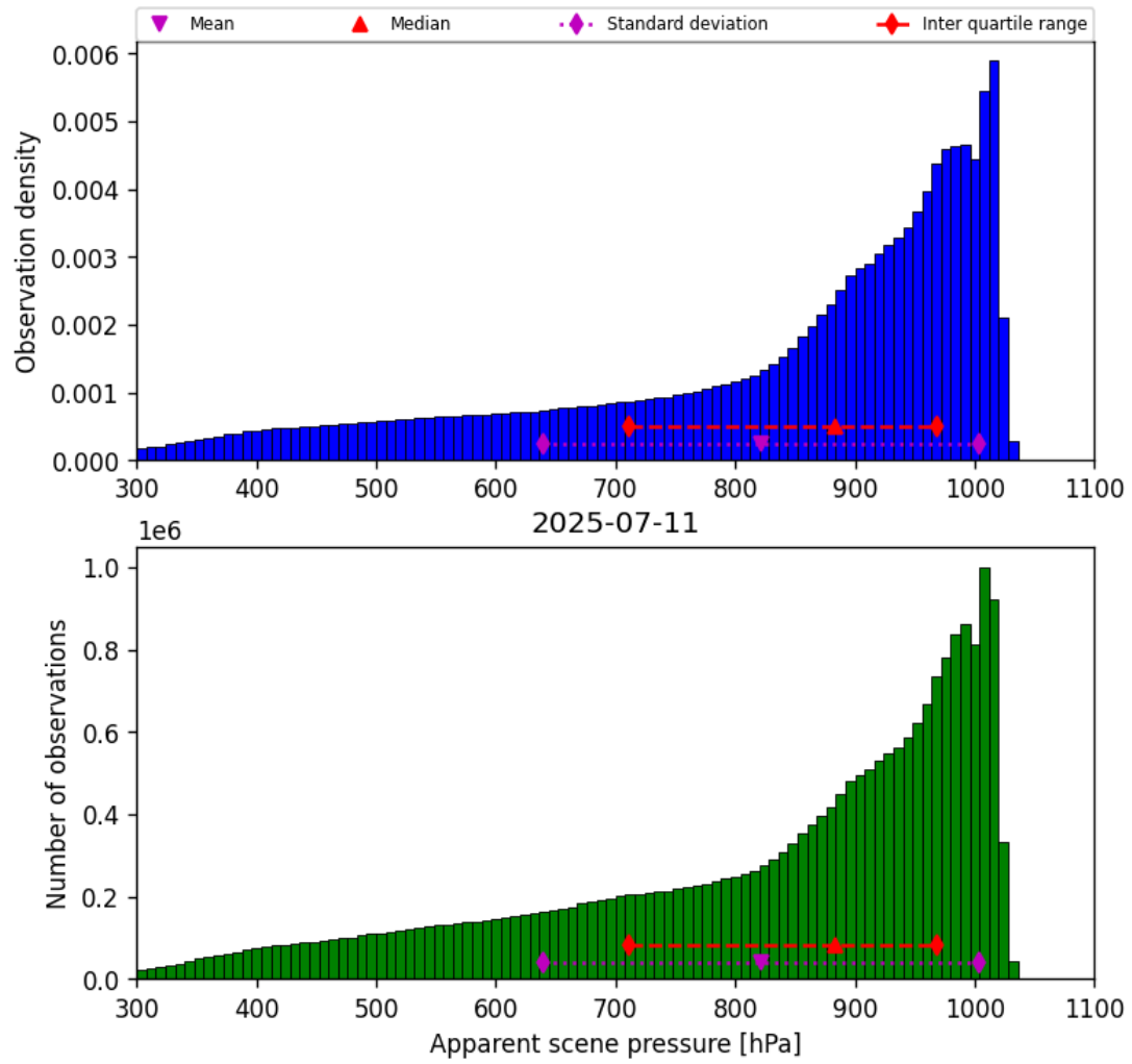
Figure 34: Histogram of “Apparent scene pressure” for 2025-07-11 to 2025-07-11
