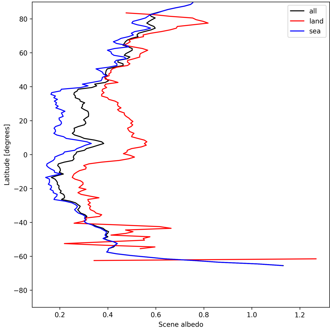
Figure 15: Zonal average of “Scene albedo” for 2025-07-11 to 2025-07-11.
