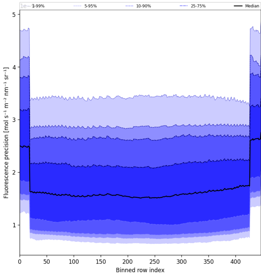
Figure 56: Along track statistics of “Fluorescence precision” for 2025-07-11 to 2025-07-11
