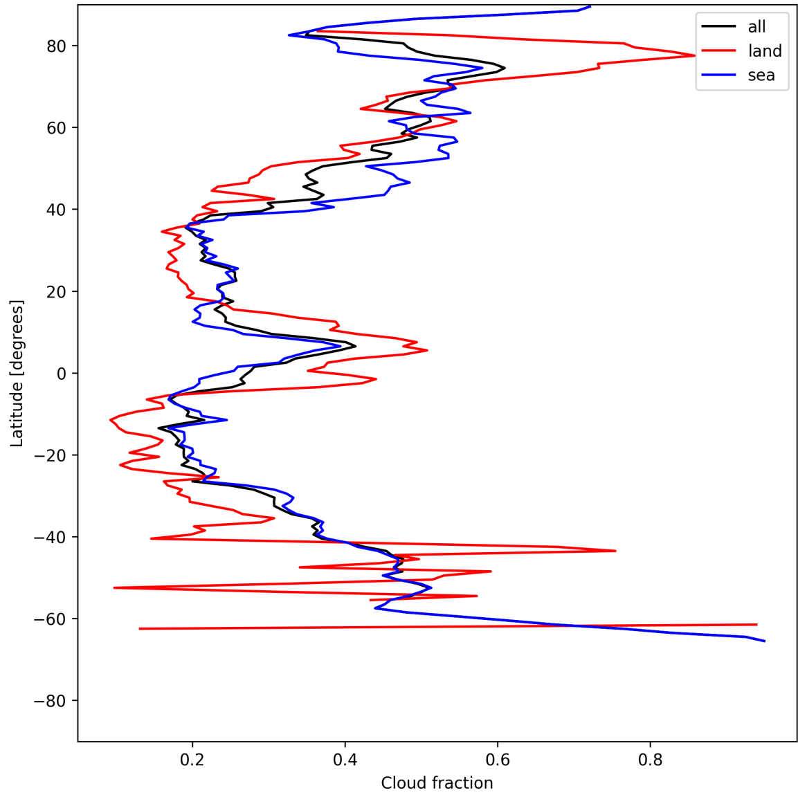
Figure 13: Zonal average of “Cloud fraction” for 2025-07-11 to 2025-07-11.
