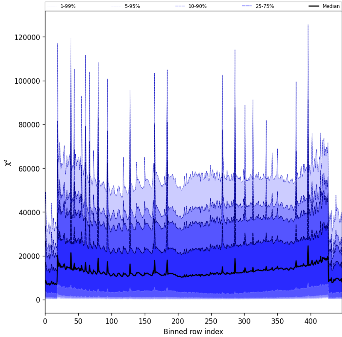
Figure 53: Along track statistics of “ \chi^2 ” for 2025-07-11 to 2025-07-11
