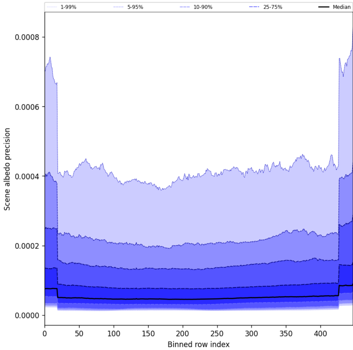
Figure 50: Along track statistics of “Scene albedo precision” for 2025-07-11 to 2025-07-11
