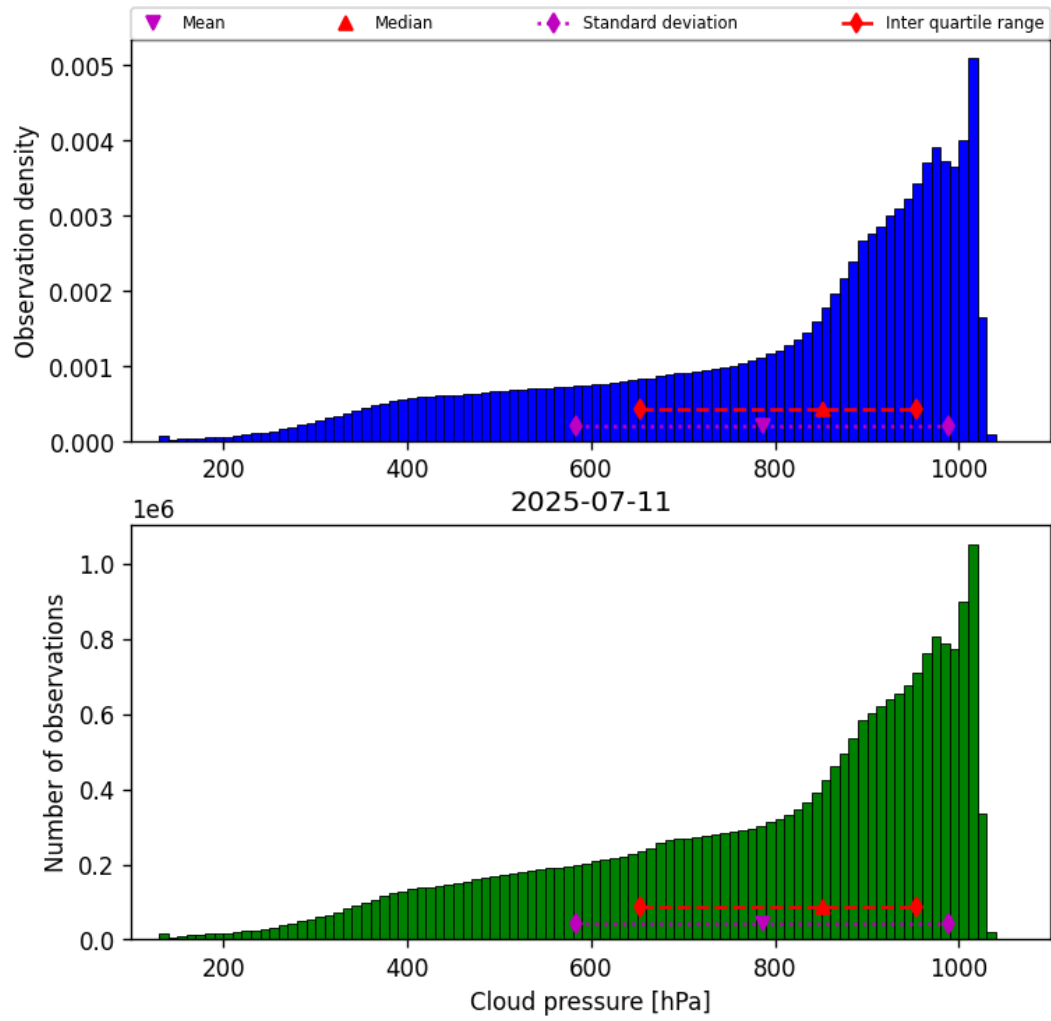
Figure 28: Histogram of “Cloud pressure” for 2025-07-11 to 2025-07-11
