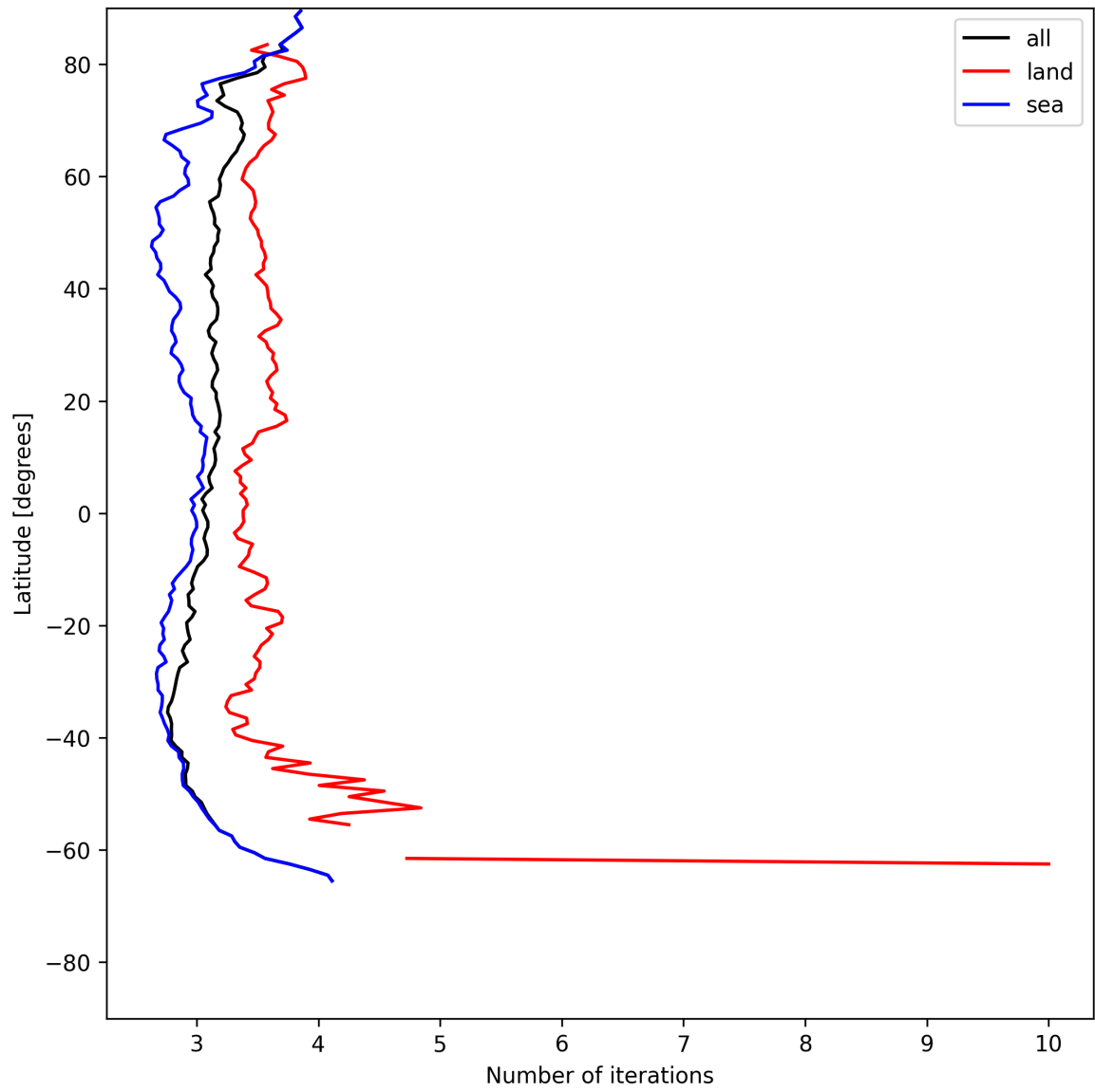
Figure 20: Zonal average of “Number of iterations” for 2025-07-11 to 2025-07-11.
