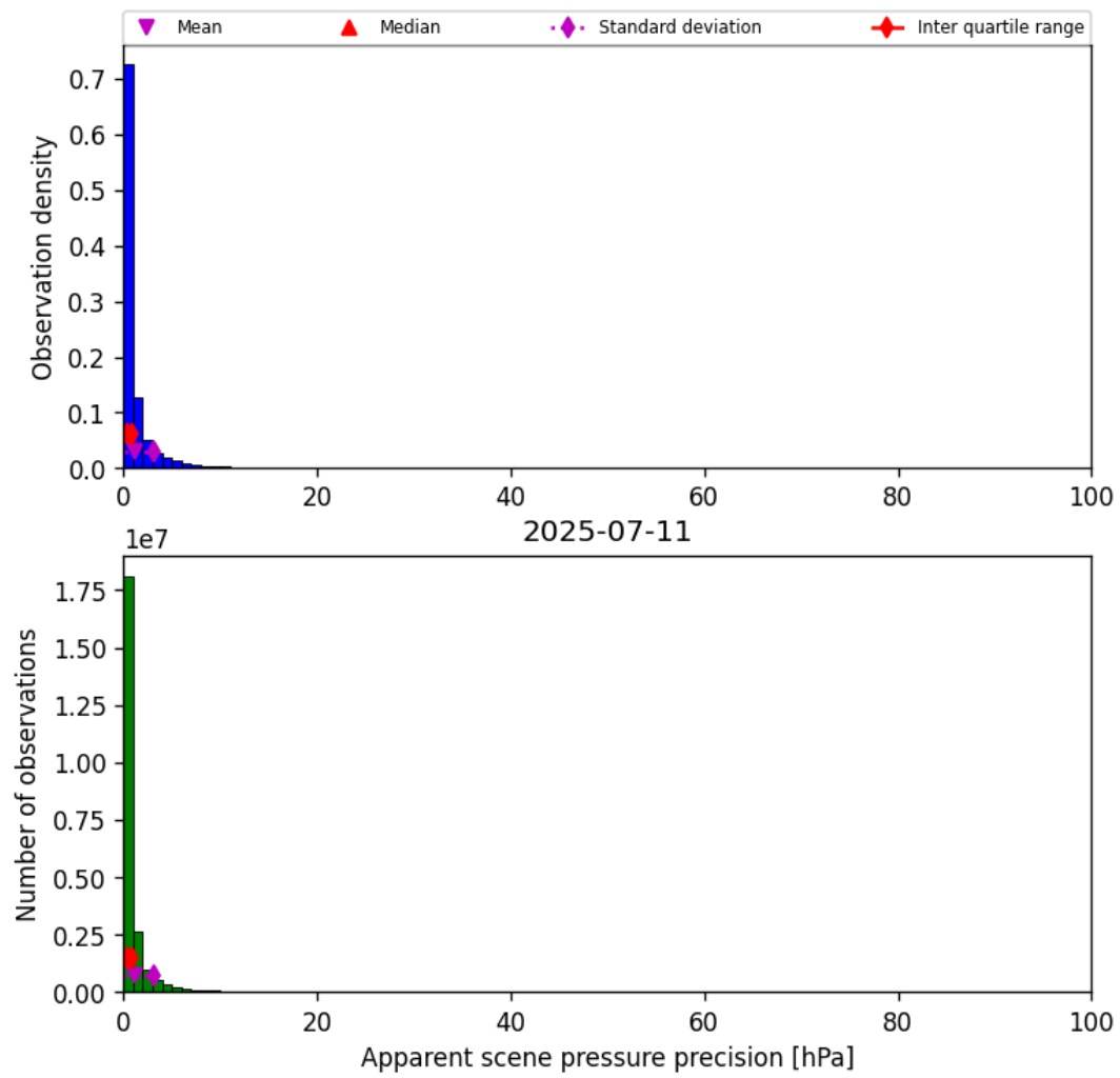
Figure 35: Histogram of “Apparent scene pressure precision” for 2025-07-11 to 2025-07-11
