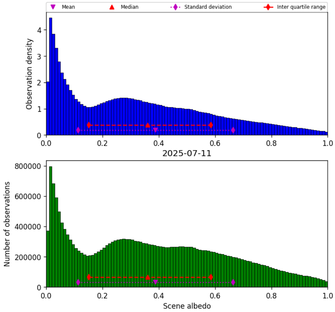
Figure 32: Histogram of “Scene albedo” for 2025-07-11 to 2025-07-11
