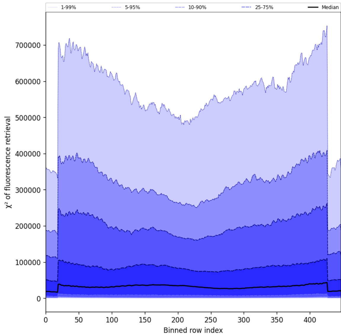
Figure 57: Along track statistics of “ \chi^2 of fluorescence retrieval” for 2025-07-11 to 2025-07-11
