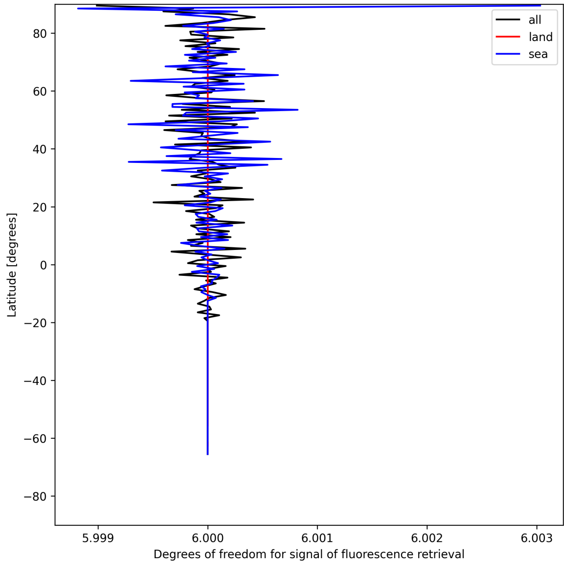
Figure 24: Zonal average of “Degrees of freedom for signal of fluorescence retrieval” for 2025-07-11 to 2025-07-11.
