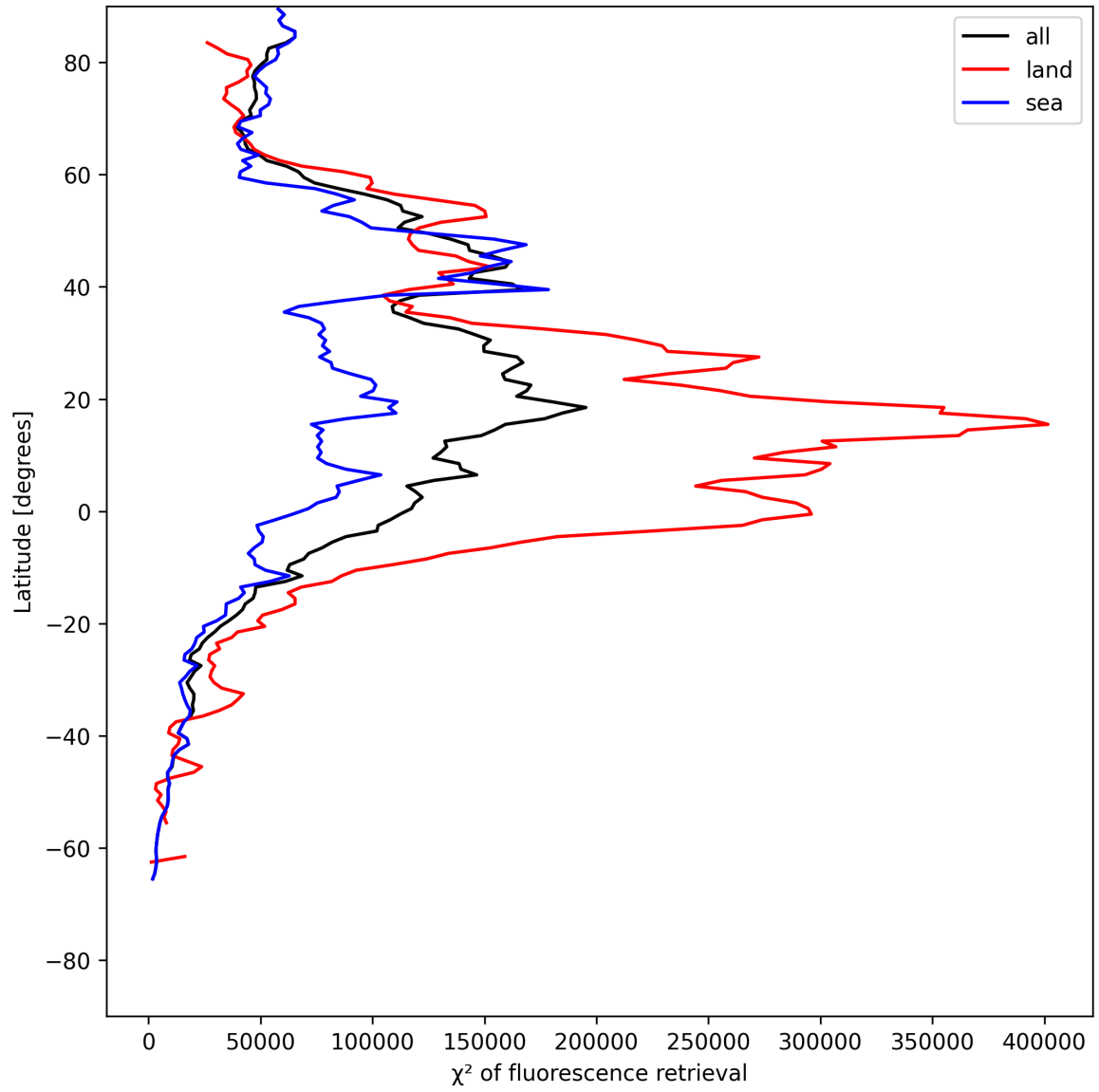
Figure 23: Zonal average of “ \chi^2 of fluorescence retrieval” for 2025-07-11 to 2025-07-11.
