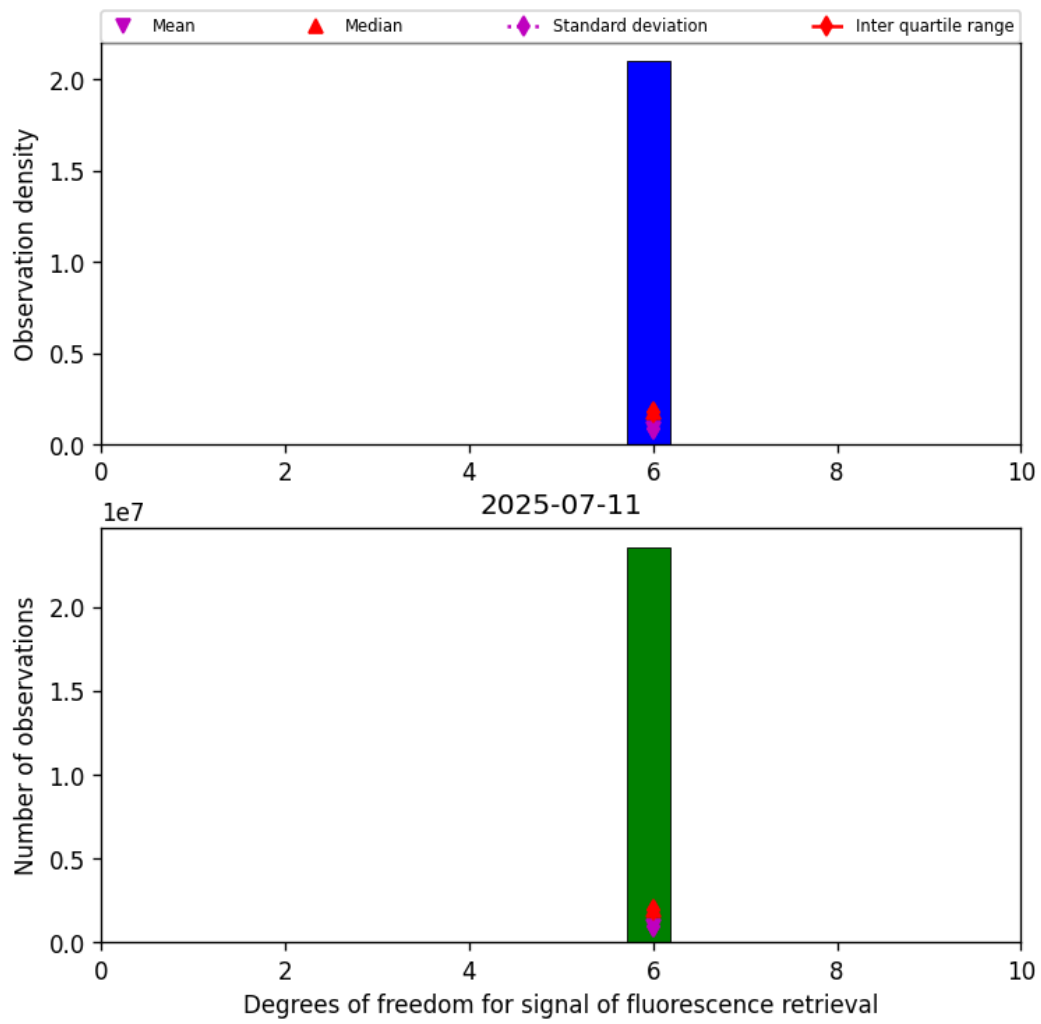
Figure 41: Histogram of “Degrees of freedom for signal of fluorescence retrieval” for 2025-07-11 to 2025-07-11
