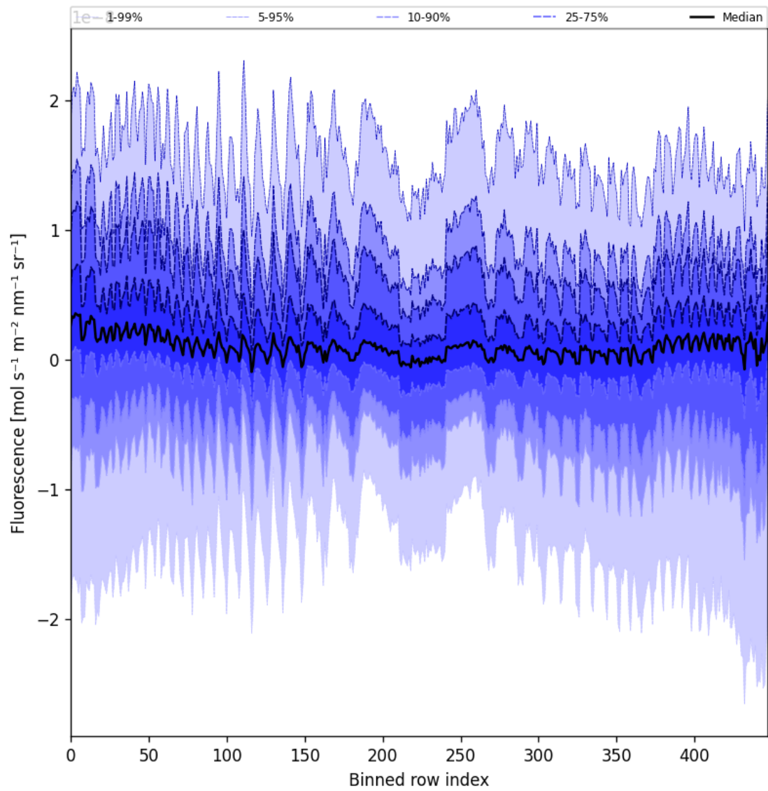
Figure 55: Along track statistics of “Fluorescence” for 2025-07-11 to 2025-07-11
