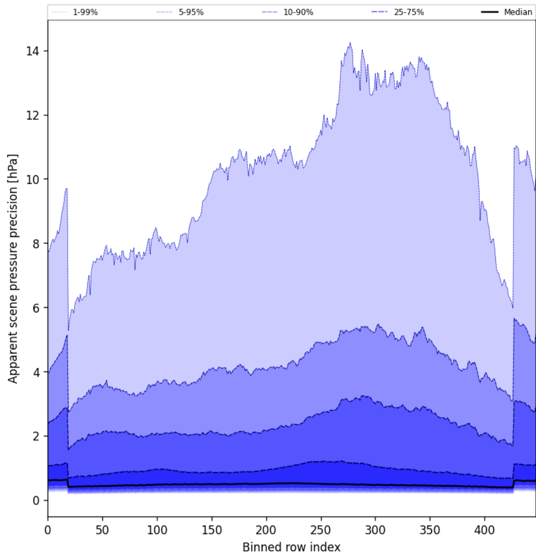
Figure 52: Along track statistics of “Apparent scene pressure precision” for 2025-07-11 to 2025-07-11
