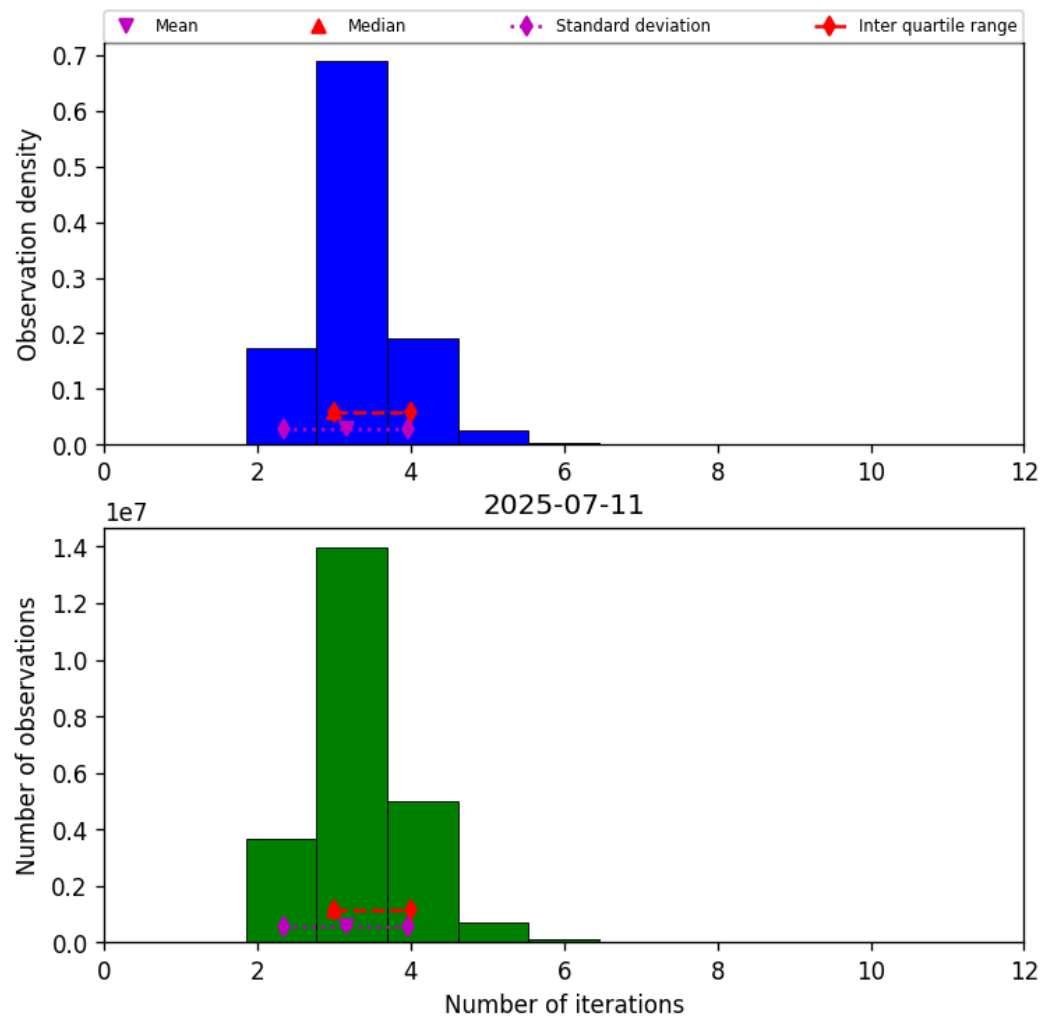
Figure 37: Histogram of “Number of iterations” for 2025-07-11 to 2025-07-11
