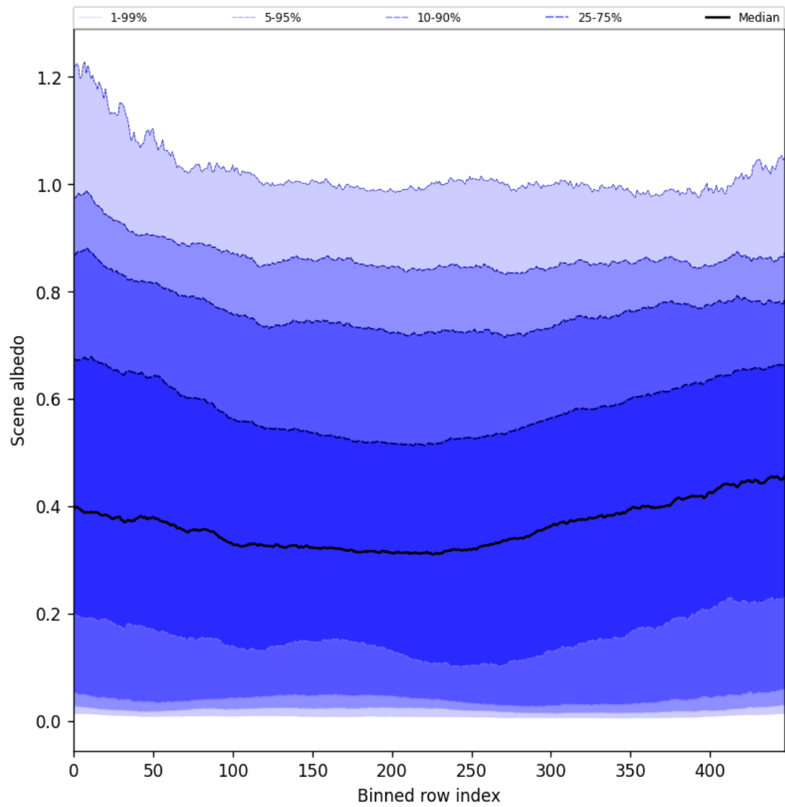
Figure 49: Along track statistics of “Scene albedo” for 2025-07-11 to 2025-07-11
