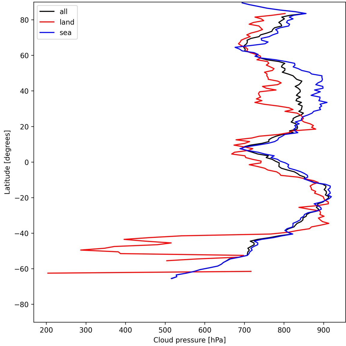
Figure 11: Zonal average of “Cloud pressure” for 2025-07-11 to 2025-07-11.
