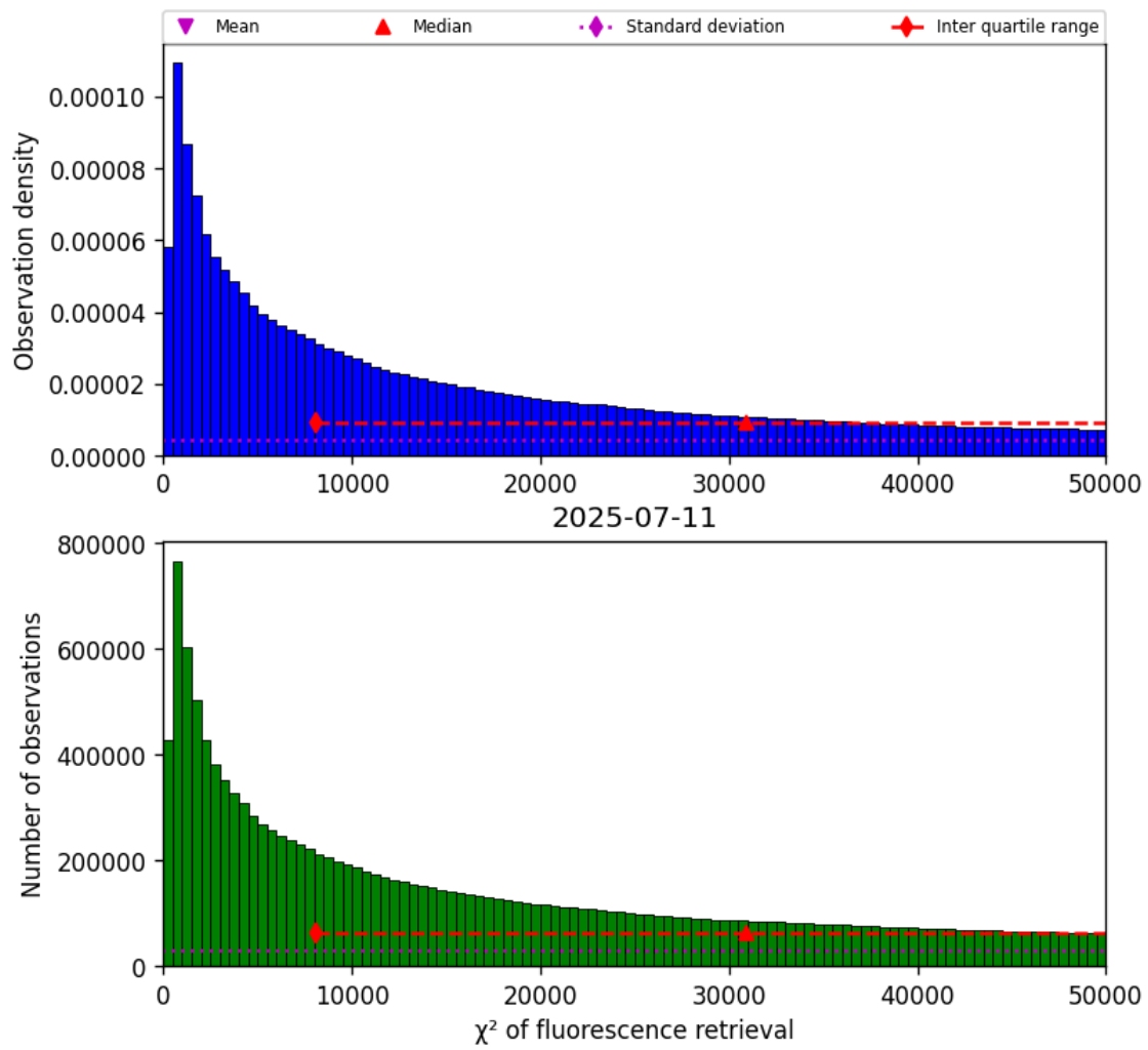
Figure 40: Histogram of “ \chi^2 of fluorescence retrieval” for 2025-07-11 to 2025-07-11
