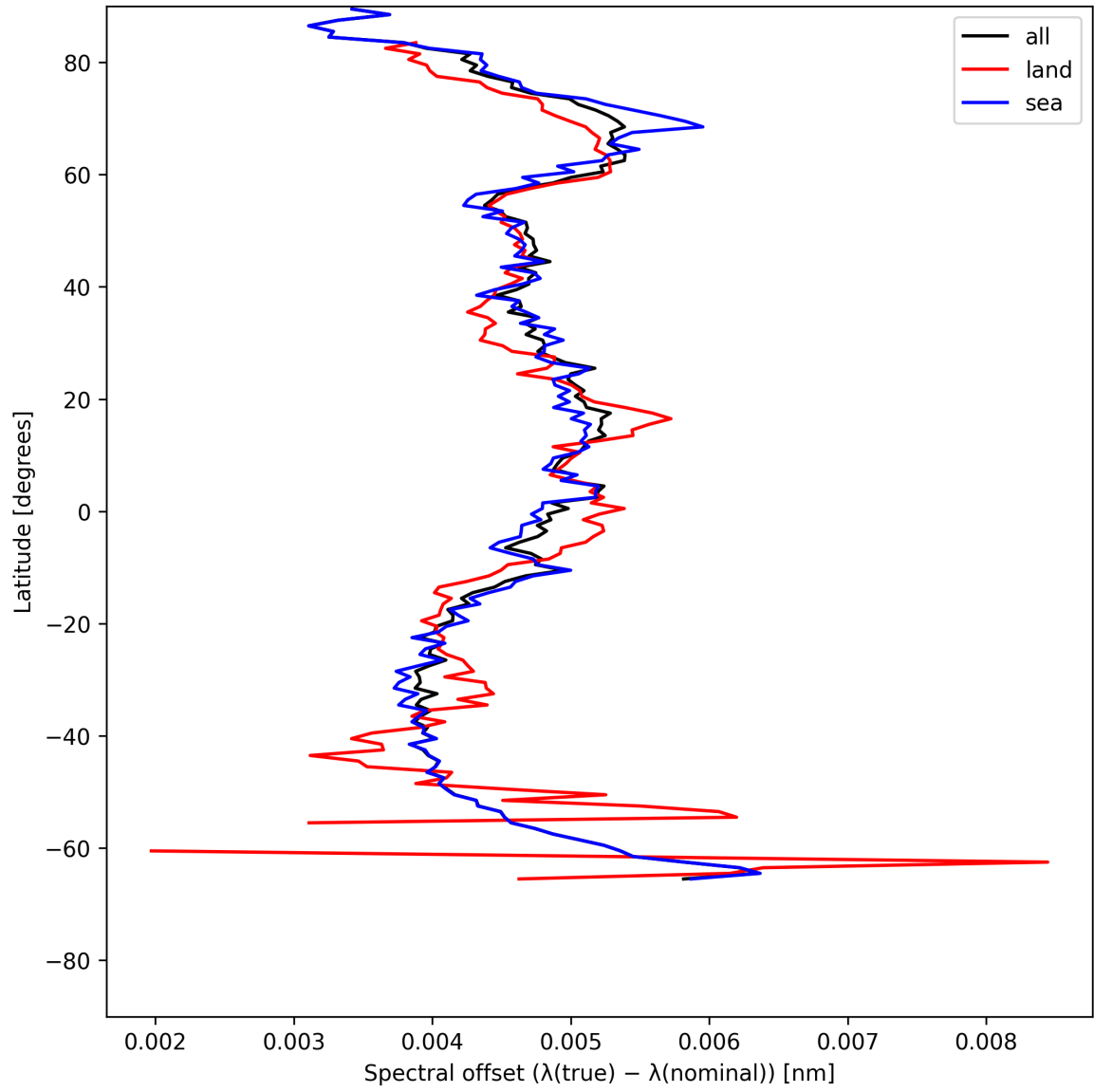
Figure 26: Zonal average of “Spectral offset ( \lambda_{\text{true}} - \lambda_{\text{nominal}} )” for 2025-07-13 to 2025-07-14.
