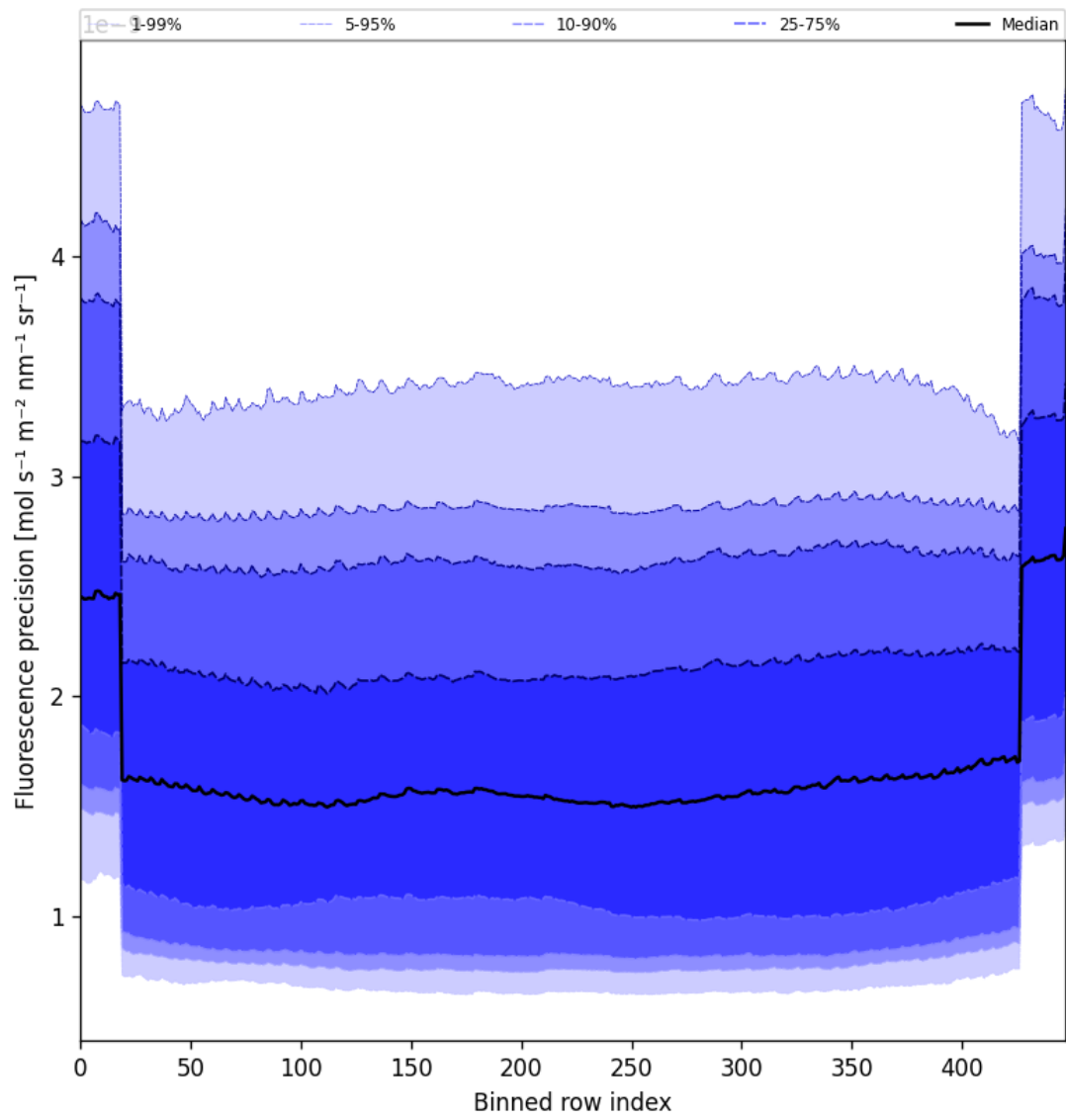
Figure 56: Along track statistics of “Fluorescence precision” for 2025-07-13 to 2025-07-14
