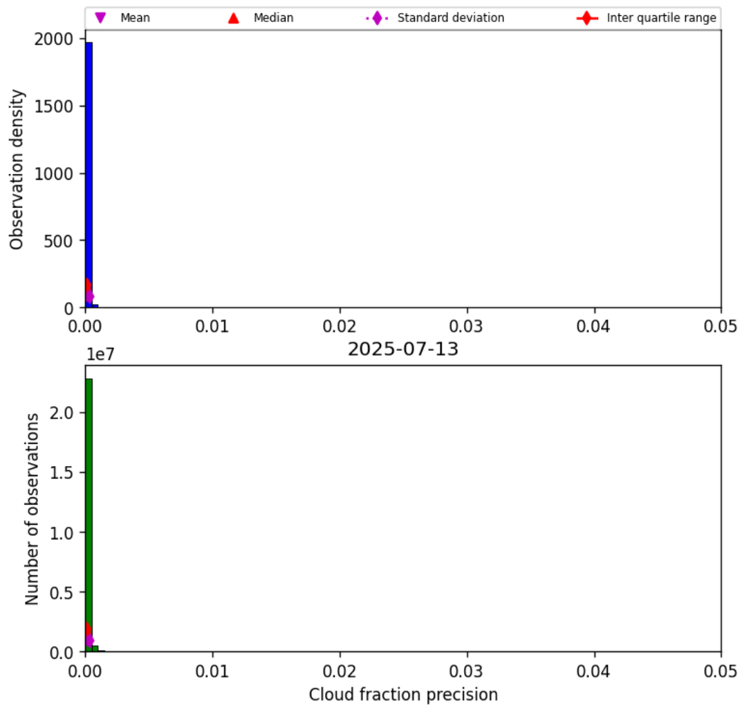
Figure 31: Histogram of “Cloud fraction precision” for 2025-07-13 to 2025-07-14
