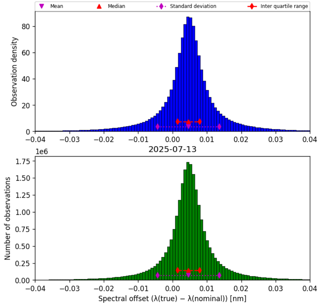
Figure 43: Histogram of “Spectral offset ( \lambda_{\text{true}} - \lambda_{\text{nominal}} )” for 2025-07-13 to 2025-07-14
