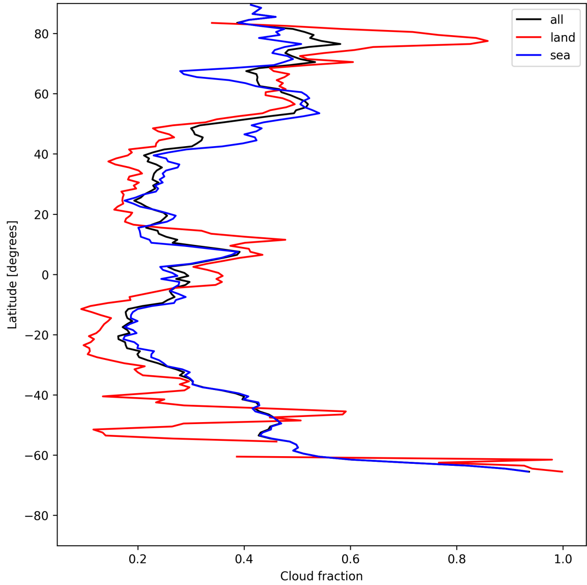
Figure 13: Zonal average of “Cloud fraction” for 2025-07-13 to 2025-07-14.
