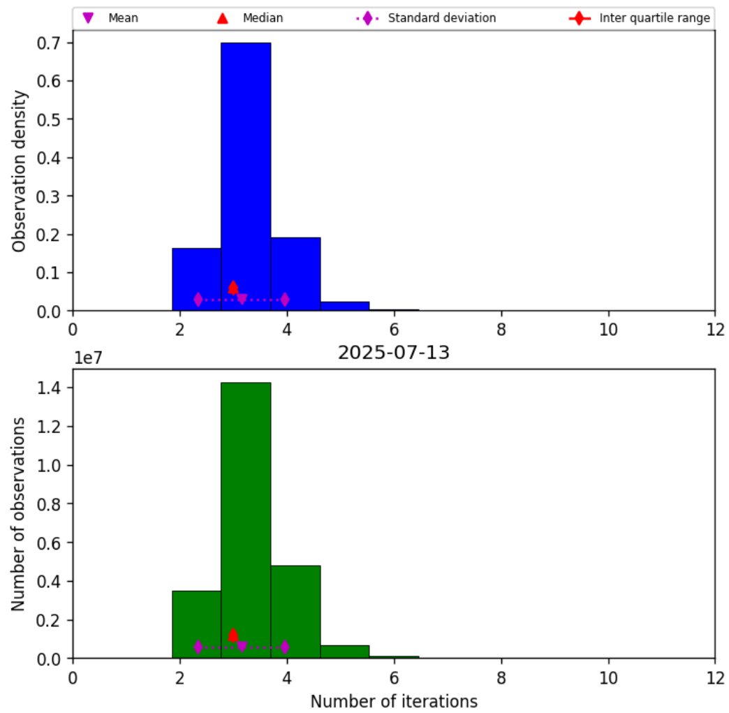
Figure 37: Histogram of “Number of iterations” for 2025-07-13 to 2025-07-14
