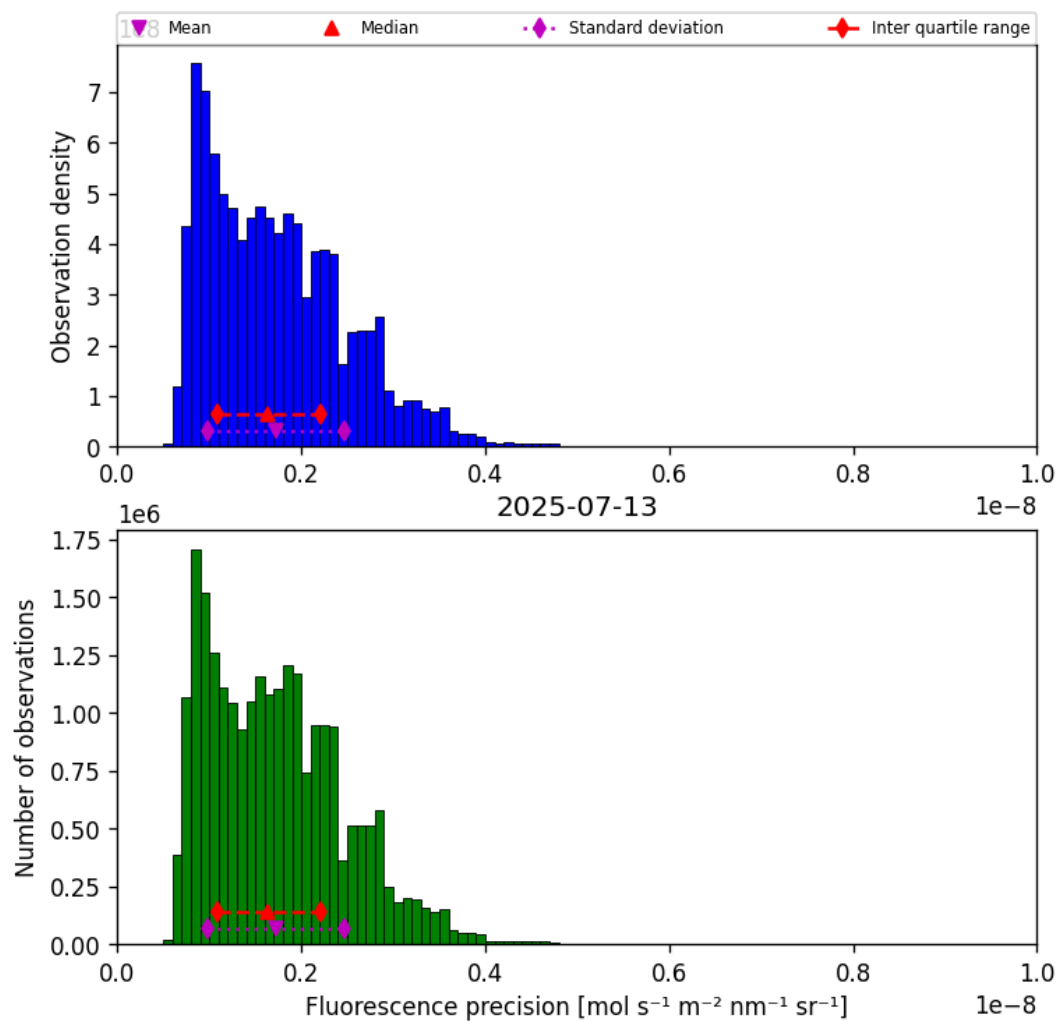
Figure 39: Histogram of “Fluorescence precision” for 2025-07-13 to 2025-07-14
