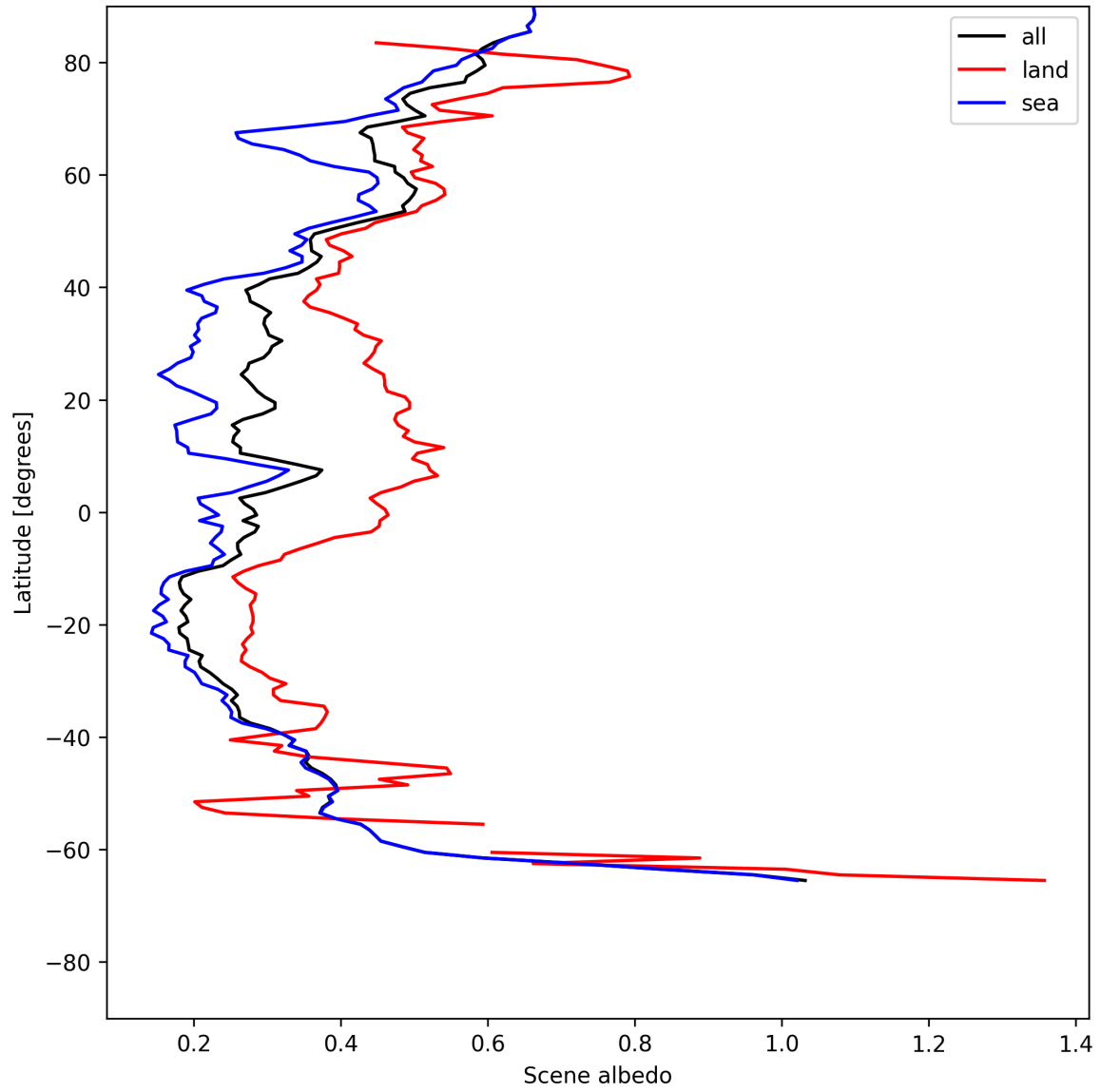
Figure 15: Zonal average of “Scene albedo” for 2025-07-13 to 2025-07-14.
