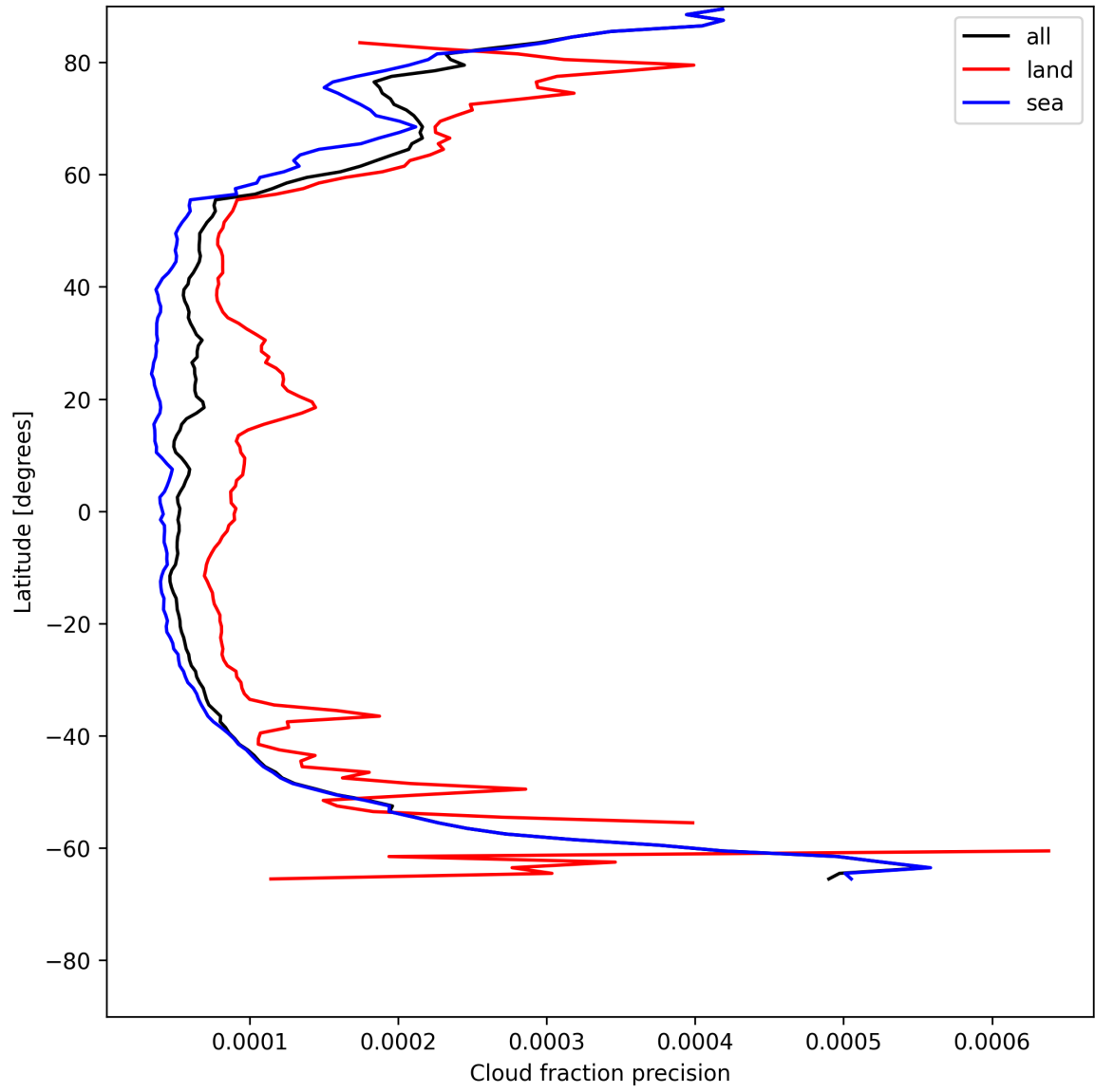
Figure 14: Zonal average of “Cloud fraction precision” for 2025-07-13 to 2025-07-14.
