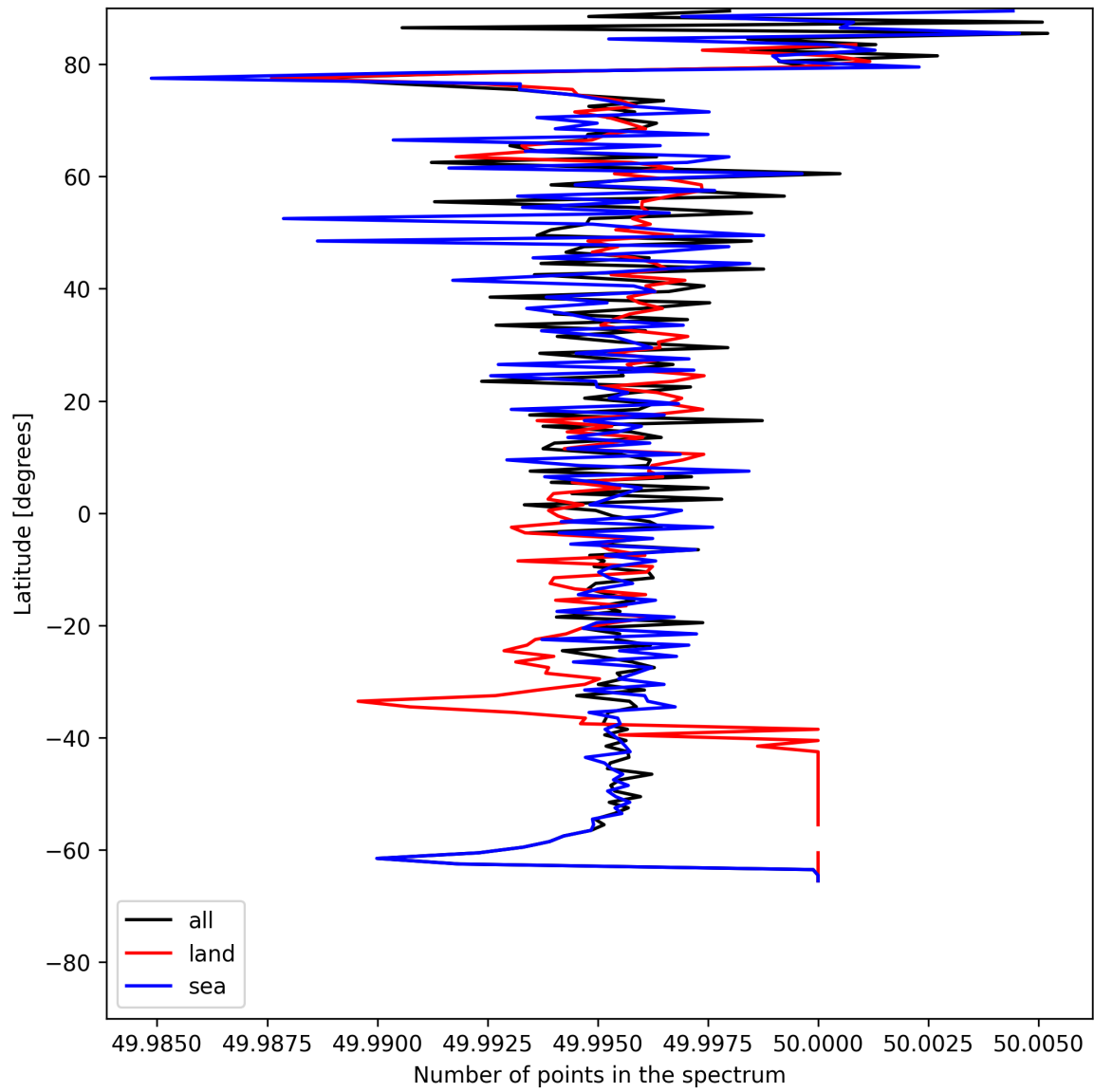
Figure 25: Zonal average of “Number of points in the spectrum” for 2025-07-13 to 2025-07-14.
