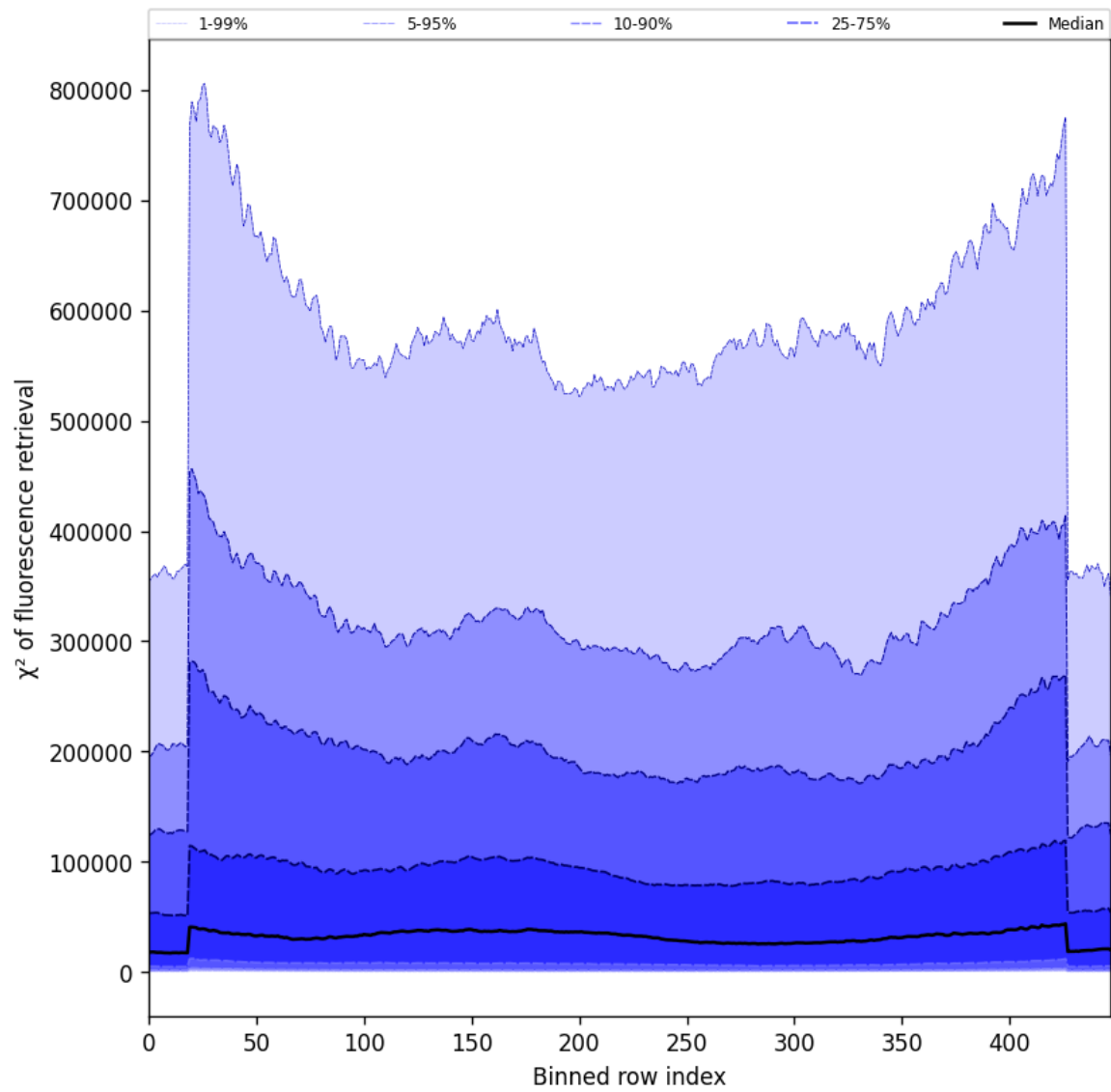
Figure 57: Along track statistics of “ \chi^2 of fluorescence retrieval” for 2025-07-13 to 2025-07-14
