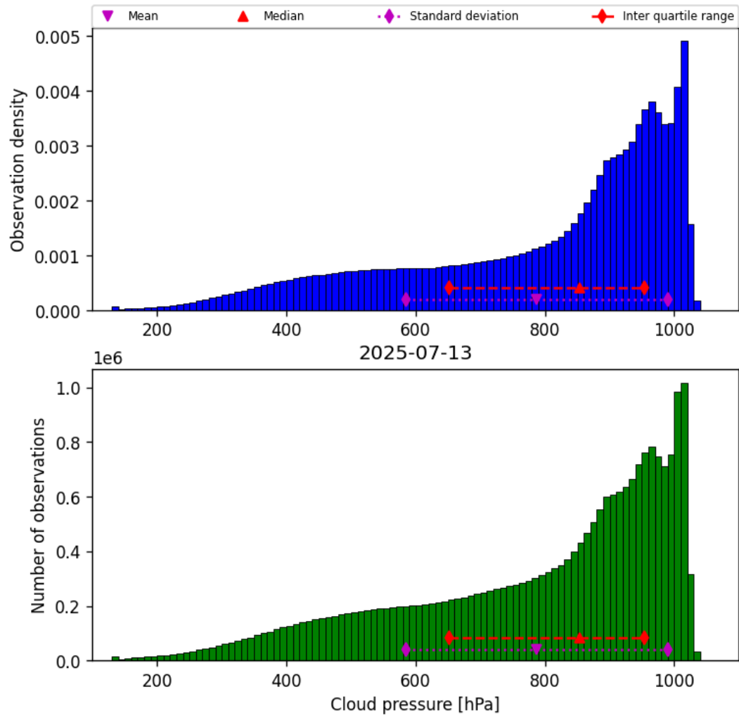
Figure 28: Histogram of “Cloud pressure” for 2025-07-13 to 2025-07-14
