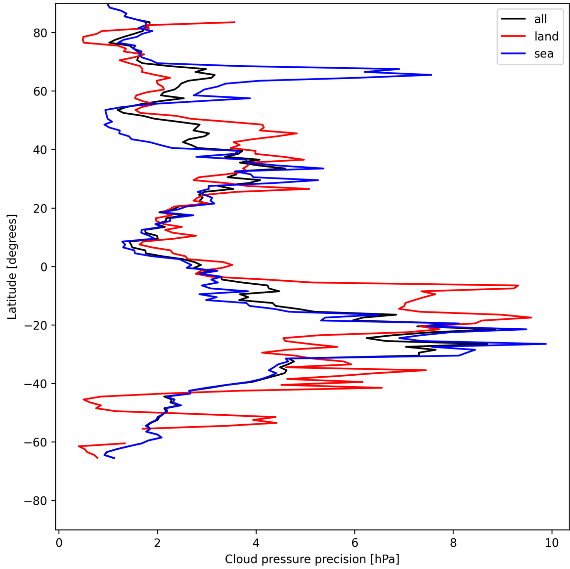
Figure 12: Zonal average of “Cloud pressure precision” for 2025-07-13 to 2025-07-14.
