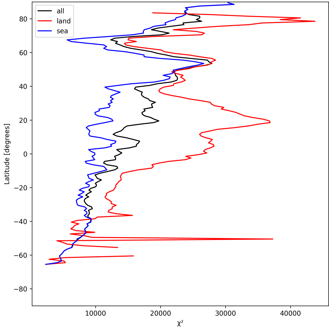
Figure 19: Zonal average of “ \chi^2 ” for 2025-07-13 to 2025-07-14.
