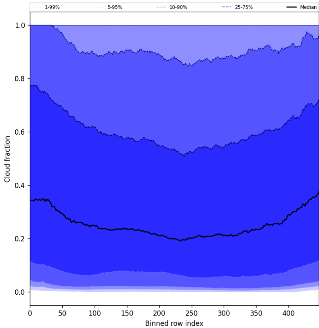
Figure 47: Along track statistics of “Cloud fraction” for 2025-07-13 to 2025-07-14
