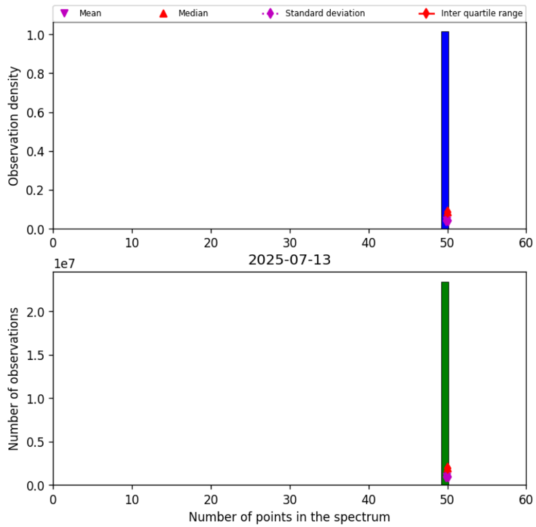
Figure 42: Histogram of “Number of points in the spectrum” for 2025-07-13 to 2025-07-14
