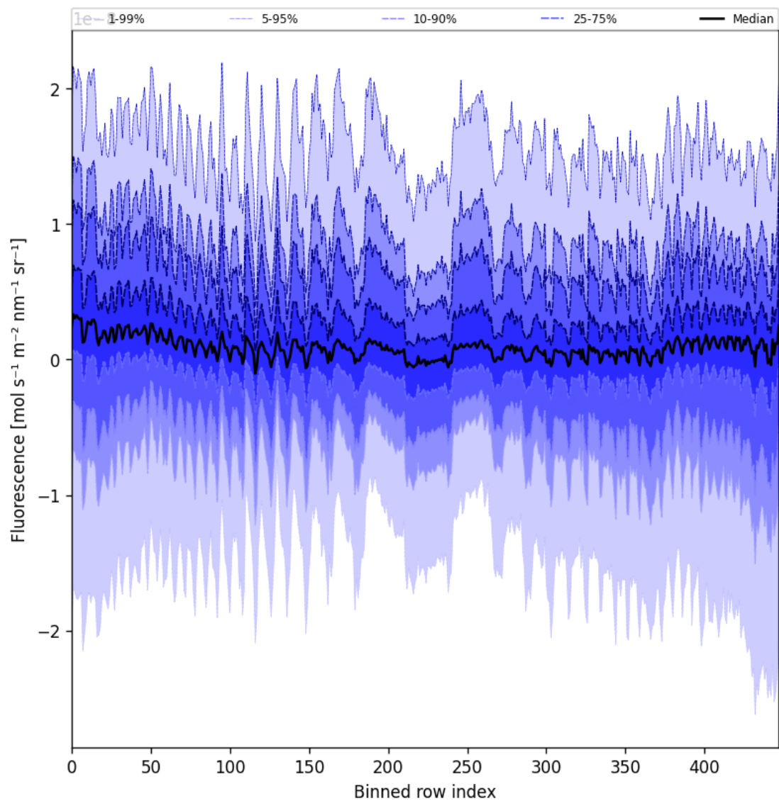
Figure 55: Along track statistics of "Fluorescence" for 2025-07-13 to 2025-07-14
