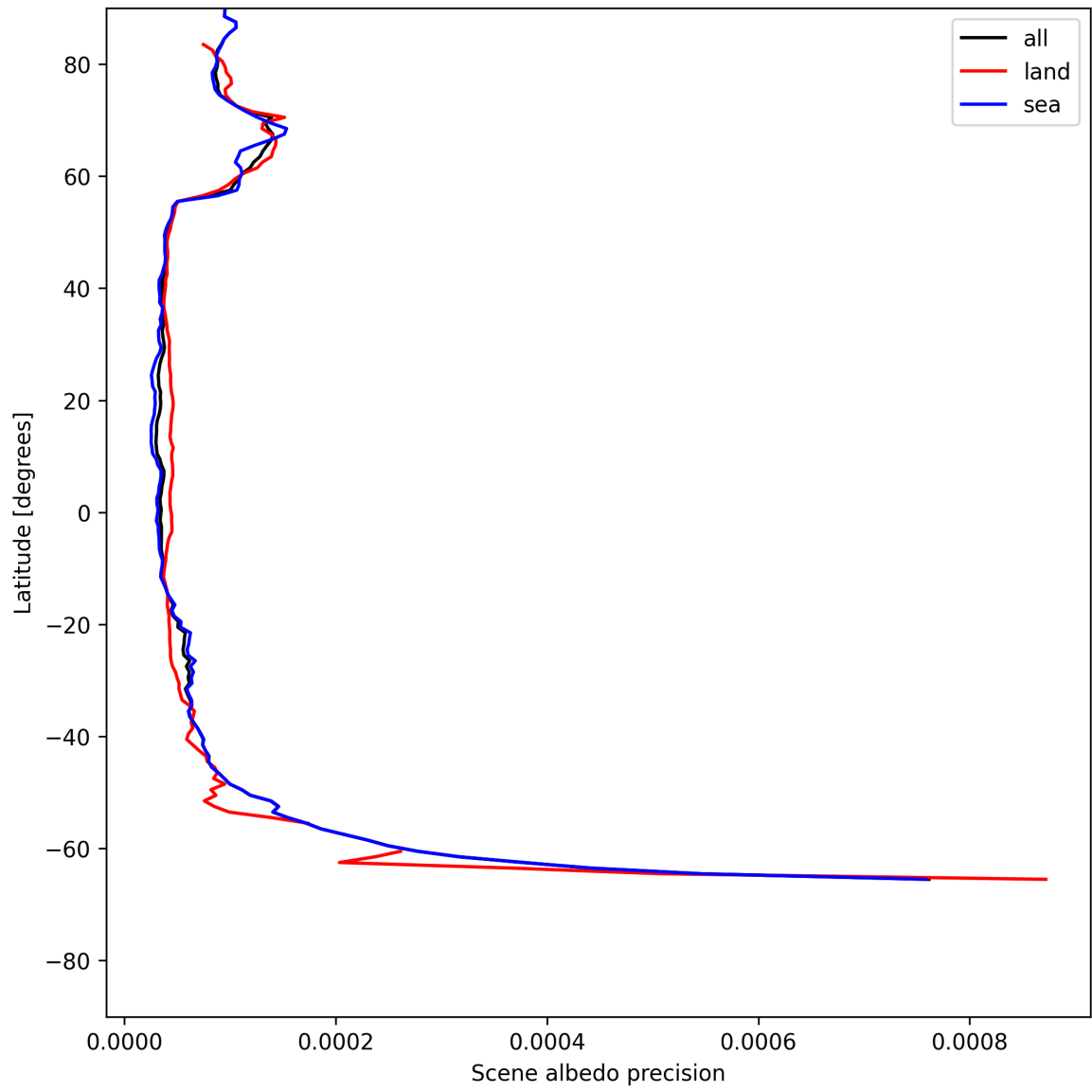
Figure 16: Zonal average of “Scene albedo precision” for 2025-07-13 to 2025-07-14.
