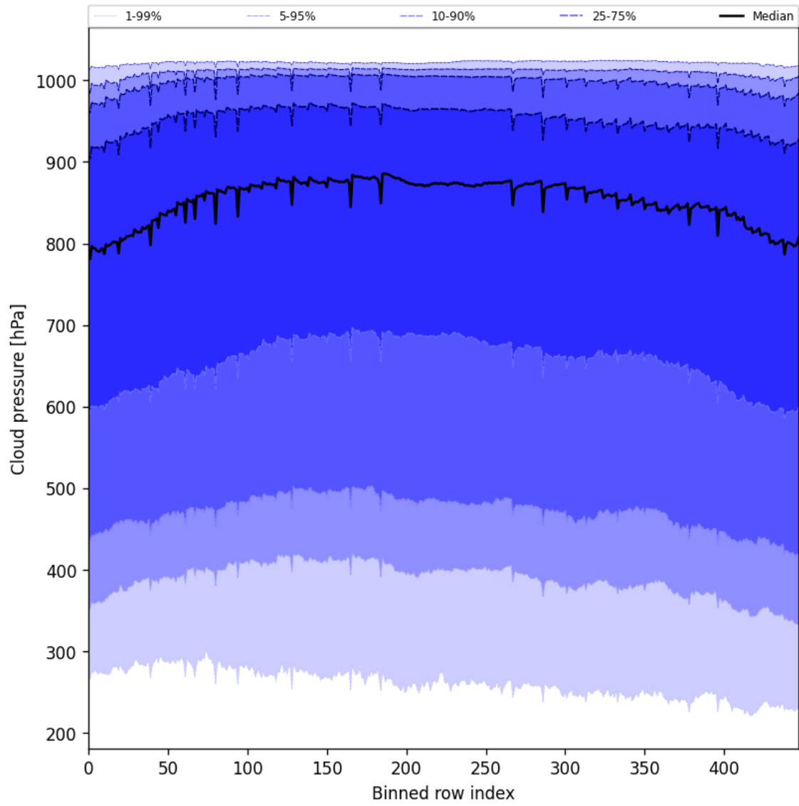
Figure 45: Along track statistics of “Cloud pressure” for 2025-07-13 to 2025-07-14
