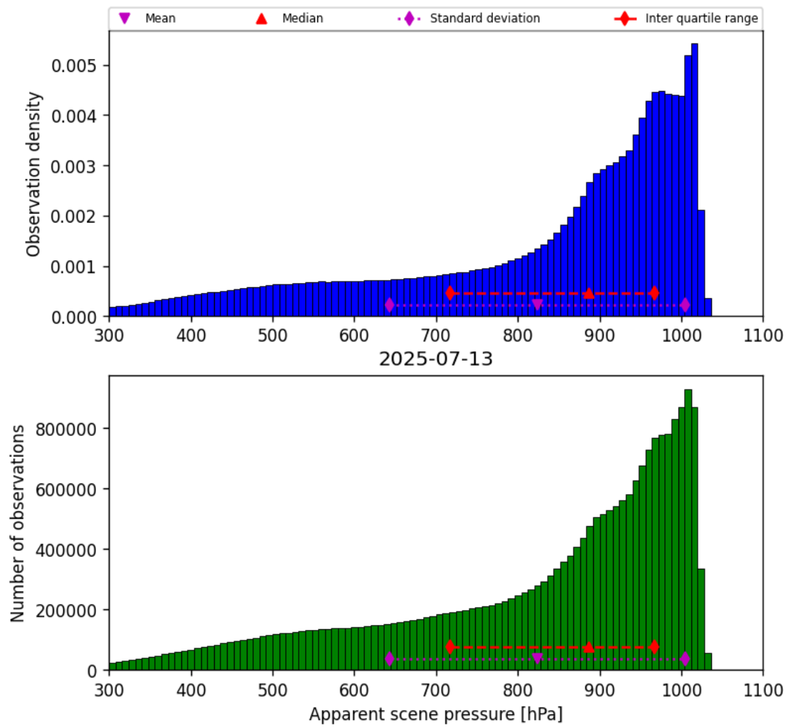
Figure 34: Histogram of “Apparent scene pressure” for 2025-07-13 to 2025-07-14
