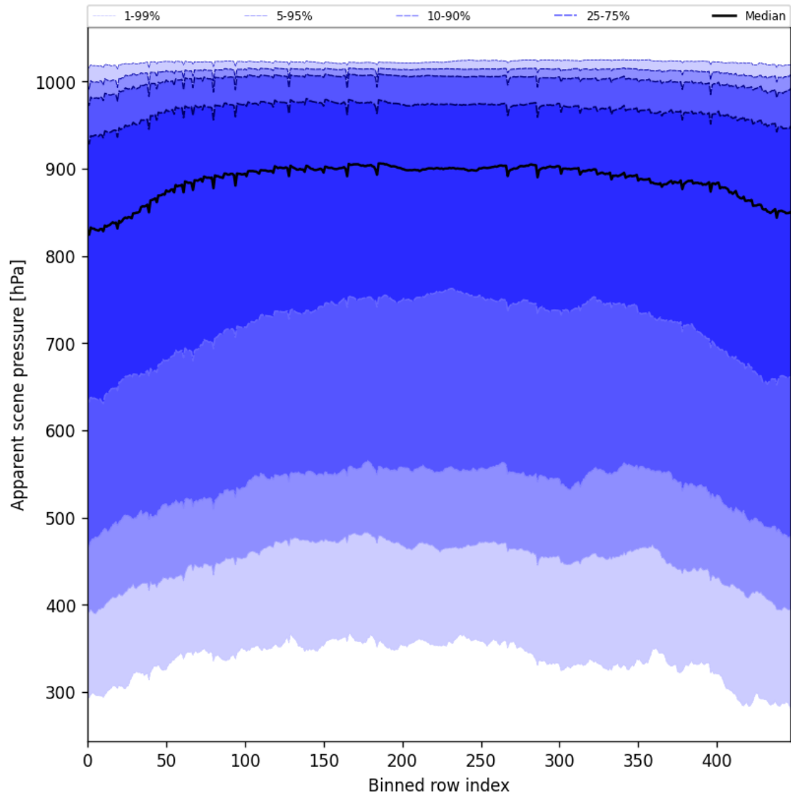
Figure 51: Along track statistics of “Apparent scene pressure” for 2025-07-13 to 2025-07-14
