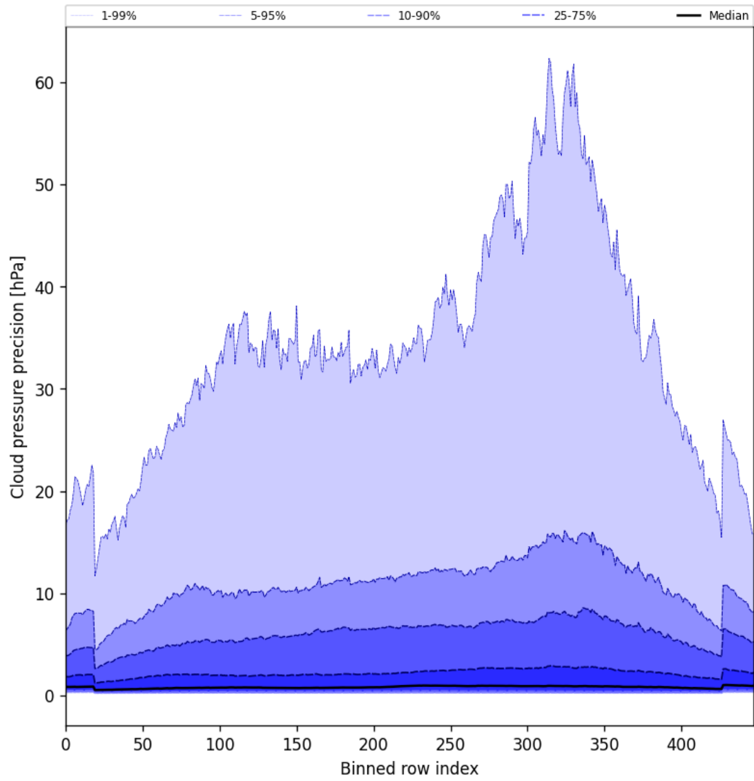
Figure 46: Along track statistics of “Cloud pressure precision” for 2025-07-13 to 2025-07-14
