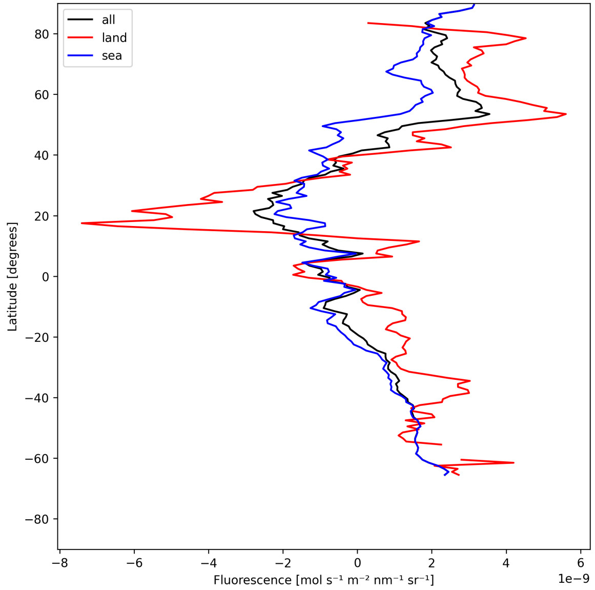
Figure 21: Zonal average of “Fluorescence” for 2025-07-13 to 2025-07-14.
