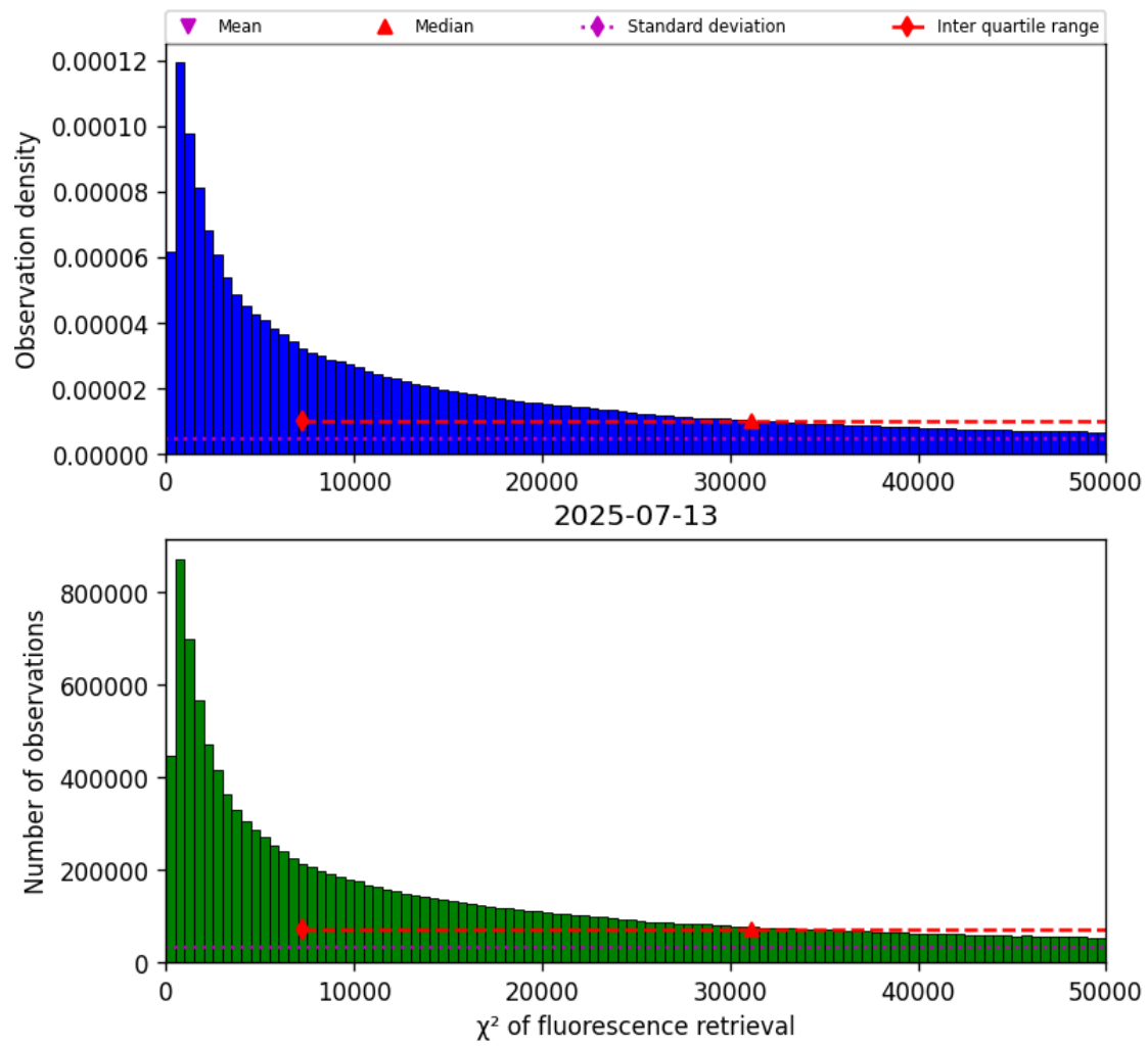
Figure 40: Histogram of “ \chi^2 of fluorescence retrieval” for 2025-07-13 to 2025-07-14
