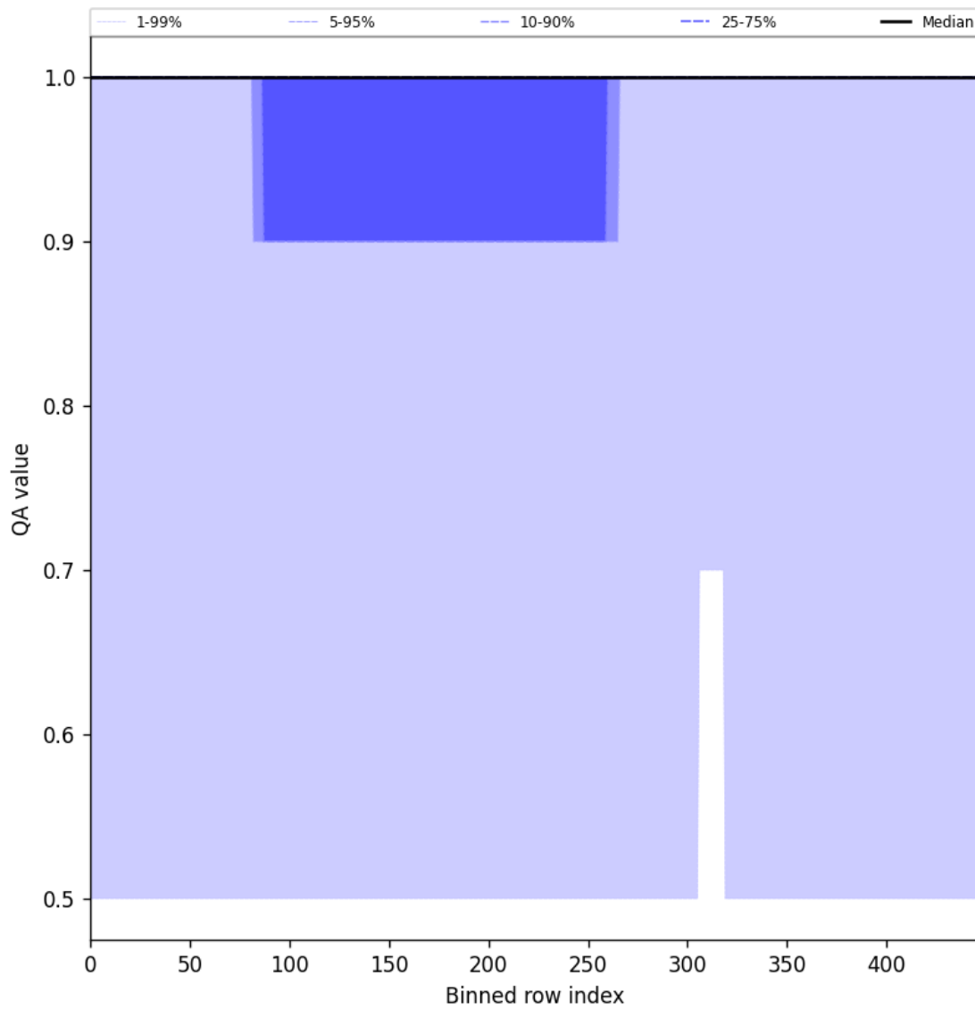
Figure 44: Along track statistics of “QA value” for 2025-07-13 to 2025-07-14
