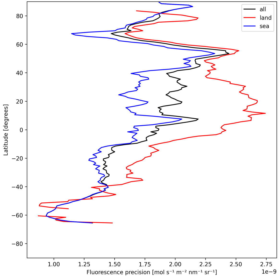
Figure 22: Zonal average of “Fluorescence precision” for 2025-07-13 to 2025-07-14.
