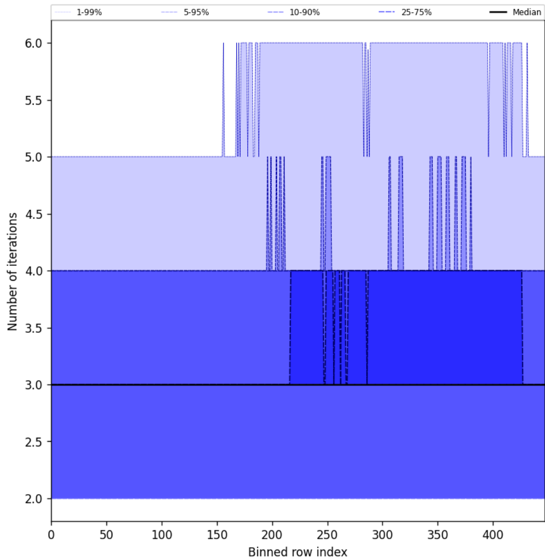
Figure 54: Along track statistics of “Number of iterations” for 2025-07-13 to 2025-07-14
