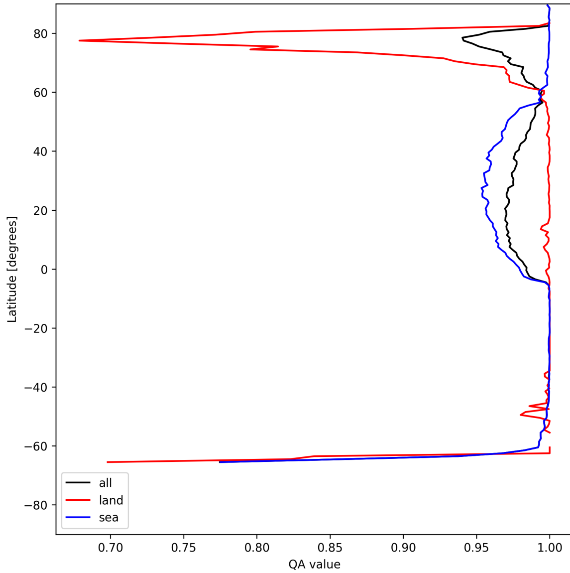
Figure 10: Zonal average of “QA value” for 2025-07-13 to 2025-07-14.
