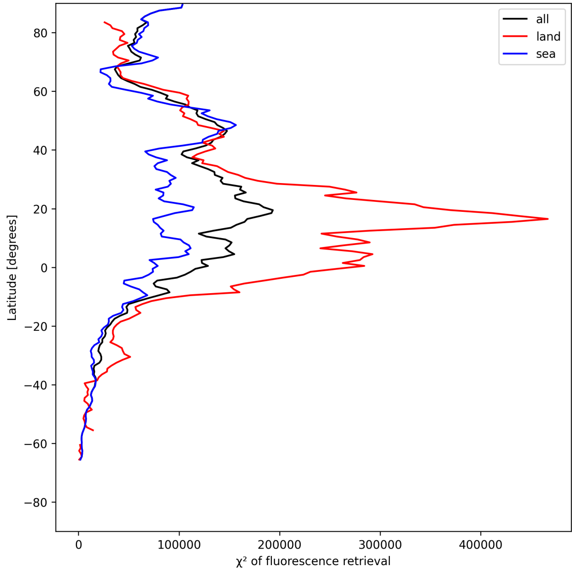
Figure 23: Zonal average of “ \chi^2 of fluorescence retrieval” for 2025-07-13 to 2025-07-14.
