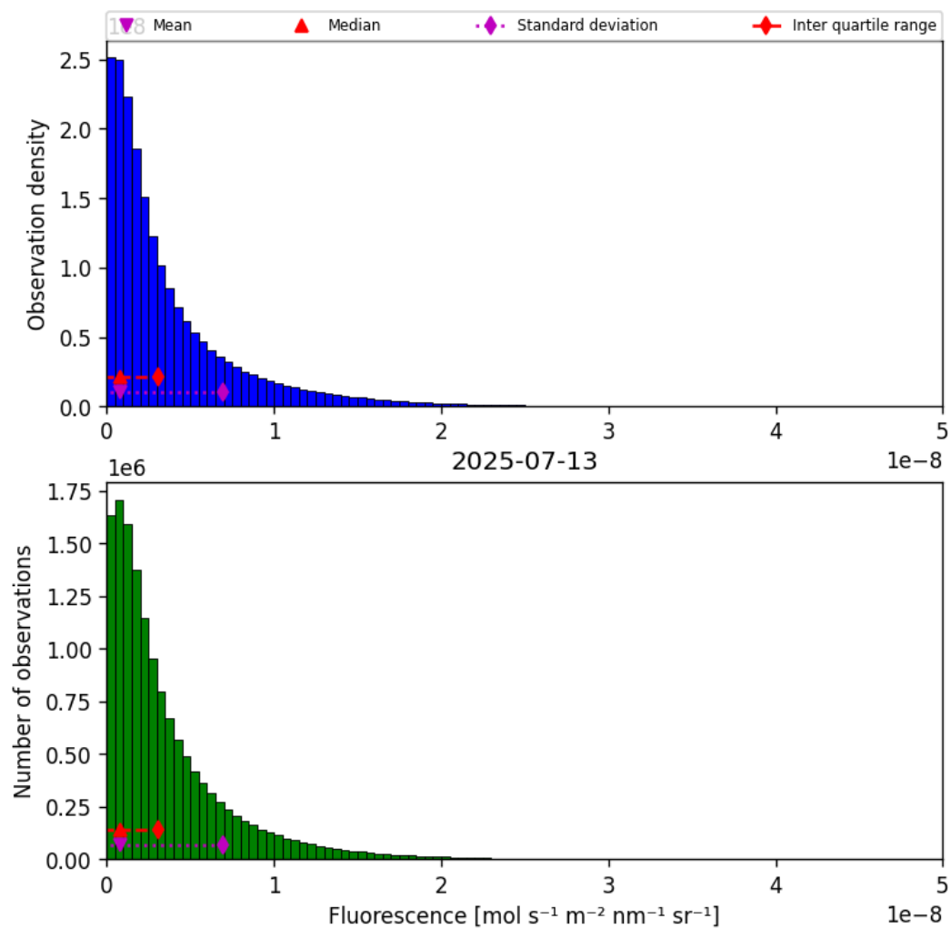
Figure 38: Histogram of “Fluorescence” for 2025-07-13 to 2025-07-14
