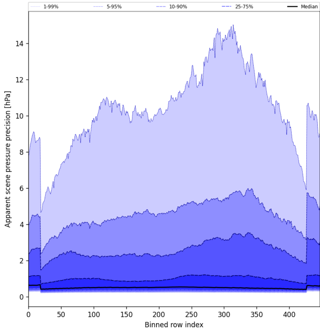
Figure 52: Along track statistics of “Apparent scene pressure precision” for 2025-07-13 to 2025-07-14
