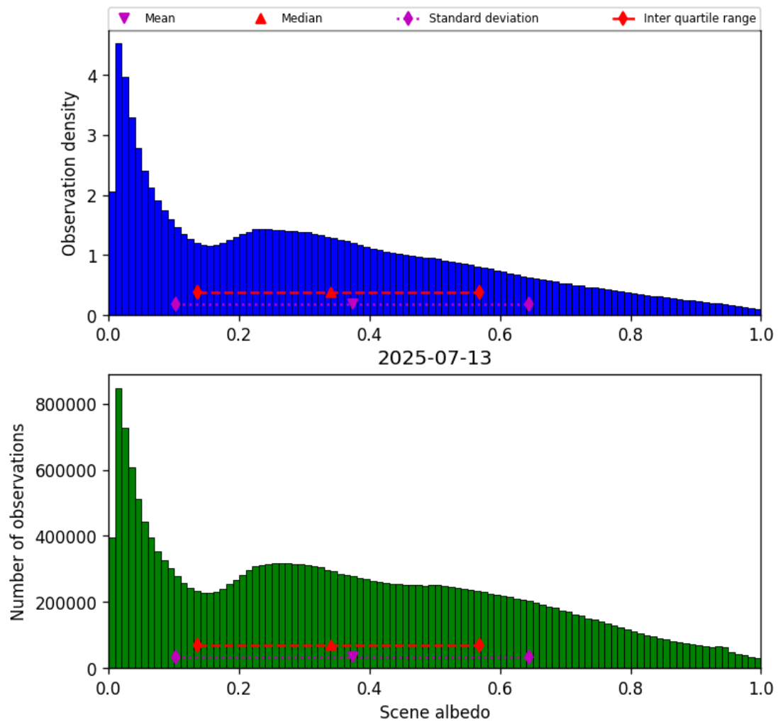
Figure 32: Histogram of “Scene albedo” for 2025-07-13 to 2025-07-14
