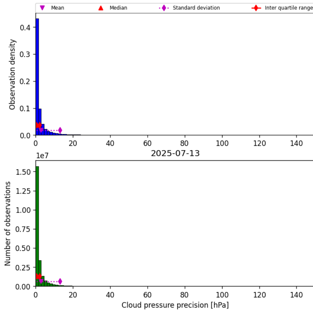
Figure 29: Histogram of “Cloud pressure precision” for 2025-07-13 to 2025-07-14
