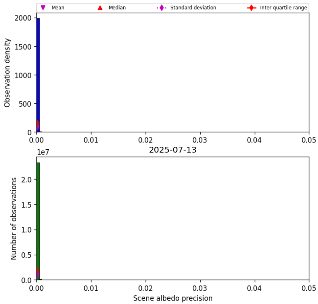
Figure 33: Histogram of “Scene albedo precision” for 2025-07-13 to 2025-07-14
