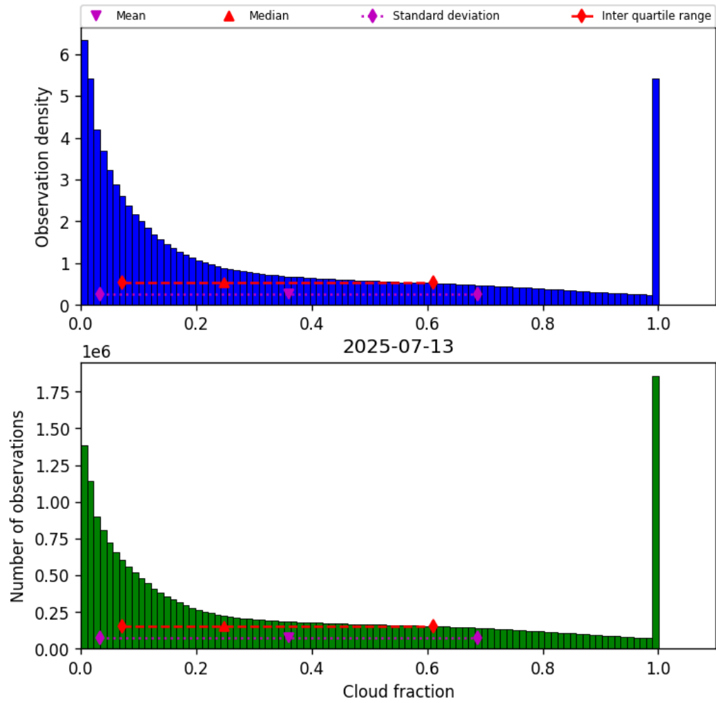
Figure 30: Histogram of “Cloud fraction” for 2025-07-13 to 2025-07-14
