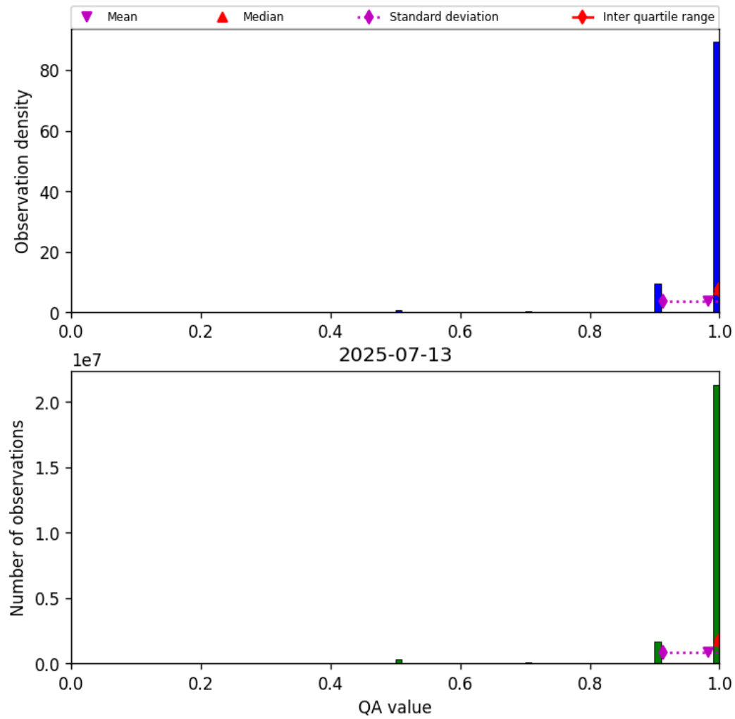
Figure 27: Histogram of “QA value” for 2025-07-13 to 2025-07-14
