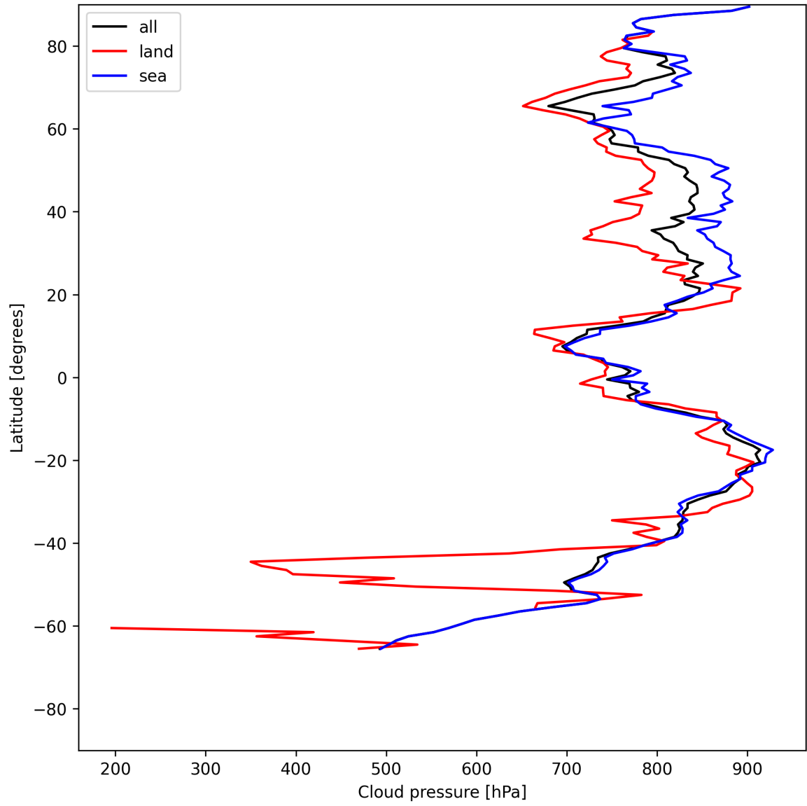
Figure 11: Zonal average of “Cloud pressure” for 2025-07-13 to 2025-07-14.
