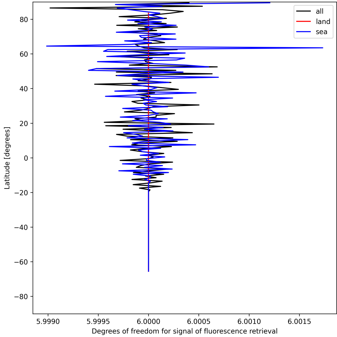
Figure 24: Zonal average of “Degrees of freedom for signal of fluorescence retrieval” for 2025-07-13 to 2025-07-14.
