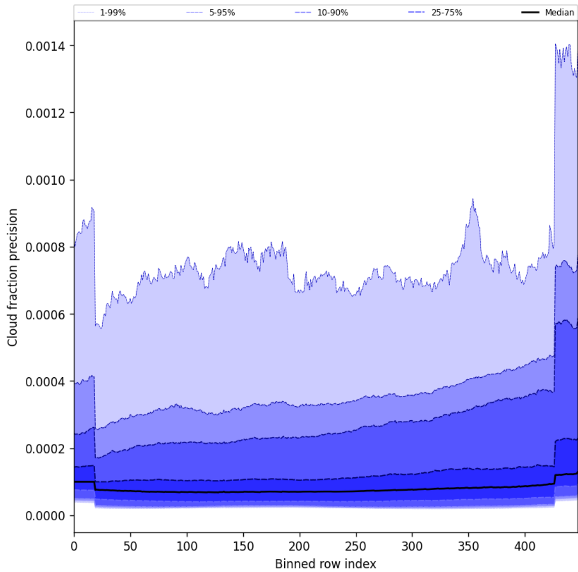
Figure 48: Along track statistics of “Cloud fraction precision” for 2025-07-13 to 2025-07-14
