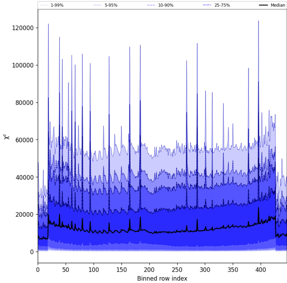
Figure 53: Along track statistics of “ \chi^2 ” for 2025-07-13 to 2025-07-14
