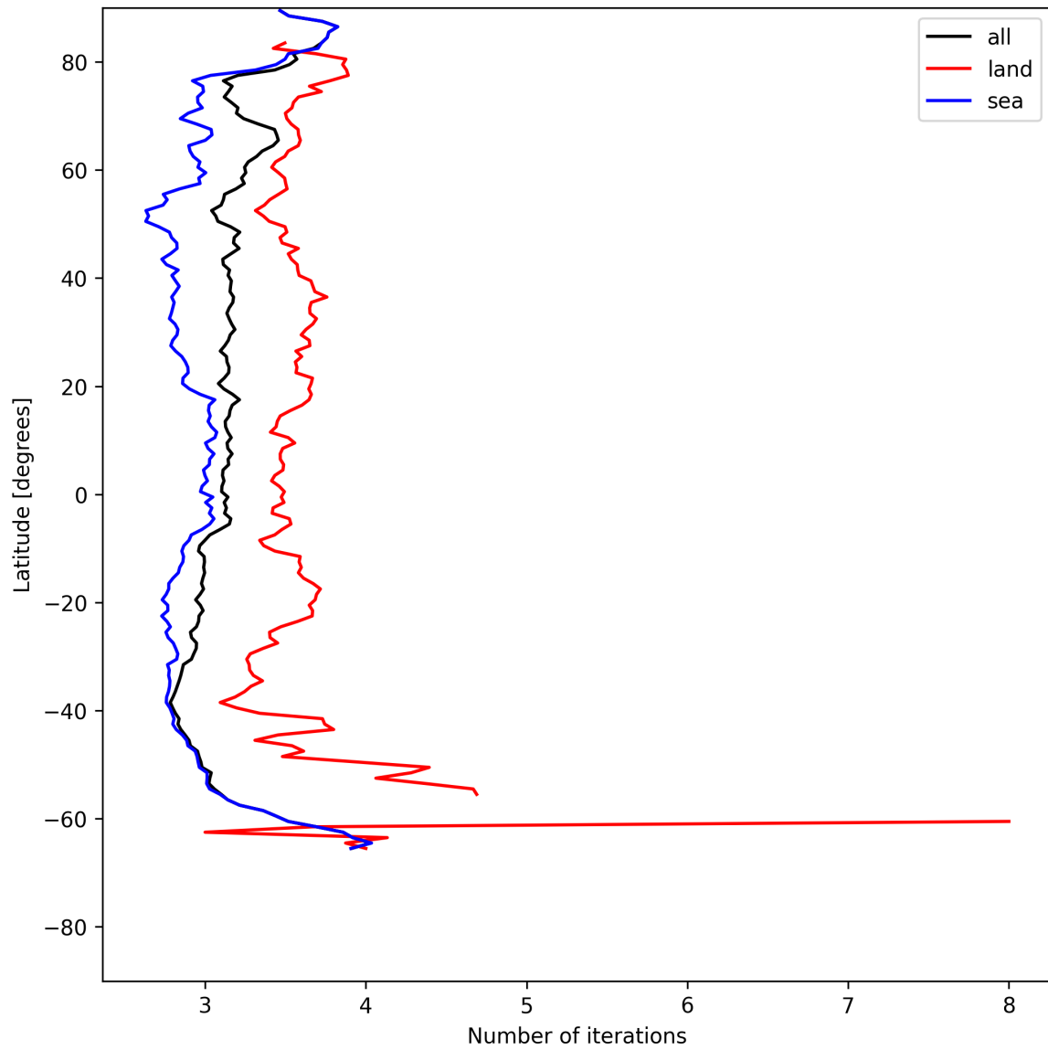
Figure 20: Zonal average of “Number of iterations” for 2025-07-13 to 2025-07-14.
