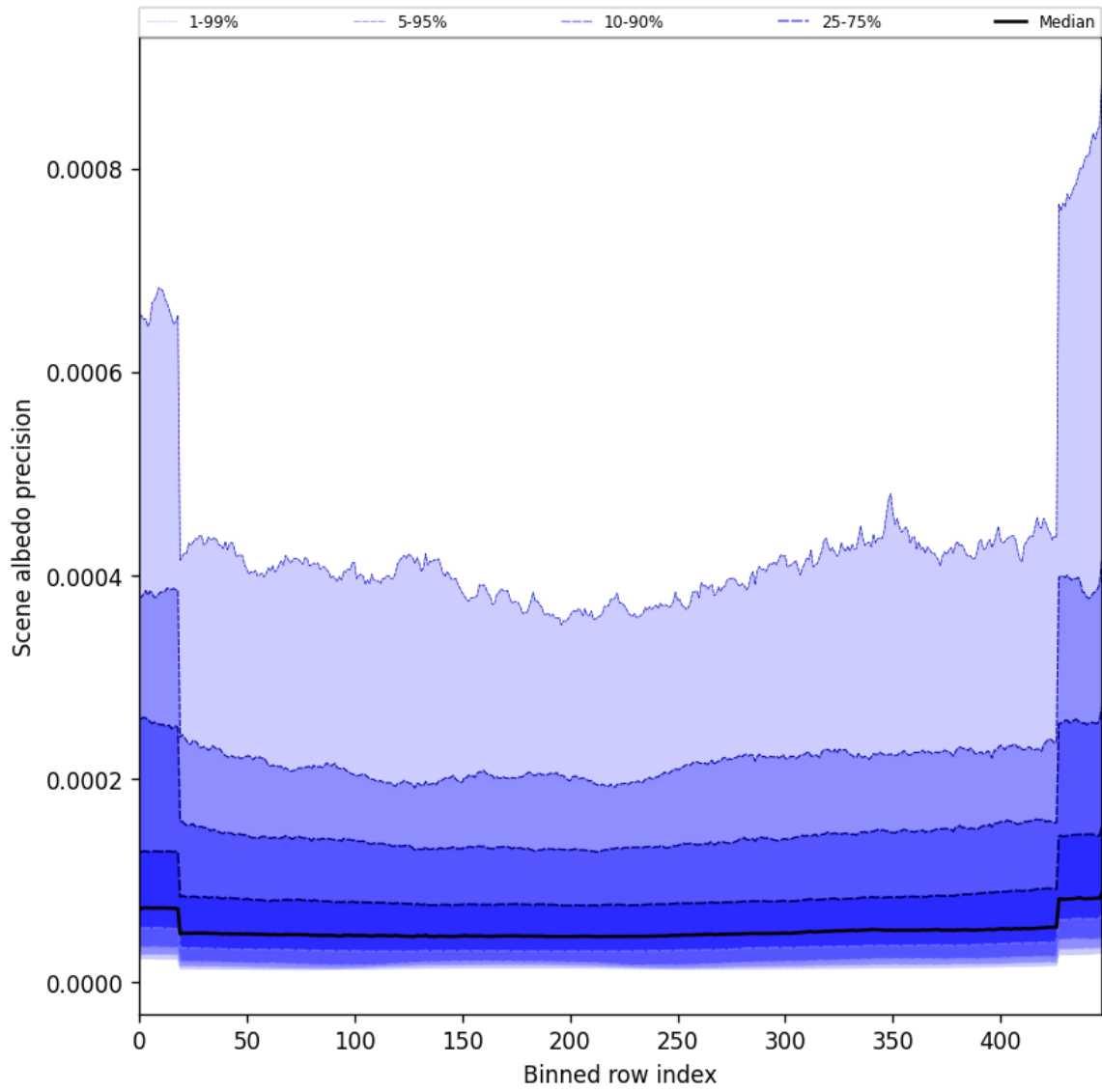
Figure 50: Along track statistics of “Scene albedo precision” for 2025-07-13 to 2025-07-14
