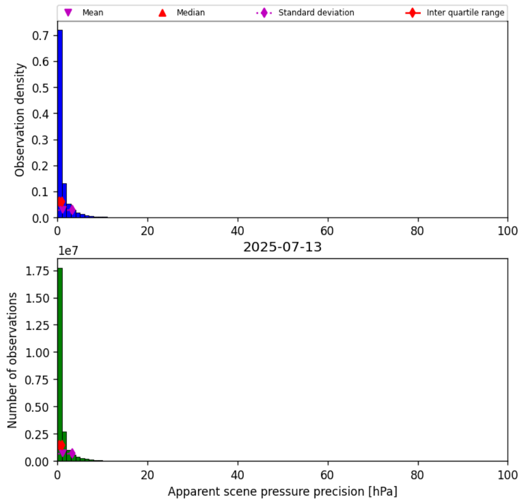
Figure 35: Histogram of “Apparent scene pressure precision” for 2025-07-13 to 2025-07-14
