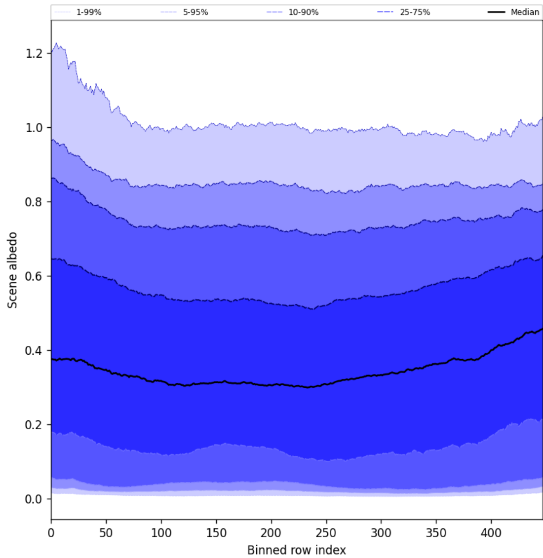
Figure 49: Along track statistics of “Scene albedo” for 2025-07-13 to 2025-07-14
