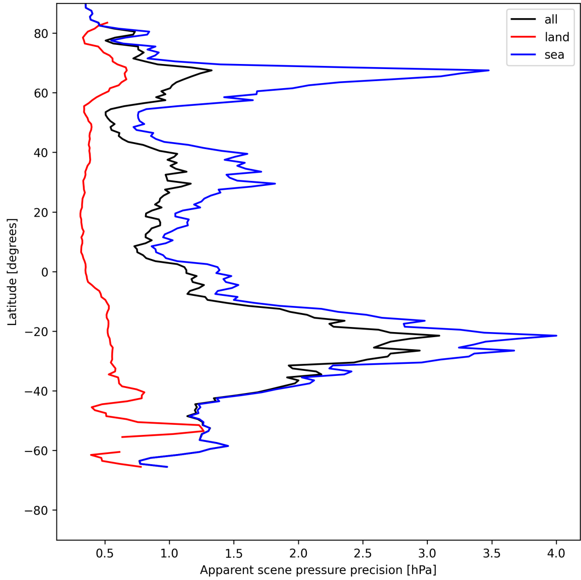
Figure 18: Zonal average of “Apparent scene pressure precision” for 2025-07-13 to 2025-07-14.
