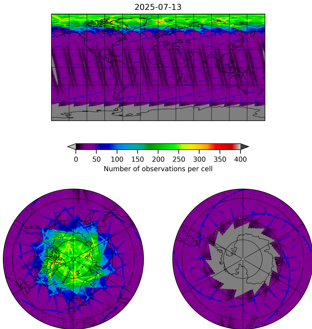
Figure 9: Map of the number of observations for 2025-07-13 to 2025-07-14
