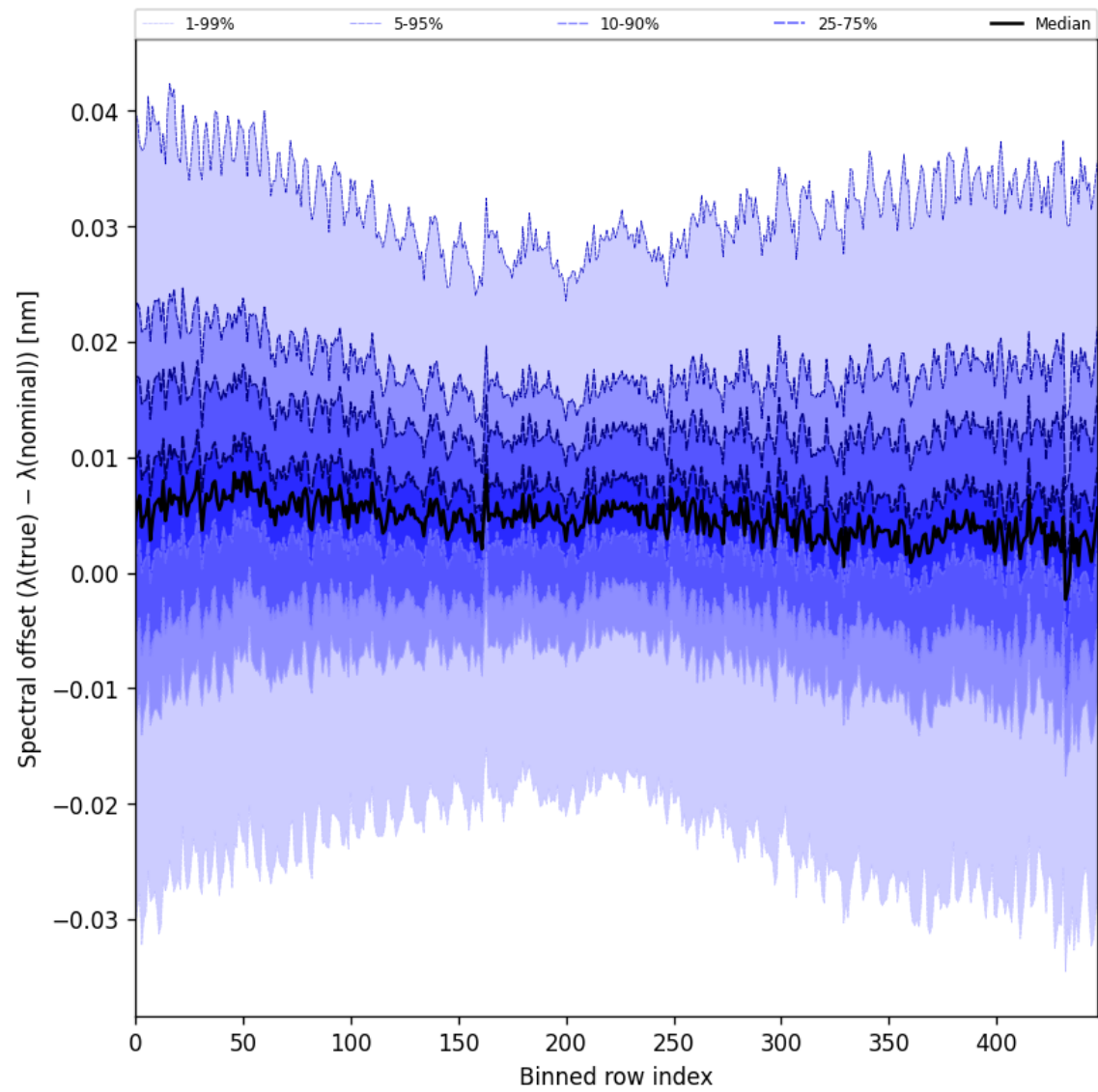
Figure 60: Along track statistics of “Spectral offset ( \lambda_{\text{true}} - \lambda_{\text{nominal}} )” for 2025-07-13 to 2025-07-14
