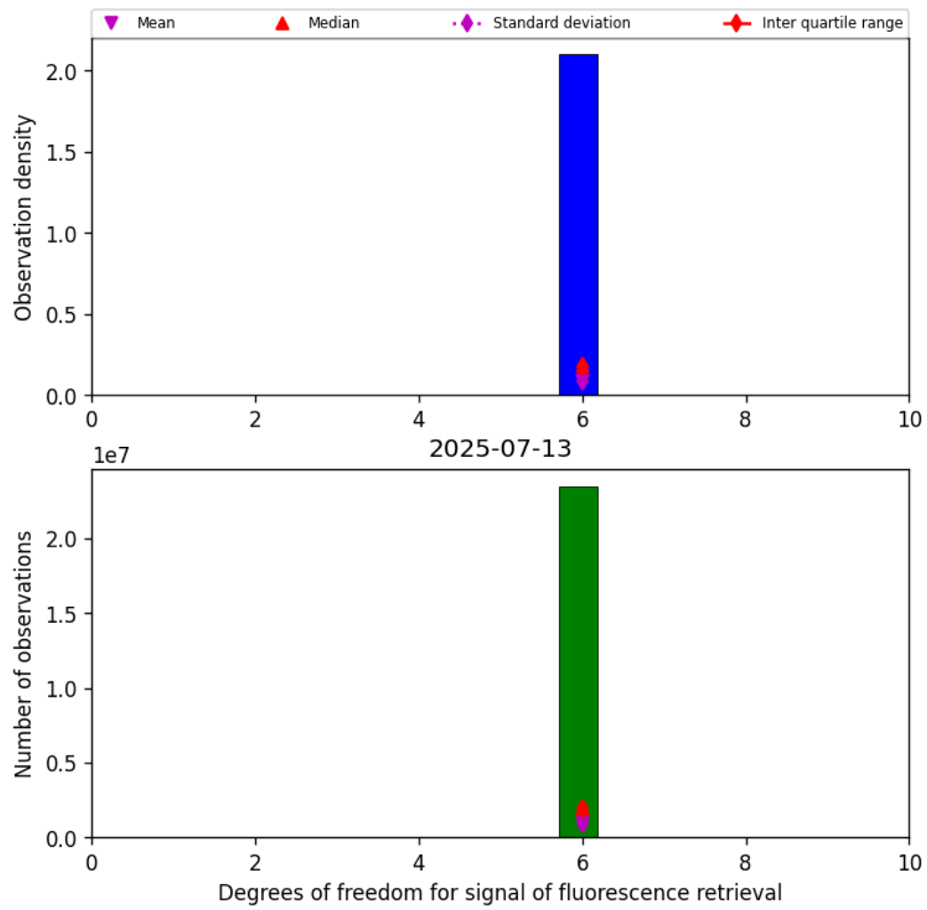
Figure 41: Histogram of “Degrees of freedom for signal of fluorescence retrieval” for 2025-07-13 to 2025-07-14
