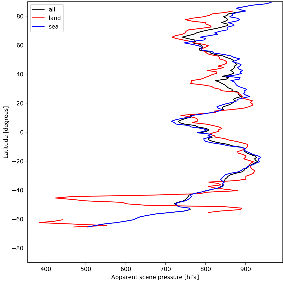
Figure 17: Zonal average of “Apparent scene pressure” for 2025-07-13 to 2025-07-14.
