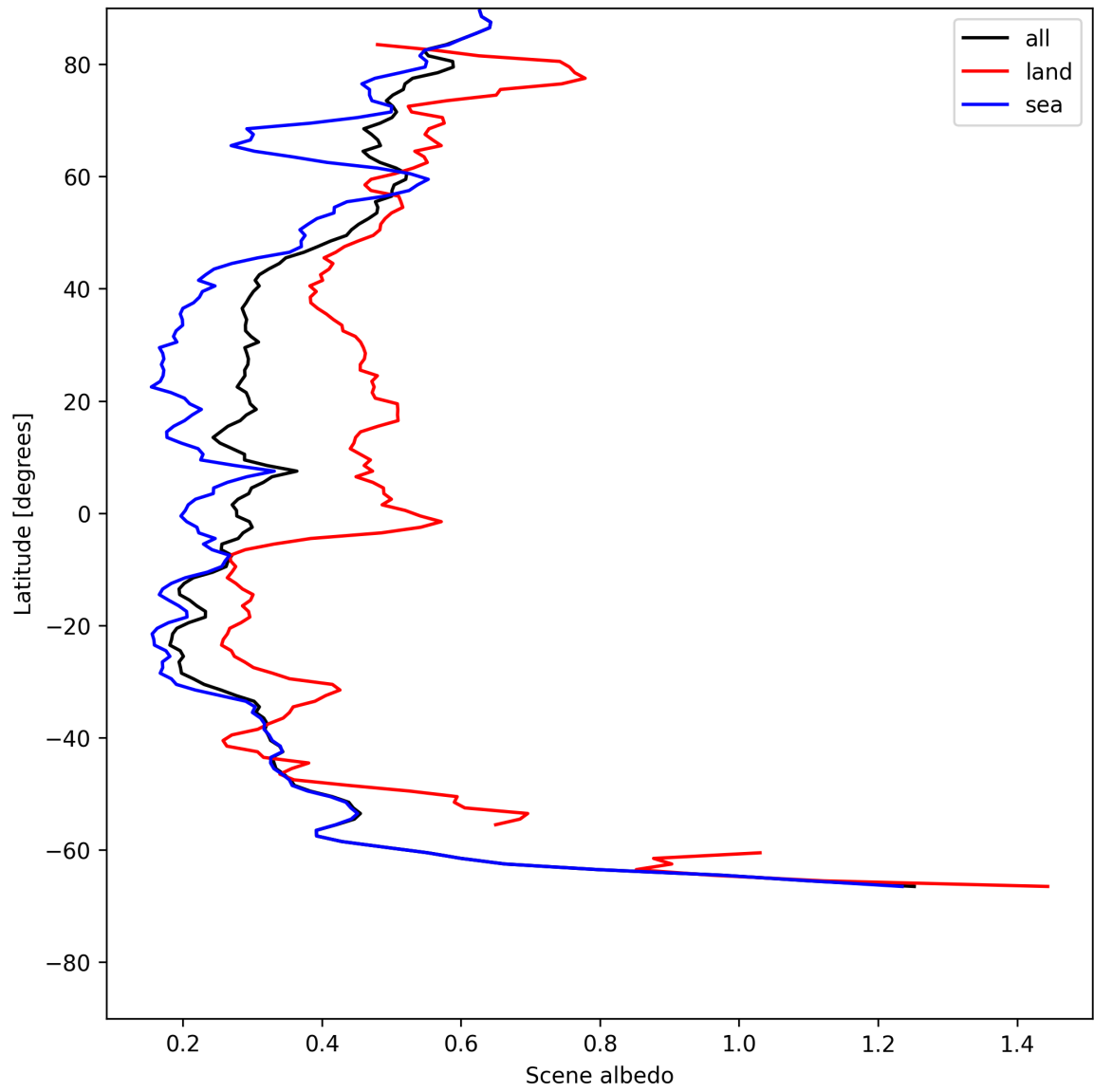
Figure 15: Zonal average of "Scene albedo" for 2025-07-14 to 2025-07-15.
