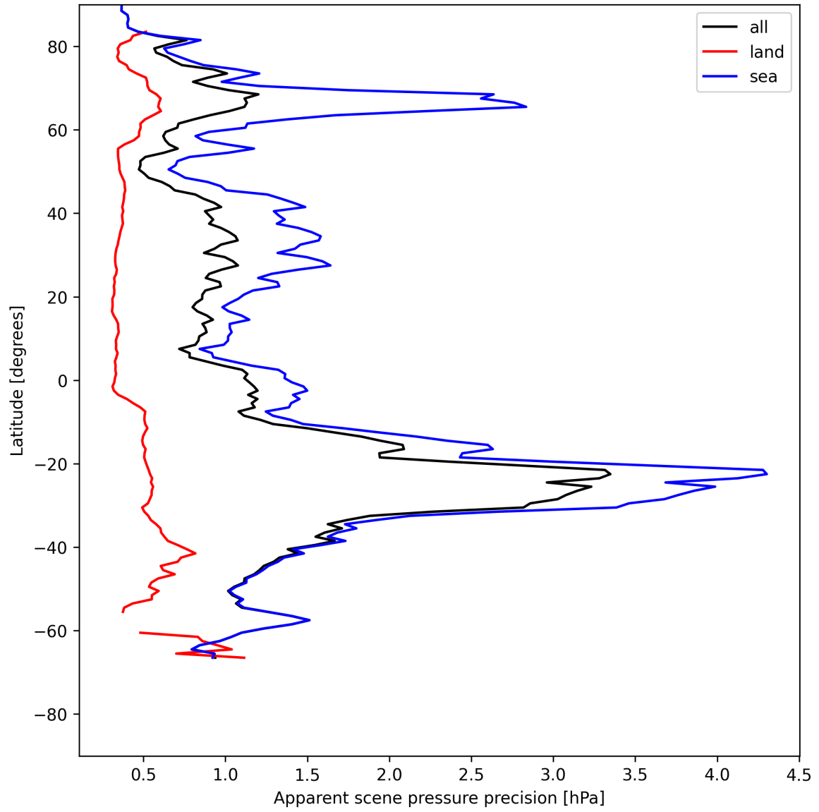
Figure 18: Zonal average of “Apparent scene pressure precision” for 2025-07-14 to 2025-07-15.
