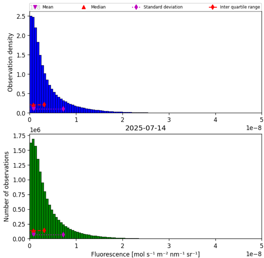
Figure 38: Histogram of “Fluorescence” for 2025-07-14 to 2025-07-15
