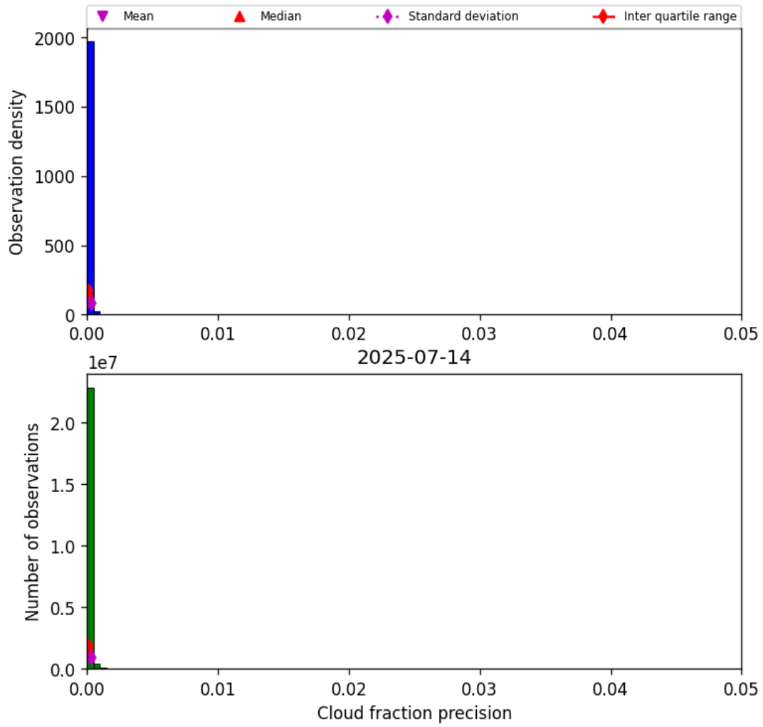
Figure 31: Histogram of “Cloud fraction precision” for 2025-07-14 to 2025-07-15
