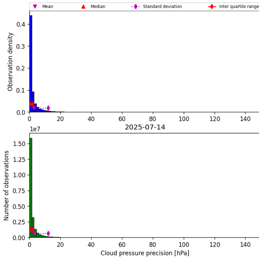
Figure 29: Histogram of “Cloud pressure precision” for 2025-07-14 to 2025-07-15
