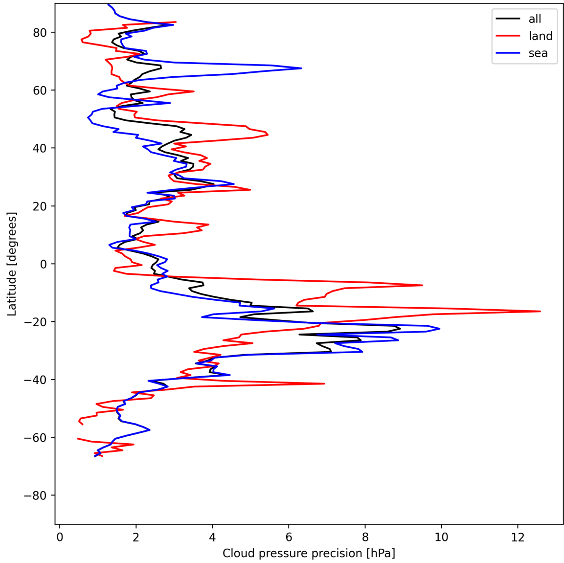
Figure 12: Zonal average of “Cloud pressure precision” for 2025-07-14 to 2025-07-15.
