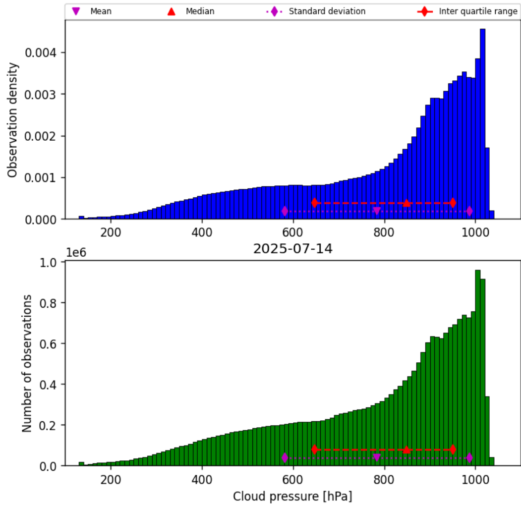
Figure 28: Histogram of “Cloud pressure” for 2025-07-14 to 2025-07-15
