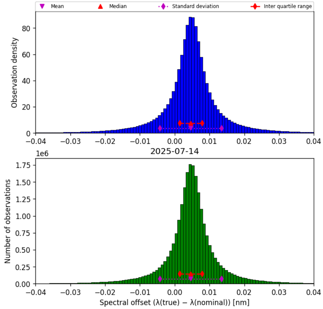
Figure 43: Histogram of “Spectral offset ( \lambda_{\text{true}} - \lambda_{\text{nominal}} )” for 2025-07-14 to 2025-07-15
