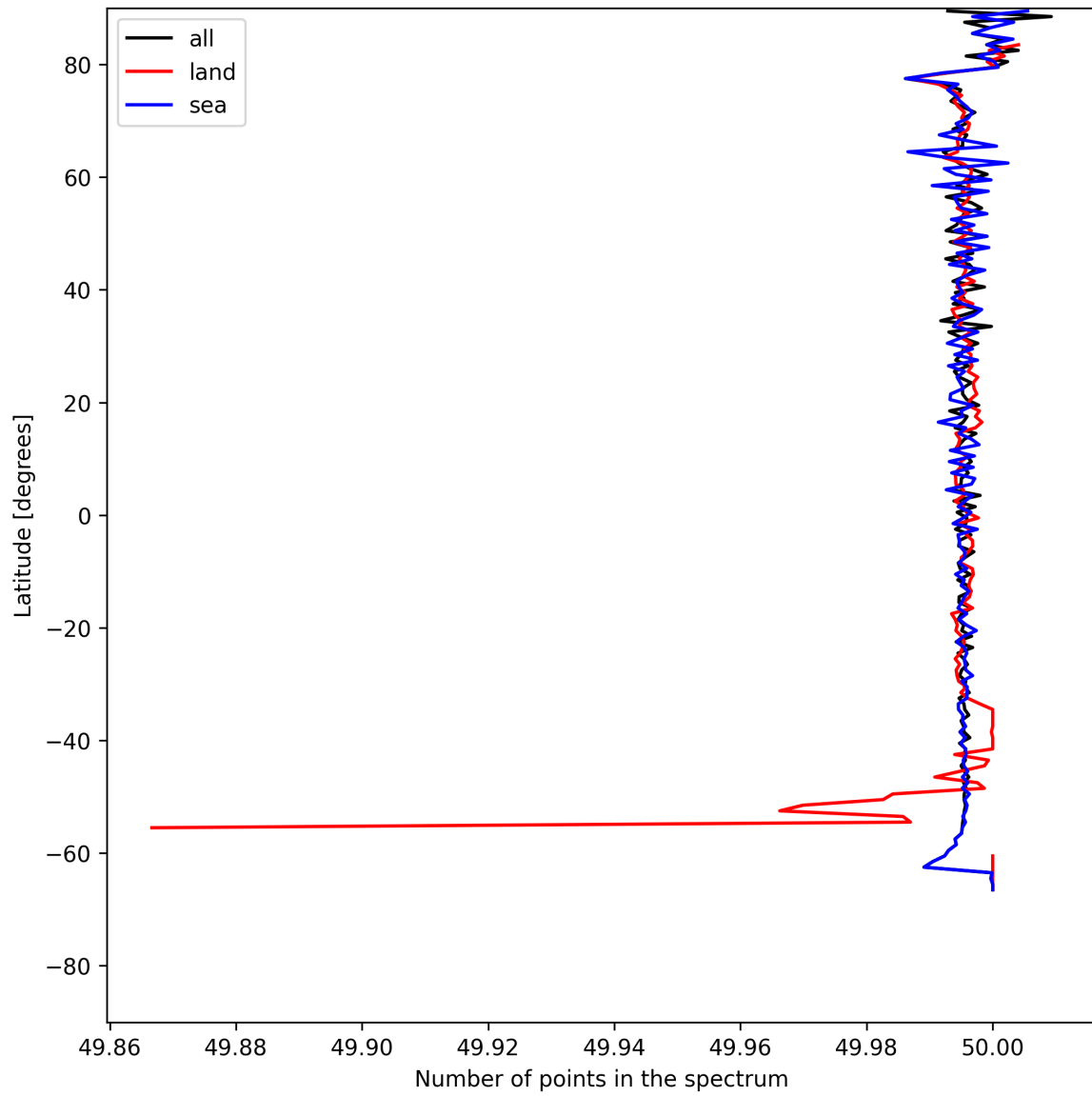
Figure 25: Zonal average of “Number of points in the spectrum” for 2025-07-14 to 2025-07-15.
