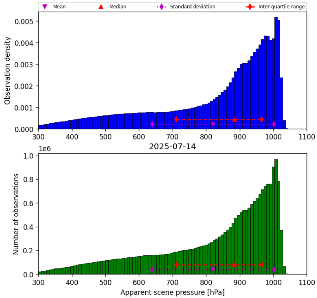
Figure 34: Histogram of “Apparent scene pressure” for 2025-07-14 to 2025-07-15
