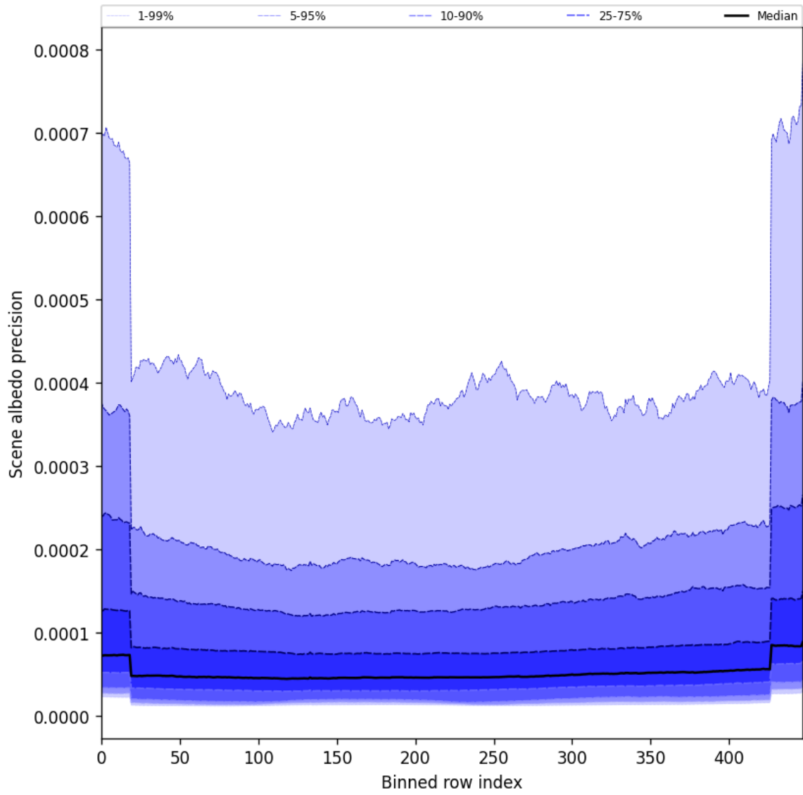
Figure 50: Along track statistics of “Scene albedo precision” for 2025-07-14 to 2025-07-15
