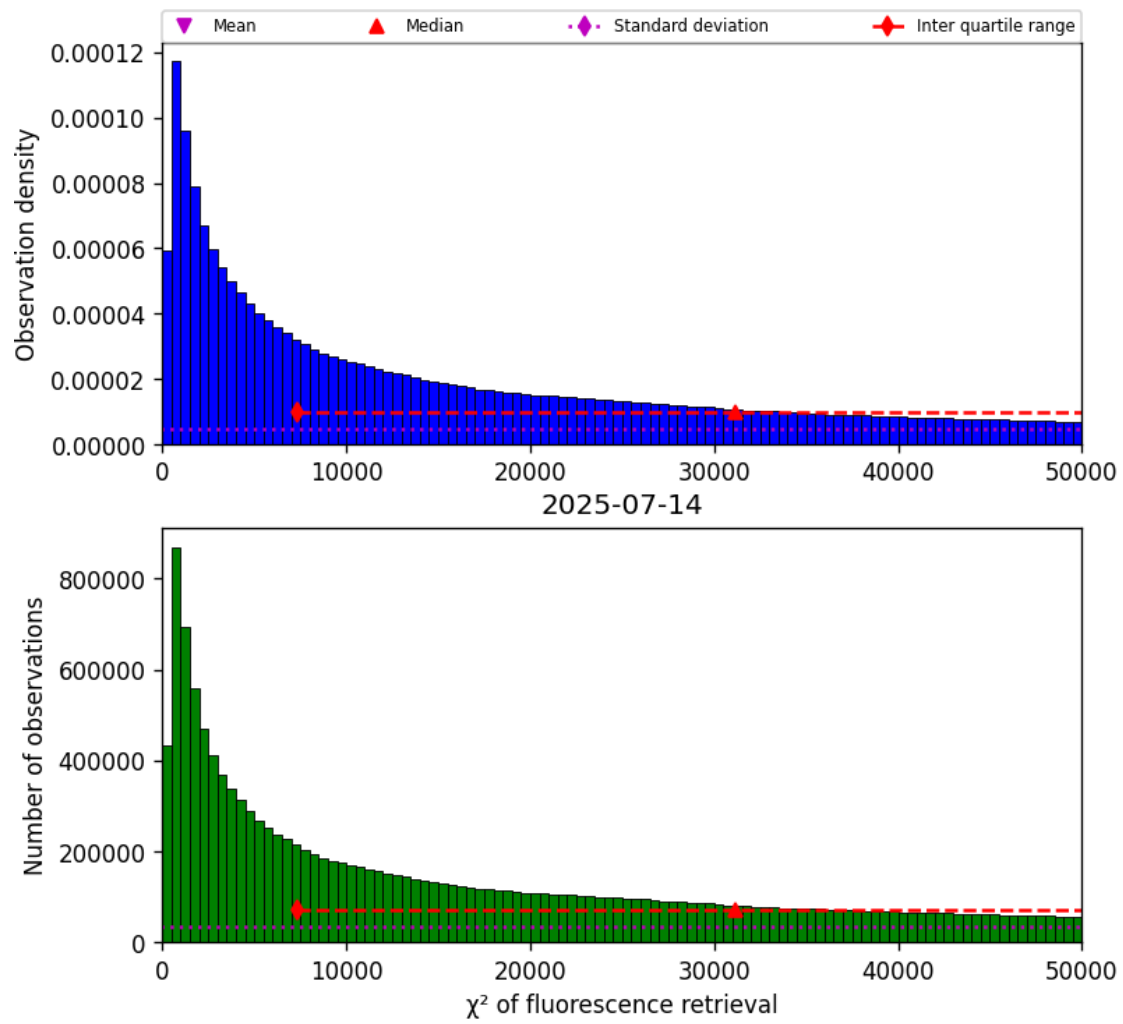
Figure 40: Histogram of “ \chi^2 of fluorescence retrieval” for 2025-07-14 to 2025-07-15
