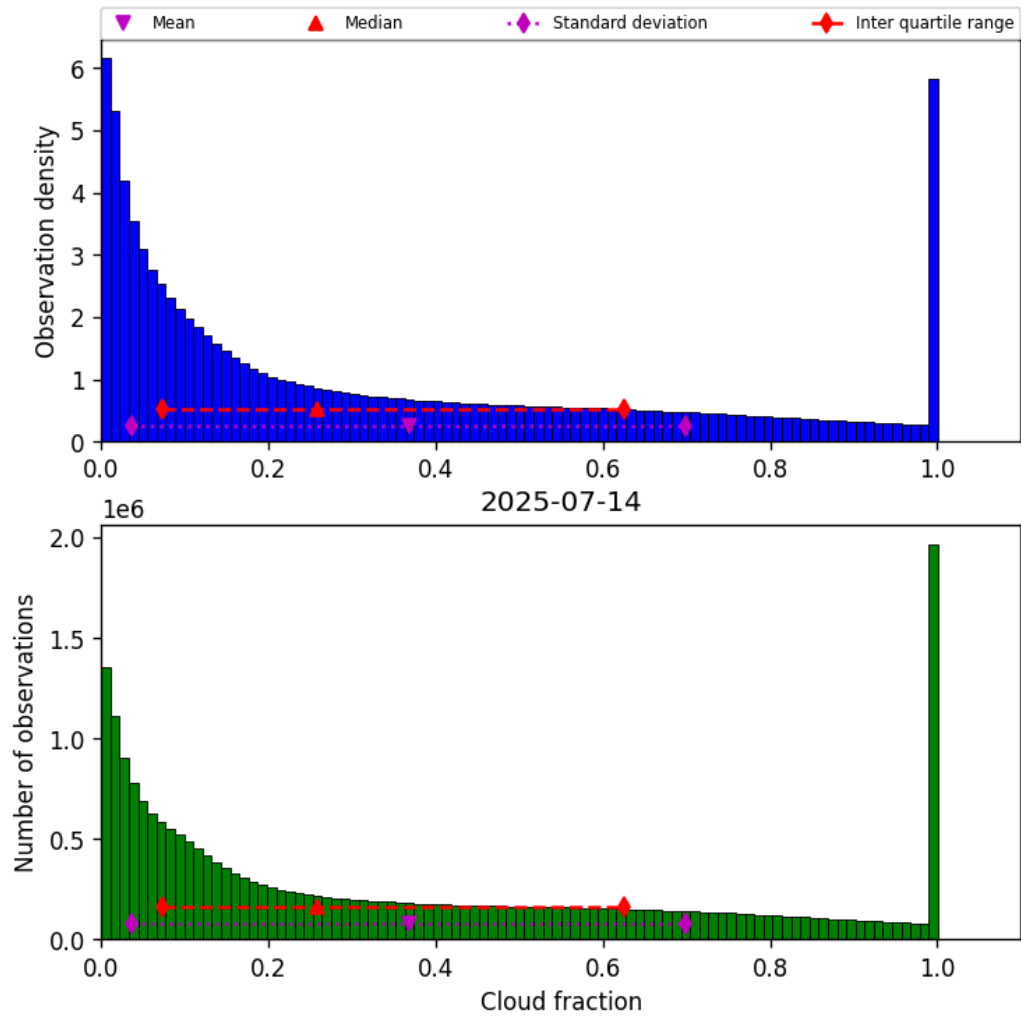
Figure 30: Histogram of “Cloud fraction” for 2025-07-14 to 2025-07-15
