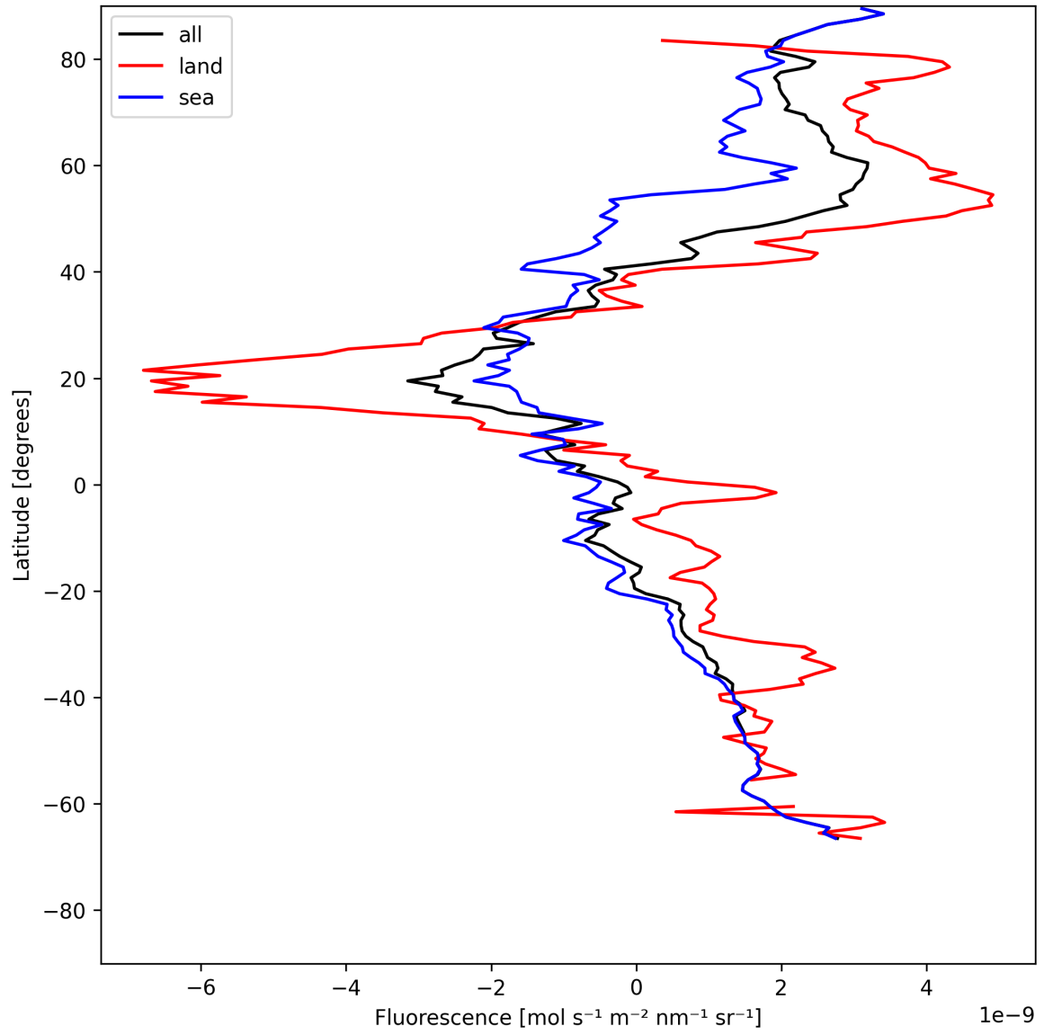
Figure 21: Zonal average of “Fluorescence” for 2025-07-14 to 2025-07-15.
