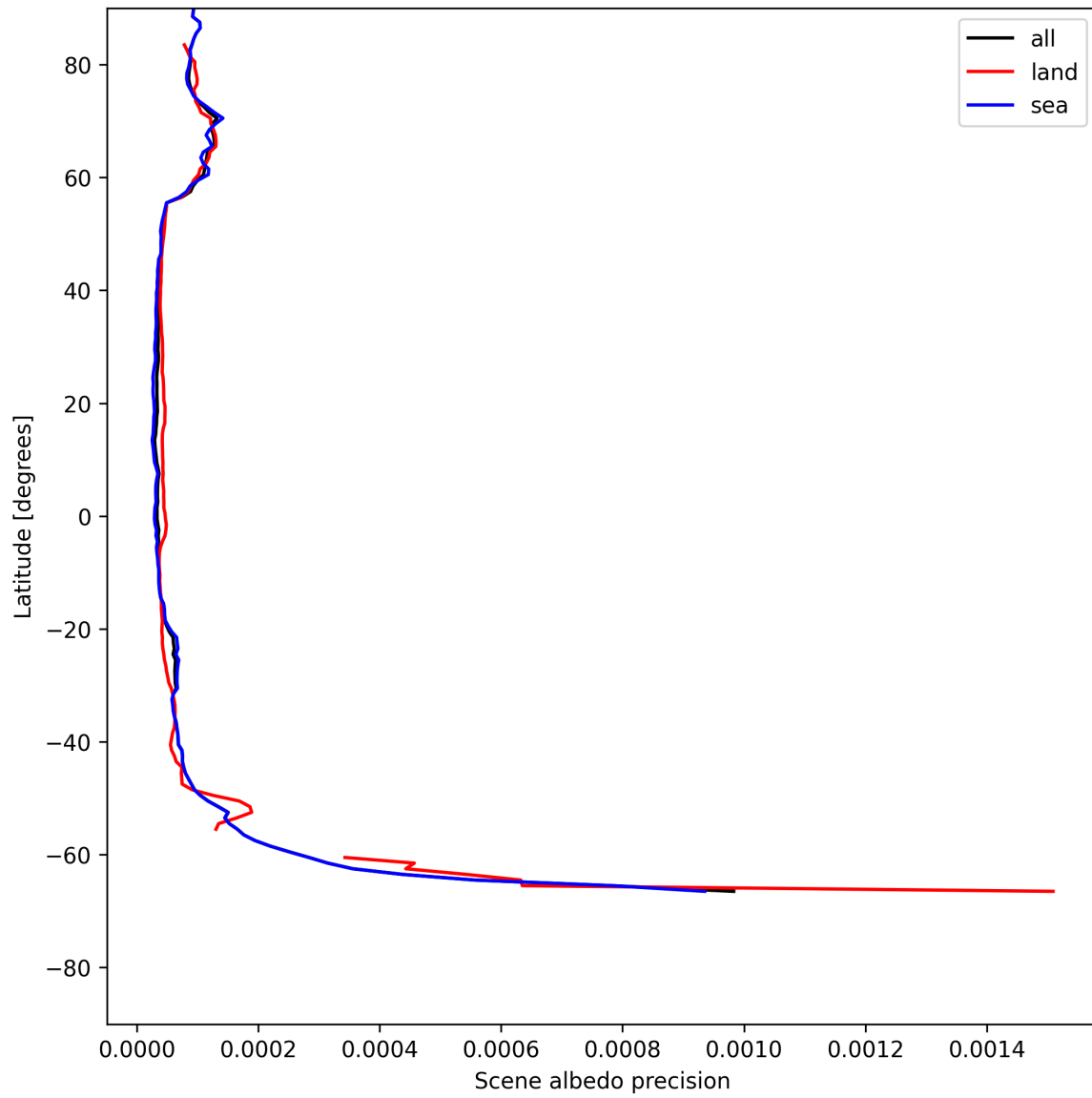
Figure 16: Zonal average of “Scene albedo precision” for 2025-07-14 to 2025-07-15.
