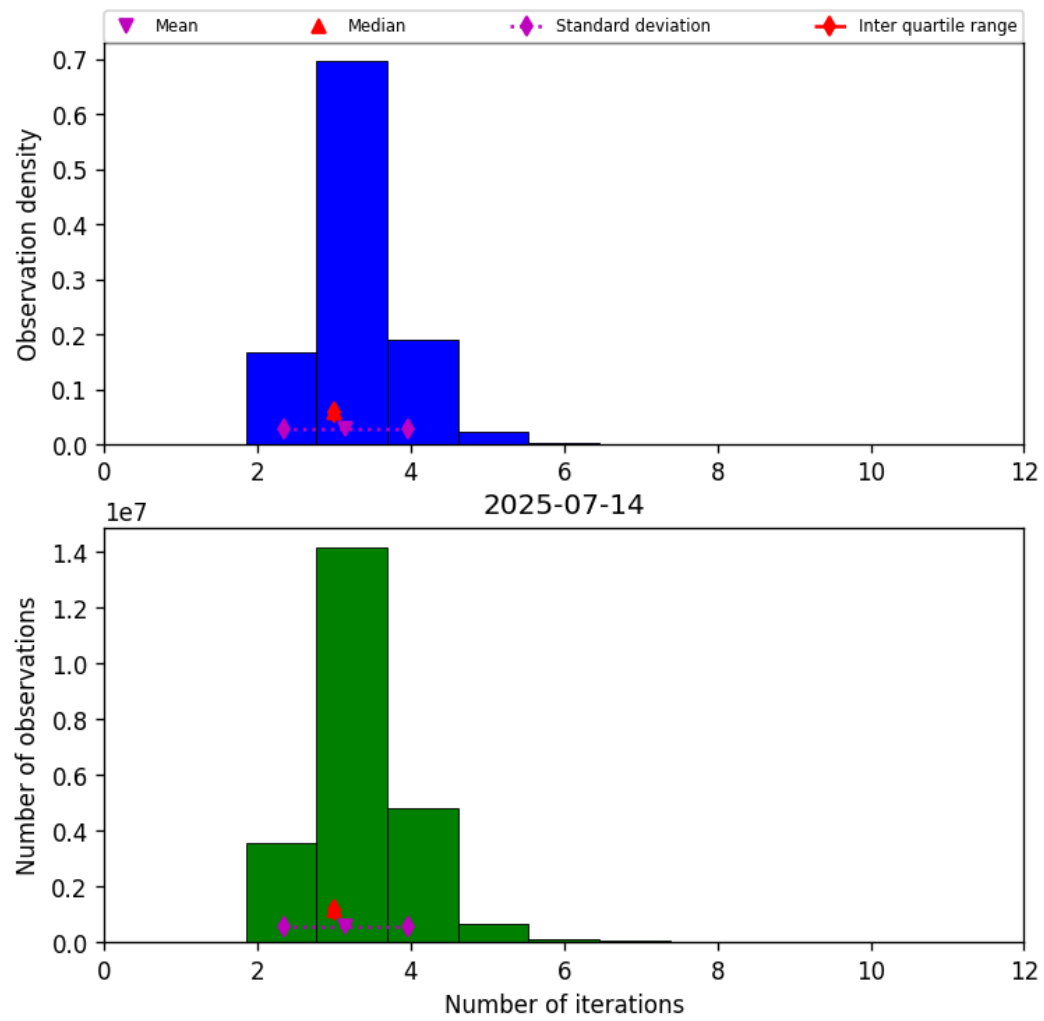
Figure 37: Histogram of “Number of iterations” for 2025-07-14 to 2025-07-15
