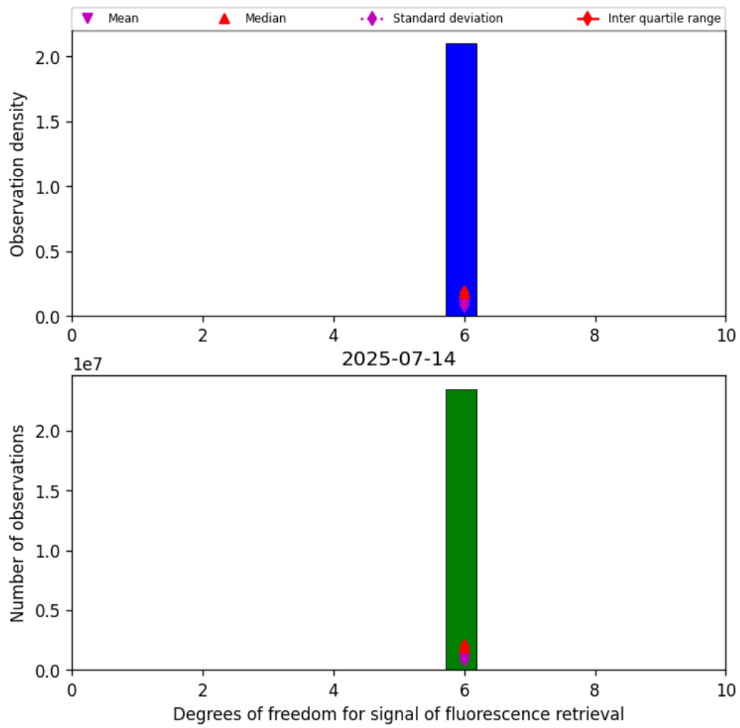
Figure 41: Histogram of “Degrees of freedom for signal of fluorescence retrieval” for 2025-07-14 to 2025-07-15
