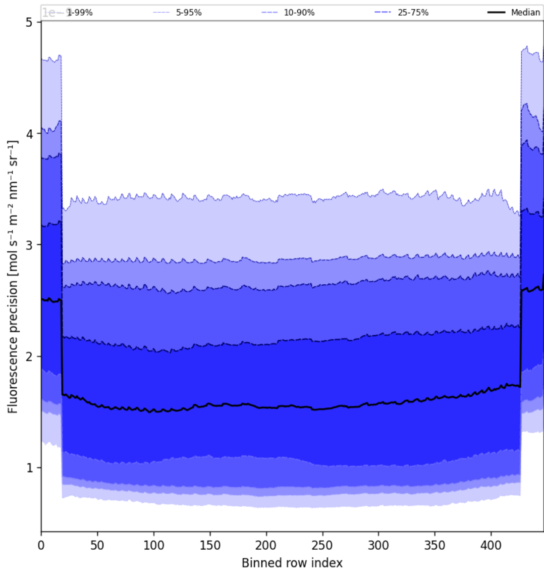
Figure 56: Along track statistics of “Fluorescence precision” for 2025-07-14 to 2025-07-15
