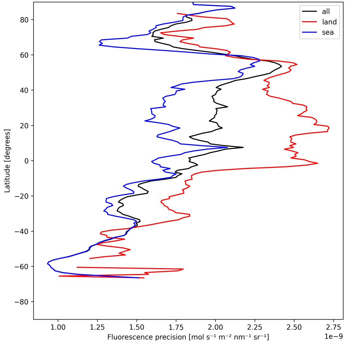
Figure 22: Zonal average of “Fluorescence precision” for 2025-07-14 to 2025-07-15.
