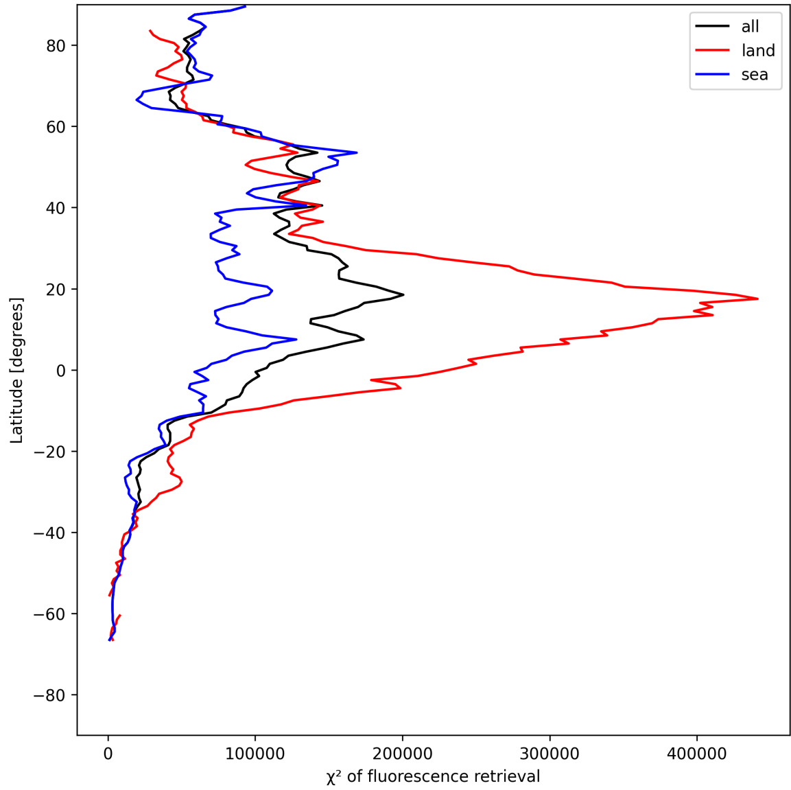
Figure 23: Zonal average of “ \chi^2 of fluorescence retrieval” for 2025-07-14 to 2025-07-15.
