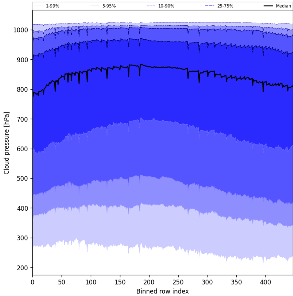
Figure 45: Along track statistics of “Cloud pressure” for 2025-07-14 to 2025-07-15
