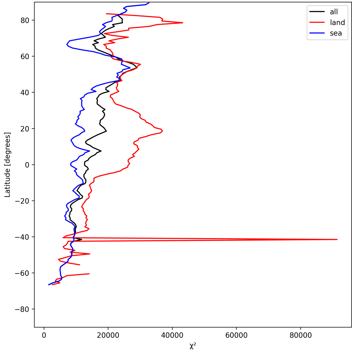
Figure 19: Zonal average of “ \chi^2 ” for 2025-07-14 to 2025-07-15.
