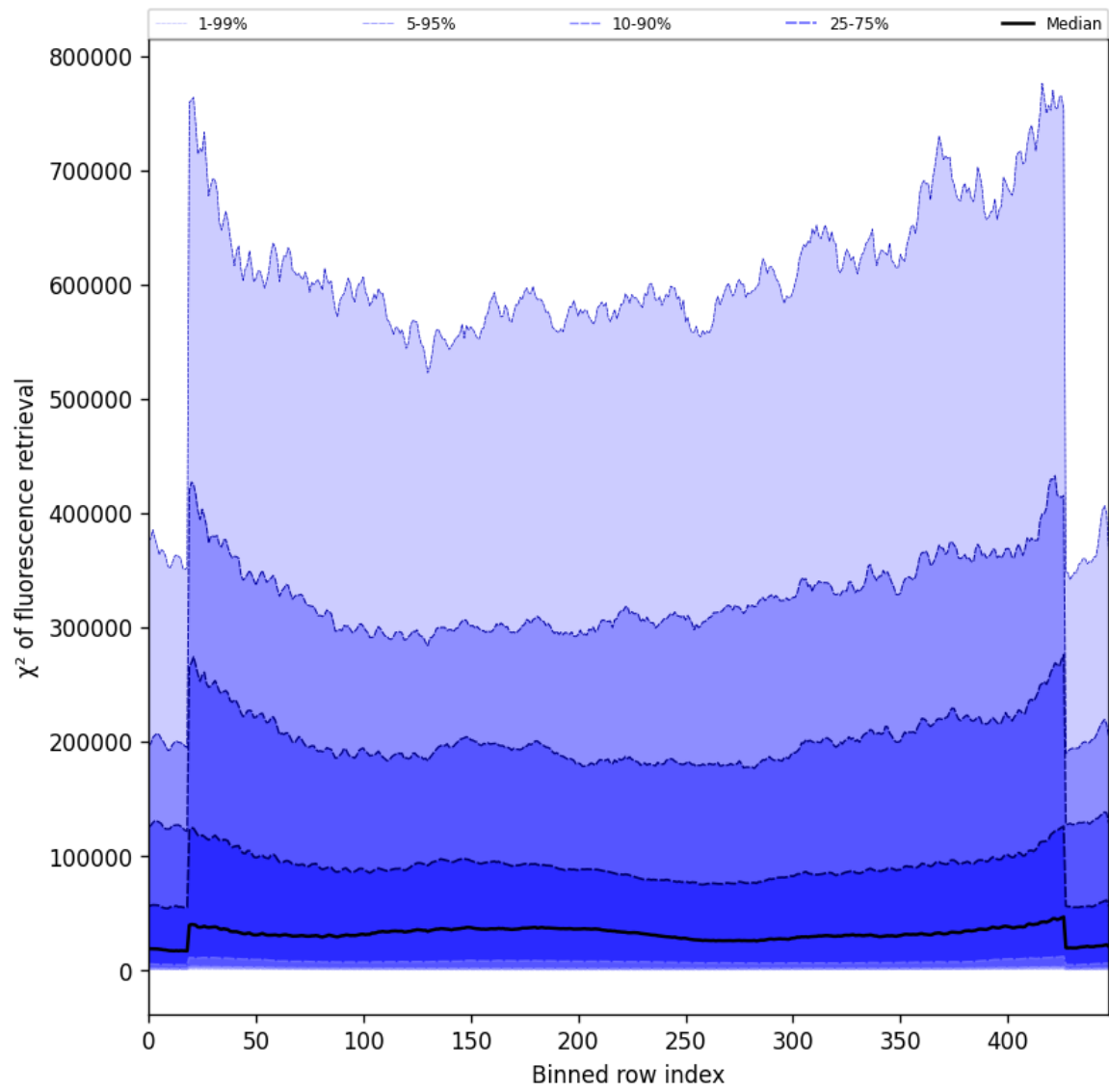
Figure 57: Along track statistics of “ \chi^2 of fluorescence retrieval” for 2025-07-14 to 2025-07-15
