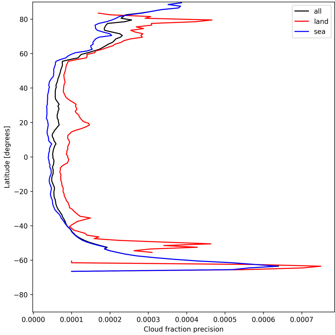
Figure 14: Zonal average of “Cloud fraction precision” for 2025-07-14 to 2025-07-15.
