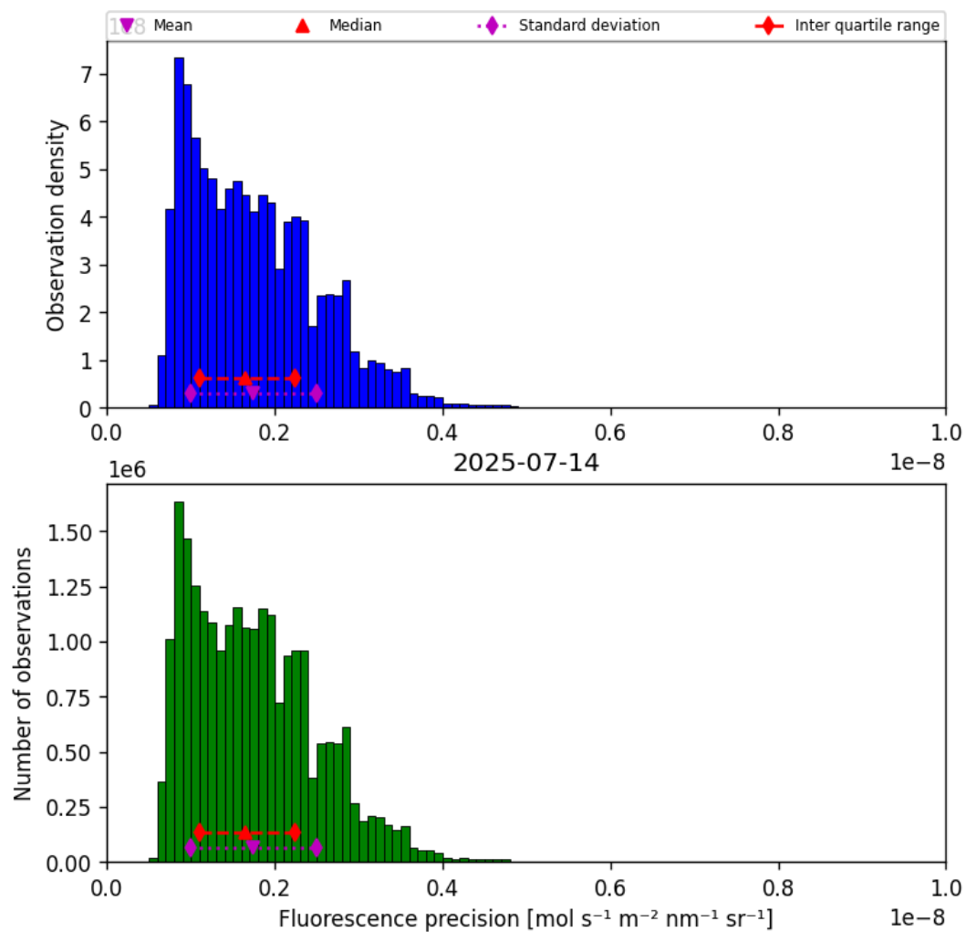
Figure 39: Histogram of “Fluorescence precision” for 2025-07-14 to 2025-07-15
