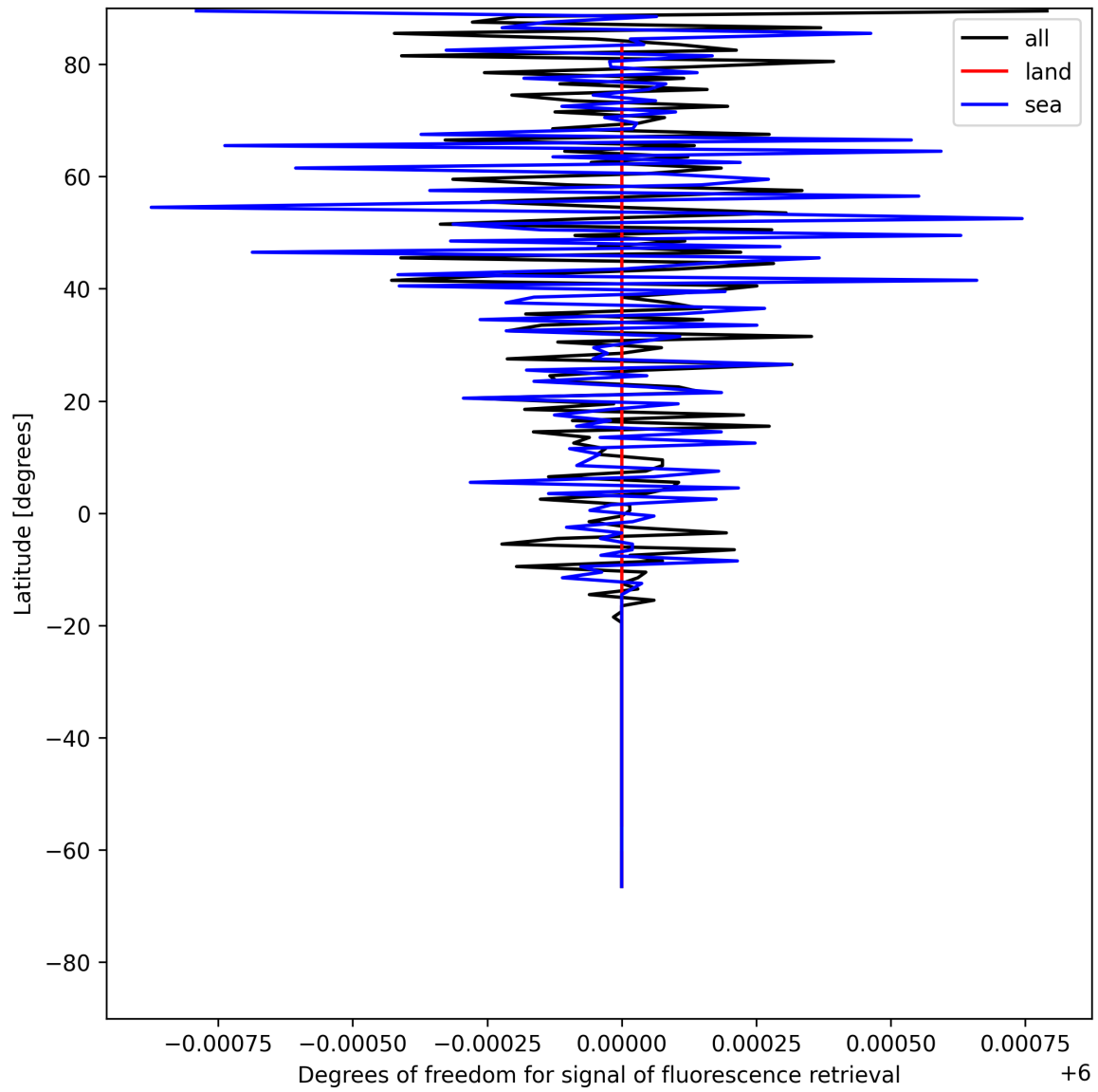
Figure 24: Zonal average of “Degrees of freedom for signal of fluorescence retrieval” for 2025-07-14 to 2025-07-15.
