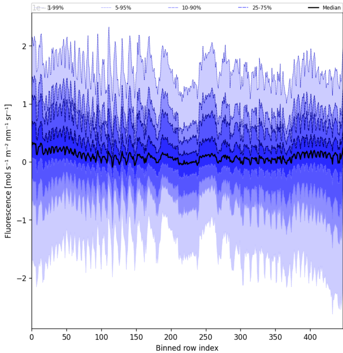
Figure 55: Along track statistics of “Fluorescence” for 2025-07-14 to 2025-07-15
