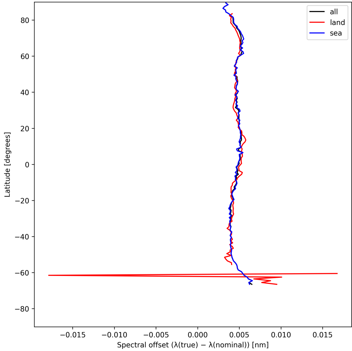
Figure 26: Zonal average of “Spectral offset ( \lambda_{\text{true}} - \lambda_{\text{nominal}} )” for 2025-07-14 to 2025-07-15.
