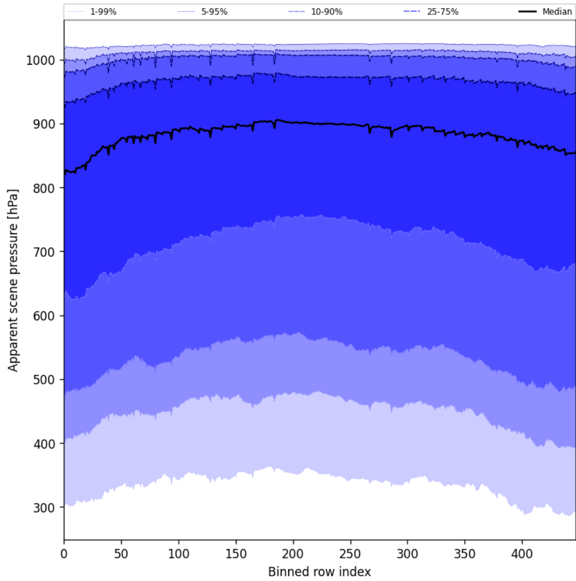
Figure 51: Along track statistics of “Apparent scene pressure” for 2025-07-14 to 2025-07-15
