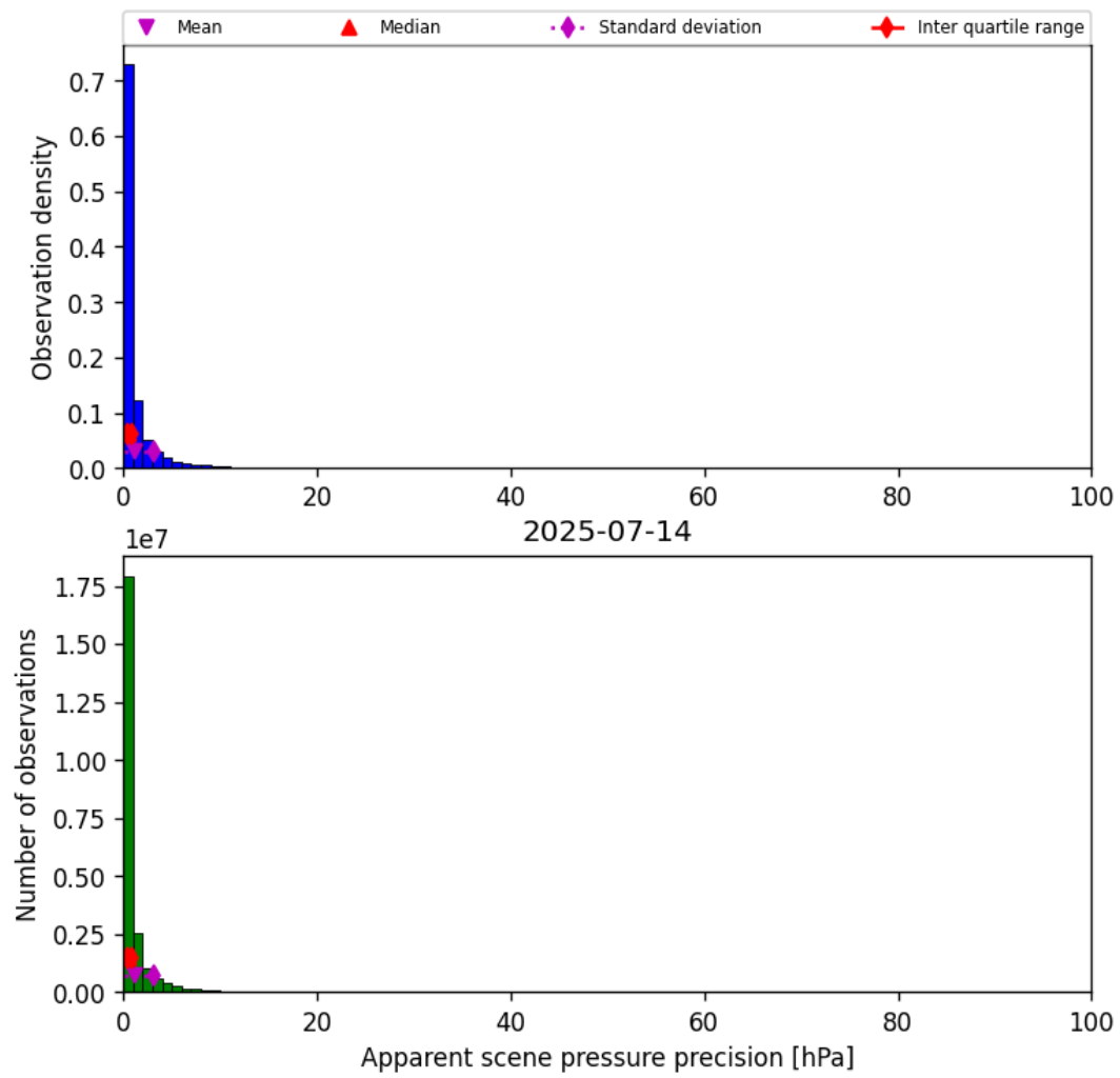
Figure 35: Histogram of “Apparent scene pressure precision” for 2025-07-14 to 2025-07-15
