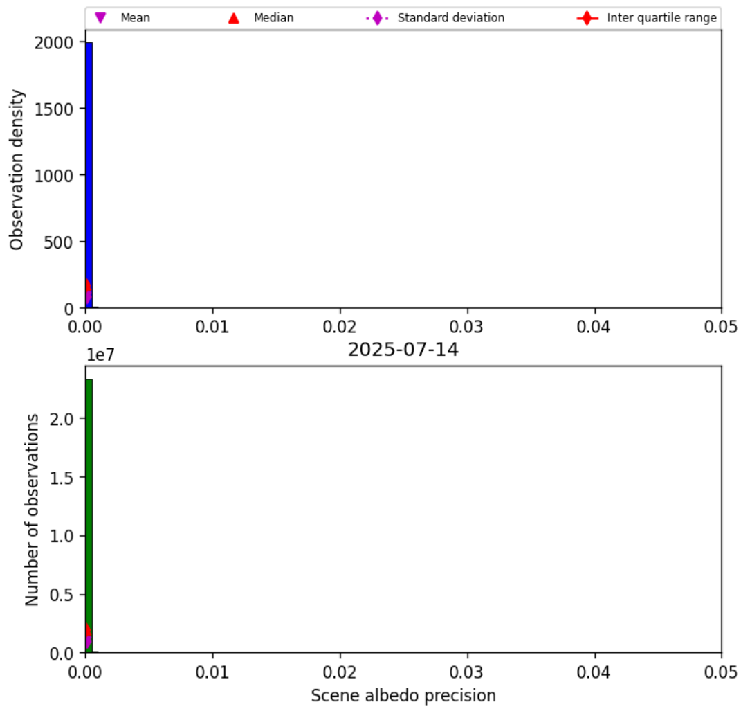
Figure 33: Histogram of “Scene albedo precision” for 2025-07-14 to 2025-07-15
