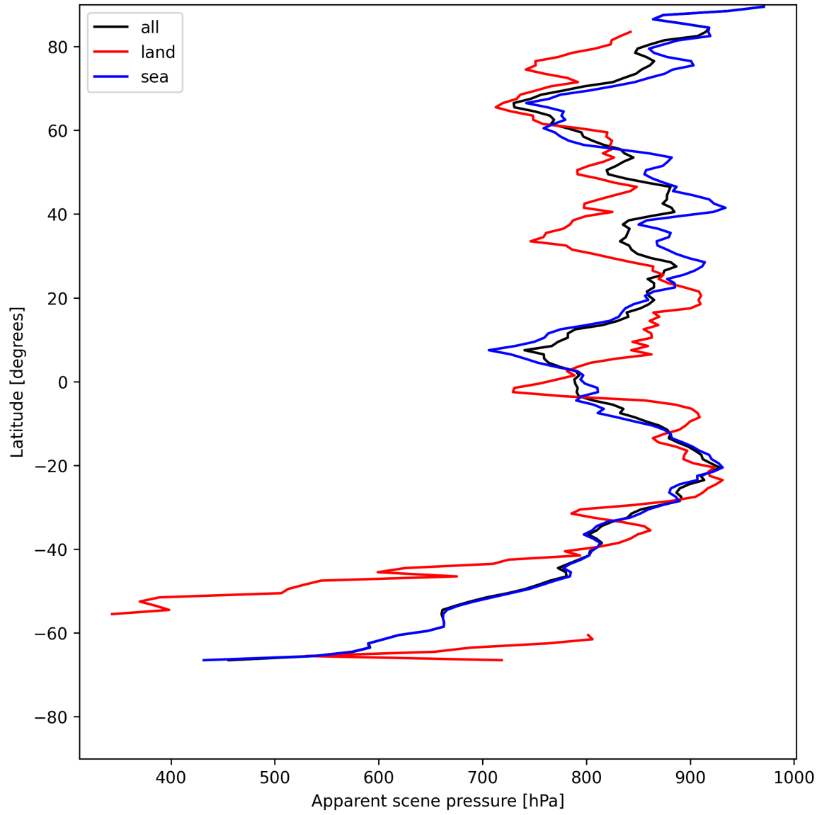
Figure 17: Zonal average of “Apparent scene pressure” for 2025-07-14 to 2025-07-15.
