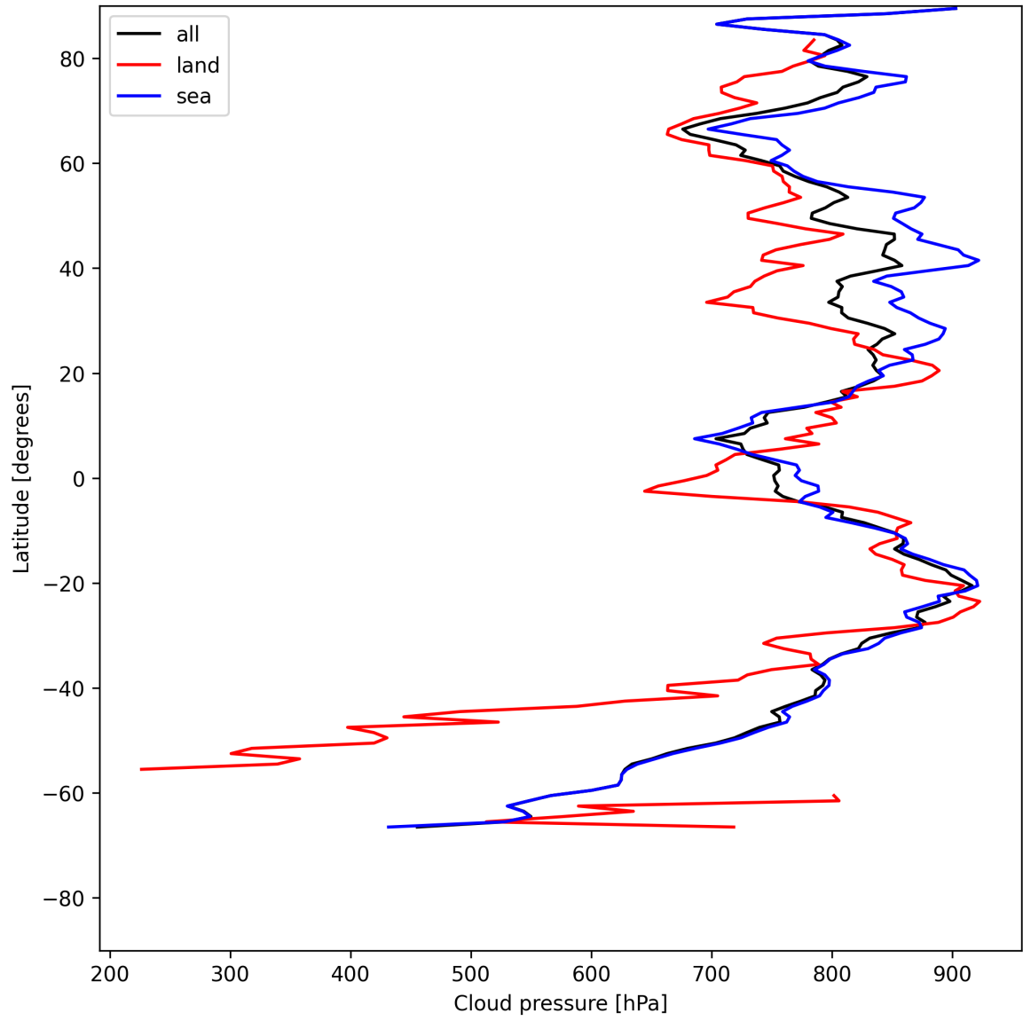
Figure 11: Zonal average of “Cloud pressure” for 2025-07-14 to 2025-07-15.
