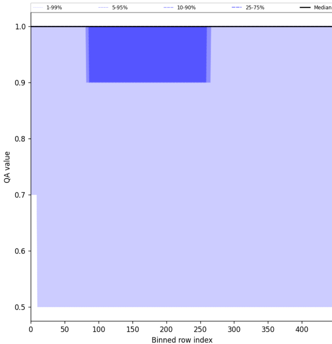
Figure 44: Along track statistics of “QA value” for 2025-07-14 to 2025-07-15
