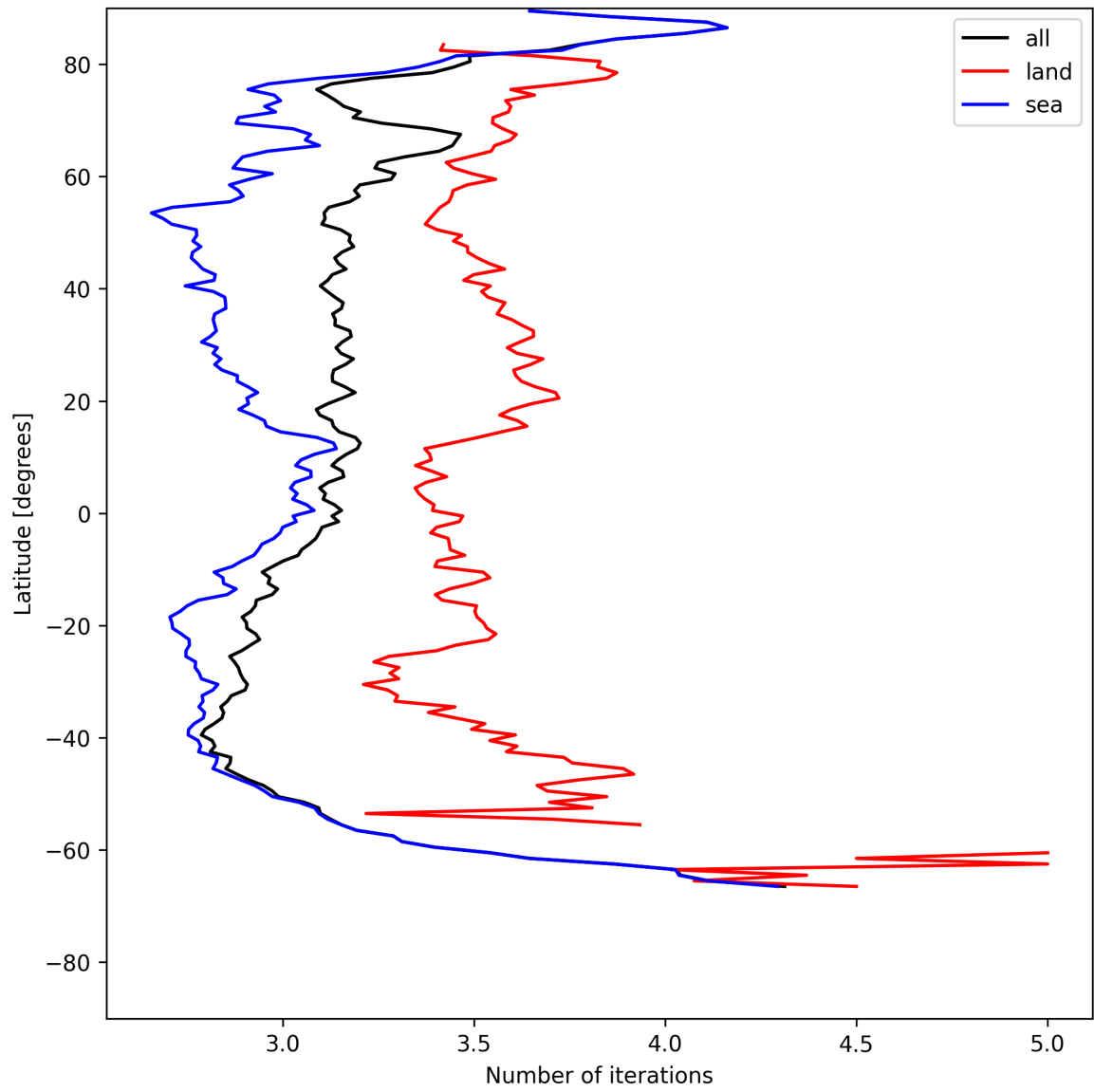
Figure 20: Zonal average of “Number of iterations” for 2025-07-14 to 2025-07-15.
