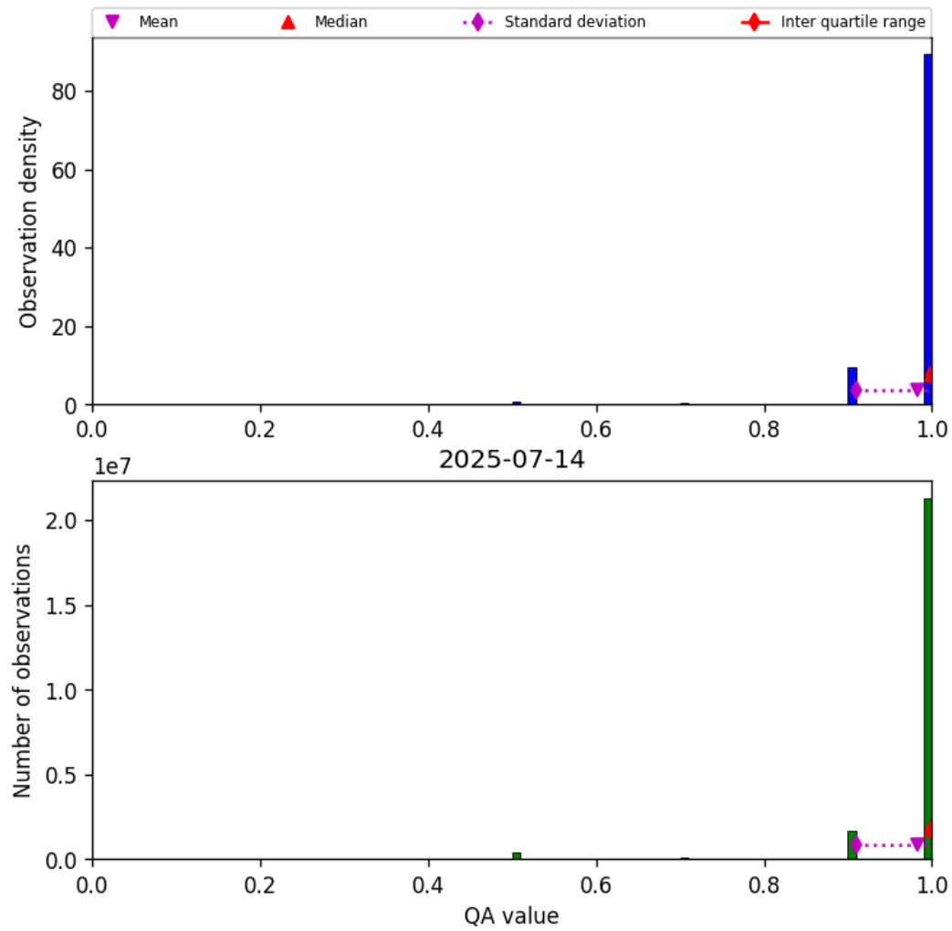
Figure 27: Histogram of “QA value” for 2025-07-14 to 2025-07-15
