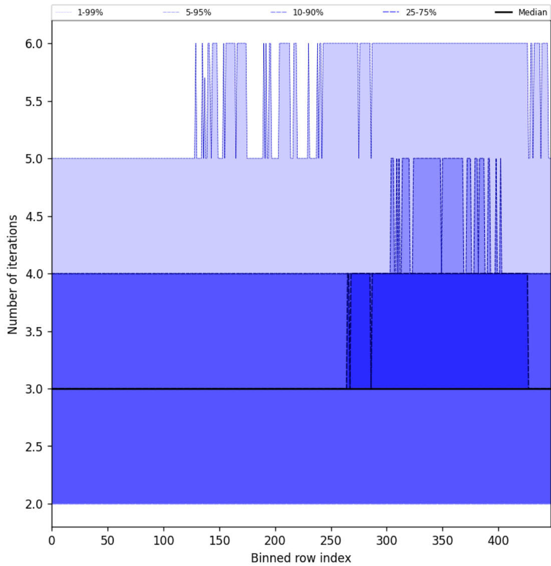
Figure 54: Along track statistics of “Number of iterations” for 2025-07-14 to 2025-07-15
