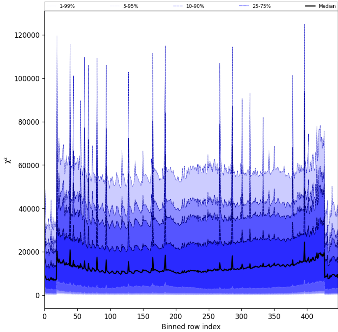
Figure 53: Along track statistics of “ \chi^2 ” for 2025-07-14 to 2025-07-15
