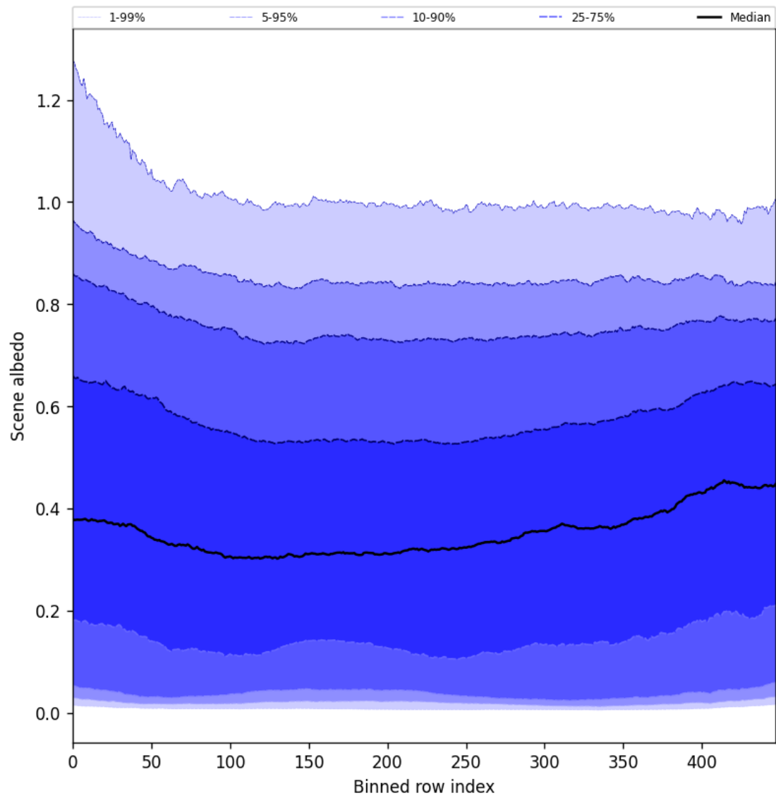
Figure 49: Along track statistics of “Scene albedo” for 2025-07-14 to 2025-07-15
