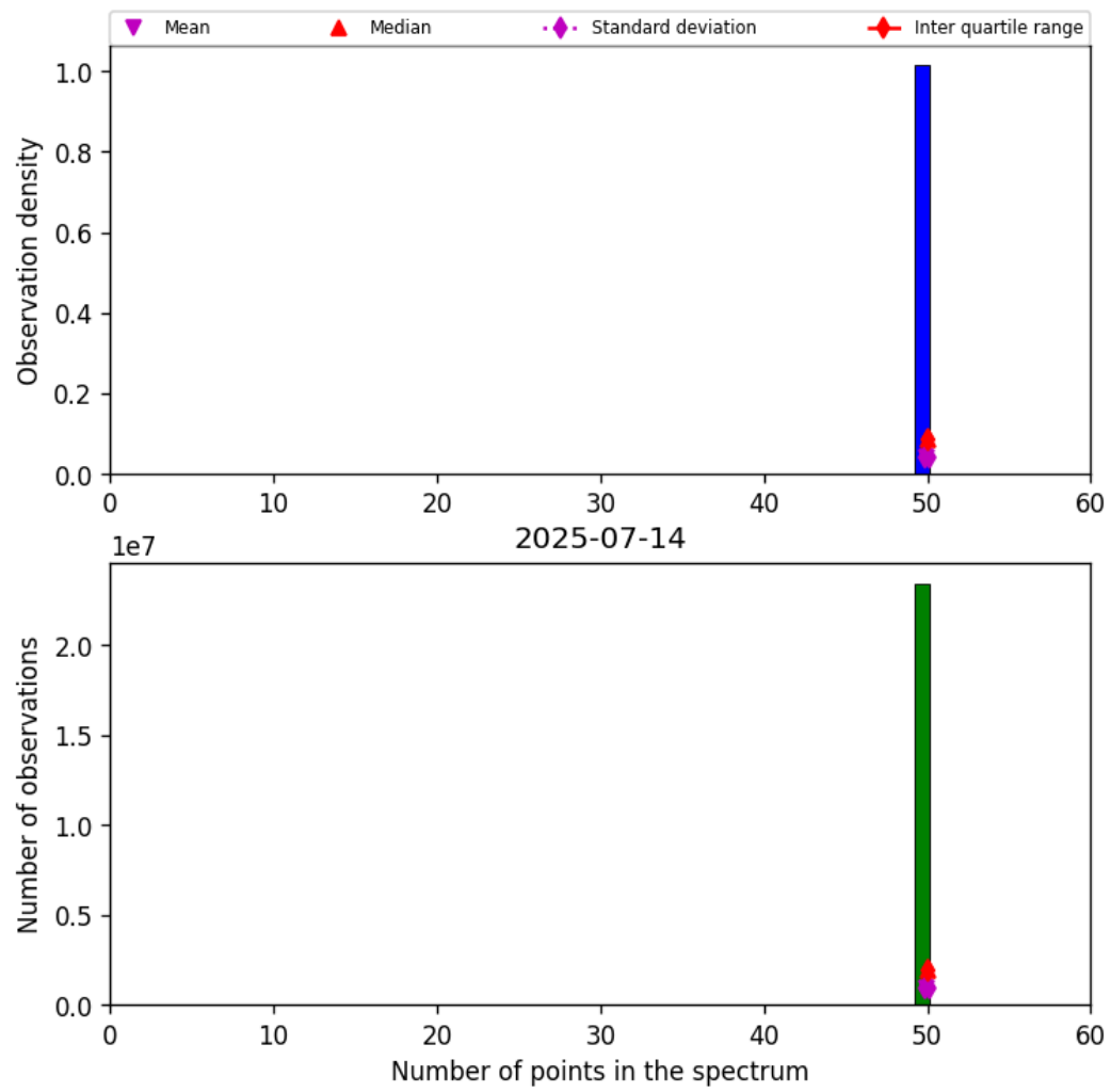
Figure 42: Histogram of “Number of points in the spectrum” for 2025-07-14 to 2025-07-15
