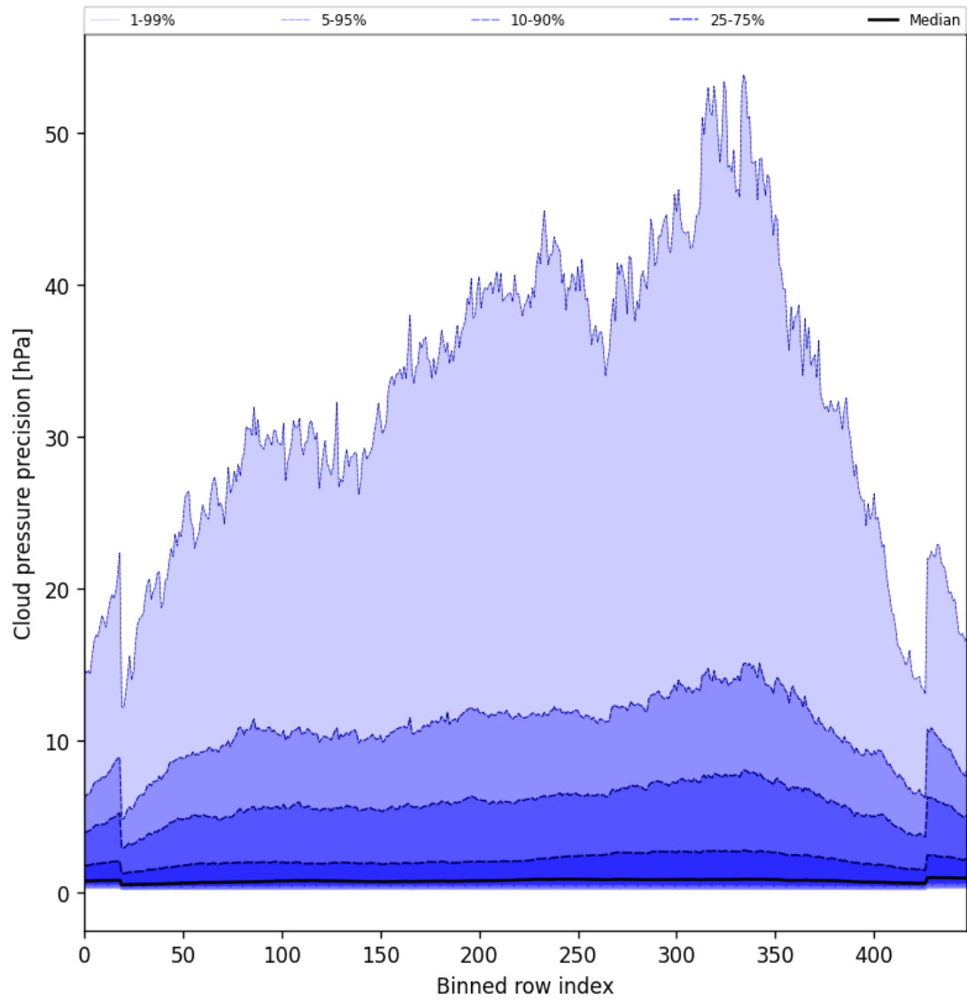
Figure 46: Along track statistics of “Cloud pressure precision” for 2025-07-14 to 2025-07-15
