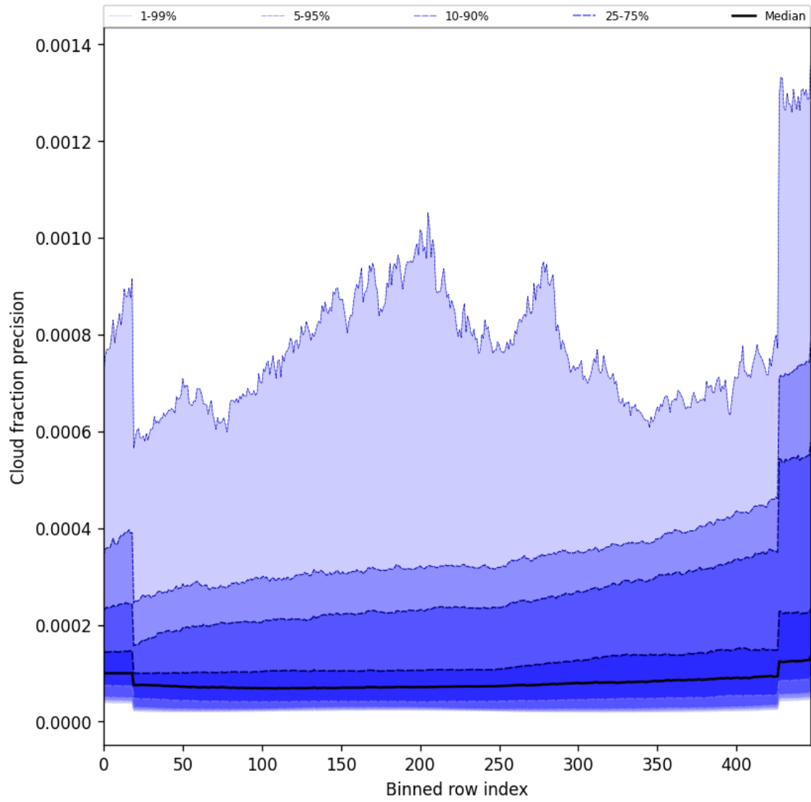
Figure 48: Along track statistics of “Cloud fraction precision” for 2025-07-14 to 2025-07-15
