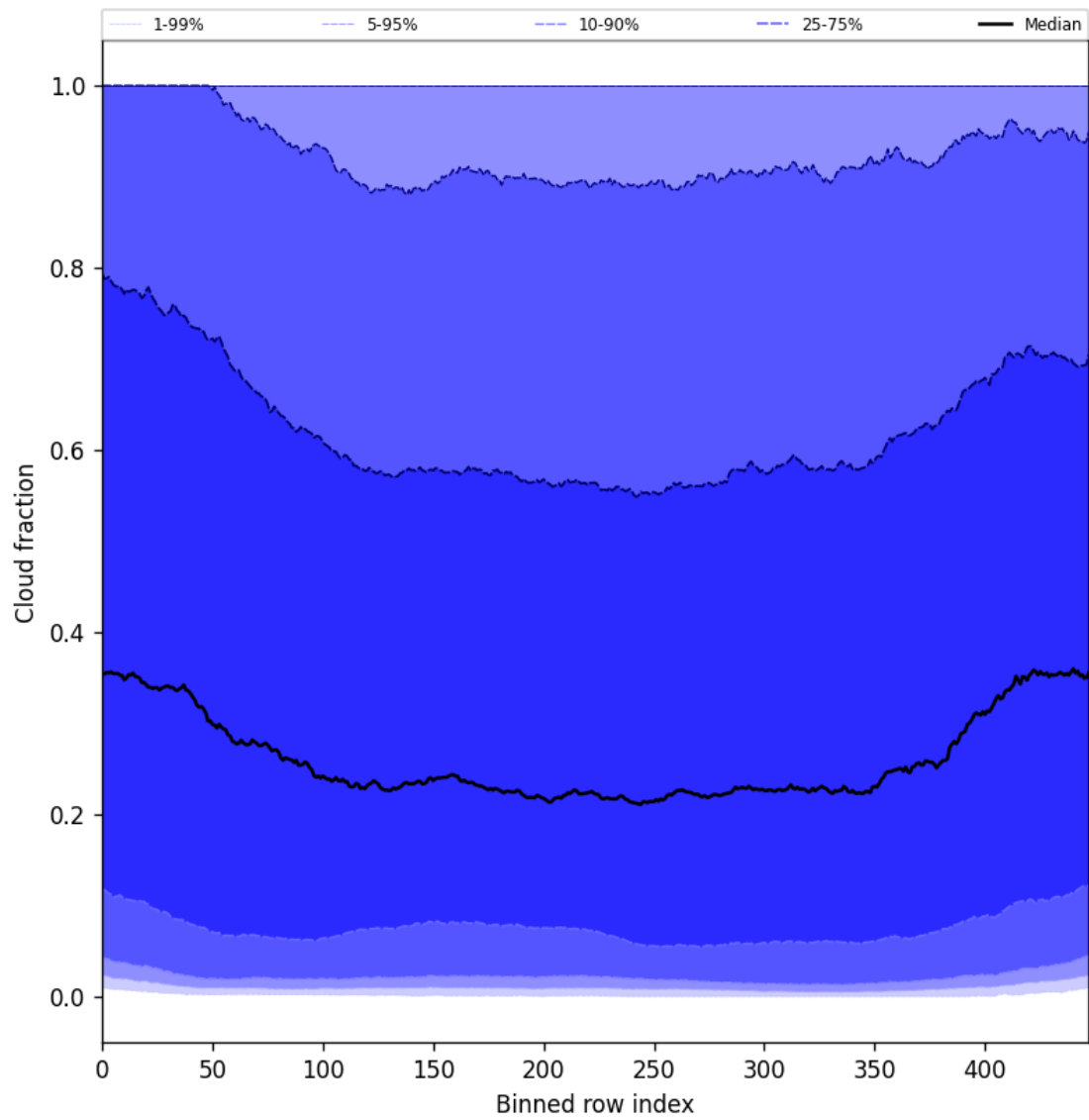
Figure 47: Along track statistics of “Cloud fraction” for 2025-07-14 to 2025-07-15
