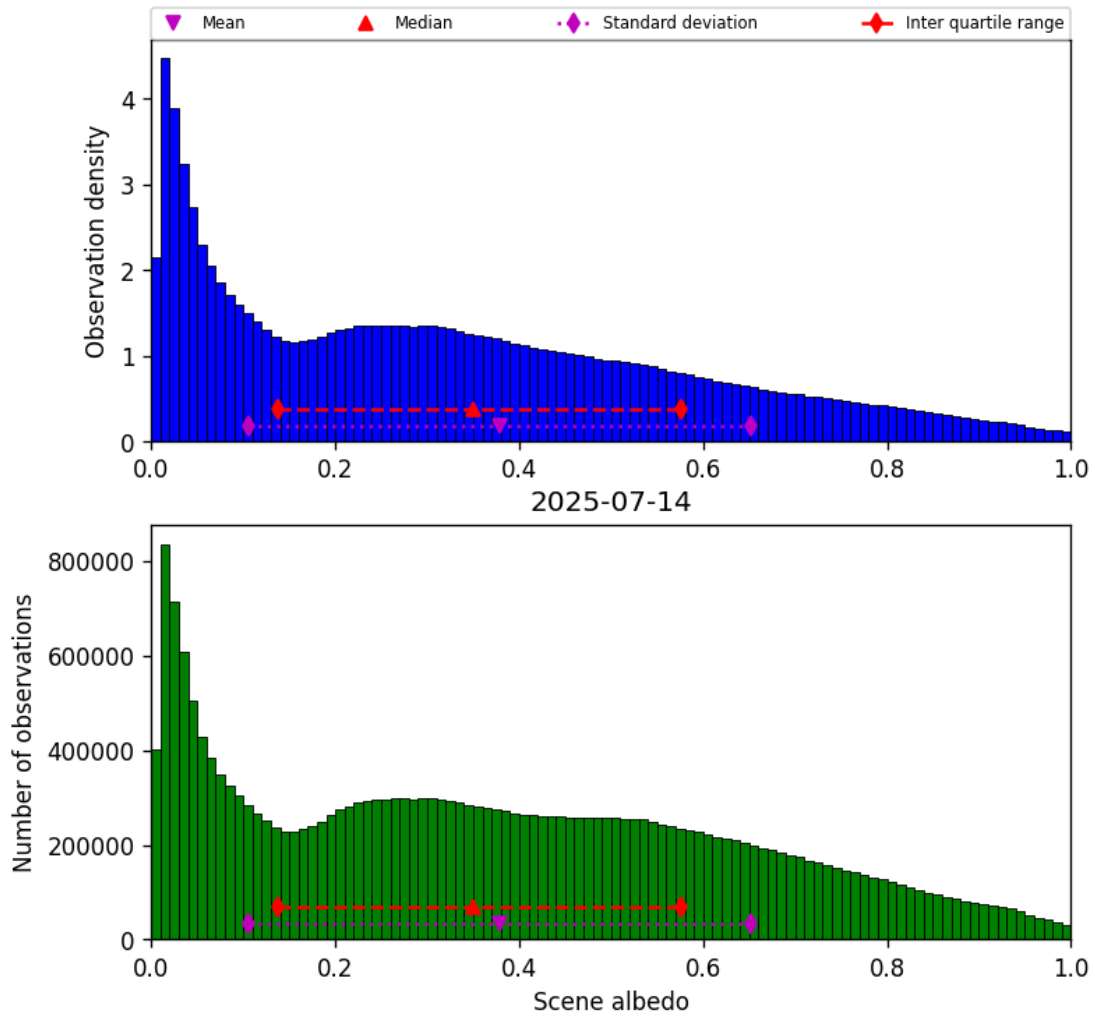
Figure 32: Histogram of “Scene albedo” for 2025-07-14 to 2025-07-15
