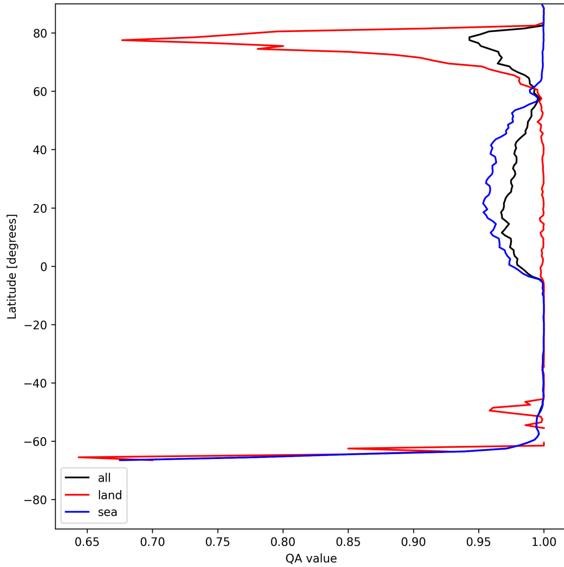
Figure 10: Zonal average of “QA value” for 2025-07-14 to 2025-07-15.
