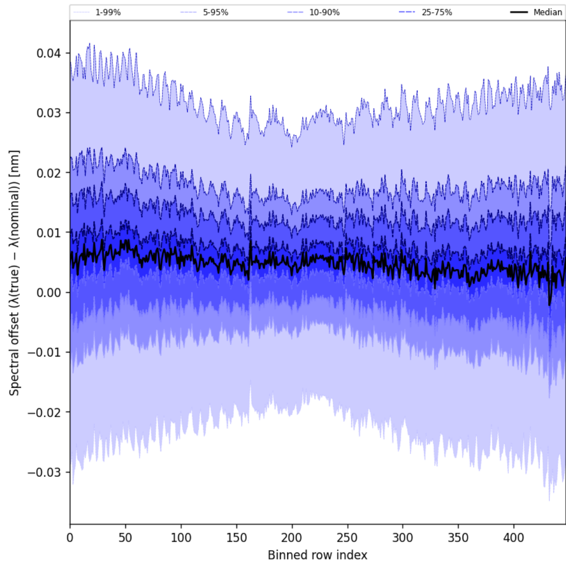
Figure 60: Along track statistics of “Spectral offset ( \lambda_{\text{true}} - \lambda_{\text{nominal}} )” for 2025-07-14 to 2025-07-15
