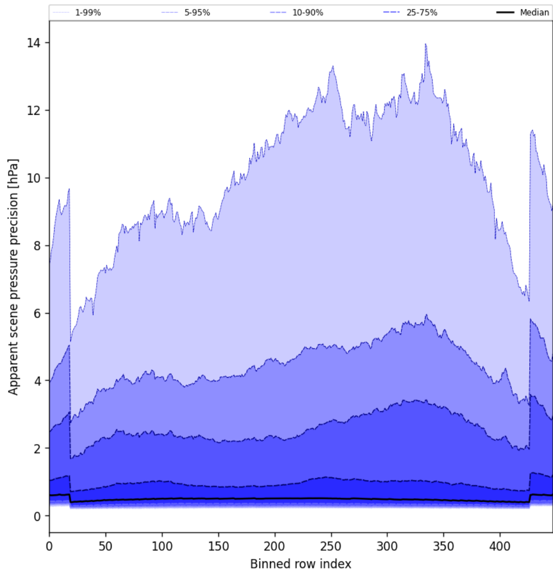
Figure 52: Along track statistics of “Apparent scene pressure precision” for 2025-07-14 to 2025-07-15
