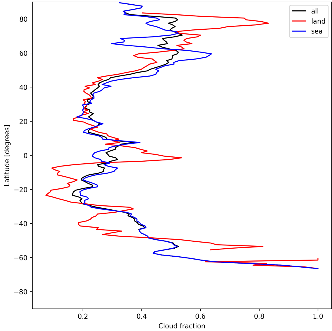
Figure 13: Zonal average of “Cloud fraction” for 2025-07-14 to 2025-07-15.
