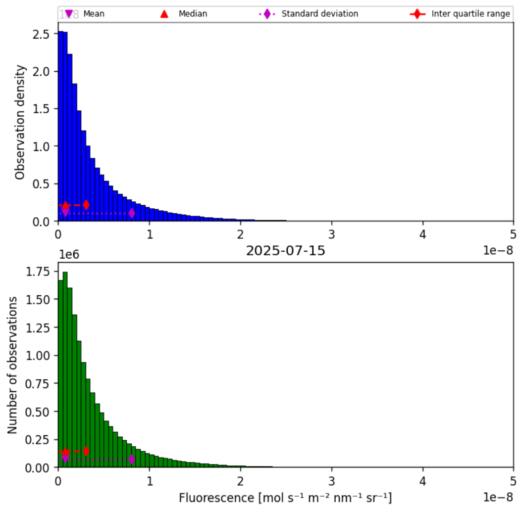
Figure 38: Histogram of “Fluorescence” for 2025-07-15 to 2025-07-16
