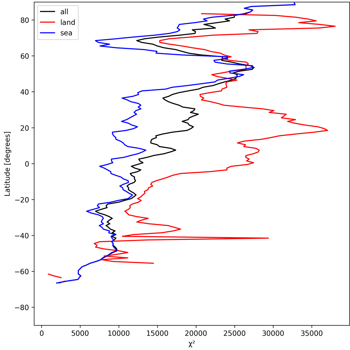
Figure 19: Zonal average of “ \chi^2 ” for 2025-07-15 to 2025-07-16.
