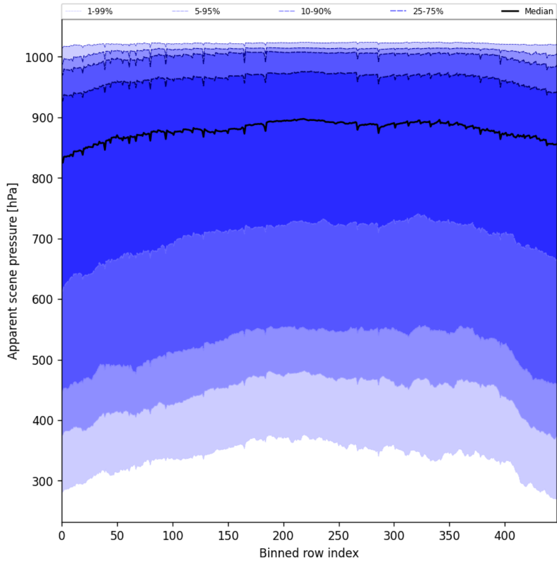
Figure 51: Along track statistics of “Apparent scene pressure” for 2025-07-15 to 2025-07-16
