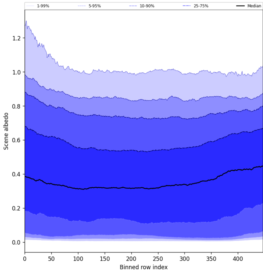
Figure 49: Along track statistics of “Scene albedo” for 2025-07-15 to 2025-07-16
