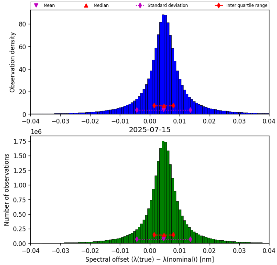
Figure 43: Histogram of “Spectral offset ( \lambda_{\text{true}} - \lambda_{\text{nominal}} )” for 2025-07-15 to 2025-07-16
