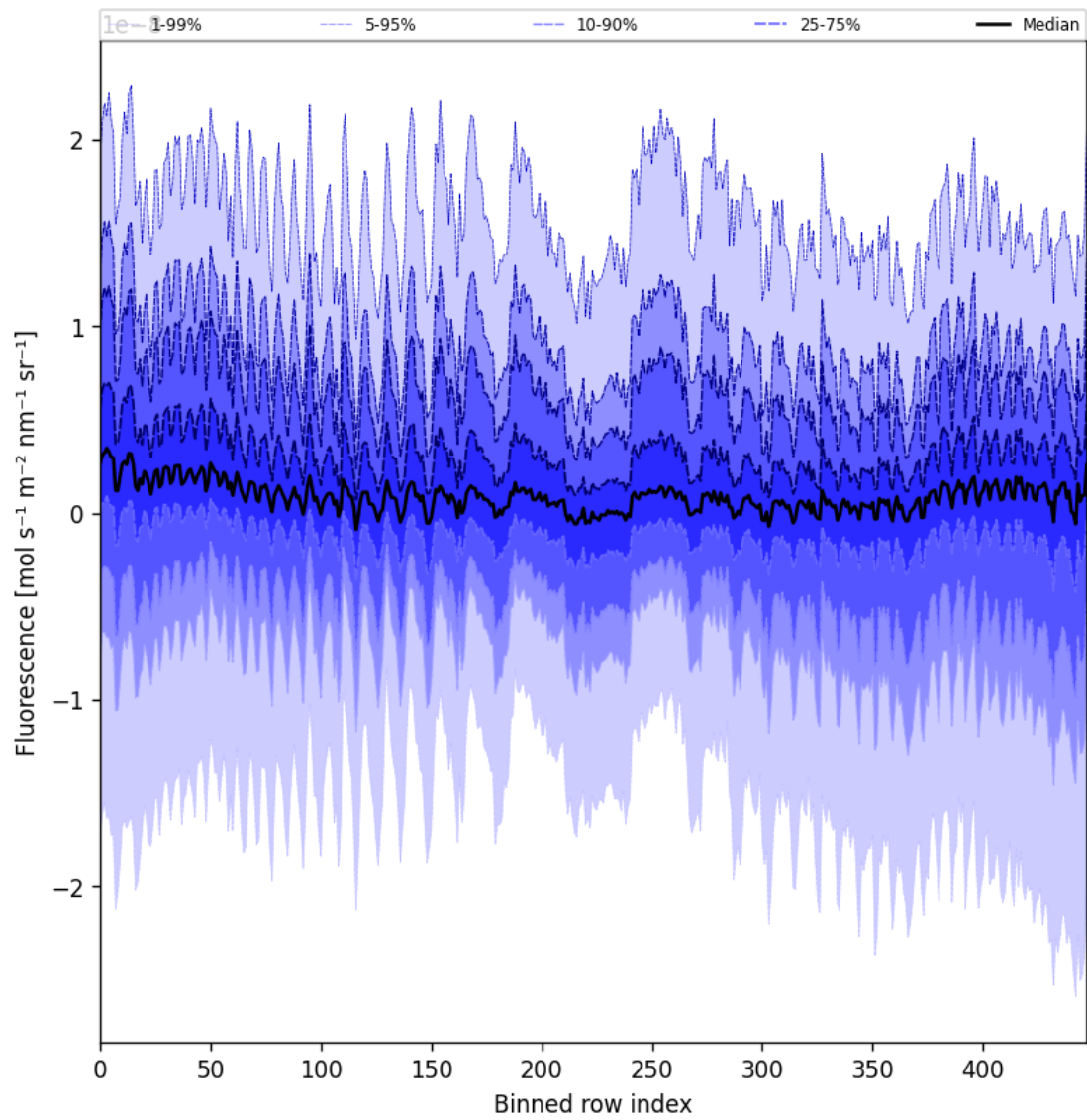
Figure 55: Along track statistics of “Fluorescence” for 2025-07-15 to 2025-07-16
