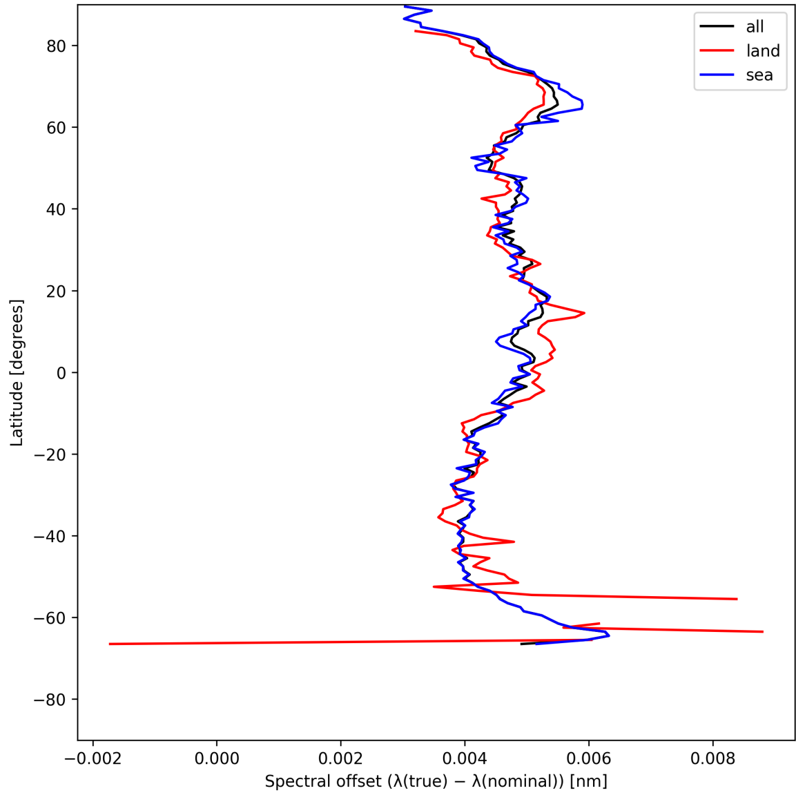
Figure 26: Zonal average of “Spectral offset ( \lambda_{\text{true}} - \lambda_{\text{nominal}} )” for 2025-07-15 to 2025-07-16.
