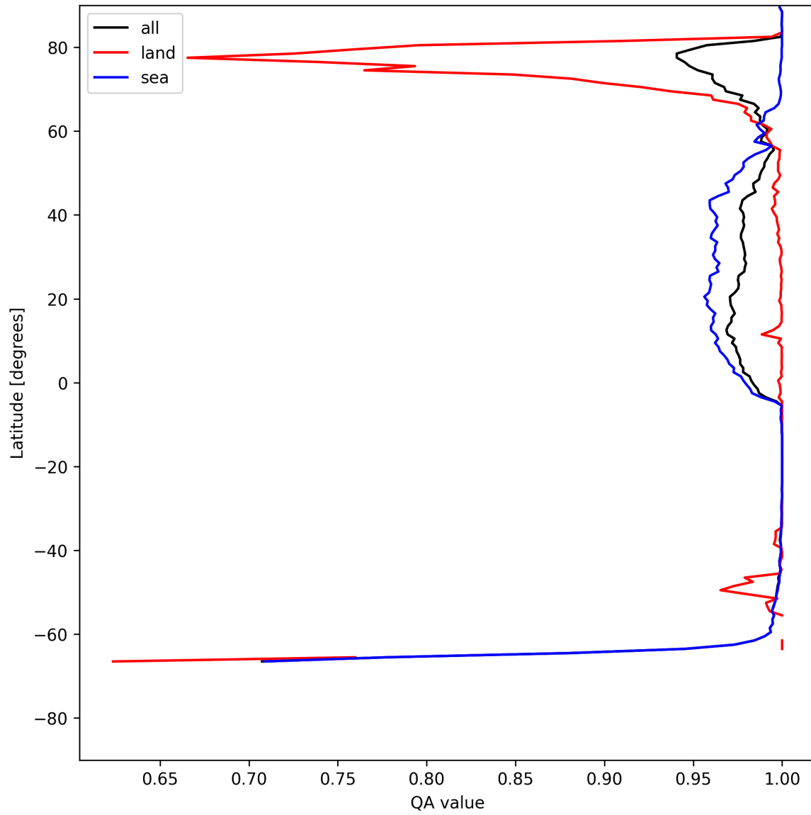
Figure 10: Zonal average of “QA value” for 2025-07-15 to 2025-07-16.
