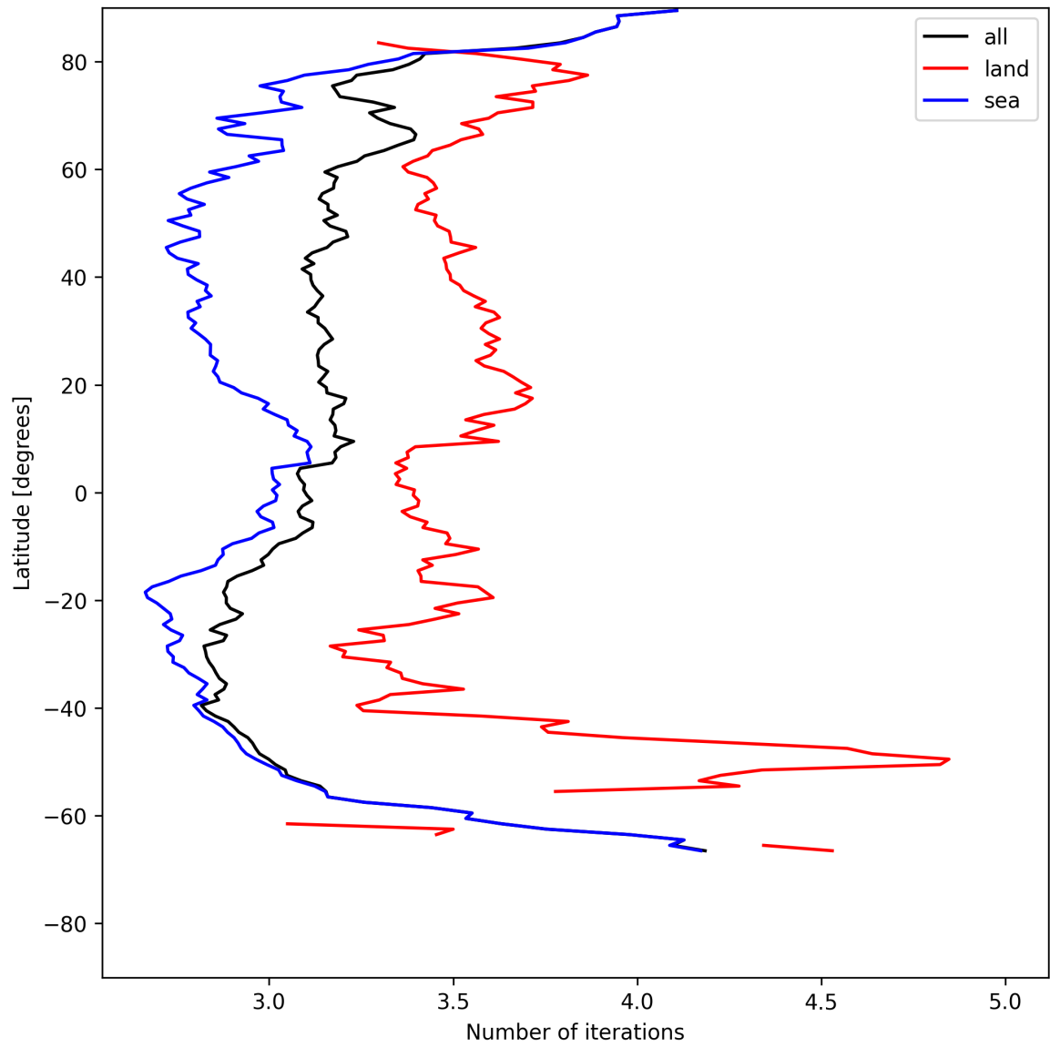
Figure 20: Zonal average of “Number of iterations” for 2025-07-15 to 2025-07-16.
