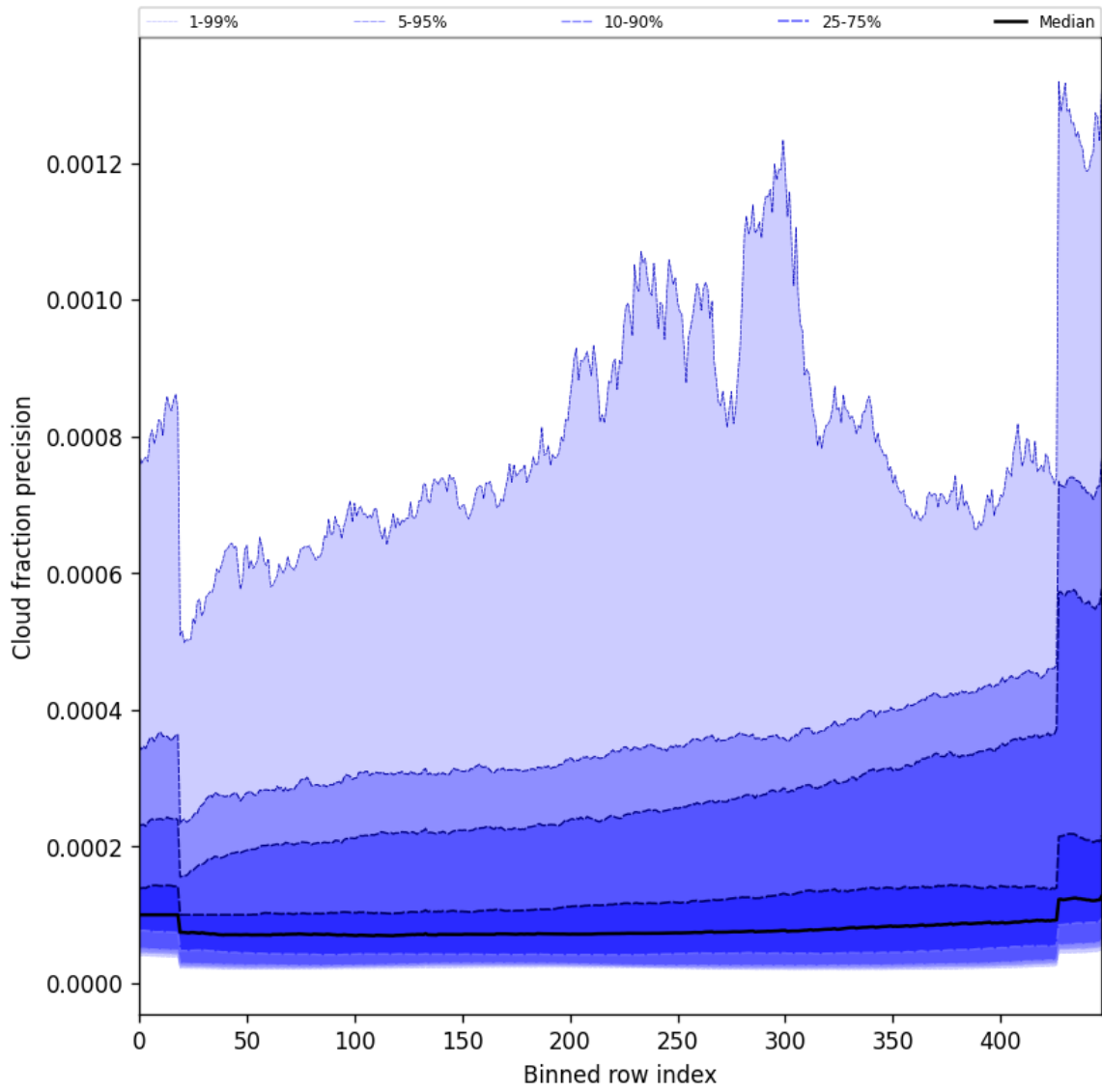
Figure 48: Along track statistics of “Cloud fraction precision” for 2025-07-15 to 2025-07-16
