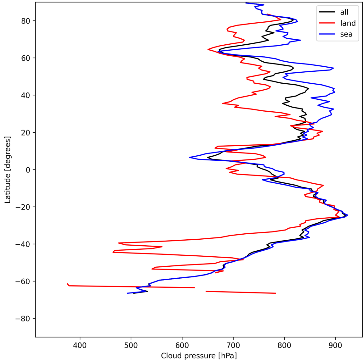
Figure 11: Zonal average of “Cloud pressure” for 2025-07-15 to 2025-07-16.
