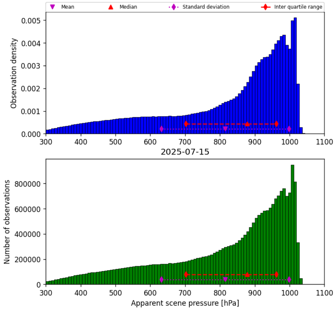
Figure 34: Histogram of “Apparent scene pressure” for 2025-07-15 to 2025-07-16
