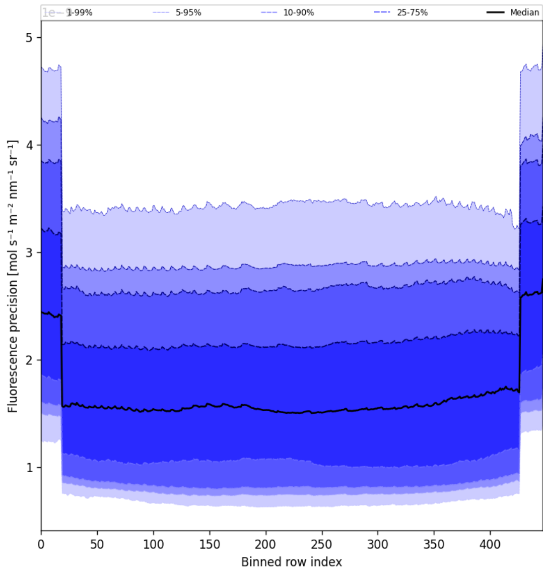
Figure 56: Along track statistics of “Fluorescence precision” for 2025-07-15 to 2025-07-16
