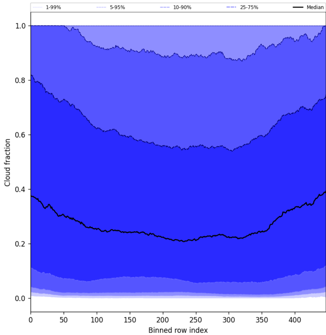
Figure 47: Along track statistics of “Cloud fraction” for 2025-07-15 to 2025-07-16
