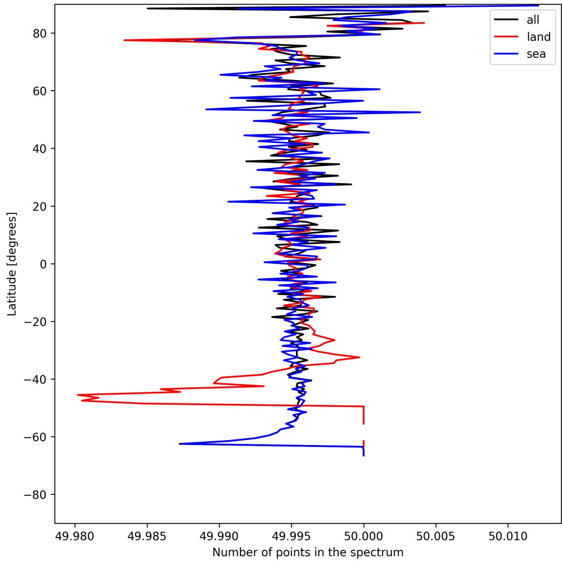
Figure 25: Zonal average of “Number of points in the spectrum” for 2025-07-15 to 2025-07-16.
