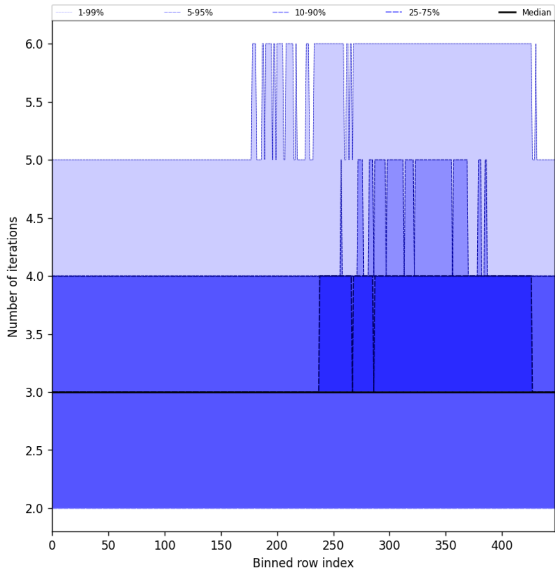
Figure 54: Along track statistics of “Number of iterations” for 2025-07-15 to 2025-07-16
