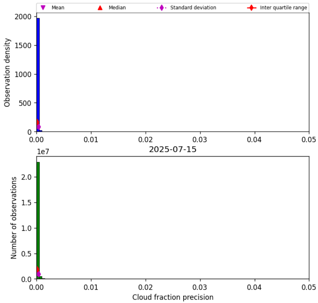
Figure 31: Histogram of “Cloud fraction precision” for 2025-07-15 to 2025-07-16
