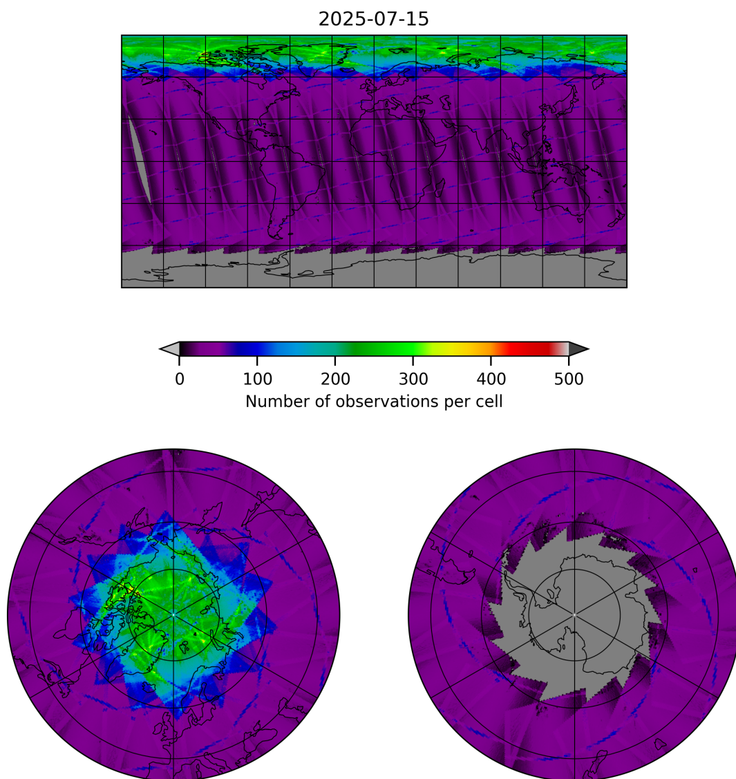
Figure 9: Map of the number of observations for 2025-07-15 to 2025-07-16
