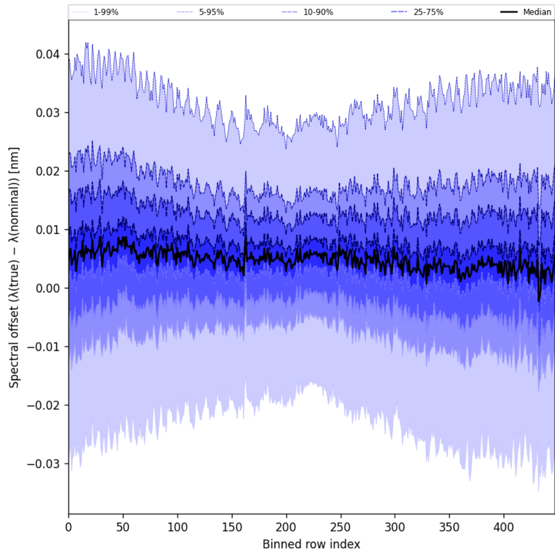
Figure 60: Along track statistics of “Spectral offset ( \lambda_{\text{true}} - \lambda_{\text{nominal}} )” for 2025-07-15 to 2025-07-16
