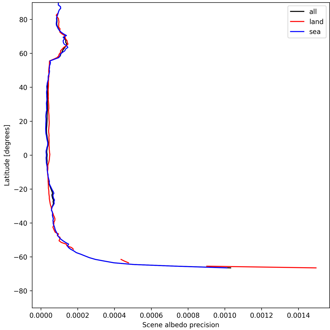
Figure 16: Zonal average of “Scene albedo precision” for 2025-07-15 to 2025-07-16.
