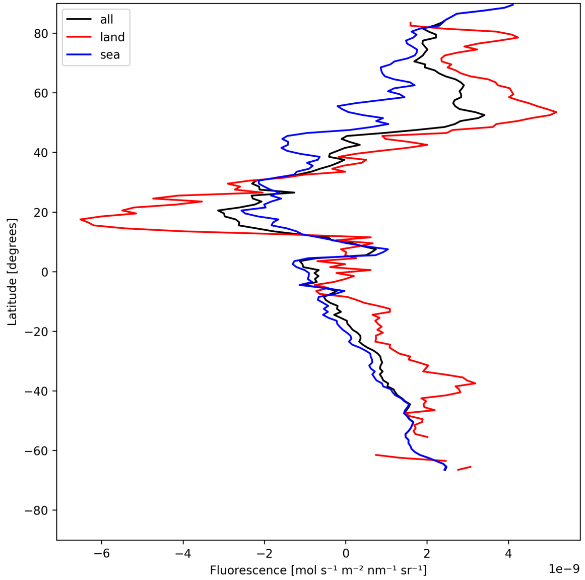
Figure 21: Zonal average of “Fluorescence” for 2025-07-15 to 2025-07-16.
