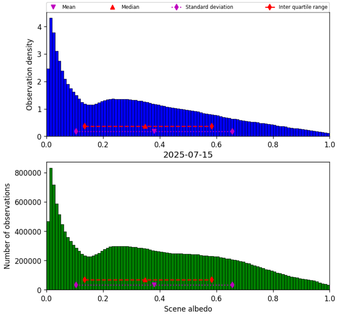
Figure 32: Histogram of “Scene albedo” for 2025-07-15 to 2025-07-16
