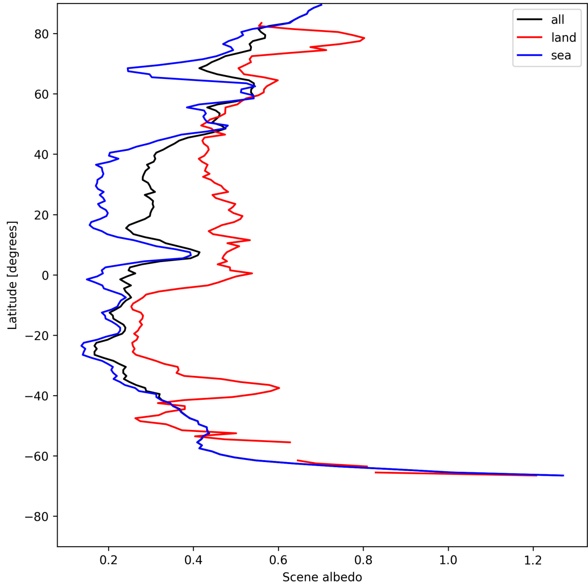
Figure 15: Zonal average of “Scene albedo” for 2025-07-15 to 2025-07-16.
