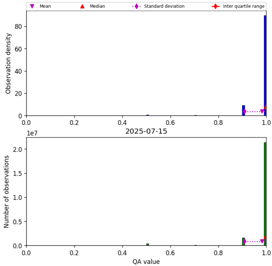
Figure 27: Histogram of “QA value” for 2025-07-15 to 2025-07-16
