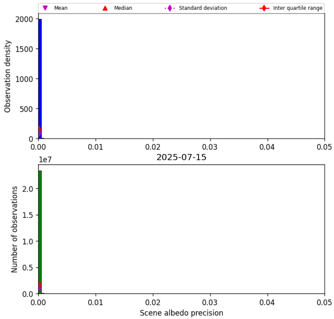
Figure 33: Histogram of “Scene albedo precision” for 2025-07-15 to 2025-07-16
