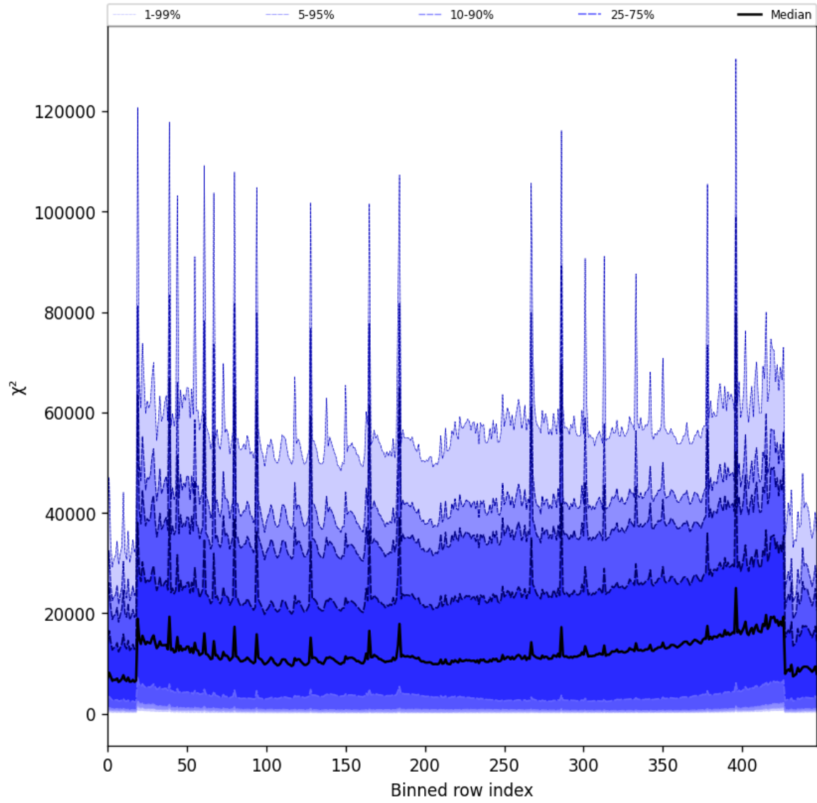
Figure 53: Along track statistics of “ \chi^2 ” for 2025-07-15 to 2025-07-16
