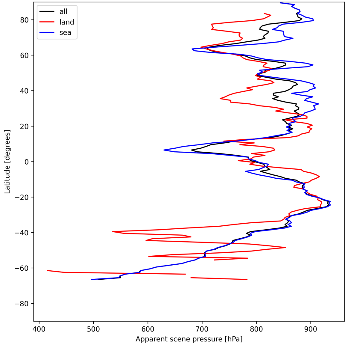
Figure 17: Zonal average of “Apparent scene pressure” for 2025-07-15 to 2025-07-16.
