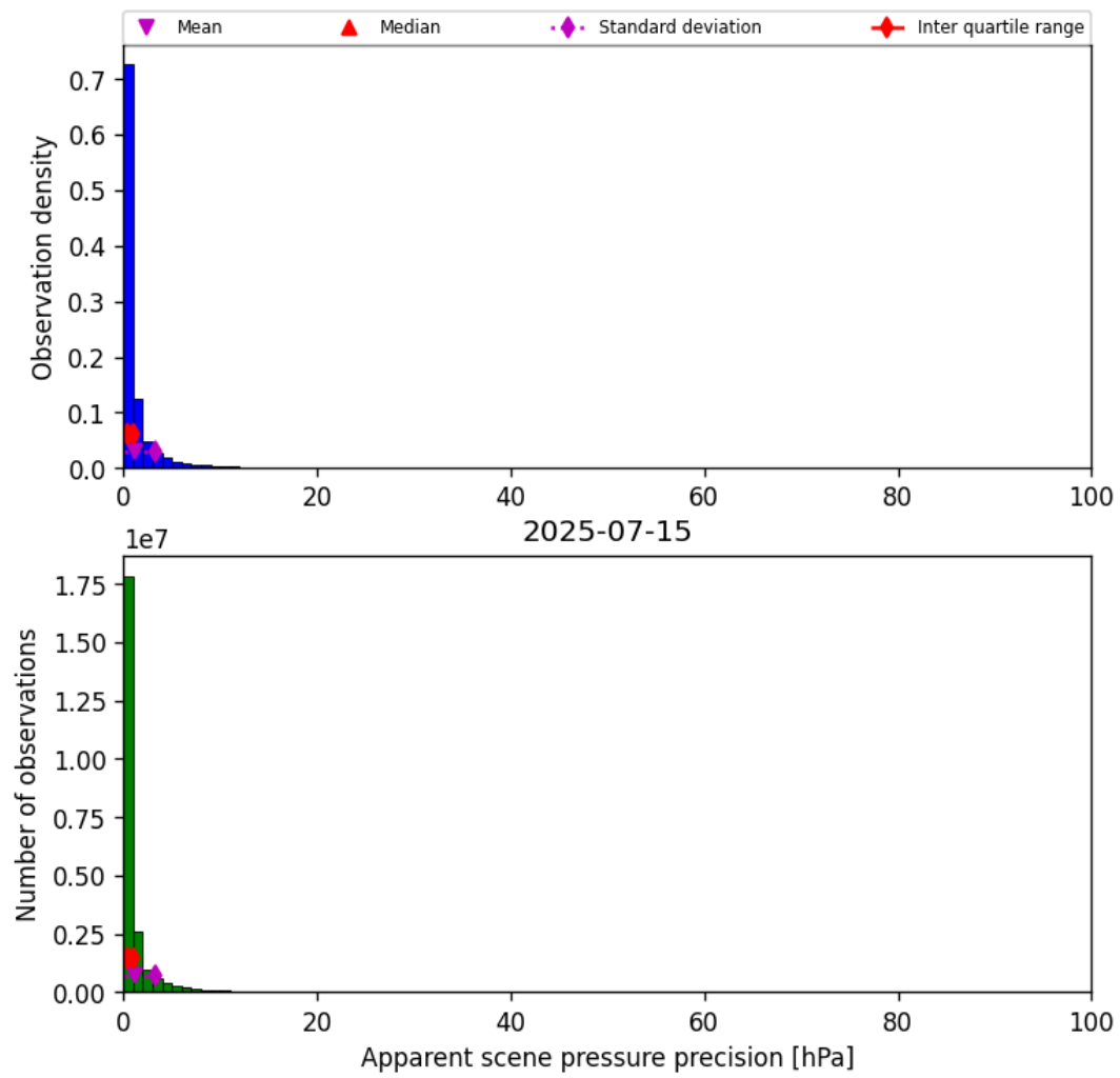
Figure 35: Histogram of “Apparent scene pressure precision” for 2025-07-15 to 2025-07-16
