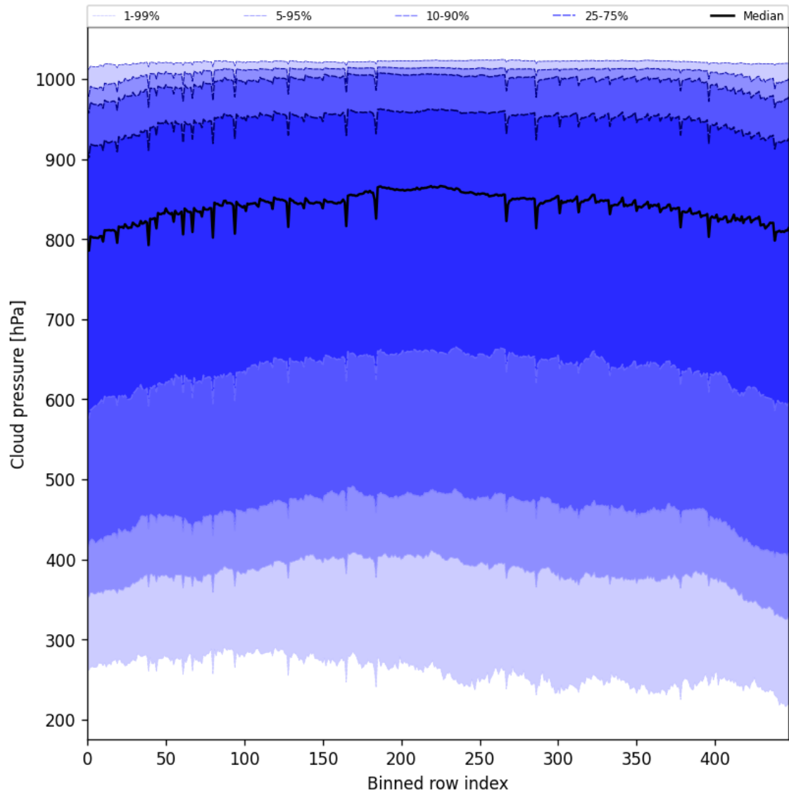
Figure 45: Along track statistics of “Cloud pressure” for 2025-07-15 to 2025-07-16
