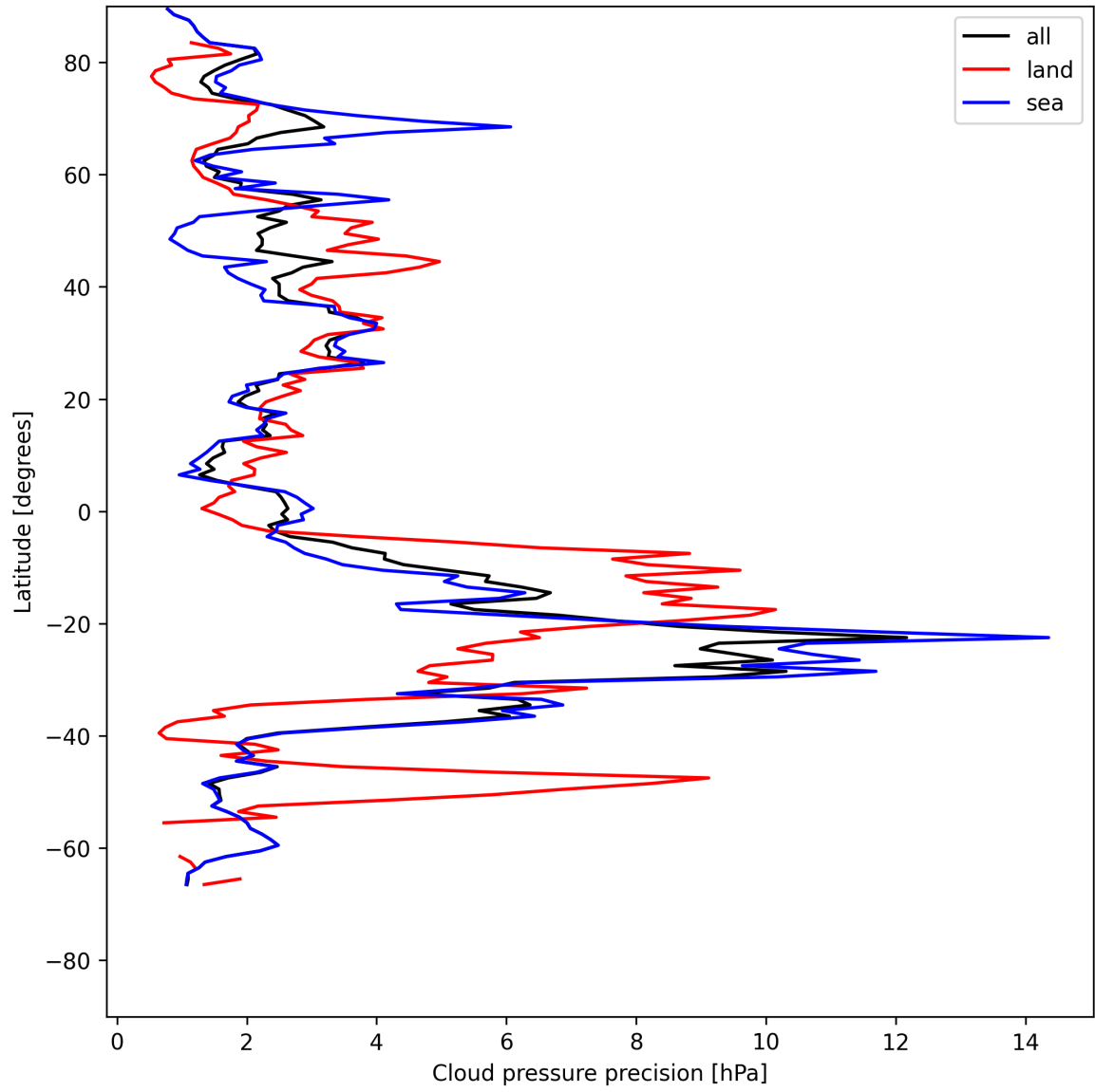
Figure 12: Zonal average of “Cloud pressure precision” for 2025-07-15 to 2025-07-16.
