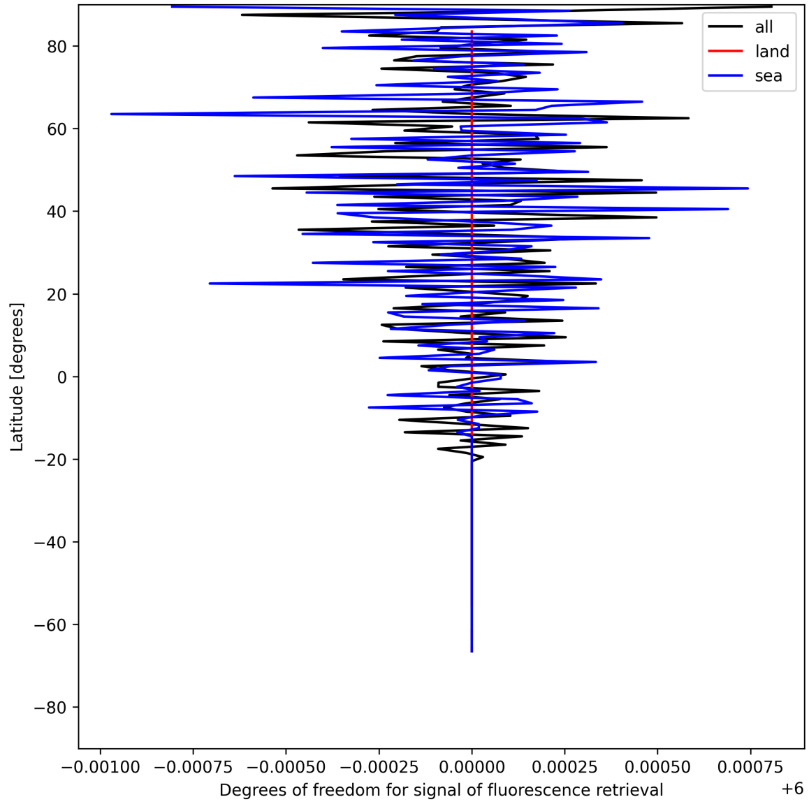
Figure 24: Zonal average of “Degrees of freedom for signal of fluorescence retrieval” for 2025-07-15 to 2025-07-16.
