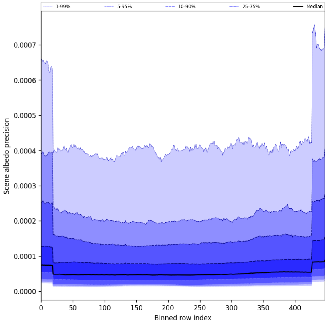
Figure 50: Along track statistics of “Scene albedo precision” for 2025-07-15 to 2025-07-16
