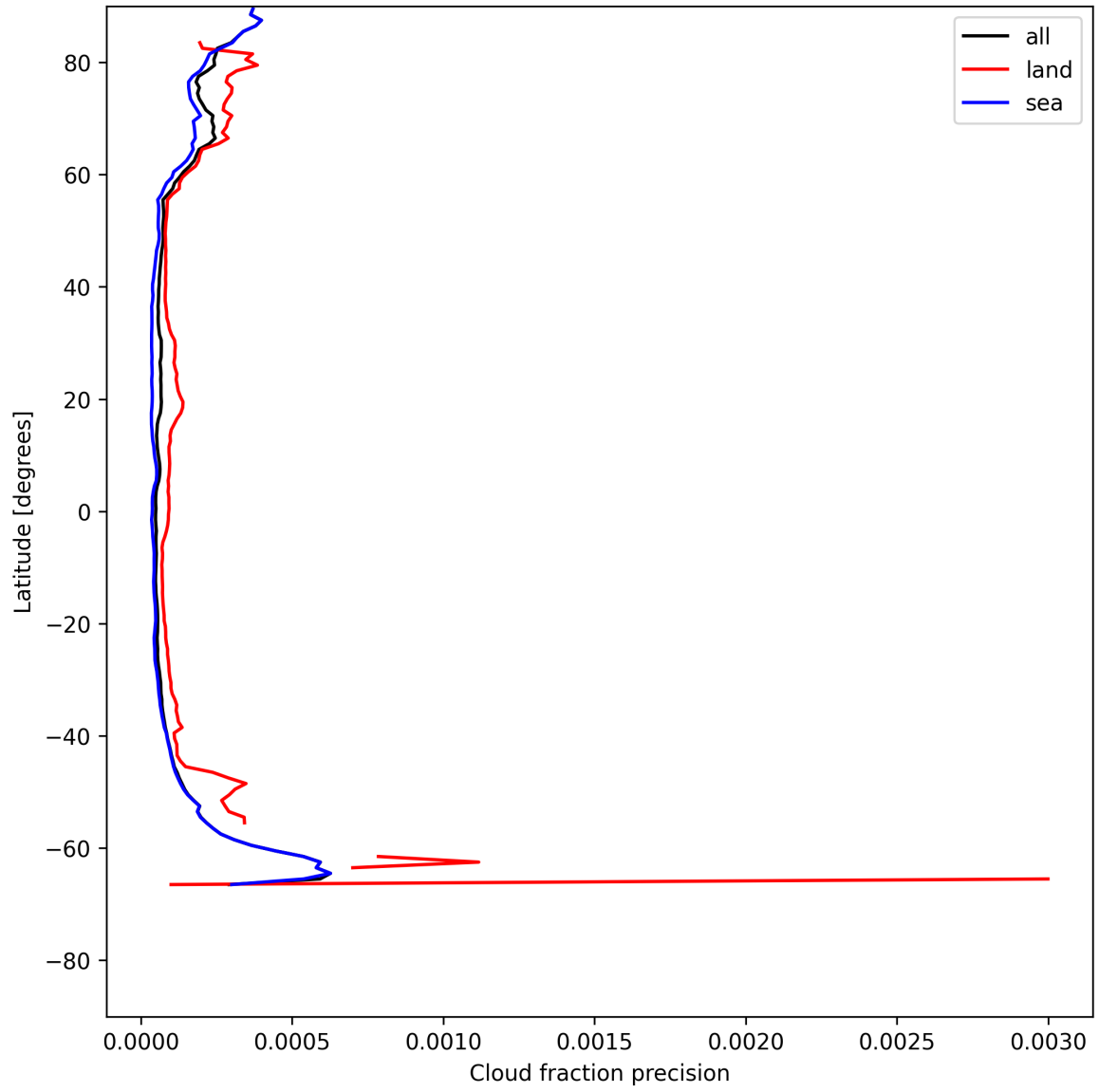
Figure 14: Zonal average of “Cloud fraction precision” for 2025-07-15 to 2025-07-16.
