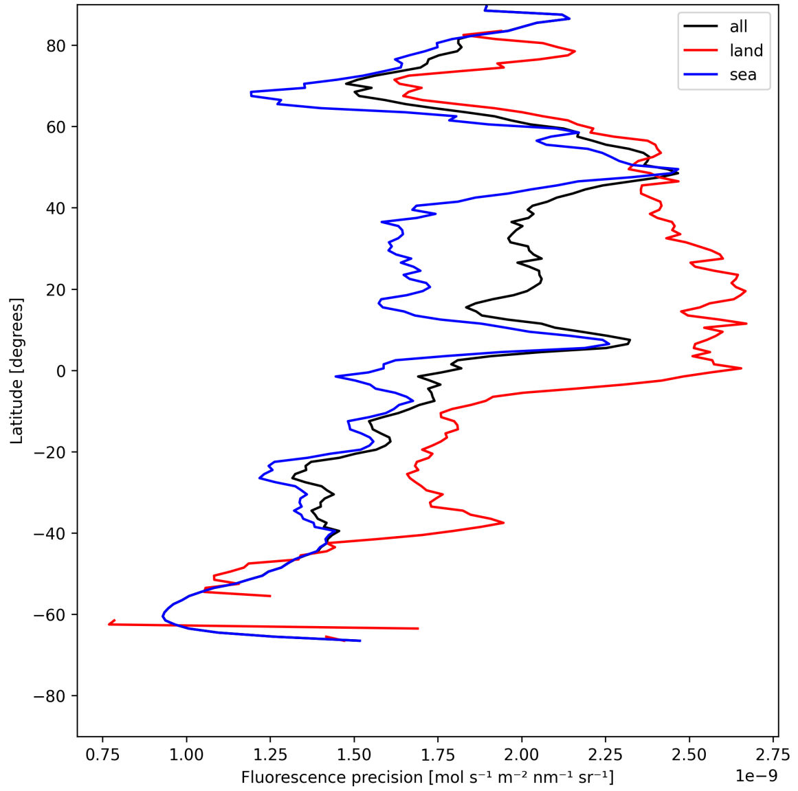
Figure 22: Zonal average of “Fluorescence precision” for 2025-07-15 to 2025-07-16.
