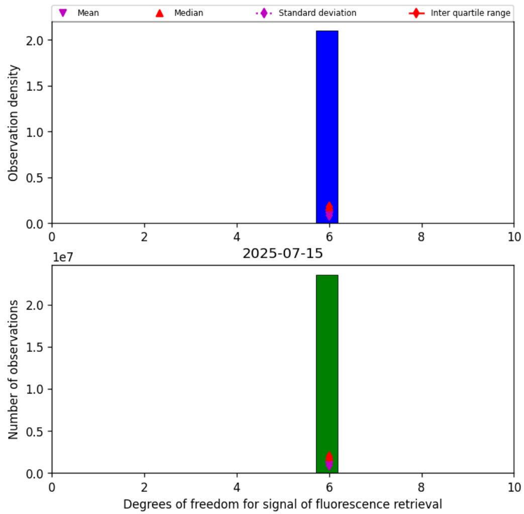
Figure 41: Histogram of “Degrees of freedom for signal of fluorescence retrieval” for 2025-07-15 to 2025-07-16
