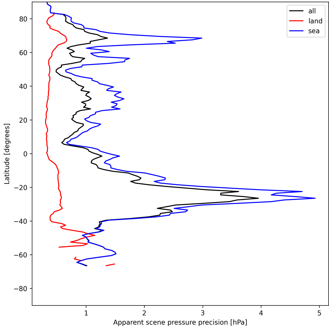
Figure 18: Zonal average of “Apparent scene pressure precision” for 2025-07-15 to 2025-07-16.
