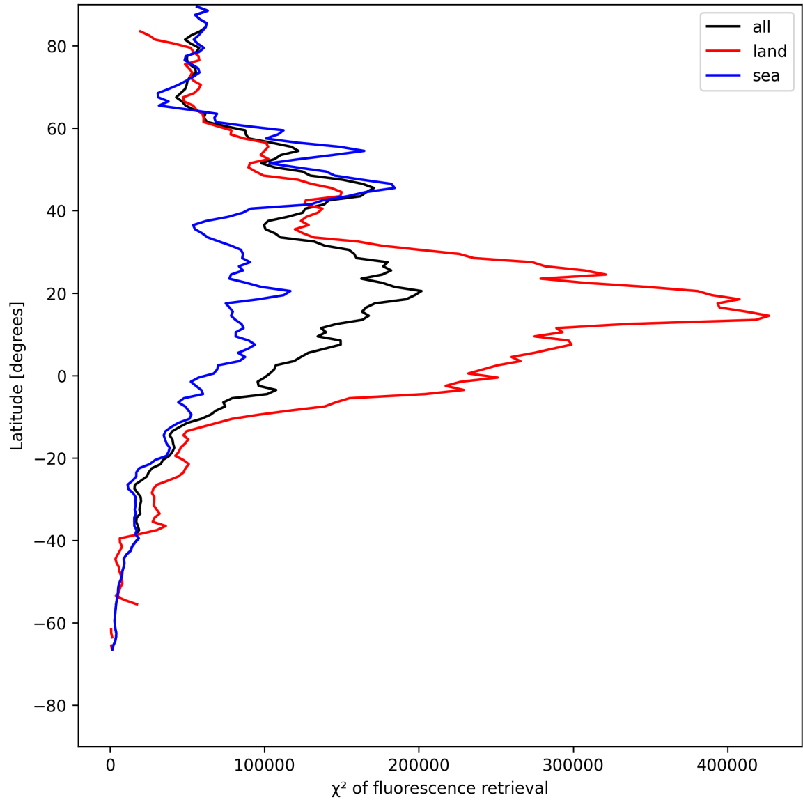
Figure 23: Zonal average of “ \chi^2 of fluorescence retrieval” for 2025-07-15 to 2025-07-16.
