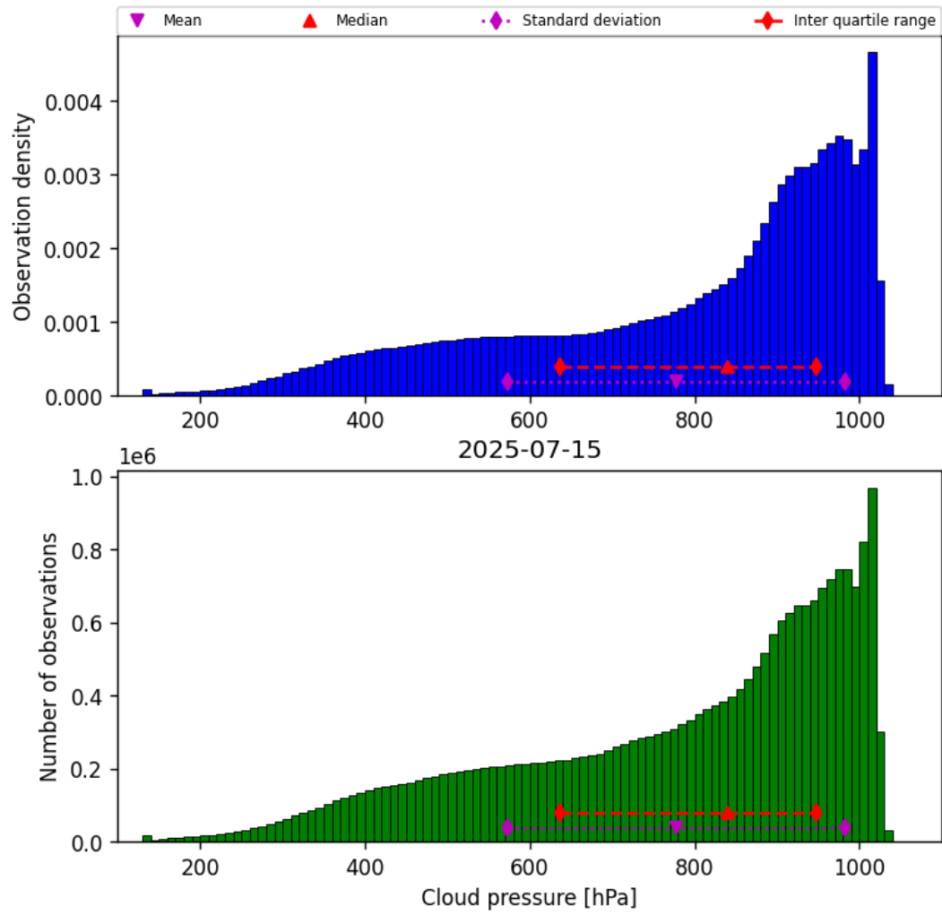
Figure 28: Histogram of “Cloud pressure” for 2025-07-15 to 2025-07-16
