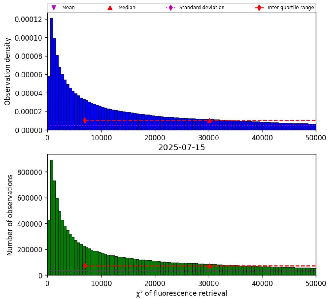
Figure 40: Histogram of “ \chi^2 of fluorescence retrieval” for 2025-07-15 to 2025-07-16
