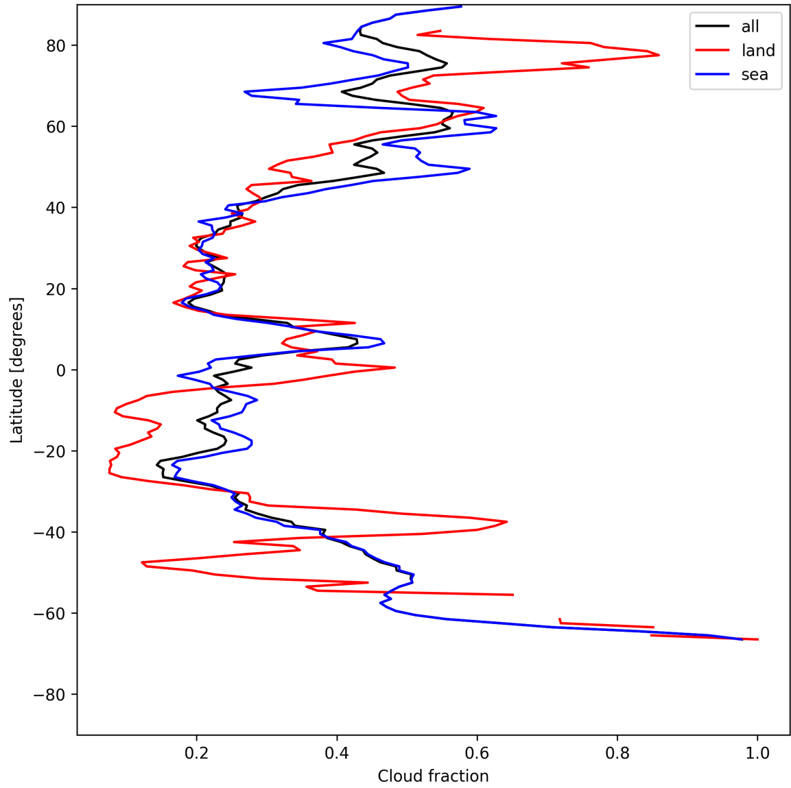
Figure 13: Zonal average of “Cloud fraction” for 2025-07-15 to 2025-07-16.
