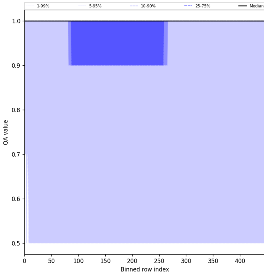
Figure 44: Along track statistics of “QA value” for 2025-07-15 to 2025-07-16
