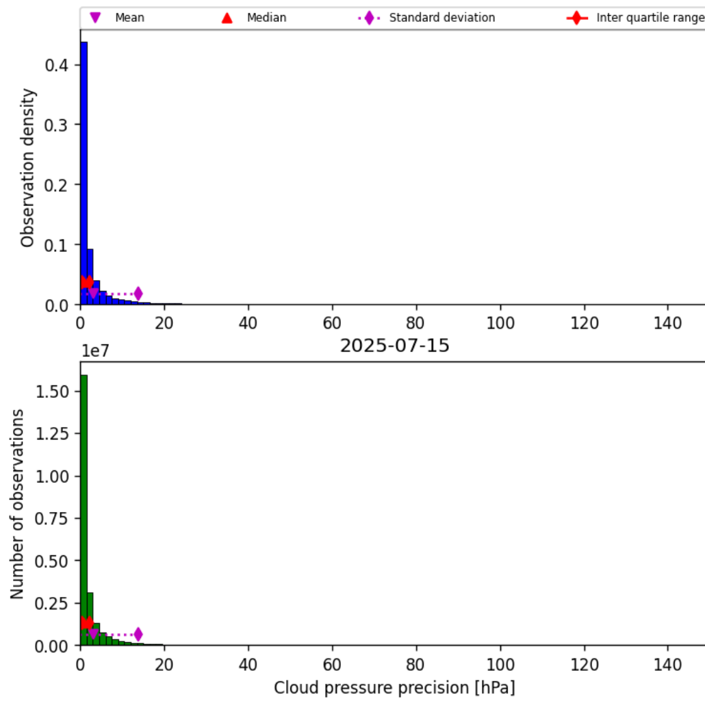
Figure 29: Histogram of “Cloud pressure precision” for 2025-07-15 to 2025-07-16
