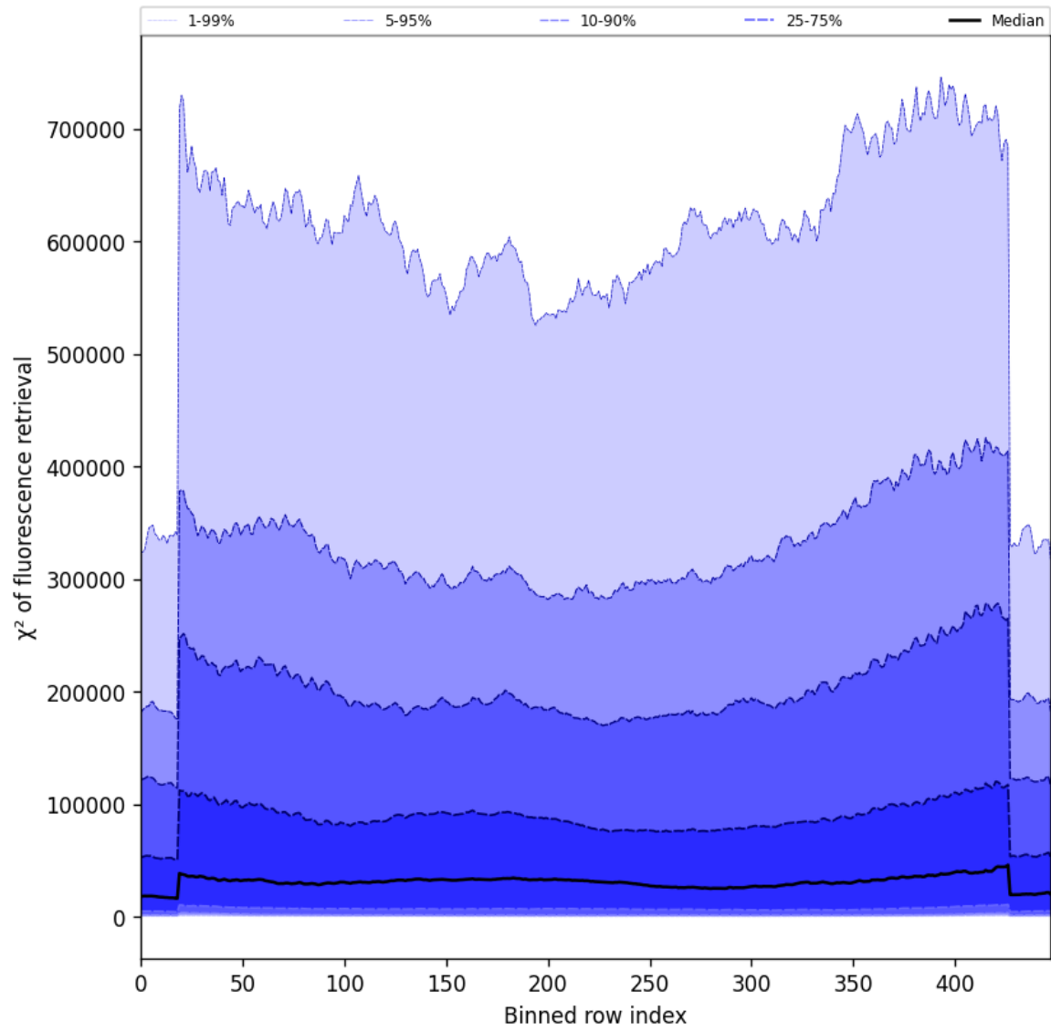
Figure 57: Along track statistics of “ \chi^2 of fluorescence retrieval” for 2025-07-15 to 2025-07-16
