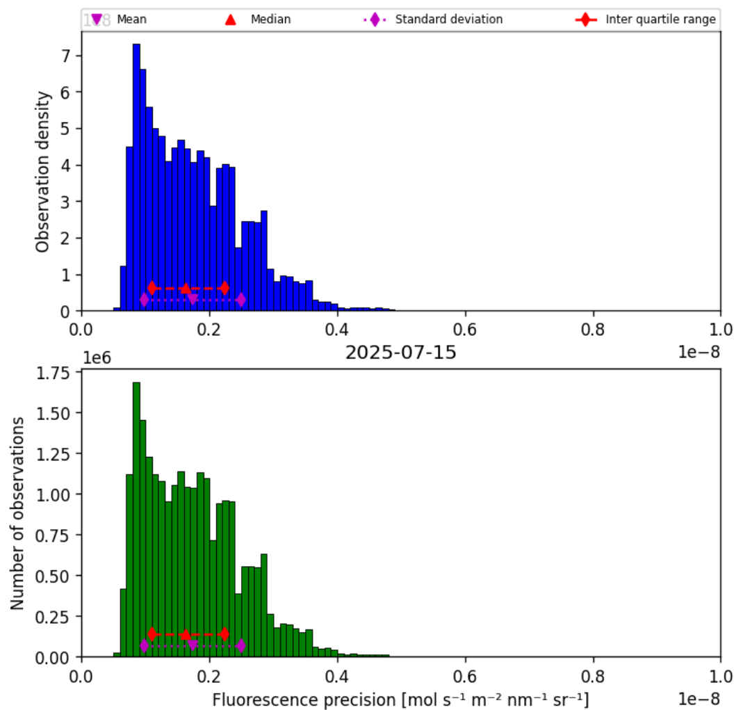
Figure 39: Histogram of “Fluorescence precision” for 2025-07-15 to 2025-07-16
