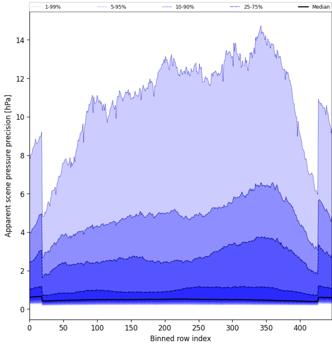
Figure 52: Along track statistics of “Apparent scene pressure precision” for 2025-07-15 to 2025-07-16
