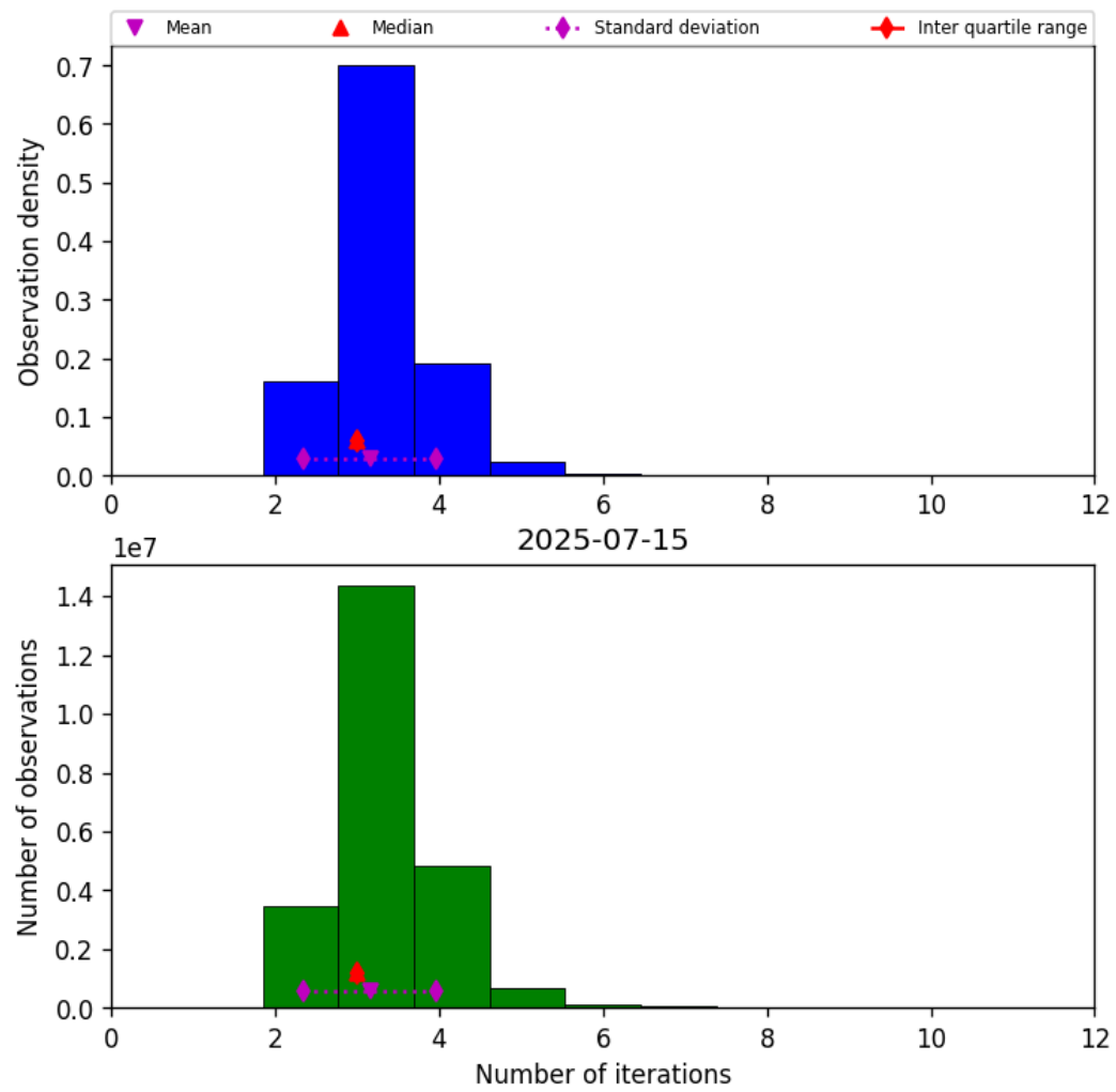
Figure 37: Histogram of “Number of iterations” for 2025-07-15 to 2025-07-16
