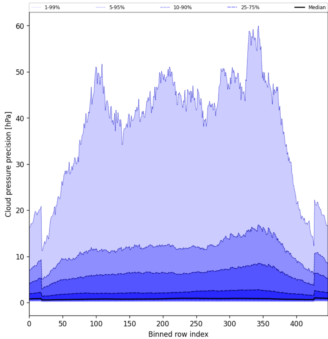
Figure 46: Along track statistics of “Cloud pressure precision” for 2025-07-15 to 2025-07-16
