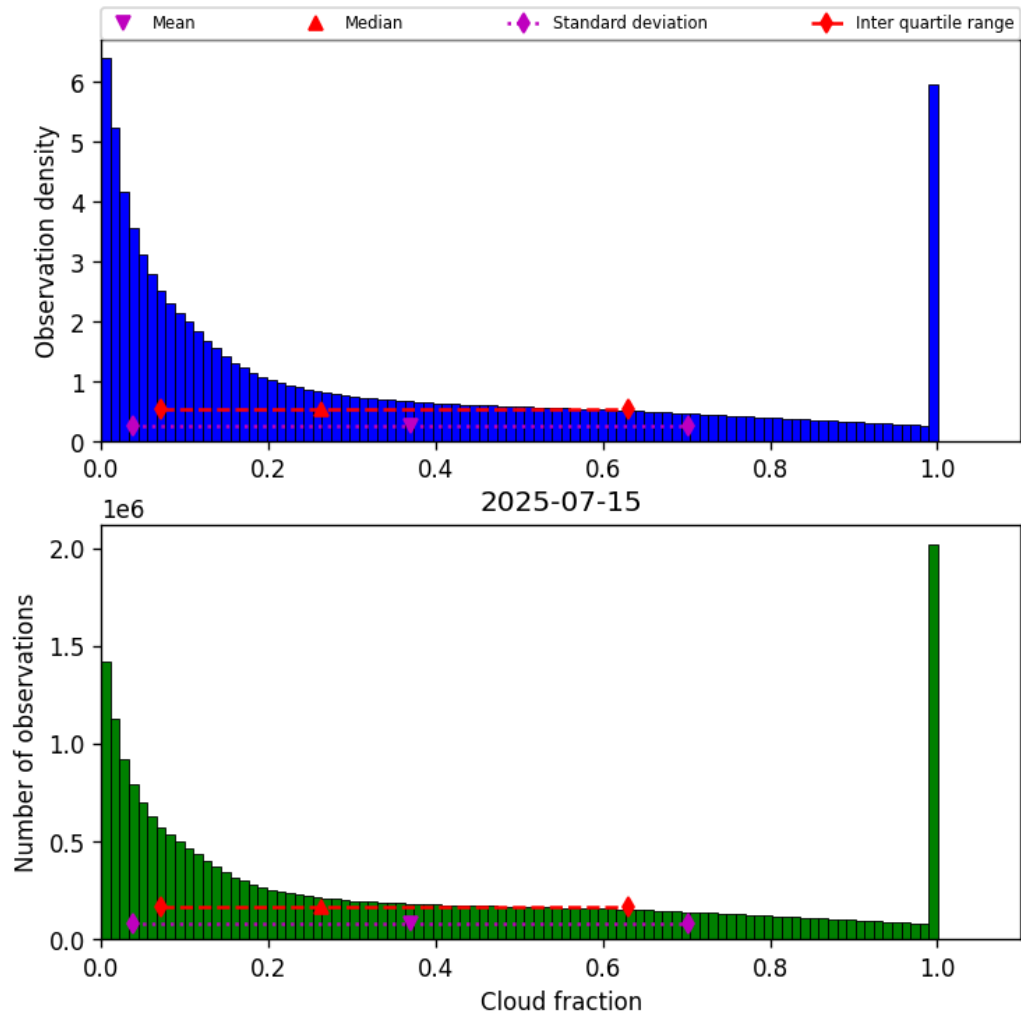
Figure 30: Histogram of “Cloud fraction” for 2025-07-15 to 2025-07-16
