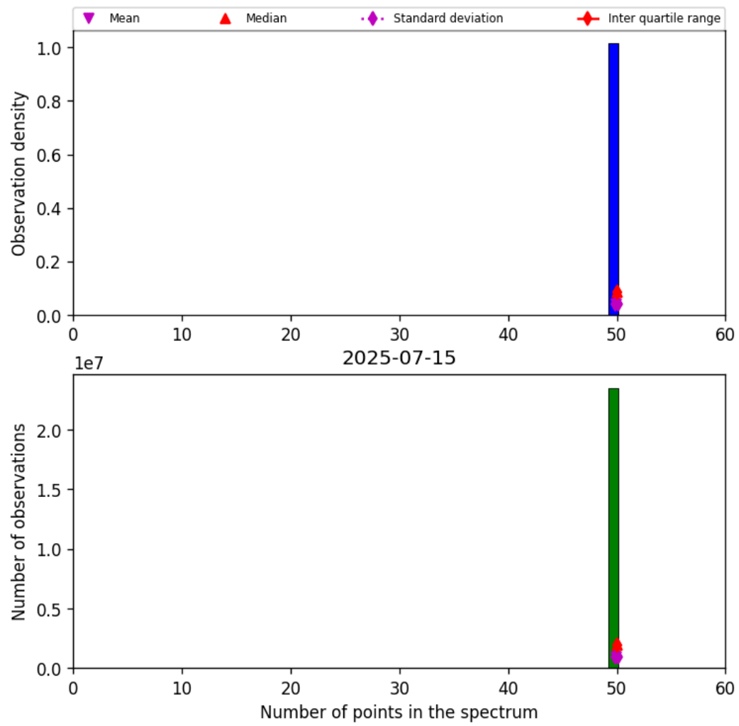
Figure 42: Histogram of “Number of points in the spectrum” for 2025-07-15 to 2025-07-16
