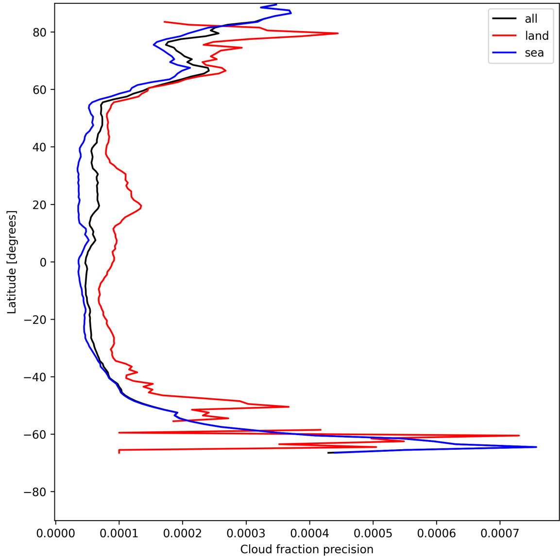
Figure 14: Zonal average of “Cloud fraction precision” for 2025-07-16 to 2025-07-16.
