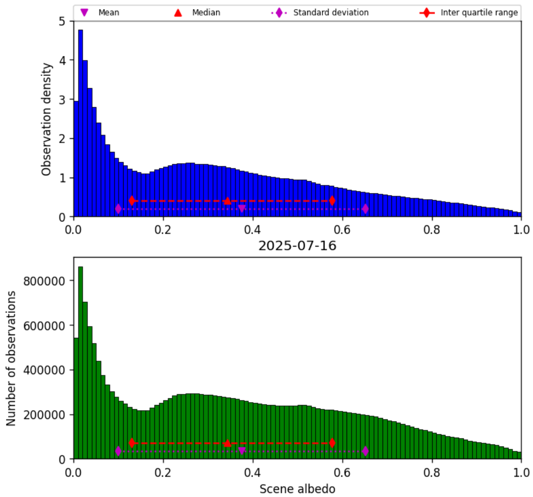
Figure 32: Histogram of “Scene albedo” for 2025-07-16 to 2025-07-16
