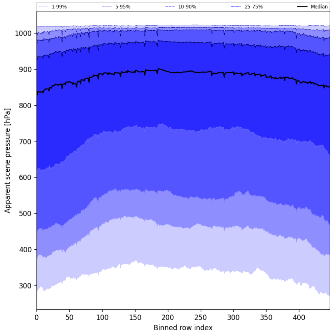
Figure 51: Along track statistics of “Apparent scene pressure” for 2025-07-16 to 2025-07-16
