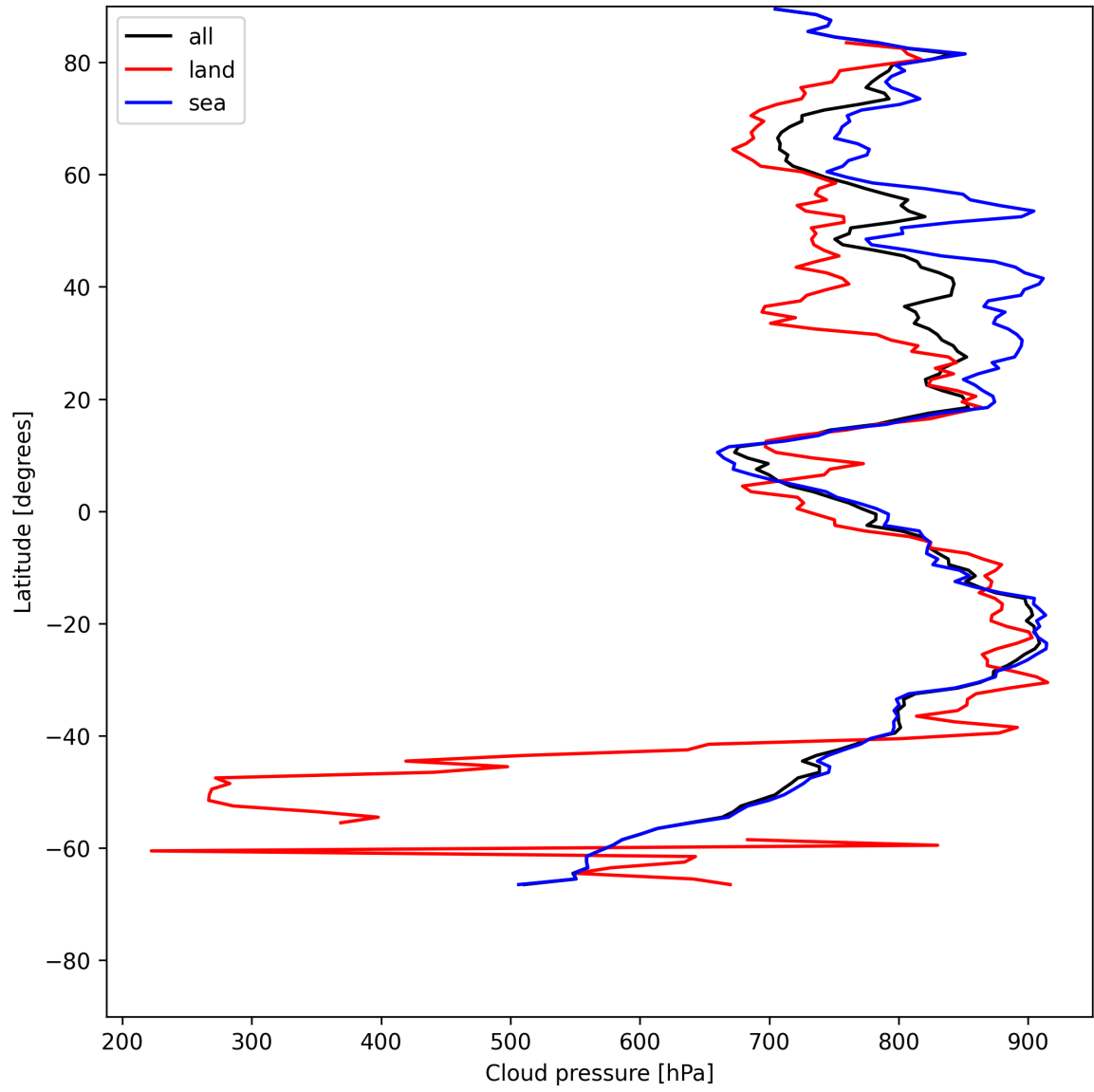
Figure 11: Zonal average of “Cloud pressure” for 2025-07-16 to 2025-07-16.
