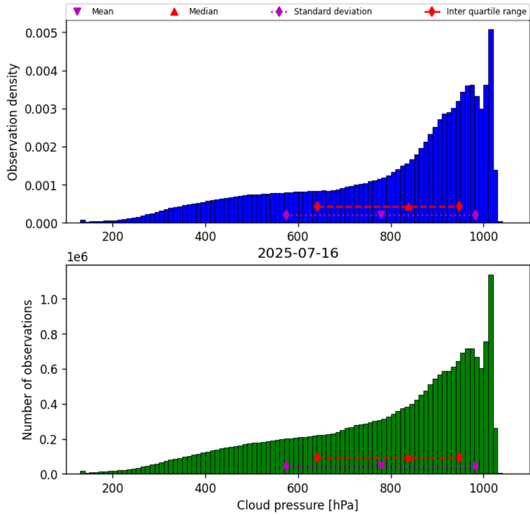
Figure 28: Histogram of “Cloud pressure” for 2025-07-16 to 2025-07-16
