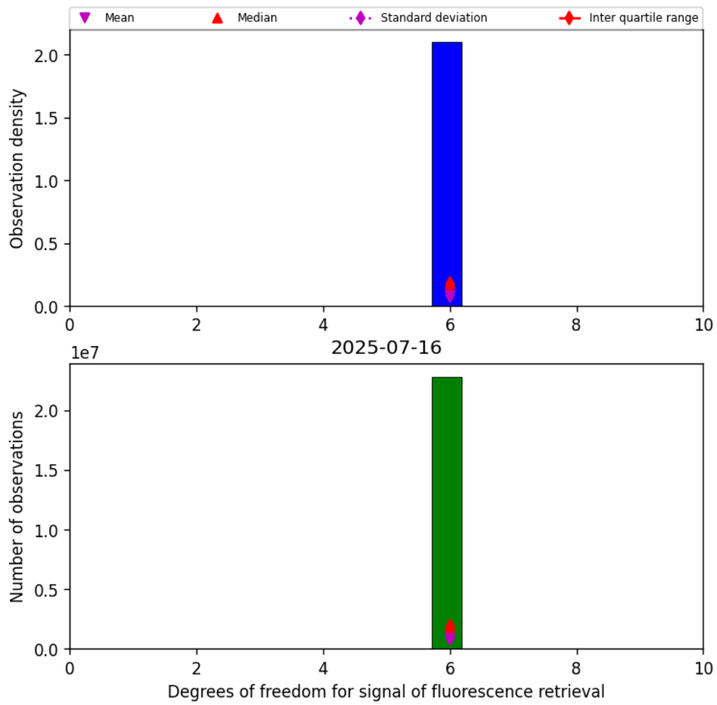
Figure 41: Histogram of “Degrees of freedom for signal of fluorescence retrieval” for 2025-07-16 to 2025-07-16
