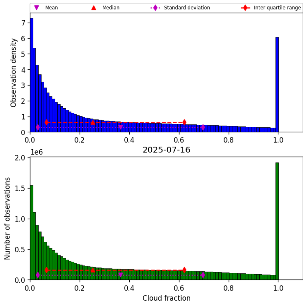
Figure 30: Histogram of “Cloud fraction” for 2025-07-16 to 2025-07-16
