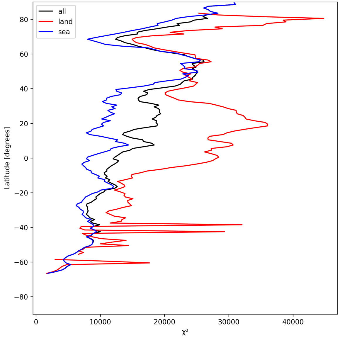
Figure 19: Zonal average of “ \chi^2 ” for 2025-07-16 to 2025-07-16.
