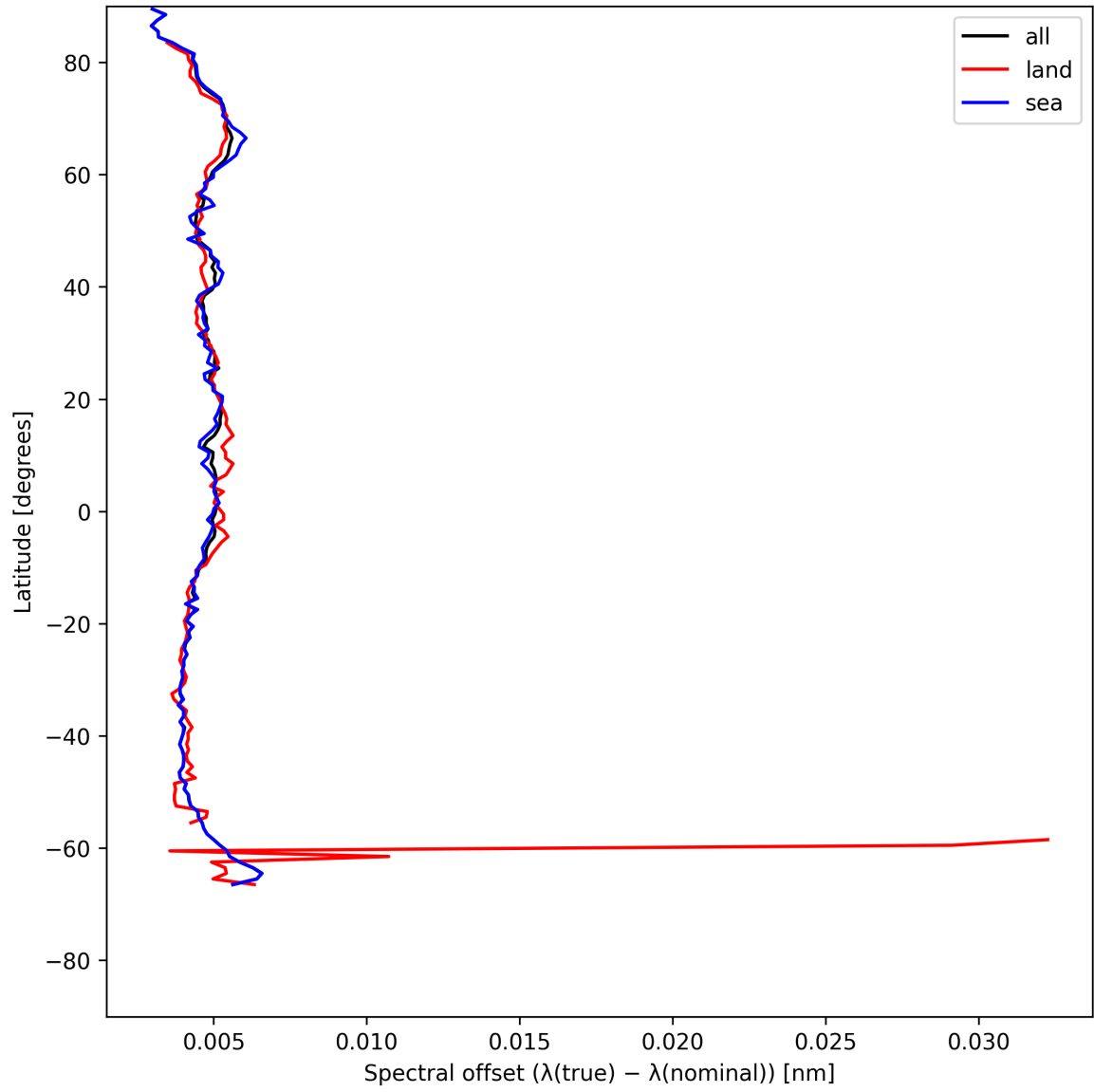
Figure 26: Zonal average of “Spectral offset ( \lambda_{\text{true}} - \lambda_{\text{nominal}} )” for 2025-07-16 to 2025-07-16.
