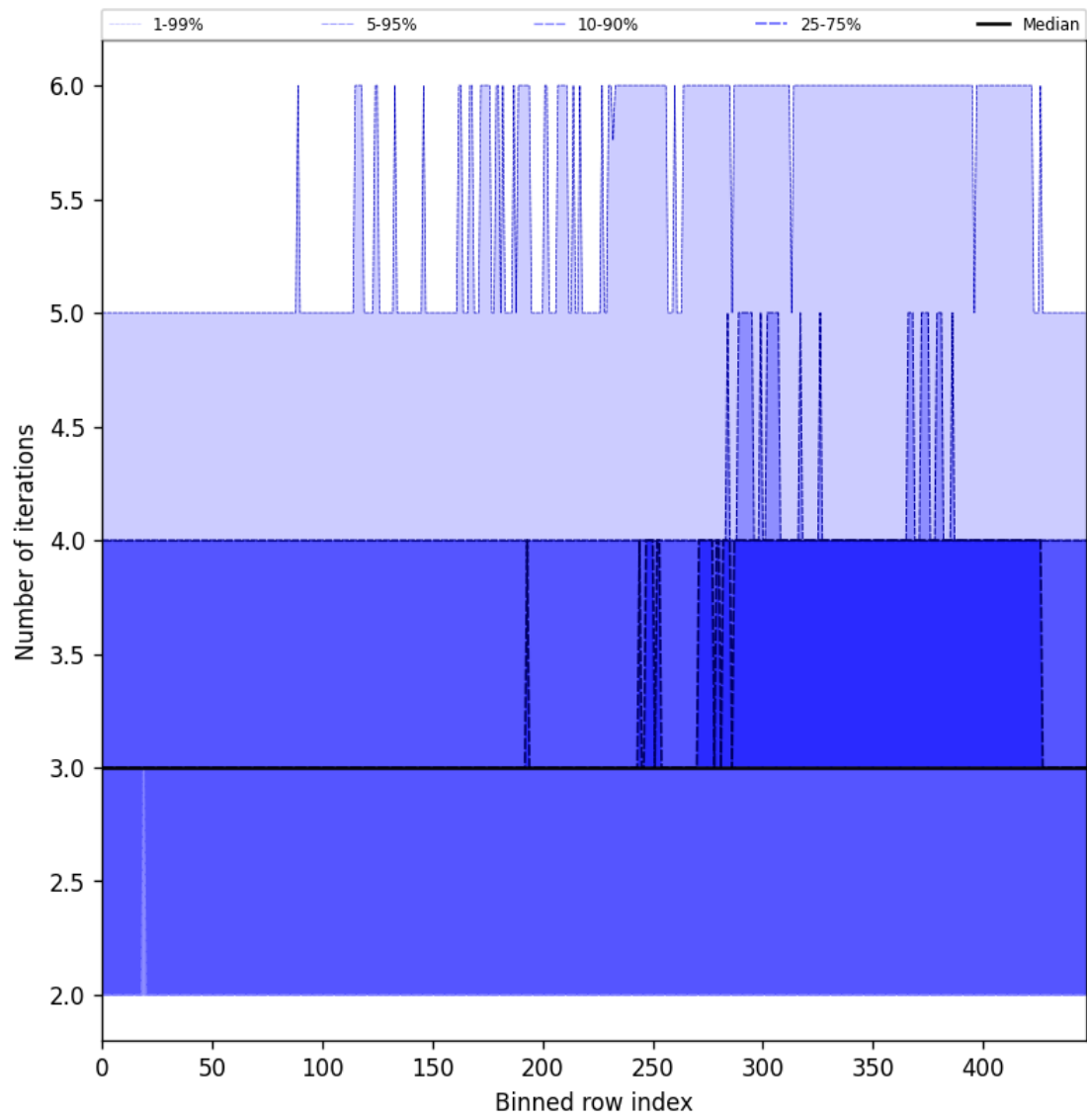
Figure 54: Along track statistics of “Number of iterations” for 2025-07-16 to 2025-07-16
