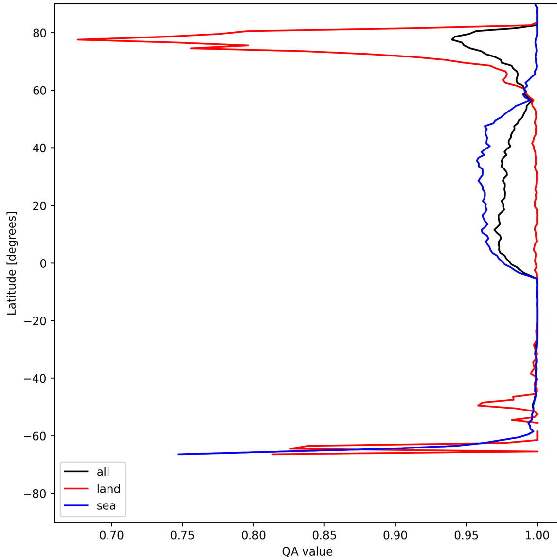
Figure 10: Zonal average of “QA value” for 2025-07-16 to 2025-07-16.
