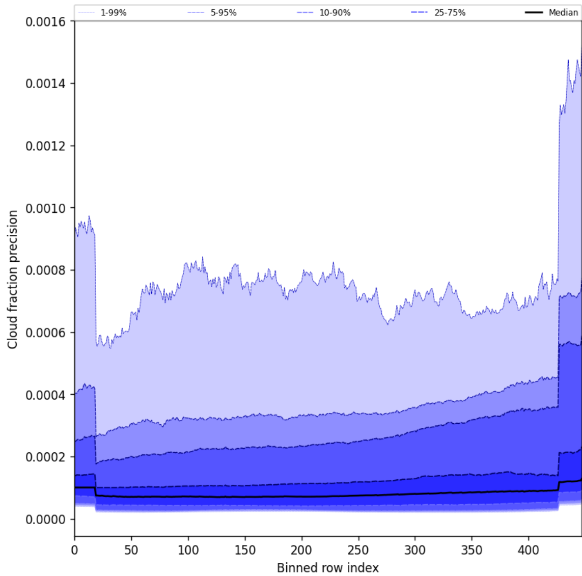
Figure 48: Along track statistics of “Cloud fraction precision” for 2025-07-16 to 2025-07-16
