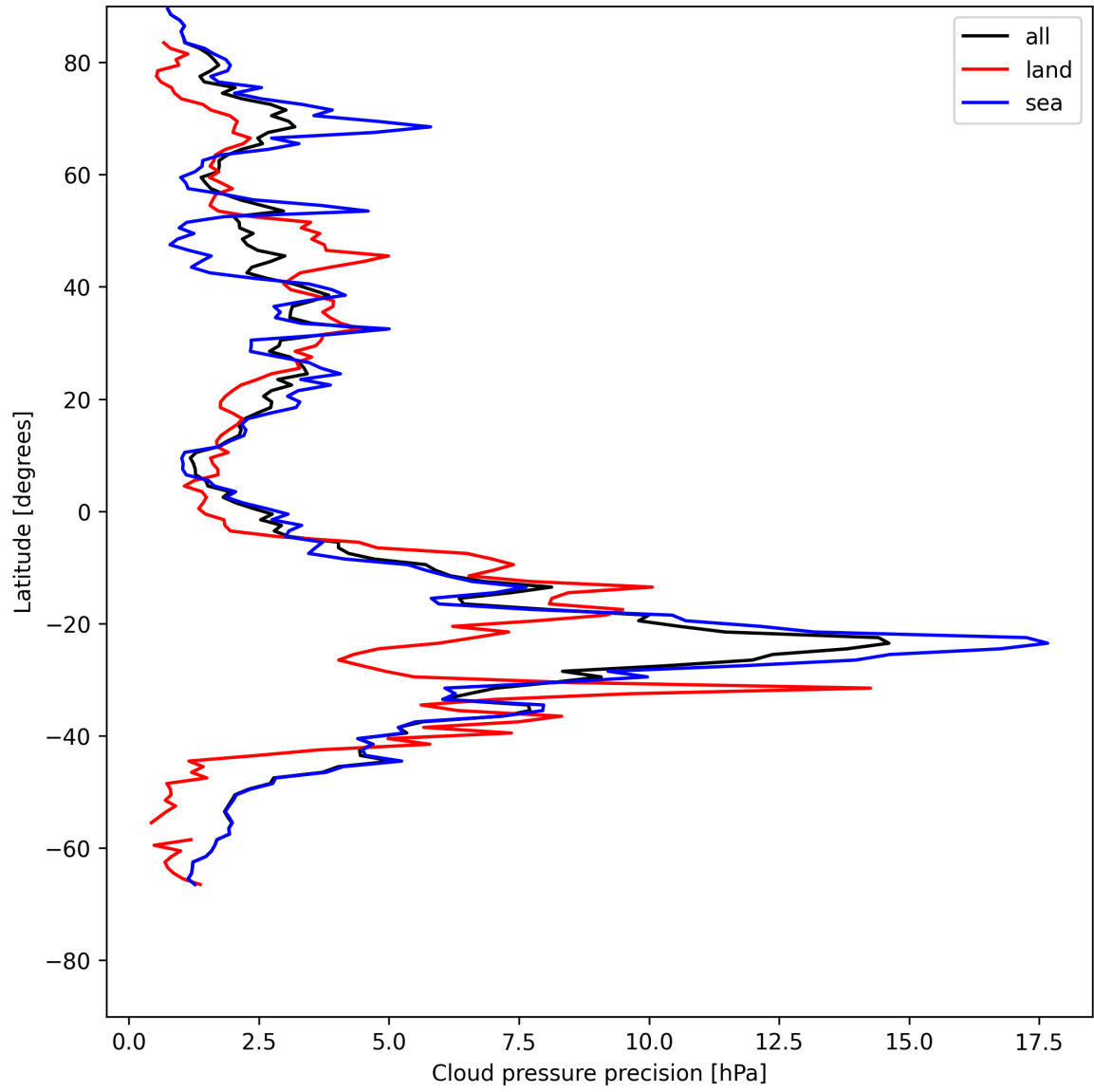
Figure 12: Zonal average of “Cloud pressure precision” for 2025-07-16 to 2025-07-16.
