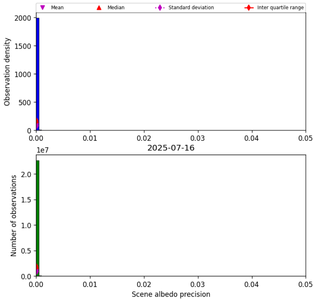
Figure 33: Histogram of “Scene albedo precision” for 2025-07-16 to 2025-07-16
