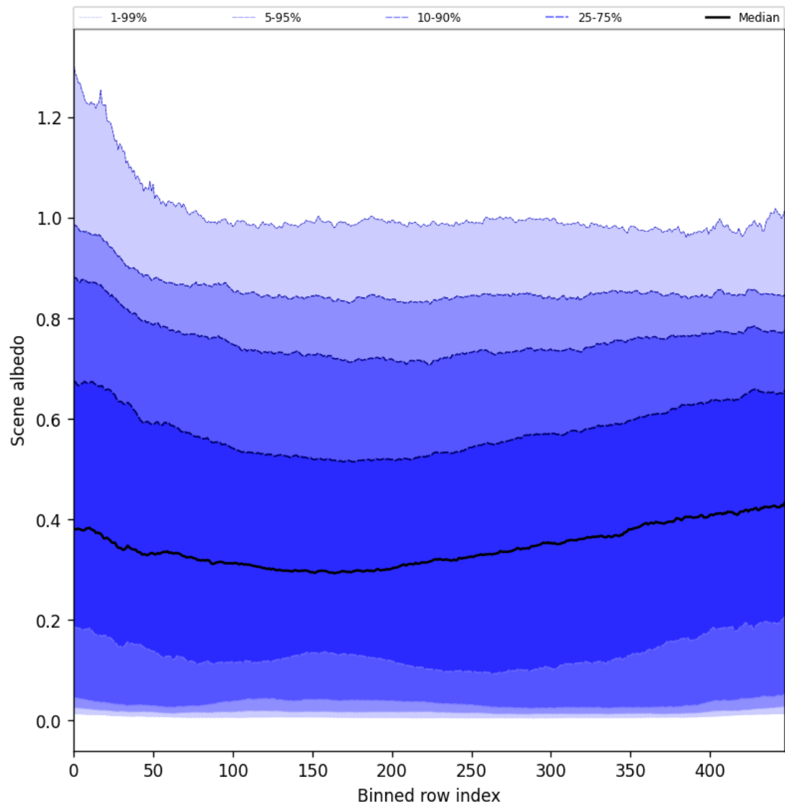
Figure 49: Along track statistics of “Scene albedo” for 2025-07-16 to 2025-07-16
