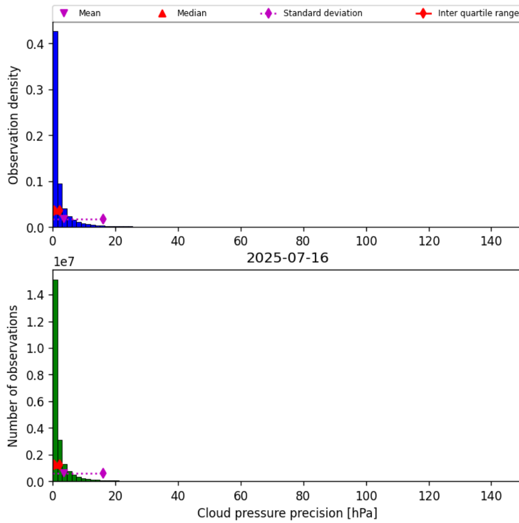
Figure 29: Histogram of “Cloud pressure precision” for 2025-07-16 to 2025-07-16
