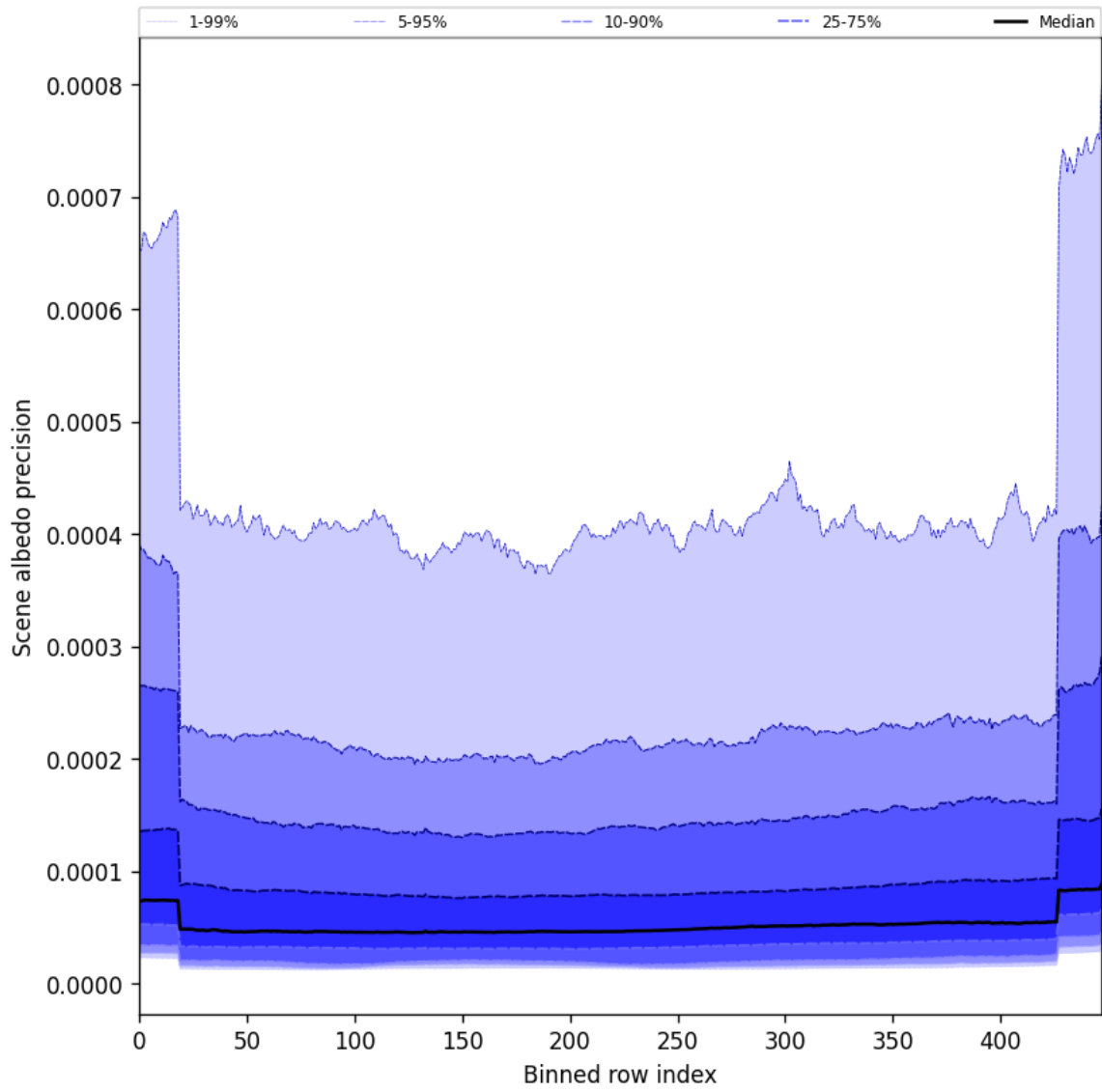
Figure 50: Along track statistics of “Scene albedo precision” for 2025-07-16 to 2025-07-16
