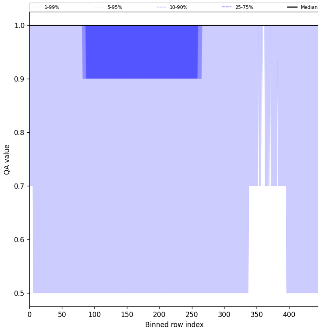
Figure 44: Along track statistics of “QA value” for 2025-07-16 to 2025-07-16
