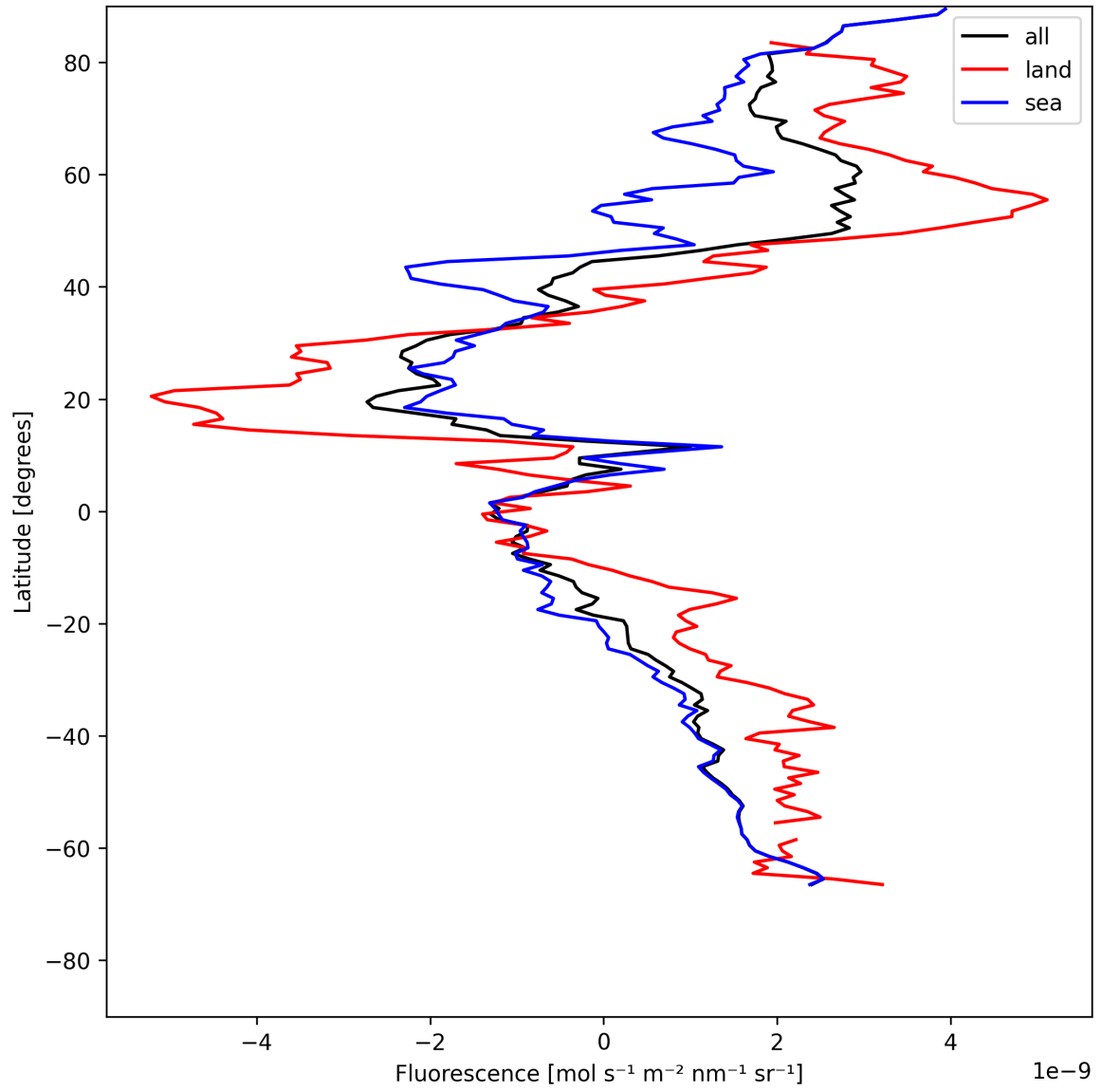
Figure 21: Zonal average of “Fluorescence” for 2025-07-16 to 2025-07-16.
