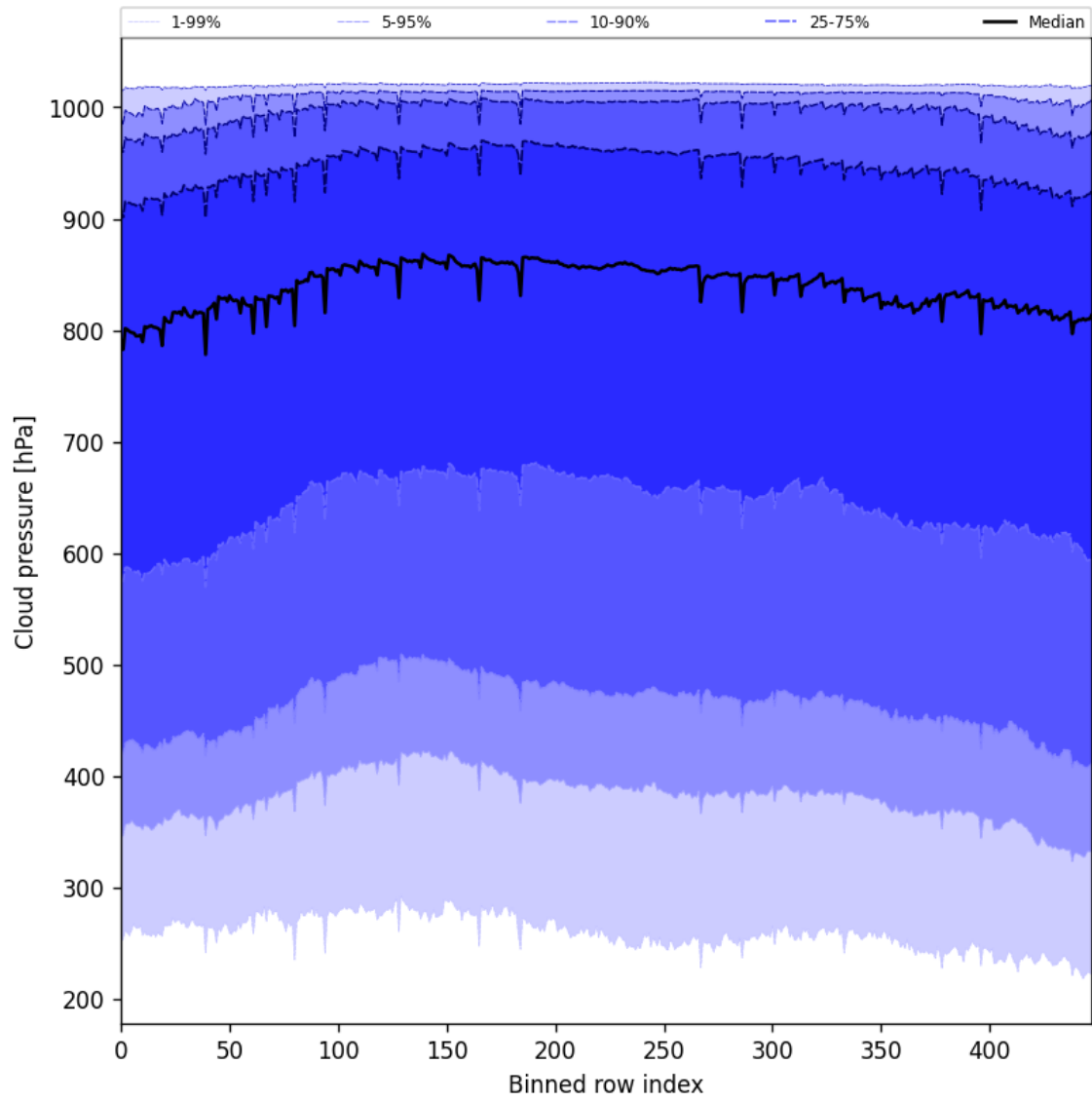
Figure 45: Along track statistics of “Cloud pressure” for 2025-07-16 to 2025-07-16
