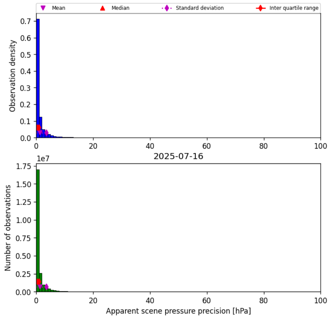
Figure 35: Histogram of “Apparent scene pressure precision” for 2025-07-16 to 2025-07-16
