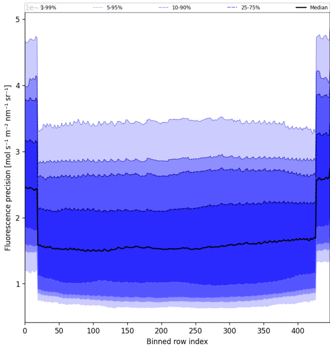
Figure 56: Along track statistics of “Fluorescence precision” for 2025-07-16 to 2025-07-16
