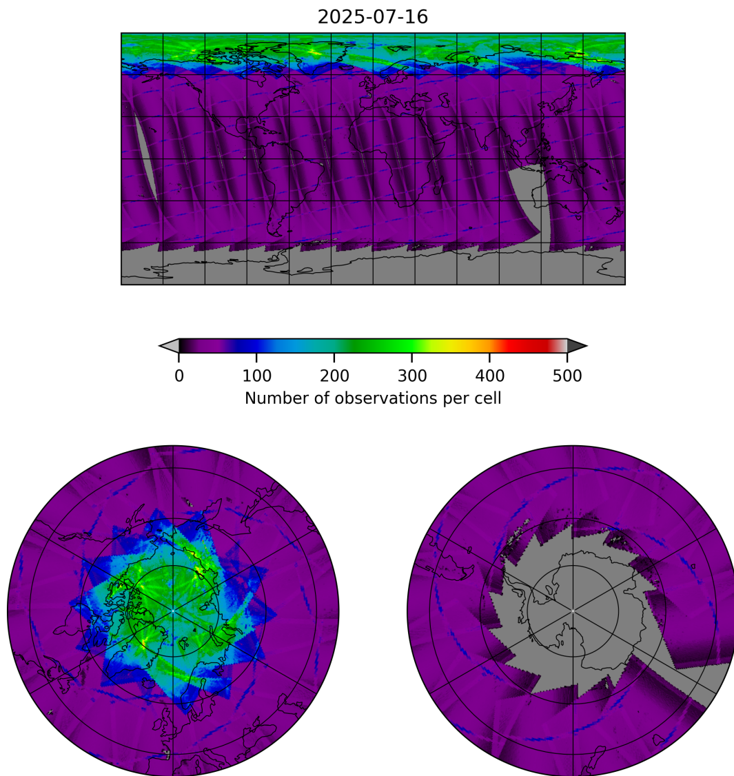
Figure 9: Map of the number of observations for 2025-07-16 to 2025-07-16
