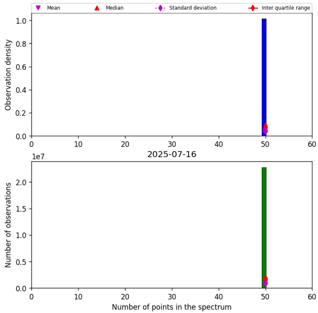
Figure 42: Histogram of "Number of points in the spectrum" for 2025-07-16 to 2025-07-16
