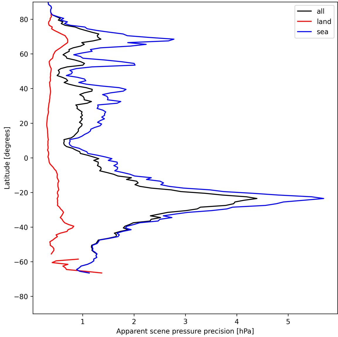
Figure 18: Zonal average of “Apparent scene pressure precision” for 2025-07-16 to 2025-07-16.
