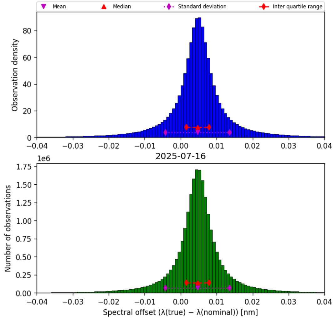
Figure 43: Histogram of “Spectral offset ( \lambda_{\text{true}} - \lambda_{\text{nominal}} )” for 2025-07-16 to 2025-07-16
