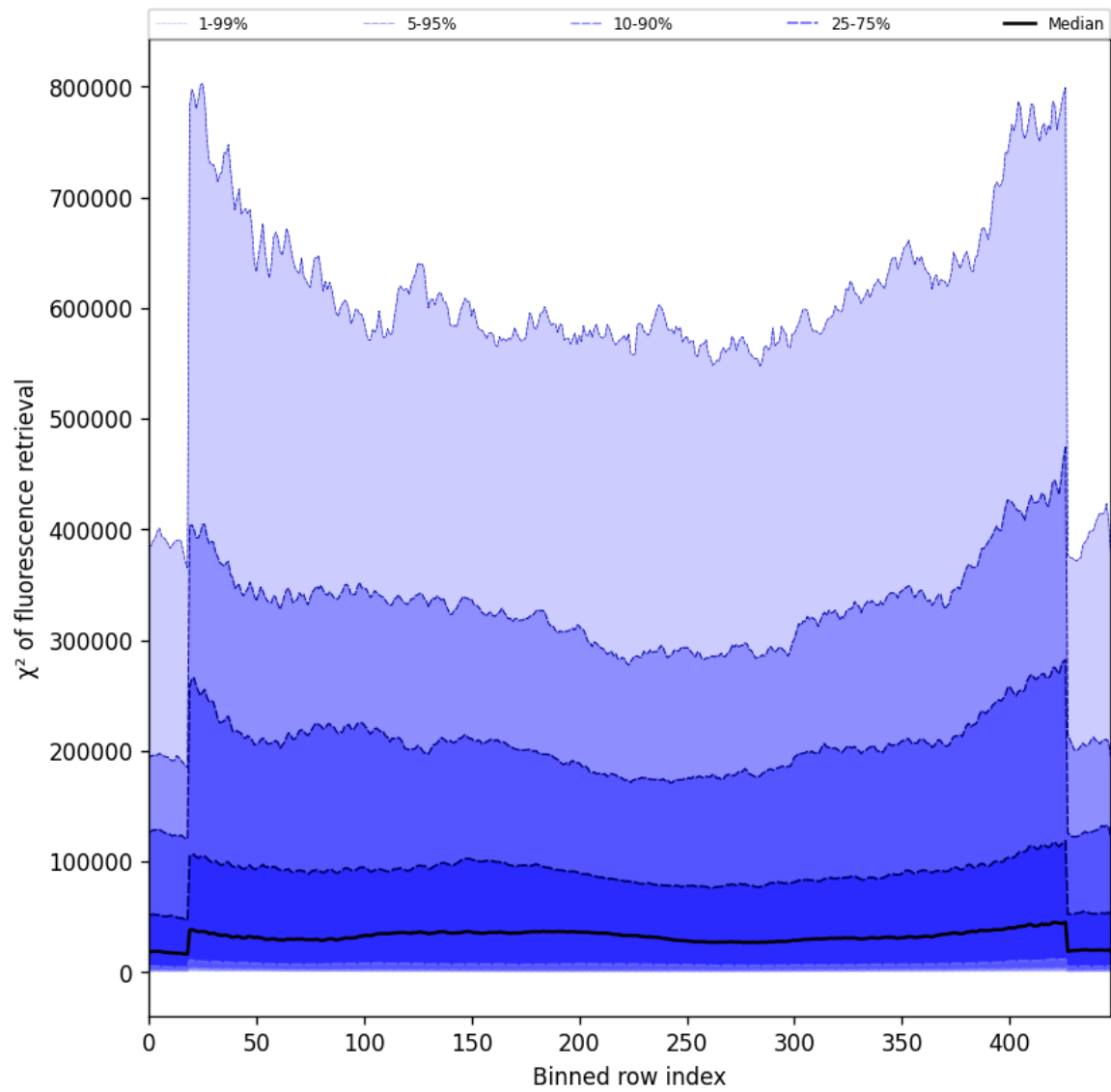
Figure 57: Along track statistics of “ \chi^2 of fluorescence retrieval” for 2025-07-16 to 2025-07-16
