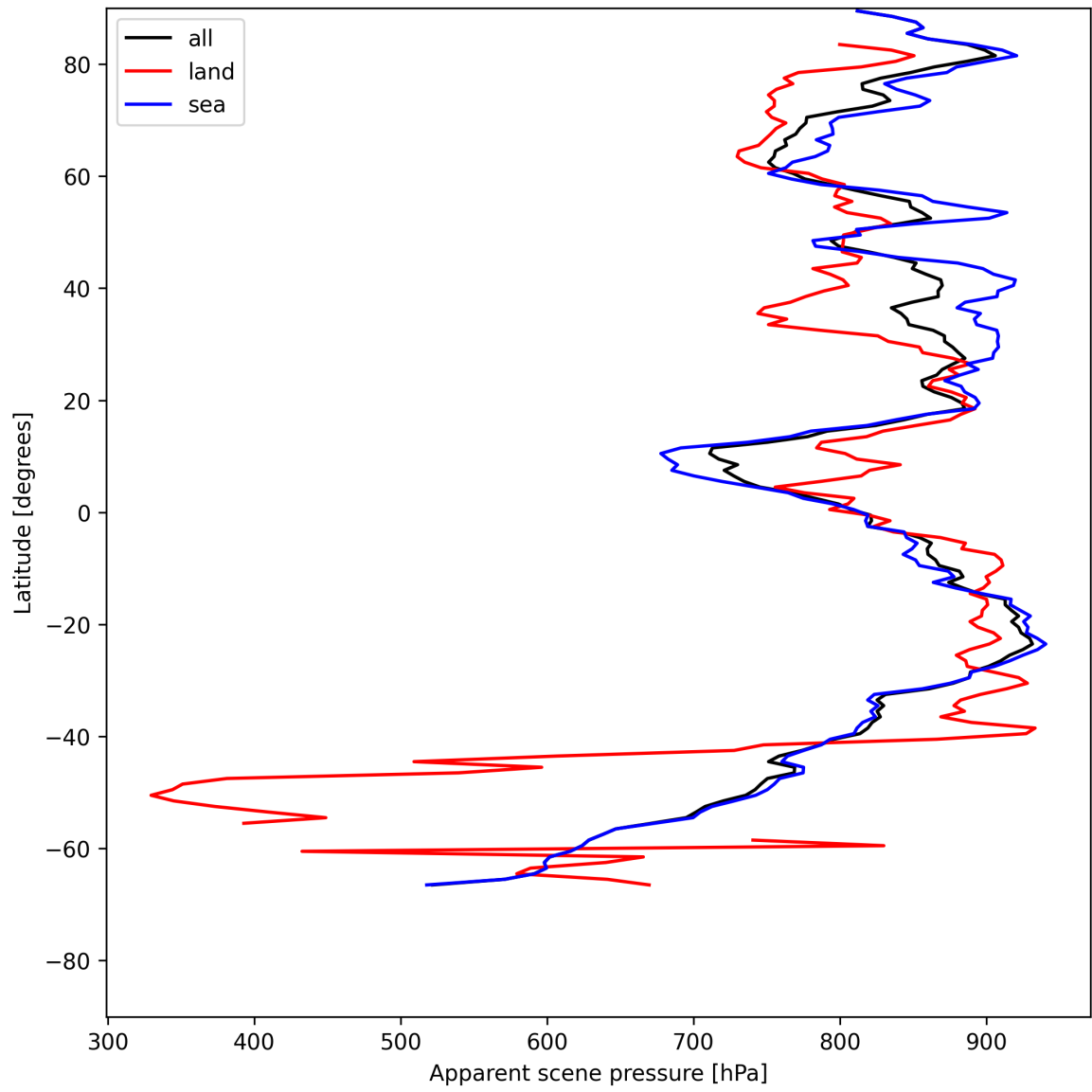
Figure 17: Zonal average of “Apparent scene pressure” for 2025-07-16 to 2025-07-16.
