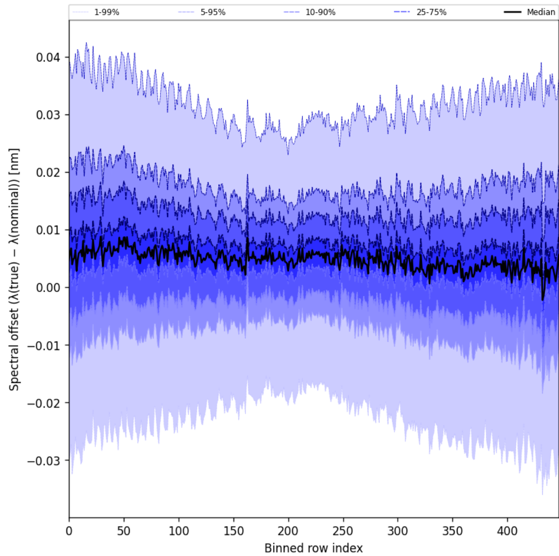
Figure 60: Along track statistics of “Spectral offset ( \lambda_{\text{true}} - \lambda_{\text{nominal}} )” for 2025-07-16 to 2025-07-16
