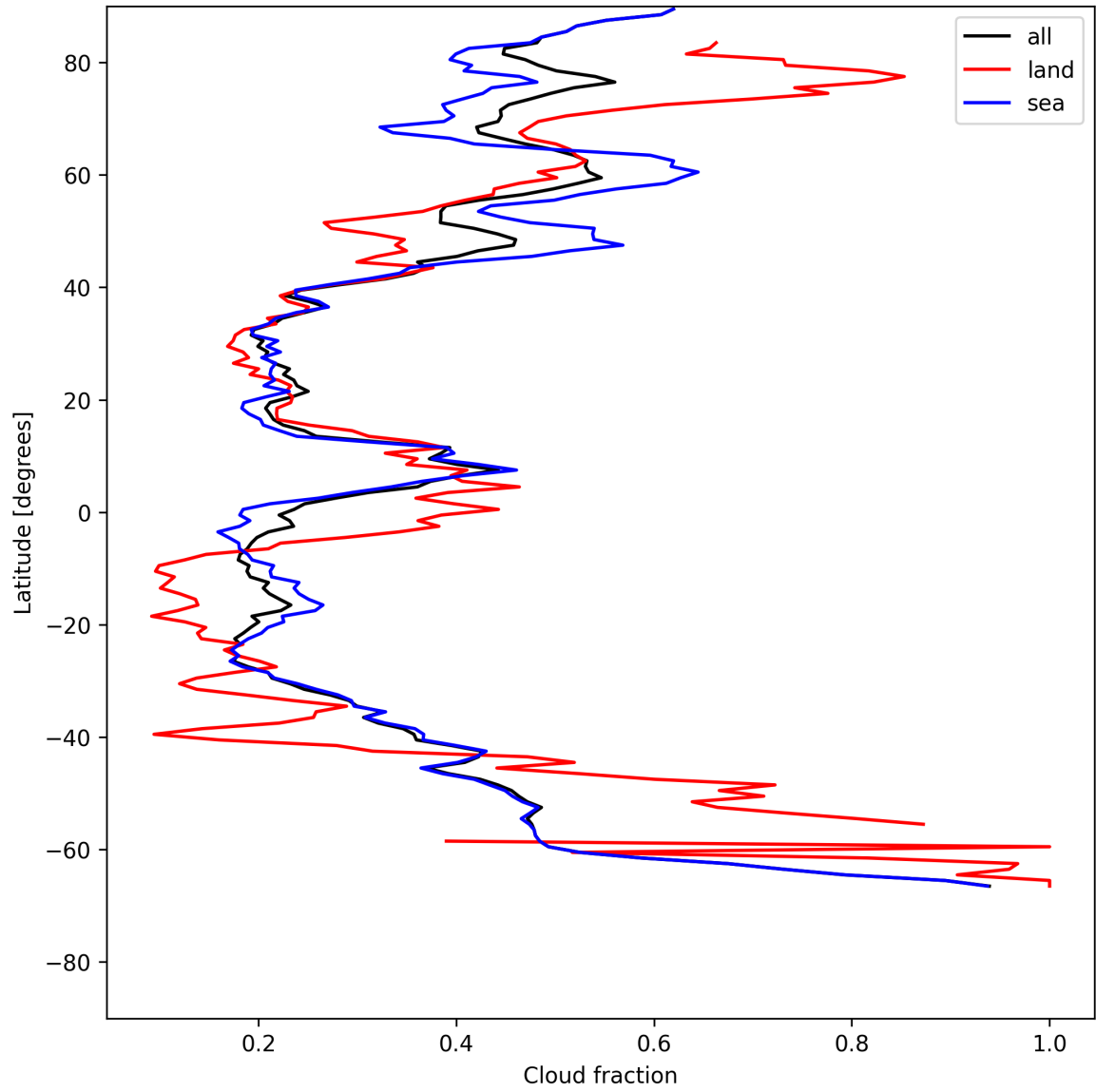
Figure 13: Zonal average of “Cloud fraction” for 2025-07-16 to 2025-07-16.
