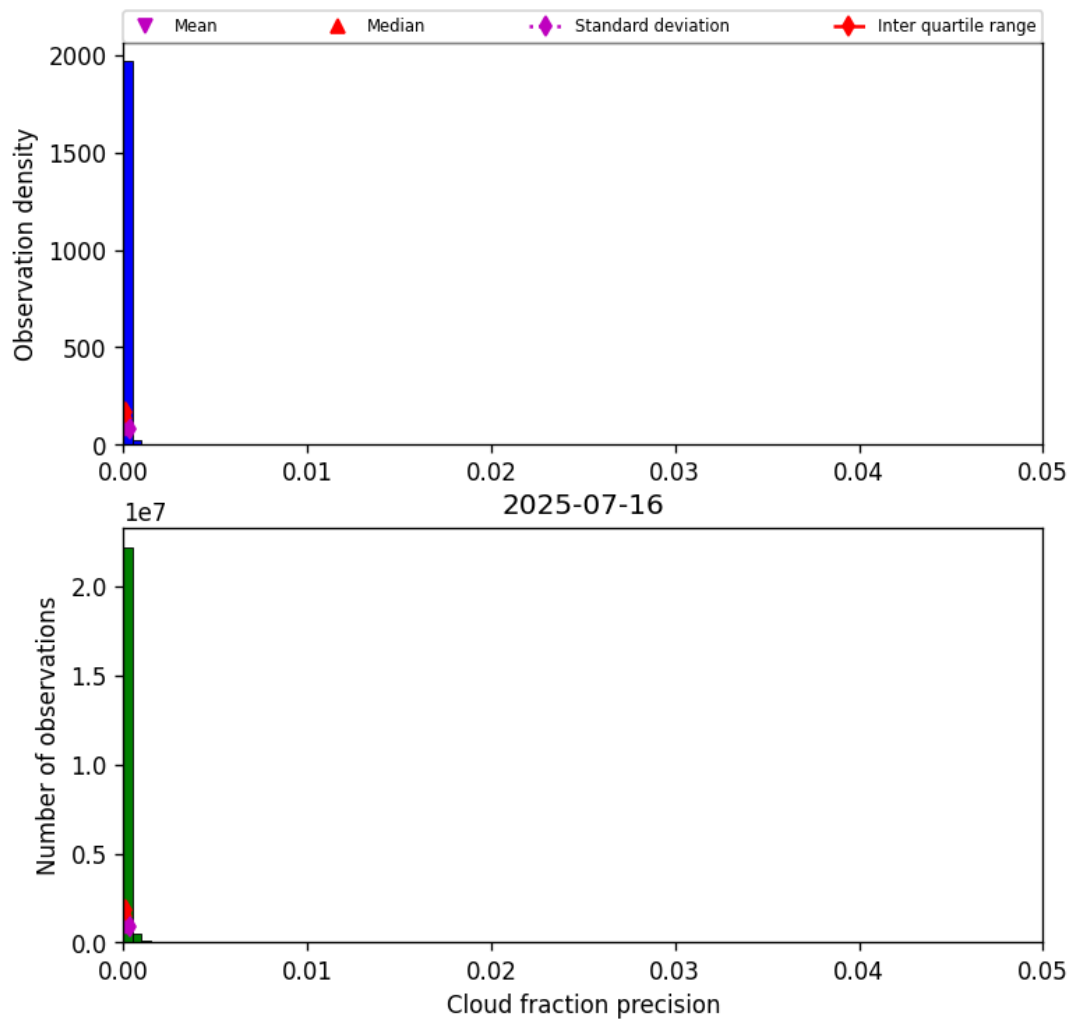
Figure 31: Histogram of “Cloud fraction precision” for 2025-07-16 to 2025-07-16
