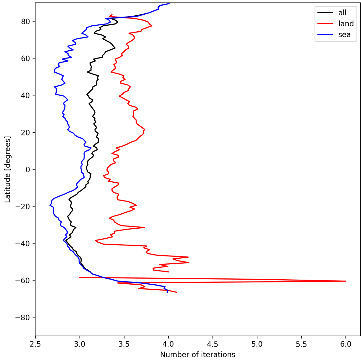
Figure 20: Zonal average of “Number of iterations” for 2025-07-16 to 2025-07-16.
