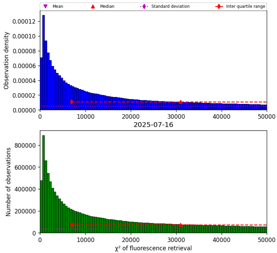
Figure 40: Histogram of “ \chi^2 of fluorescence retrieval” for 2025-07-16 to 2025-07-16
