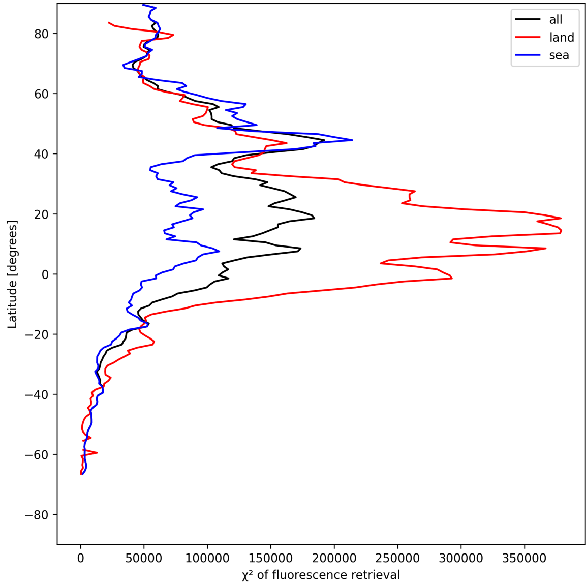
Figure 23: Zonal average of “ \chi^2 of fluorescence retrieval” for 2025-07-16 to 2025-07-16.
