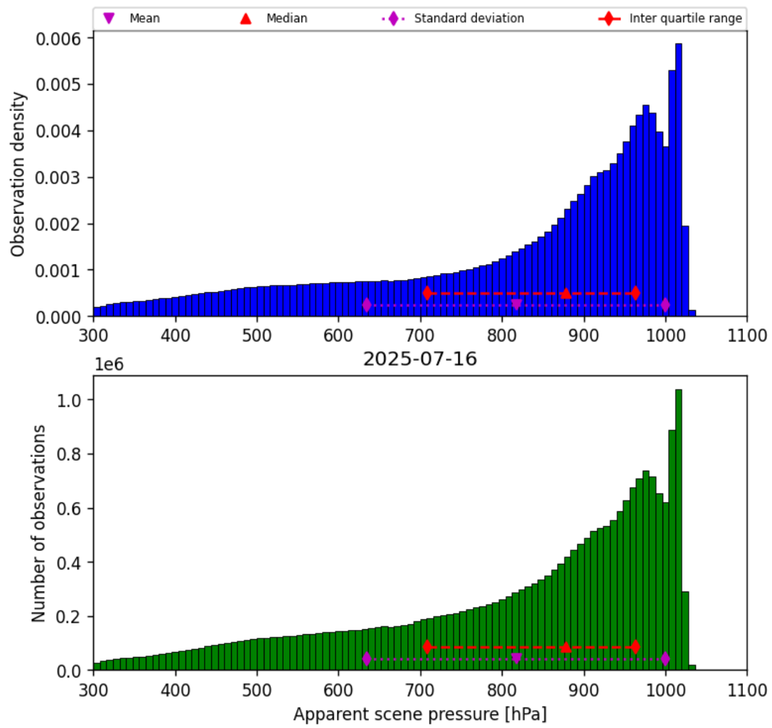
Figure 34: Histogram of “Apparent scene pressure” for 2025-07-16 to 2025-07-16
