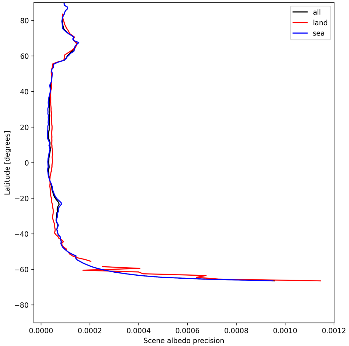
Figure 16: Zonal average of “Scene albedo precision” for 2025-07-16 to 2025-07-16.
