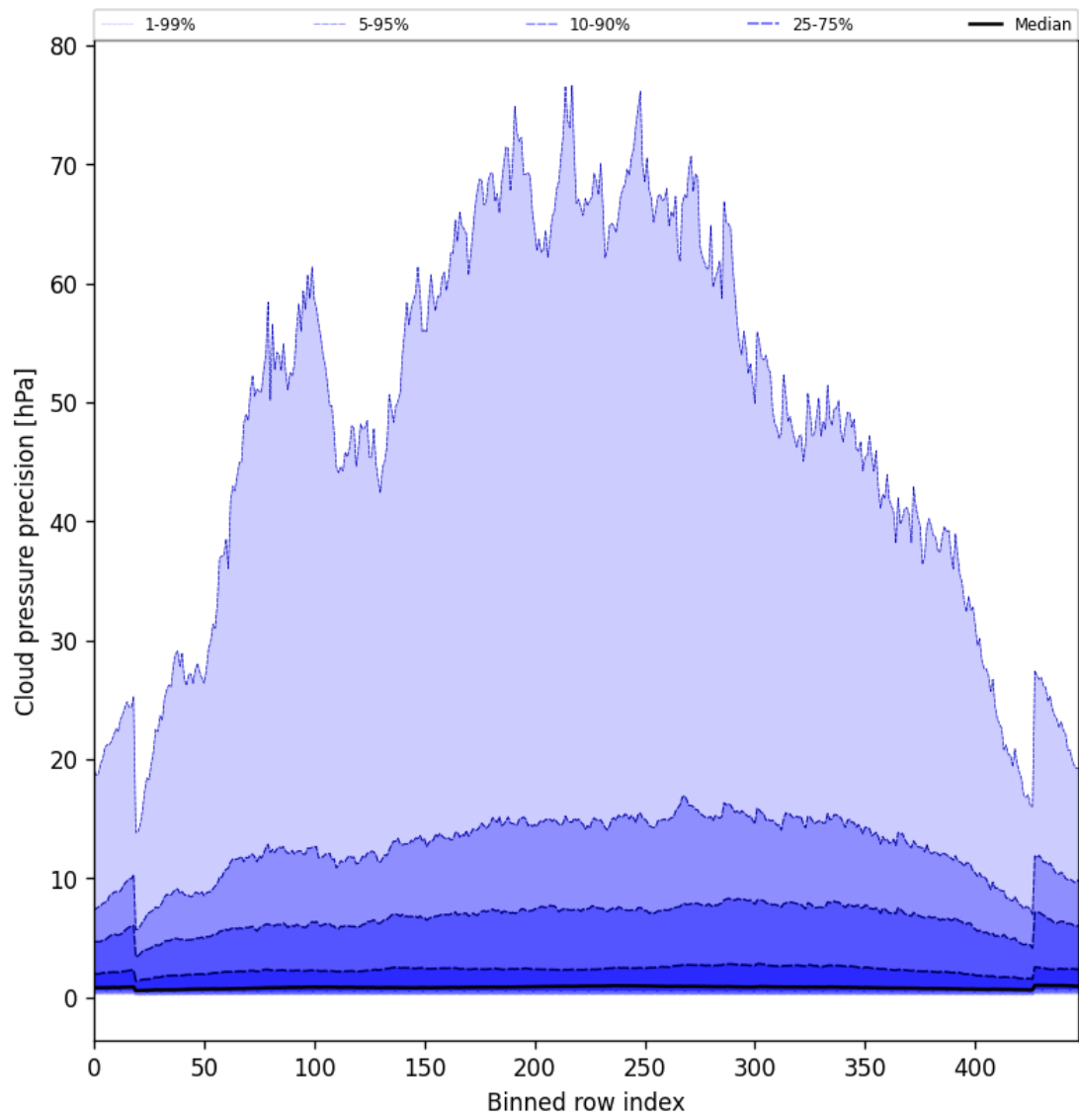
Figure 46: Along track statistics of “Cloud pressure precision” for 2025-07-16 to 2025-07-16
