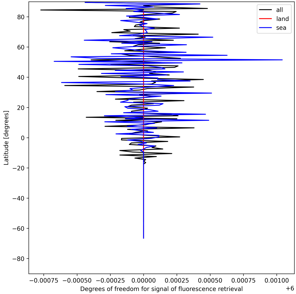
Figure 24: Zonal average of “Degrees of freedom for signal of fluorescence retrieval” for 2025-07-16 to 2025-07-16.
