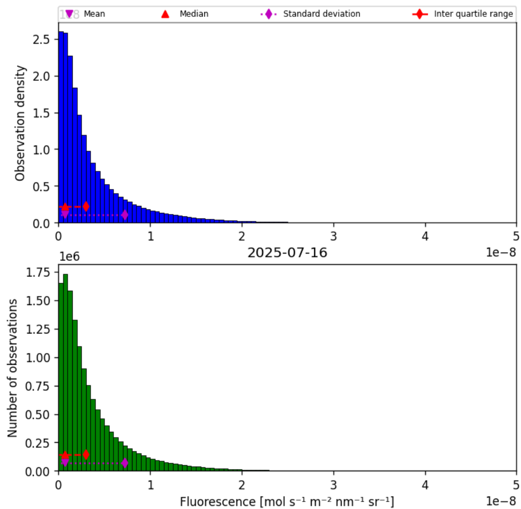
Figure 38: Histogram of “Fluorescence” for 2025-07-16 to 2025-07-16
