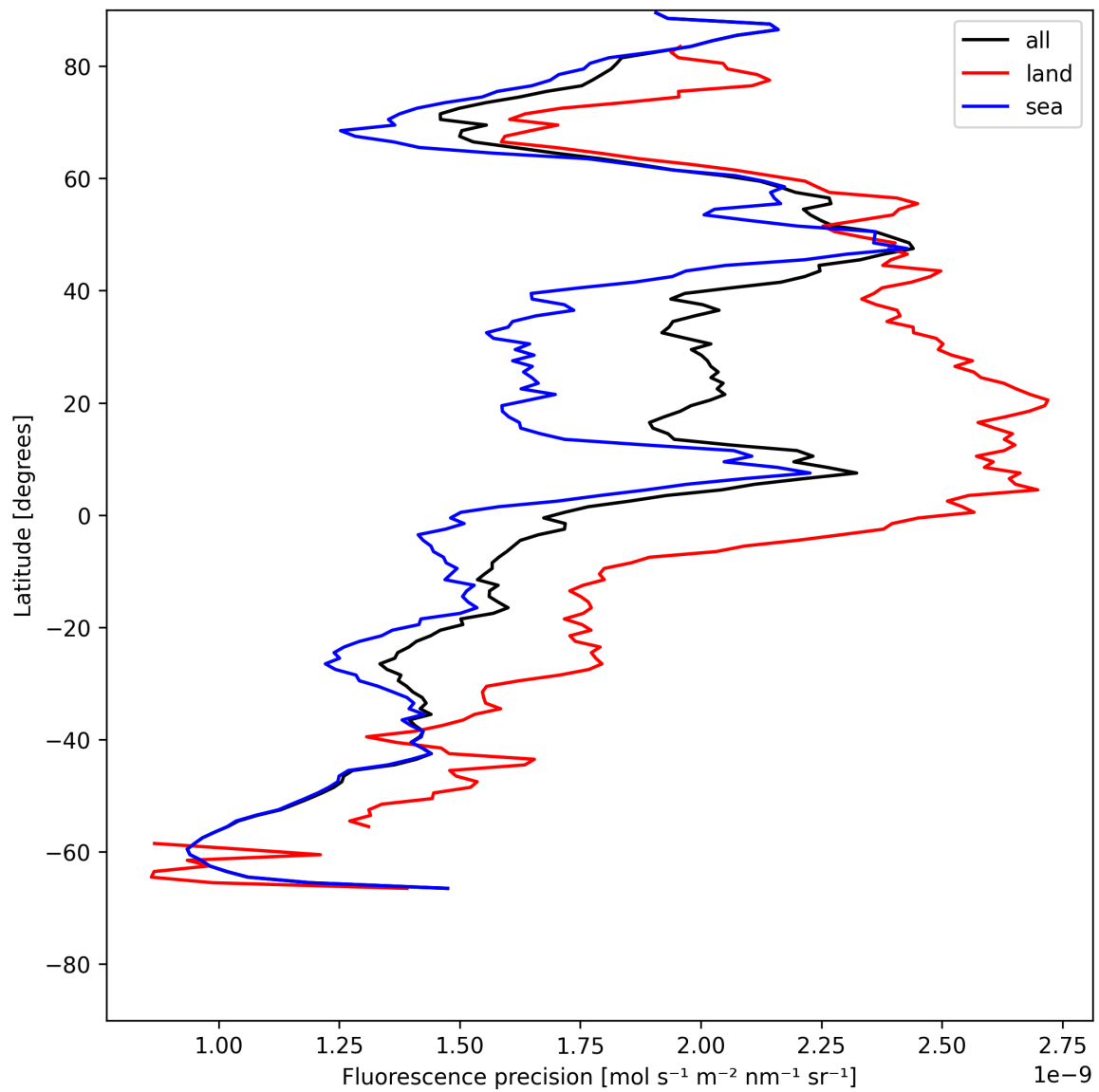
Figure 22: Zonal average of “Fluorescence precision” for 2025-07-16 to 2025-07-16.
