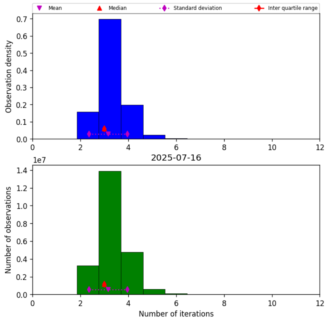
Figure 37: Histogram of “Number of iterations” for 2025-07-16 to 2025-07-16
