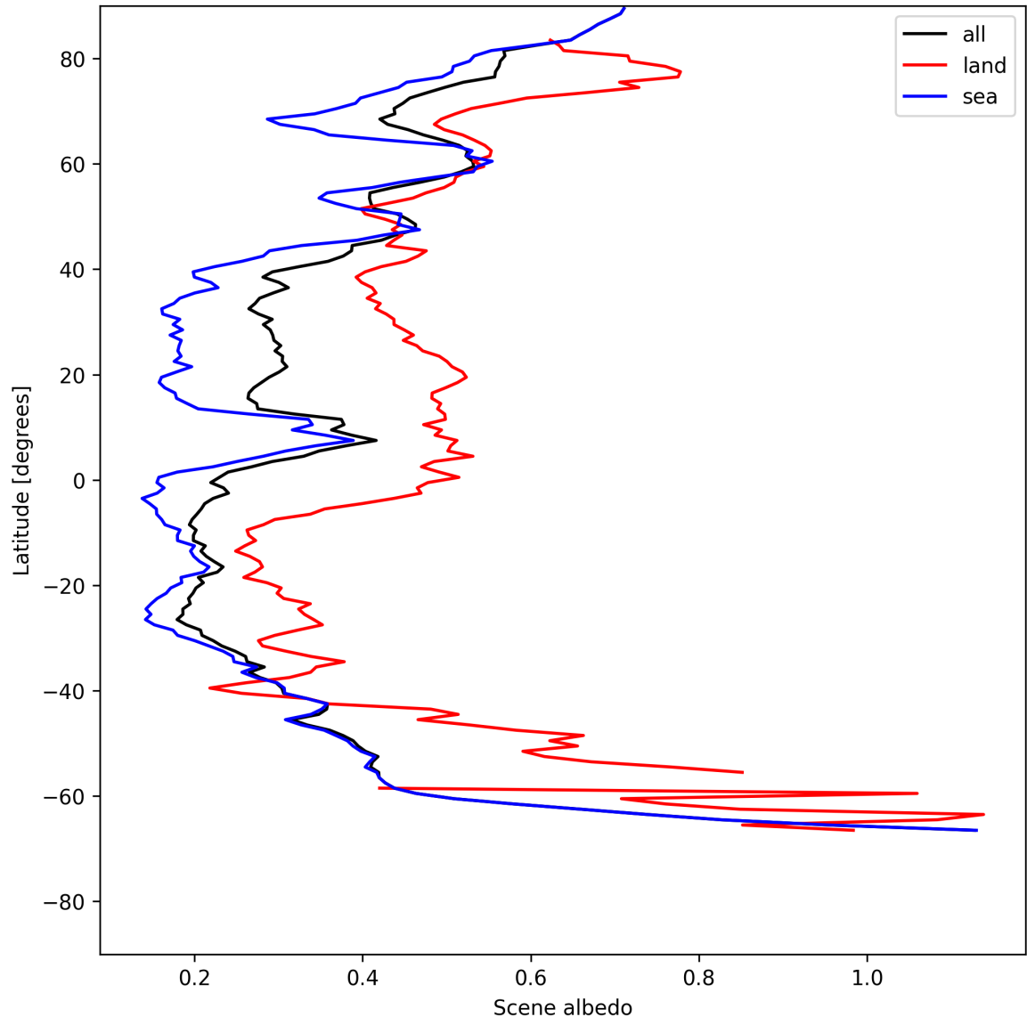
Figure 15: Zonal average of “Scene albedo” for 2025-07-16 to 2025-07-16.
