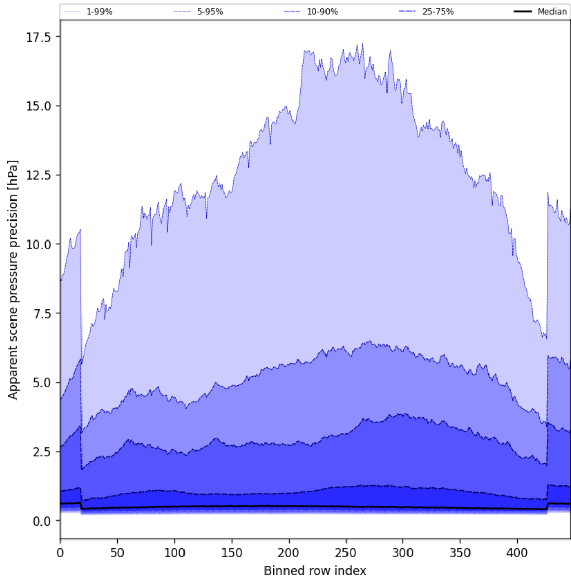
Figure 52: Along track statistics of “Apparent scene pressure precision” for 2025-07-16 to 2025-07-16
