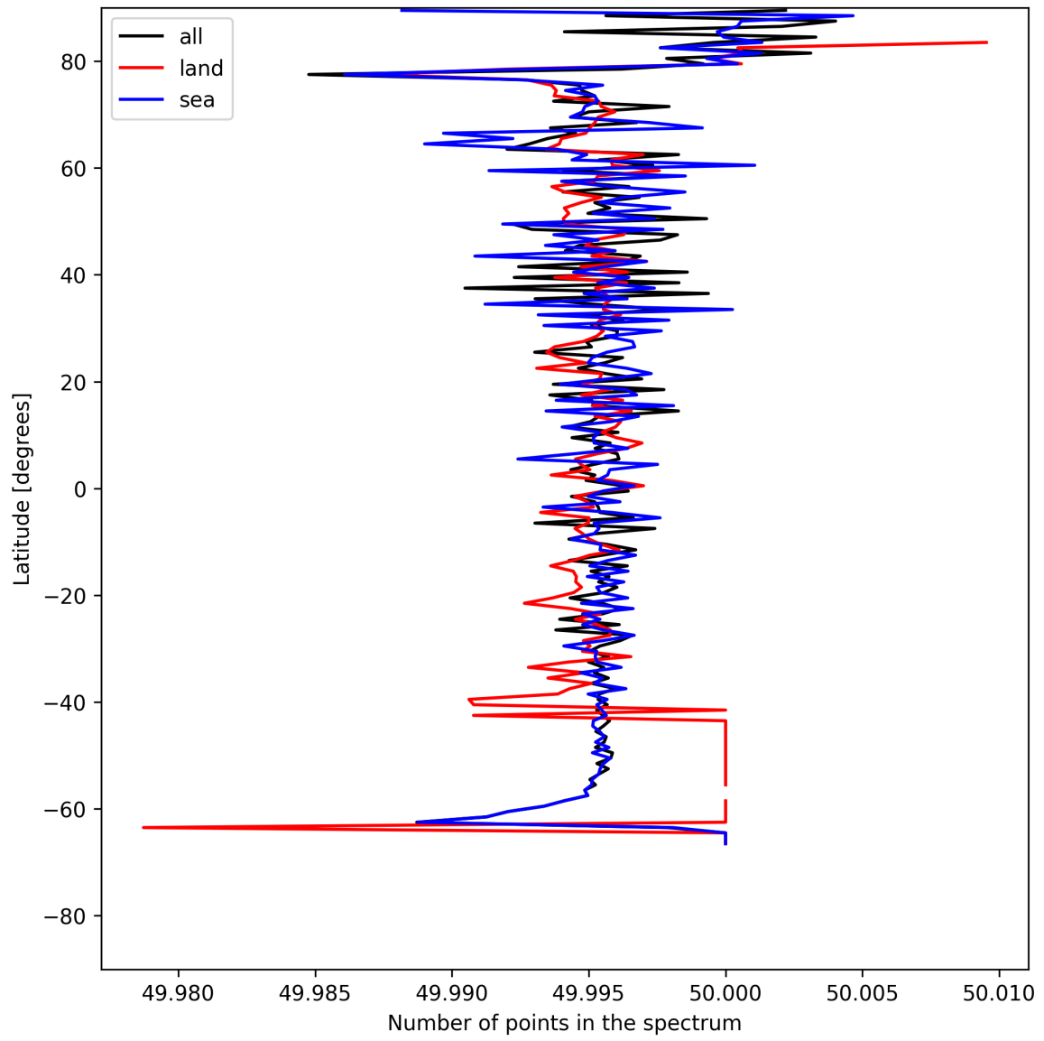
Figure 25: Zonal average of “Number of points in the spectrum” for 2025-07-16 to 2025-07-16.
