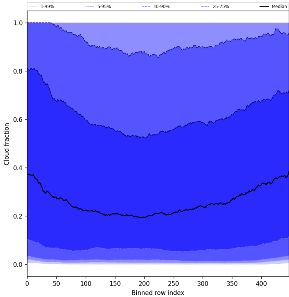
Figure 47: Along track statistics of “Cloud fraction” for 2025-07-16 to 2025-07-16
