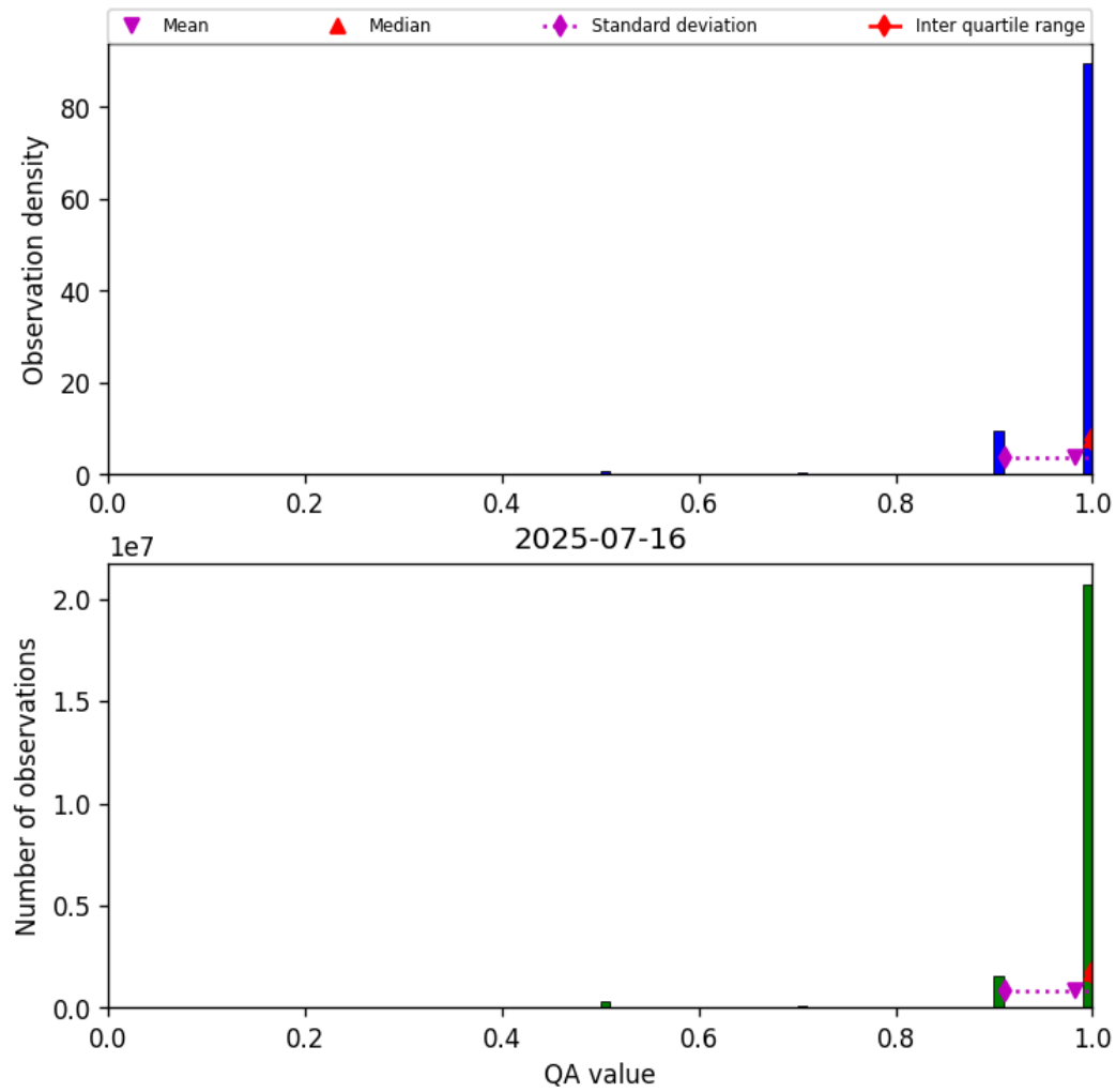
Figure 27: Histogram of “QA value” for 2025-07-16 to 2025-07-16
