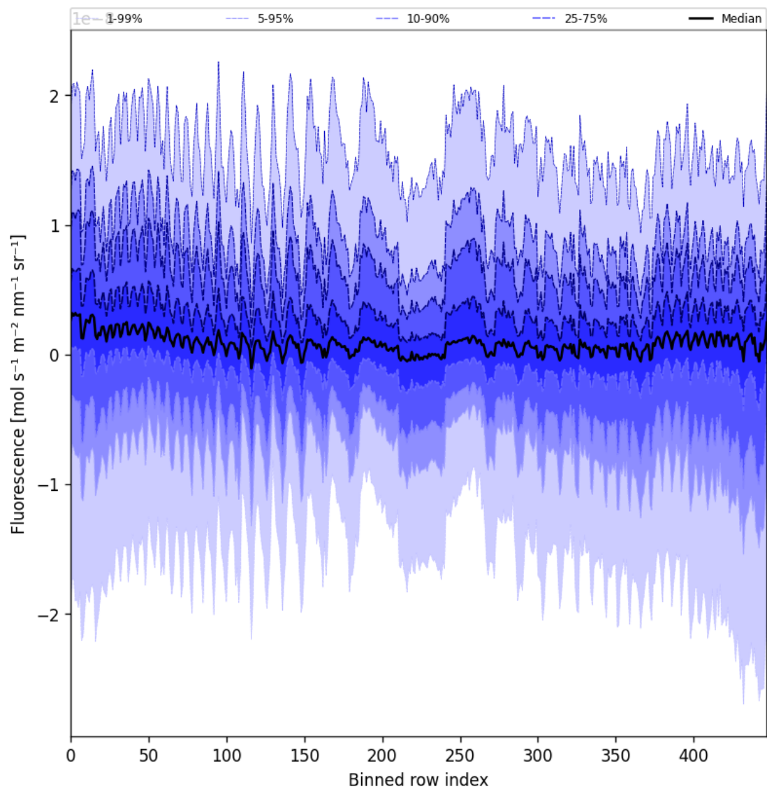
Figure 55: Along track statistics of “Fluorescence” for 2025-07-16 to 2025-07-16
