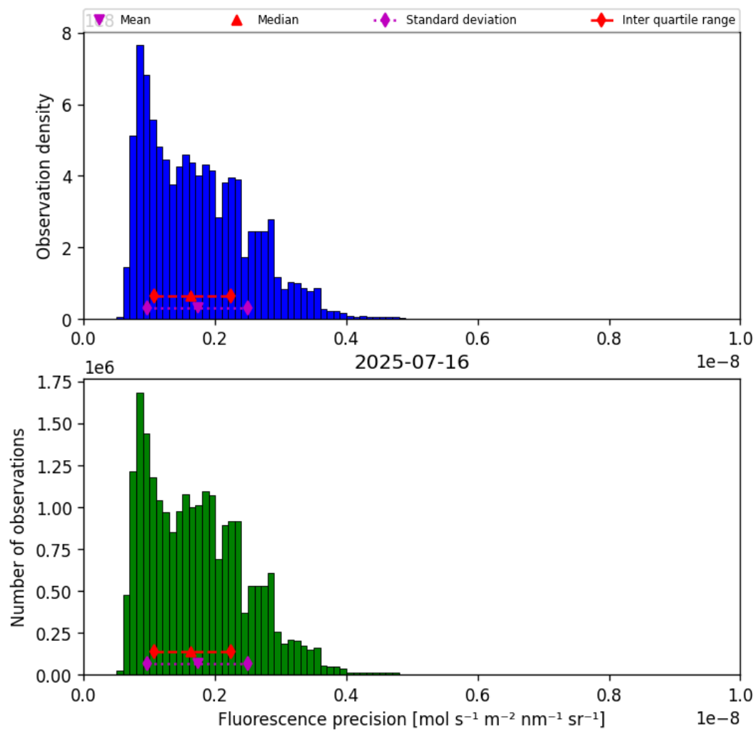
Figure 39: Histogram of “Fluorescence precision” for 2025-07-16 to 2025-07-16
