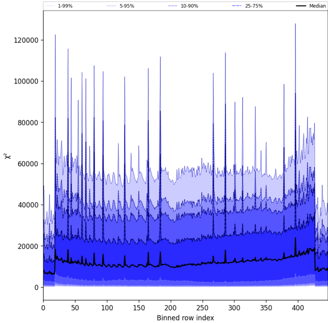
Figure 53: Along track statistics of “ \chi^2 ” for 2025-07-16 to 2025-07-16
