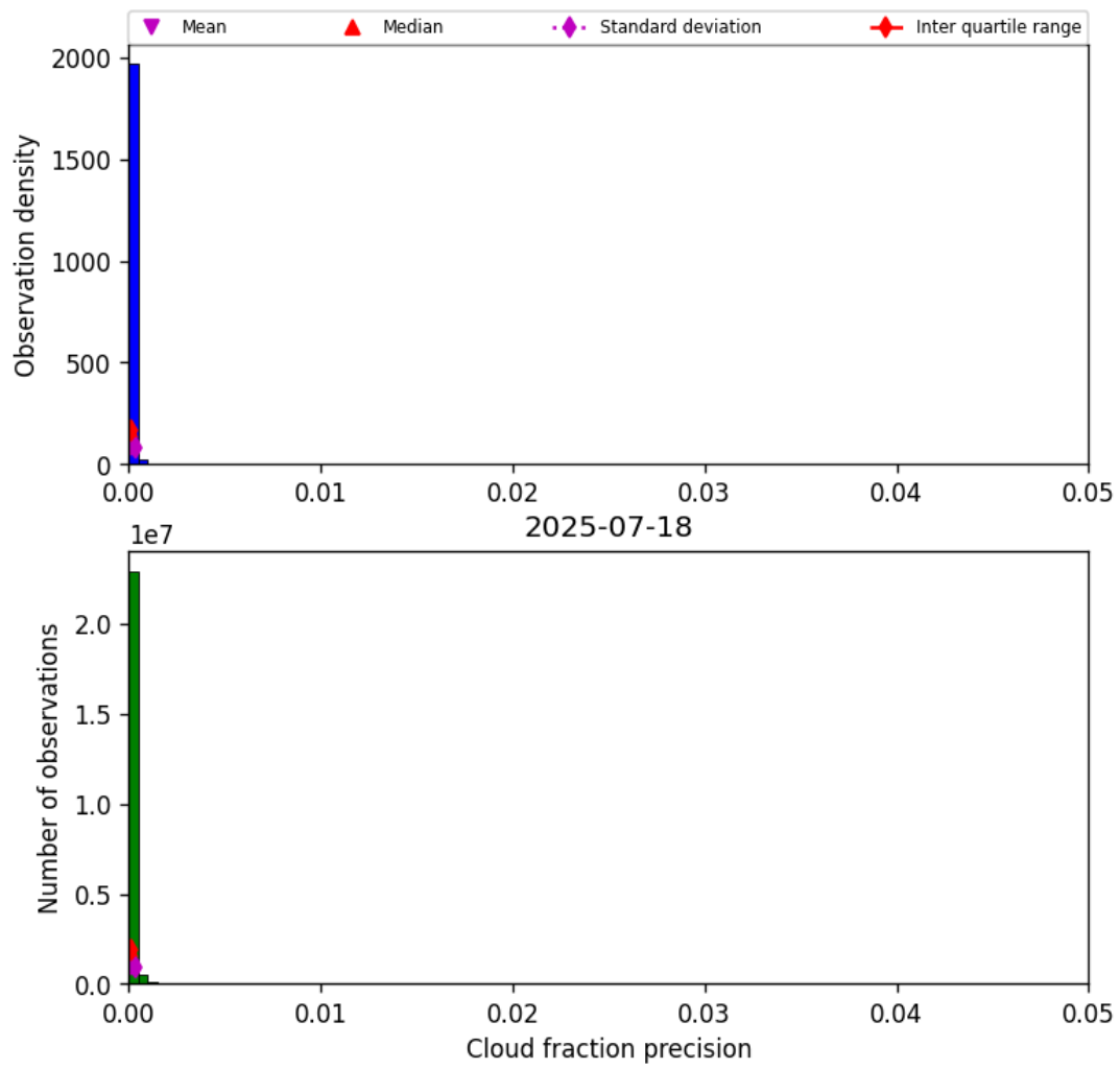
Figure 31: Histogram of “Cloud fraction precision” for 2025-07-18 to 2025-07-19
