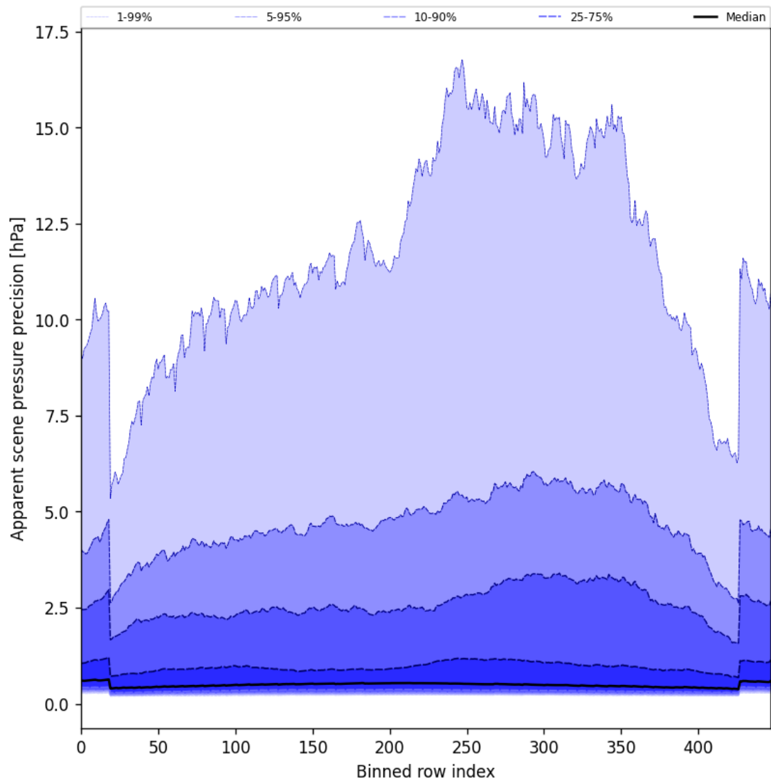
Figure 52: Along track statistics of “Apparent scene pressure precision” for 2025-07-18 to 2025-07-19
