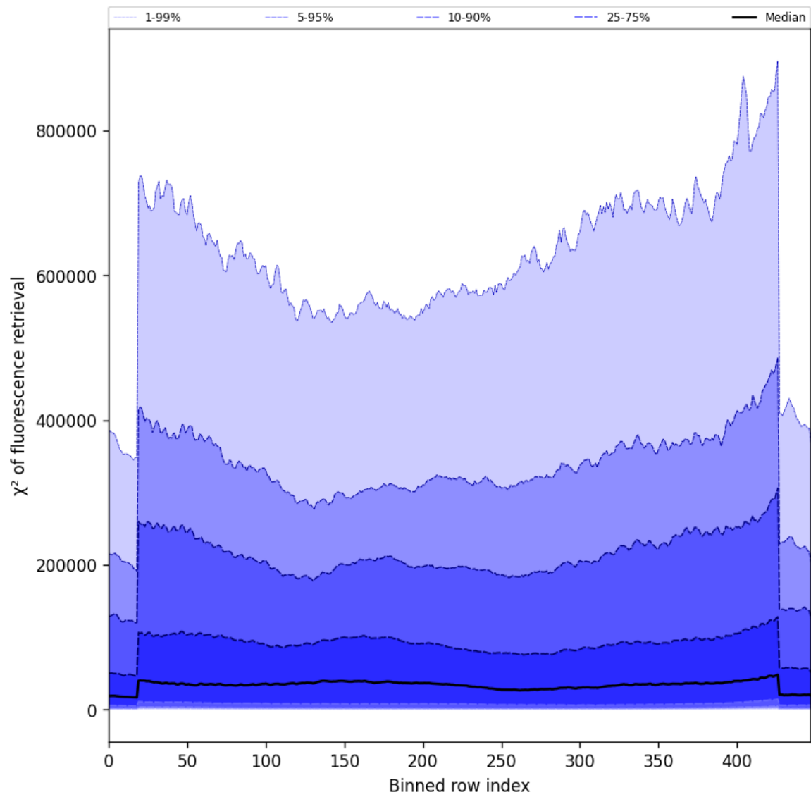
Figure 57: Along track statistics of “ \chi^2 of fluorescence retrieval” for 2025-07-18 to 2025-07-19
