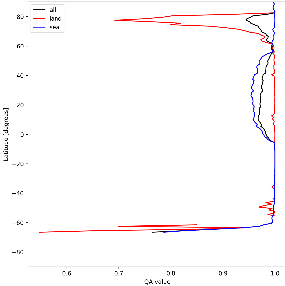
Figure 10: Zonal average of “QA value” for 2025-07-18 to 2025-07-19.
