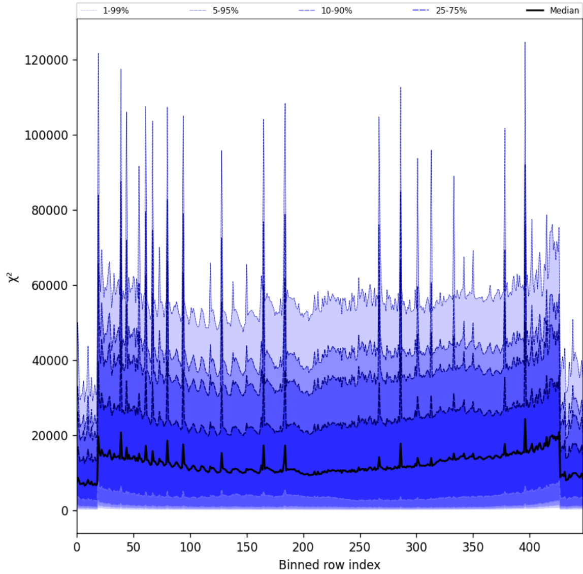
Figure 53: Along track statistics of “ \chi^2 ” for 2025-07-18 to 2025-07-19
