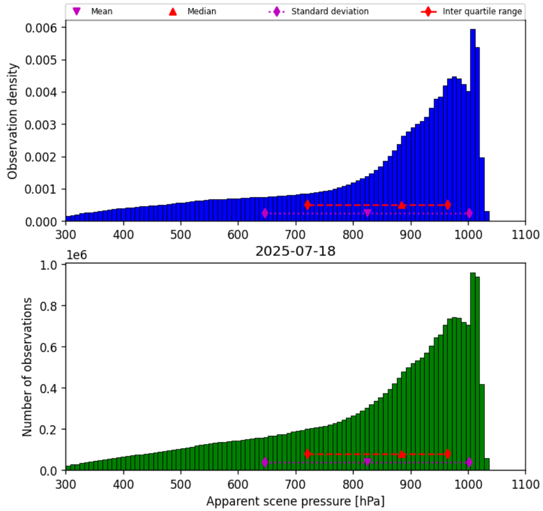
Figure 34: Histogram of “Apparent scene pressure” for 2025-07-18 to 2025-07-19
