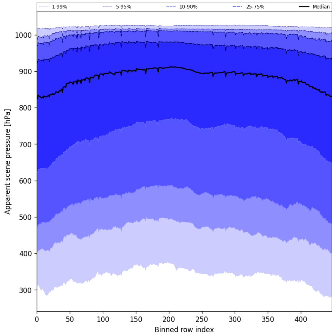
Figure 51: Along track statistics of “Apparent scene pressure” for 2025-07-18 to 2025-07-19
