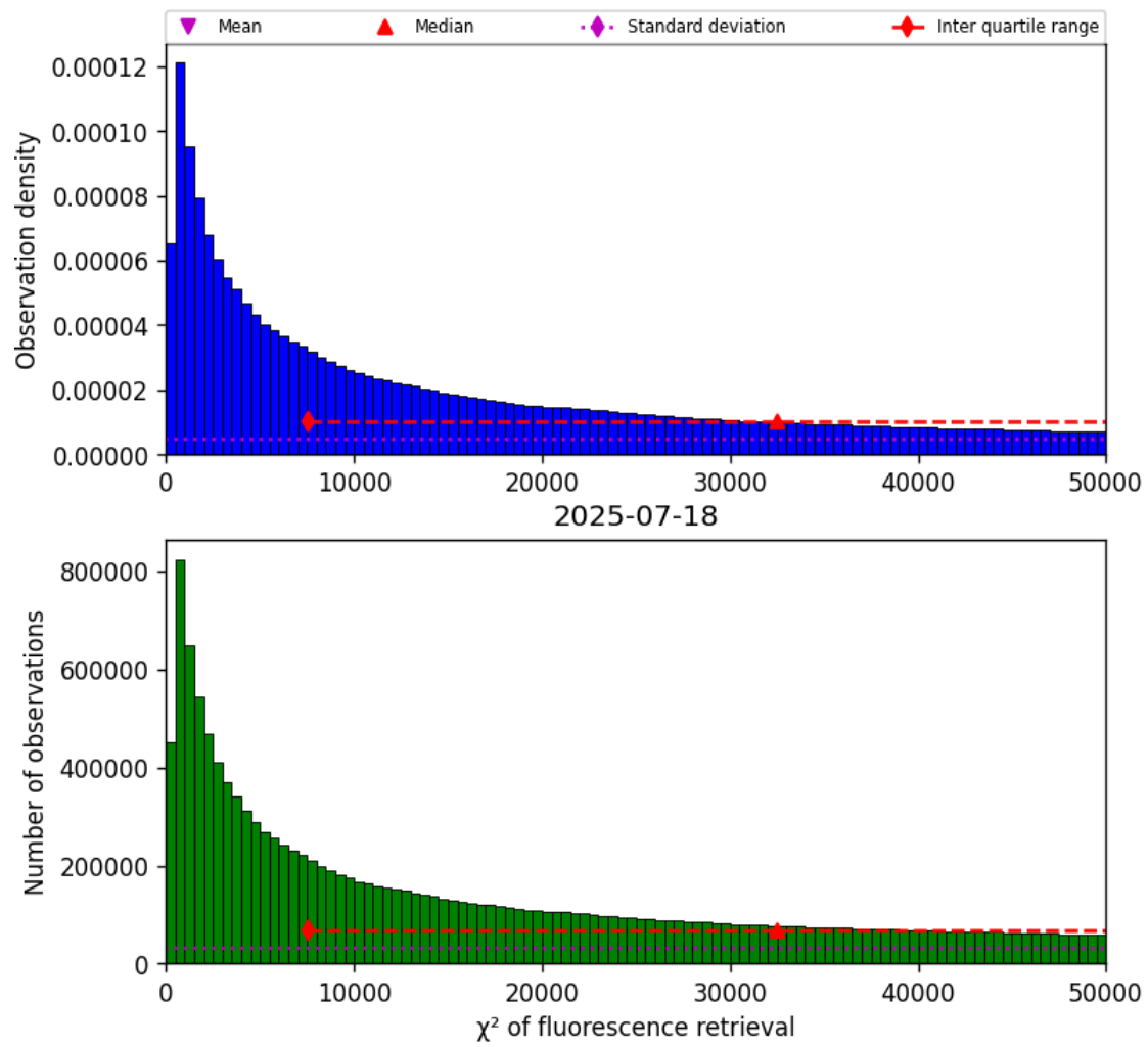
Figure 40: Histogram of “ \chi^2 of fluorescence retrieval” for 2025-07-18 to 2025-07-19
