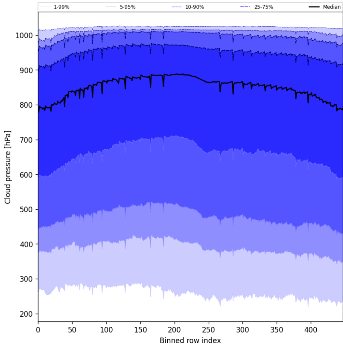
Figure 45: Along track statistics of “Cloud pressure” for 2025-07-18 to 2025-07-19
