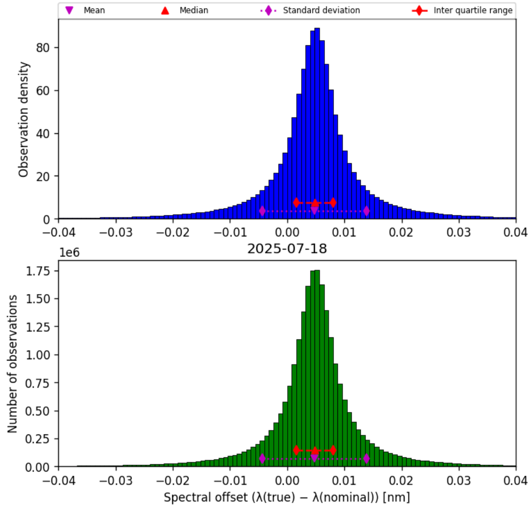
Figure 43: Histogram of “Spectral offset ( \lambda_{\text{true}} - \lambda_{\text{nominal}} )” for 2025-07-18 to 2025-07-19
