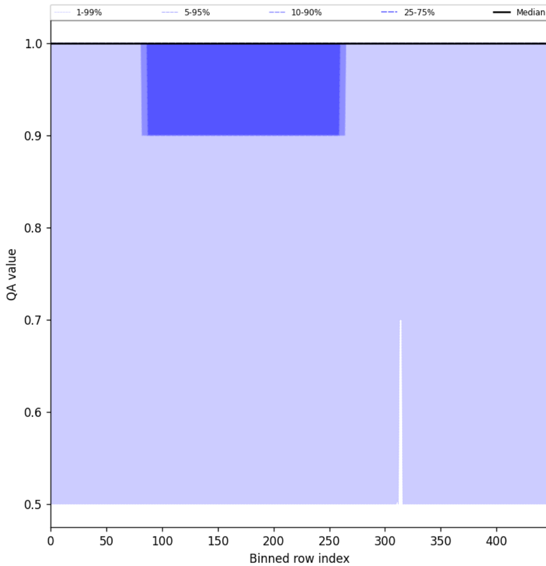
Figure 44: Along track statistics of “QA value” for 2025-07-18 to 2025-07-19
