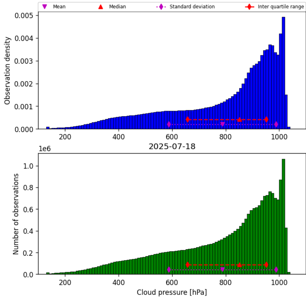
Figure 28: Histogram of “Cloud pressure” for 2025-07-18 to 2025-07-19
