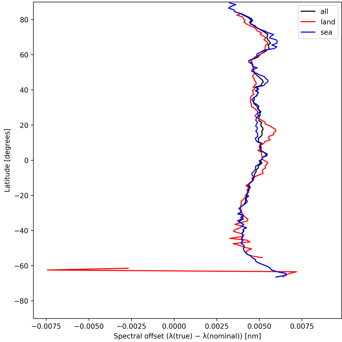
Figure 26: Zonal average of “Spectral offset ( \lambda_{\text{true}} - \lambda_{\text{nominal}} )” for 2025-07-18 to 2025-07-19.
