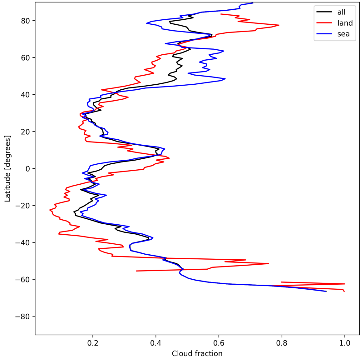
Figure 13: Zonal average of “Cloud fraction” for 2025-07-18 to 2025-07-19.
