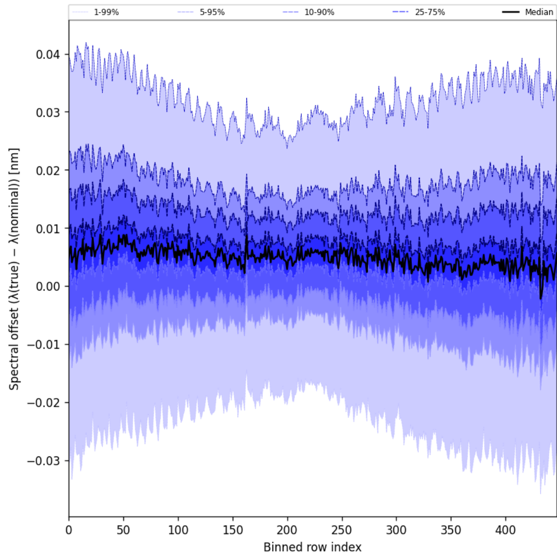
Figure 60: Along track statistics of “Spectral offset ( \lambda_{\text{true}} - \lambda_{\text{nominal}} )” for 2025-07-18 to 2025-07-19
