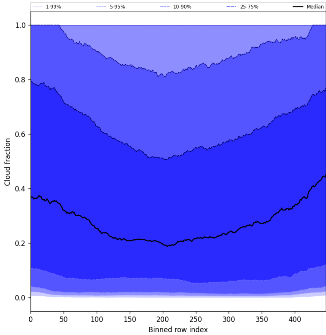
Figure 47: Along track statistics of “Cloud fraction” for 2025-07-18 to 2025-07-19
