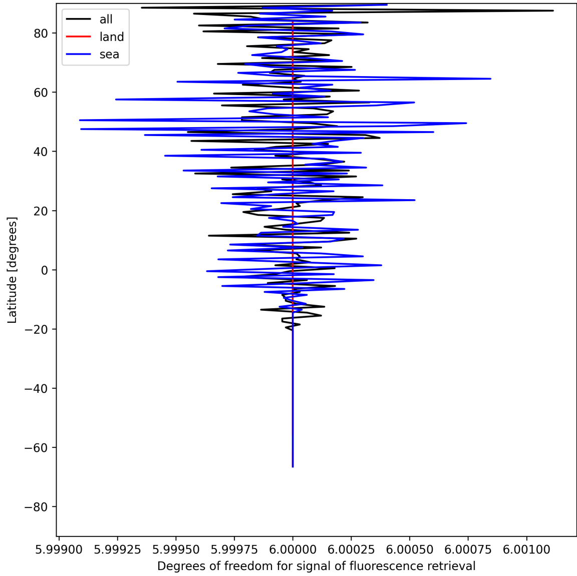
Figure 24: Zonal average of “Degrees of freedom for signal of fluorescence retrieval” for 2025-07-18 to 2025-07-19.
