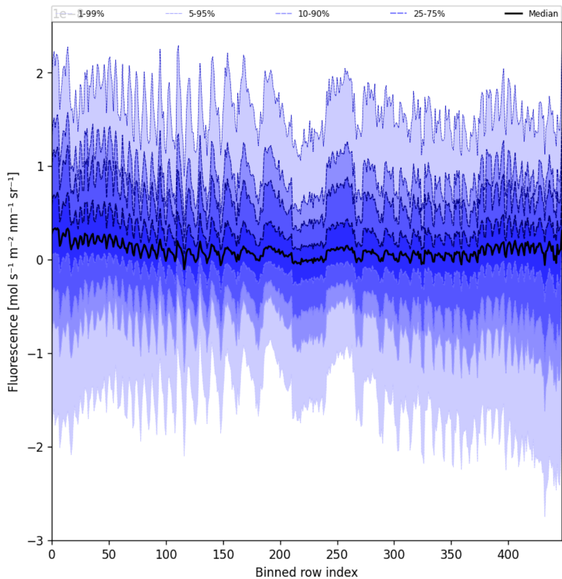
Figure 55: Along track statistics of "Fluorescence" for 2025-07-18 to 2025-07-19
