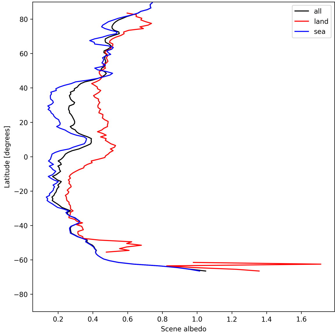
Figure 15: Zonal average of “Scene albedo” for 2025-07-18 to 2025-07-19.
