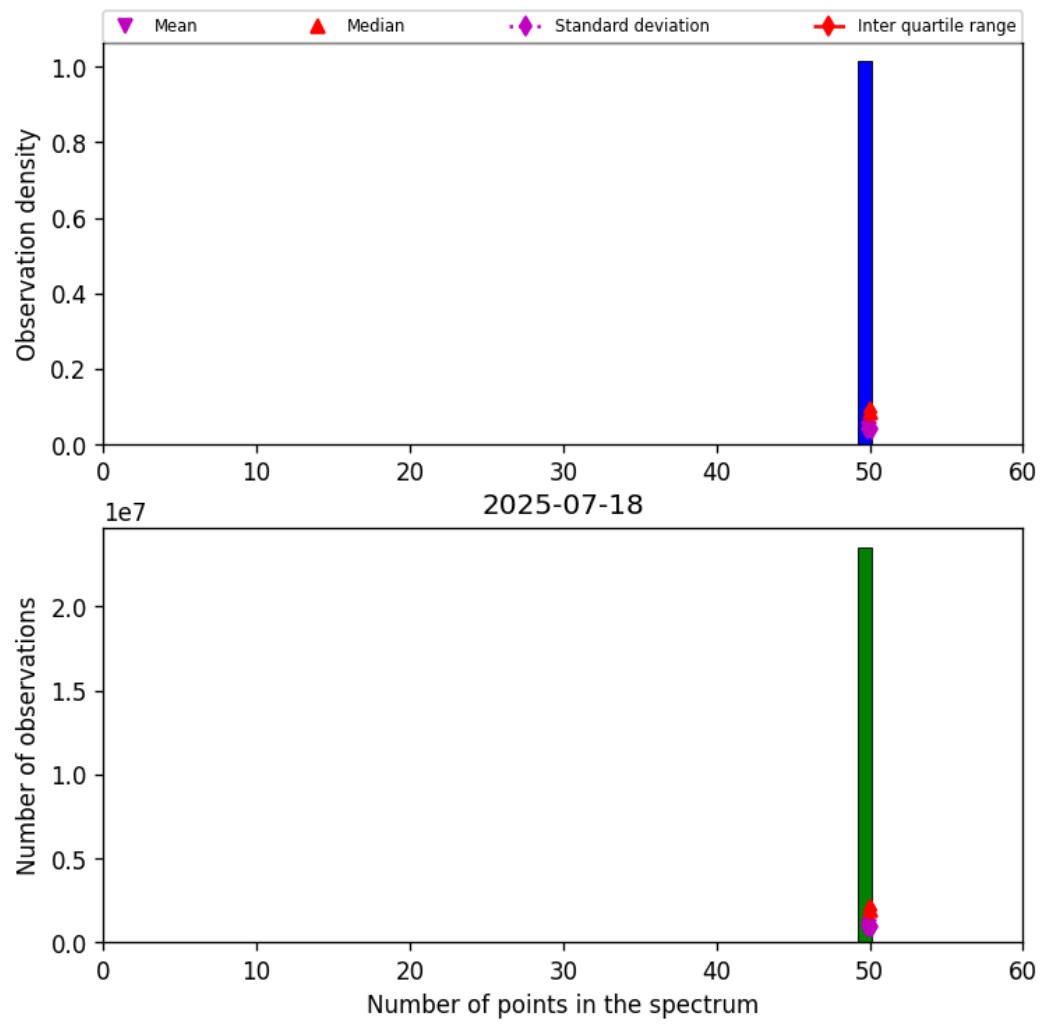
Figure 42: Histogram of “Number of points in the spectrum” for 2025-07-18 to 2025-07-19
