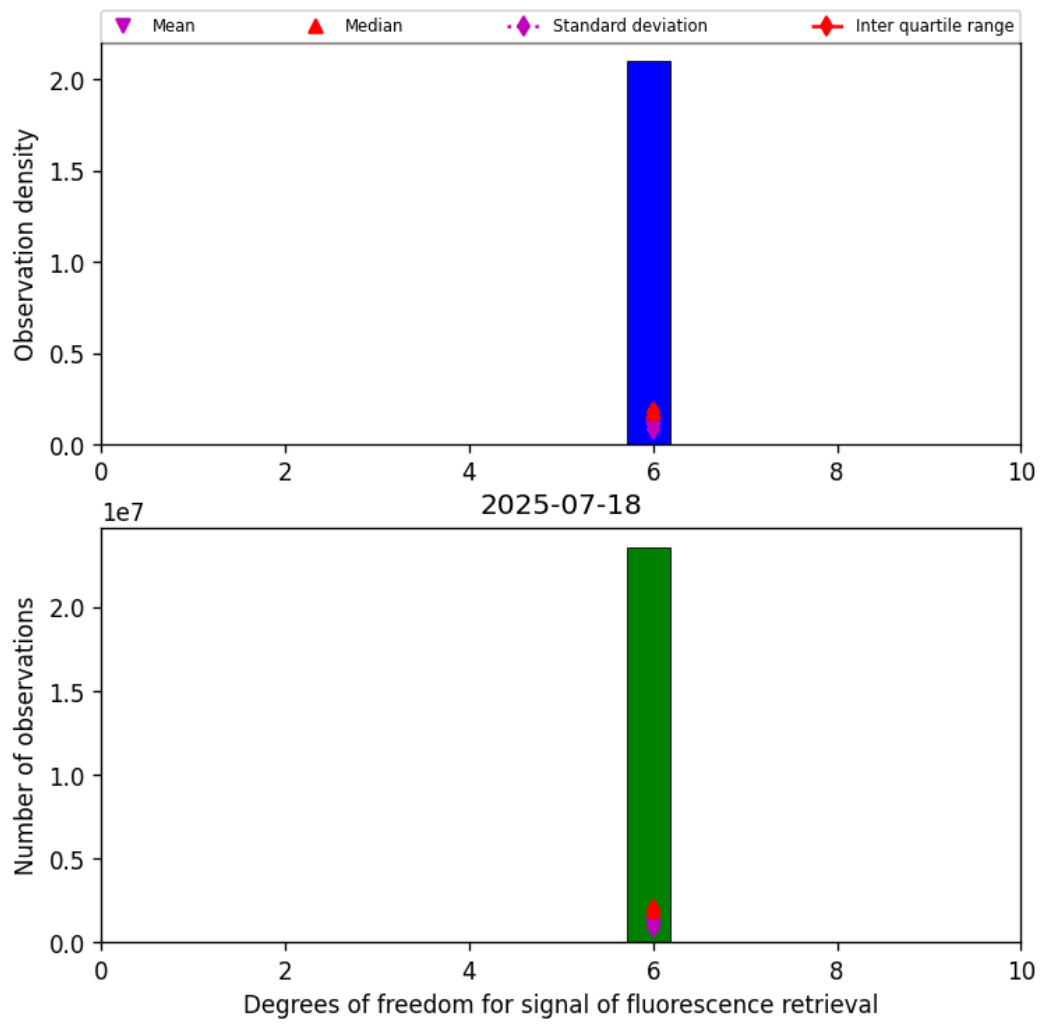
Figure 41: Histogram of “Degrees of freedom for signal of fluorescence retrieval” for 2025-07-18 to 2025-07-19
