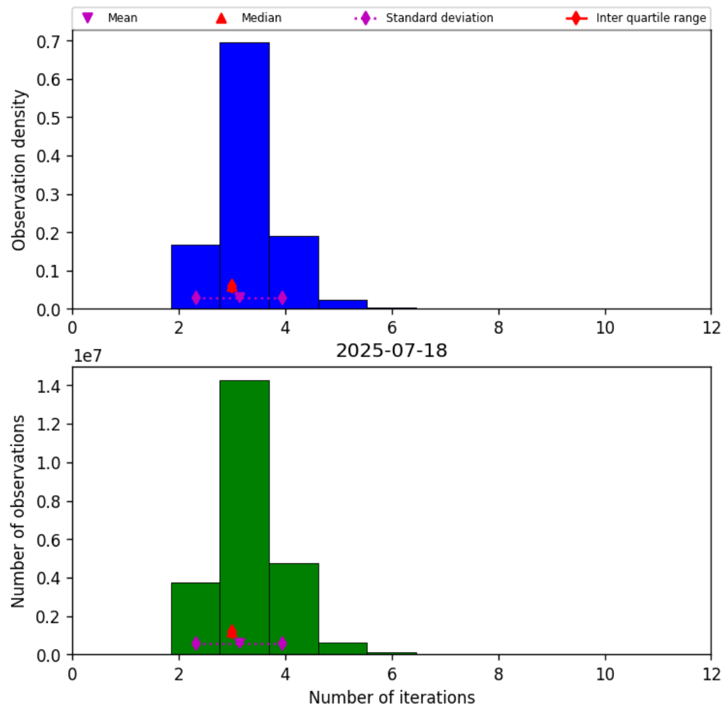
Figure 37: Histogram of “Number of iterations” for 2025-07-18 to 2025-07-19
