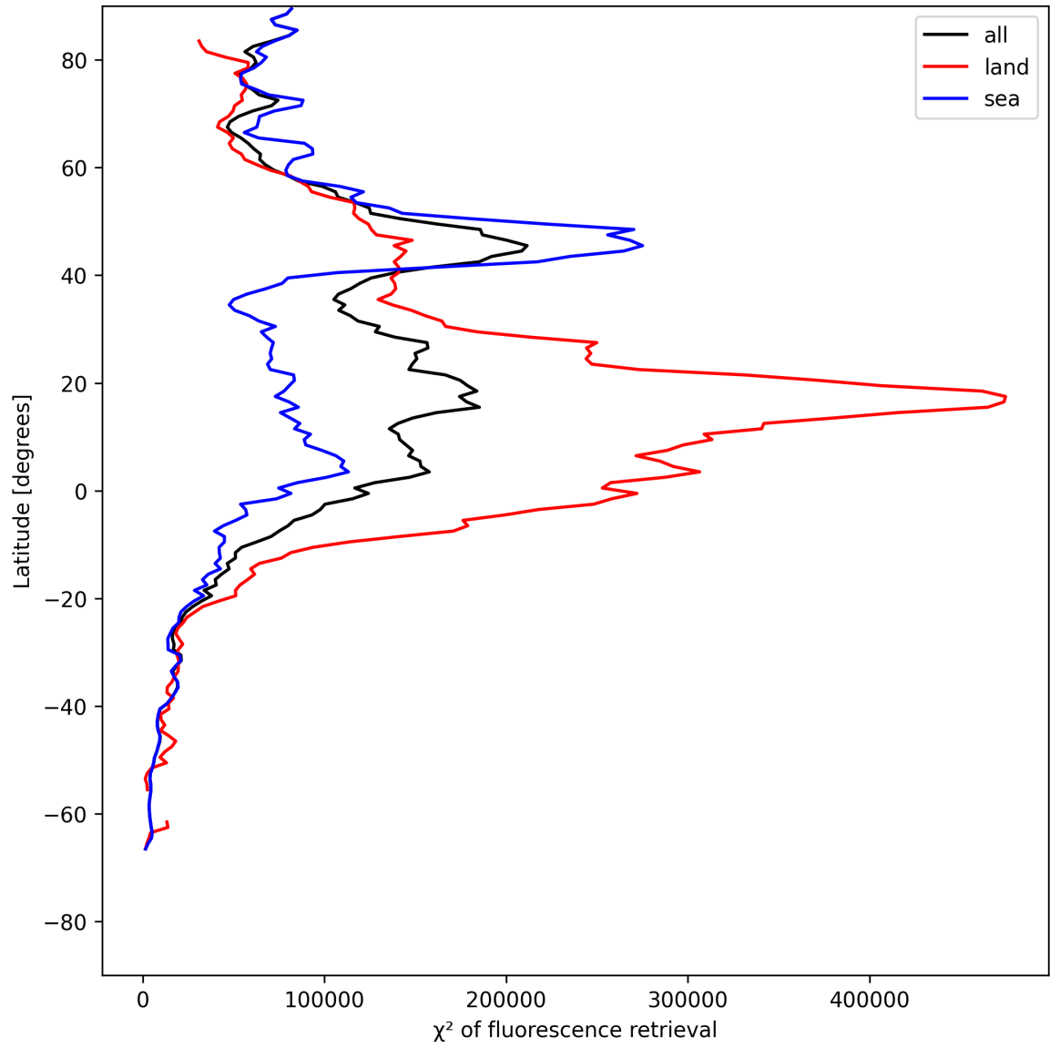
Figure 23: Zonal average of “ \chi^2 of fluorescence retrieval” for 2025-07-18 to 2025-07-19.
