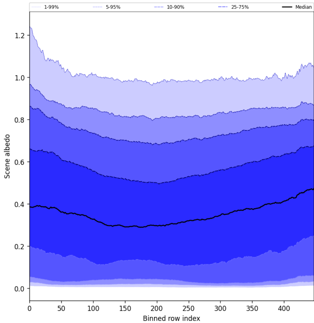
Figure 49: Along track statistics of “Scene albedo” for 2025-07-18 to 2025-07-19
