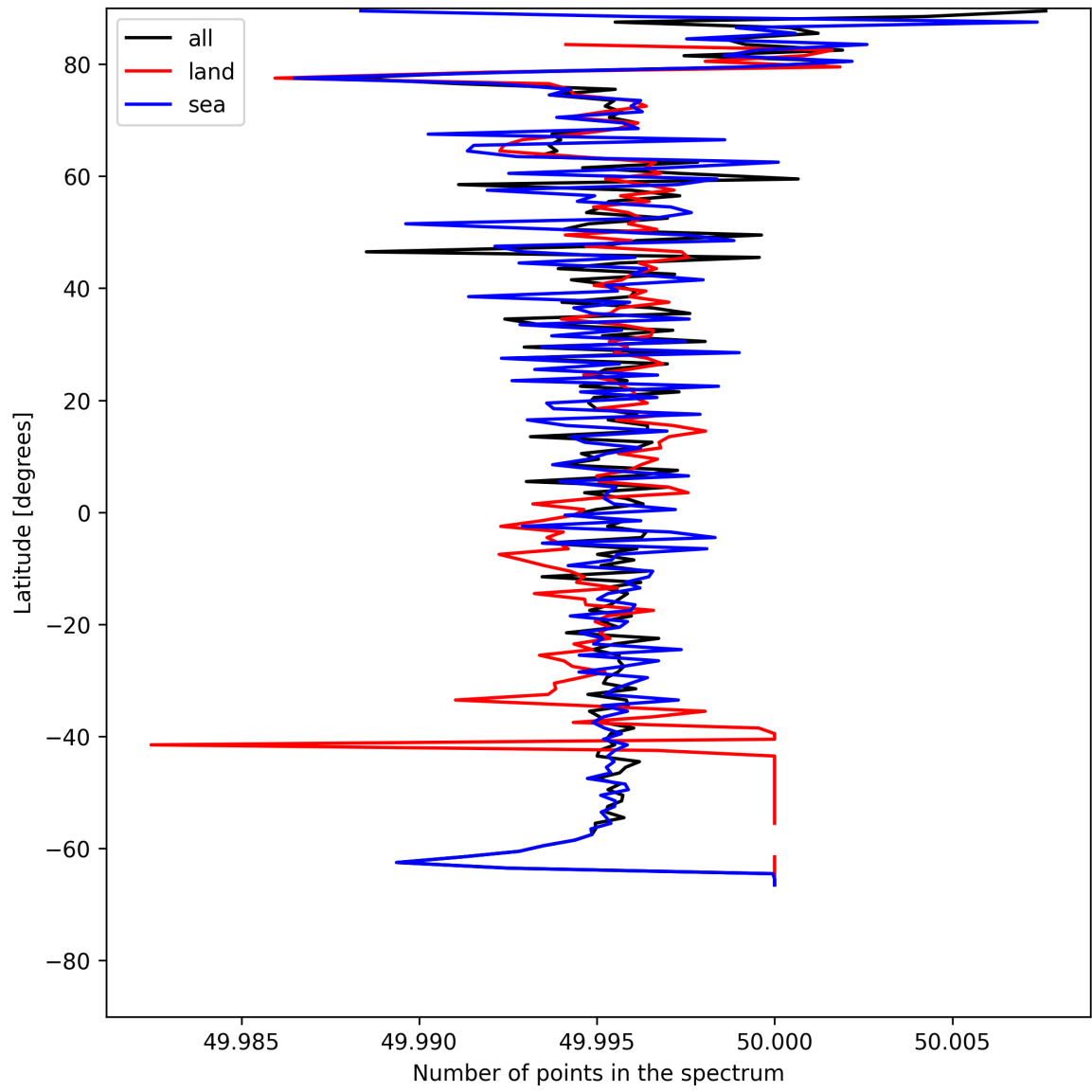
Figure 25: Zonal average of “Number of points in the spectrum” for 2025-07-18 to 2025-07-19.
