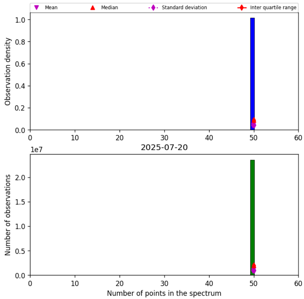
Figure 42: Histogram of “Number of points in the spectrum” for 2025-07-20 to 2025-07-21
