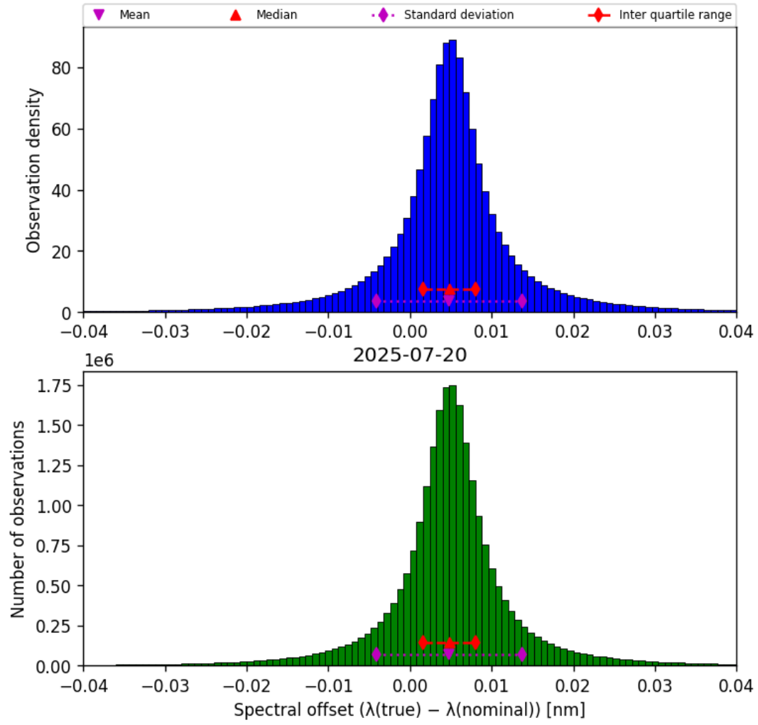
Figure 43: Histogram of “Spectral offset ( \lambda_{\text{true}} - \lambda_{\text{nominal}} )” for 2025-07-20 to 2025-07-21
