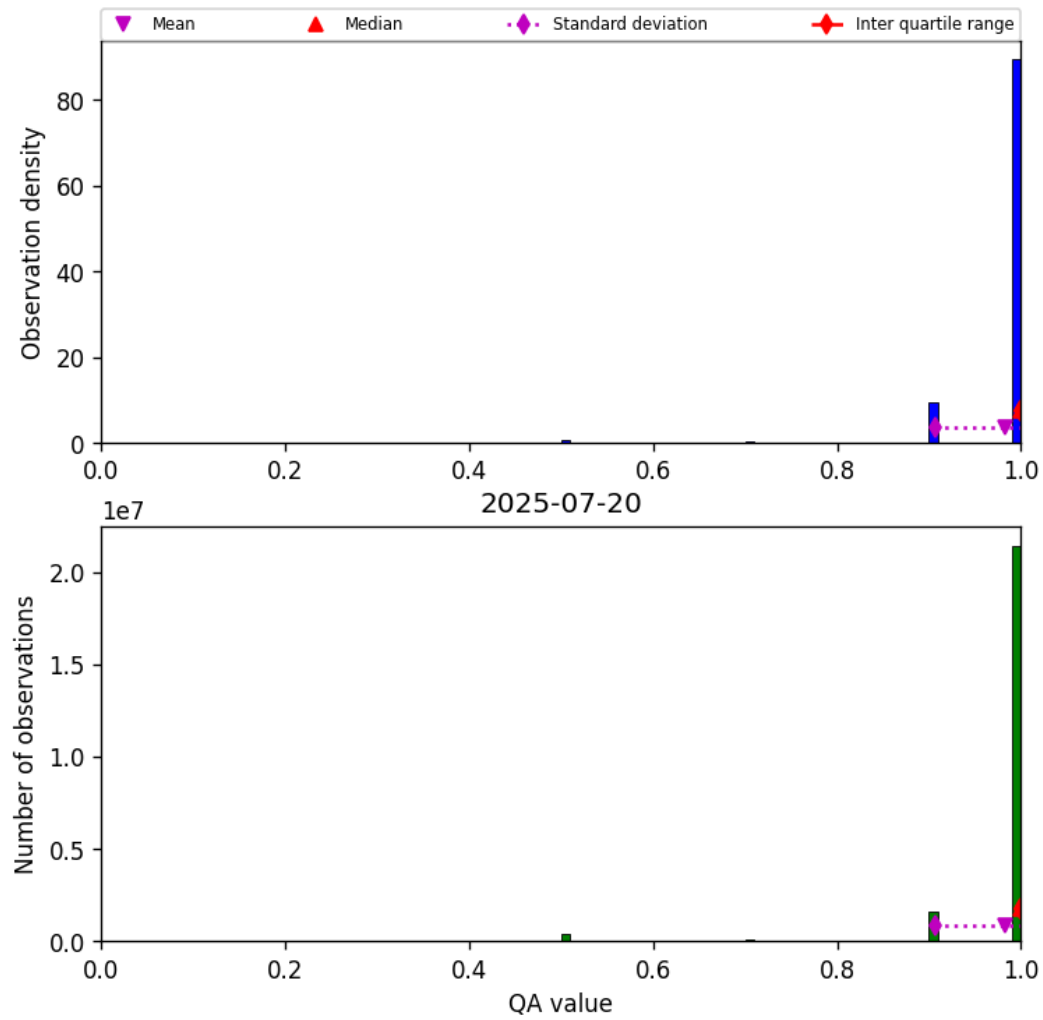
Figure 27: Histogram of “QA value” for 2025-07-20 to 2025-07-21
