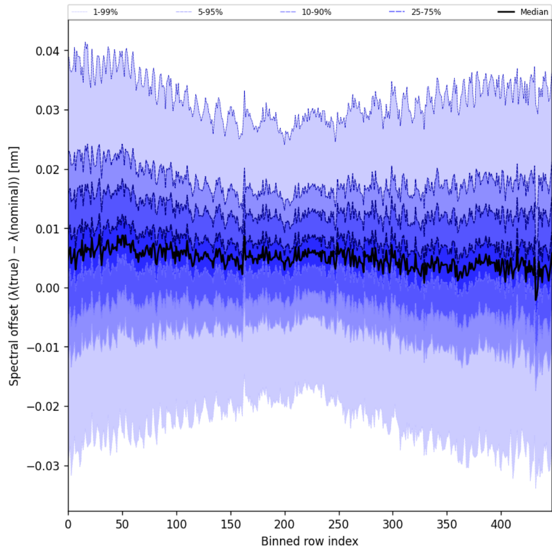
Figure 60: Along track statistics of “Spectral offset ( \lambda_{\text{true}} - \lambda_{\text{nominal}} )” for 2025-07-20 to 2025-07-21
