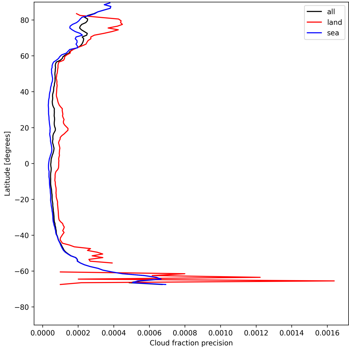
Figure 14: Zonal average of “Cloud fraction precision” for 2025-07-20 to 2025-07-21.
