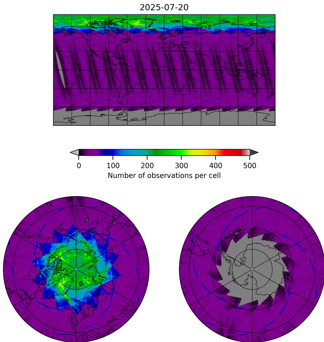
Figure 9: Map of the number of observations for 2025-07-20 to 2025-07-21
