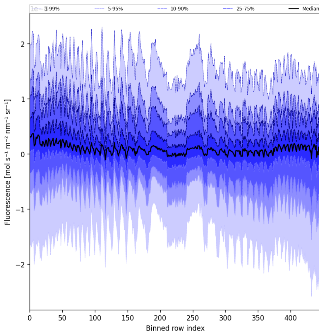
Figure 55: Along track statistics of “Fluorescence” for 2025-07-20 to 2025-07-21
