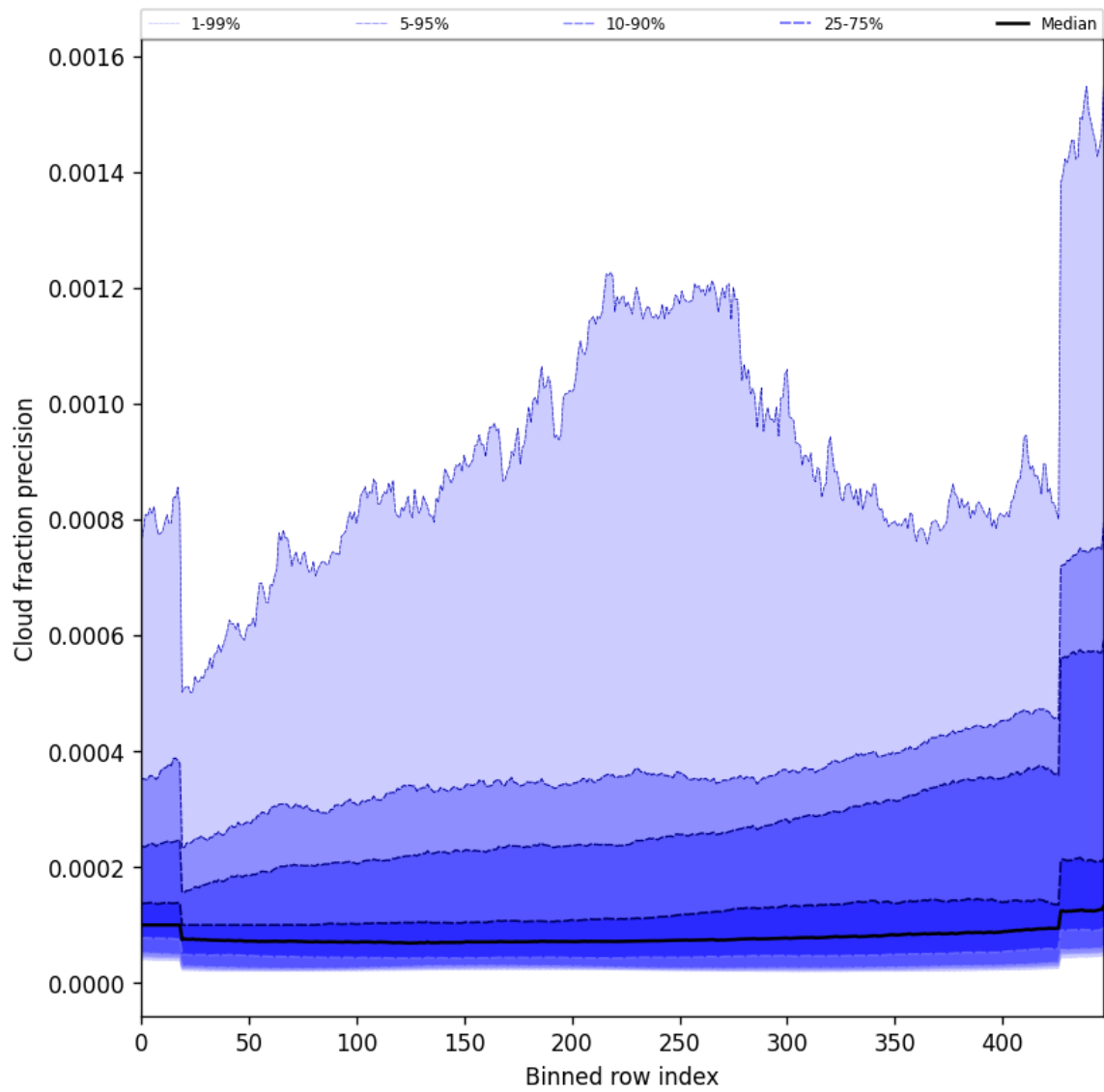
Figure 48: Along track statistics of “Cloud fraction precision” for 2025-07-20 to 2025-07-21
