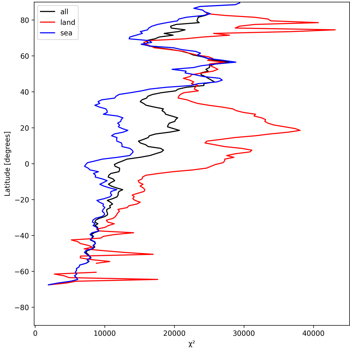
Figure 19: Zonal average of “ \chi^2 ” for 2025-07-20 to 2025-07-21.
