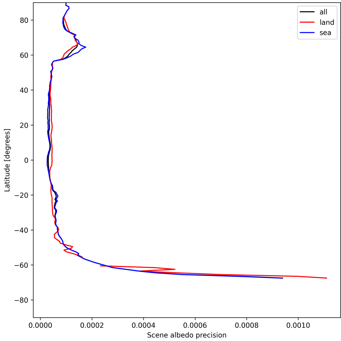
Figure 16: Zonal average of “Scene albedo precision” for 2025-07-20 to 2025-07-21.
