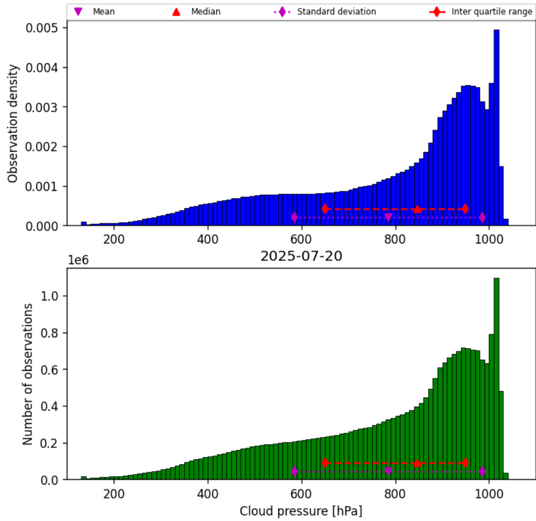
Figure 28: Histogram of “Cloud pressure” for 2025-07-20 to 2025-07-21
