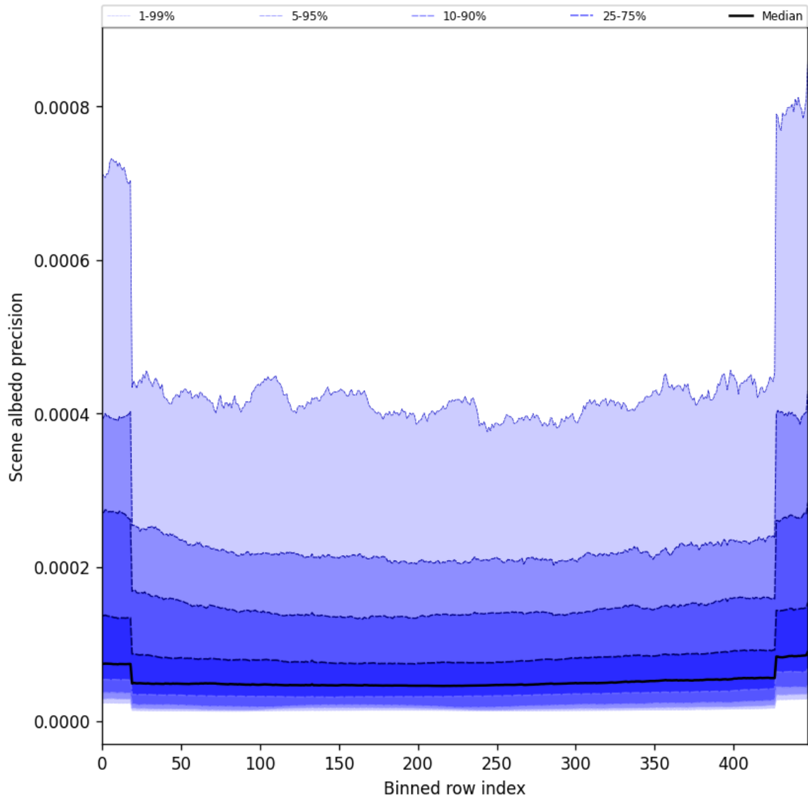
Figure 50: Along track statistics of “Scene albedo precision” for 2025-07-20 to 2025-07-21
