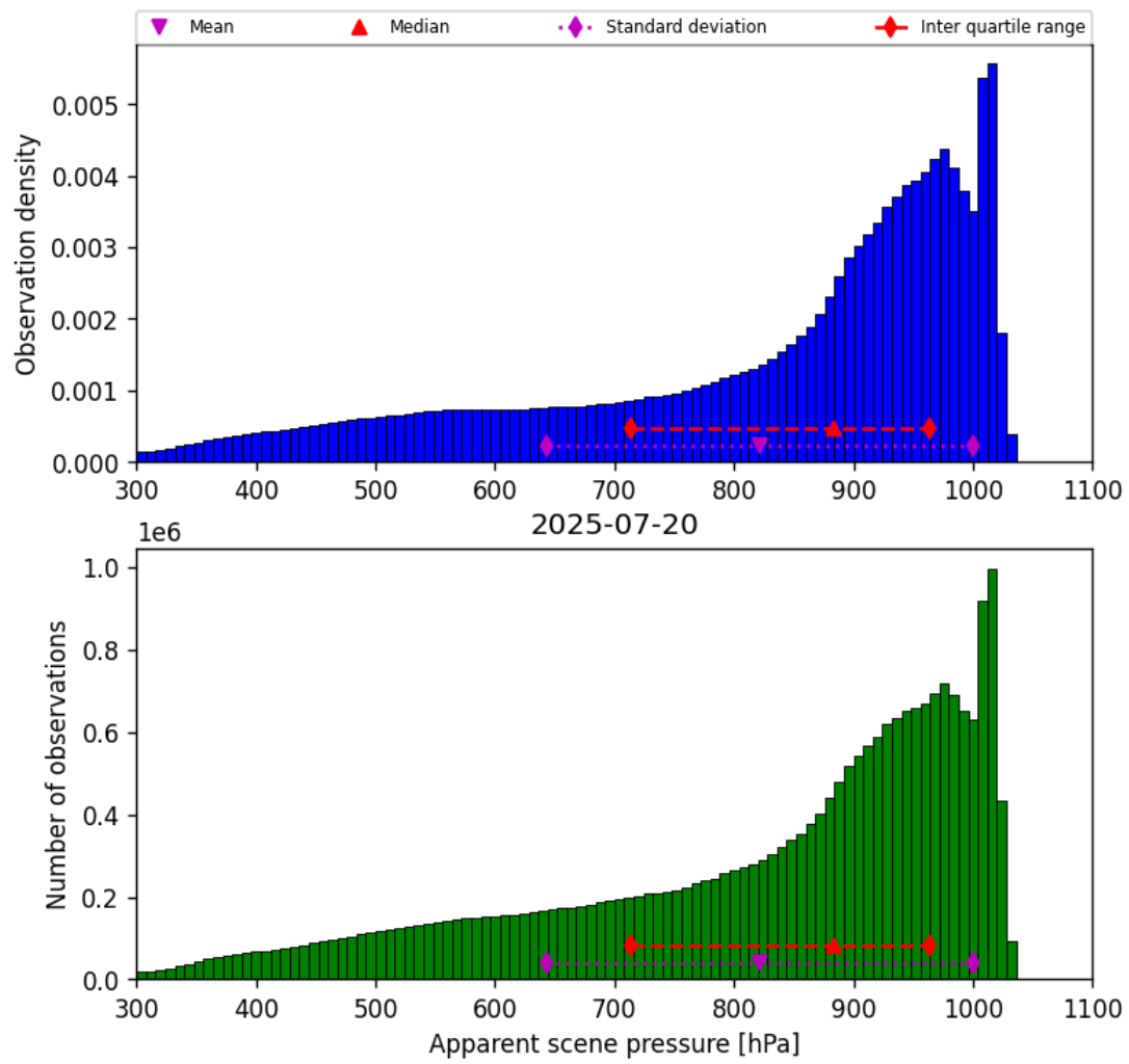
Figure 34: Histogram of “Apparent scene pressure” for 2025-07-20 to 2025-07-21
