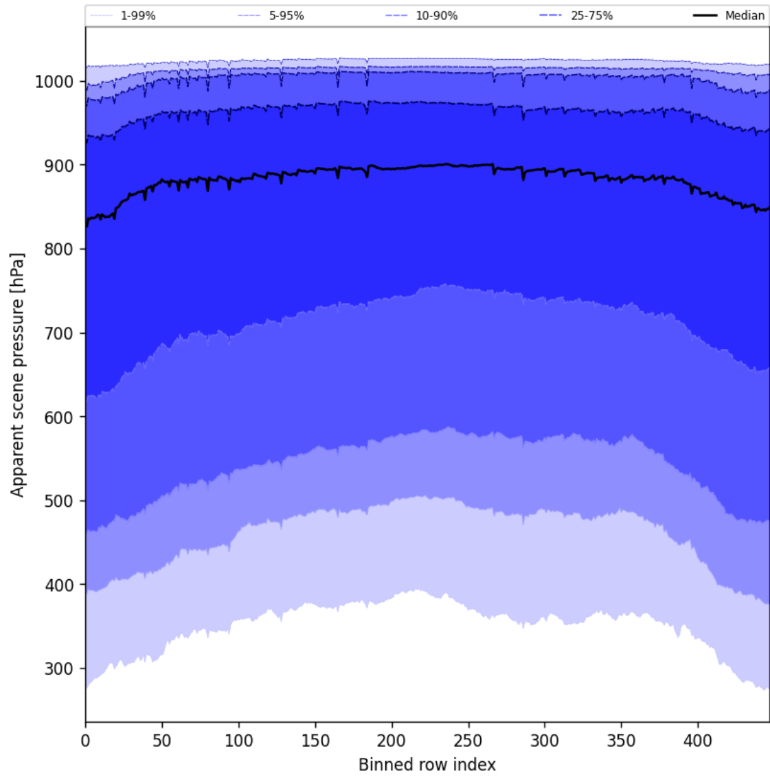
Figure 51: Along track statistics of “Apparent scene pressure” for 2025-07-20 to 2025-07-21
