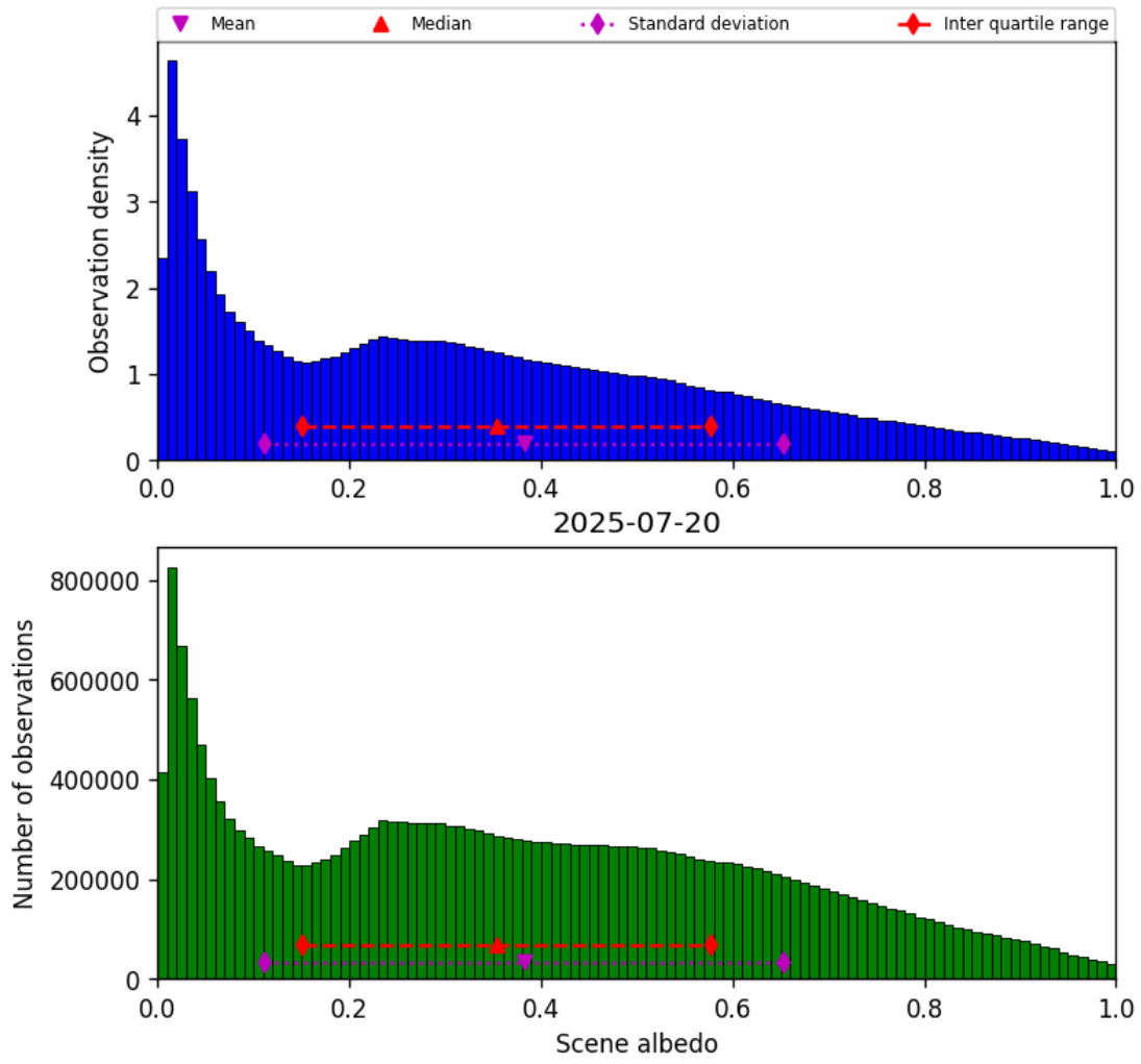
Figure 32: Histogram of “Scene albedo” for 2025-07-20 to 2025-07-21
