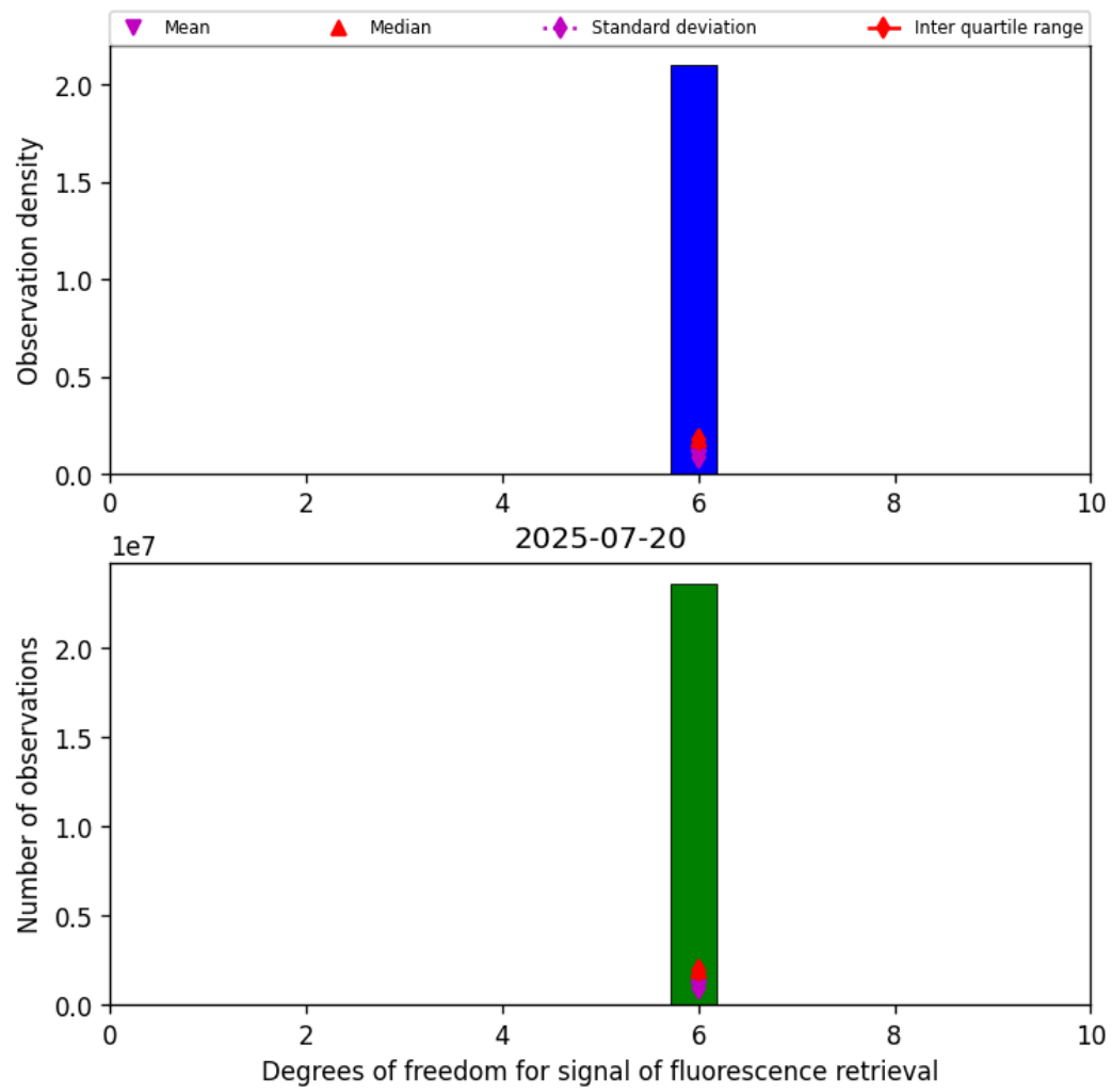
Figure 41: Histogram of “Degrees of freedom for signal of fluorescence retrieval” for 2025-07-20 to 2025-07-21
