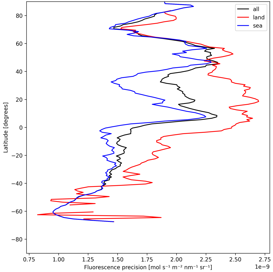
Figure 22: Zonal average of “Fluorescence precision” for 2025-07-20 to 2025-07-21.
