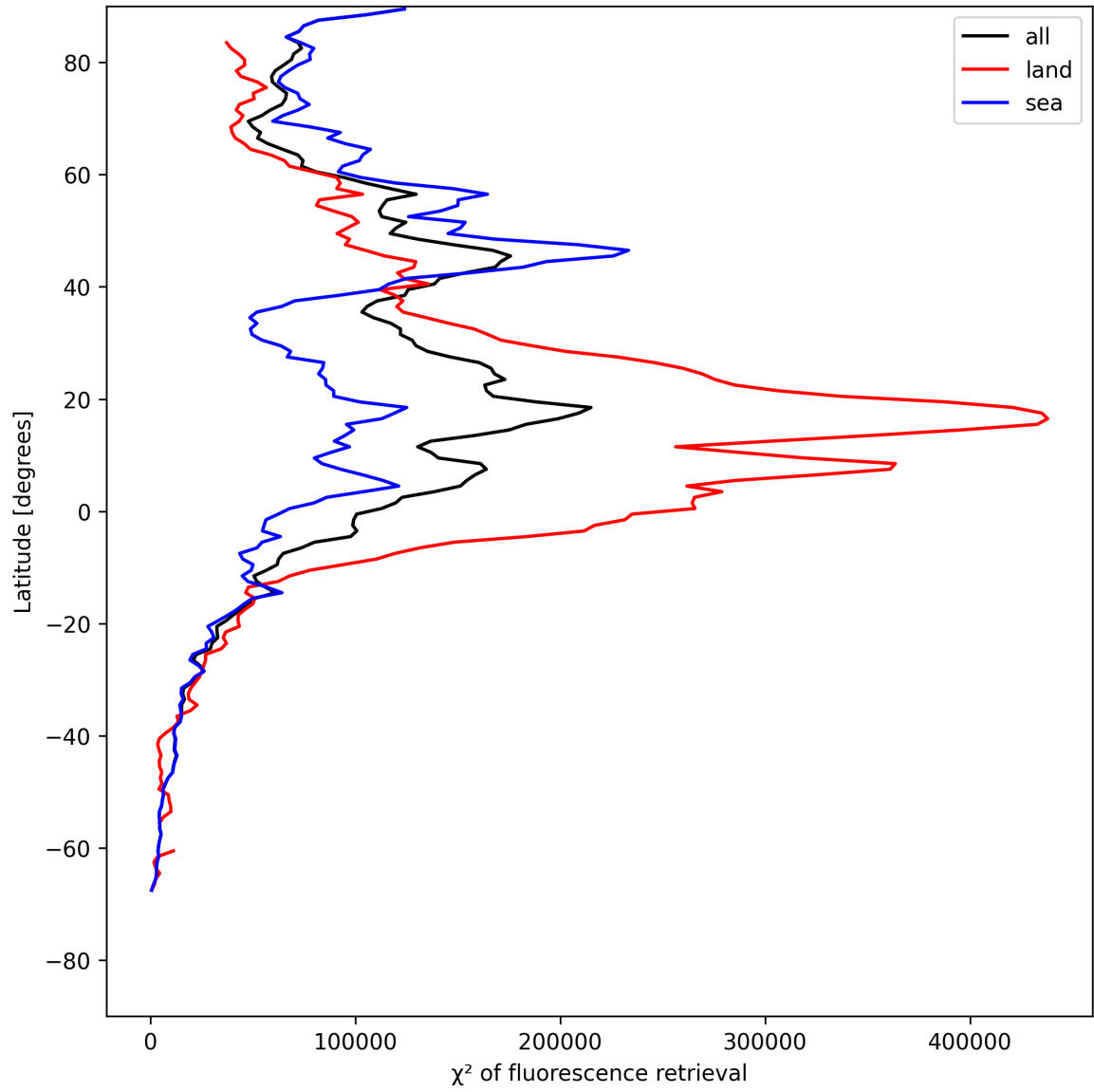
Figure 23: Zonal average of “ \chi^2 of fluorescence retrieval” for 2025-07-20 to 2025-07-21.
