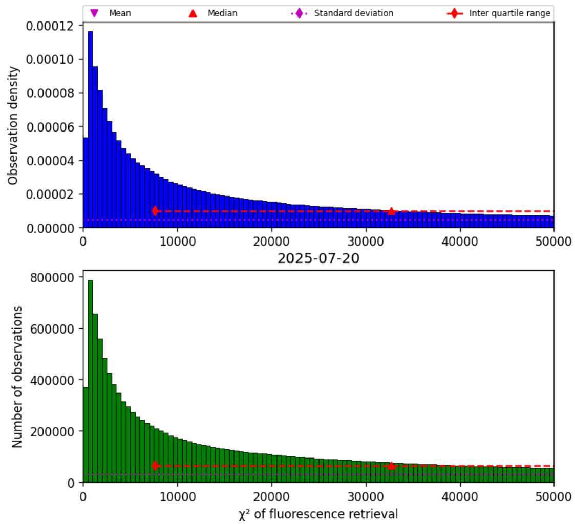
Figure 40: Histogram of “ \chi^2 of fluorescence retrieval” for 2025-07-20 to 2025-07-21
