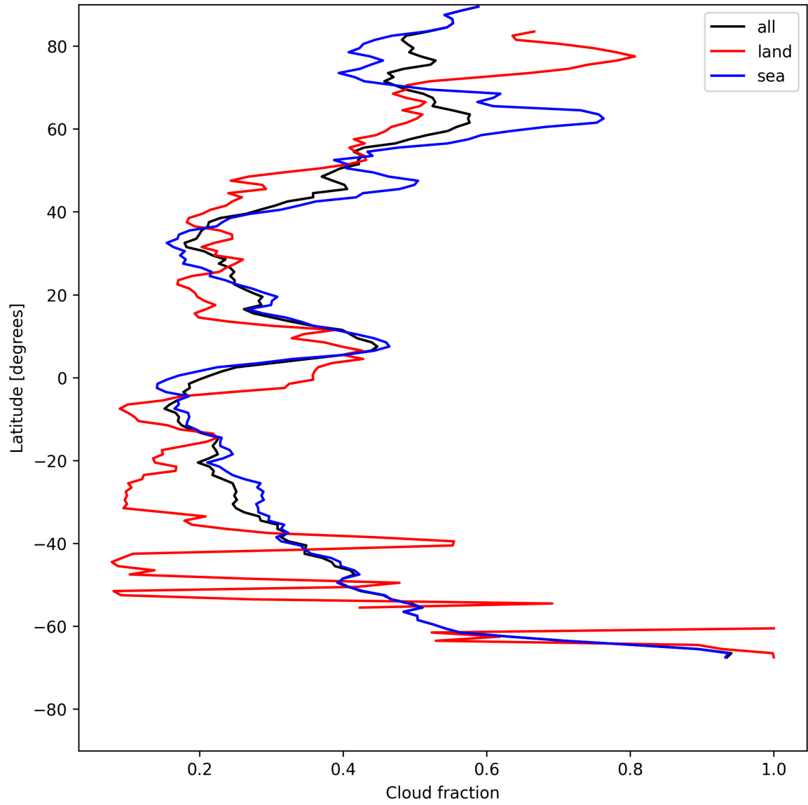
Figure 13: Zonal average of “Cloud fraction” for 2025-07-20 to 2025-07-21.
