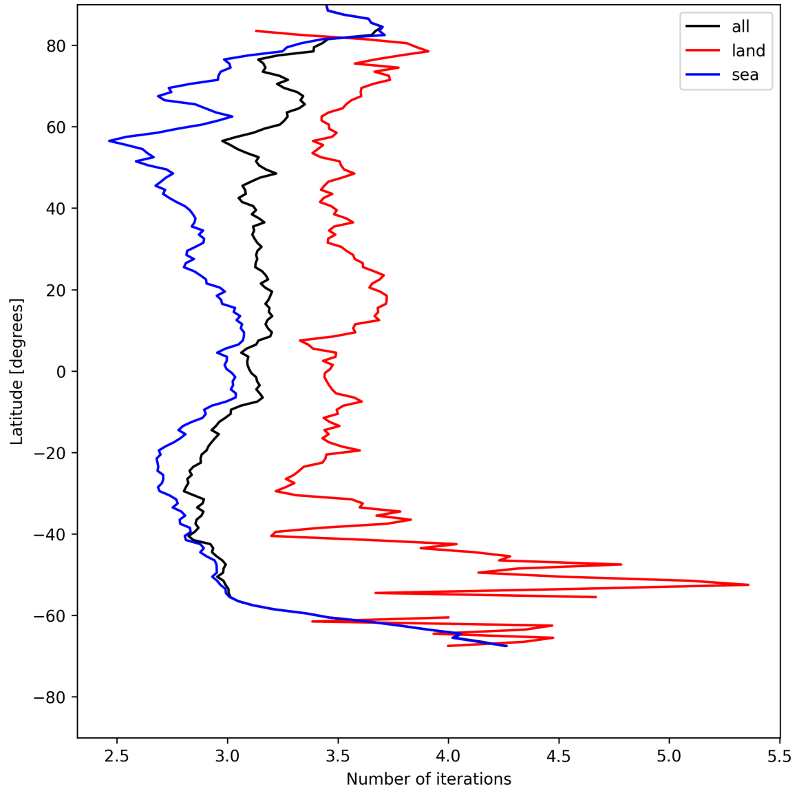
Figure 20: Zonal average of “Number of iterations” for 2025-07-20 to 2025-07-21.
