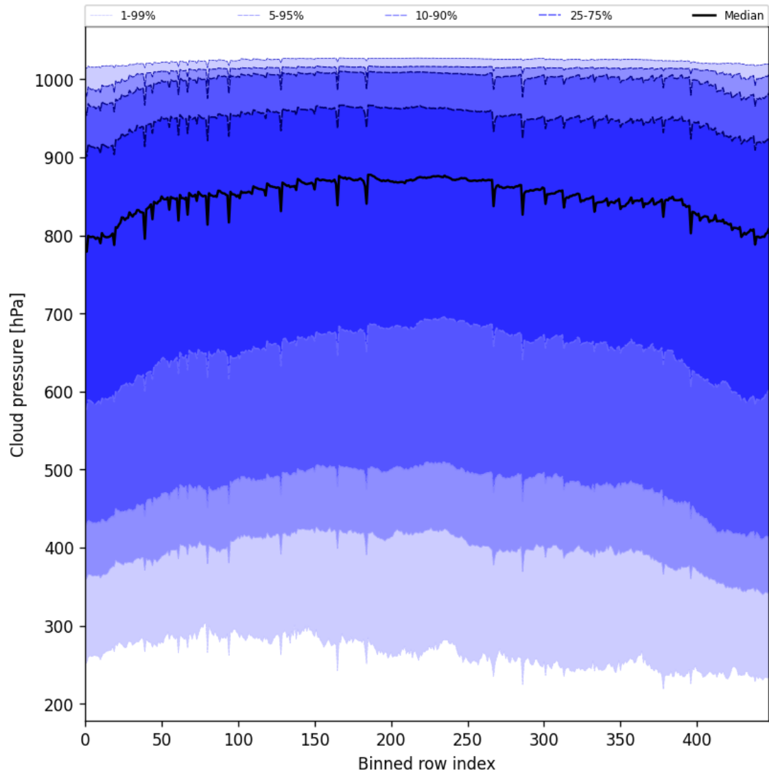
Figure 45: Along track statistics of “Cloud pressure” for 2025-07-20 to 2025-07-21
