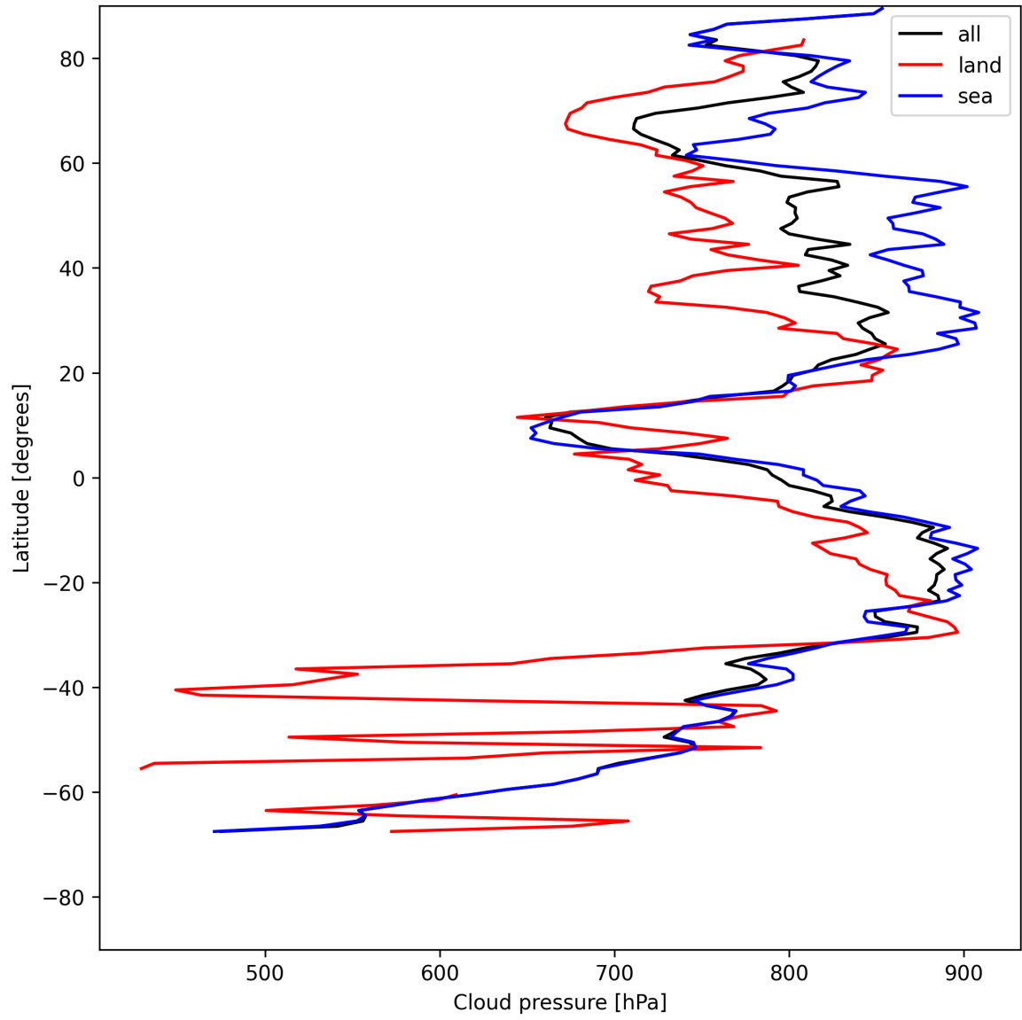
Figure 11: Zonal average of “Cloud pressure” for 2025-07-20 to 2025-07-21.
