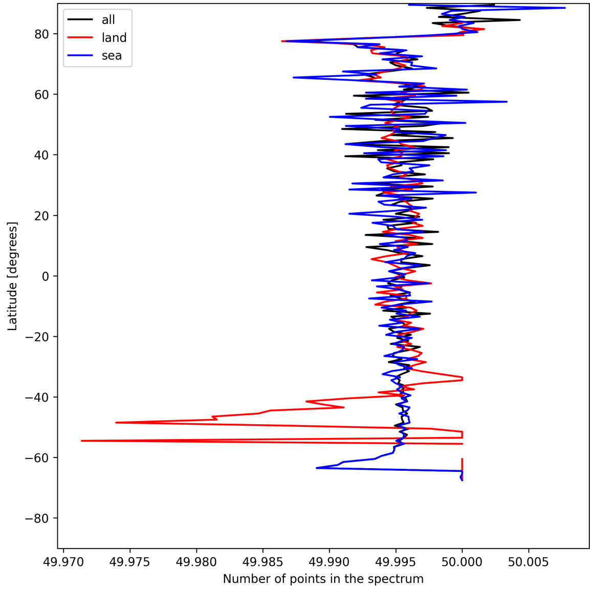
Figure 25: Zonal average of “Number of points in the spectrum” for 2025-07-20 to 2025-07-21.
