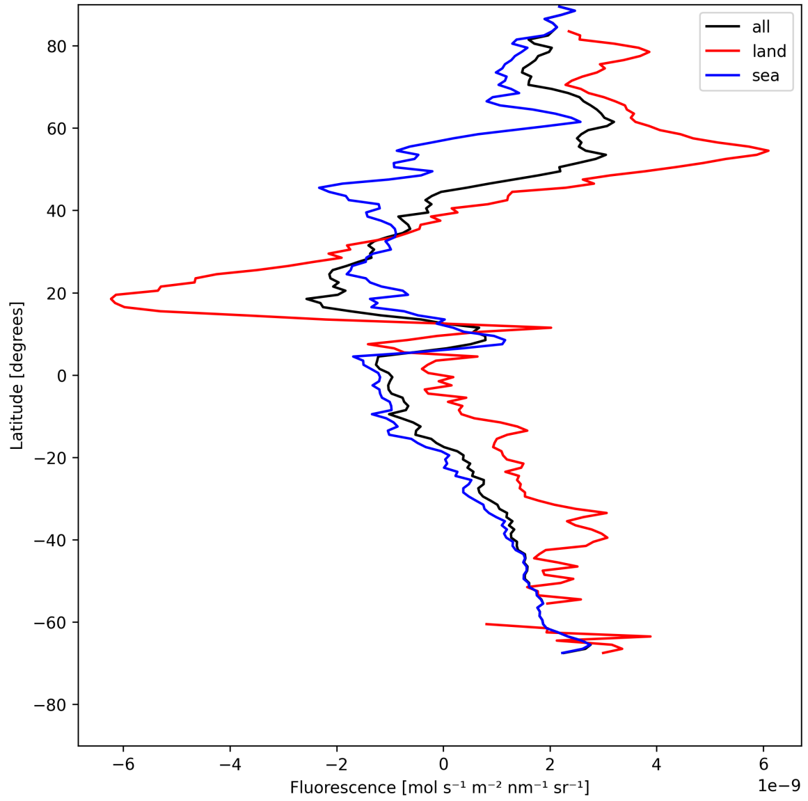
Figure 21: Zonal average of “Fluorescence” for 2025-07-20 to 2025-07-21.
