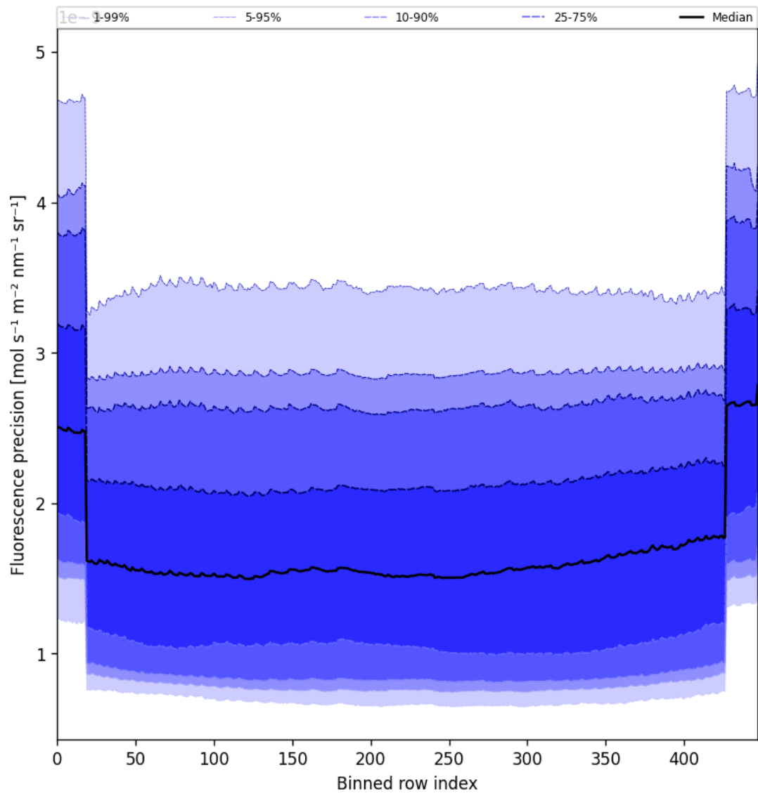
Figure 56: Along track statistics of “Fluorescence precision” for 2025-07-20 to 2025-07-21
