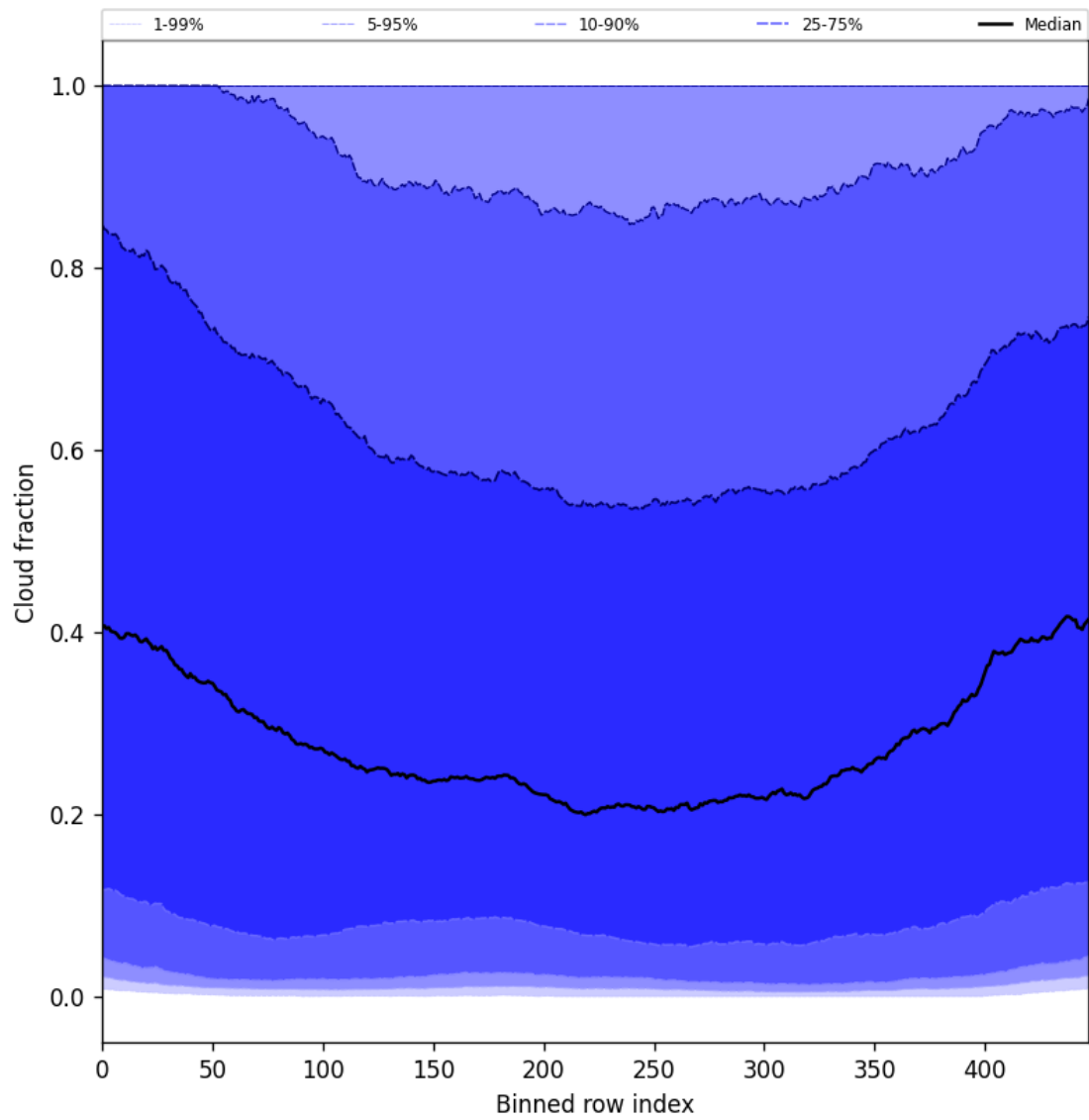
Figure 47: Along track statistics of “Cloud fraction” for 2025-07-20 to 2025-07-21
