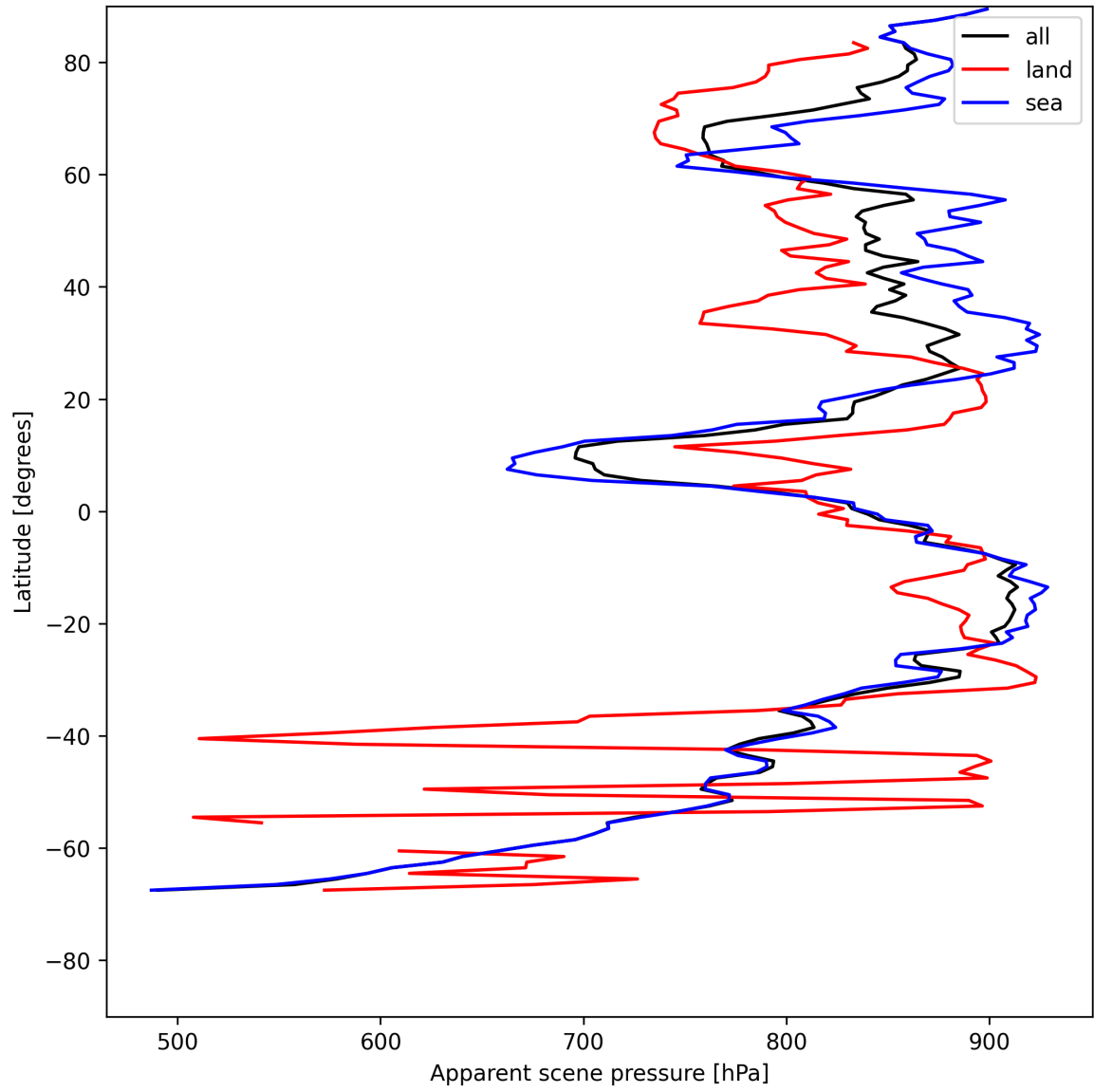
Figure 17: Zonal average of “Apparent scene pressure” for 2025-07-20 to 2025-07-21.
