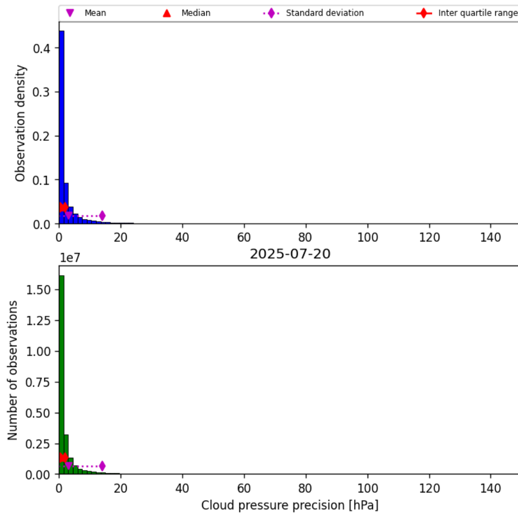
Figure 29: Histogram of “Cloud pressure precision” for 2025-07-20 to 2025-07-21
