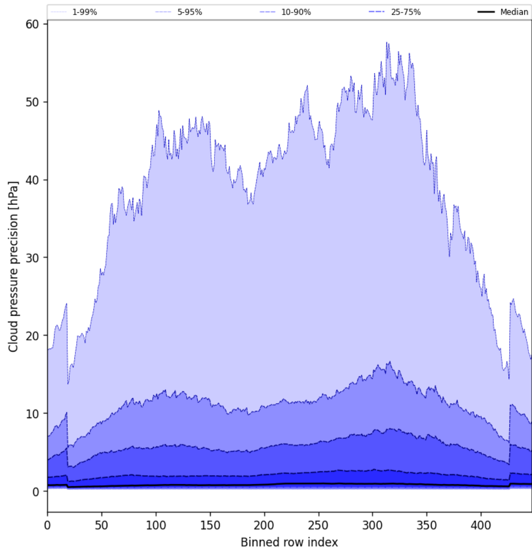
Figure 46: Along track statistics of “Cloud pressure precision” for 2025-07-20 to 2025-07-21
