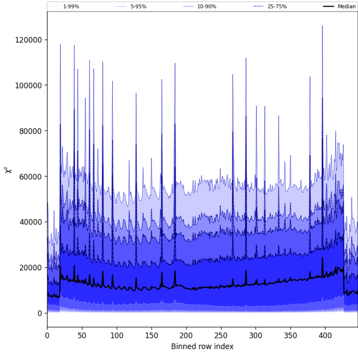
Figure 53: Along track statistics of “ \chi^2 ” for 2025-07-20 to 2025-07-21
