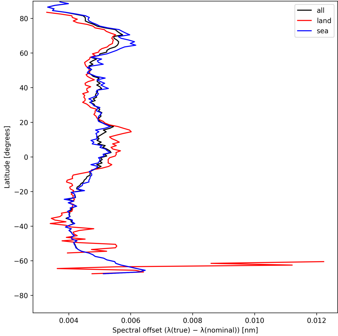
Figure 26: Zonal average of “Spectral offset ( \lambda_{\text{true}} - \lambda_{\text{nominal}} )” for 2025-07-20 to 2025-07-21.
