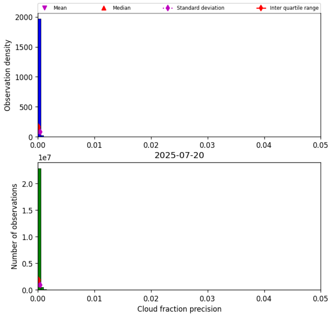
Figure 31: Histogram of “Cloud fraction precision” for 2025-07-20 to 2025-07-21
