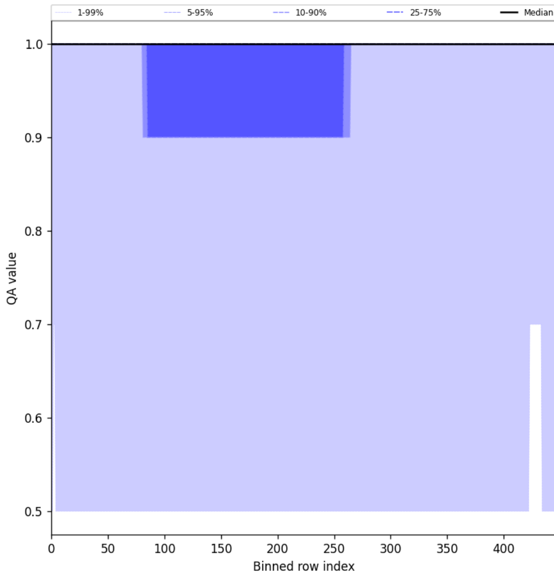
Figure 44: Along track statistics of “QA value” for 2025-07-20 to 2025-07-21
