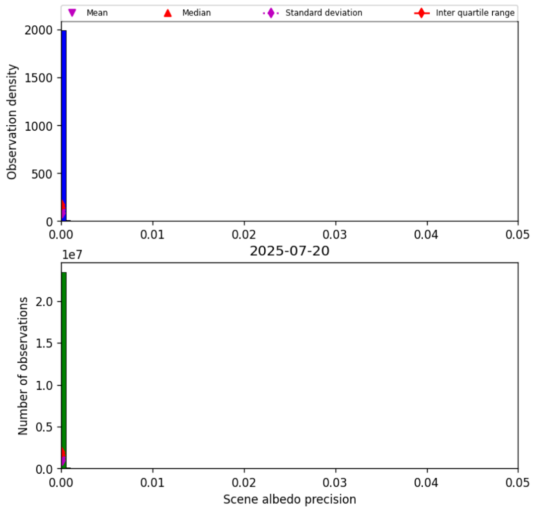
Figure 33: Histogram of “Scene albedo precision” for 2025-07-20 to 2025-07-21
