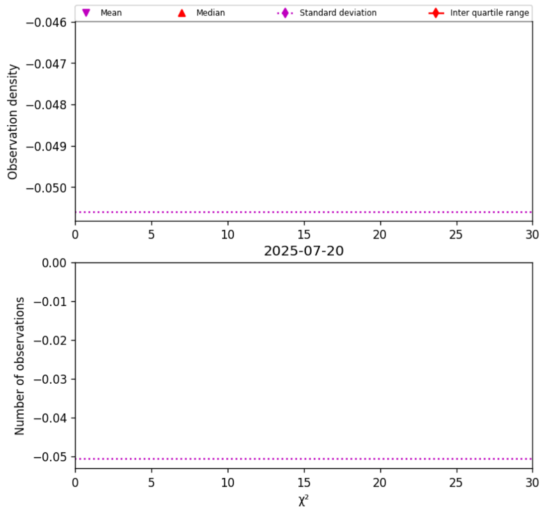
Figure 36: Histogram of " \chi^2 " for 2025-07-20 to 2025-07-21
