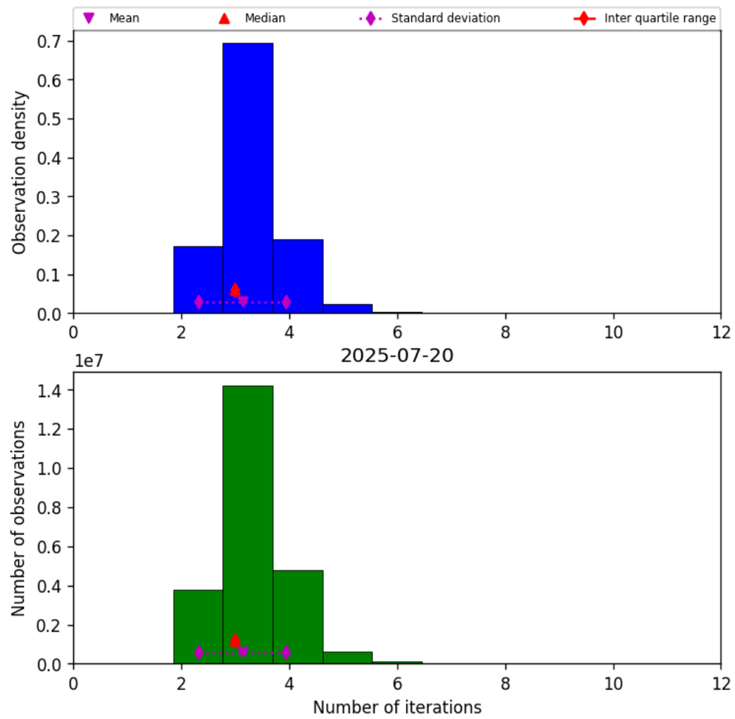
Figure 37: Histogram of “Number of iterations” for 2025-07-20 to 2025-07-21
