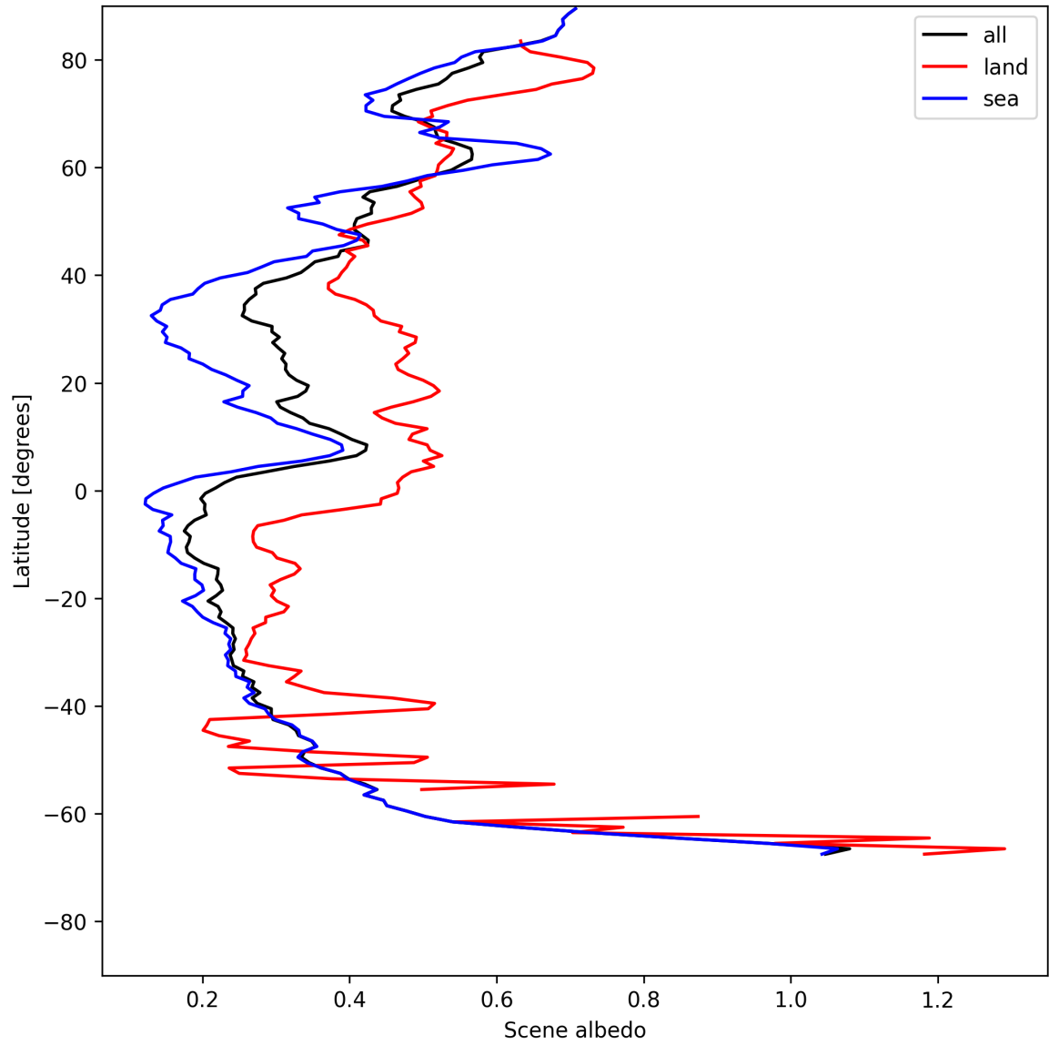
Figure 15: Zonal average of “Scene albedo” for 2025-07-20 to 2025-07-21.
