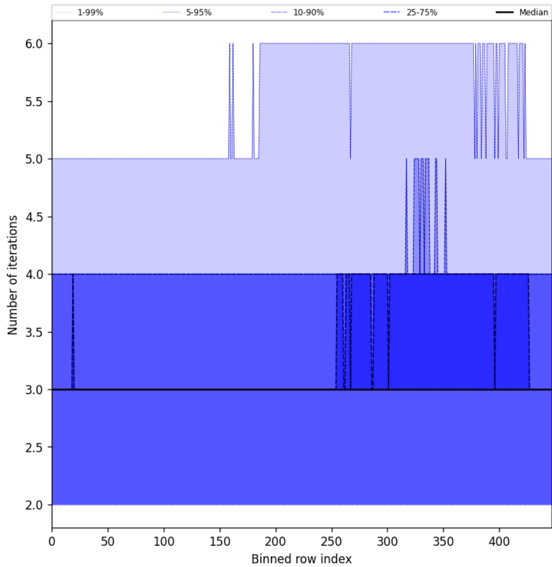
Figure 54: Along track statistics of “Number of iterations” for 2025-07-20 to 2025-07-21
