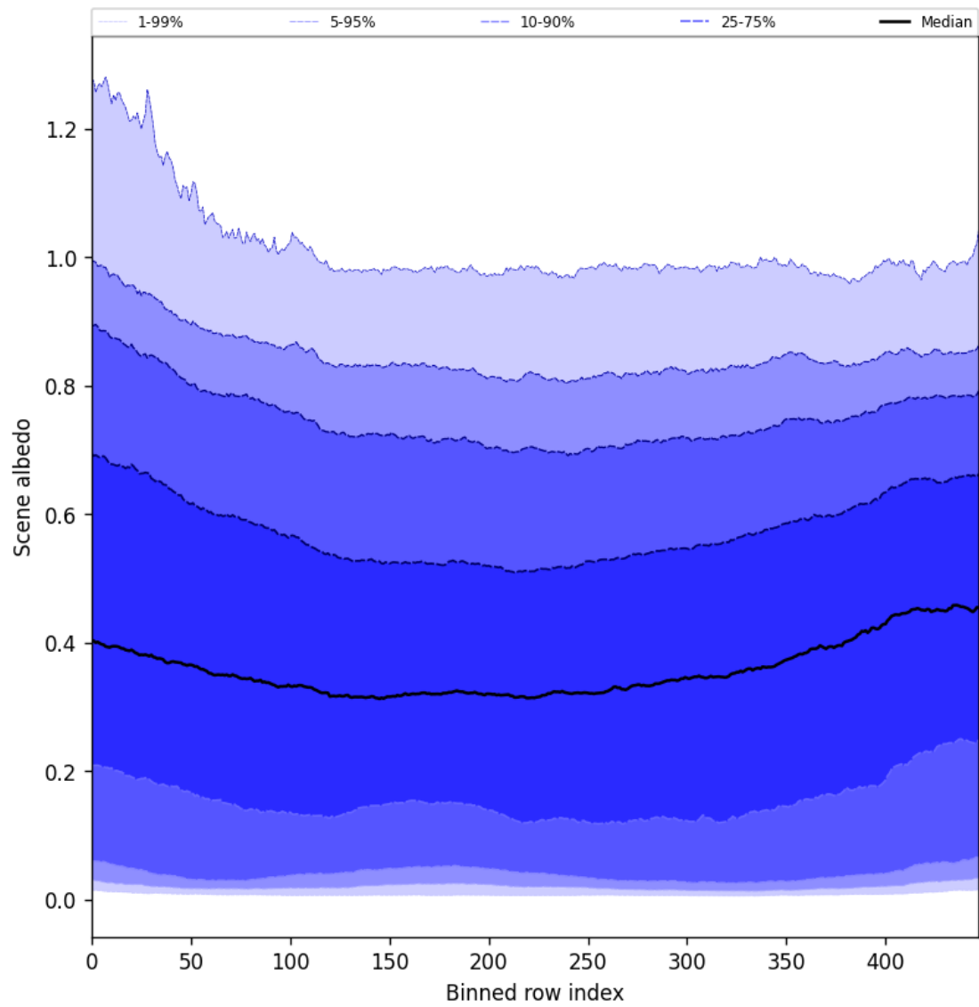
Figure 49: Along track statistics of “Scene albedo” for 2025-07-20 to 2025-07-21
