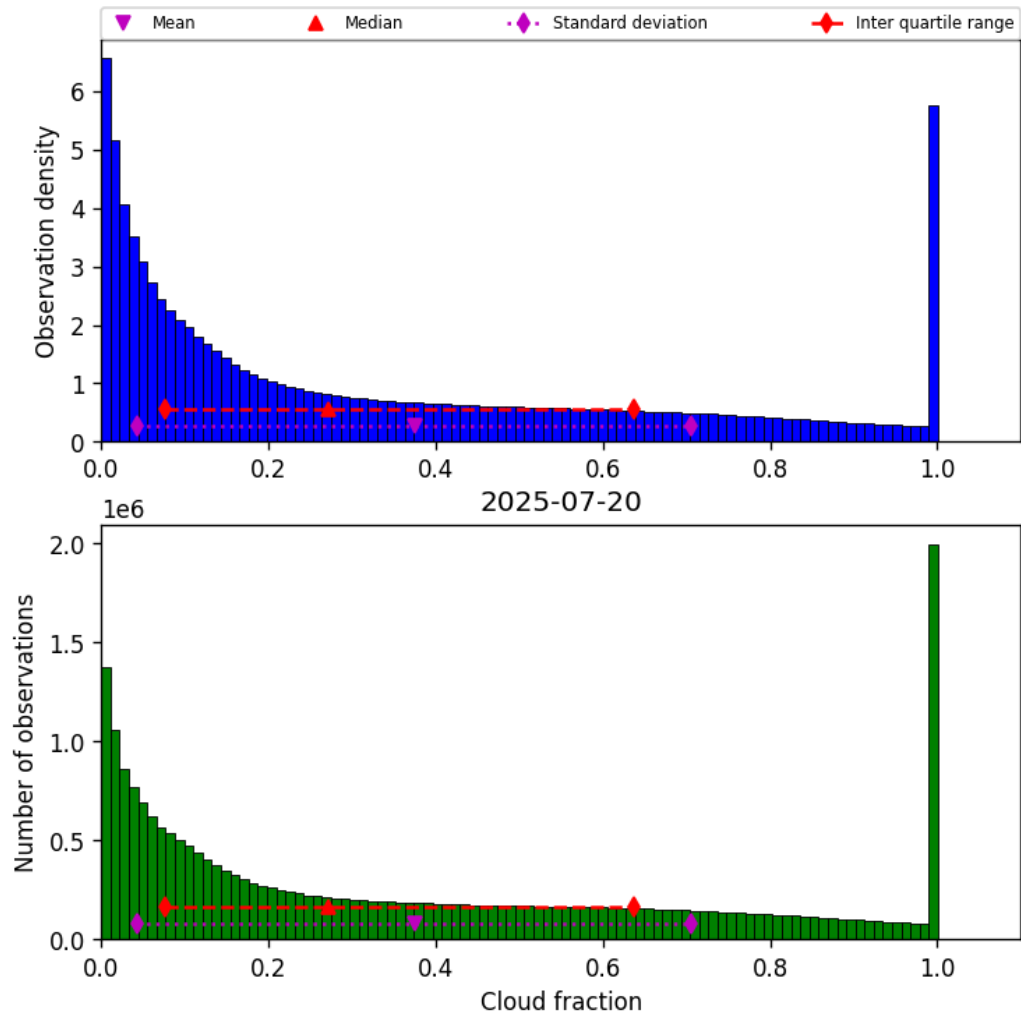
Figure 30: Histogram of “Cloud fraction” for 2025-07-20 to 2025-07-21
