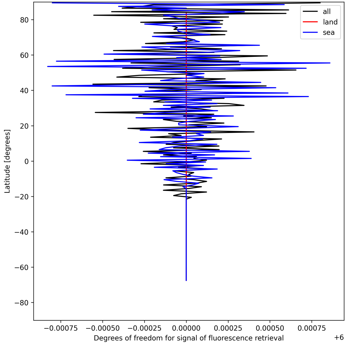
Figure 24: Zonal average of “Degrees of freedom for signal of fluorescence retrieval” for 2025-07-20 to 2025-07-21.
