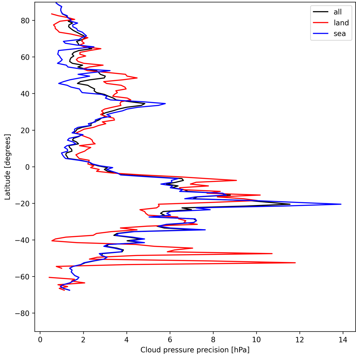
Figure 12: Zonal average of "Cloud pressure precision" for 2025-07-20 to 2025-07-21.
