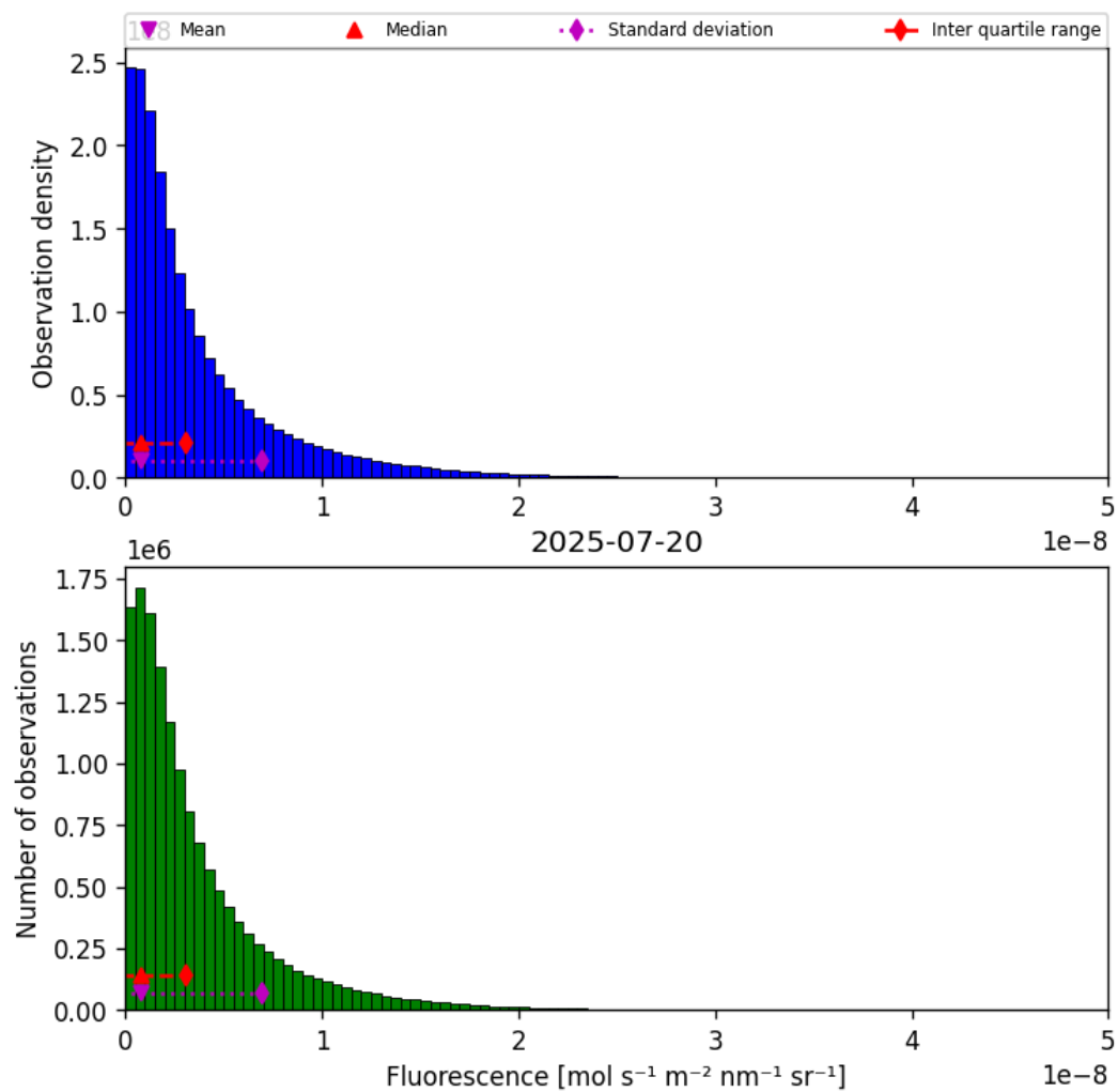
Figure 38: Histogram of “Fluorescence” for 2025-07-20 to 2025-07-21
