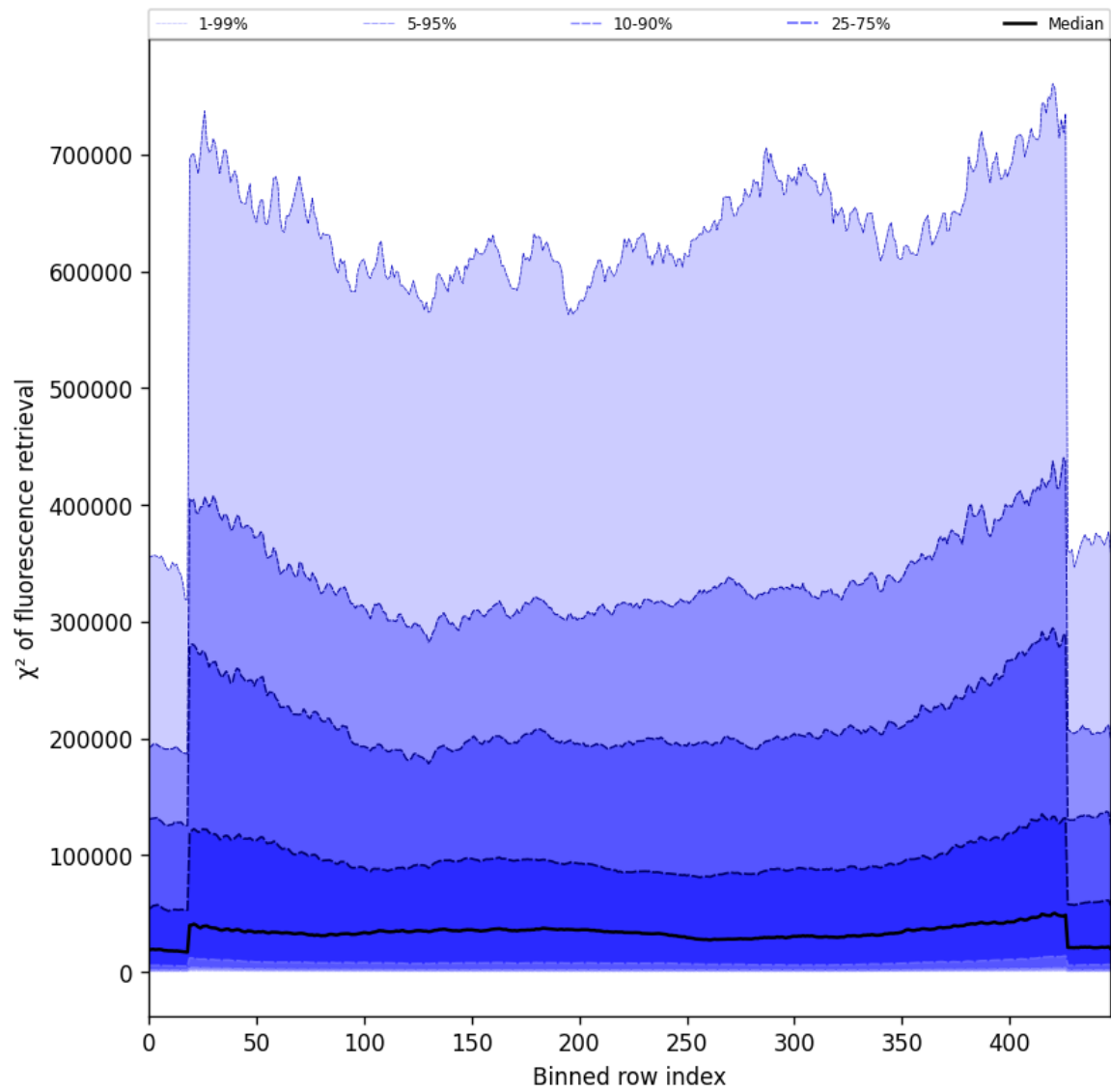
Figure 57: Along track statistics of “ \chi^2 of fluorescence retrieval” for 2025-07-20 to 2025-07-21
