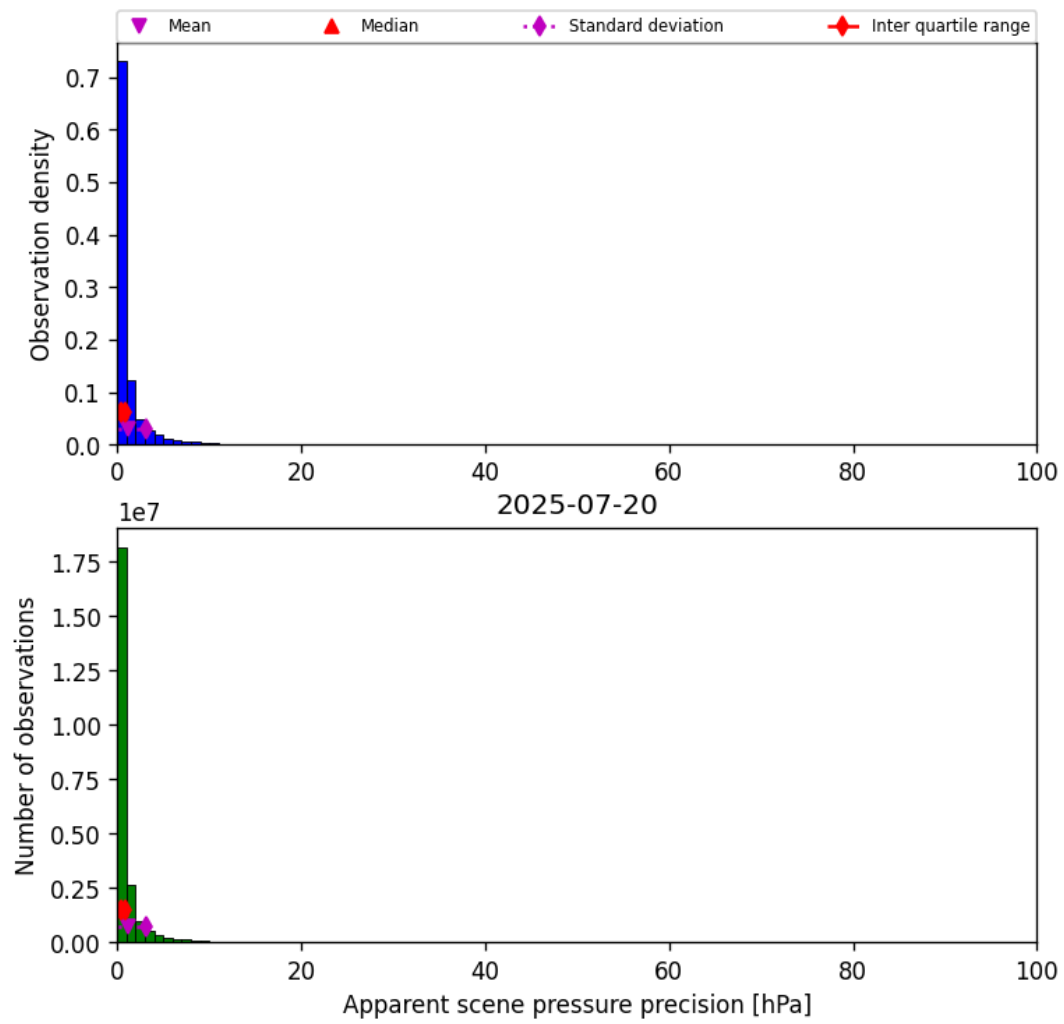
Figure 35: Histogram of “Apparent scene pressure precision” for 2025-07-20 to 2025-07-21
