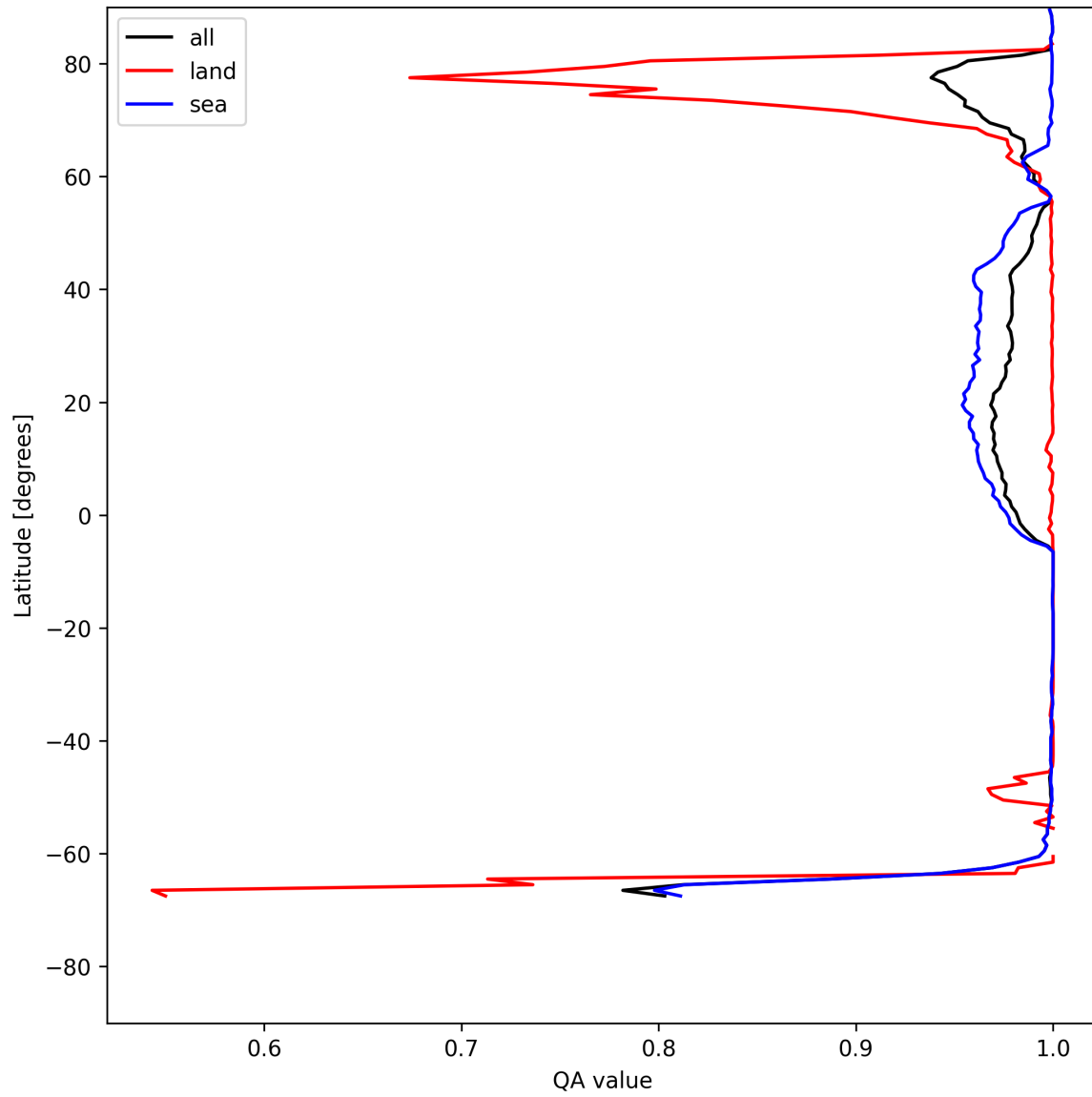
Figure 10: Zonal average of "QA value" for 2025-07-20 to 2025-07-21.
