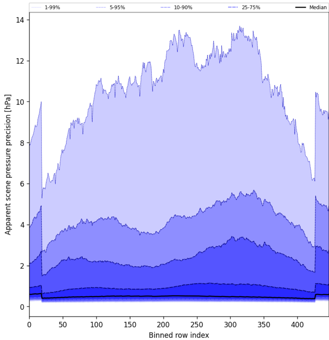
Figure 52: Along track statistics of “Apparent scene pressure precision” for 2025-07-20 to 2025-07-21
