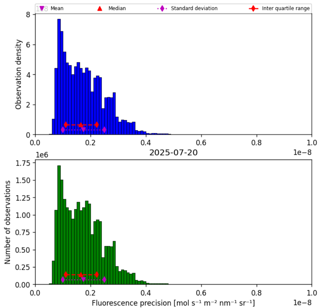
Figure 39: Histogram of “Fluorescence precision” for 2025-07-20 to 2025-07-21
