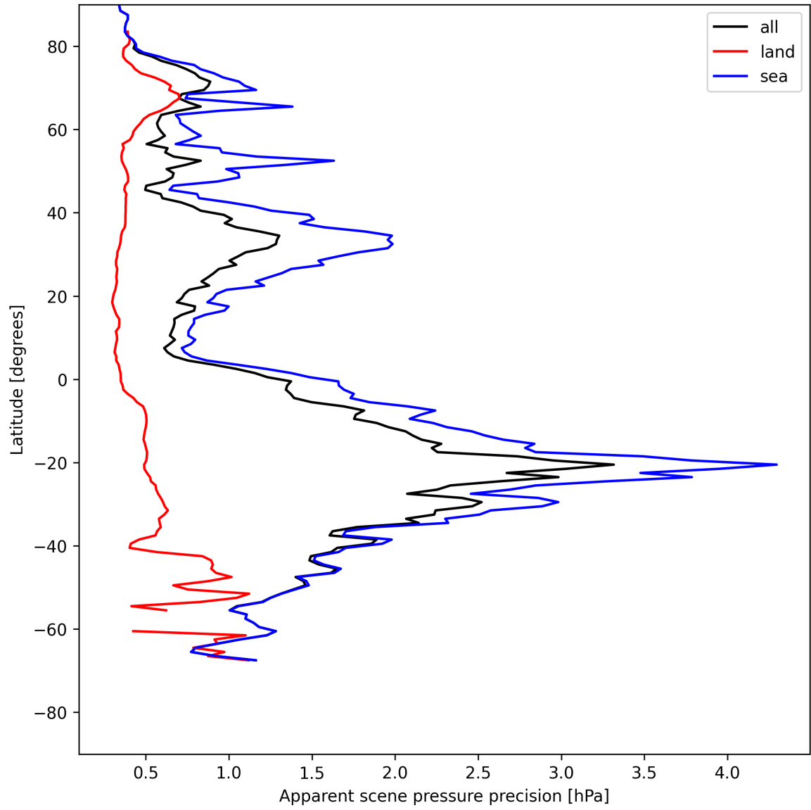
Figure 18: Zonal average of “Apparent scene pressure precision” for 2025-07-20 to 2025-07-21.
