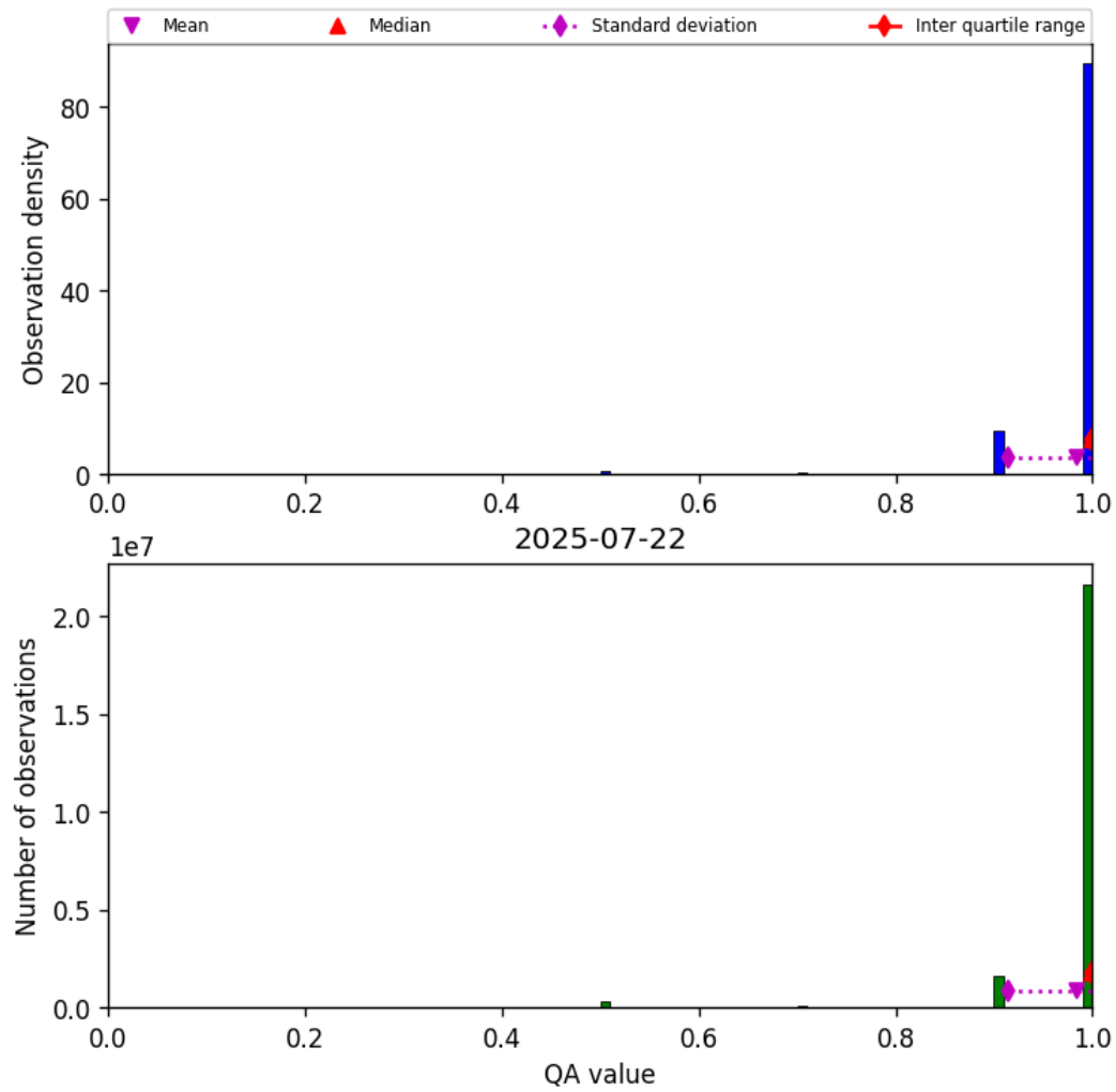
Figure 27: Histogram of “QA value” for 2025-07-22 to 2025-07-22
