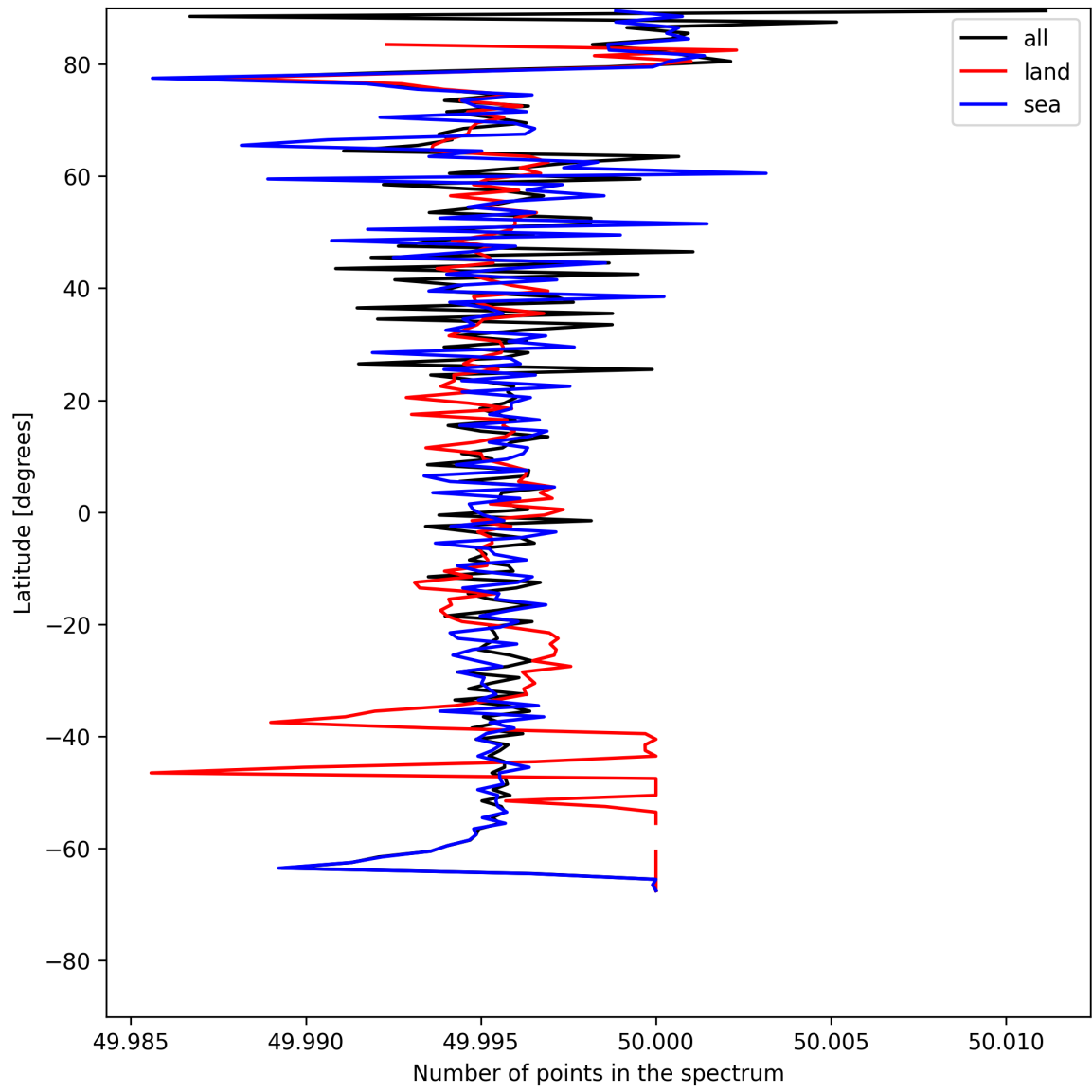
Figure 25: Zonal average of “Number of points in the spectrum” for 2025-07-22 to 2025-07-22.
