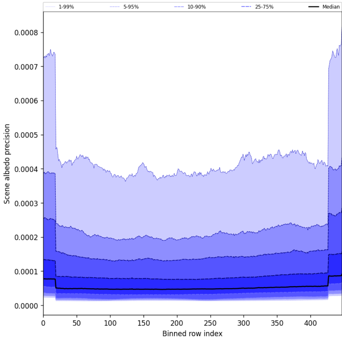
Figure 50: Along track statistics of “Scene albedo precision” for 2025-07-22 to 2025-07-22
