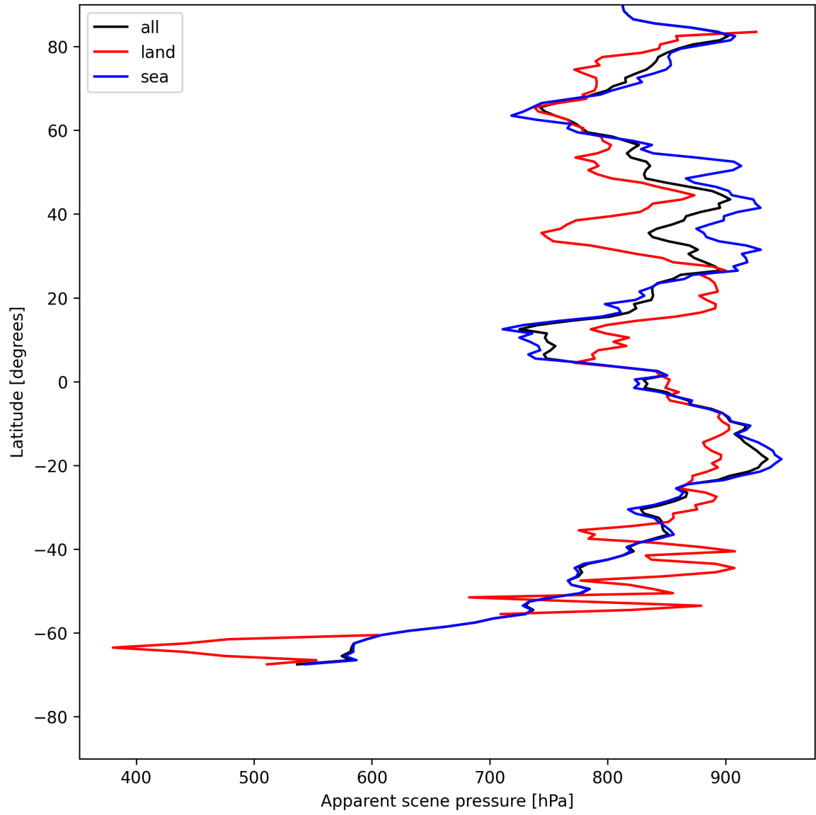
Figure 17: Zonal average of “Apparent scene pressure” for 2025-07-22 to 2025-07-22.
