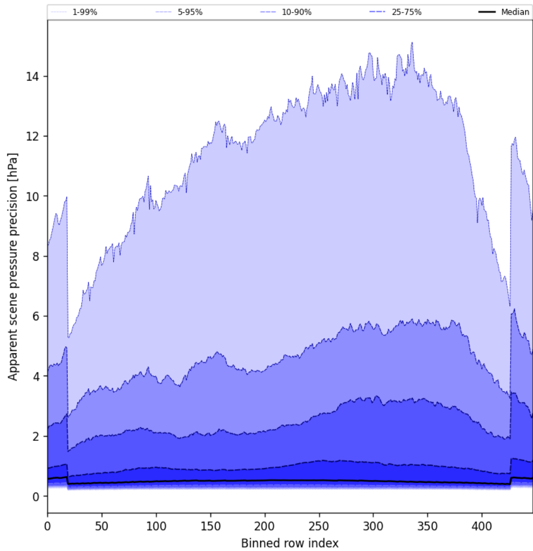
Figure 52: Along track statistics of “Apparent scene pressure precision” for 2025-07-22 to 2025-07-22
