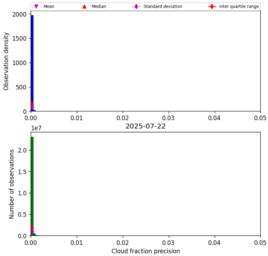
Figure 31: Histogram of “Cloud fraction precision” for 2025-07-22 to 2025-07-22
