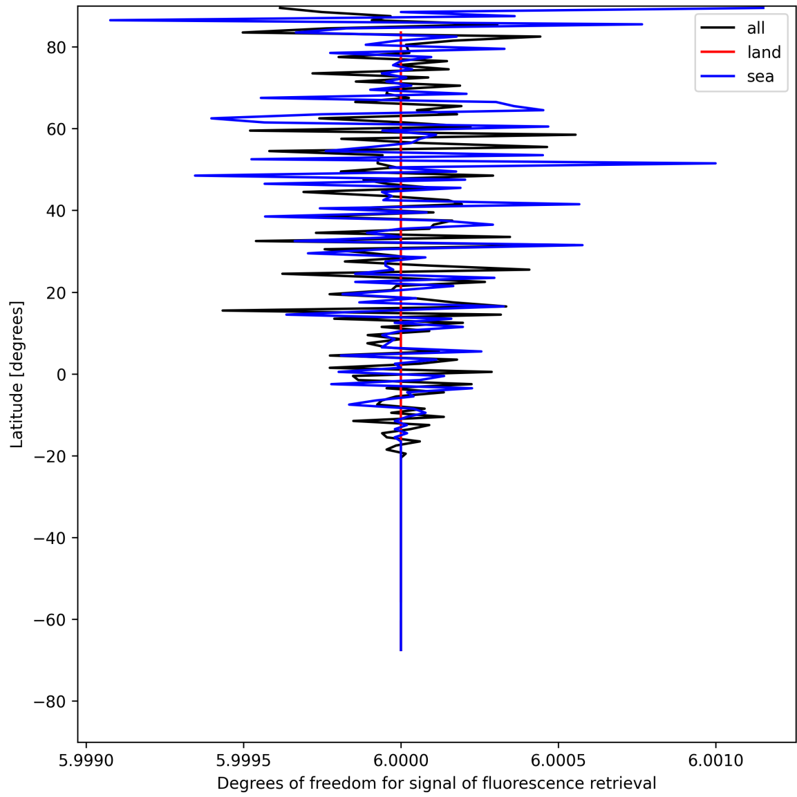
Figure 24: Zonal average of “Degrees of freedom for signal of fluorescence retrieval” for 2025-07-22 to 2025-07-22.
