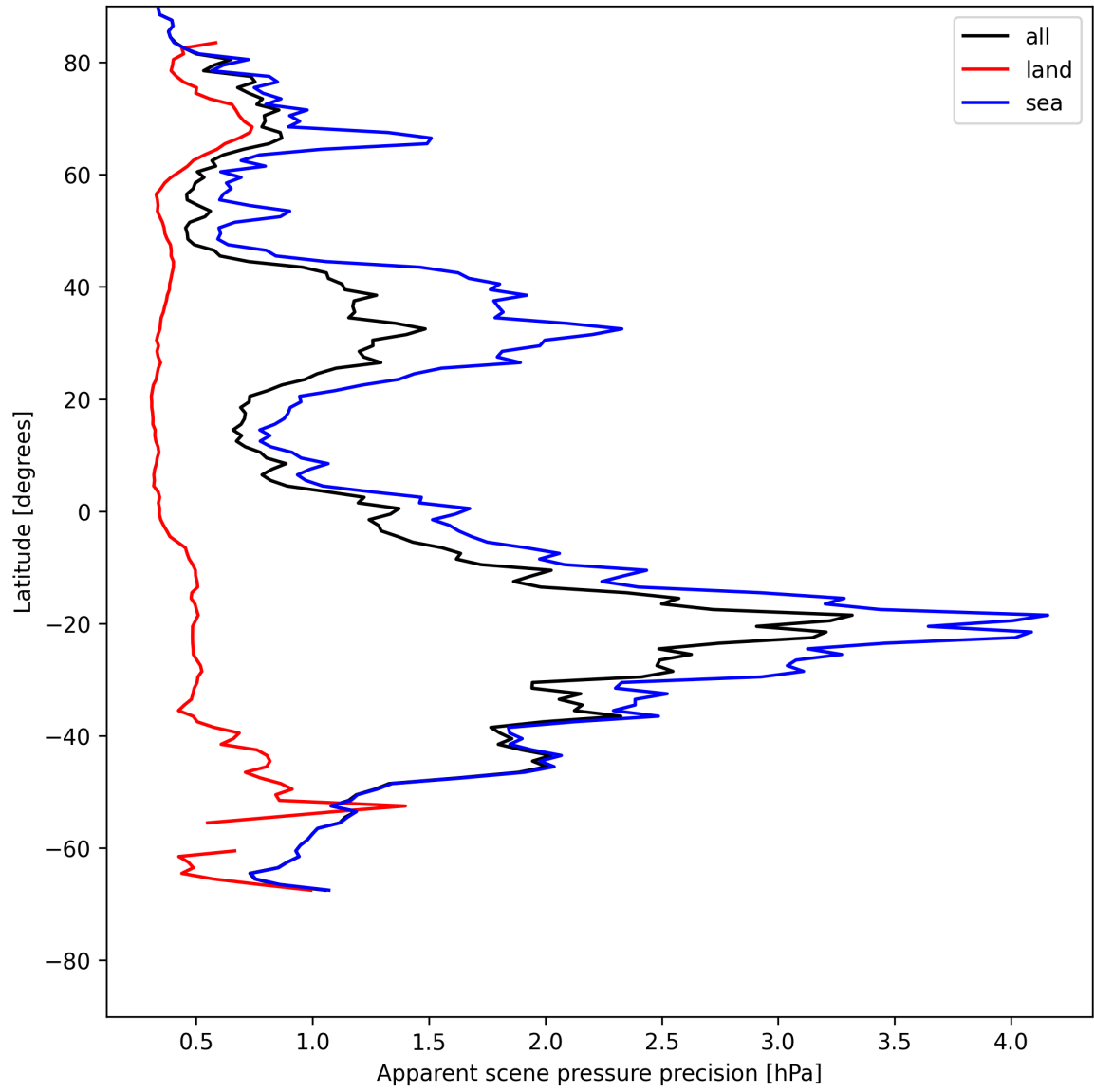
Figure 18: Zonal average of “Apparent scene pressure precision” for 2025-07-22 to 2025-07-22.
