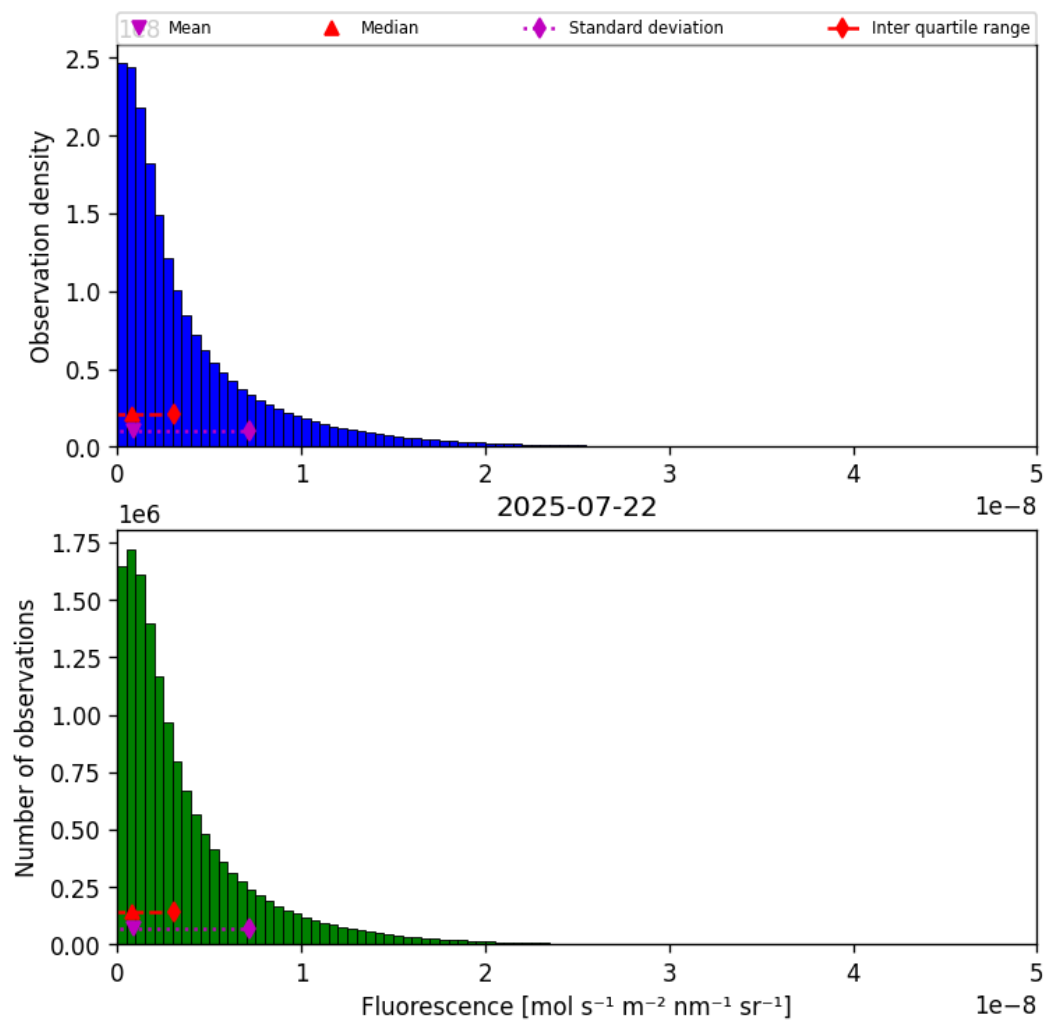
Figure 38: Histogram of “Fluorescence” for 2025-07-22 to 2025-07-22
