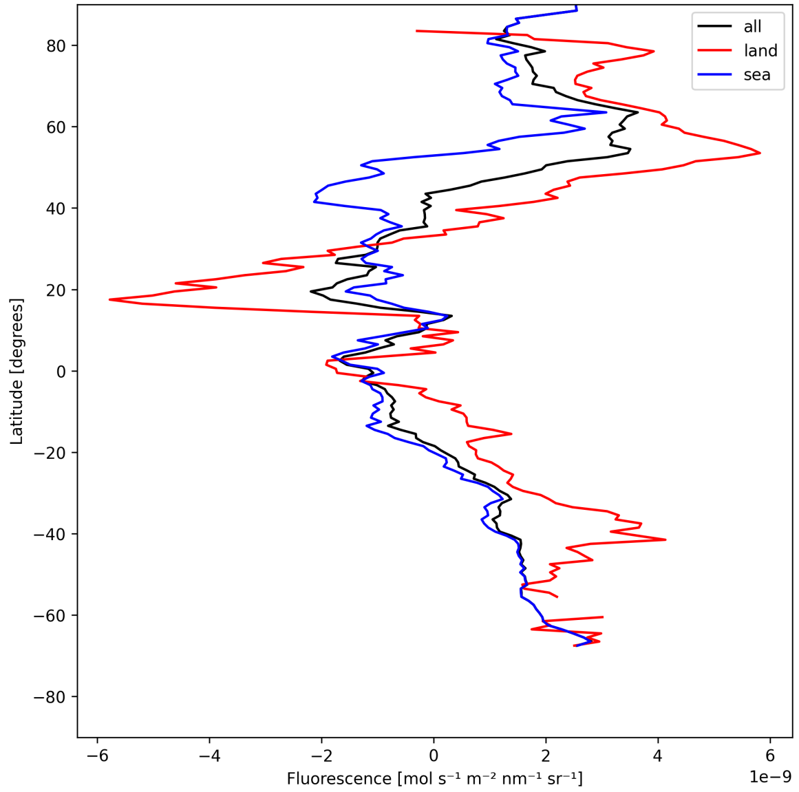
Figure 21: Zonal average of “Fluorescence” for 2025-07-22 to 2025-07-22.
