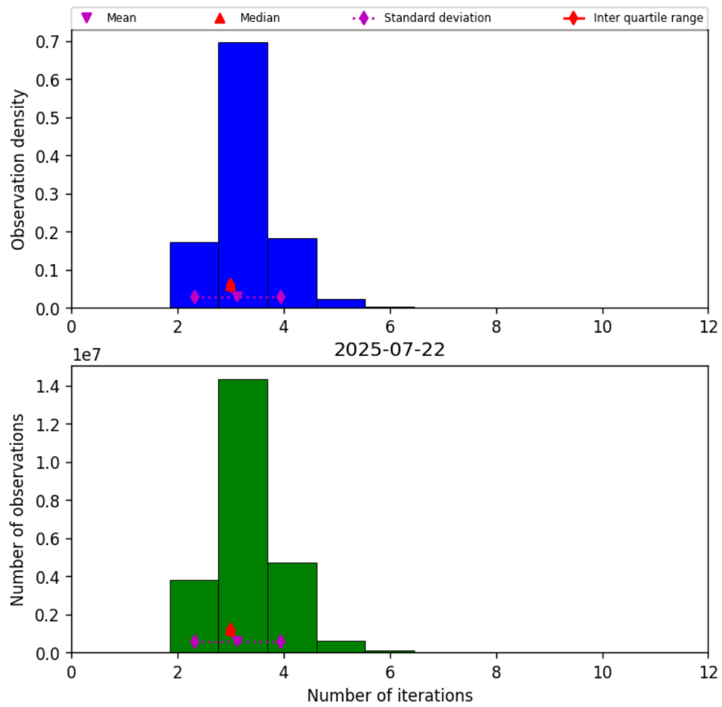
Figure 37: Histogram of “Number of iterations” for 2025-07-22 to 2025-07-22
