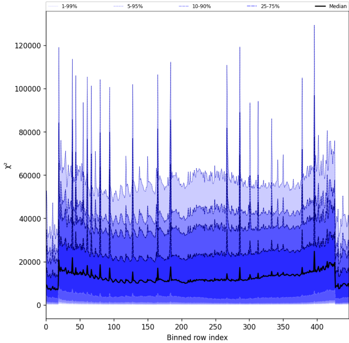
Figure 53: Along track statistics of “ \chi^2 ” for 2025-07-22 to 2025-07-22
