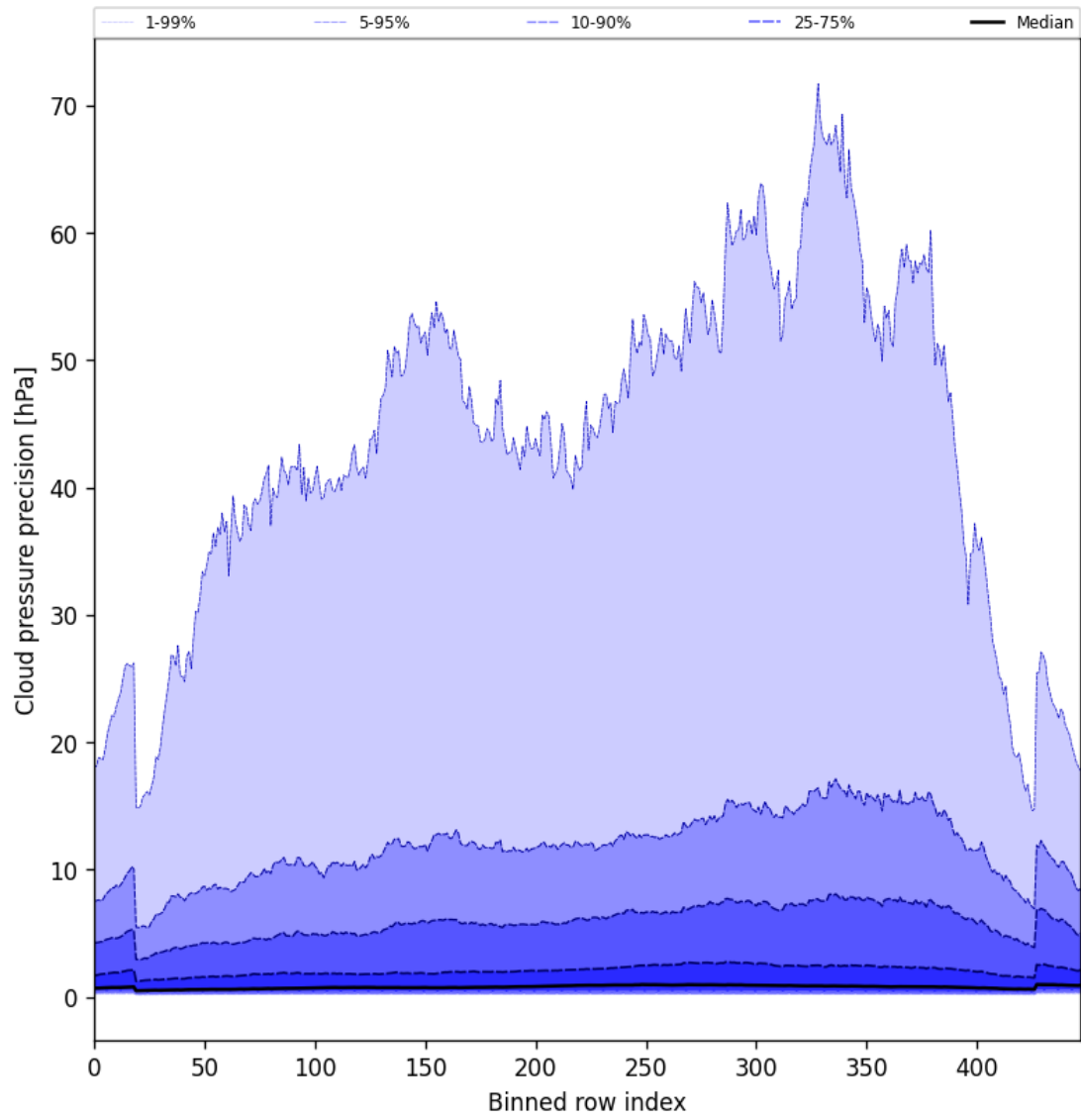
Figure 46: Along track statistics of “Cloud pressure precision” for 2025-07-22 to 2025-07-22
