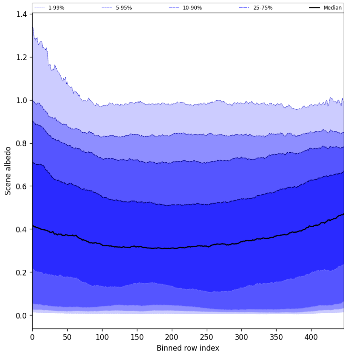
Figure 49: Along track statistics of “Scene albedo” for 2025-07-22 to 2025-07-22
