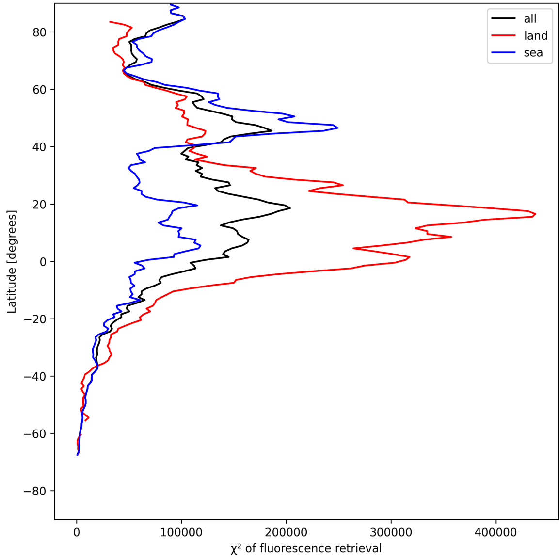
Figure 23: Zonal average of “ \chi^2 of fluorescence retrieval” for 2025-07-22 to 2025-07-22.
