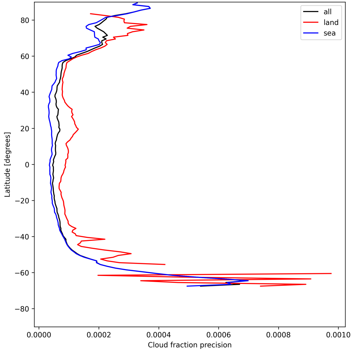
Figure 14: Zonal average of “Cloud fraction precision” for 2025-07-22 to 2025-07-22.
