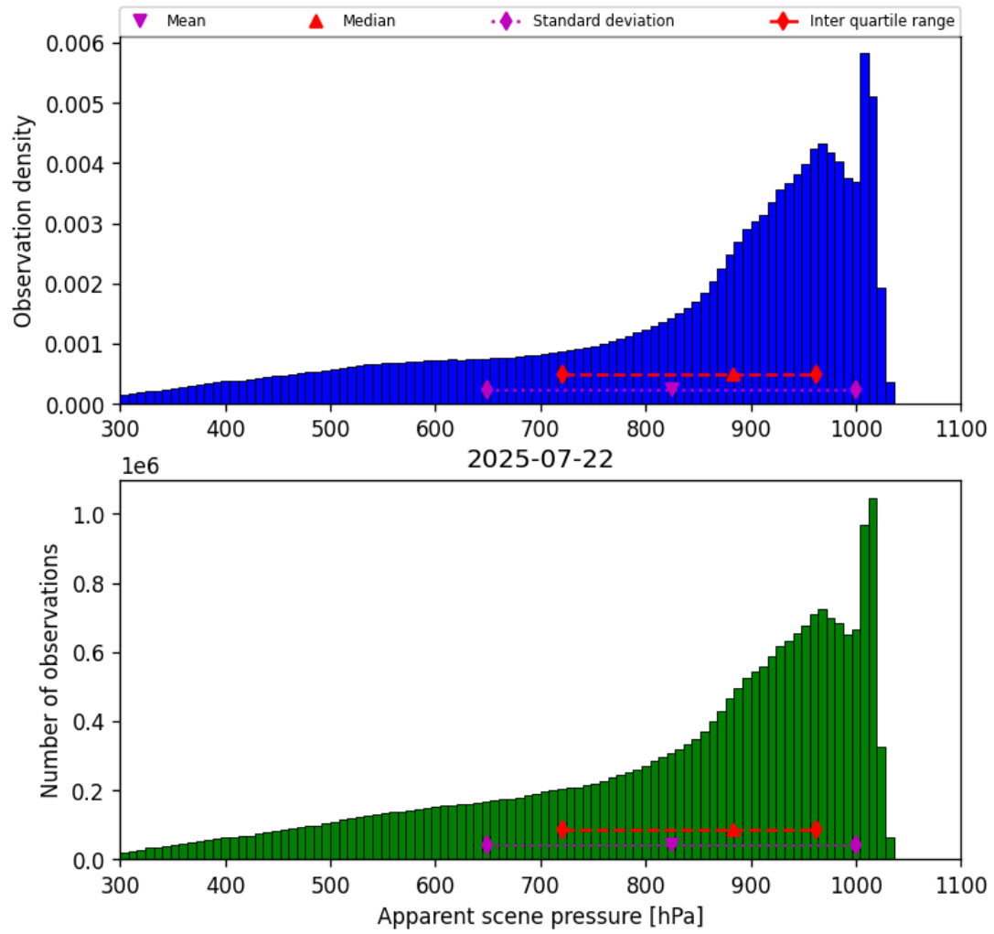
Figure 34: Histogram of “Apparent scene pressure” for 2025-07-22 to 2025-07-22
