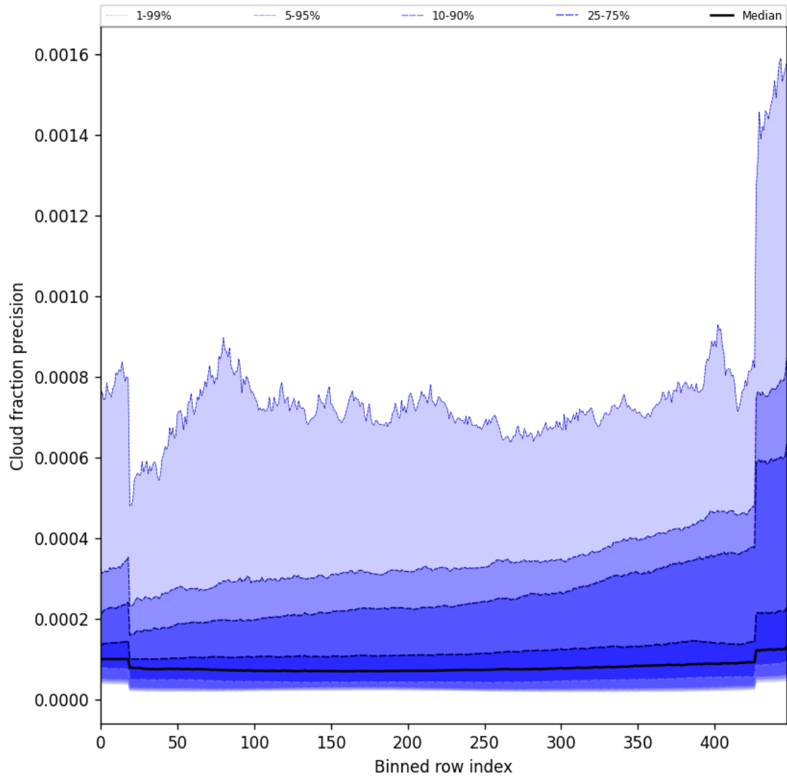
Figure 48: Along track statistics of “Cloud fraction precision” for 2025-07-22 to 2025-07-22
