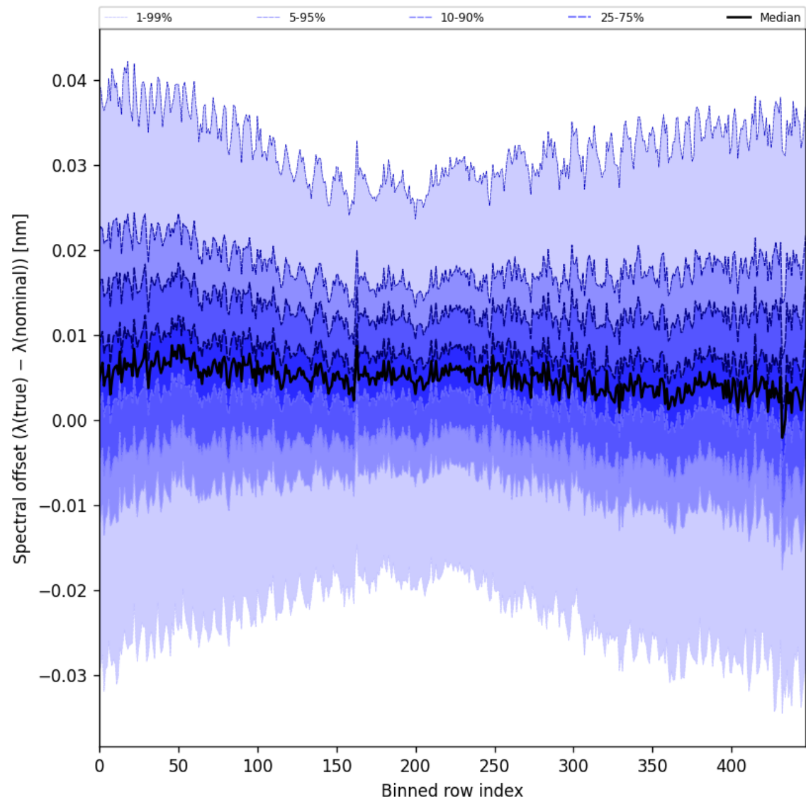
Figure 60: Along track statistics of “Spectral offset ( \lambda_{\text{true}} - \lambda_{\text{nominal}} )” for 2025-07-22 to 2025-07-22
