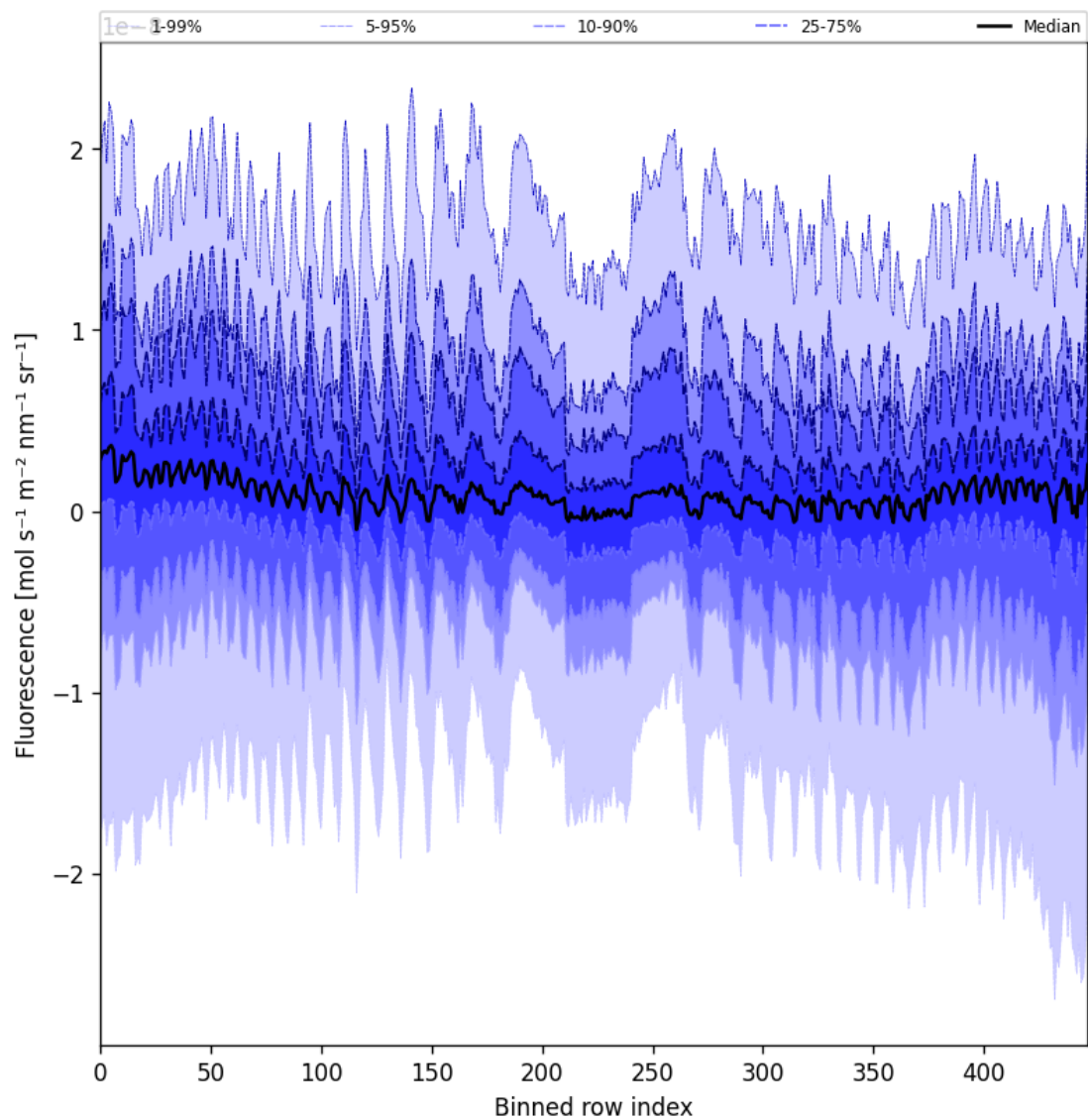
Figure 55: Along track statistics of “Fluorescence” for 2025-07-22 to 2025-07-22
