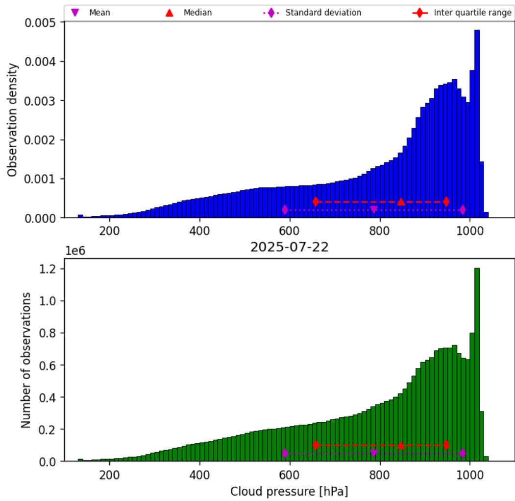
Figure 28: Histogram of “Cloud pressure” for 2025-07-22 to 2025-07-22
