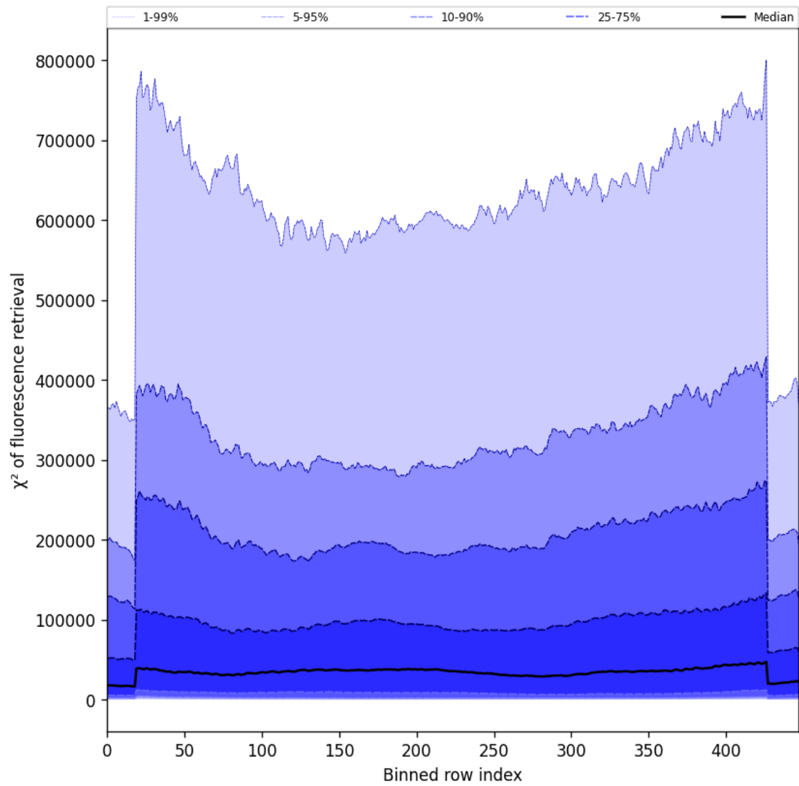
Figure 57: Along track statistics of “ \chi^2 of fluorescence retrieval” for 2025-07-22 to 2025-07-22
