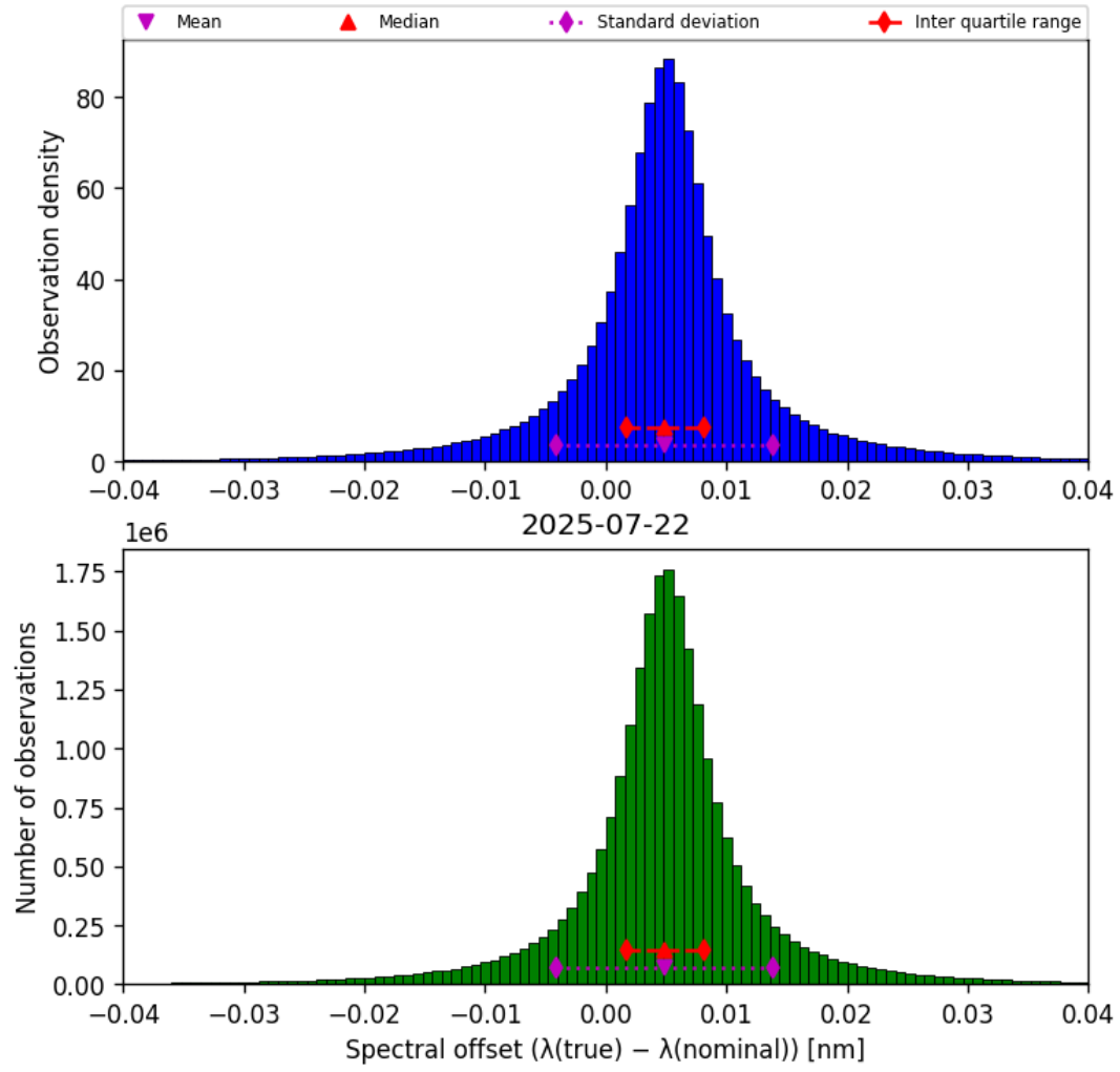
Figure 43: Histogram of “Spectral offset ( \lambda_{\text{true}} - \lambda_{\text{nominal}} )” for 2025-07-22 to 2025-07-22
