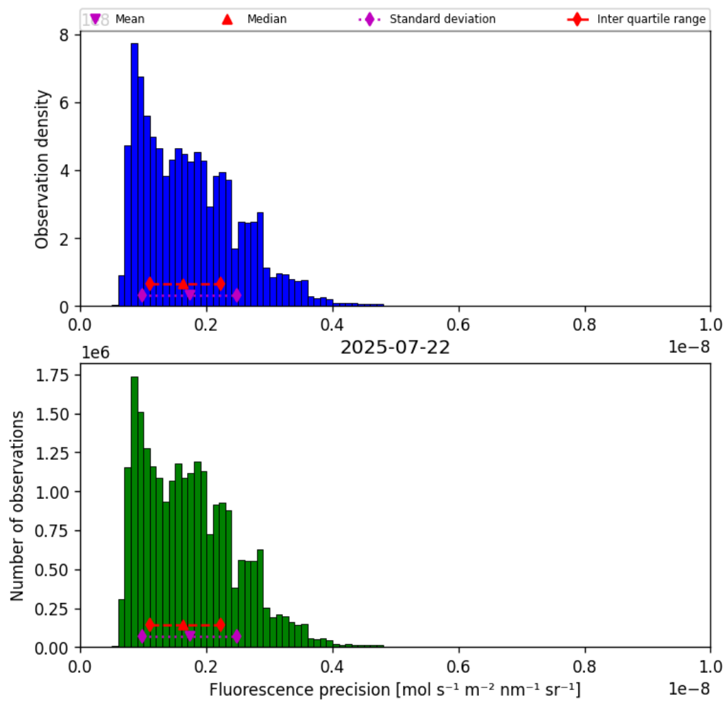
Figure 39: Histogram of “Fluorescence precision” for 2025-07-22 to 2025-07-22
