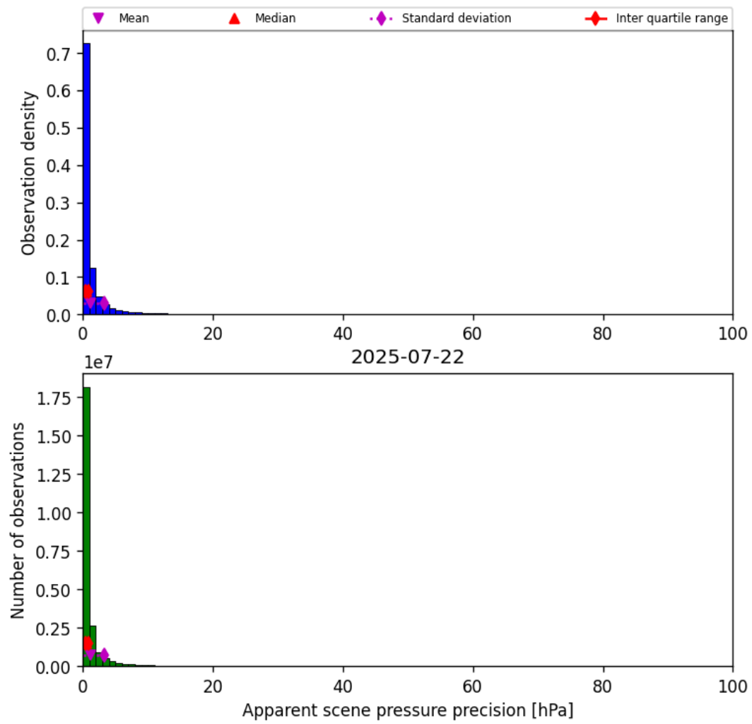
Figure 35: Histogram of “Apparent scene pressure precision” for 2025-07-22 to 2025-07-22
