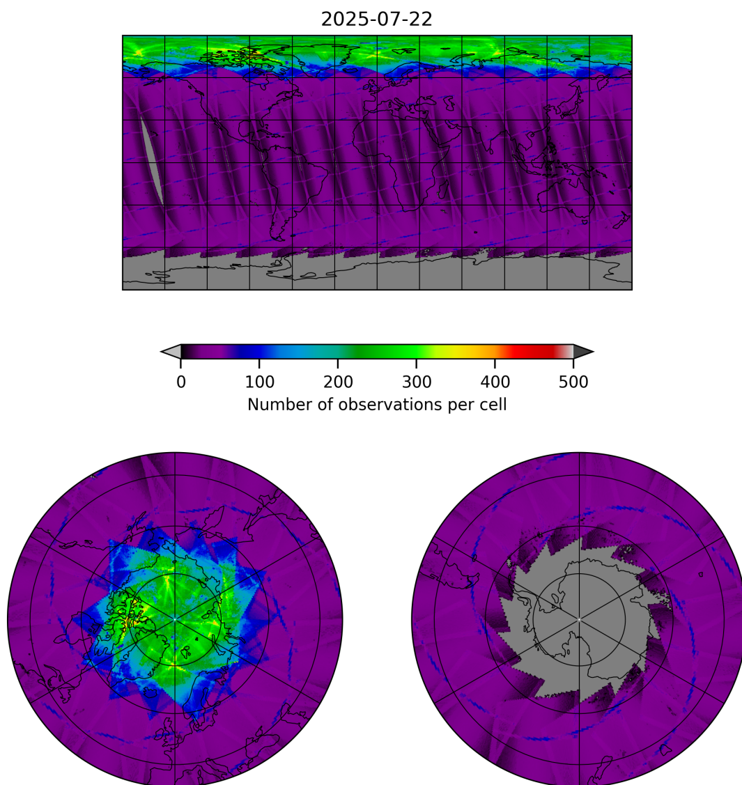
Figure 9: Map of the number of observations for 2025-07-22 to 2025-07-22
