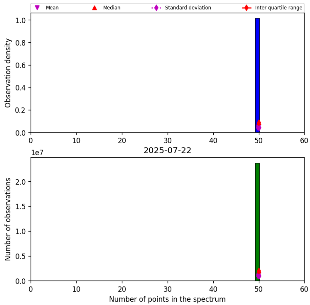
Figure 42: Histogram of "Number of points in the spectrum" for 2025-07-22 to 2025-07-22
