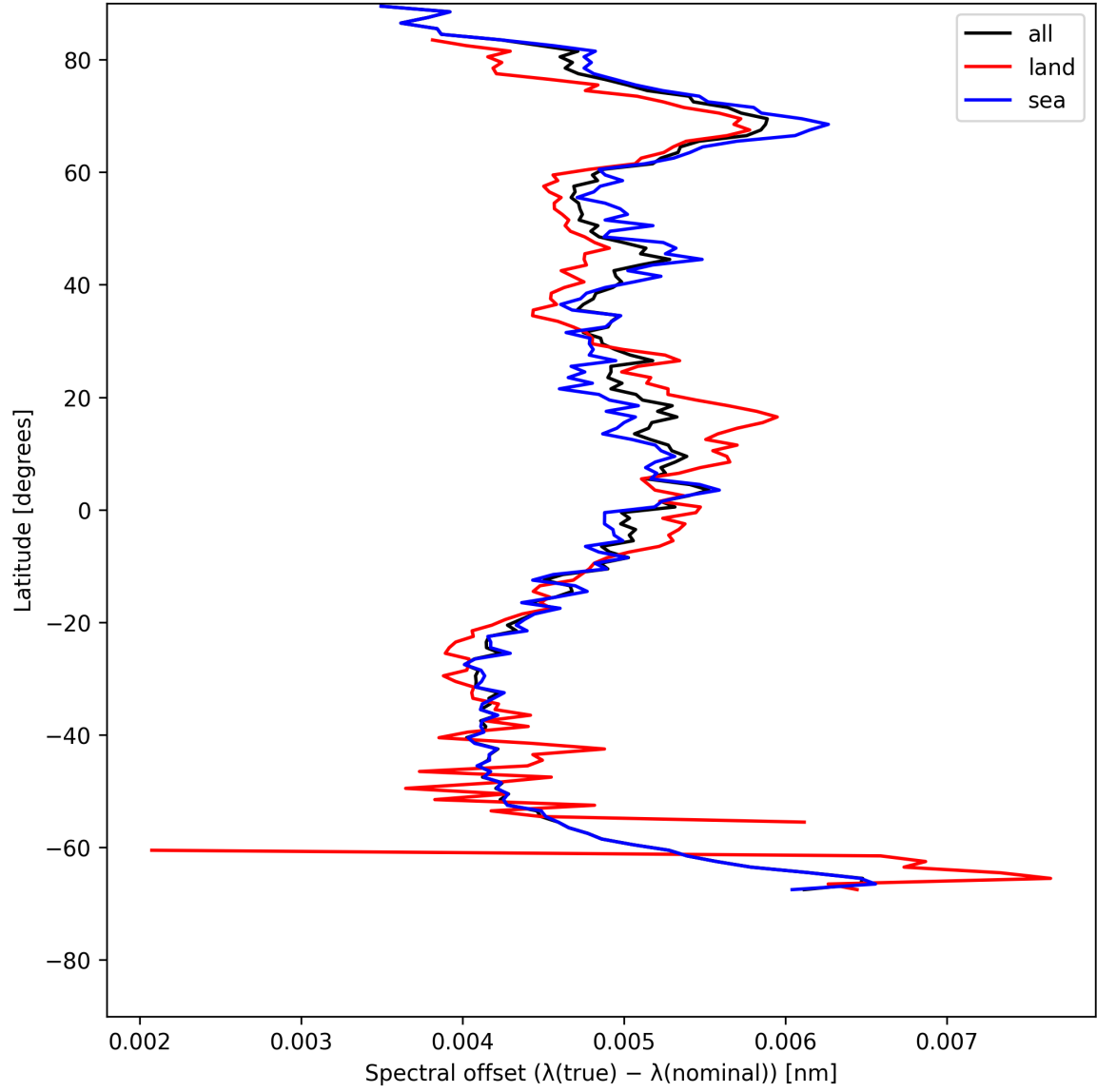
Figure 26: Zonal average of “Spectral offset ( \lambda_{\text{true}} - \lambda_{\text{nominal}} )” for 2025-07-22 to 2025-07-22.
