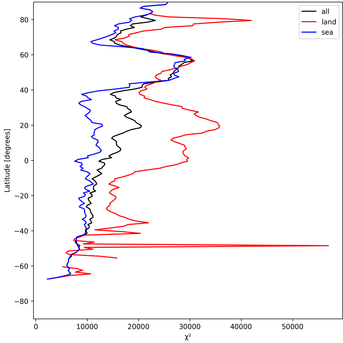
Figure 19: Zonal average of “ \chi^2 ” for 2025-07-22 to 2025-07-22.
