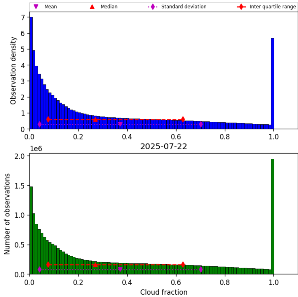
Figure 30: Histogram of “Cloud fraction” for 2025-07-22 to 2025-07-22
