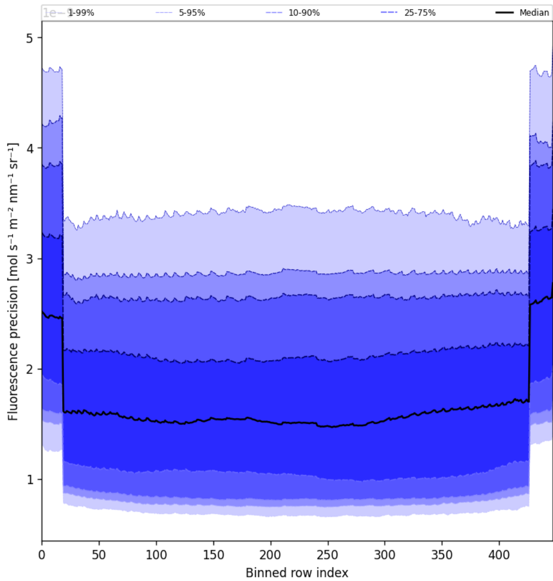
Figure 56: Along track statistics of “Fluorescence precision” for 2025-07-22 to 2025-07-22
