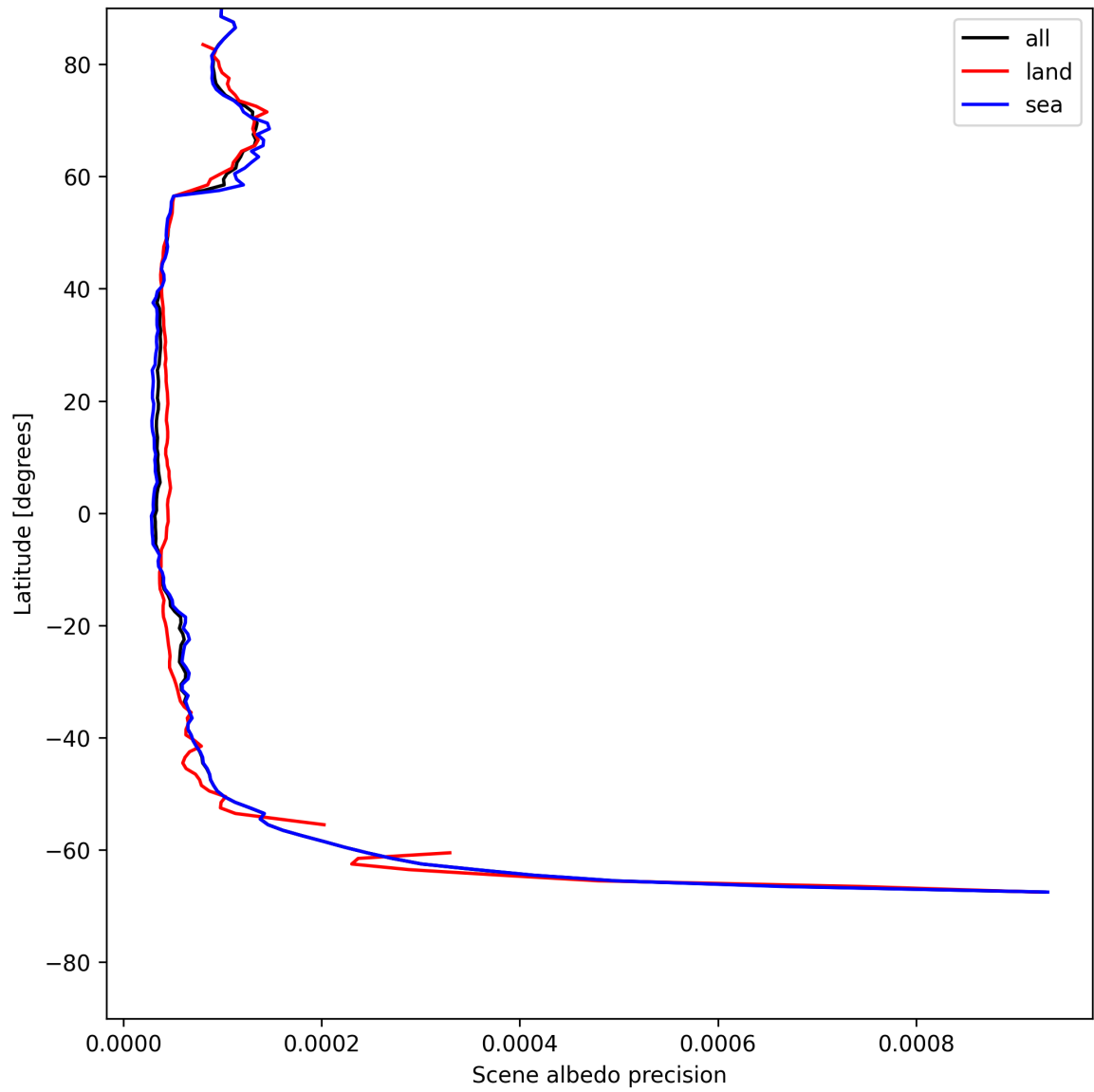
Figure 16: Zonal average of “Scene albedo precision” for 2025-07-22 to 2025-07-22.
