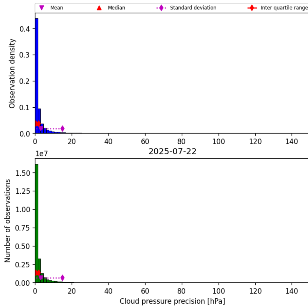
Figure 29: Histogram of “Cloud pressure precision” for 2025-07-22 to 2025-07-22
