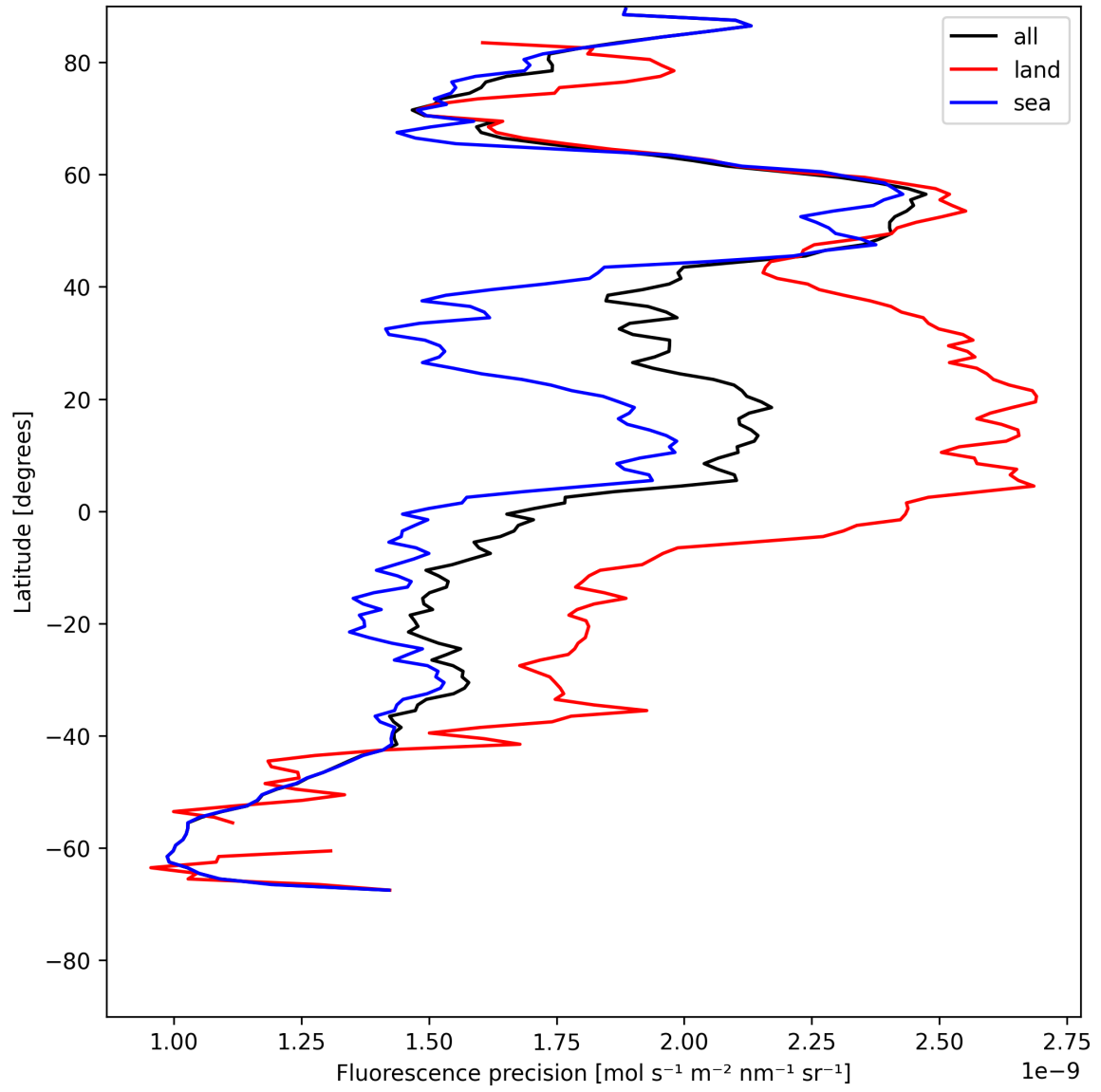
Figure 22: Zonal average of “Fluorescence precision” for 2025-07-22 to 2025-07-22.
