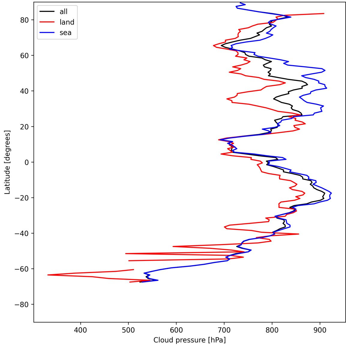
Figure 11: Zonal average of “Cloud pressure” for 2025-07-22 to 2025-07-22.
