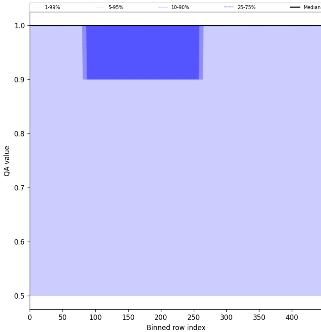
Figure 44: Along track statistics of “QA value” for 2025-07-22 to 2025-07-22
