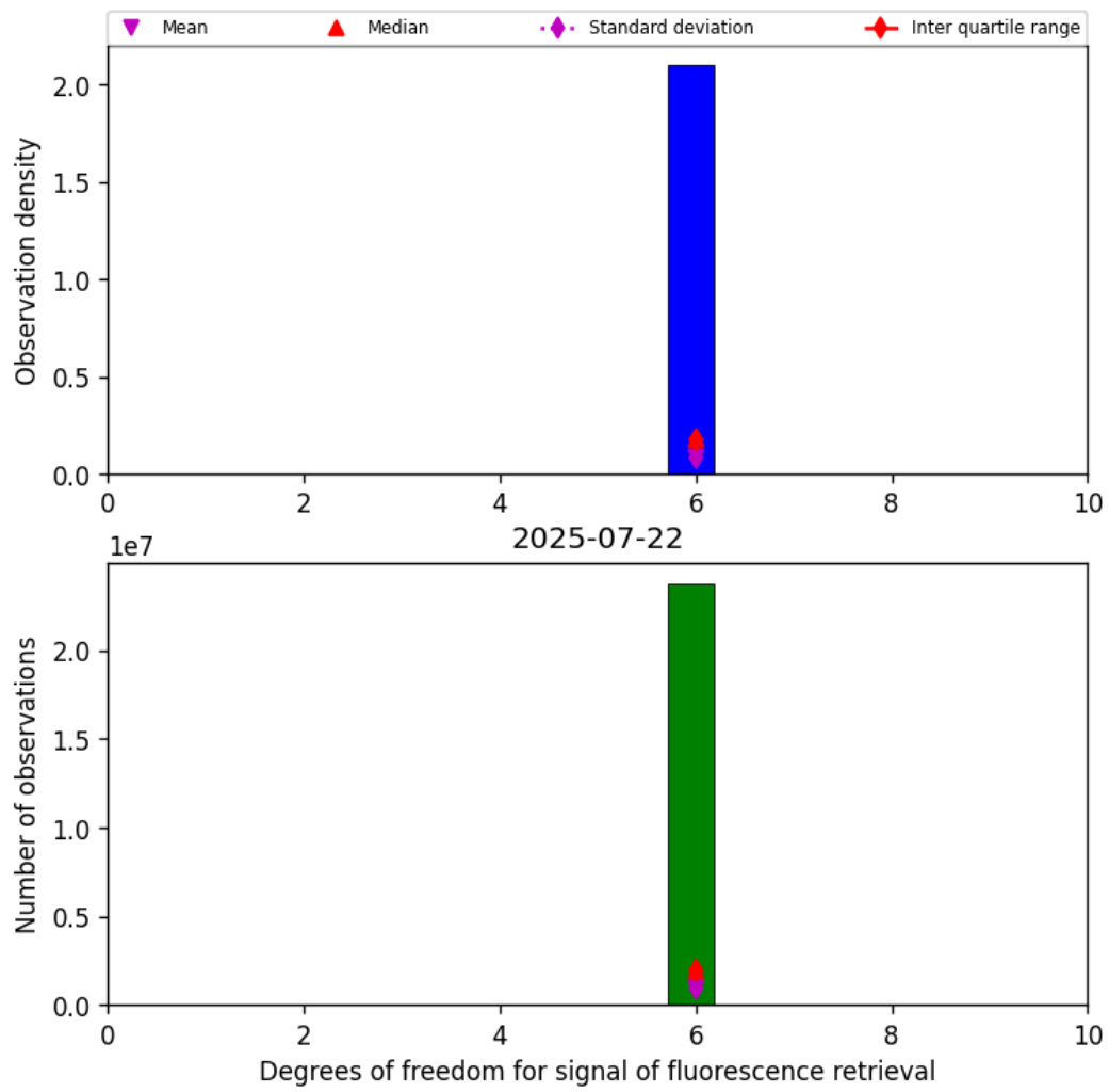
Figure 41: Histogram of “Degrees of freedom for signal of fluorescence retrieval” for 2025-07-22 to 2025-07-22
