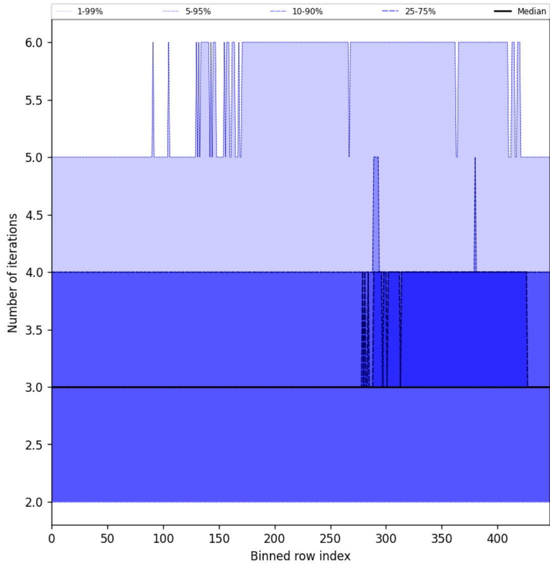
Figure 54: Along track statistics of “Number of iterations” for 2025-07-22 to 2025-07-22
