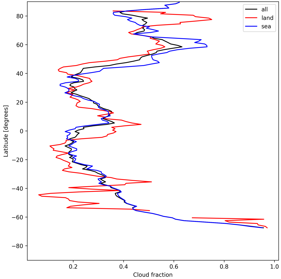
Figure 13: Zonal average of “Cloud fraction” for 2025-07-22 to 2025-07-22.
