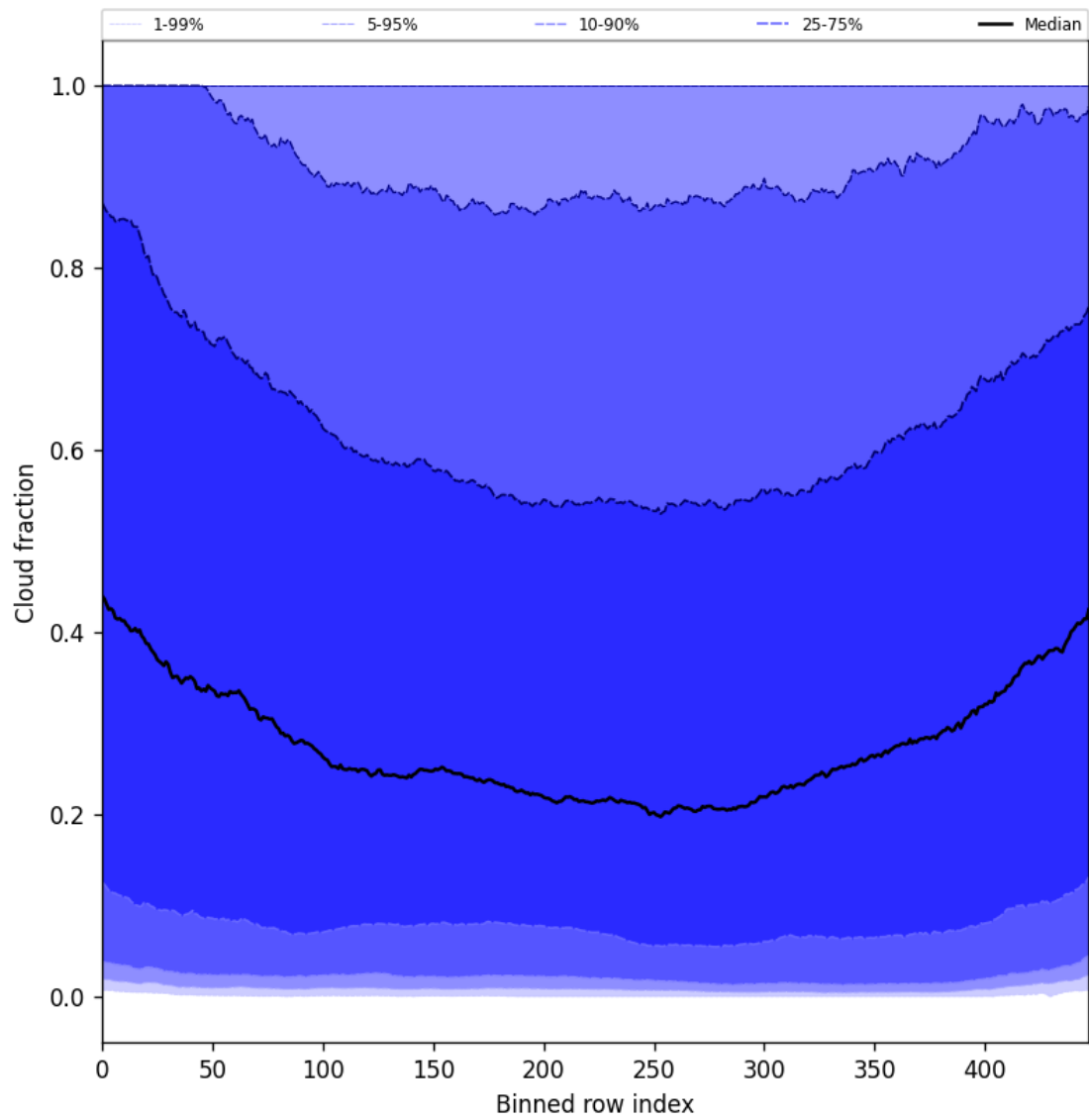
Figure 47: Along track statistics of “Cloud fraction” for 2025-07-22 to 2025-07-22
