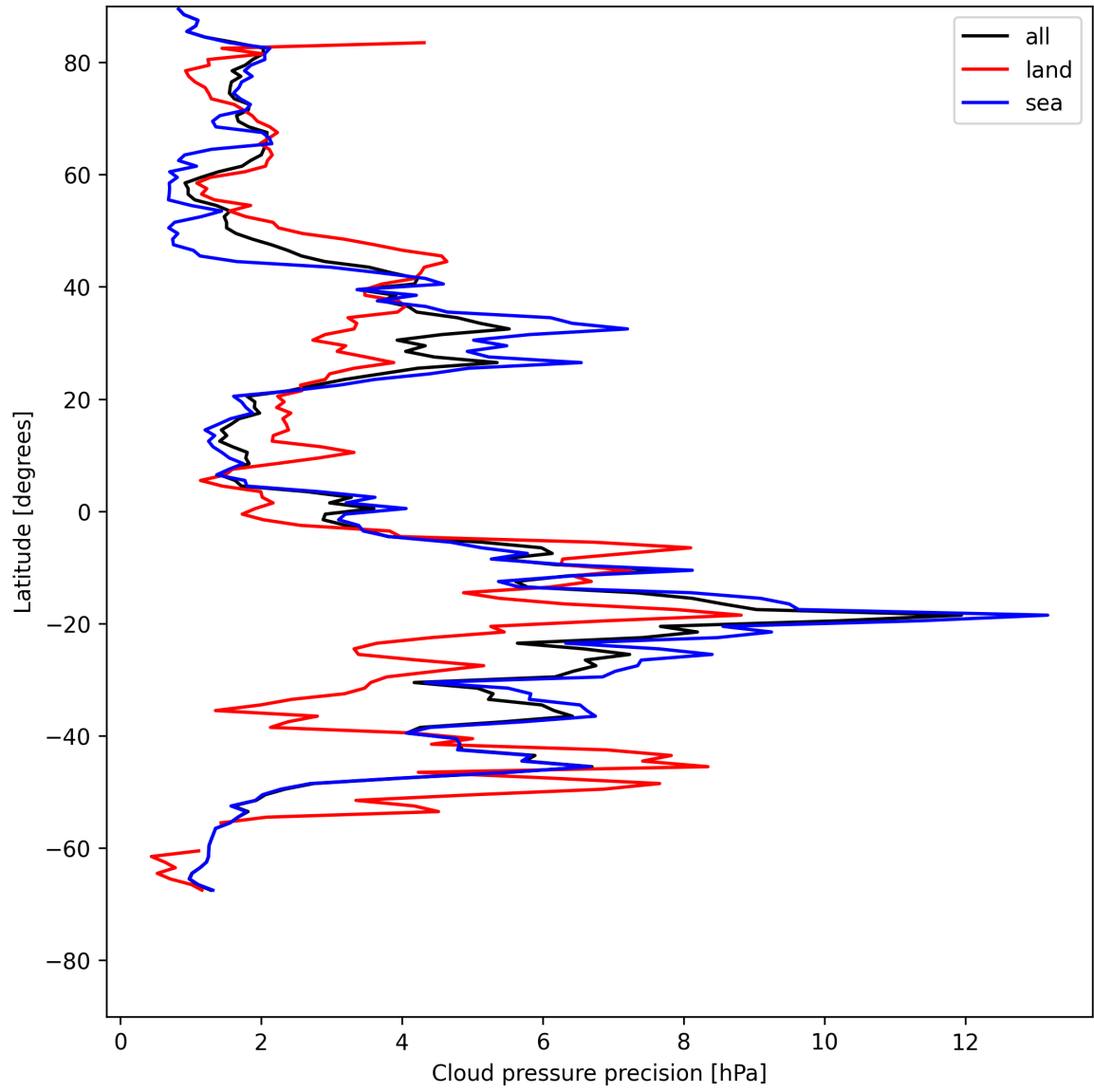
Figure 12: Zonal average of “Cloud pressure precision” for 2025-07-22 to 2025-07-22.
