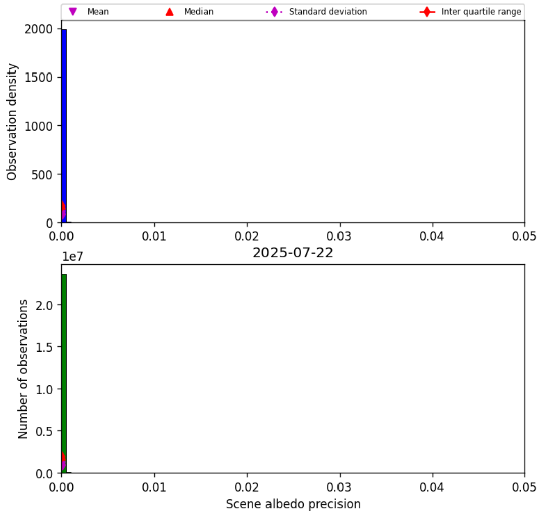
Figure 33: Histogram of “Scene albedo precision” for 2025-07-22 to 2025-07-22
