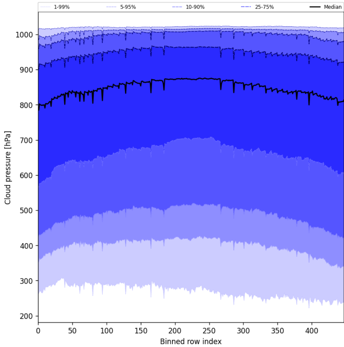
Figure 45: Along track statistics of “Cloud pressure” for 2025-07-22 to 2025-07-22
