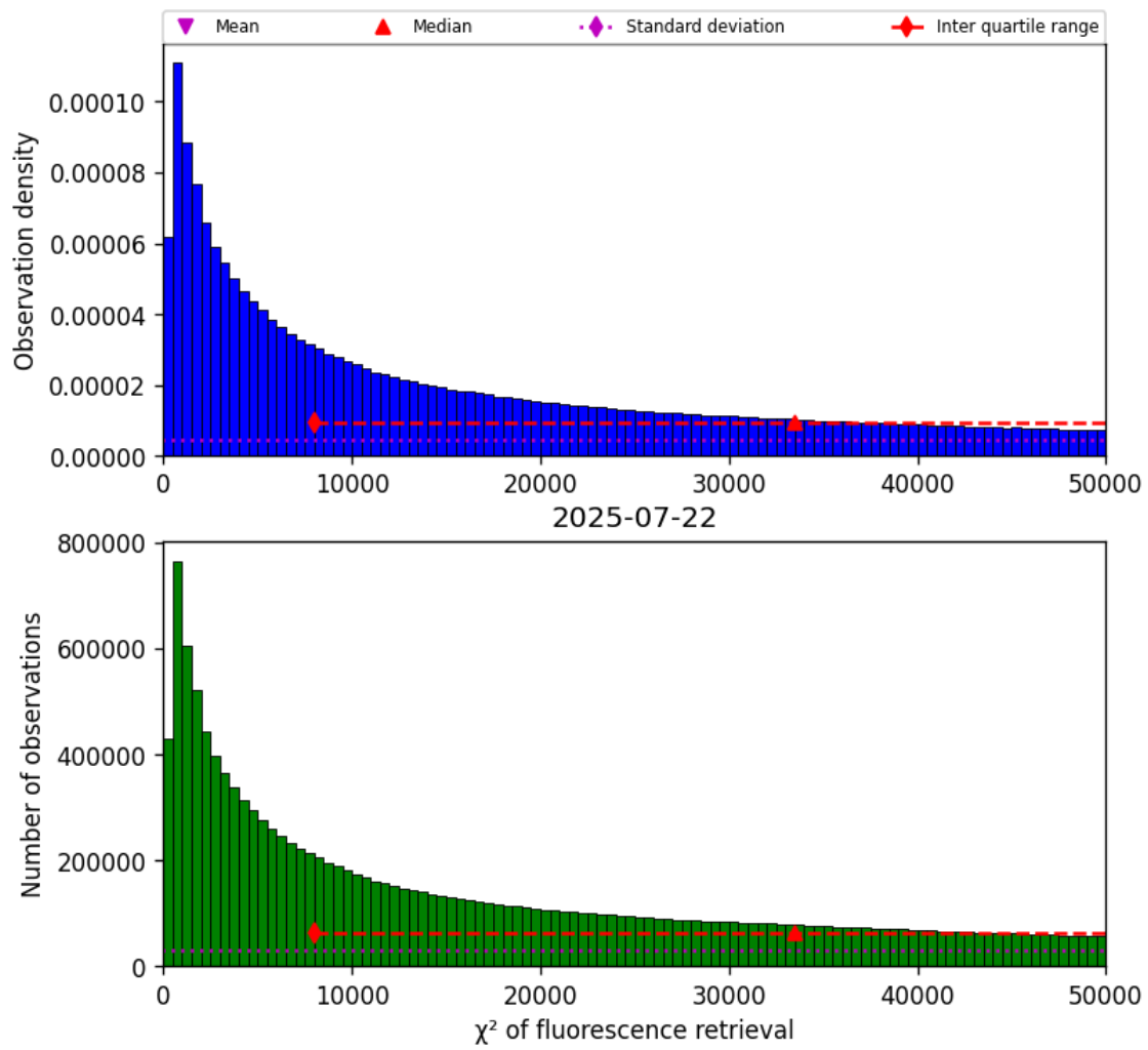
Figure 40: Histogram of “ \chi^2 of fluorescence retrieval” for 2025-07-22 to 2025-07-22
