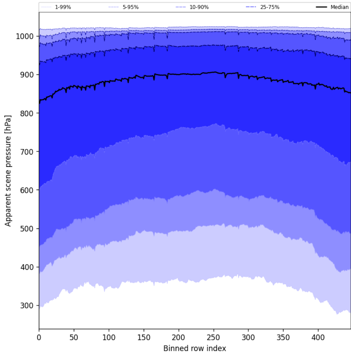
Figure 51: Along track statistics of “Apparent scene pressure” for 2025-07-22 to 2025-07-22
