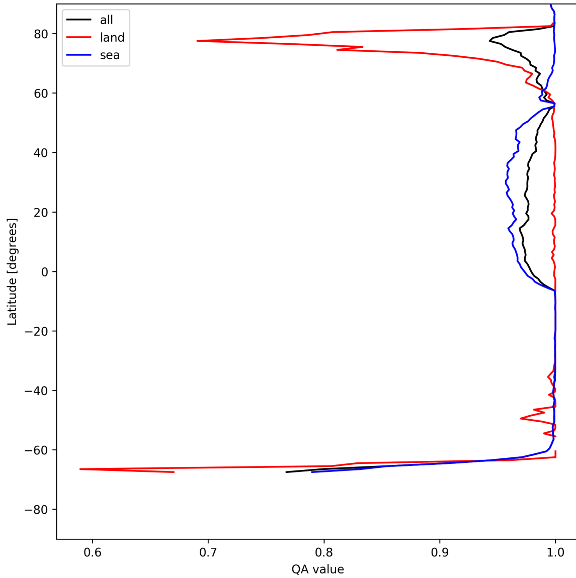
Figure 10: Zonal average of “QA value” for 2025-07-22 to 2025-07-22.
