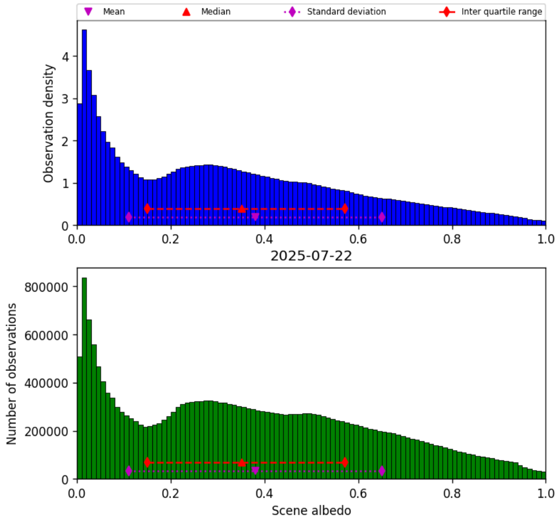
Figure 32: Histogram of “Scene albedo” for 2025-07-22 to 2025-07-22
