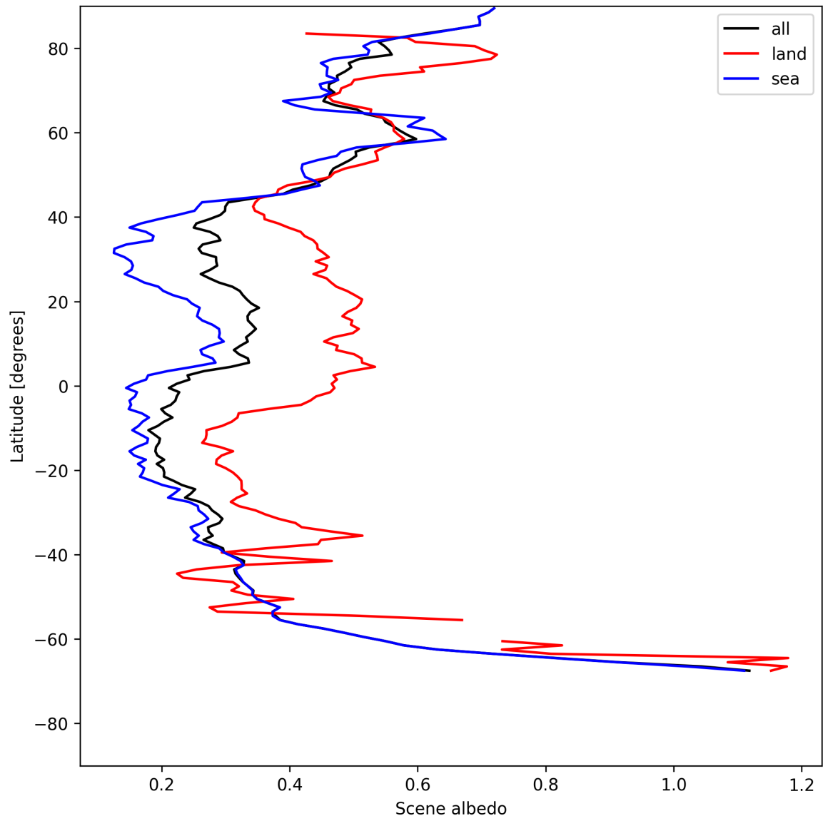
Figure 15: Zonal average of “Scene albedo” for 2025-07-22 to 2025-07-22.
