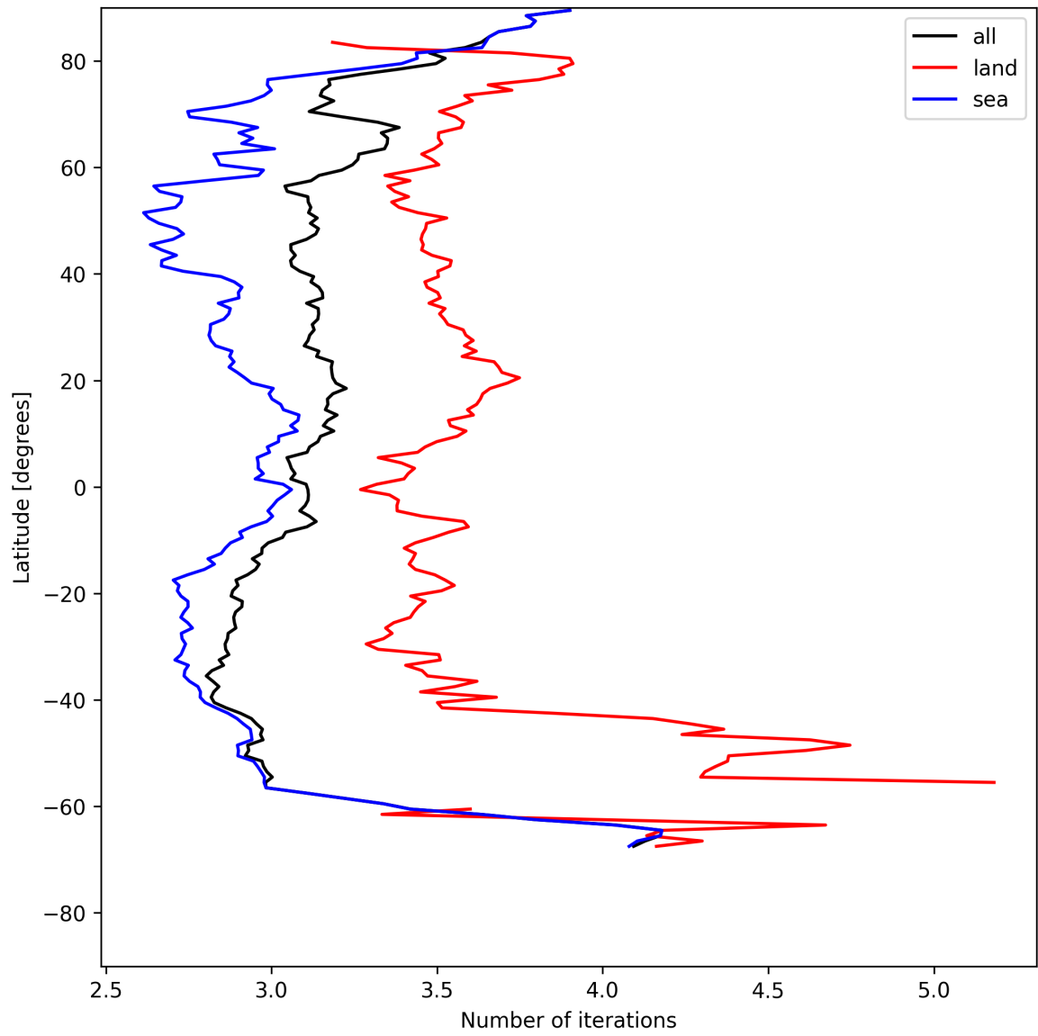
Figure 20: Zonal average of “Number of iterations” for 2025-07-22 to 2025-07-22.
