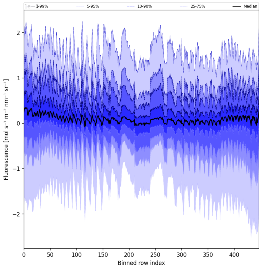
Figure 55: Along track statistics of “Fluorescence” for 2025-07-23 to 2025-07-24
