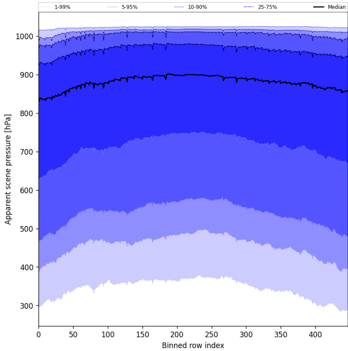
Figure 51: Along track statistics of “Apparent scene pressure” for 2025-07-23 to 2025-07-24
