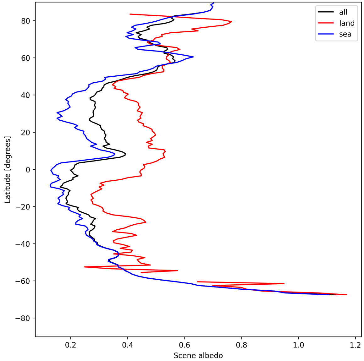
Figure 15: Zonal average of “Scene albedo” for 2025-07-23 to 2025-07-24.
