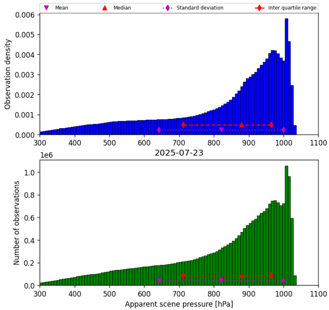
Figure 34: Histogram of “Apparent scene pressure” for 2025-07-23 to 2025-07-24
