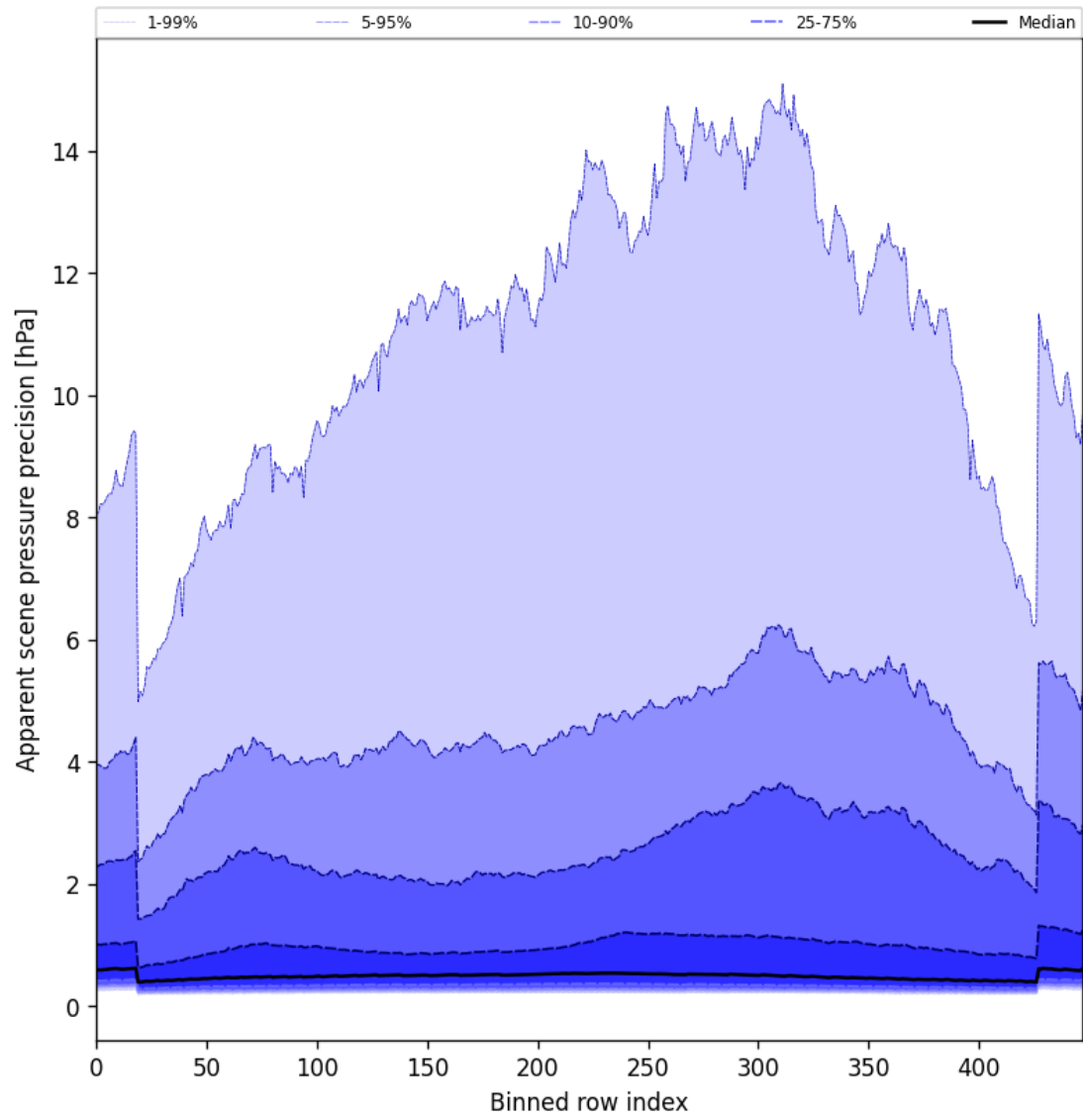
Figure 52: Along track statistics of “Apparent scene pressure precision” for 2025-07-23 to 2025-07-24
