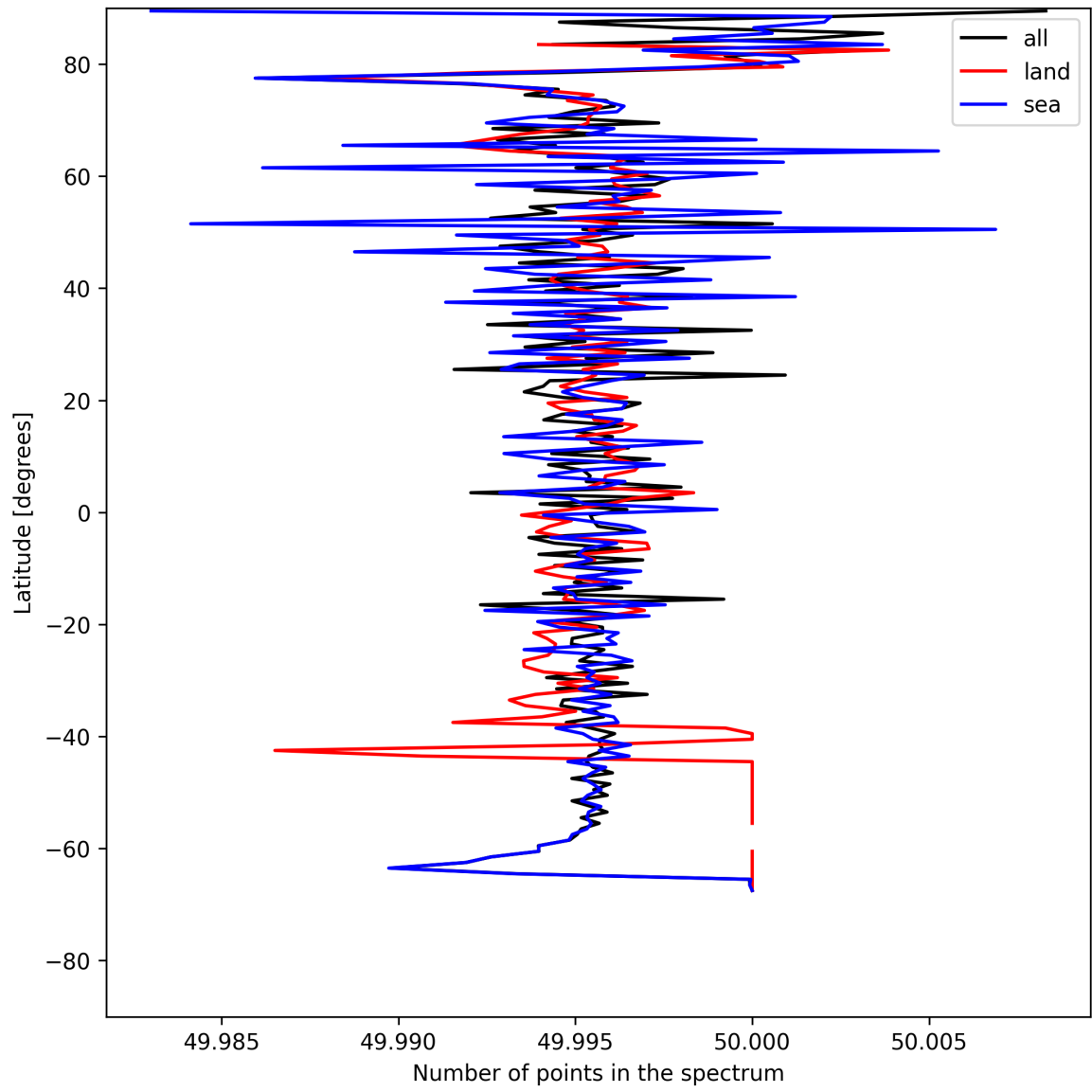
Figure 25: Zonal average of “Number of points in the spectrum” for 2025-07-23 to 2025-07-24.
