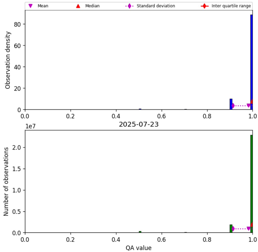
Figure 27: Histogram of “QA value” for 2025-07-23 to 2025-07-24
