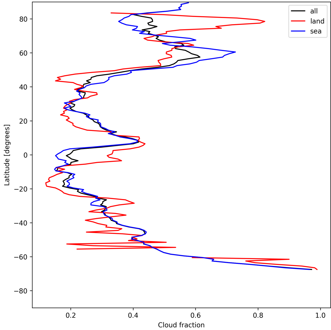
Figure 13: Zonal average of “Cloud fraction” for 2025-07-23 to 2025-07-24.
