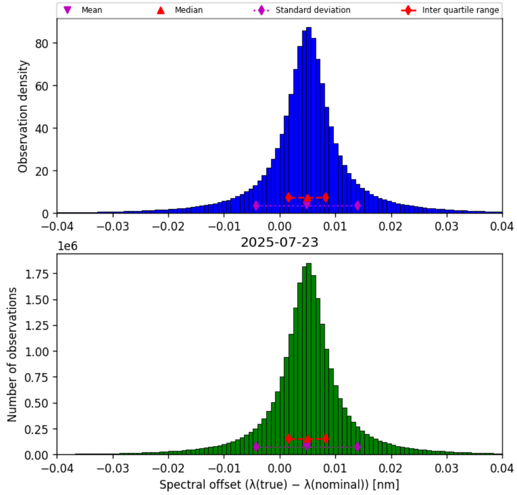
Figure 43: Histogram of “Spectral offset ( \lambda_{\text{true}} - \lambda_{\text{nominal}} )” for 2025-07-23 to 2025-07-24
