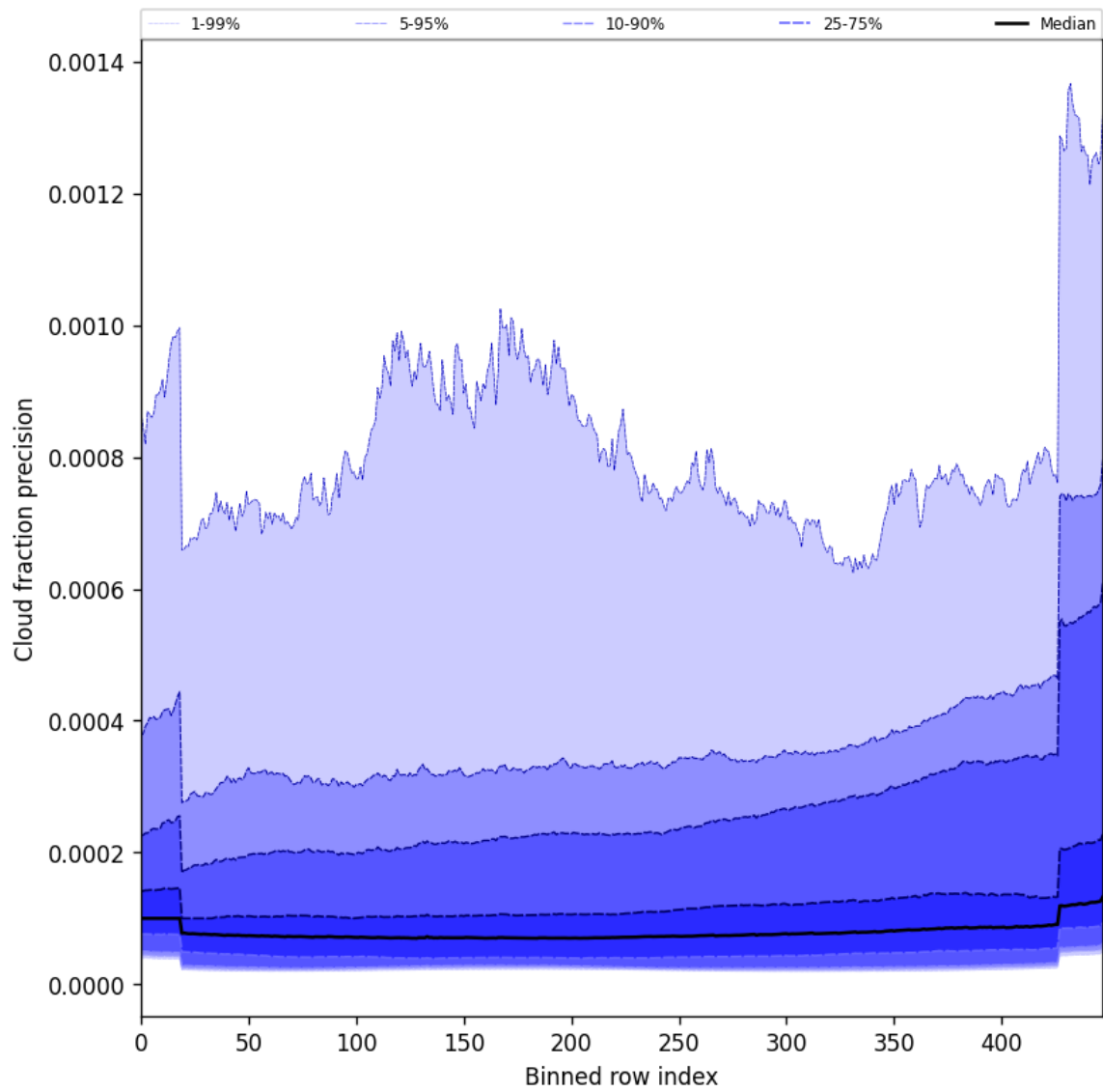
Figure 48: Along track statistics of “Cloud fraction precision” for 2025-07-23 to 2025-07-24
