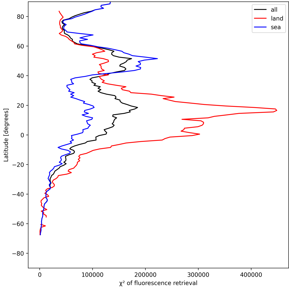
Figure 23: Zonal average of “ \chi^2 of fluorescence retrieval” for 2025-07-23 to 2025-07-24.
