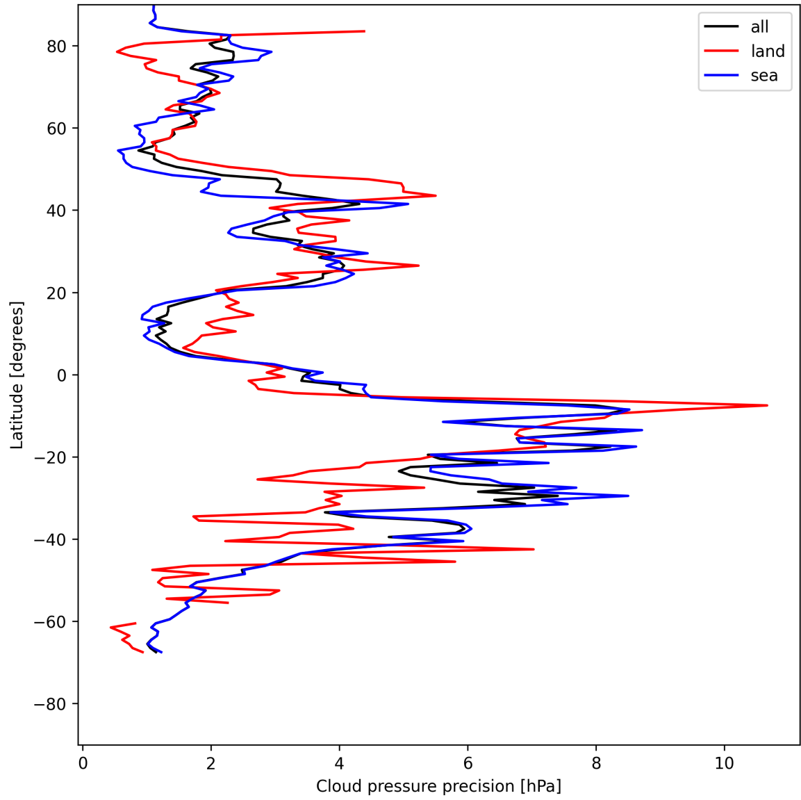
Figure 12: Zonal average of "Cloud pressure precision" for 2025-07-23 to 2025-07-24.
