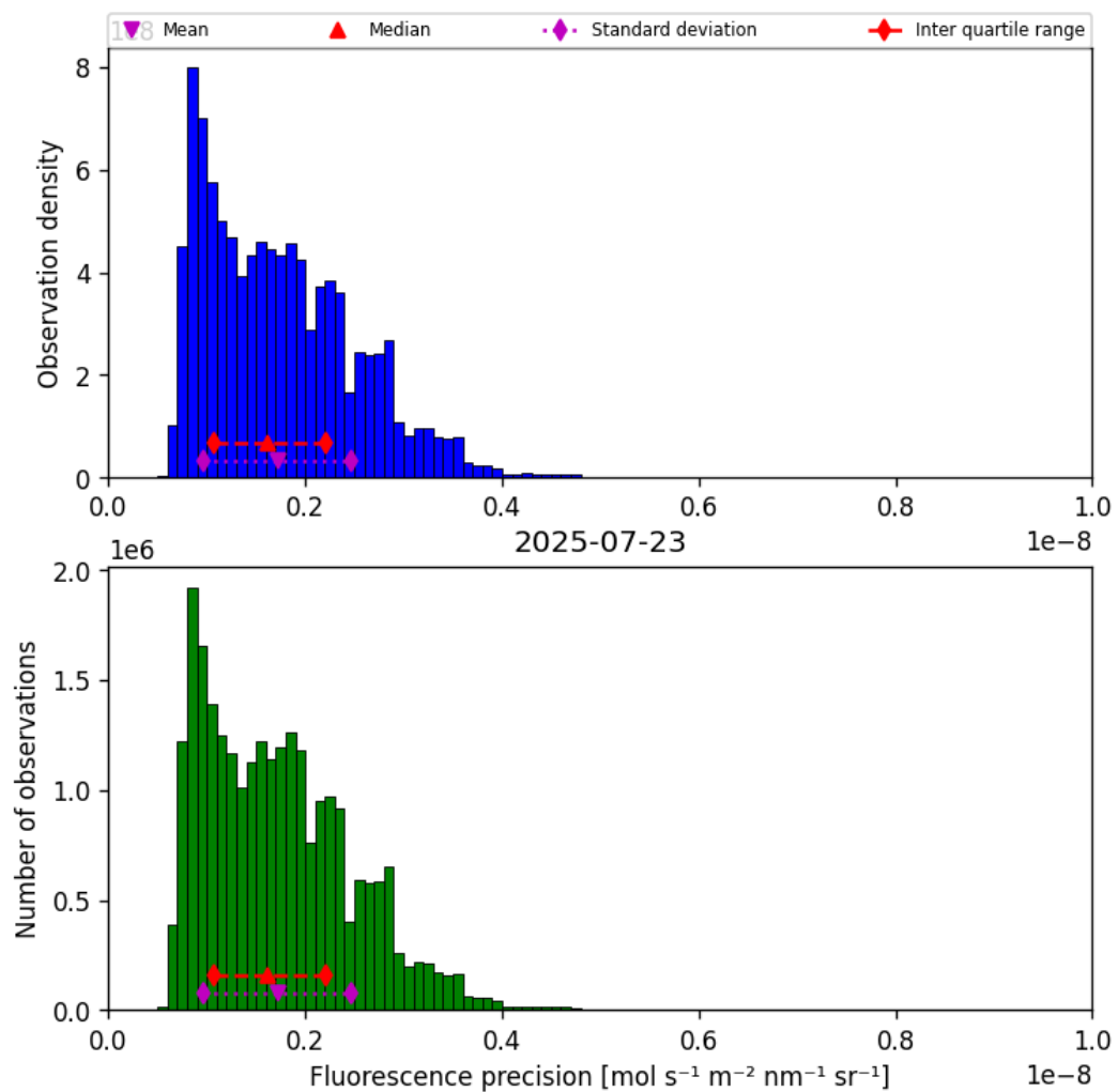
Figure 39: Histogram of “Fluorescence precision” for 2025-07-23 to 2025-07-24
