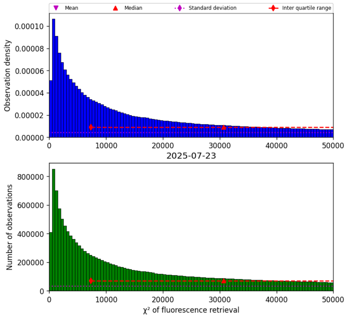
Figure 40: Histogram of “ \chi^2 of fluorescence retrieval” for 2025-07-23 to 2025-07-24
