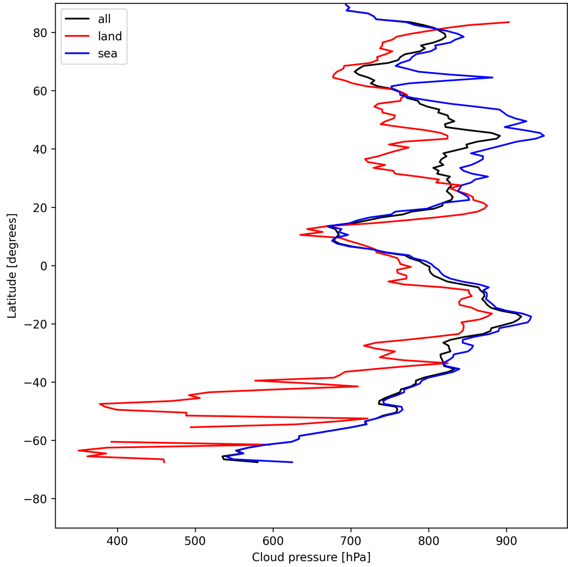
Figure 11: Zonal average of “Cloud pressure” for 2025-07-23 to 2025-07-24.
