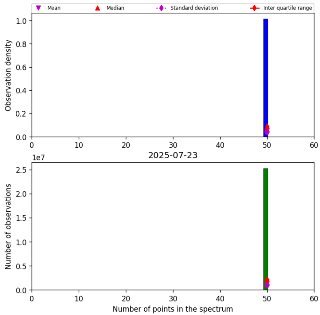
Figure 42: Histogram of “Number of points in the spectrum” for 2025-07-23 to 2025-07-24
