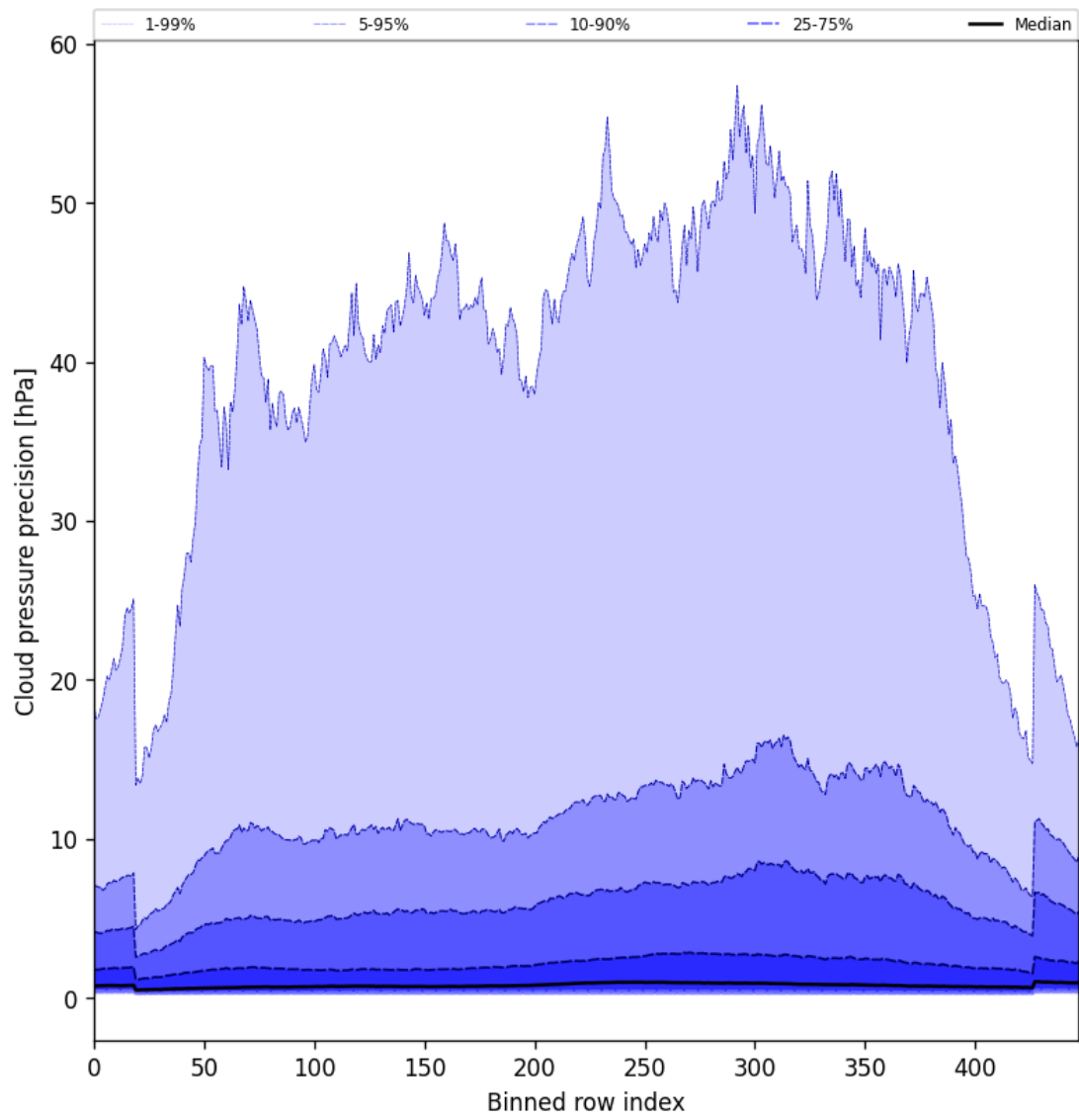
Figure 46: Along track statistics of “Cloud pressure precision” for 2025-07-23 to 2025-07-24
