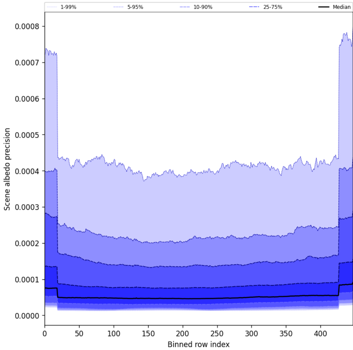
Figure 50: Along track statistics of “Scene albedo precision” for 2025-07-23 to 2025-07-24
