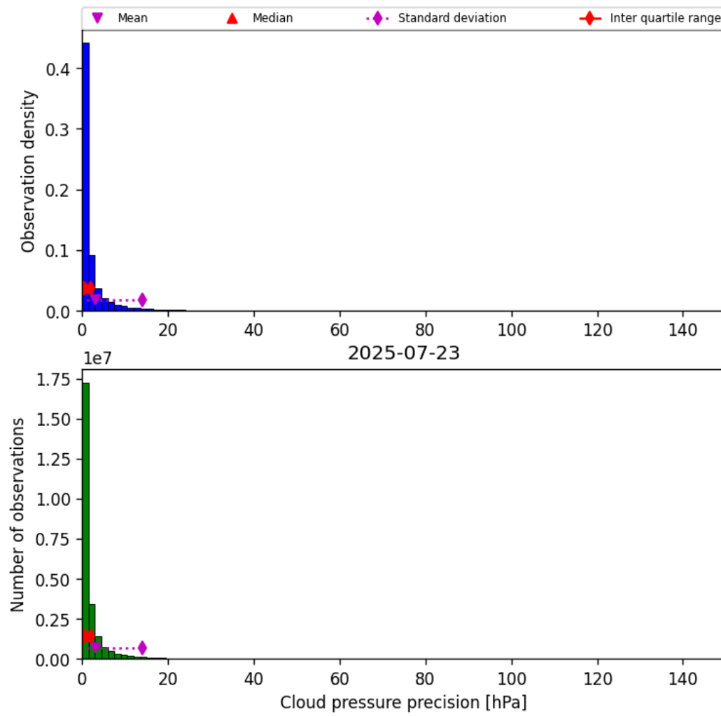
Figure 29: Histogram of “Cloud pressure precision” for 2025-07-23 to 2025-07-24
