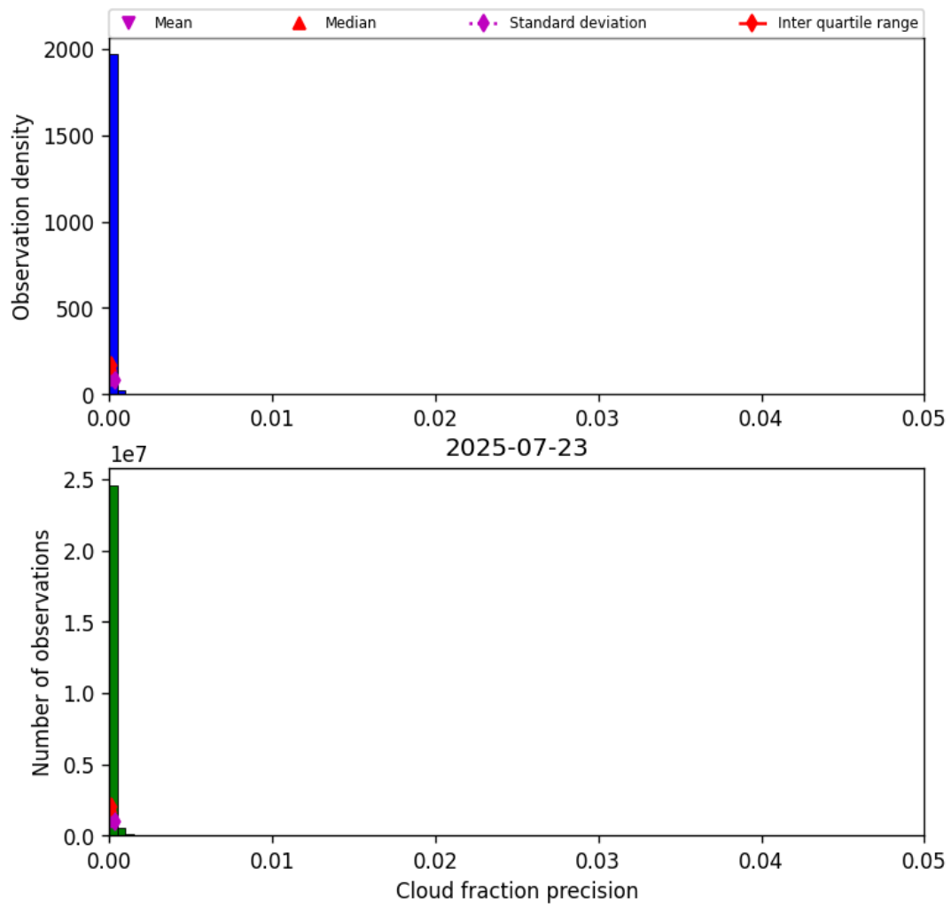
Figure 31: Histogram of “Cloud fraction precision” for 2025-07-23 to 2025-07-24
