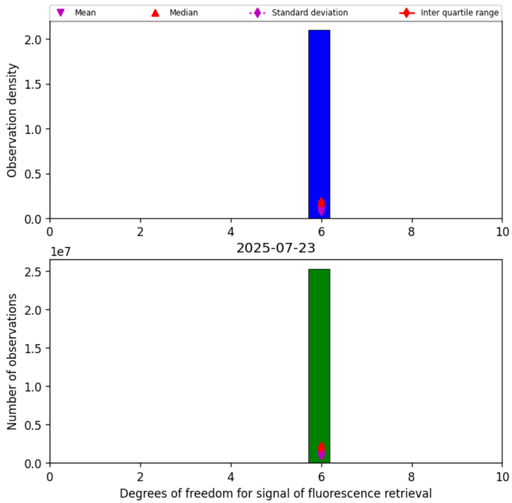
Figure 41: Histogram of “Degrees of freedom for signal of fluorescence retrieval” for 2025-07-23 to 2025-07-24
