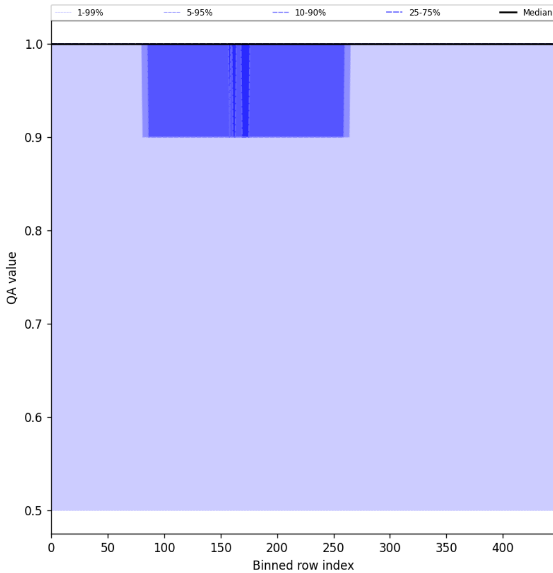
Figure 44: Along track statistics of “QA value” for 2025-07-23 to 2025-07-24
