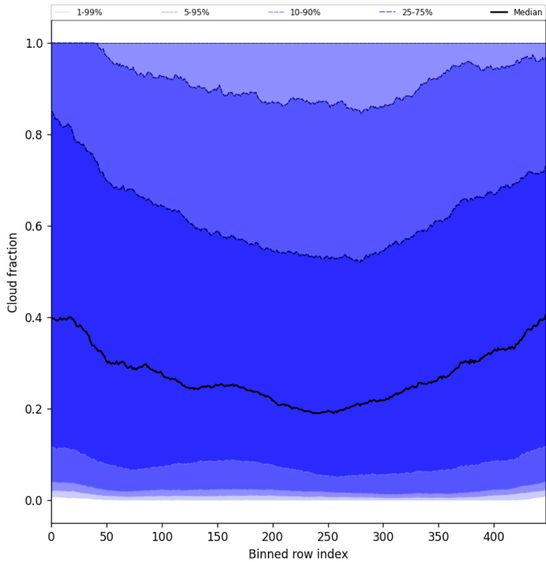
Figure 47: Along track statistics of “Cloud fraction” for 2025-07-23 to 2025-07-24
