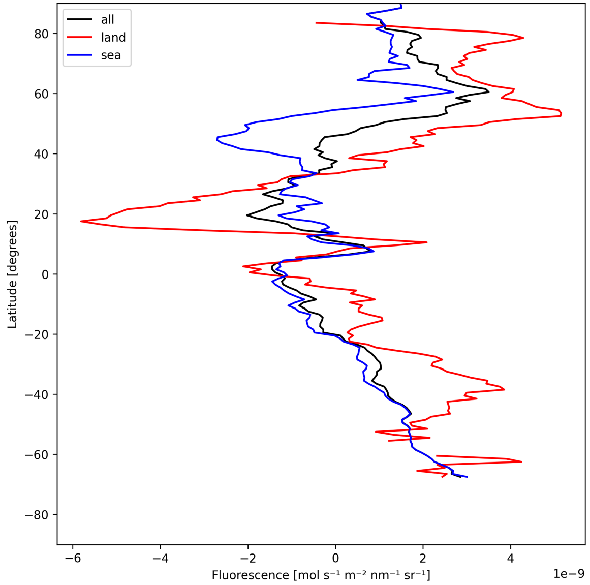
Figure 21: Zonal average of “Fluorescence” for 2025-07-23 to 2025-07-24.
