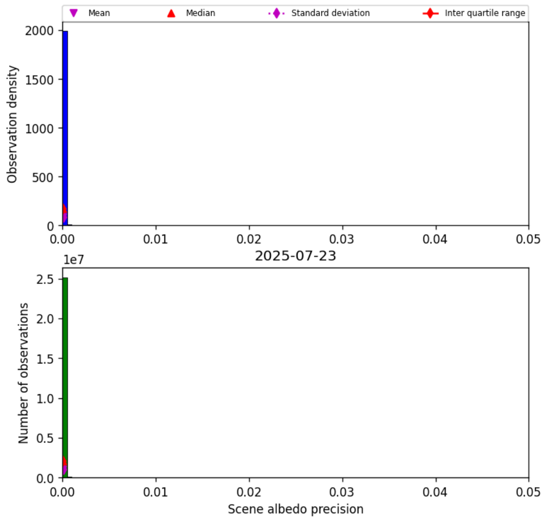
Figure 33: Histogram of “Scene albedo precision” for 2025-07-23 to 2025-07-24
