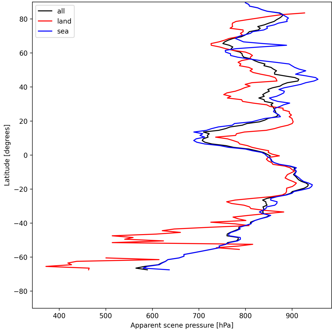
Figure 17: Zonal average of “Apparent scene pressure” for 2025-07-23 to 2025-07-24.
