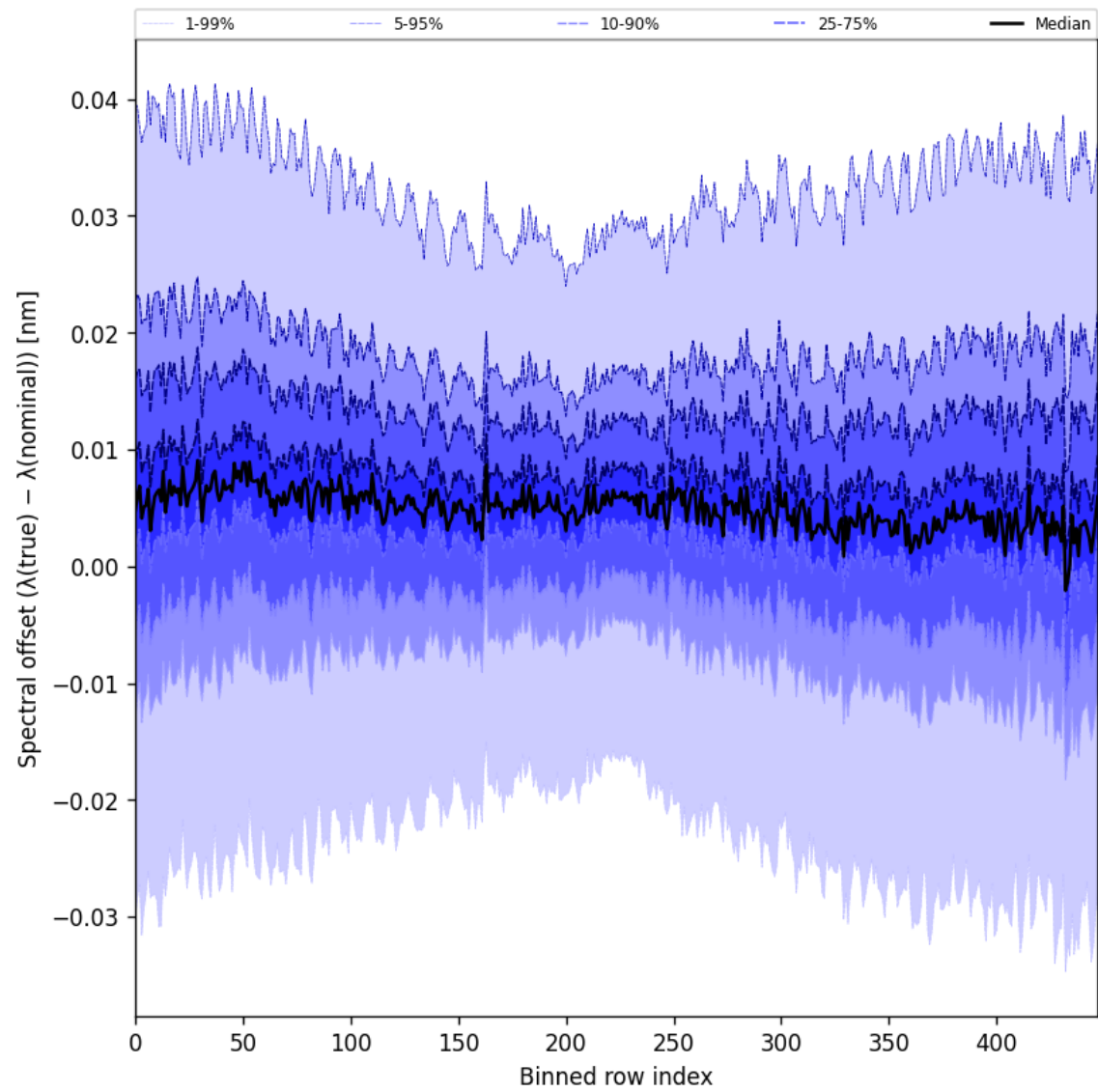
Figure 60: Along track statistics of “Spectral offset ( \lambda_{\text{true}} - \lambda_{\text{nominal}} )” for 2025-07-23 to 2025-07-24
