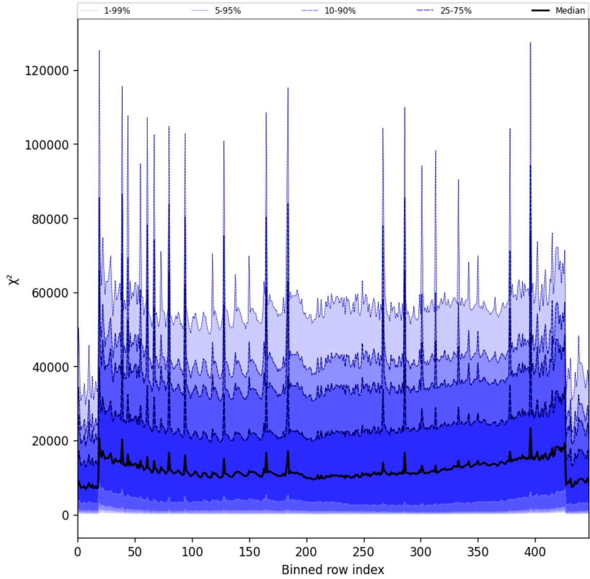
Figure 53: Along track statistics of “ \chi^2 ” for 2025-07-23 to 2025-07-24
