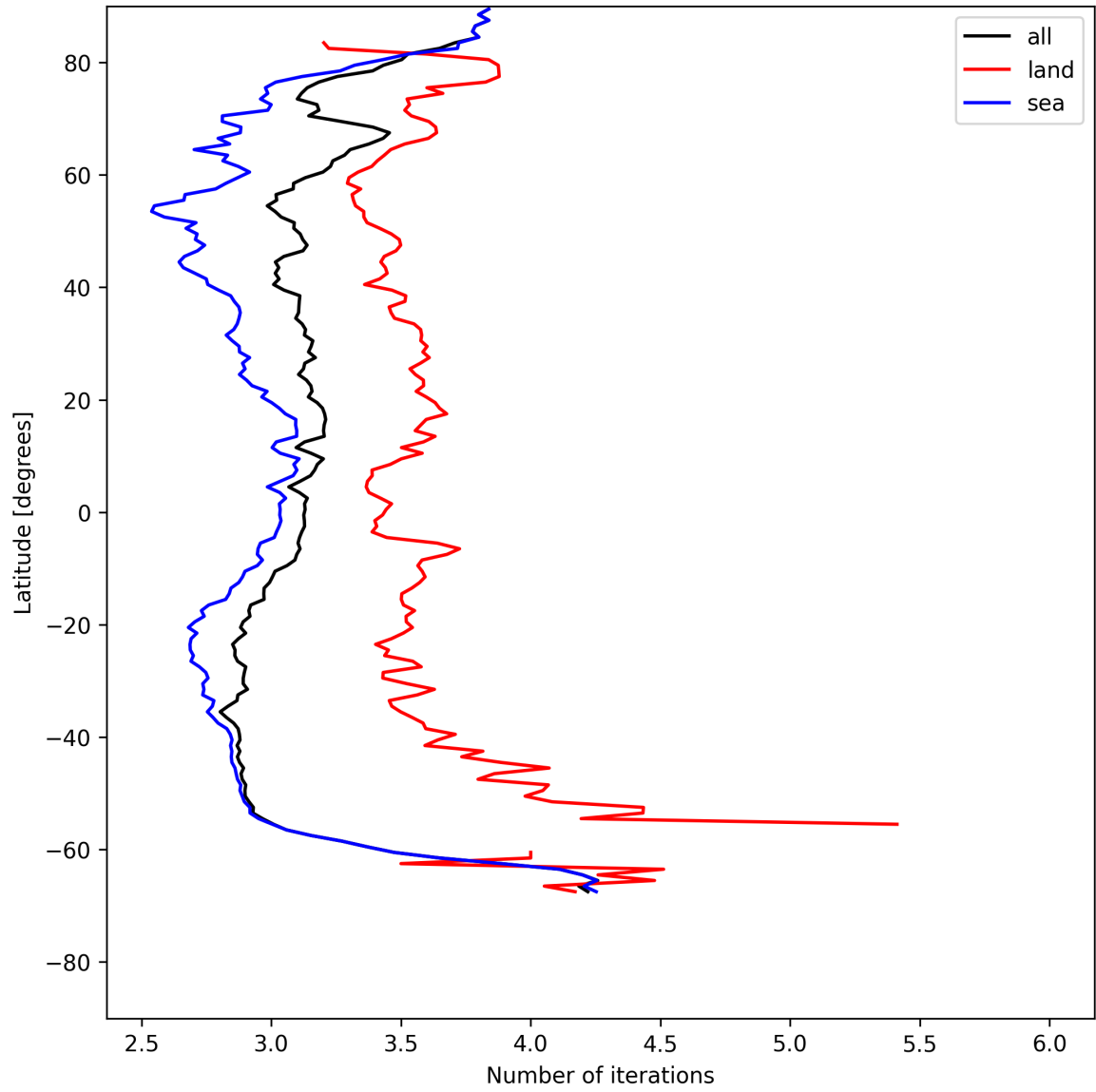
Figure 20: Zonal average of “Number of iterations” for 2025-07-23 to 2025-07-24.
