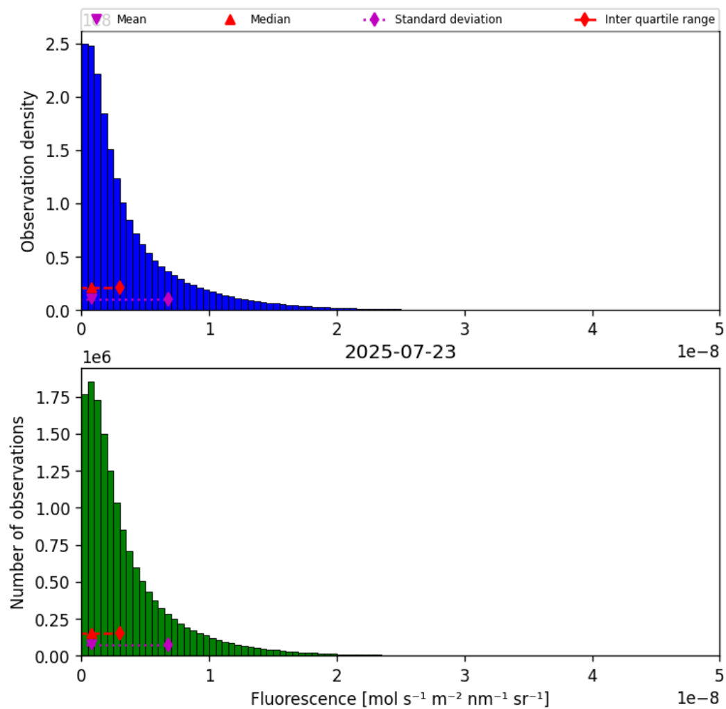
Figure 38: Histogram of “Fluorescence” for 2025-07-23 to 2025-07-24
