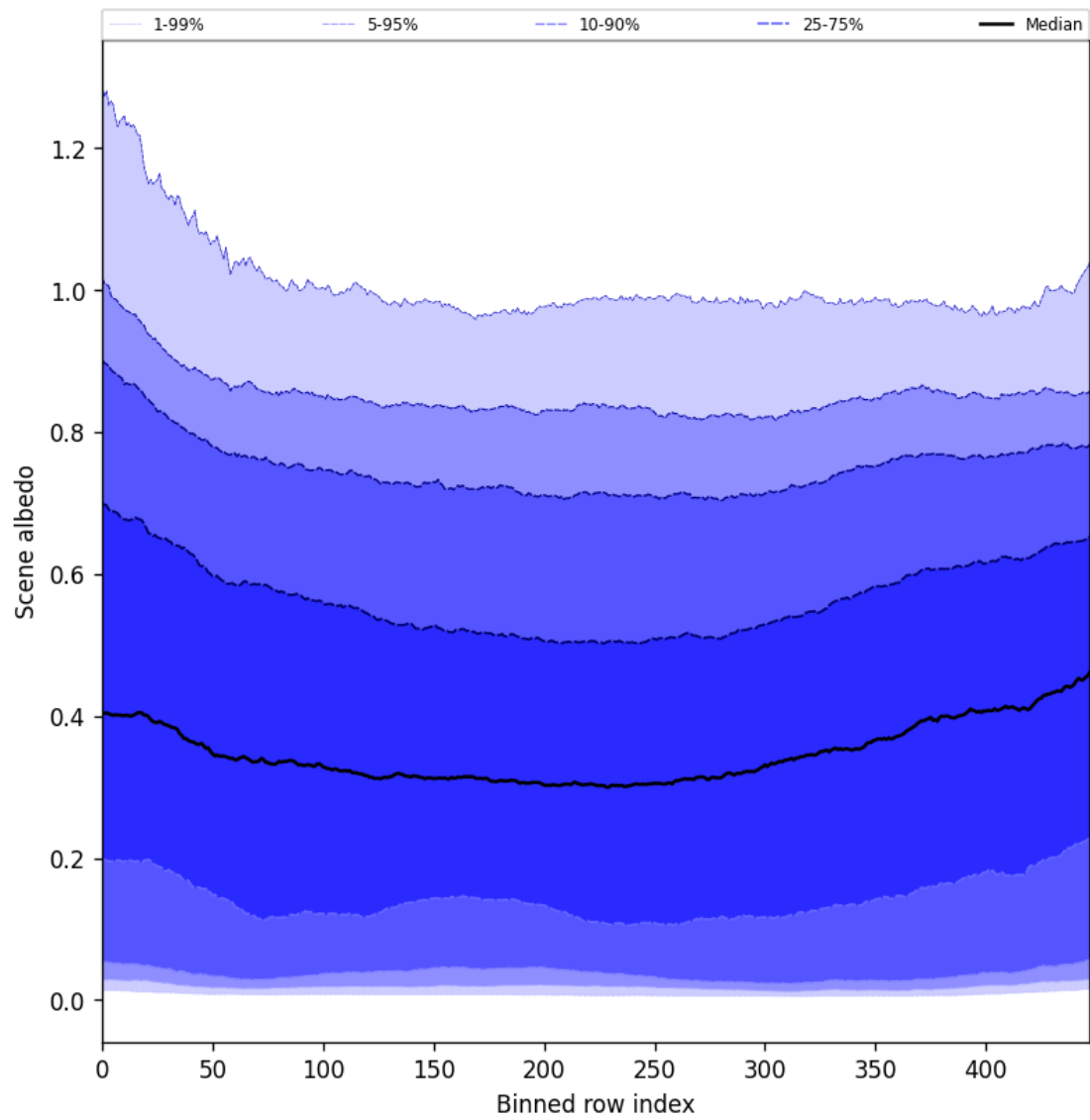
Figure 49: Along track statistics of “Scene albedo” for 2025-07-23 to 2025-07-24
