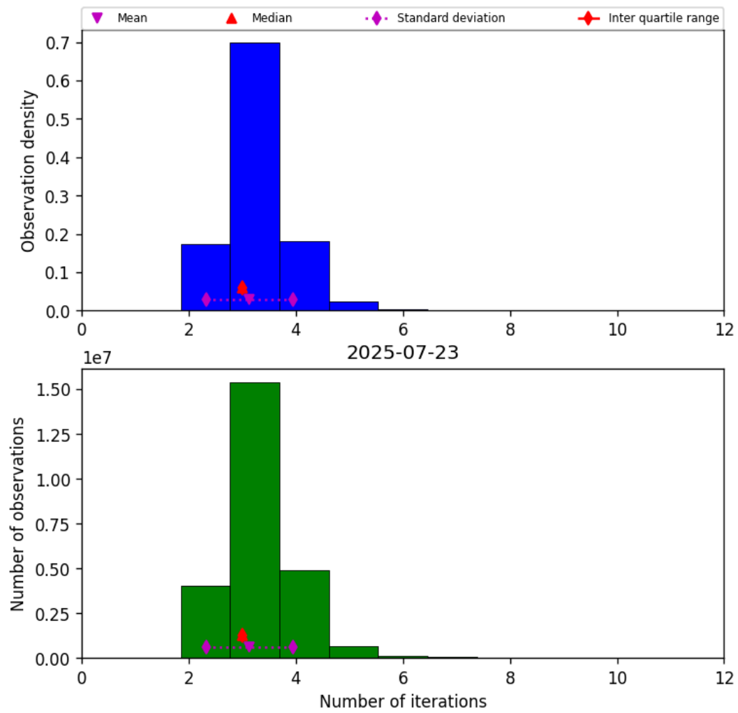
Figure 37: Histogram of “Number of iterations” for 2025-07-23 to 2025-07-24
