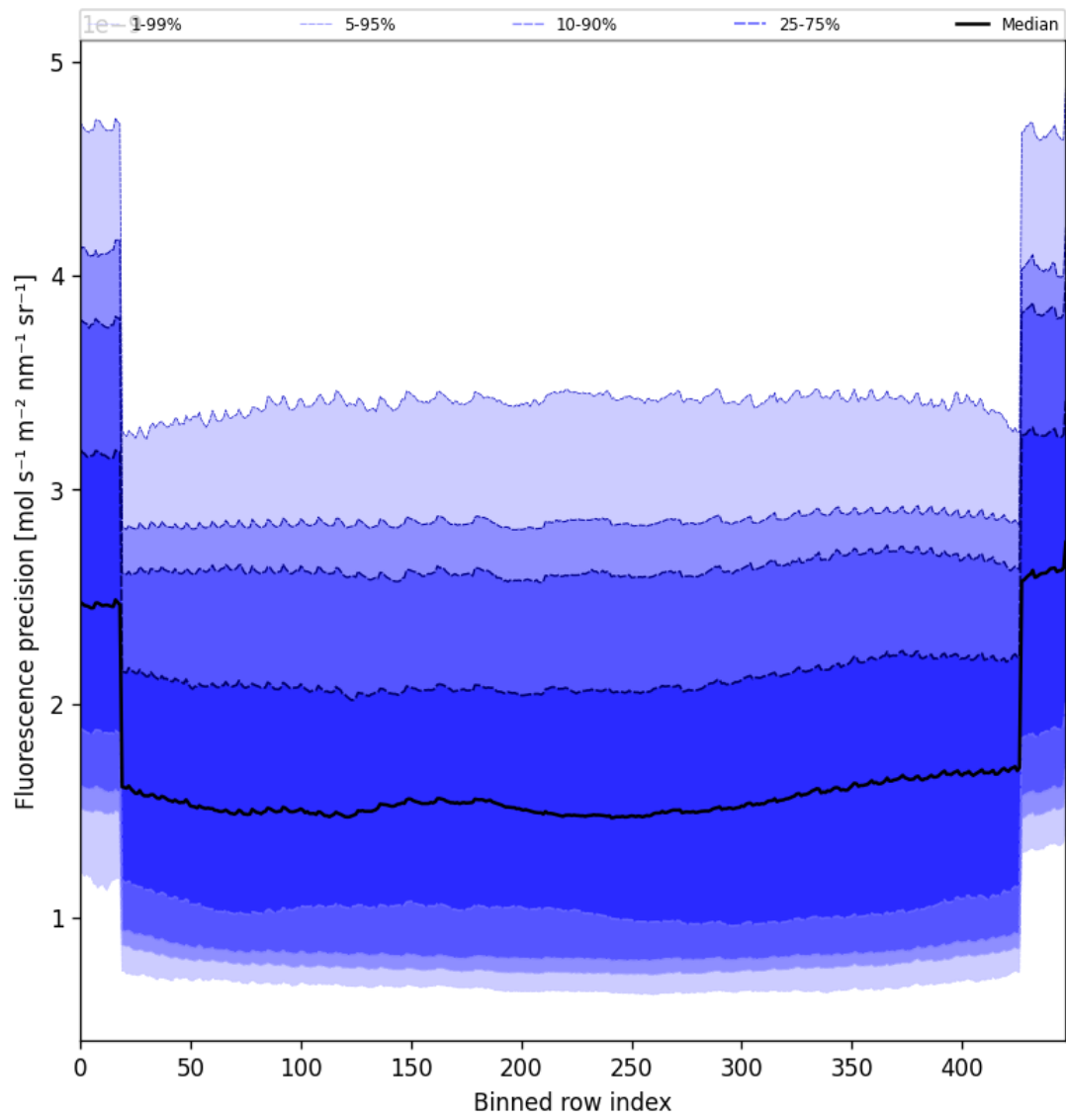
Figure 56: Along track statistics of “Fluorescence precision” for 2025-07-23 to 2025-07-24
