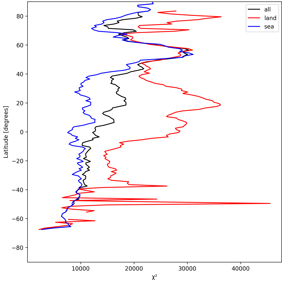
Figure 19: Zonal average of “ \chi^2 ” for 2025-07-23 to 2025-07-24.
