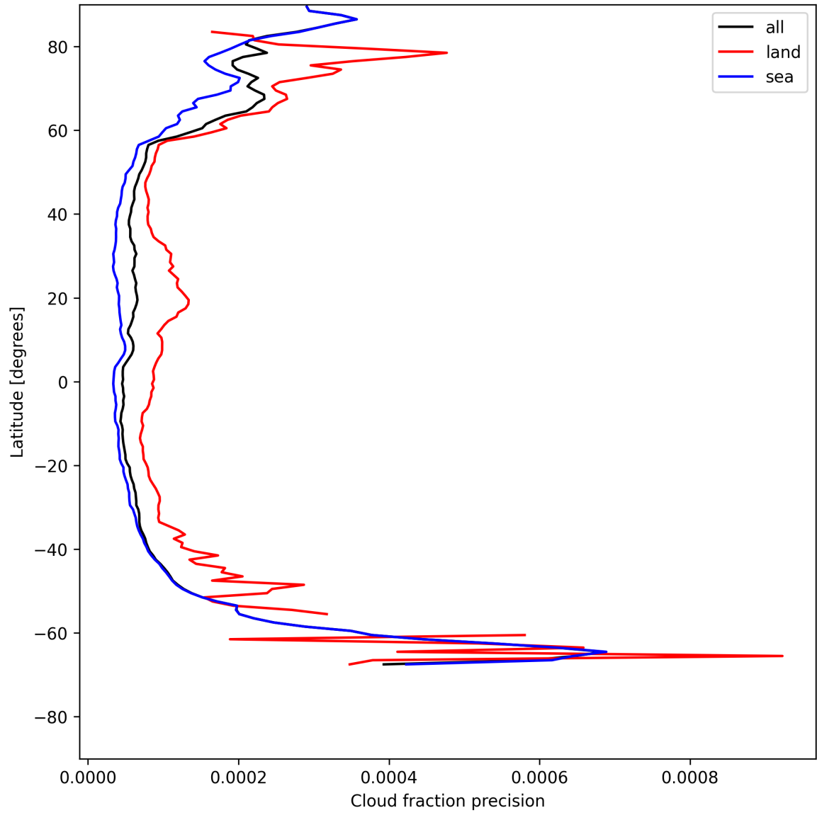
Figure 14: Zonal average of “Cloud fraction precision” for 2025-07-23 to 2025-07-24.
