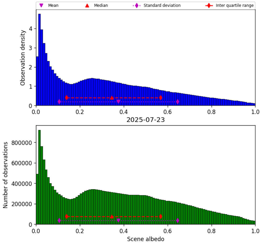
Figure 32: Histogram of “Scene albedo” for 2025-07-23 to 2025-07-24
