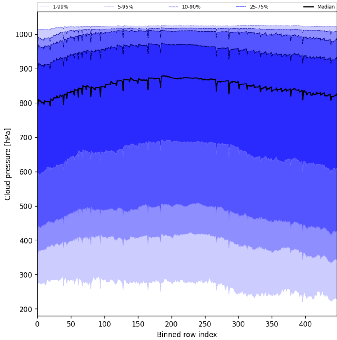
Figure 45: Along track statistics of “Cloud pressure” for 2025-07-23 to 2025-07-24
