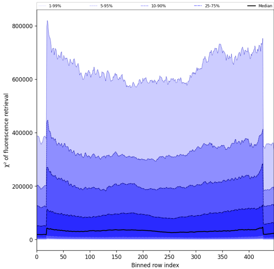
Figure 57: Along track statistics of “ \chi^2 of fluorescence retrieval” for 2025-07-23 to 2025-07-24
