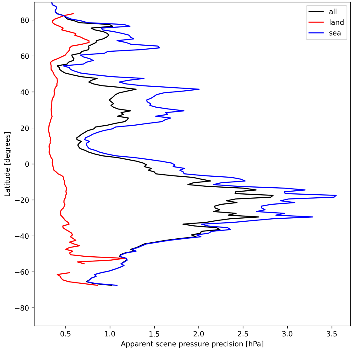
Figure 18: Zonal average of “Apparent scene pressure precision” for 2025-07-23 to 2025-07-24.
