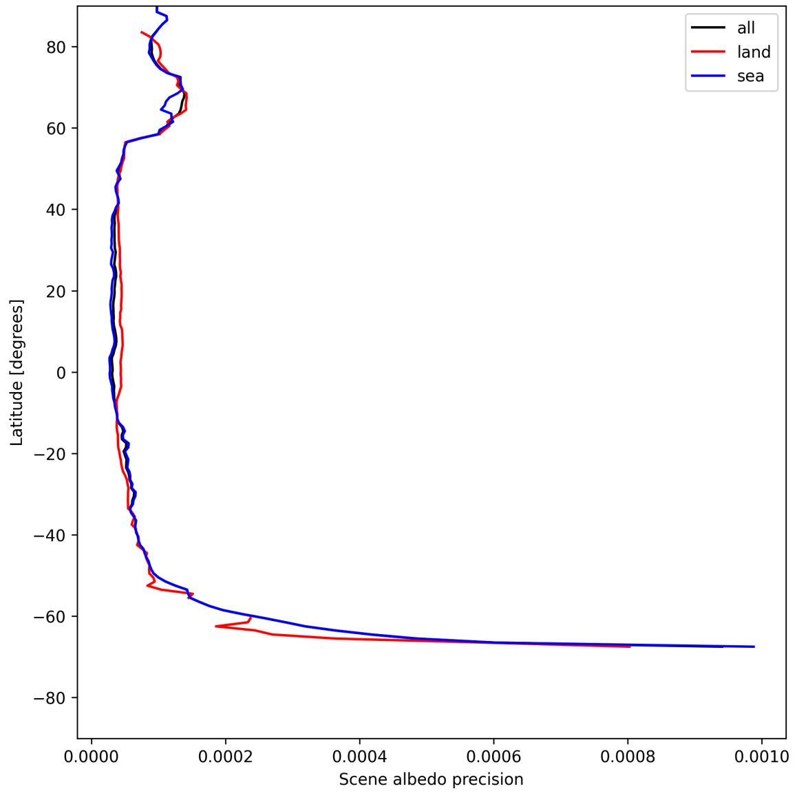
Figure 16: Zonal average of “Scene albedo precision” for 2025-07-23 to 2025-07-24.
