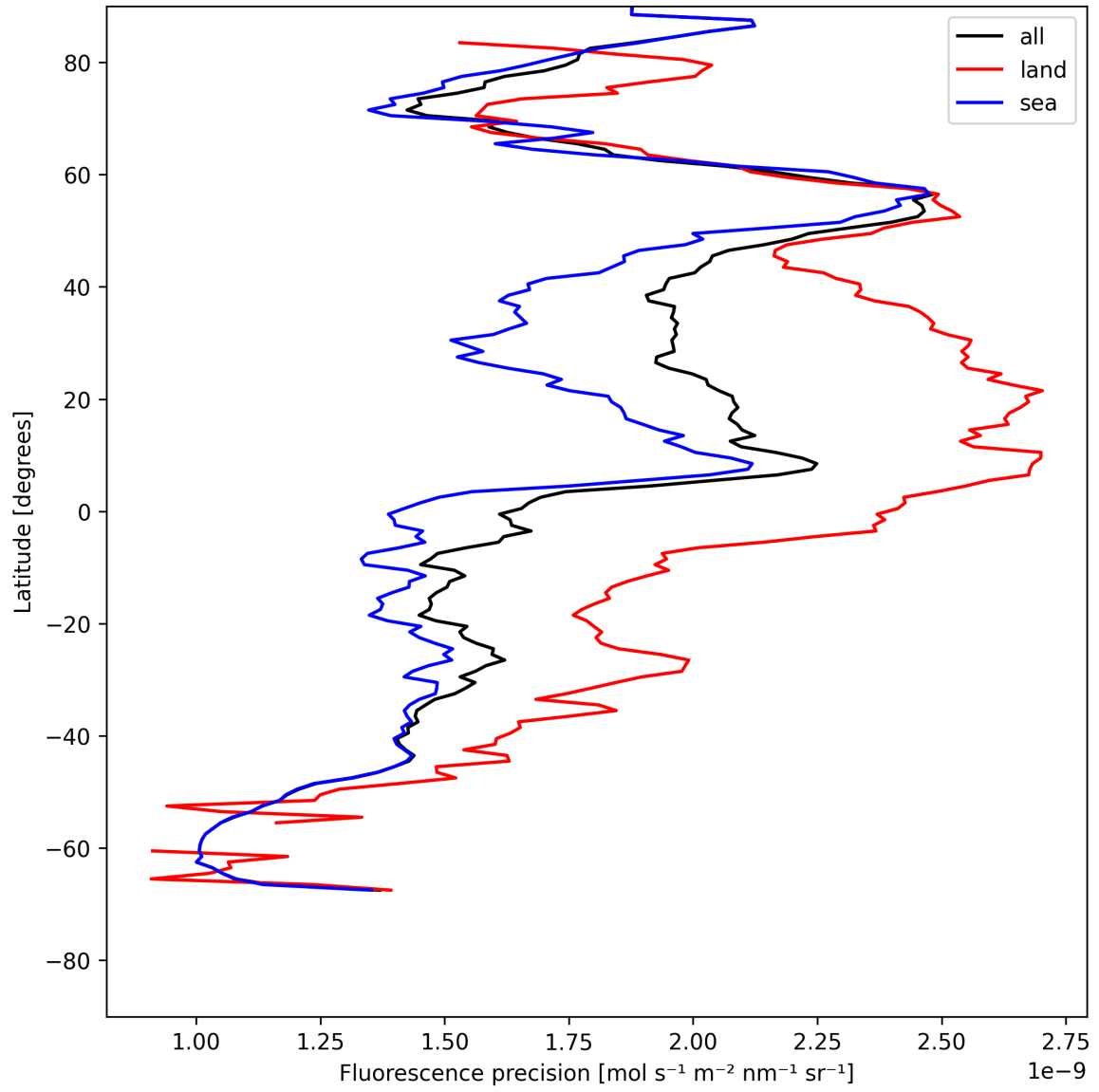
Figure 22: Zonal average of “Fluorescence precision” for 2025-07-23 to 2025-07-24.
