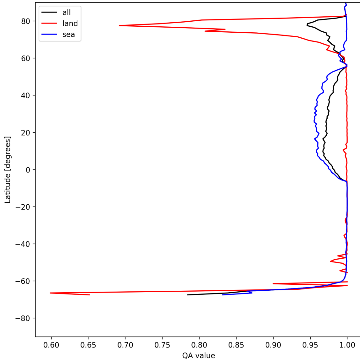
Figure 10: Zonal average of “QA value” for 2025-07-23 to 2025-07-24.
