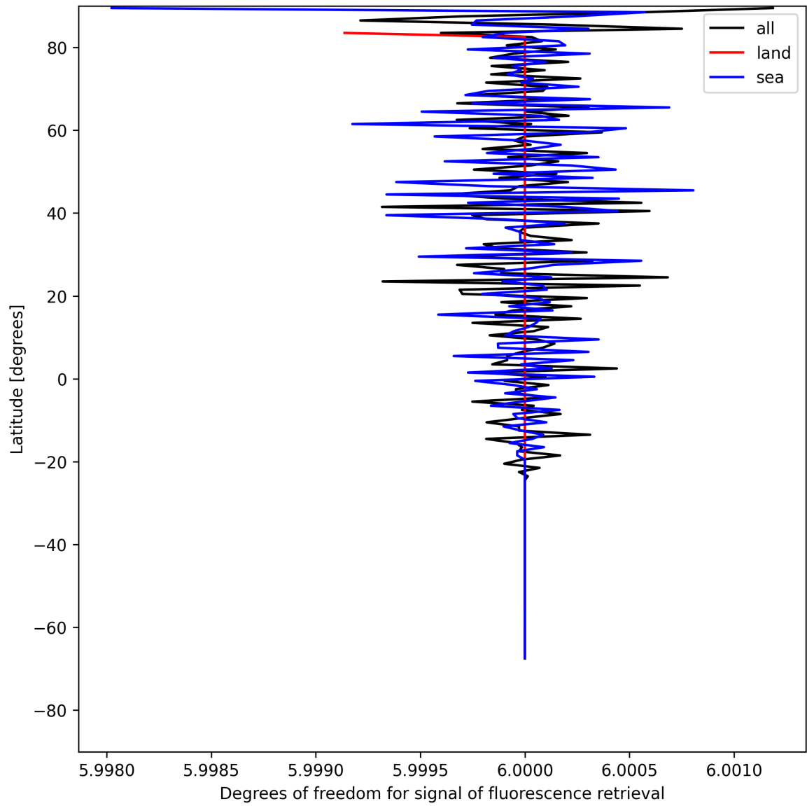
Figure 24: Zonal average of “Degrees of freedom for signal of fluorescence retrieval” for 2025-07-23 to 2025-07-24.
