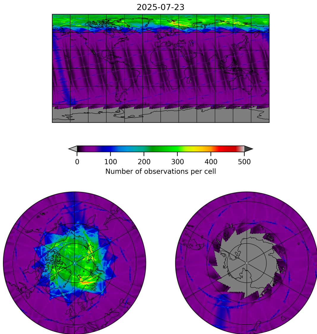
Figure 9: Map of the number of observations for 2025-07-23 to 2025-07-24
