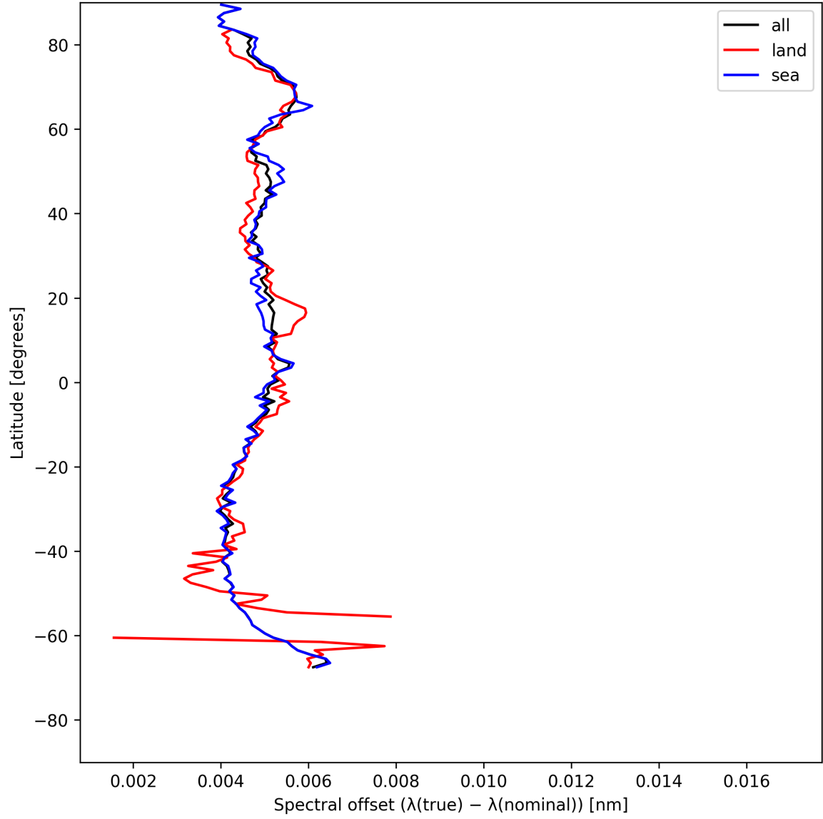
Figure 26: Zonal average of “Spectral offset ( \lambda_{\text{true}} - \lambda_{\text{nominal}} )” for 2025-07-23 to 2025-07-24.
