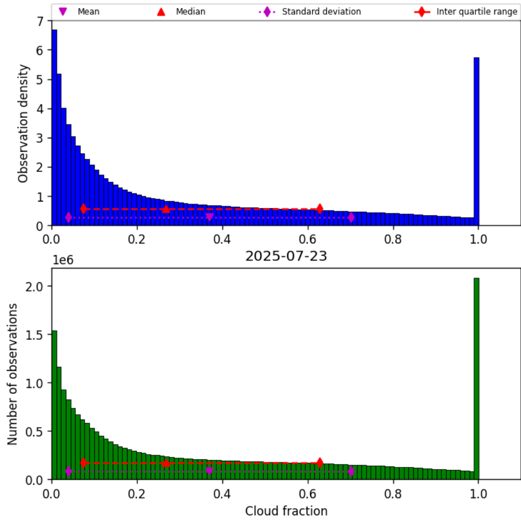
Figure 30: Histogram of “Cloud fraction” for 2025-07-23 to 2025-07-24
