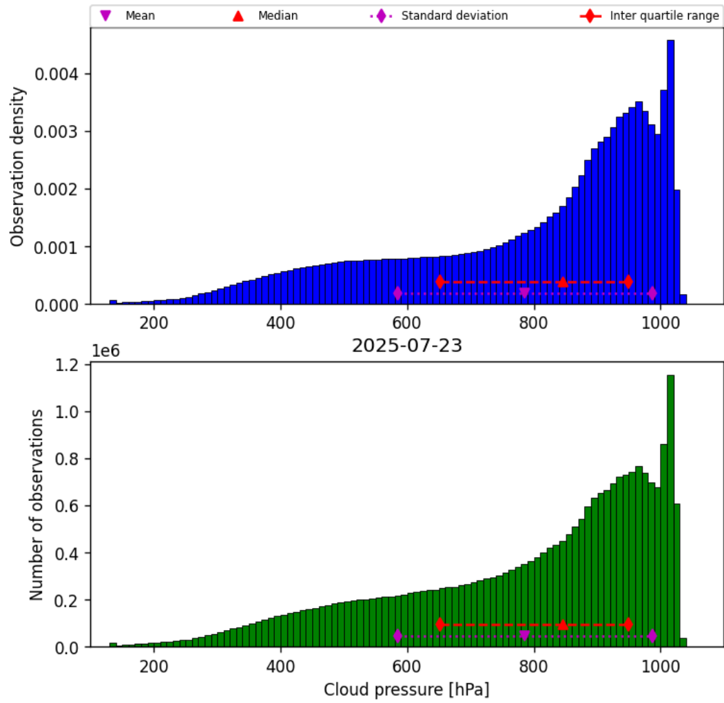
Figure 28: Histogram of “Cloud pressure” for 2025-07-23 to 2025-07-24
