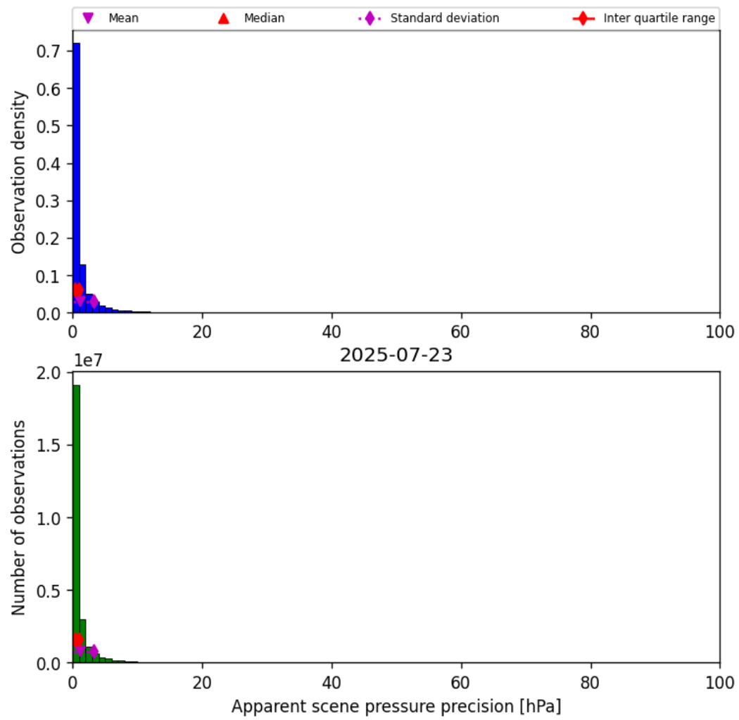
Figure 35: Histogram of “Apparent scene pressure precision” for 2025-07-23 to 2025-07-24
