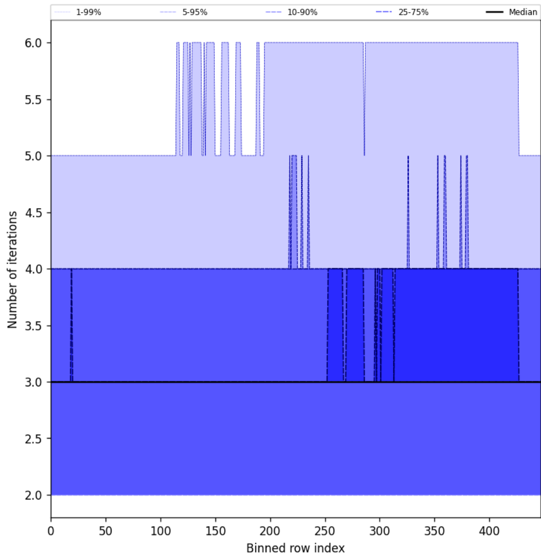
Figure 54: Along track statistics of “Number of iterations” for 2025-07-23 to 2025-07-24
