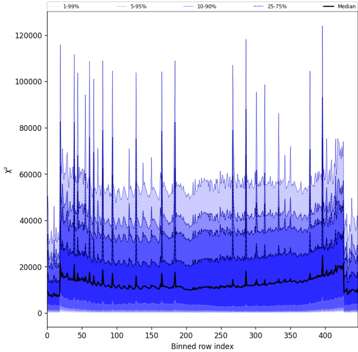
Figure 53: Along track statistics of “ \chi^2 ” for 2025-07-25 to 2025-07-26
