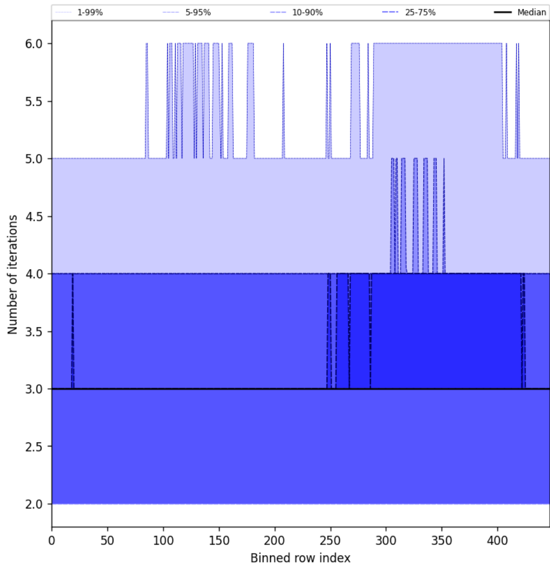
Figure 54: Along track statistics of “Number of iterations” for 2025-07-25 to 2025-07-26
