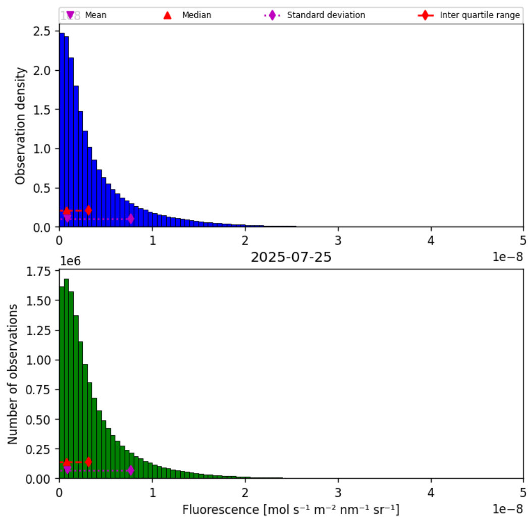
Figure 38: Histogram of “Fluorescence” for 2025-07-25 to 2025-07-26
