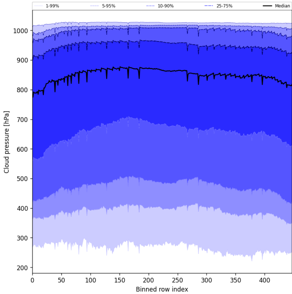
Figure 45: Along track statistics of “Cloud pressure” for 2025-07-25 to 2025-07-26
