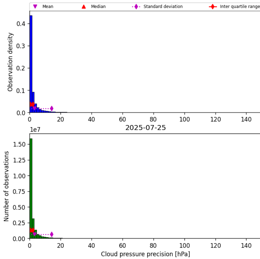
Figure 29: Histogram of “Cloud pressure precision” for 2025-07-25 to 2025-07-26
