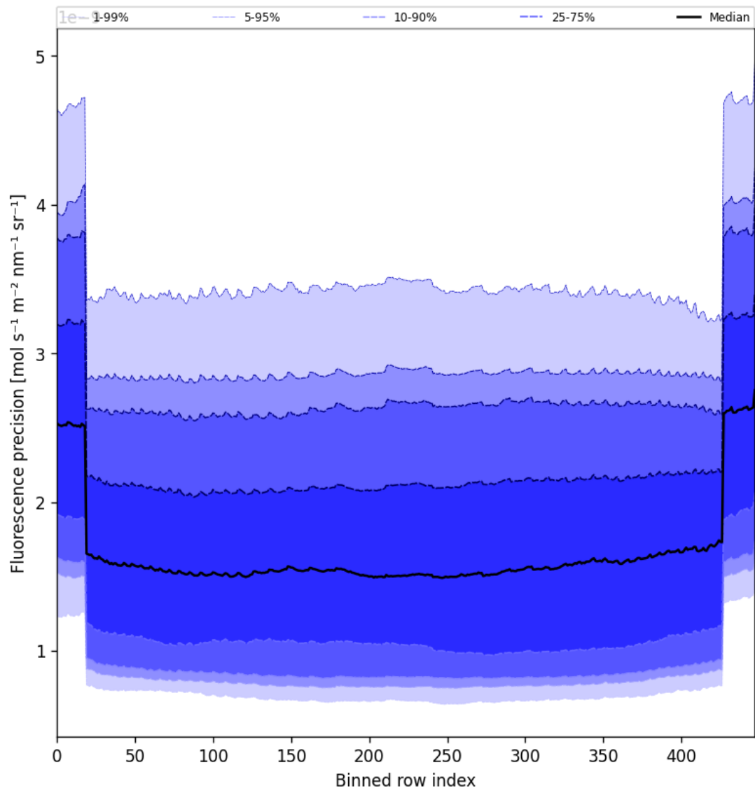
Figure 56: Along track statistics of “Fluorescence precision” for 2025-07-25 to 2025-07-26
