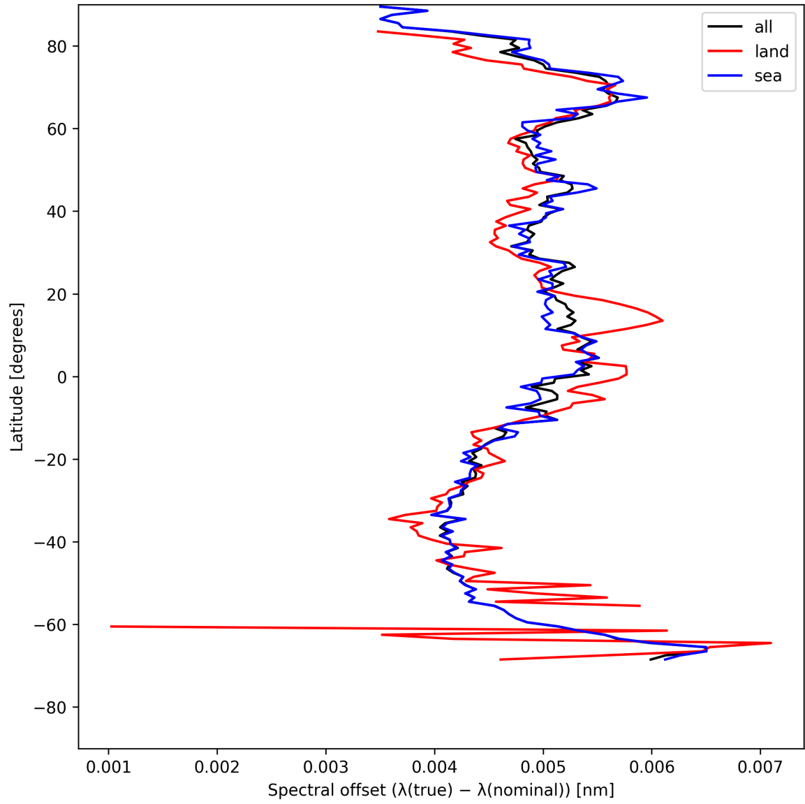
Figure 26: Zonal average of “Spectral offset ( \lambda_{\text{true}} - \lambda_{\text{nominal}} )” for 2025-07-25 to 2025-07-26.
