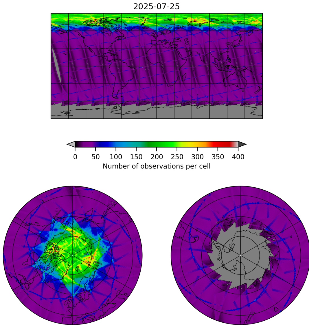
Figure 9: Map of the number of observations for 2025-07-25 to 2025-07-26
