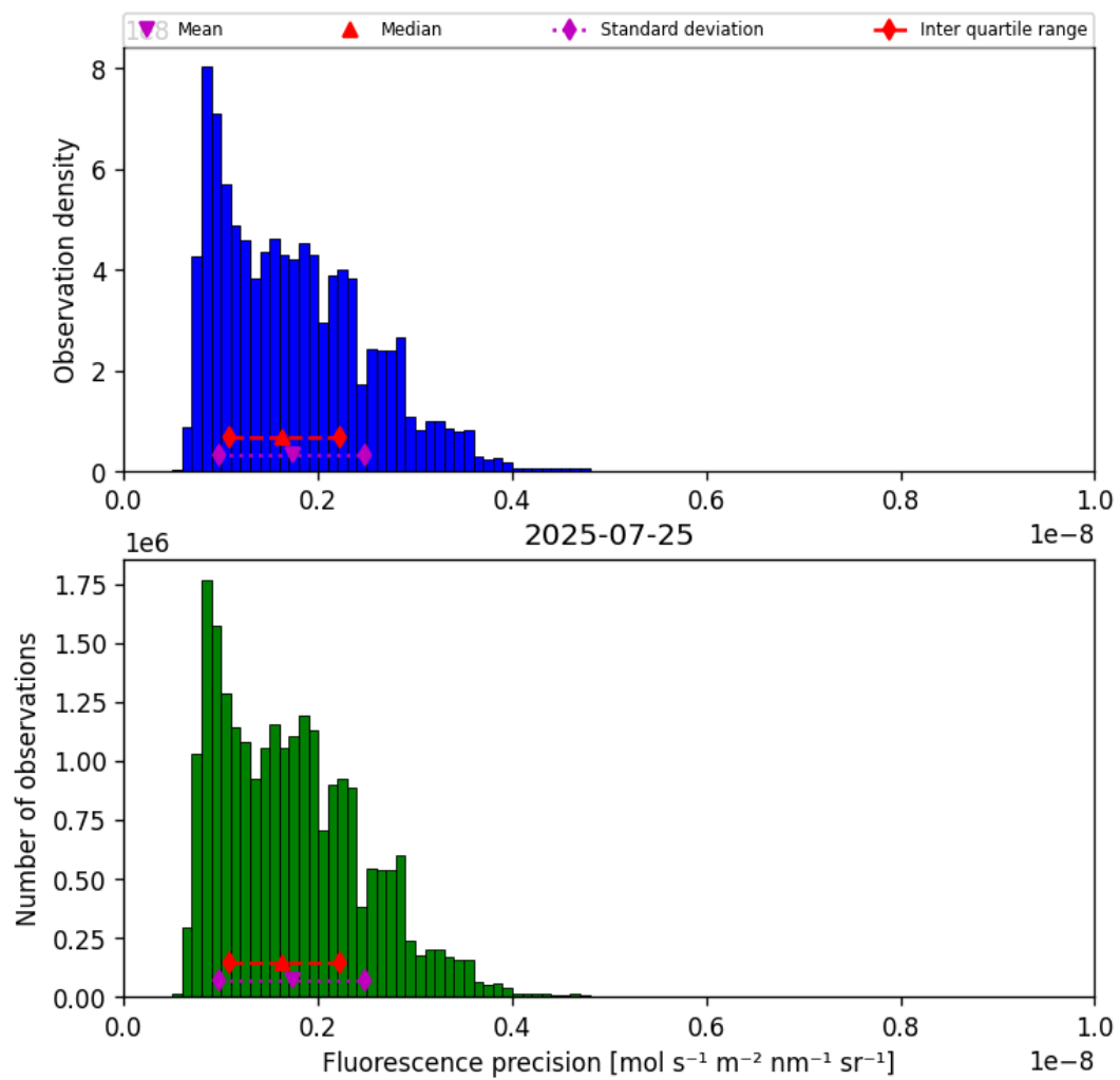
Figure 39: Histogram of “Fluorescence precision” for 2025-07-25 to 2025-07-26
