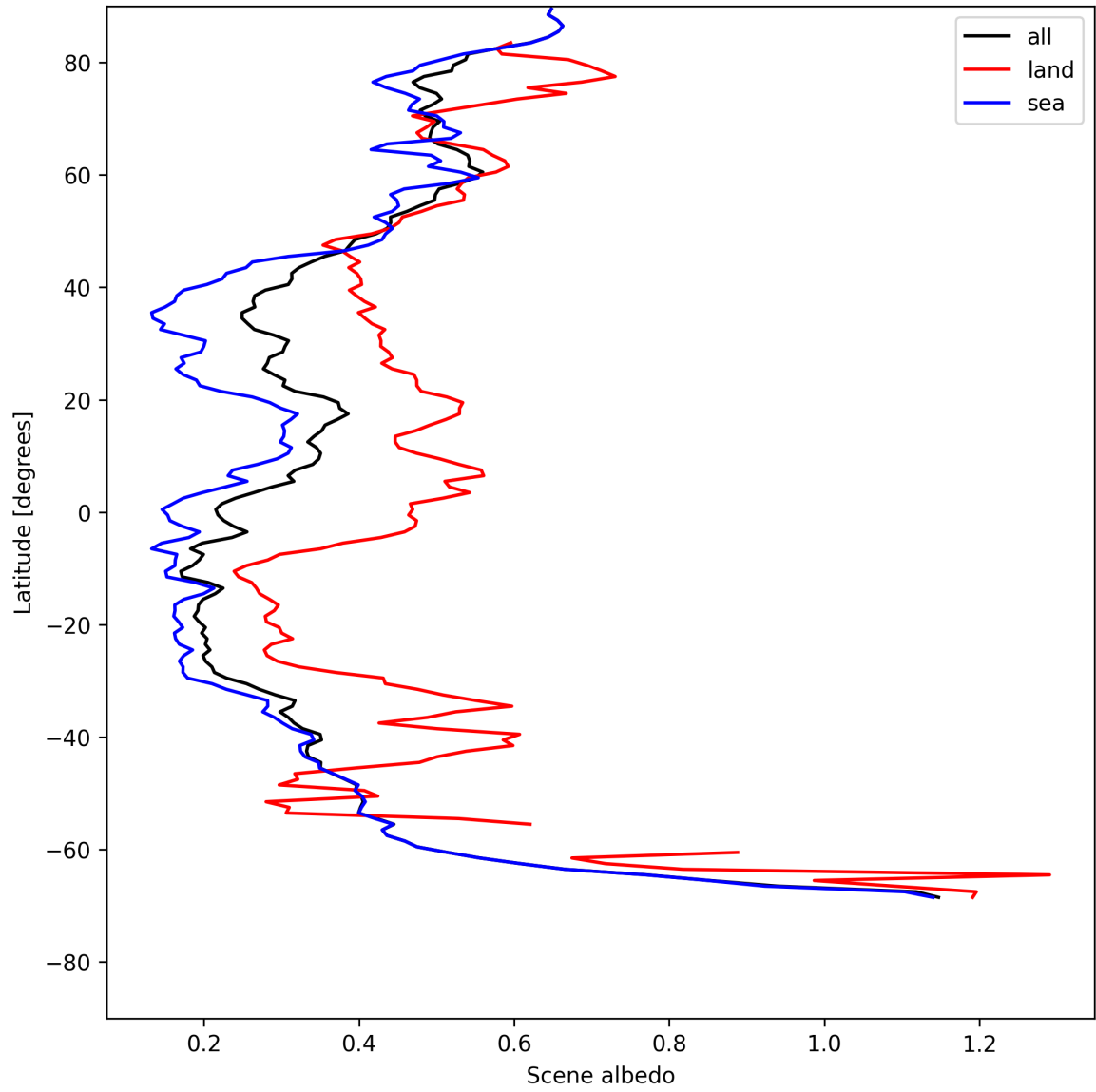
Figure 15: Zonal average of “Scene albedo” for 2025-07-25 to 2025-07-26.
