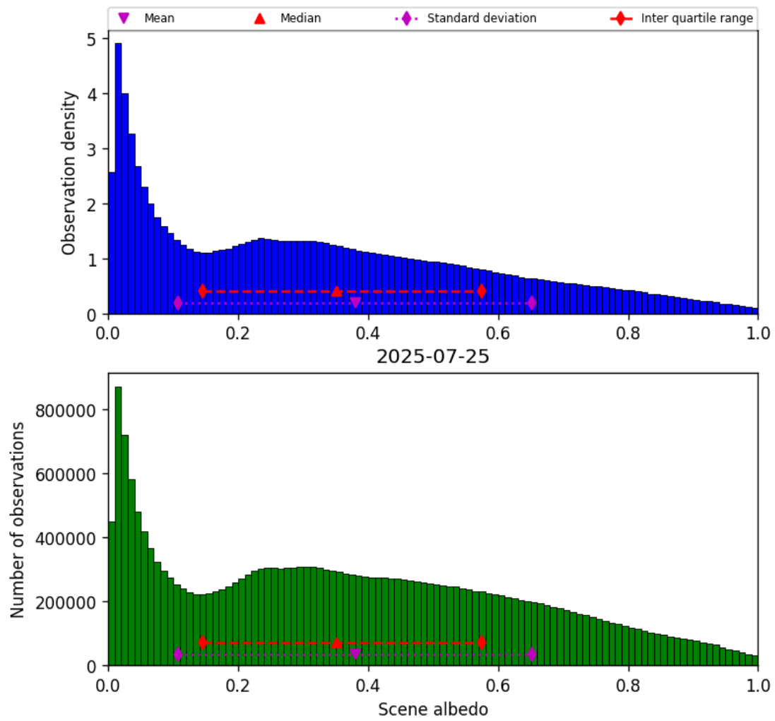
Figure 32: Histogram of “Scene albedo” for 2025-07-25 to 2025-07-26
