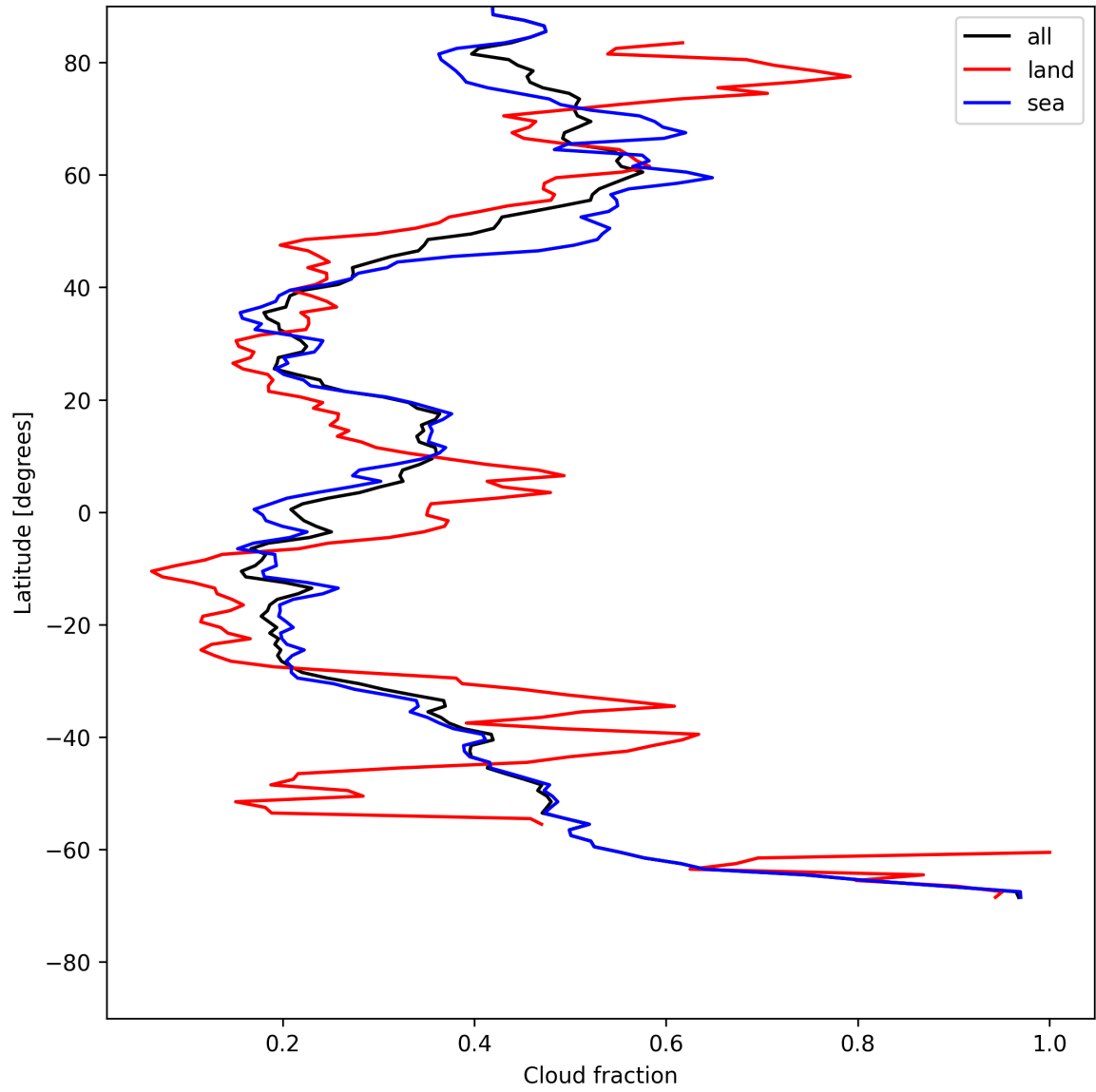
Figure 13: Zonal average of “Cloud fraction” for 2025-07-25 to 2025-07-26.
