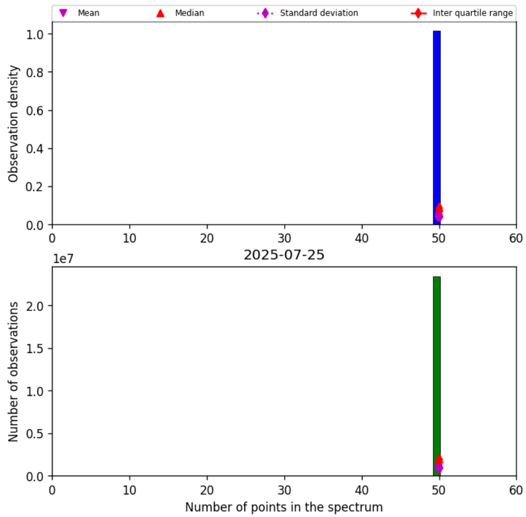
Figure 42: Histogram of “Number of points in the spectrum” for 2025-07-25 to 2025-07-26
