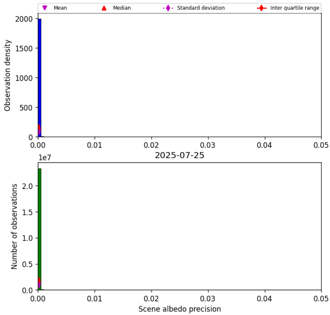
Figure 33: Histogram of “Scene albedo precision” for 2025-07-25 to 2025-07-26
