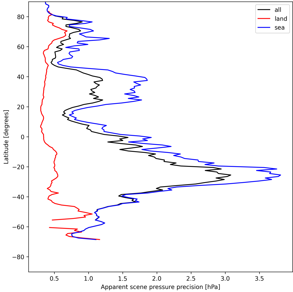
Figure 18: Zonal average of “Apparent scene pressure precision” for 2025-07-25 to 2025-07-26.
