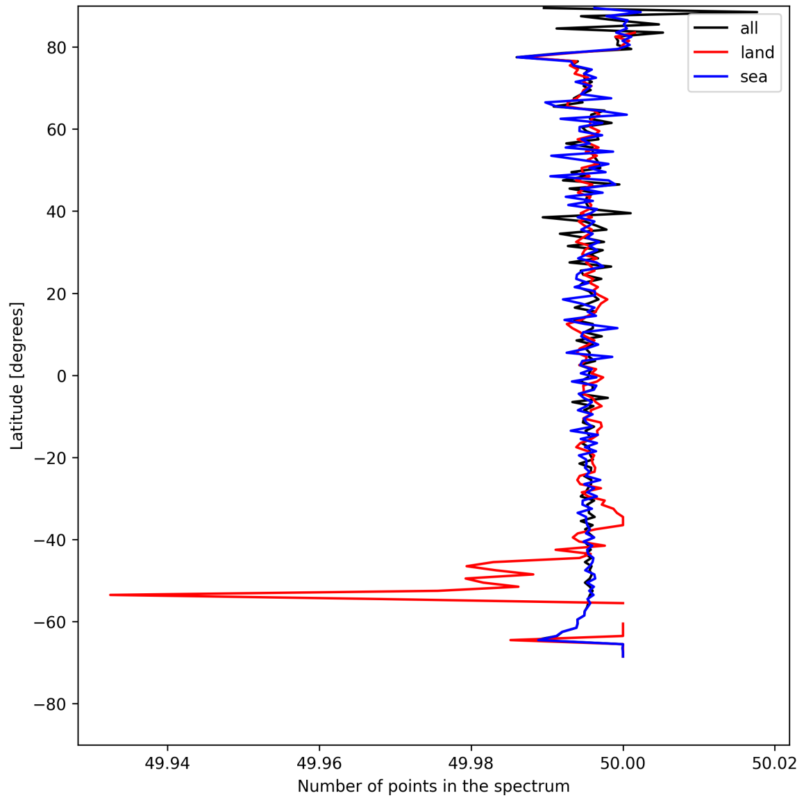
Figure 25: Zonal average of “Number of points in the spectrum” for 2025-07-25 to 2025-07-26.
