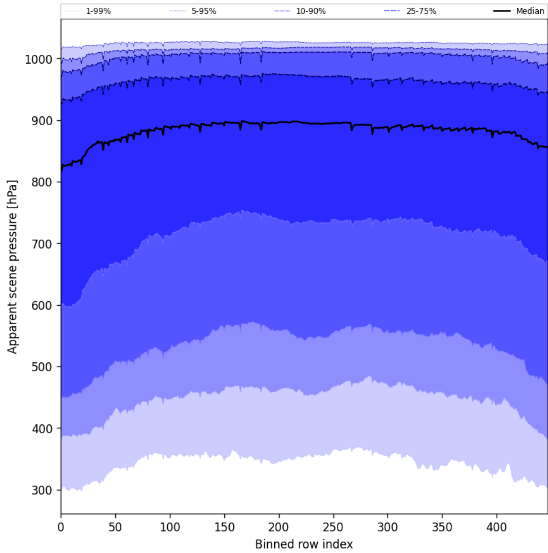
Figure 51: Along track statistics of “Apparent scene pressure” for 2025-07-25 to 2025-07-26
