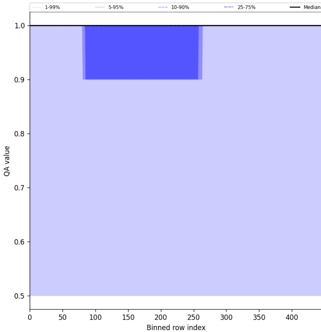
Figure 44: Along track statistics of “QA value” for 2025-07-25 to 2025-07-26
