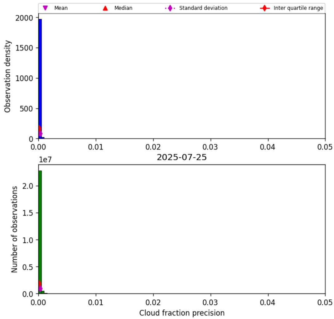
Figure 31: Histogram of “Cloud fraction precision” for 2025-07-25 to 2025-07-26
