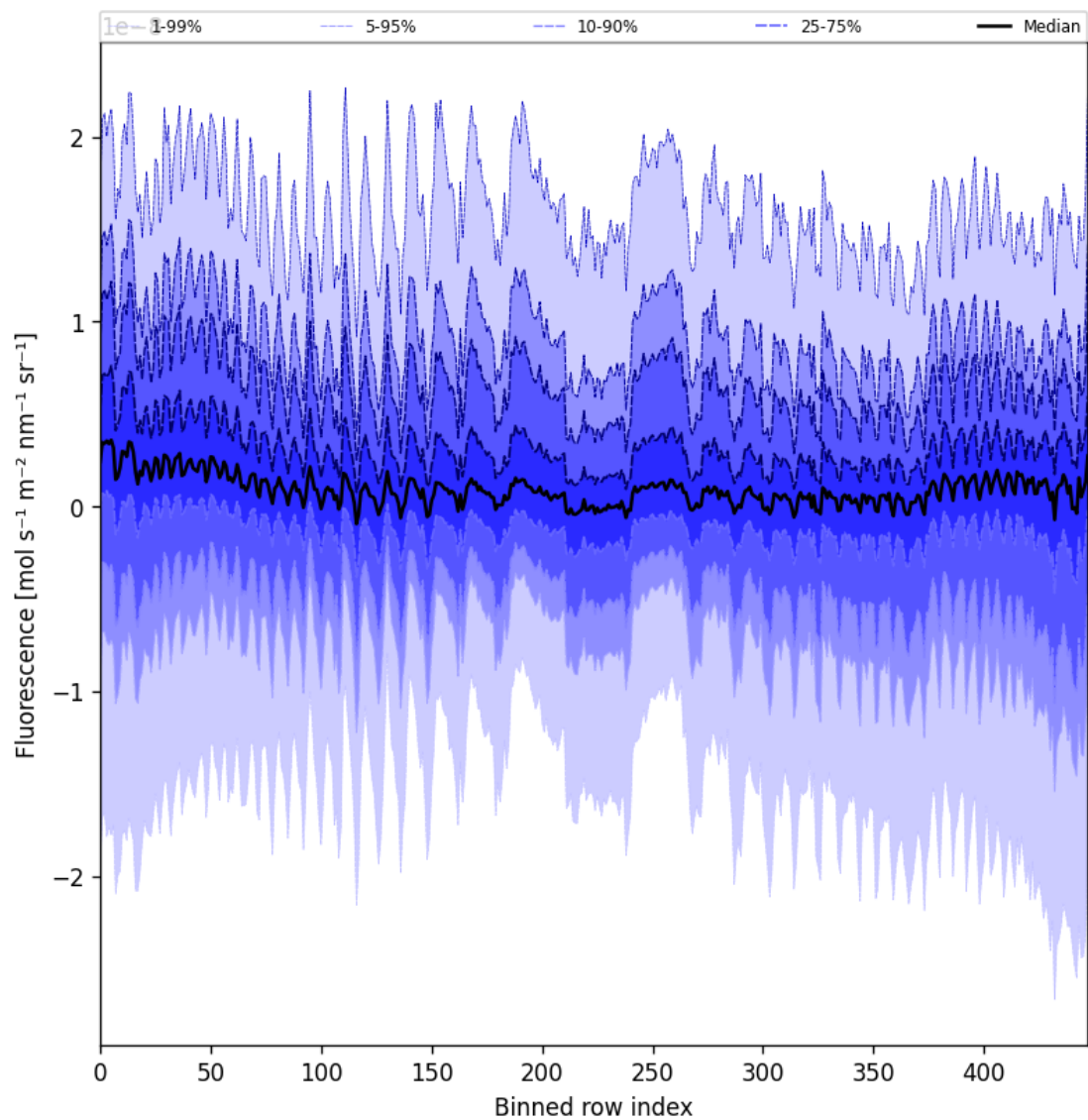
Figure 55: Along track statistics of “Fluorescence” for 2025-07-25 to 2025-07-26
