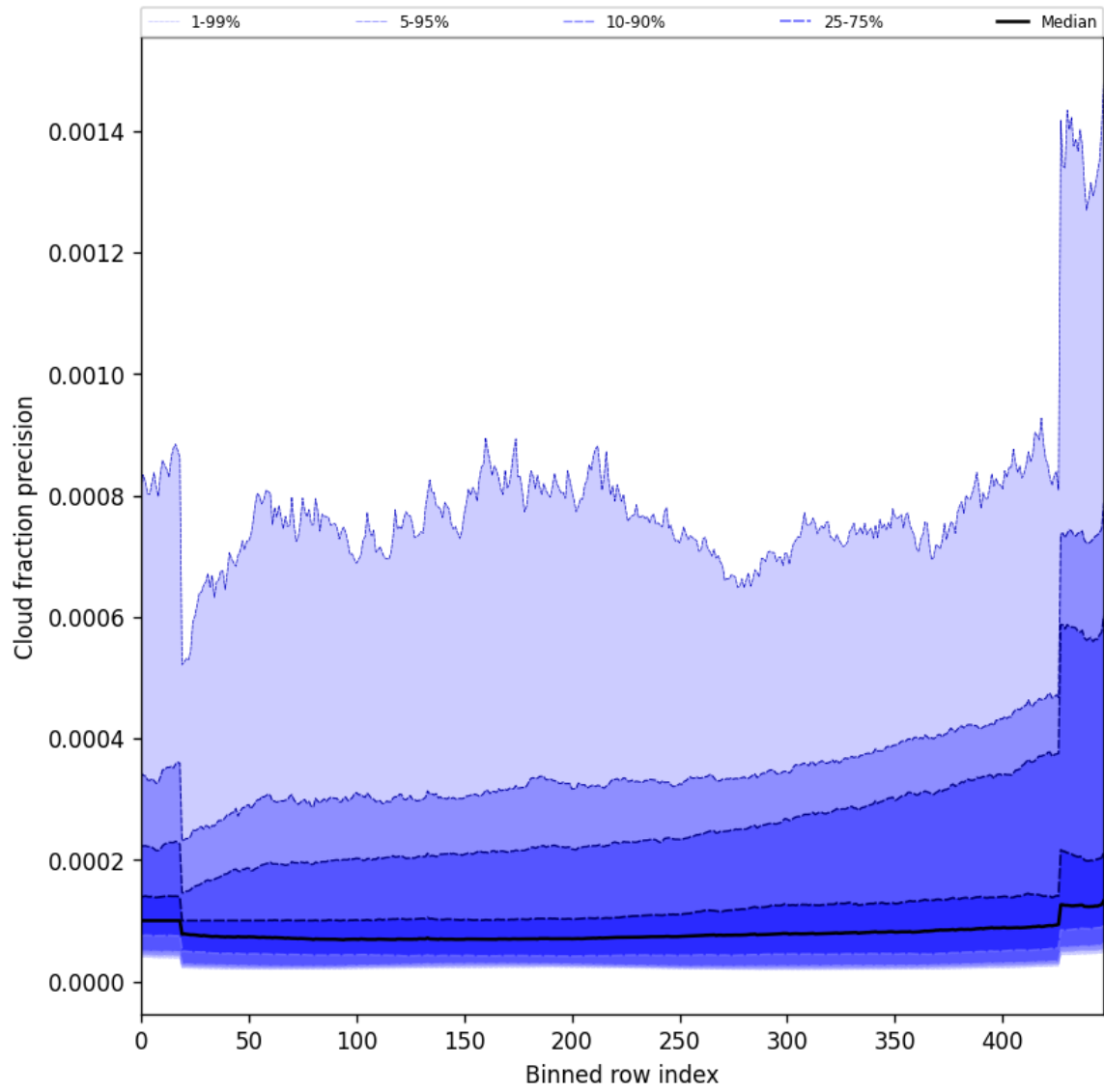
Figure 48: Along track statistics of “Cloud fraction precision” for 2025-07-25 to 2025-07-26
