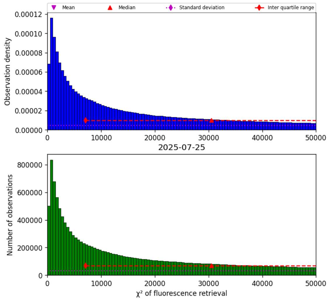
Figure 40: Histogram of “ \chi^2 of fluorescence retrieval” for 2025-07-25 to 2025-07-26
