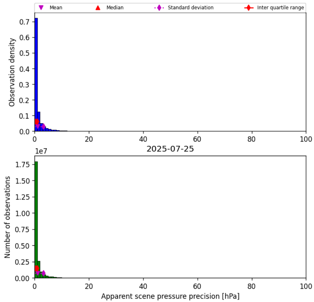
Figure 35: Histogram of “Apparent scene pressure precision” for 2025-07-25 to 2025-07-26
