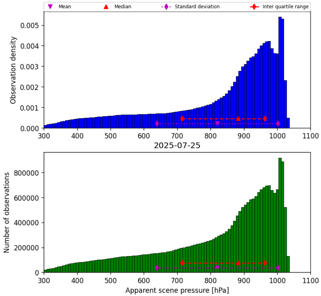
Figure 34: Histogram of “Apparent scene pressure” for 2025-07-25 to 2025-07-26
