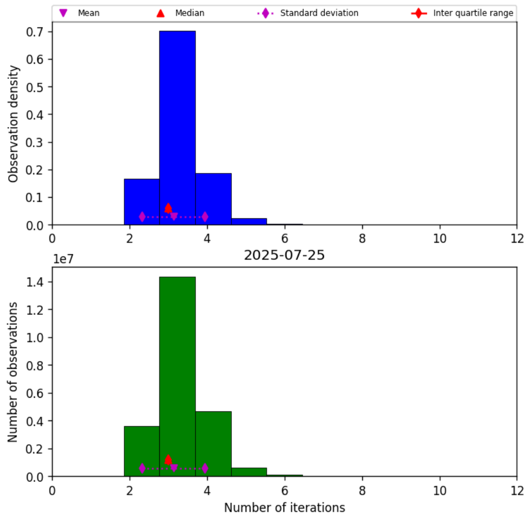
Figure 37: Histogram of “Number of iterations” for 2025-07-25 to 2025-07-26
