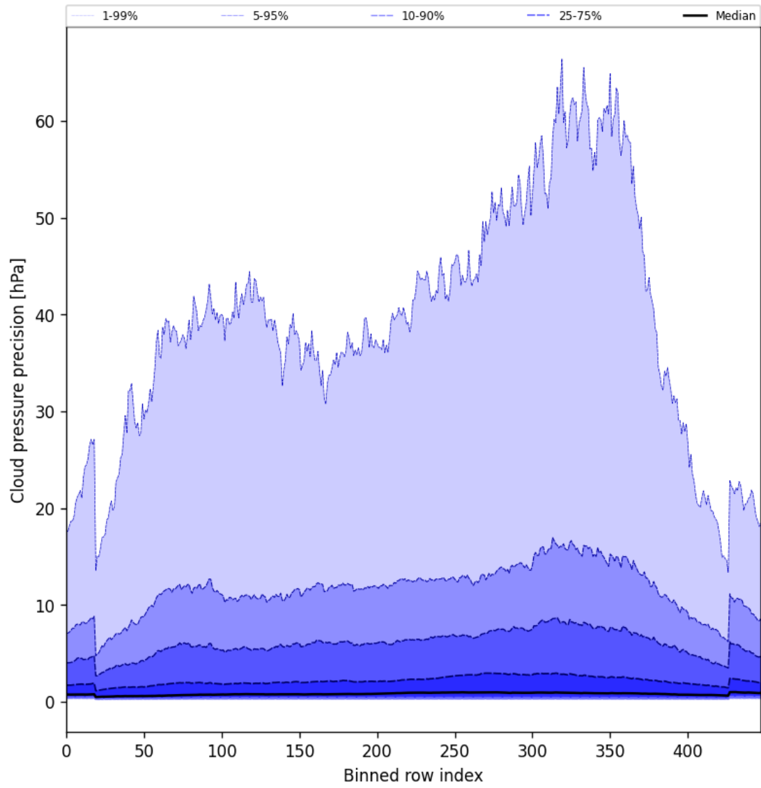
Figure 46: Along track statistics of “Cloud pressure precision” for 2025-07-25 to 2025-07-26
