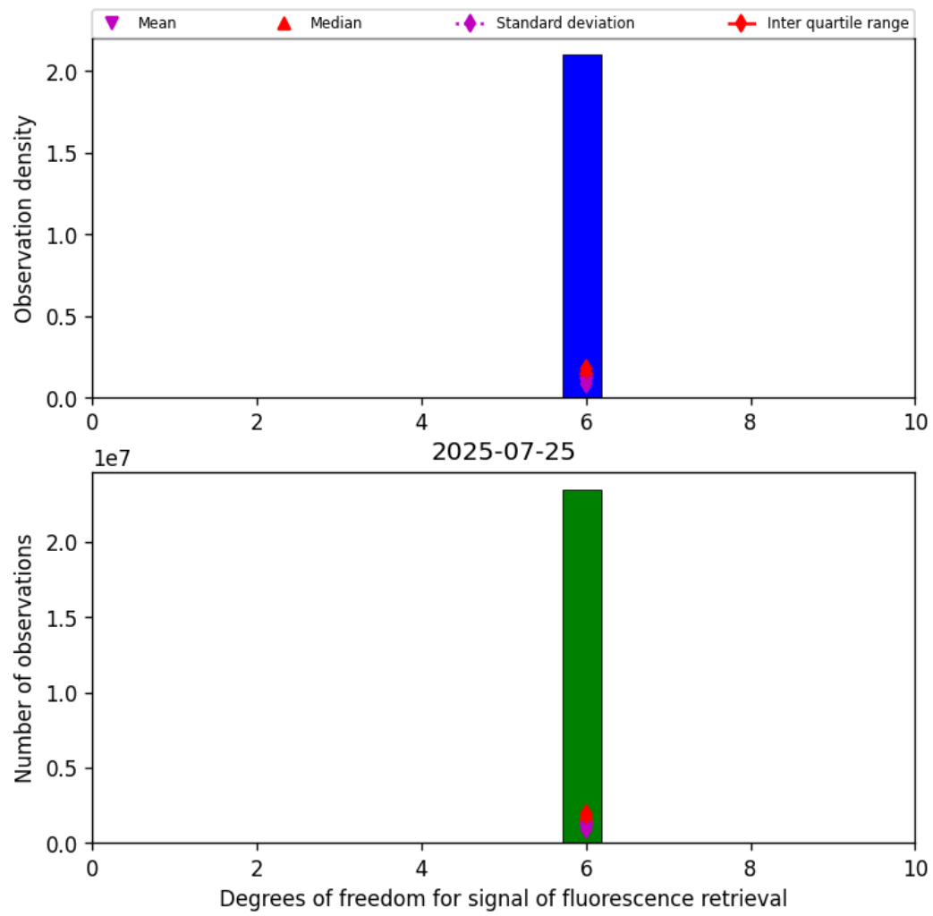
Figure 41: Histogram of “Degrees of freedom for signal of fluorescence retrieval” for 2025-07-25 to 2025-07-26
