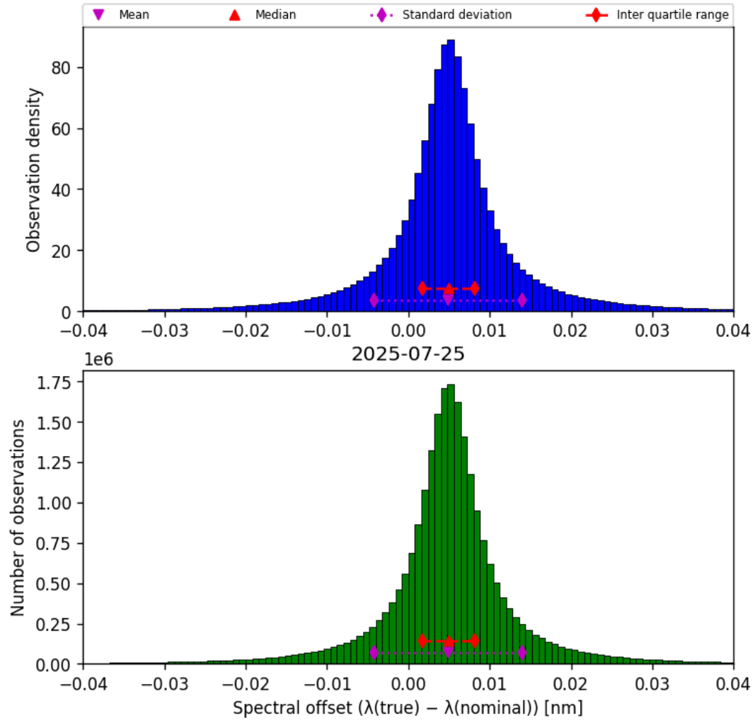
Figure 43: Histogram of “Spectral offset ( \lambda_{\text{true}} - \lambda_{\text{nominal}} )” for 2025-07-25 to 2025-07-26
