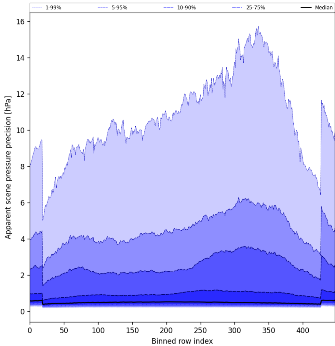
Figure 52: Along track statistics of “Apparent scene pressure precision” for 2025-07-25 to 2025-07-26
