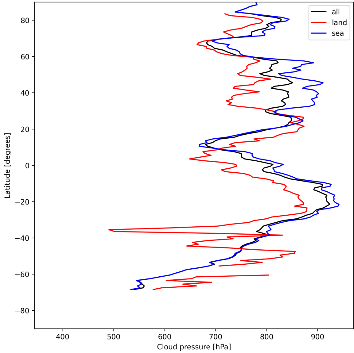
Figure 11: Zonal average of “Cloud pressure” for 2025-07-25 to 2025-07-26.
