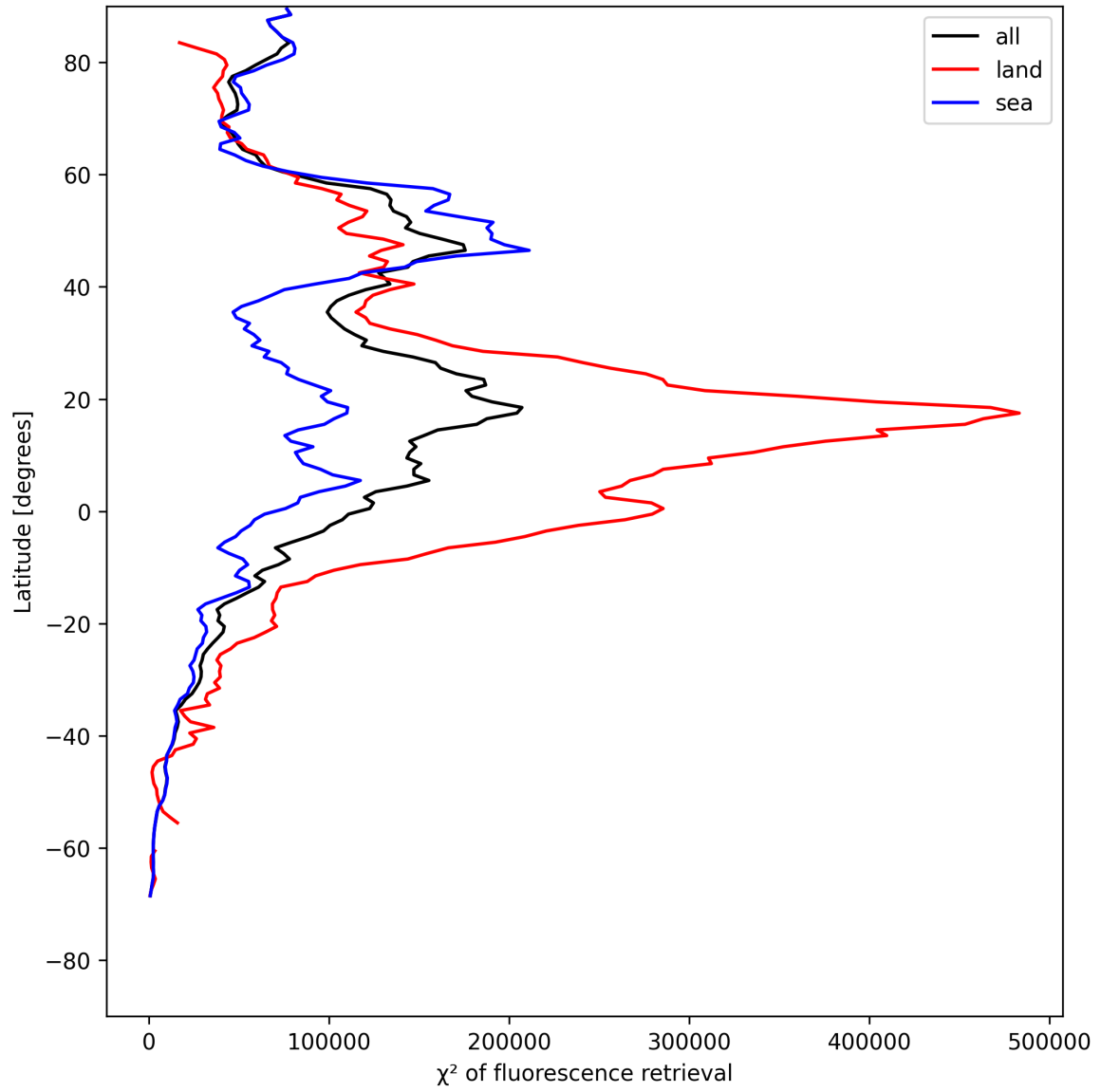
Figure 23: Zonal average of “ \chi^2 of fluorescence retrieval” for 2025-07-25 to 2025-07-26.
