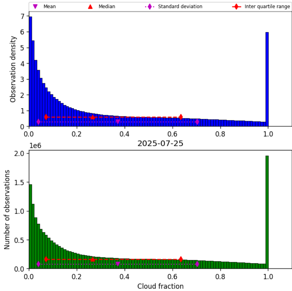
Figure 30: Histogram of “Cloud fraction” for 2025-07-25 to 2025-07-26
