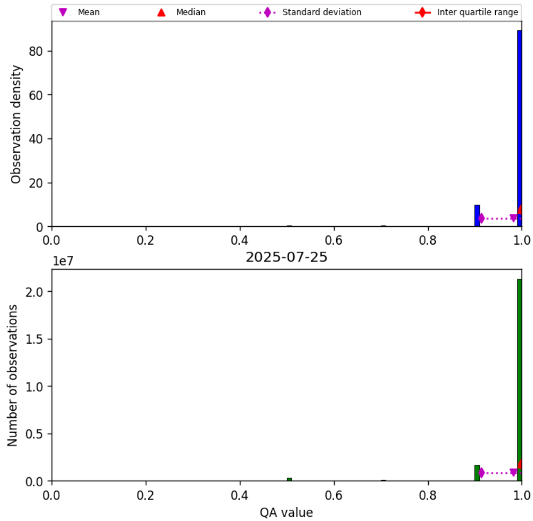
Figure 27: Histogram of “QA value” for 2025-07-25 to 2025-07-26
