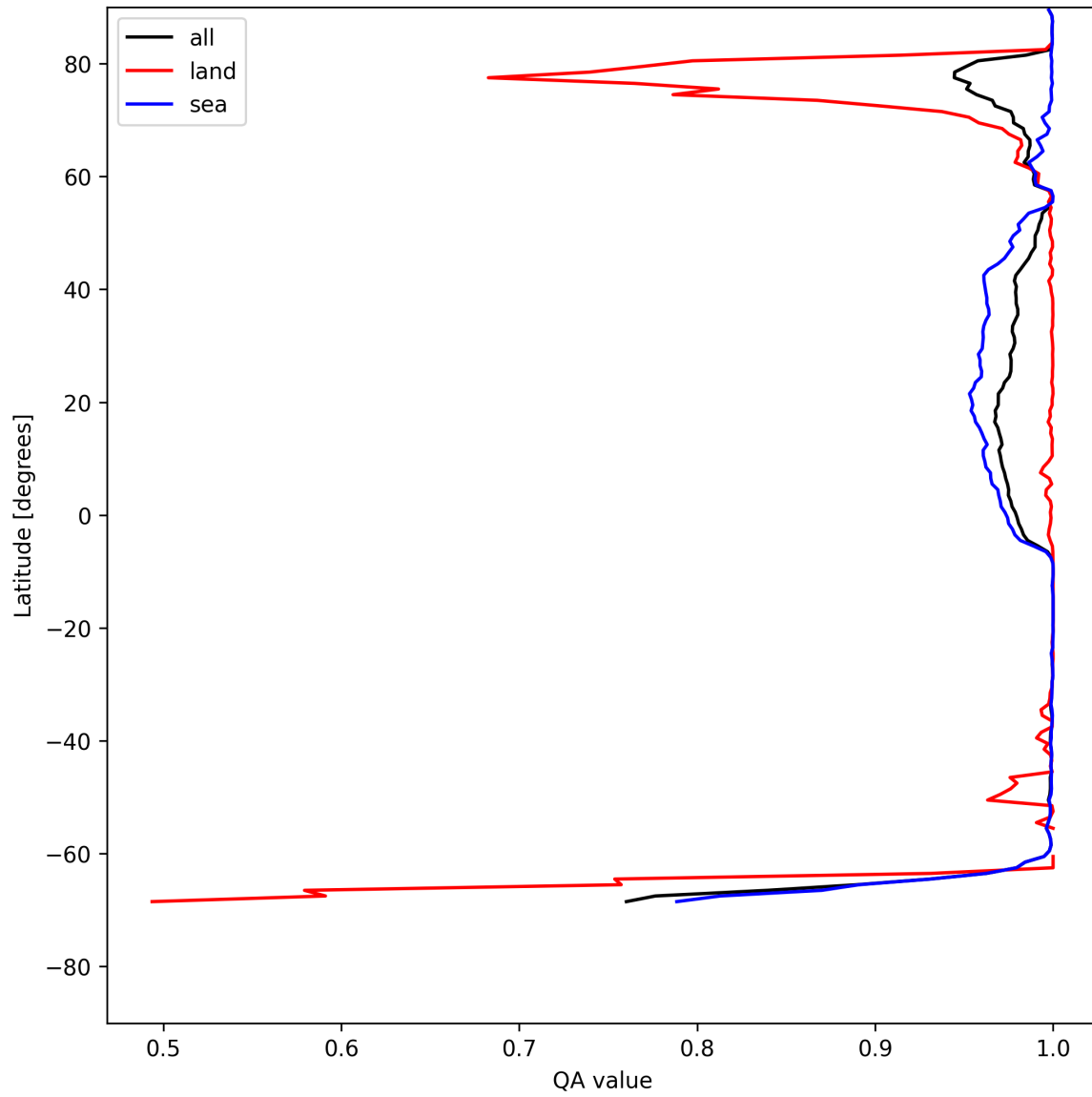
Figure 10: Zonal average of "QA value" for 2025-07-25 to 2025-07-26.
