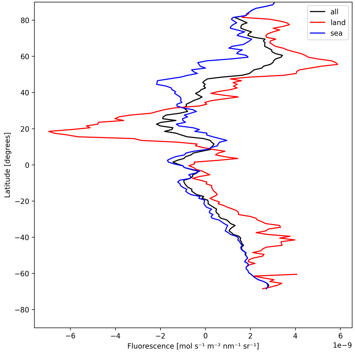
Figure 21: Zonal average of “Fluorescence” for 2025-07-25 to 2025-07-26.
