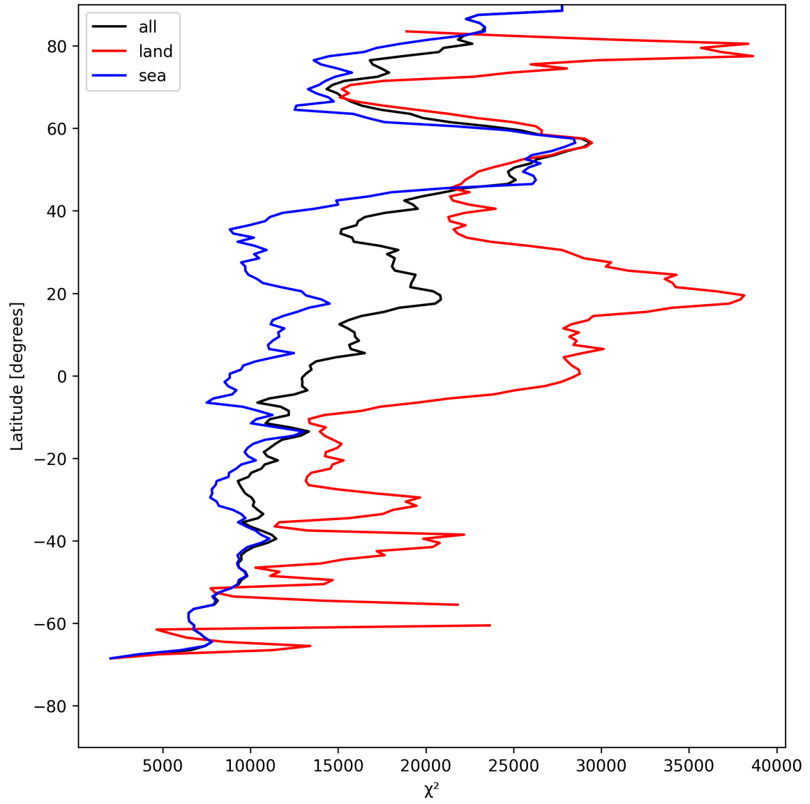
Figure 19: Zonal average of “ \chi^2 ” for 2025-07-25 to 2025-07-26.
