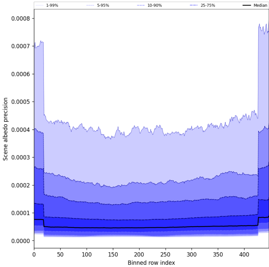
Figure 50: Along track statistics of “Scene albedo precision” for 2025-07-25 to 2025-07-26
