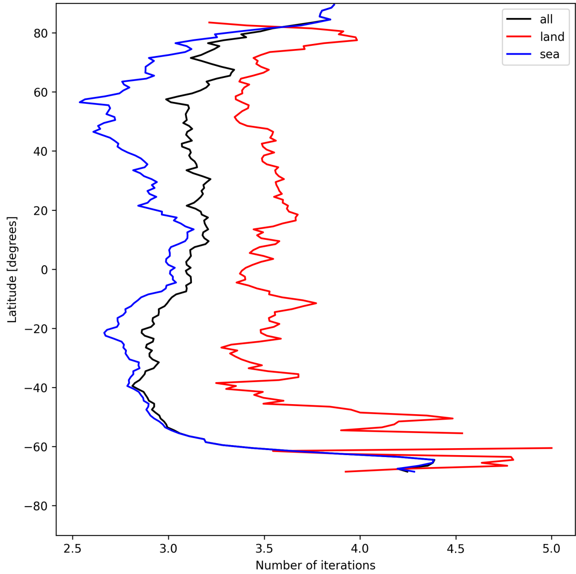
Figure 20: Zonal average of “Number of iterations” for 2025-07-25 to 2025-07-26.
