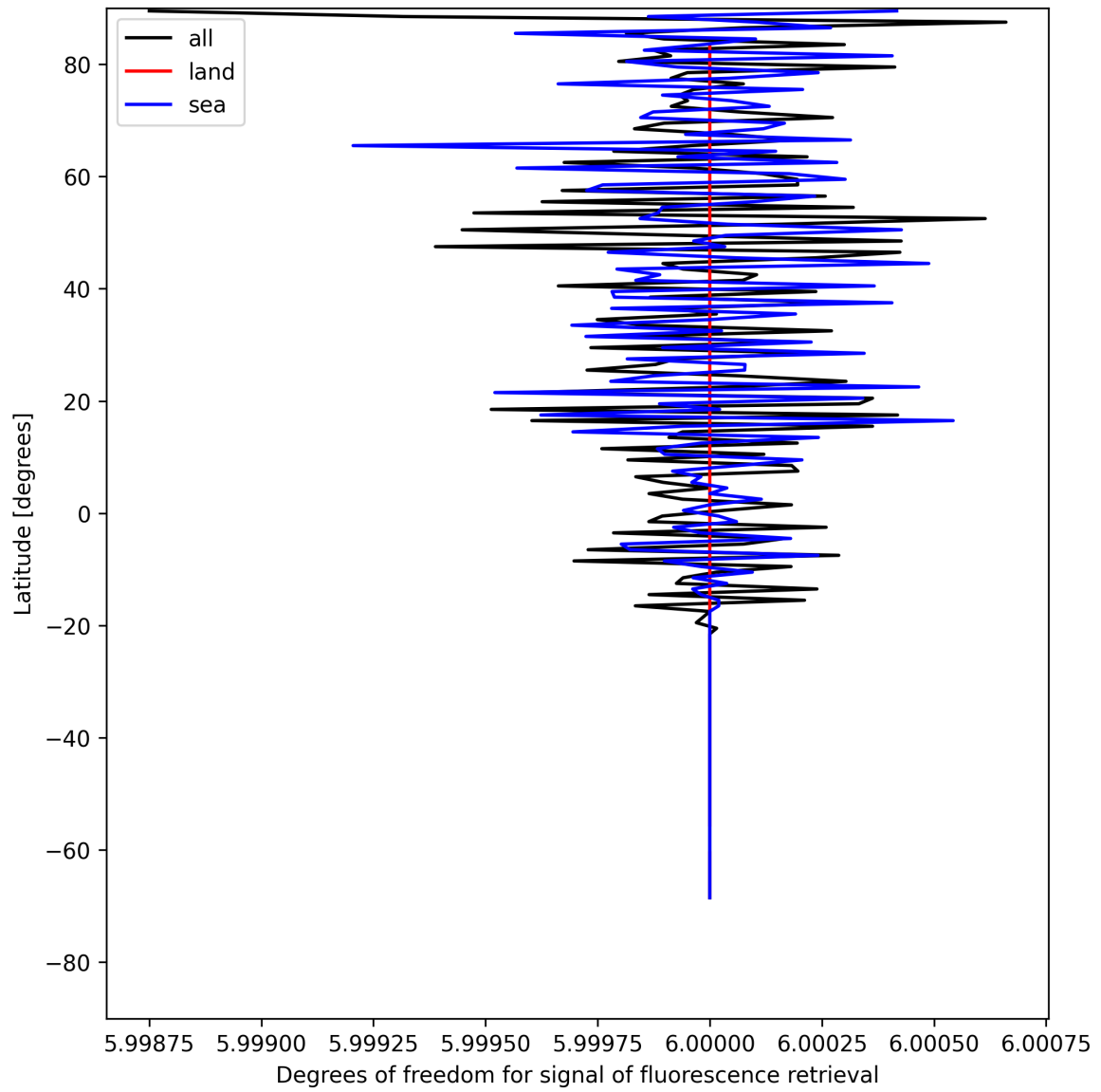
Figure 24: Zonal average of “Degrees of freedom for signal of fluorescence retrieval” for 2025-07-25 to 2025-07-26.
