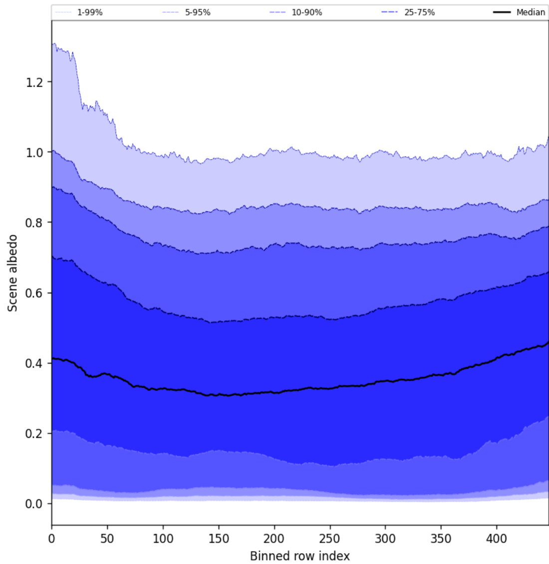
Figure 49: Along track statistics of “Scene albedo” for 2025-07-25 to 2025-07-26
