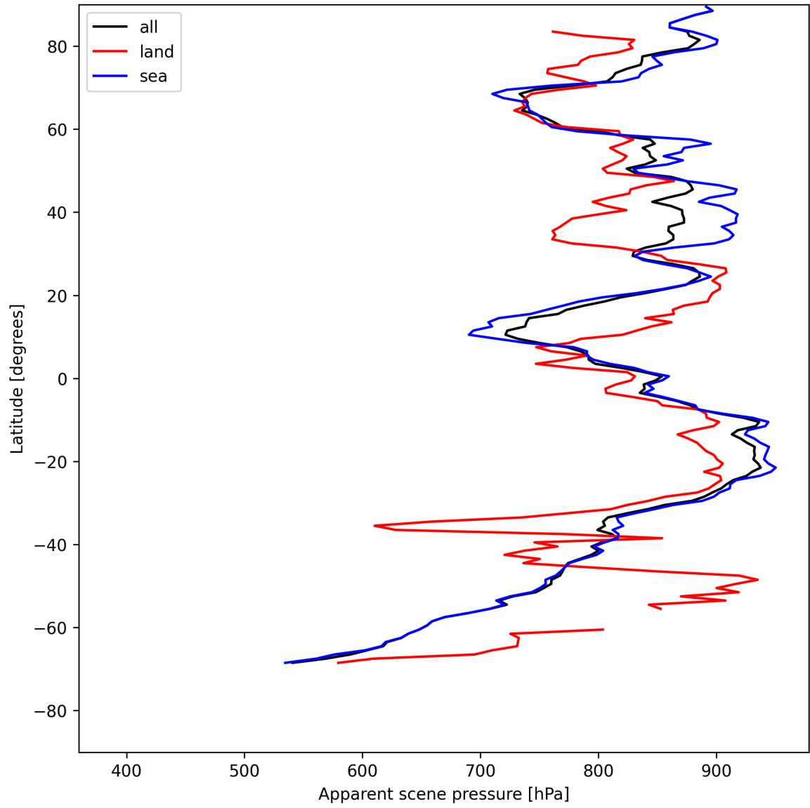
Figure 17: Zonal average of “Apparent scene pressure” for 2025-07-25 to 2025-07-26.
