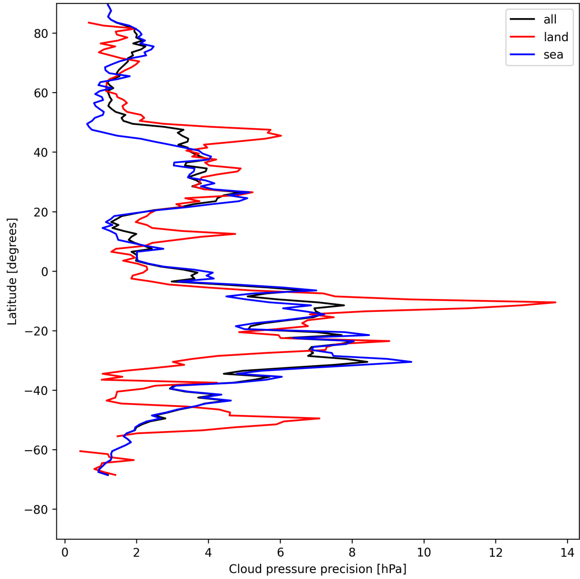
Figure 12: Zonal average of “Cloud pressure precision” for 2025-07-25 to 2025-07-26.
