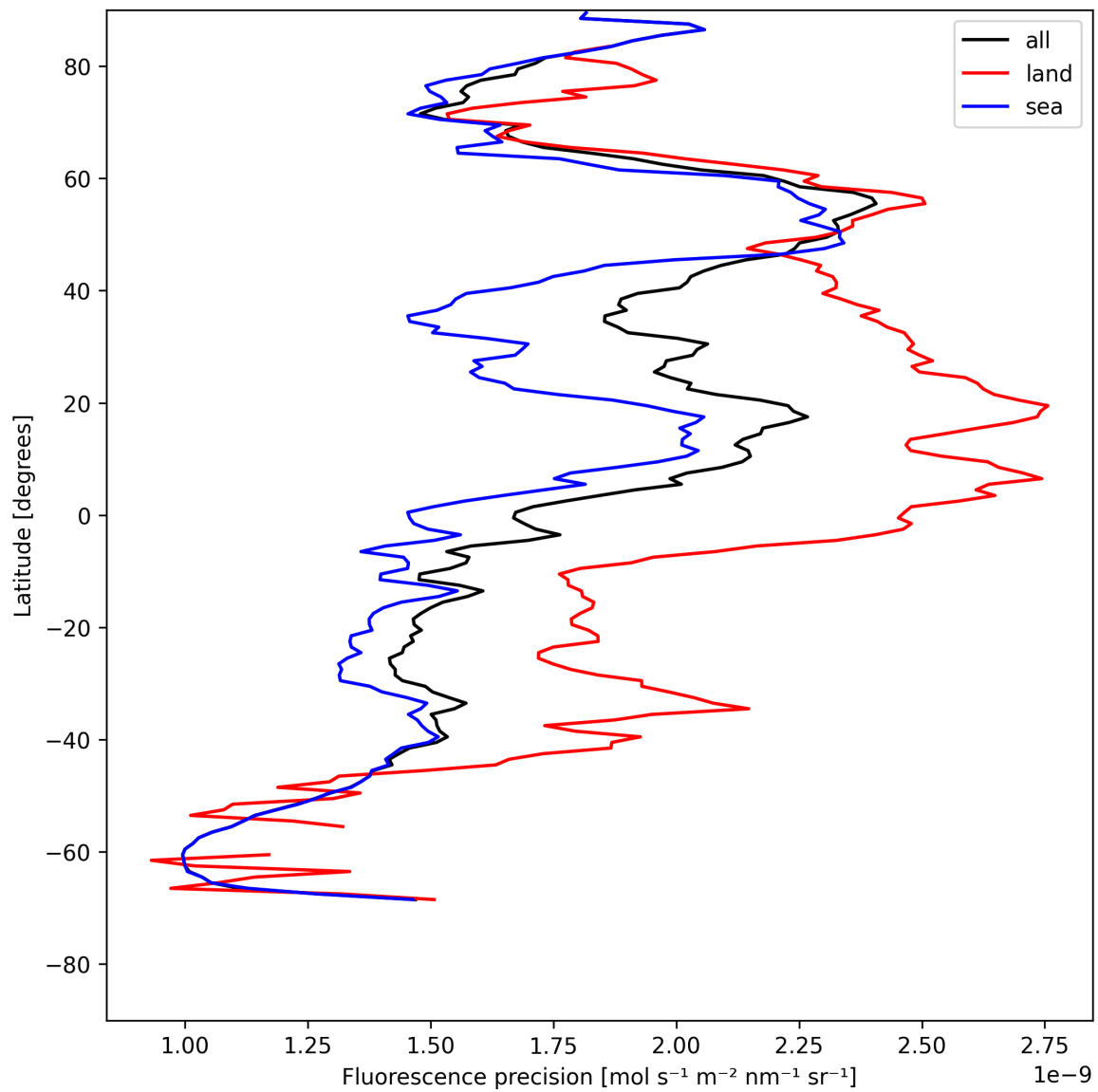
Figure 22: Zonal average of “Fluorescence precision” for 2025-07-25 to 2025-07-26.
