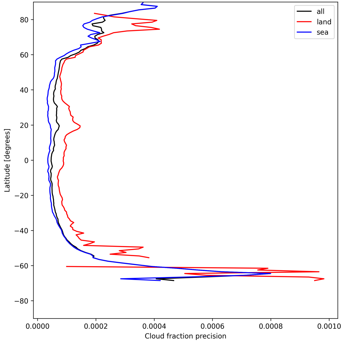
Figure 14: Zonal average of “Cloud fraction precision” for 2025-07-25 to 2025-07-26.
