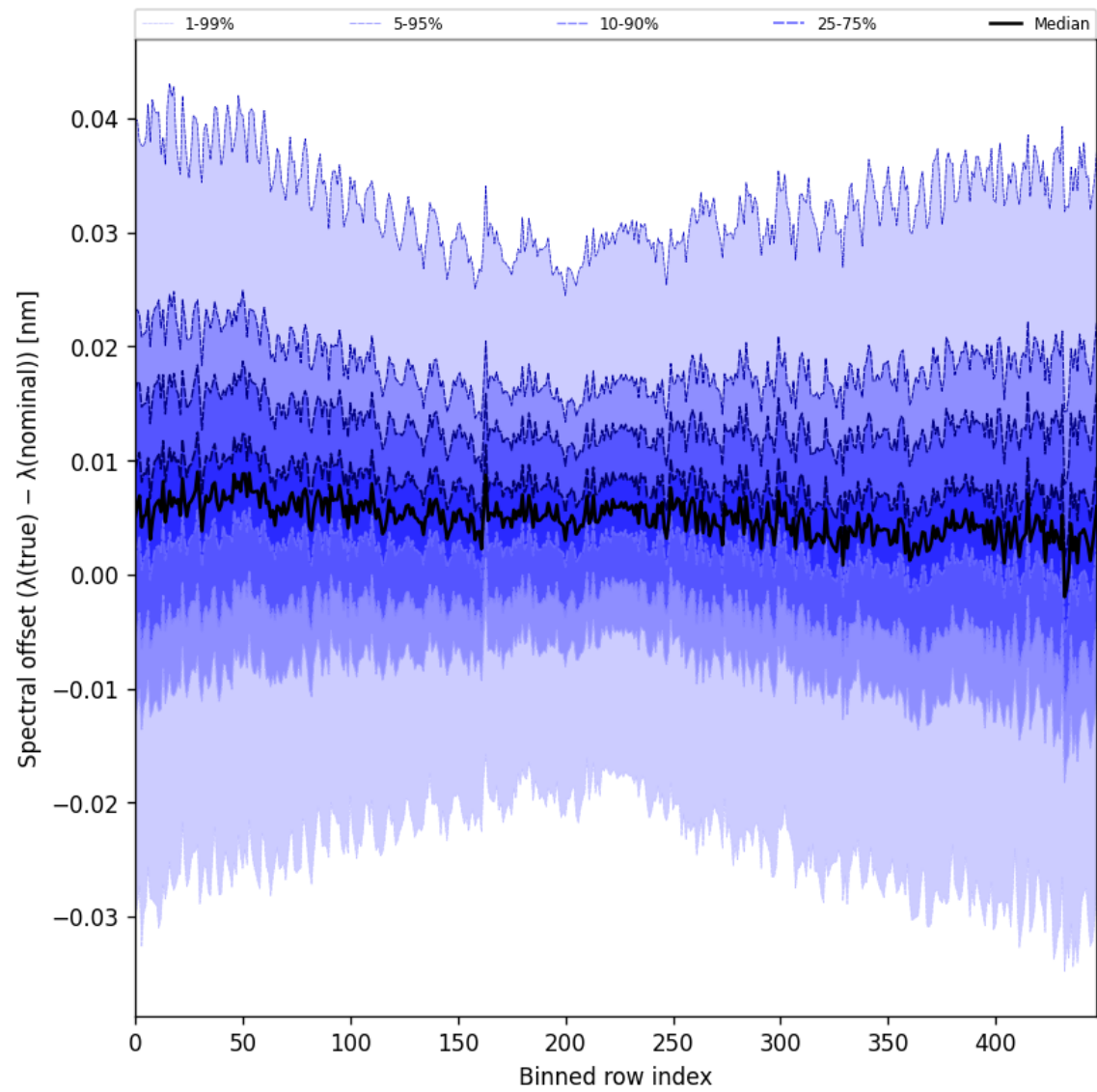
Figure 60: Along track statistics of “Spectral offset ( \lambda_{\text{true}} - \lambda_{\text{nominal}} )” for 2025-07-25 to 2025-07-26
