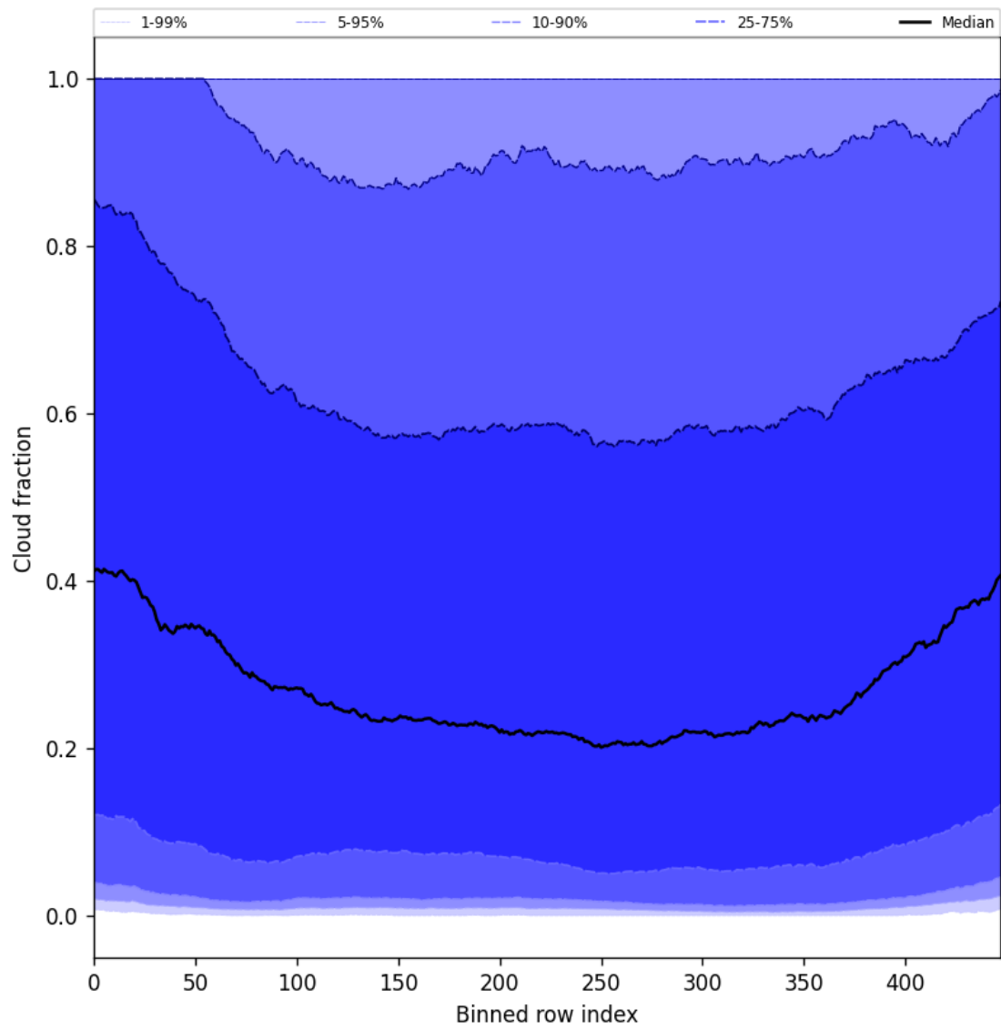
Figure 47: Along track statistics of “Cloud fraction” for 2025-07-25 to 2025-07-26
