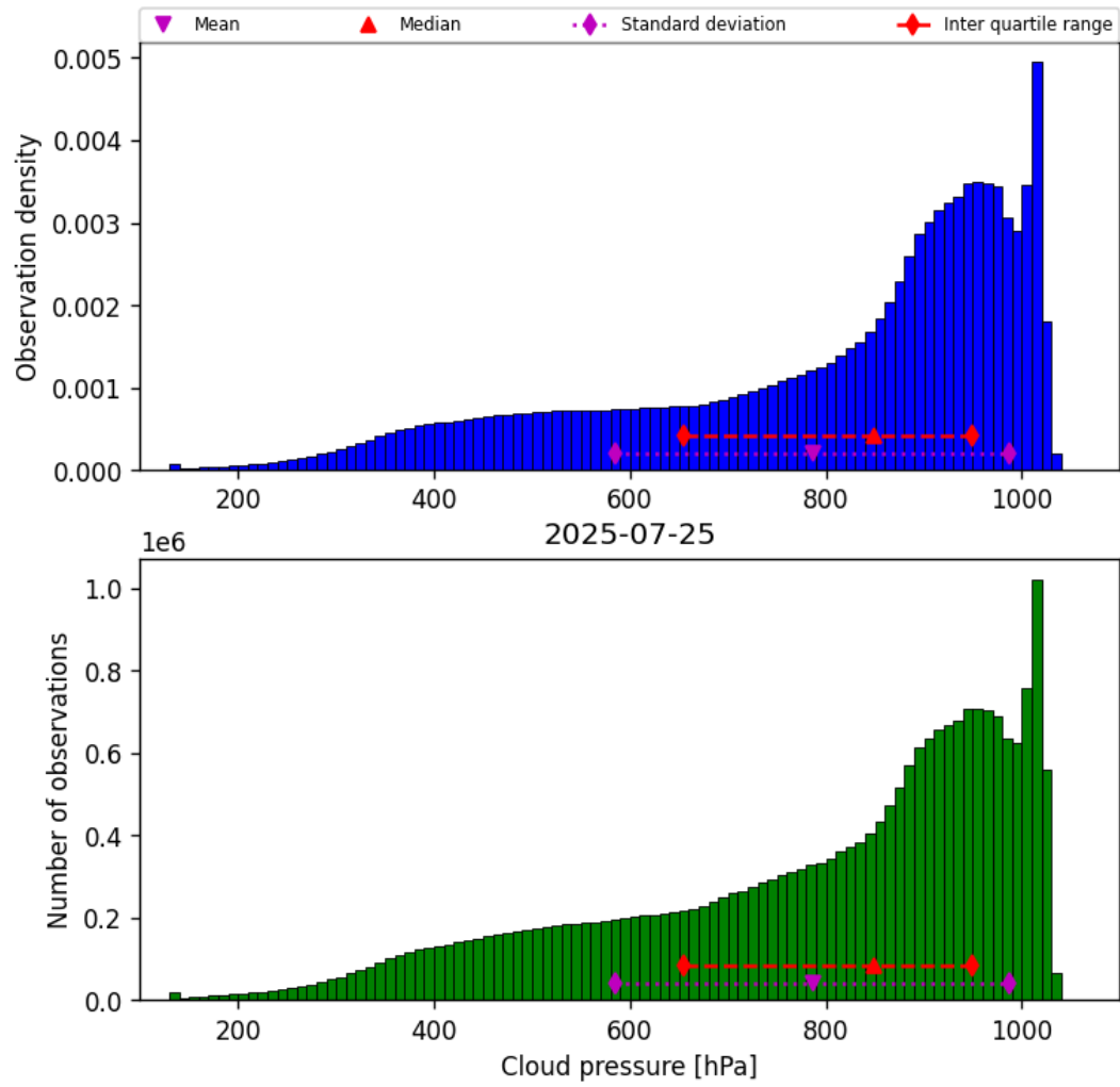
Figure 28: Histogram of “Cloud pressure” for 2025-07-25 to 2025-07-26
