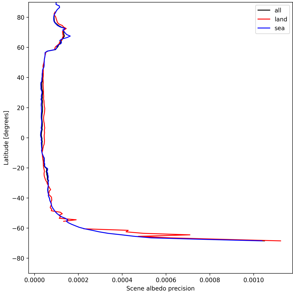
Figure 16: Zonal average of “Scene albedo precision” for 2025-07-25 to 2025-07-26.
