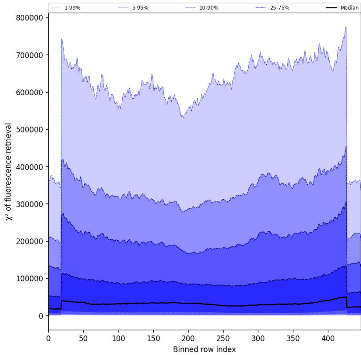
Figure 57: Along track statistics of “ \chi^2 of fluorescence retrieval” for 2025-07-25 to 2025-07-26
