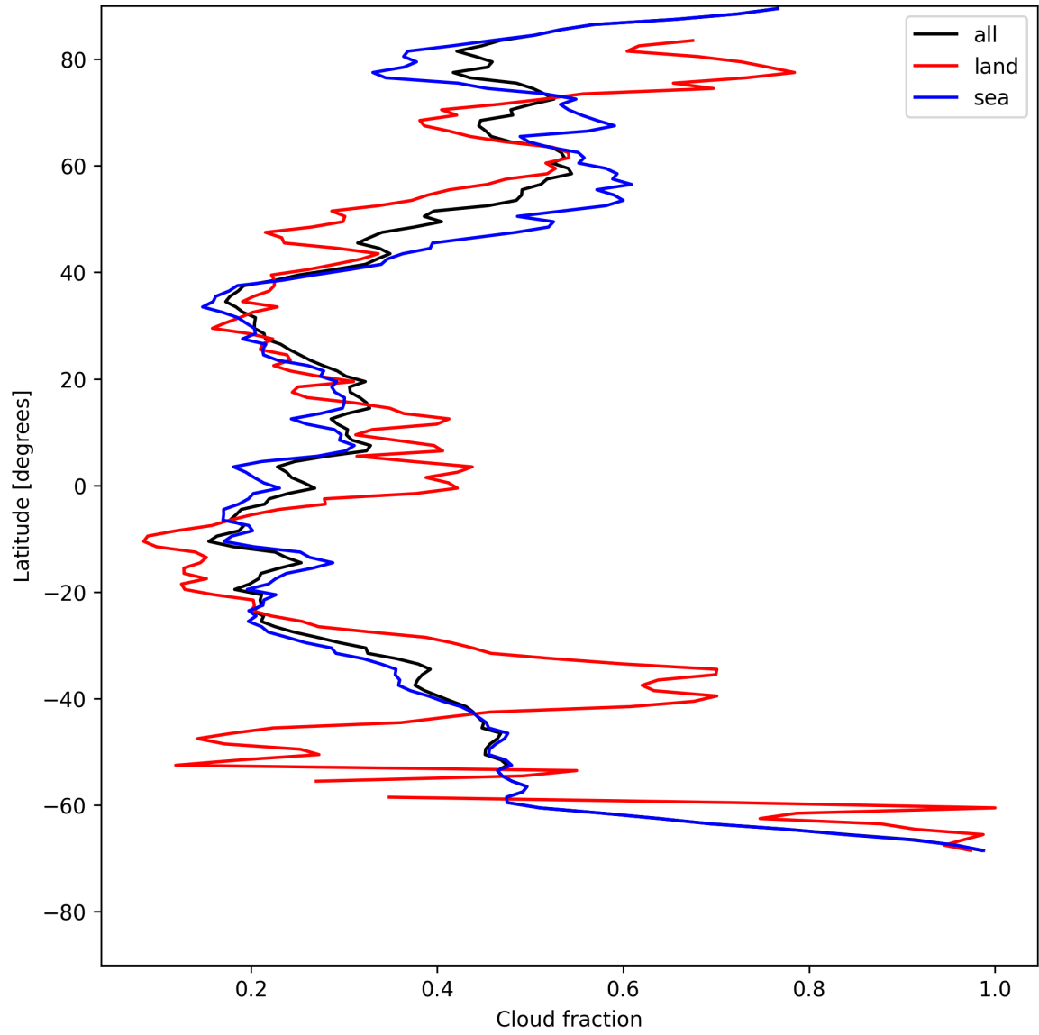
Figure 13: Zonal average of “Cloud fraction” for 2025-07-26 to 2025-07-27.
