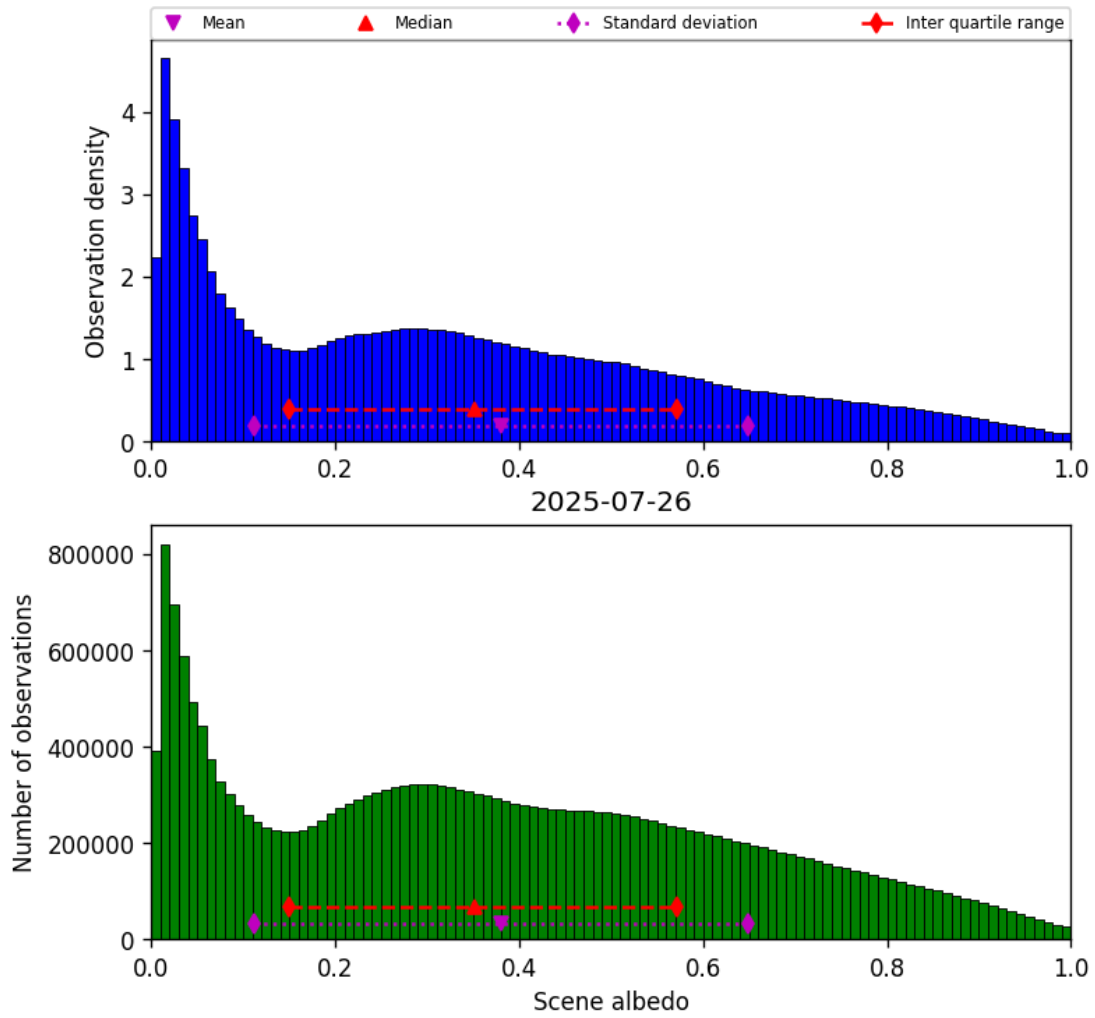
Figure 32: Histogram of “Scene albedo” for 2025-07-26 to 2025-07-27
