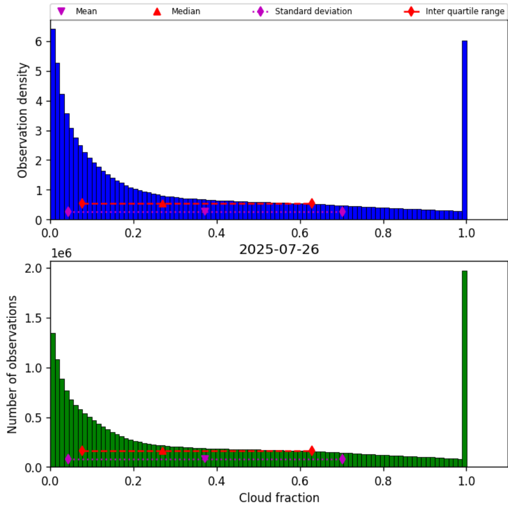
Figure 30: Histogram of “Cloud fraction” for 2025-07-26 to 2025-07-27
