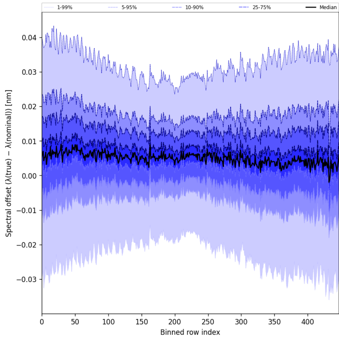
Figure 60: Along track statistics of “Spectral offset ( \lambda_{\text{true}} - \lambda_{\text{nominal}} )” for 2025-07-26 to 2025-07-27
