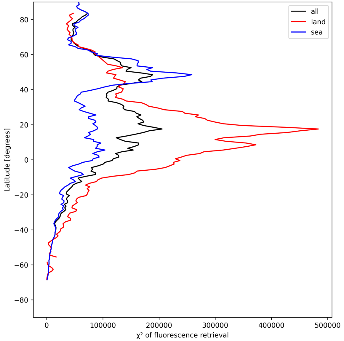
Figure 23: Zonal average of “ \chi^2 of fluorescence retrieval” for 2025-07-26 to 2025-07-27.
