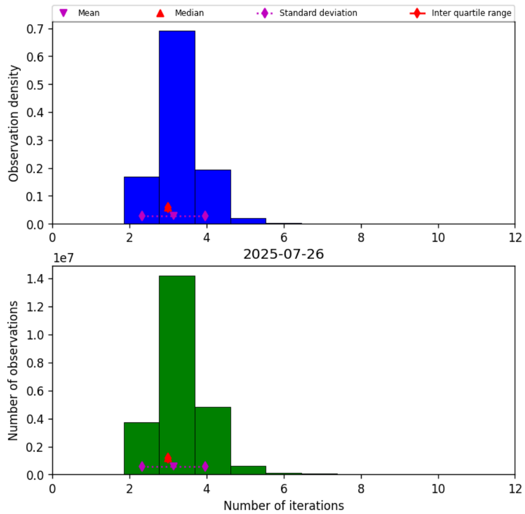
Figure 37: Histogram of “Number of iterations” for 2025-07-26 to 2025-07-27
