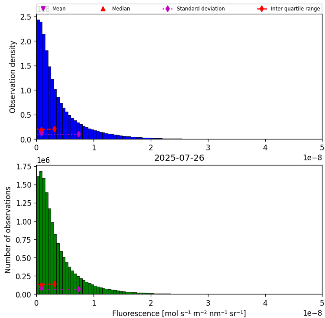
Figure 38: Histogram of “Fluorescence” for 2025-07-26 to 2025-07-27
