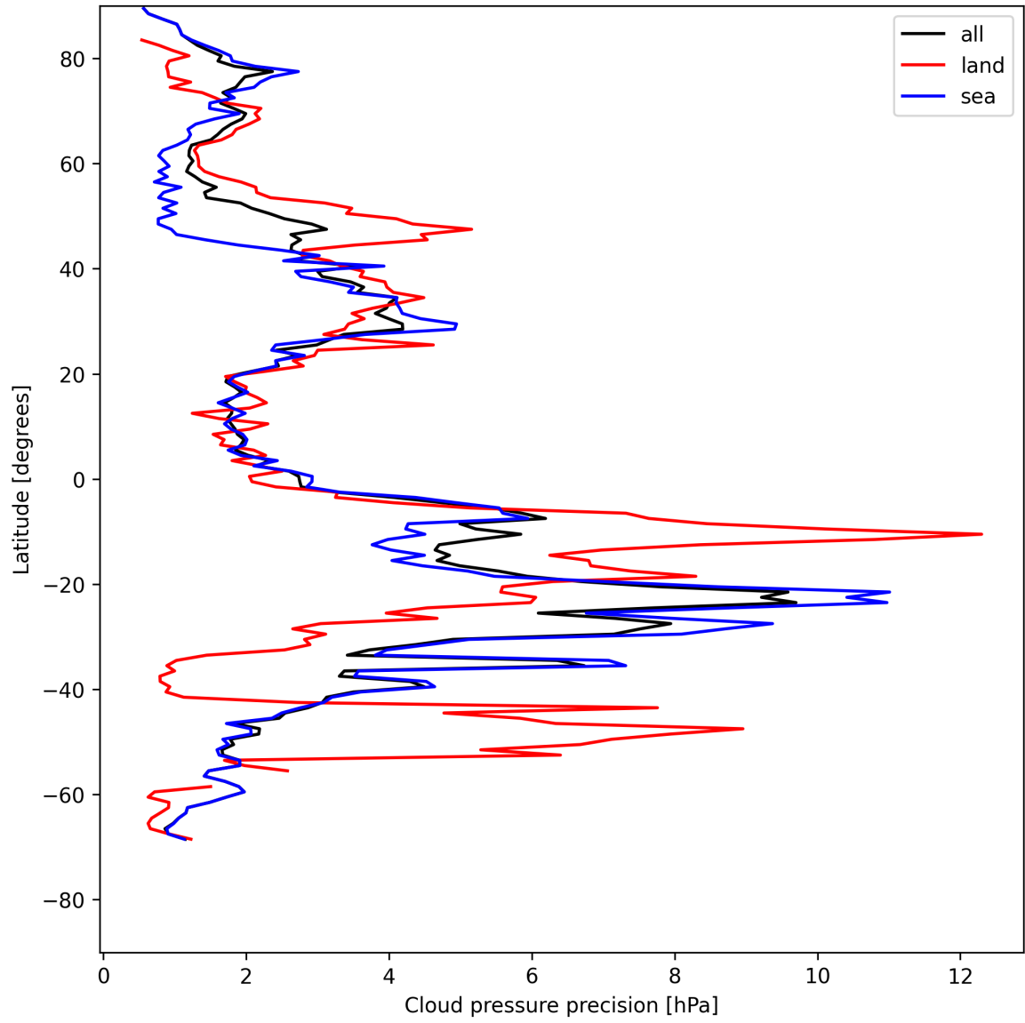
Figure 12: Zonal average of “Cloud pressure precision” for 2025-07-26 to 2025-07-27.
