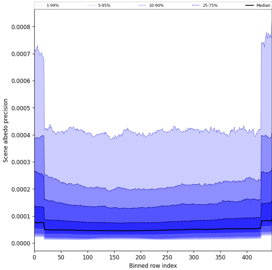
Figure 50: Along track statistics of “Scene albedo precision” for 2025-07-26 to 2025-07-27
