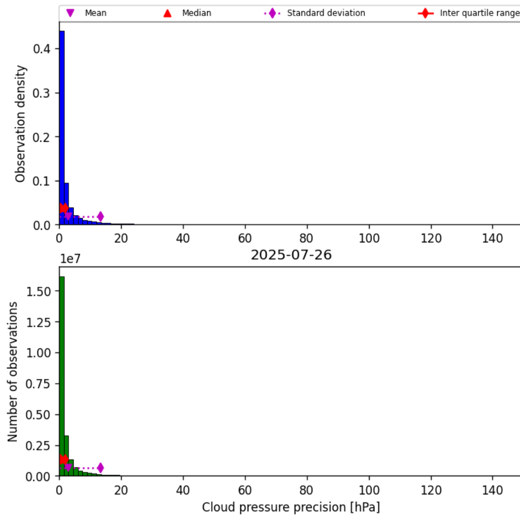
Figure 29: Histogram of “Cloud pressure precision” for 2025-07-26 to 2025-07-27
