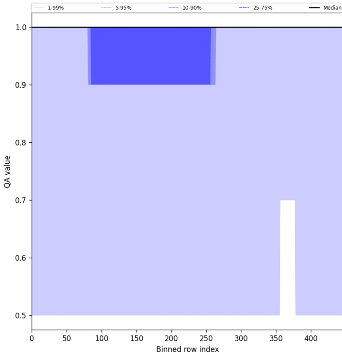
Figure 44: Along track statistics of “QA value” for 2025-07-26 to 2025-07-27
