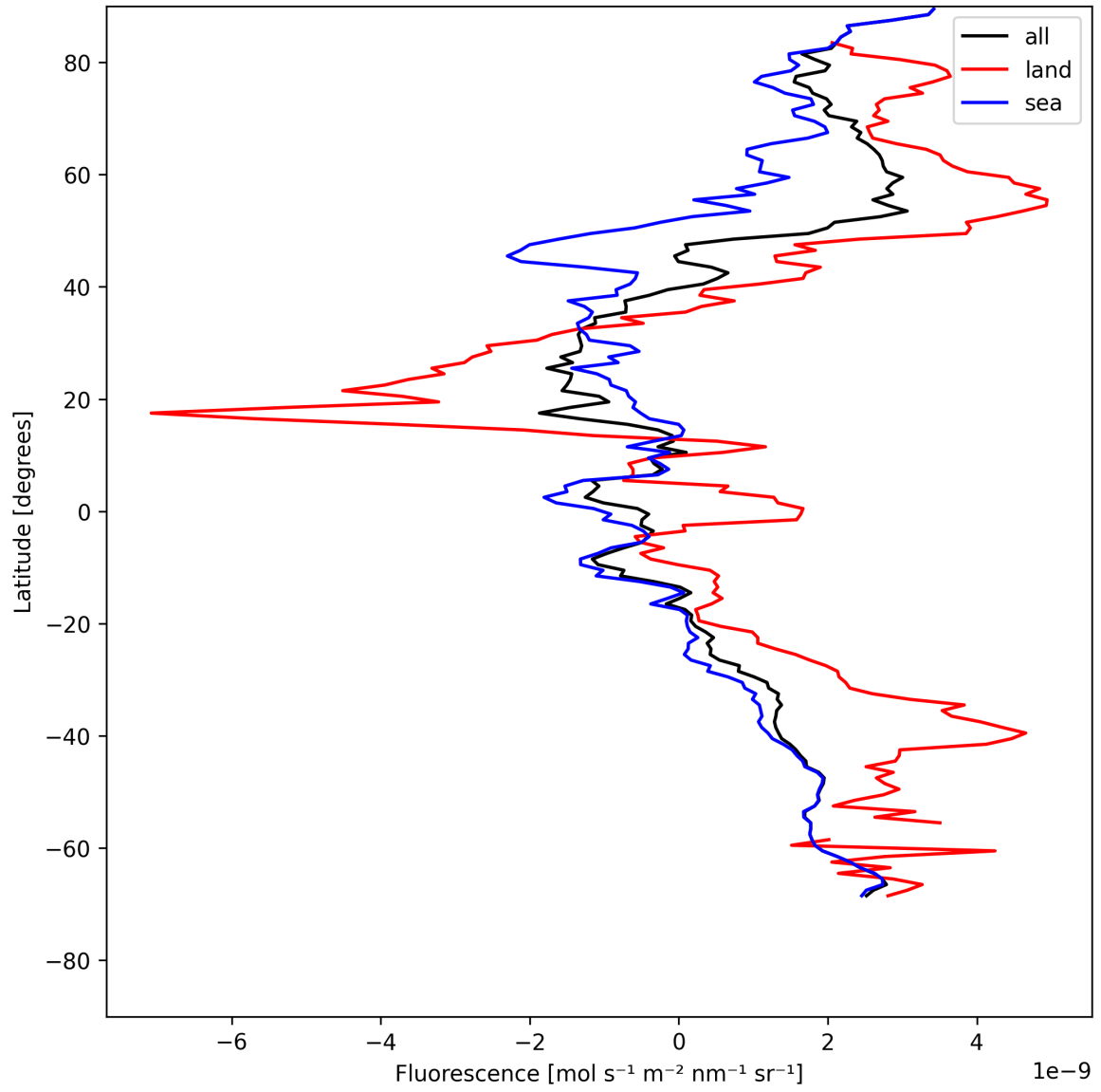
Figure 21: Zonal average of “Fluorescence” for 2025-07-26 to 2025-07-27.
