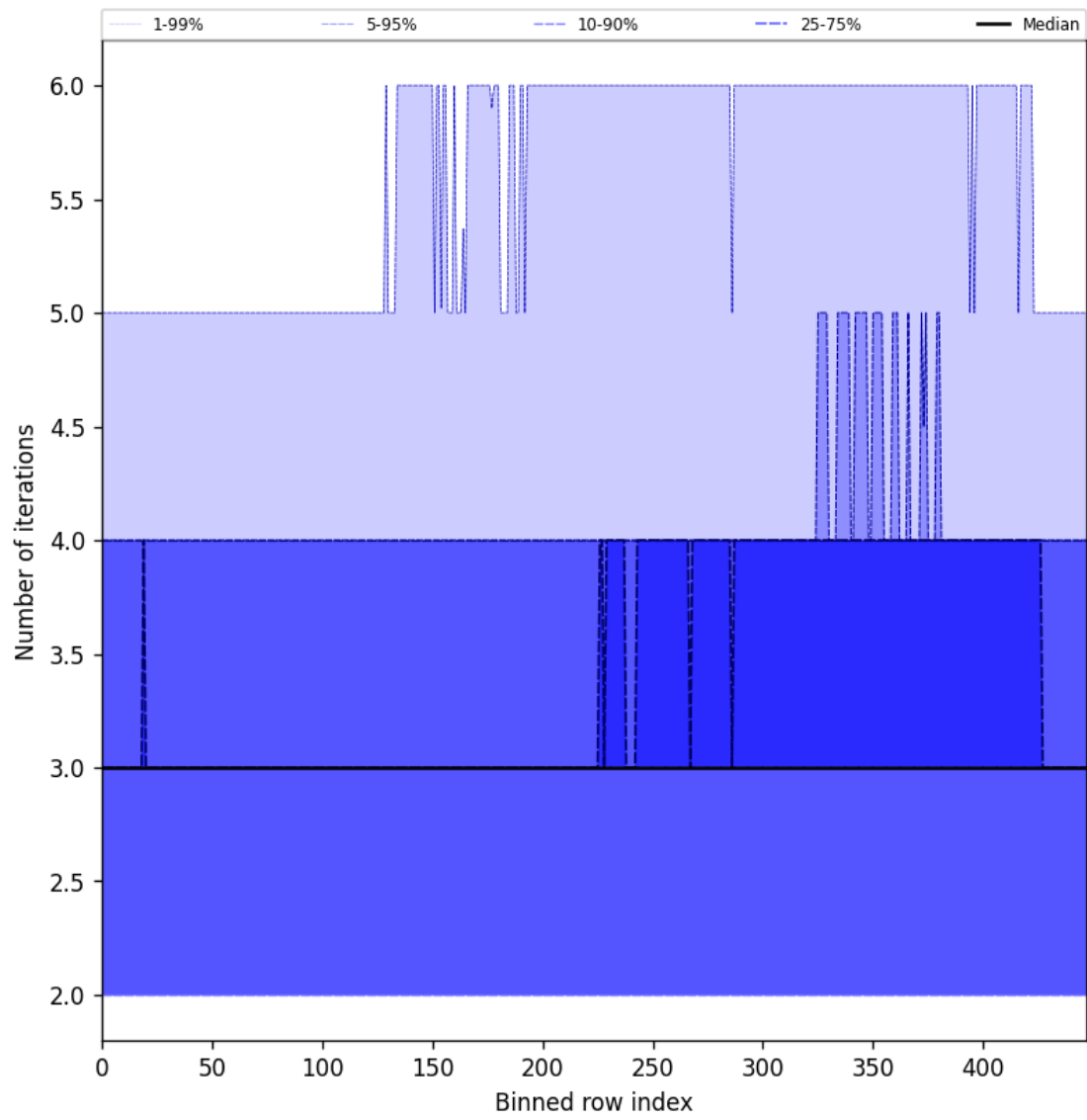
Figure 54: Along track statistics of “Number of iterations” for 2025-07-26 to 2025-07-27
