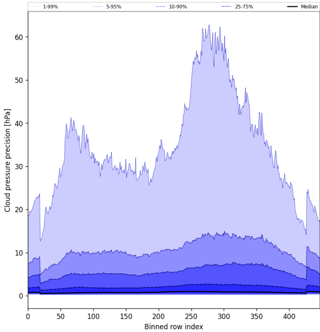
Figure 46: Along track statistics of “Cloud pressure precision” for 2025-07-26 to 2025-07-27
