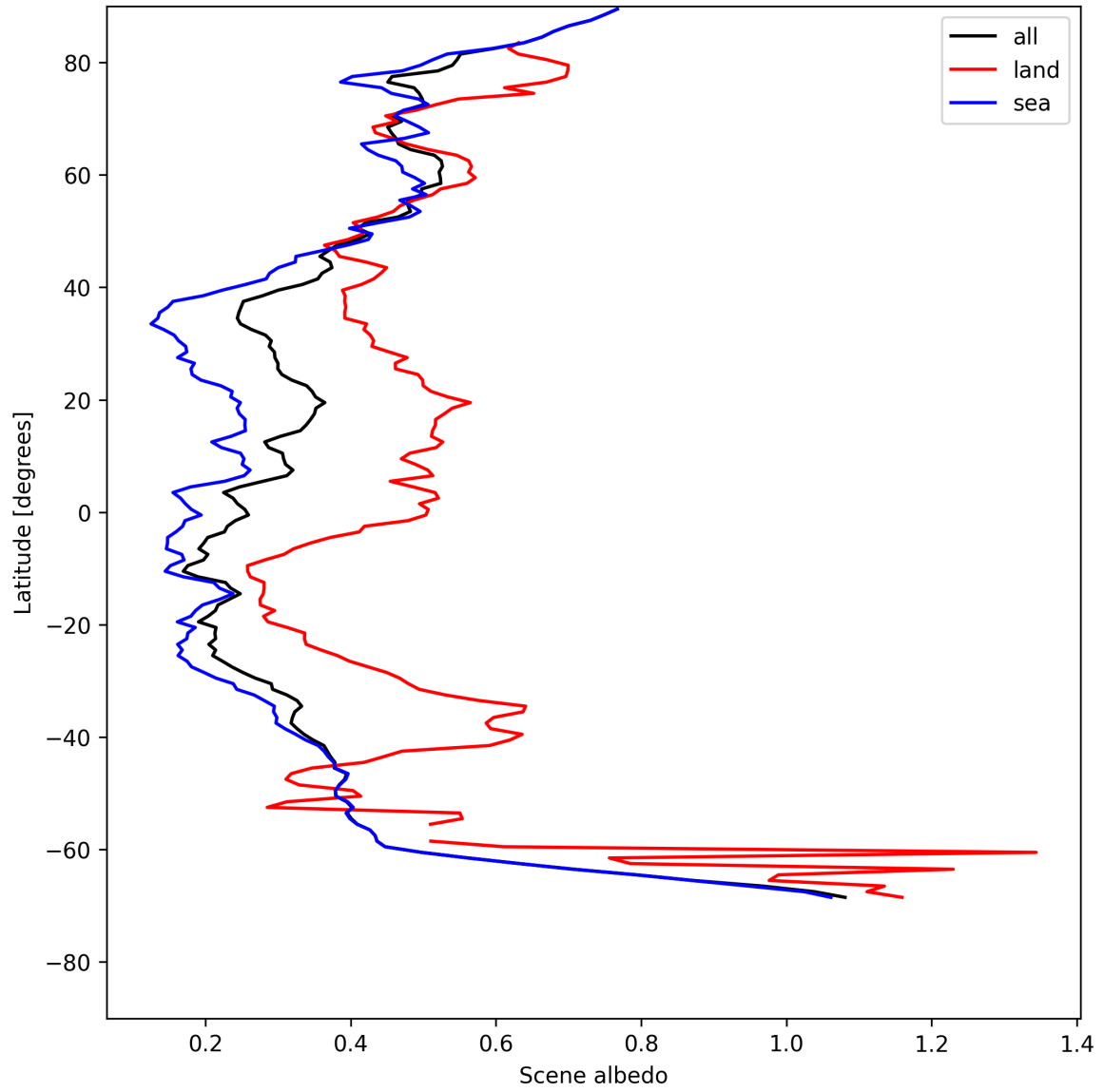
Figure 15: Zonal average of “Scene albedo” for 2025-07-26 to 2025-07-27.
