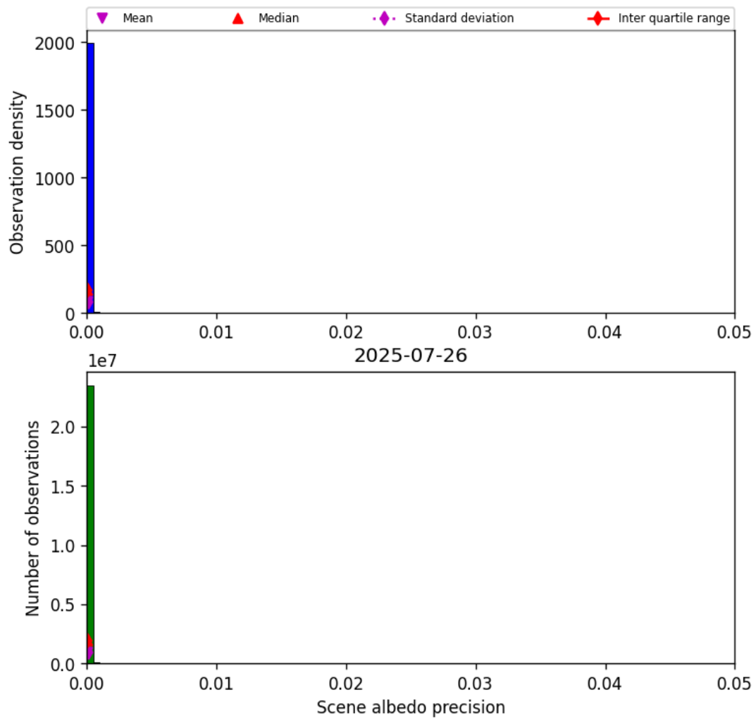
Figure 33: Histogram of “Scene albedo precision” for 2025-07-26 to 2025-07-27
