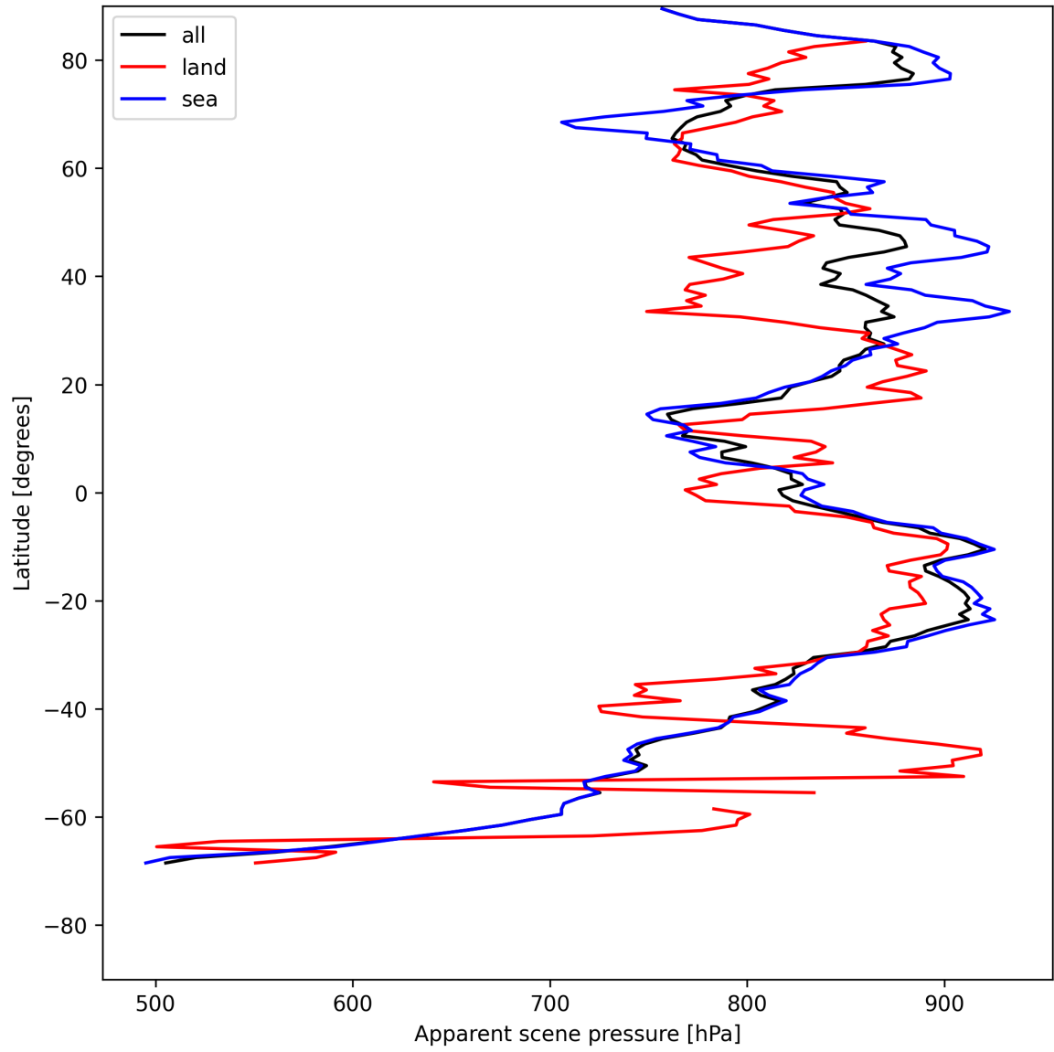
Figure 17: Zonal average of “Apparent scene pressure” for 2025-07-26 to 2025-07-27.
