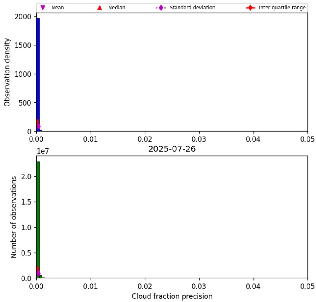
Figure 31: Histogram of “Cloud fraction precision” for 2025-07-26 to 2025-07-27
