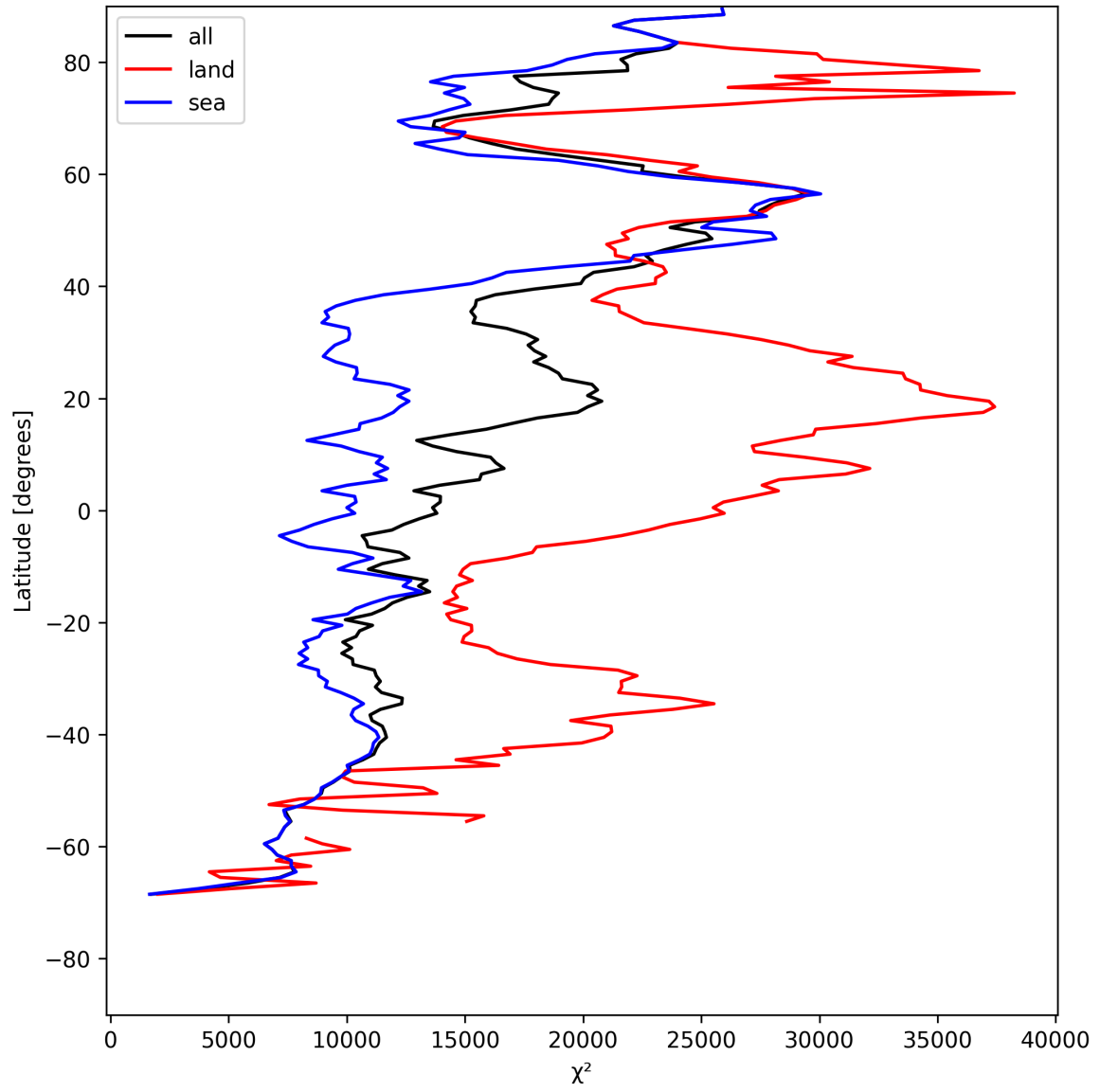
Figure 19: Zonal average of “ \chi^2 ” for 2025-07-26 to 2025-07-27.
