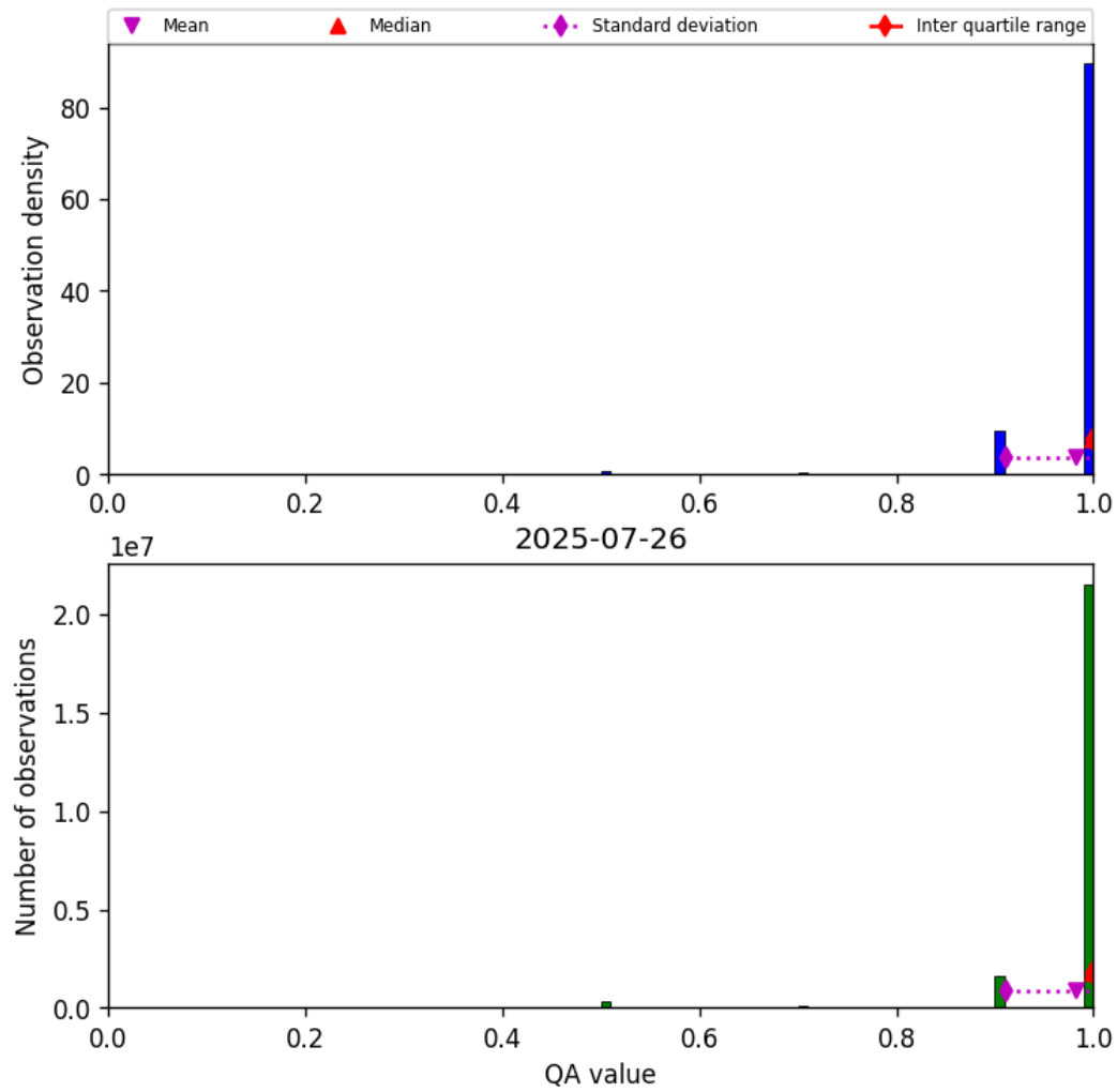
Figure 27: Histogram of “QA value” for 2025-07-26 to 2025-07-27
