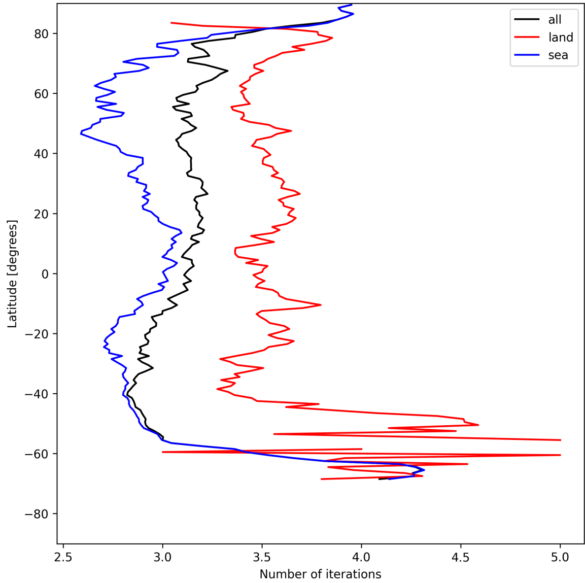
Figure 20: Zonal average of “Number of iterations” for 2025-07-26 to 2025-07-27.
