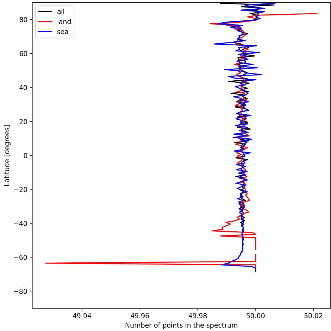
Figure 25: Zonal average of “Number of points in the spectrum” for 2025-07-26 to 2025-07-27.
