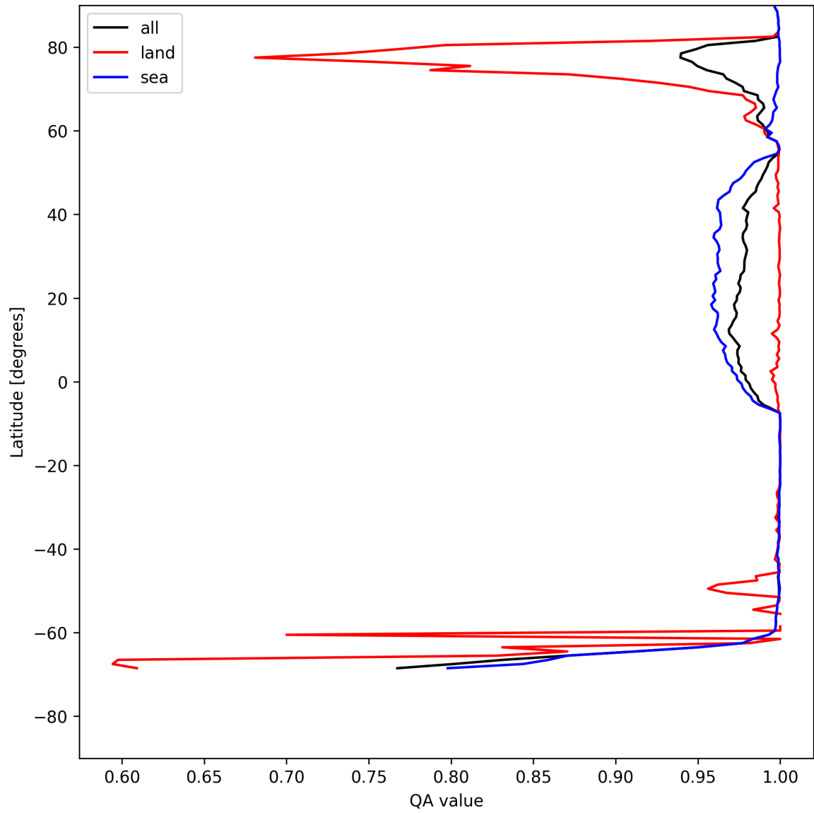
Figure 10: Zonal average of “QA value” for 2025-07-26 to 2025-07-27.
