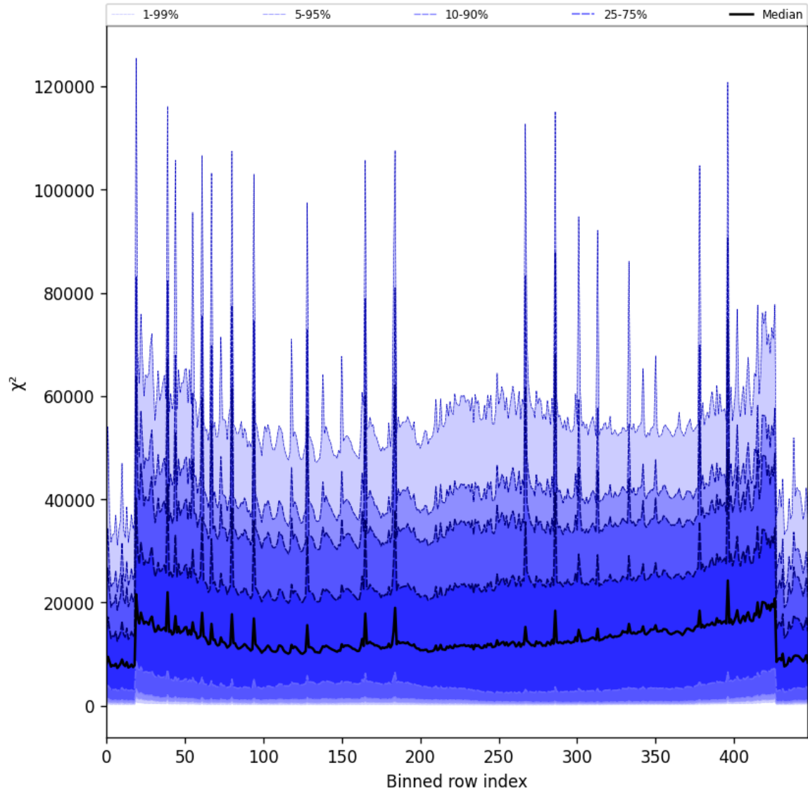
Figure 53: Along track statistics of “ \chi^2 ” for 2025-07-26 to 2025-07-27
