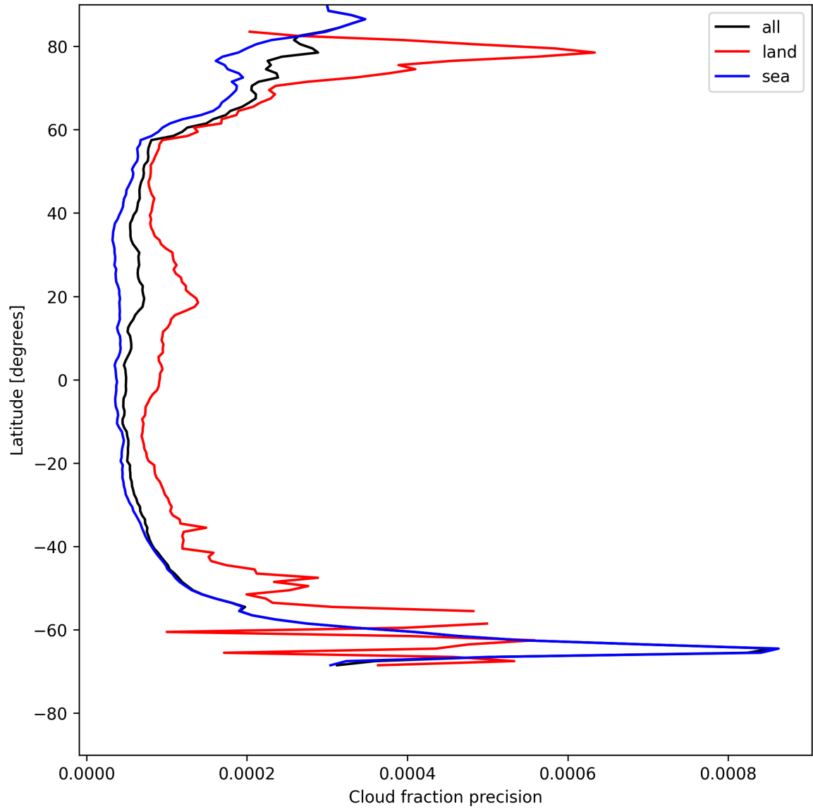
Figure 14: Zonal average of “Cloud fraction precision” for 2025-07-26 to 2025-07-27.
