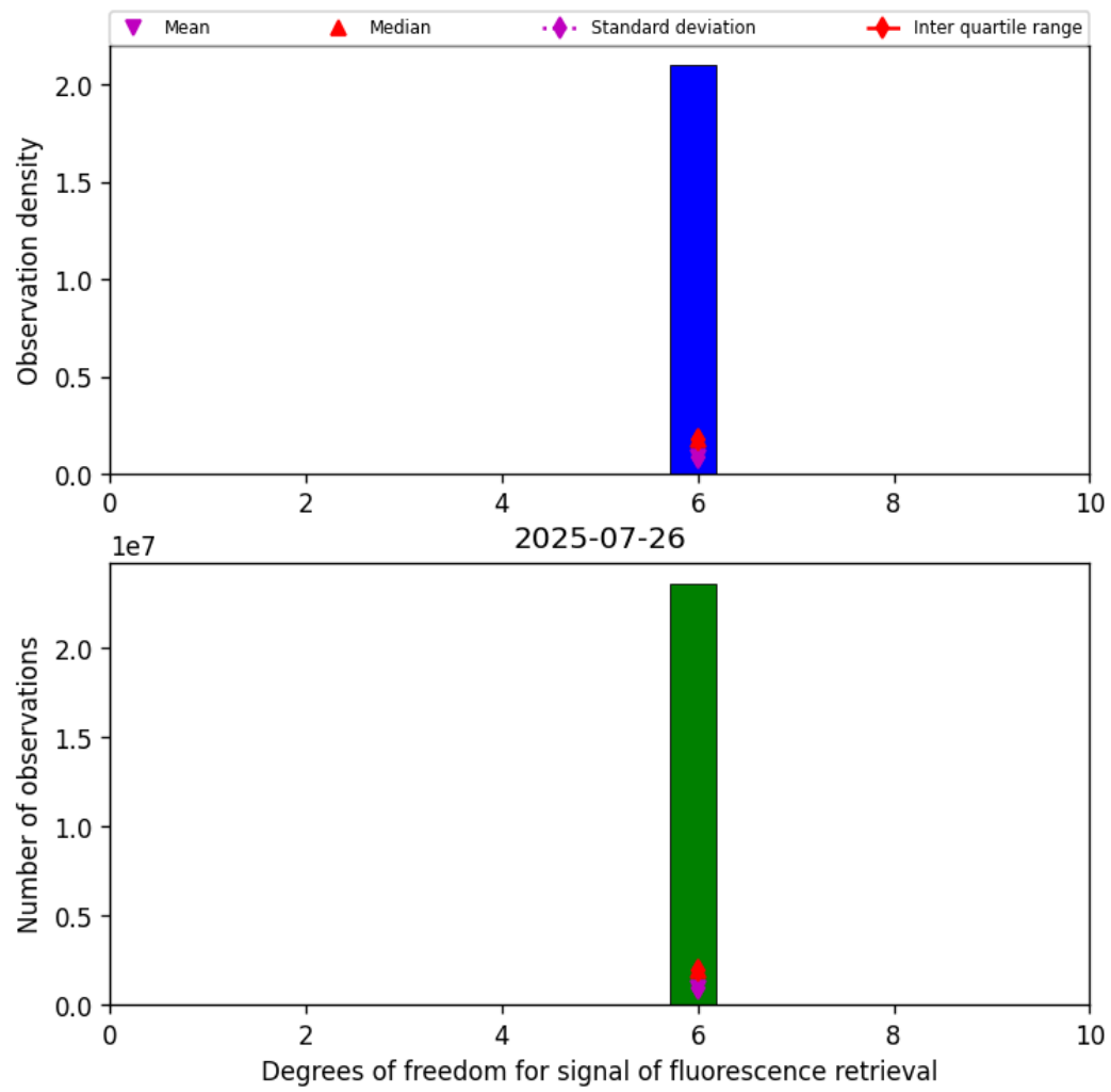
Figure 41: Histogram of “Degrees of freedom for signal of fluorescence retrieval” for 2025-07-26 to 2025-07-27
