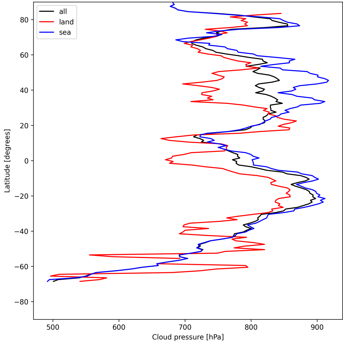
Figure 11: Zonal average of “Cloud pressure” for 2025-07-26 to 2025-07-27.
