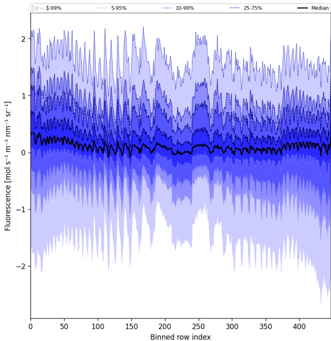
Figure 55: Along track statistics of “Fluorescence” for 2025-07-26 to 2025-07-27
