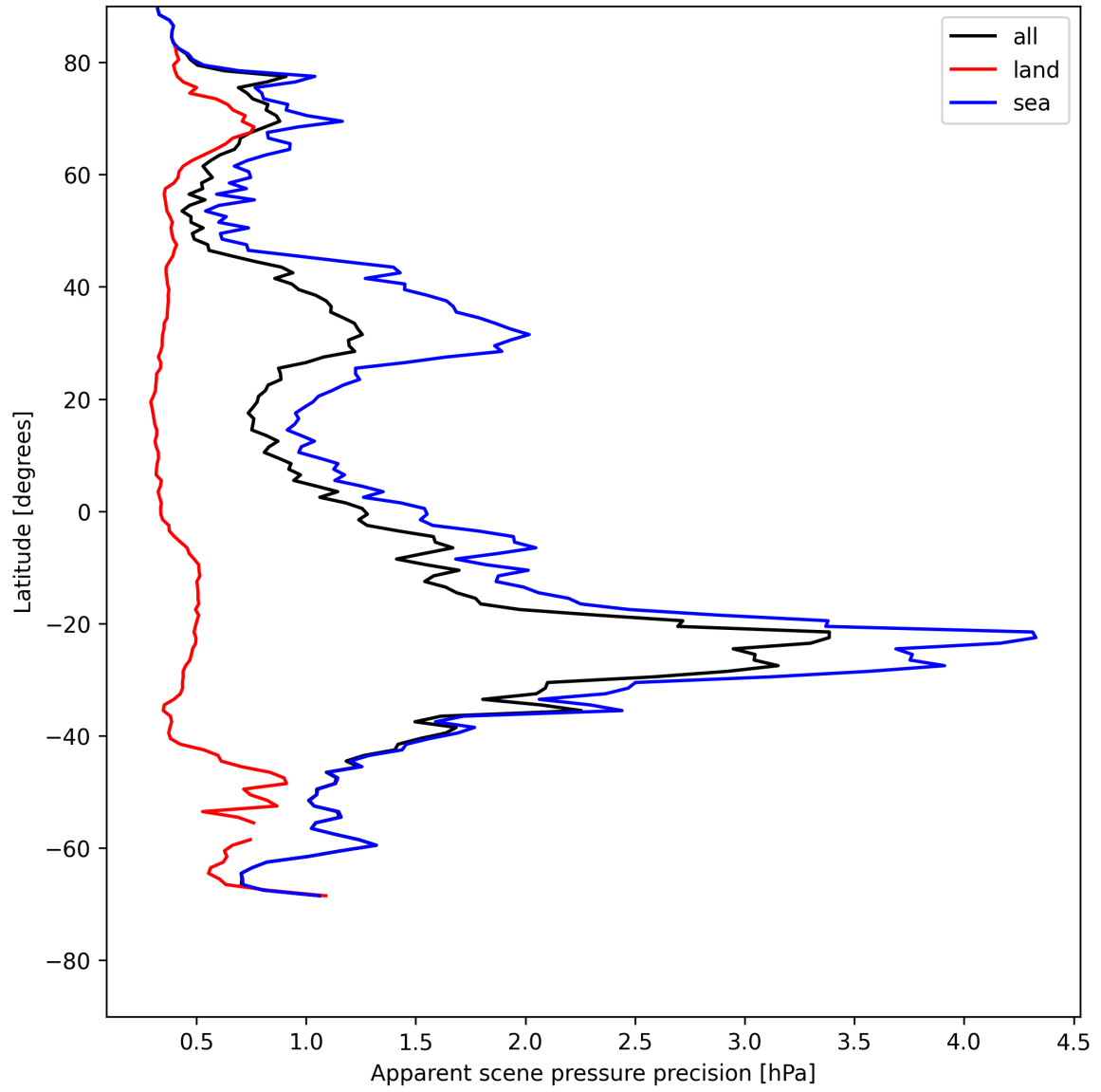
Figure 18: Zonal average of “Apparent scene pressure precision” for 2025-07-26 to 2025-07-27.
