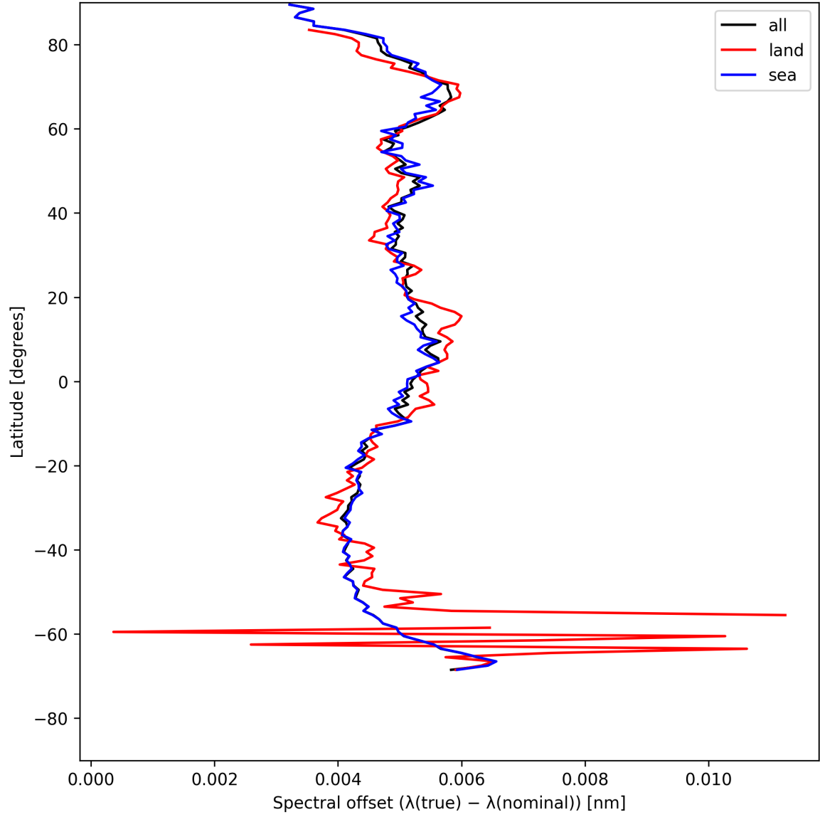
Figure 26: Zonal average of “Spectral offset ( \lambda_{\text{true}} - \lambda_{\text{nominal}} )” for 2025-07-26 to 2025-07-27.
