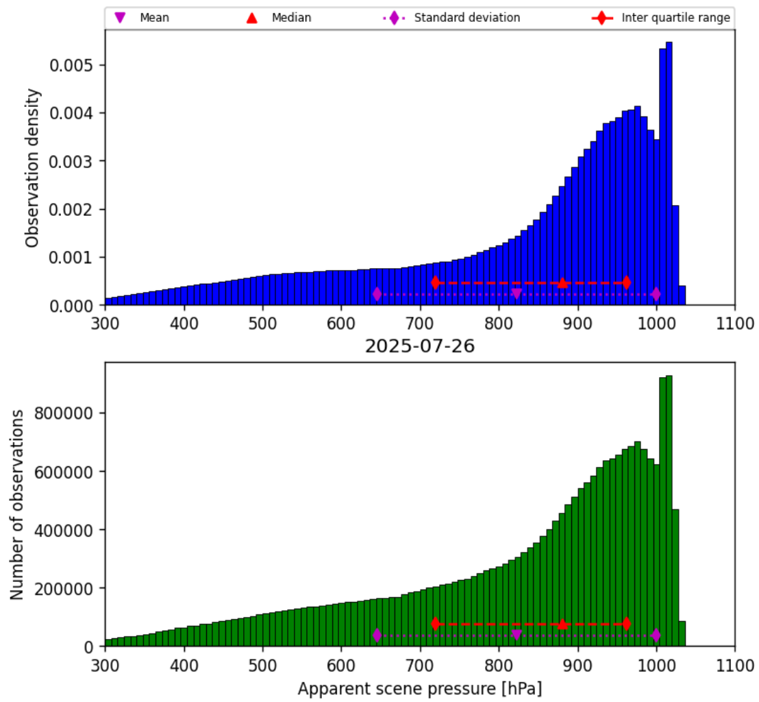
Figure 34: Histogram of “Apparent scene pressure” for 2025-07-26 to 2025-07-27
