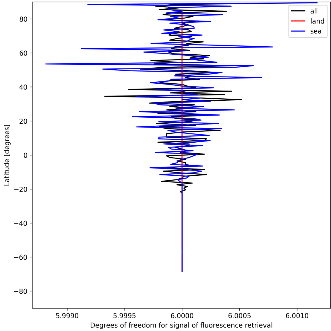
Figure 24: Zonal average of “Degrees of freedom for signal of fluorescence retrieval” for 2025-07-26 to 2025-07-27.
