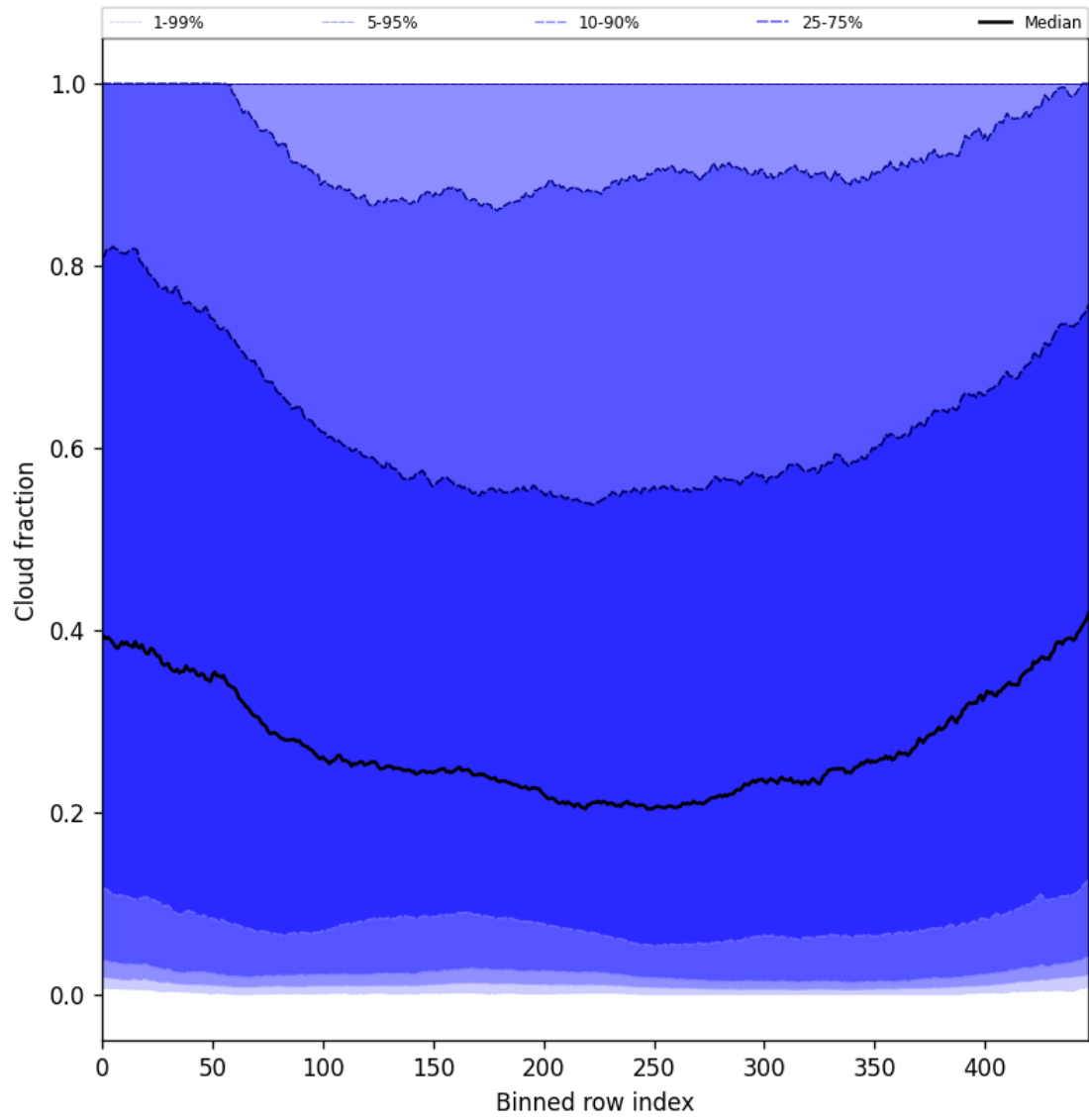
Figure 47: Along track statistics of “Cloud fraction” for 2025-07-26 to 2025-07-27
