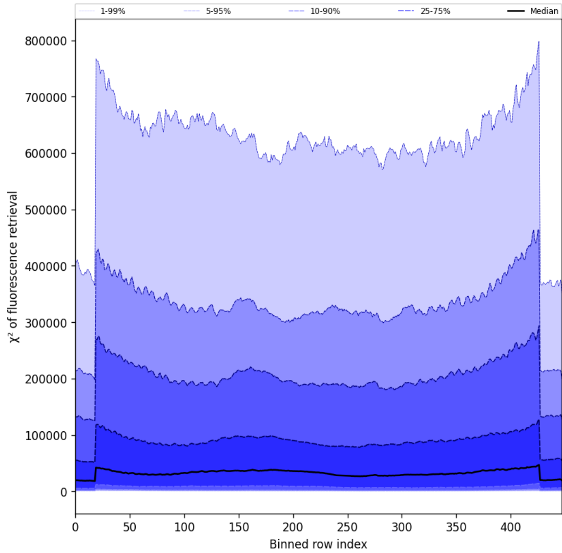
Figure 57: Along track statistics of “ \chi^2 of fluorescence retrieval” for 2025-07-26 to 2025-07-27
