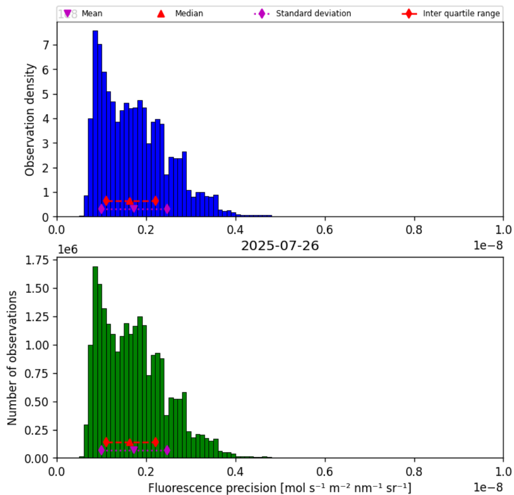
Figure 39: Histogram of “Fluorescence precision” for 2025-07-26 to 2025-07-27
