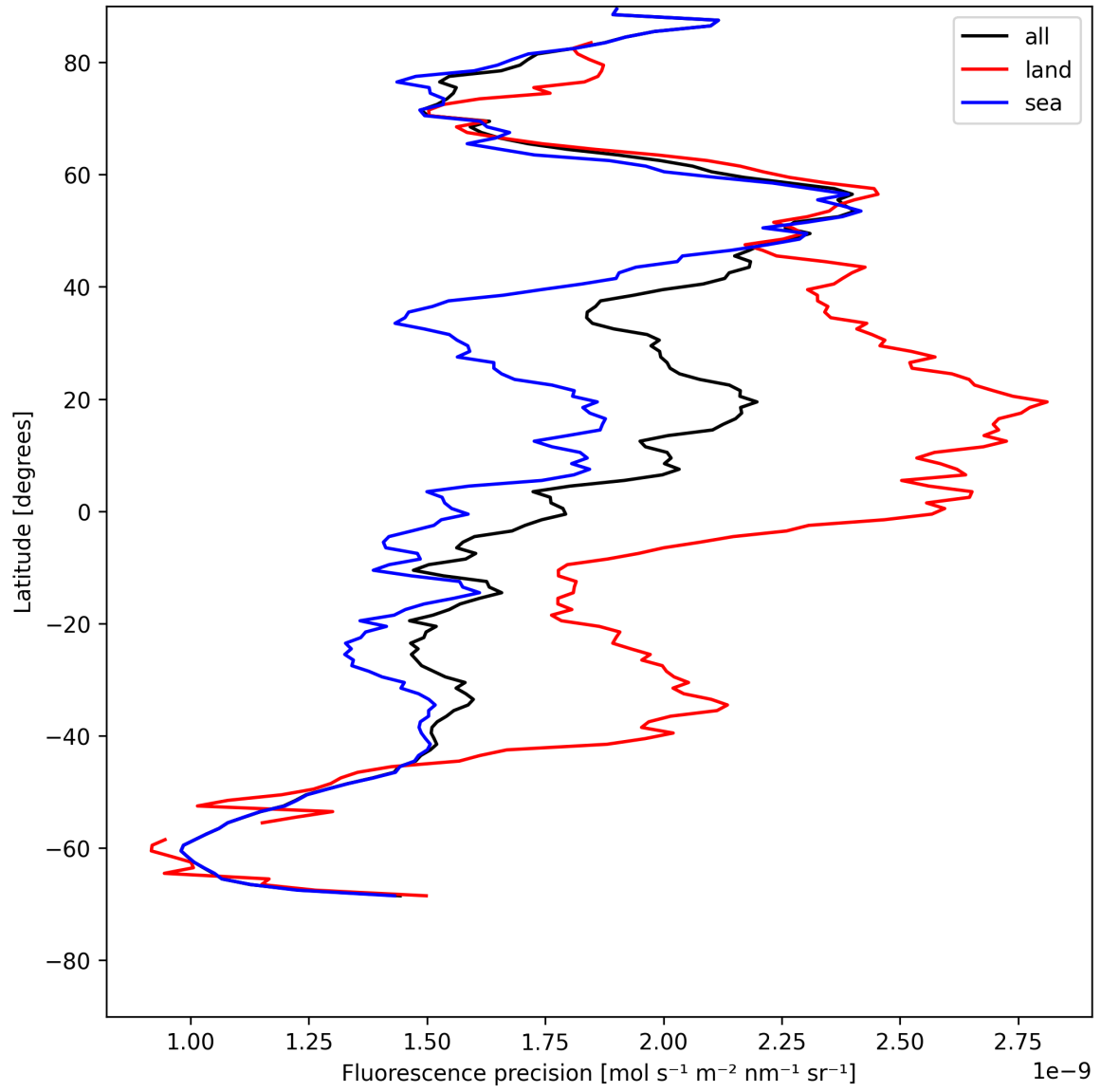
Figure 22: Zonal average of “Fluorescence precision” for 2025-07-26 to 2025-07-27.
