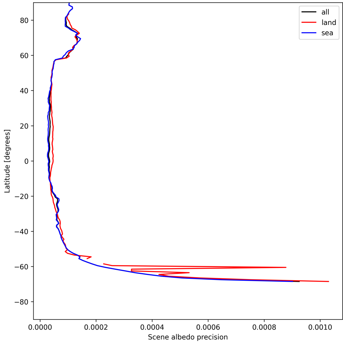
Figure 16: Zonal average of “Scene albedo precision” for 2025-07-26 to 2025-07-27.
