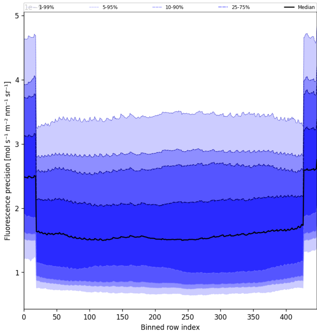
Figure 56: Along track statistics of “Fluorescence precision” for 2025-07-26 to 2025-07-27
