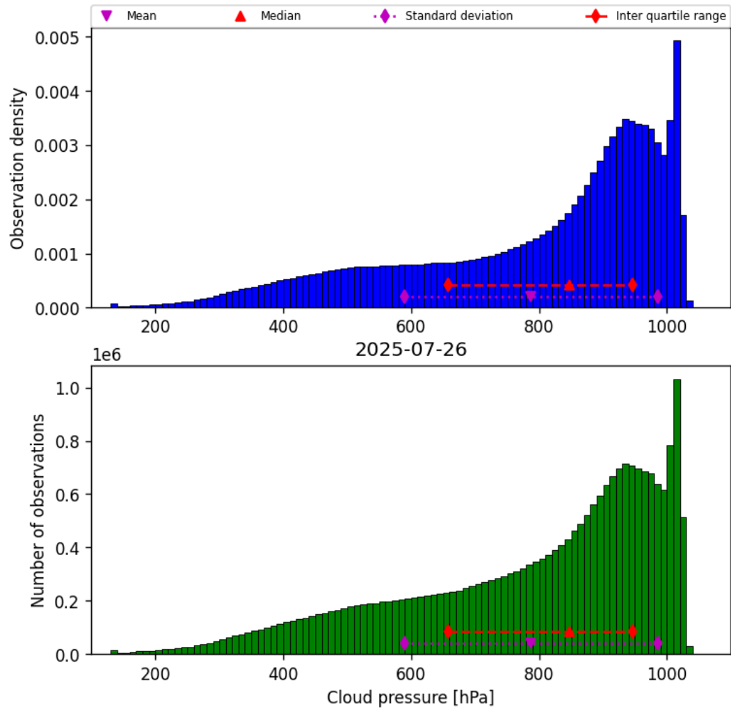
Figure 28: Histogram of “Cloud pressure” for 2025-07-26 to 2025-07-27
