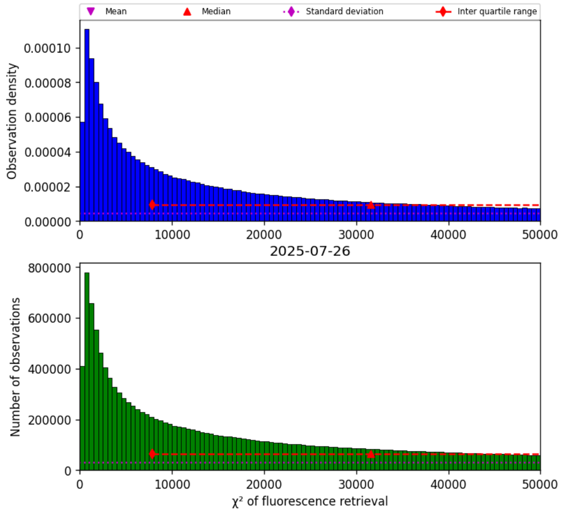
Figure 40: Histogram of “ \chi^2 of fluorescence retrieval” for 2025-07-26 to 2025-07-27
