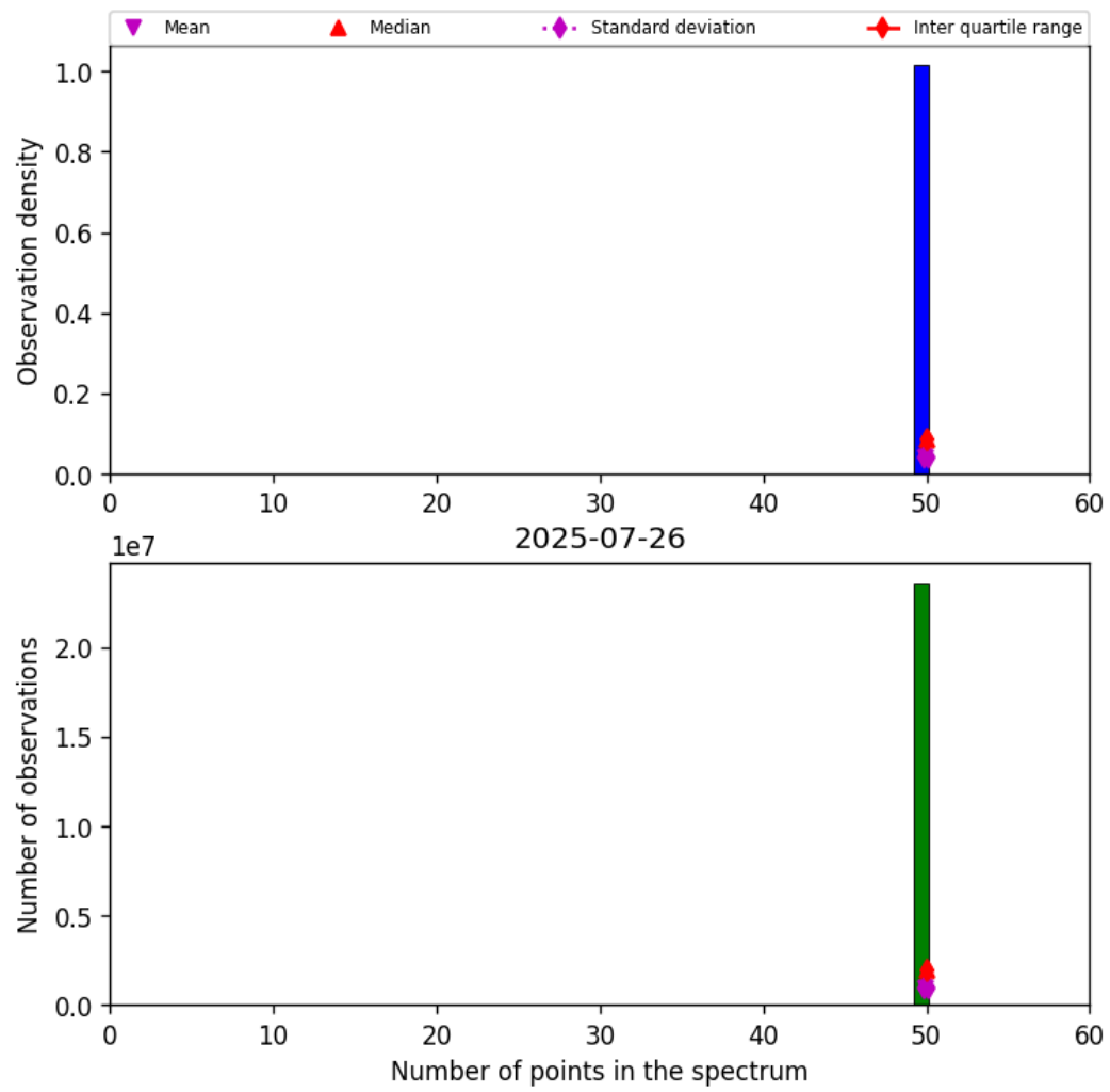
Figure 42: Histogram of “Number of points in the spectrum” for 2025-07-26 to 2025-07-27
