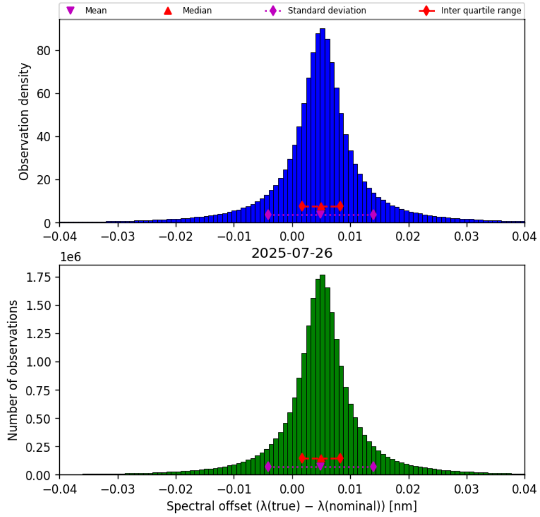
Figure 43: Histogram of “Spectral offset ( \lambda_{\text{true}} - \lambda_{\text{nominal}} )” for 2025-07-26 to 2025-07-27
