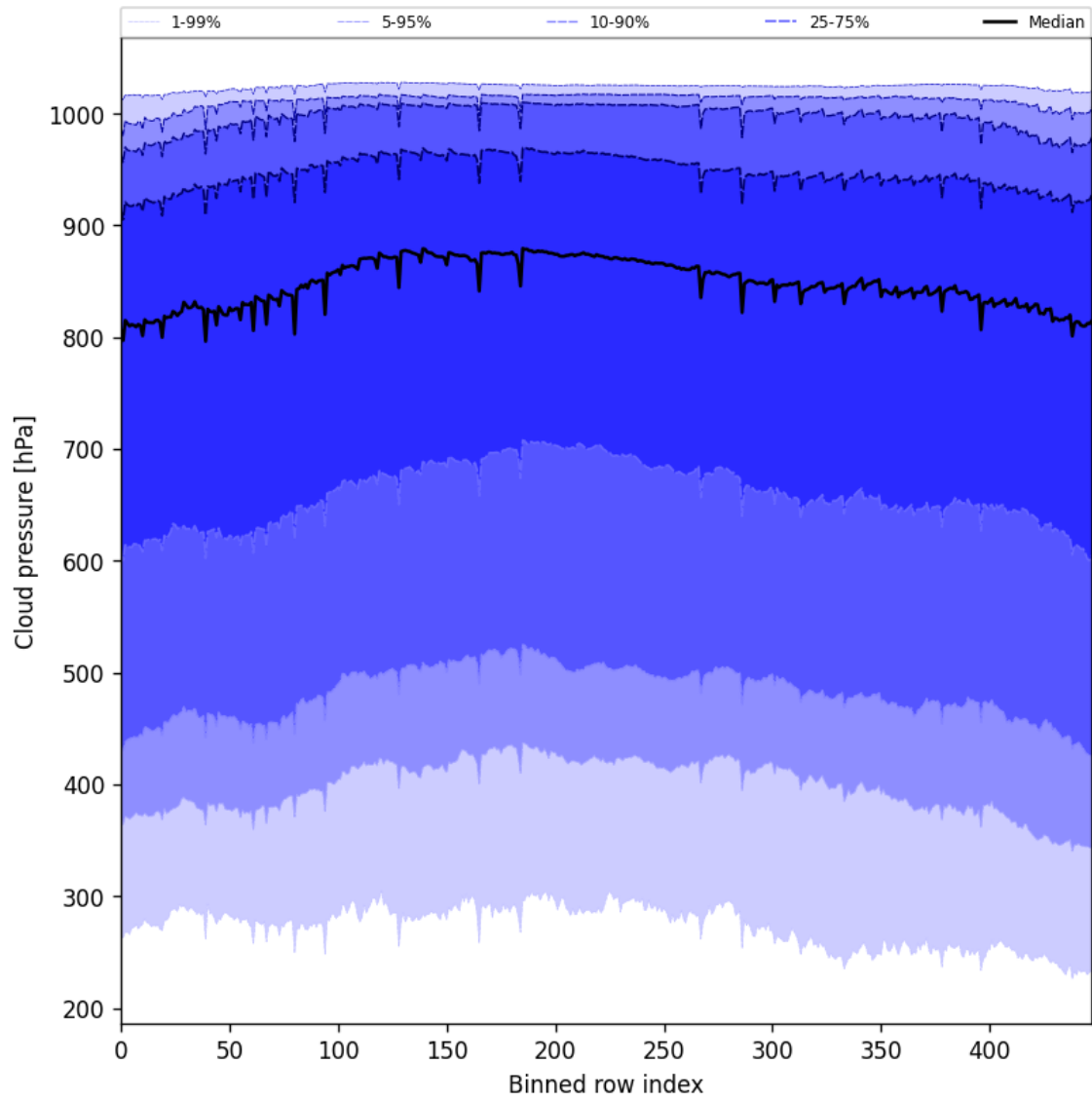
Figure 45: Along track statistics of “Cloud pressure” for 2025-07-26 to 2025-07-27
