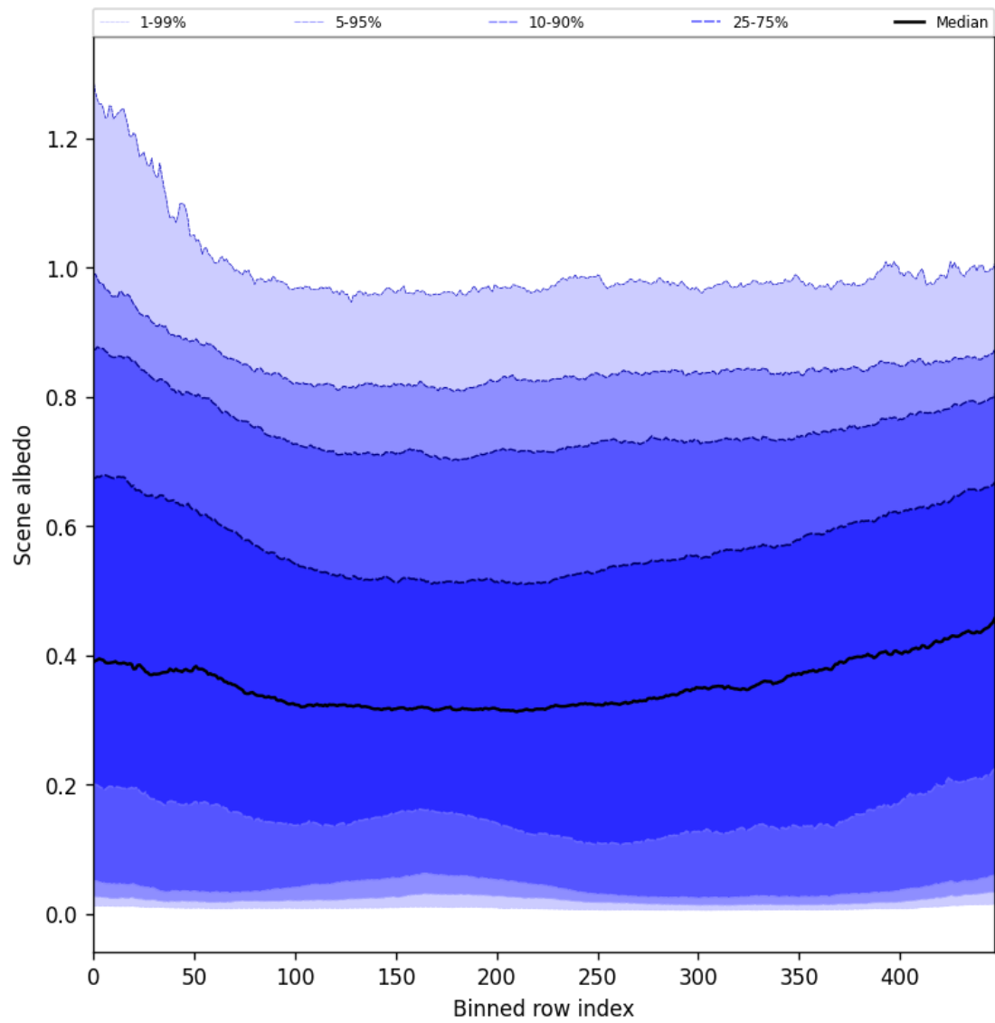
Figure 49: Along track statistics of “Scene albedo” for 2025-07-26 to 2025-07-27
