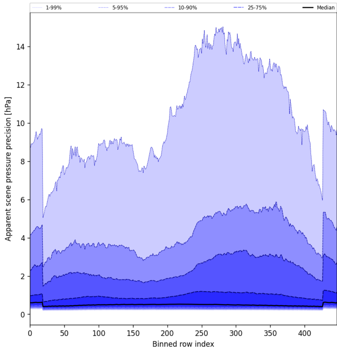
Figure 52: Along track statistics of “Apparent scene pressure precision” for 2025-07-26 to 2025-07-27
