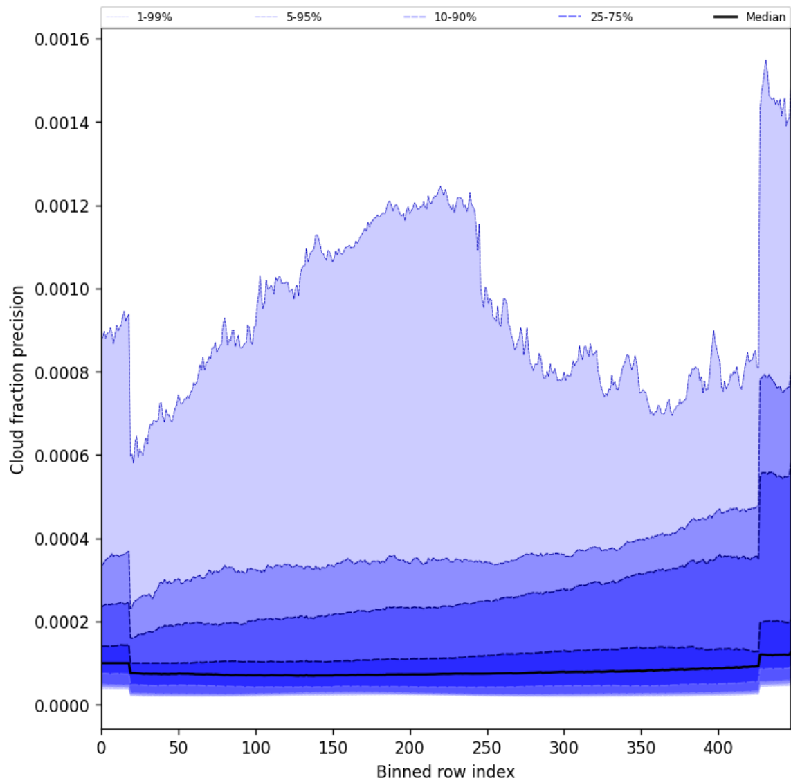
Figure 48: Along track statistics of “Cloud fraction precision” for 2025-07-26 to 2025-07-27
