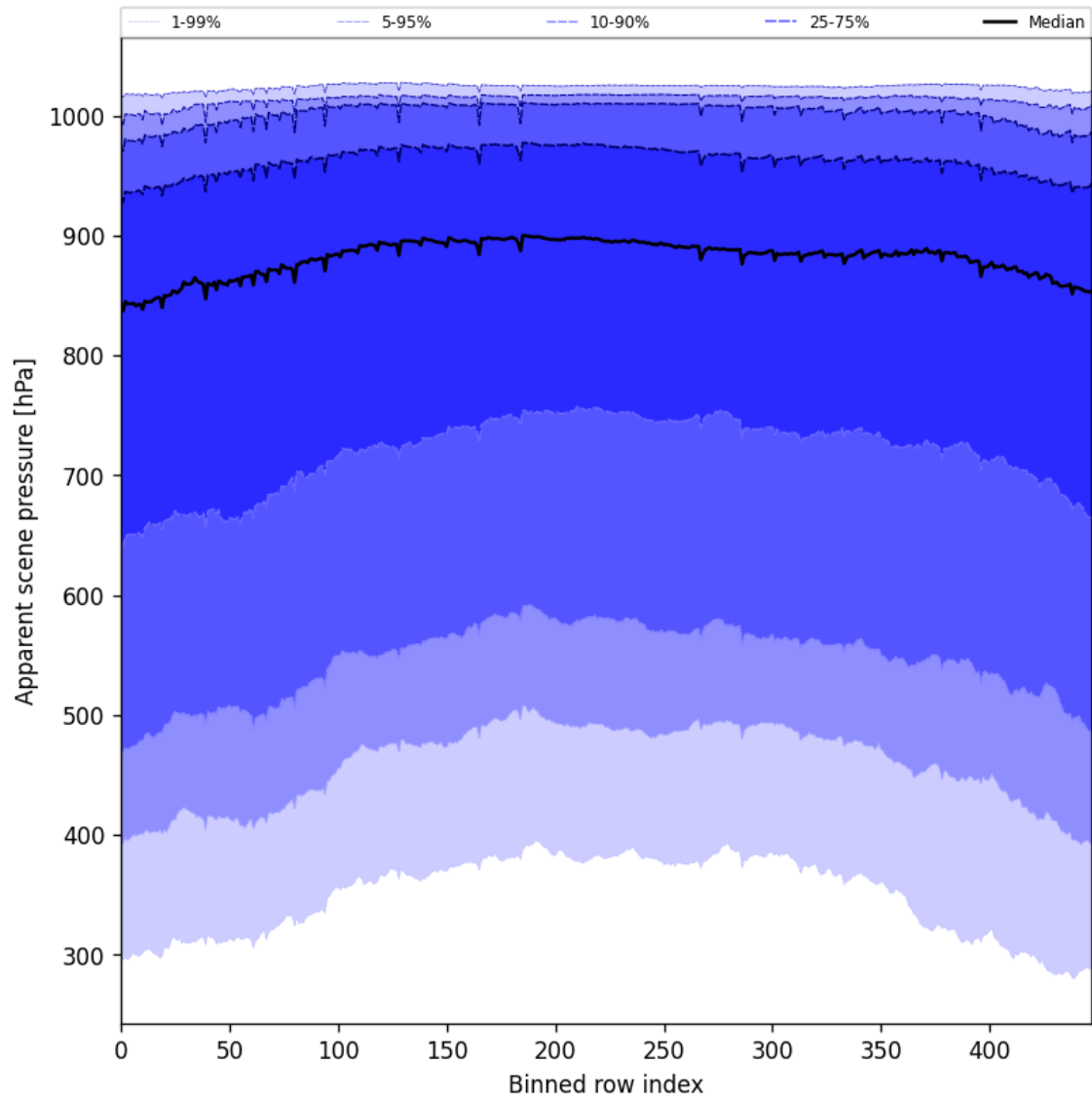
Figure 51: Along track statistics of “Apparent scene pressure” for 2025-07-26 to 2025-07-27
