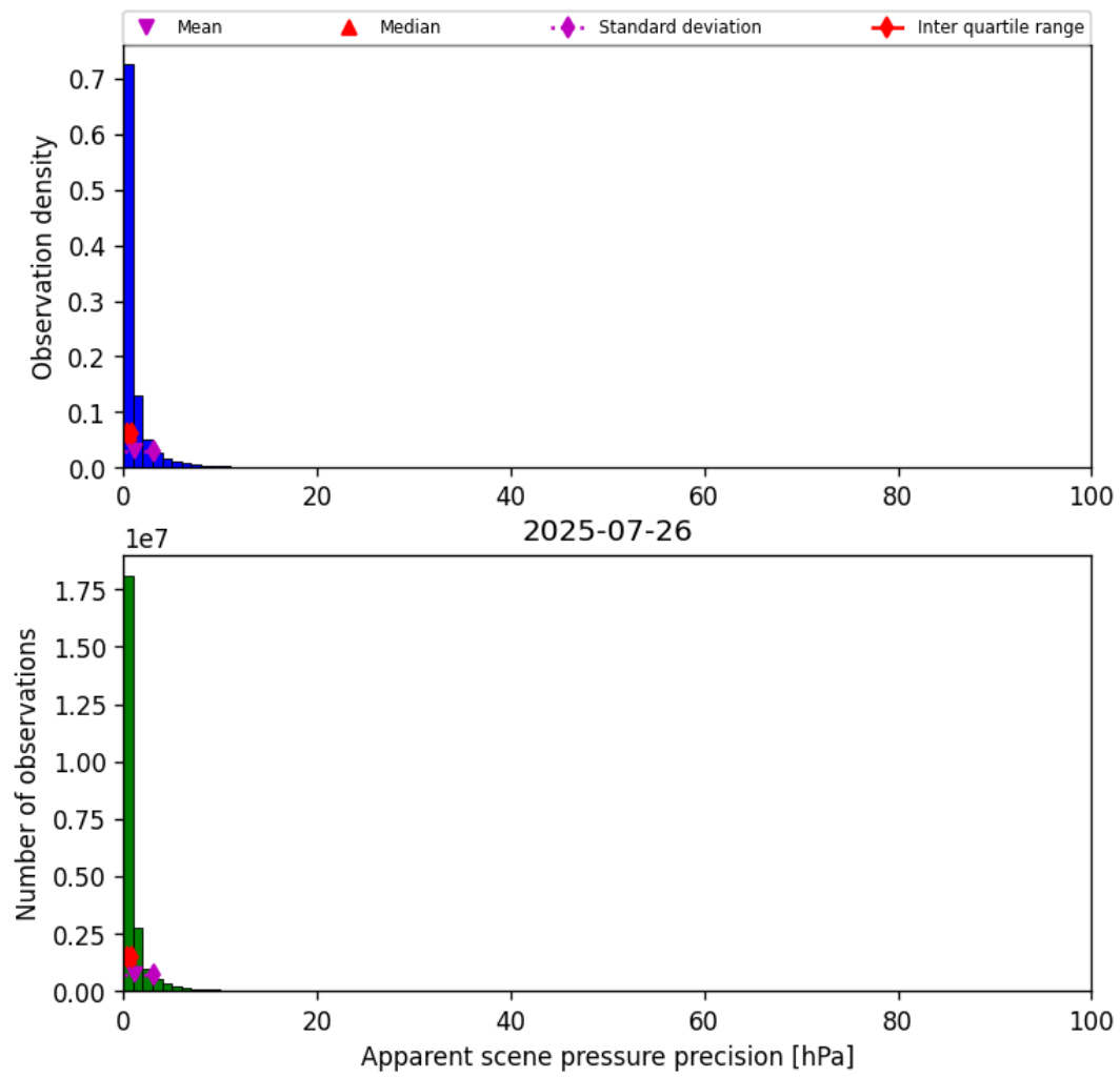
Figure 35: Histogram of “Apparent scene pressure precision” for 2025-07-26 to 2025-07-27
