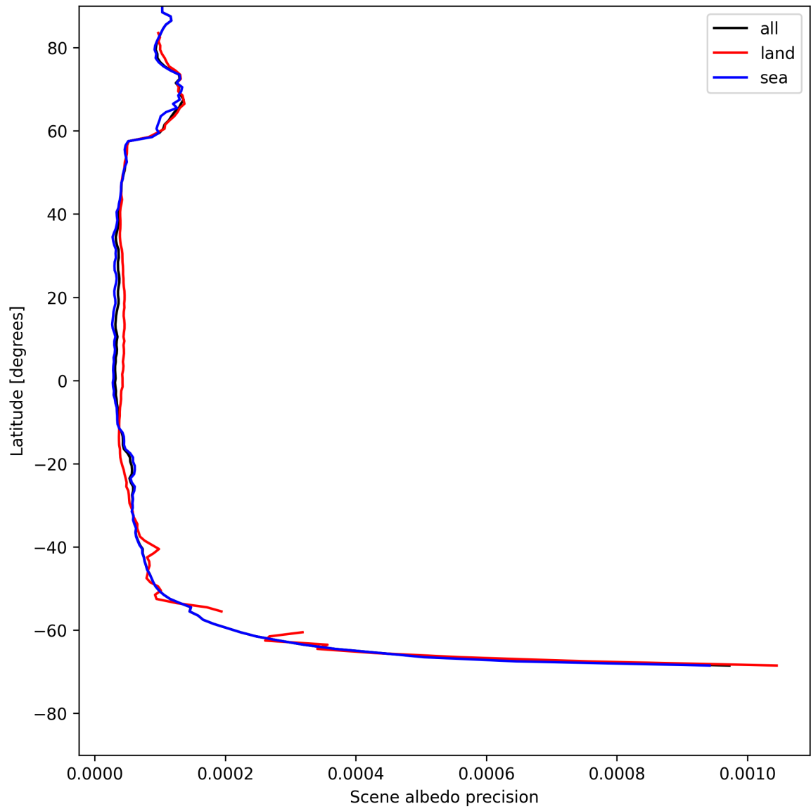
Figure 16: Zonal average of "Scene albedo precision" for 2025-07-27 to 2025-07-27.
