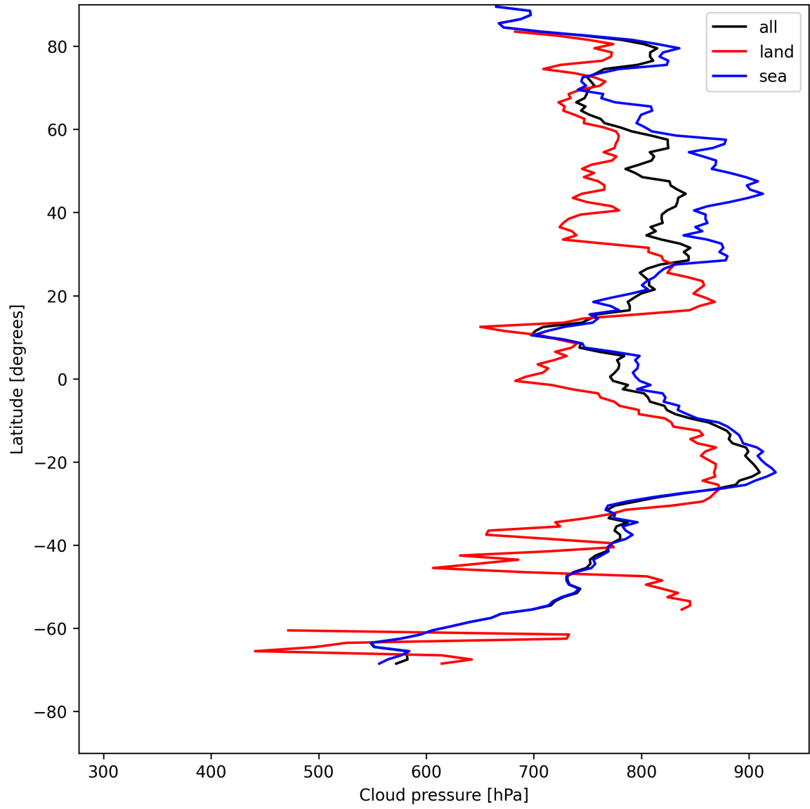
Figure 11: Zonal average of “Cloud pressure” for 2025-07-27 to 2025-07-27.
