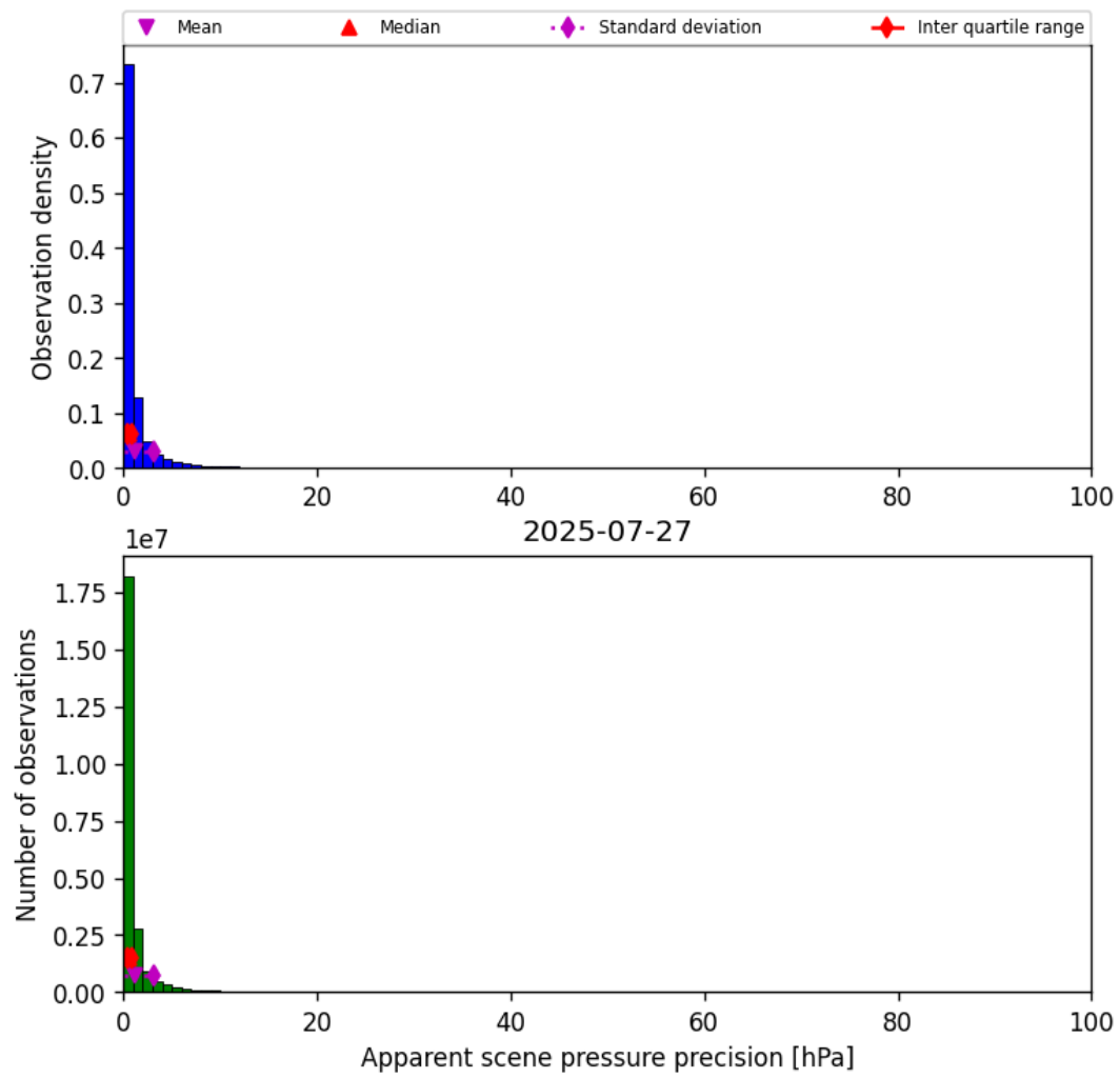
Figure 35: Histogram of “Apparent scene pressure precision” for 2025-07-27 to 2025-07-27
