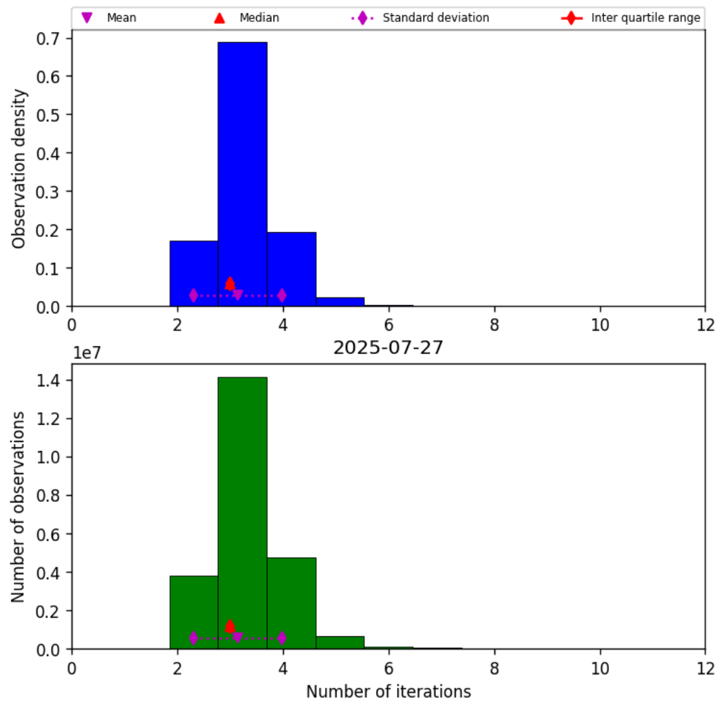
Figure 37: Histogram of “Number of iterations” for 2025-07-27 to 2025-07-27
