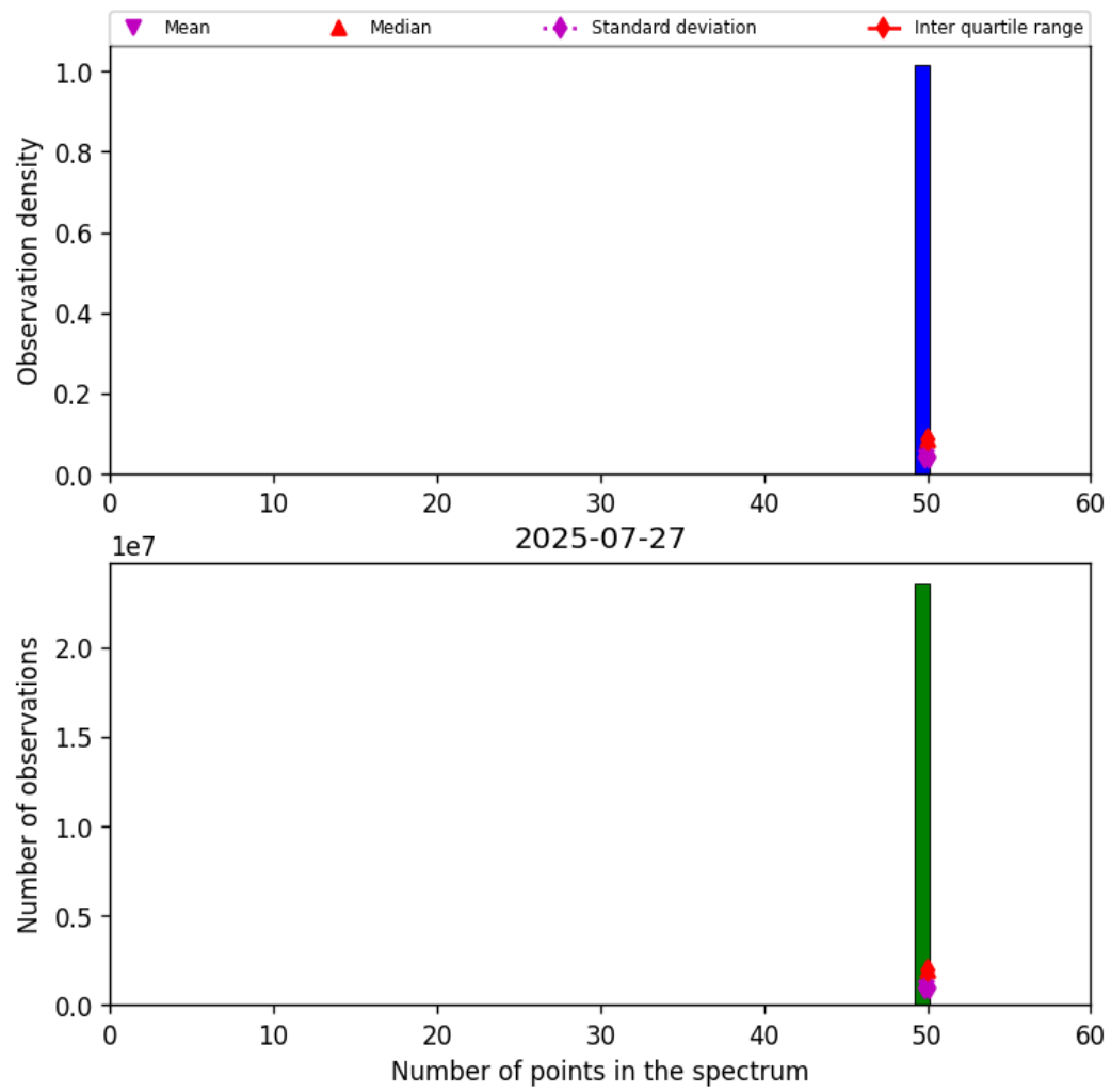
Figure 42: Histogram of “Number of points in the spectrum” for 2025-07-27 to 2025-07-27
