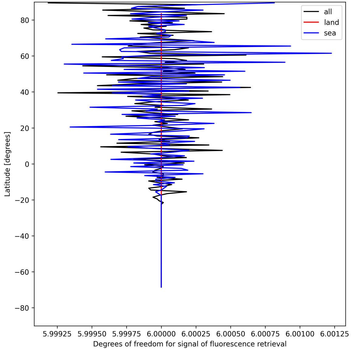
Figure 24: Zonal average of “Degrees of freedom for signal of fluorescence retrieval” for 2025-07-27 to 2025-07-27.
