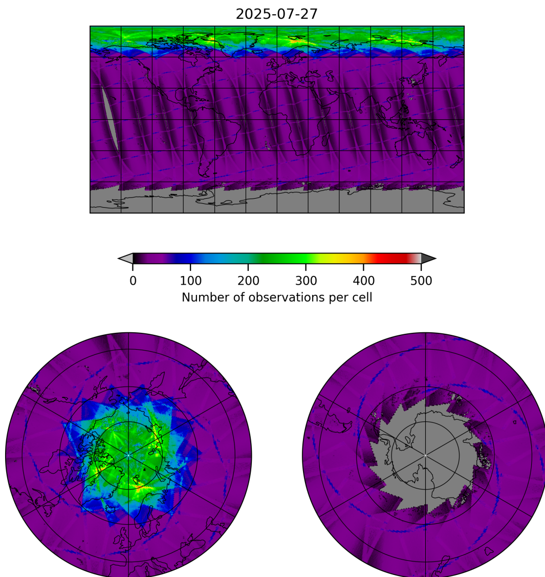
Figure 9: Map of the number of observations for 2025-07-27 to 2025-07-27
