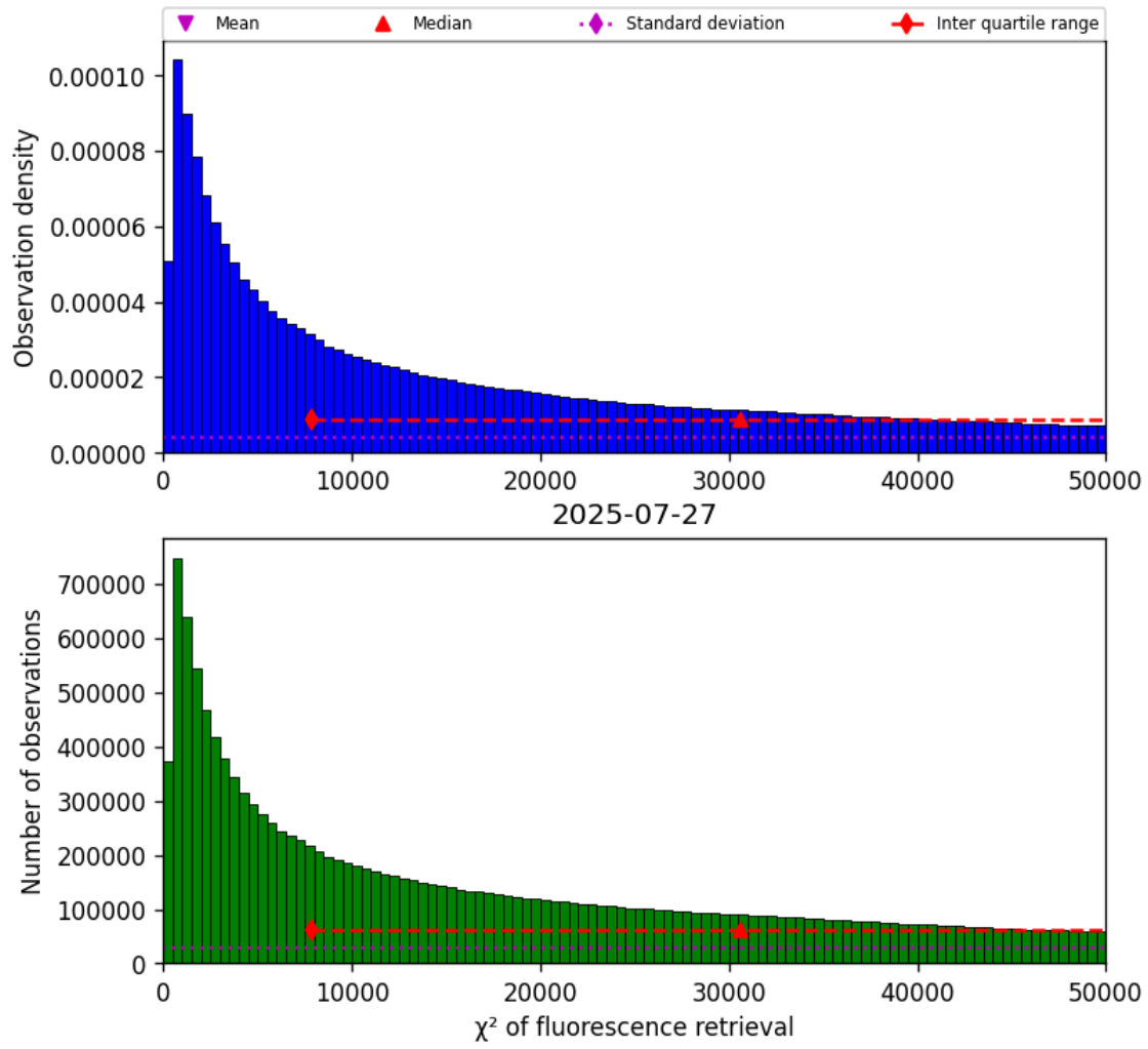
Figure 40: Histogram of “ \chi^2 of fluorescence retrieval” for 2025-07-27 to 2025-07-27
