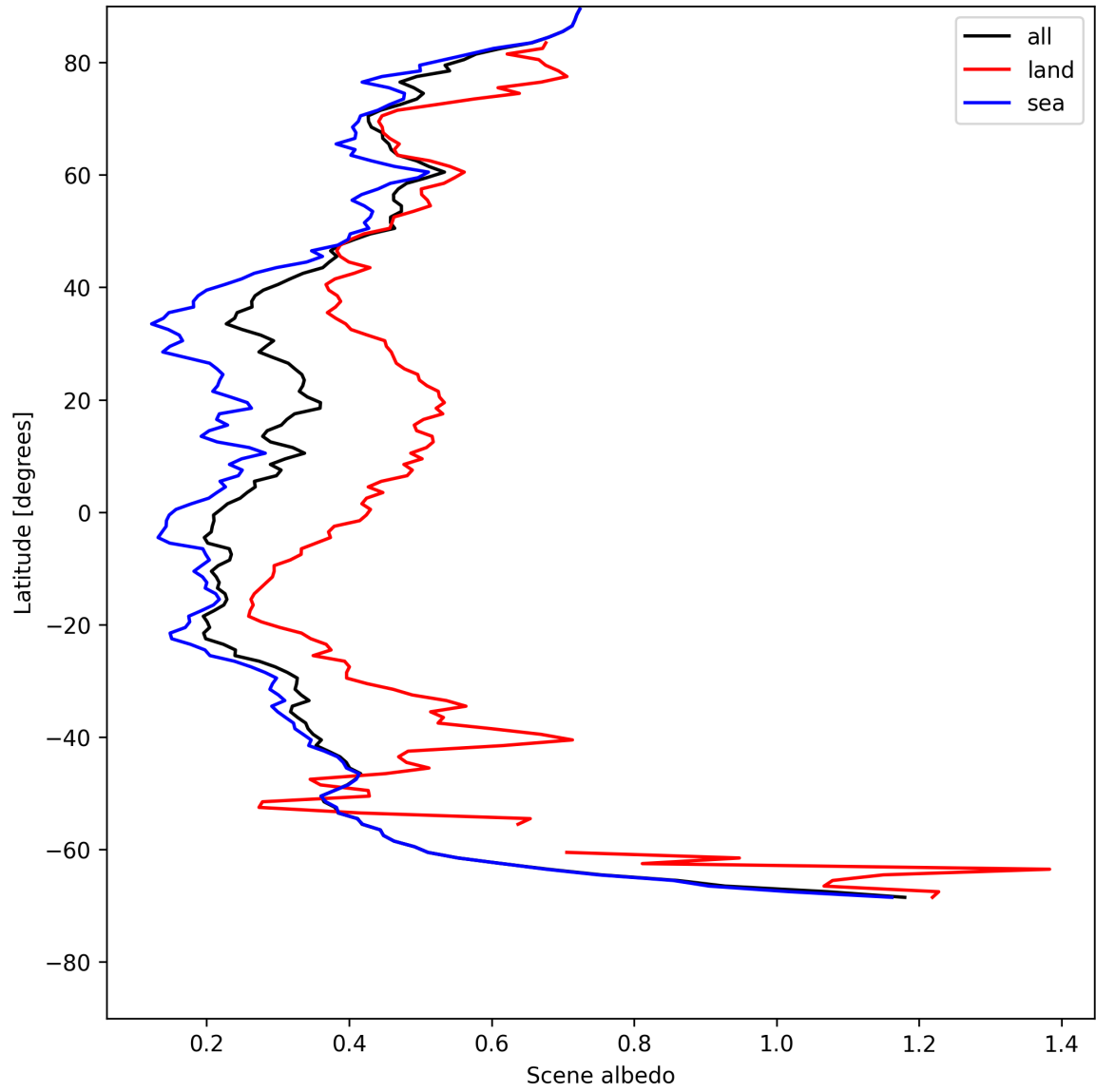
Figure 15: Zonal average of “Scene albedo” for 2025-07-27 to 2025-07-27.
