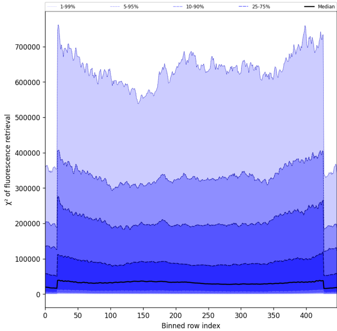
Figure 57: Along track statistics of “ \chi^2 of fluorescence retrieval” for 2025-07-27 to 2025-07-27
