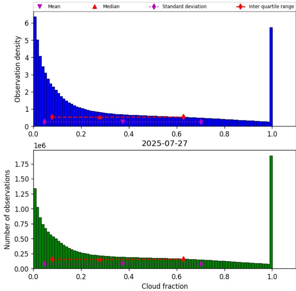
Figure 30: Histogram of “Cloud fraction” for 2025-07-27 to 2025-07-27
