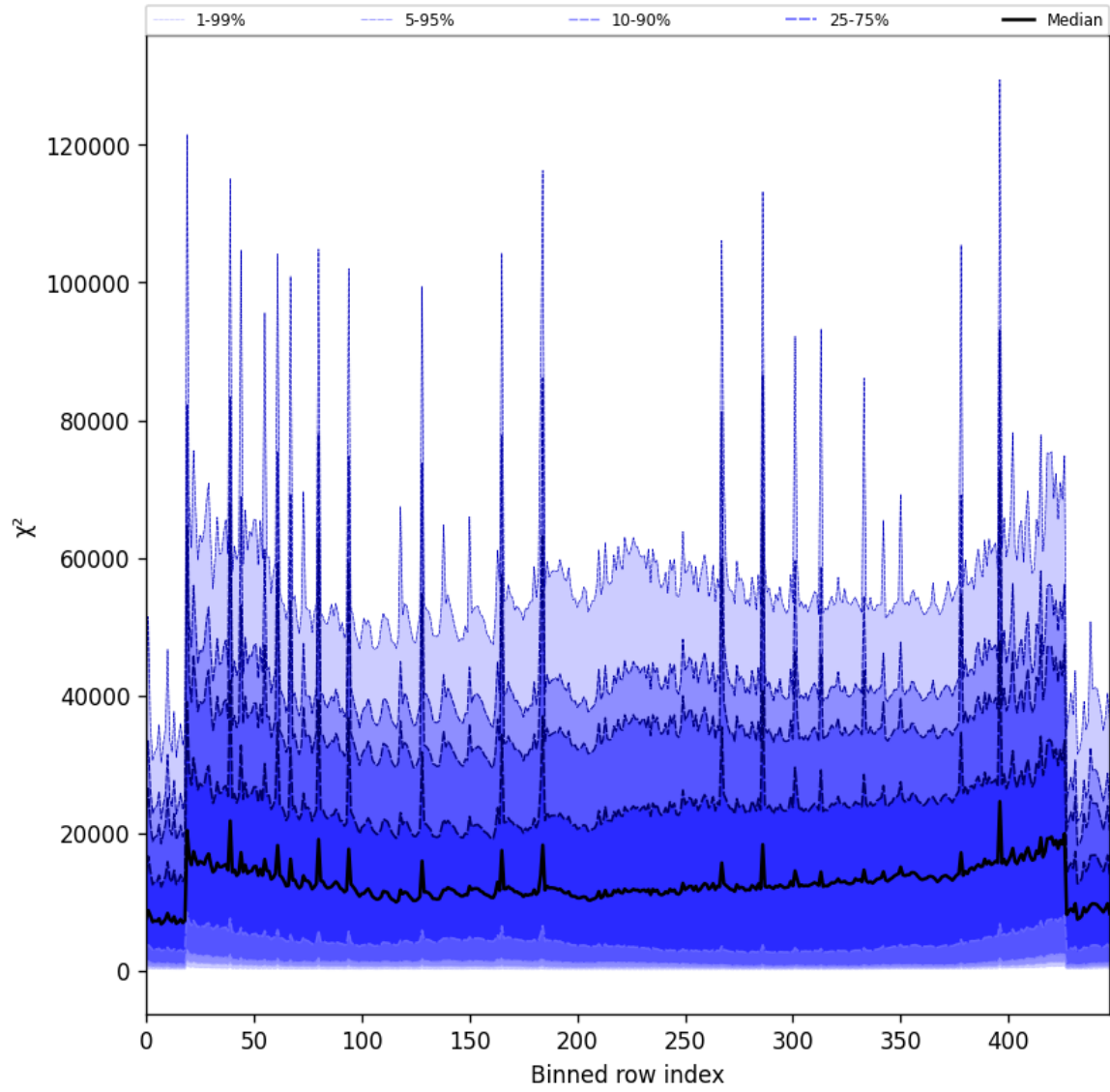
Figure 53: Along track statistics of “ \chi^2 ” for 2025-07-27 to 2025-07-27
