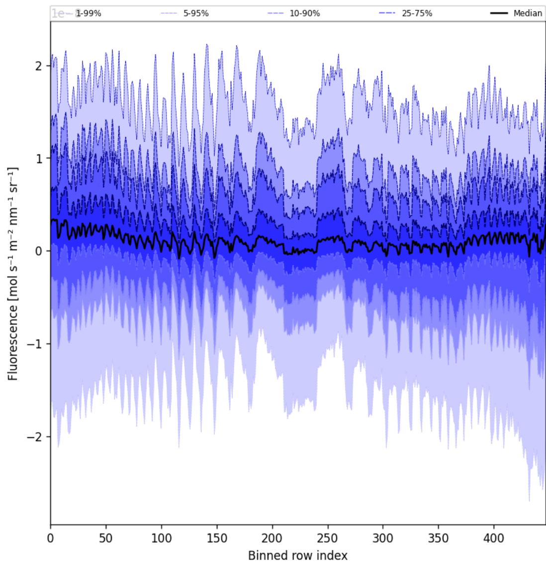
Figure 55: Along track statistics of “Fluorescence” for 2025-07-27 to 2025-07-27
