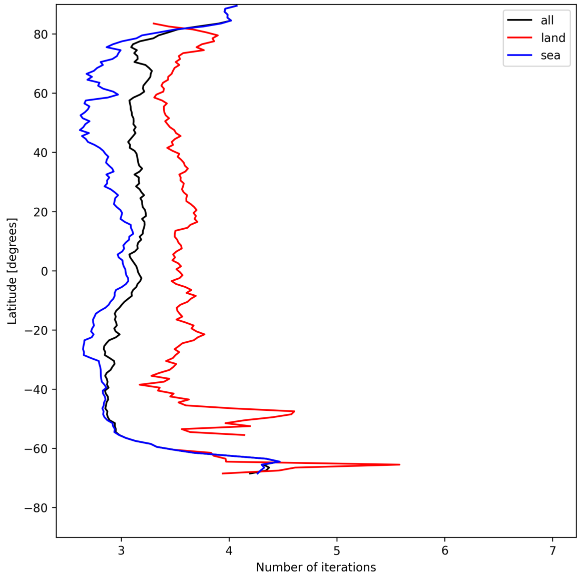
Figure 20: Zonal average of “Number of iterations” for 2025-07-27 to 2025-07-27.
