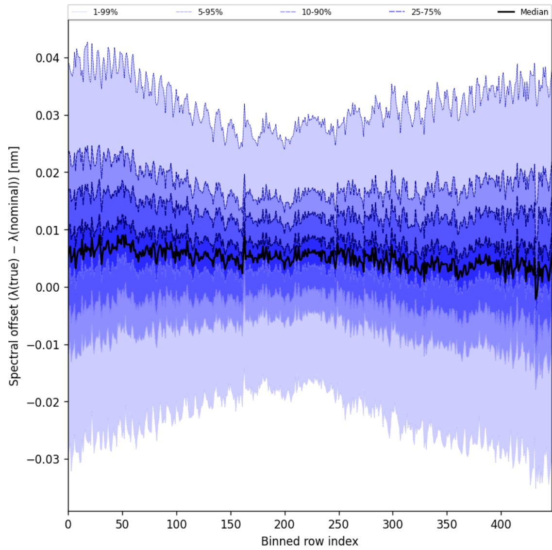
Figure 60: Along track statistics of “Spectral offset ( \lambda_{\text{true}} - \lambda_{\text{nominal}} )” for 2025-07-27 to 2025-07-27
