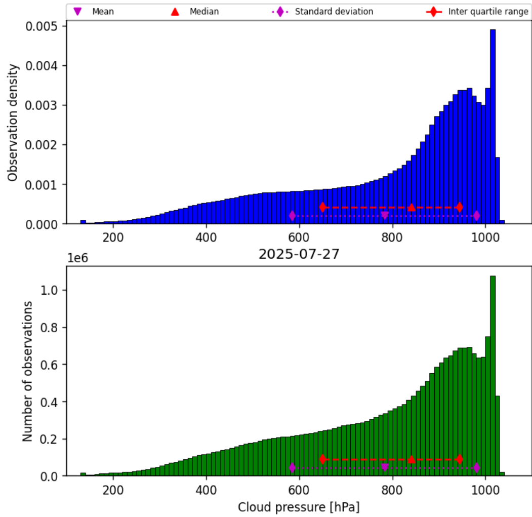
Figure 28: Histogram of “Cloud pressure” for 2025-07-27 to 2025-07-27
