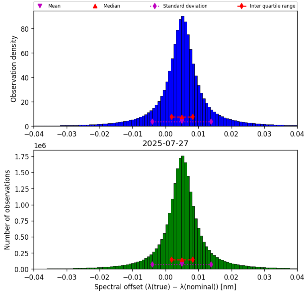
Figure 43: Histogram of “Spectral offset ( \lambda_{\text{true}} - \lambda_{\text{nominal}} )” for 2025-07-27 to 2025-07-27
