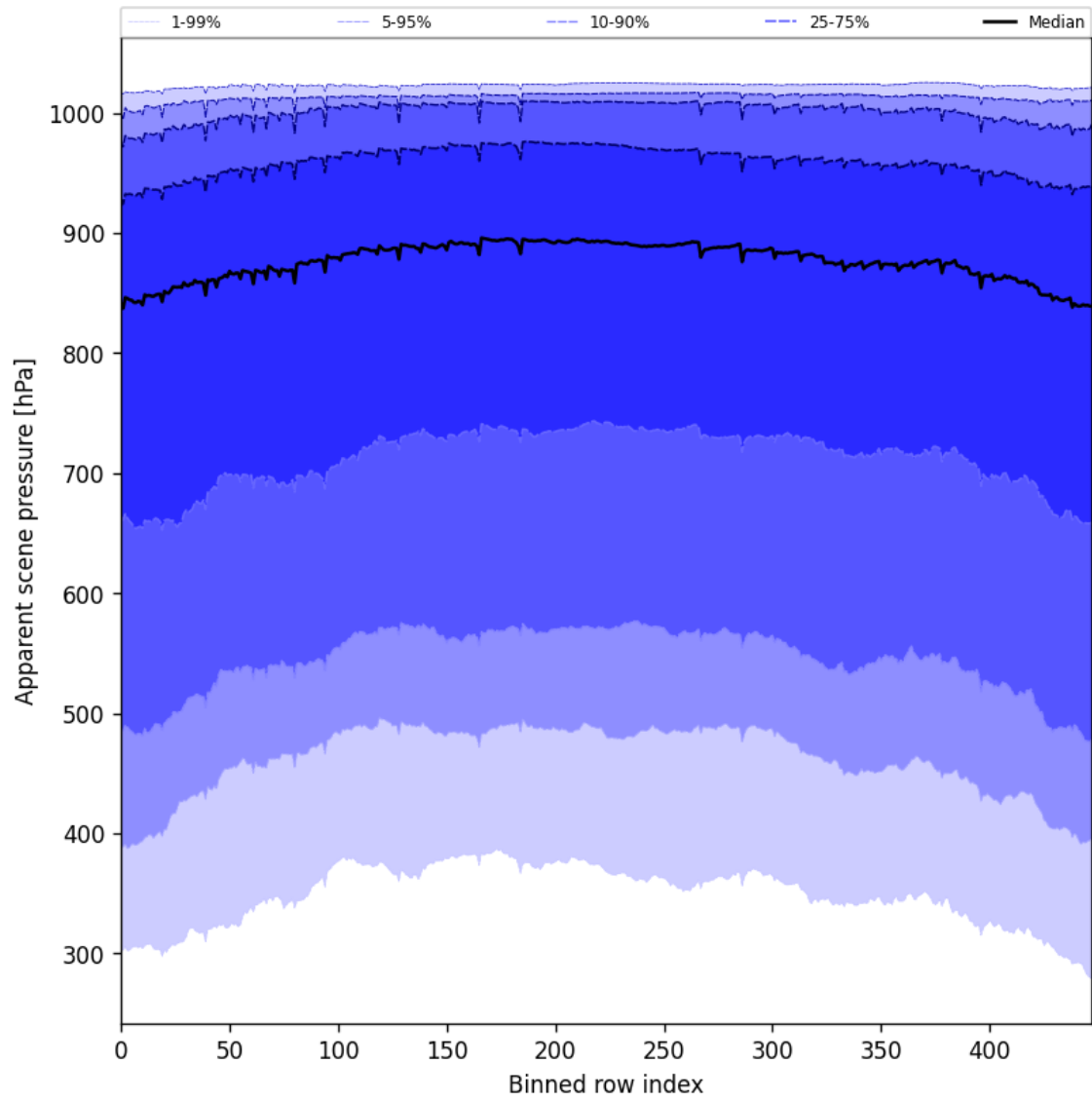
Figure 51: Along track statistics of “Apparent scene pressure” for 2025-07-27 to 2025-07-27
