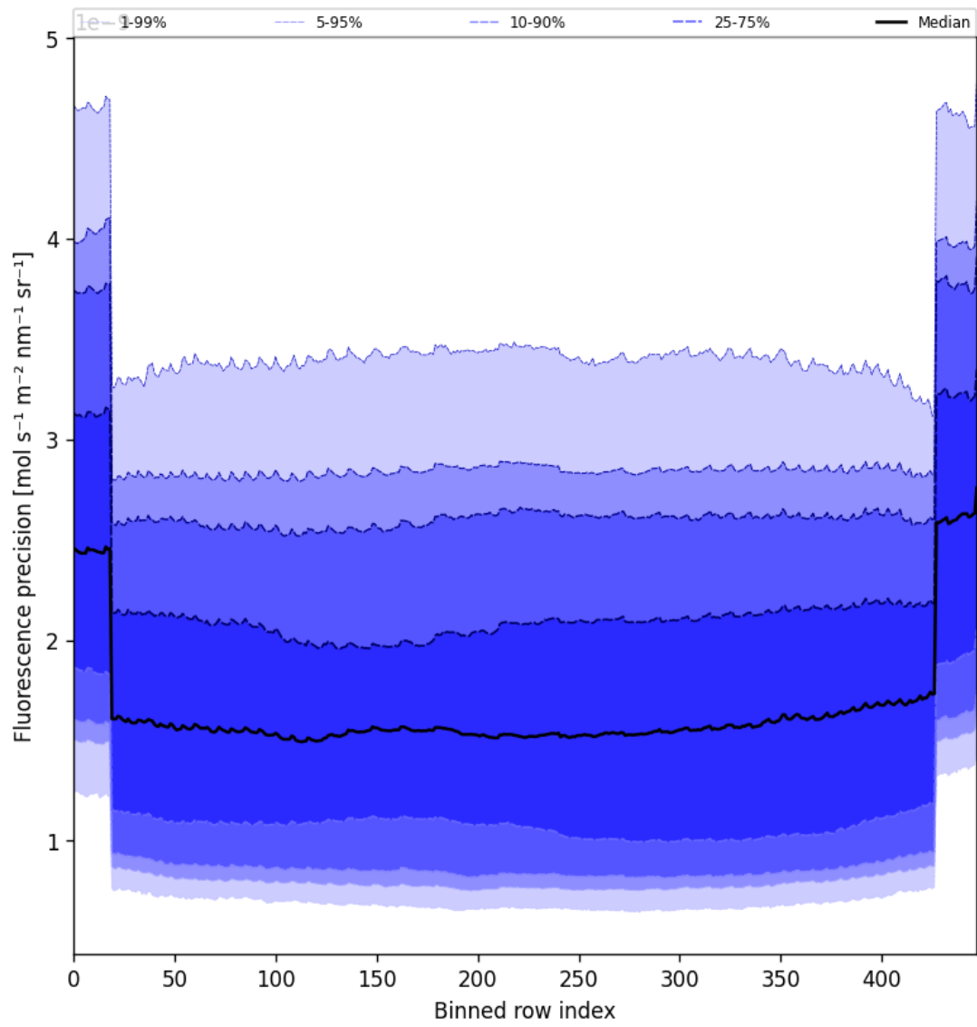
Figure 56: Along track statistics of “Fluorescence precision” for 2025-07-27 to 2025-07-27
