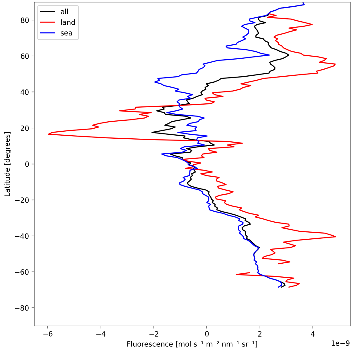
Figure 21: Zonal average of “Fluorescence” for 2025-07-27 to 2025-07-27.
