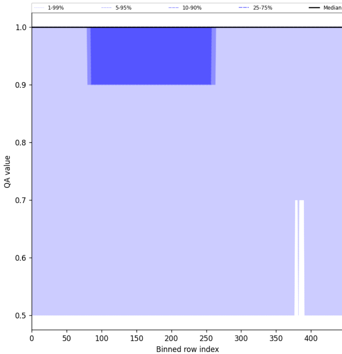
Figure 44: Along track statistics of “QA value” for 2025-07-27 to 2025-07-27
