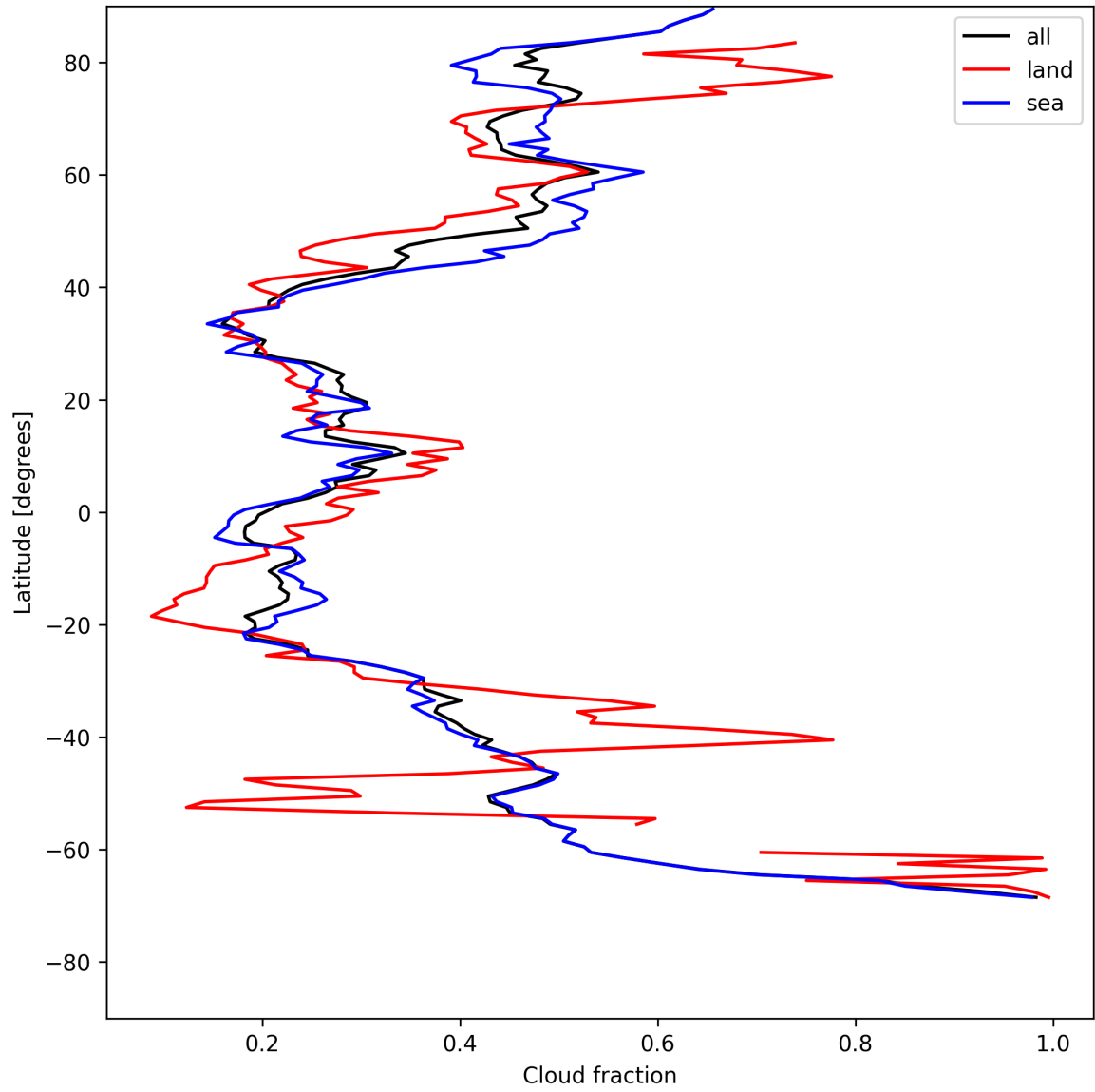
Figure 13: Zonal average of “Cloud fraction” for 2025-07-27 to 2025-07-27.
