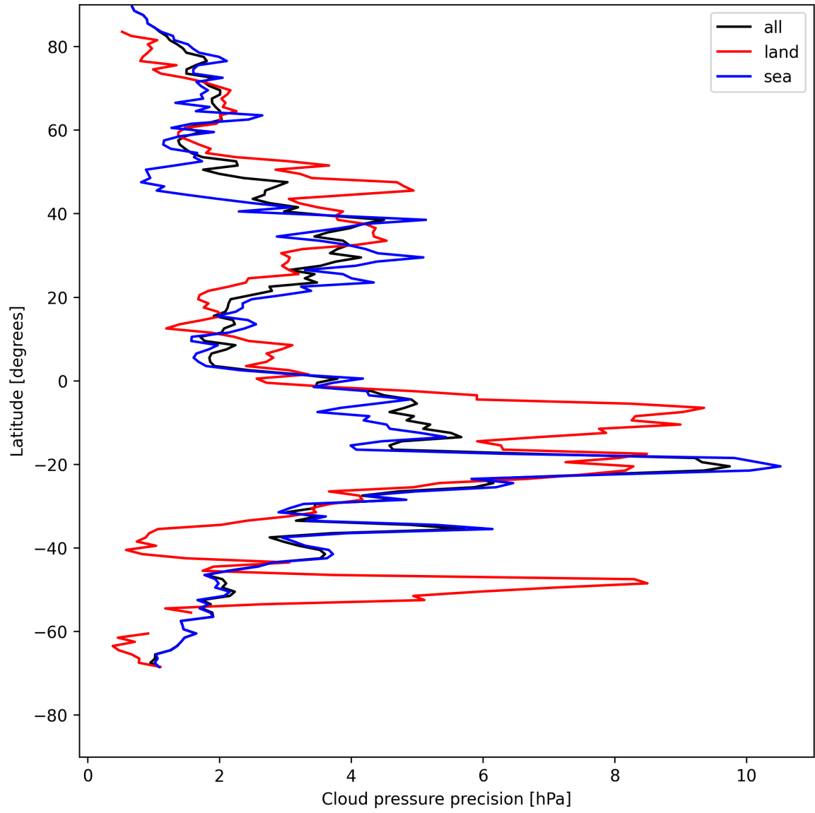
Figure 12: Zonal average of “Cloud pressure precision” for 2025-07-27 to 2025-07-27.
