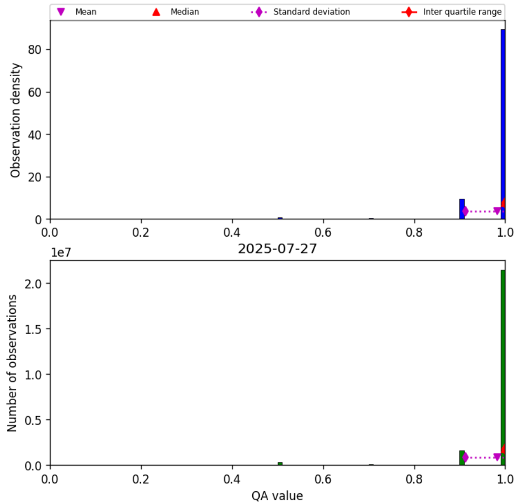
Figure 27: Histogram of “QA value” for 2025-07-27 to 2025-07-27
