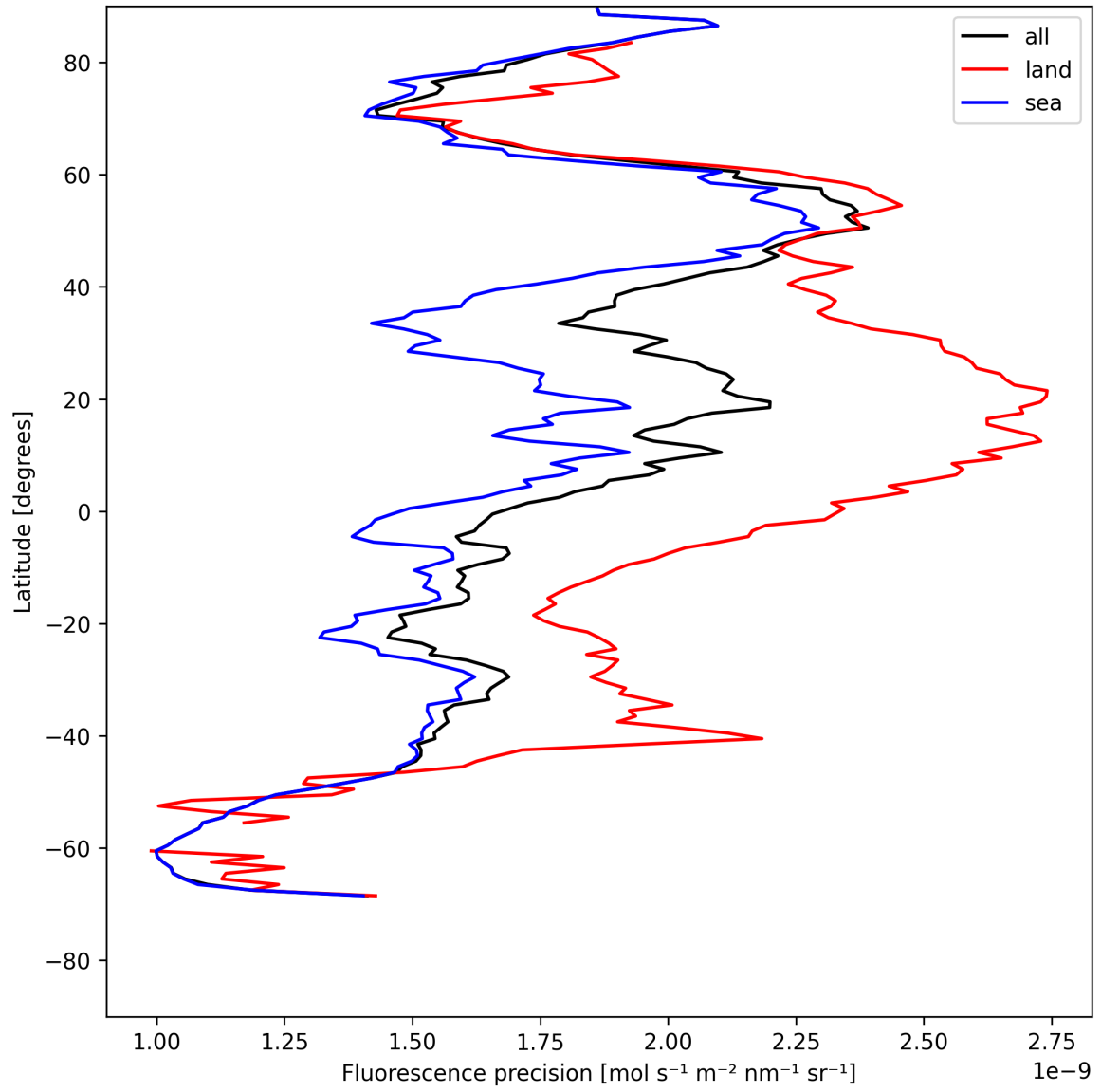
Figure 22: Zonal average of “Fluorescence precision” for 2025-07-27 to 2025-07-27.
