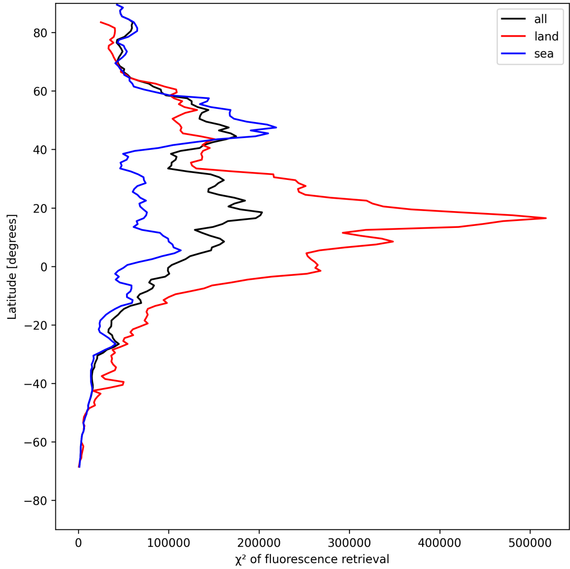
Figure 23: Zonal average of “ \chi^2 of fluorescence retrieval” for 2025-07-27 to 2025-07-27.
