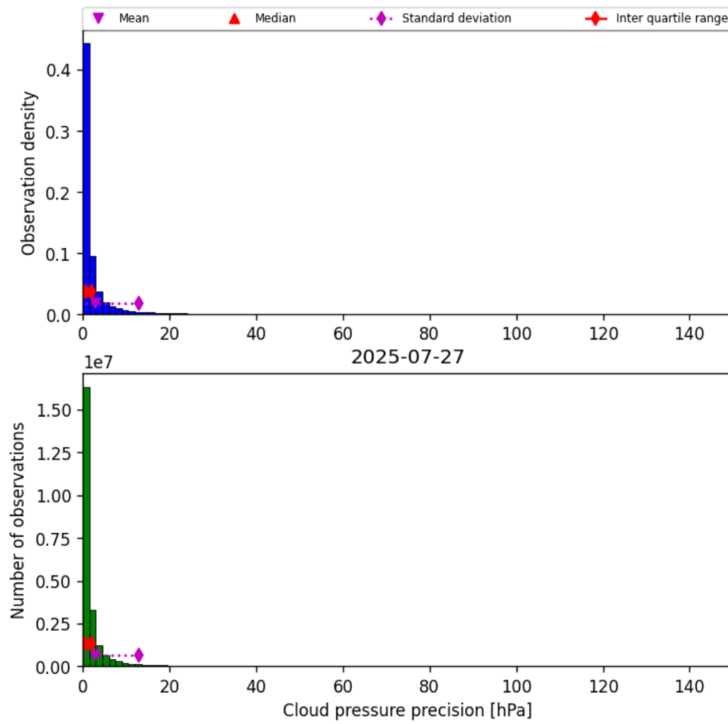
Figure 29: Histogram of “Cloud pressure precision” for 2025-07-27 to 2025-07-27
