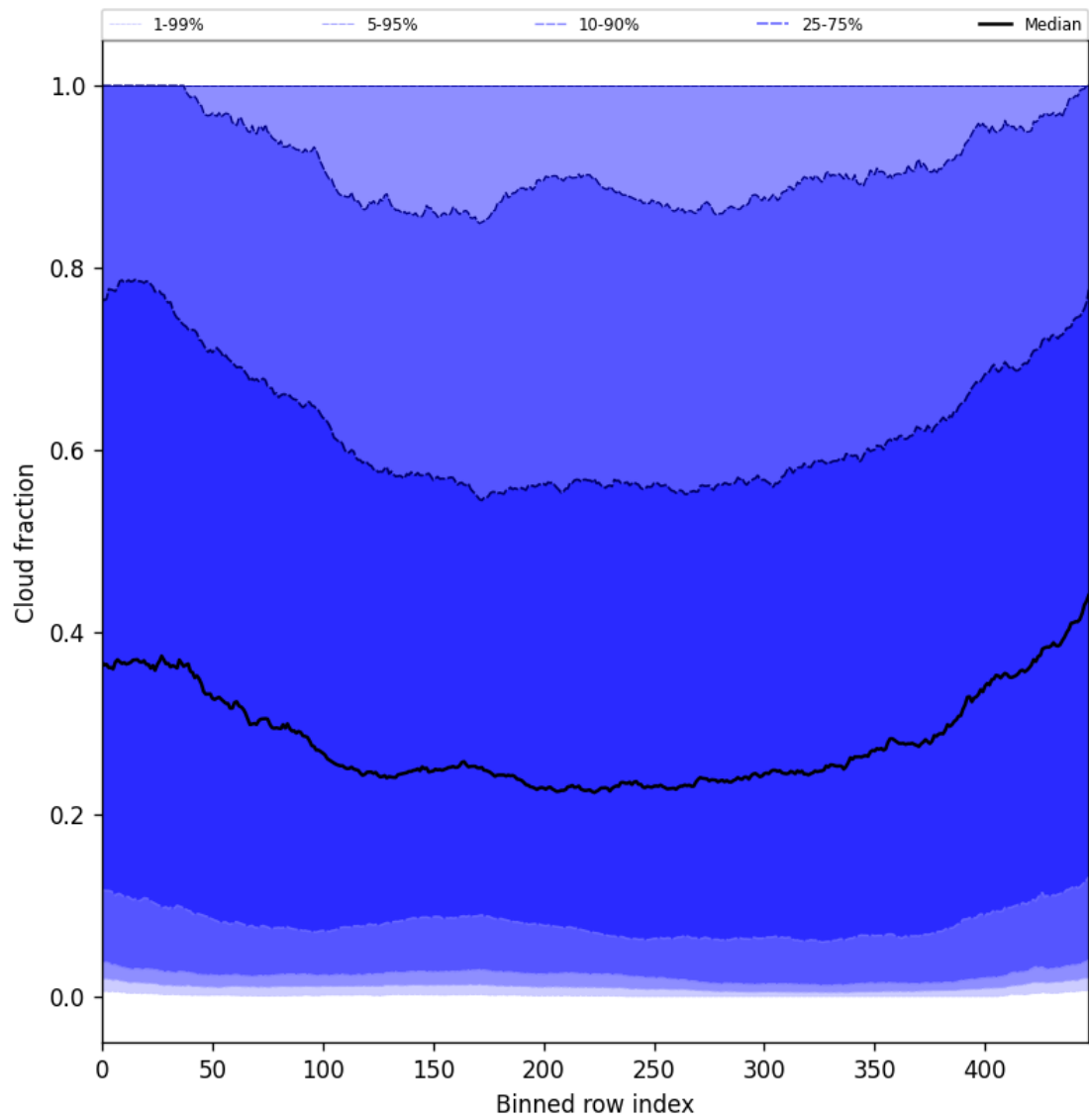
Figure 47: Along track statistics of “Cloud fraction” for 2025-07-27 to 2025-07-27
