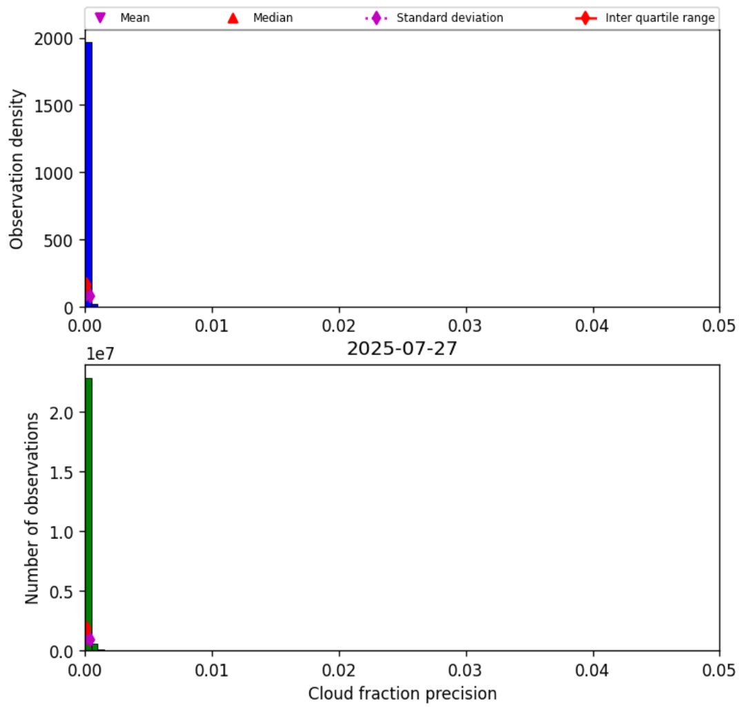
Figure 31: Histogram of “Cloud fraction precision” for 2025-07-27 to 2025-07-27
