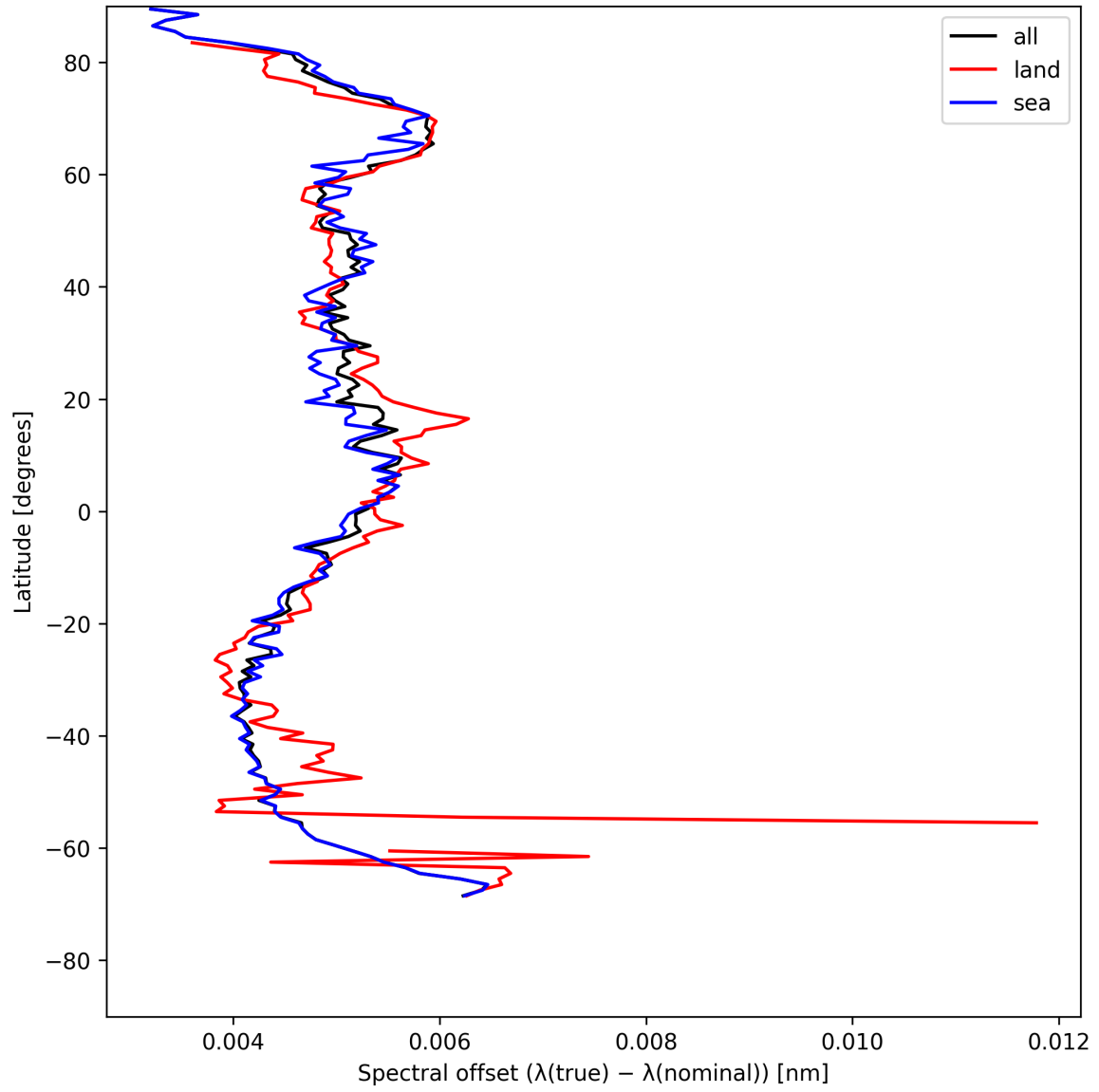
Figure 26: Zonal average of “Spectral offset ( \lambda_{\text{true}} - \lambda_{\text{nominal}} )” for 2025-07-27 to 2025-07-27.
