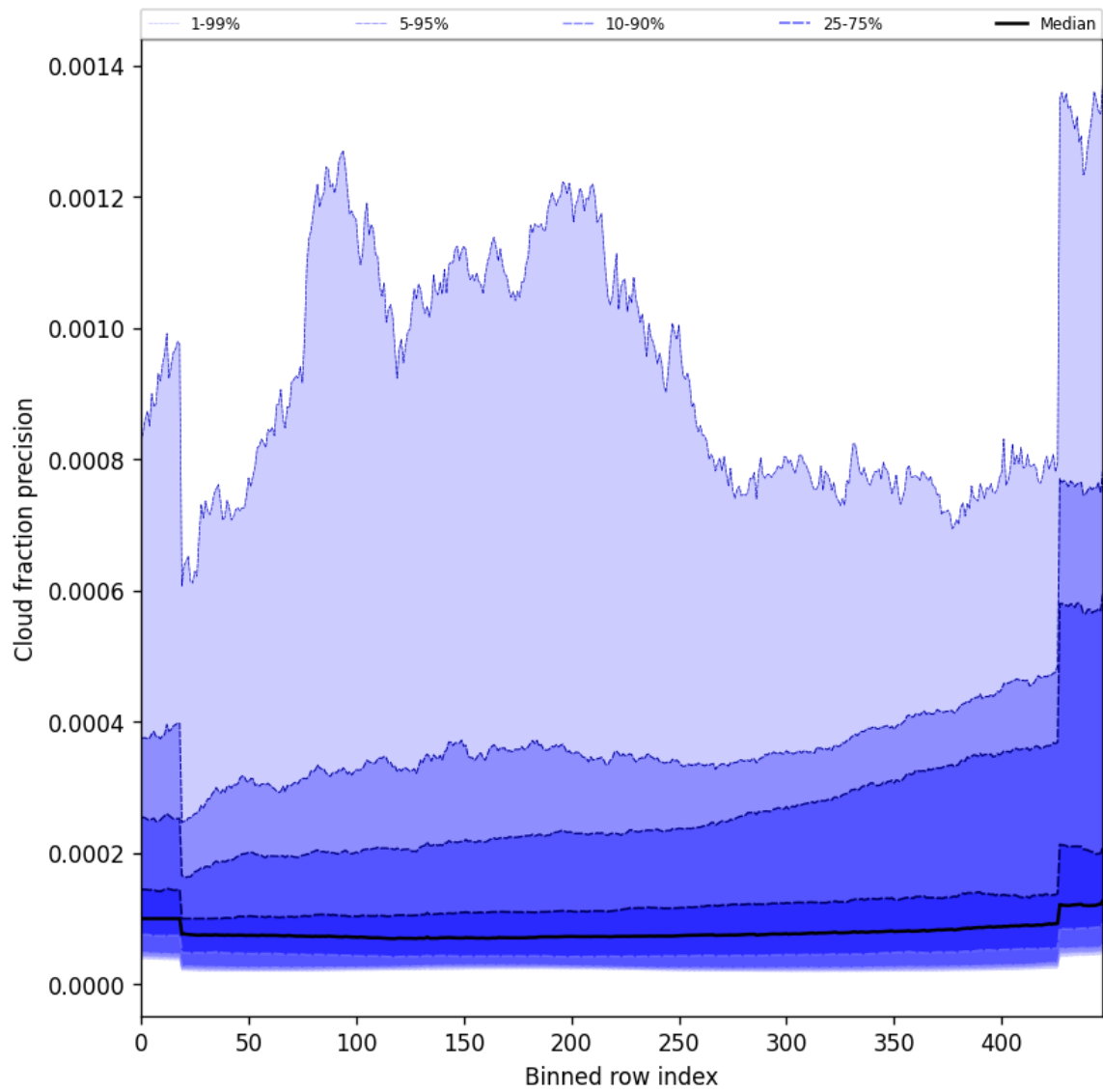
Figure 48: Along track statistics of “Cloud fraction precision” for 2025-07-27 to 2025-07-27
