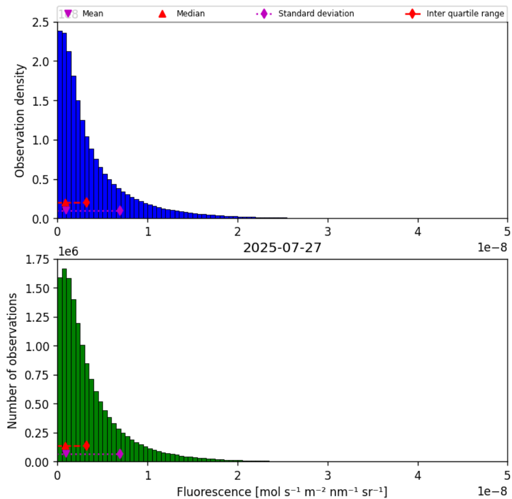
Figure 38: Histogram of “Fluorescence” for 2025-07-27 to 2025-07-27
