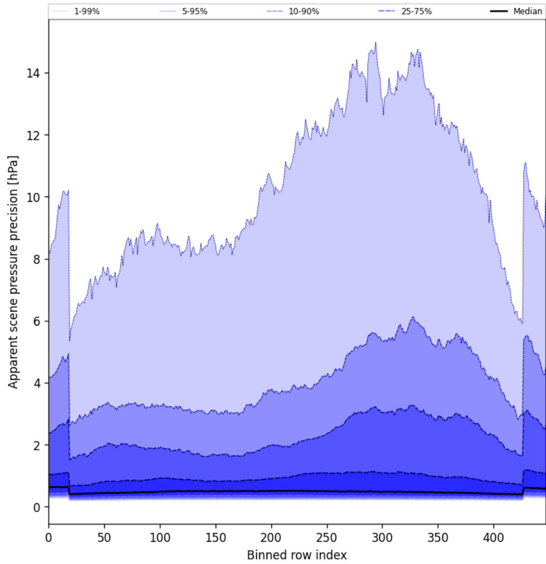
Figure 52: Along track statistics of “Apparent scene pressure precision” for 2025-07-27 to 2025-07-27
