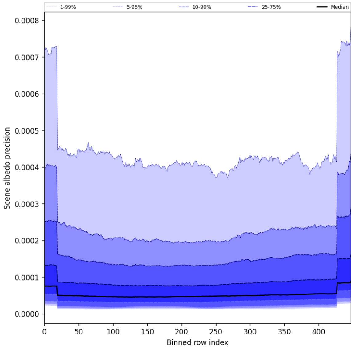
Figure 50: Along track statistics of “Scene albedo precision” for 2025-07-27 to 2025-07-27
