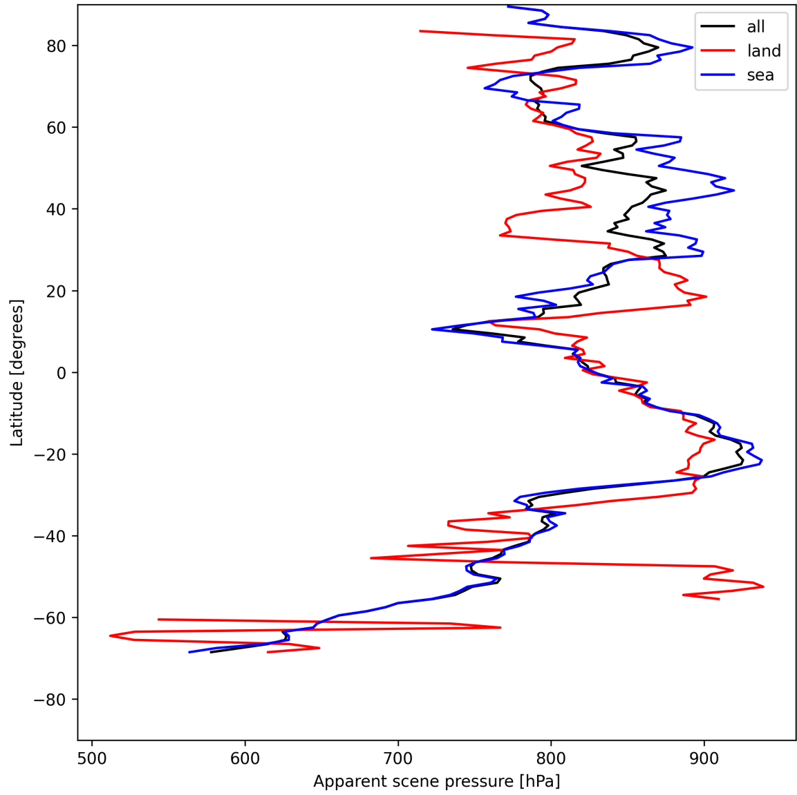
Figure 17: Zonal average of “Apparent scene pressure” for 2025-07-27 to 2025-07-27.
