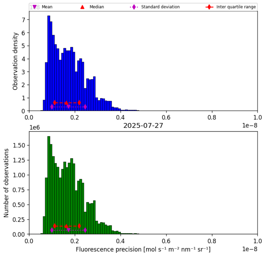
Figure 39: Histogram of “Fluorescence precision” for 2025-07-27 to 2025-07-27
