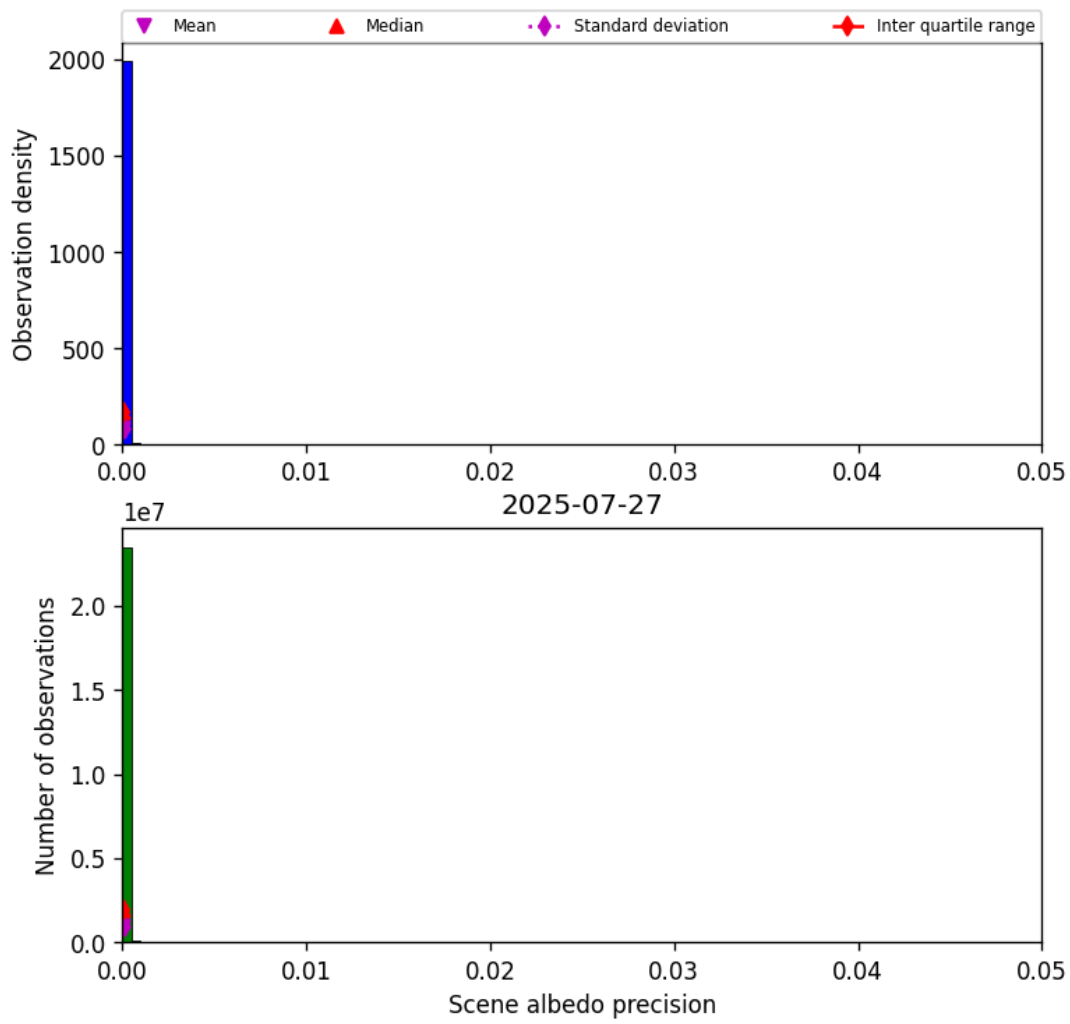
Figure 33: Histogram of “Scene albedo precision” for 2025-07-27 to 2025-07-27
