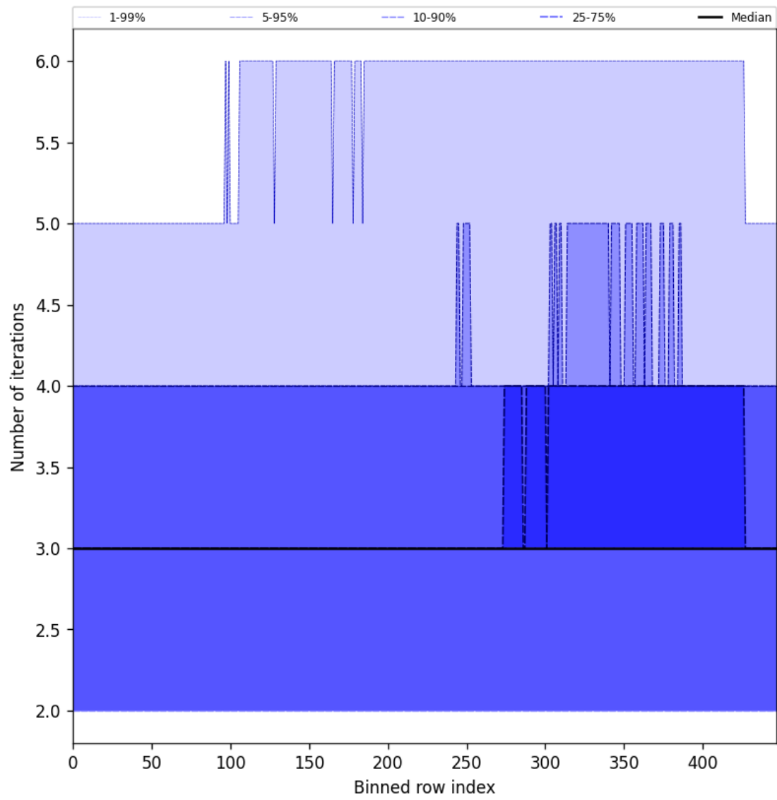
Figure 54: Along track statistics of “Number of iterations” for 2025-07-27 to 2025-07-27
