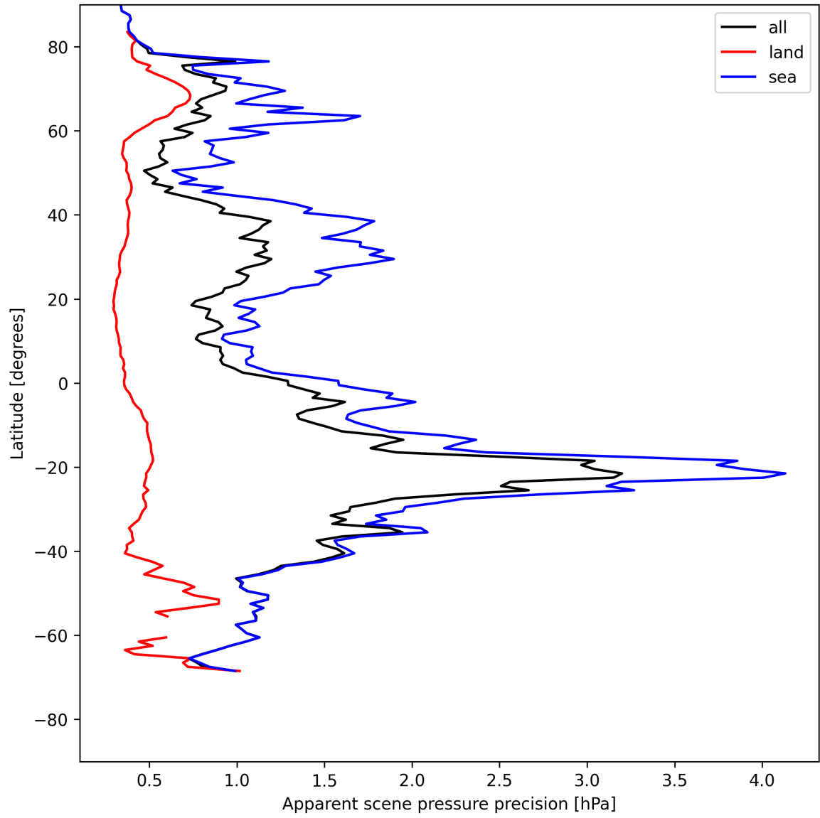
Figure 18: Zonal average of “Apparent scene pressure precision” for 2025-07-27 to 2025-07-27.
