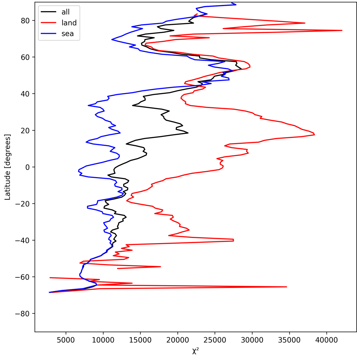
Figure 19: Zonal average of “ \chi^2 ” for 2025-07-27 to 2025-07-27.
