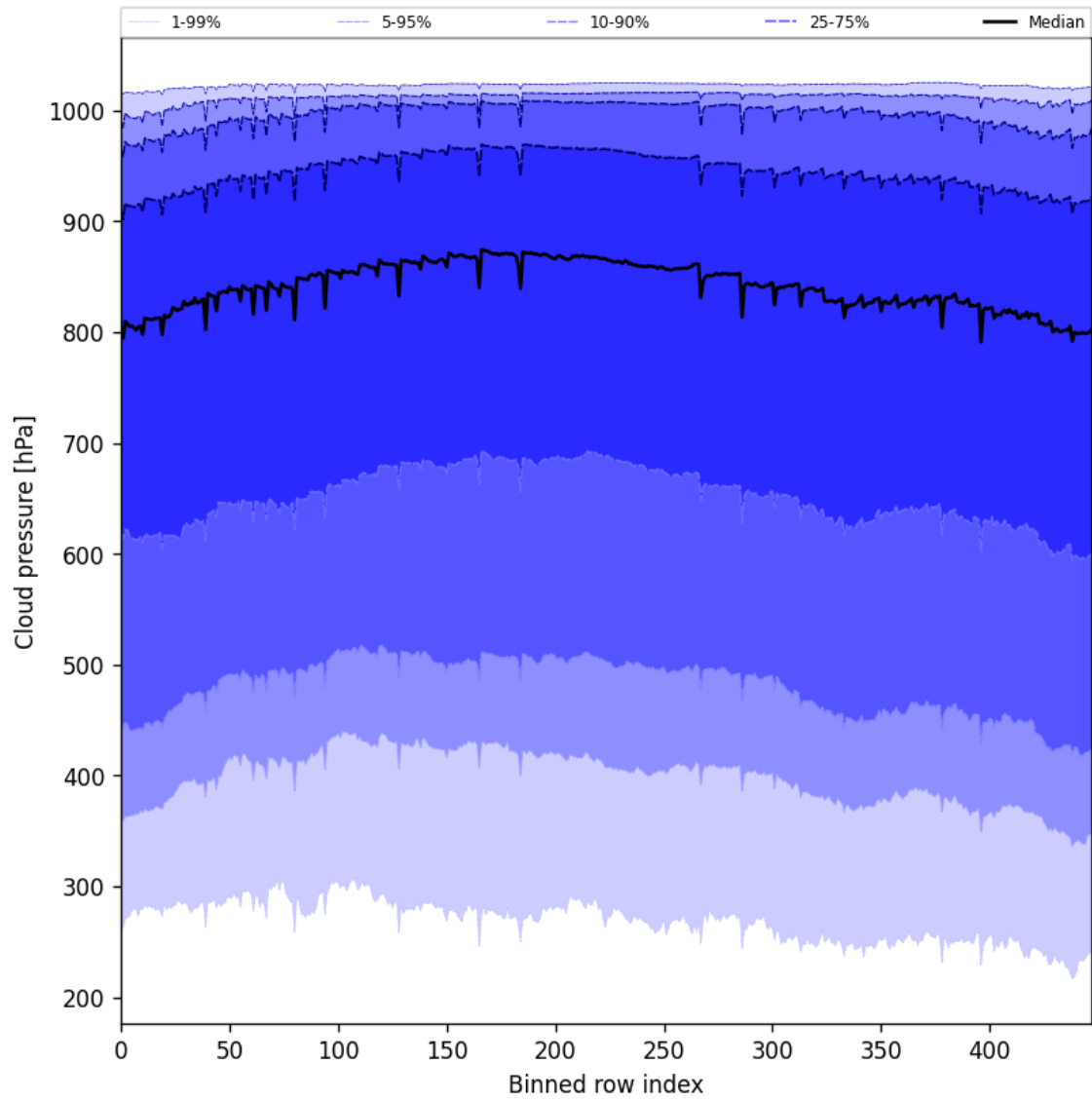
Figure 45: Along track statistics of “Cloud pressure” for 2025-07-27 to 2025-07-27
