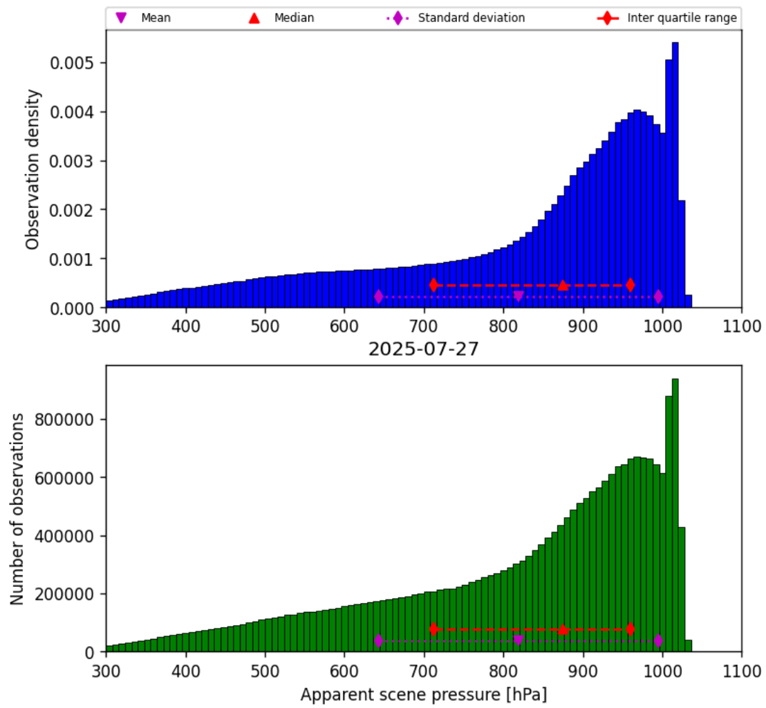
Figure 34: Histogram of “Apparent scene pressure” for 2025-07-27 to 2025-07-27
