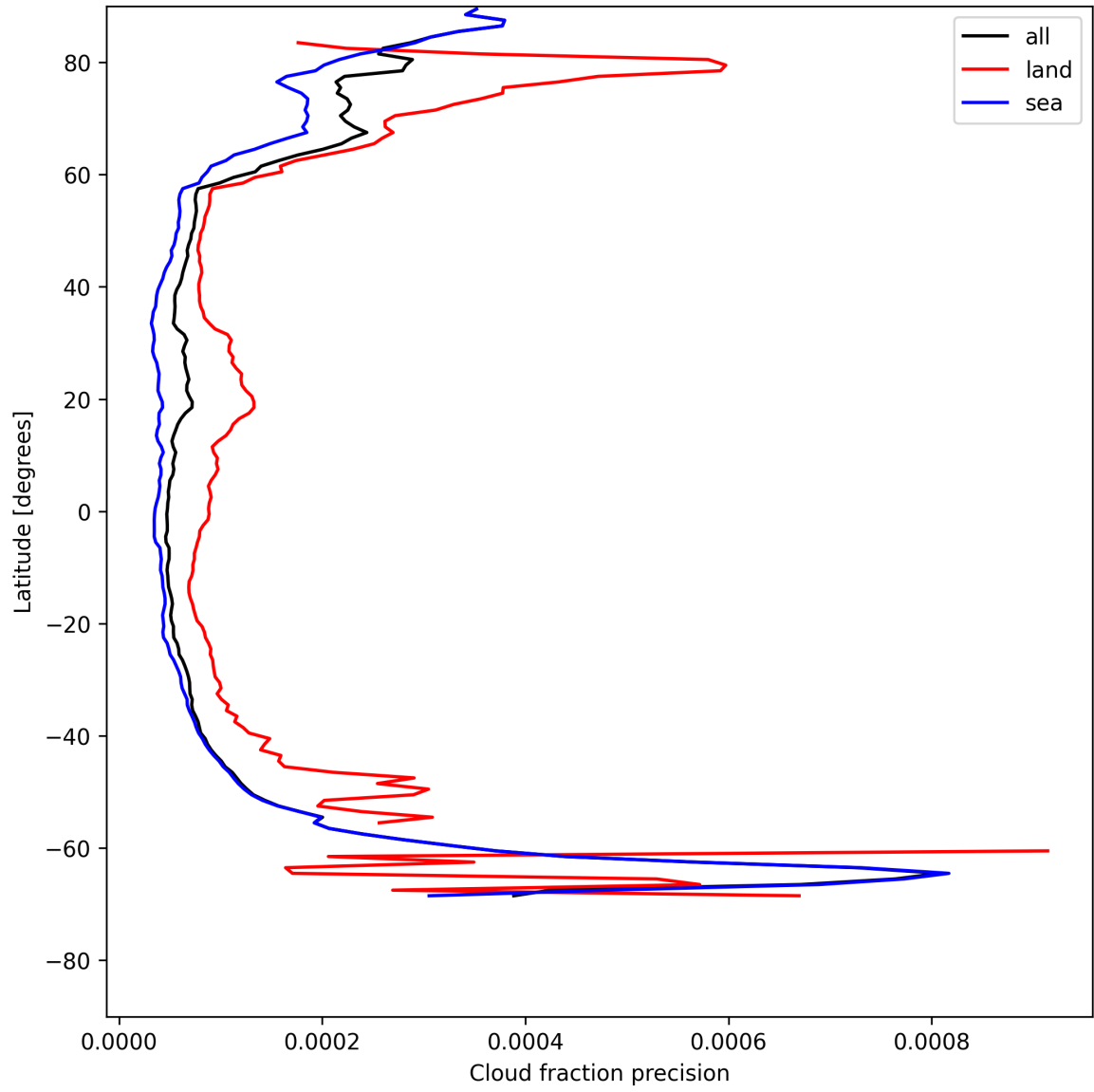
Figure 14: Zonal average of “Cloud fraction precision” for 2025-07-27 to 2025-07-27.
