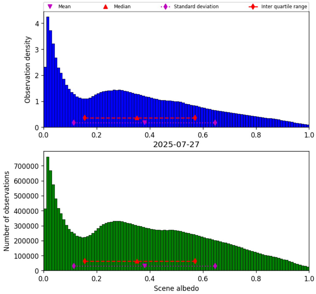
Figure 32: Histogram of “Scene albedo” for 2025-07-27 to 2025-07-27
