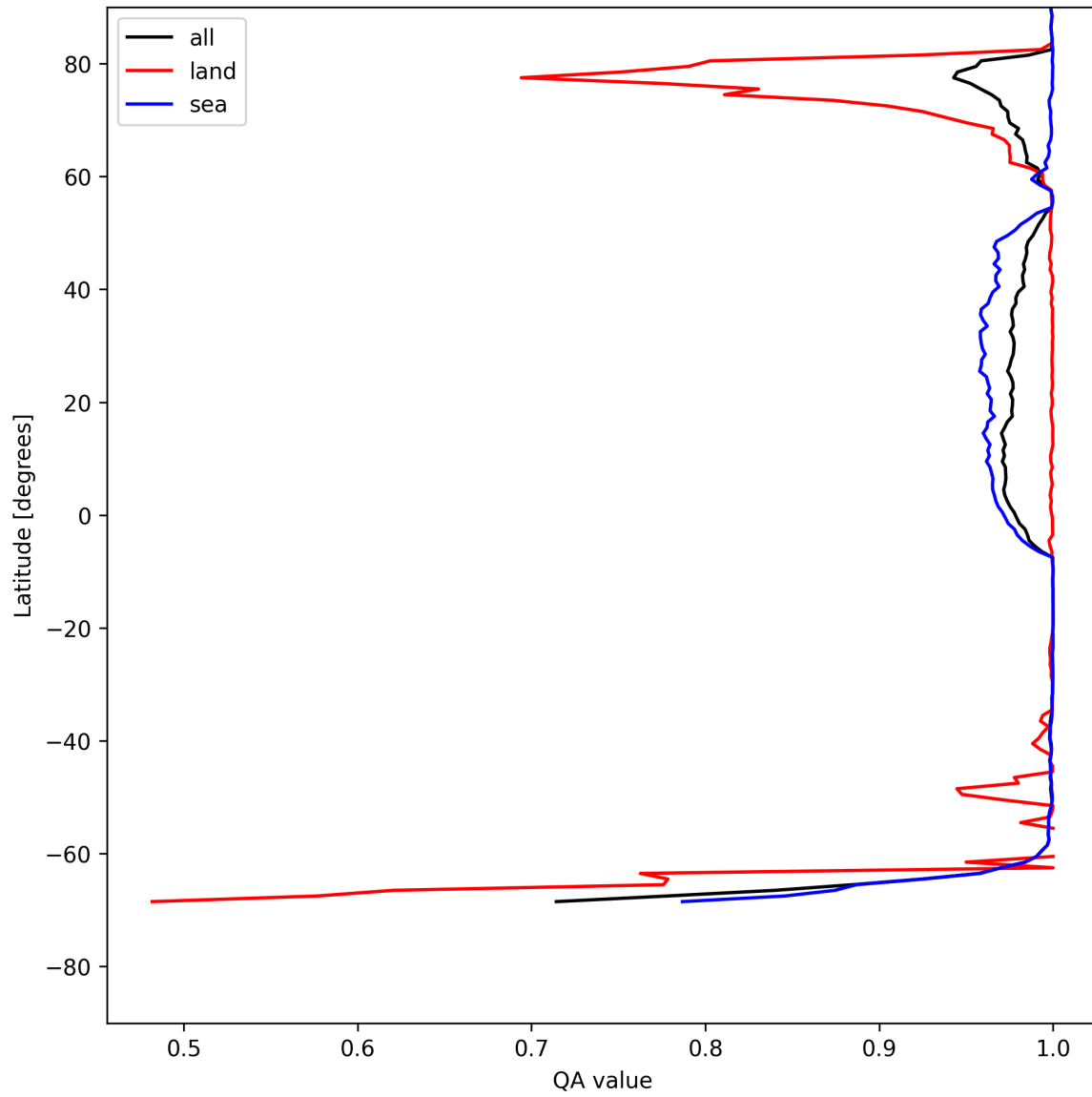
Figure 10: Zonal average of “QA value” for 2025-07-27 to 2025-07-27.
