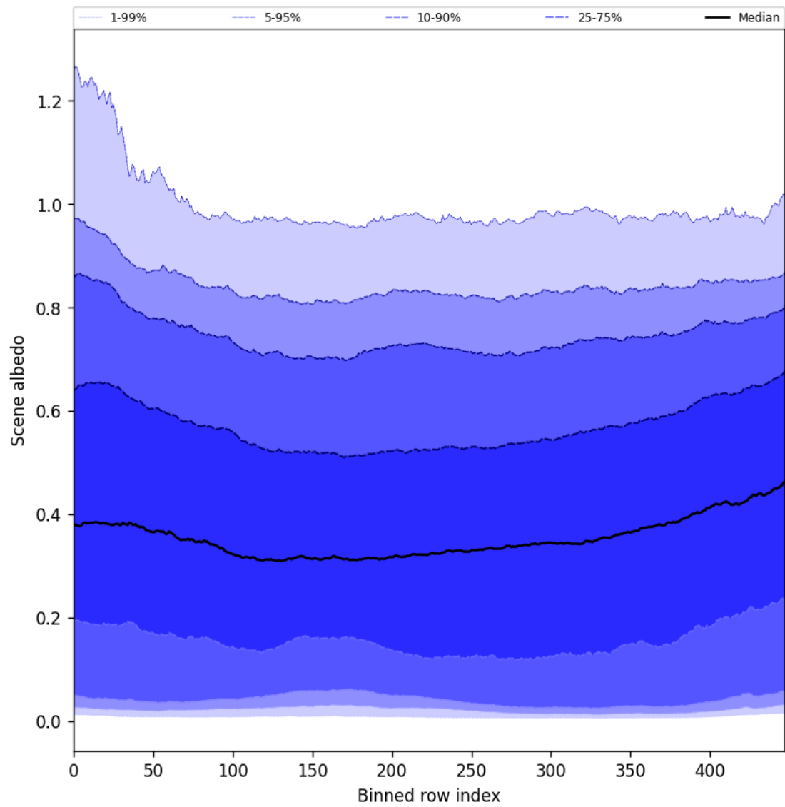
Figure 49: Along track statistics of “Scene albedo” for 2025-07-27 to 2025-07-27
