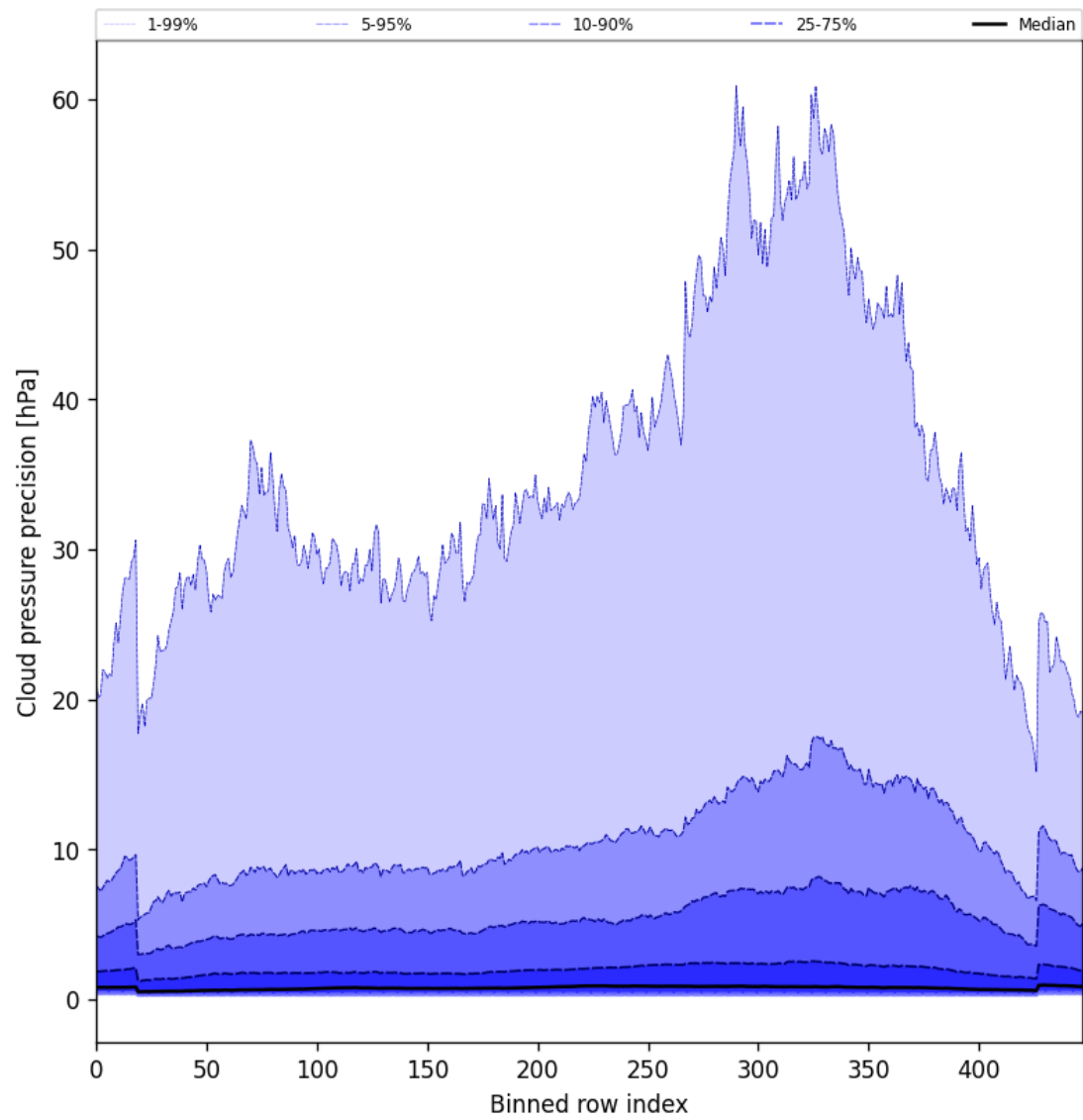
Figure 46: Along track statistics of “Cloud pressure precision” for 2025-07-27 to 2025-07-27
