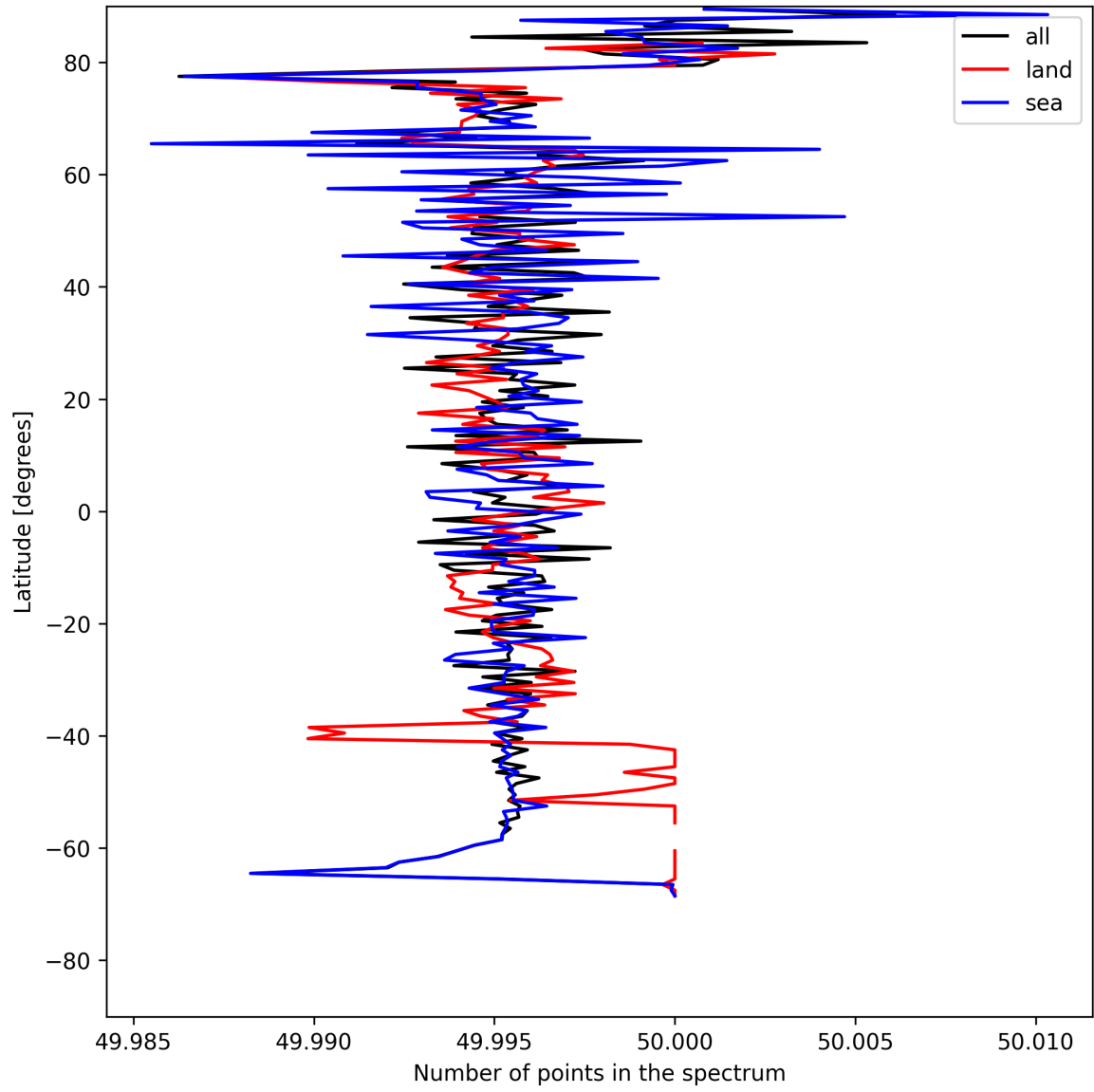
Figure 25: Zonal average of “Number of points in the spectrum” for 2025-07-27 to 2025-07-27.
