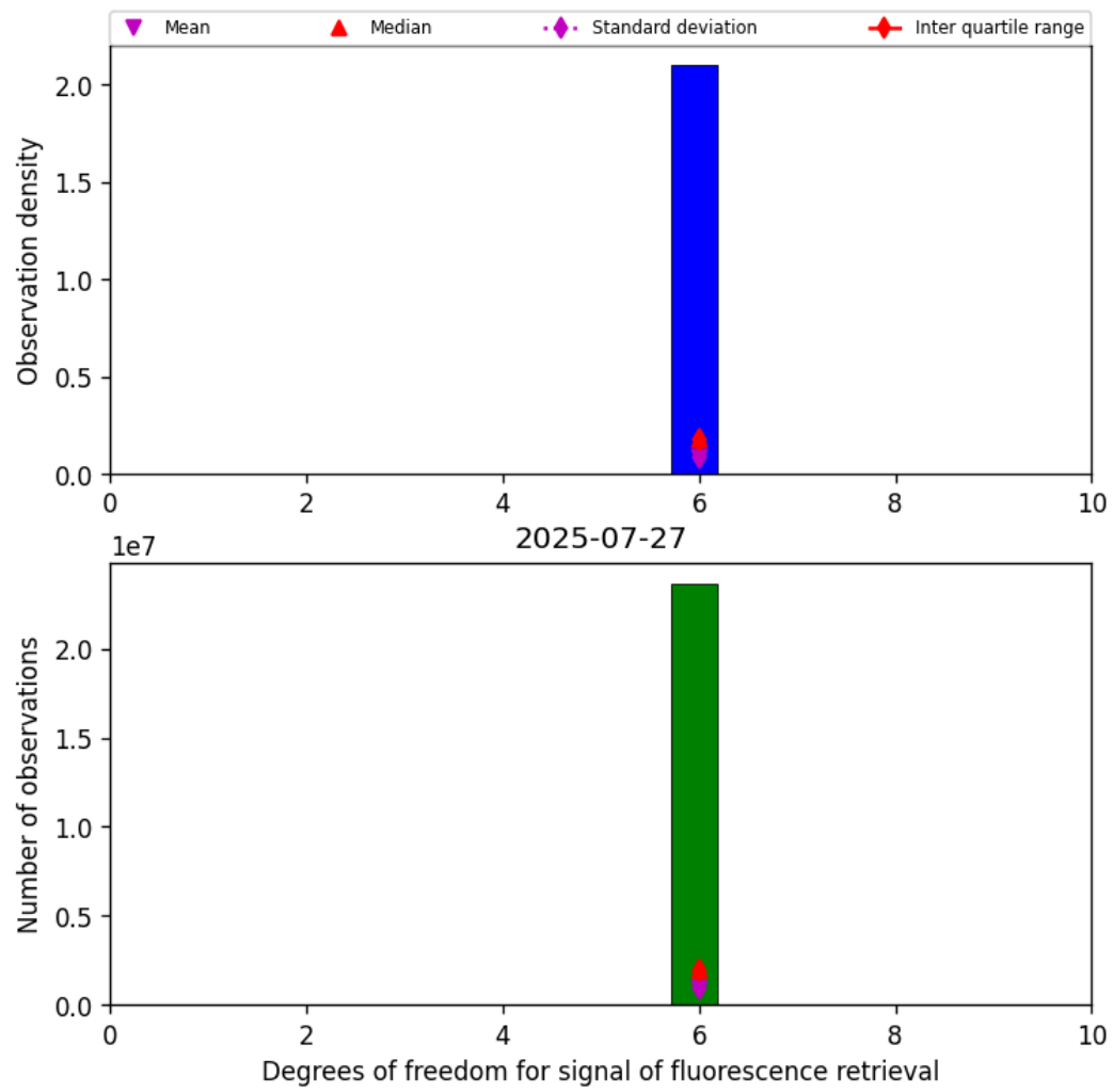
Figure 41: Histogram of “Degrees of freedom for signal of fluorescence retrieval” for 2025-07-27 to 2025-07-27
