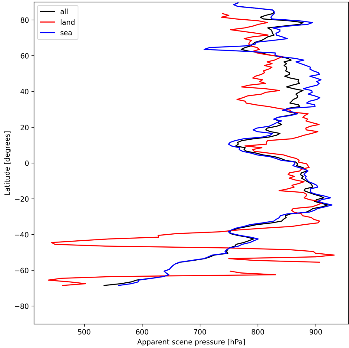
Figure 17: Zonal average of “Apparent scene pressure” for 2025-07-28 to 2025-07-29.
