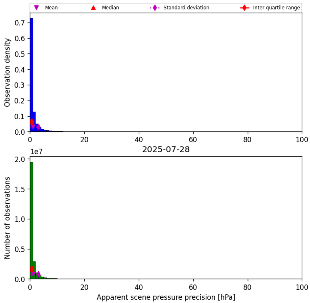
Figure 35: Histogram of “Apparent scene pressure precision” for 2025-07-28 to 2025-07-29
