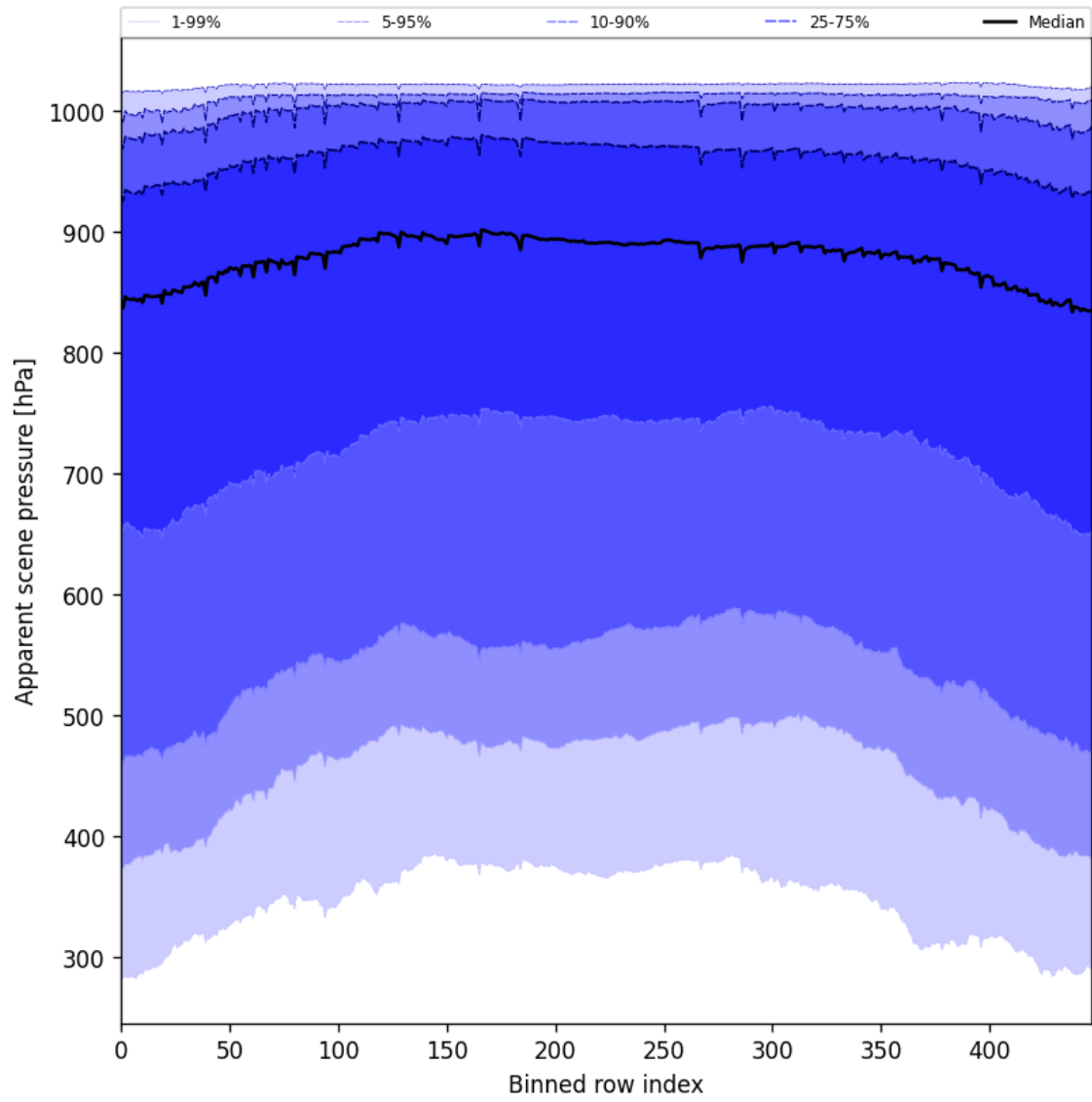
Figure 51: Along track statistics of “Apparent scene pressure” for 2025-07-28 to 2025-07-29
