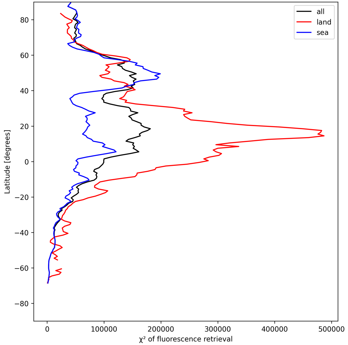
Figure 23: Zonal average of “ \chi^2 of fluorescence retrieval” for 2025-07-28 to 2025-07-29.
