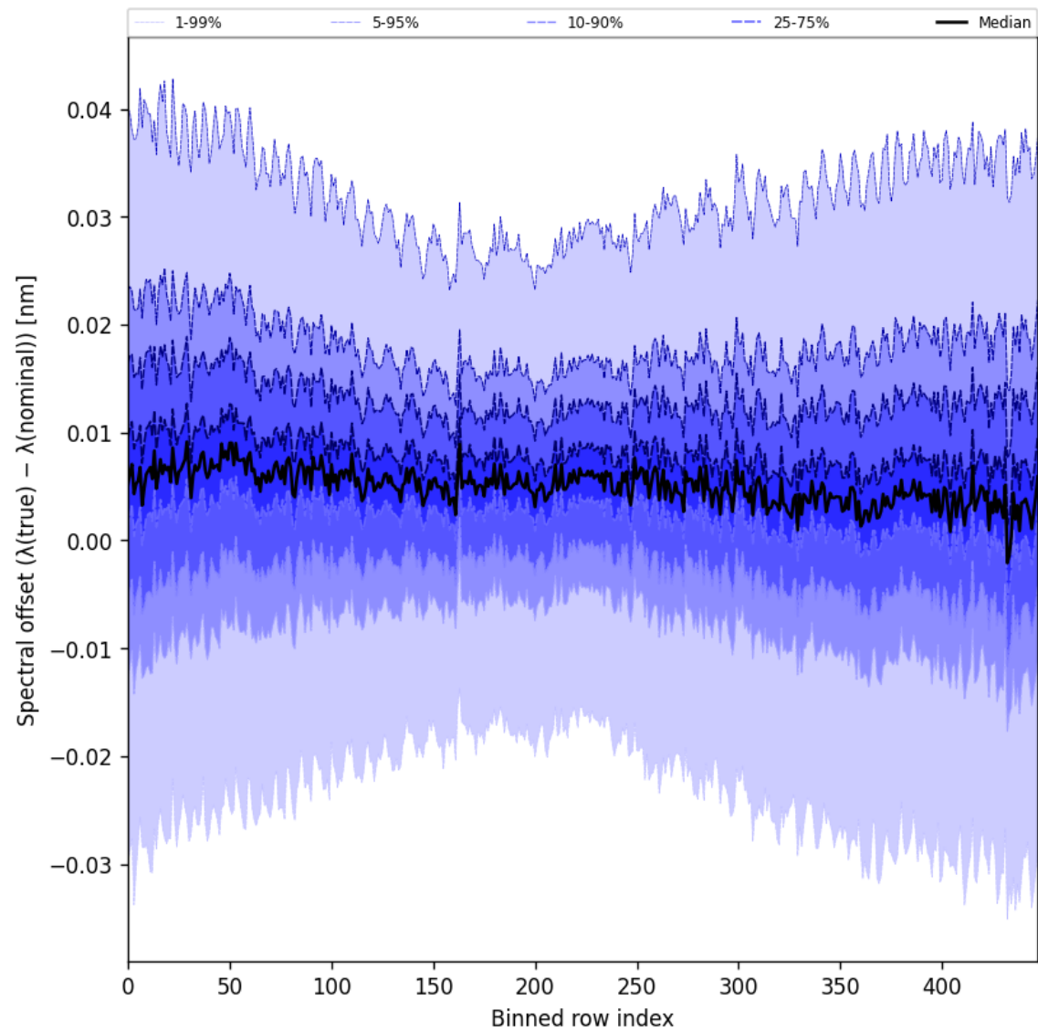
Figure 60: Along track statistics of “Spectral offset ( \lambda_{\text{true}} - \lambda_{\text{nominal}} )” for 2025-07-28 to 2025-07-29
