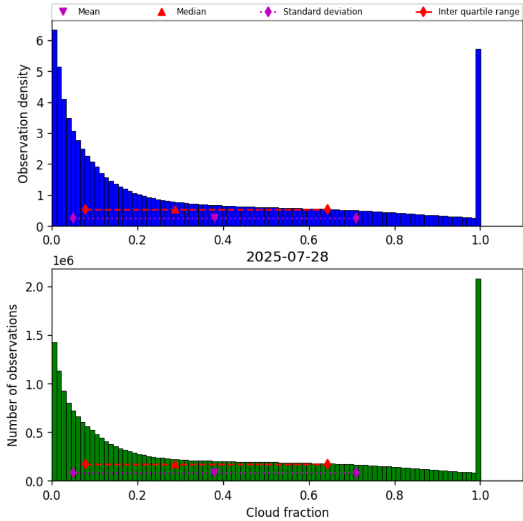
Figure 30: Histogram of “Cloud fraction” for 2025-07-28 to 2025-07-29
