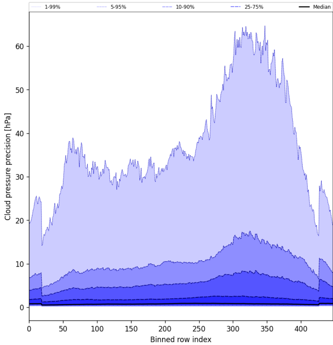
Figure 46: Along track statistics of “Cloud pressure precision” for 2025-07-28 to 2025-07-29
