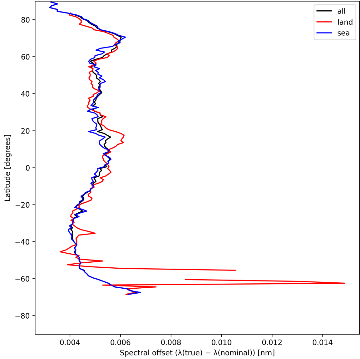
Figure 26: Zonal average of “Spectral offset ( \lambda_{\text{true}} - \lambda_{\text{nominal}} )” for 2025-07-28 to 2025-07-29.
