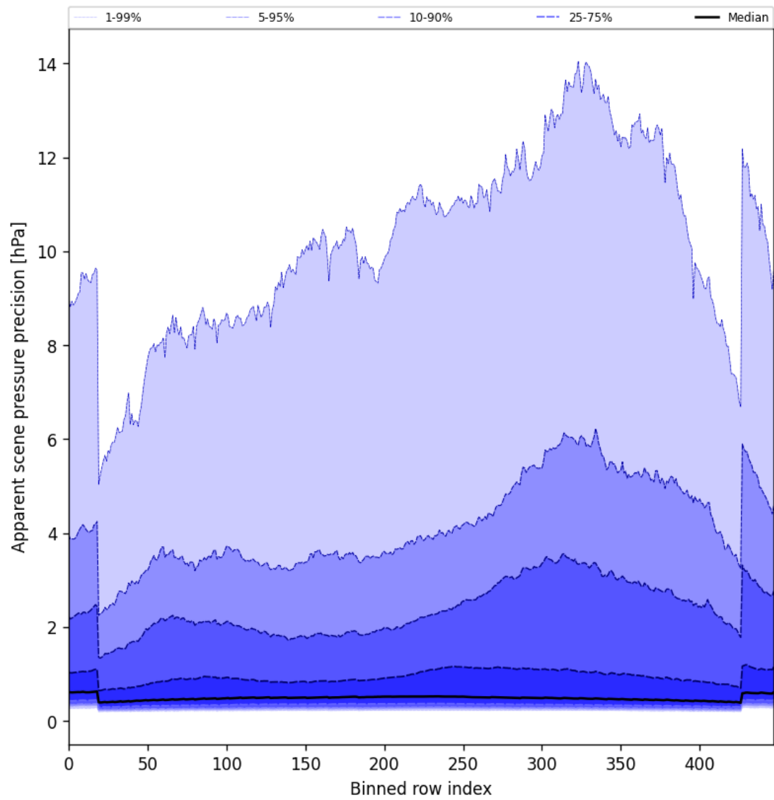
Figure 52: Along track statistics of “Apparent scene pressure precision” for 2025-07-28 to 2025-07-29
