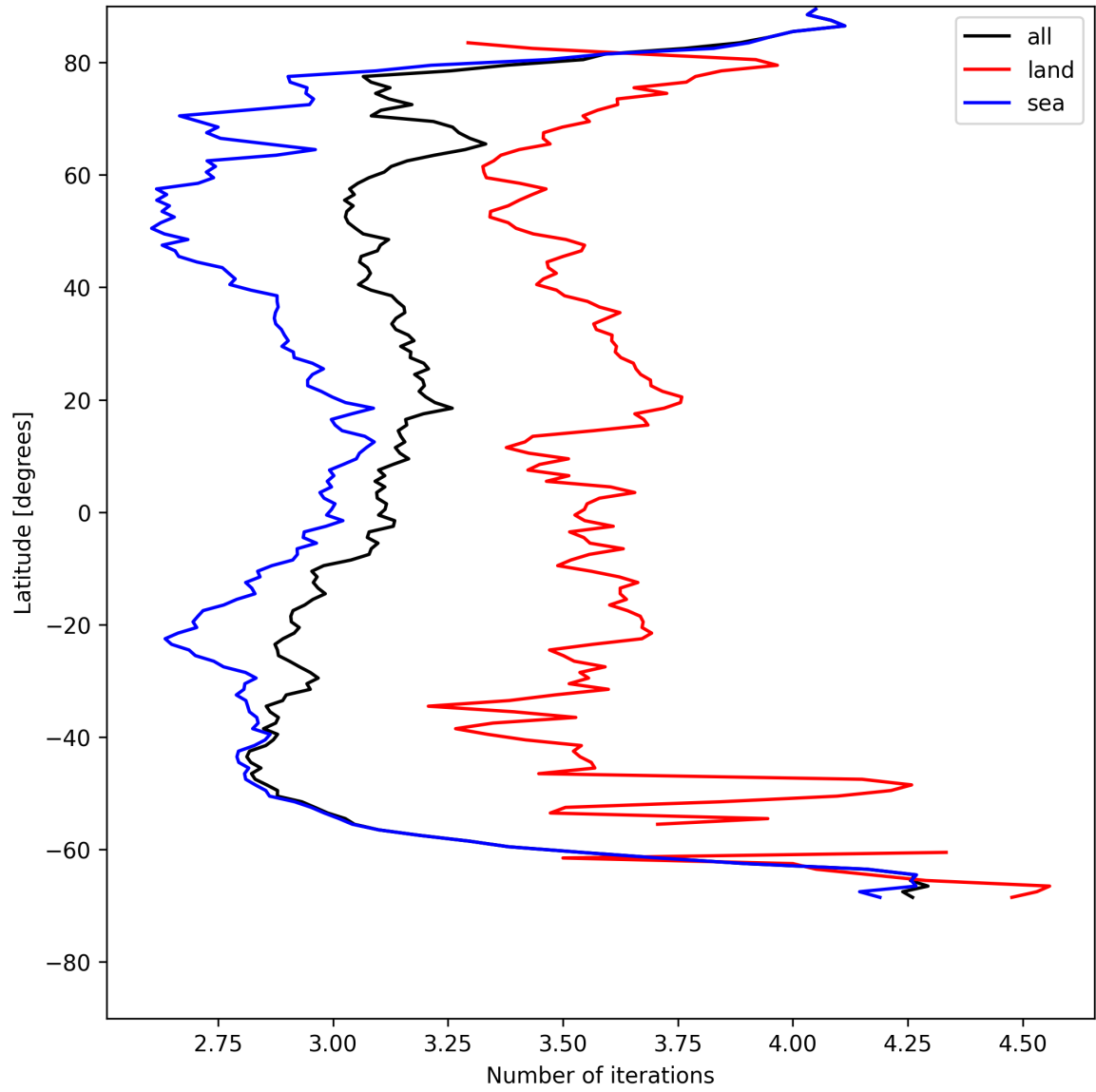
Figure 20: Zonal average of “Number of iterations” for 2025-07-28 to 2025-07-29.
