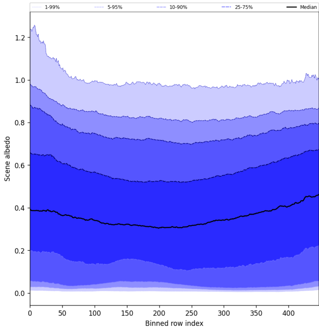
Figure 49: Along track statistics of “Scene albedo” for 2025-07-28 to 2025-07-29
