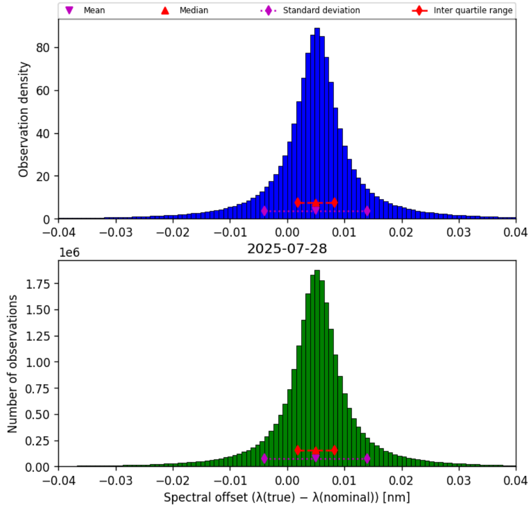
Figure 43: Histogram of “Spectral offset ( \lambda_{\text{true}} - \lambda_{\text{nominal}} )” for 2025-07-28 to 2025-07-29
