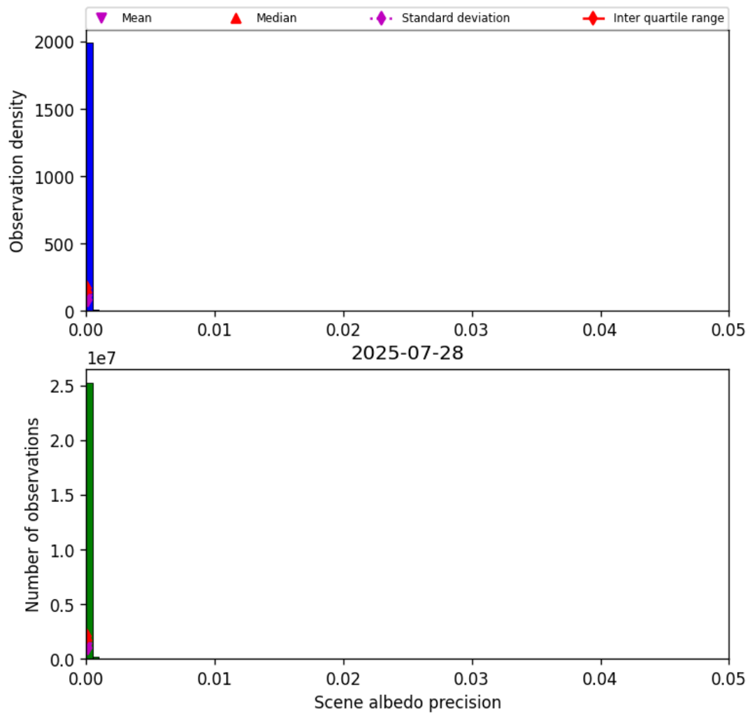
Figure 33: Histogram of “Scene albedo precision” for 2025-07-28 to 2025-07-29
