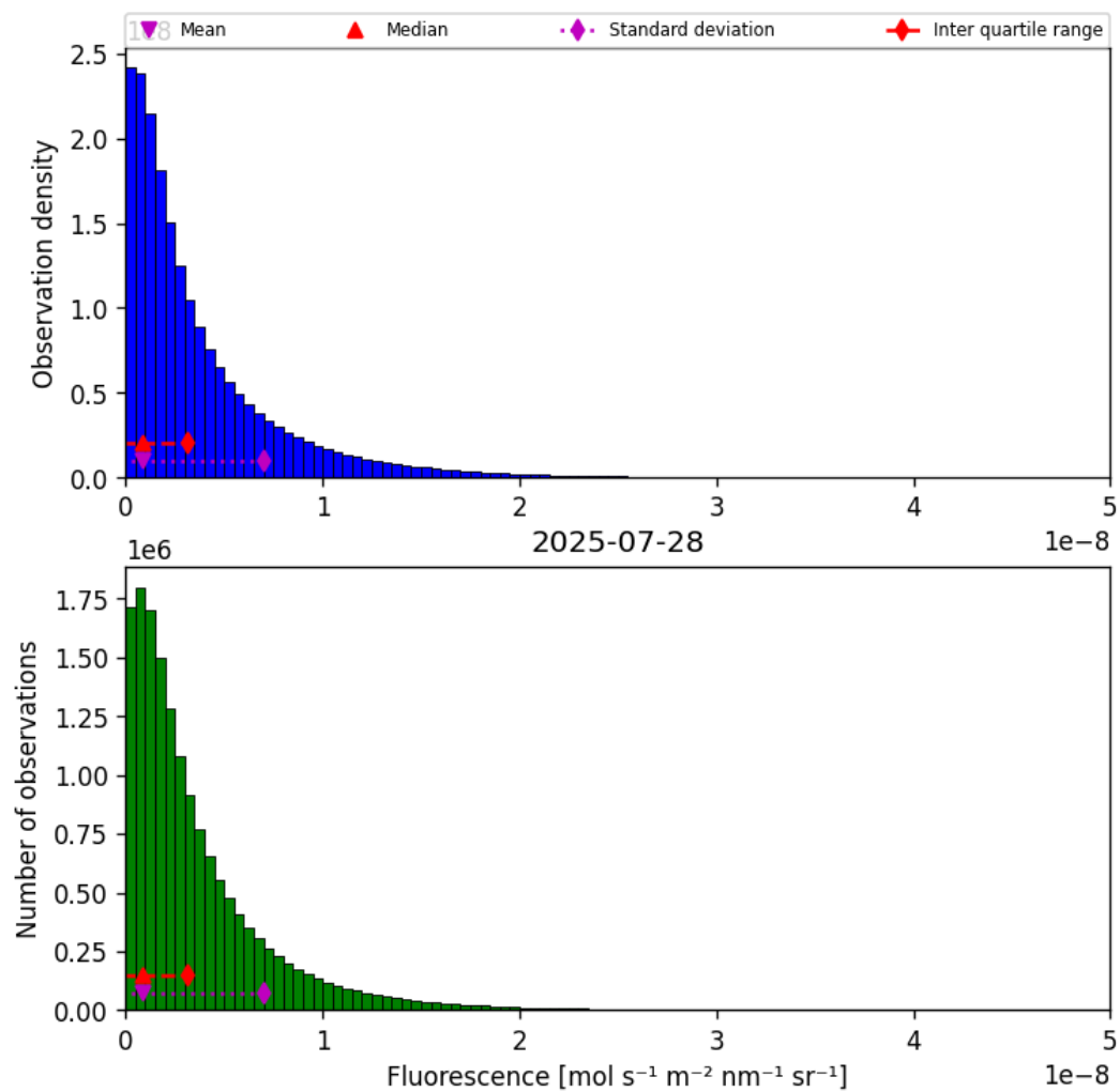
Figure 38: Histogram of “Fluorescence” for 2025-07-28 to 2025-07-29
