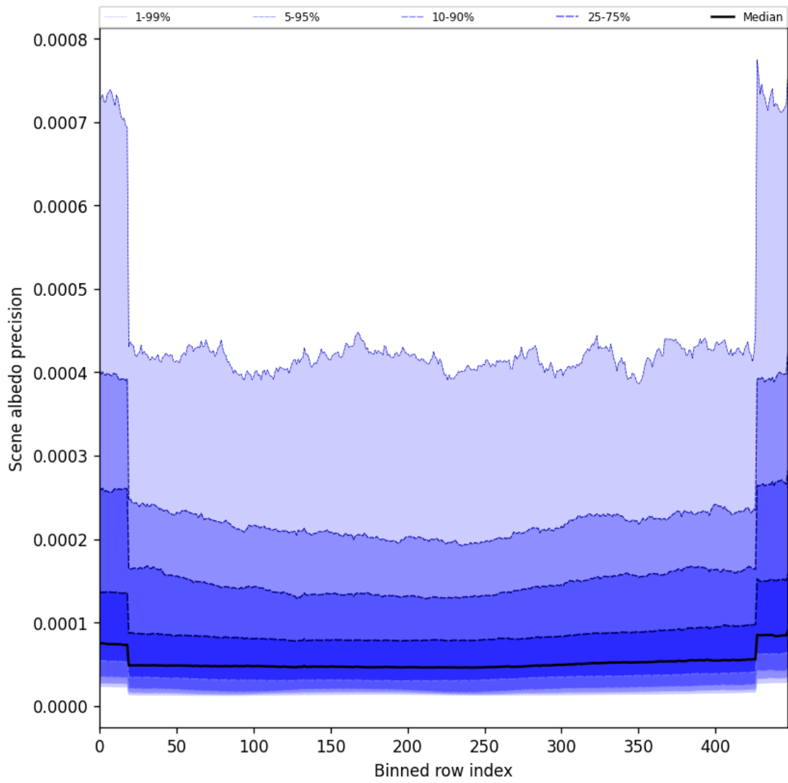
Figure 50: Along track statistics of “Scene albedo precision” for 2025-07-28 to 2025-07-29
