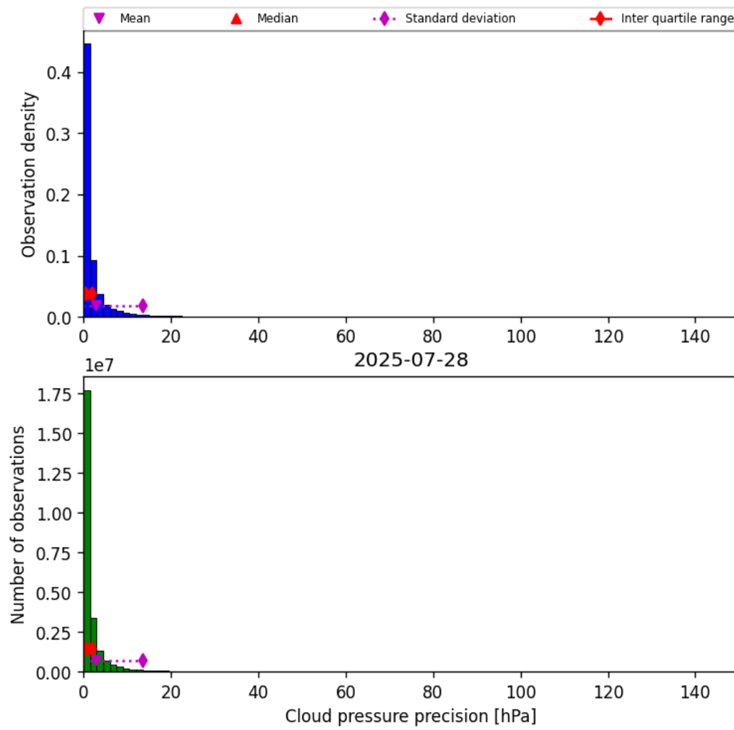
Figure 29: Histogram of “Cloud pressure precision” for 2025-07-28 to 2025-07-29
