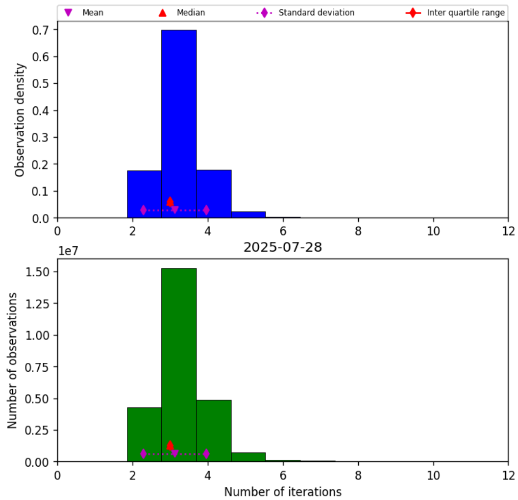
Figure 37: Histogram of “Number of iterations” for 2025-07-28 to 2025-07-29
