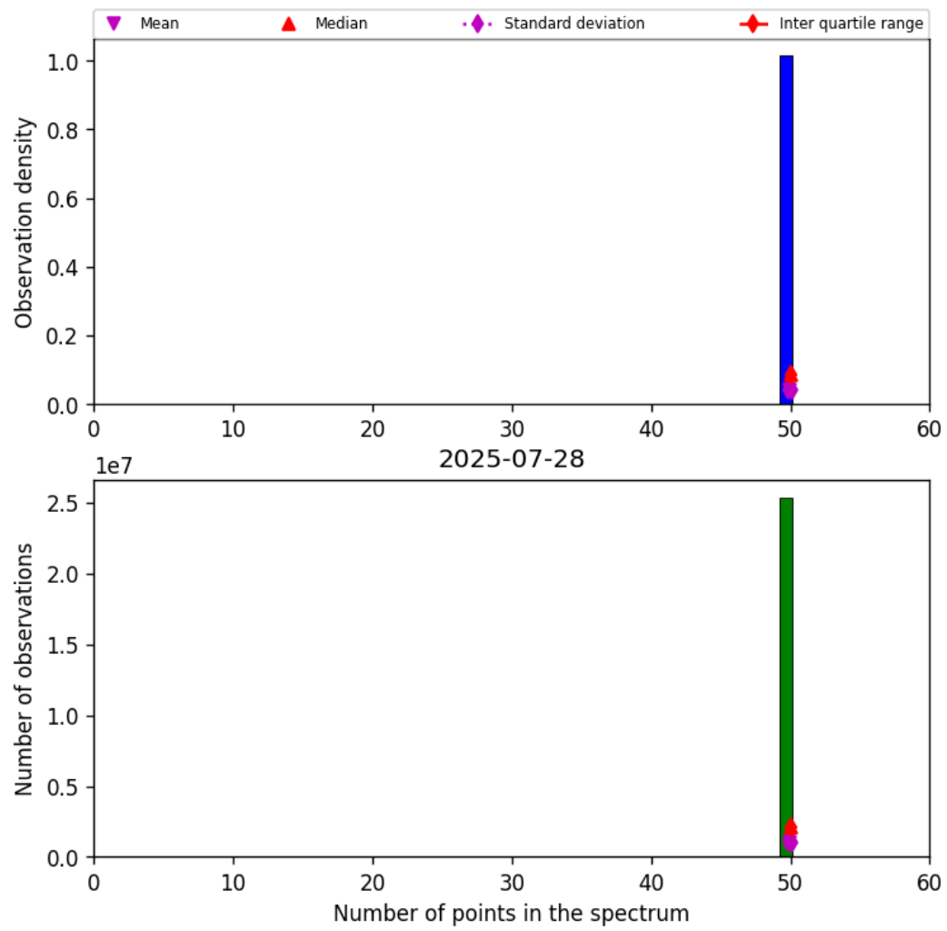
Figure 42: Histogram of “Number of points in the spectrum” for 2025-07-28 to 2025-07-29
