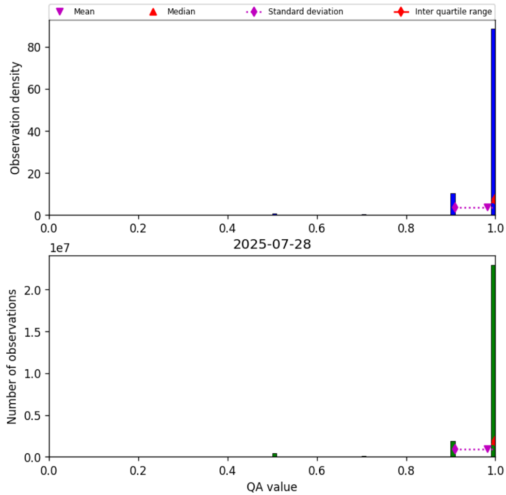
Figure 27: Histogram of “QA value” for 2025-07-28 to 2025-07-29
