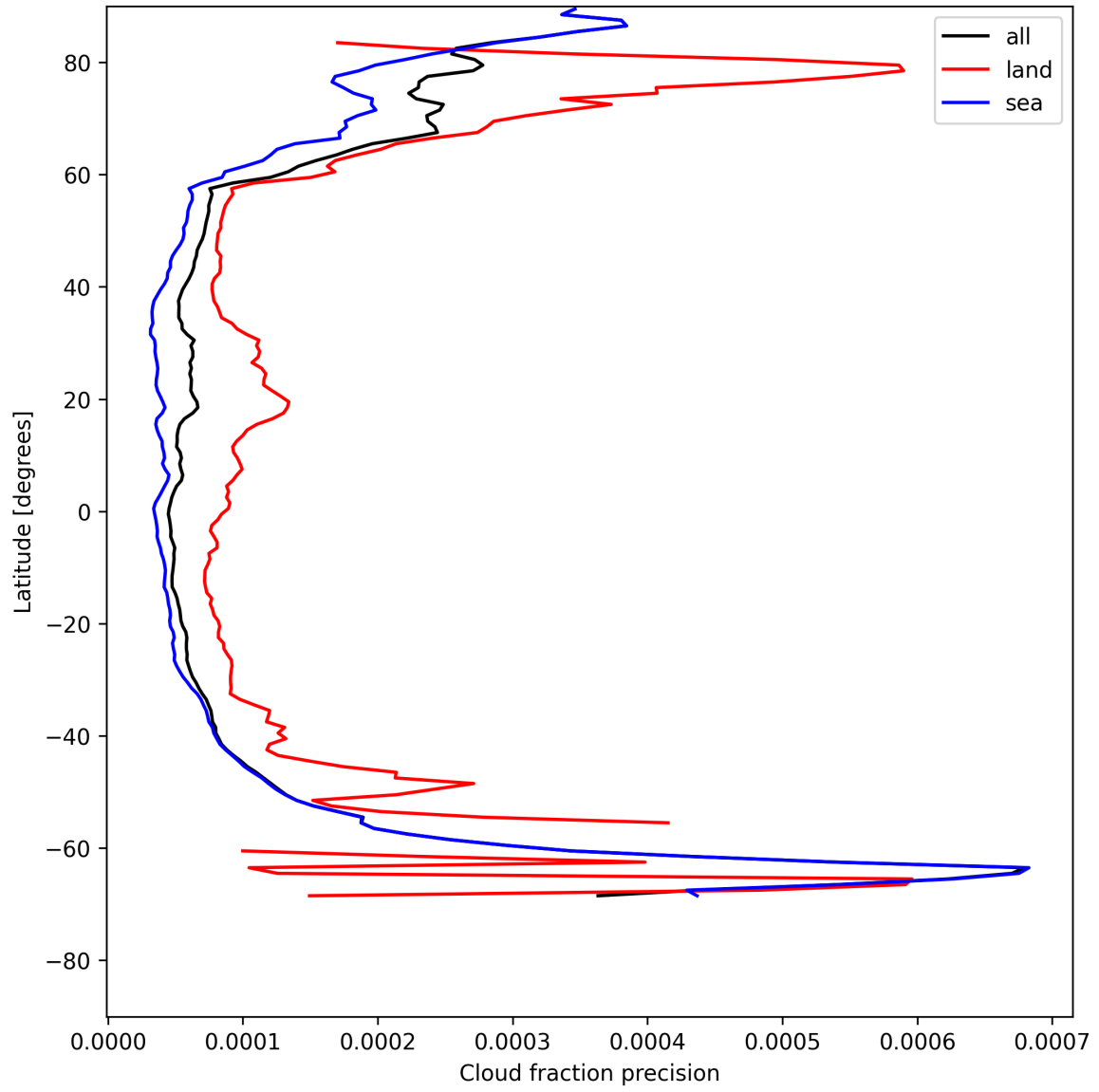
Figure 14: Zonal average of “Cloud fraction precision” for 2025-07-28 to 2025-07-29.
