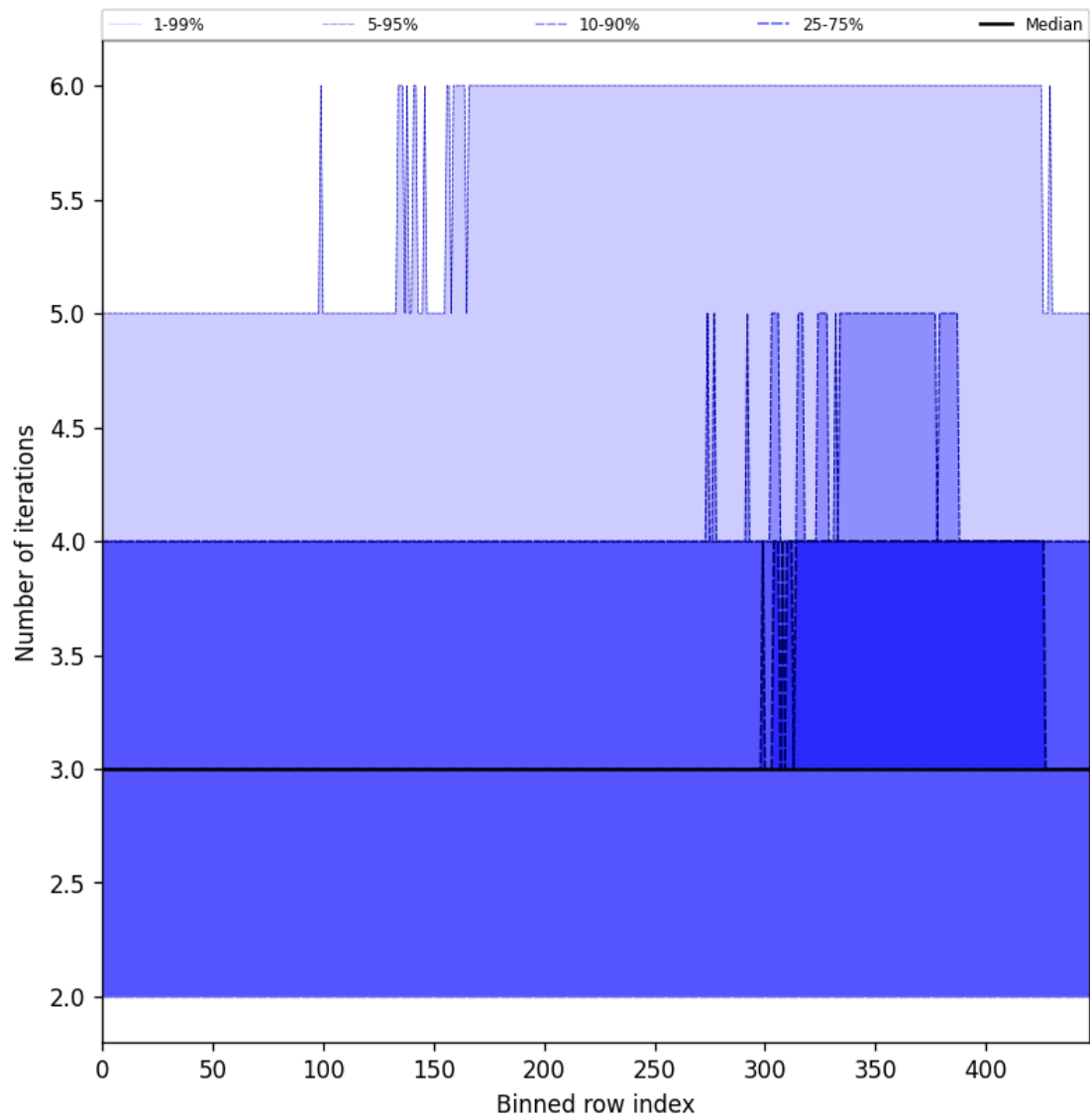
Figure 54: Along track statistics of “Number of iterations” for 2025-07-28 to 2025-07-29
