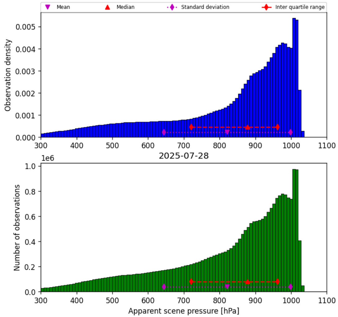
Figure 34: Histogram of “Apparent scene pressure” for 2025-07-28 to 2025-07-29
