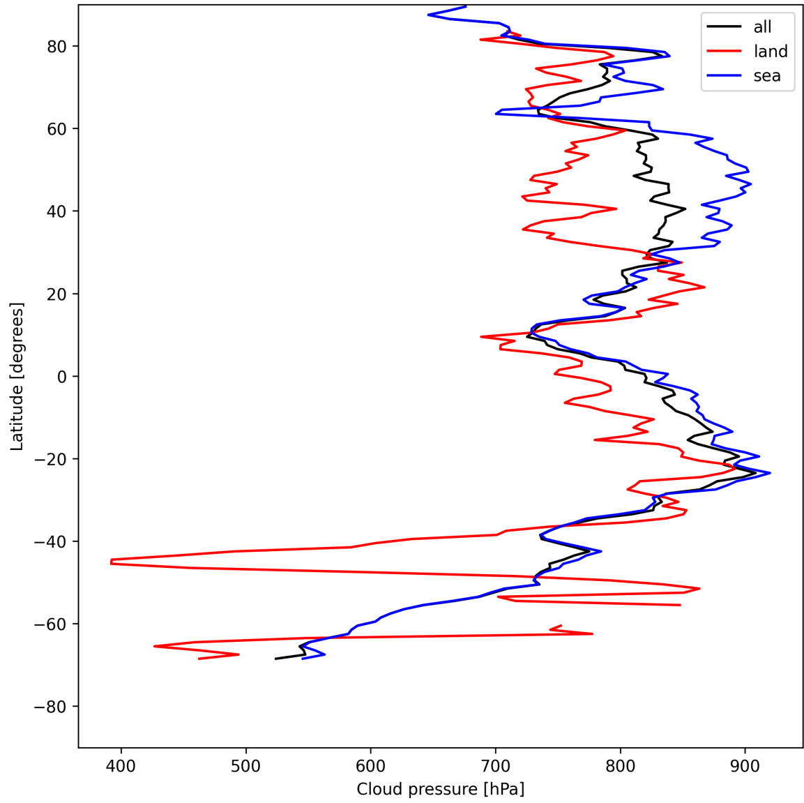
Figure 11: Zonal average of “Cloud pressure” for 2025-07-28 to 2025-07-29.
