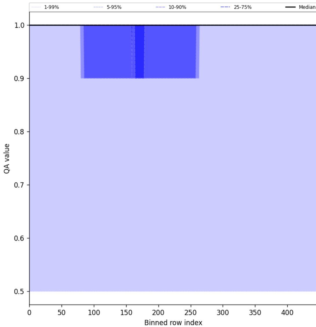
Figure 44: Along track statistics of “QA value” for 2025-07-28 to 2025-07-29
