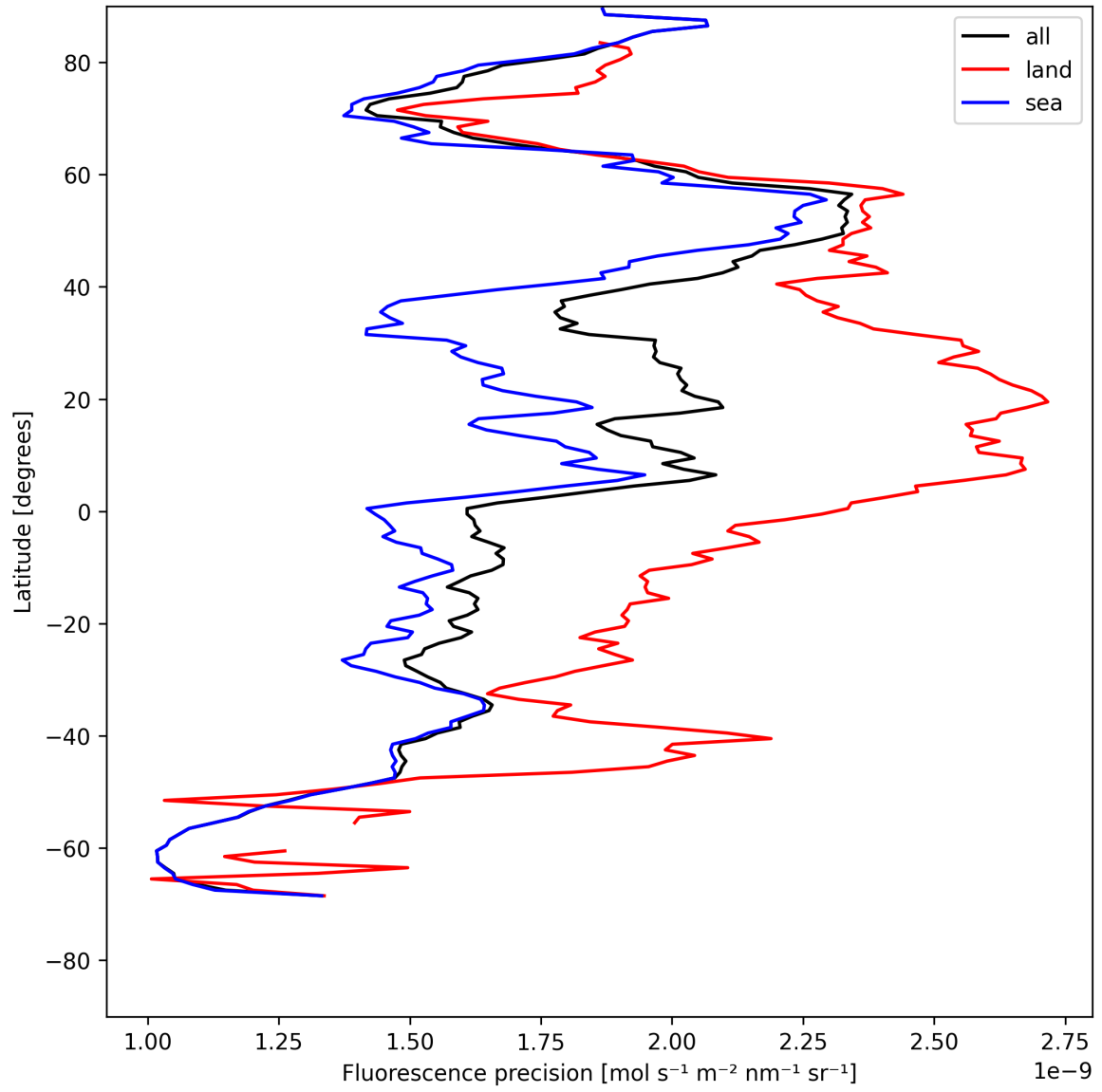
Figure 22: Zonal average of “Fluorescence precision” for 2025-07-28 to 2025-07-29.
