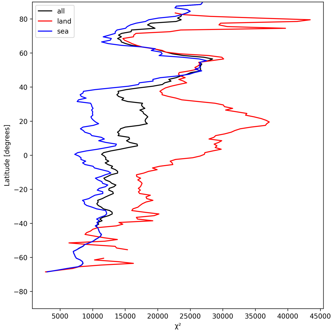
Figure 19: Zonal average of “ \chi^2 ” for 2025-07-28 to 2025-07-29.
