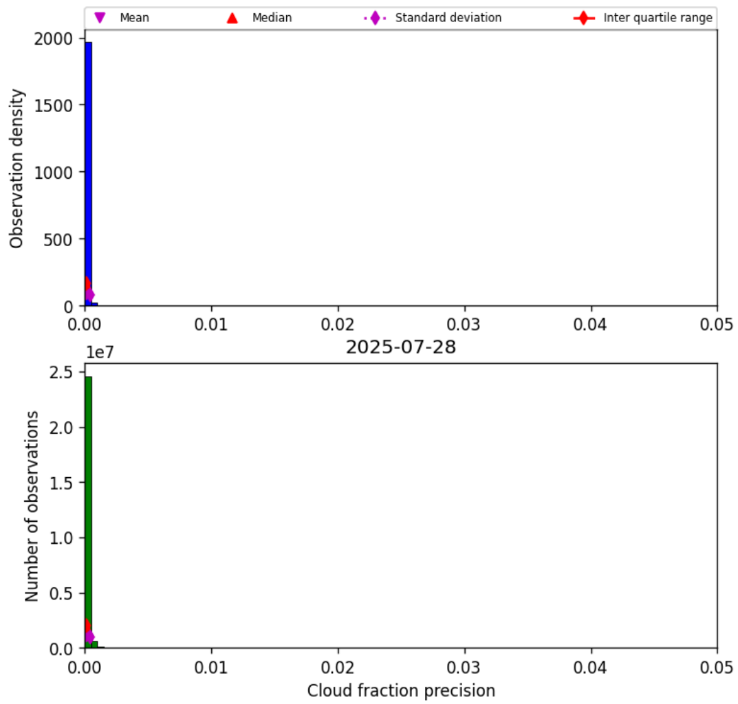
Figure 31: Histogram of “Cloud fraction precision” for 2025-07-28 to 2025-07-29
