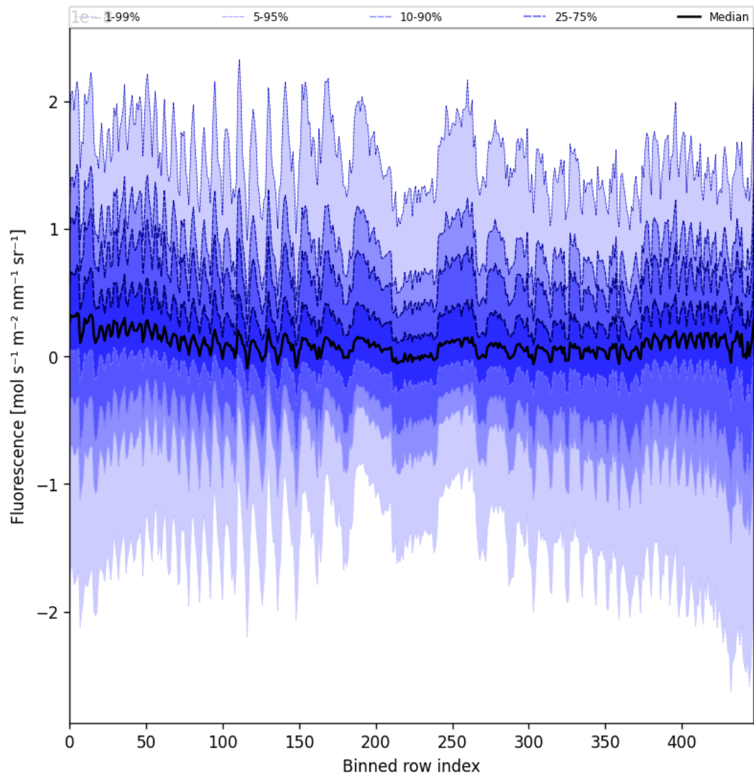
Figure 55: Along track statistics of “Fluorescence” for 2025-07-28 to 2025-07-29
