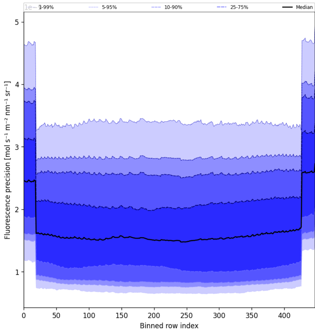
Figure 56: Along track statistics of “Fluorescence precision” for 2025-07-28 to 2025-07-29
