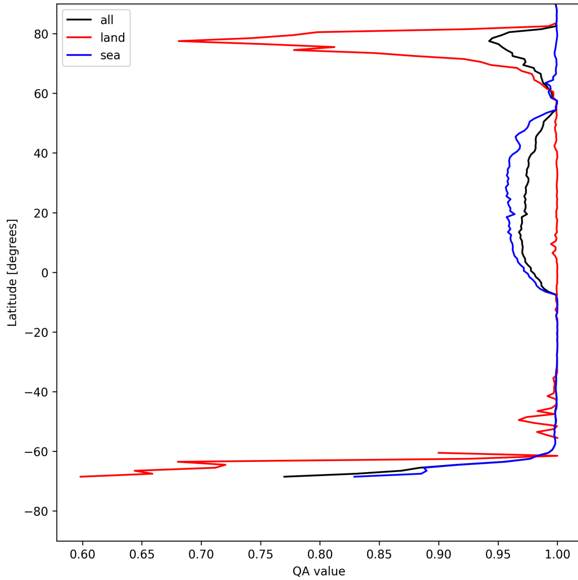
Figure 10: Zonal average of “QA value” for 2025-07-28 to 2025-07-29.
