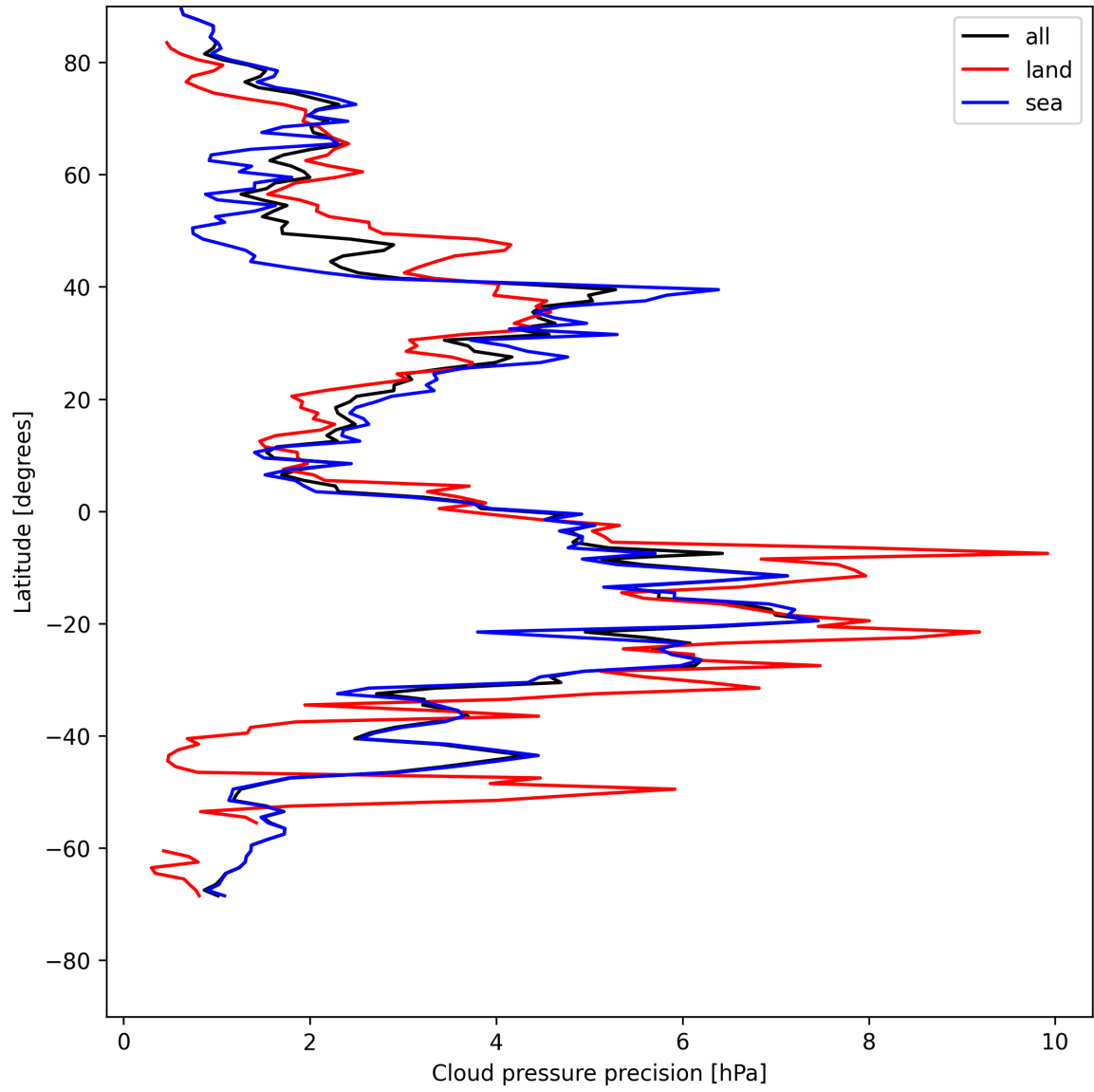
Figure 12: Zonal average of “Cloud pressure precision” for 2025-07-28 to 2025-07-29.
