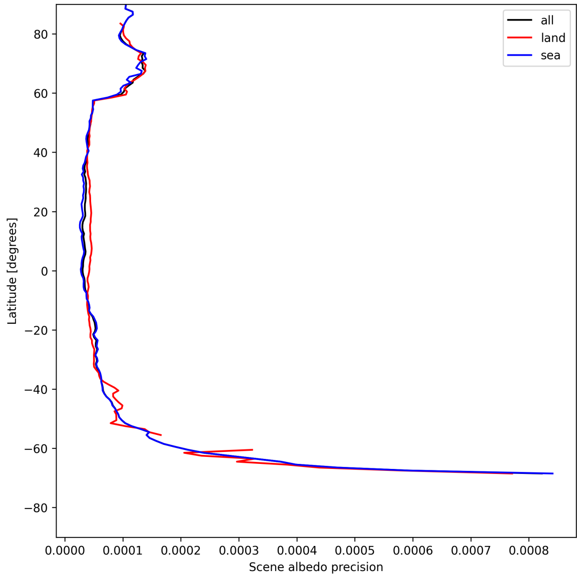
Figure 16: Zonal average of “Scene albedo precision” for 2025-07-28 to 2025-07-29.
