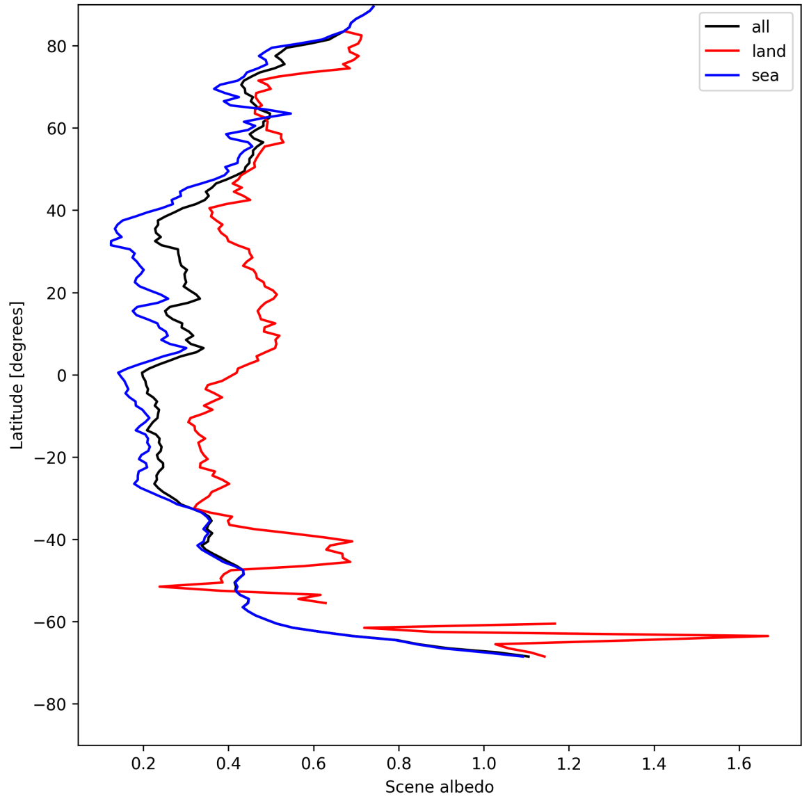
Figure 15: Zonal average of “Scene albedo” for 2025-07-28 to 2025-07-29.
