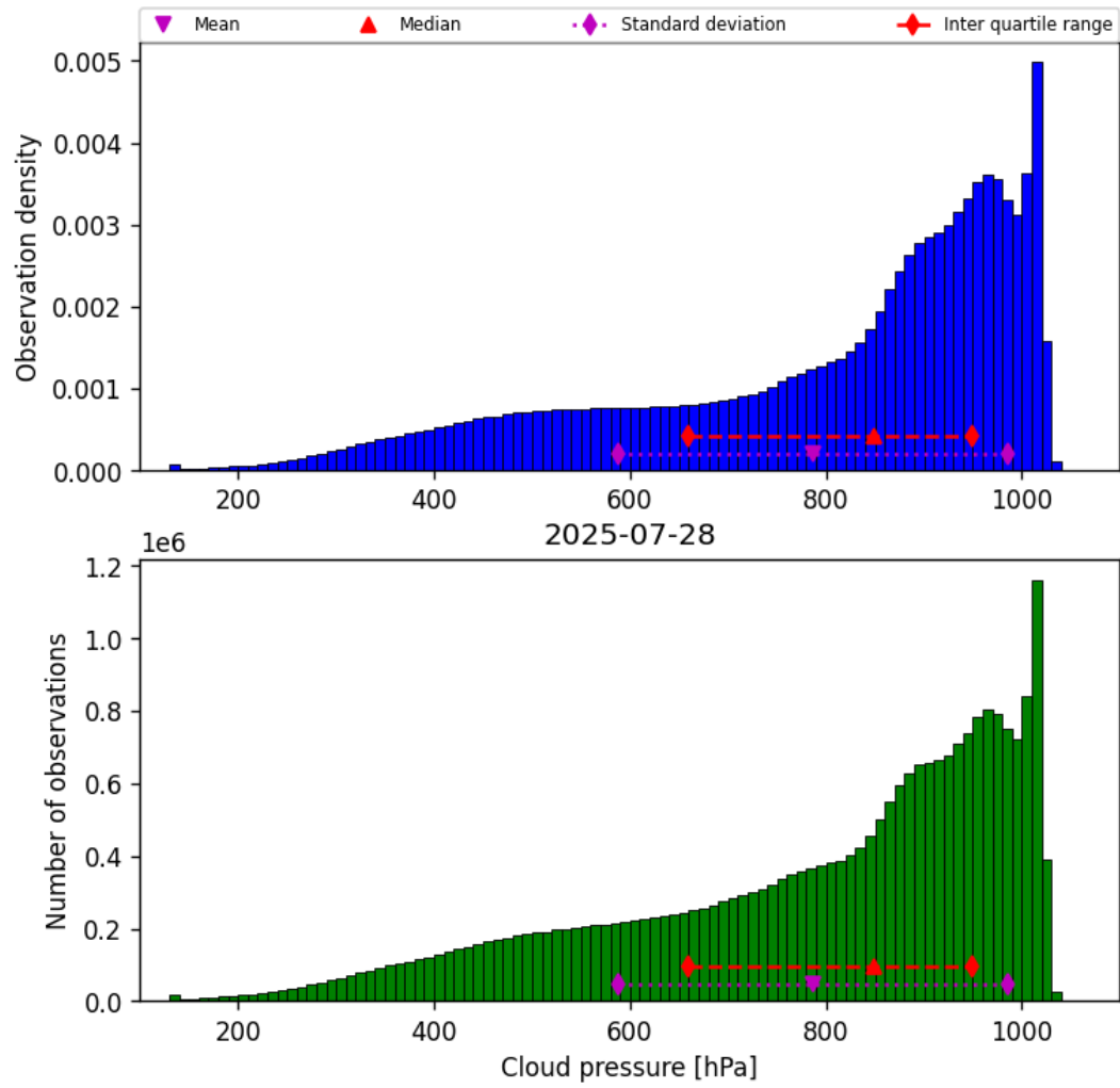
Figure 28: Histogram of “Cloud pressure” for 2025-07-28 to 2025-07-29
