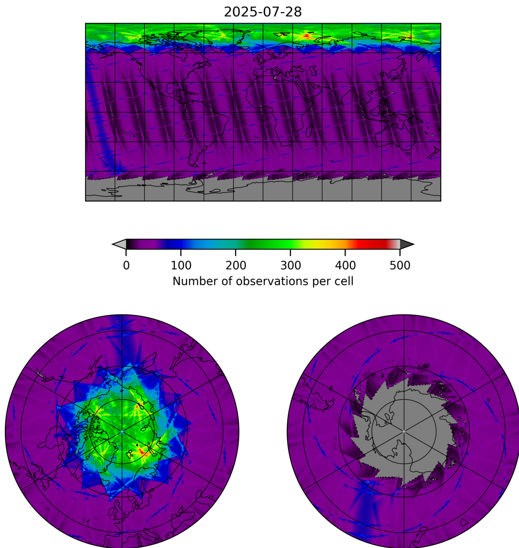
Figure 9: Map of the number of observations for 2025-07-28 to 2025-07-29
