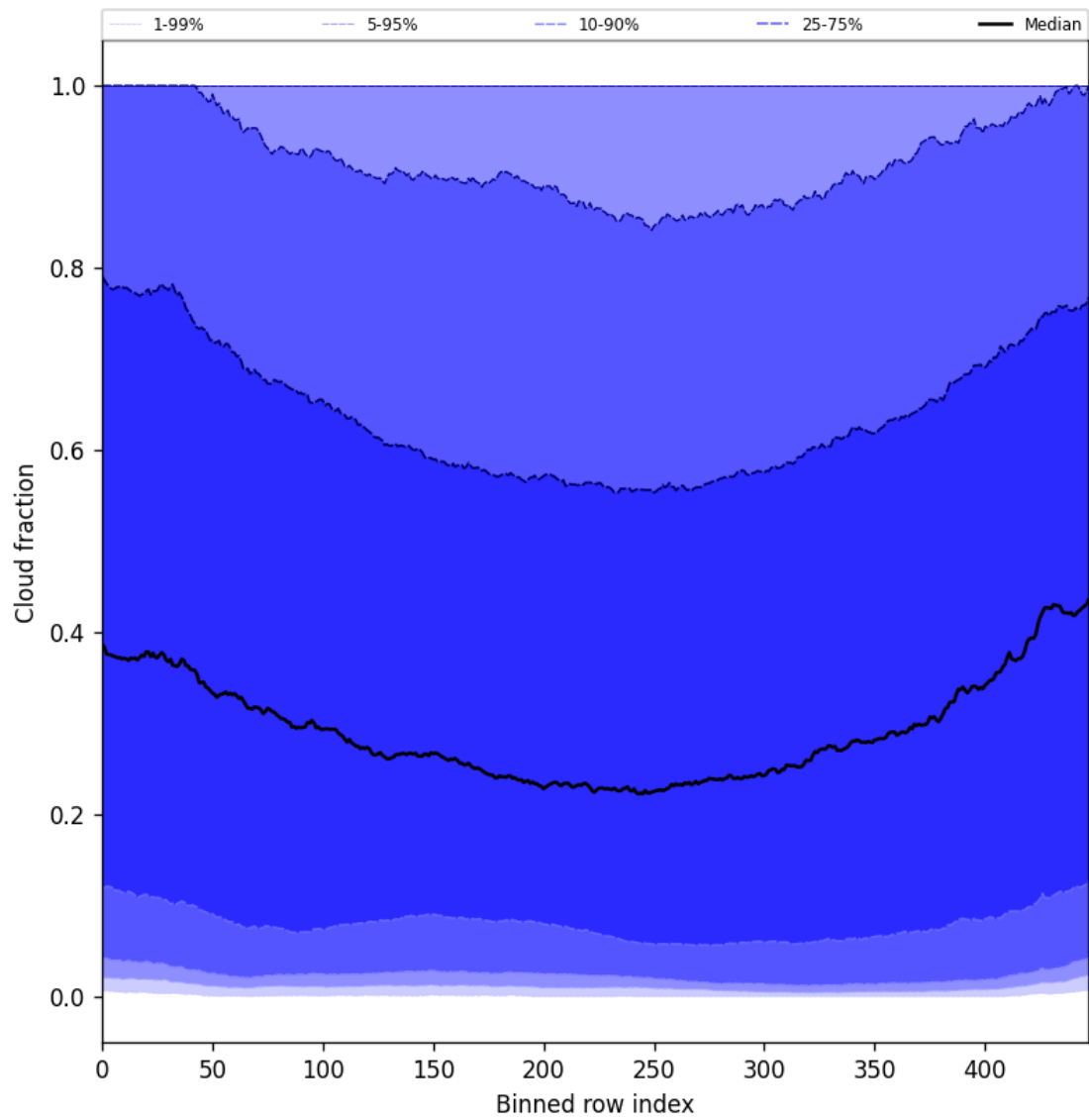
Figure 47: Along track statistics of “Cloud fraction” for 2025-07-28 to 2025-07-29
