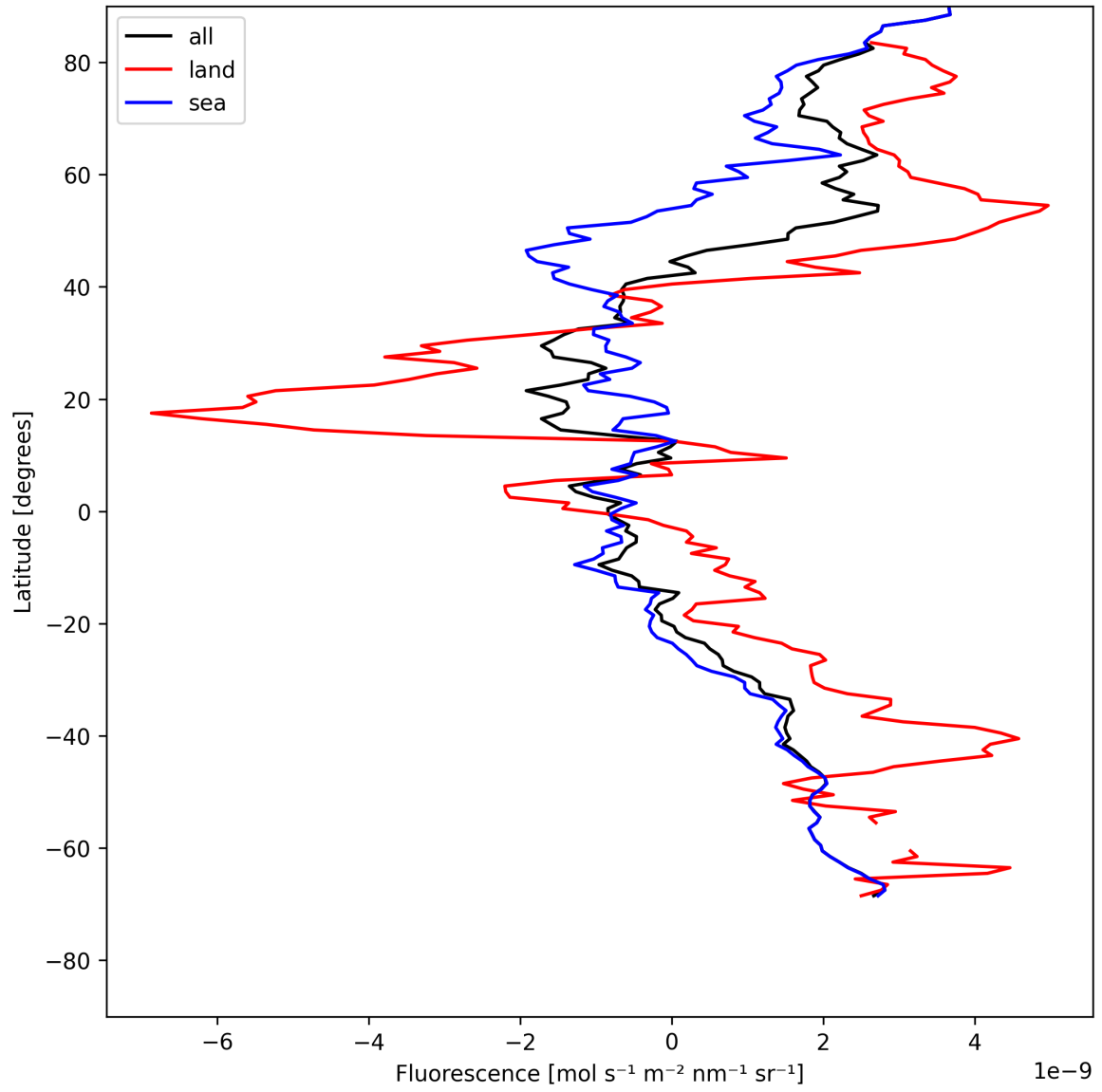
Figure 21: Zonal average of “Fluorescence” for 2025-07-28 to 2025-07-29.
