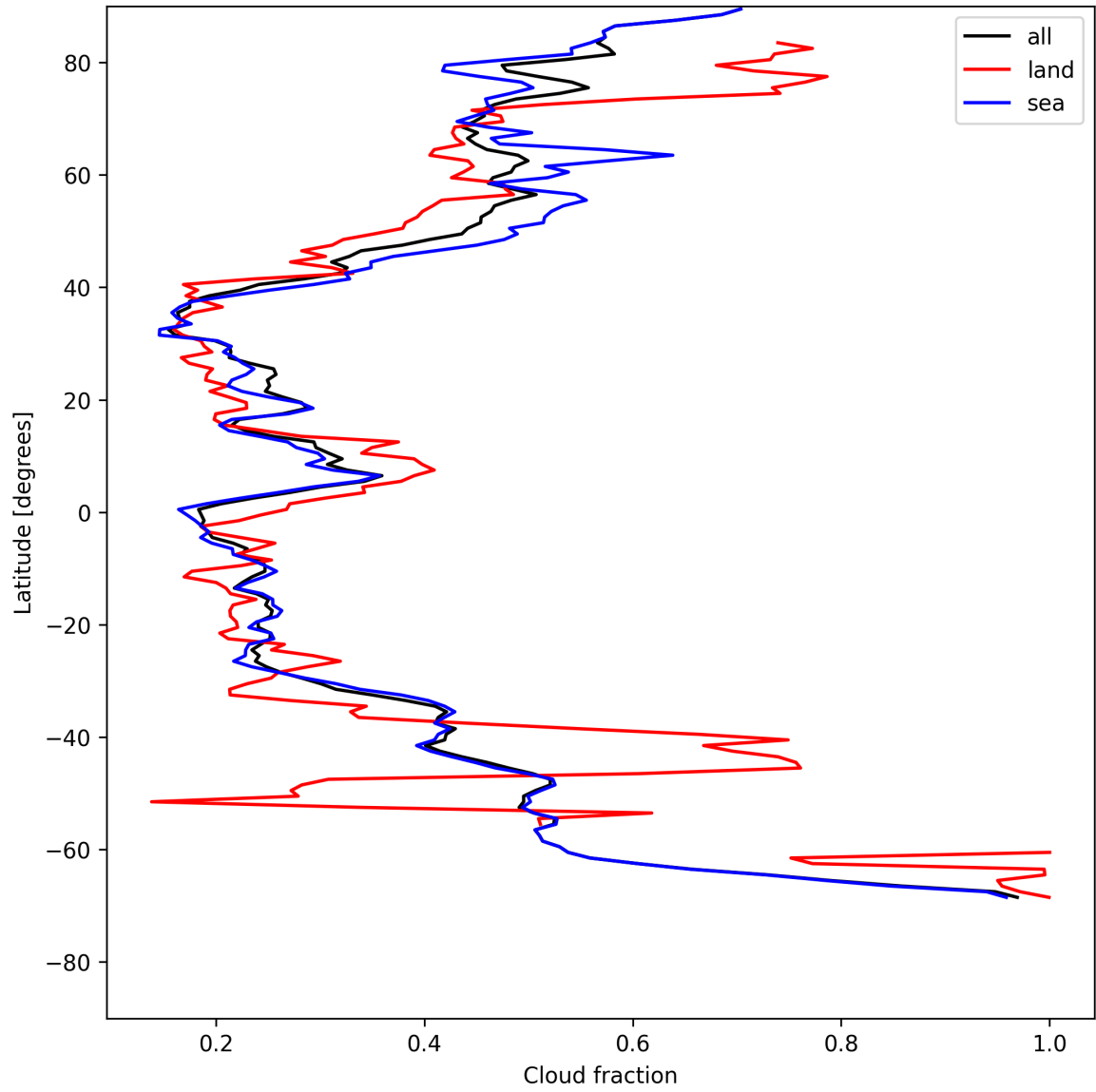
Figure 13: Zonal average of “Cloud fraction” for 2025-07-28 to 2025-07-29.
