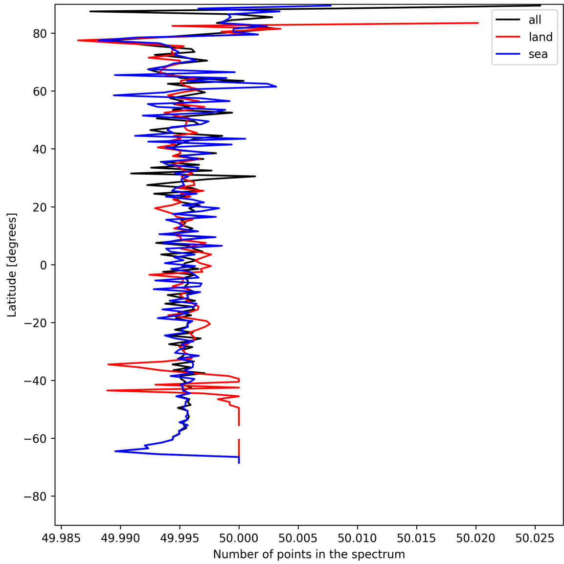
Figure 25: Zonal average of “Number of points in the spectrum” for 2025-07-28 to 2025-07-29.
