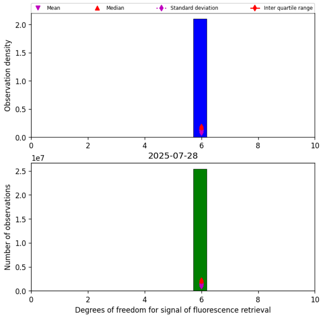
Figure 41: Histogram of “Degrees of freedom for signal of fluorescence retrieval” for 2025-07-28 to 2025-07-29
