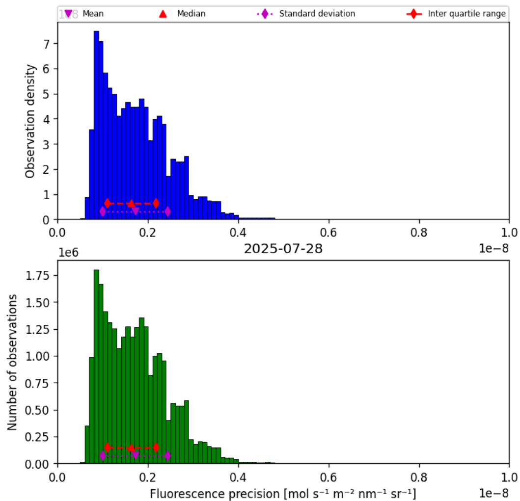
Figure 39: Histogram of “Fluorescence precision” for 2025-07-28 to 2025-07-29
