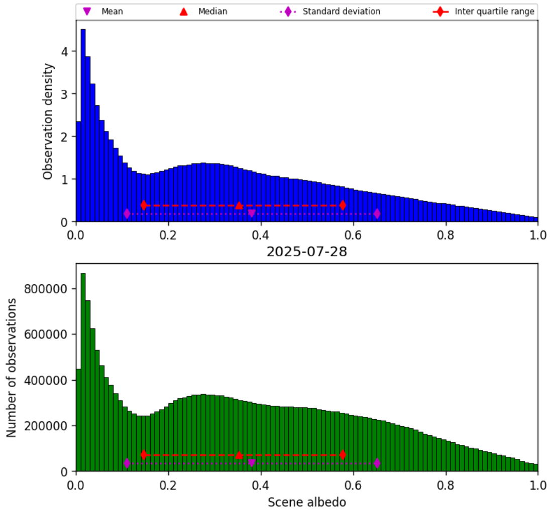
Figure 32: Histogram of “Scene albedo” for 2025-07-28 to 2025-07-29
