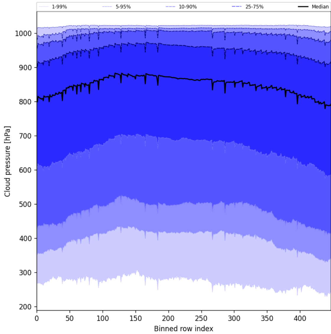
Figure 45: Along track statistics of “Cloud pressure” for 2025-07-28 to 2025-07-29
