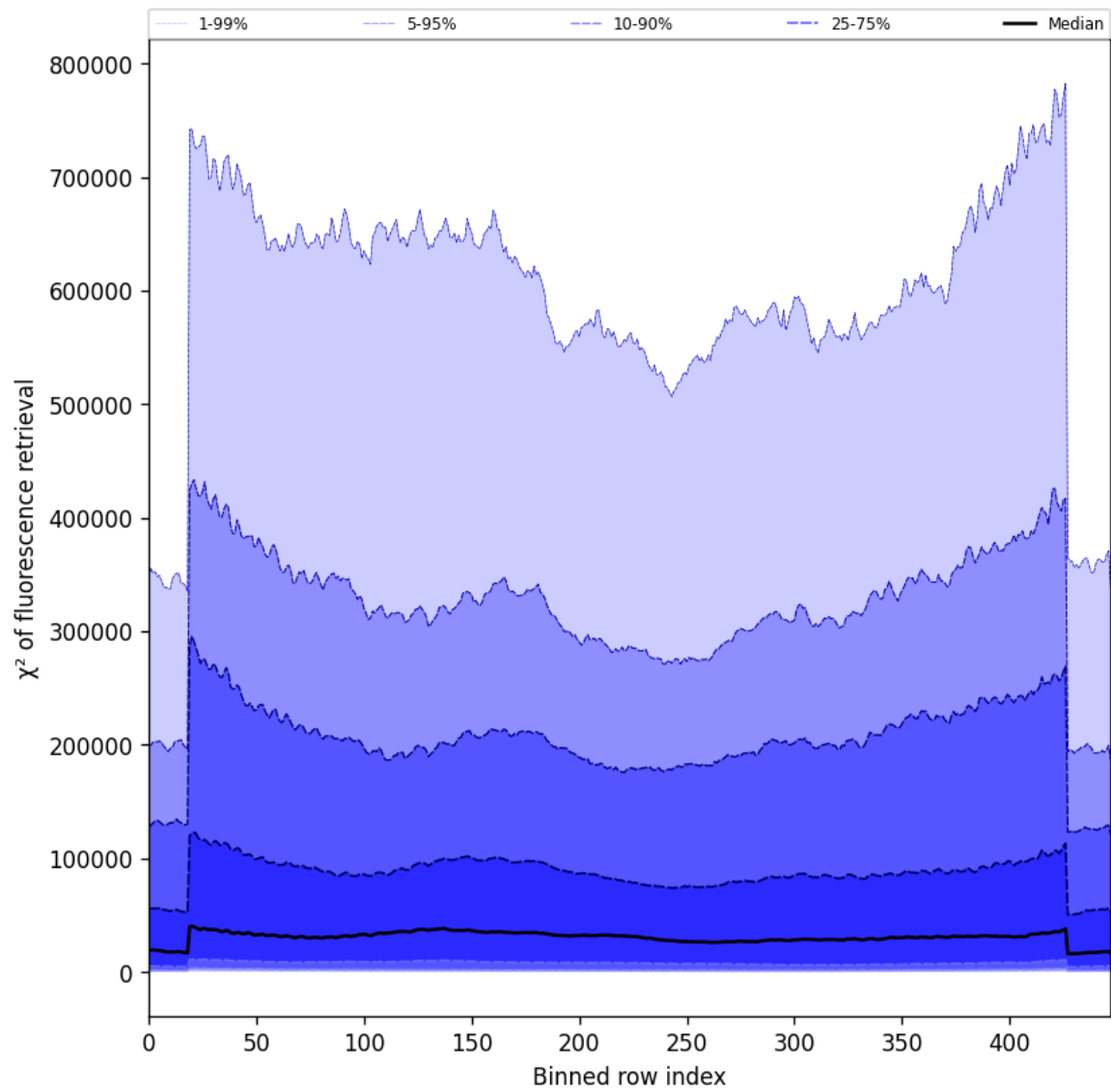
Figure 57: Along track statistics of “ \chi^2 of fluorescence retrieval” for 2025-07-28 to 2025-07-29
