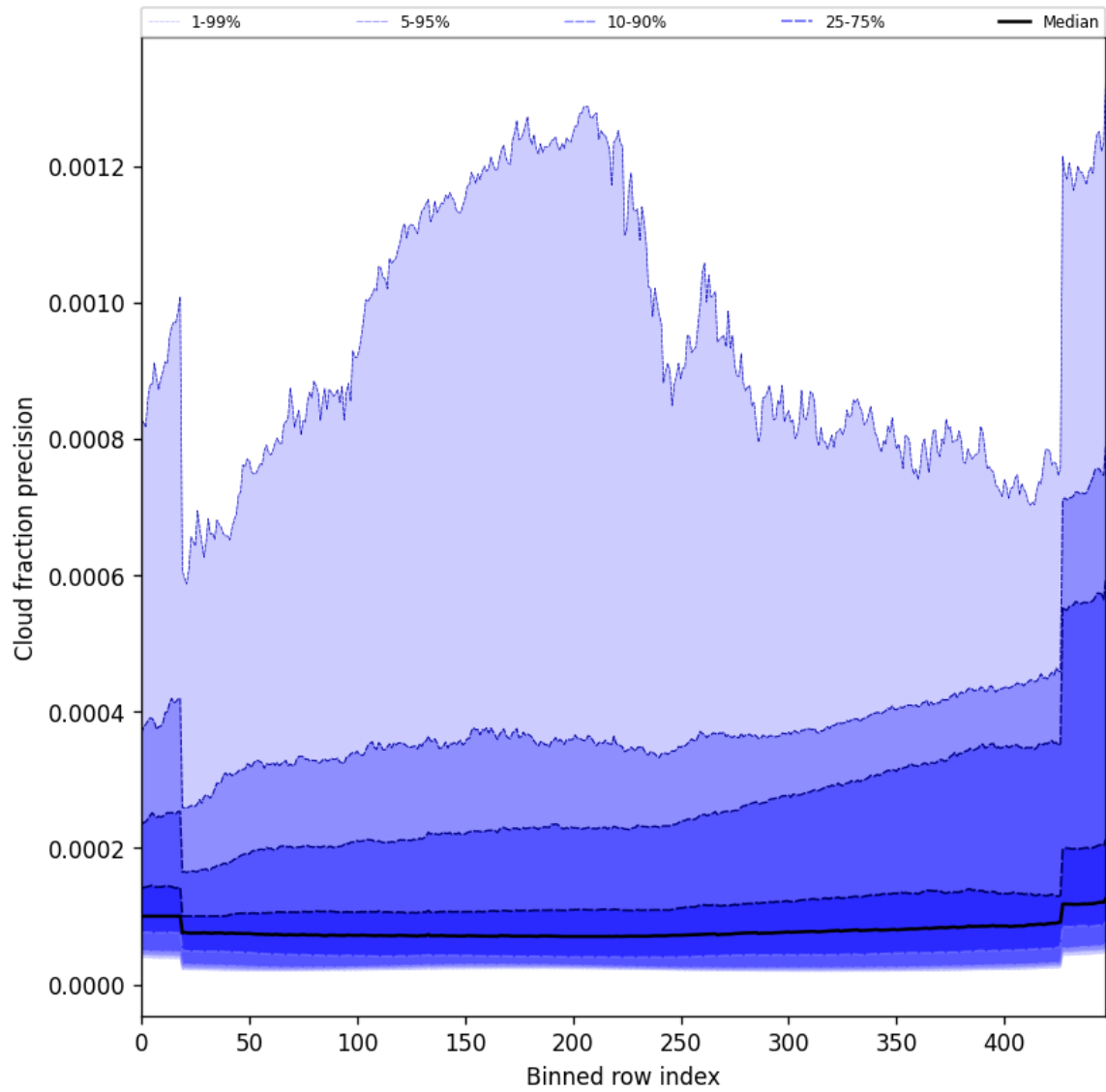
Figure 48: Along track statistics of “Cloud fraction precision” for 2025-07-28 to 2025-07-29
