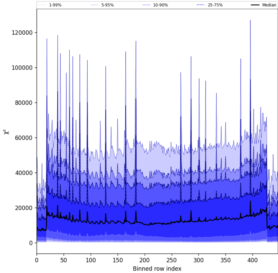
Figure 53: Along track statistics of “ \chi^2 ” for 2025-07-28 to 2025-07-29
