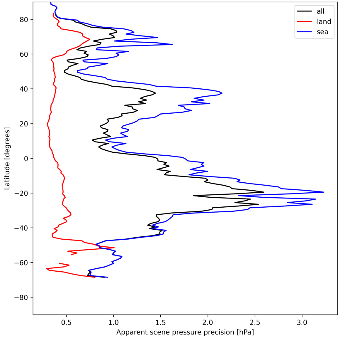
Figure 18: Zonal average of “Apparent scene pressure precision” for 2025-07-28 to 2025-07-29.
