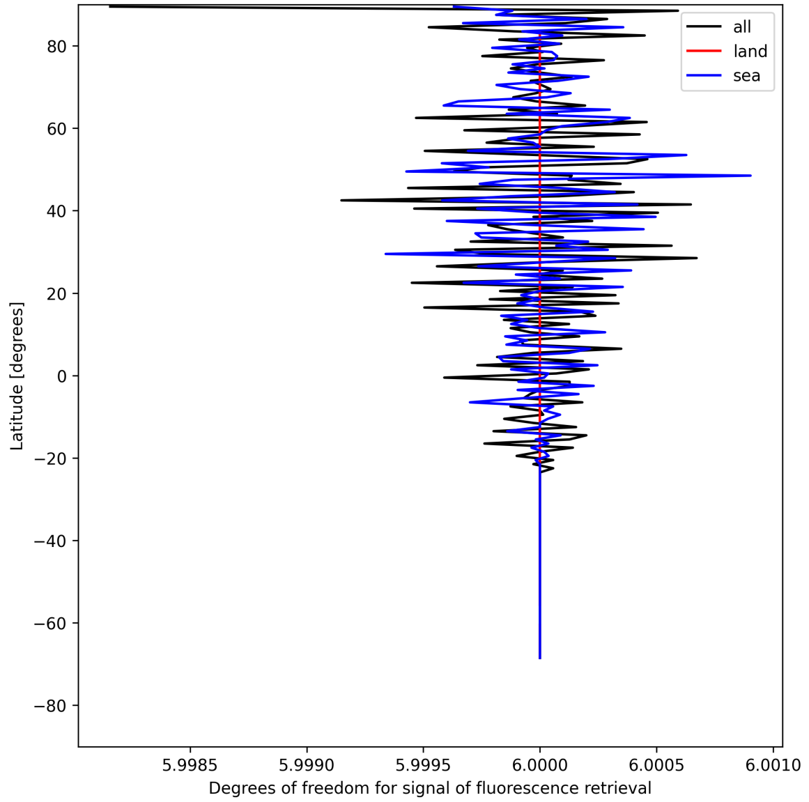
Figure 24: Zonal average of “Degrees of freedom for signal of fluorescence retrieval” for 2025-07-28 to 2025-07-29.
