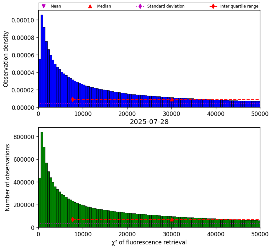
Figure 40: Histogram of “ \chi^2 of fluorescence retrieval” for 2025-07-28 to 2025-07-29
