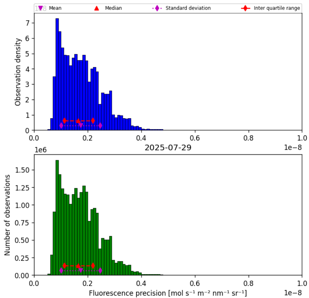
Figure 39: Histogram of “Fluorescence precision” for 2025-07-29 to 2025-07-30
