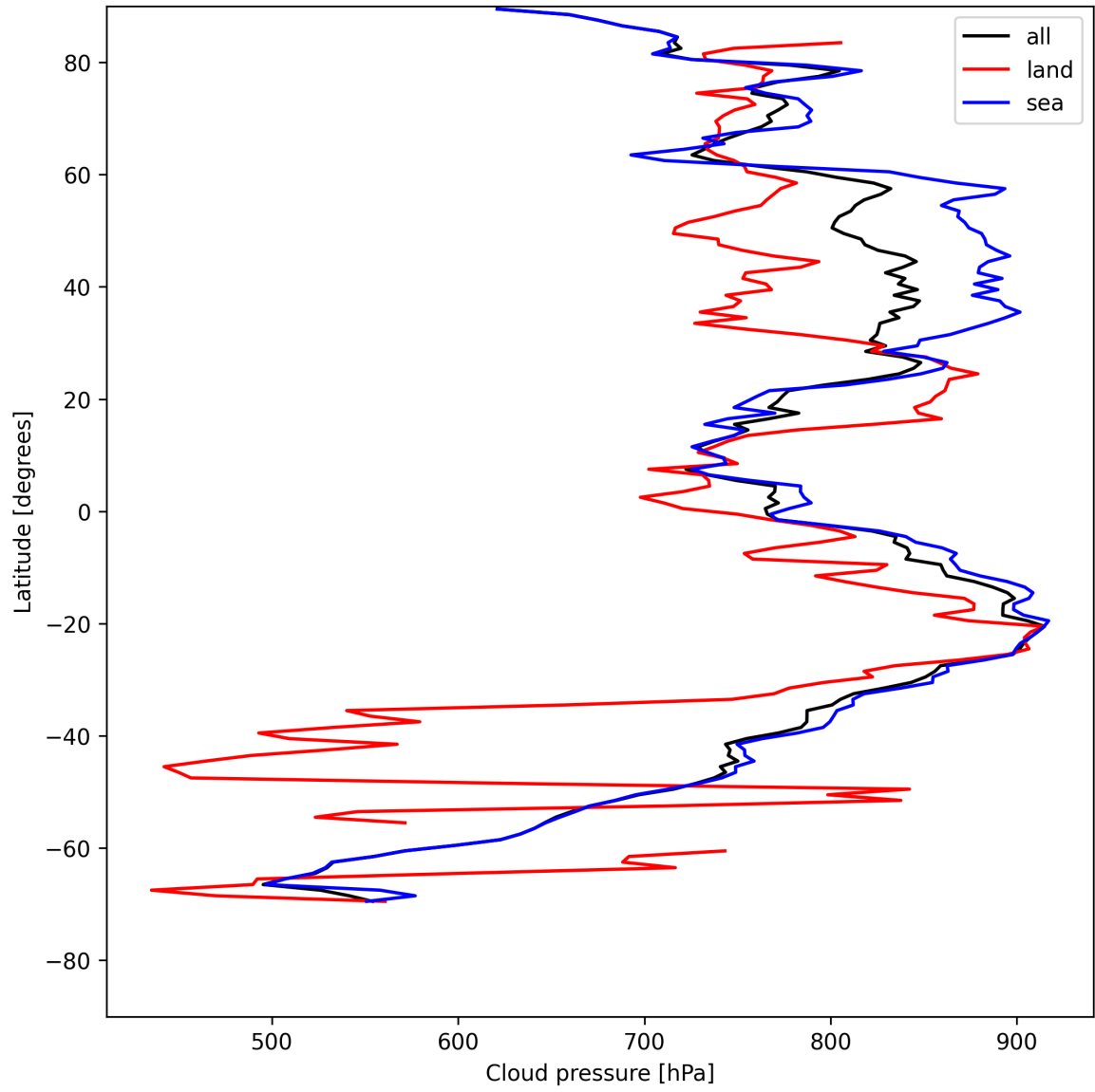
Figure 11: Zonal average of “Cloud pressure” for 2025-07-29 to 2025-07-30.
