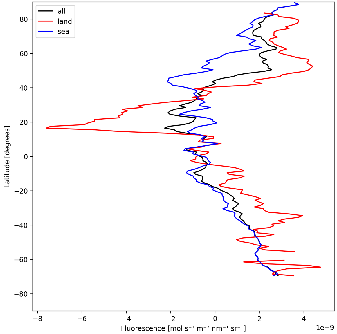
Figure 21: Zonal average of “Fluorescence” for 2025-07-29 to 2025-07-30.
