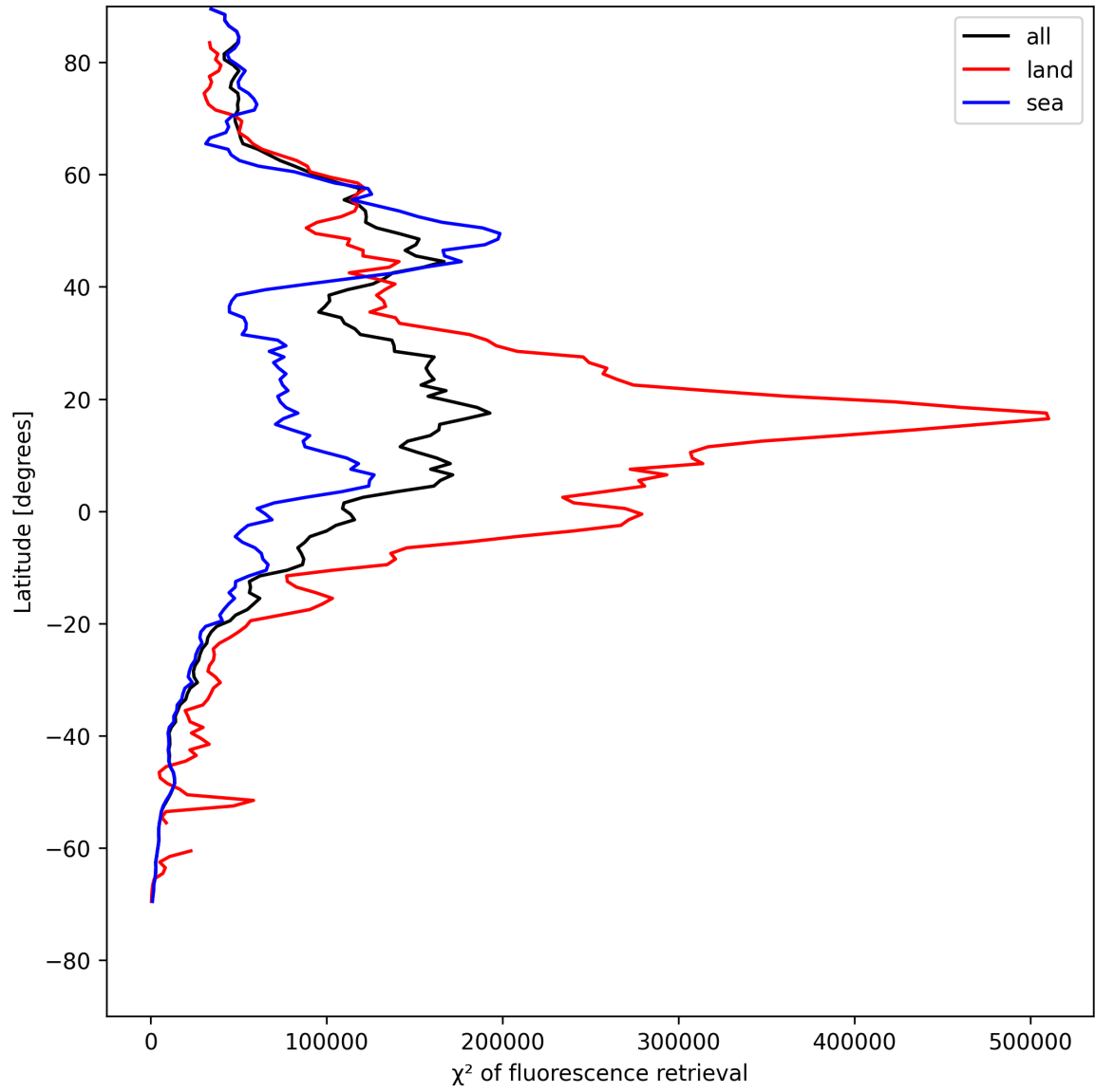
Figure 23: Zonal average of “ \chi^2 of fluorescence retrieval” for 2025-07-29 to 2025-07-30.
