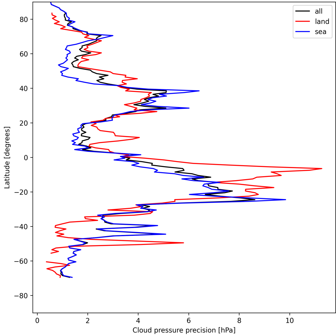
Figure 12: Zonal average of “Cloud pressure precision” for 2025-07-29 to 2025-07-30.
