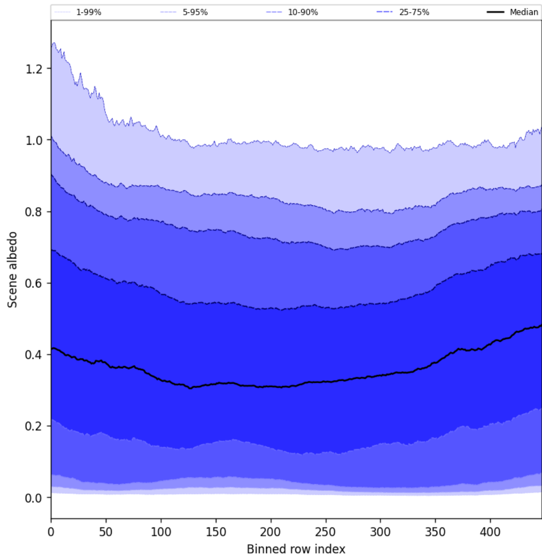
Figure 49: Along track statistics of “Scene albedo” for 2025-07-29 to 2025-07-30
