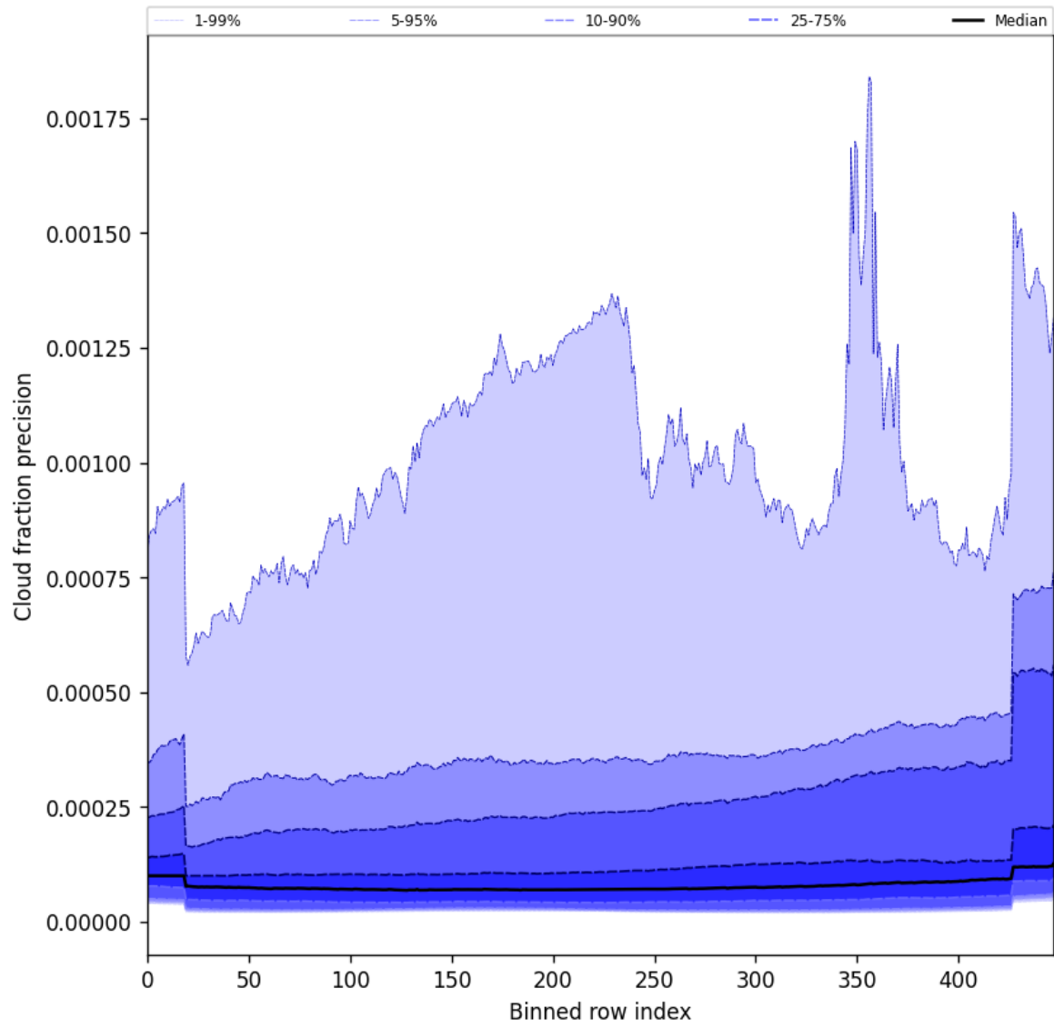
Figure 48: Along track statistics of “Cloud fraction precision” for 2025-07-29 to 2025-07-30
