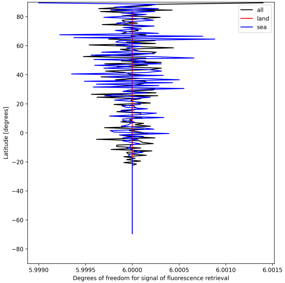
Figure 24: Zonal average of “Degrees of freedom for signal of fluorescence retrieval” for 2025-07-29 to 2025-07-30.
