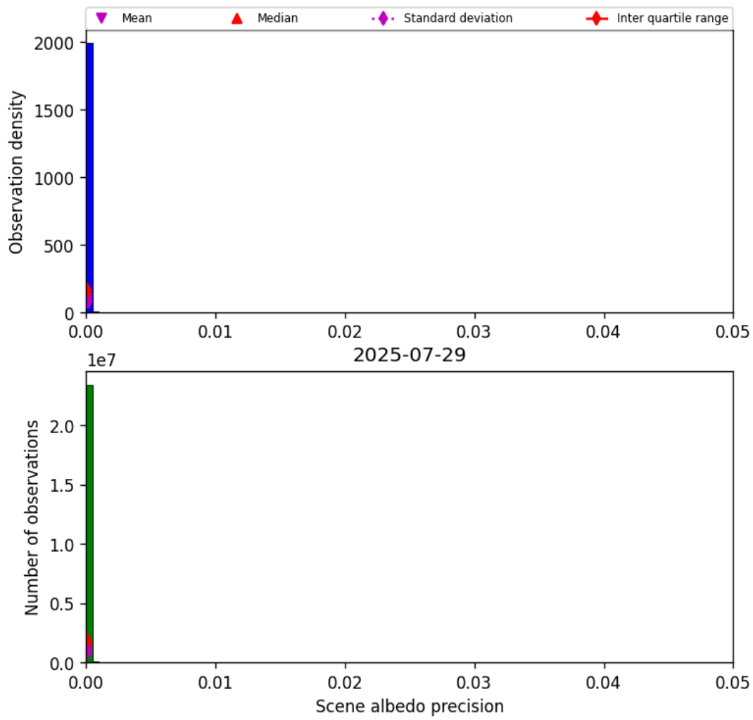
Figure 33: Histogram of “Scene albedo precision” for 2025-07-29 to 2025-07-30
