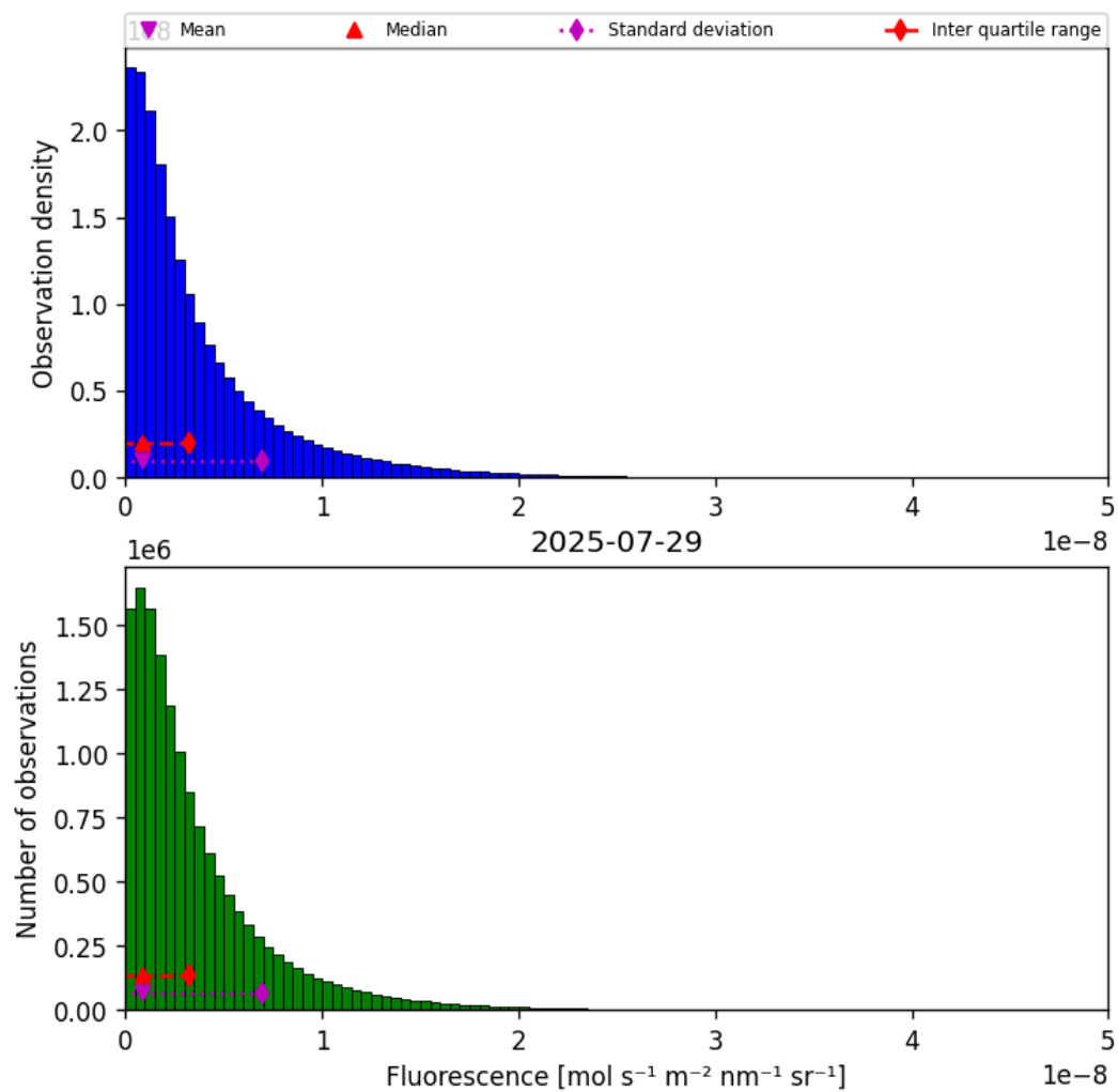
Figure 38: Histogram of “Fluorescence” for 2025-07-29 to 2025-07-30
