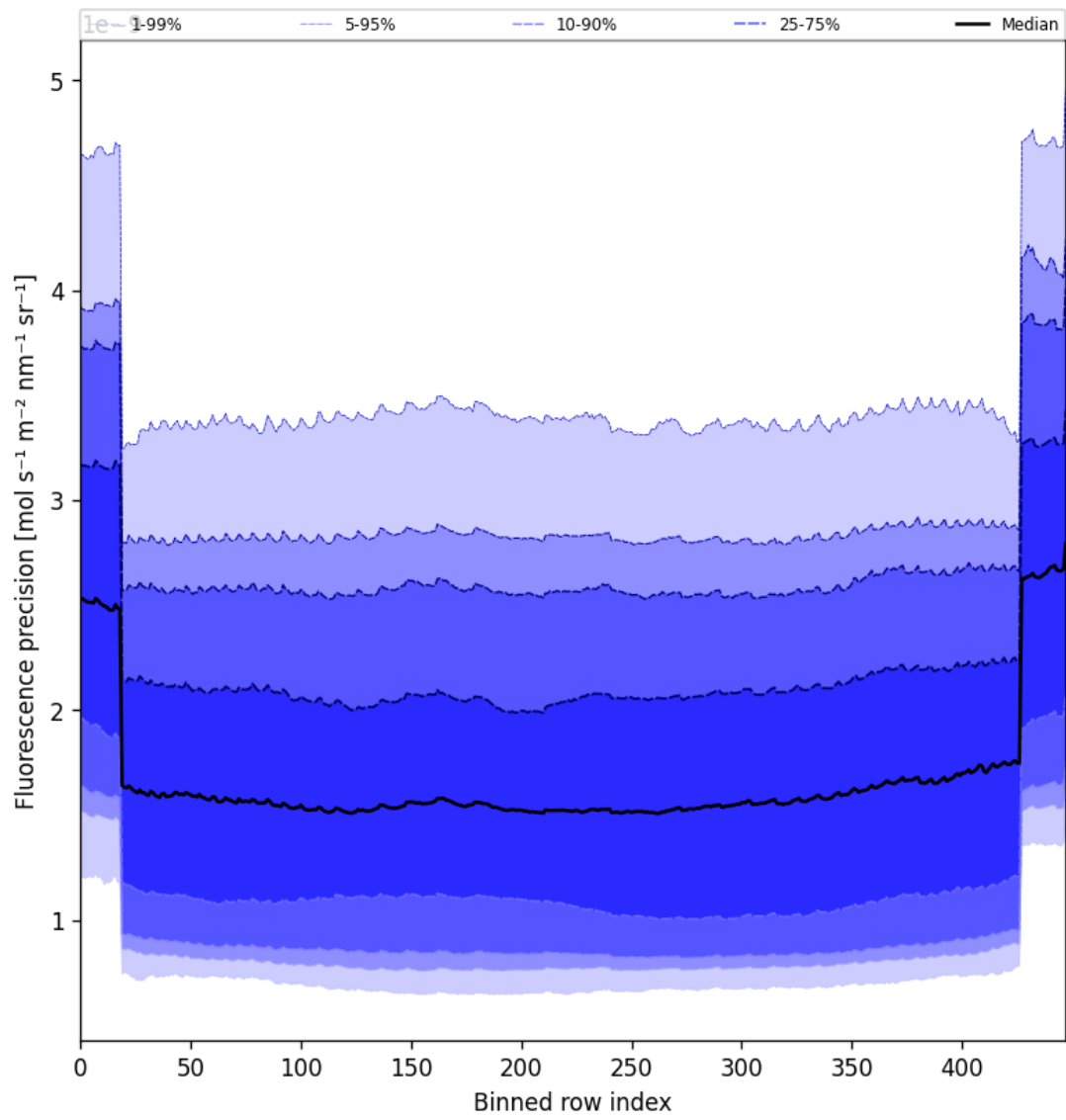
Figure 56: Along track statistics of “Fluorescence precision” for 2025-07-29 to 2025-07-30
