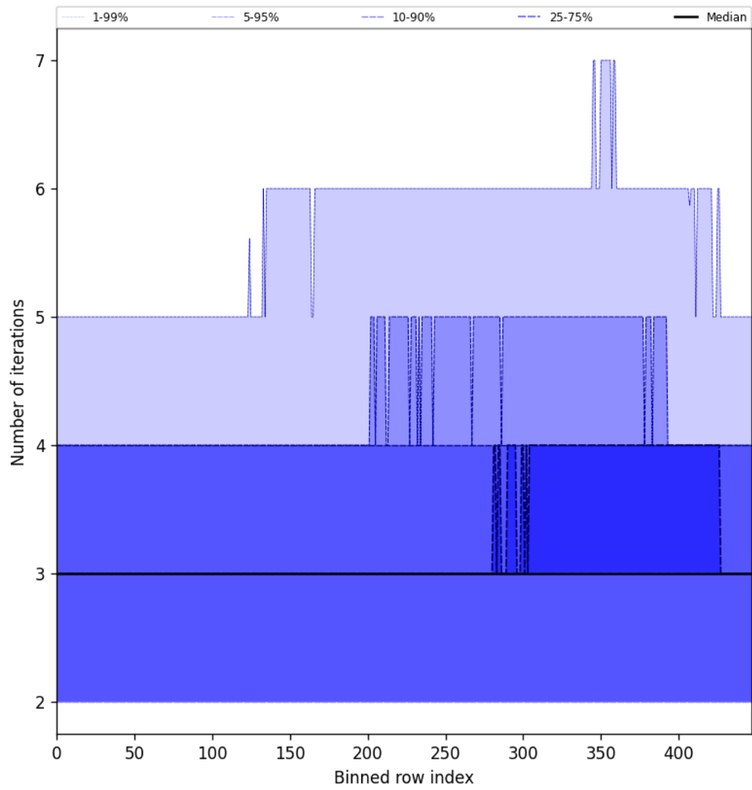
Figure 54: Along track statistics of “Number of iterations” for 2025-07-29 to 2025-07-30
