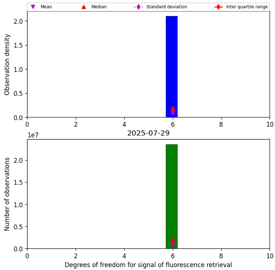
Figure 41: Histogram of “Degrees of freedom for signal of fluorescence retrieval” for 2025-07-29 to 2025-07-30
