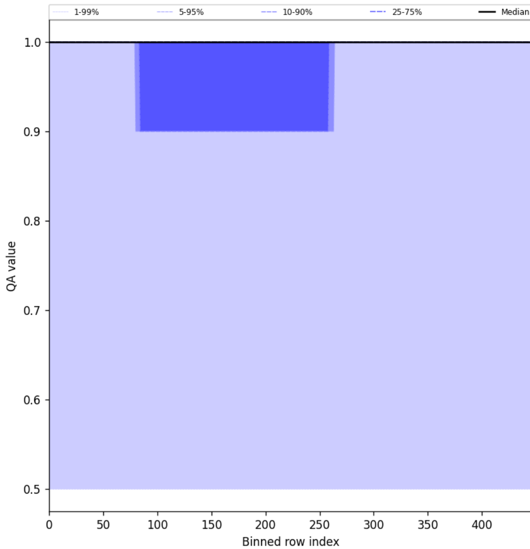
Figure 44: Along track statistics of “QA value” for 2025-07-29 to 2025-07-30
