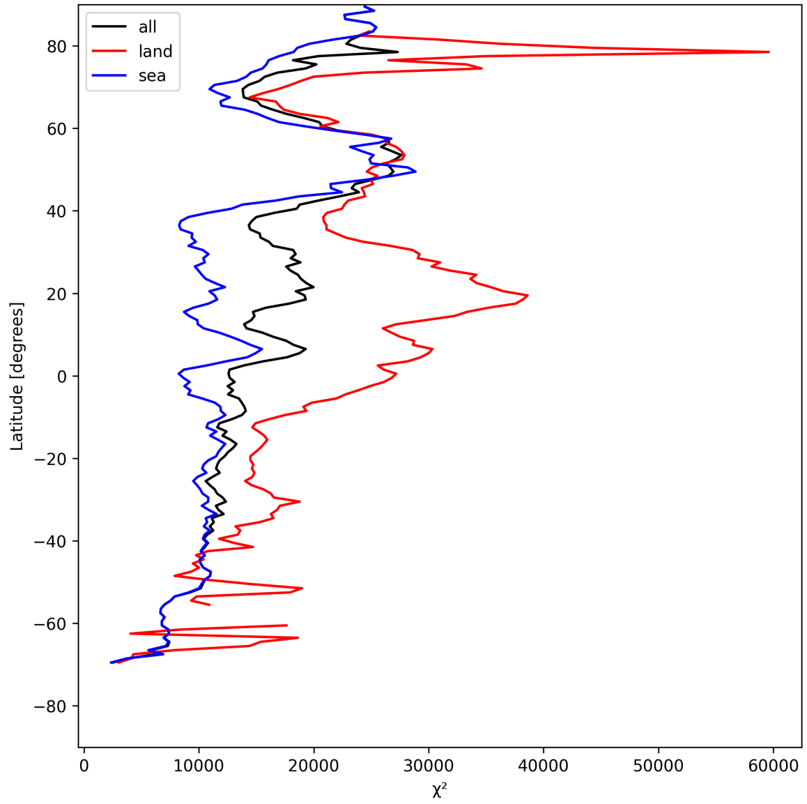
Figure 19: Zonal average of “ \chi^2 ” for 2025-07-29 to 2025-07-30.
