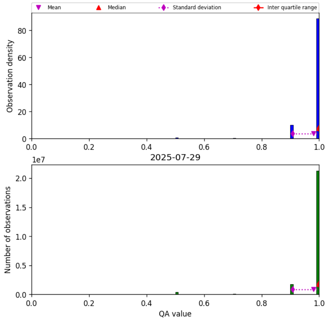
Figure 27: Histogram of “QA value” for 2025-07-29 to 2025-07-30
