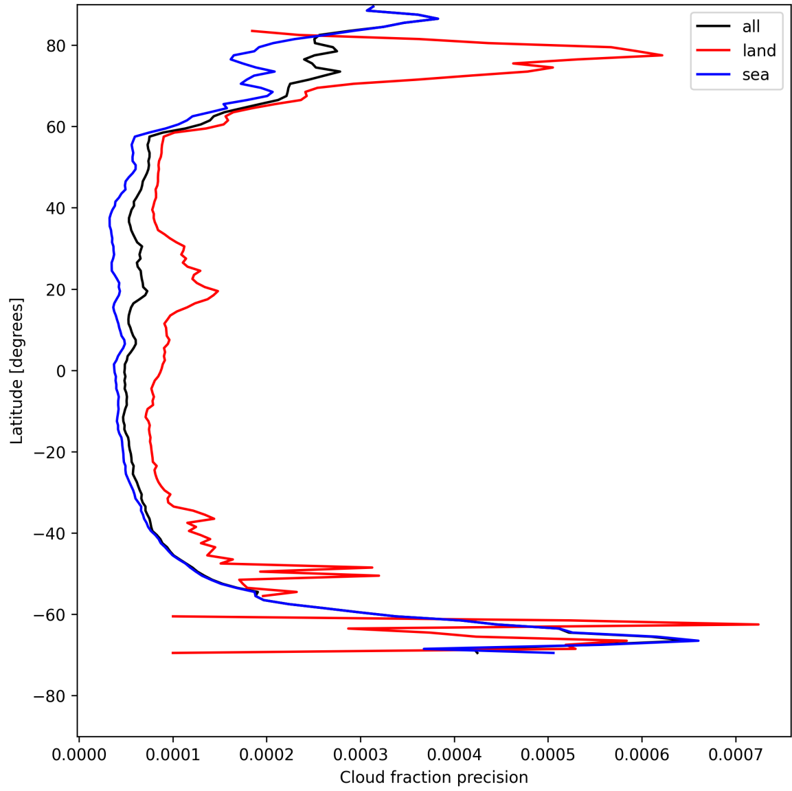
Figure 14: Zonal average of “Cloud fraction precision” for 2025-07-29 to 2025-07-30.
