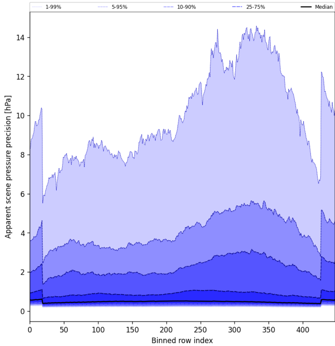
Figure 52: Along track statistics of “Apparent scene pressure precision” for 2025-07-29 to 2025-07-30
