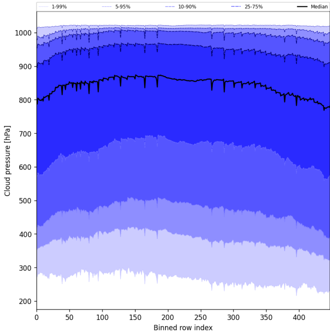
Figure 45: Along track statistics of “Cloud pressure” for 2025-07-29 to 2025-07-30
