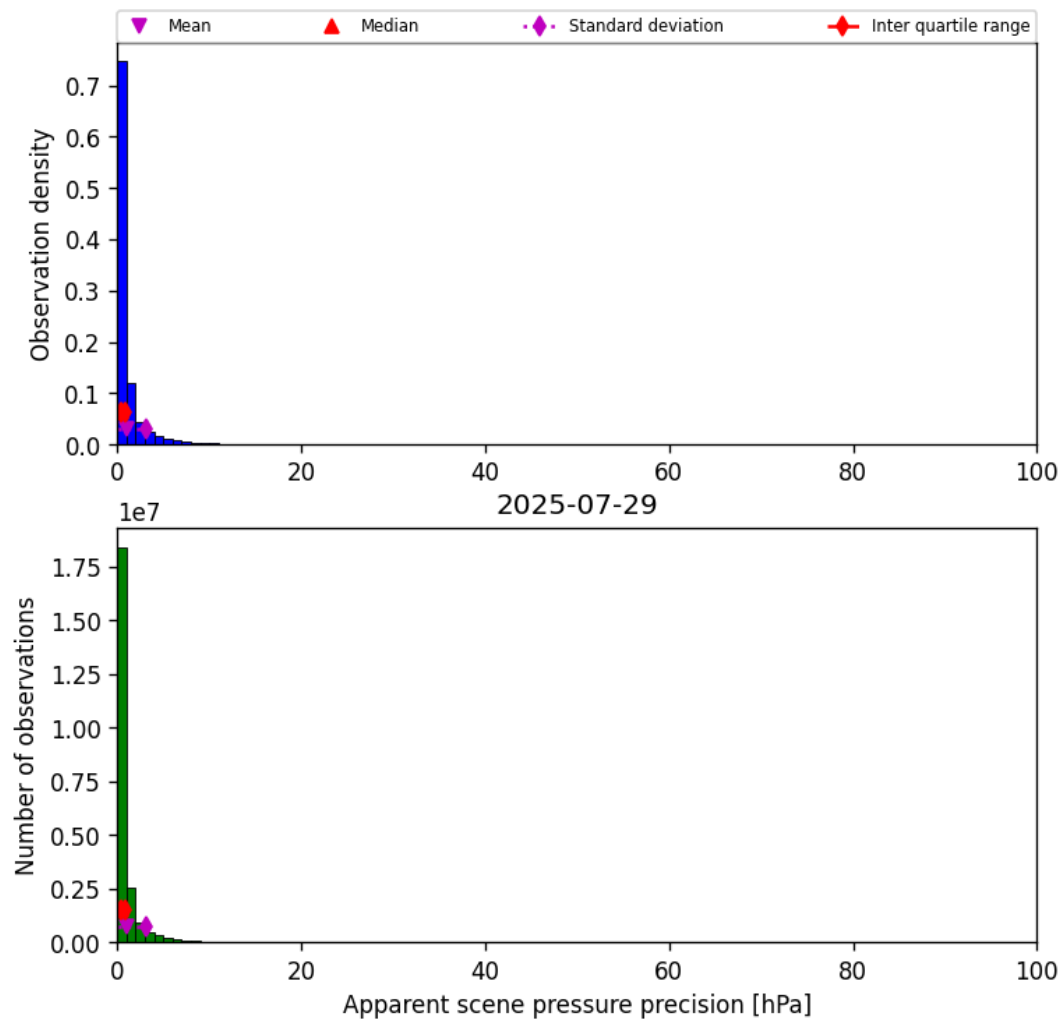
Figure 35: Histogram of “Apparent scene pressure precision” for 2025-07-29 to 2025-07-30
