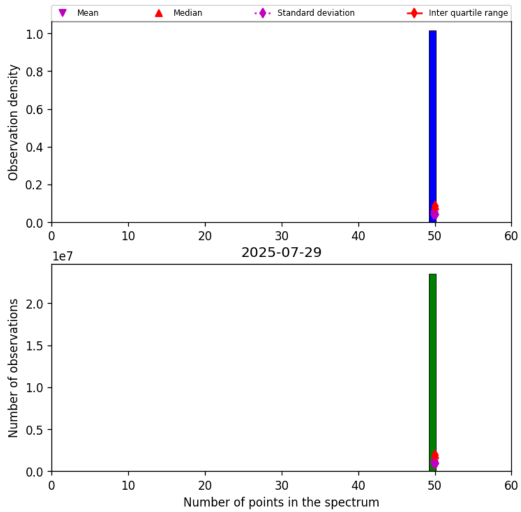
Figure 42: Histogram of “Number of points in the spectrum” for 2025-07-29 to 2025-07-30
