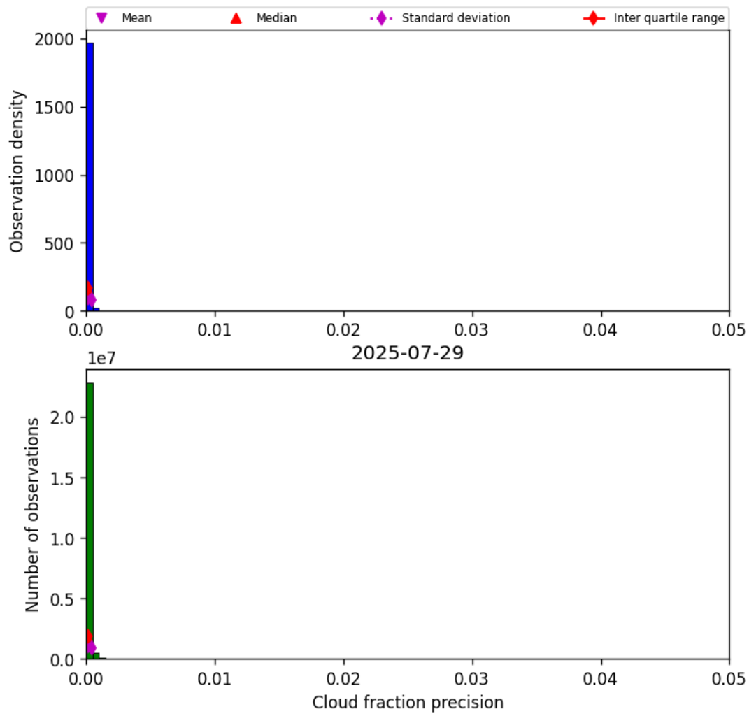
Figure 31: Histogram of “Cloud fraction precision” for 2025-07-29 to 2025-07-30
