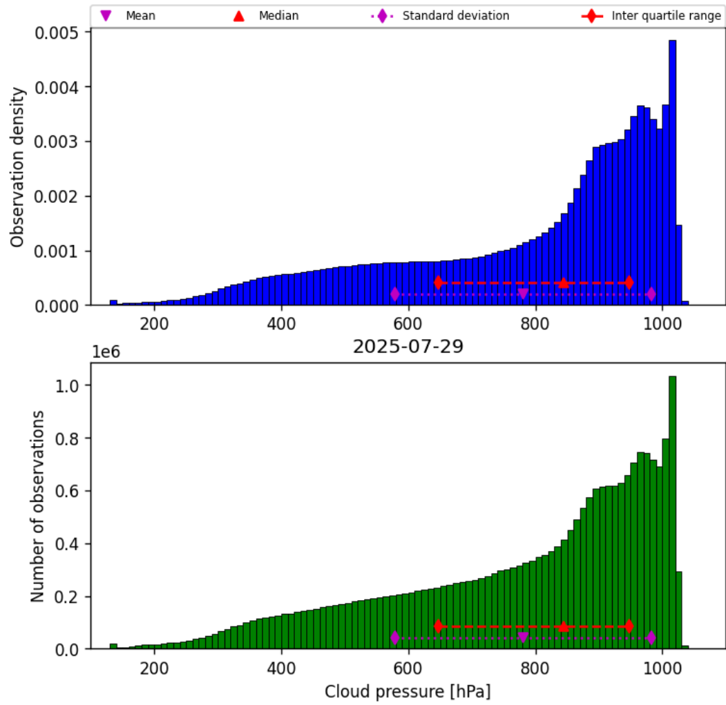
Figure 28: Histogram of “Cloud pressure” for 2025-07-29 to 2025-07-30
