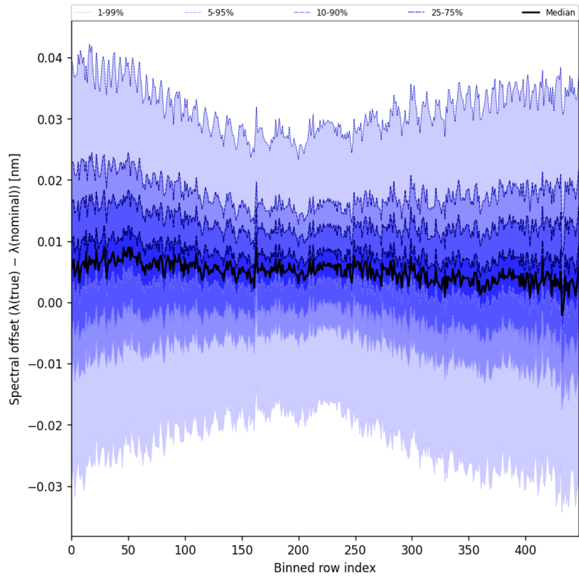
Figure 60: Along track statistics of “Spectral offset ( \lambda_{\text{true}} - \lambda_{\text{nominal}} )” for 2025-07-29 to 2025-07-30
