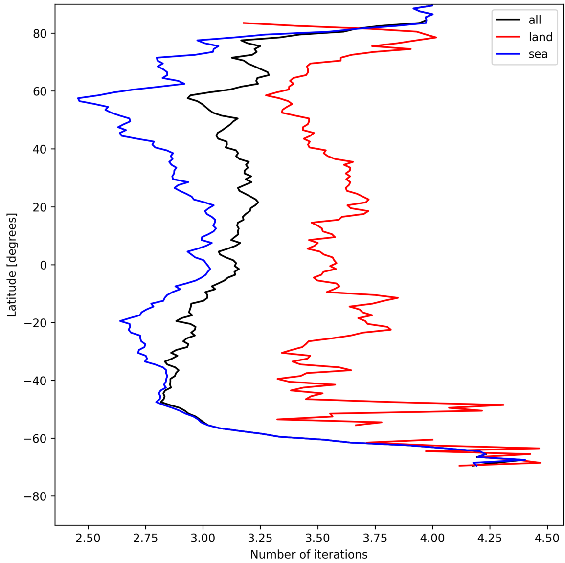
Figure 20: Zonal average of “Number of iterations” for 2025-07-29 to 2025-07-30.
