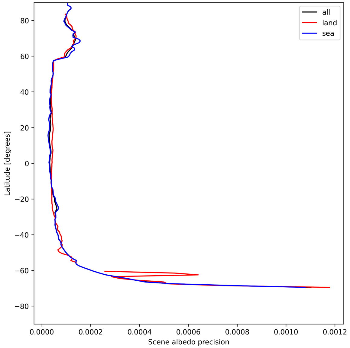
Figure 16: Zonal average of “Scene albedo precision” for 2025-07-29 to 2025-07-30.
