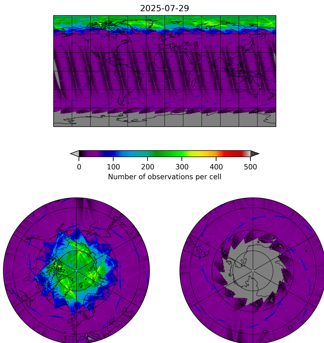
Figure 9: Map of the number of observations for 2025-07-29 to 2025-07-30
