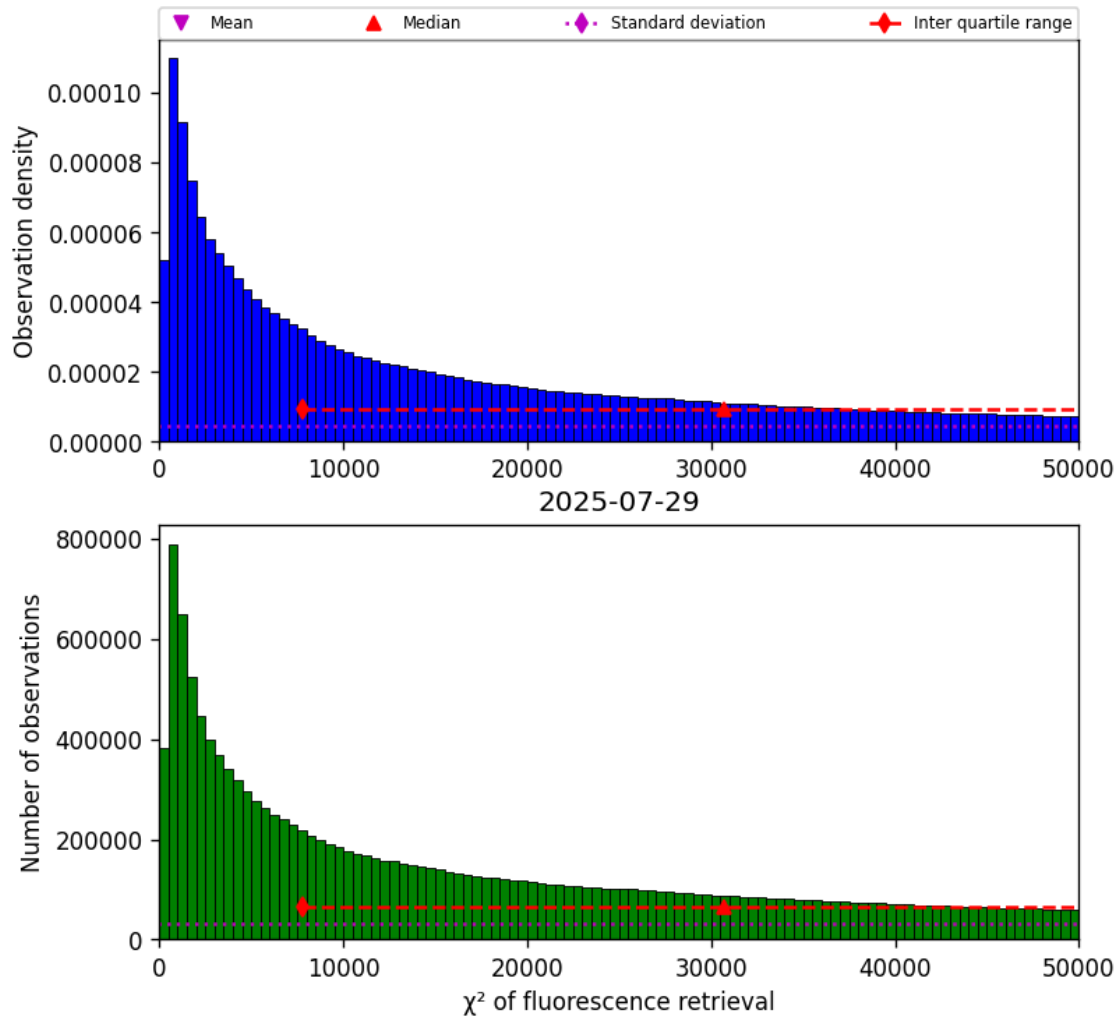
Figure 40: Histogram of “ \chi^2 of fluorescence retrieval” for 2025-07-29 to 2025-07-30
