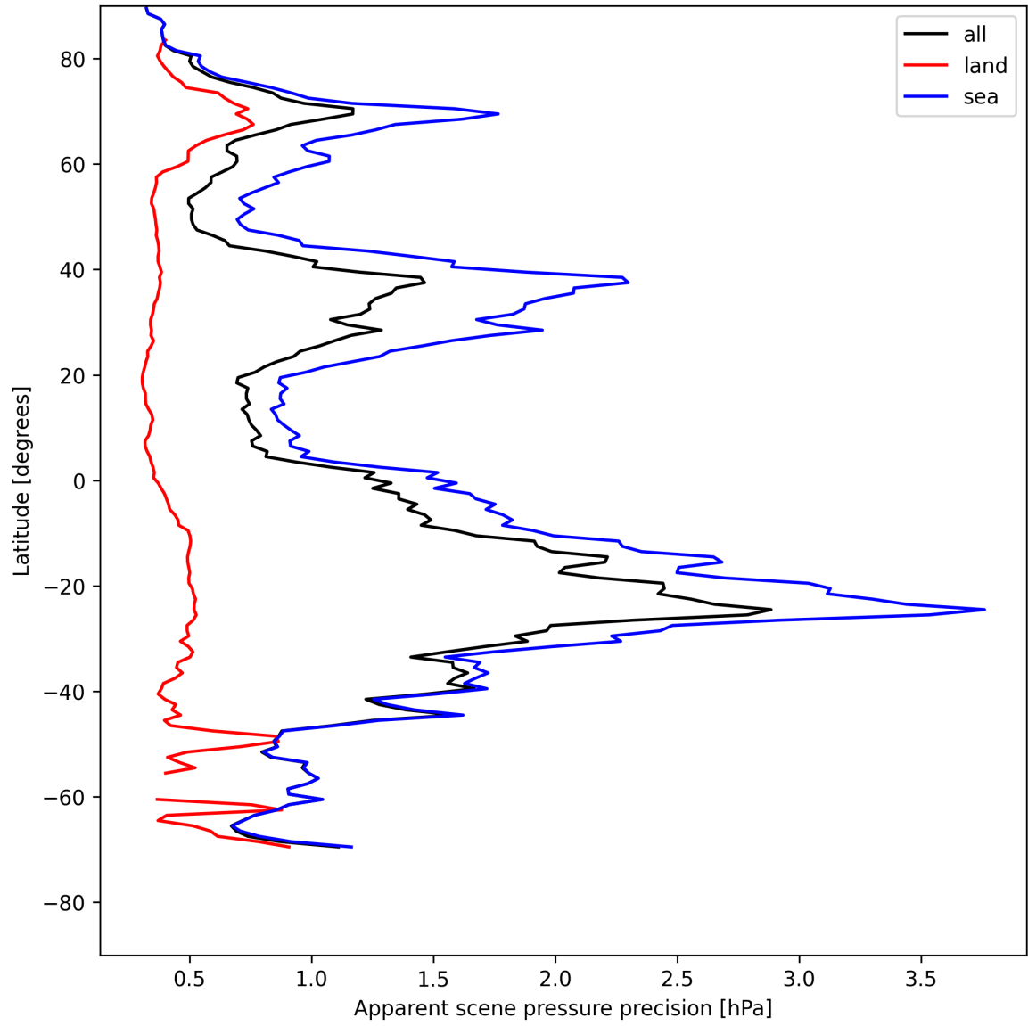
Figure 18: Zonal average of “Apparent scene pressure precision” for 2025-07-29 to 2025-07-30.
