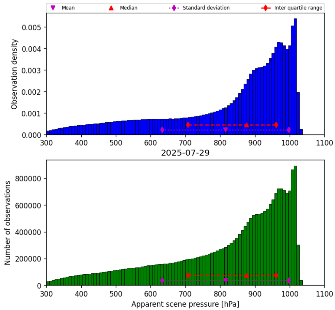
Figure 34: Histogram of “Apparent scene pressure” for 2025-07-29 to 2025-07-30
