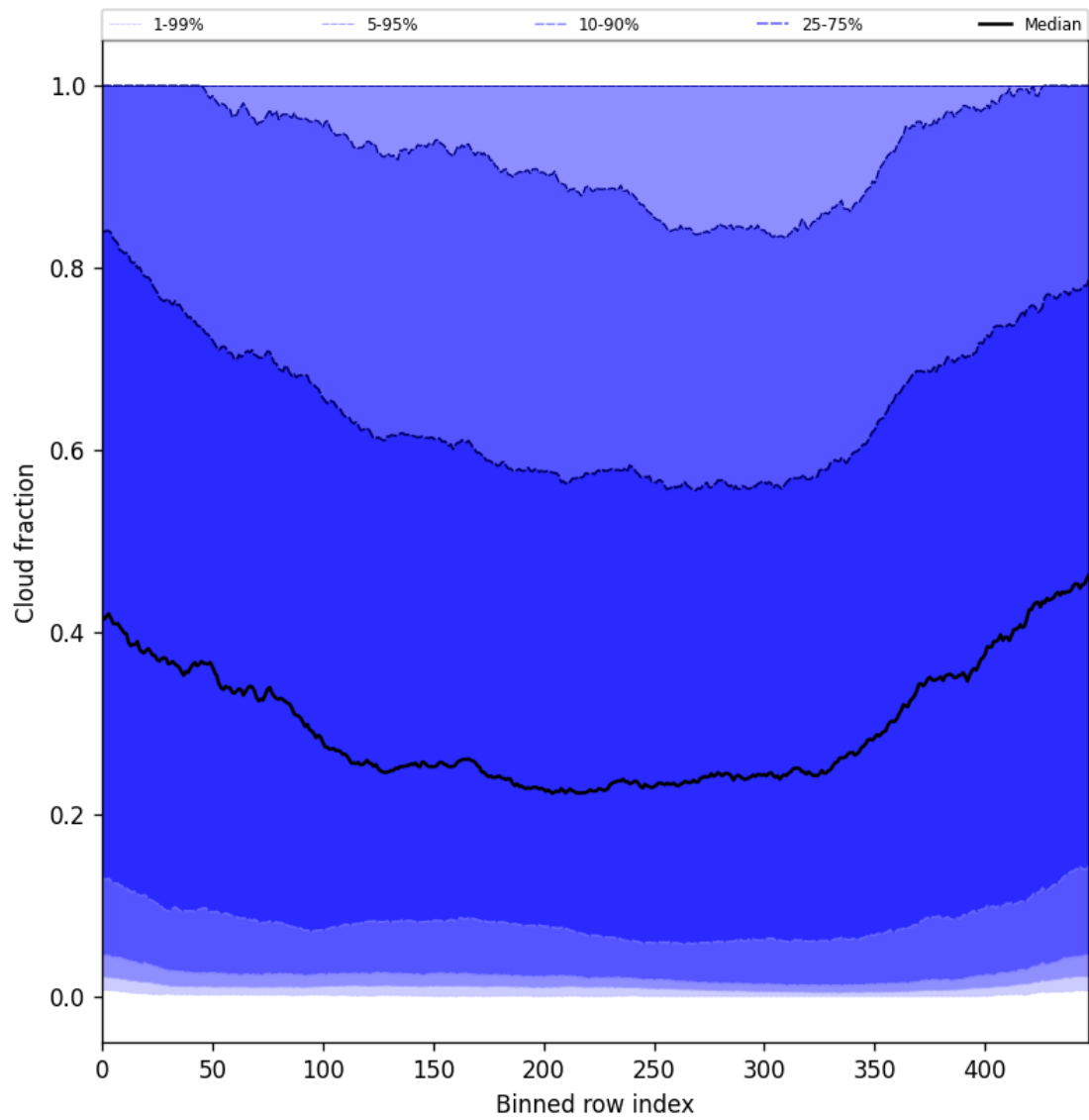
Figure 47: Along track statistics of “Cloud fraction” for 2025-07-29 to 2025-07-30
