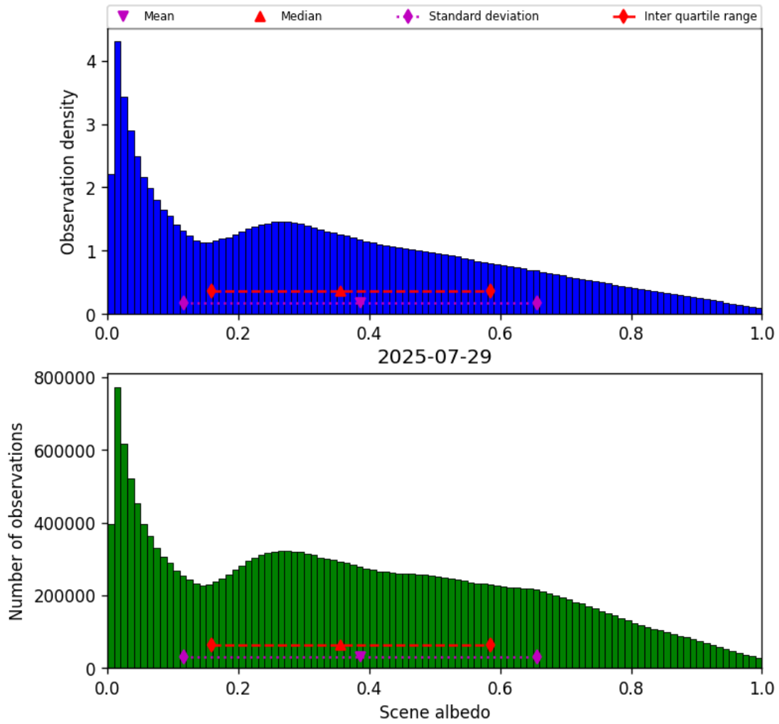
Figure 32: Histogram of “Scene albedo” for 2025-07-29 to 2025-07-30
