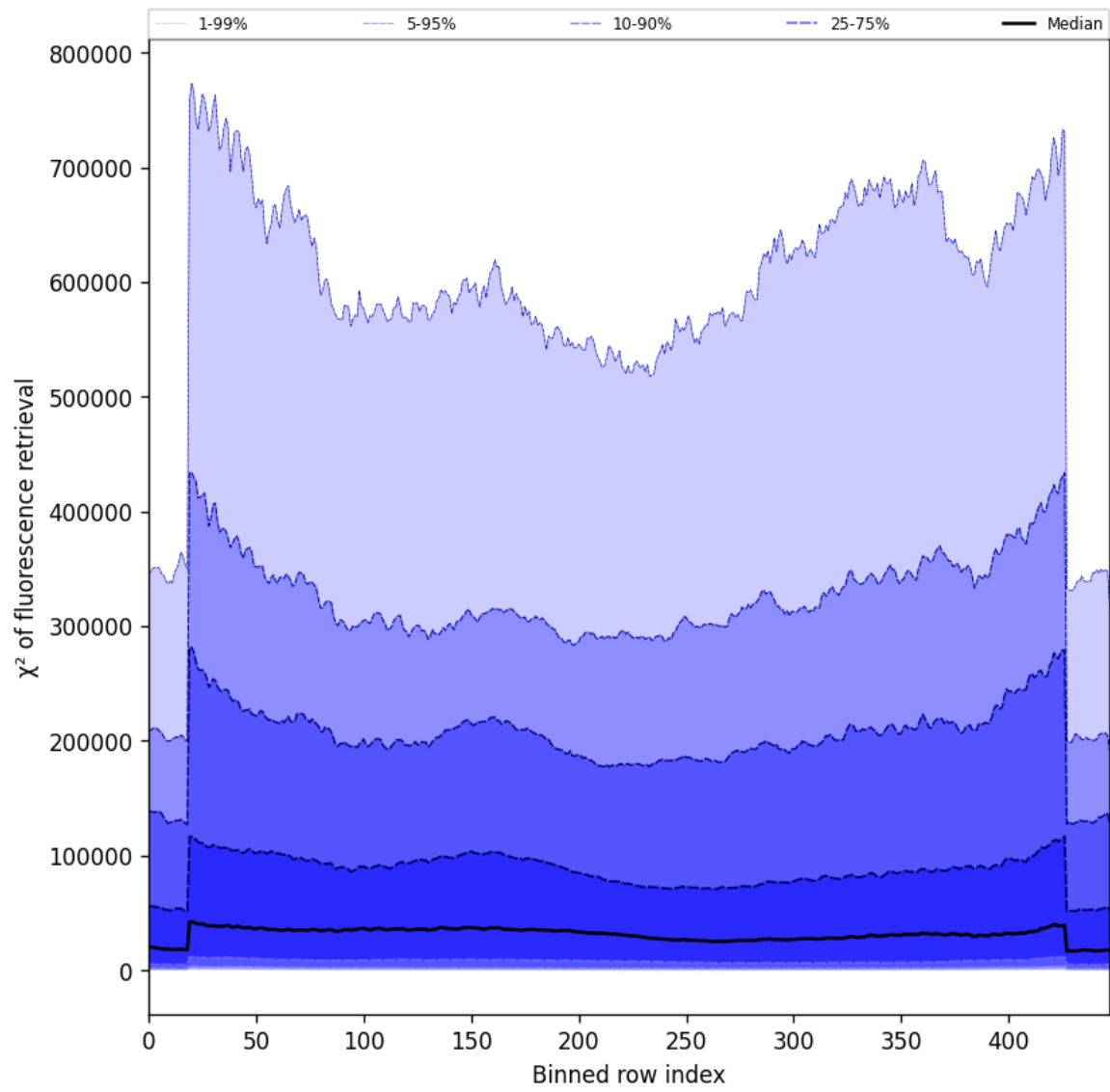
Figure 57: Along track statistics of “ \chi^2 of fluorescence retrieval” for 2025-07-29 to 2025-07-30
