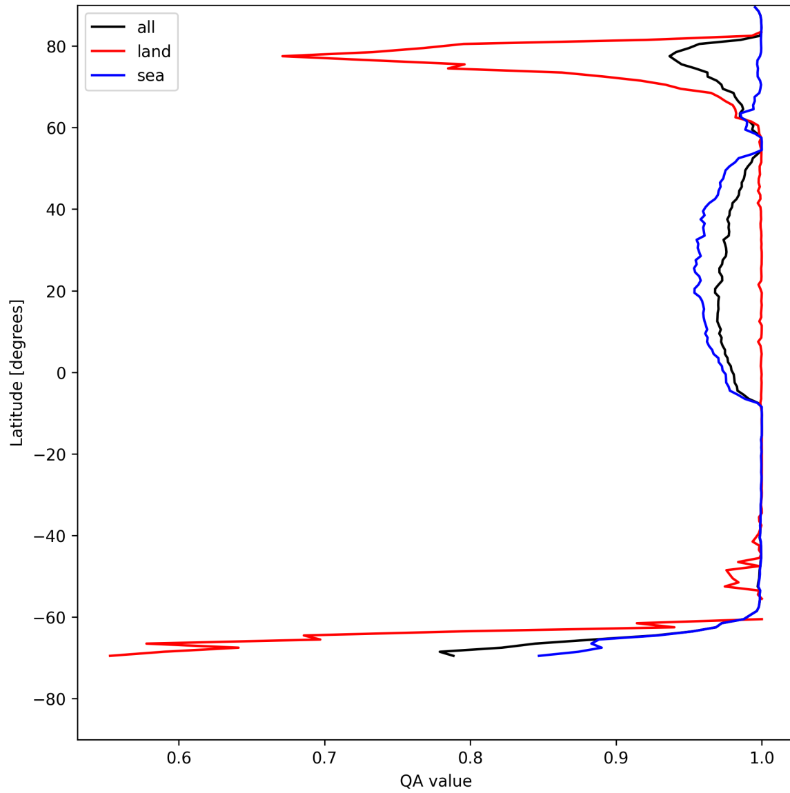
Figure 10: Zonal average of “QA value” for 2025-07-29 to 2025-07-30.
