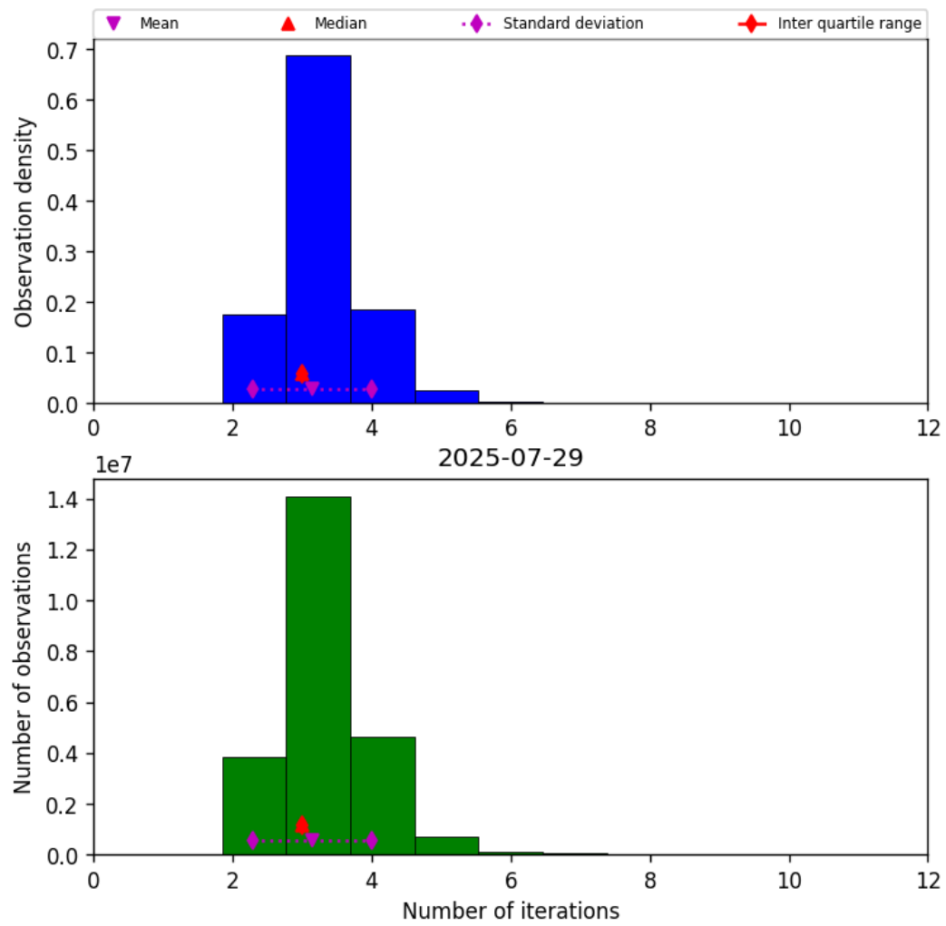
Figure 37: Histogram of “Number of iterations” for 2025-07-29 to 2025-07-30
