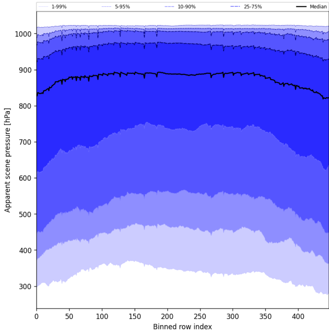
Figure 51: Along track statistics of “Apparent scene pressure” for 2025-07-29 to 2025-07-30
