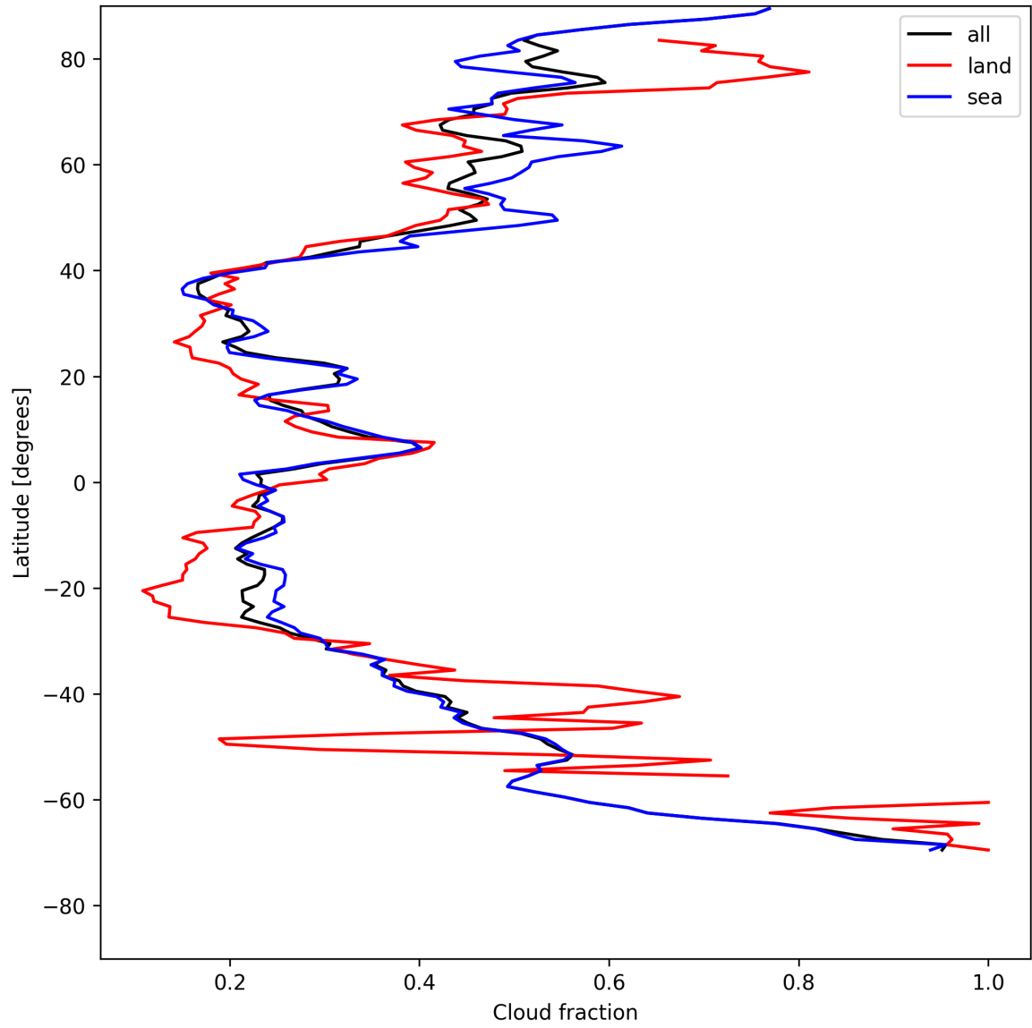
Figure 13: Zonal average of “Cloud fraction” for 2025-07-29 to 2025-07-30.
