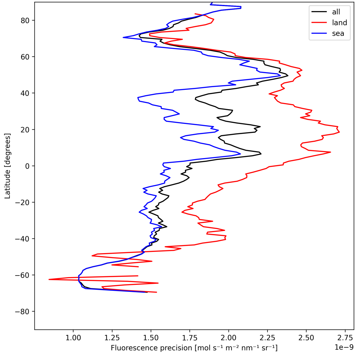
Figure 22: Zonal average of “Fluorescence precision” for 2025-07-29 to 2025-07-30.
