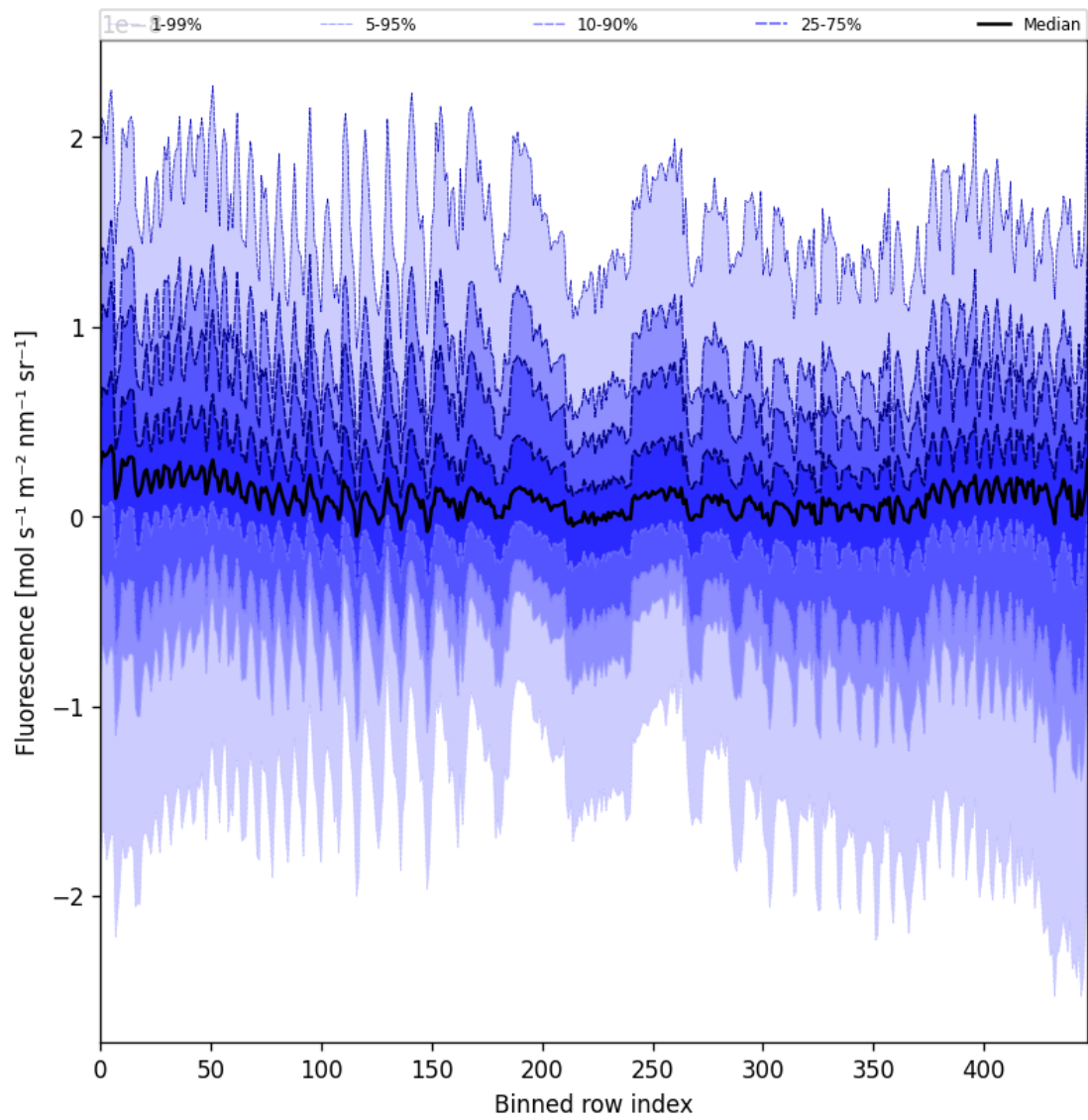
Figure 55: Along track statistics of “Fluorescence” for 2025-07-29 to 2025-07-30
