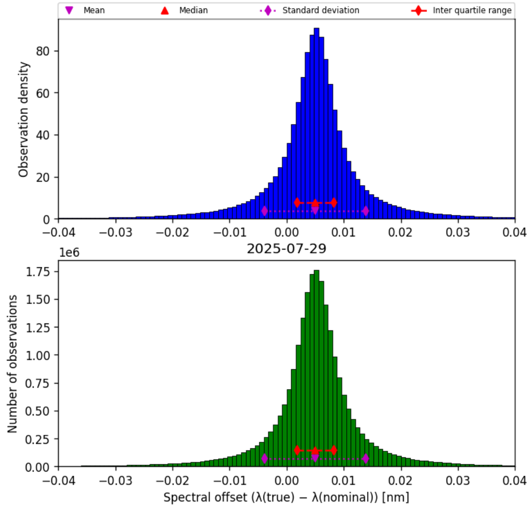
Figure 43: Histogram of “Spectral offset ( \lambda_{\text{true}} - \lambda_{\text{nominal}} )” for 2025-07-29 to 2025-07-30
