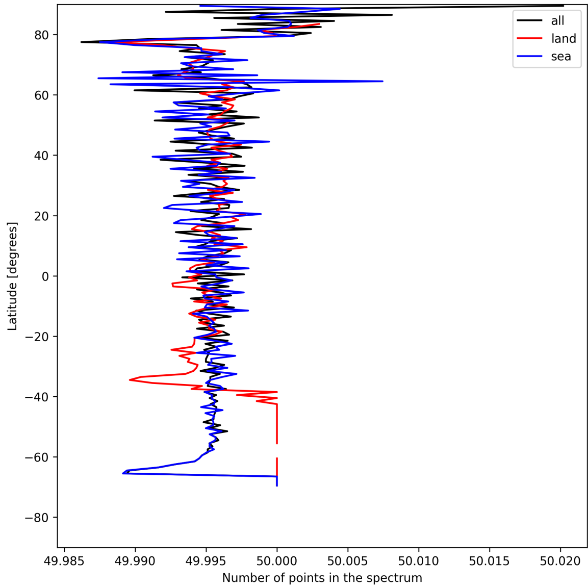
Figure 25: Zonal average of “Number of points in the spectrum” for 2025-07-29 to 2025-07-30.
