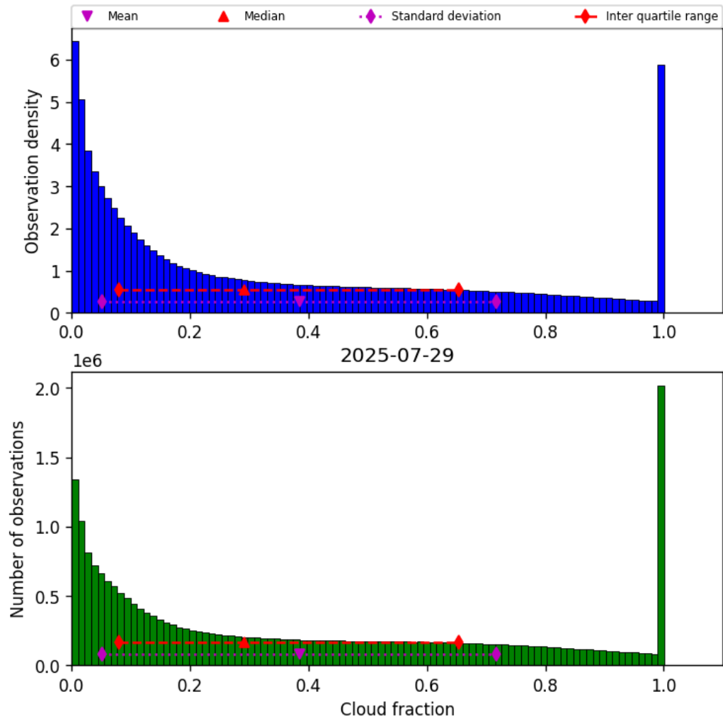
Figure 30: Histogram of “Cloud fraction” for 2025-07-29 to 2025-07-30
