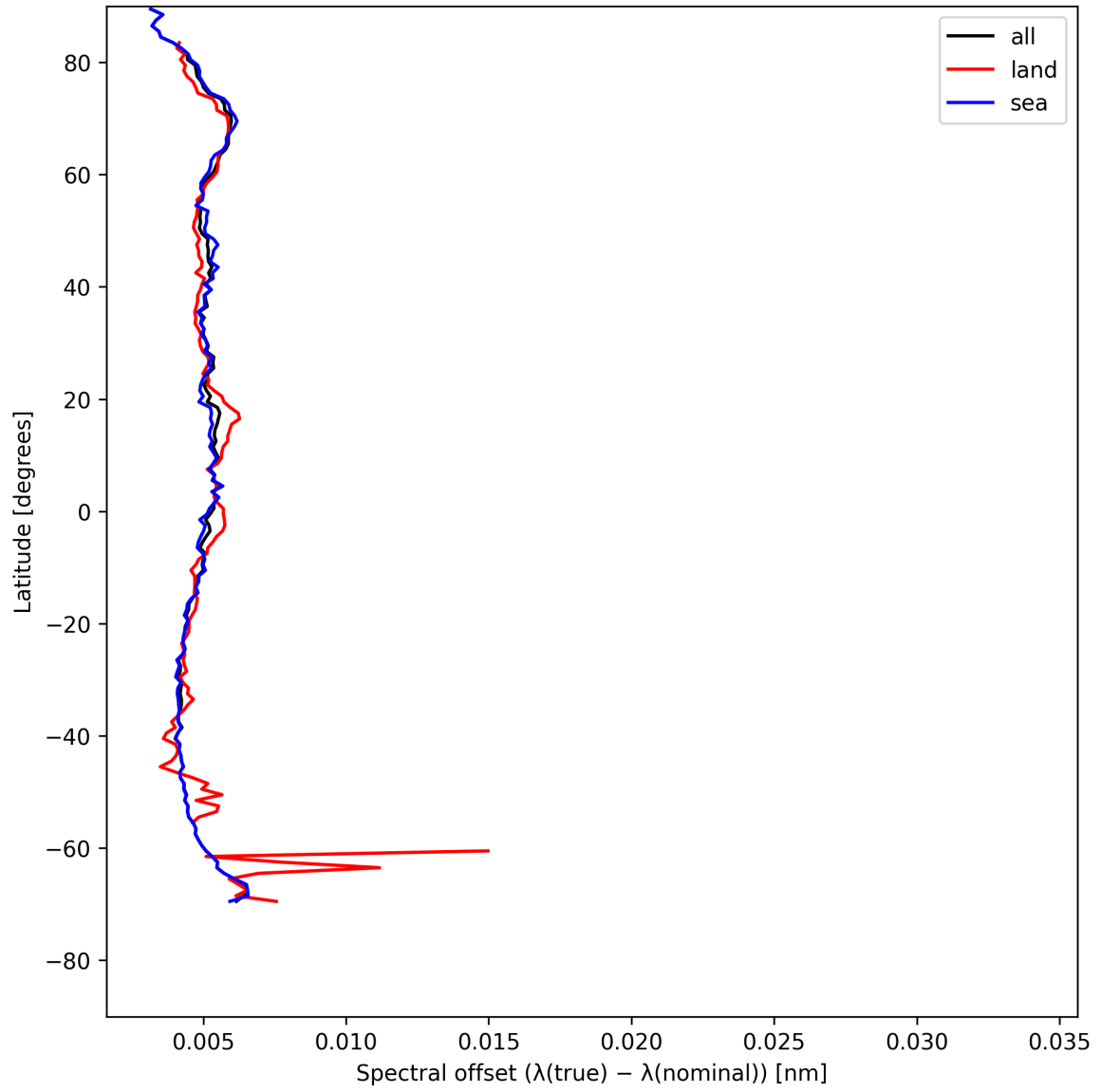
Figure 26: Zonal average of “Spectral offset ( \lambda_{\text{true}} - \lambda_{\text{nominal}} )” for 2025-07-29 to 2025-07-30.
