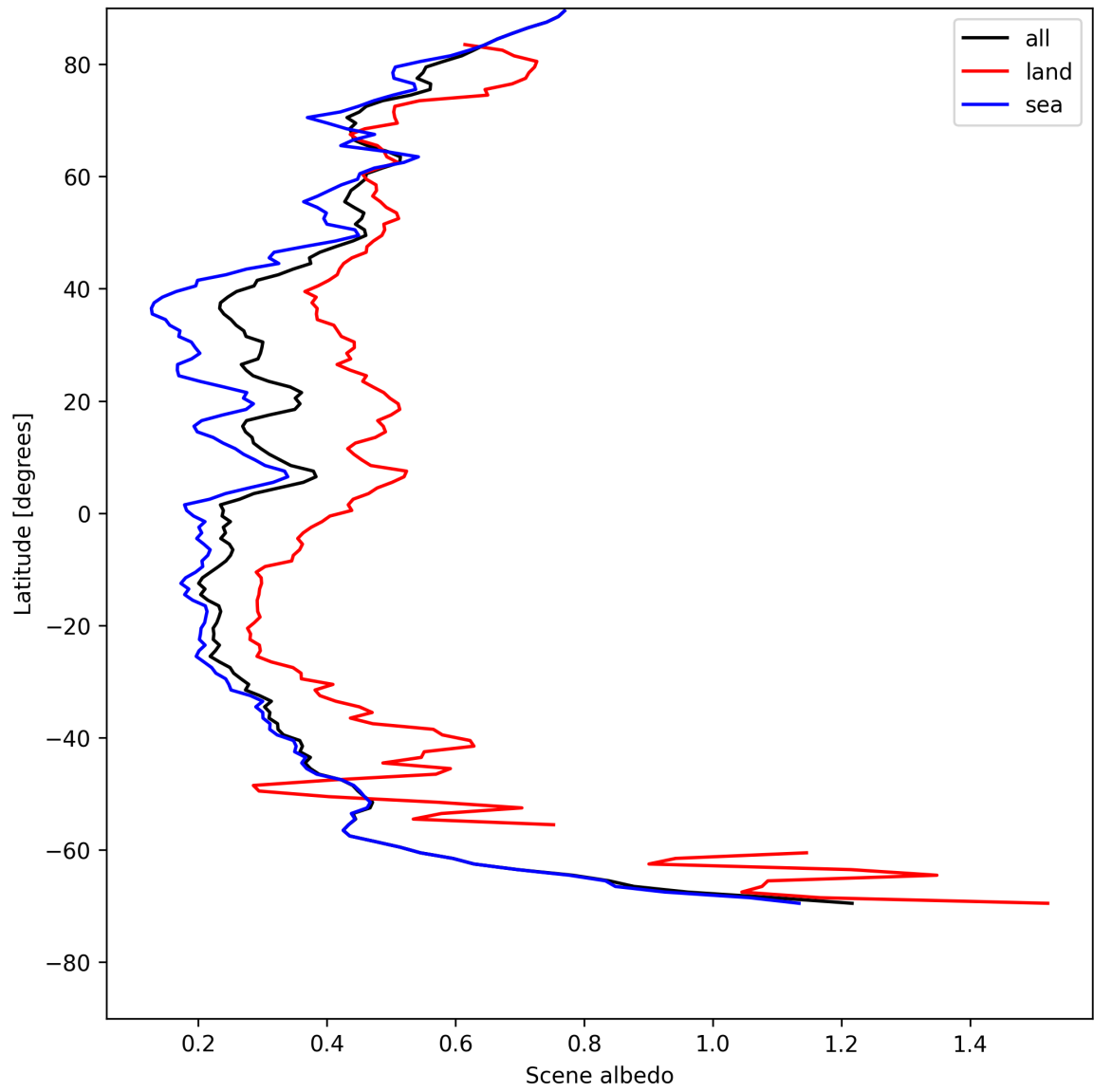
Figure 15: Zonal average of “Scene albedo” for 2025-07-29 to 2025-07-30.
