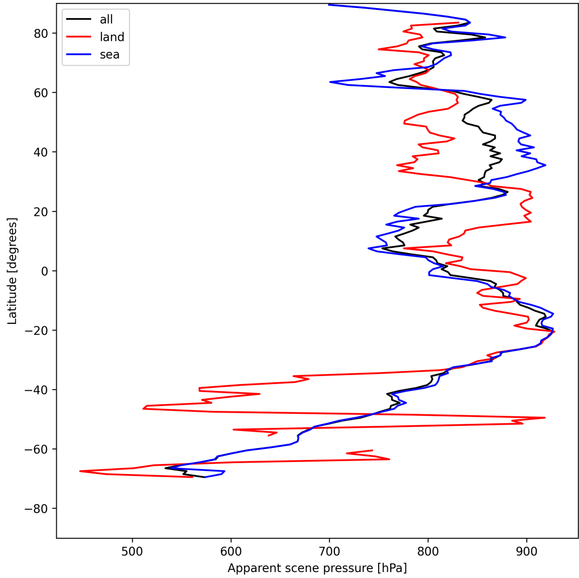
Figure 17: Zonal average of “Apparent scene pressure” for 2025-07-29 to 2025-07-30.
