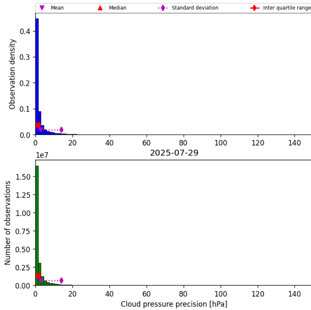
Figure 29: Histogram of “Cloud pressure precision” for 2025-07-29 to 2025-07-30
