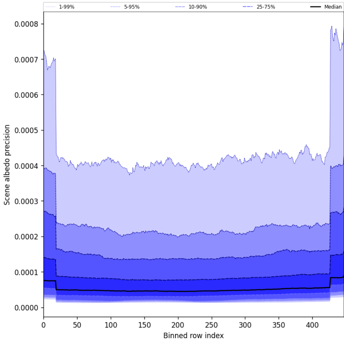
Figure 50: Along track statistics of “Scene albedo precision” for 2025-07-29 to 2025-07-30
