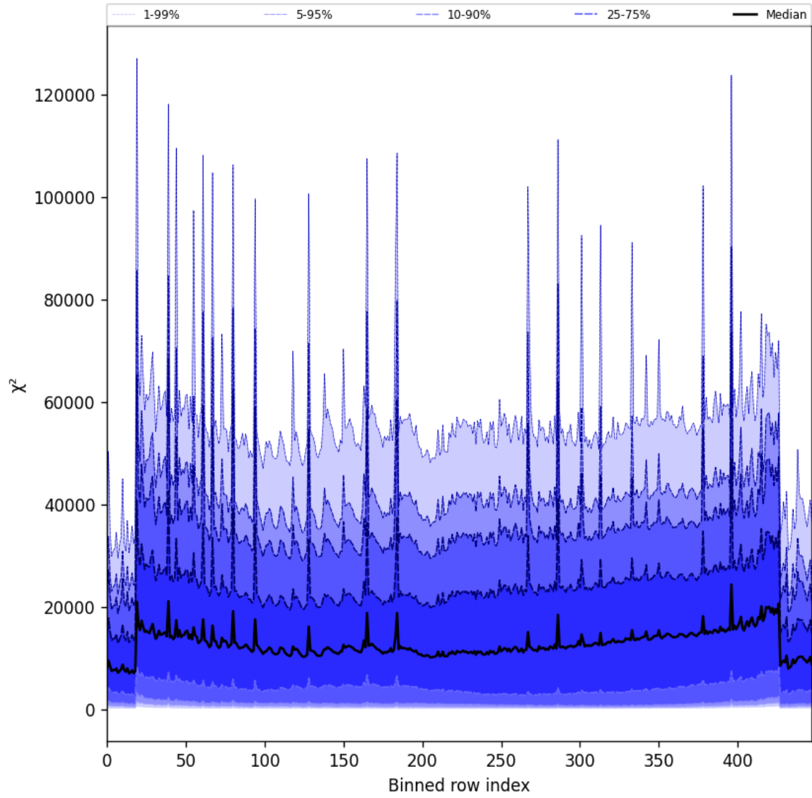
Figure 53: Along track statistics of “ \chi^2 ” for 2025-07-29 to 2025-07-30
