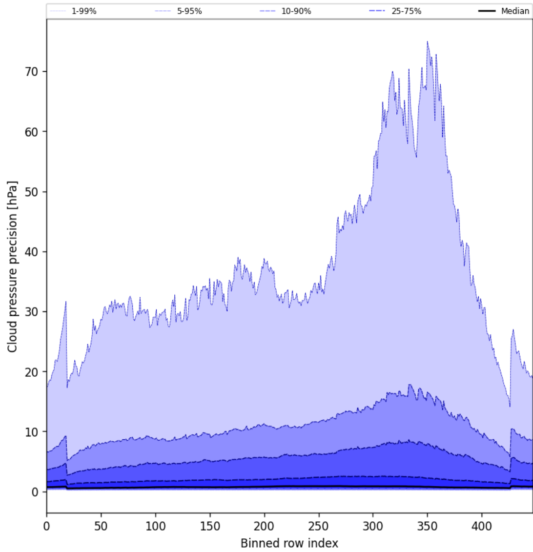
Figure 46: Along track statistics of “Cloud pressure precision” for 2025-07-29 to 2025-07-30
