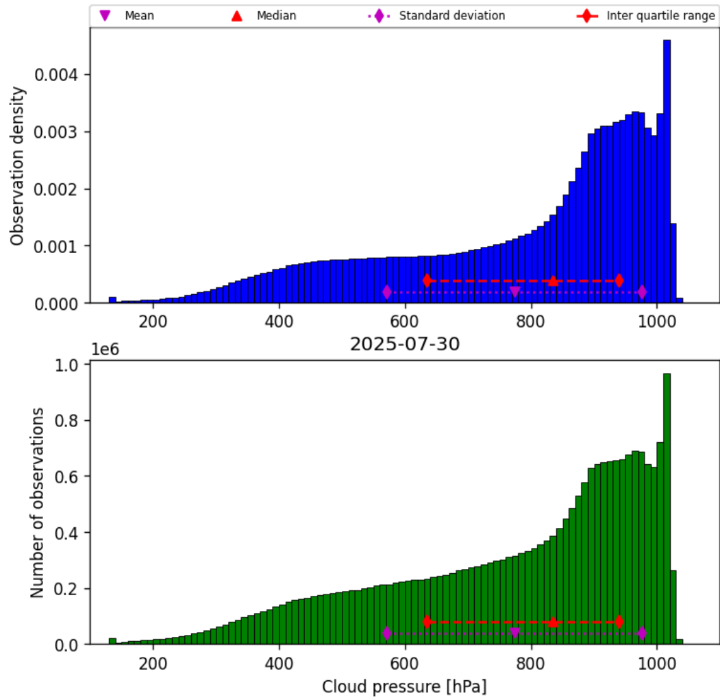
Figure 28: Histogram of “Cloud pressure” for 2025-07-30 to 2025-07-31
