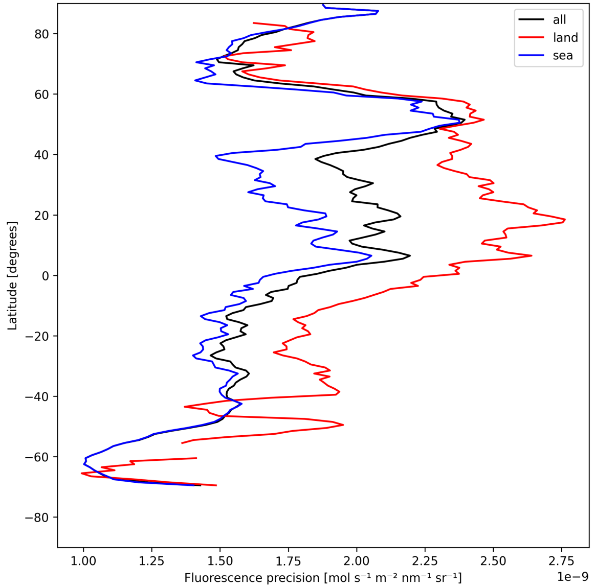
Figure 22: Zonal average of “Fluorescence precision” for 2025-07-30 to 2025-07-31.
