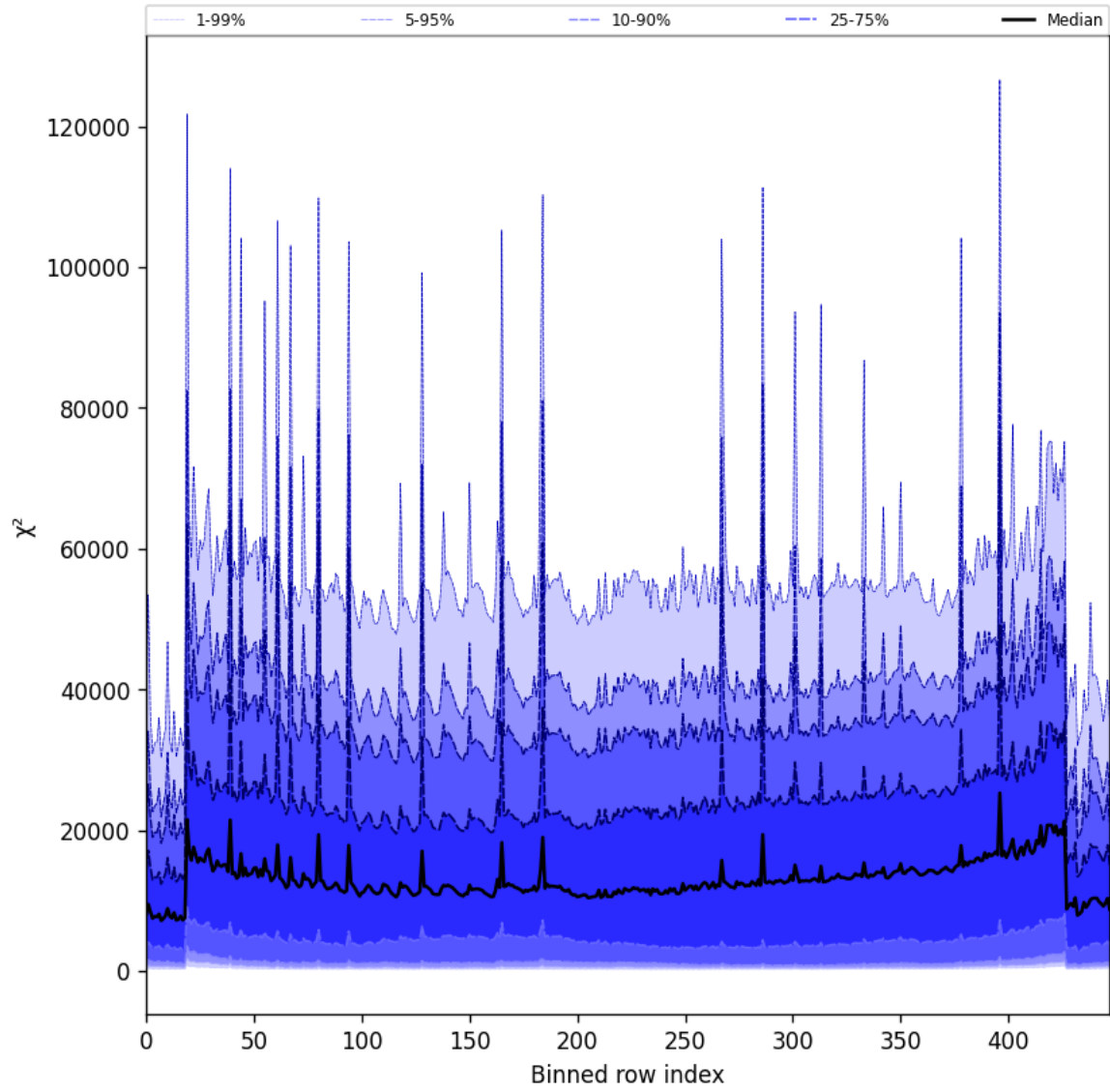
Figure 53: Along track statistics of “ \chi^2 ” for 2025-07-30 to 2025-07-31
