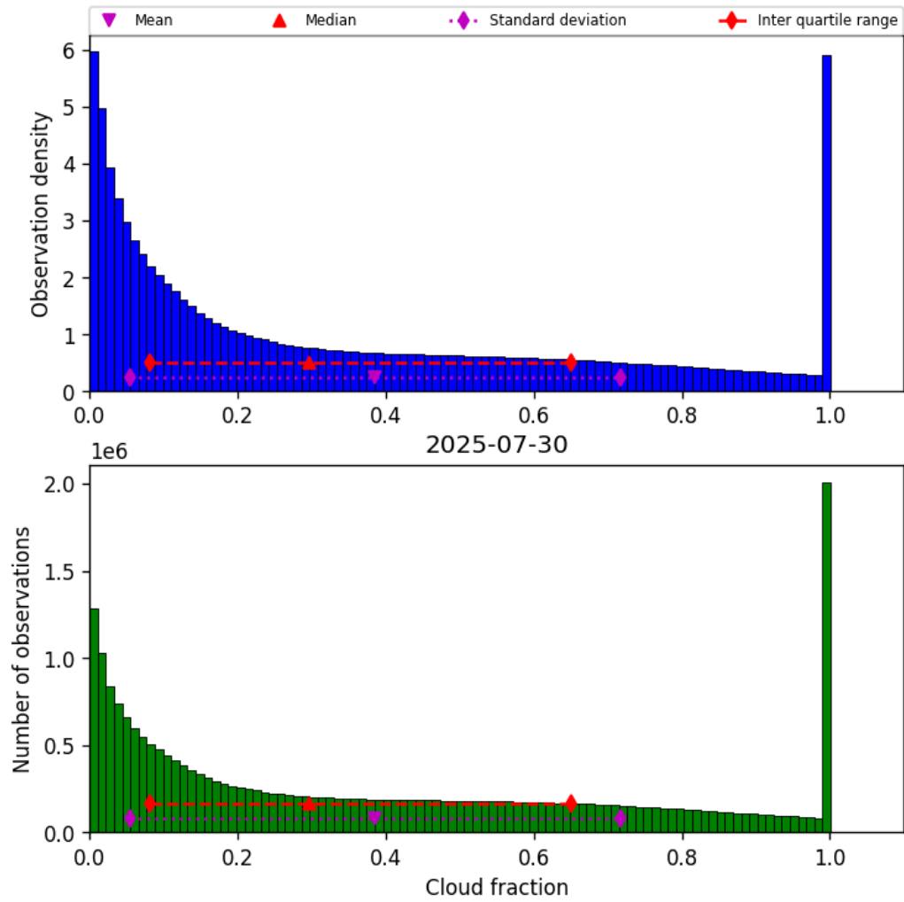
Figure 30: Histogram of “Cloud fraction” for 2025-07-30 to 2025-07-31
