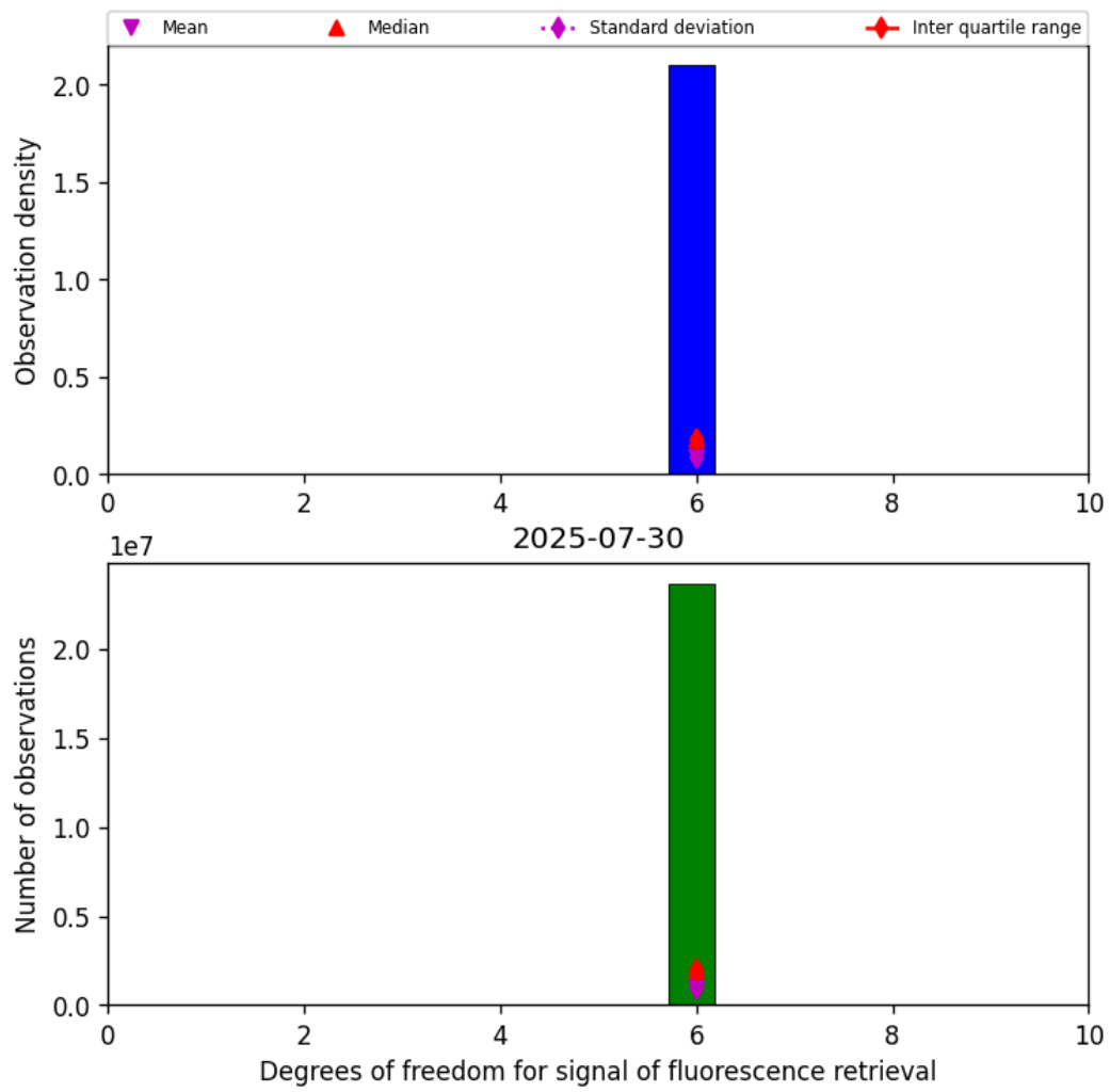
Figure 41: Histogram of “Degrees of freedom for signal of fluorescence retrieval” for 2025-07-30 to 2025-07-31
