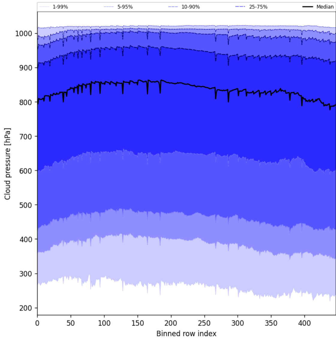
Figure 45: Along track statistics of “Cloud pressure” for 2025-07-30 to 2025-07-31
