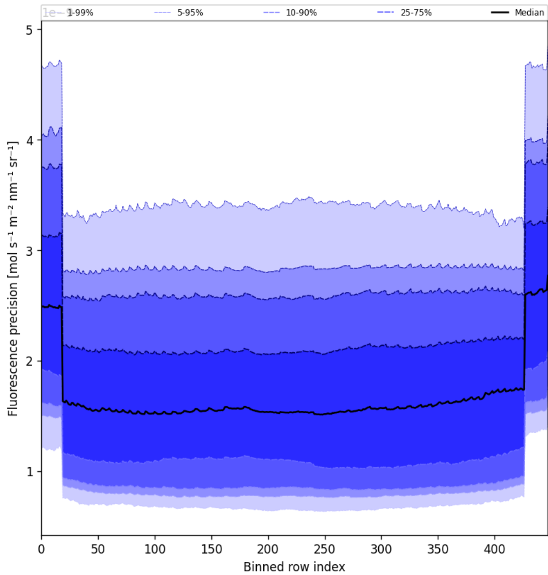
Figure 56: Along track statistics of “Fluorescence precision” for 2025-07-30 to 2025-07-31
