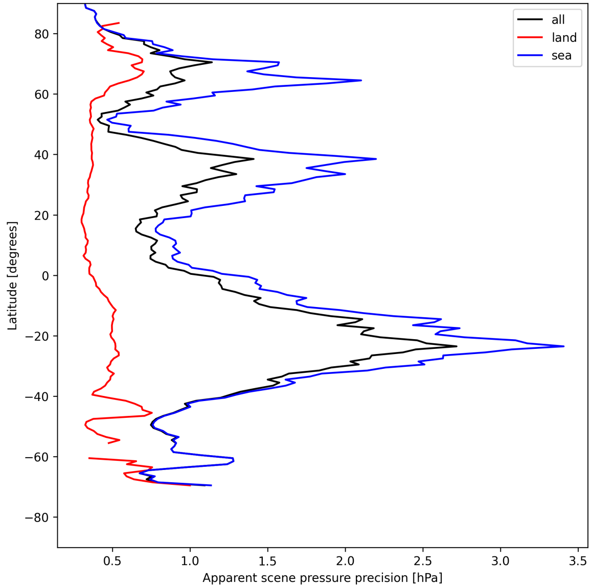
Figure 18: Zonal average of “Apparent scene pressure precision” for 2025-07-30 to 2025-07-31.
