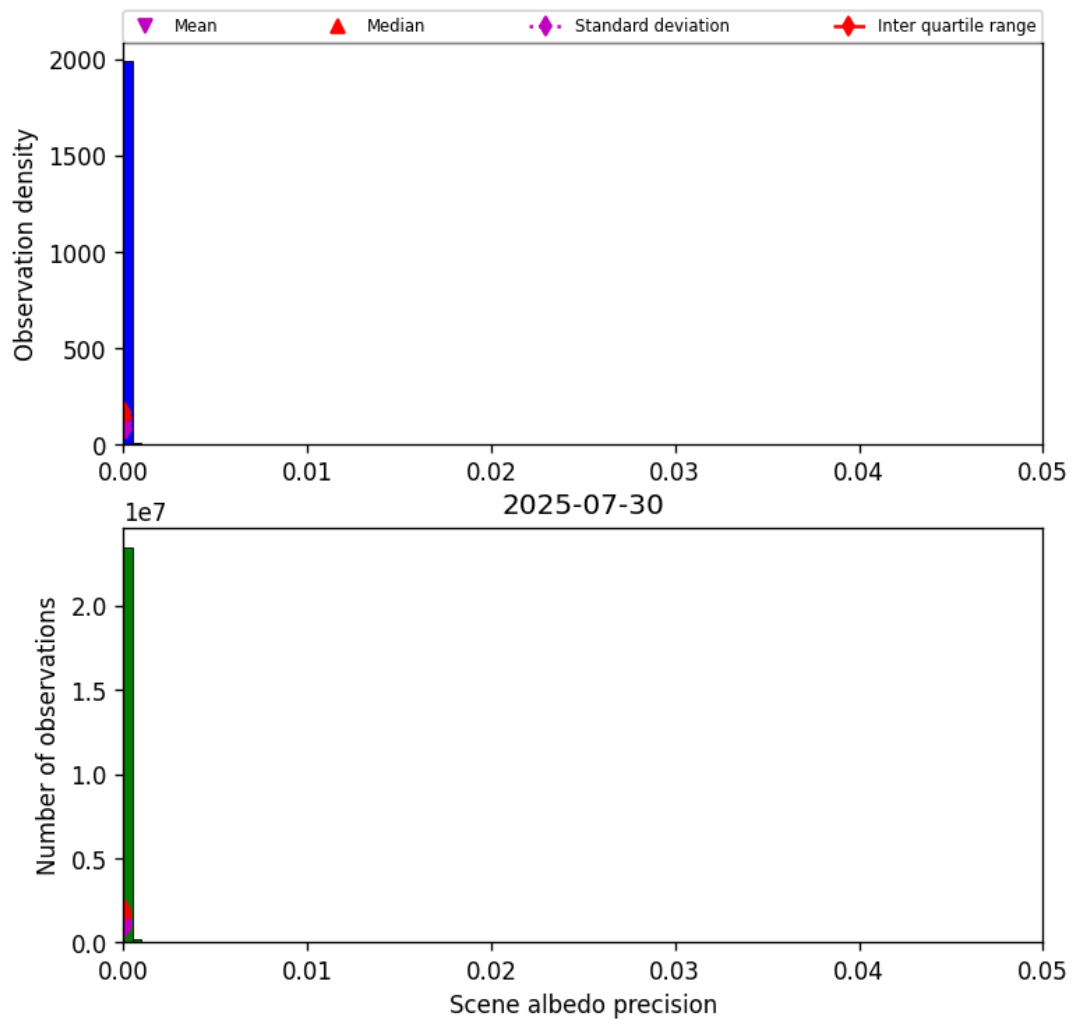
Figure 33: Histogram of “Scene albedo precision” for 2025-07-30 to 2025-07-31
