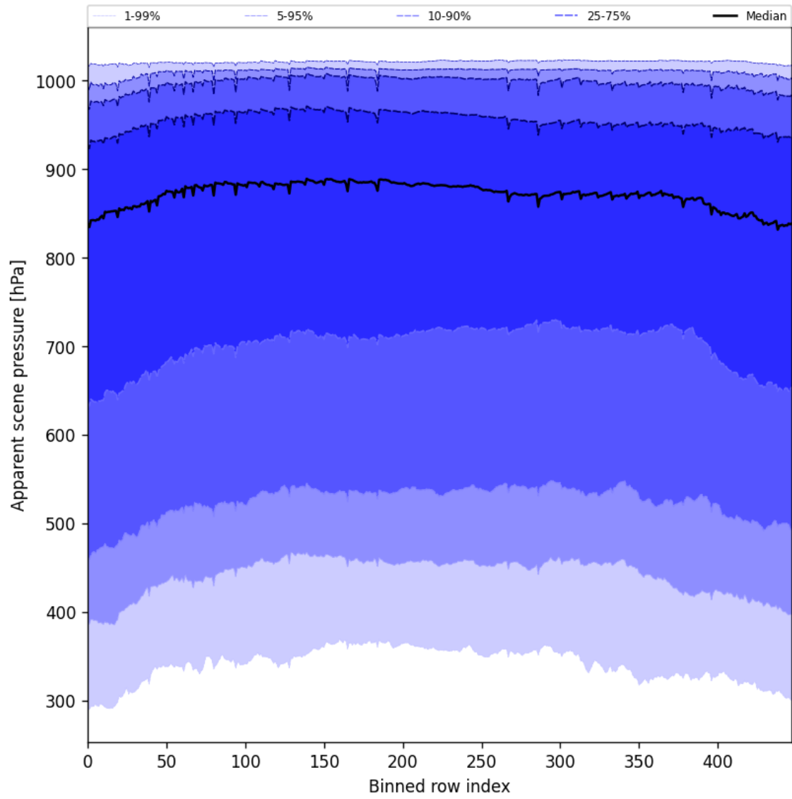
Figure 51: Along track statistics of “Apparent scene pressure” for 2025-07-30 to 2025-07-31
