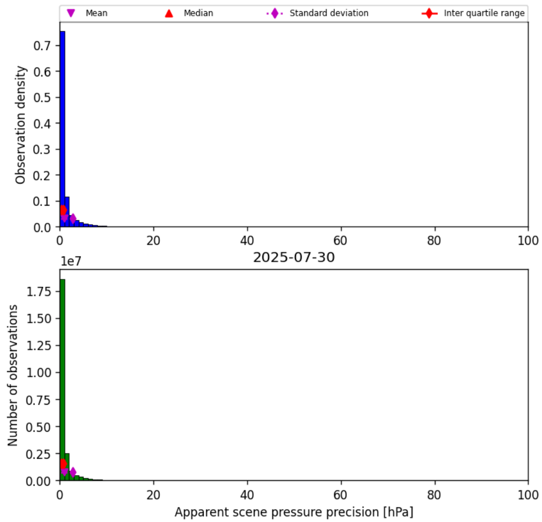
Figure 35: Histogram of “Apparent scene pressure precision” for 2025-07-30 to 2025-07-31
