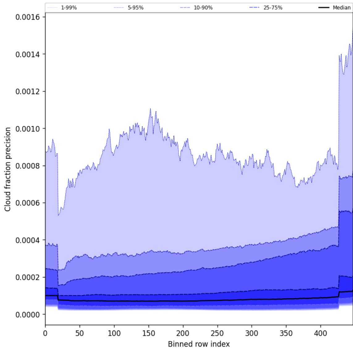
Figure 48: Along track statistics of “Cloud fraction precision” for 2025-07-30 to 2025-07-31
