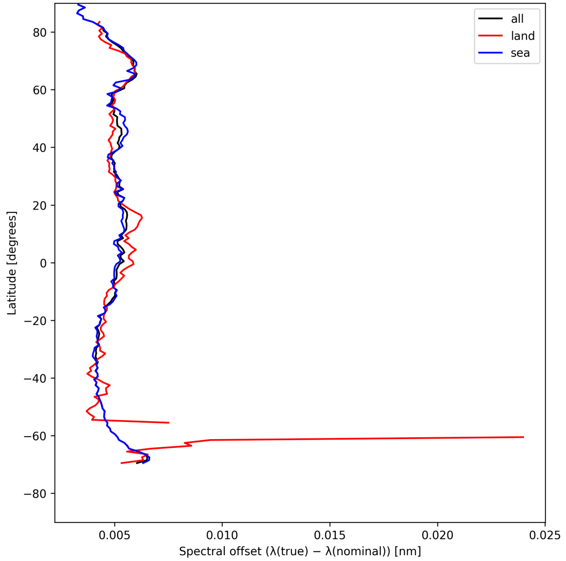
Figure 26: Zonal average of “Spectral offset ( \lambda_{\text{true}} - \lambda_{\text{nominal}} )” for 2025-07-30 to 2025-07-31.
