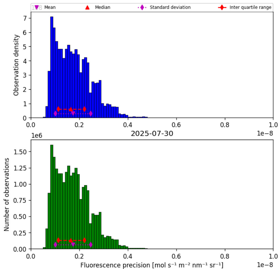
Figure 39: Histogram of “Fluorescence precision” for 2025-07-30 to 2025-07-31
