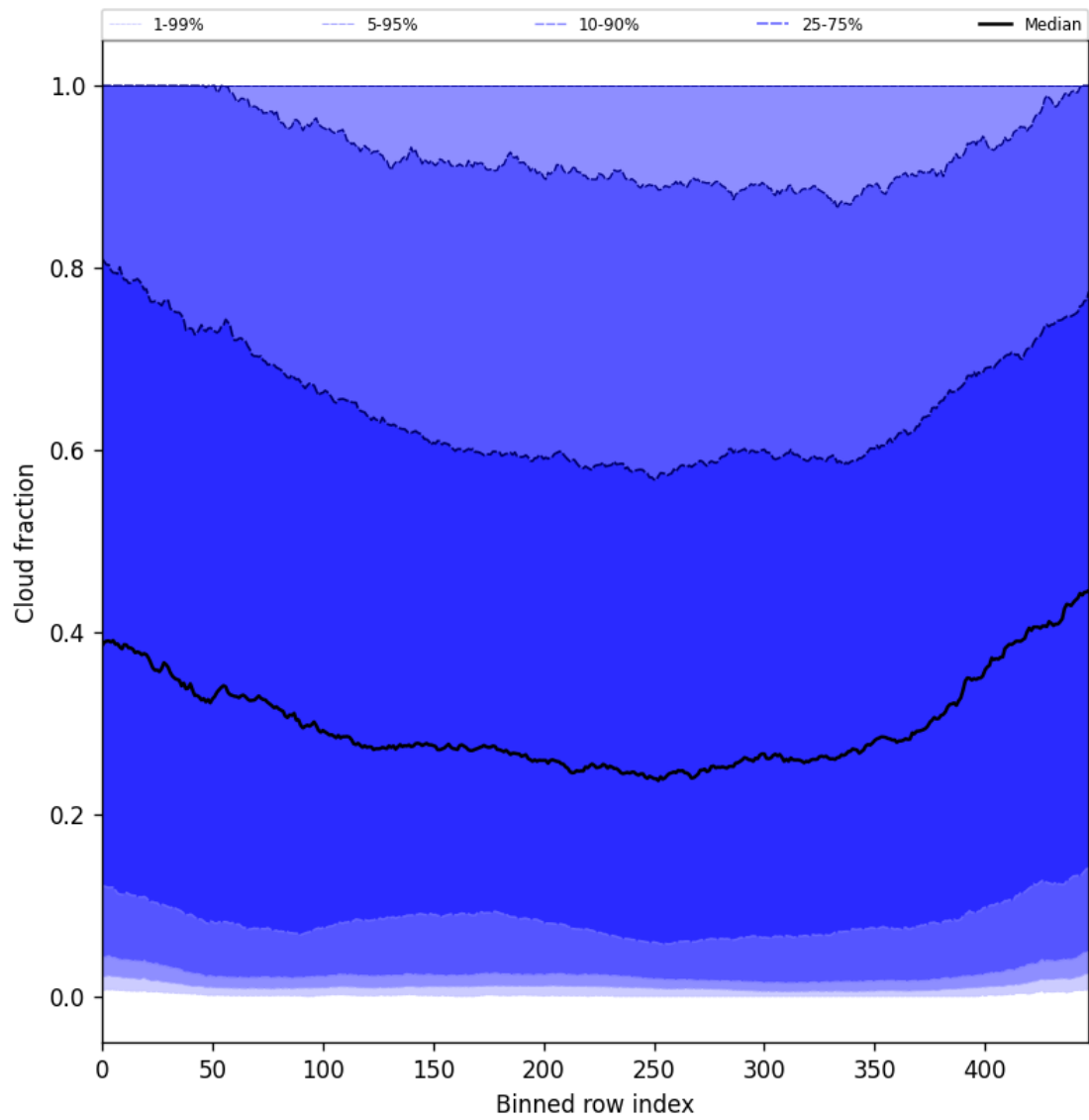
Figure 47: Along track statistics of “Cloud fraction” for 2025-07-30 to 2025-07-31
