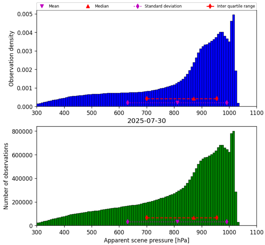
Figure 34: Histogram of “Apparent scene pressure” for 2025-07-30 to 2025-07-31
