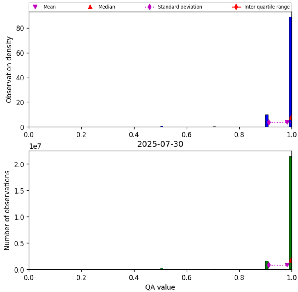
Figure 27: Histogram of “QA value” for 2025-07-30 to 2025-07-31
