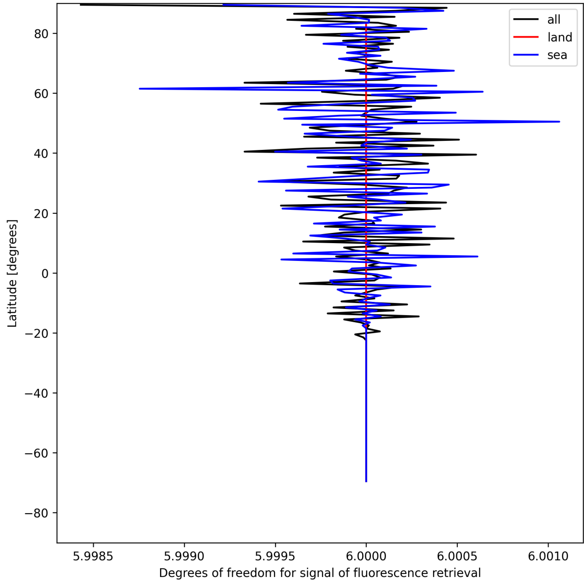
Figure 24: Zonal average of “Degrees of freedom for signal of fluorescence retrieval” for 2025-07-30 to 2025-07-31.
