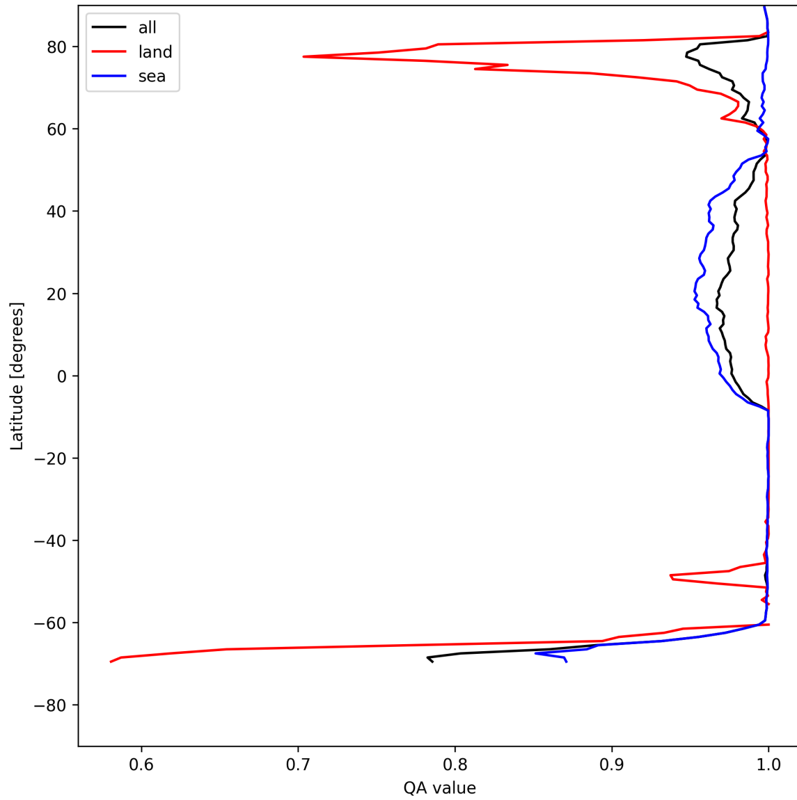
Figure 10: Zonal average of “QA value” for 2025-07-30 to 2025-07-31.
