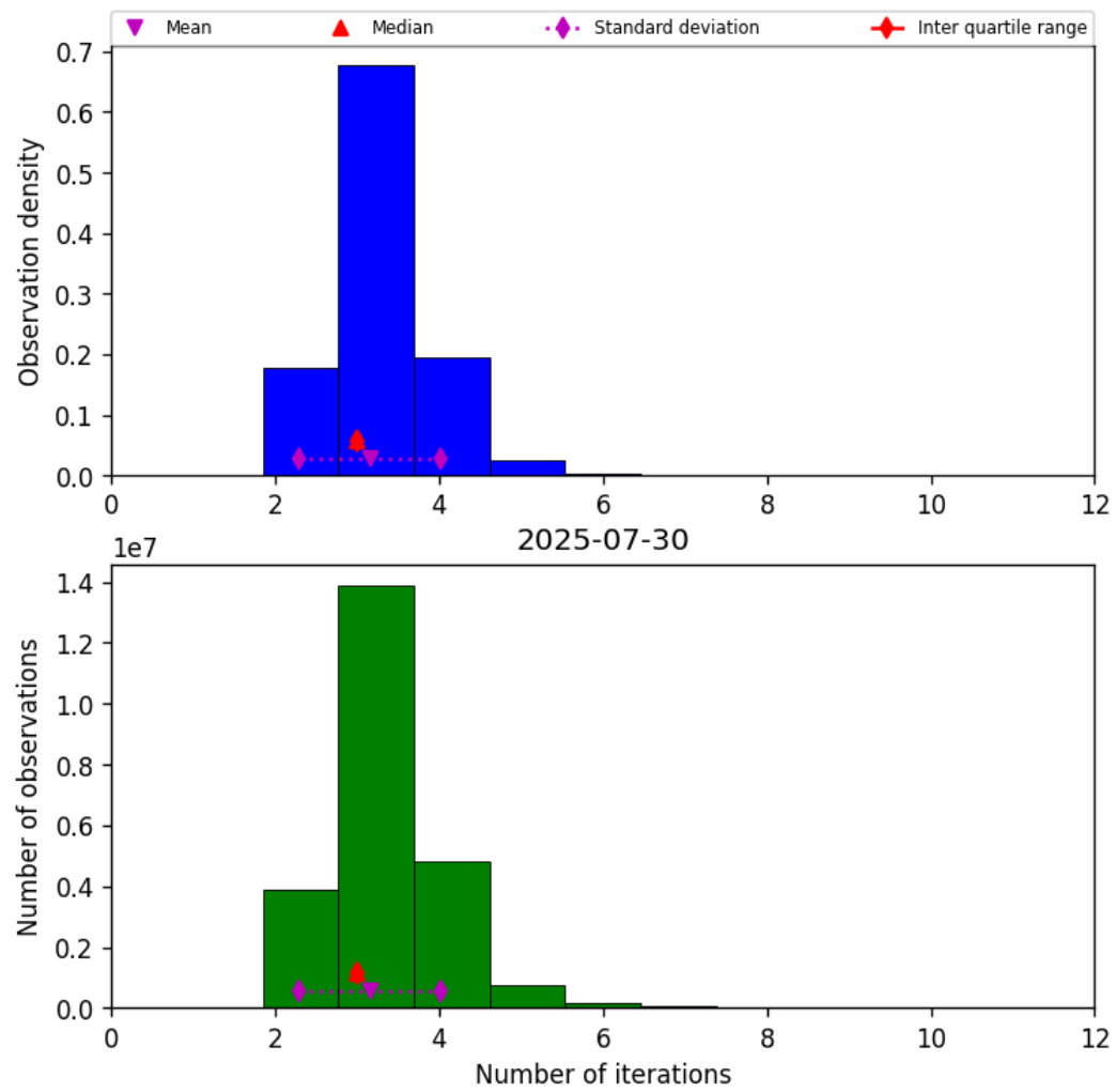
Figure 37: Histogram of “Number of iterations” for 2025-07-30 to 2025-07-31
