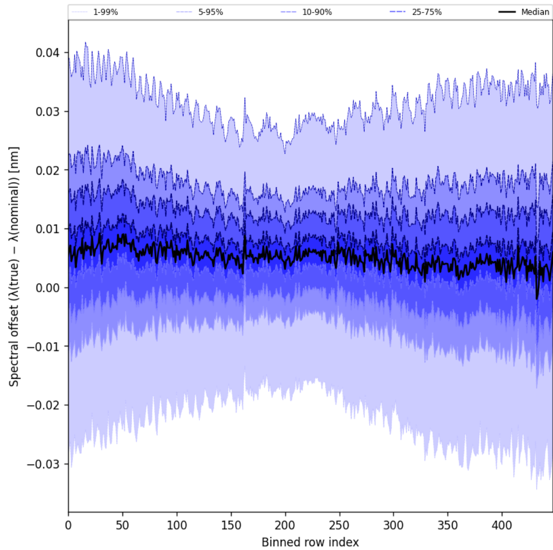
Figure 60: Along track statistics of “Spectral offset ( \lambda_{\text{true}} - \lambda_{\text{nominal}} )” for 2025-07-30 to 2025-07-31
