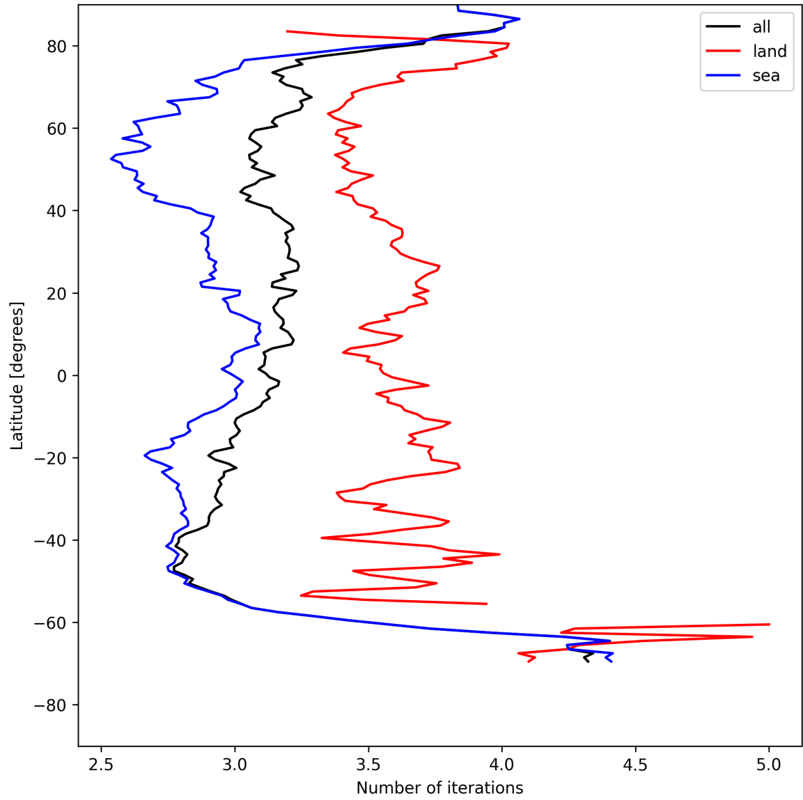
Figure 20: Zonal average of “Number of iterations” for 2025-07-30 to 2025-07-31.
