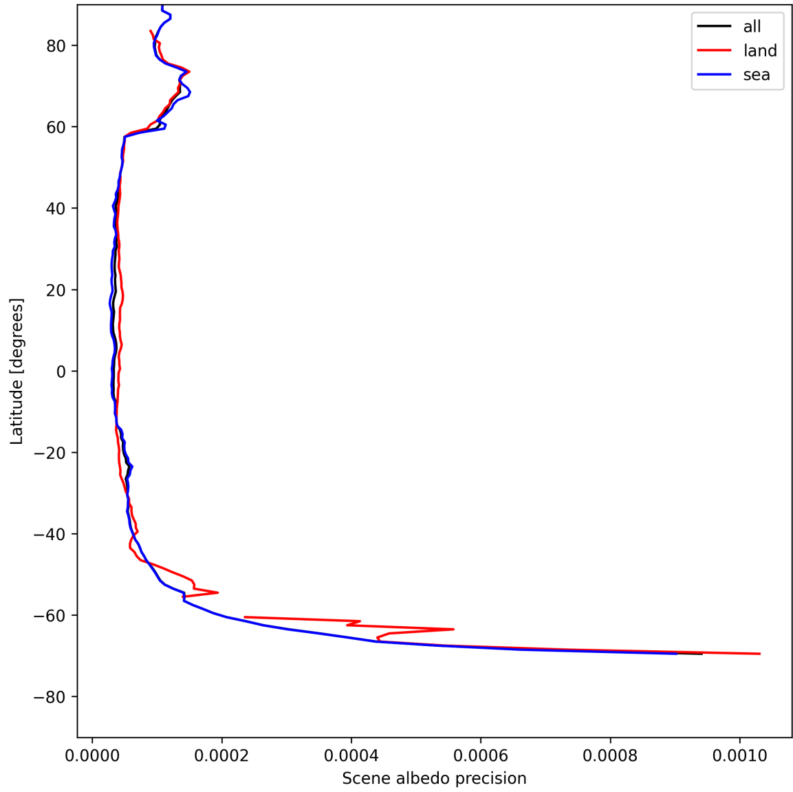
Figure 16: Zonal average of “Scene albedo precision” for 2025-07-30 to 2025-07-31.
