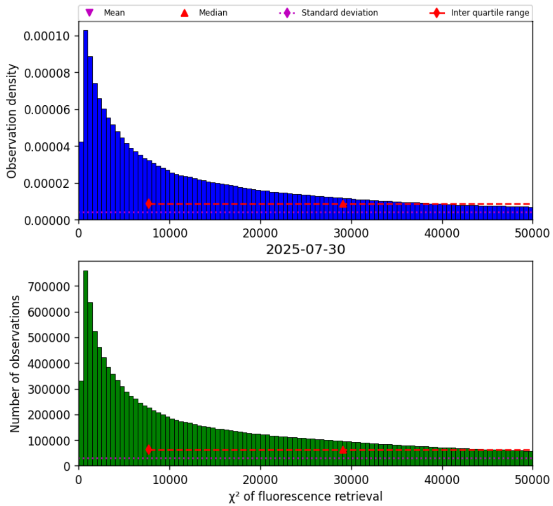
Figure 40: Histogram of “ \chi^2 of fluorescence retrieval” for 2025-07-30 to 2025-07-31
