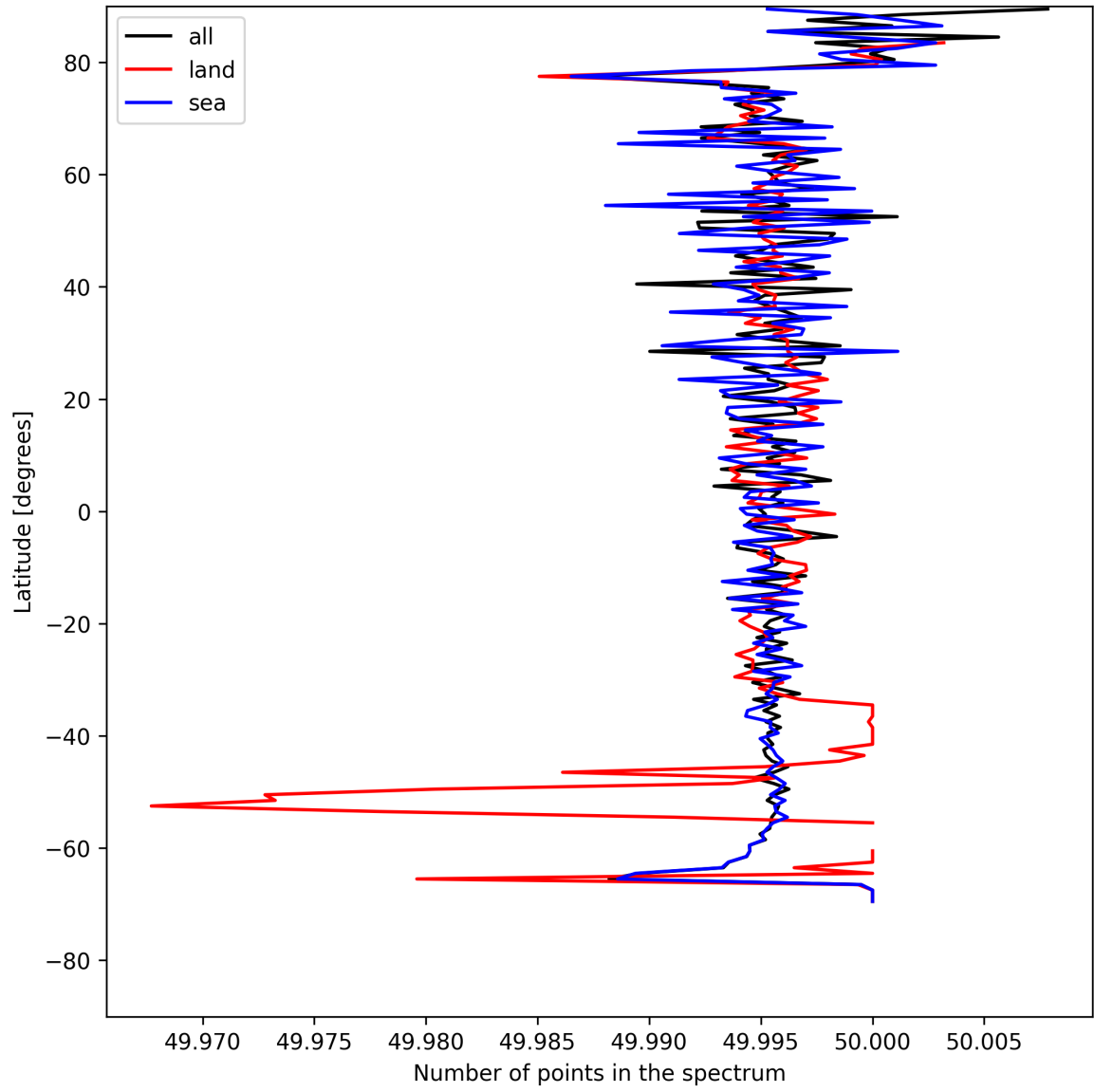
Figure 25: Zonal average of “Number of points in the spectrum” for 2025-07-30 to 2025-07-31.
