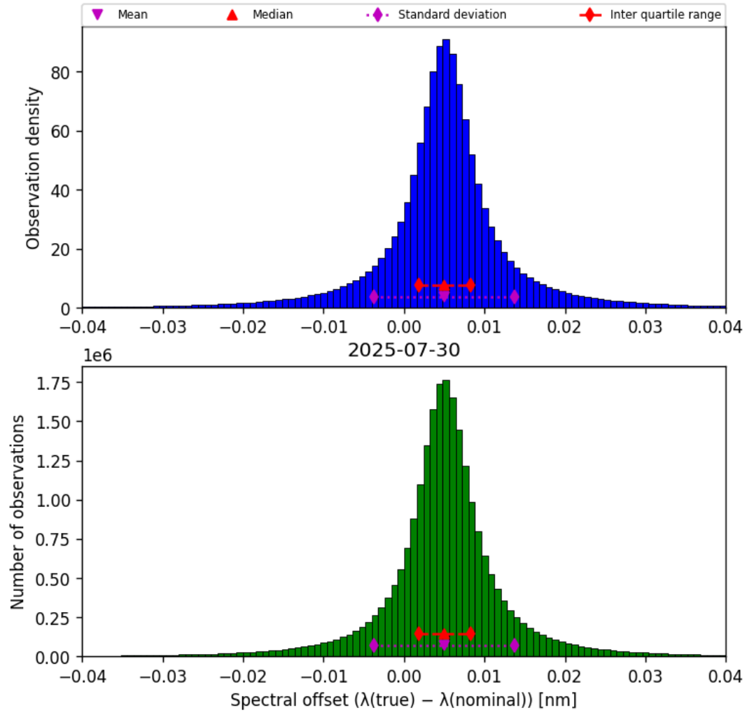
Figure 43: Histogram of “Spectral offset ( \lambda_{\text{true}} - \lambda_{\text{nominal}} )” for 2025-07-30 to 2025-07-31
