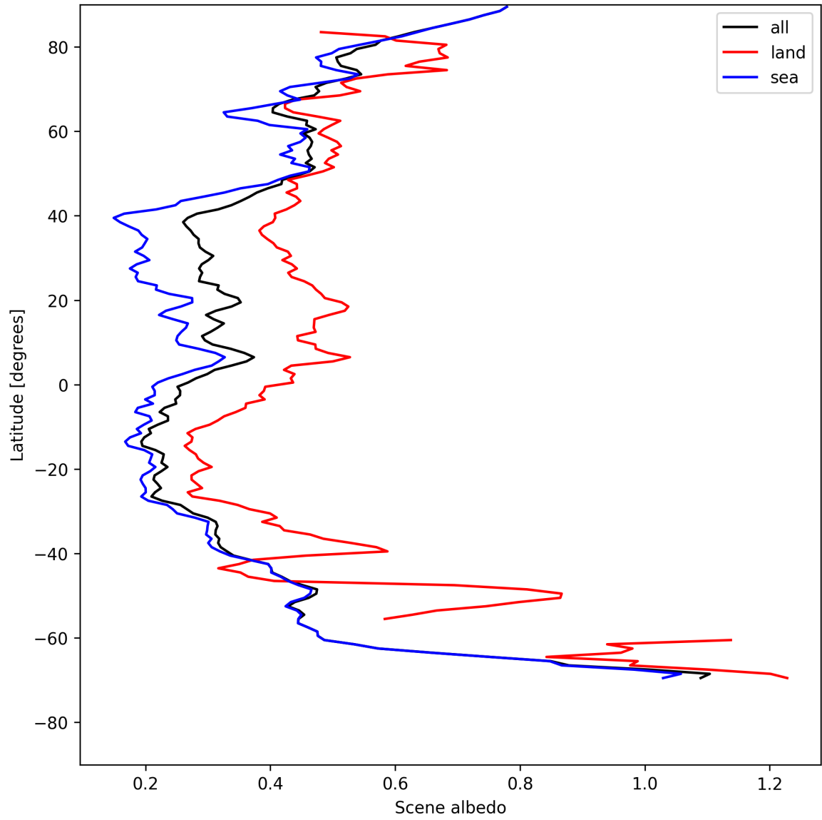
Figure 15: Zonal average of “Scene albedo” for 2025-07-30 to 2025-07-31.
