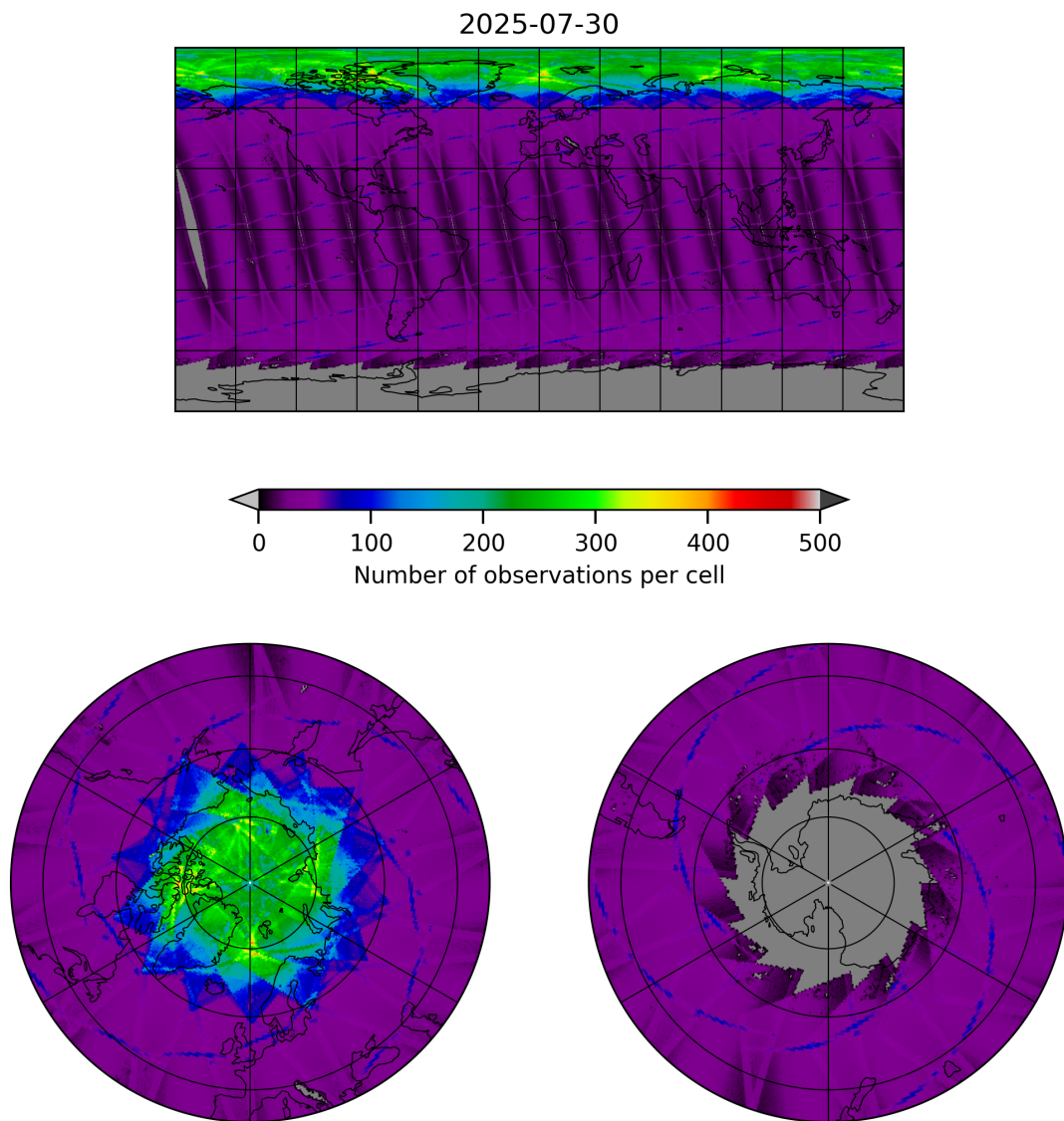
Figure 9: Map of the number of observations for 2025-07-30 to 2025-07-31
