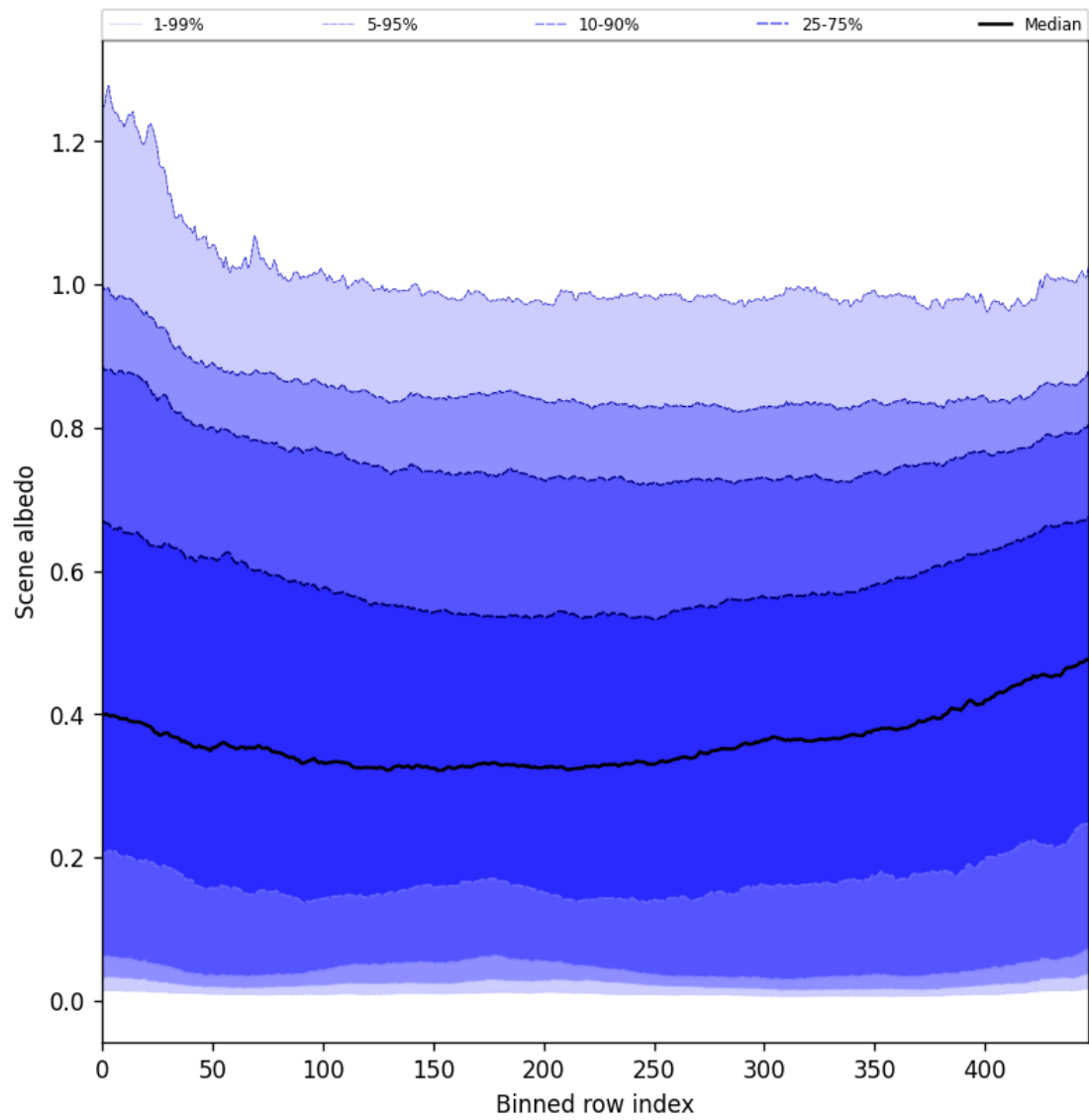
Figure 49: Along track statistics of “Scene albedo” for 2025-07-30 to 2025-07-31
