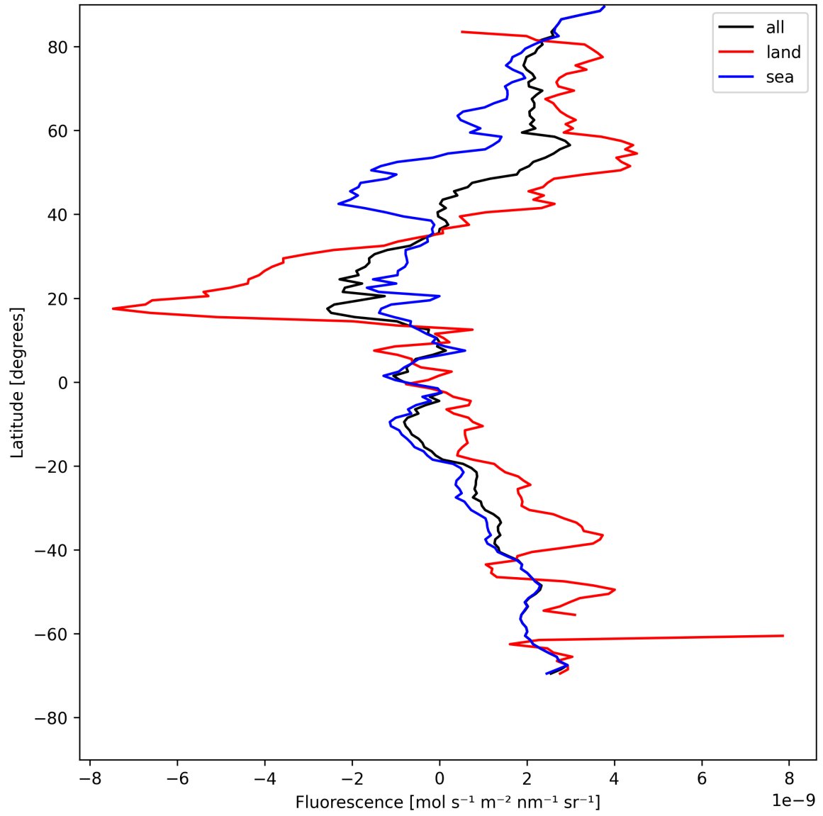
Figure 21: Zonal average of “Fluorescence” for 2025-07-30 to 2025-07-31.
