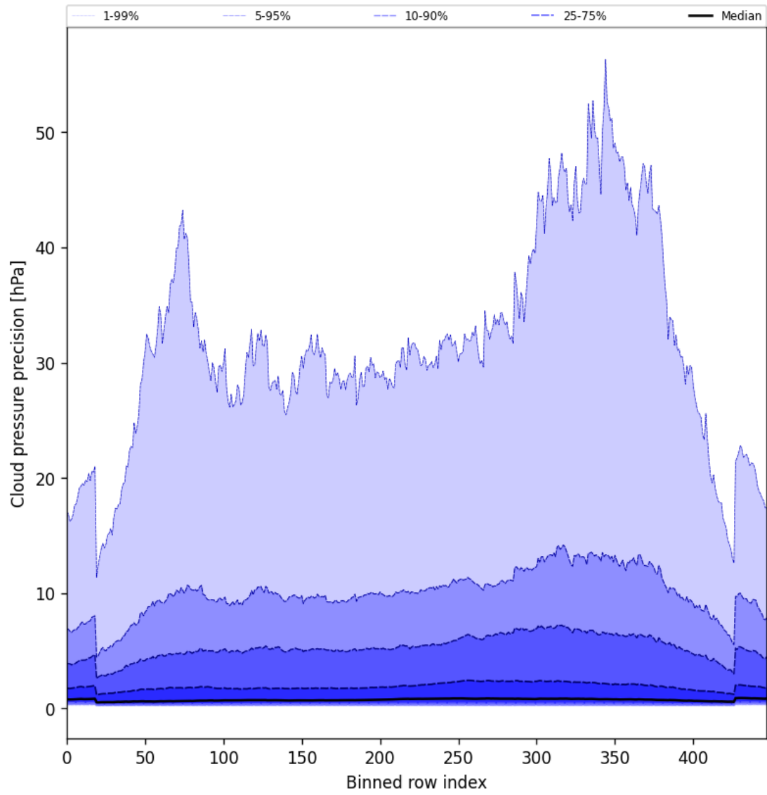
Figure 46: Along track statistics of “Cloud pressure precision” for 2025-07-30 to 2025-07-31
