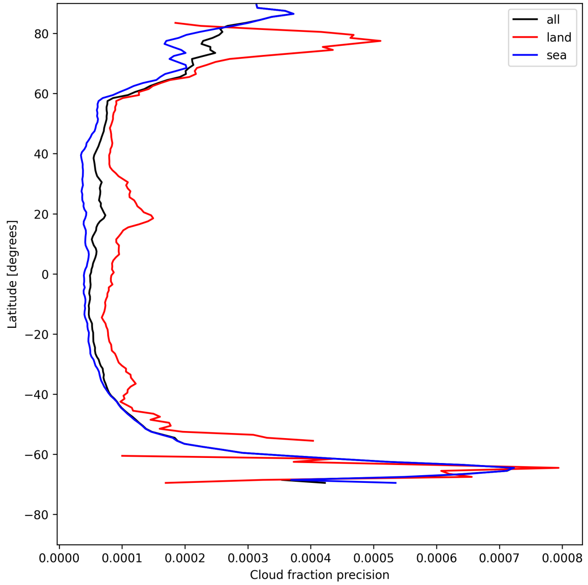
Figure 14: Zonal average of “Cloud fraction precision” for 2025-07-30 to 2025-07-31.
