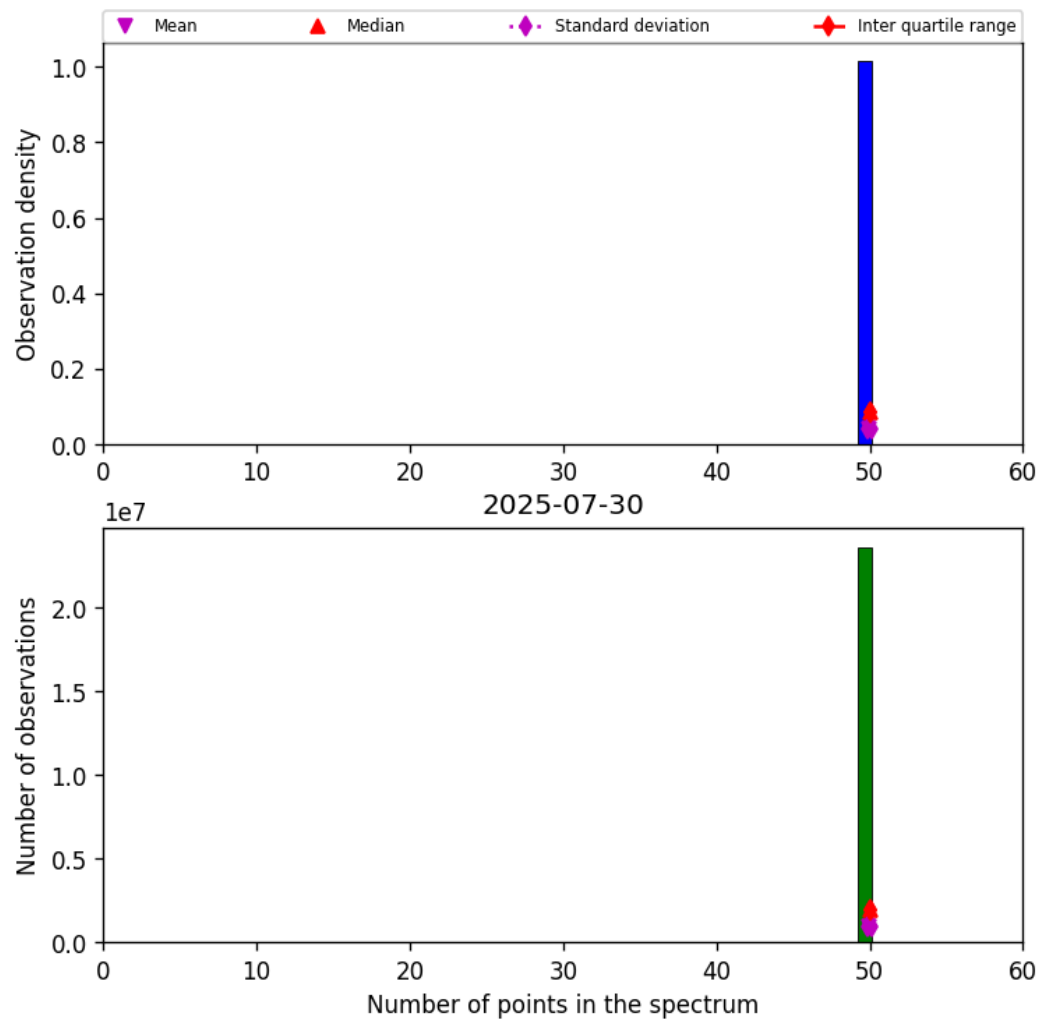
Figure 42: Histogram of “Number of points in the spectrum” for 2025-07-30 to 2025-07-31
