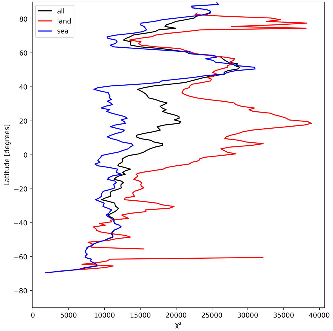
Figure 19: Zonal average of “ \chi^2 ” for 2025-07-30 to 2025-07-31.
