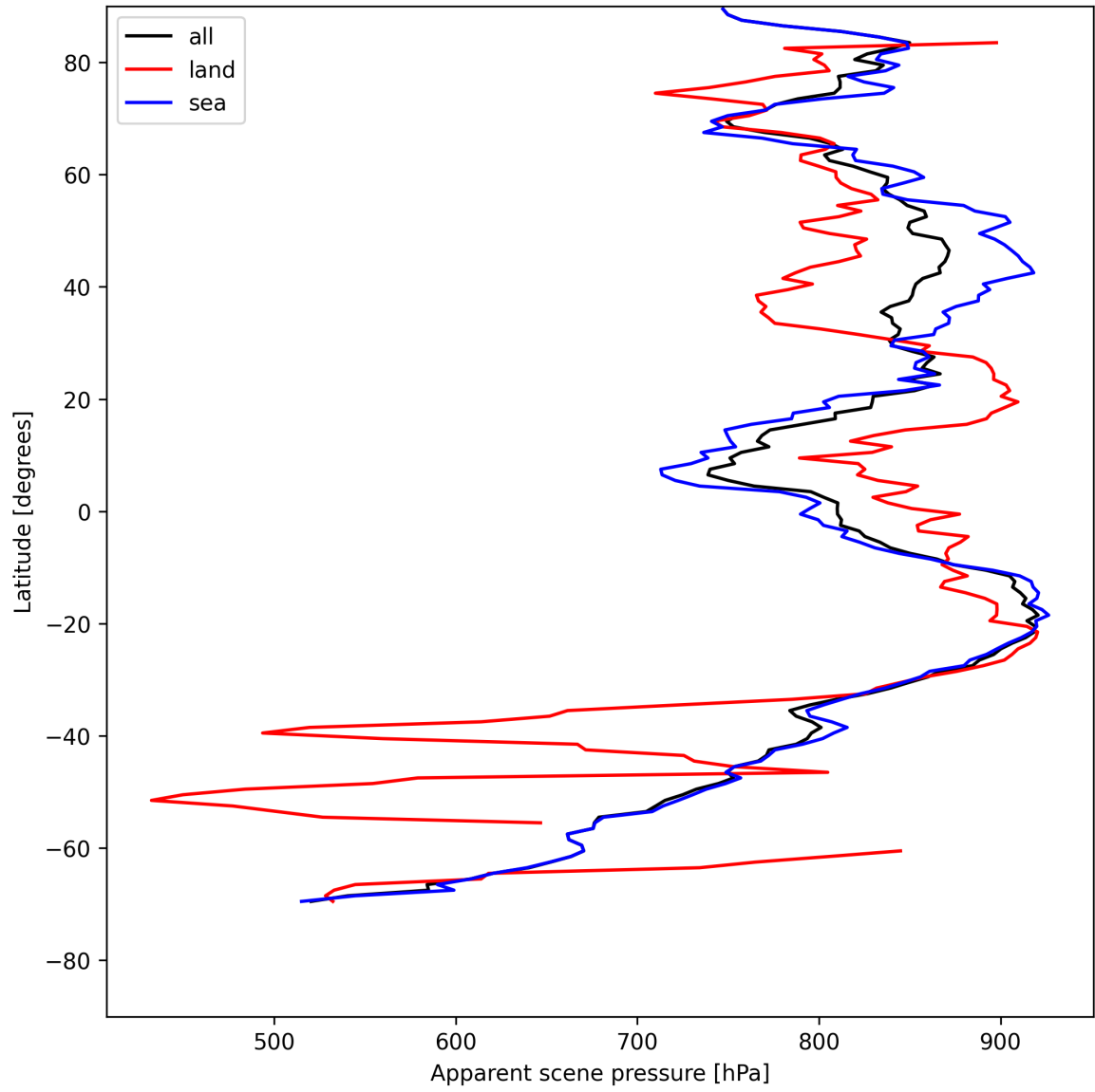
Figure 17: Zonal average of “Apparent scene pressure” for 2025-07-30 to 2025-07-31.
