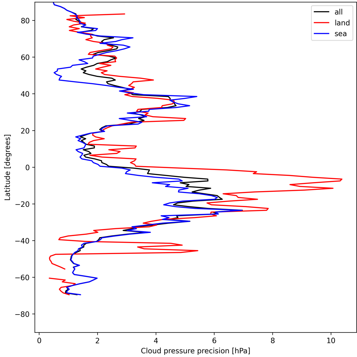
Figure 12: Zonal average of “Cloud pressure precision” for 2025-07-30 to 2025-07-31.
