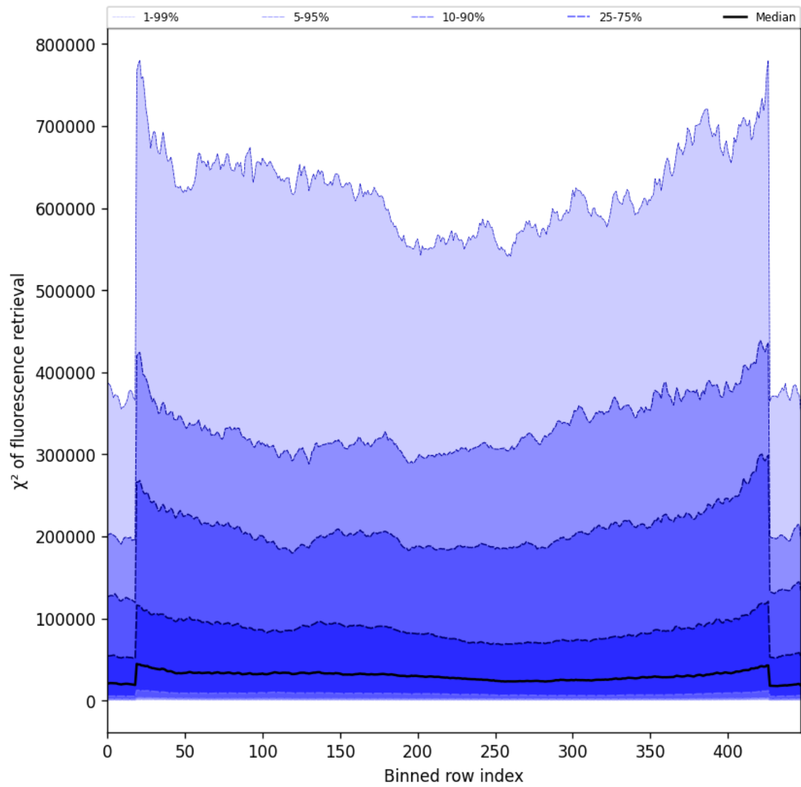
Figure 57: Along track statistics of “ \chi^2 of fluorescence retrieval” for 2025-07-30 to 2025-07-31
