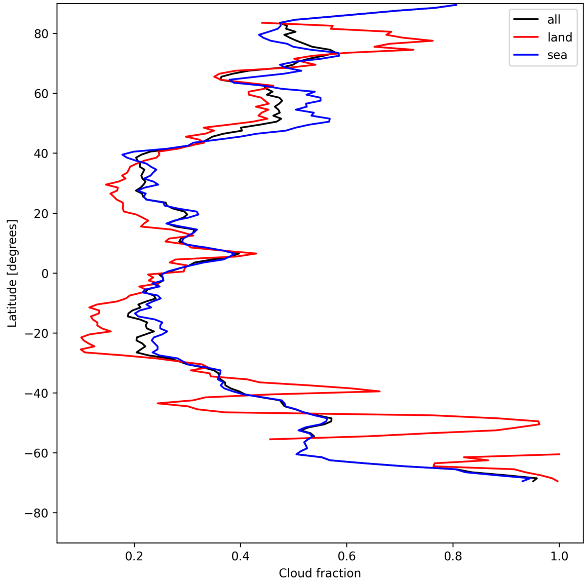
Figure 13: Zonal average of “Cloud fraction” for 2025-07-30 to 2025-07-31.
