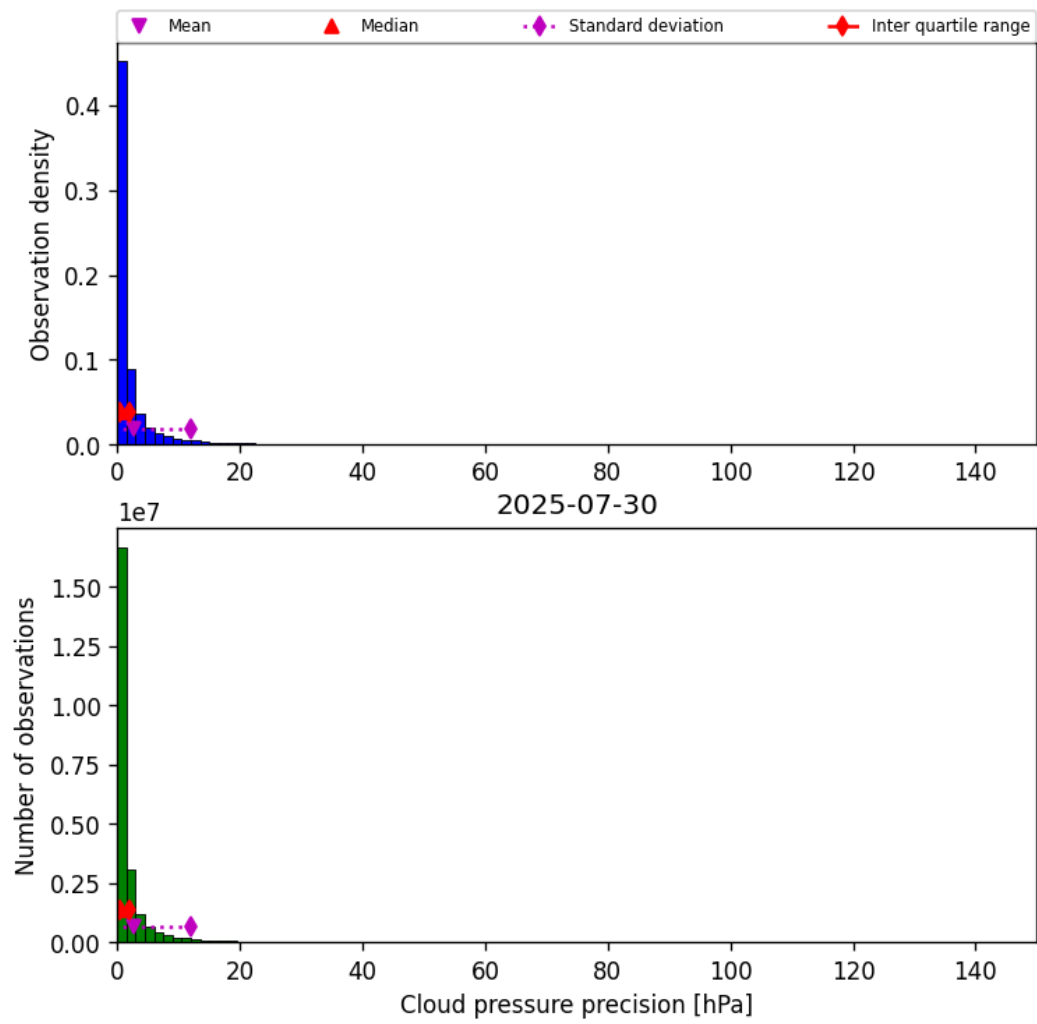
Figure 29: Histogram of “Cloud pressure precision” for 2025-07-30 to 2025-07-31
