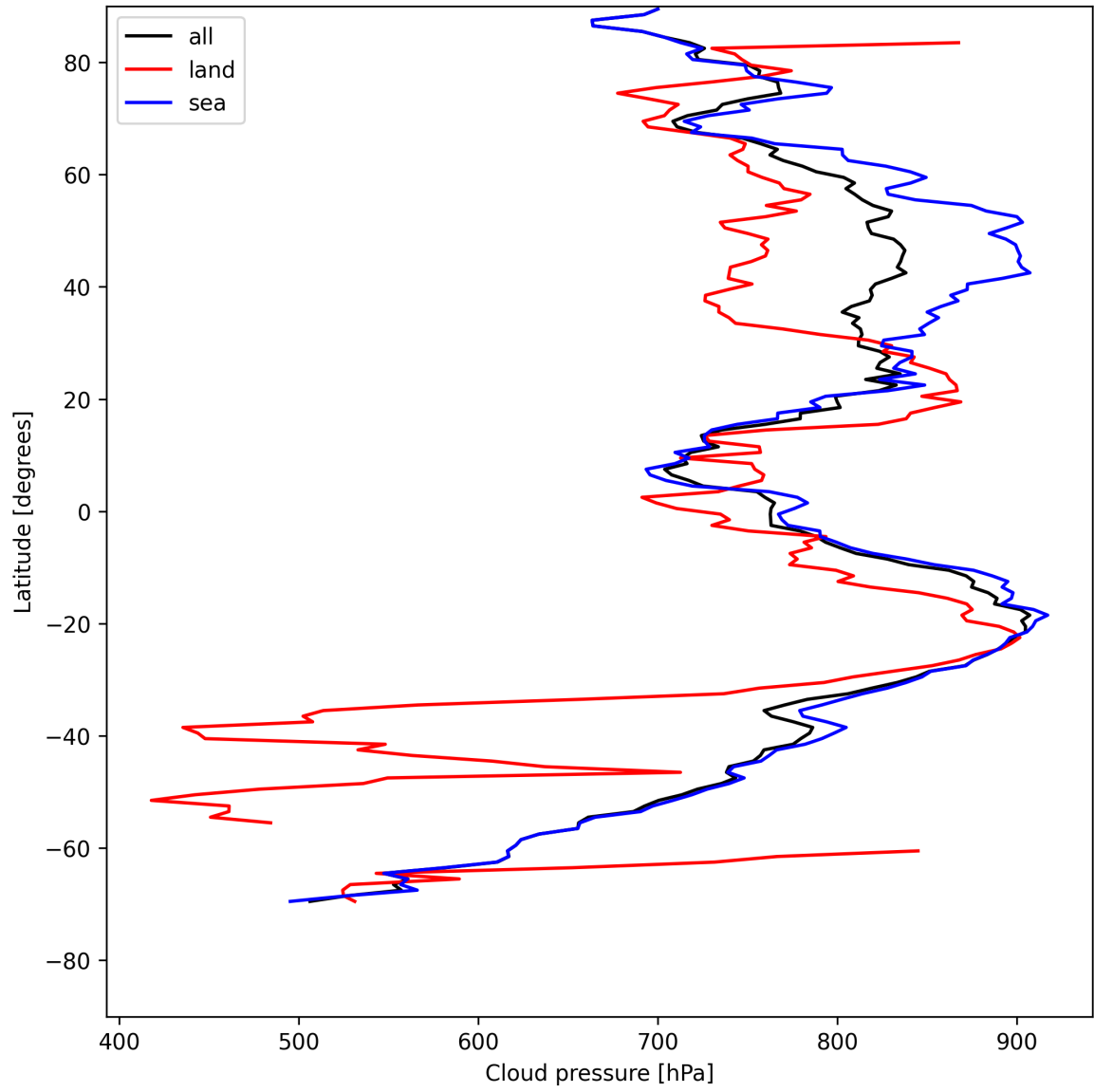
Figure 11: Zonal average of “Cloud pressure” for 2025-07-30 to 2025-07-31.
