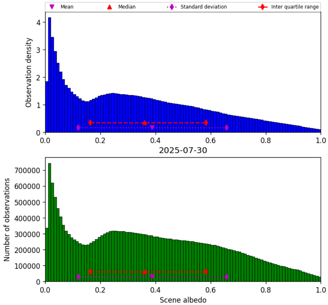
Figure 32: Histogram of “Scene albedo” for 2025-07-30 to 2025-07-31
