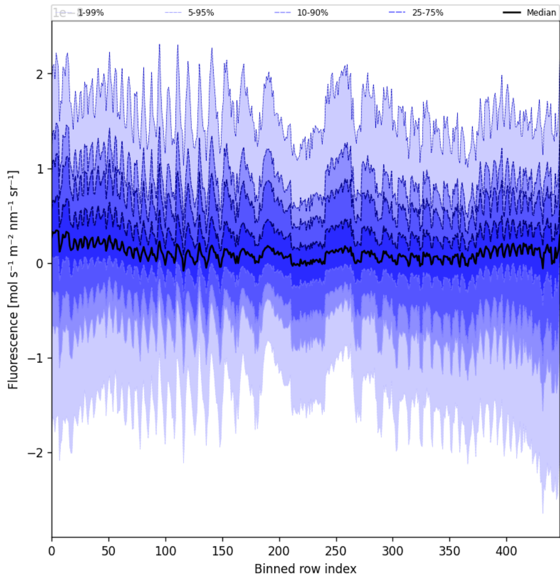
Figure 55: Along track statistics of “Fluorescence” for 2025-07-30 to 2025-07-31
