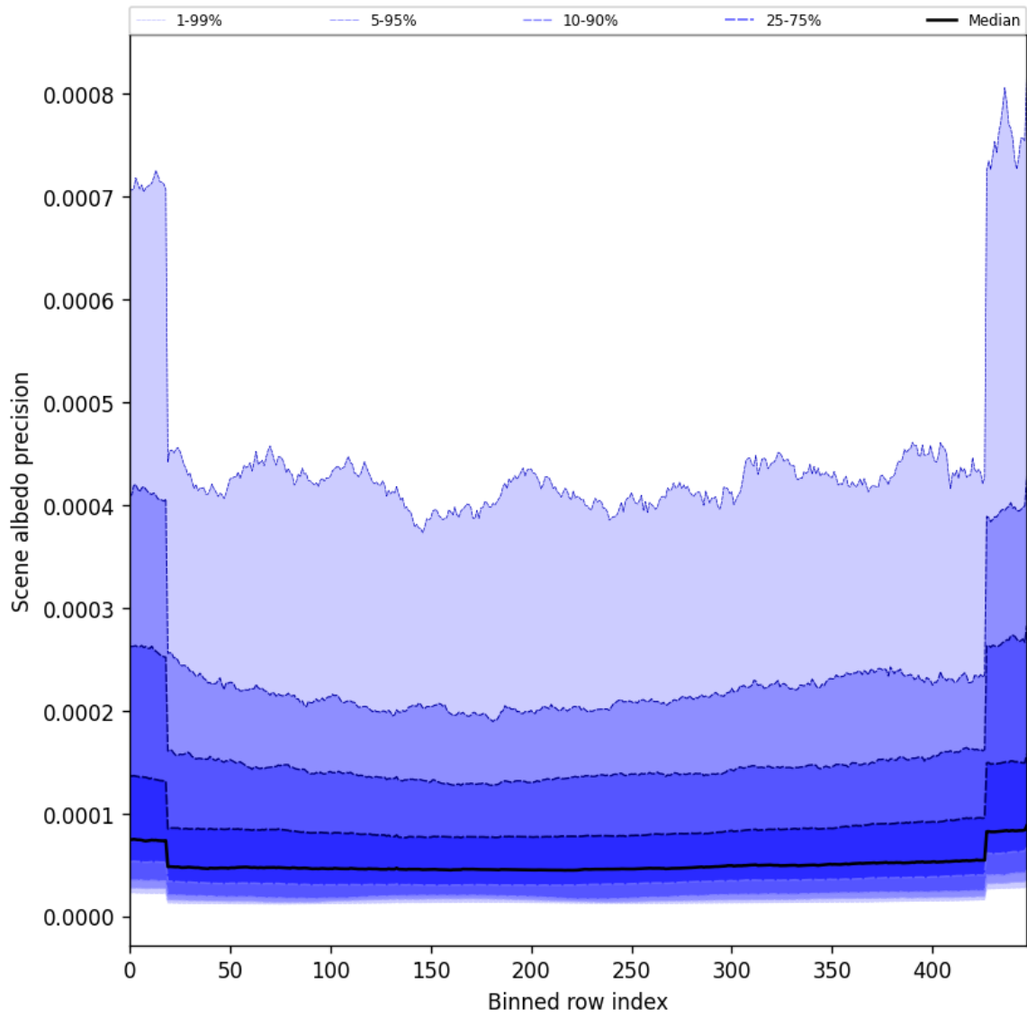
Figure 50: Along track statistics of “Scene albedo precision” for 2025-07-30 to 2025-07-31
