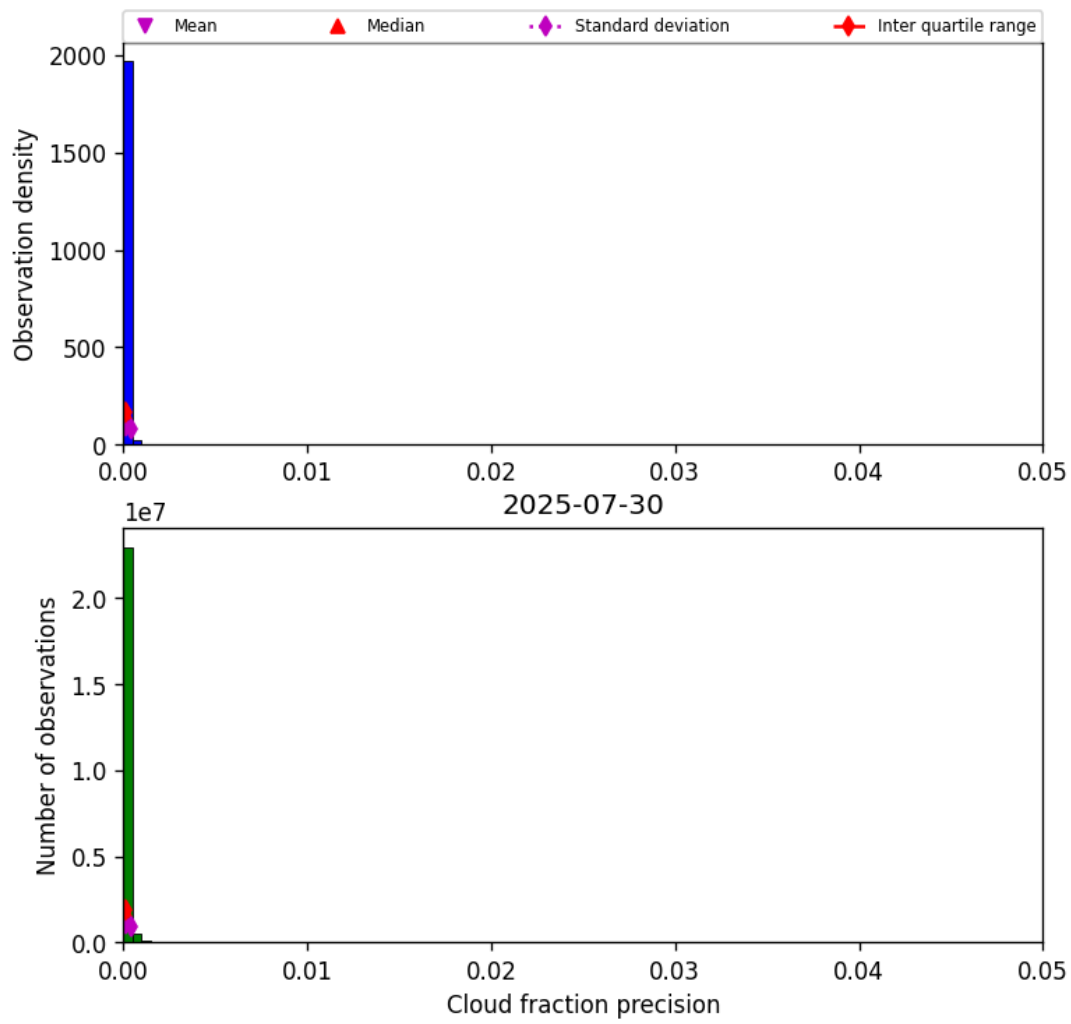
Figure 31: Histogram of “Cloud fraction precision” for 2025-07-30 to 2025-07-31
