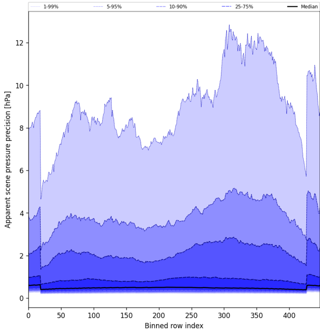
Figure 52: Along track statistics of “Apparent scene pressure precision” for 2025-07-30 to 2025-07-31
