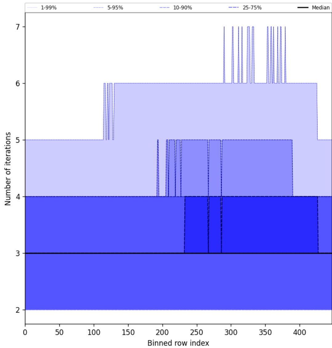
Figure 54: Along track statistics of “Number of iterations” for 2025-07-30 to 2025-07-31
