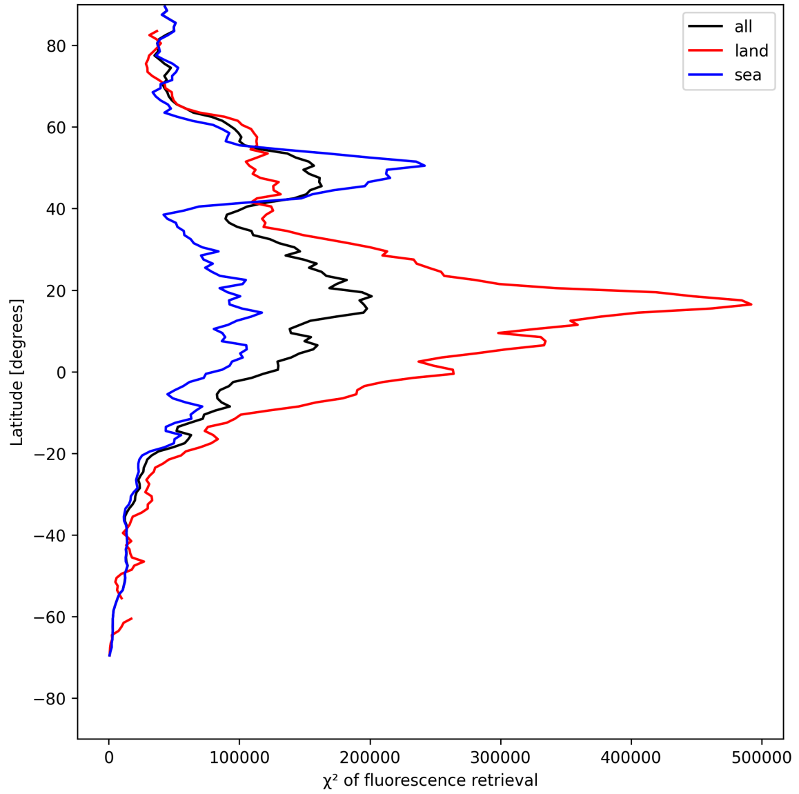
Figure 23: Zonal average of “ \chi^2 of fluorescence retrieval” for 2025-07-30 to 2025-07-31.
