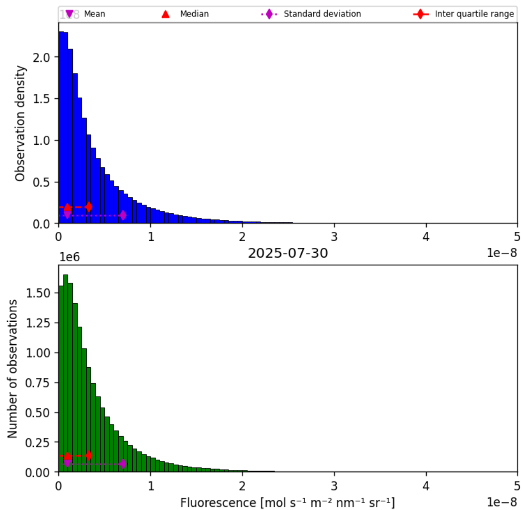
Figure 38: Histogram of “Fluorescence” for 2025-07-30 to 2025-07-31
