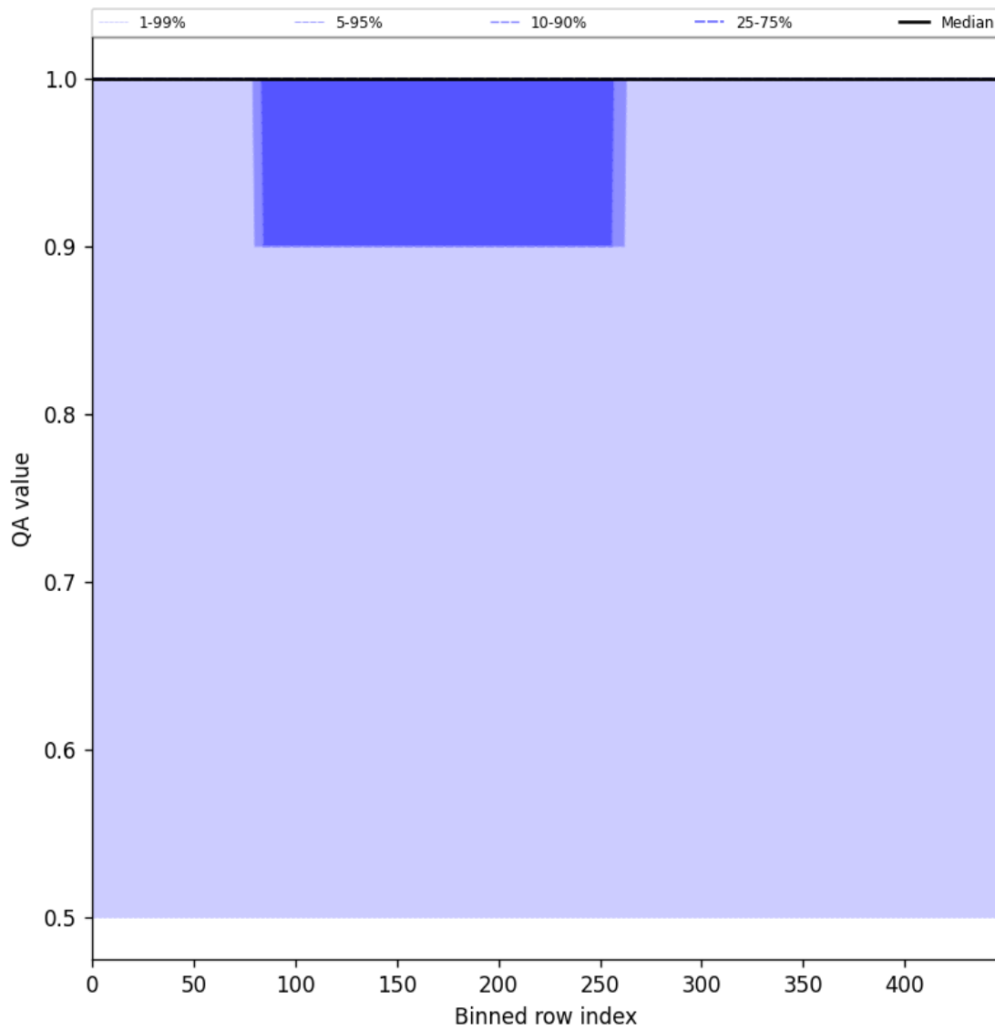
Figure 44: Along track statistics of “QA value” for 2025-07-30 to 2025-07-31
