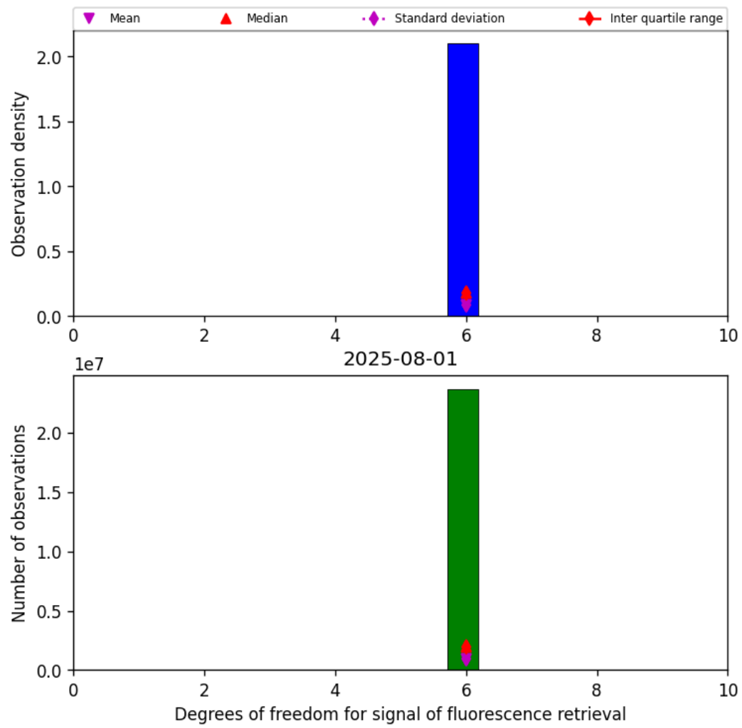
Figure 41: Histogram of “Degrees of freedom for signal of fluorescence retrieval” for 2025-08-01 to 2025-08-01
