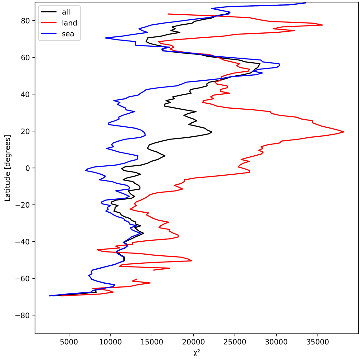
Figure 19: Zonal average of “ \chi^2 ” for 2025-08-01 to 2025-08-01.
