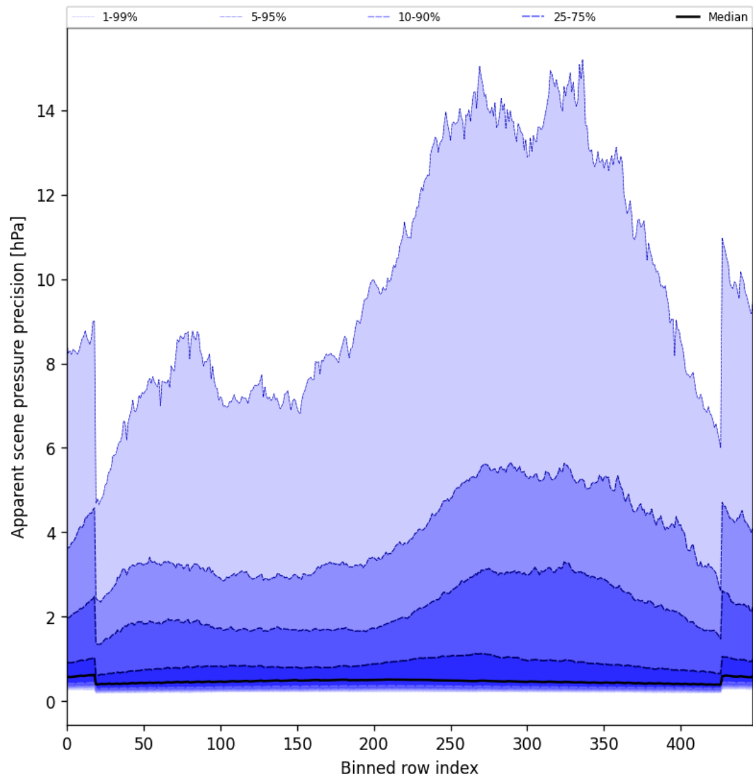
Figure 52: Along track statistics of “Apparent scene pressure precision” for 2025-08-01 to 2025-08-01
