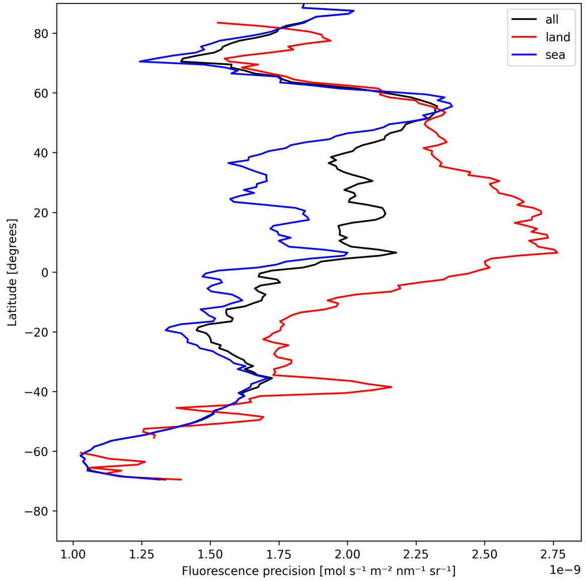
Figure 22: Zonal average of “Fluorescence precision” for 2025-08-01 to 2025-08-01.
