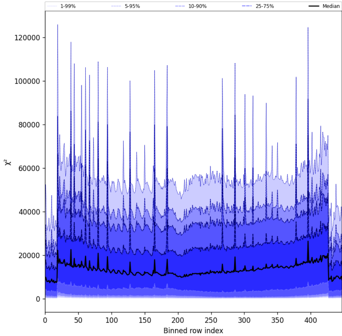
Figure 53: Along track statistics of “ \chi^2 ” for 2025-08-01 to 2025-08-01
