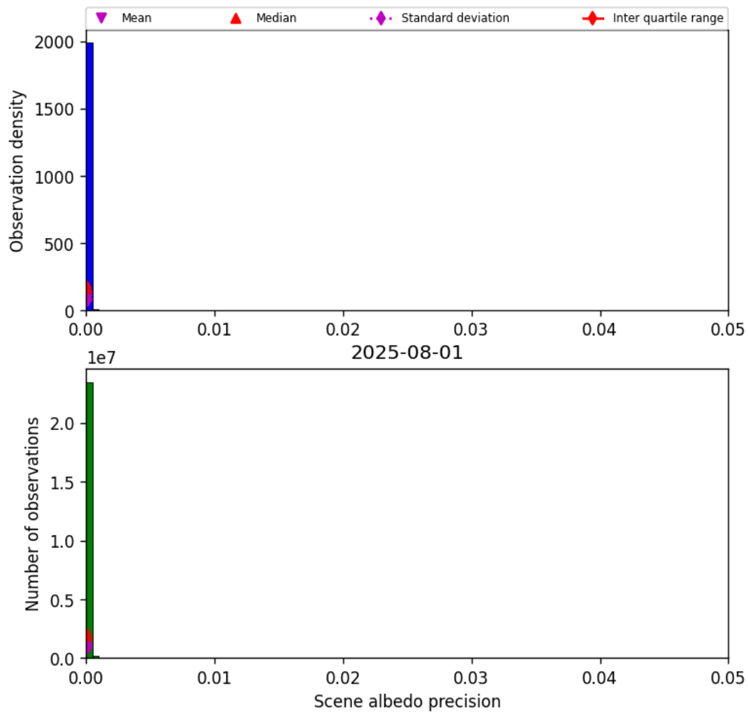
Figure 33: Histogram of “Scene albedo precision” for 2025-08-01 to 2025-08-01
