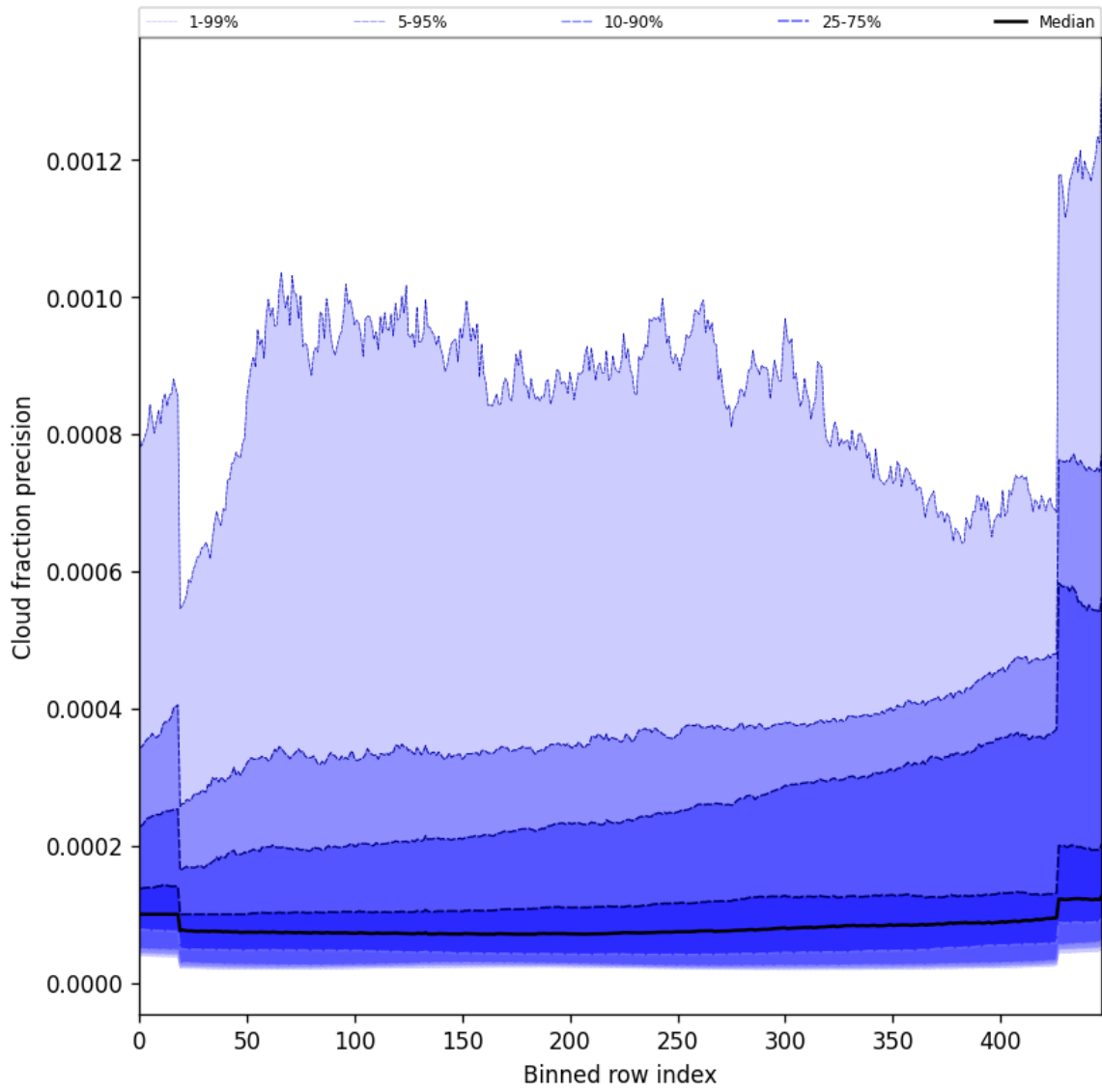
Figure 48: Along track statistics of “Cloud fraction precision” for 2025-08-01 to 2025-08-01
