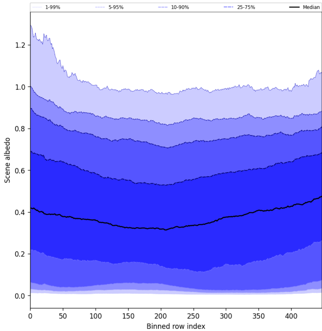
Figure 49: Along track statistics of “Scene albedo” for 2025-08-01 to 2025-08-01
