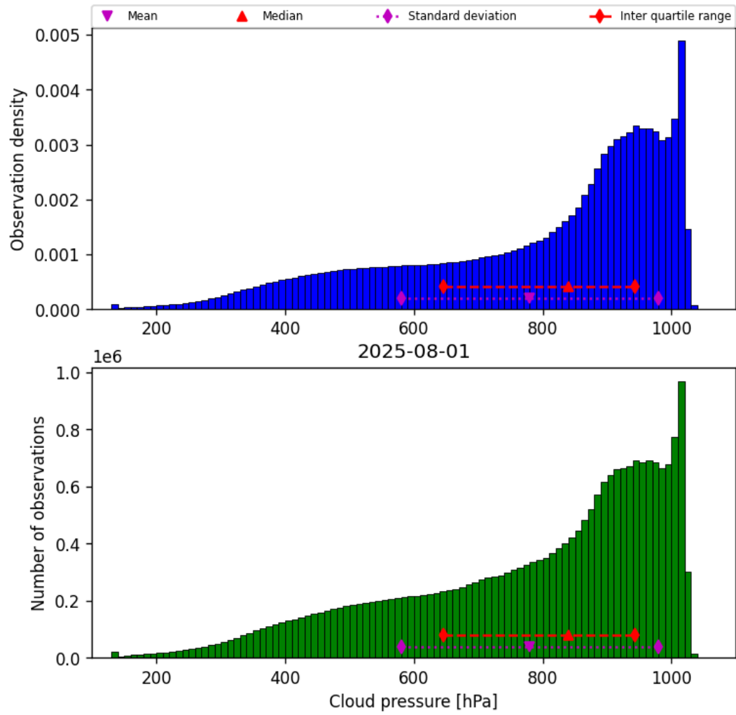
Figure 28: Histogram of “Cloud pressure” for 2025-08-01 to 2025-08-01
