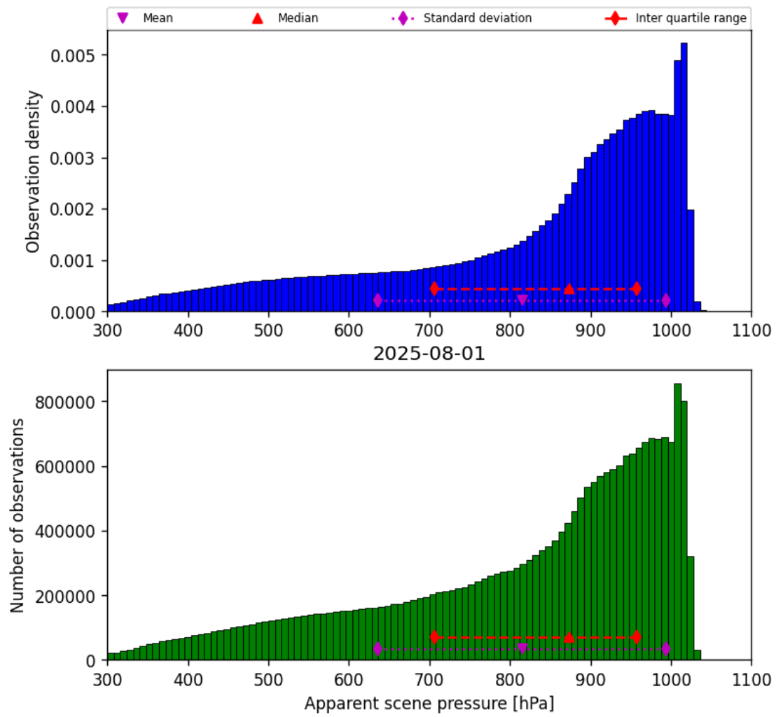
Figure 34: Histogram of “Apparent scene pressure” for 2025-08-01 to 2025-08-01
