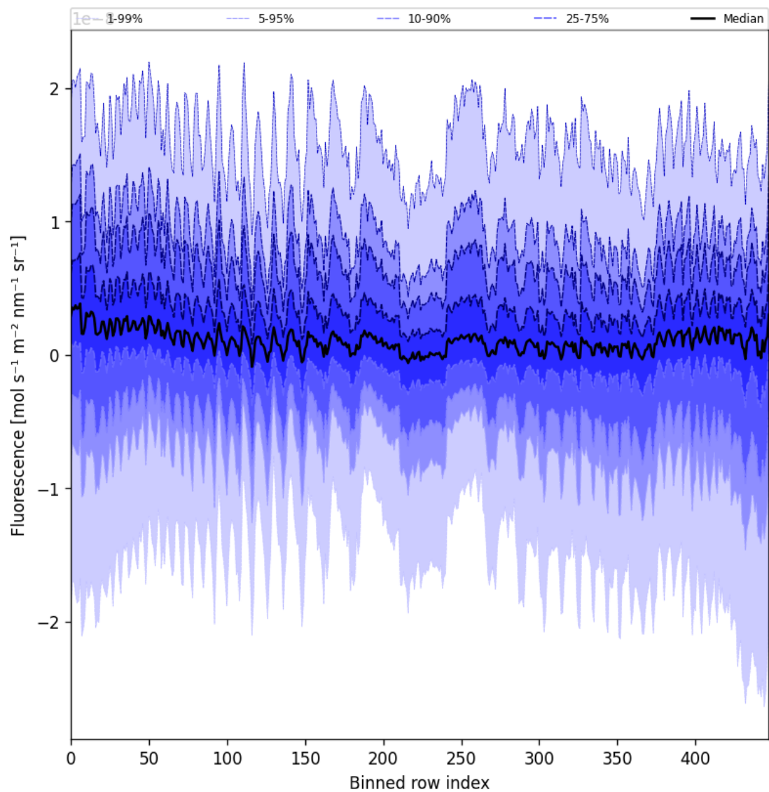
Figure 55: Along track statistics of “Fluorescence” for 2025-08-01 to 2025-08-01
