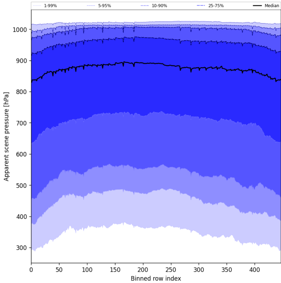
Figure 51: Along track statistics of “Apparent scene pressure” for 2025-08-01 to 2025-08-01
