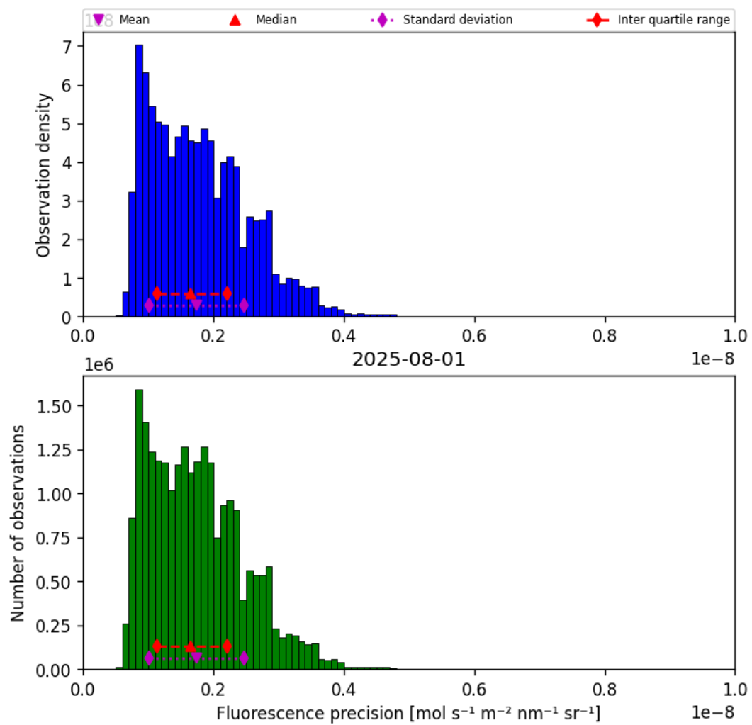
Figure 39: Histogram of “Fluorescence precision” for 2025-08-01 to 2025-08-01
