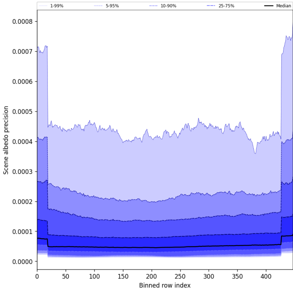
Figure 50: Along track statistics of “Scene albedo precision” for 2025-08-01 to 2025-08-01
