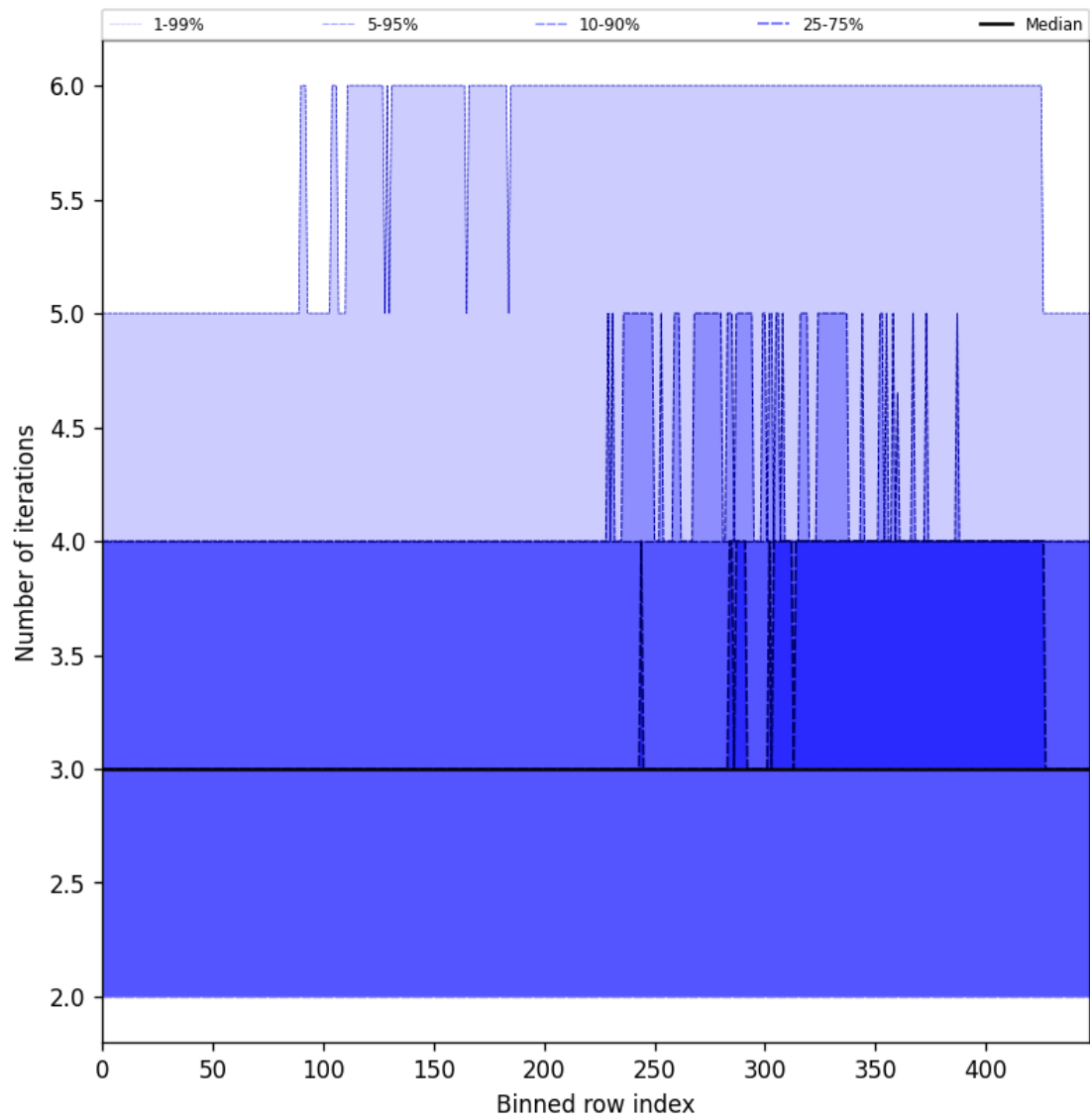
Figure 54: Along track statistics of “Number of iterations” for 2025-08-01 to 2025-08-01
