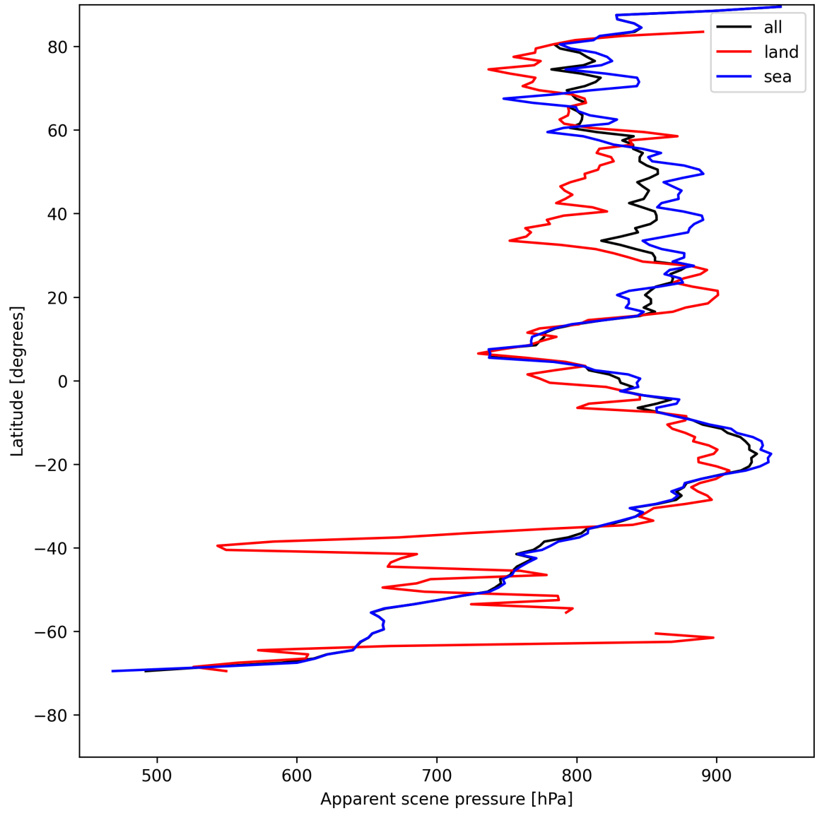
Figure 17: Zonal average of “Apparent scene pressure” for 2025-08-01 to 2025-08-01.
