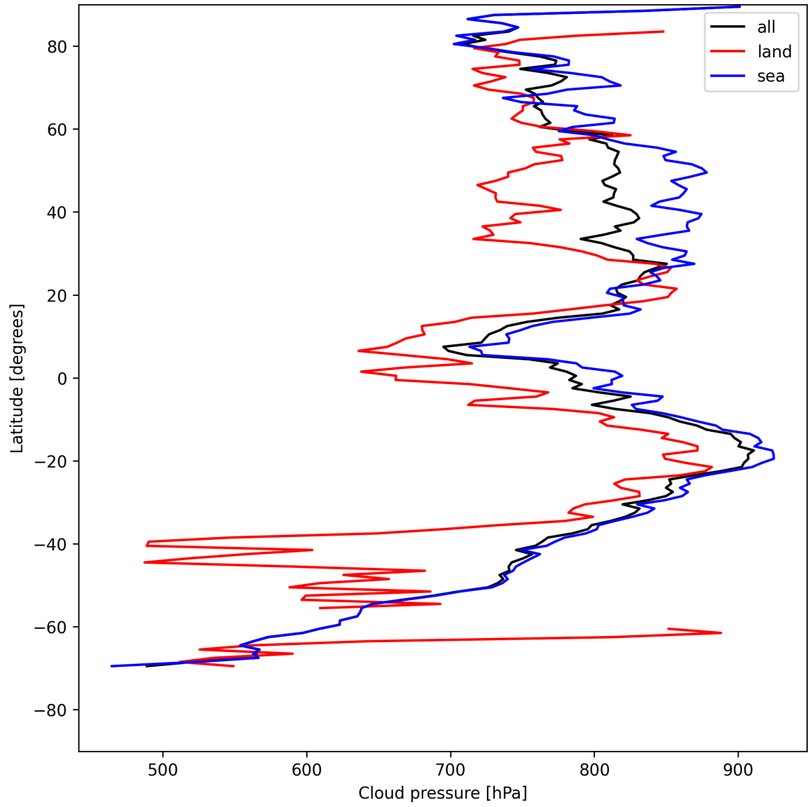
Figure 11: Zonal average of “Cloud pressure” for 2025-08-01 to 2025-08-01.
