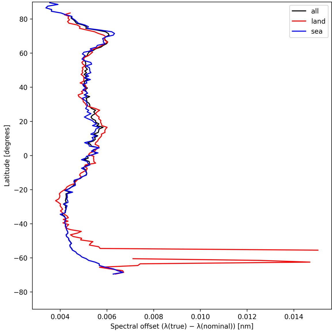
Figure 26: Zonal average of “Spectral offset ( \lambda_{\text{true}} - \lambda_{\text{nominal}} )” for 2025-08-01 to 2025-08-01.
