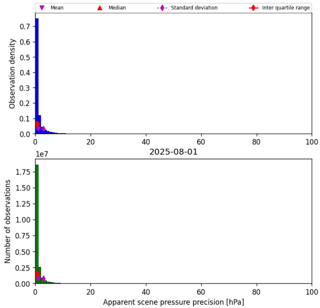
Figure 35: Histogram of “Apparent scene pressure precision” for 2025-08-01 to 2025-08-01
