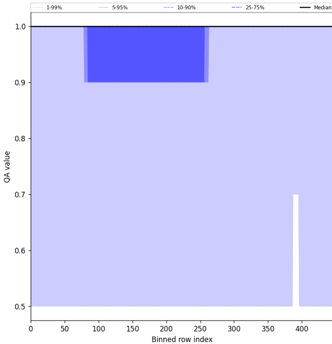
Figure 44: Along track statistics of “QA value” for 2025-08-01 to 2025-08-01
