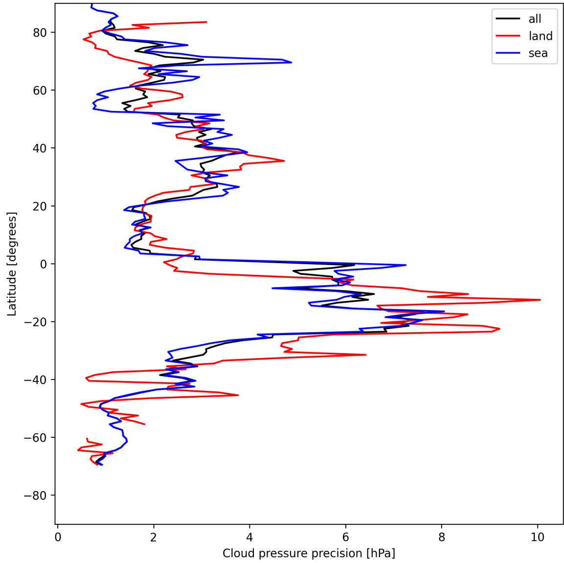
Figure 12: Zonal average of "Cloud pressure precision" for 2025-08-01 to 2025-08-01.
