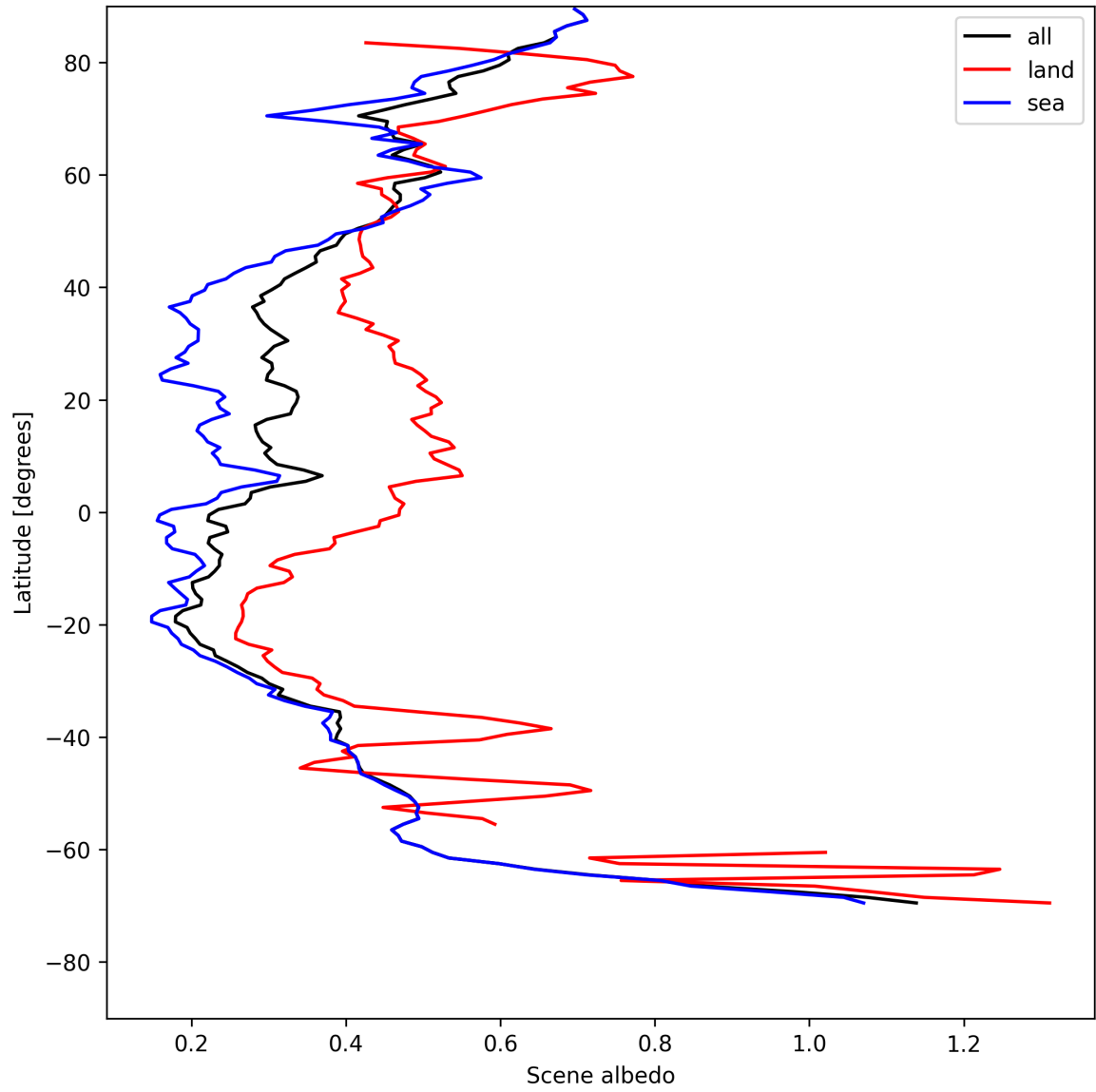
Figure 15: Zonal average of “Scene albedo” for 2025-08-01 to 2025-08-01.
