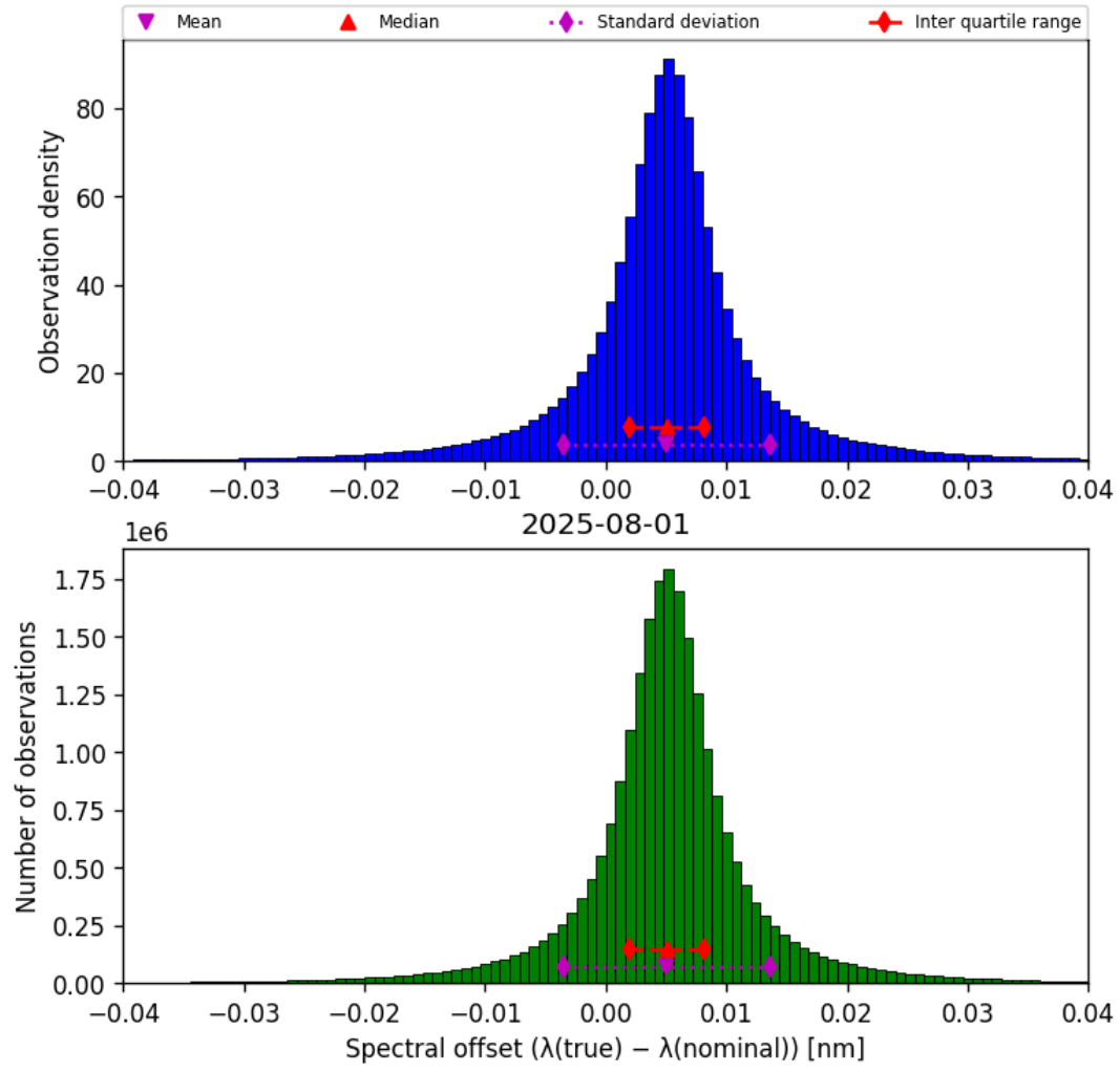
Figure 43: Histogram of “Spectral offset ( \lambda_{\text{true}} - \lambda_{\text{nominal}} )” for 2025-08-01 to 2025-08-01
