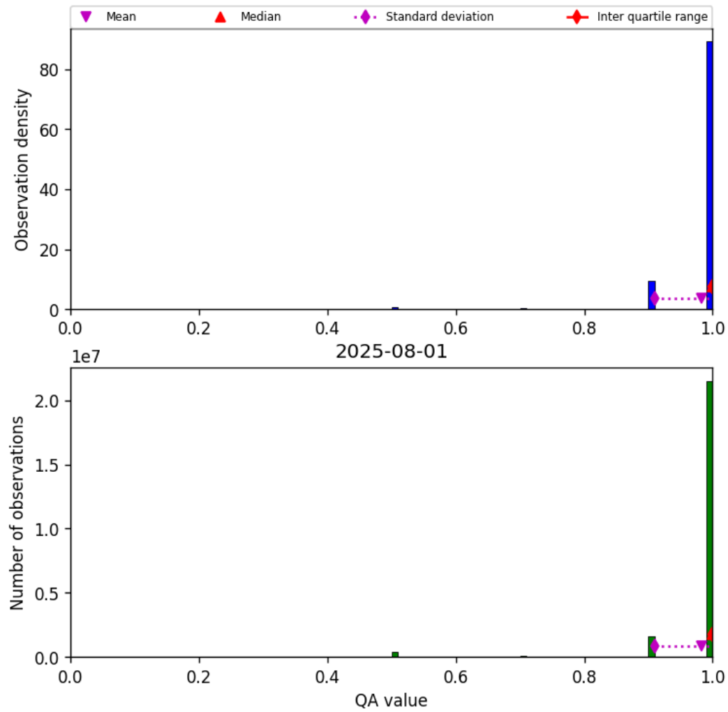
Figure 27: Histogram of “QA value” for 2025-08-01 to 2025-08-01
