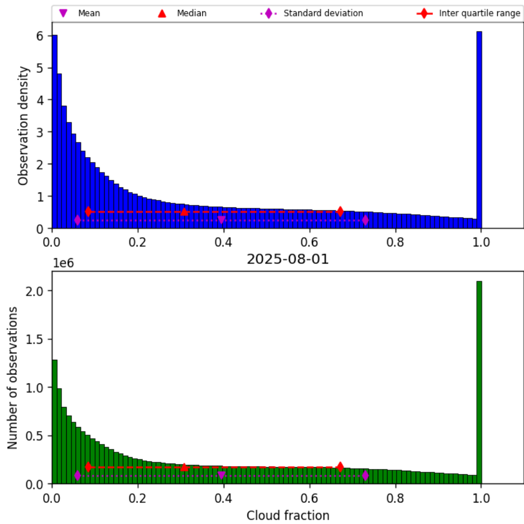
Figure 30: Histogram of “Cloud fraction” for 2025-08-01 to 2025-08-01
