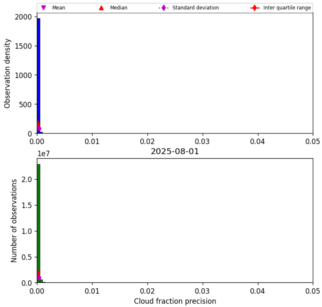
Figure 31: Histogram of “Cloud fraction precision” for 2025-08-01 to 2025-08-01
