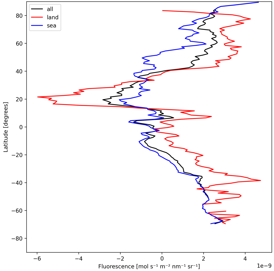
Figure 21: Zonal average of “Fluorescence” for 2025-08-01 to 2025-08-01.
