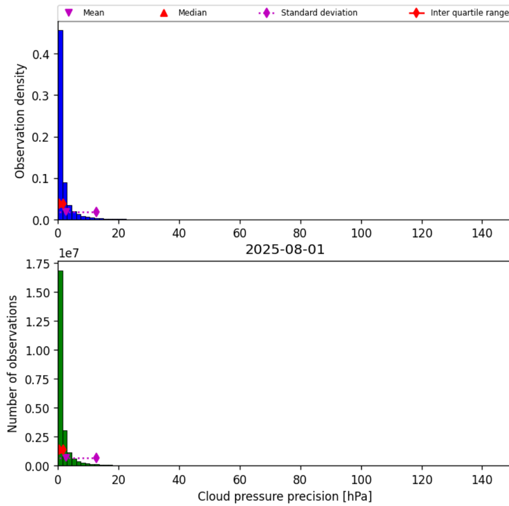
Figure 29: Histogram of “Cloud pressure precision” for 2025-08-01 to 2025-08-01
