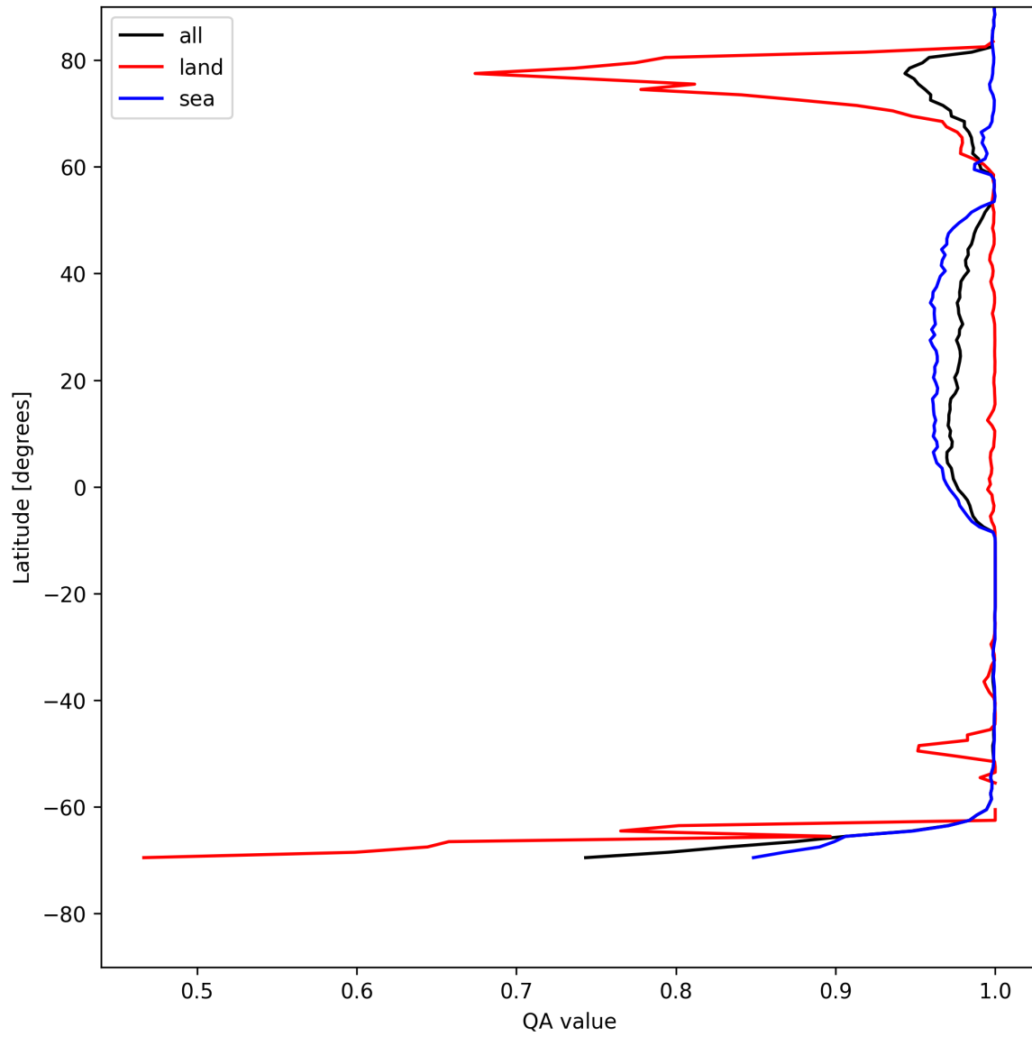
Figure 10: Zonal average of “QA value” for 2025-08-01 to 2025-08-01.
