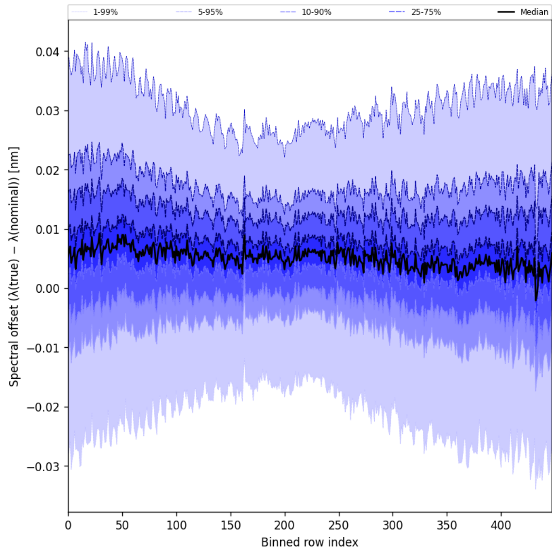
Figure 60: Along track statistics of “Spectral offset ( \lambda_{\text{true}} - \lambda_{\text{nominal}} )” for 2025-08-01 to 2025-08-01
