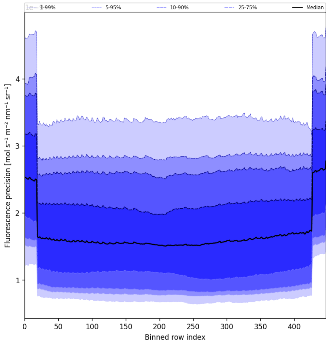
Figure 56: Along track statistics of “Fluorescence precision” for 2025-08-01 to 2025-08-01
