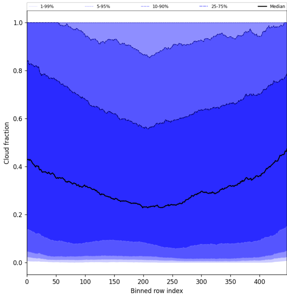
Figure 47: Along track statistics of “Cloud fraction” for 2025-08-01 to 2025-08-01
