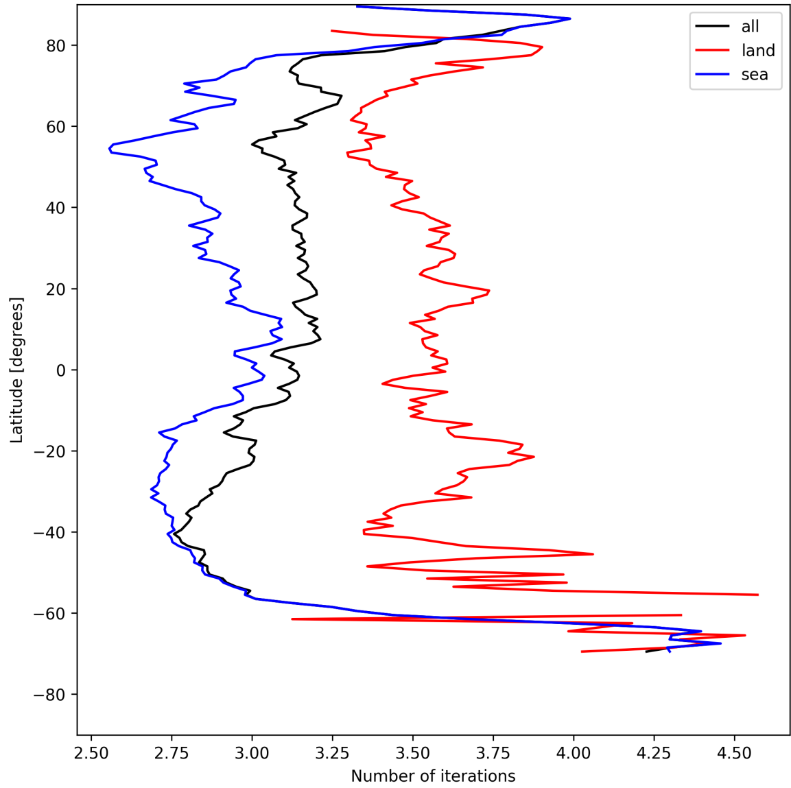
Figure 20: Zonal average of “Number of iterations” for 2025-08-01 to 2025-08-01.
