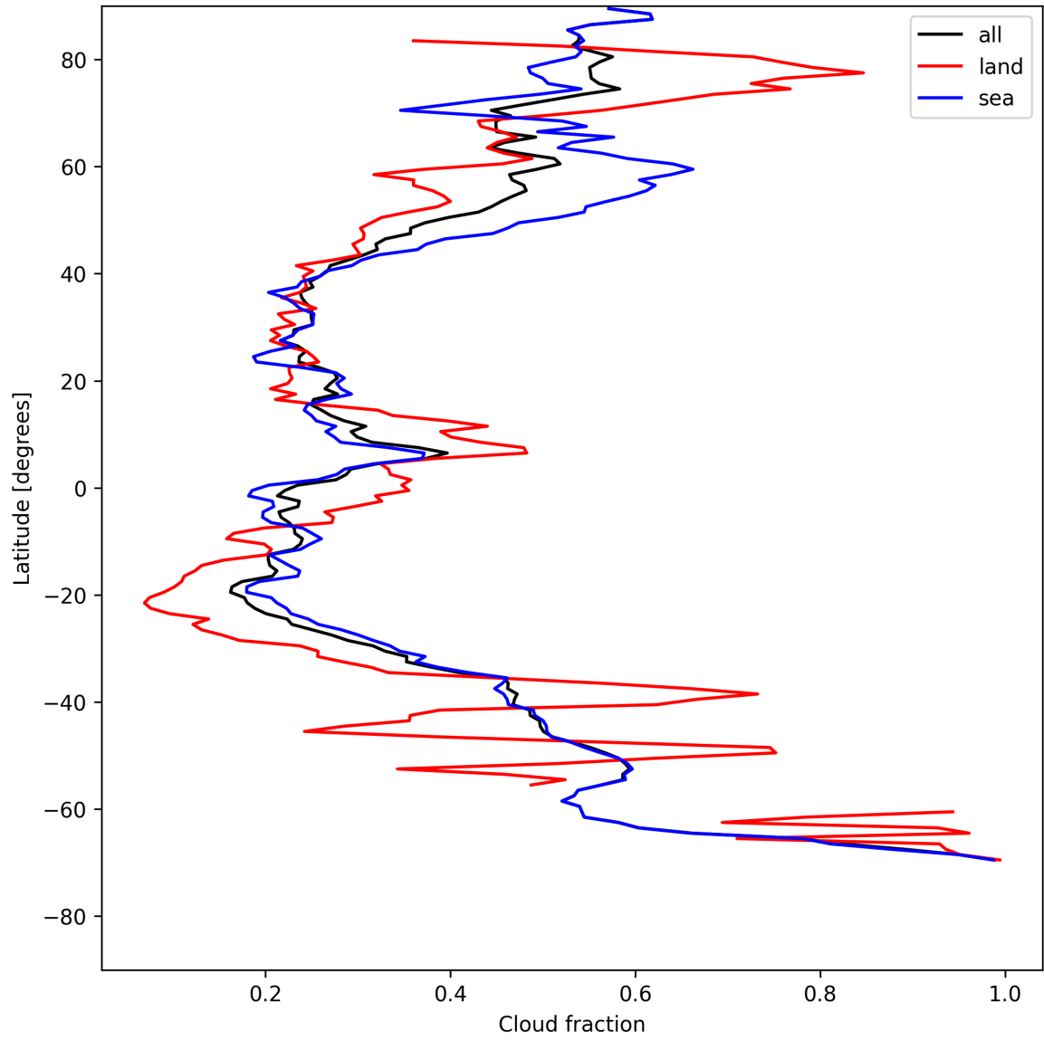
Figure 13: Zonal average of “Cloud fraction” for 2025-08-01 to 2025-08-01.
