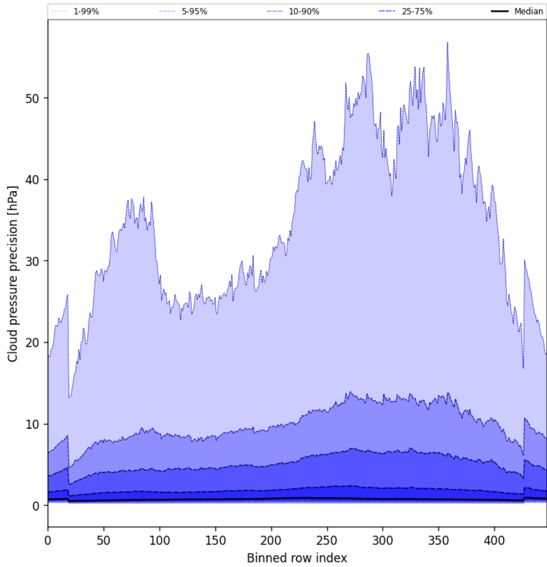
Figure 46: Along track statistics of “Cloud pressure precision” for 2025-08-01 to 2025-08-01
