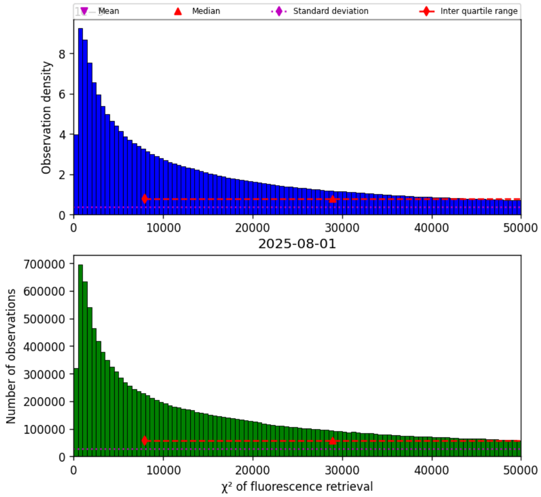
Figure 40: Histogram of “ \chi^2 of fluorescence retrieval” for 2025-08-01 to 2025-08-01
