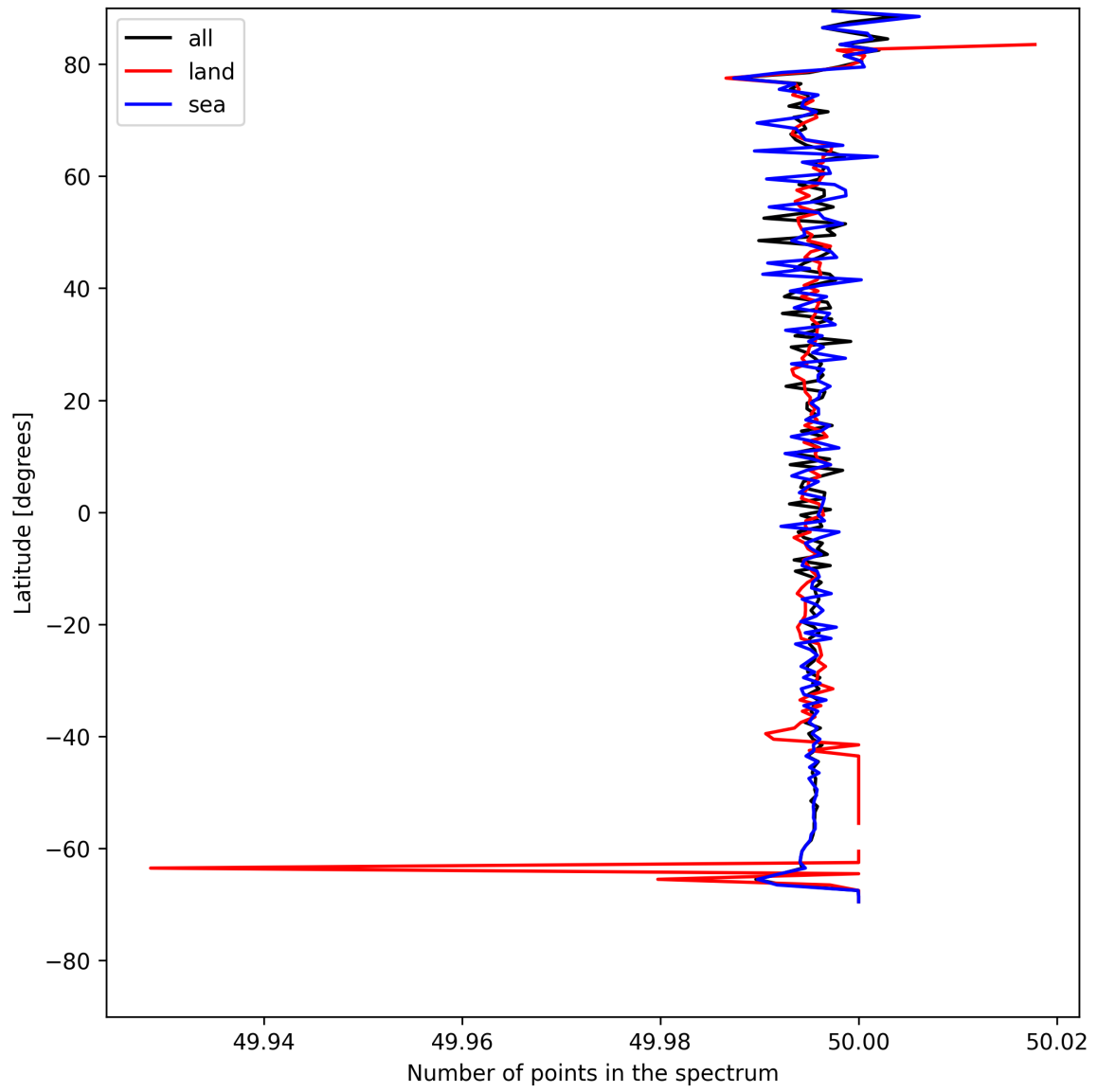
Figure 25: Zonal average of “Number of points in the spectrum” for 2025-08-01 to 2025-08-01.
