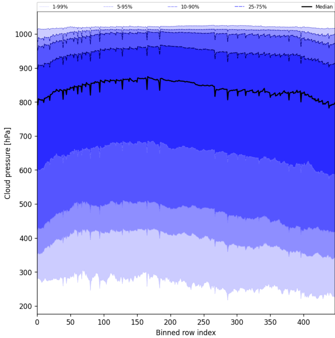
Figure 45: Along track statistics of “Cloud pressure” for 2025-08-01 to 2025-08-01
