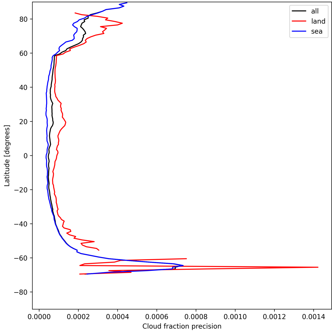
Figure 14: Zonal average of “Cloud fraction precision” for 2025-08-01 to 2025-08-01.
