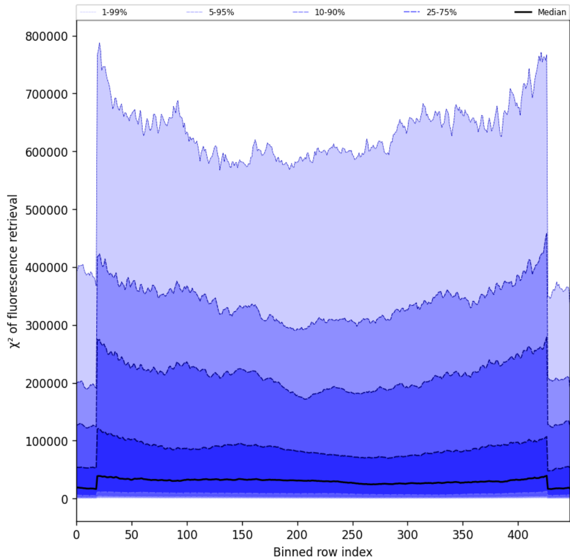
Figure 57: Along track statistics of “ \chi^2 of fluorescence retrieval” for 2025-08-01 to 2025-08-01
