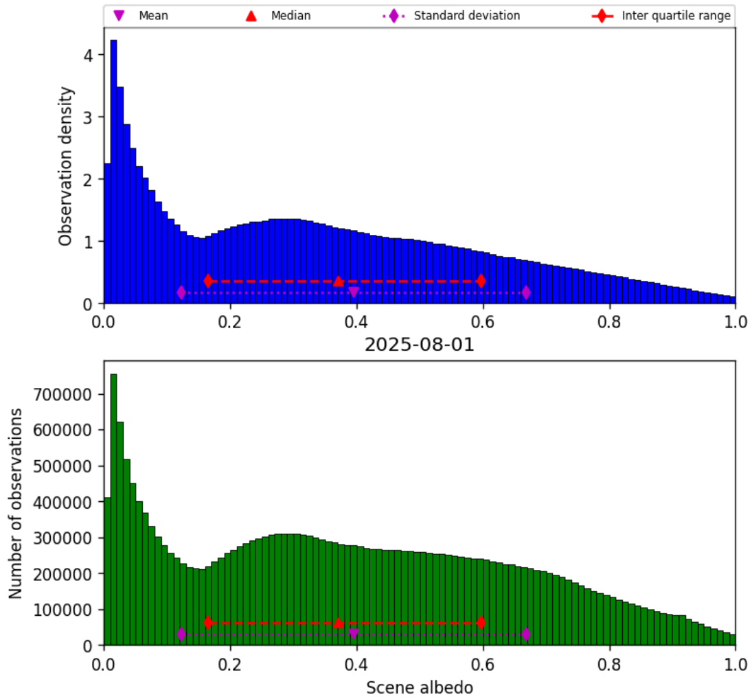
Figure 32: Histogram of “Scene albedo” for 2025-08-01 to 2025-08-01
