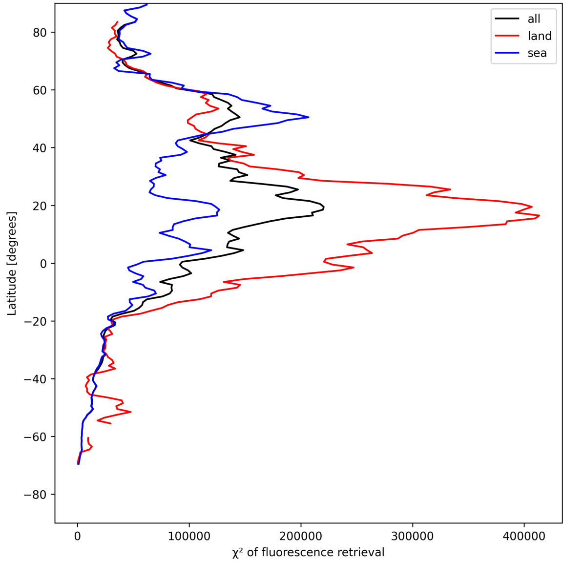
Figure 23: Zonal average of “ \chi^2 of fluorescence retrieval” for 2025-08-01 to 2025-08-01.
