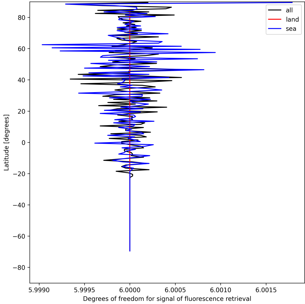
Figure 24: Zonal average of “Degrees of freedom for signal of fluorescence retrieval” for 2025-08-01 to 2025-08-01.
