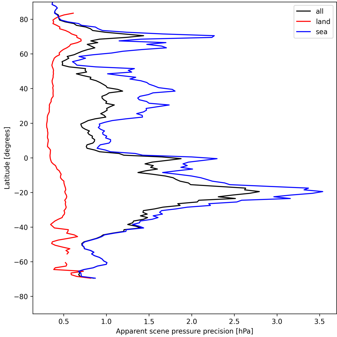
Figure 18: Zonal average of “Apparent scene pressure precision” for 2025-08-01 to 2025-08-01.
