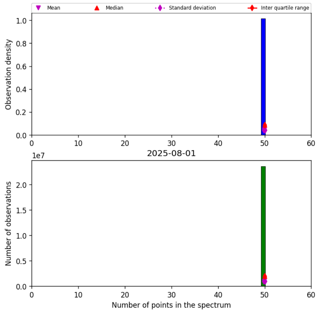
Figure 42: Histogram of “Number of points in the spectrum” for 2025-08-01 to 2025-08-01
