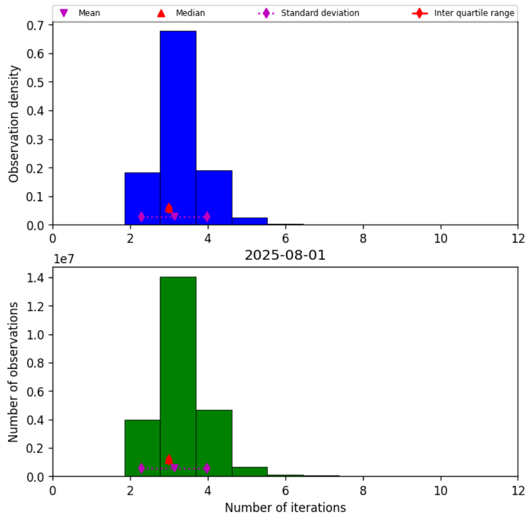
Figure 37: Histogram of “Number of iterations” for 2025-08-01 to 2025-08-01
