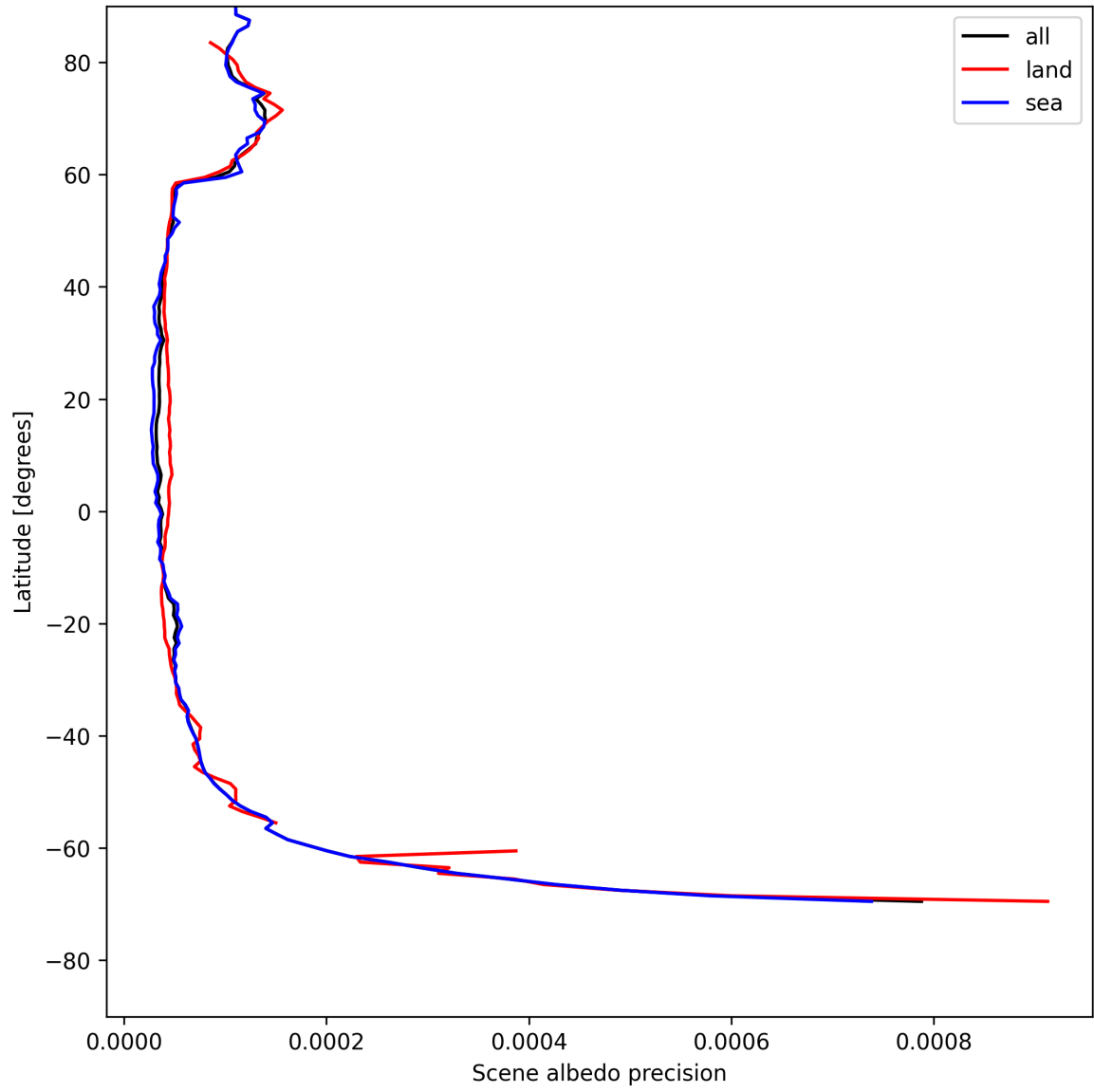
Figure 16: Zonal average of “Scene albedo precision” for 2025-08-01 to 2025-08-01.
