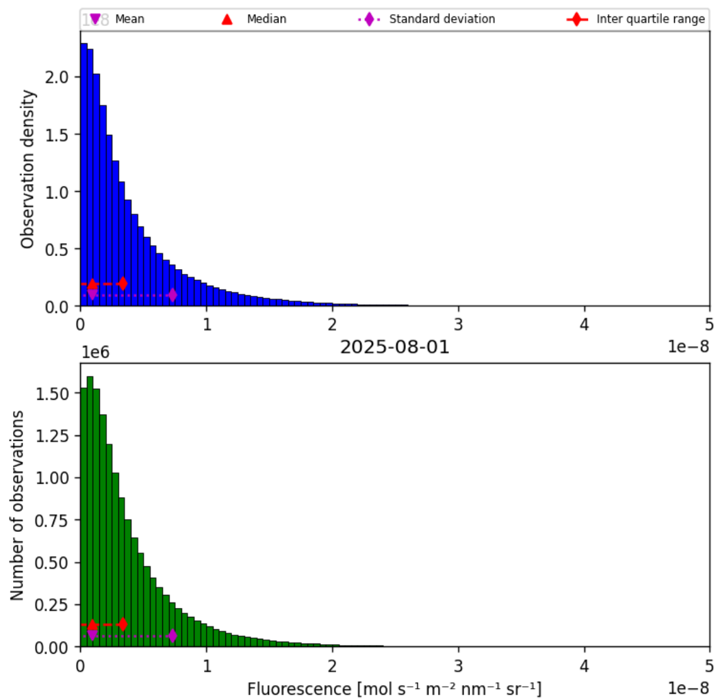
Figure 38: Histogram of “Fluorescence” for 2025-08-01 to 2025-08-01
