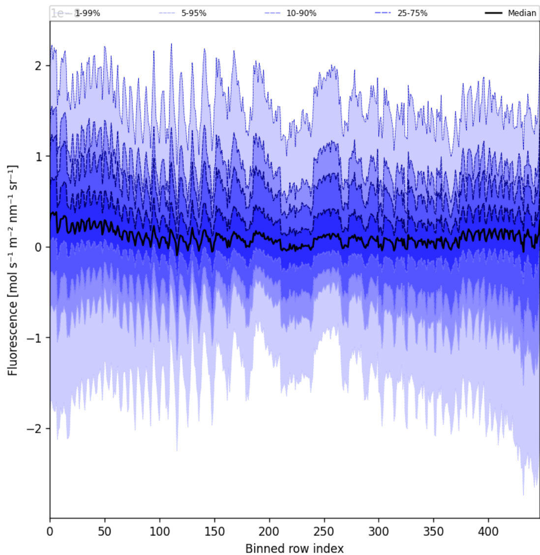
Figure 55: Along track statistics of “Fluorescence” for 2025-08-02 to 2025-08-03
