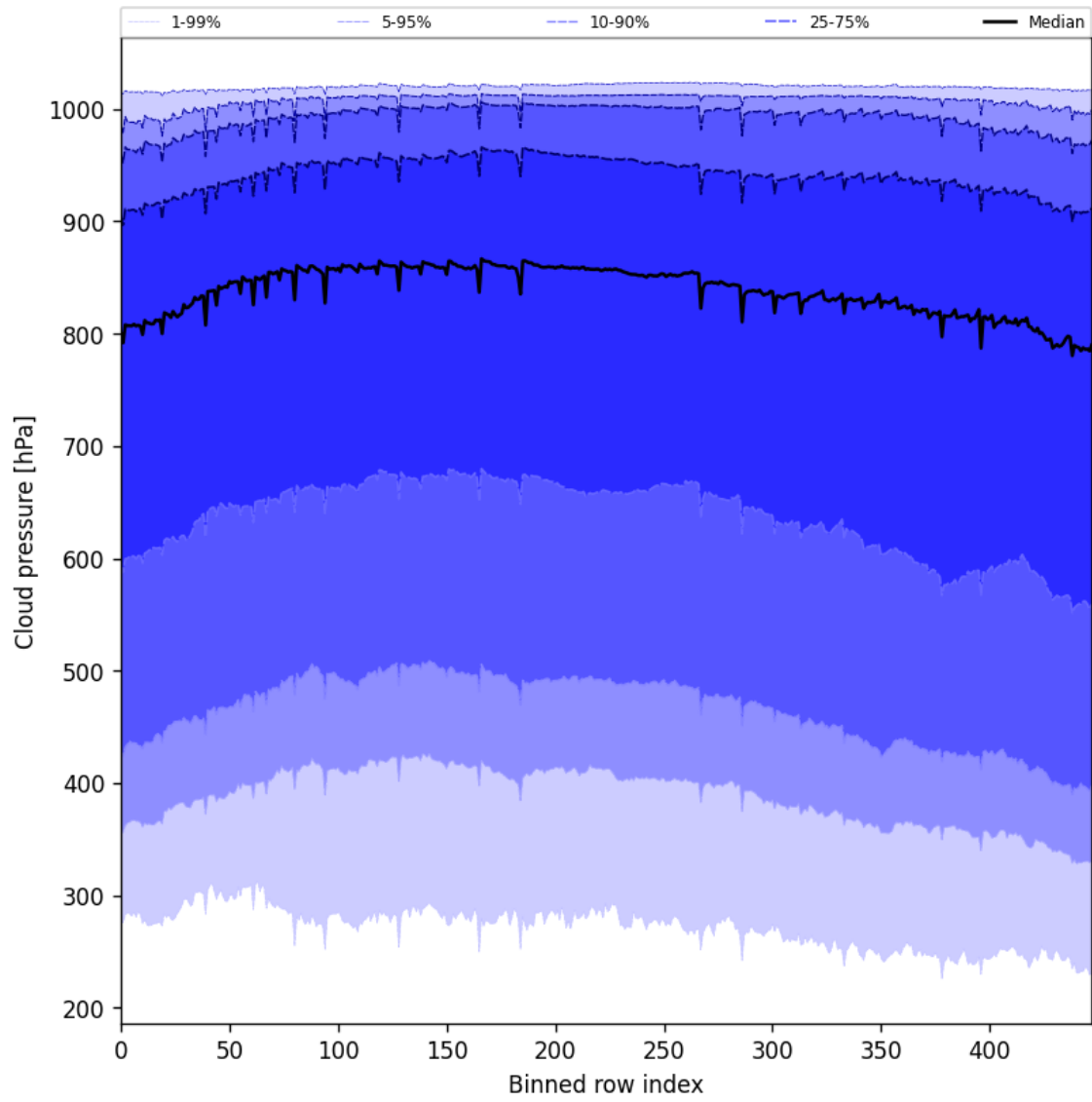
Figure 45: Along track statistics of “Cloud pressure” for 2025-08-02 to 2025-08-03
