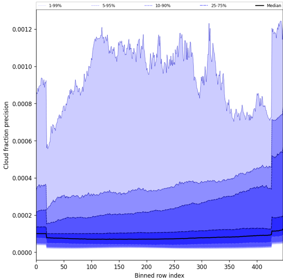
Figure 48: Along track statistics of “Cloud fraction precision” for 2025-08-02 to 2025-08-03
