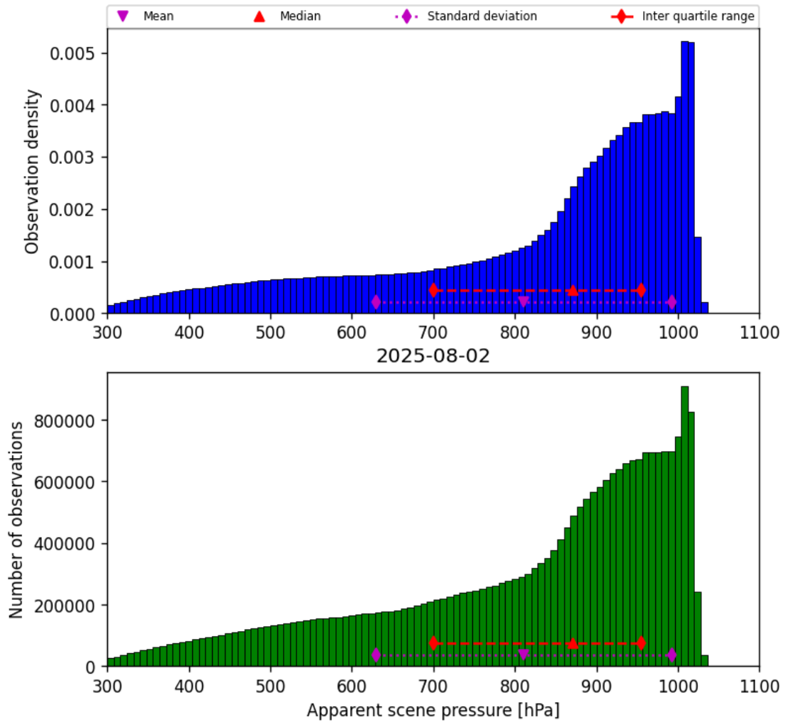
Figure 34: Histogram of “Apparent scene pressure” for 2025-08-02 to 2025-08-03
