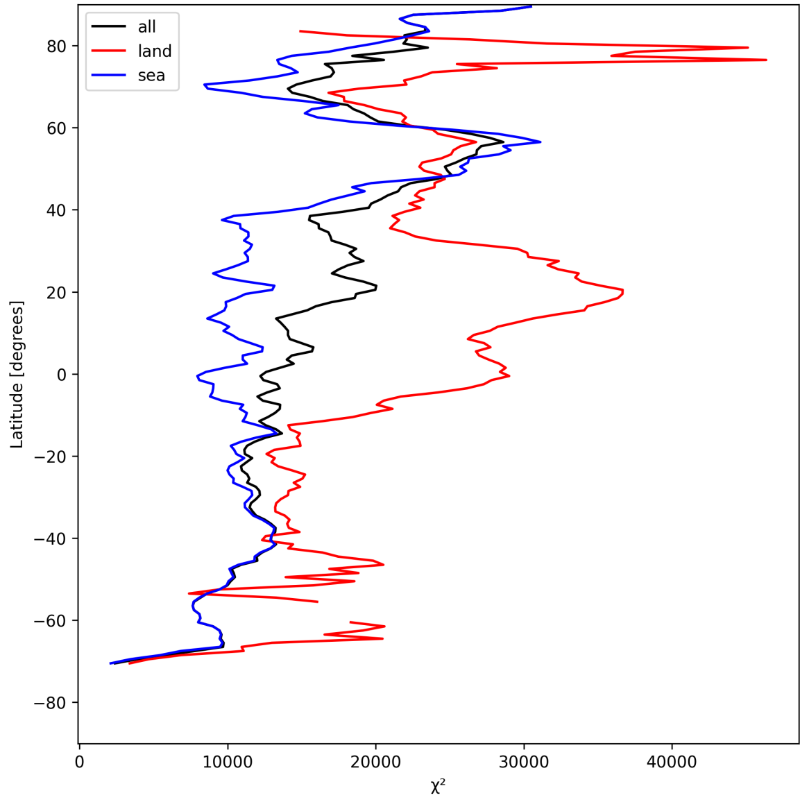
Figure 19: Zonal average of “ \chi^2 ” for 2025-08-02 to 2025-08-03.
