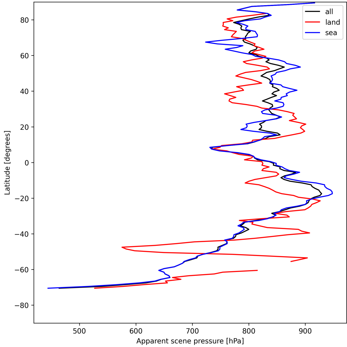
Figure 17: Zonal average of “Apparent scene pressure” for 2025-08-02 to 2025-08-03.
