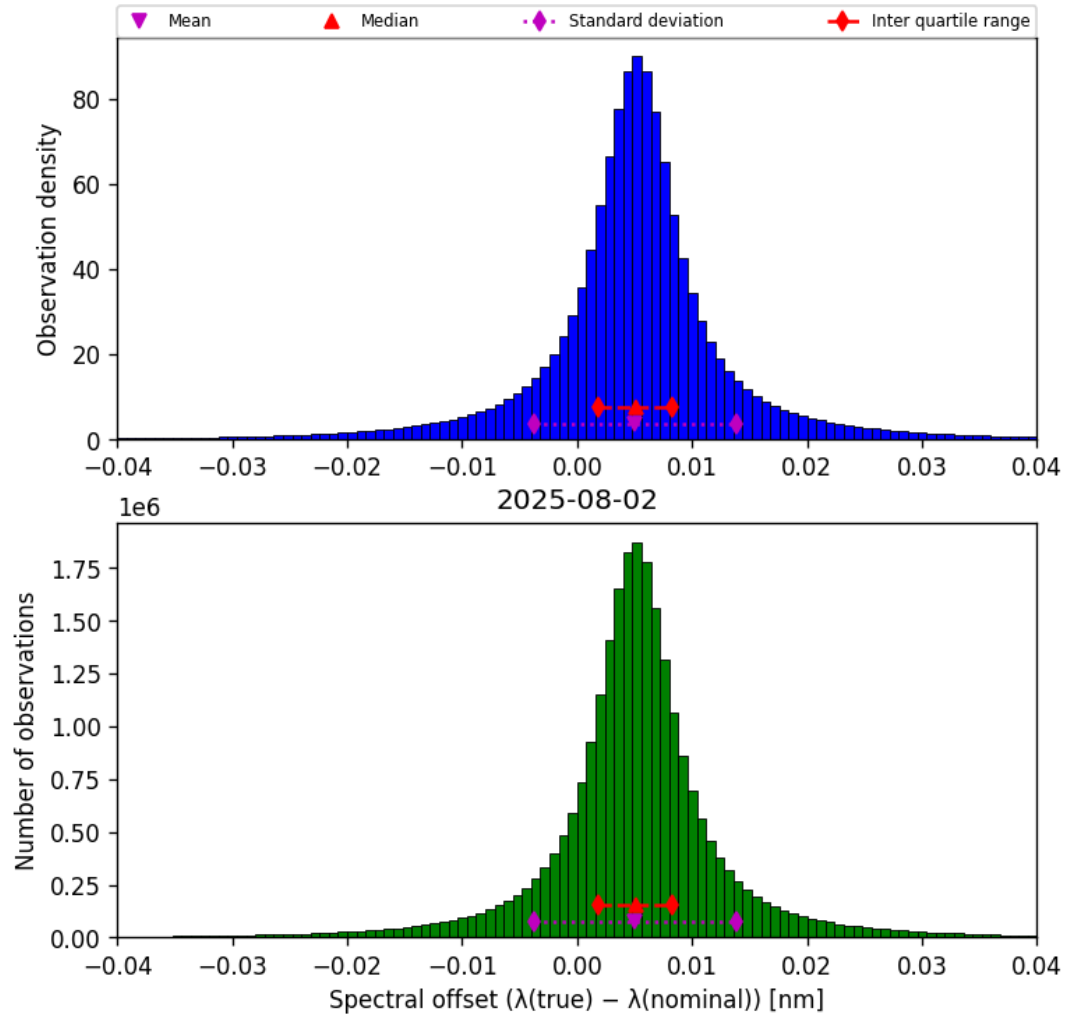
Figure 43: Histogram of “Spectral offset ( \lambda_{\text{true}} - \lambda_{\text{nominal}} )” for 2025-08-02 to 2025-08-03
