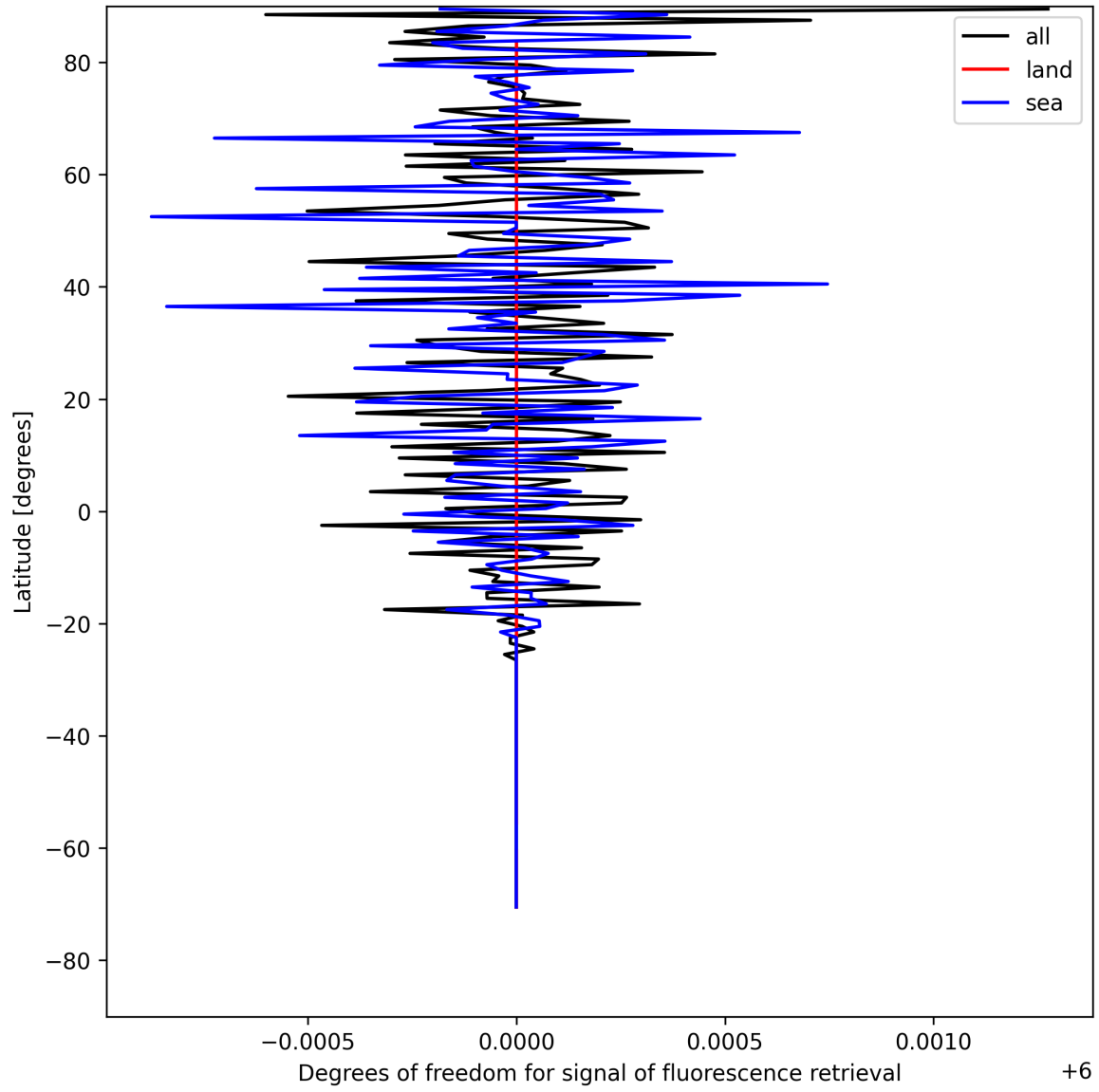
Figure 24: Zonal average of “Degrees of freedom for signal of fluorescence retrieval” for 2025-08-02 to 2025-08-03.
