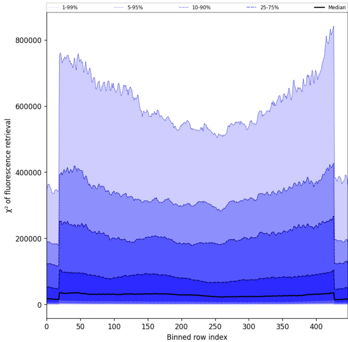
Figure 57: Along track statistics of “ \chi^2 of fluorescence retrieval” for 2025-08-02 to 2025-08-03
