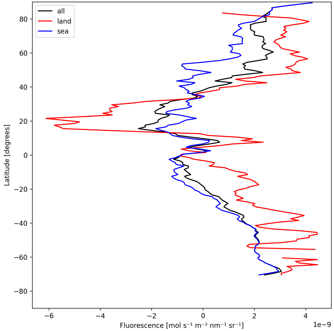
Figure 21: Zonal average of “Fluorescence” for 2025-08-02 to 2025-08-03.
