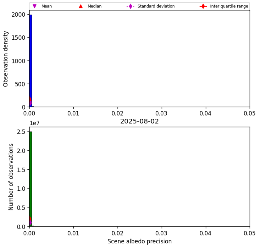
Figure 33: Histogram of “Scene albedo precision” for 2025-08-02 to 2025-08-03
