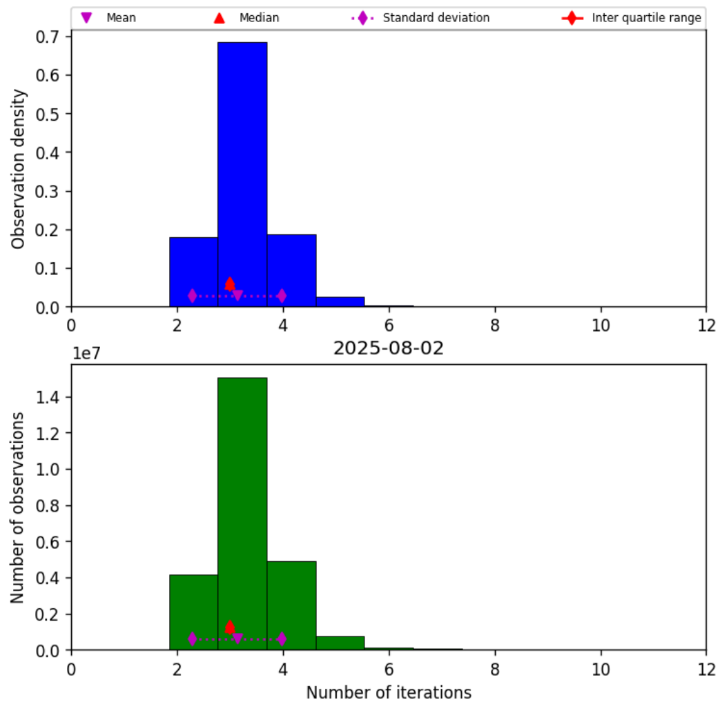
Figure 37: Histogram of “Number of iterations” for 2025-08-02 to 2025-08-03
