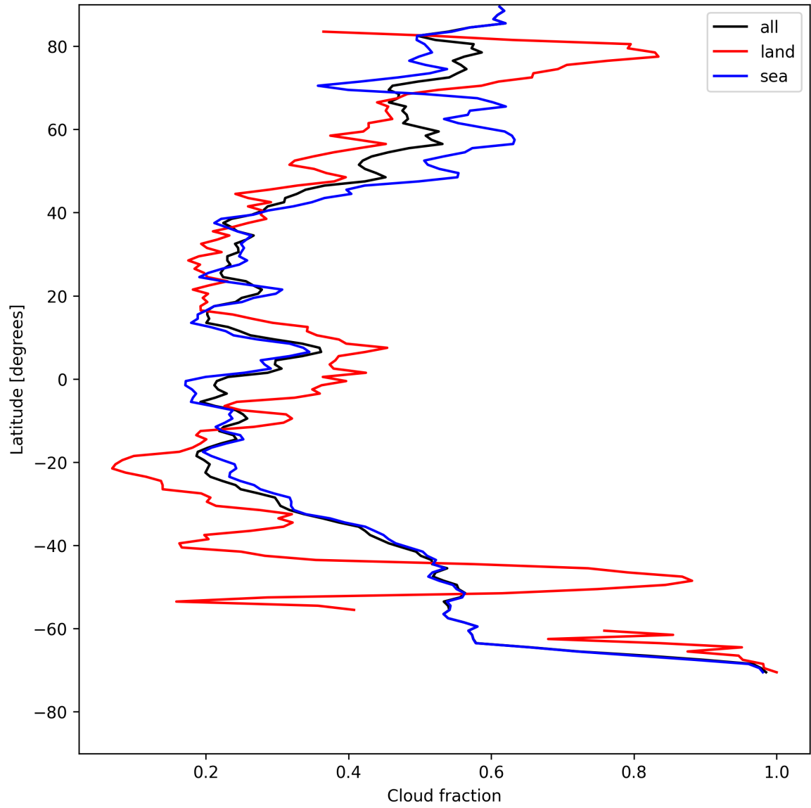
Figure 13: Zonal average of “Cloud fraction” for 2025-08-02 to 2025-08-03.
