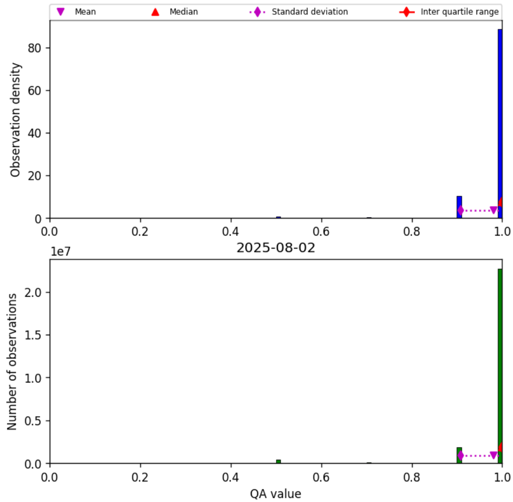
Figure 27: Histogram of “QA value” for 2025-08-02 to 2025-08-03
