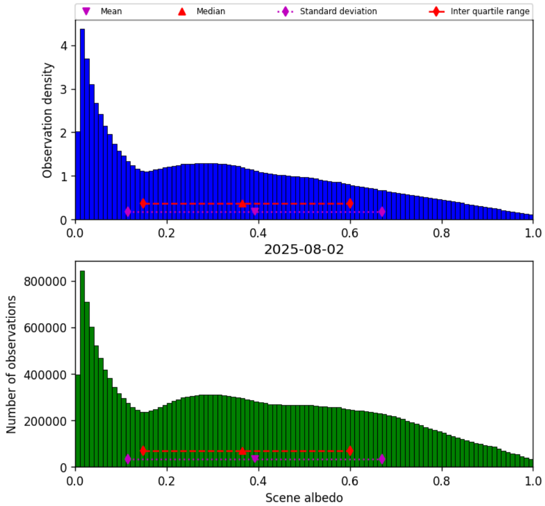
Figure 32: Histogram of “Scene albedo” for 2025-08-02 to 2025-08-03
