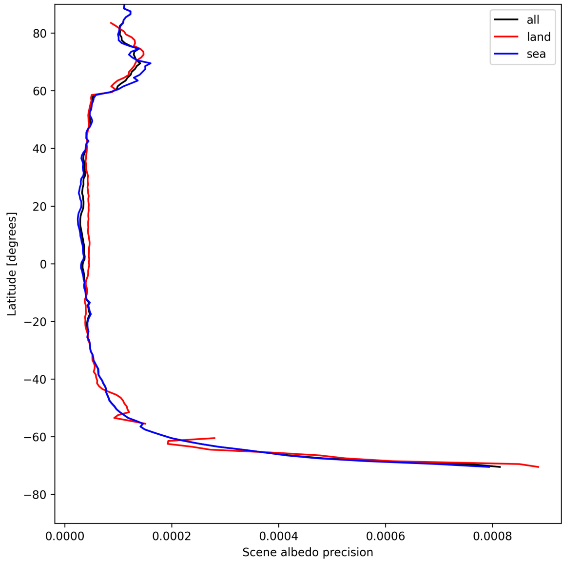
Figure 16: Zonal average of “Scene albedo precision” for 2025-08-02 to 2025-08-03.
