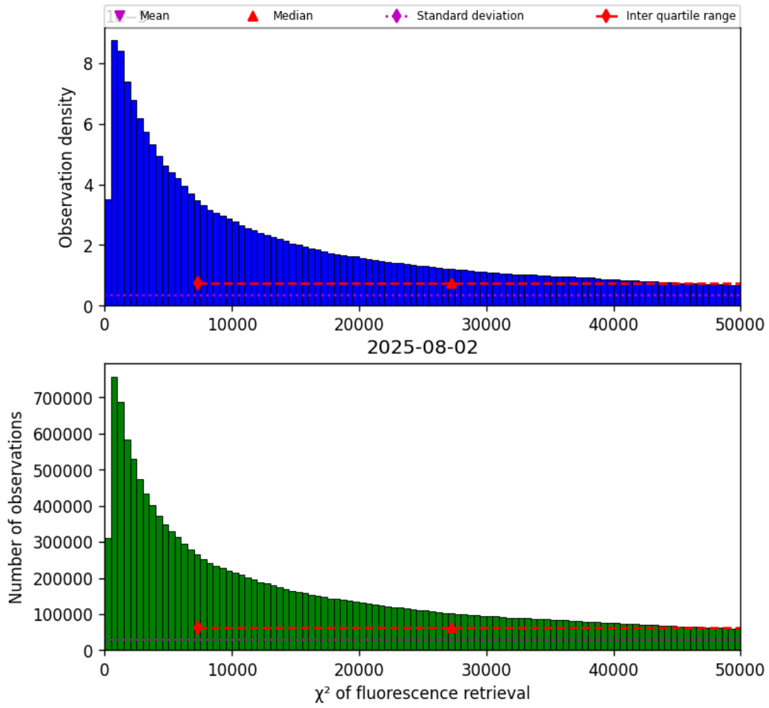
Figure 40: Histogram of “ \chi^2 of fluorescence retrieval” for 2025-08-02 to 2025-08-03
