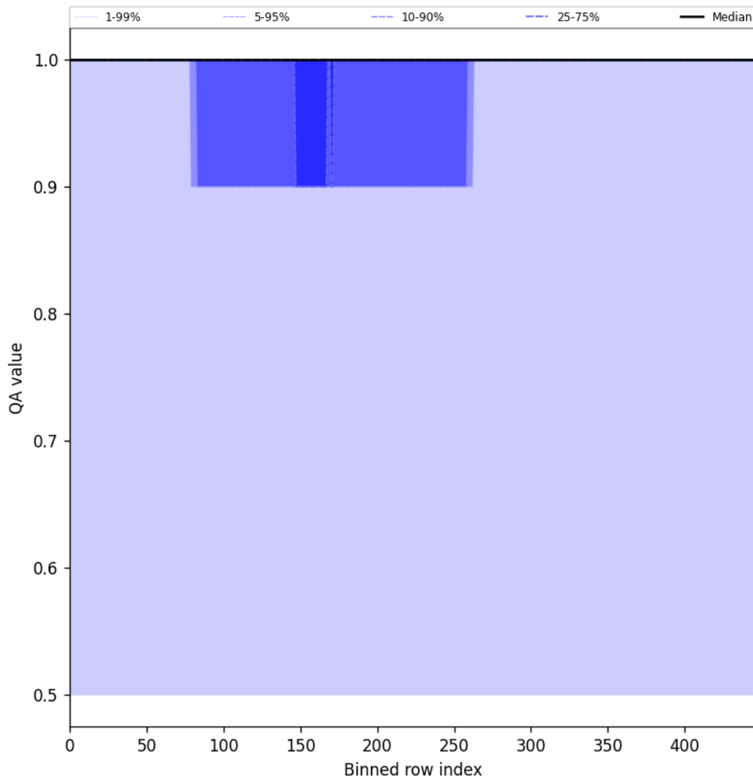
Figure 44: Along track statistics of “QA value” for 2025-08-02 to 2025-08-03
