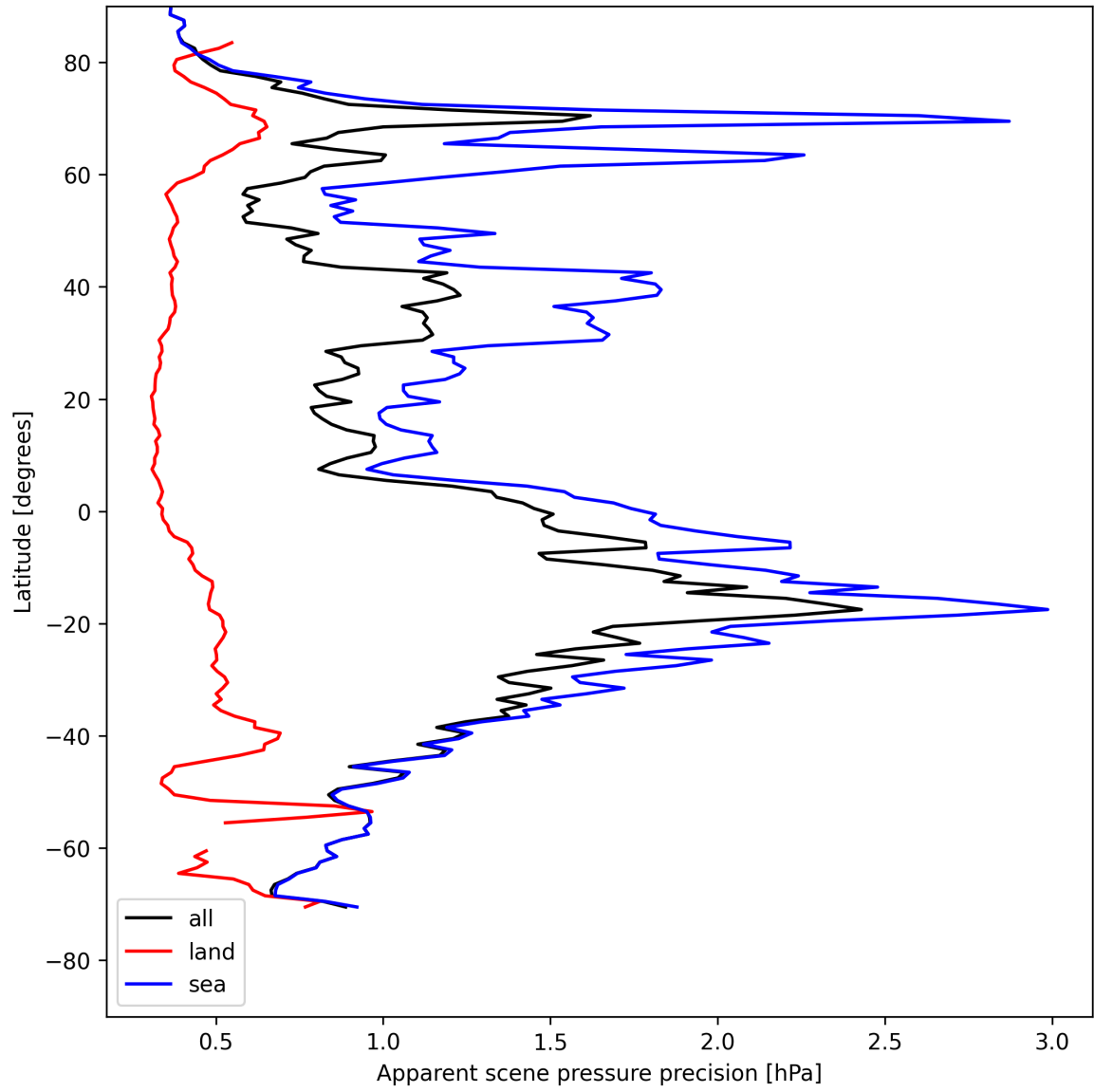
Figure 18: Zonal average of “Apparent scene pressure precision” for 2025-08-02 to 2025-08-03.
