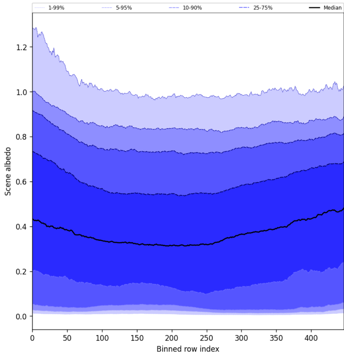
Figure 49: Along track statistics of “Scene albedo” for 2025-08-02 to 2025-08-03
