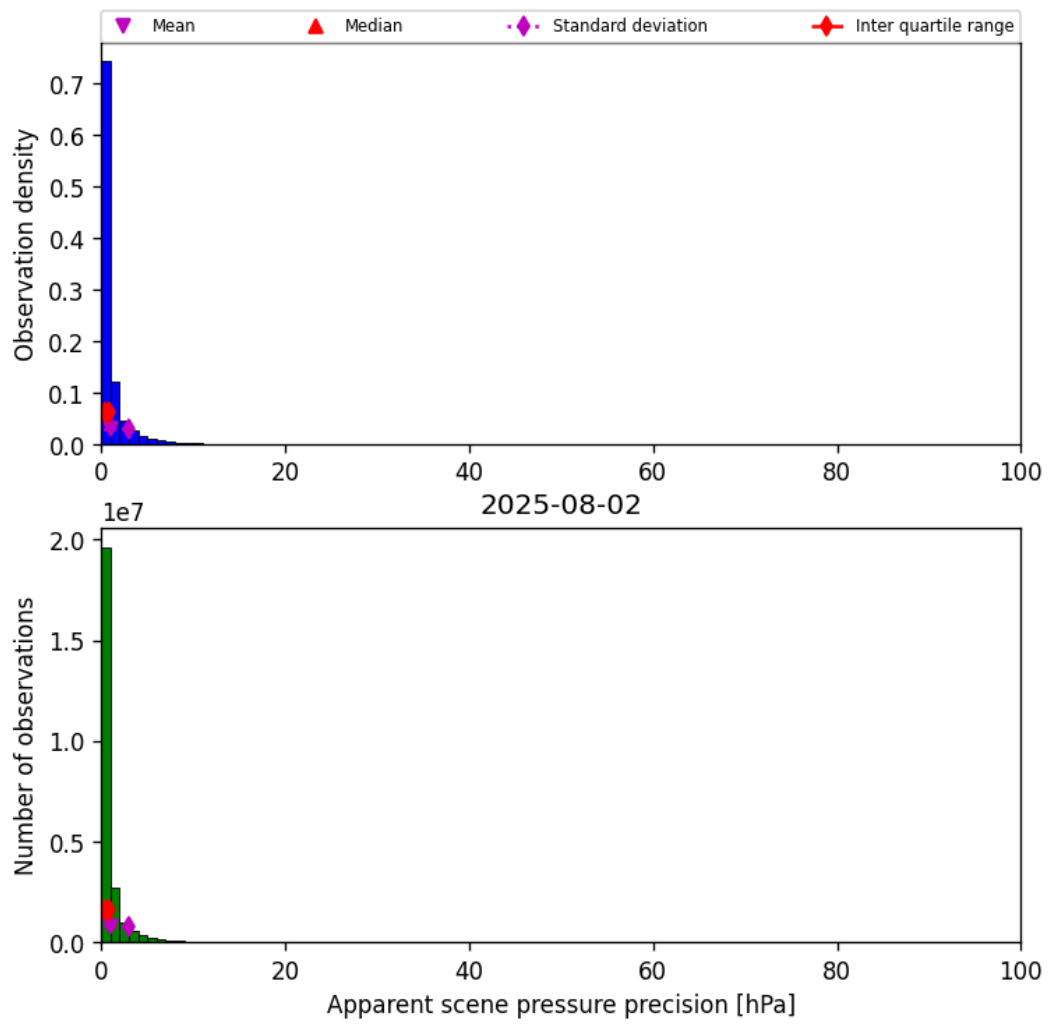
Figure 35: Histogram of “Apparent scene pressure precision” for 2025-08-02 to 2025-08-03
