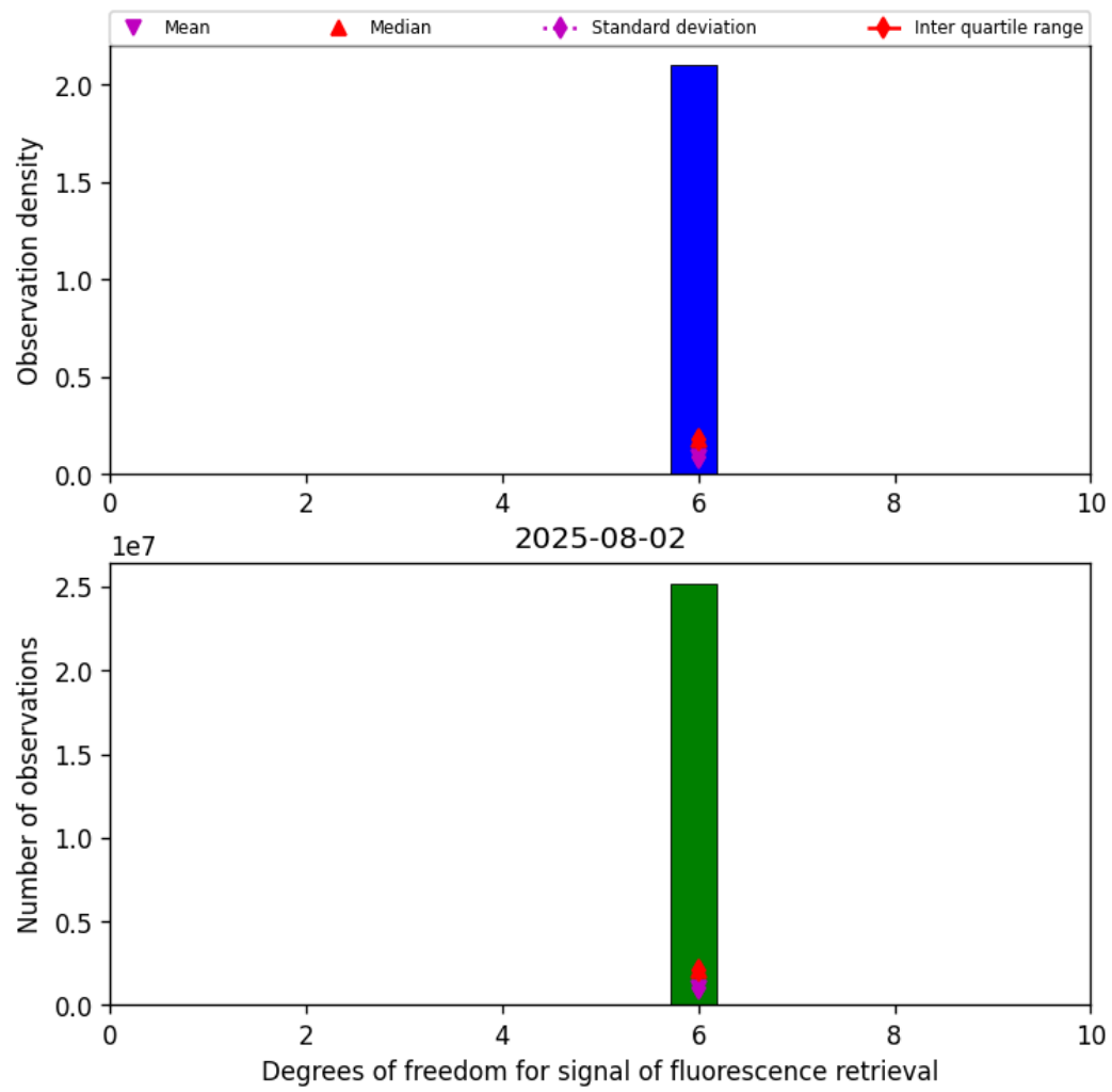
Figure 41: Histogram of "Degrees of freedom for signal of fluorescence retrieval" for 2025-08-02 to 2025-08-03
