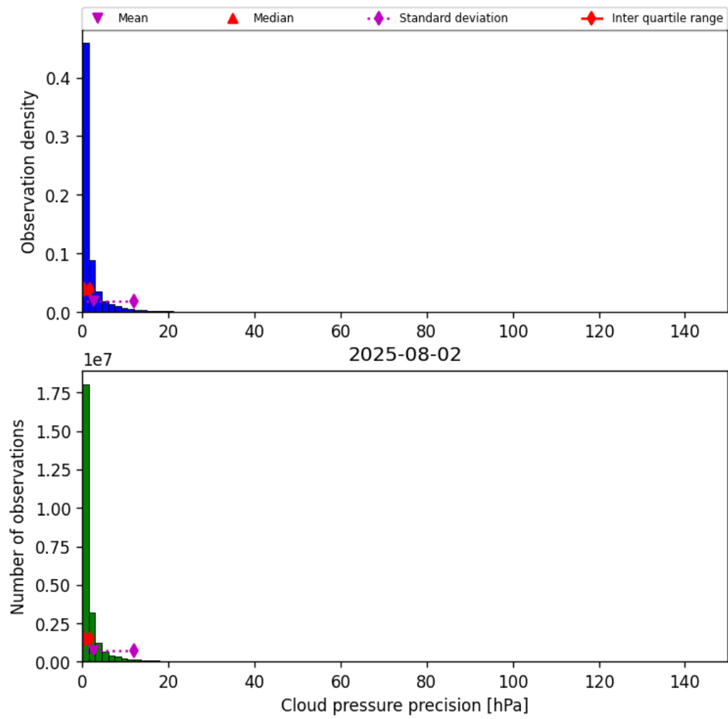
Figure 29: Histogram of “Cloud pressure precision” for 2025-08-02 to 2025-08-03
