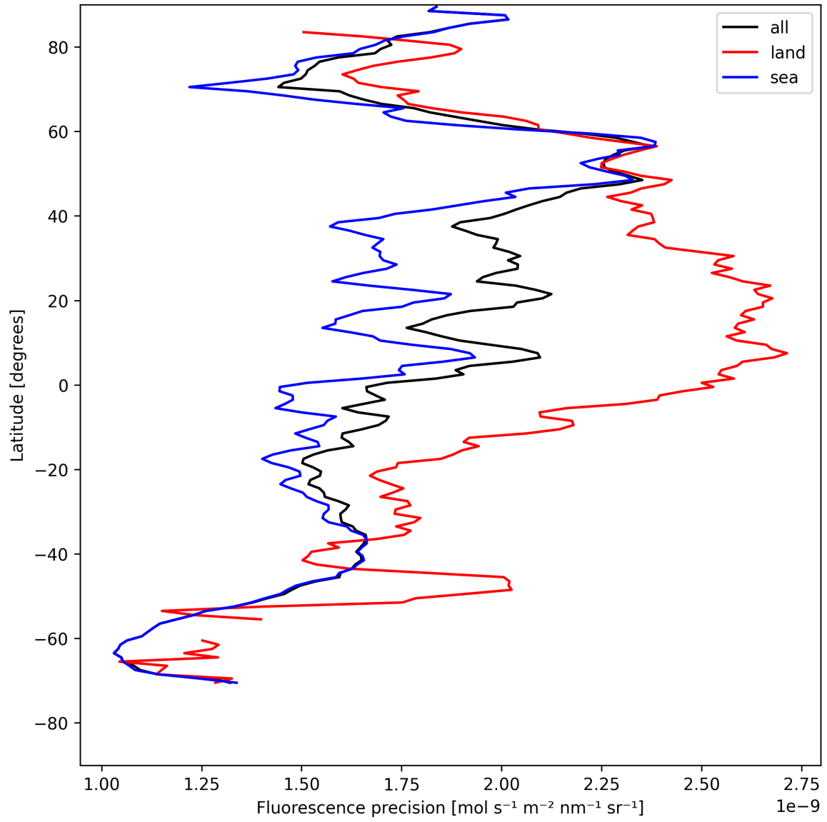
Figure 22: Zonal average of “Fluorescence precision” for 2025-08-02 to 2025-08-03.
