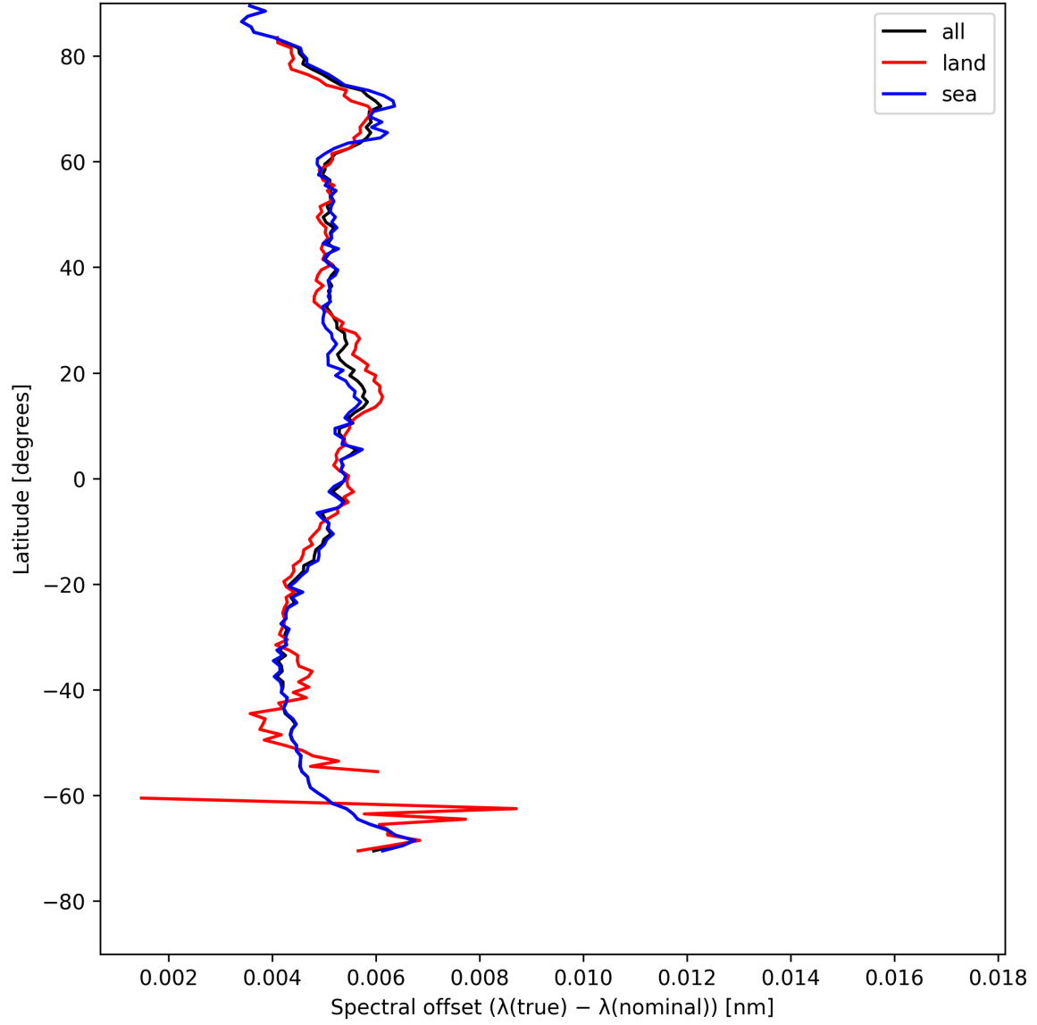
Figure 26: Zonal average of “Spectral offset ( \lambda_{\text{true}} - \lambda_{\text{nominal}} )” for 2025-08-02 to 2025-08-03.
