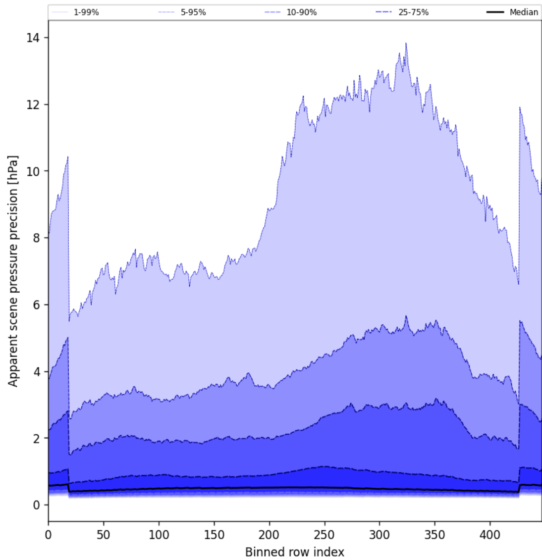
Figure 52: Along track statistics of “Apparent scene pressure precision” for 2025-08-02 to 2025-08-03
