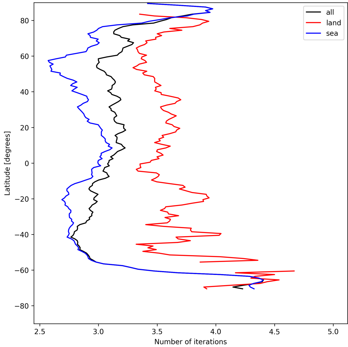
Figure 20: Zonal average of “Number of iterations” for 2025-08-02 to 2025-08-03.
