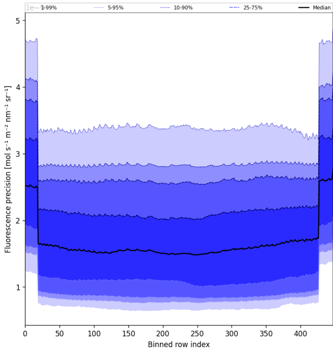
Figure 56: Along track statistics of “Fluorescence precision” for 2025-08-02 to 2025-08-03
