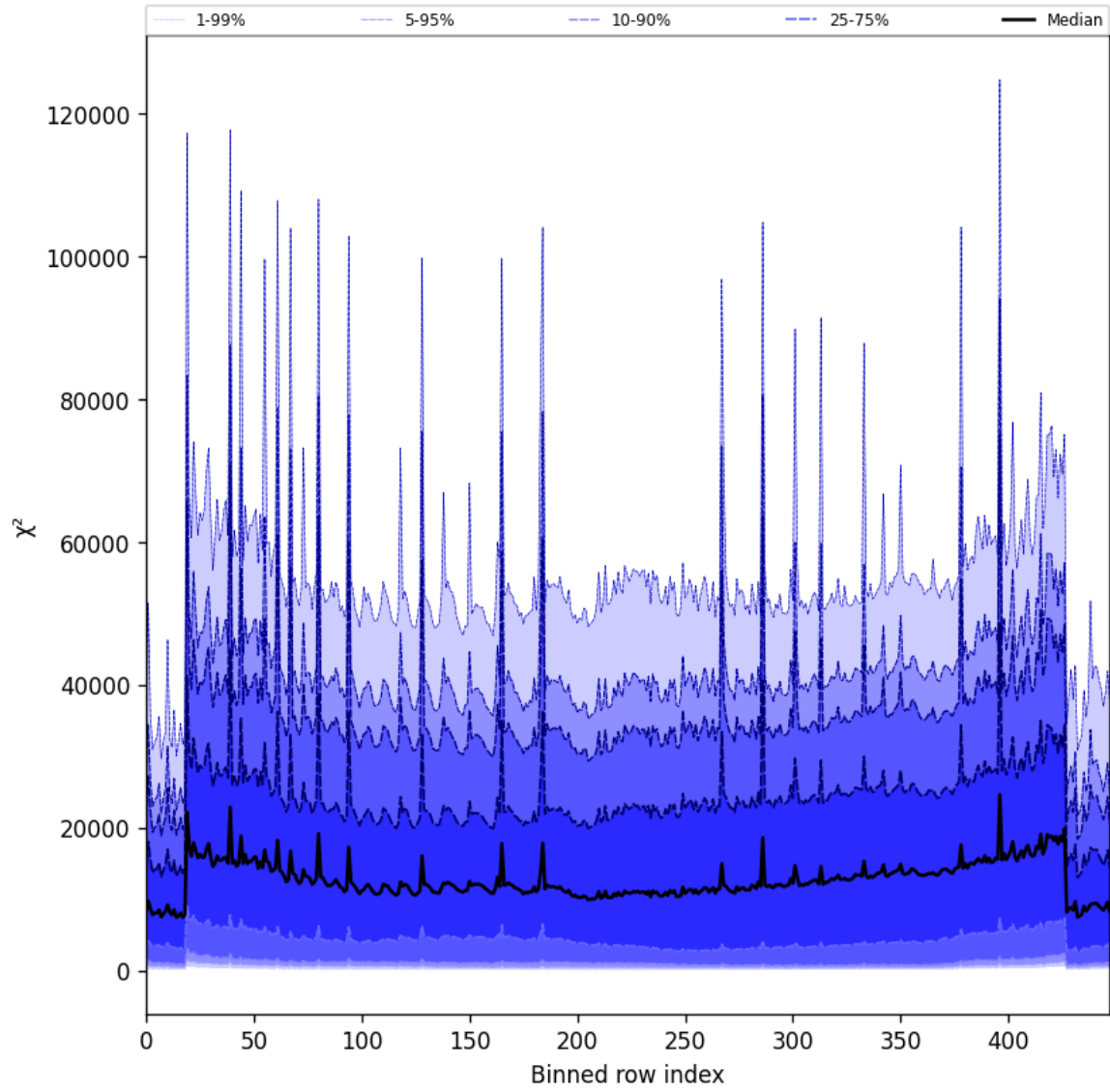
Figure 53: Along track statistics of “ \chi^2 ” for 2025-08-02 to 2025-08-03
