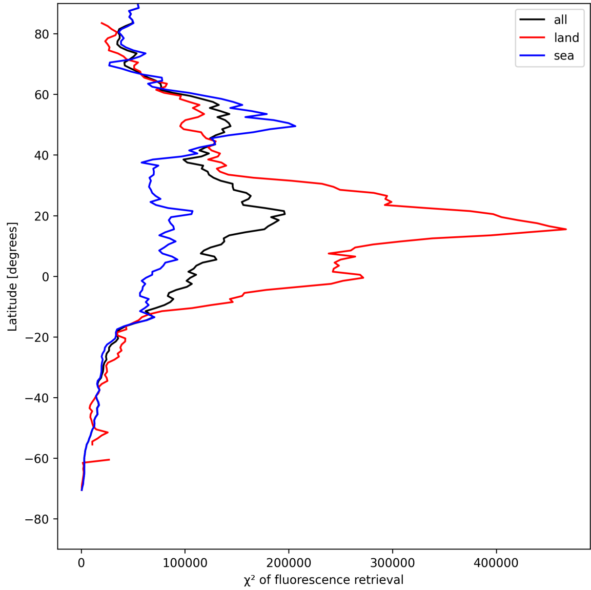
Figure 23: Zonal average of “ \chi^2 of fluorescence retrieval” for 2025-08-02 to 2025-08-03.
