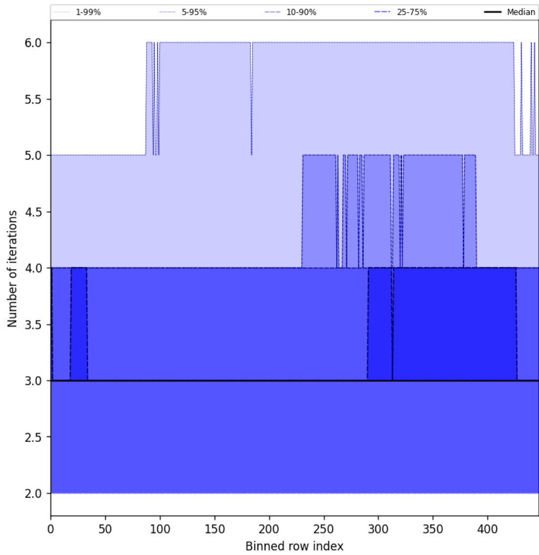
Figure 54: Along track statistics of “Number of iterations” for 2025-08-02 to 2025-08-03
