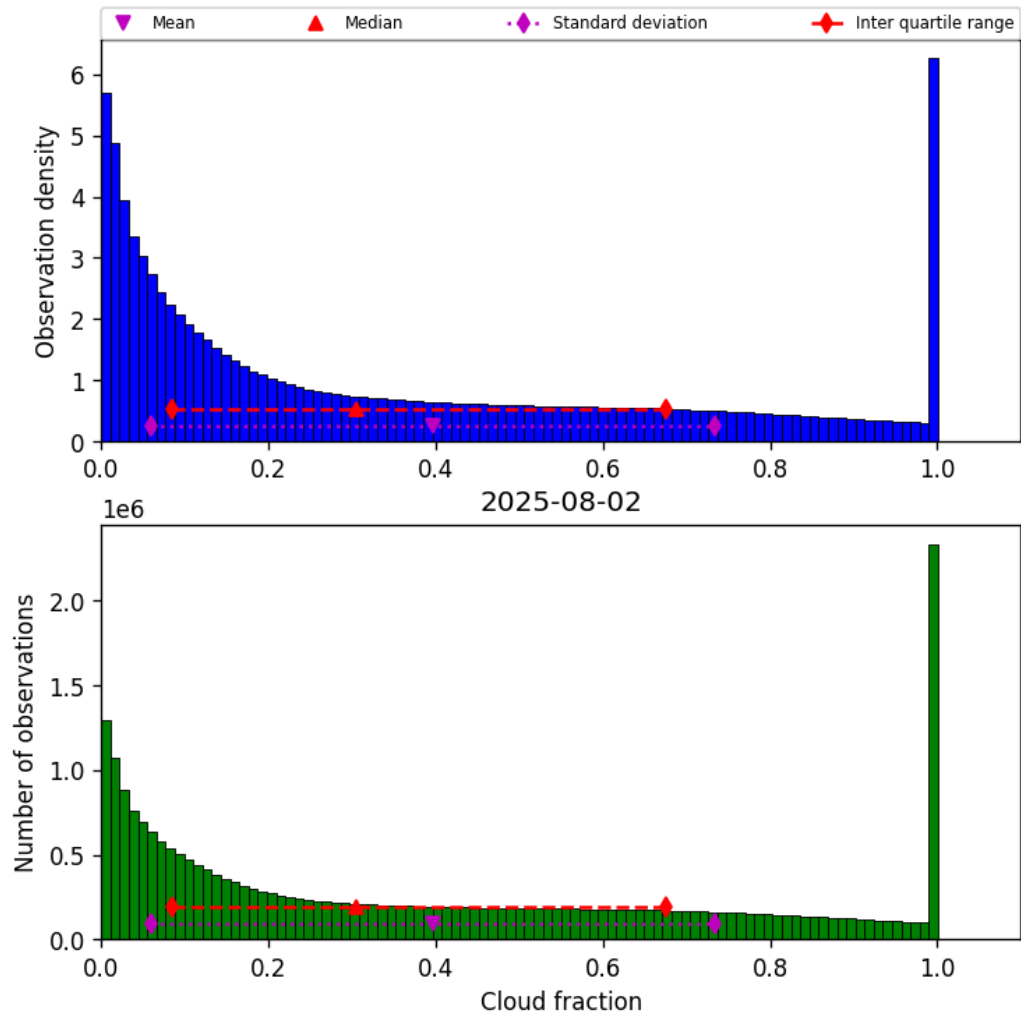
Figure 30: Histogram of “Cloud fraction” for 2025-08-02 to 2025-08-03
