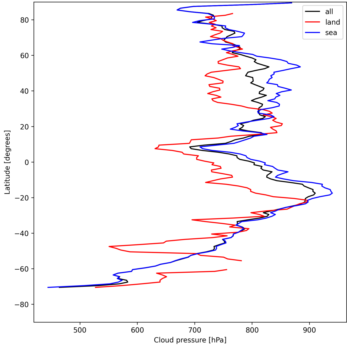
Figure 11: Zonal average of “Cloud pressure” for 2025-08-02 to 2025-08-03.
