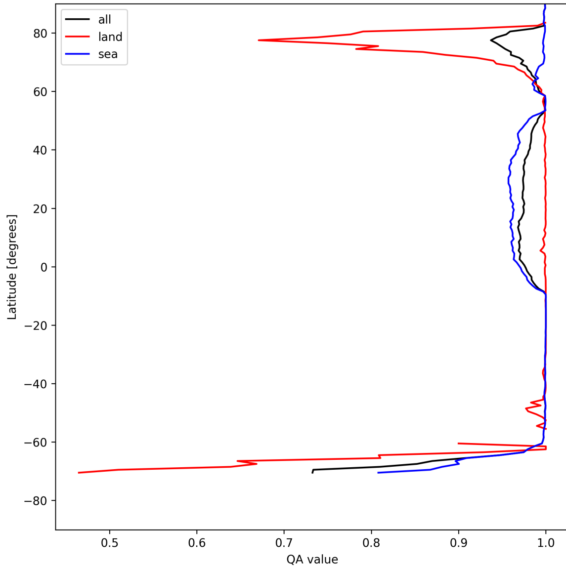
Figure 10: Zonal average of “QA value” for 2025-08-02 to 2025-08-03.
