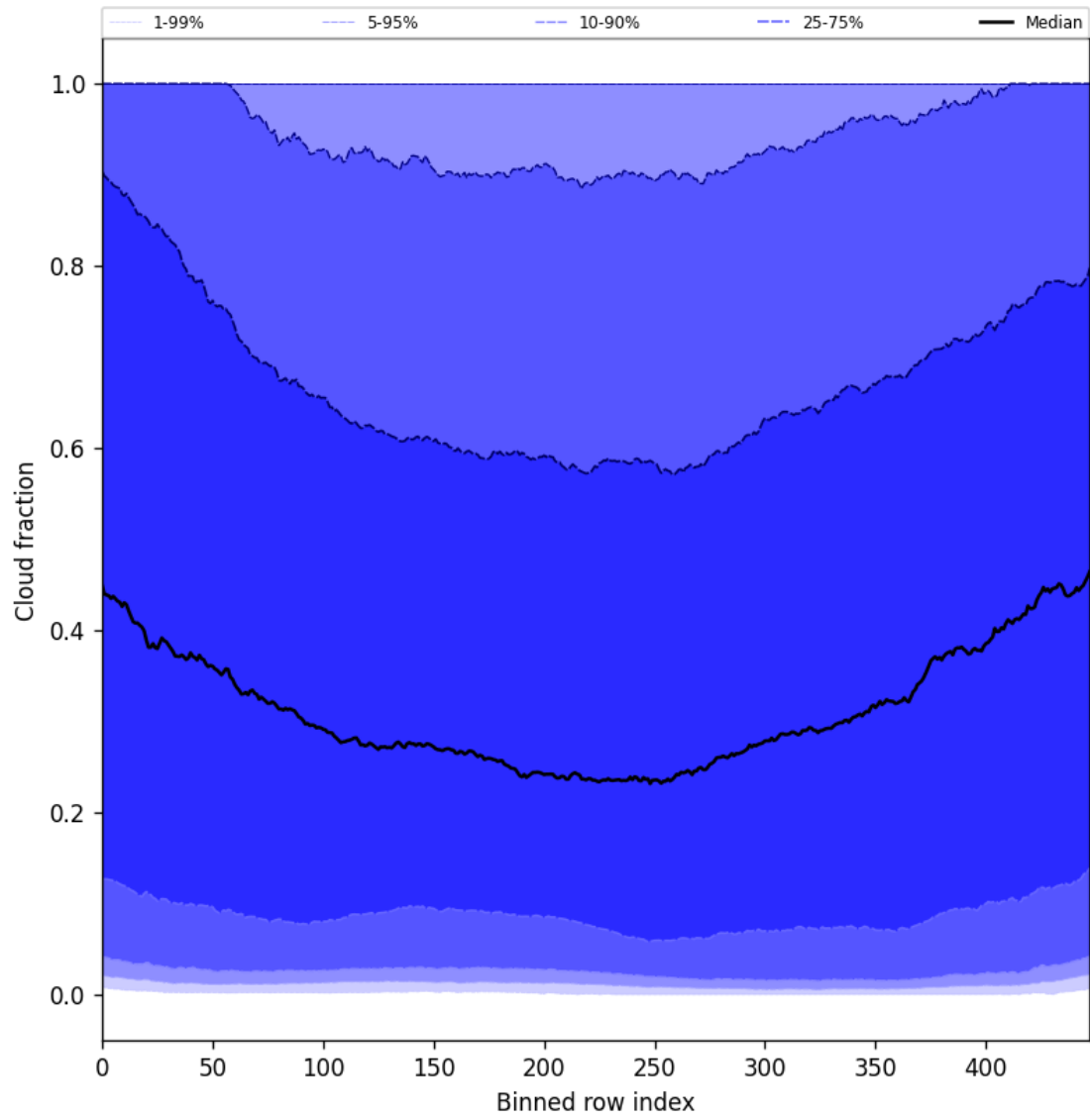
Figure 47: Along track statistics of “Cloud fraction” for 2025-08-02 to 2025-08-03
