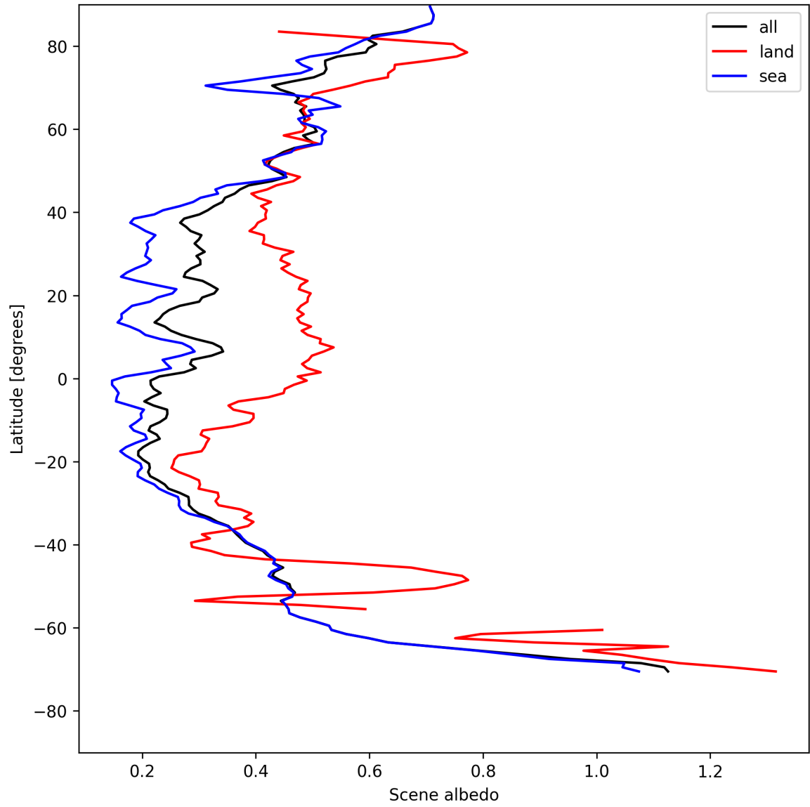
Figure 15: Zonal average of “Scene albedo” for 2025-08-02 to 2025-08-03.
