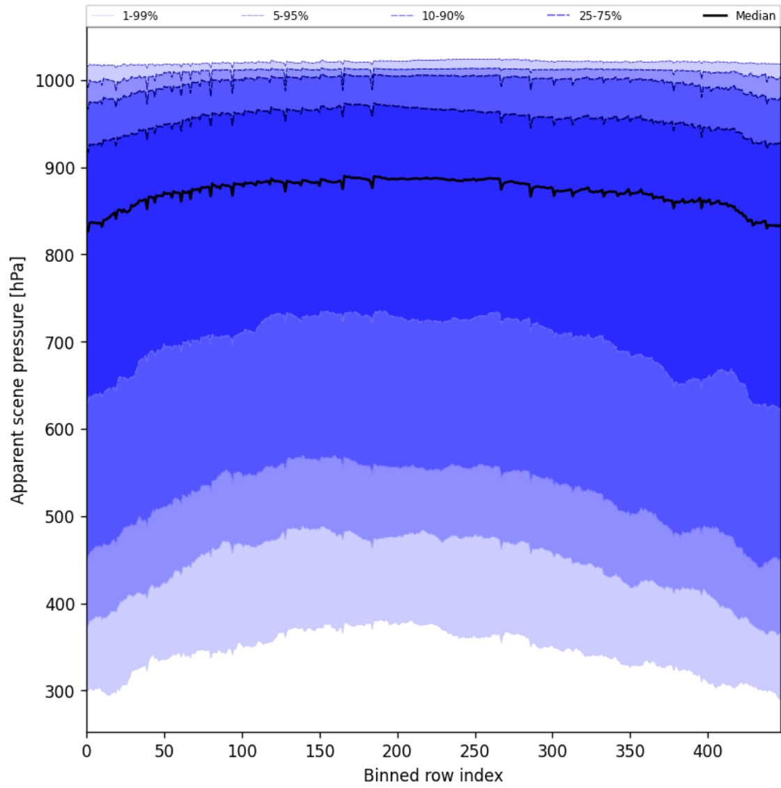
Figure 51: Along track statistics of “Apparent scene pressure” for 2025-08-02 to 2025-08-03
