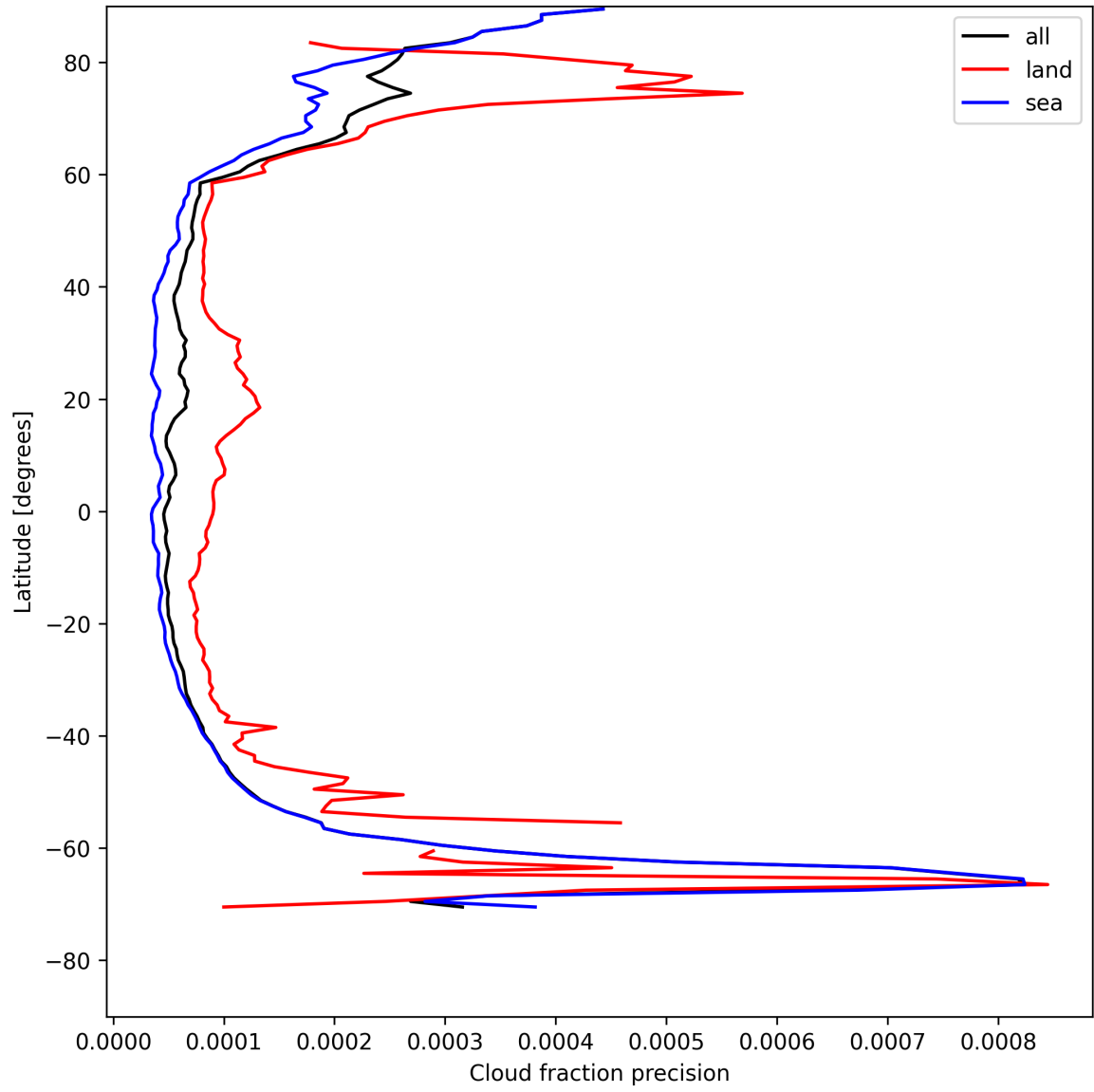
Figure 14: Zonal average of “Cloud fraction precision” for 2025-08-02 to 2025-08-03.
