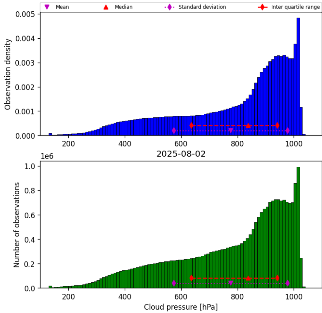
Figure 28: Histogram of “Cloud pressure” for 2025-08-02 to 2025-08-03
