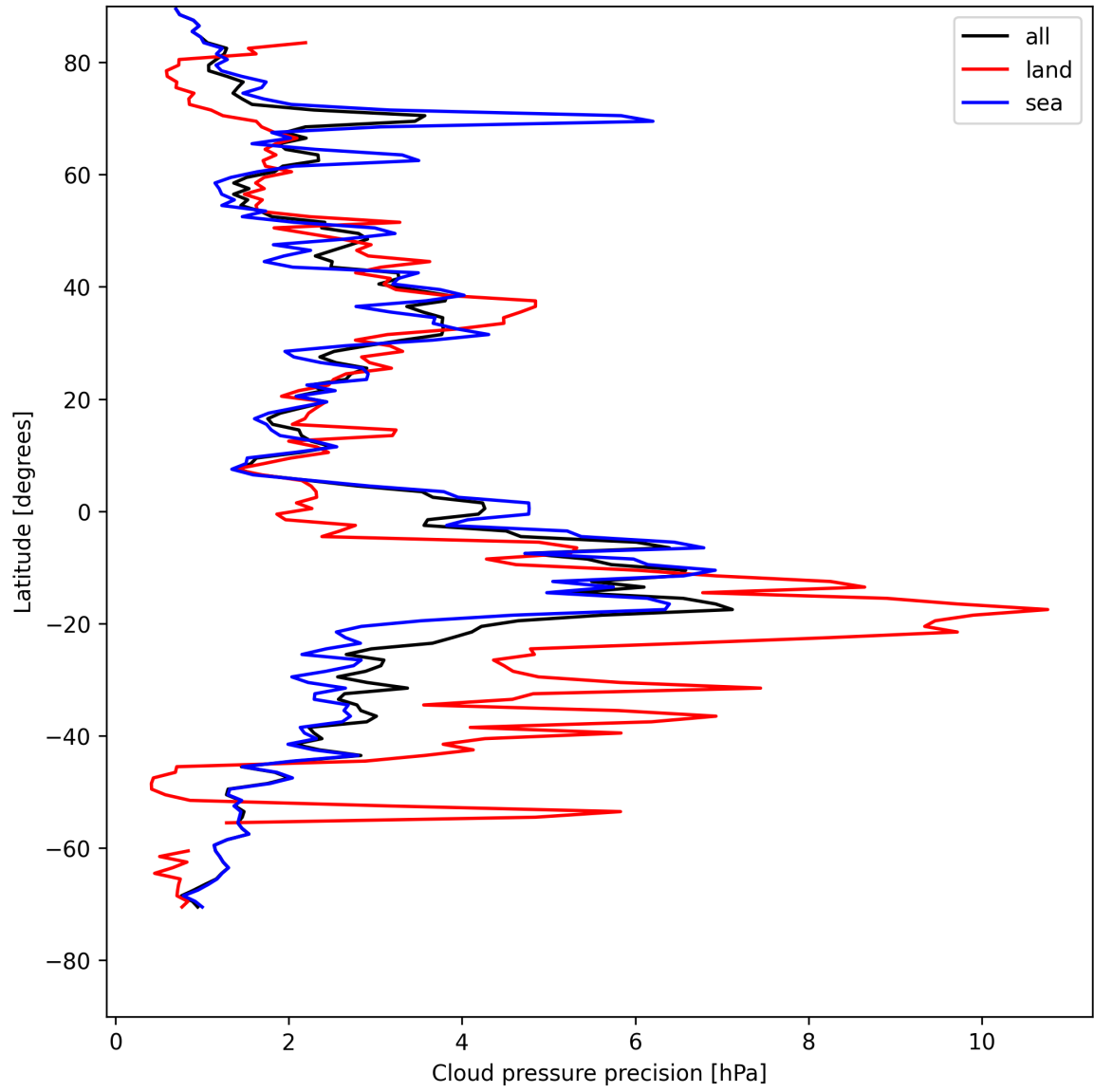
Figure 12: Zonal average of “Cloud pressure precision” for 2025-08-02 to 2025-08-03.
