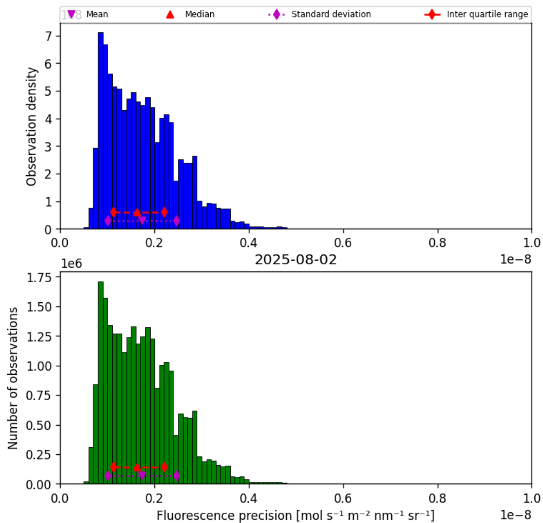
Figure 39: Histogram of “Fluorescence precision” for 2025-08-02 to 2025-08-03
