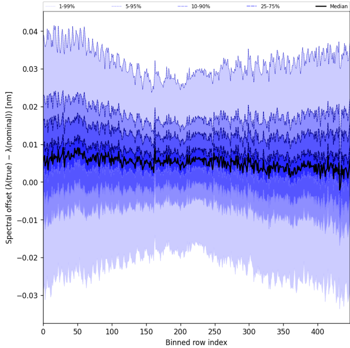
Figure 60: Along track statistics of “Spectral offset ( \lambda_{\text{true}} - \lambda_{\text{nominal}} )” for 2025-08-02 to 2025-08-03
