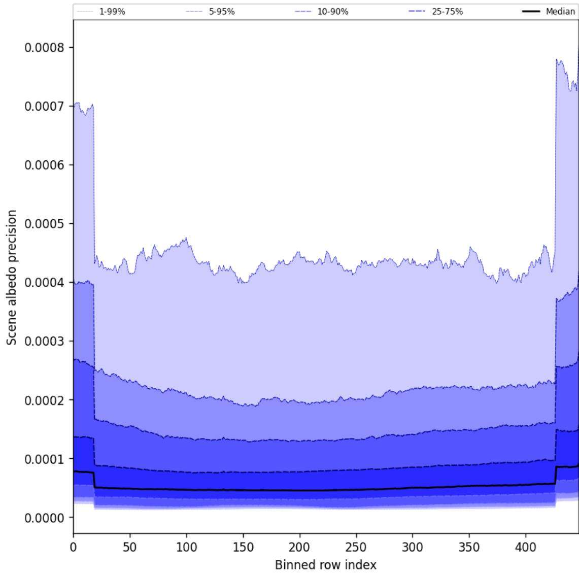
Figure 50: Along track statistics of “Scene albedo precision” for 2025-08-02 to 2025-08-03
