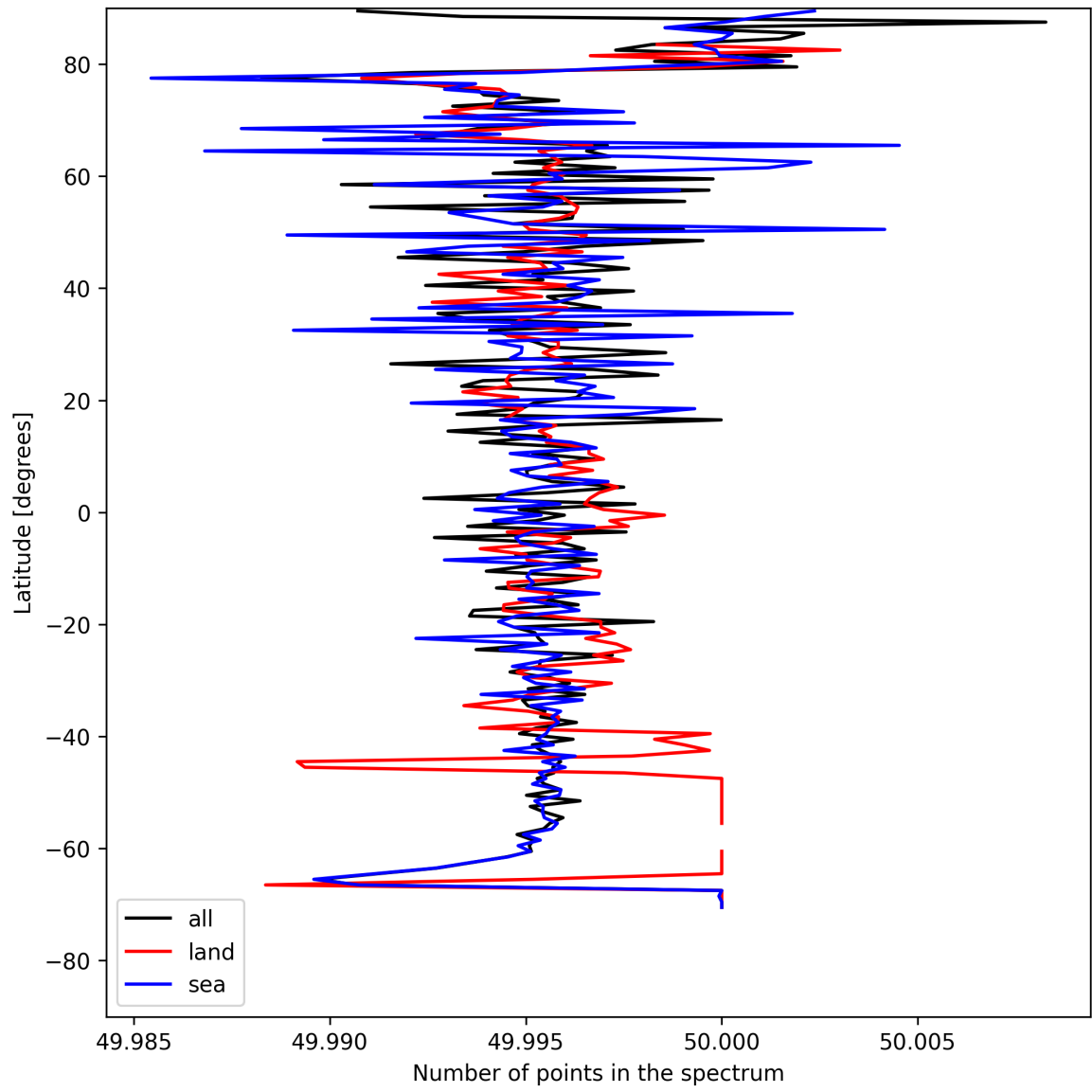
Figure 25: Zonal average of “Number of points in the spectrum” for 2025-08-02 to 2025-08-03.
