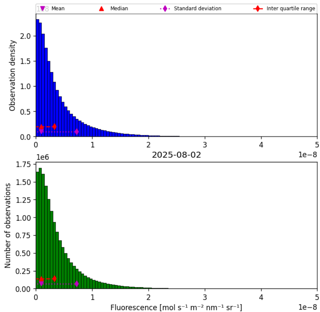
Figure 38: Histogram of “Fluorescence” for 2025-08-02 to 2025-08-03
