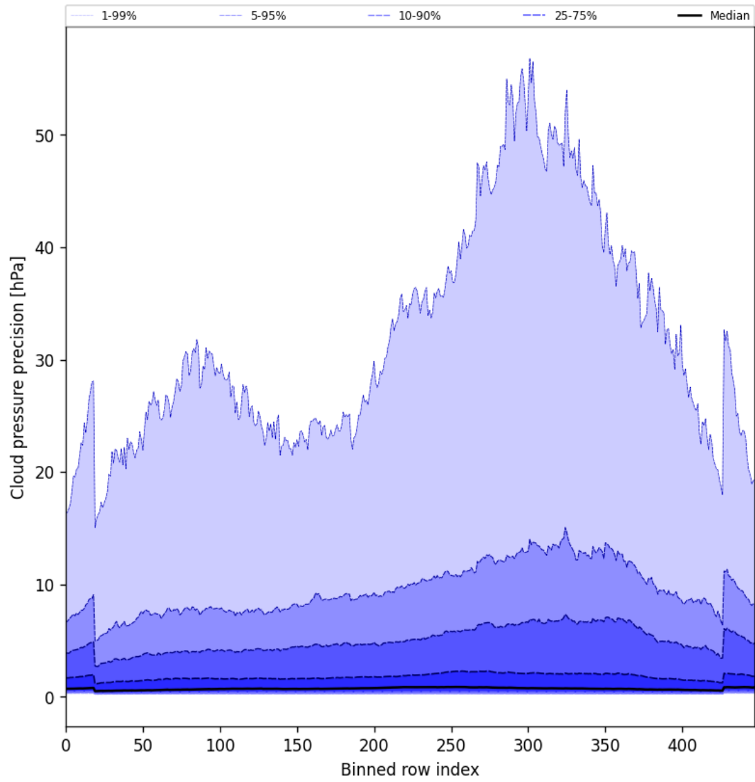
Figure 46: Along track statistics of “Cloud pressure precision” for 2025-08-02 to 2025-08-03
