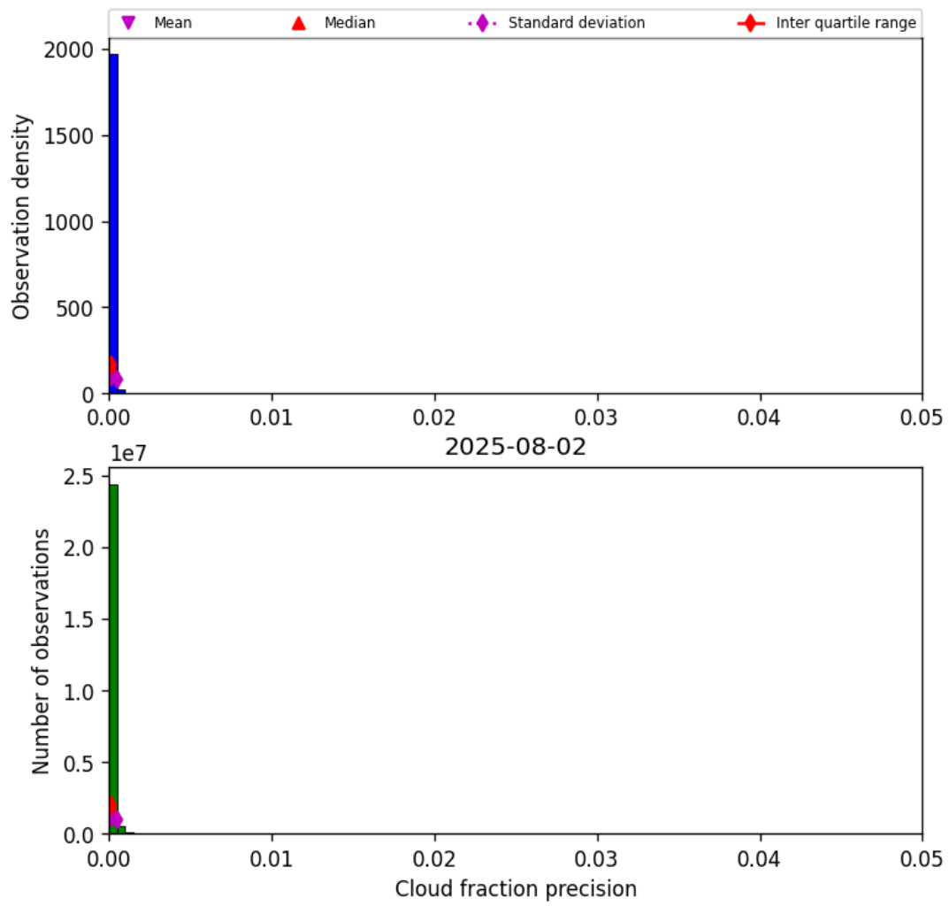
Figure 31: Histogram of “Cloud fraction precision” for 2025-08-02 to 2025-08-03
