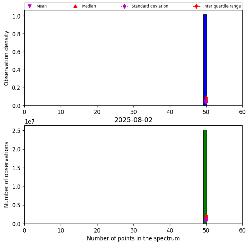
Figure 42: Histogram of “Number of points in the spectrum” for 2025-08-02 to 2025-08-03
