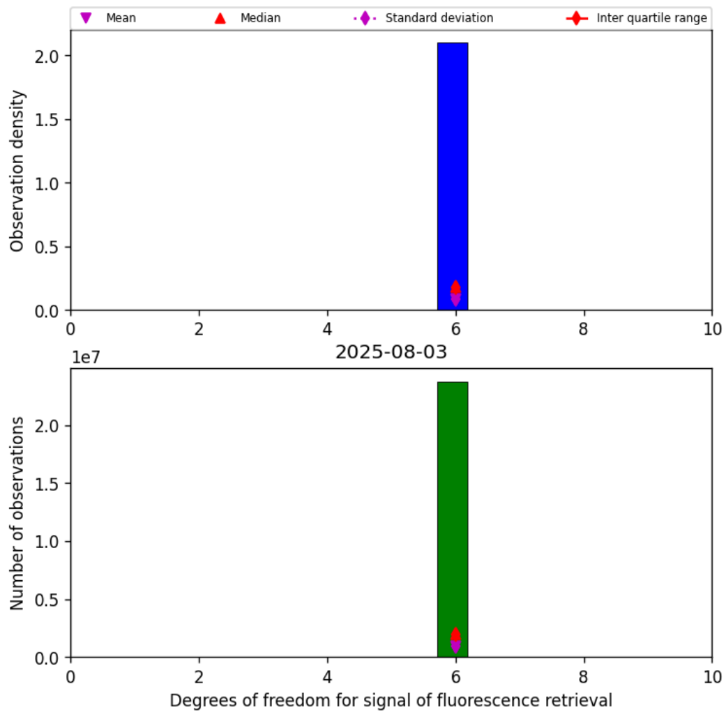
Figure 41: Histogram of “Degrees of freedom for signal of fluorescence retrieval” for 2025-08-03 to 2025-08-04
