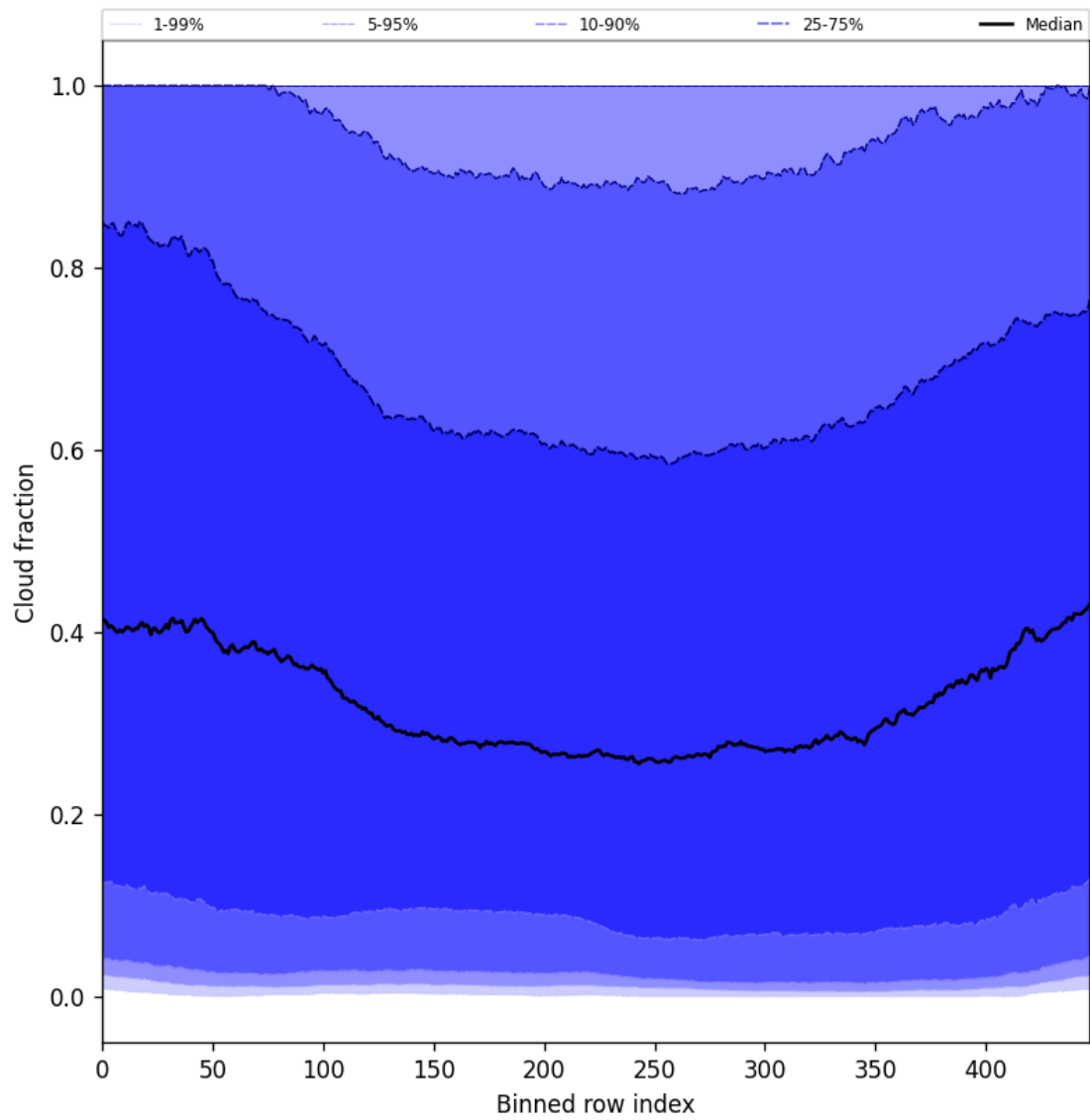
Figure 47: Along track statistics of “Cloud fraction” for 2025-08-03 to 2025-08-04
