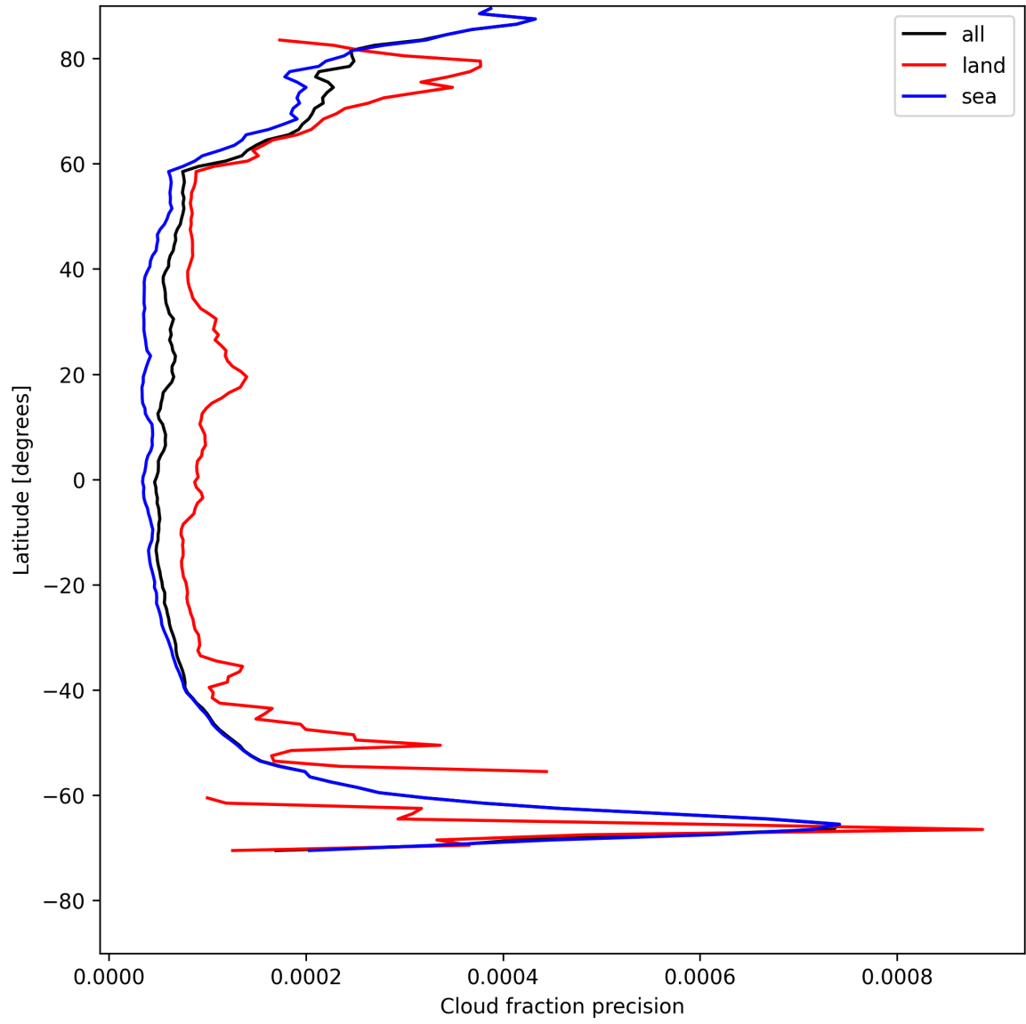
Figure 14: Zonal average of “Cloud fraction precision” for 2025-08-03 to 2025-08-04.
