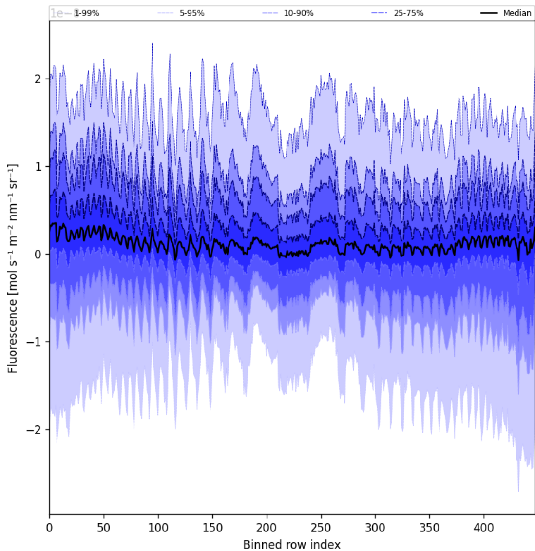
Figure 55: Along track statistics of “Fluorescence” for 2025-08-03 to 2025-08-04
