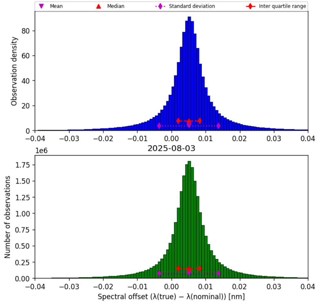
Figure 43: Histogram of “Spectral offset ( \lambda_{\text{true}} - \lambda_{\text{nominal}} )” for 2025-08-03 to 2025-08-04
