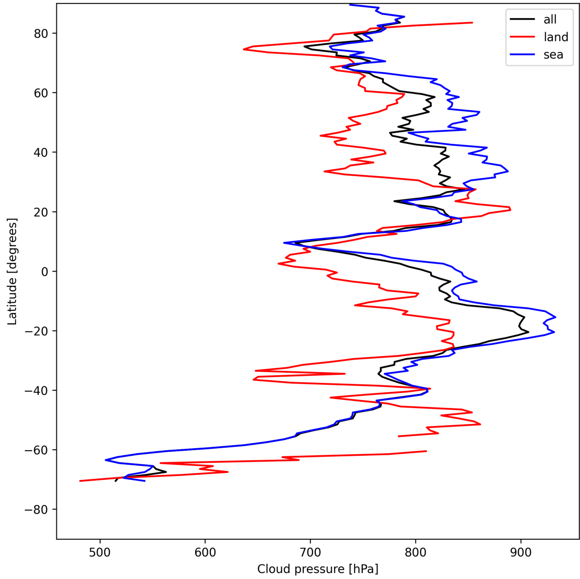
Figure 11: Zonal average of “Cloud pressure” for 2025-08-03 to 2025-08-04.
