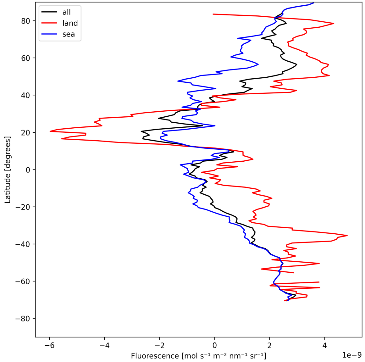
Figure 21: Zonal average of “Fluorescence” for 2025-08-03 to 2025-08-04.
