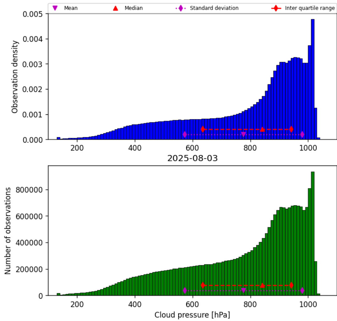
Figure 28: Histogram of “Cloud pressure” for 2025-08-03 to 2025-08-04
