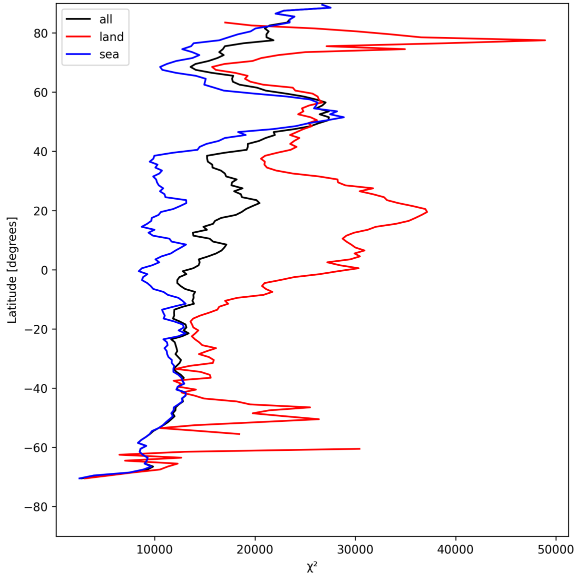
Figure 19: Zonal average of “ \chi^2 ” for 2025-08-03 to 2025-08-04.
