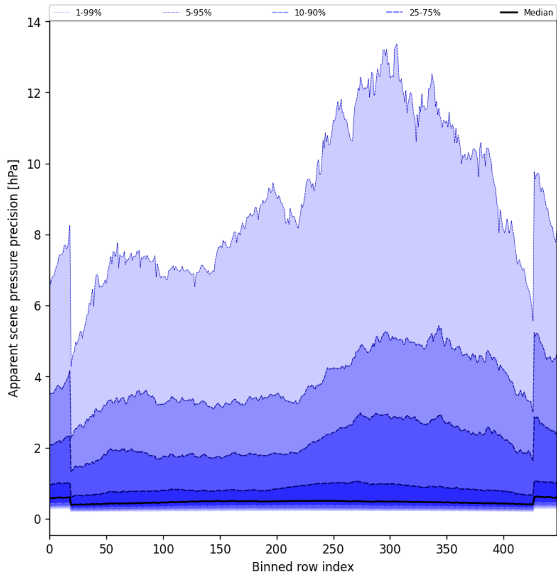
Figure 52: Along track statistics of “Apparent scene pressure precision” for 2025-08-03 to 2025-08-04
