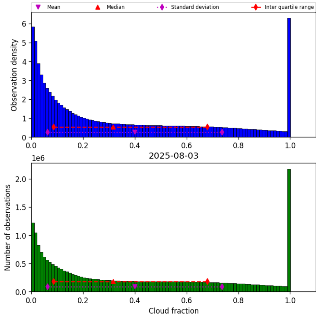
Figure 30: Histogram of “Cloud fraction” for 2025-08-03 to 2025-08-04
