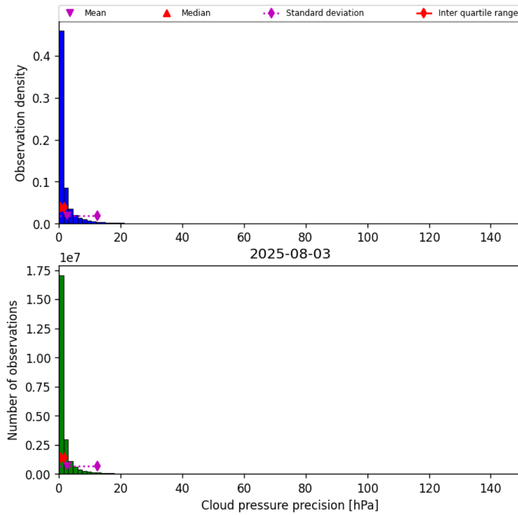
Figure 29: Histogram of “Cloud pressure precision” for 2025-08-03 to 2025-08-04
