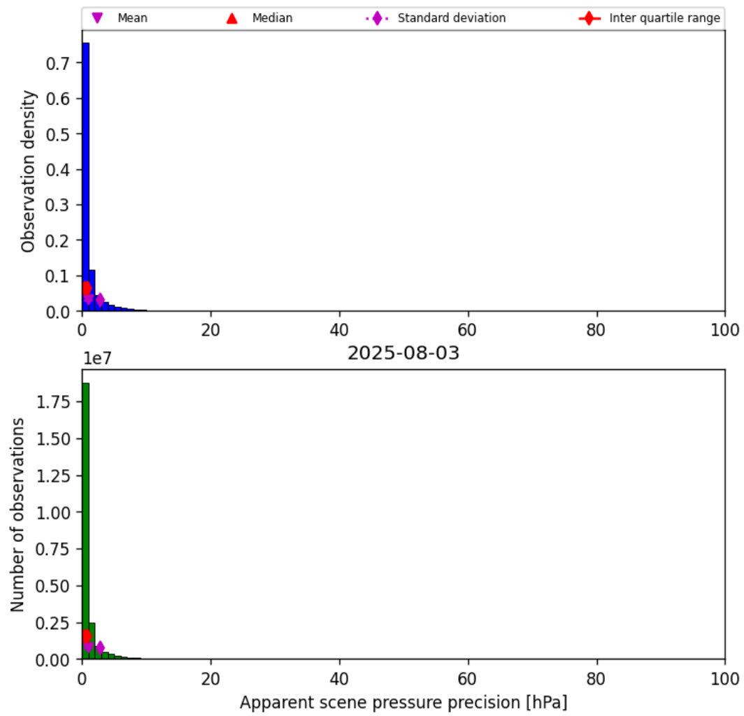
Figure 35: Histogram of “Apparent scene pressure precision” for 2025-08-03 to 2025-08-04
