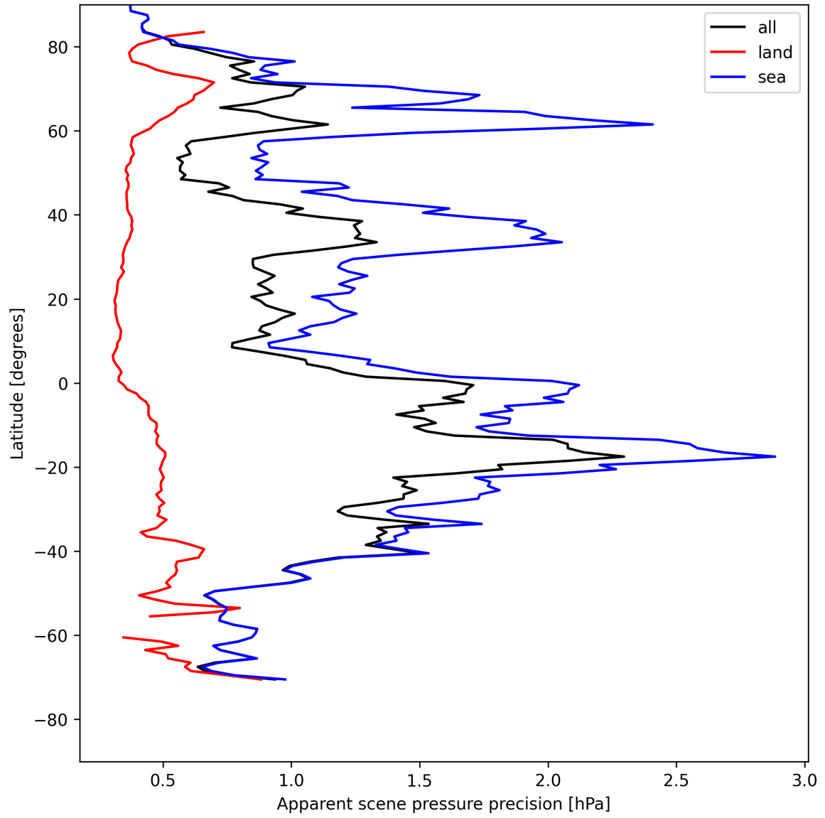
Figure 18: Zonal average of “Apparent scene pressure precision” for 2025-08-03 to 2025-08-04.
