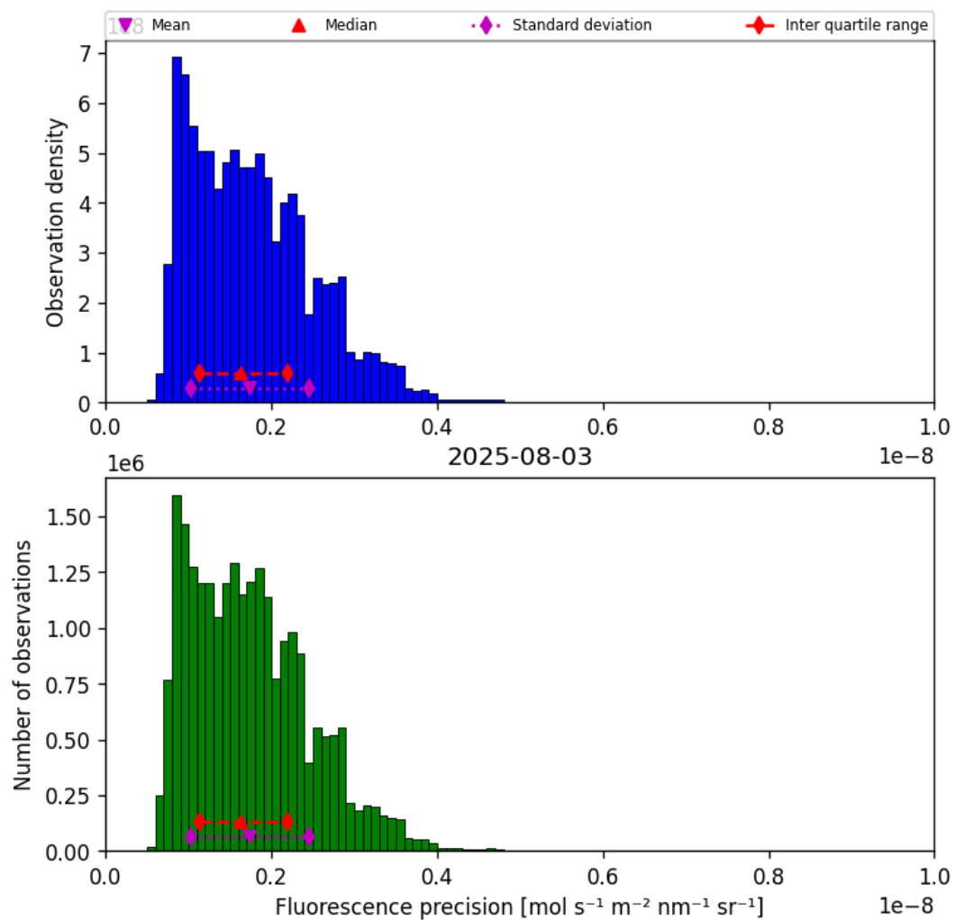
Figure 39: Histogram of “Fluorescence precision” for 2025-08-03 to 2025-08-04
