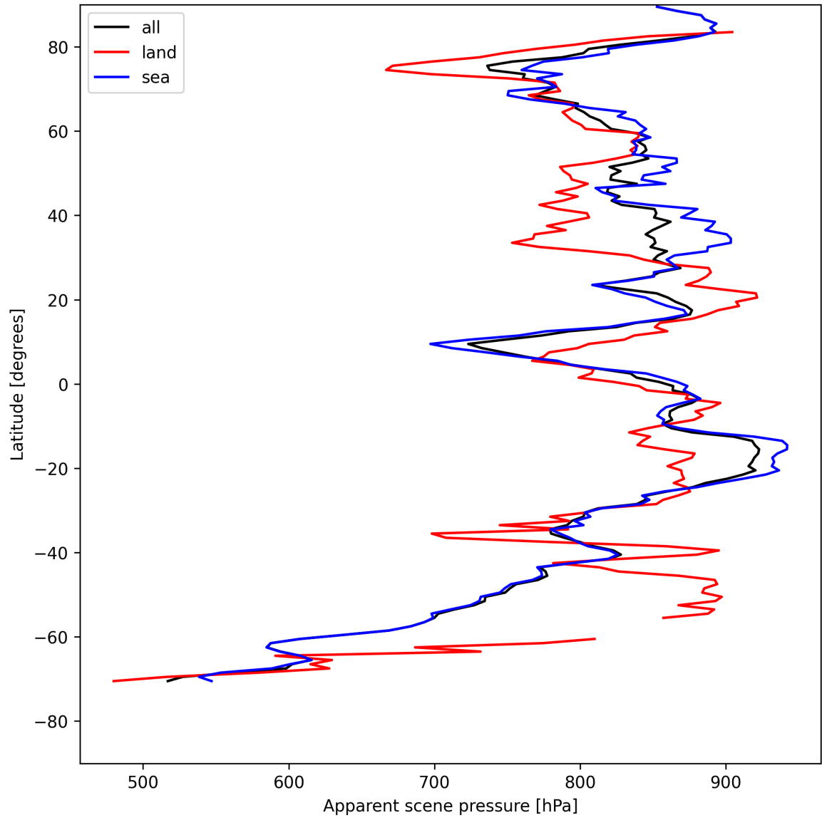
Figure 17: Zonal average of “Apparent scene pressure” for 2025-08-03 to 2025-08-04.
