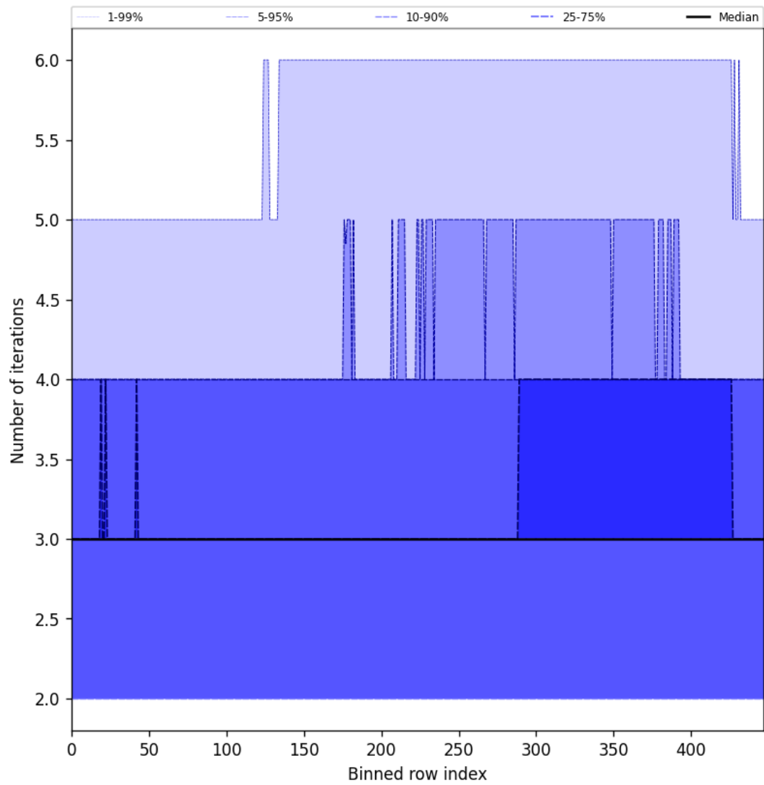
Figure 54: Along track statistics of “Number of iterations” for 2025-08-03 to 2025-08-04
