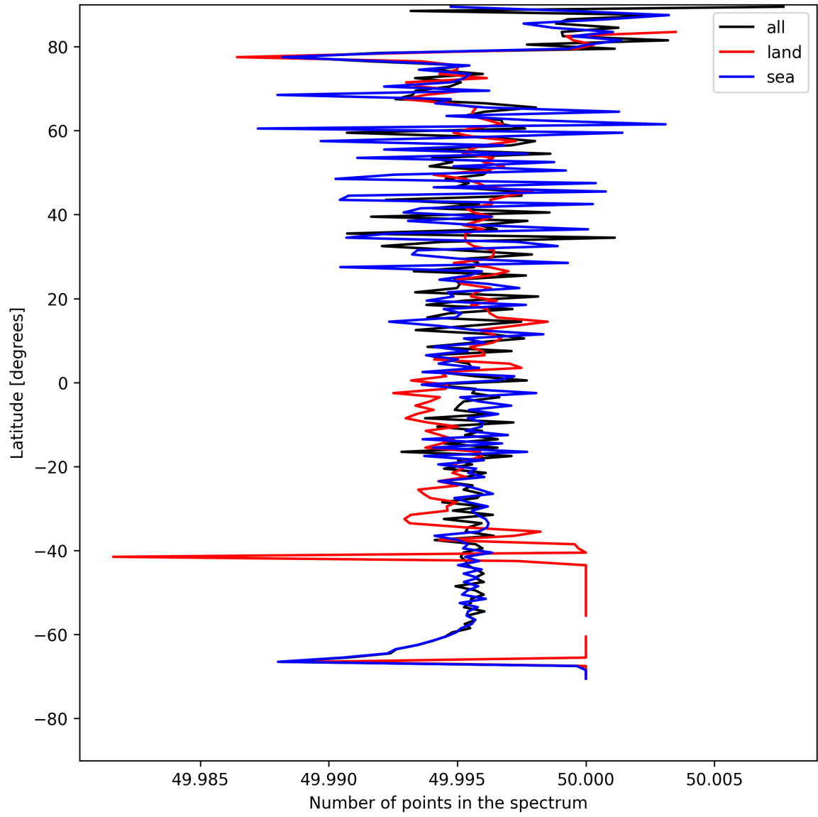
Figure 25: Zonal average of “Number of points in the spectrum” for 2025-08-03 to 2025-08-04.
