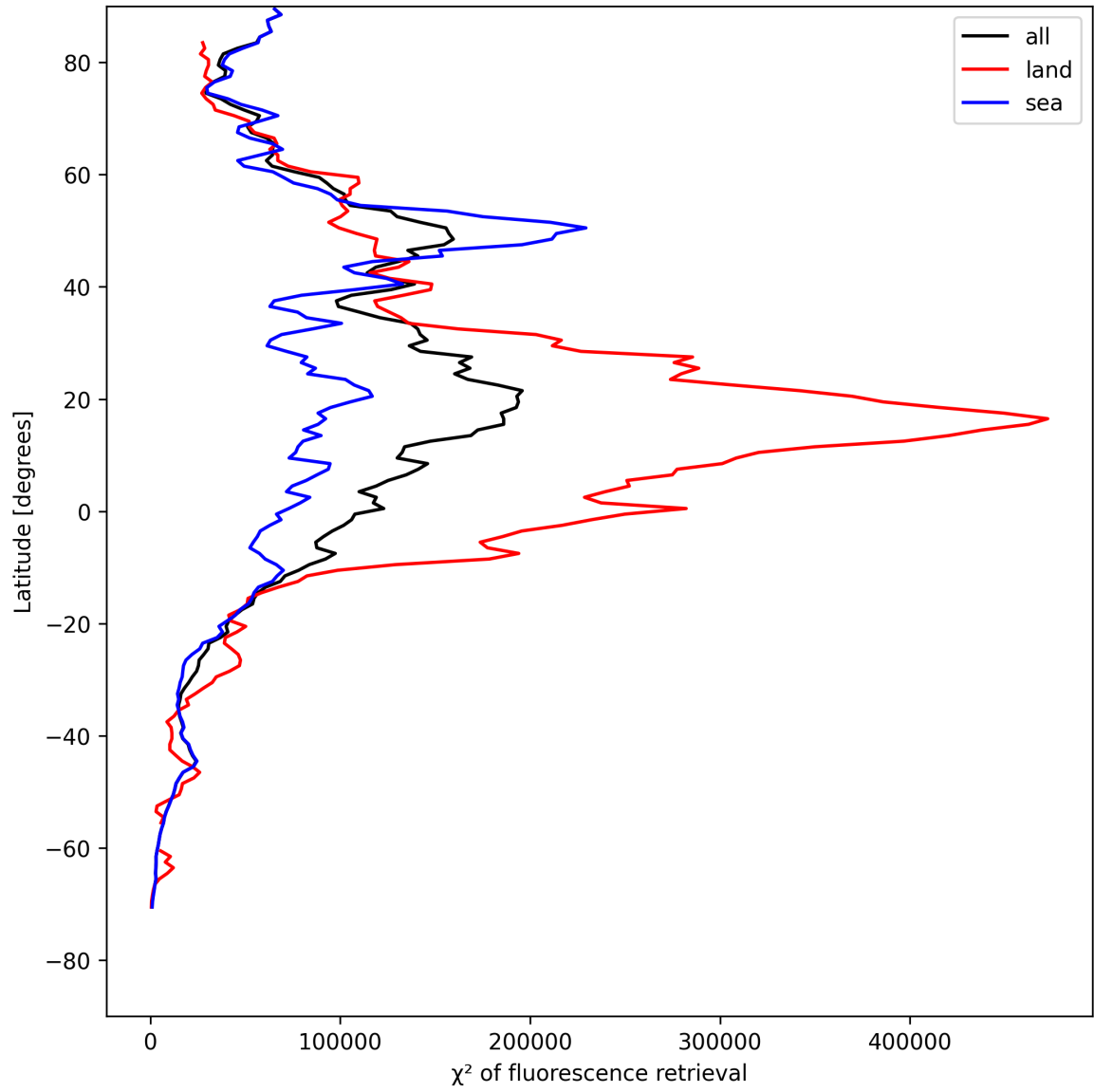
Figure 23: Zonal average of “ \chi^2 of fluorescence retrieval” for 2025-08-03 to 2025-08-04.
