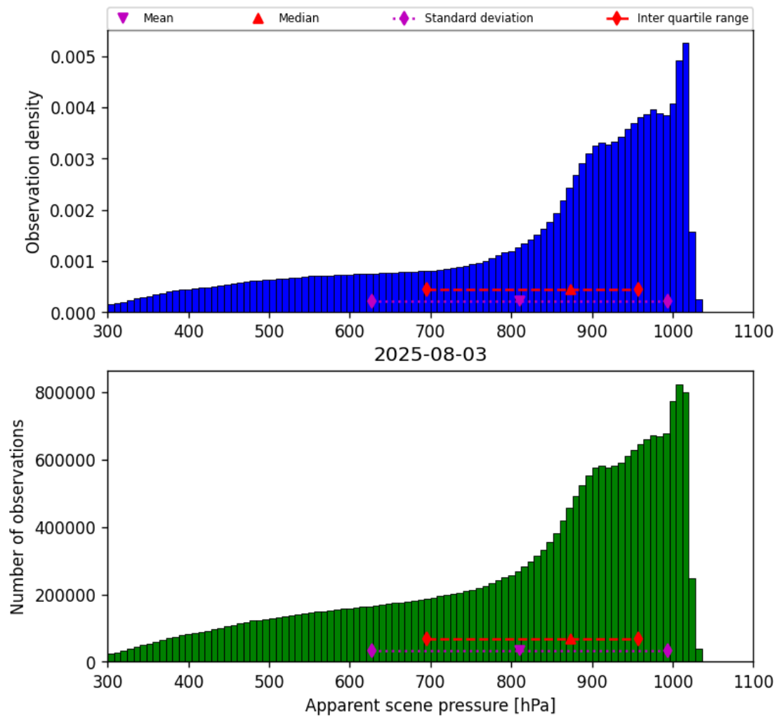
Figure 34: Histogram of “Apparent scene pressure” for 2025-08-03 to 2025-08-04
