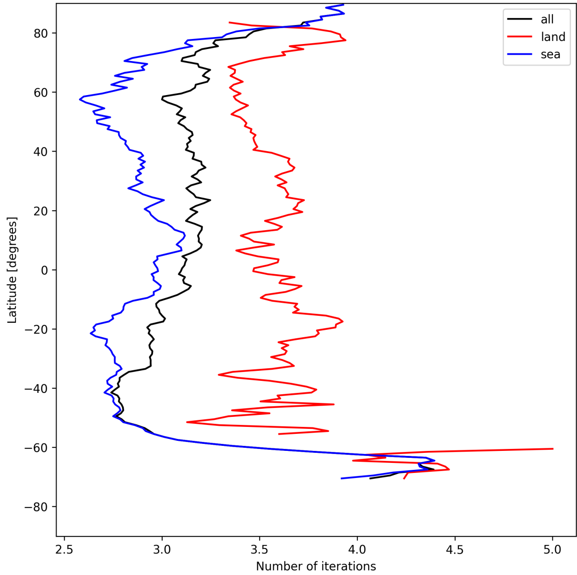
Figure 20: Zonal average of “Number of iterations” for 2025-08-03 to 2025-08-04.
