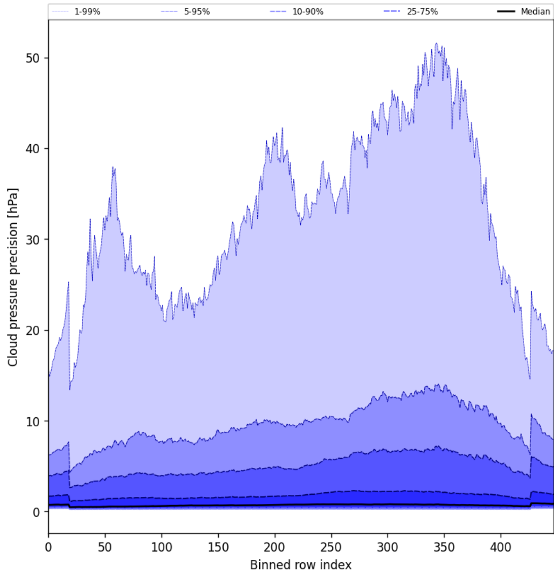
Figure 46: Along track statistics of “Cloud pressure precision” for 2025-08-03 to 2025-08-04
