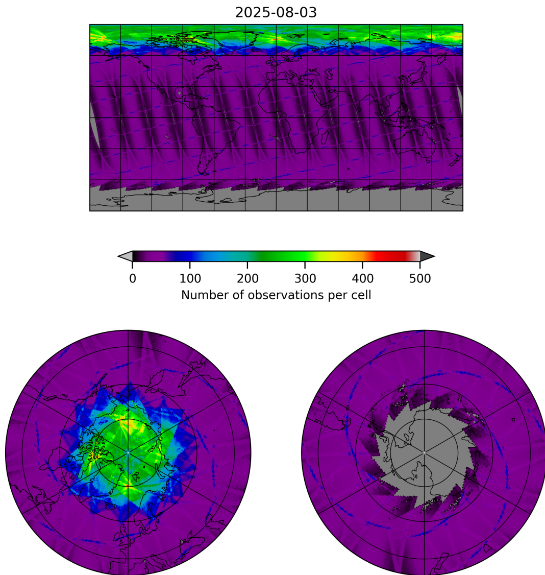
Figure 9: Map of the number of observations for 2025-08-03 to 2025-08-04
