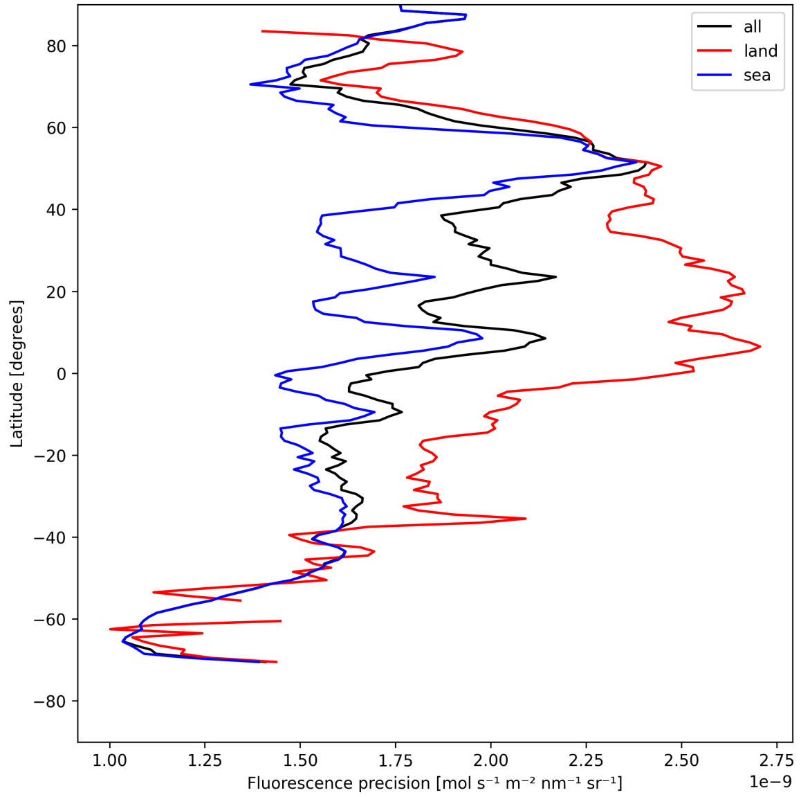
Figure 22: Zonal average of “Fluorescence precision” for 2025-08-03 to 2025-08-04.
