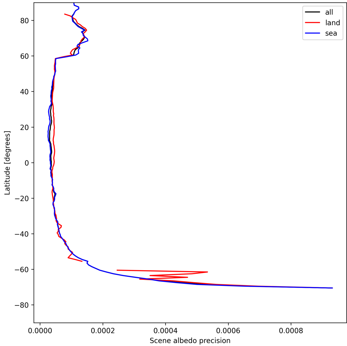
Figure 16: Zonal average of “Scene albedo precision” for 2025-08-03 to 2025-08-04.
