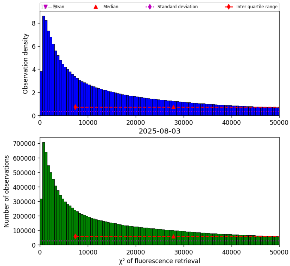
Figure 40: Histogram of “ \chi^2 of fluorescence retrieval” for 2025-08-03 to 2025-08-04
