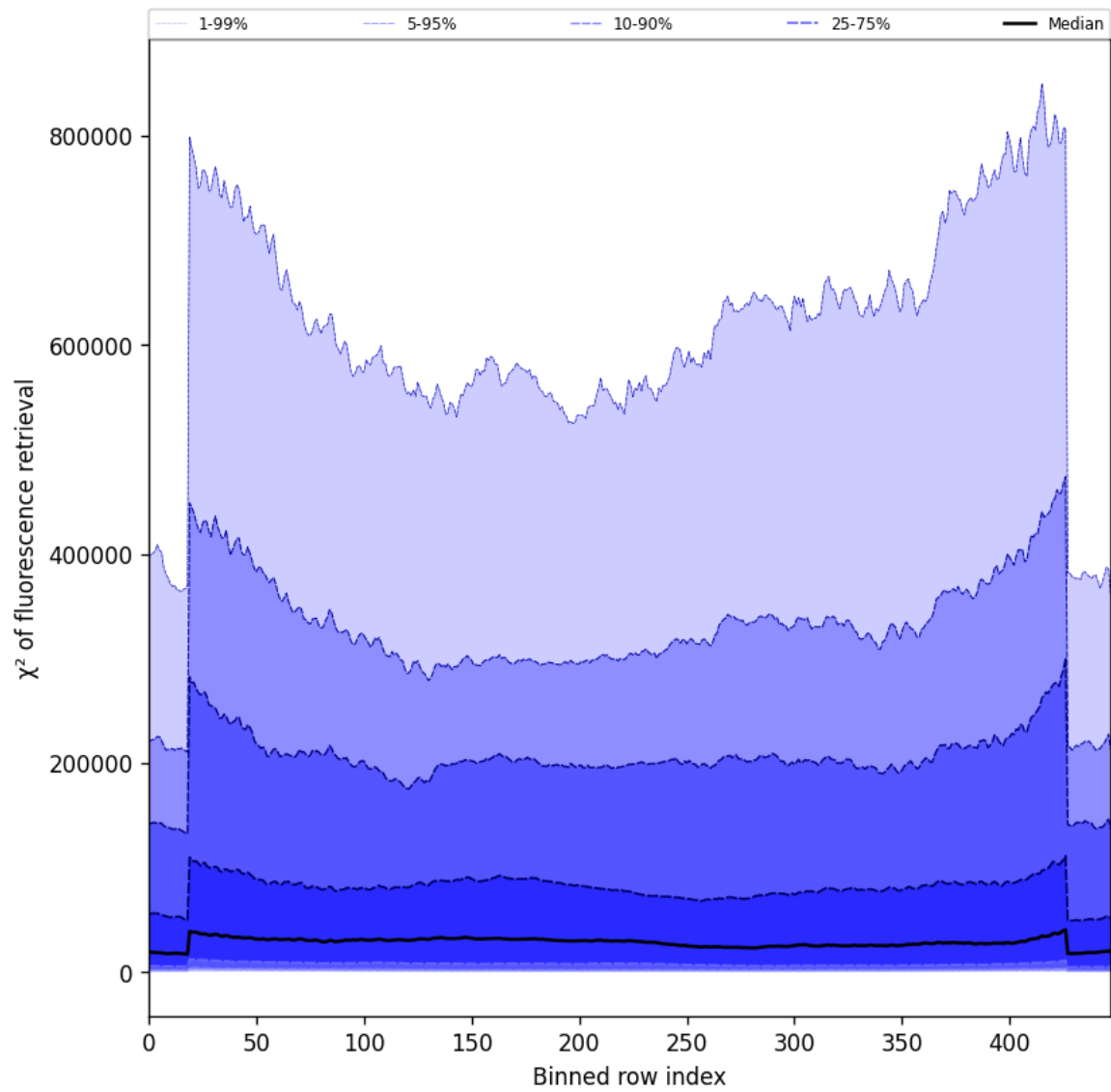
Figure 57: Along track statistics of “ \chi^2 of fluorescence retrieval” for 2025-08-03 to 2025-08-04
