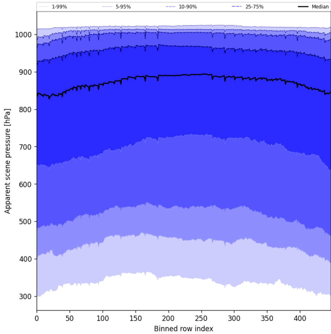
Figure 51: Along track statistics of “Apparent scene pressure” for 2025-08-03 to 2025-08-04
