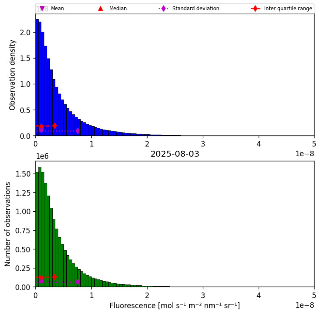
Figure 38: Histogram of “Fluorescence” for 2025-08-03 to 2025-08-04
