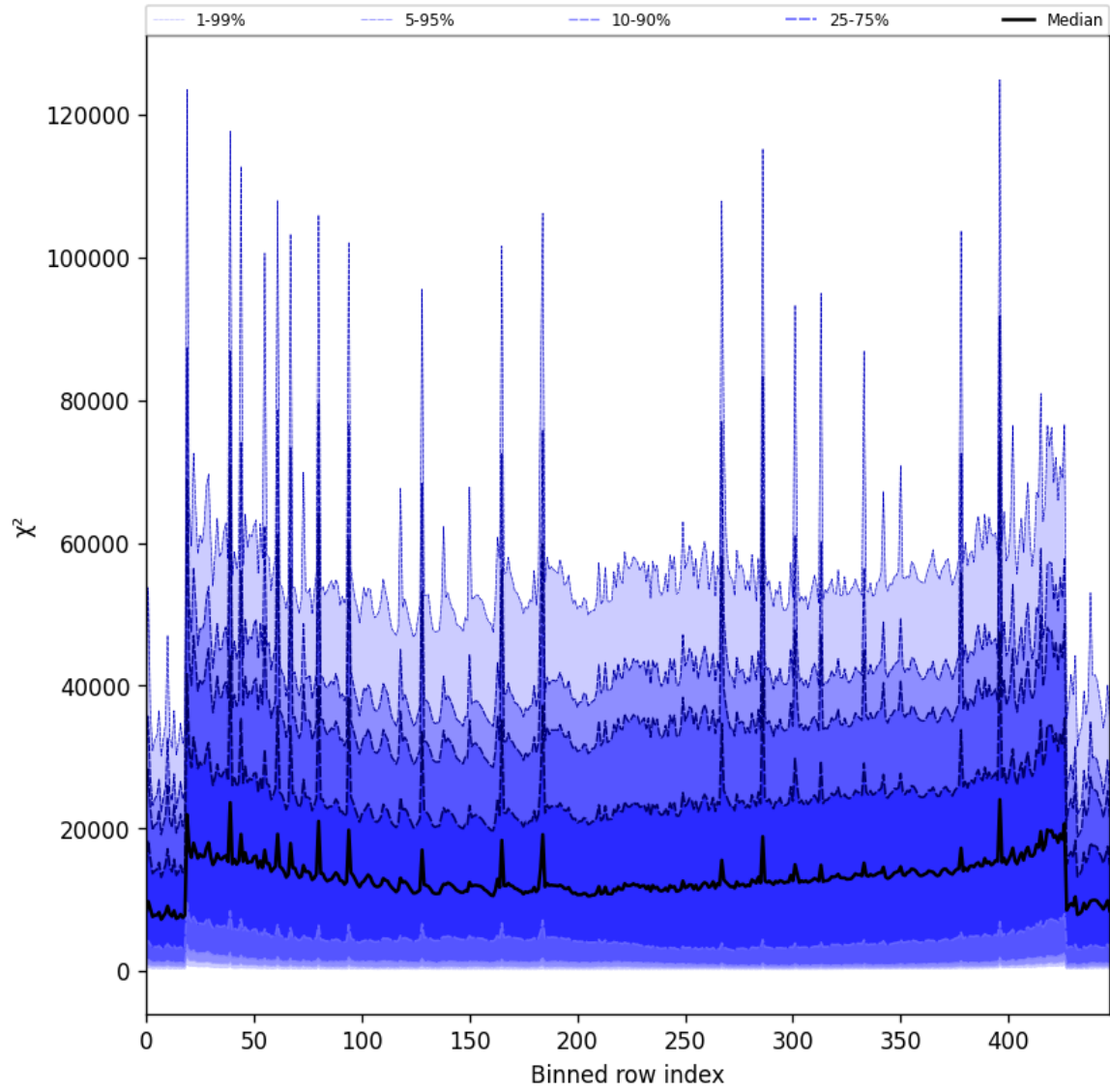
Figure 53: Along track statistics of “ \chi^2 ” for 2025-08-03 to 2025-08-04
