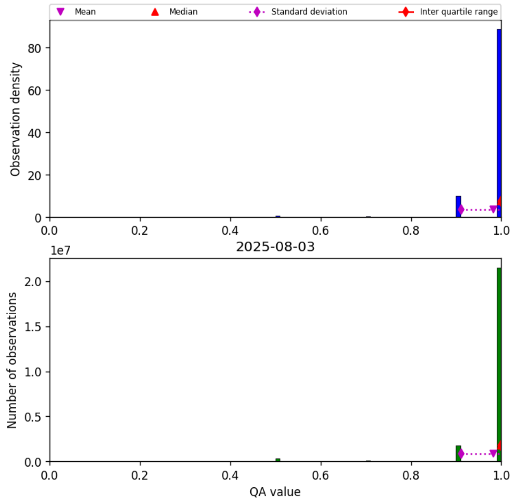
Figure 27: Histogram of “QA value” for 2025-08-03 to 2025-08-04
