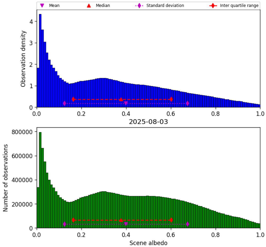
Figure 32: Histogram of “Scene albedo” for 2025-08-03 to 2025-08-04
