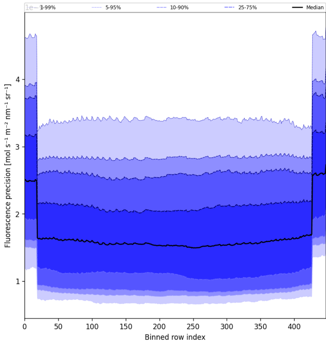
Figure 56: Along track statistics of “Fluorescence precision” for 2025-08-03 to 2025-08-04
