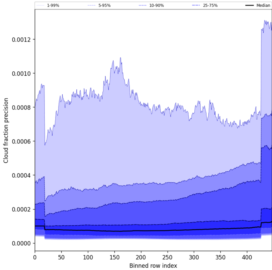
Figure 48: Along track statistics of “Cloud fraction precision” for 2025-08-03 to 2025-08-04
