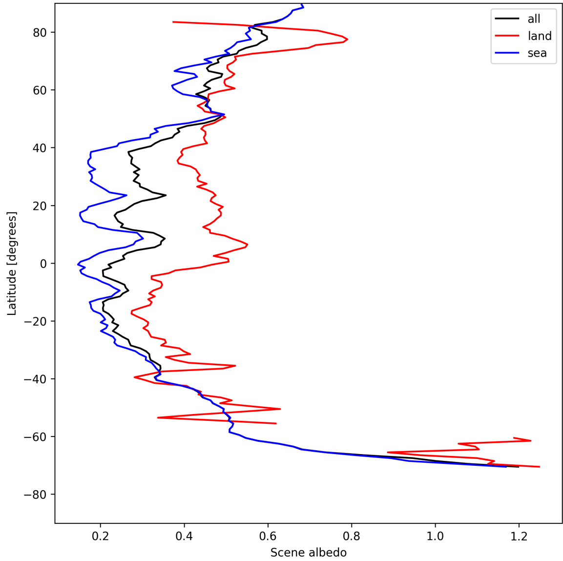
Figure 15: Zonal average of “Scene albedo” for 2025-08-03 to 2025-08-04.
