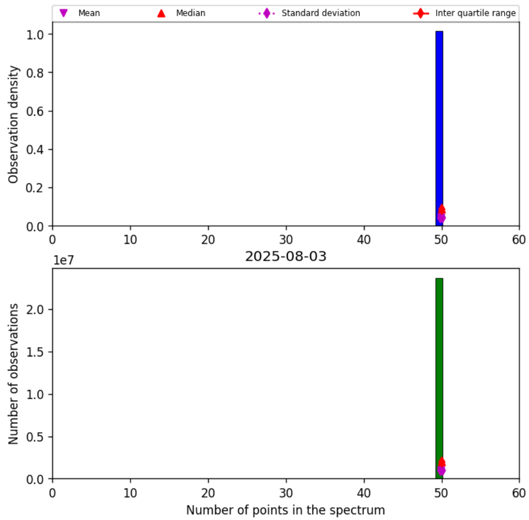
Figure 42: Histogram of “Number of points in the spectrum” for 2025-08-03 to 2025-08-04
