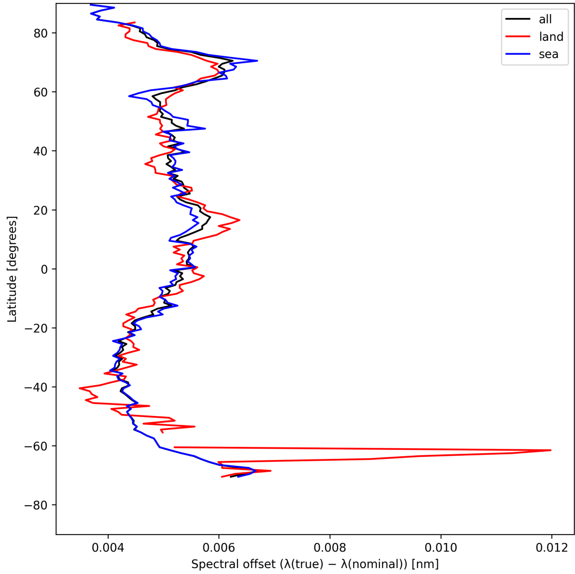
Figure 26: Zonal average of “Spectral offset ( \lambda_{\text{true}} - \lambda_{\text{nominal}} )” for 2025-08-03 to 2025-08-04.
