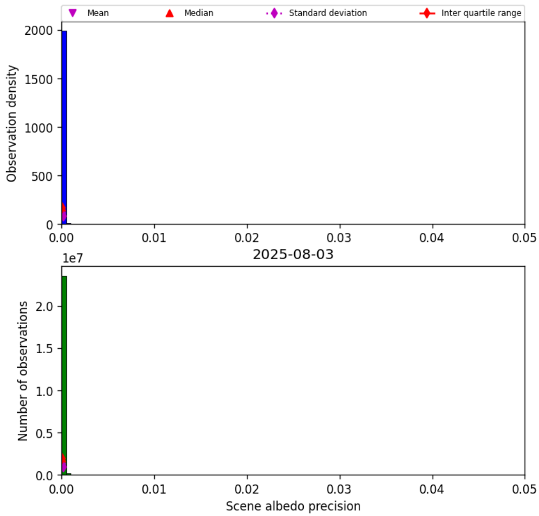
Figure 33: Histogram of “Scene albedo precision” for 2025-08-03 to 2025-08-04
