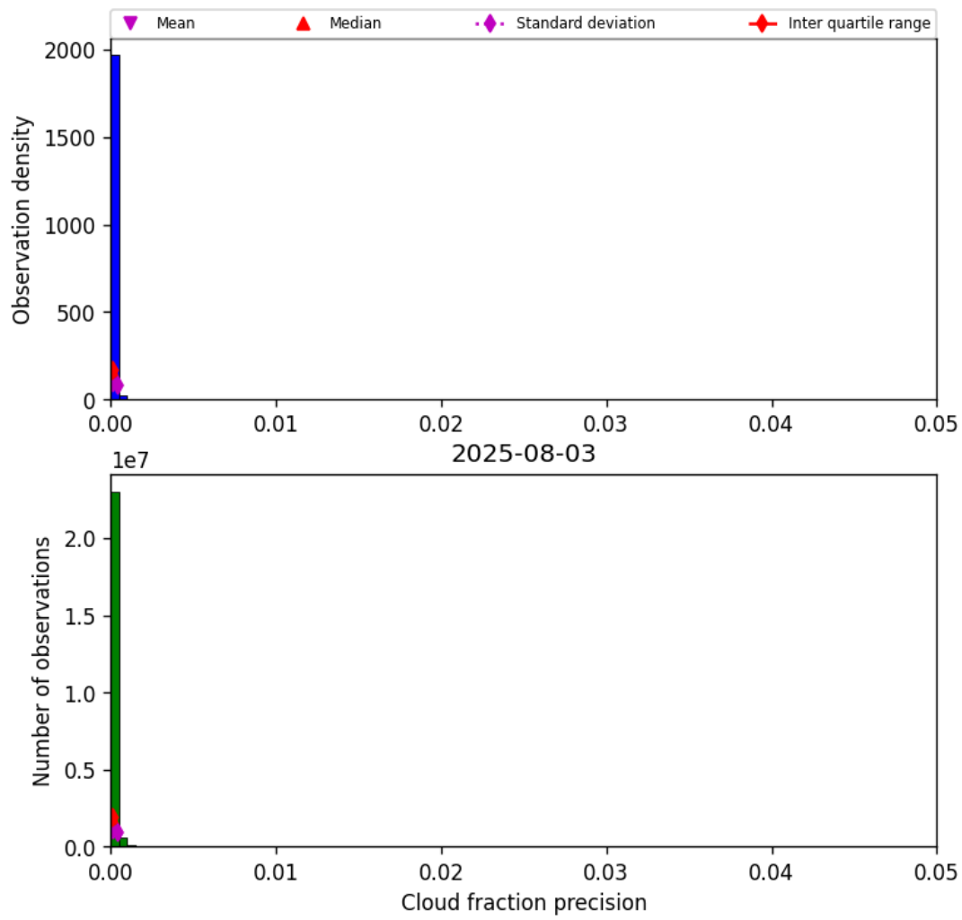
Figure 31: Histogram of “Cloud fraction precision” for 2025-08-03 to 2025-08-04
