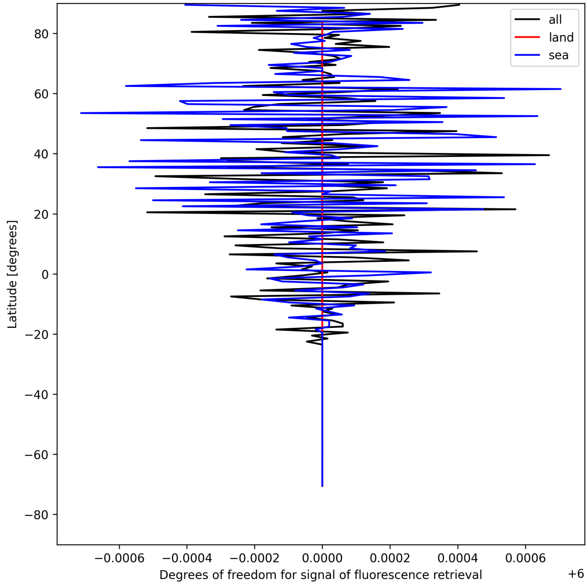
Figure 24: Zonal average of “Degrees of freedom for signal of fluorescence retrieval” for 2025-08-03 to 2025-08-04.
