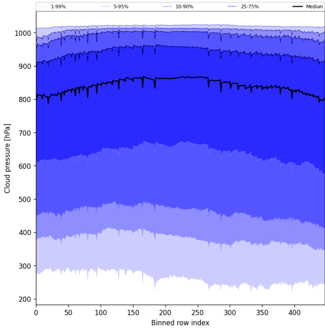
Figure 45: Along track statistics of “Cloud pressure” for 2025-08-03 to 2025-08-04
