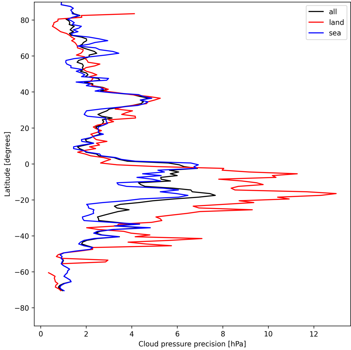
Figure 12: Zonal average of "Cloud pressure precision" for 2025-08-03 to 2025-08-04.
