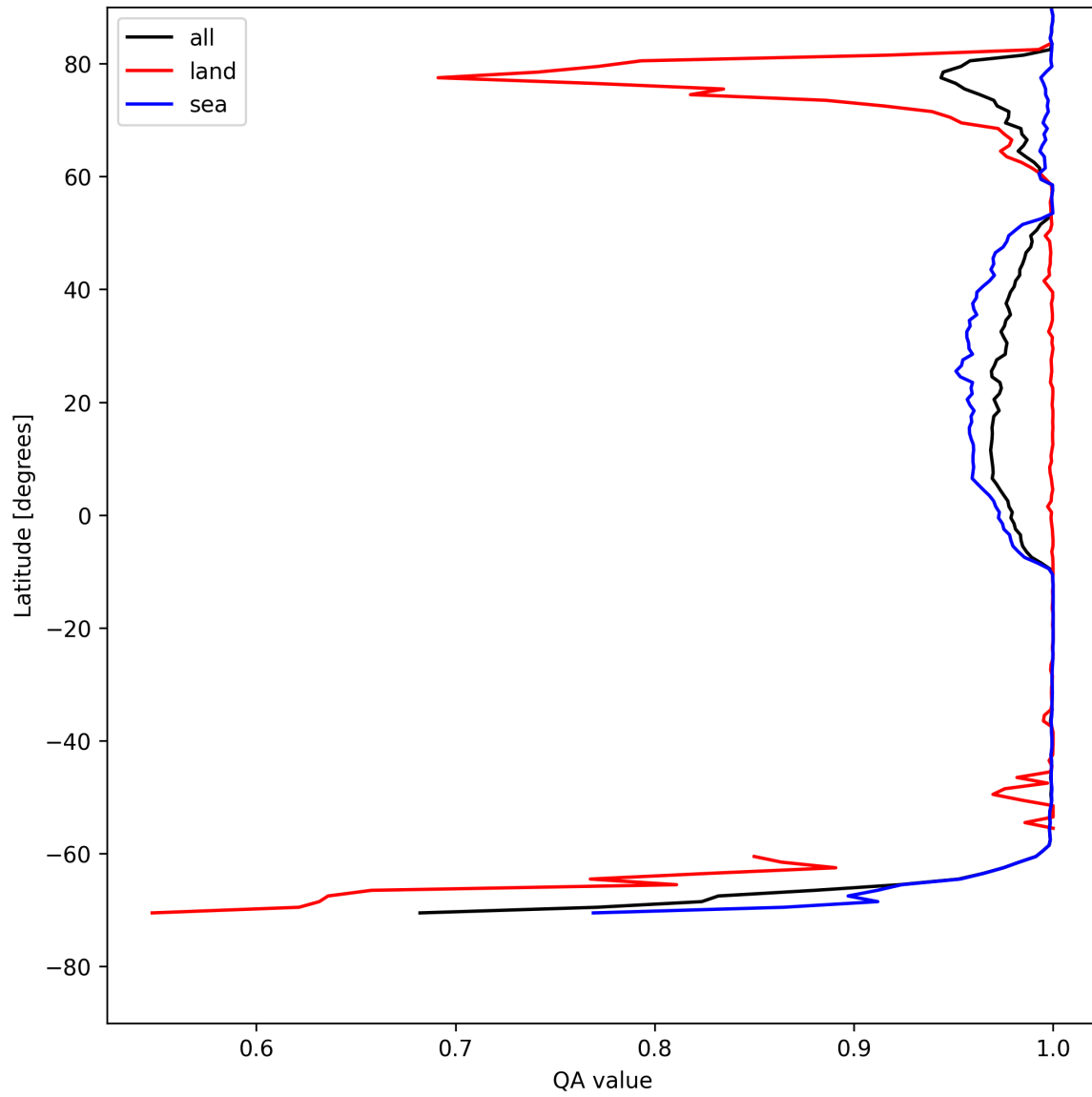
Figure 10: Zonal average of “QA value” for 2025-08-03 to 2025-08-04.
