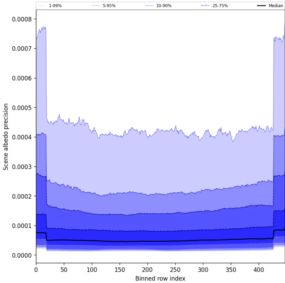
Figure 50: Along track statistics of “Scene albedo precision” for 2025-08-03 to 2025-08-04
