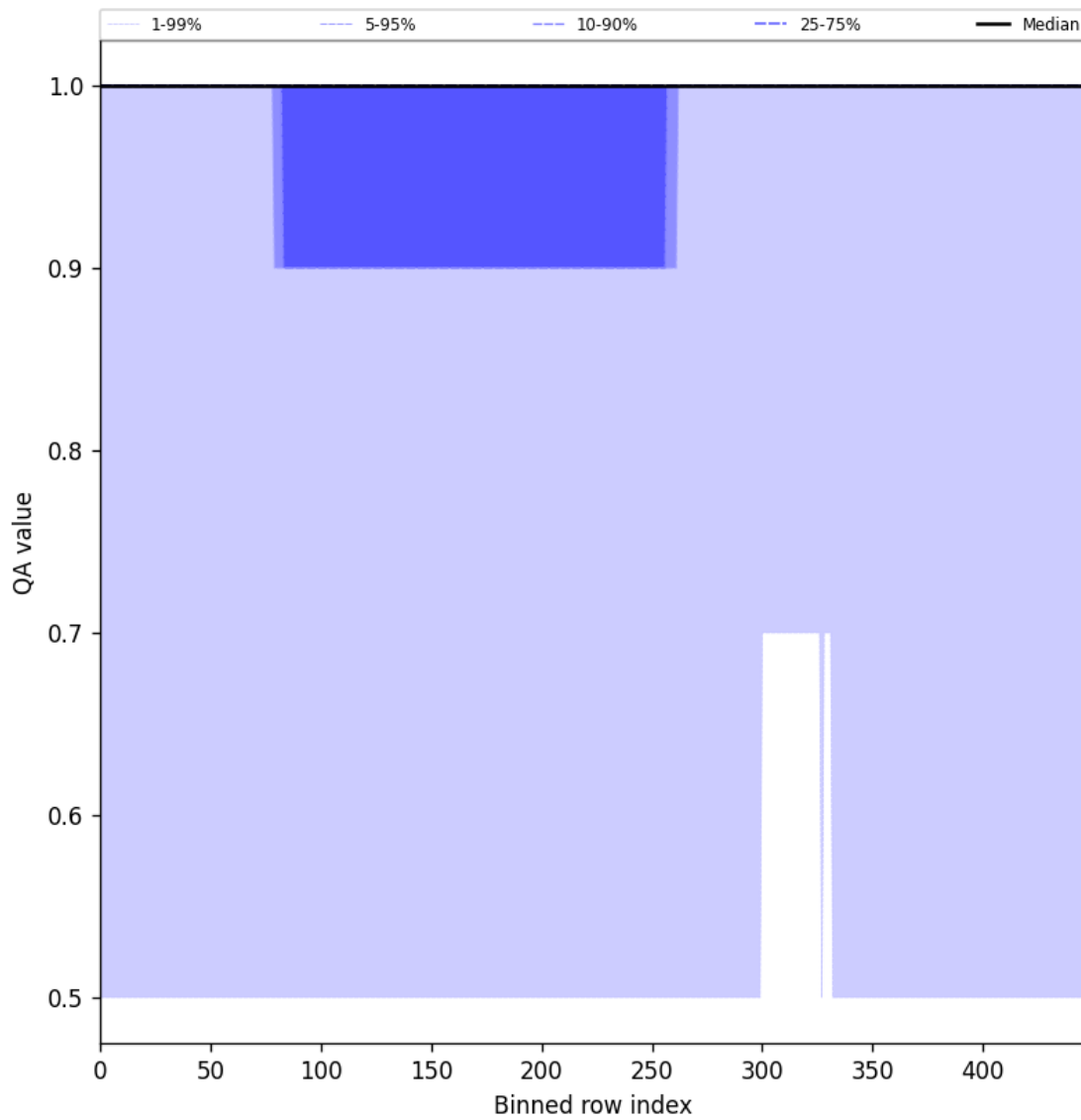
Figure 44: Along track statistics of “QA value” for 2025-08-03 to 2025-08-04
