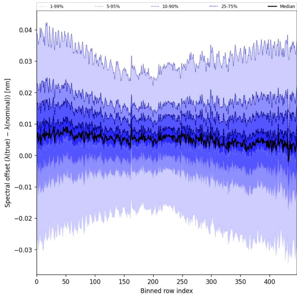
Figure 60: Along track statistics of “Spectral offset ( \lambda_{\text{true}} - \lambda_{\text{nominal}} )” for 2025-08-03 to 2025-08-04
