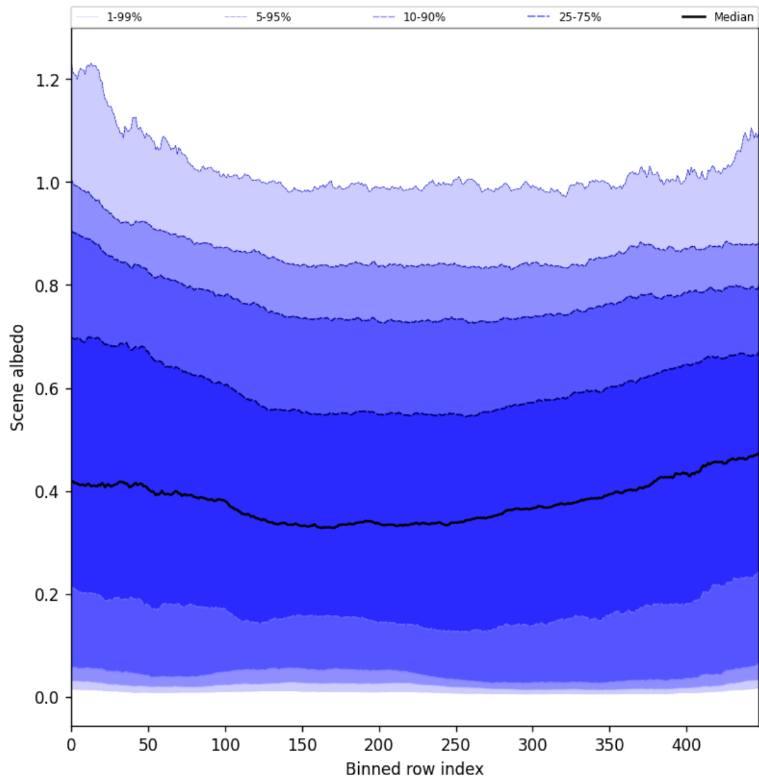
Figure 49: Along track statistics of “Scene albedo” for 2025-08-03 to 2025-08-04
