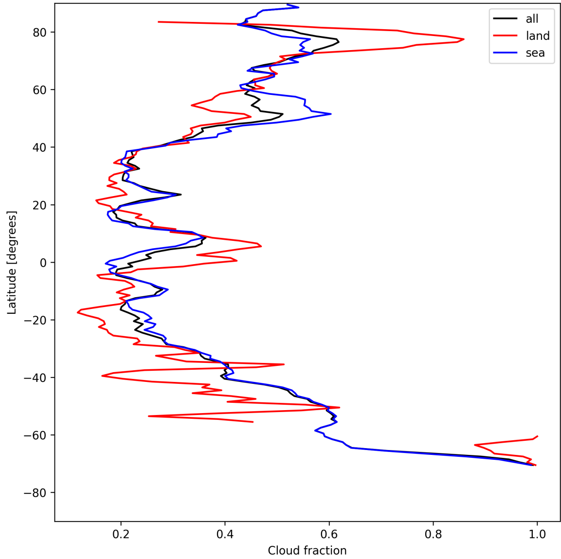
Figure 13: Zonal average of “Cloud fraction” for 2025-08-03 to 2025-08-04.
