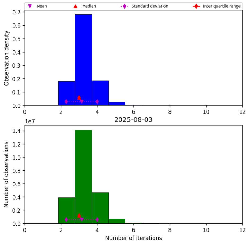
Figure 37: Histogram of “Number of iterations” for 2025-08-03 to 2025-08-04
