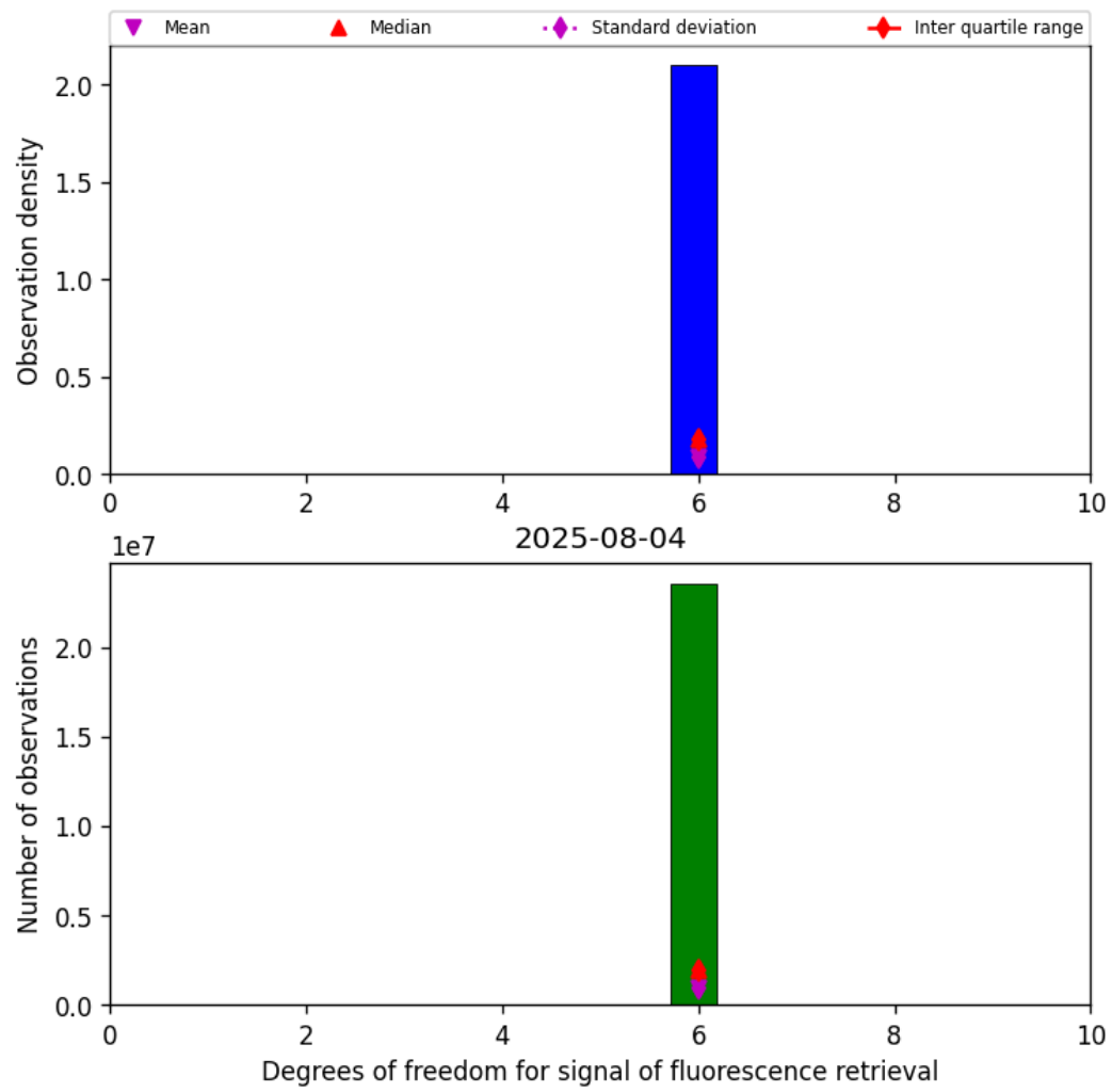
Figure 41: Histogram of “Degrees of freedom for signal of fluorescence retrieval” for 2025-08-04 to 2025-08-05
