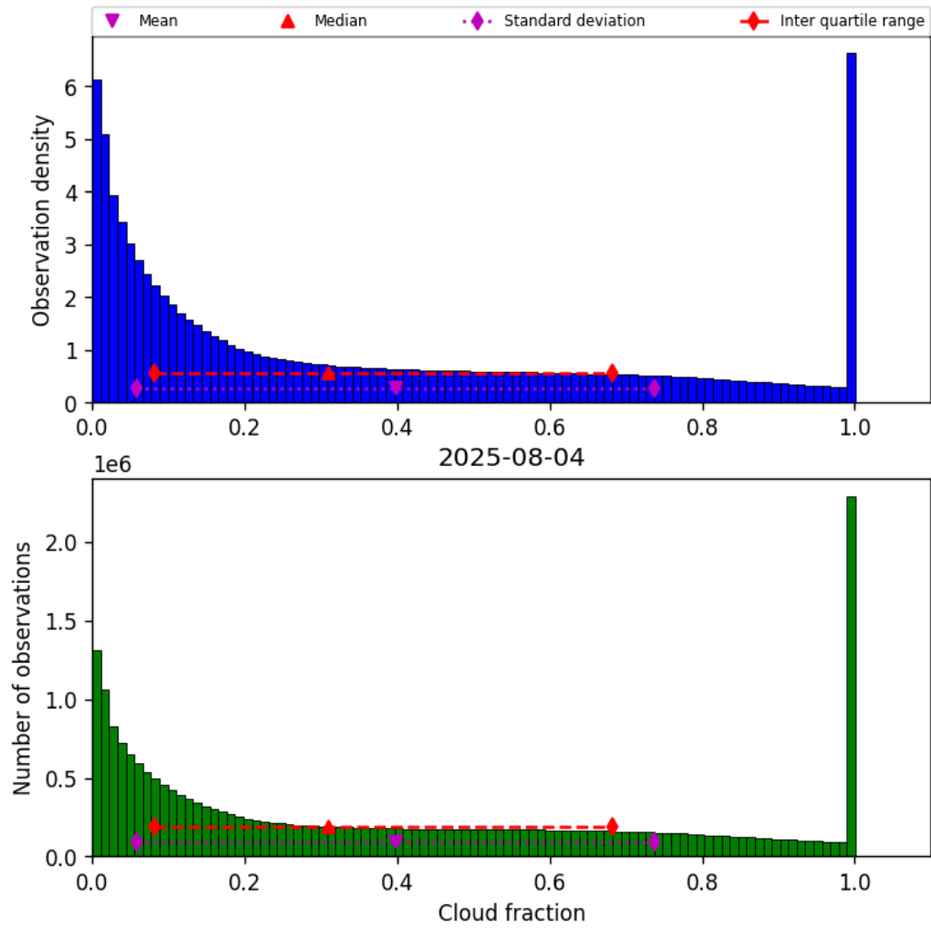
Figure 30: Histogram of “Cloud fraction” for 2025-08-04 to 2025-08-05
