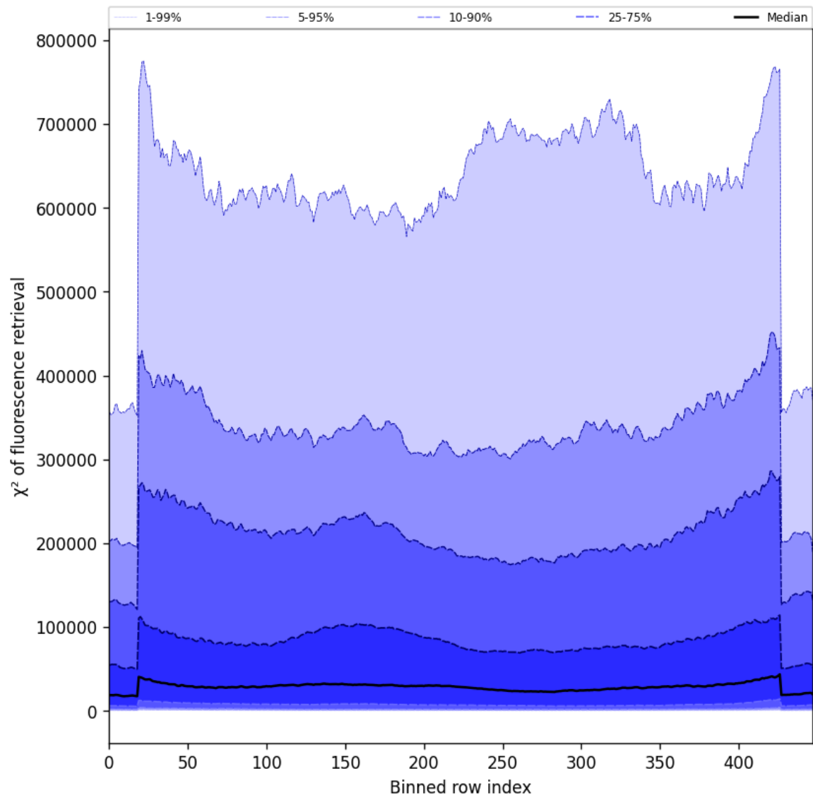
Figure 57: Along track statistics of “ \chi^2 of fluorescence retrieval” for 2025-08-04 to 2025-08-05
