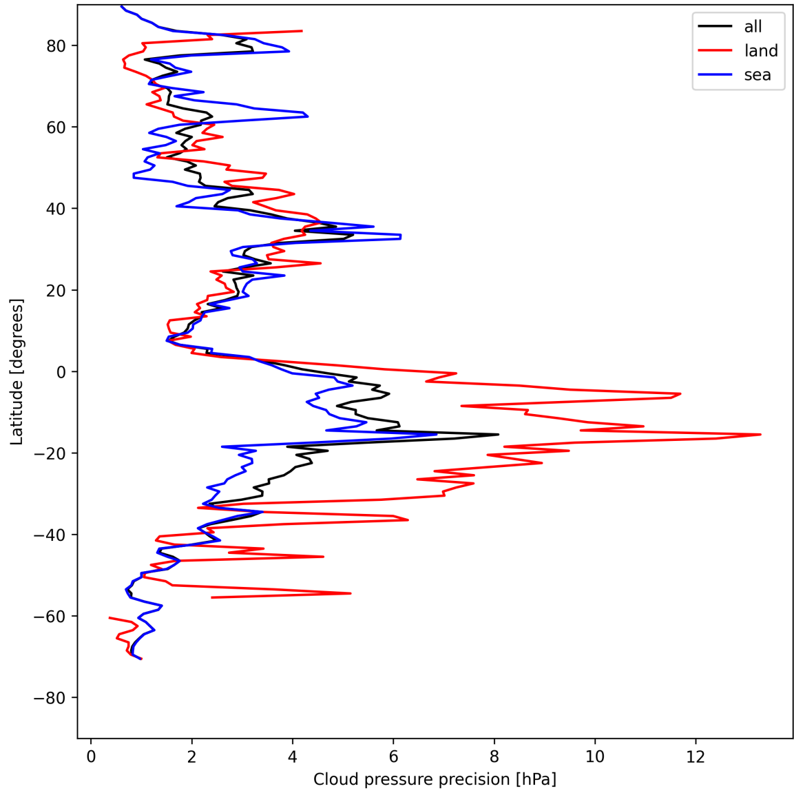
Figure 12: Zonal average of "Cloud pressure precision" for 2025-08-04 to 2025-08-05.
