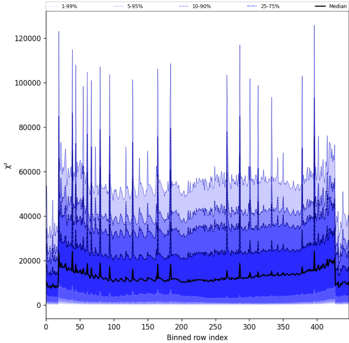
Figure 53: Along track statistics of “ \chi^2 ” for 2025-08-04 to 2025-08-05
