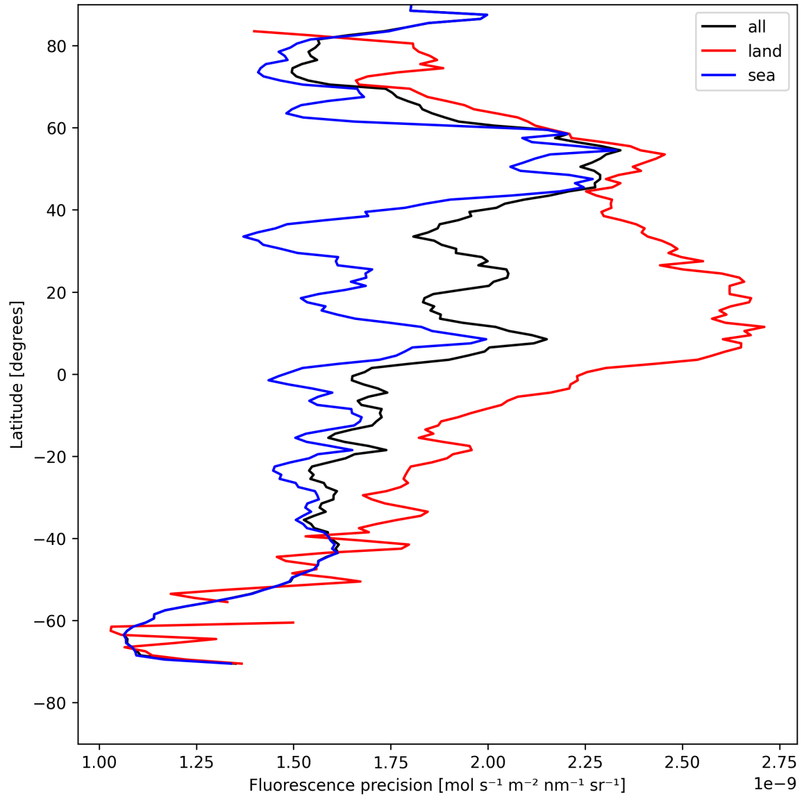
Figure 22: Zonal average of “Fluorescence precision” for 2025-08-04 to 2025-08-05.
