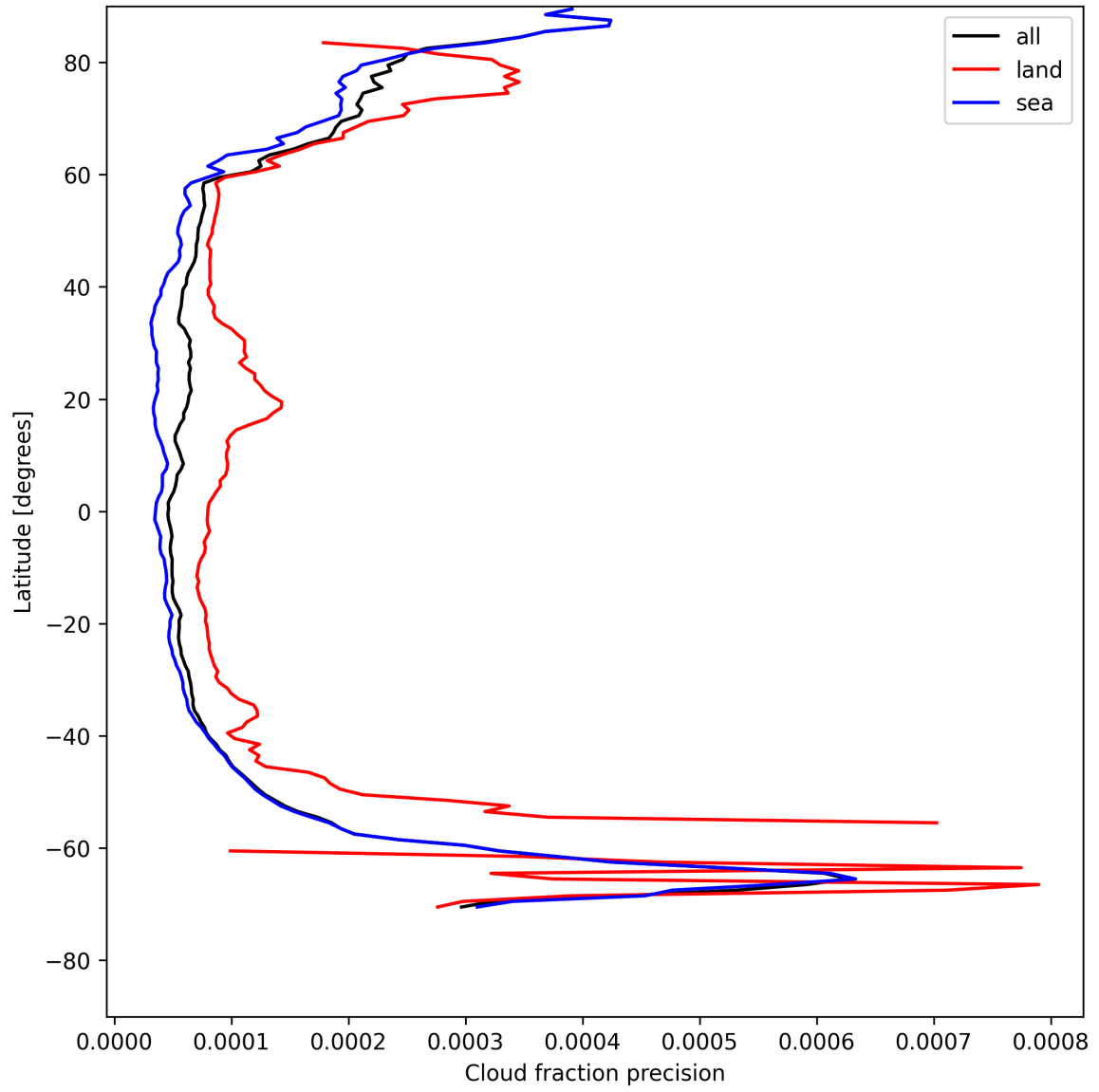
Figure 14: Zonal average of “Cloud fraction precision” for 2025-08-04 to 2025-08-05.
