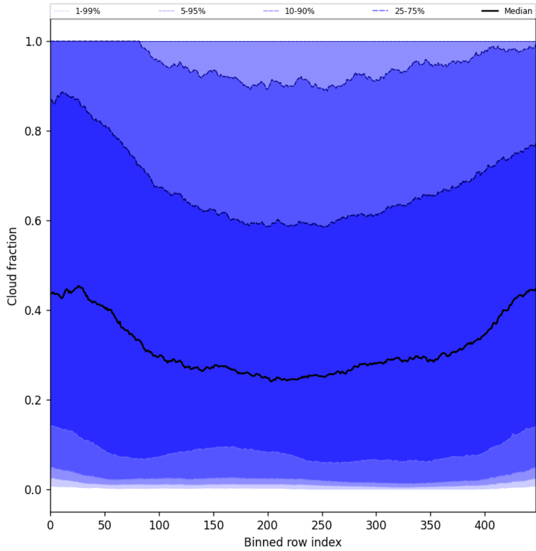
Figure 47: Along track statistics of “Cloud fraction” for 2025-08-04 to 2025-08-05
