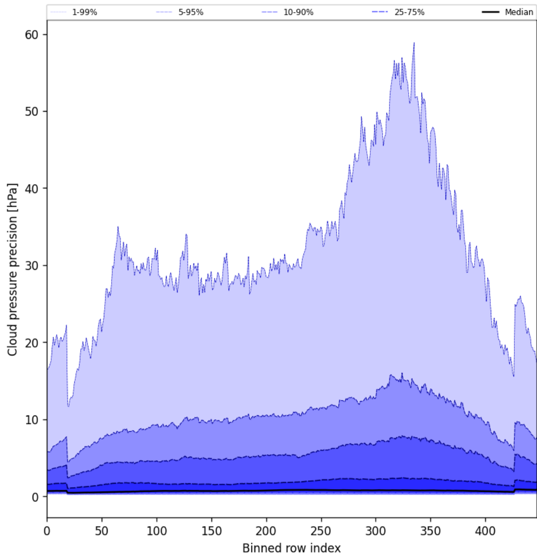
Figure 46: Along track statistics of “Cloud pressure precision” for 2025-08-04 to 2025-08-05
