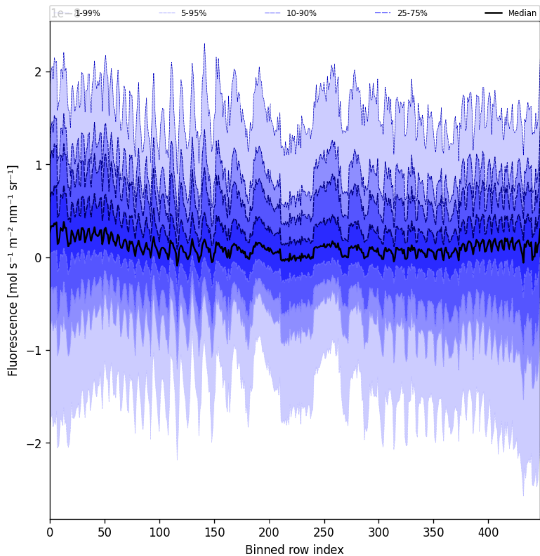
Figure 55: Along track statistics of “Fluorescence” for 2025-08-04 to 2025-08-05
