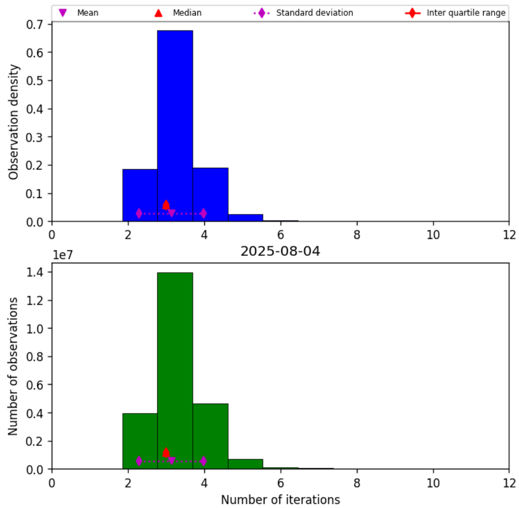
Figure 37: Histogram of “Number of iterations” for 2025-08-04 to 2025-08-05
