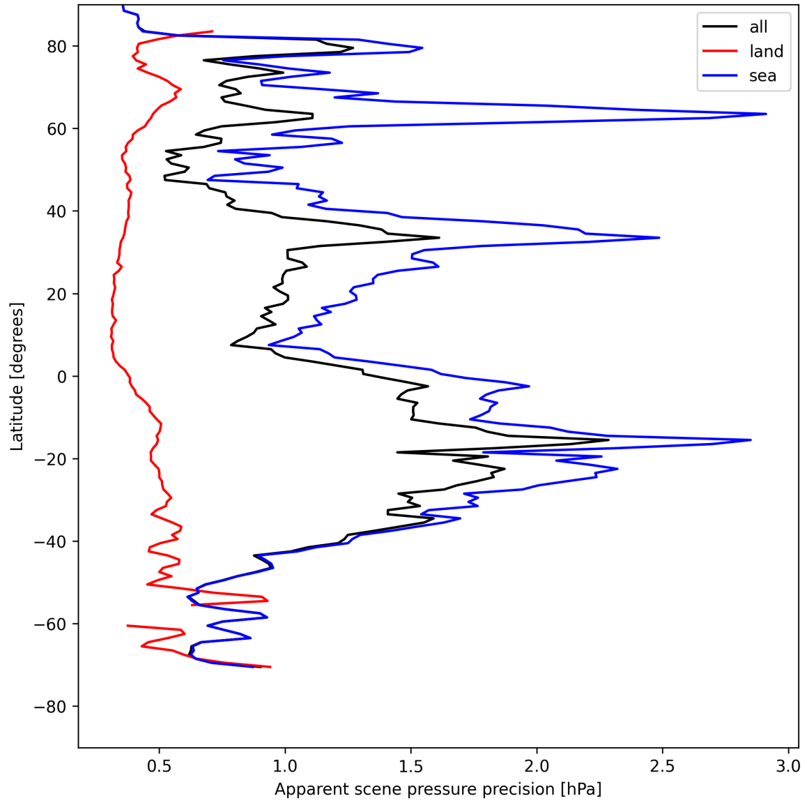
Figure 18: Zonal average of “Apparent scene pressure precision” for 2025-08-04 to 2025-08-05.
