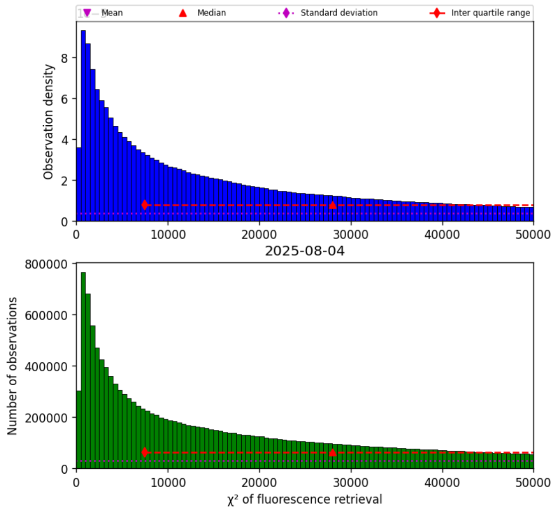
Figure 40: Histogram of “ \chi^2 of fluorescence retrieval” for 2025-08-04 to 2025-08-05
