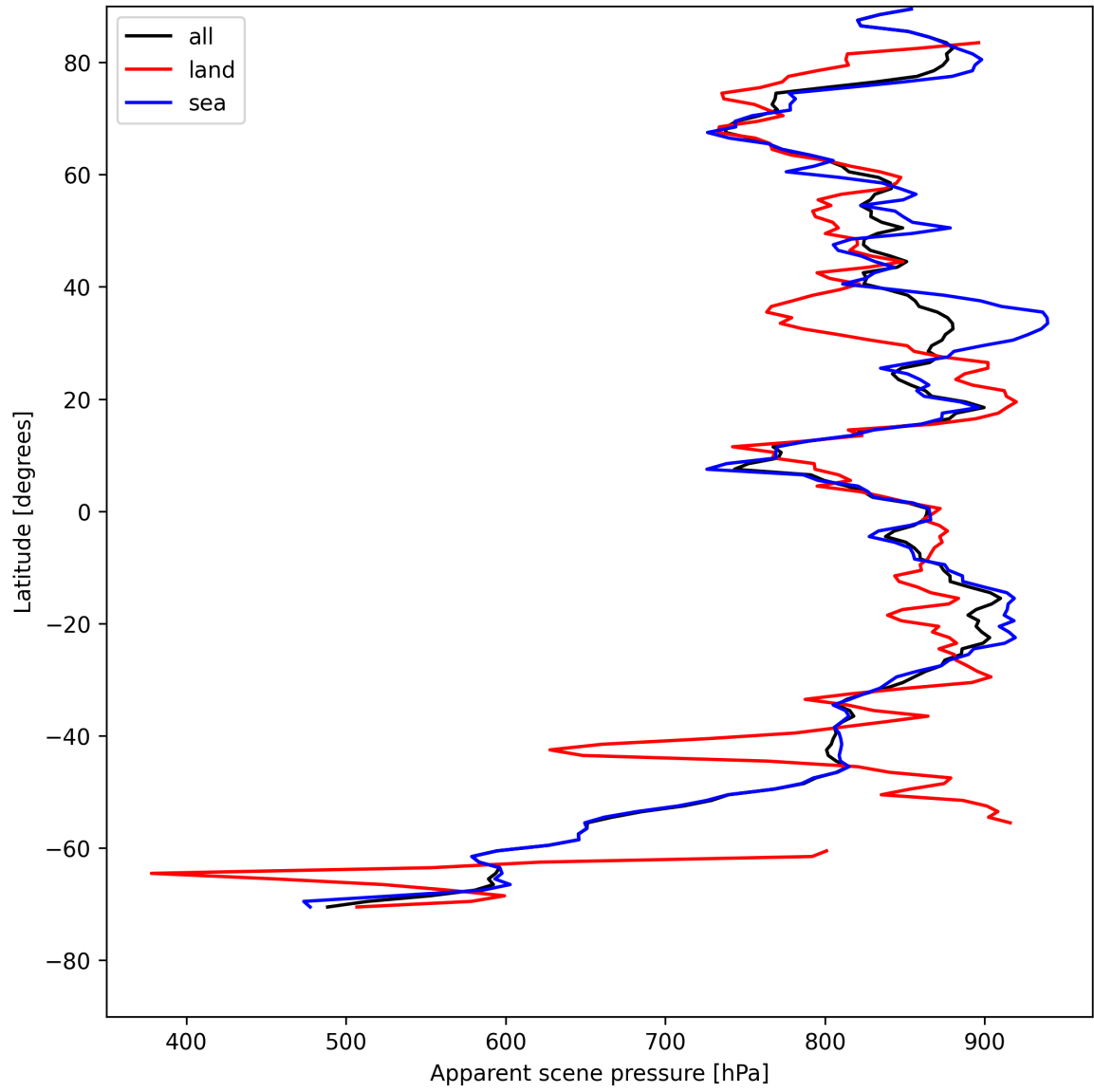
Figure 17: Zonal average of “Apparent scene pressure” for 2025-08-04 to 2025-08-05.
