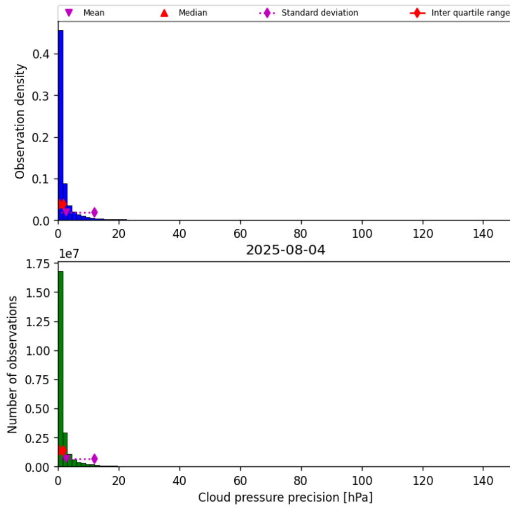
Figure 29: Histogram of “Cloud pressure precision” for 2025-08-04 to 2025-08-05
