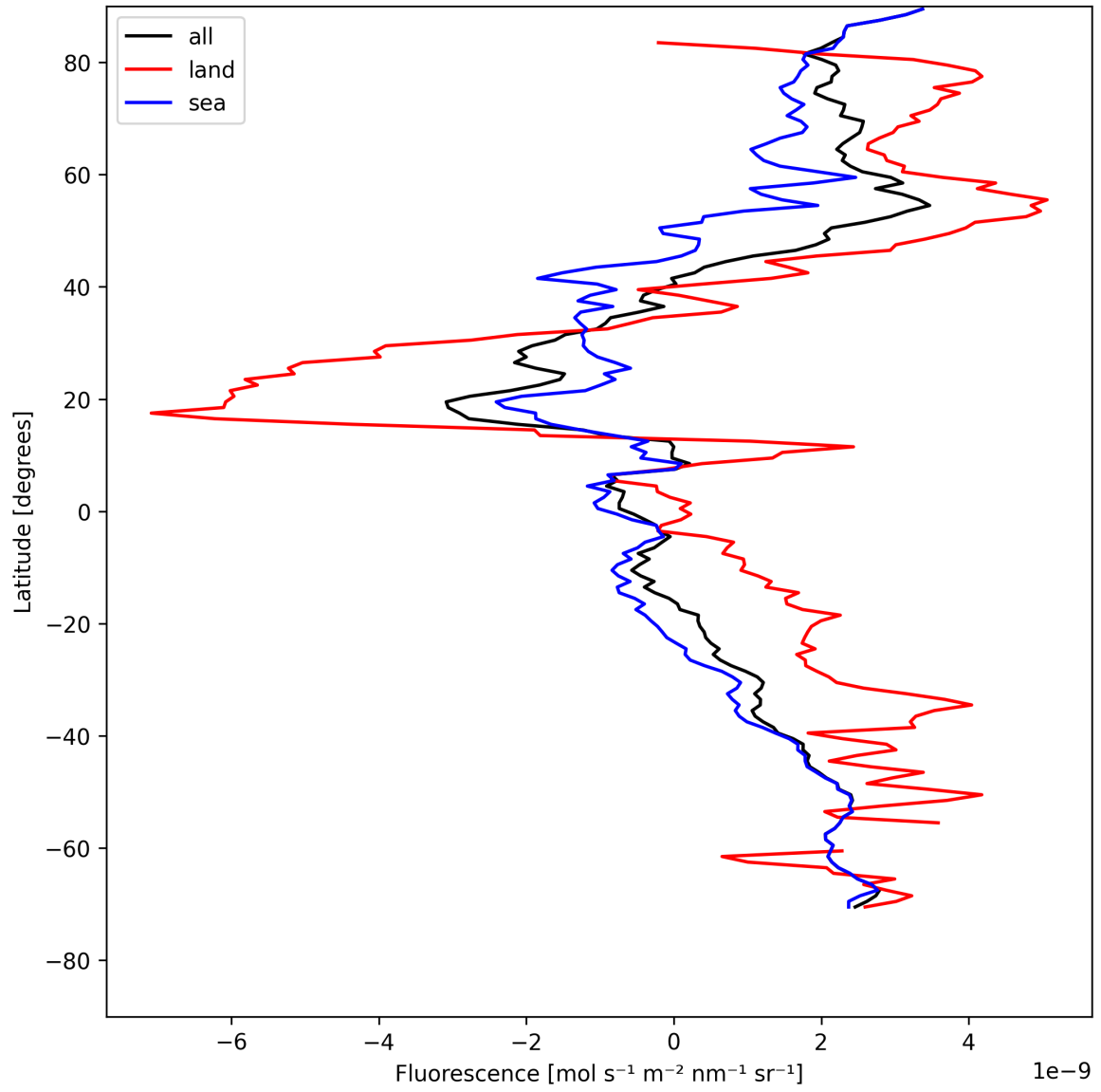
Figure 21: Zonal average of “Fluorescence” for 2025-08-04 to 2025-08-05.
