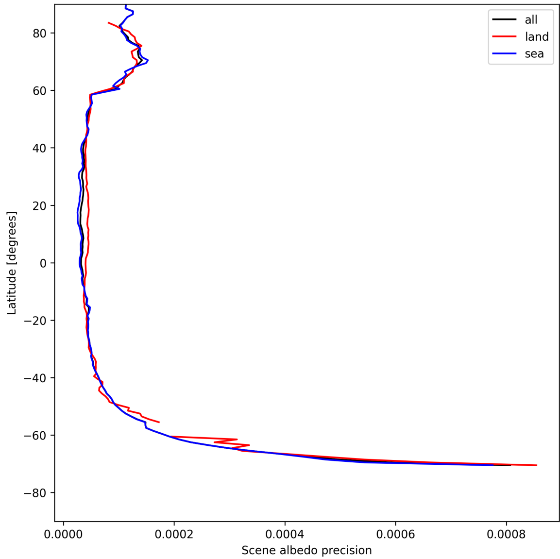
Figure 16: Zonal average of “Scene albedo precision” for 2025-08-04 to 2025-08-05.
