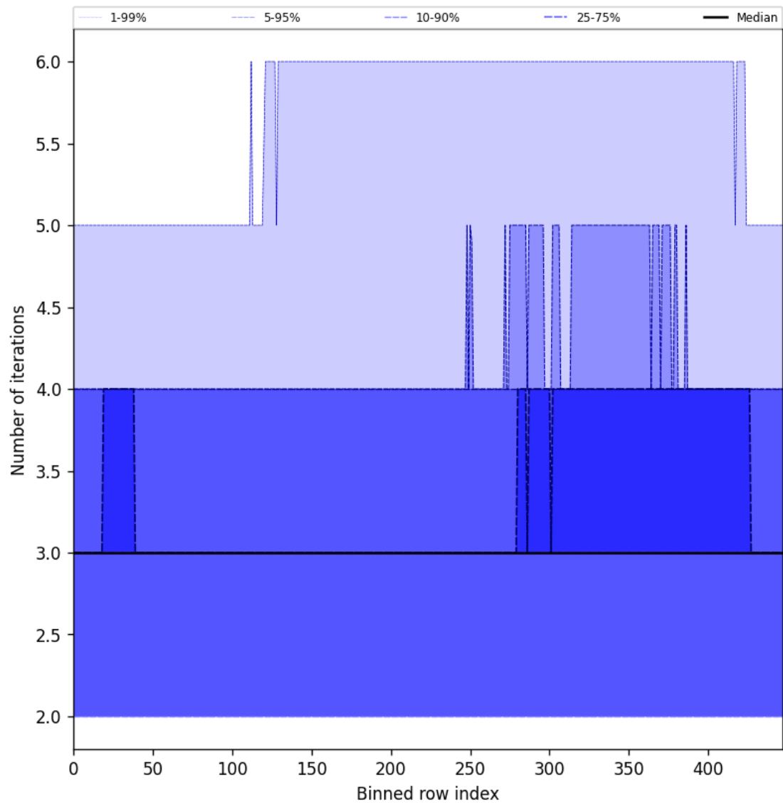
Figure 54: Along track statistics of “Number of iterations” for 2025-08-04 to 2025-08-05
