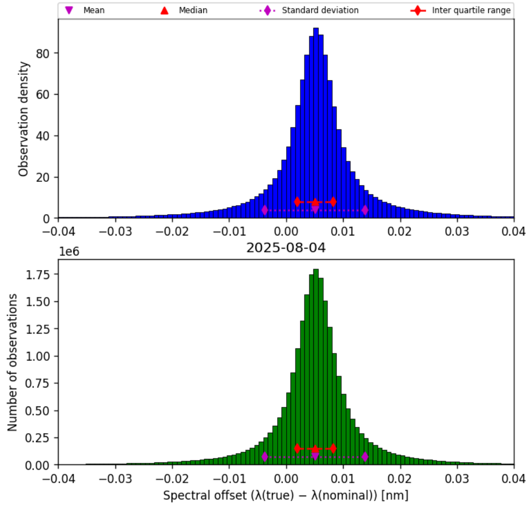
Figure 43: Histogram of “Spectral offset ( \lambda_{\text{true}} - \lambda_{\text{nominal}} )” for 2025-08-04 to 2025-08-05
