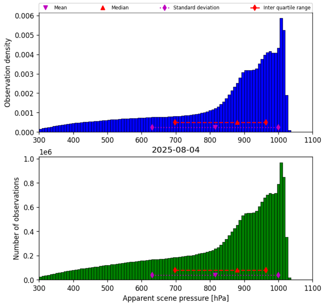
Figure 34: Histogram of “Apparent scene pressure” for 2025-08-04 to 2025-08-05
