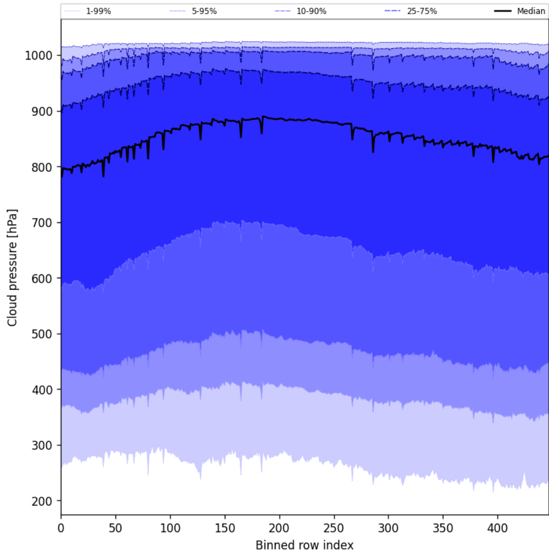
Figure 45: Along track statistics of “Cloud pressure” for 2025-08-04 to 2025-08-05
