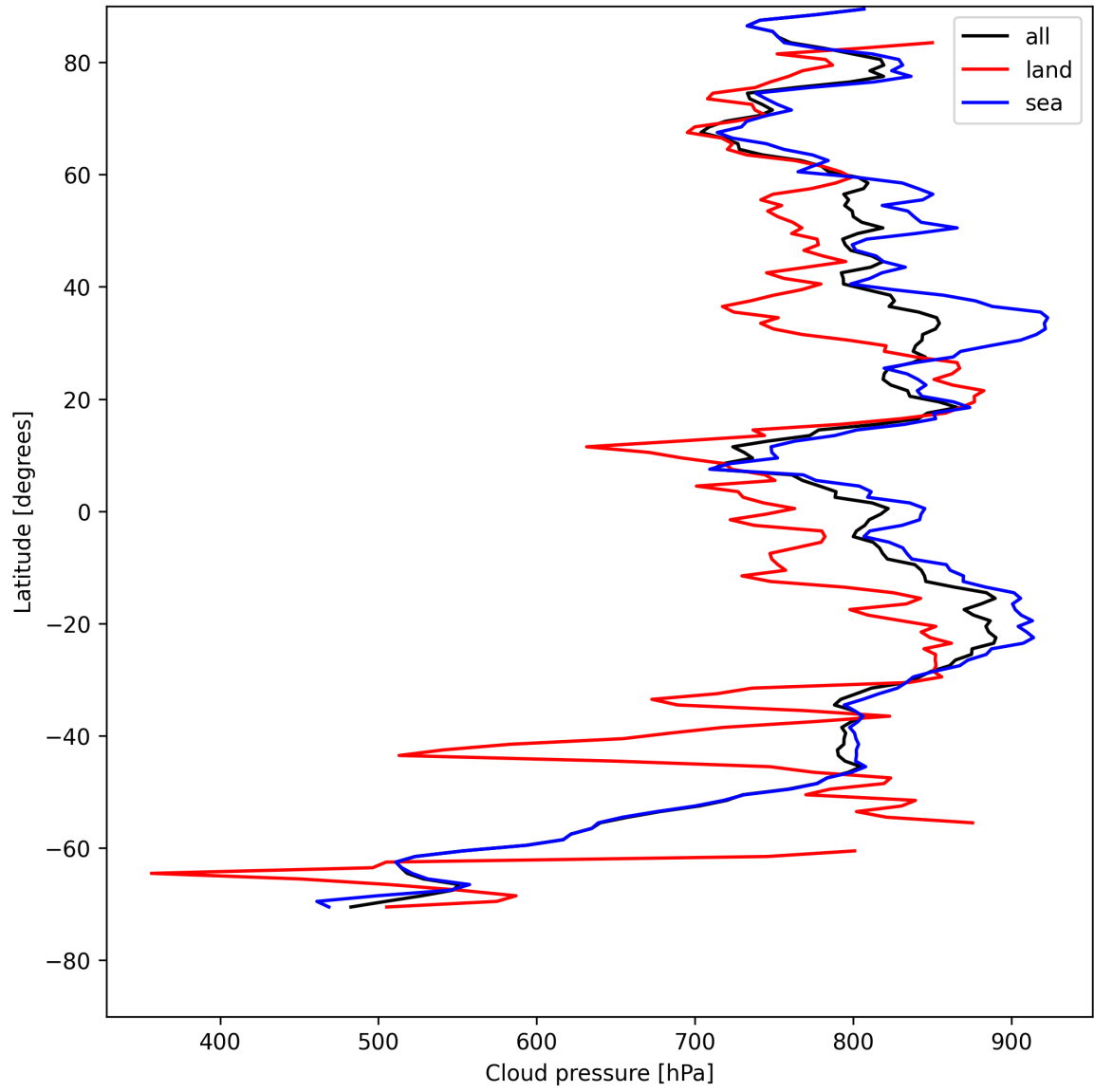
Figure 11: Zonal average of “Cloud pressure” for 2025-08-04 to 2025-08-05.
