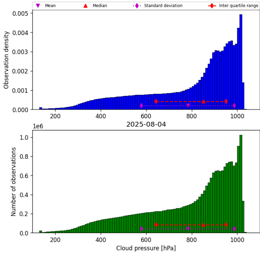
Figure 28: Histogram of “Cloud pressure” for 2025-08-04 to 2025-08-05
