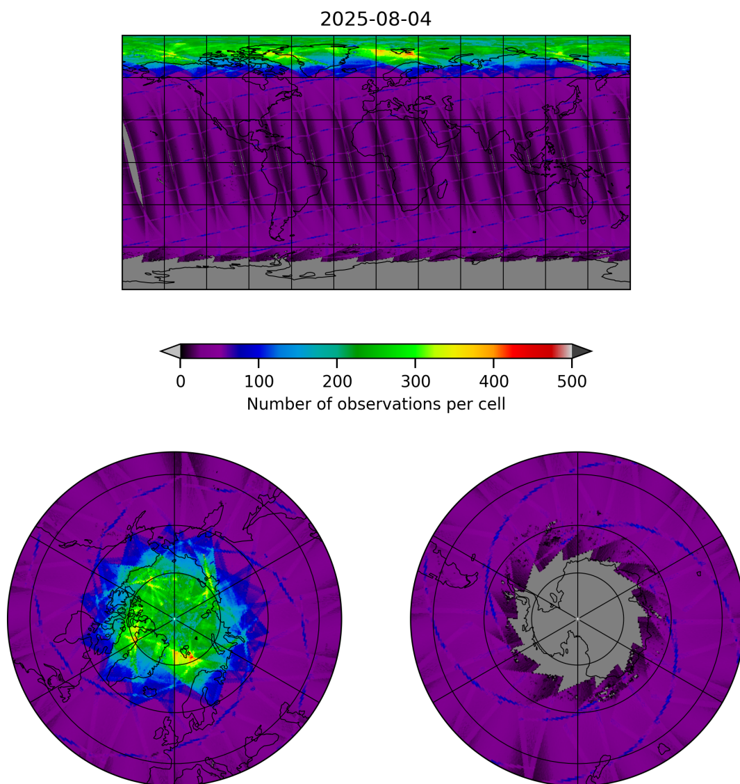
Figure 9: Map of the number of observations for 2025-08-04 to 2025-08-05
