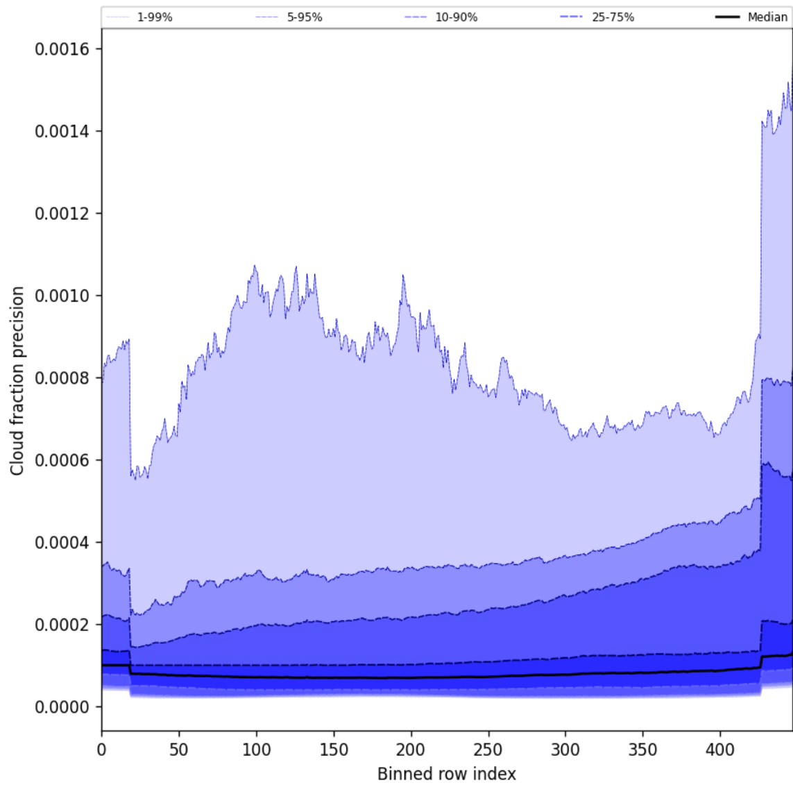
Figure 48: Along track statistics of “Cloud fraction precision” for 2025-08-04 to 2025-08-05
