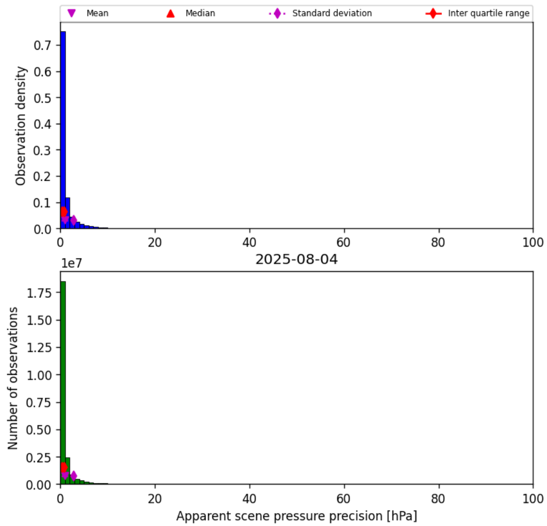
Figure 35: Histogram of “Apparent scene pressure precision” for 2025-08-04 to 2025-08-05
