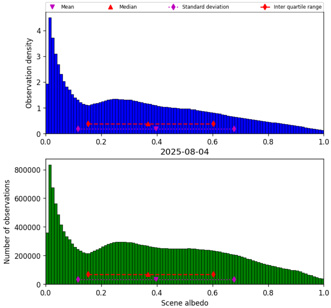
Figure 32: Histogram of “Scene albedo” for 2025-08-04 to 2025-08-05
