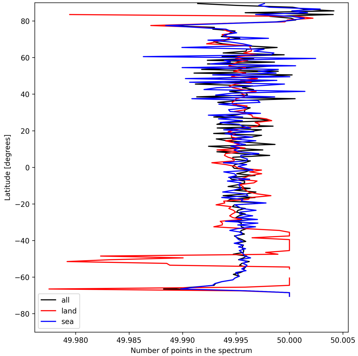
Figure 25: Zonal average of “Number of points in the spectrum” for 2025-08-04 to 2025-08-05.
