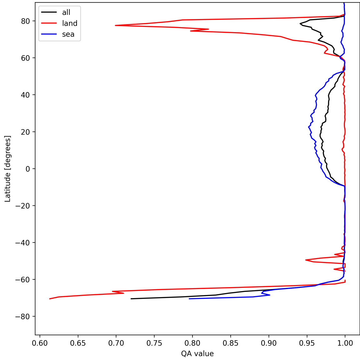
Figure 10: Zonal average of “QA value” for 2025-08-04 to 2025-08-05.
