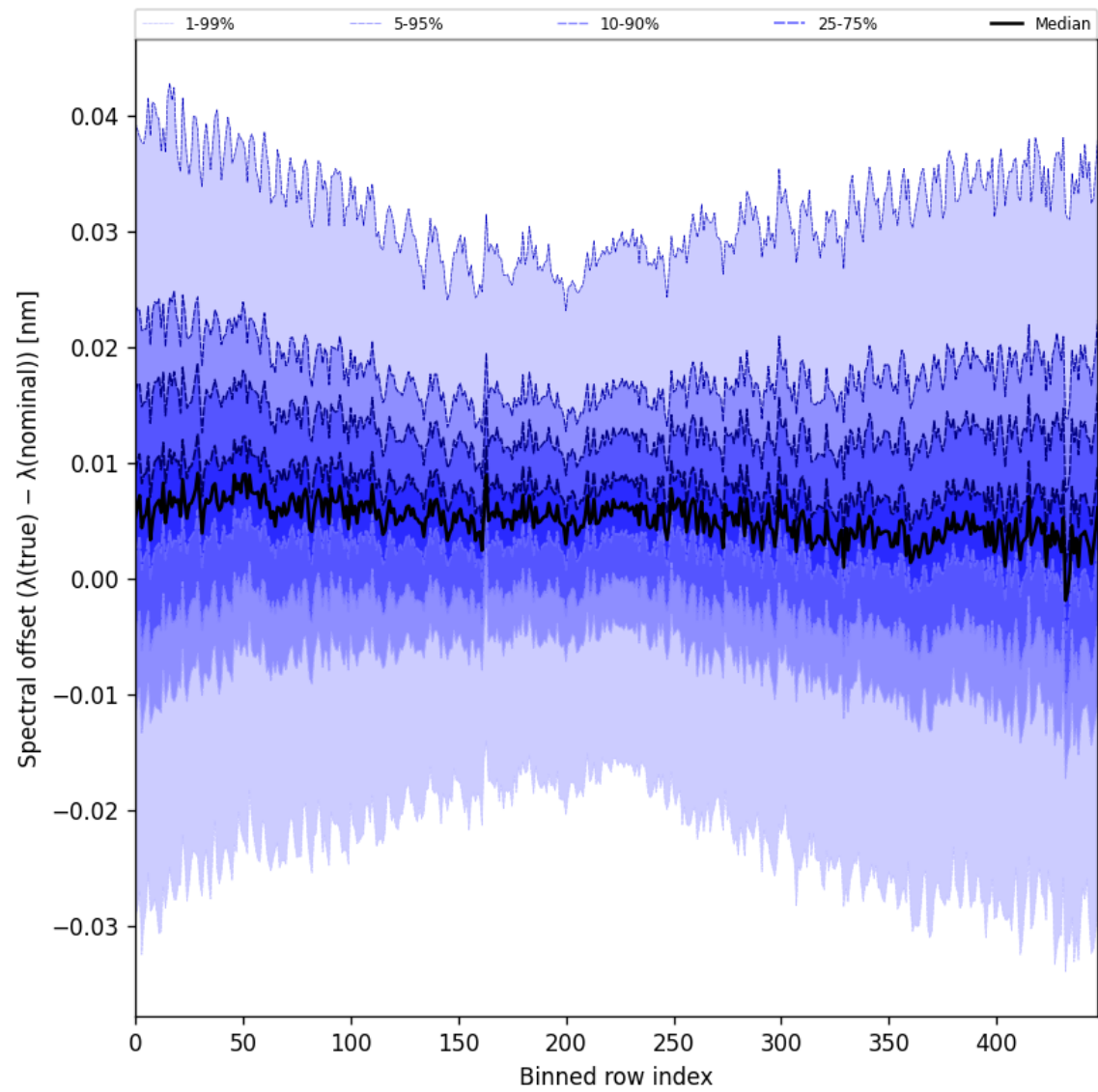
Figure 60: Along track statistics of “Spectral offset ( \lambda_{\text{true}} - \lambda_{\text{nominal}} )” for 2025-08-04 to 2025-08-05
