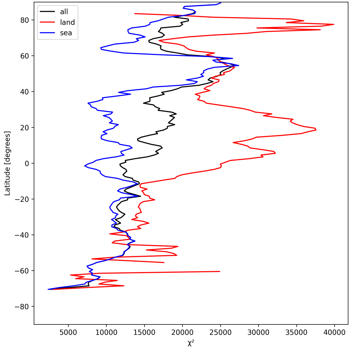
Figure 19: Zonal average of “ \chi^2 ” for 2025-08-04 to 2025-08-05.
