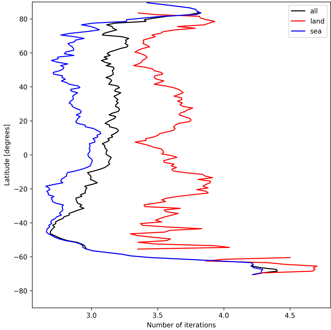
Figure 20: Zonal average of “Number of iterations” for 2025-08-04 to 2025-08-05.
