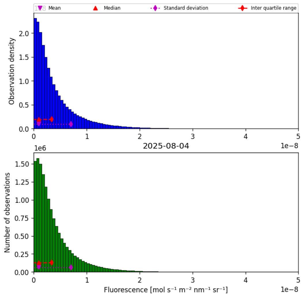
Figure 38: Histogram of “Fluorescence” for 2025-08-04 to 2025-08-05
