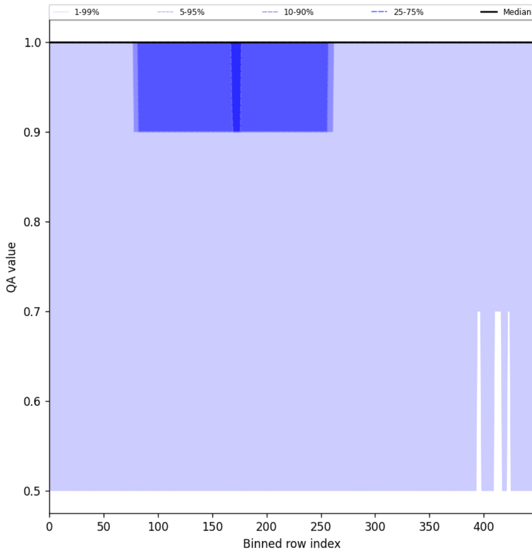
Figure 44: Along track statistics of “QA value” for 2025-08-04 to 2025-08-05
