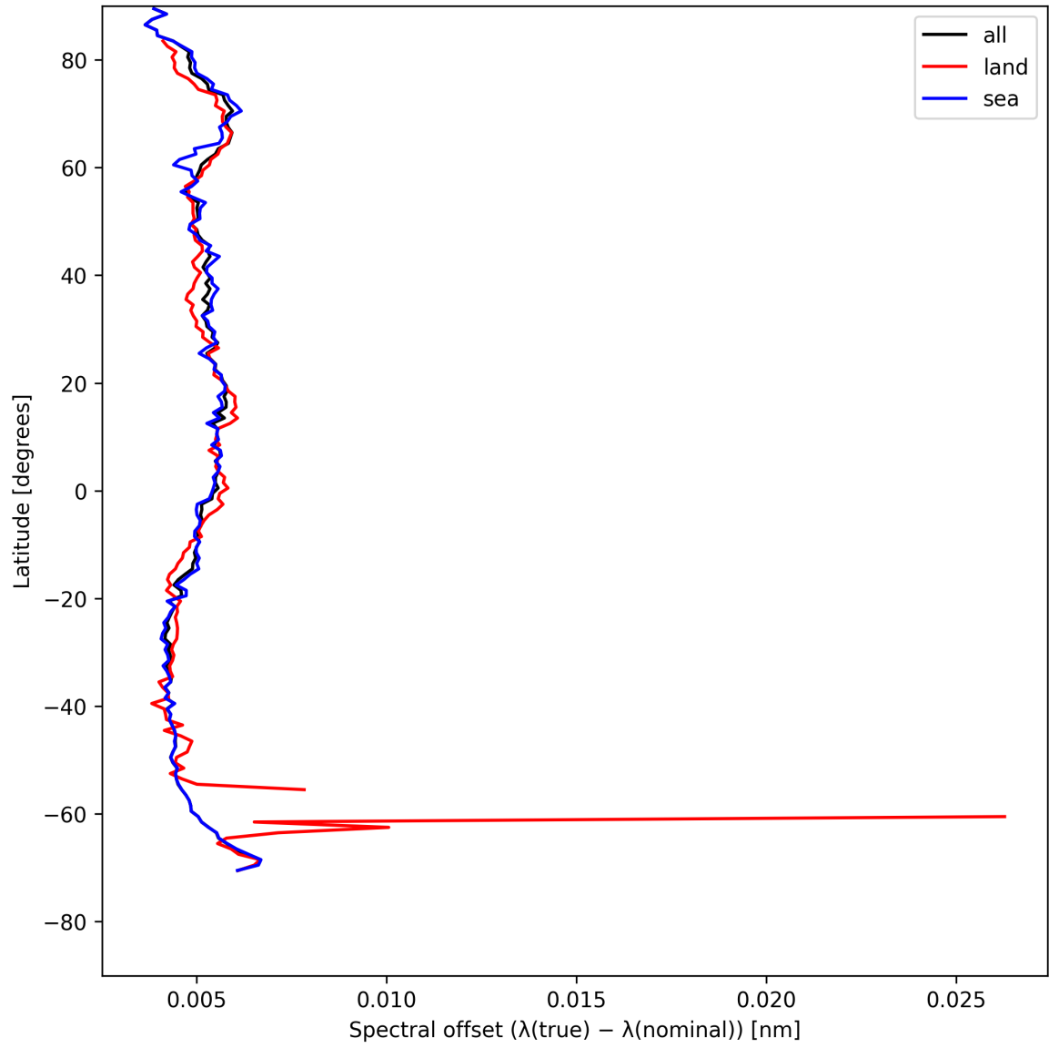
Figure 26: Zonal average of “Spectral offset ( \lambda_{\text{true}} - \lambda_{\text{nominal}} )” for 2025-08-04 to 2025-08-05.
