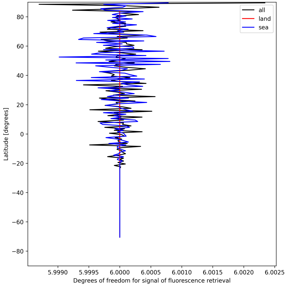
Figure 24: Zonal average of “Degrees of freedom for signal of fluorescence retrieval” for 2025-08-04 to 2025-08-05.
