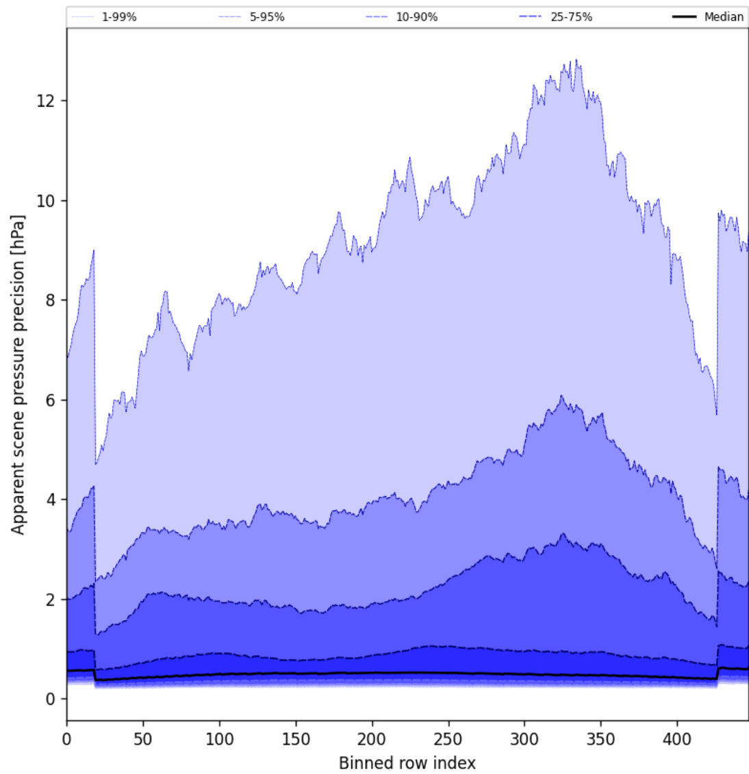
Figure 52: Along track statistics of “Apparent scene pressure precision” for 2025-08-04 to 2025-08-05
