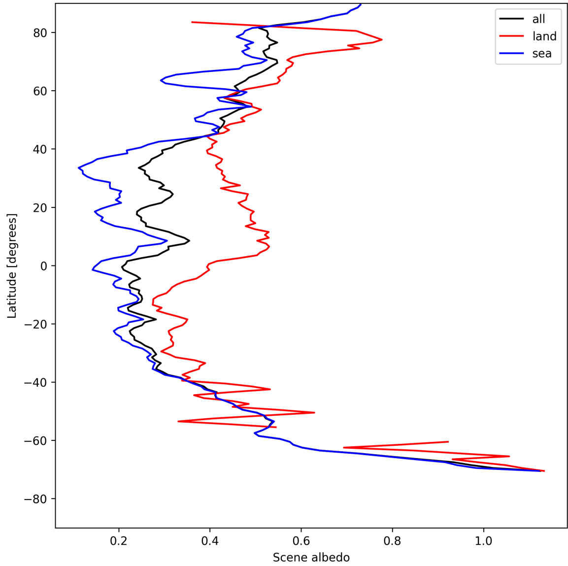
Figure 15: Zonal average of “Scene albedo” for 2025-08-04 to 2025-08-05.
