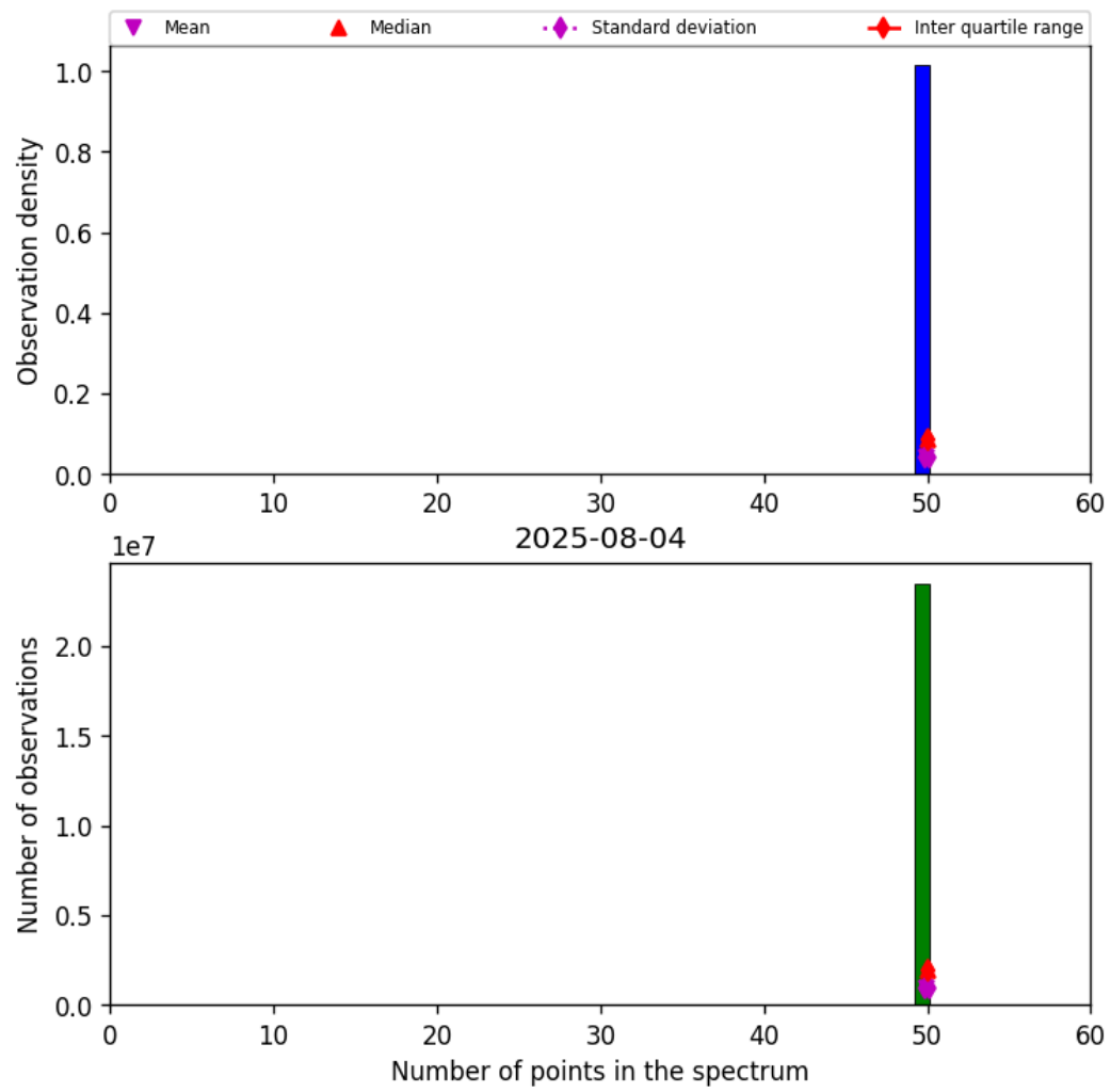
Figure 42: Histogram of “Number of points in the spectrum” for 2025-08-04 to 2025-08-05
