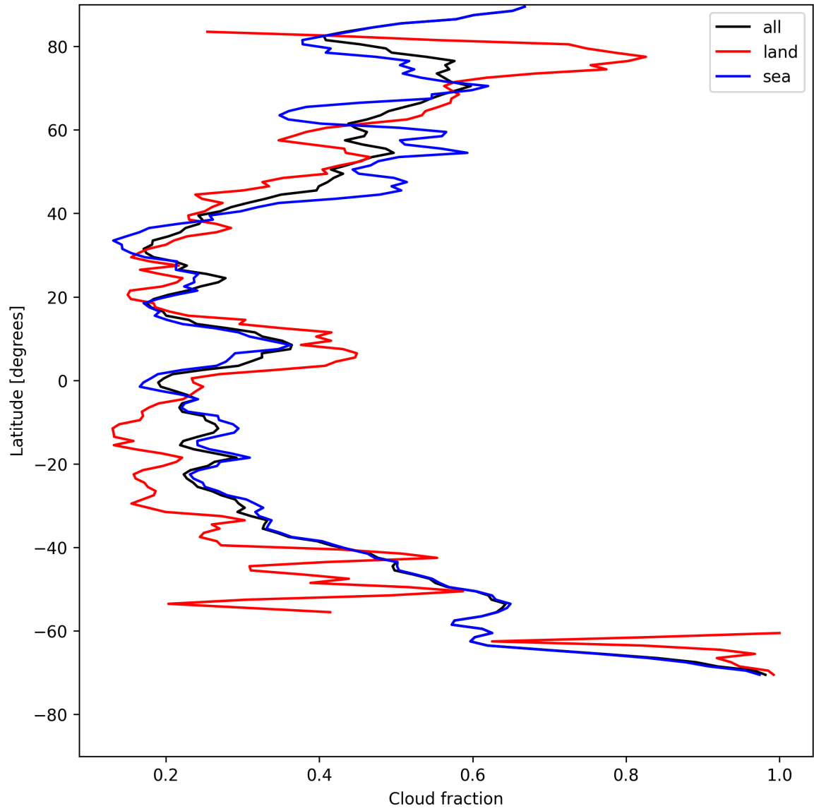
Figure 13: Zonal average of “Cloud fraction” for 2025-08-04 to 2025-08-05.
