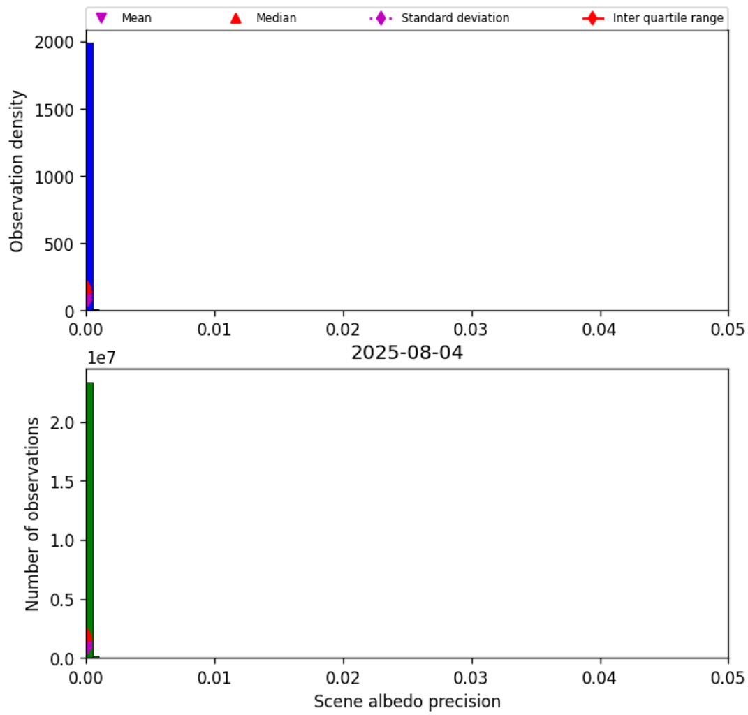
Figure 33: Histogram of “Scene albedo precision” for 2025-08-04 to 2025-08-05
