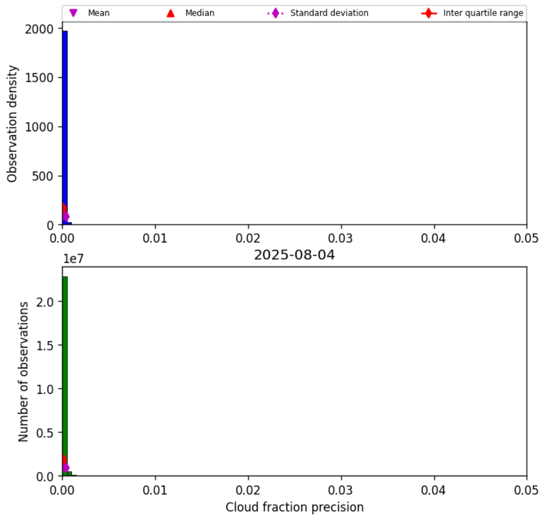
Figure 31: Histogram of “Cloud fraction precision” for 2025-08-04 to 2025-08-05
