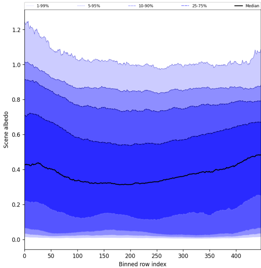
Figure 49: Along track statistics of “Scene albedo” for 2025-08-04 to 2025-08-05
