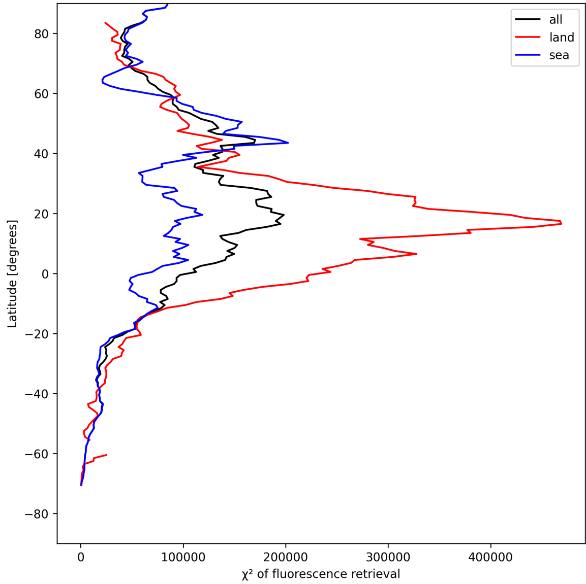
Figure 23: Zonal average of “ \chi^2 of fluorescence retrieval” for 2025-08-04 to 2025-08-05.
