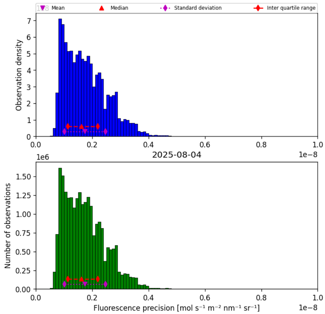
Figure 39: Histogram of “Fluorescence precision” for 2025-08-04 to 2025-08-05
