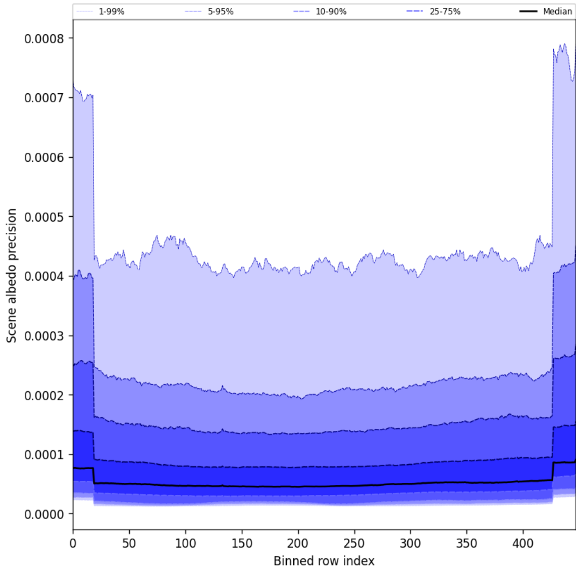
Figure 50: Along track statistics of “Scene albedo precision” for 2025-08-04 to 2025-08-05
