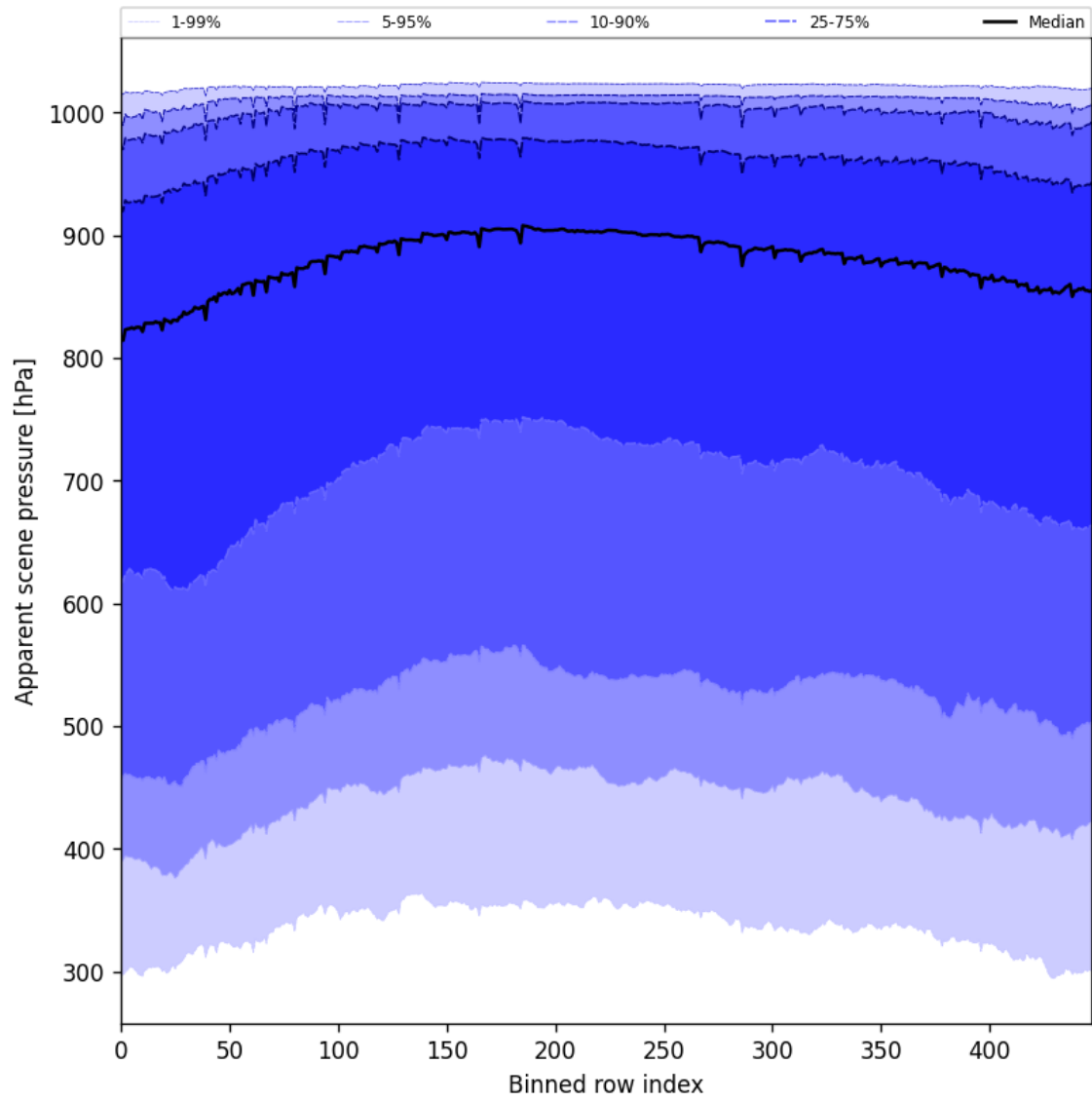
Figure 51: Along track statistics of “Apparent scene pressure” for 2025-08-04 to 2025-08-05
