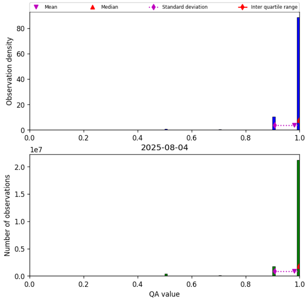
Figure 27: Histogram of “QA value” for 2025-08-04 to 2025-08-05
