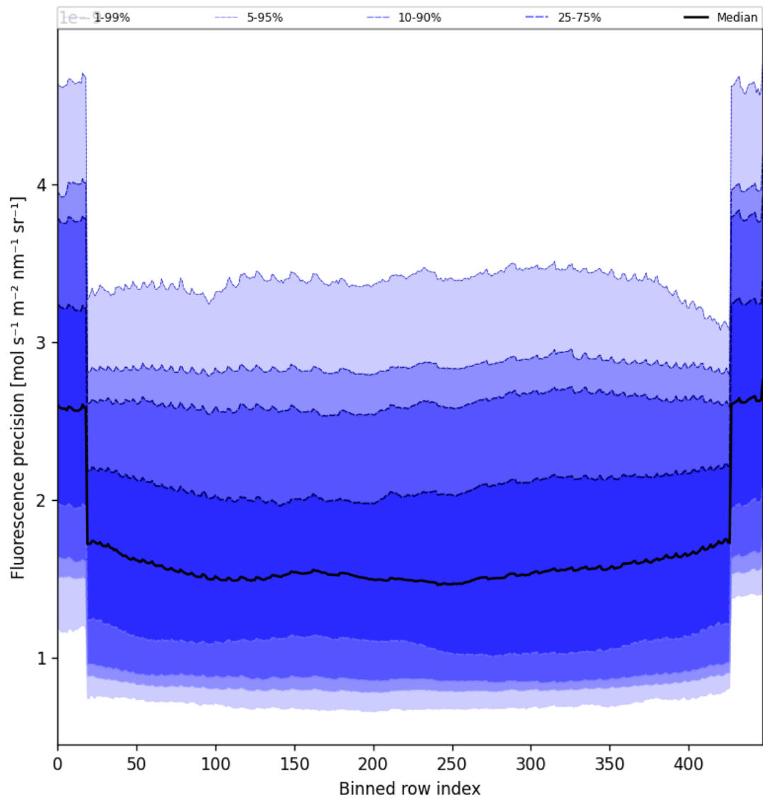
Figure 56: Along track statistics of “Fluorescence precision” for 2025-08-04 to 2025-08-05
