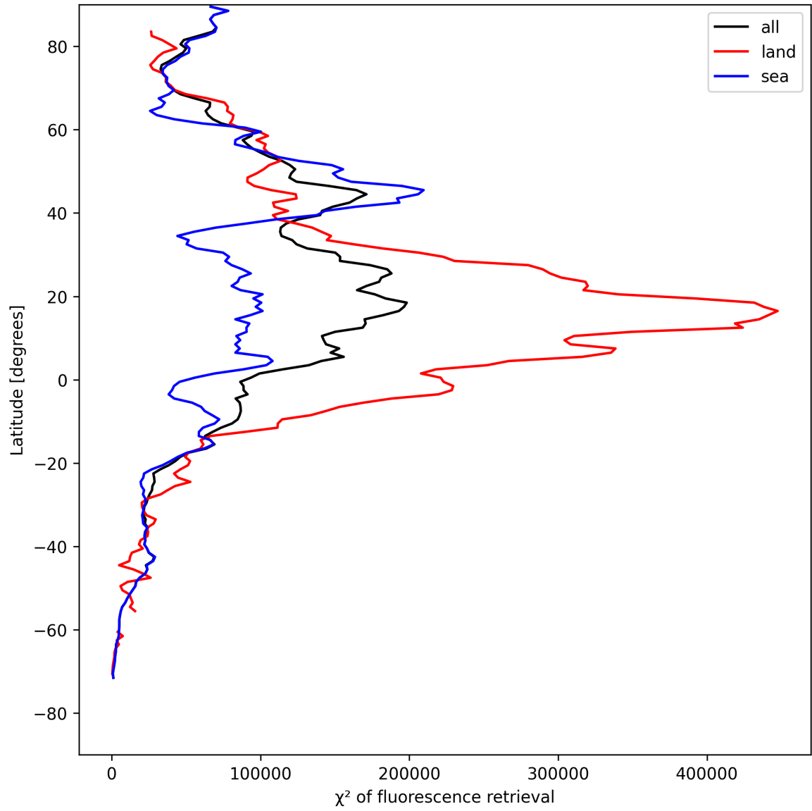
Figure 23: Zonal average of “ \chi^2 of fluorescence retrieval” for 2025-08-05 to 2025-08-06.
