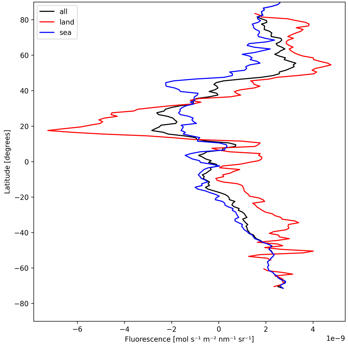
Figure 21: Zonal average of “Fluorescence” for 2025-08-05 to 2025-08-06.
