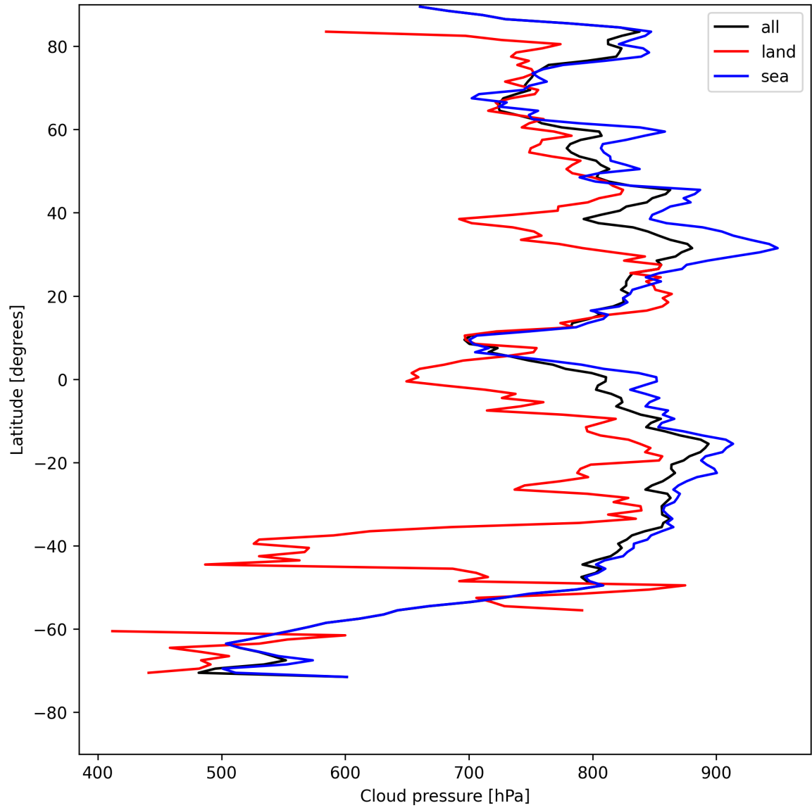
Figure 11: Zonal average of “Cloud pressure” for 2025-08-05 to 2025-08-06.
