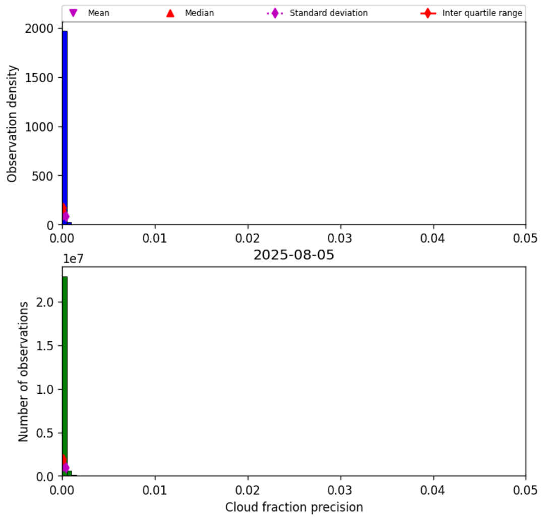
Figure 31: Histogram of “Cloud fraction precision” for 2025-08-05 to 2025-08-06
