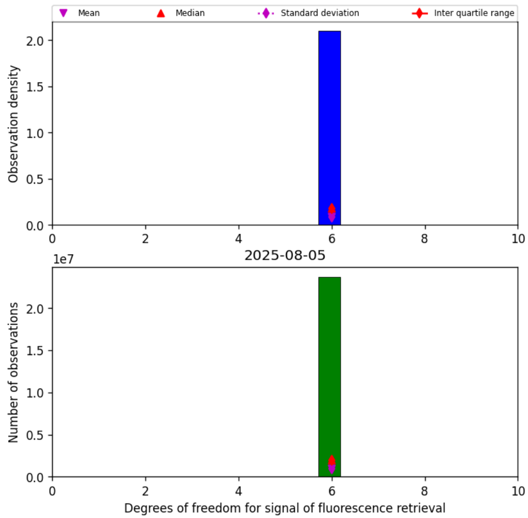
Figure 41: Histogram of “Degrees of freedom for signal of fluorescence retrieval” for 2025-08-05 to 2025-08-06
