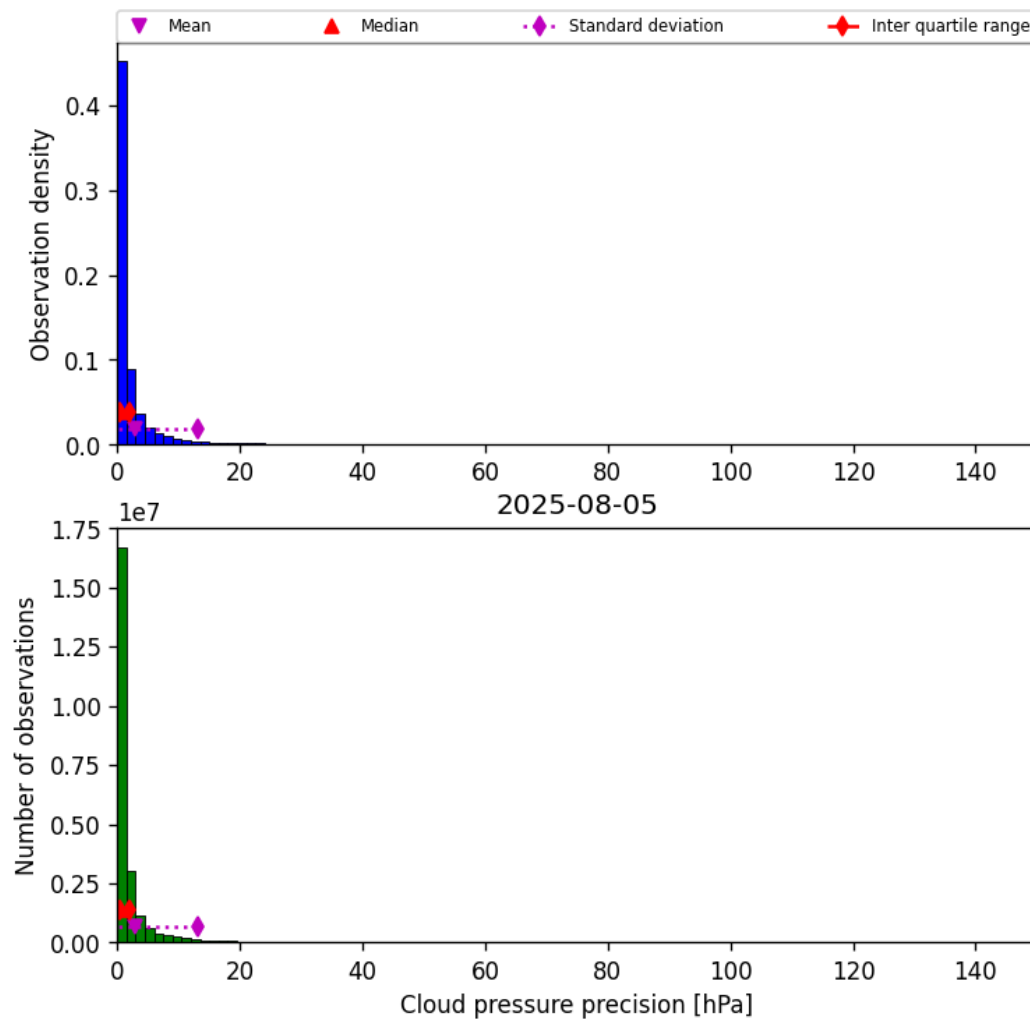
Figure 29: Histogram of “Cloud pressure precision” for 2025-08-05 to 2025-08-06
