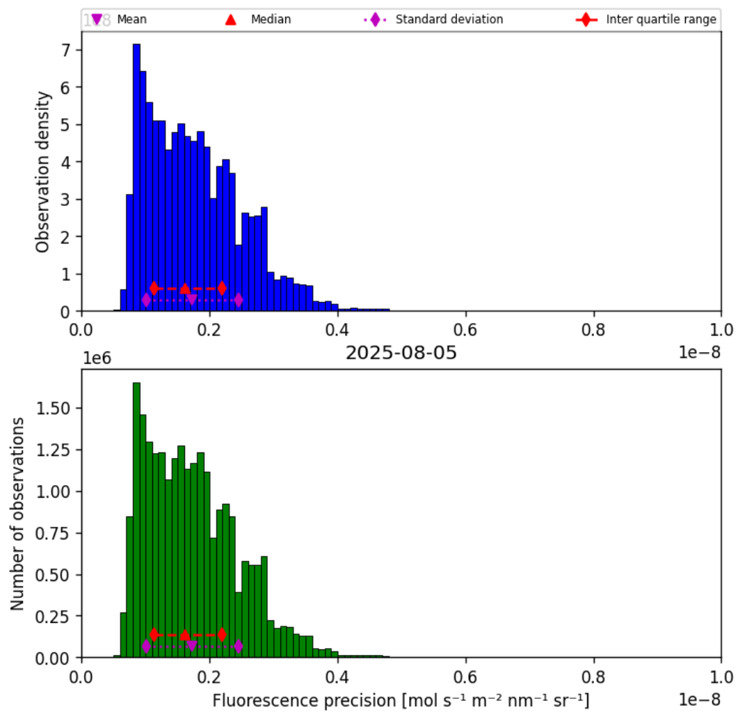
Figure 39: Histogram of “Fluorescence precision” for 2025-08-05 to 2025-08-06
