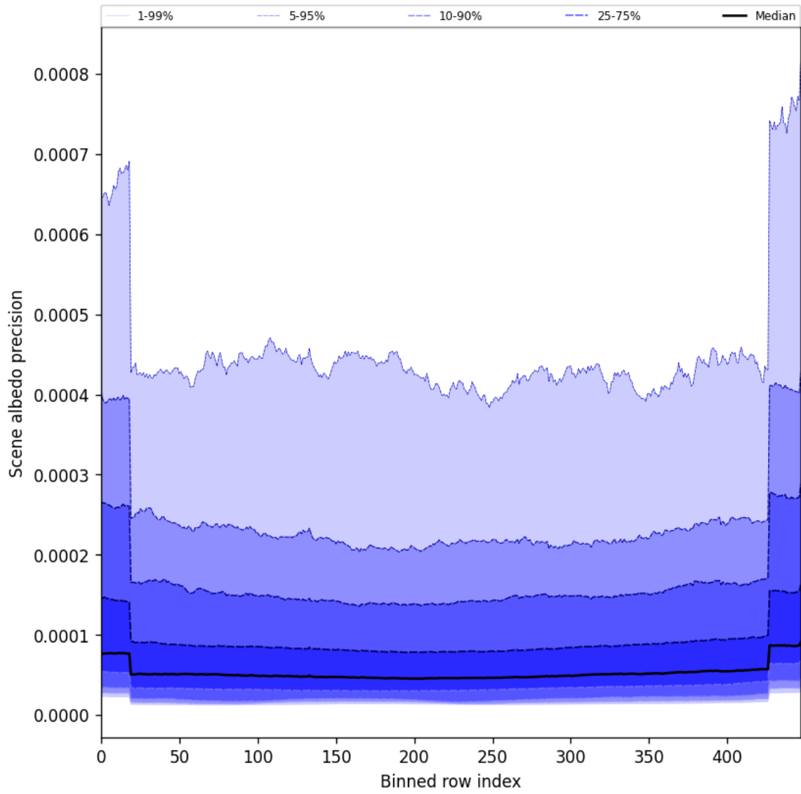
Figure 50: Along track statistics of “Scene albedo precision” for 2025-08-05 to 2025-08-06
