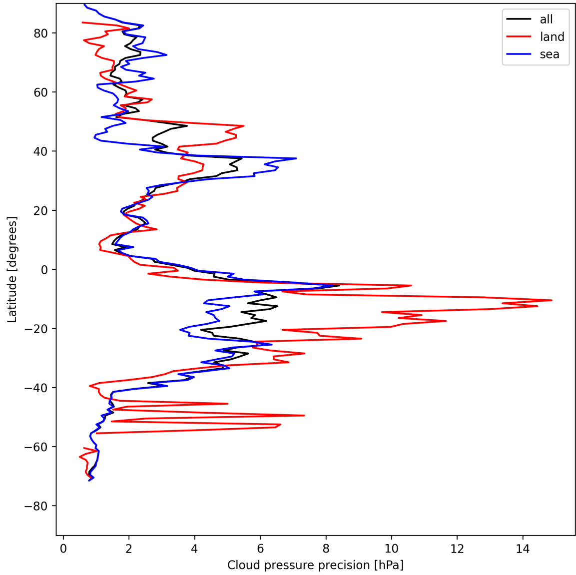
Figure 12: Zonal average of "Cloud pressure precision" for 2025-08-05 to 2025-08-06.
