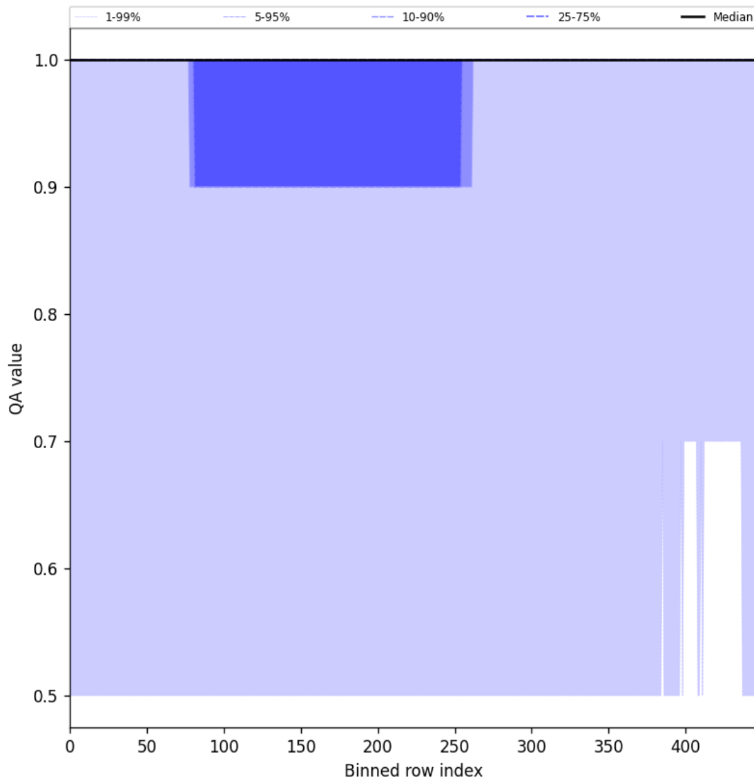
Figure 44: Along track statistics of “QA value” for 2025-08-05 to 2025-08-06
