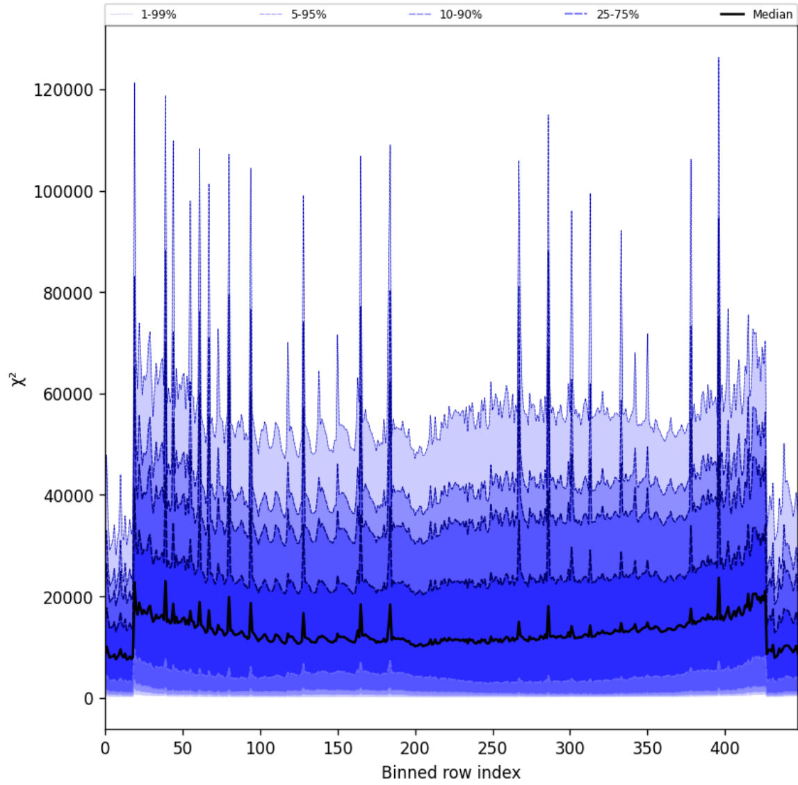
Figure 53: Along track statistics of “ \chi^2 ” for 2025-08-05 to 2025-08-06
