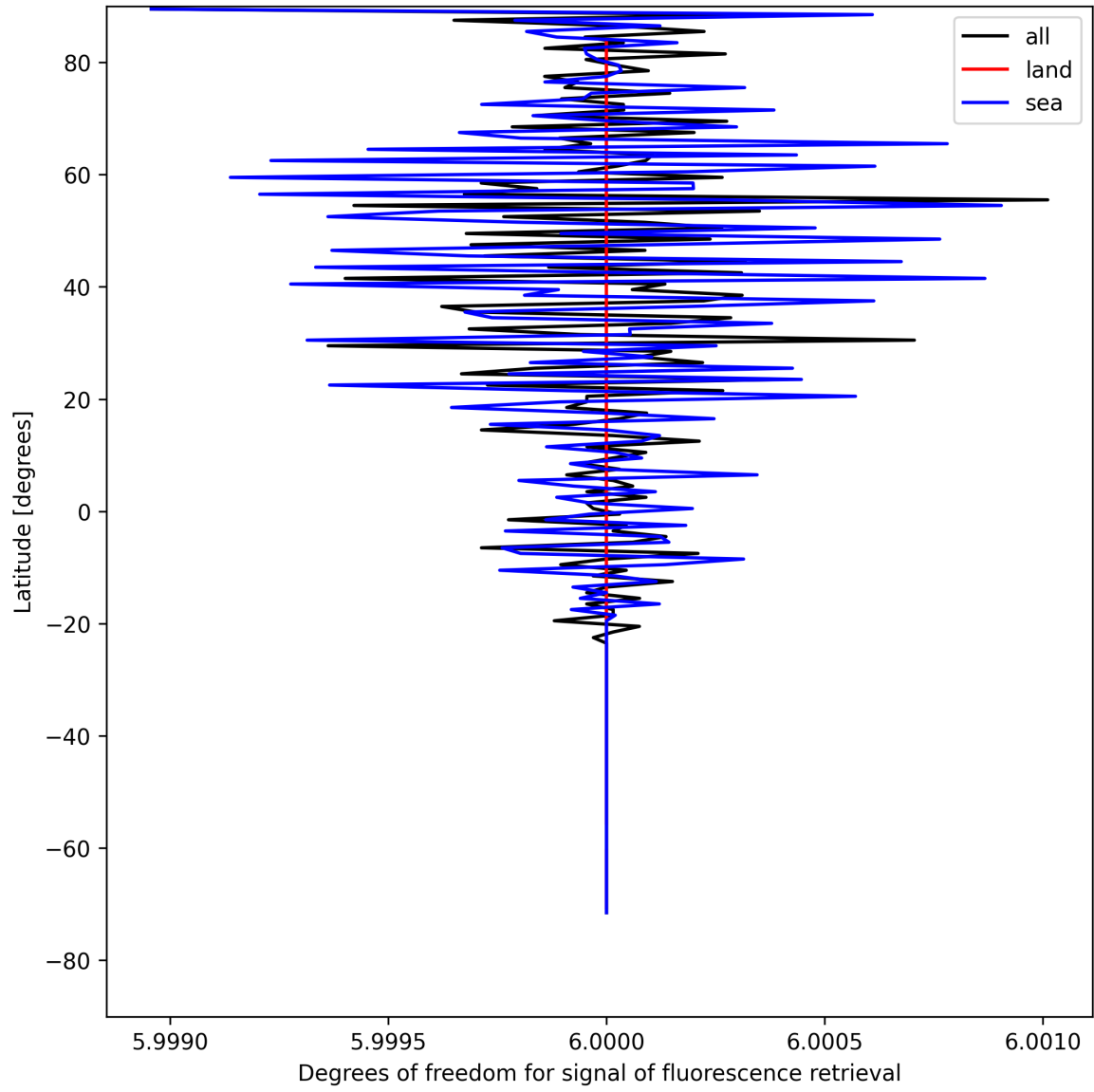
Figure 24: Zonal average of “Degrees of freedom for signal of fluorescence retrieval” for 2025-08-05 to 2025-08-06.
