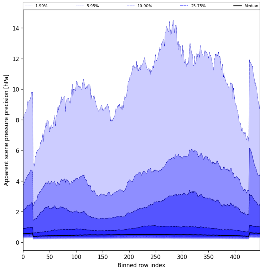
Figure 52: Along track statistics of “Apparent scene pressure precision” for 2025-08-05 to 2025-08-06
