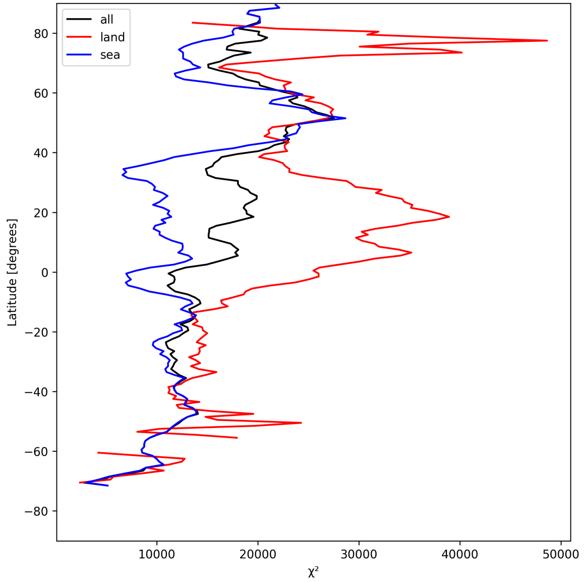
Figure 19: Zonal average of “ \chi^2 ” for 2025-08-05 to 2025-08-06.
