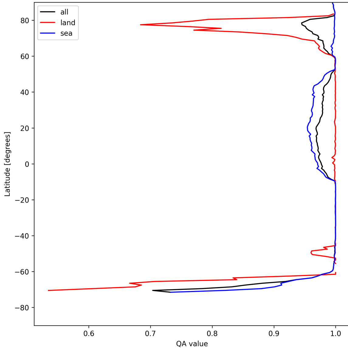
Figure 10: Zonal average of "QA value" for 2025-08-05 to 2025-08-06.
