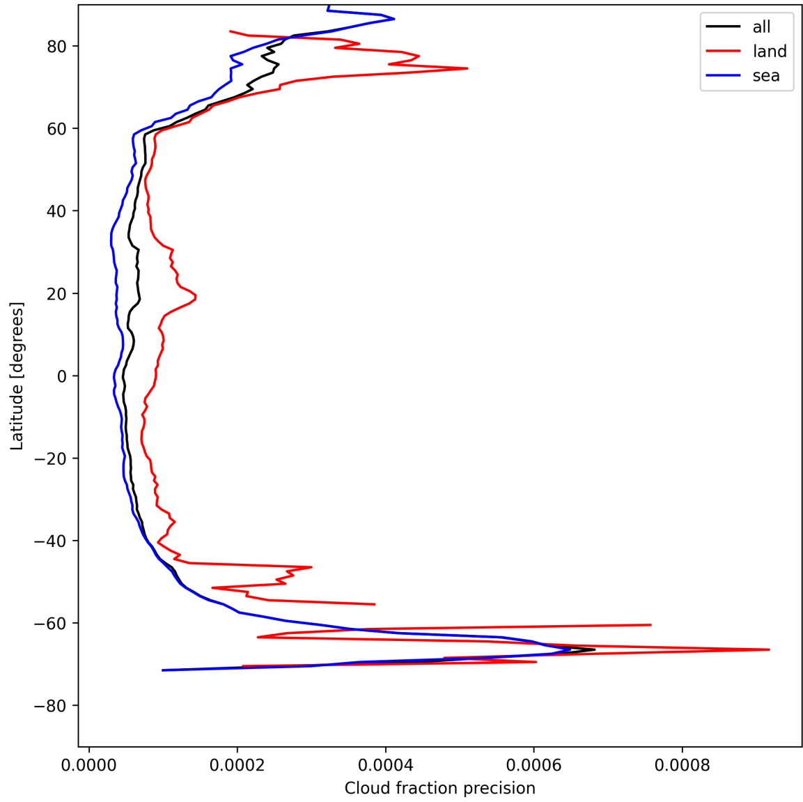
Figure 14: Zonal average of “Cloud fraction precision” for 2025-08-05 to 2025-08-06.
