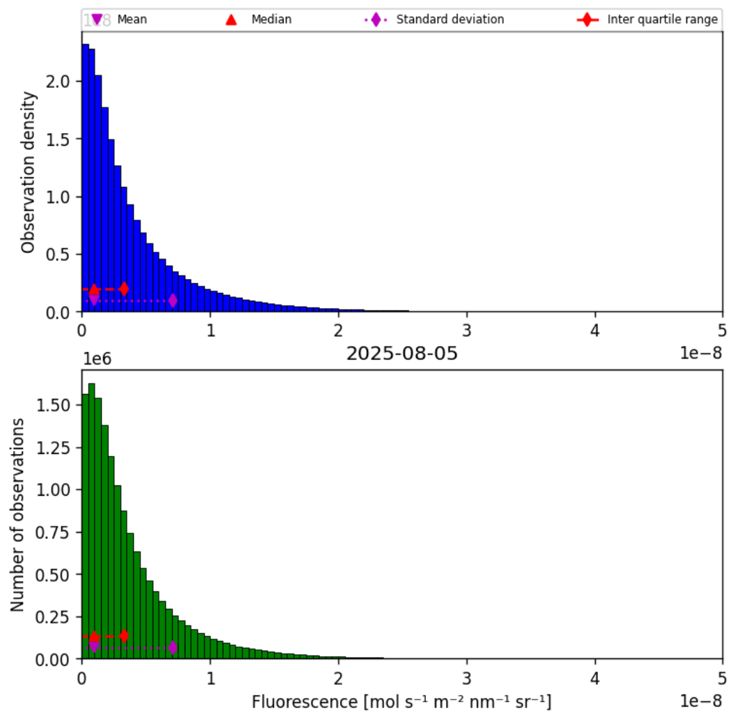
Figure 38: Histogram of “Fluorescence” for 2025-08-05 to 2025-08-06
