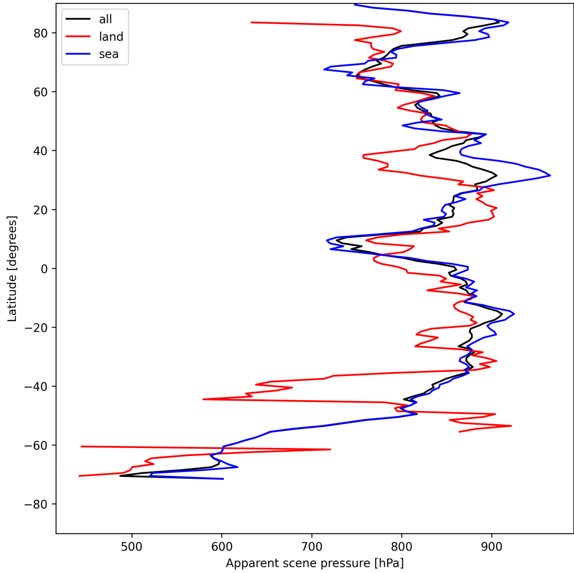
Figure 17: Zonal average of “Apparent scene pressure” for 2025-08-05 to 2025-08-06.
