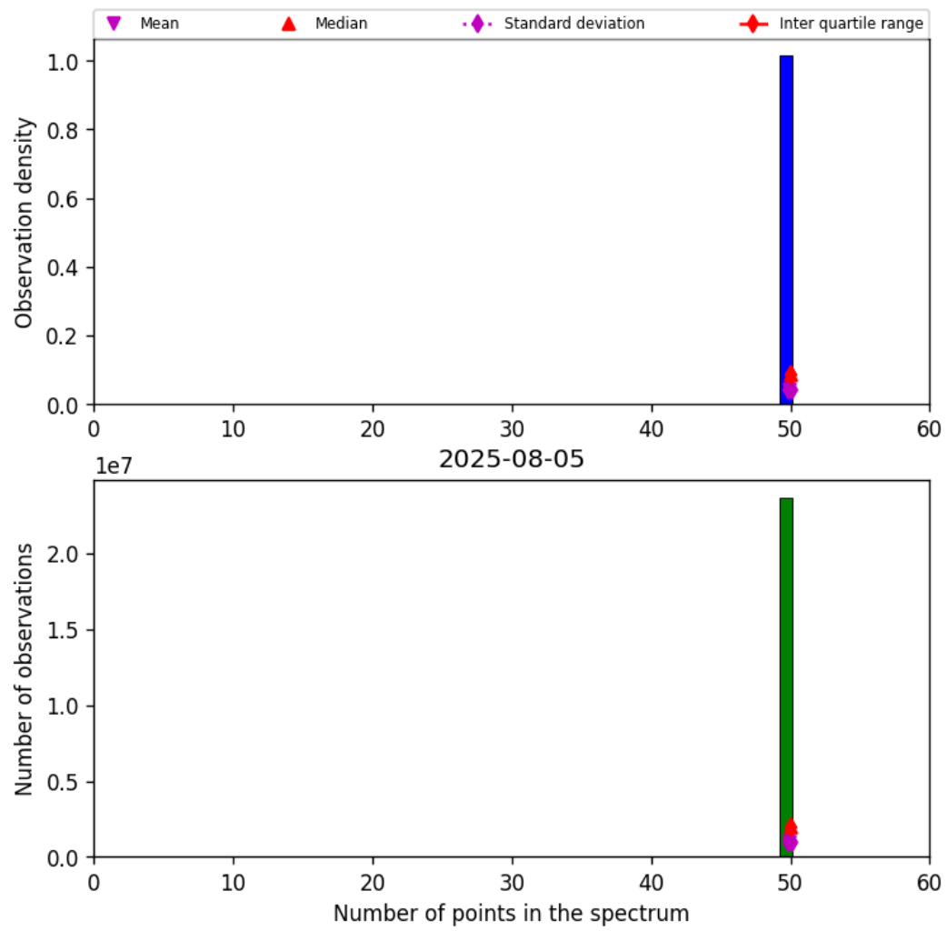
Figure 42: Histogram of "Number of points in the spectrum" for 2025-08-05 to 2025-08-06
