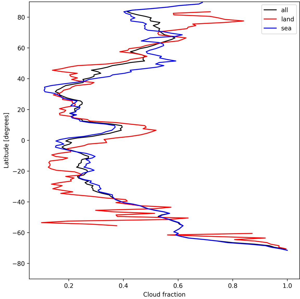
Figure 13: Zonal average of “Cloud fraction” for 2025-08-05 to 2025-08-06.
