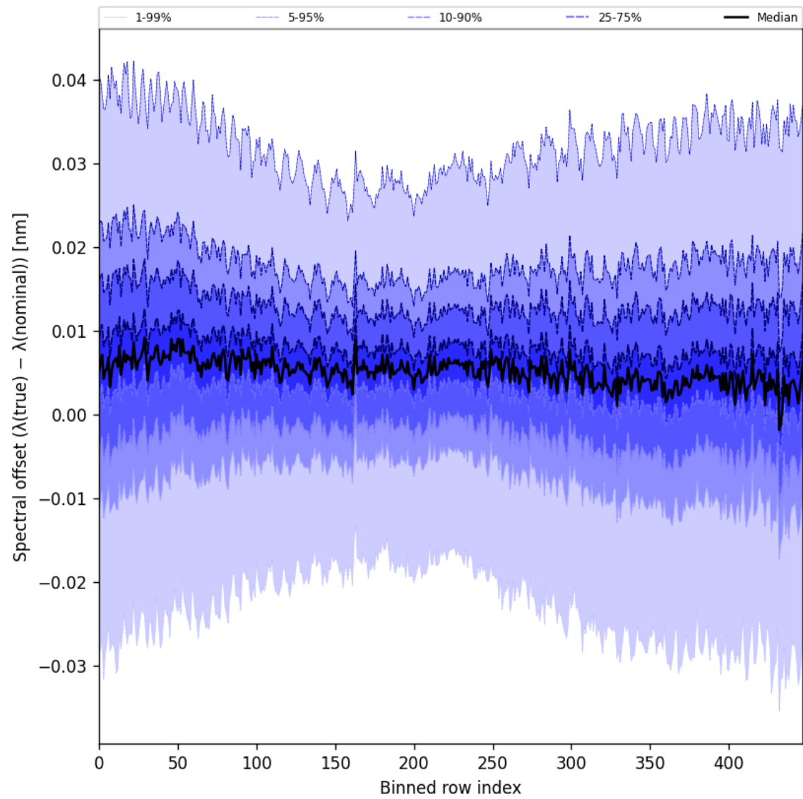
Figure 60: Along track statistics of “Spectral offset ( \lambda_{\text{true}} - \lambda_{\text{nominal}} )” for 2025-08-05 to 2025-08-06
