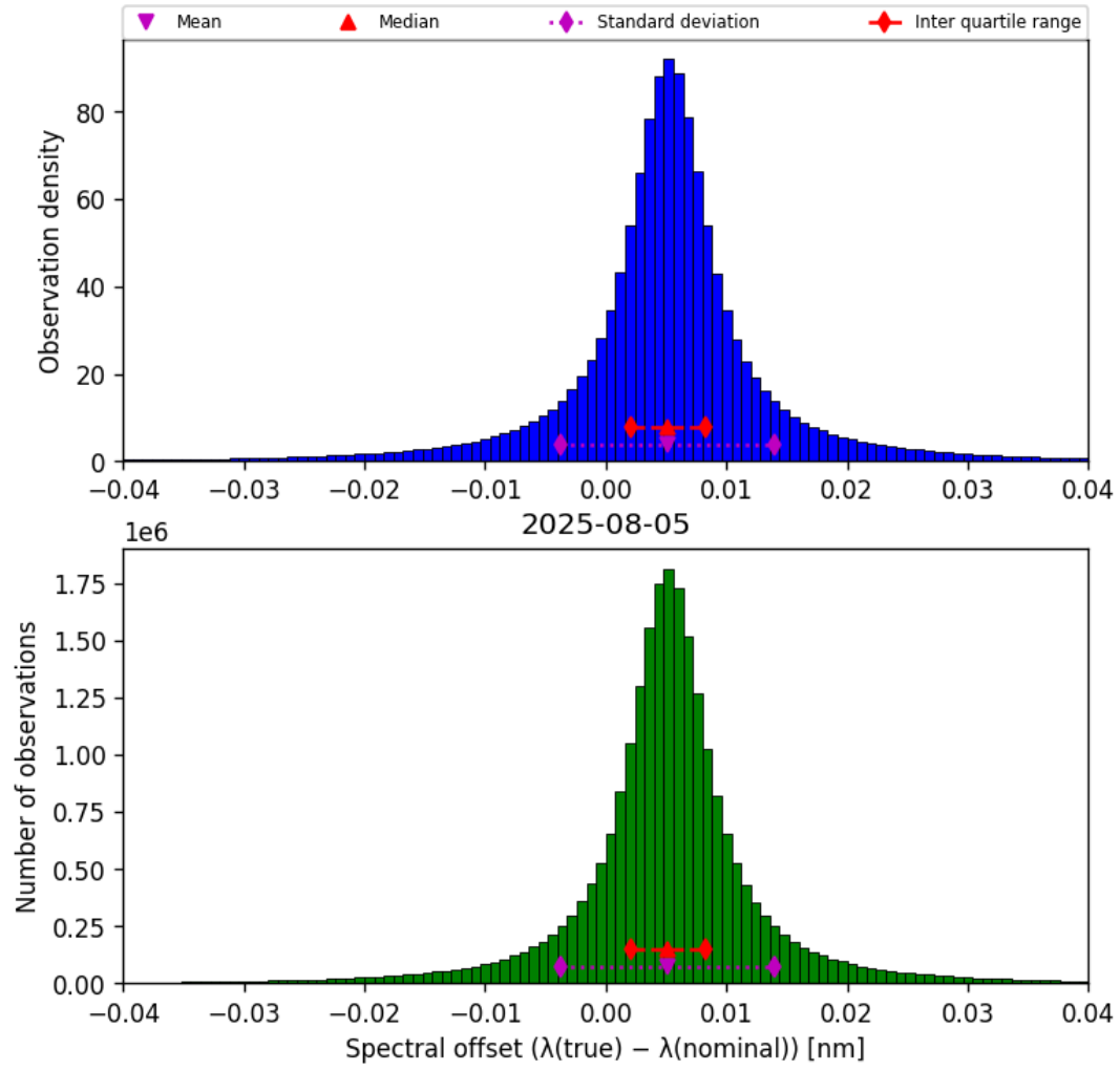
Figure 43: Histogram of “Spectral offset ( \lambda_{\text{true}} - \lambda_{\text{nominal}} )” for 2025-08-05 to 2025-08-06
