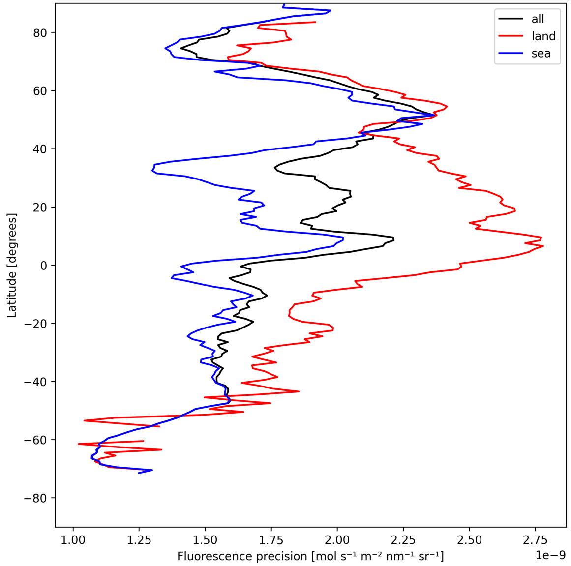
Figure 22: Zonal average of “Fluorescence precision” for 2025-08-05 to 2025-08-06.
