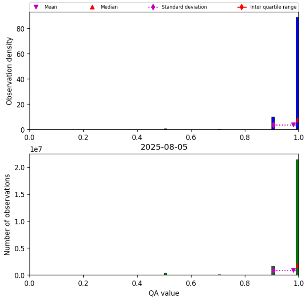
Figure 27: Histogram of “QA value” for 2025-08-05 to 2025-08-06
