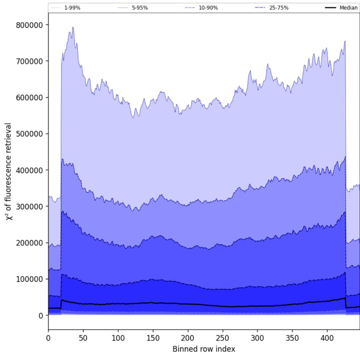
Figure 57: Along track statistics of “ \chi^2 of fluorescence retrieval” for 2025-08-05 to 2025-08-06
