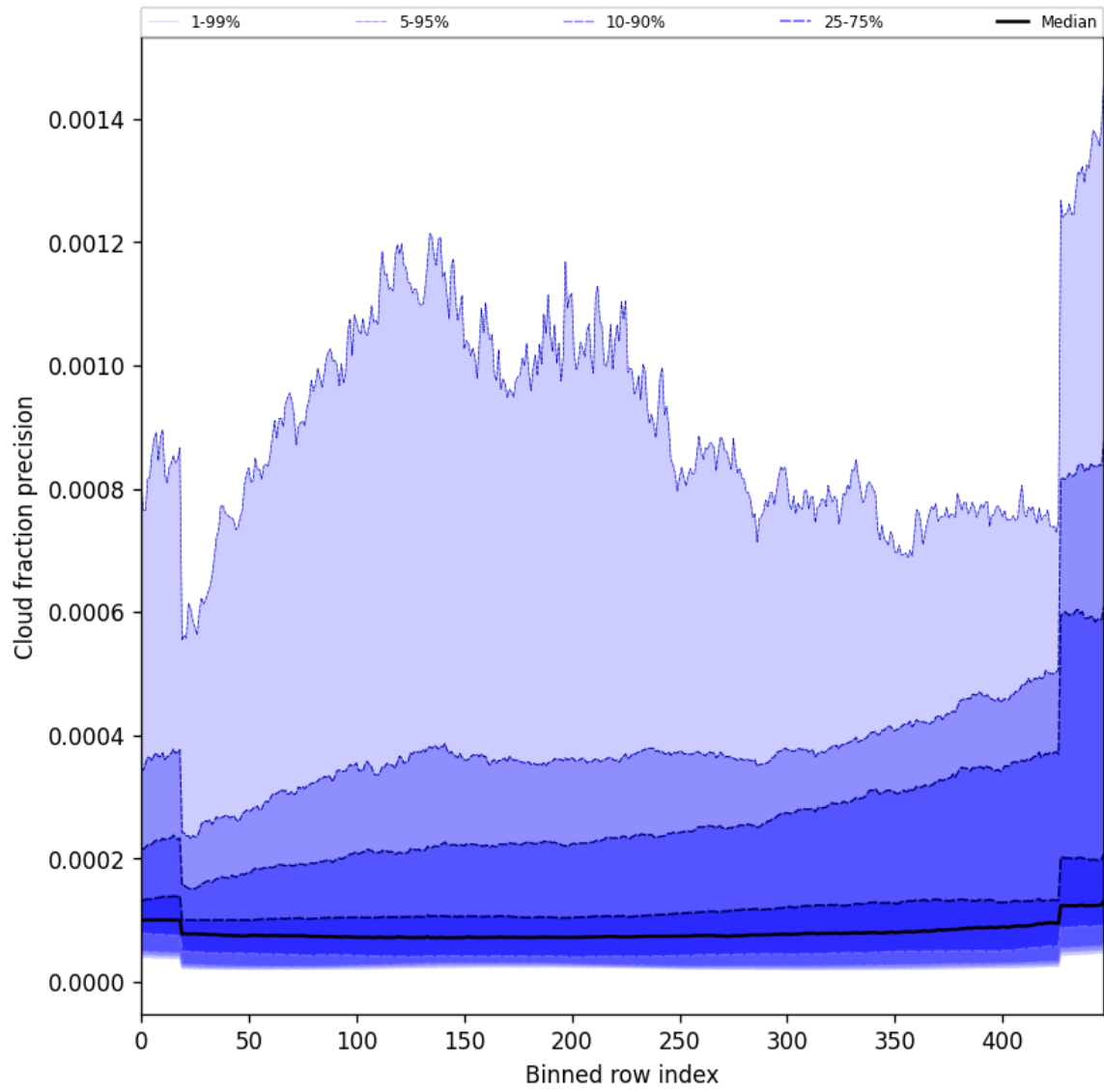
Figure 48: Along track statistics of “Cloud fraction precision” for 2025-08-05 to 2025-08-06
