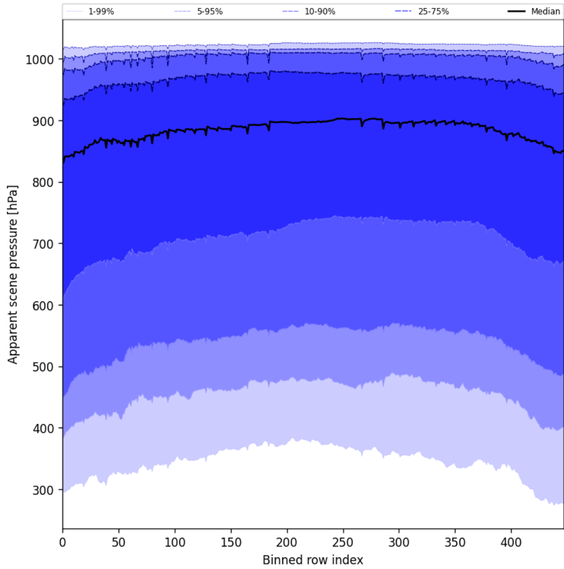
Figure 51: Along track statistics of “Apparent scene pressure” for 2025-08-05 to 2025-08-06
