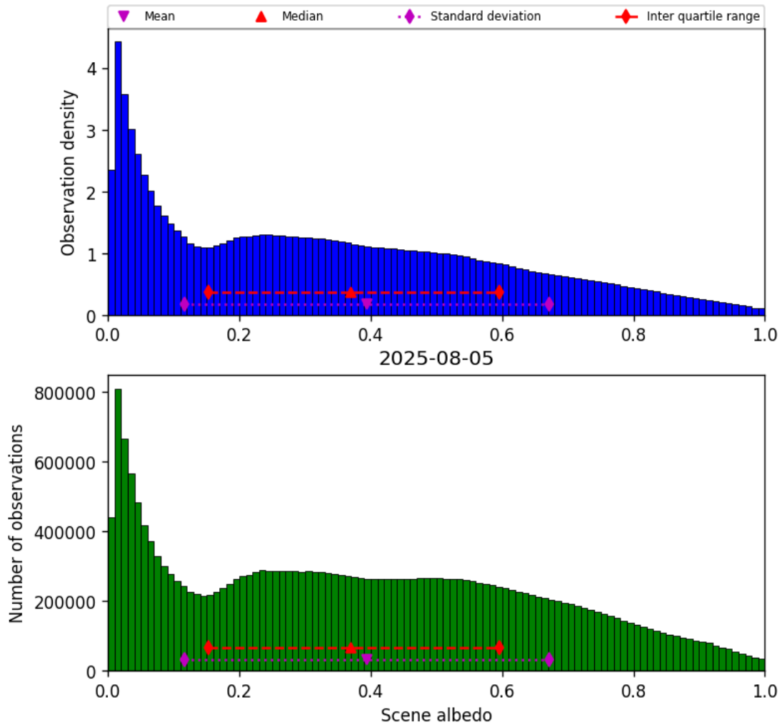
Figure 32: Histogram of “Scene albedo” for 2025-08-05 to 2025-08-06
