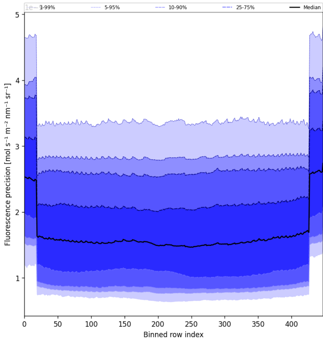
Figure 56: Along track statistics of “Fluorescence precision” for 2025-08-05 to 2025-08-06
