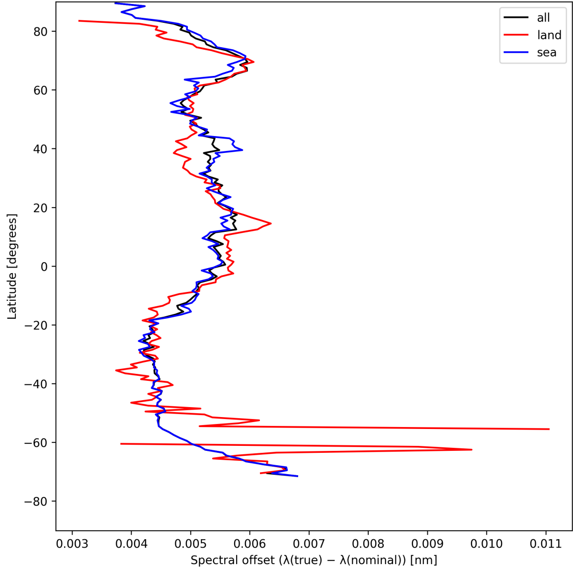
Figure 26: Zonal average of “Spectral offset ( \lambda_{\text{true}} - \lambda_{\text{nominal}} )” for 2025-08-05 to 2025-08-06.
