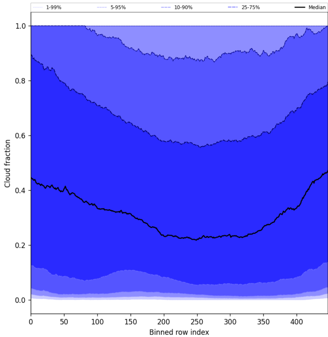
Figure 47: Along track statistics of “Cloud fraction” for 2025-08-05 to 2025-08-06
