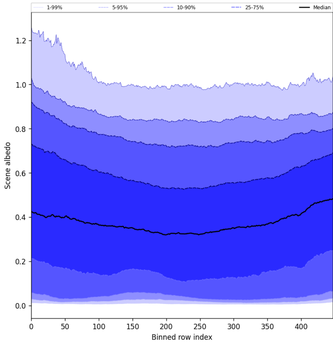
Figure 49: Along track statistics of “Scene albedo” for 2025-08-05 to 2025-08-06
