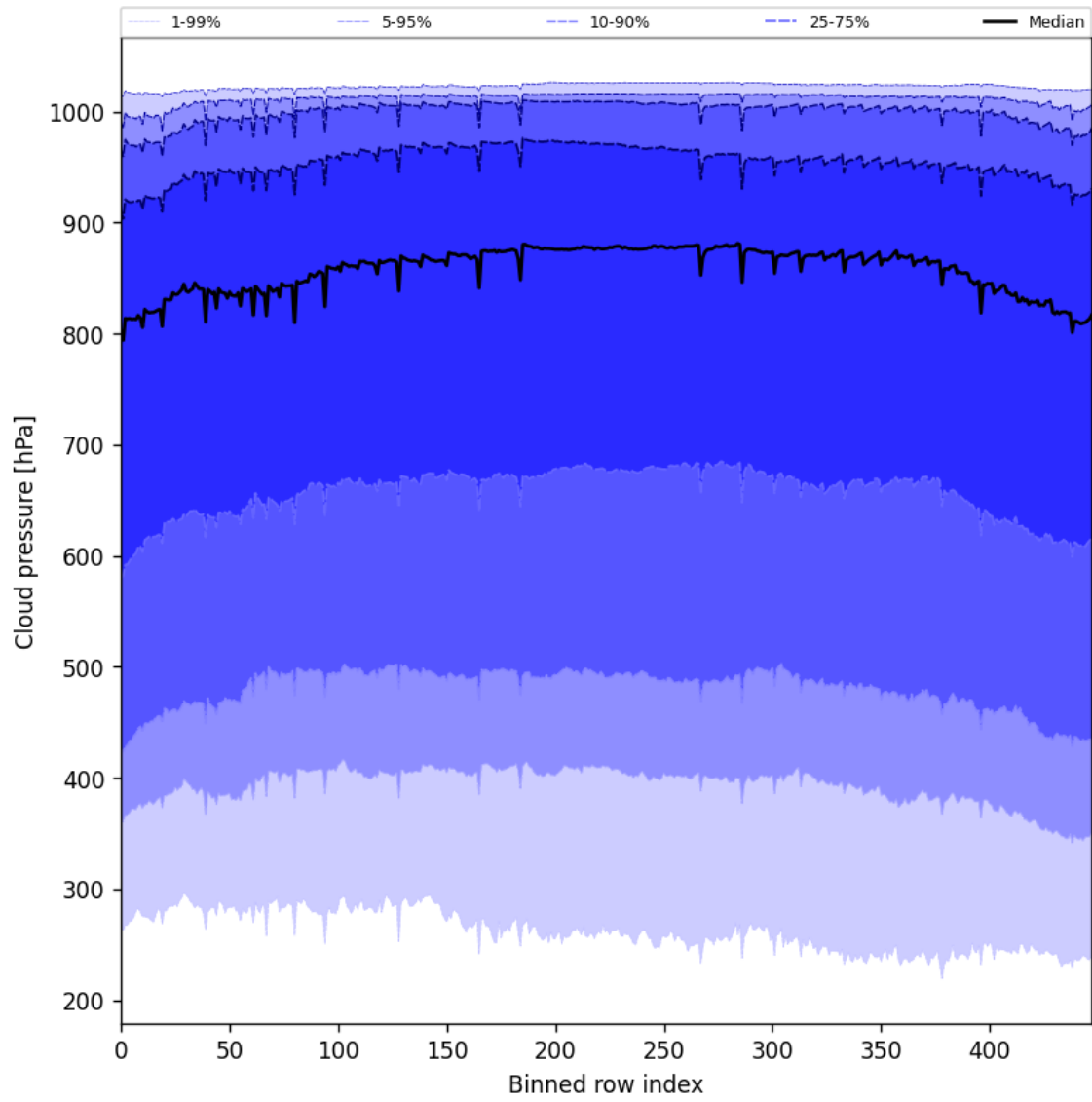
Figure 45: Along track statistics of “Cloud pressure” for 2025-08-05 to 2025-08-06
