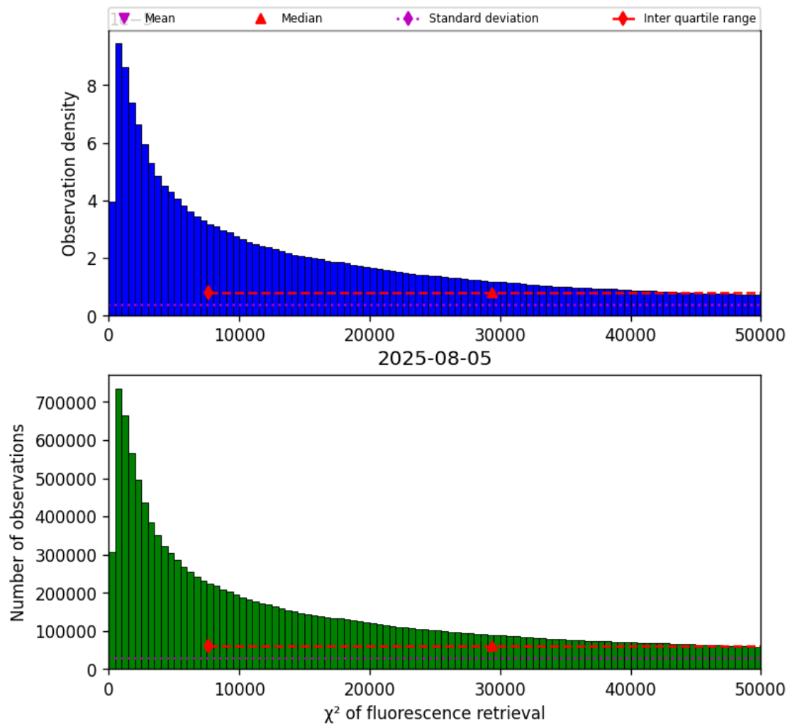
Figure 40: Histogram of “ \chi^2 of fluorescence retrieval” for 2025-08-05 to 2025-08-06
