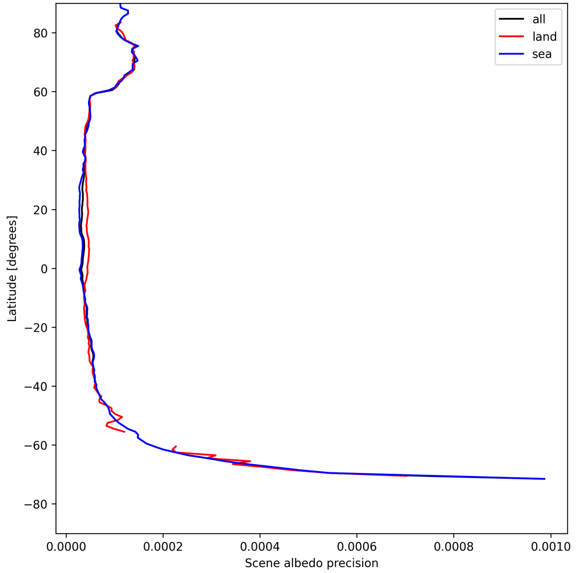
Figure 16: Zonal average of “Scene albedo precision” for 2025-08-05 to 2025-08-06.
