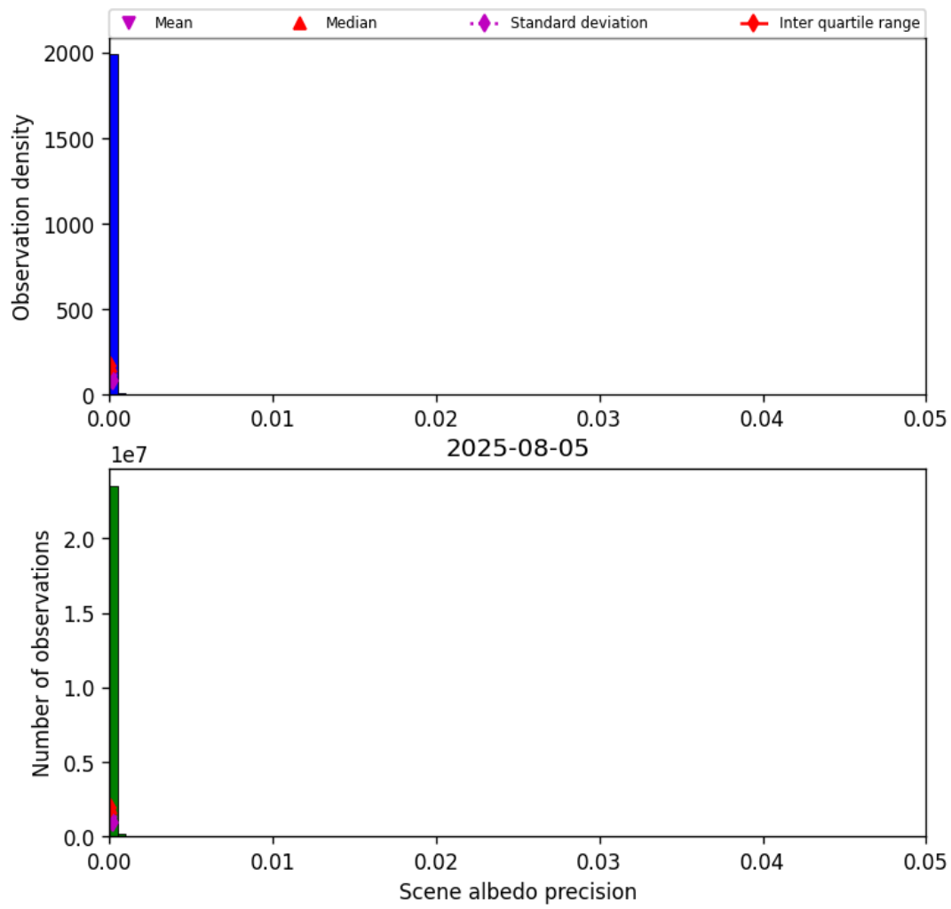
Figure 33: Histogram of “Scene albedo precision” for 2025-08-05 to 2025-08-06
