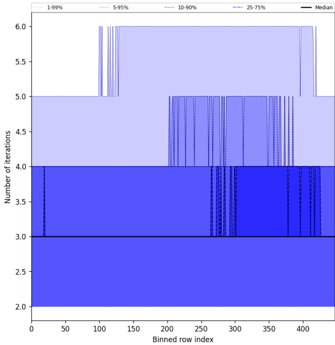
Figure 54: Along track statistics of “Number of iterations” for 2025-08-05 to 2025-08-06
