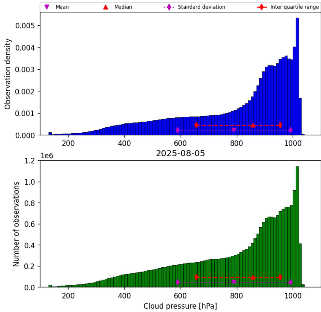
Figure 28: Histogram of “Cloud pressure” for 2025-08-05 to 2025-08-06
