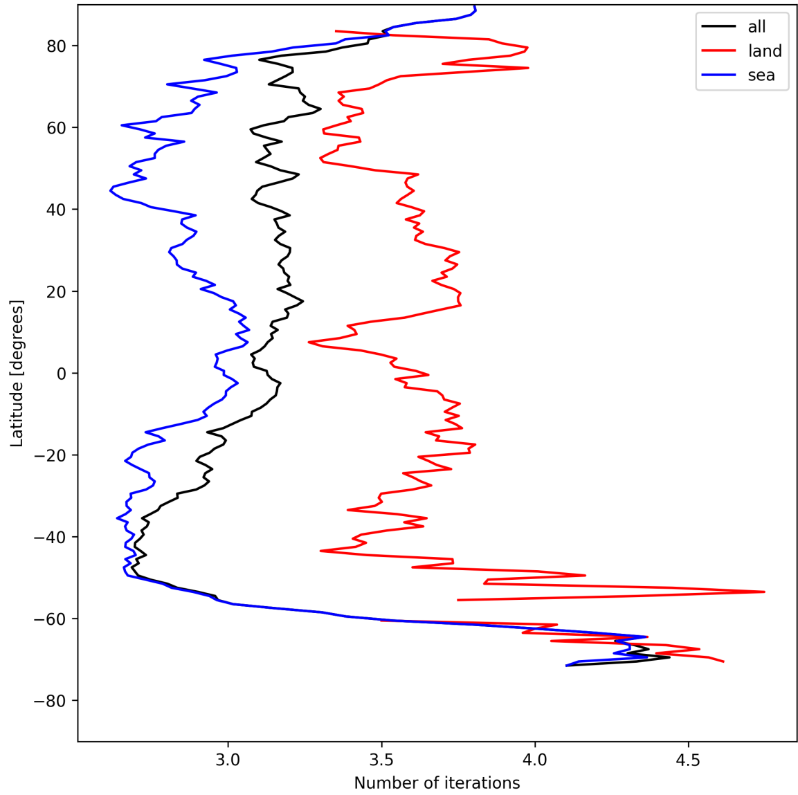
Figure 20: Zonal average of “Number of iterations” for 2025-08-05 to 2025-08-06.
