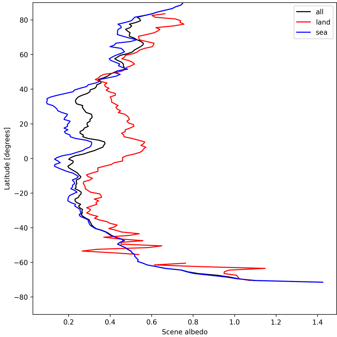
Figure 15: Zonal average of “Scene albedo” for 2025-08-05 to 2025-08-06.
