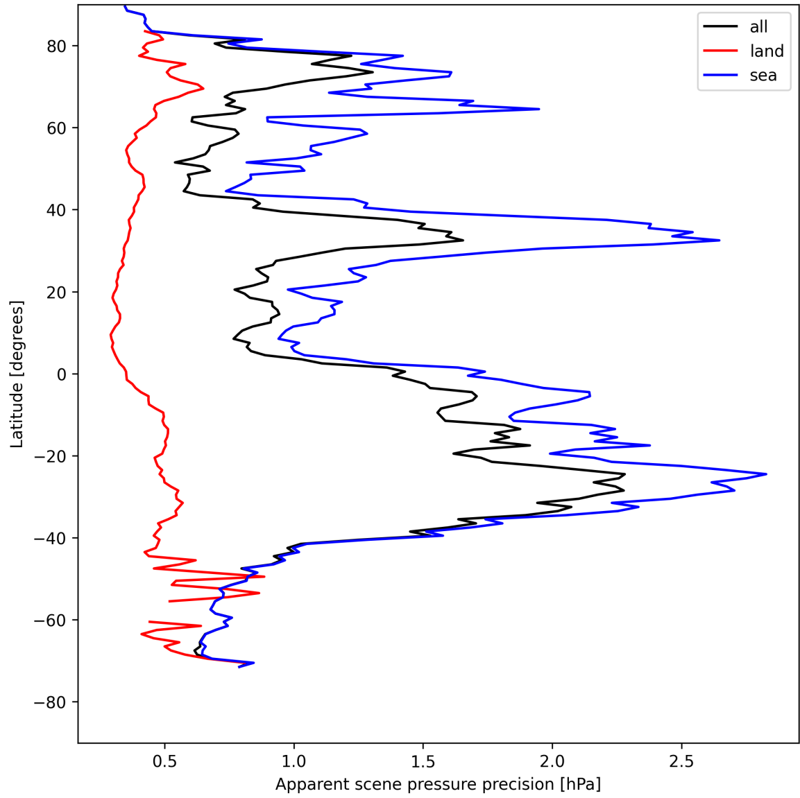
Figure 18: Zonal average of “Apparent scene pressure precision” for 2025-08-05 to 2025-08-06.
