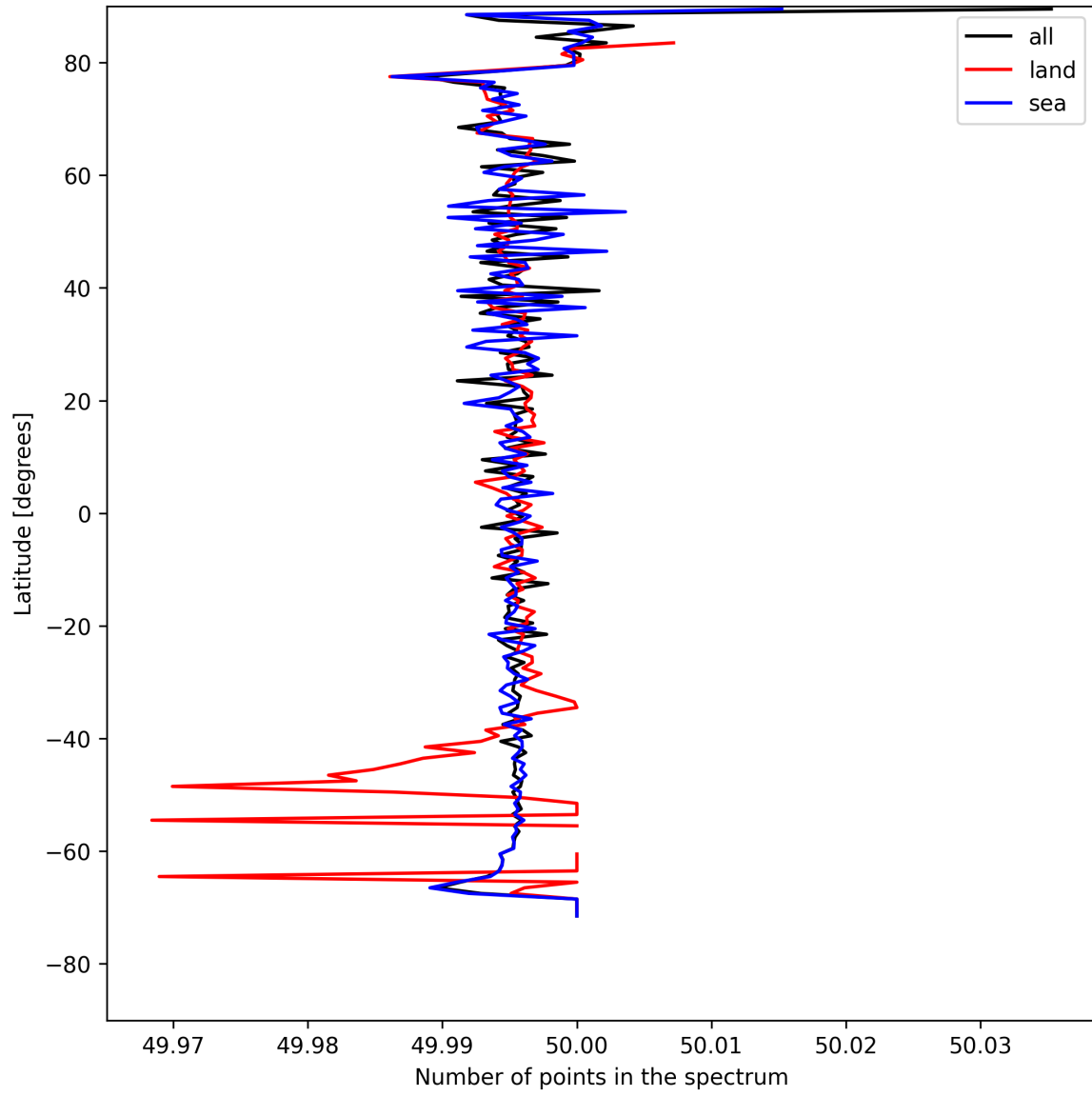
Figure 25: Zonal average of “Number of points in the spectrum” for 2025-08-05 to 2025-08-06.
