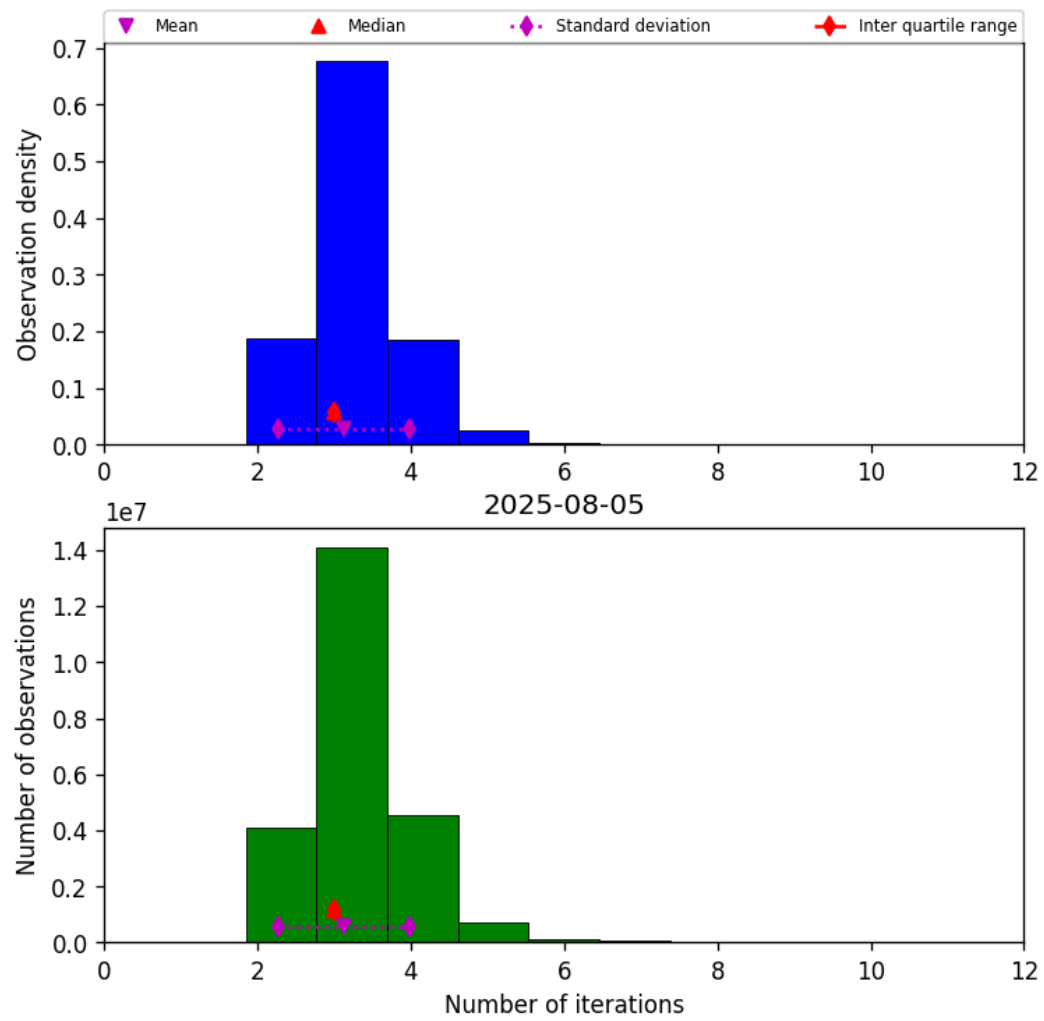
Figure 37: Histogram of “Number of iterations” for 2025-08-05 to 2025-08-06
