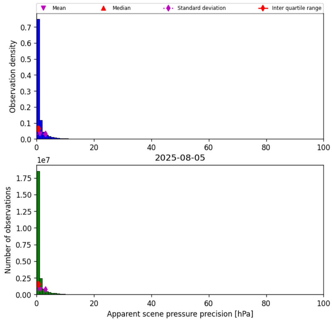
Figure 35: Histogram of “Apparent scene pressure precision” for 2025-08-05 to 2025-08-06
