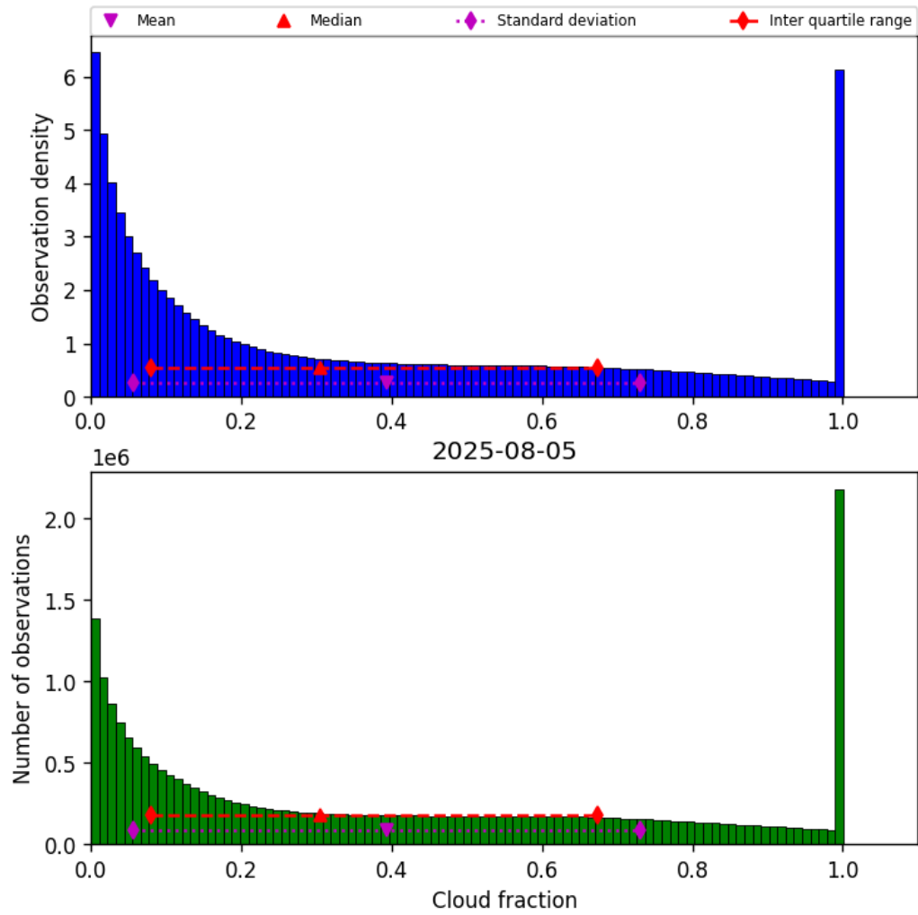
Figure 30: Histogram of “Cloud fraction” for 2025-08-05 to 2025-08-06
