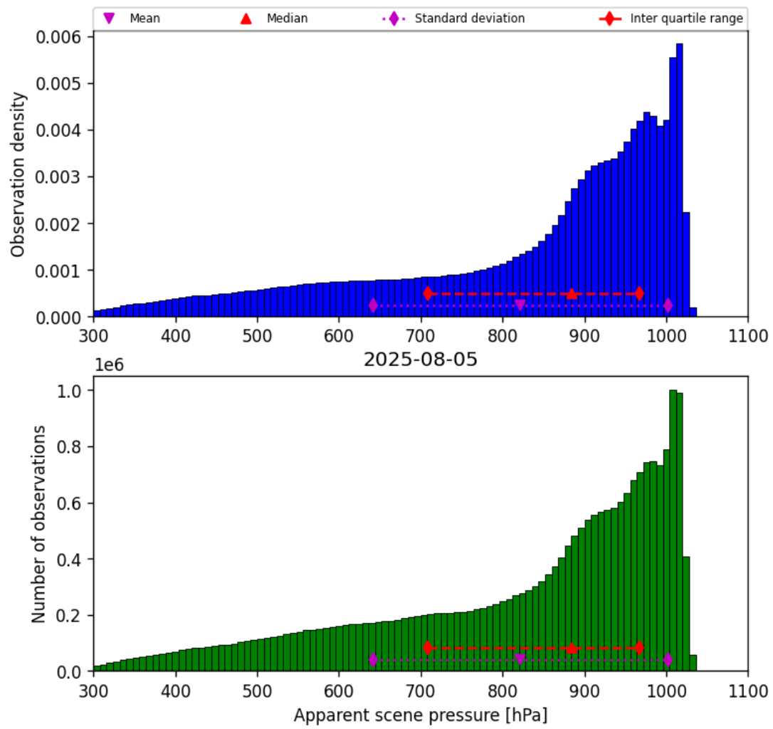
Figure 34: Histogram of “Apparent scene pressure” for 2025-08-05 to 2025-08-06
