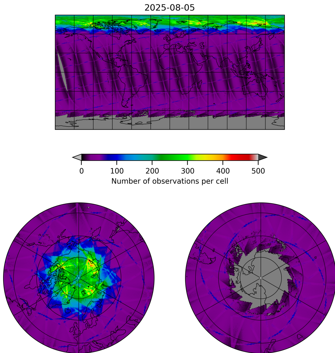
Figure 9: Map of the number of observations for 2025-08-05 to 2025-08-06
