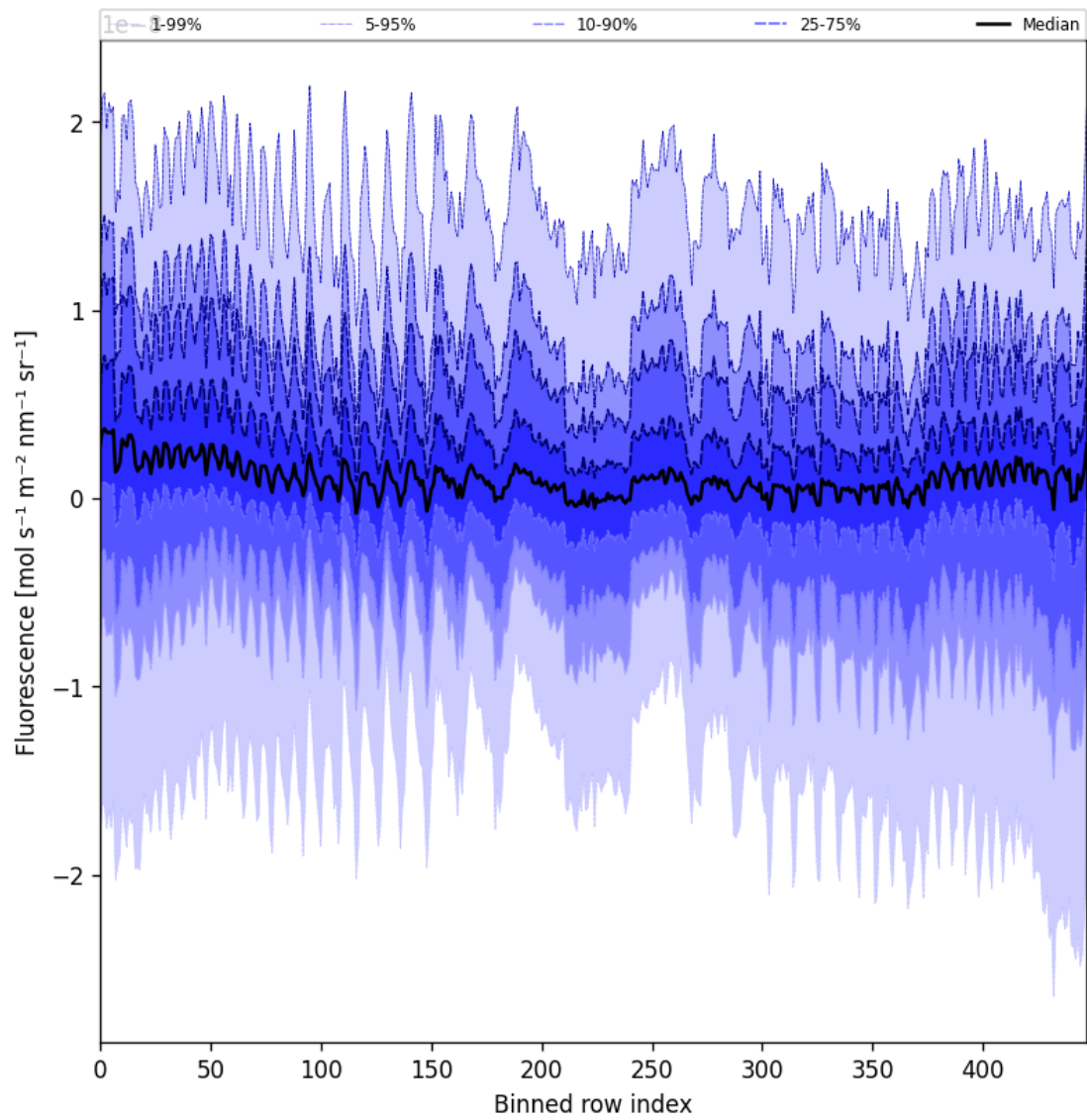
Figure 55: Along track statistics of “Fluorescence” for 2025-08-05 to 2025-08-06
