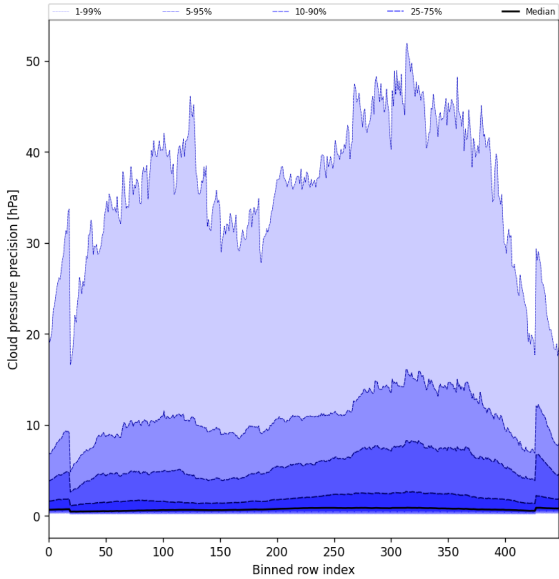
Figure 46: Along track statistics of “Cloud pressure precision” for 2025-08-05 to 2025-08-06
