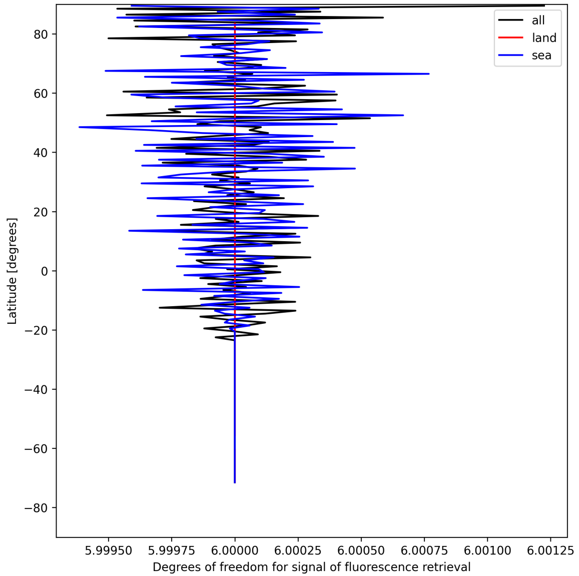
Figure 24: Zonal average of “Degrees of freedom for signal of fluorescence retrieval” for 2025-08-06 to 2025-08-07.
