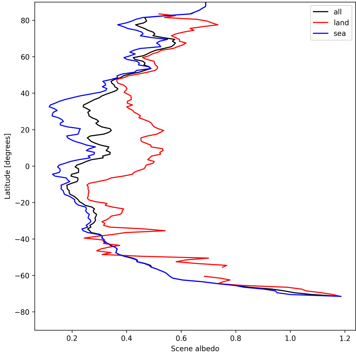
Figure 15: Zonal average of “Scene albedo” for 2025-08-06 to 2025-08-07.
