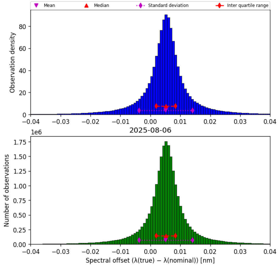
Figure 43: Histogram of “Spectral offset ( \lambda_{\text{true}} - \lambda_{\text{nominal}} )” for 2025-08-06 to 2025-08-07
