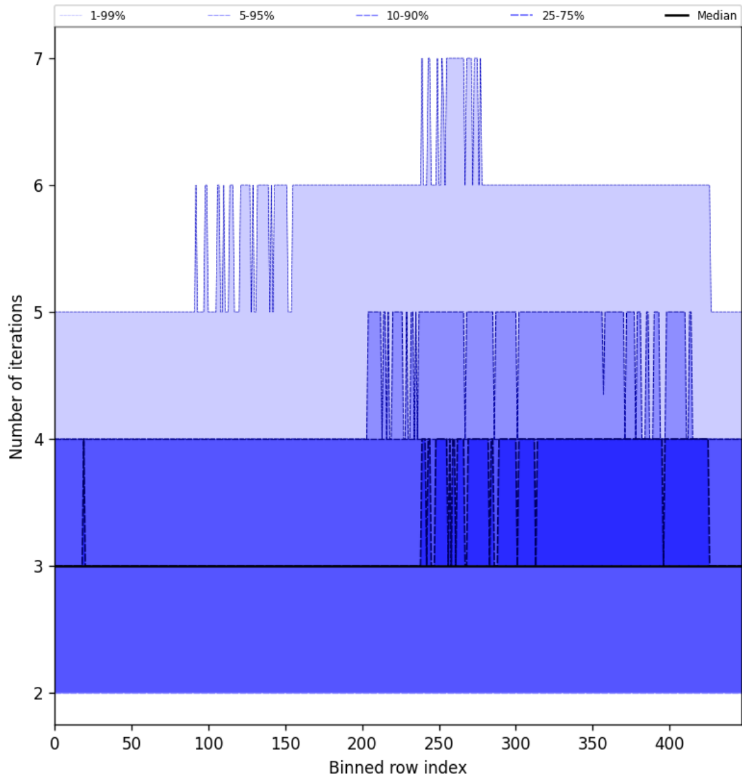
Figure 54: Along track statistics of “Number of iterations” for 2025-08-06 to 2025-08-07
