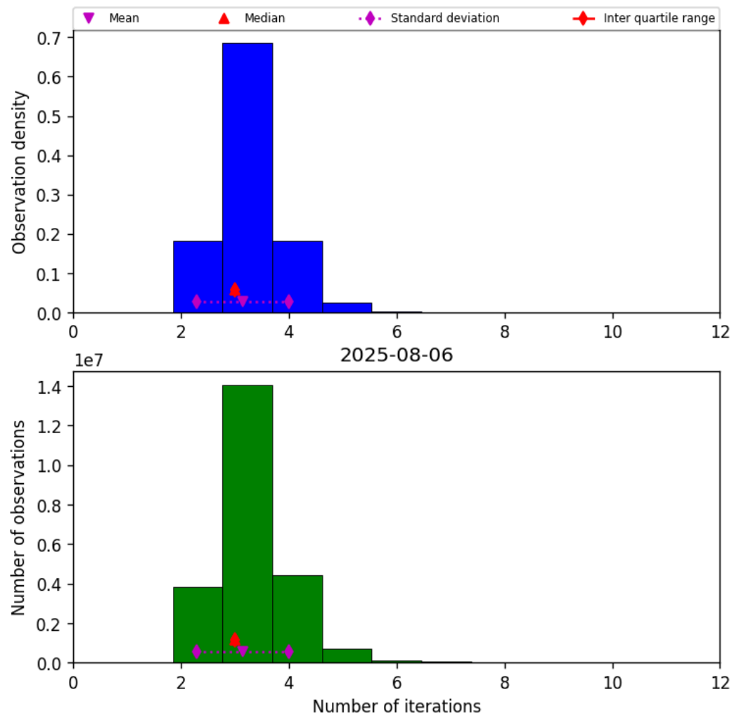
Figure 37: Histogram of “Number of iterations” for 2025-08-06 to 2025-08-07
