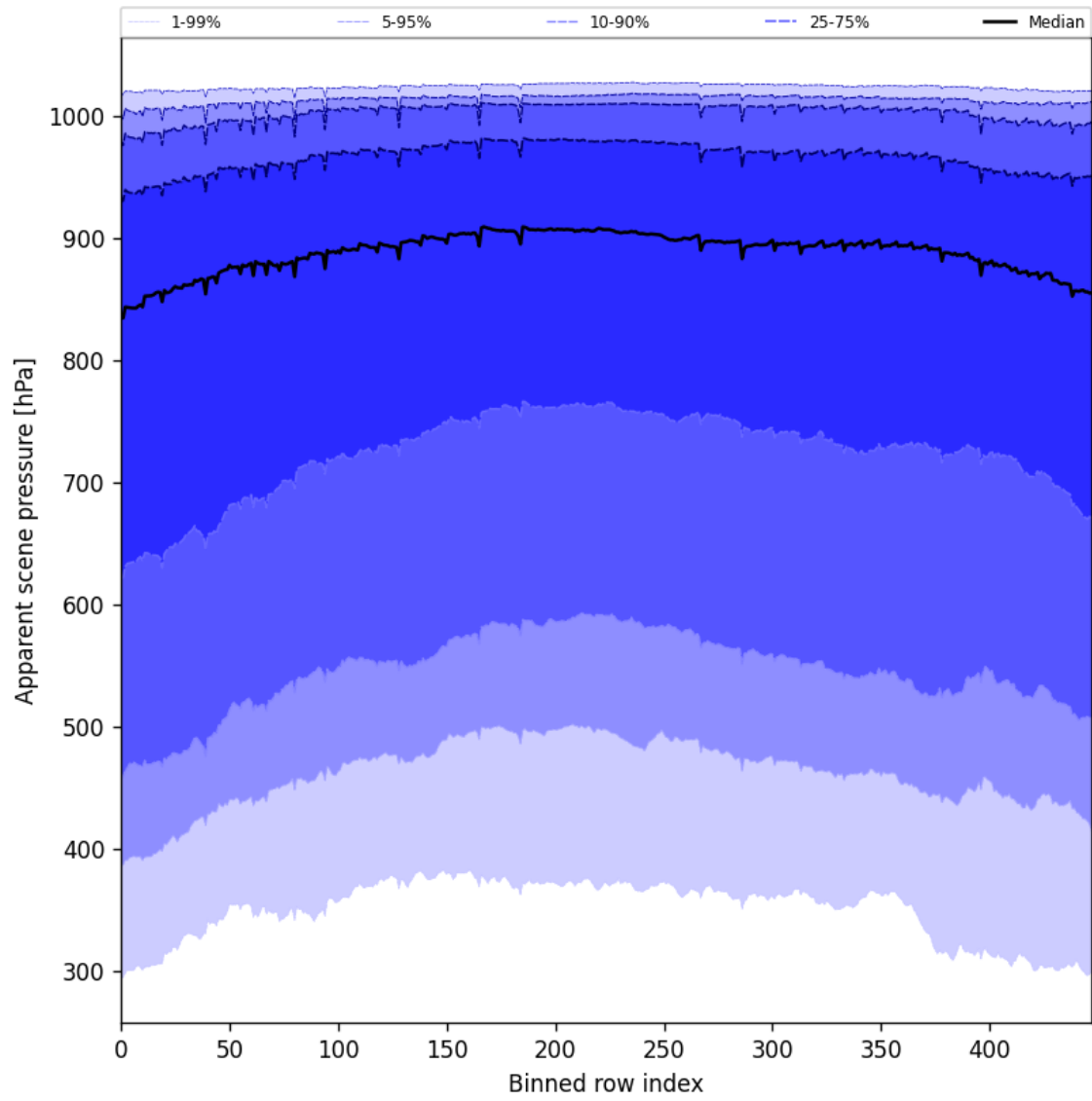
Figure 51: Along track statistics of “Apparent scene pressure” for 2025-08-06 to 2025-08-07
