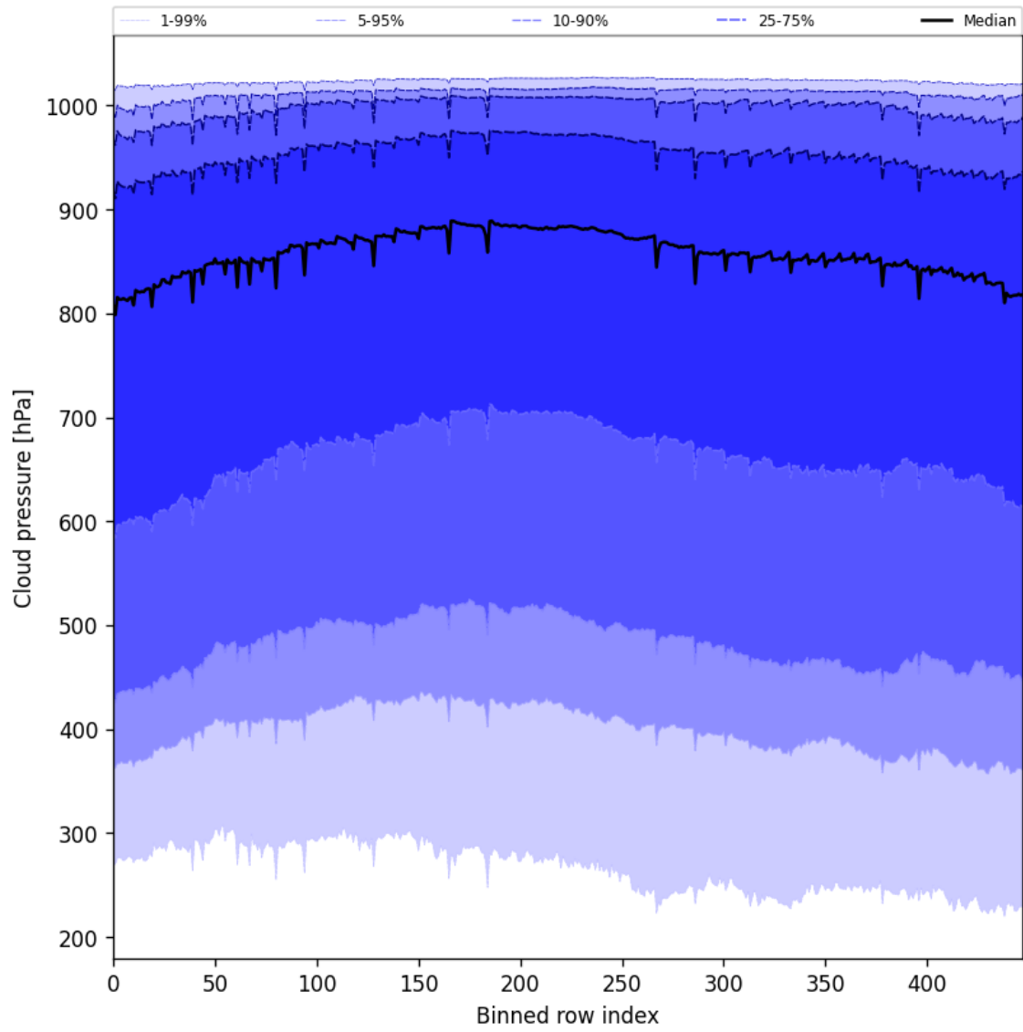
Figure 45: Along track statistics of “Cloud pressure” for 2025-08-06 to 2025-08-07
