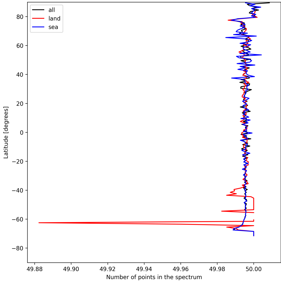
Figure 25: Zonal average of “Number of points in the spectrum” for 2025-08-06 to 2025-08-07.
