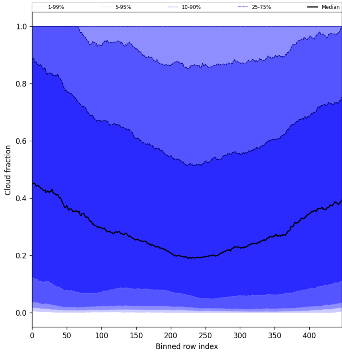
Figure 47: Along track statistics of “Cloud fraction” for 2025-08-06 to 2025-08-07
