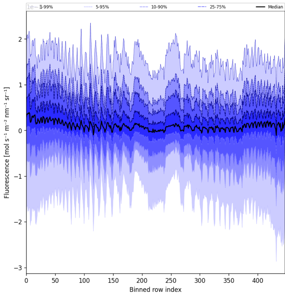
Figure 55: Along track statistics of "Fluorescence" for 2025-08-06 to 2025-08-07
