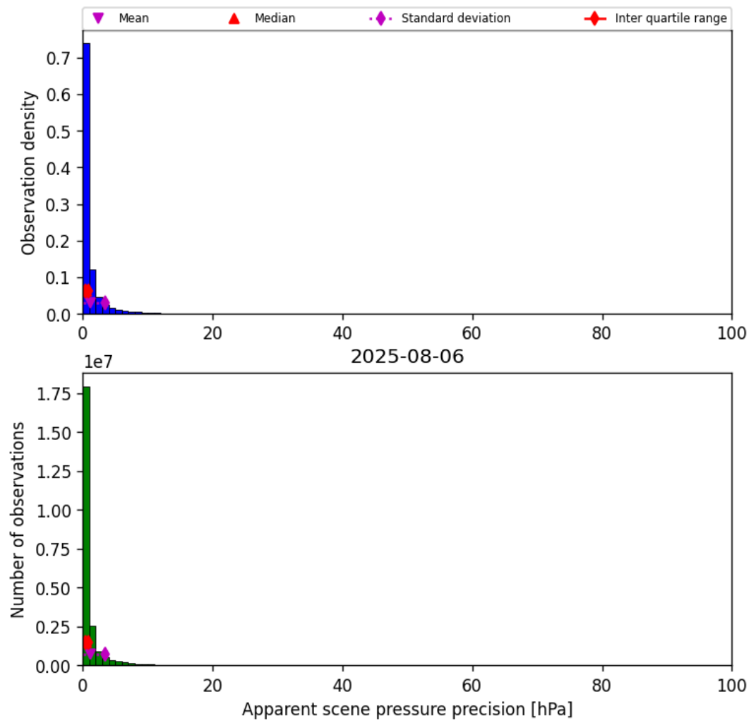
Figure 35: Histogram of “Apparent scene pressure precision” for 2025-08-06 to 2025-08-07
