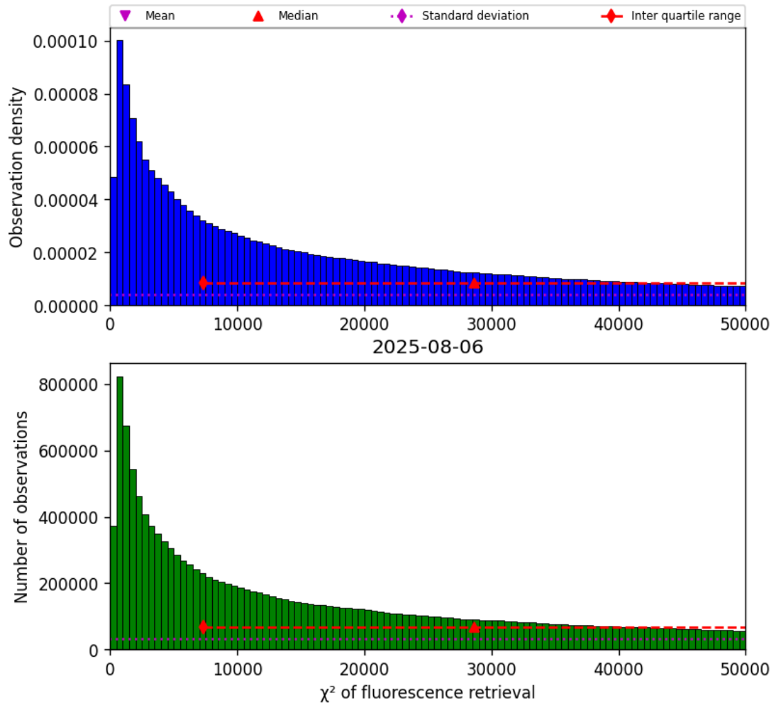
Figure 40: Histogram of “ \chi^2 of fluorescence retrieval” for 2025-08-06 to 2025-08-07
