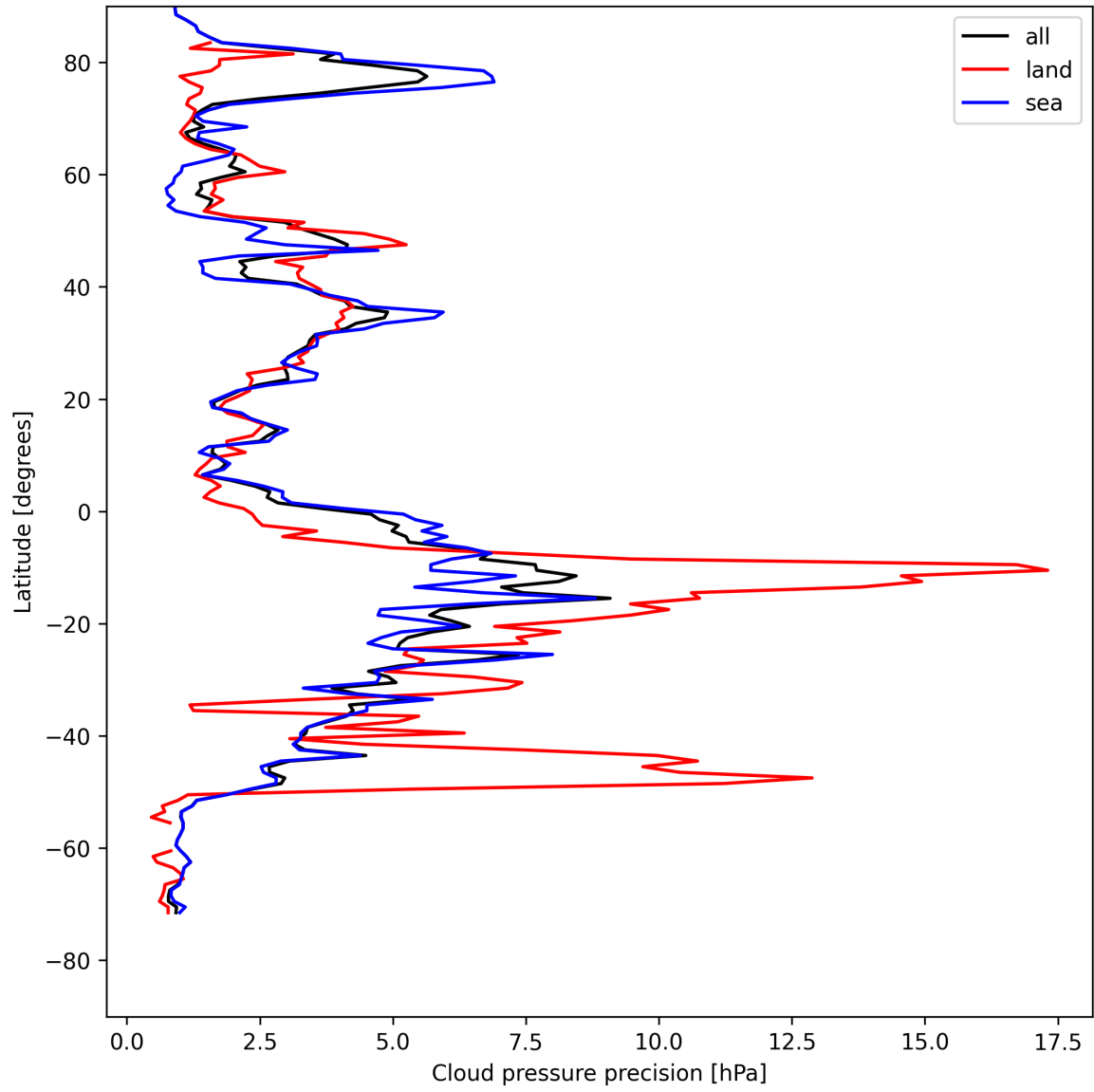
Figure 12: Zonal average of "Cloud pressure precision" for 2025-08-06 to 2025-08-07.
