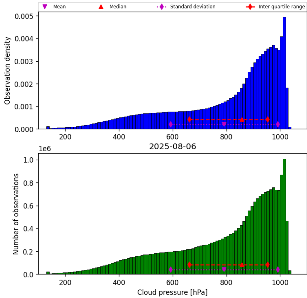
Figure 28: Histogram of “Cloud pressure” for 2025-08-06 to 2025-08-07
