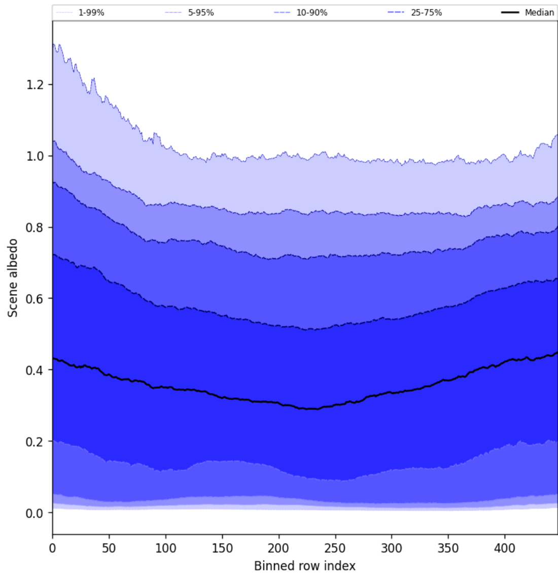
Figure 49: Along track statistics of “Scene albedo” for 2025-08-06 to 2025-08-07
