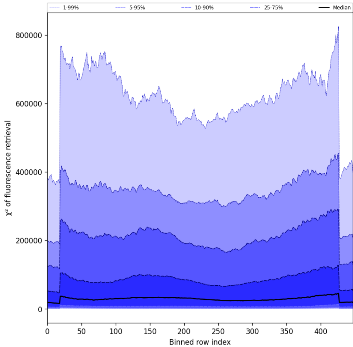
Figure 57: Along track statistics of “ \chi^2 of fluorescence retrieval” for 2025-08-06 to 2025-08-07
