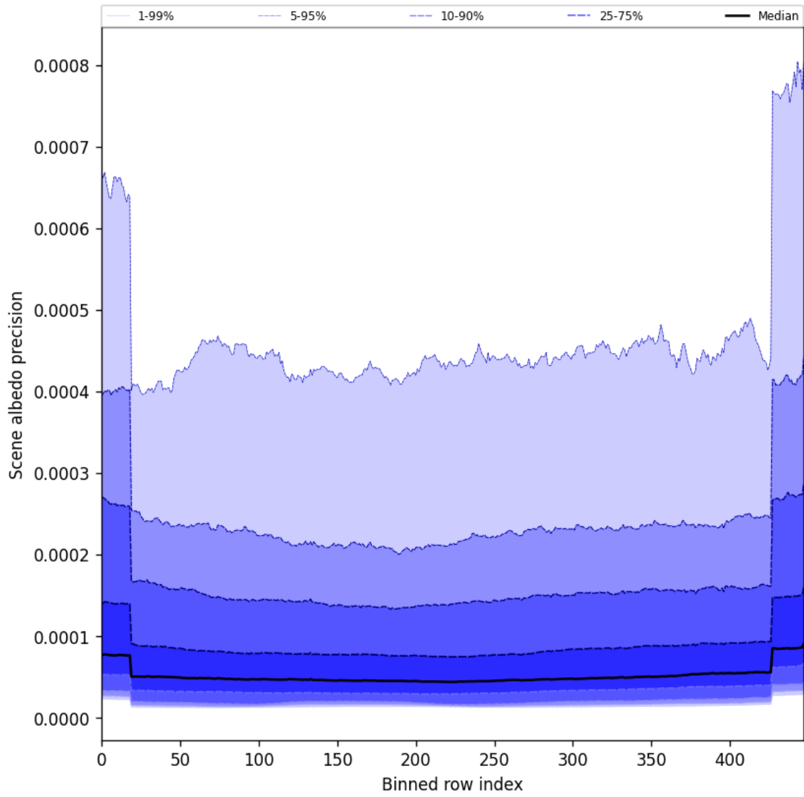
Figure 50: Along track statistics of “Scene albedo precision” for 2025-08-06 to 2025-08-07
