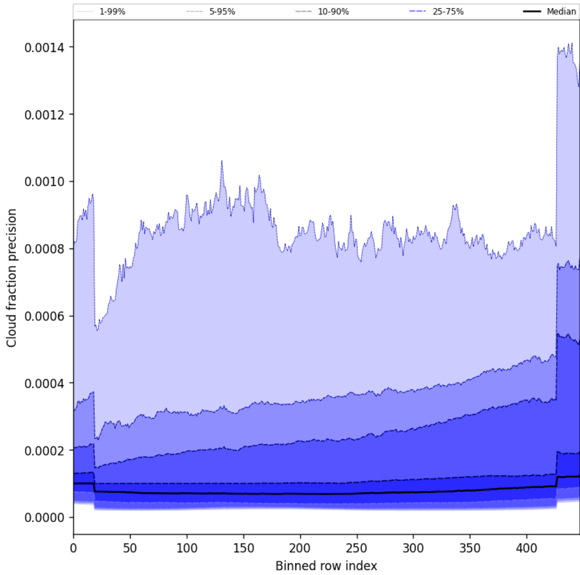
Figure 48: Along track statistics of “Cloud fraction precision” for 2025-08-06 to 2025-08-07
