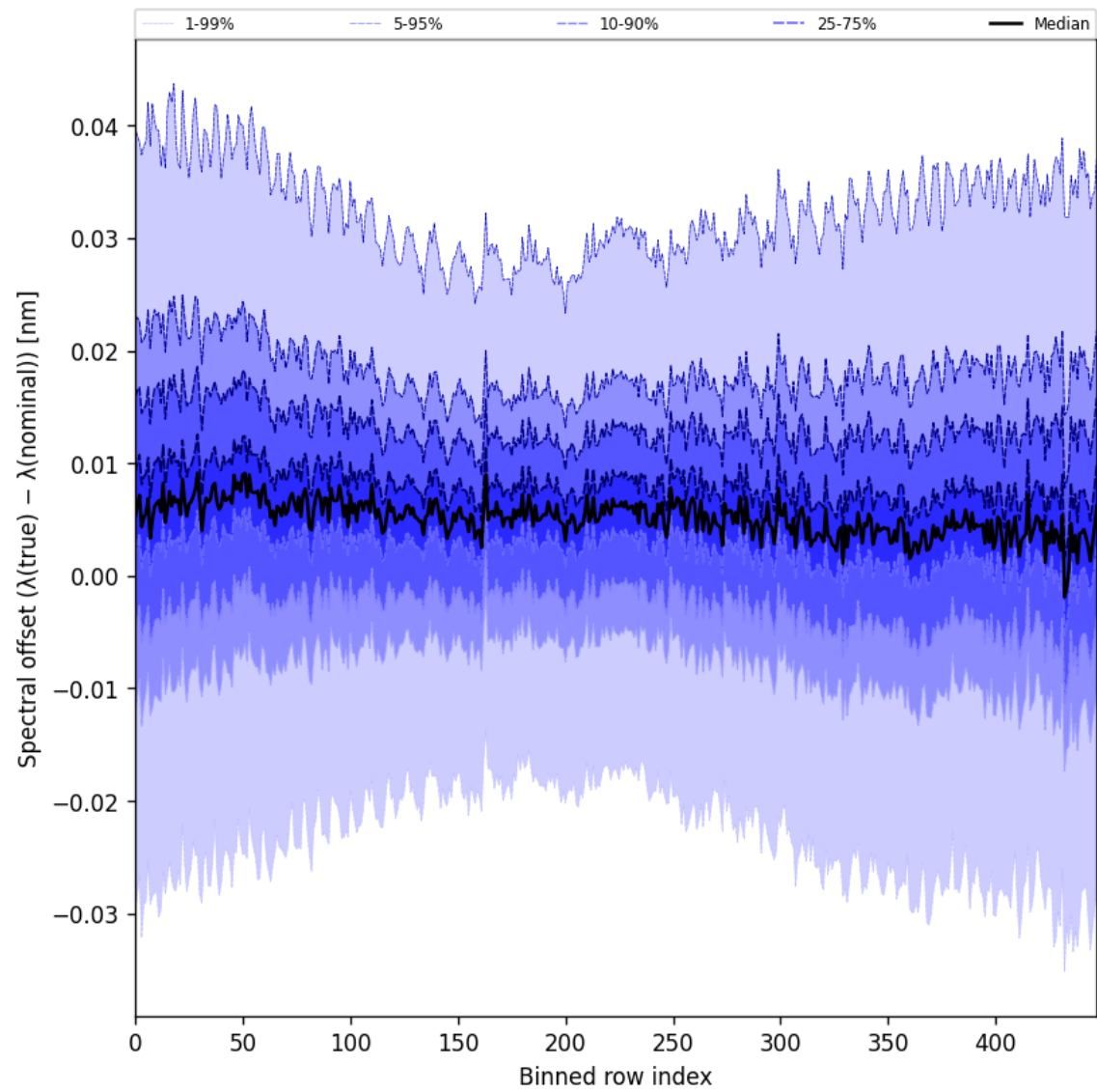
Figure 60: Along track statistics of “Spectral offset ( \lambda_{\text{true}} - \lambda_{\text{nominal}} )” for 2025-08-06 to 2025-08-07
