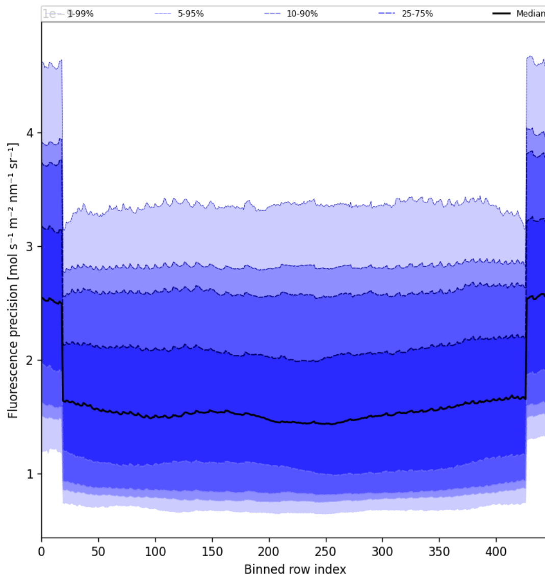
Figure 56: Along track statistics of “Fluorescence precision” for 2025-08-06 to 2025-08-07
