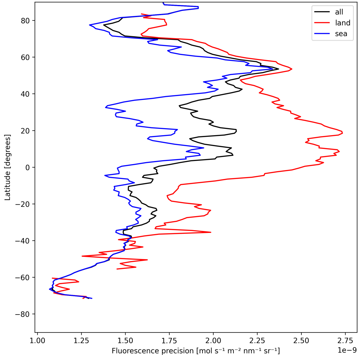
Figure 22: Zonal average of "Fluorescence precision" for 2025-08-06 to 2025-08-07.
