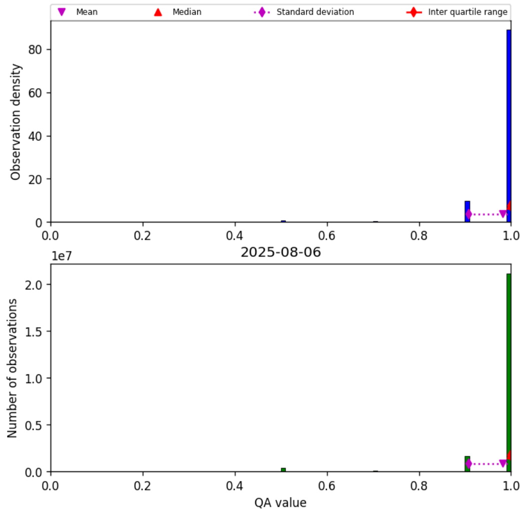
Figure 27: Histogram of “QA value” for 2025-08-06 to 2025-08-07
