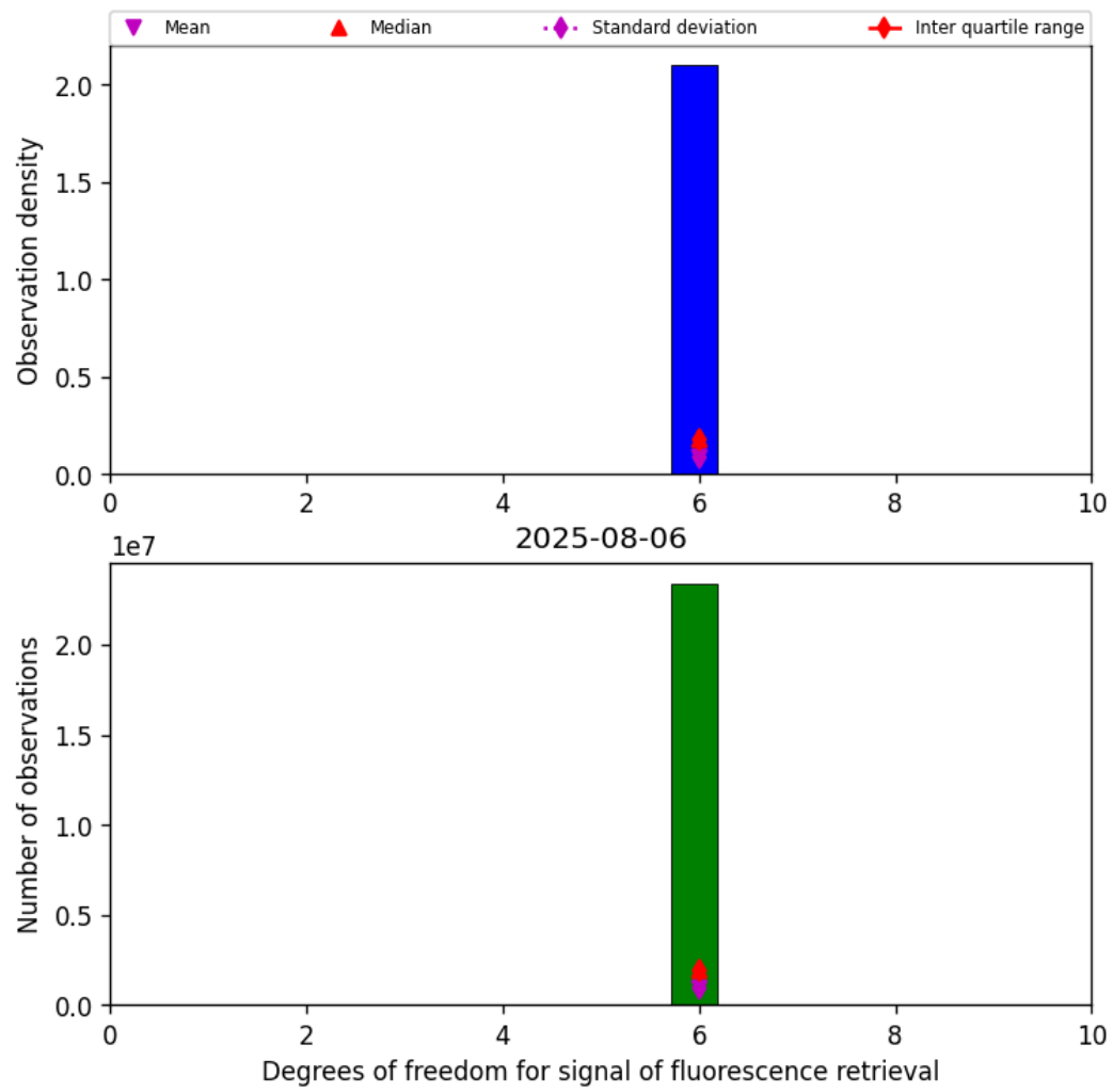
Figure 41: Histogram of “Degrees of freedom for signal of fluorescence retrieval” for 2025-08-06 to 2025-08-07
