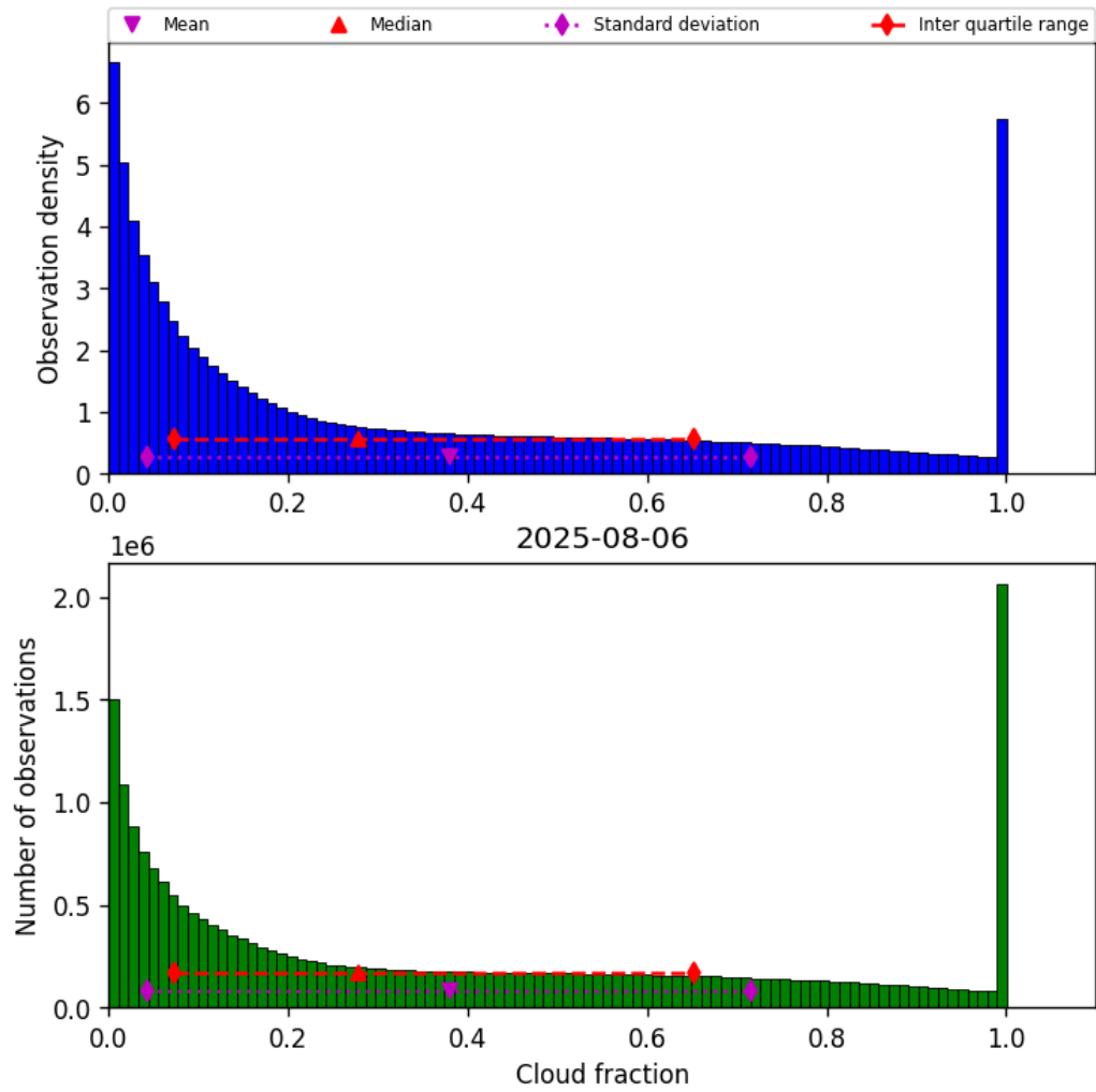
Figure 30: Histogram of “Cloud fraction” for 2025-08-06 to 2025-08-07
