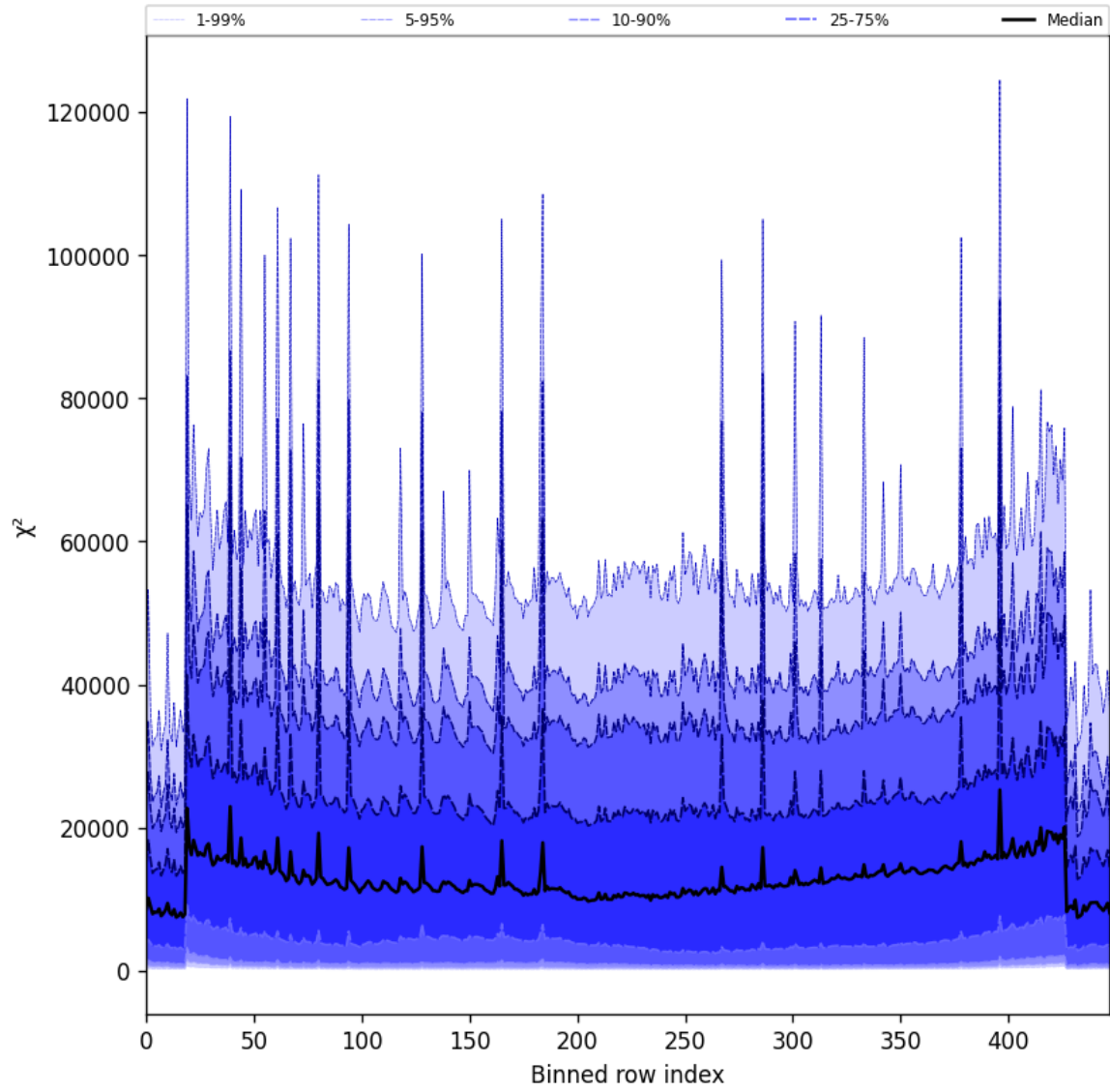
Figure 53: Along track statistics of “ \chi^2 ” for 2025-08-06 to 2025-08-07
