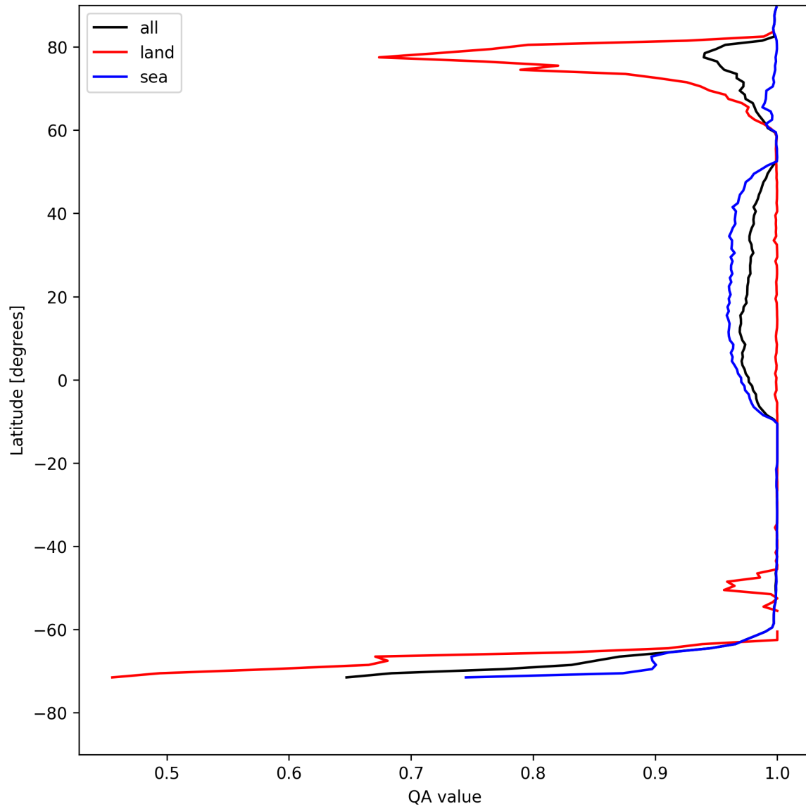
Figure 10: Zonal average of “QA value” for 2025-08-06 to 2025-08-07.
