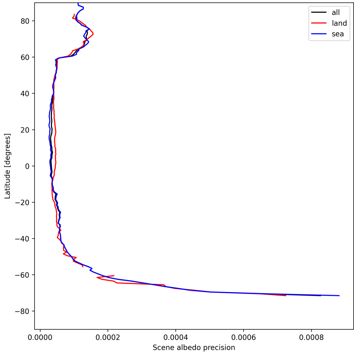
Figure 16: Zonal average of “Scene albedo precision” for 2025-08-06 to 2025-08-07.
