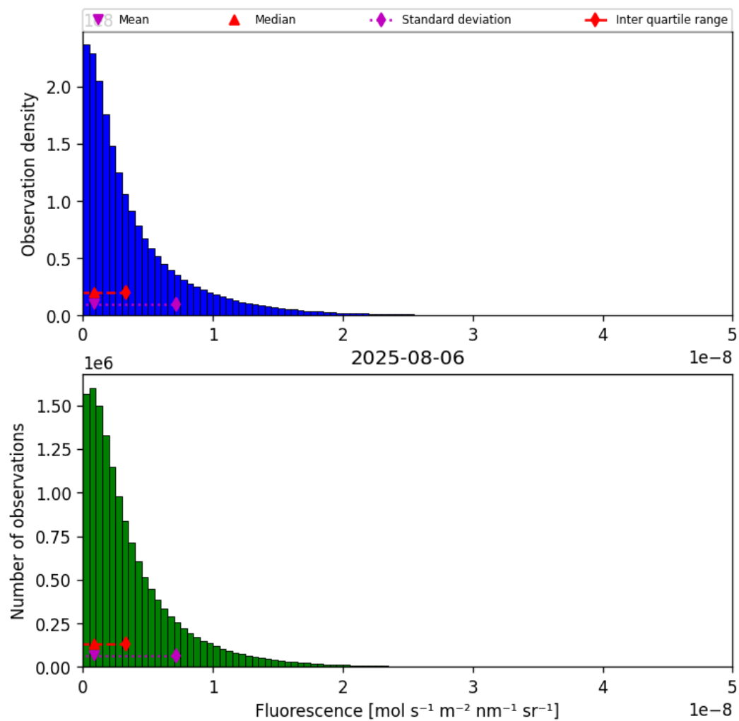
Figure 38: Histogram of “Fluorescence” for 2025-08-06 to 2025-08-07
