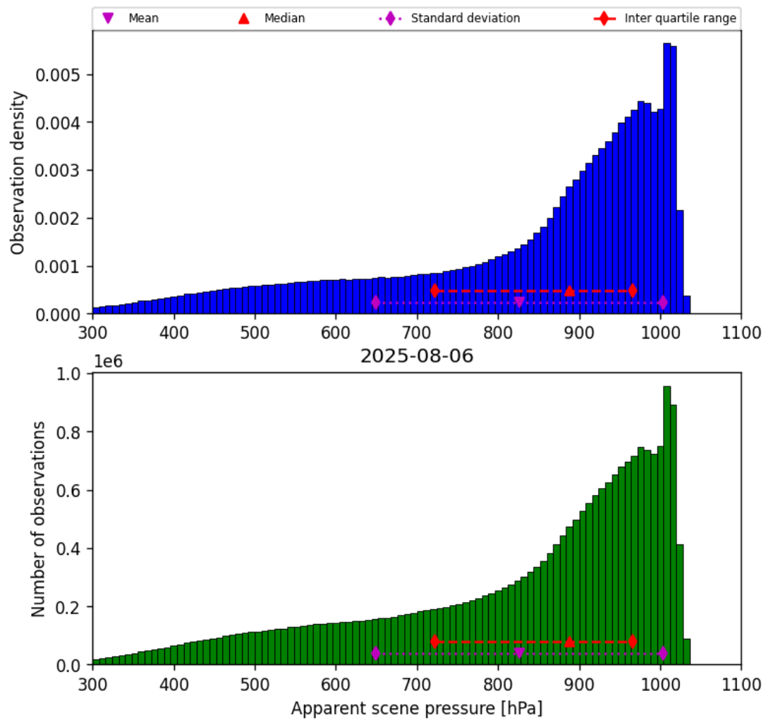
Figure 34: Histogram of “Apparent scene pressure” for 2025-08-06 to 2025-08-07
