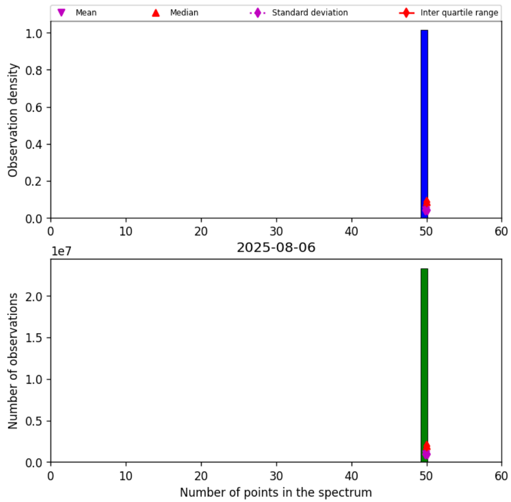
Figure 42: Histogram of "Number of points in the spectrum" for 2025-08-06 to 2025-08-07
