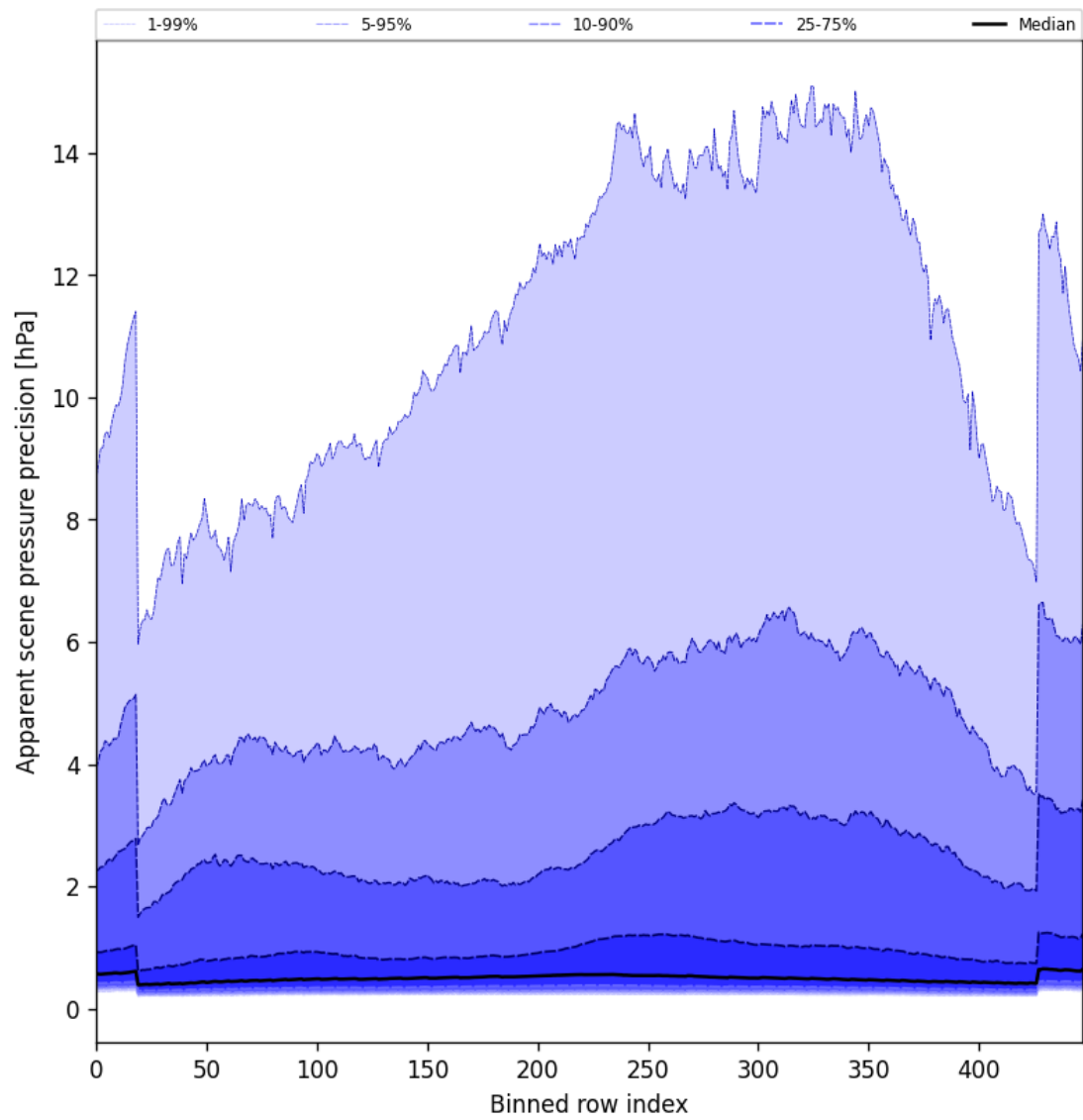
Figure 52: Along track statistics of “Apparent scene pressure precision” for 2025-08-06 to 2025-08-07
