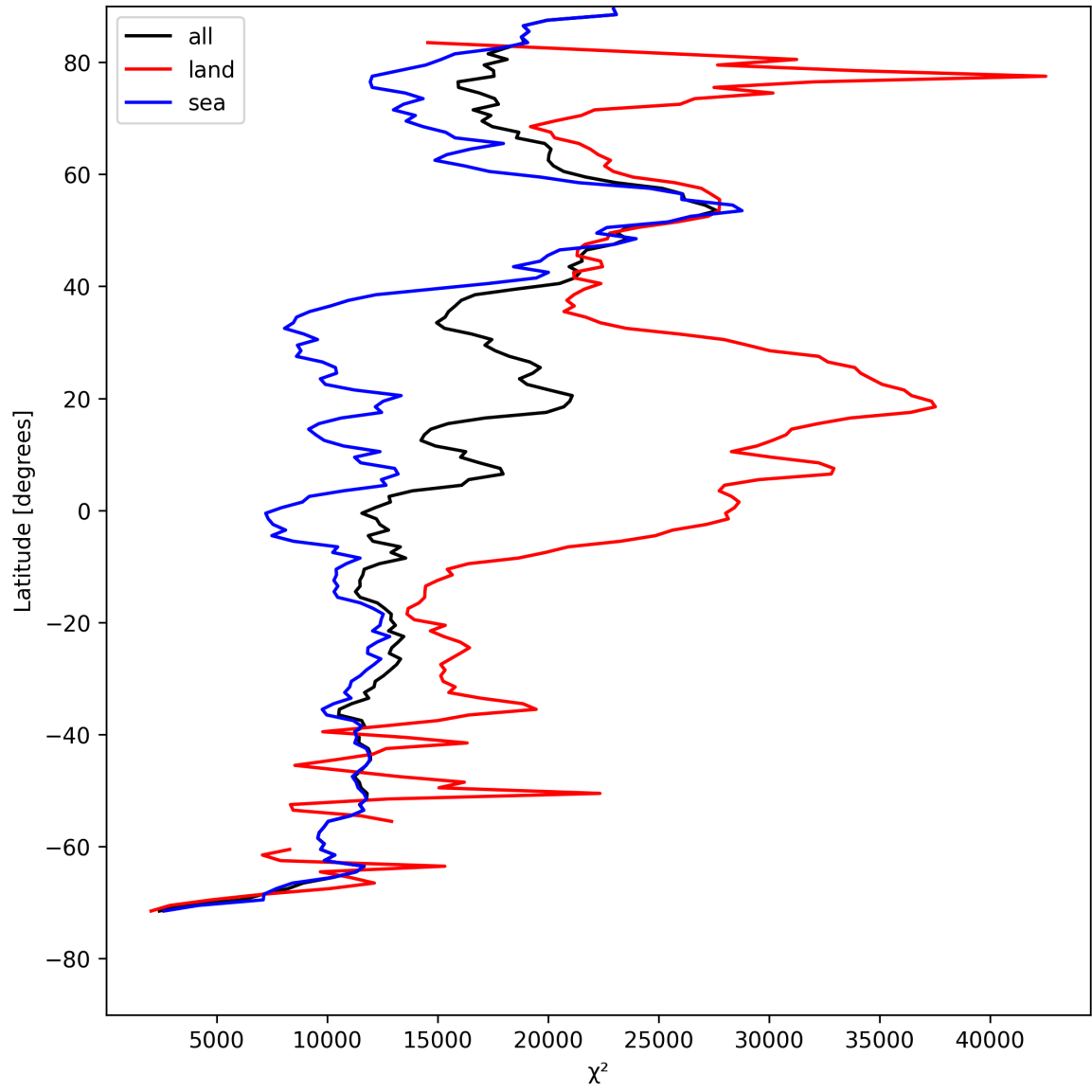
Figure 19: Zonal average of “ \chi^2 ” for 2025-08-06 to 2025-08-07.
