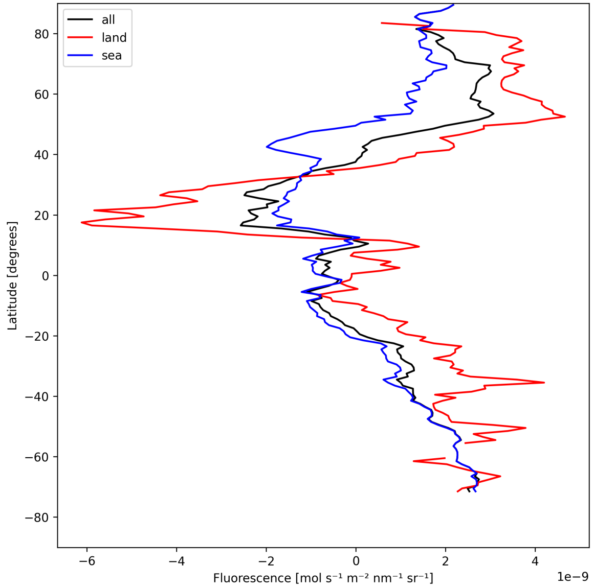
Figure 21: Zonal average of “Fluorescence” for 2025-08-06 to 2025-08-07.
