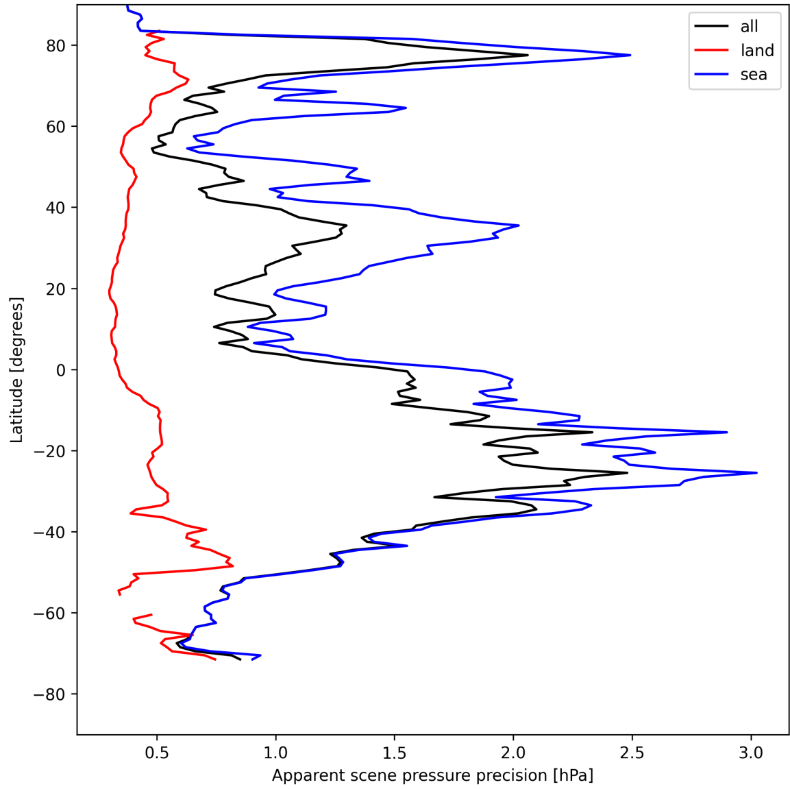
Figure 18: Zonal average of “Apparent scene pressure precision” for 2025-08-06 to 2025-08-07.
