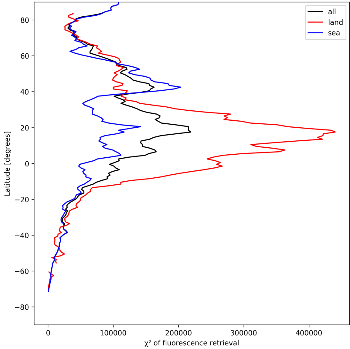
Figure 23: Zonal average of “ \chi^2 of fluorescence retrieval” for 2025-08-06 to 2025-08-07.
