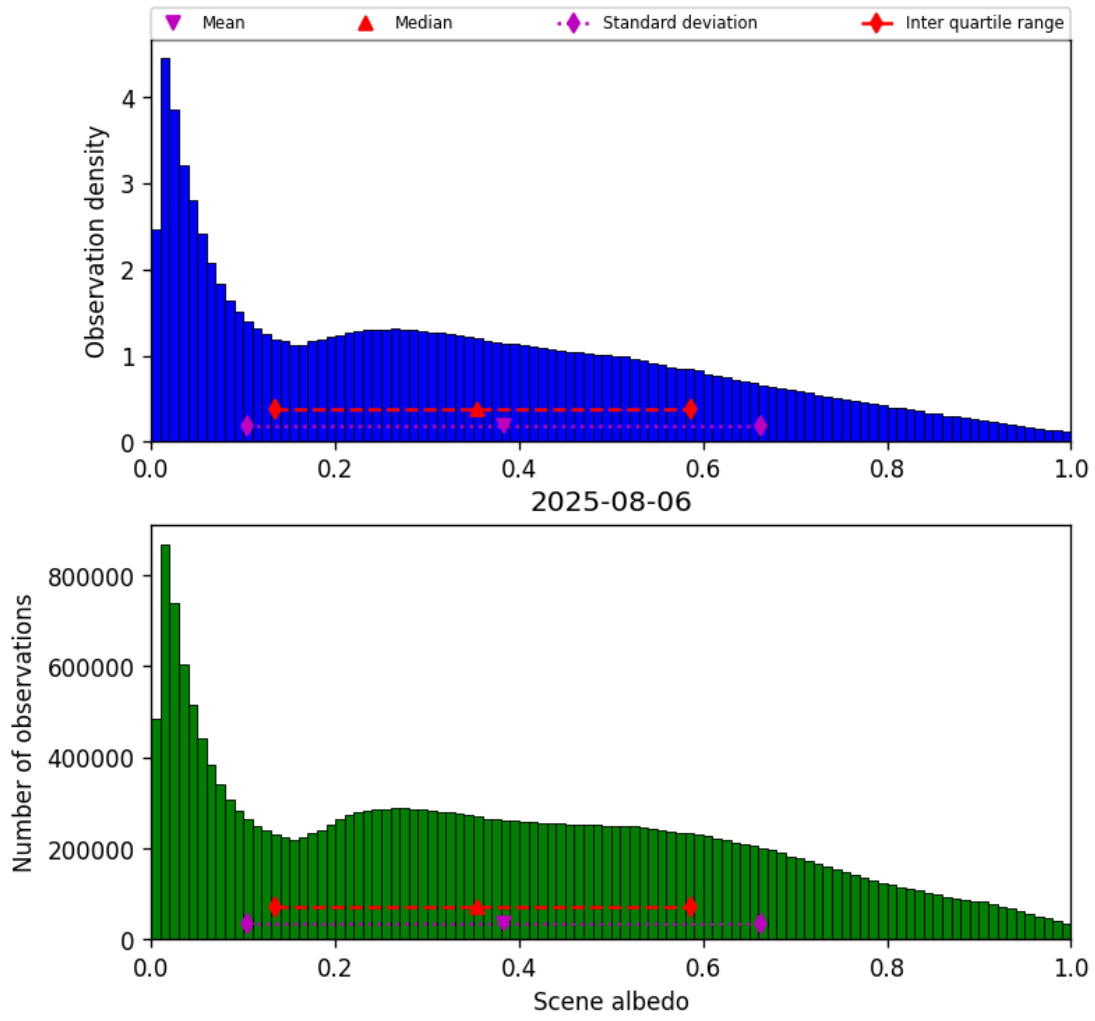
Figure 32: Histogram of “Scene albedo” for 2025-08-06 to 2025-08-07
