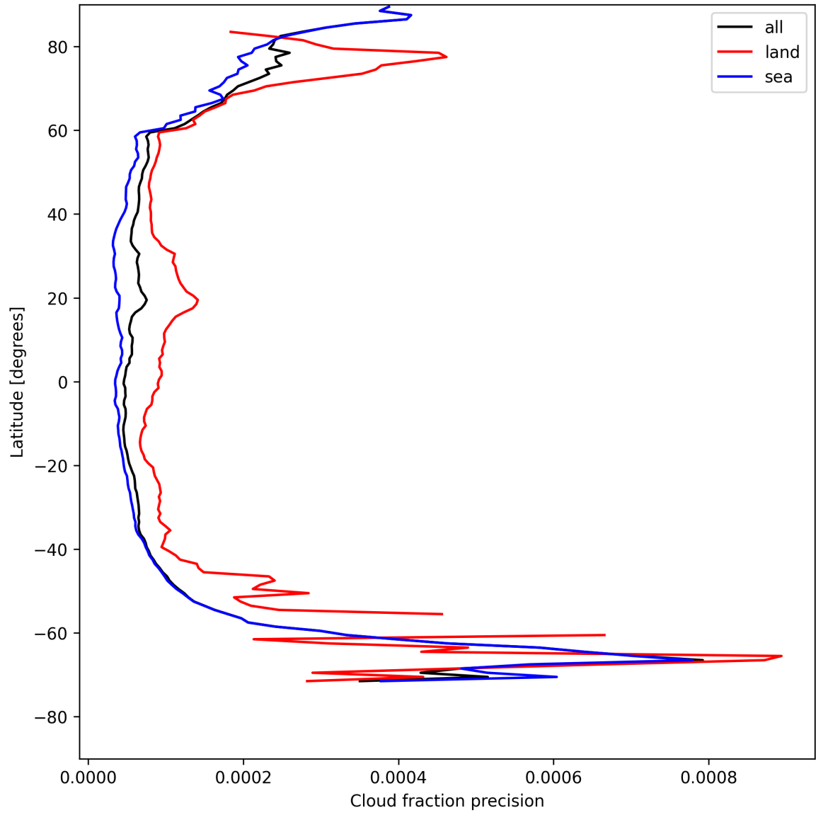
Figure 14: Zonal average of “Cloud fraction precision” for 2025-08-06 to 2025-08-07.
