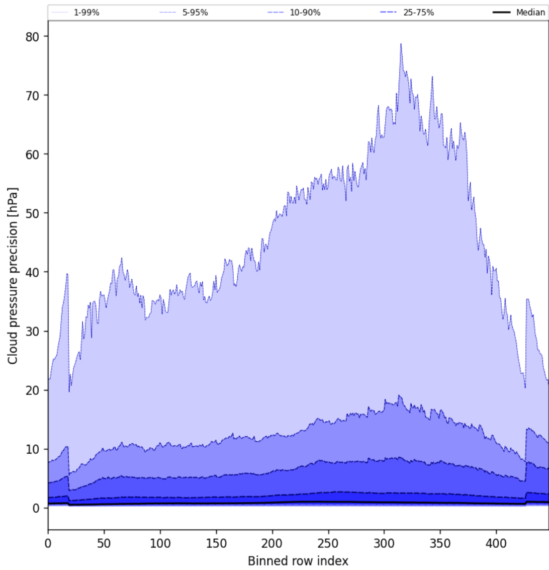
Figure 46: Along track statistics of “Cloud pressure precision” for 2025-08-06 to 2025-08-07
