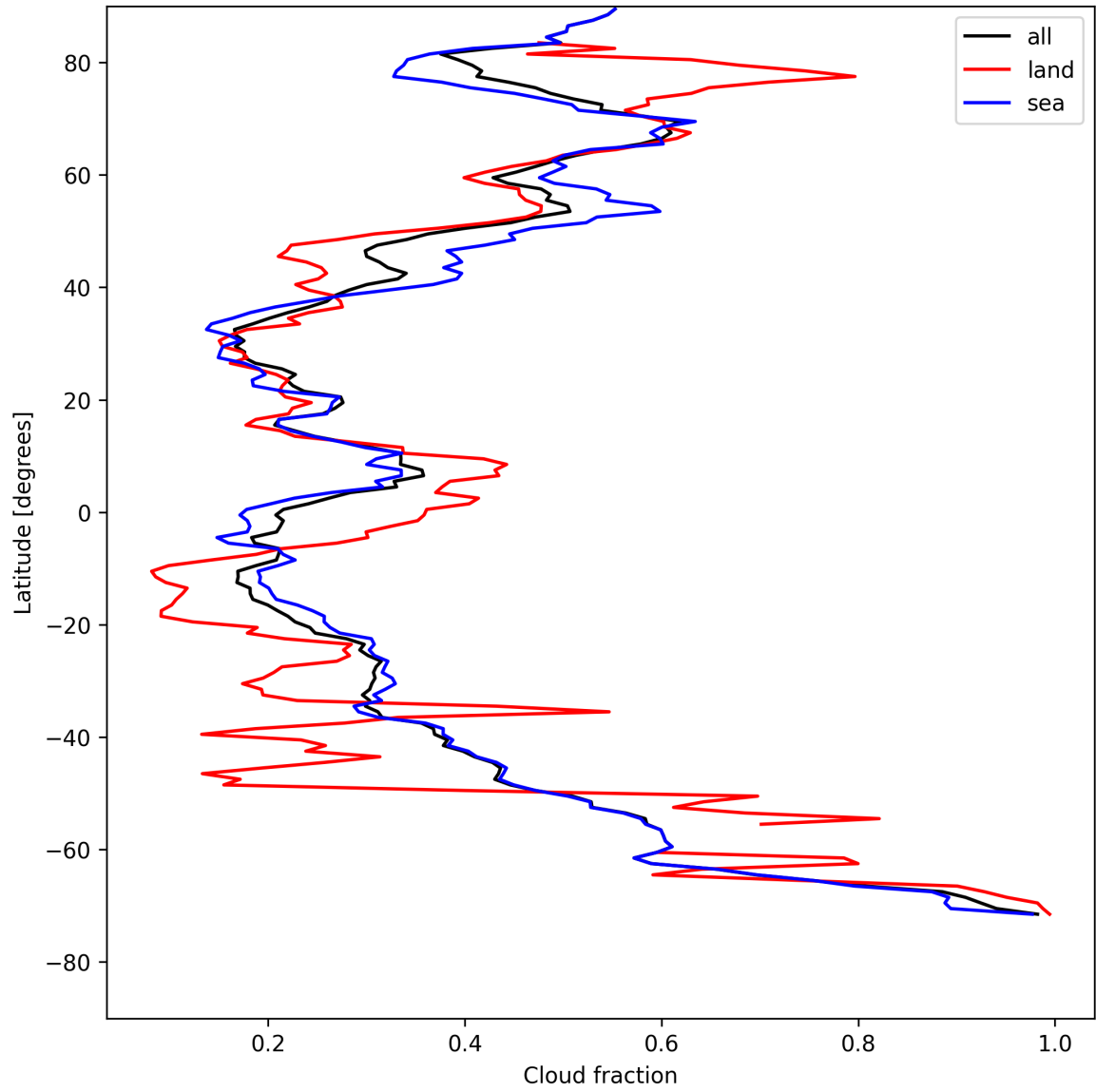
Figure 13: Zonal average of “Cloud fraction” for 2025-08-06 to 2025-08-07.
