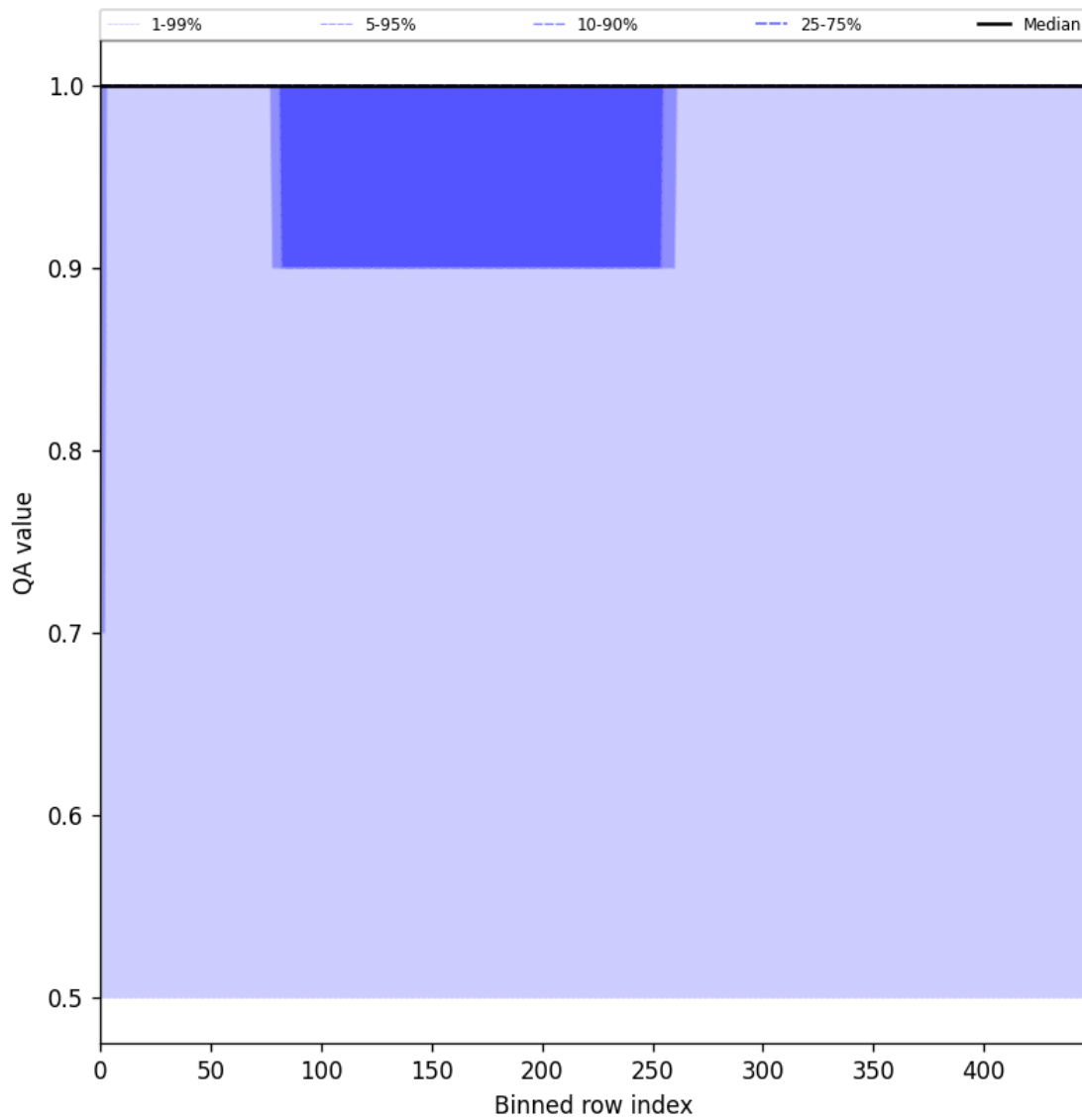
Figure 44: Along track statistics of “QA value” for 2025-08-06 to 2025-08-07
