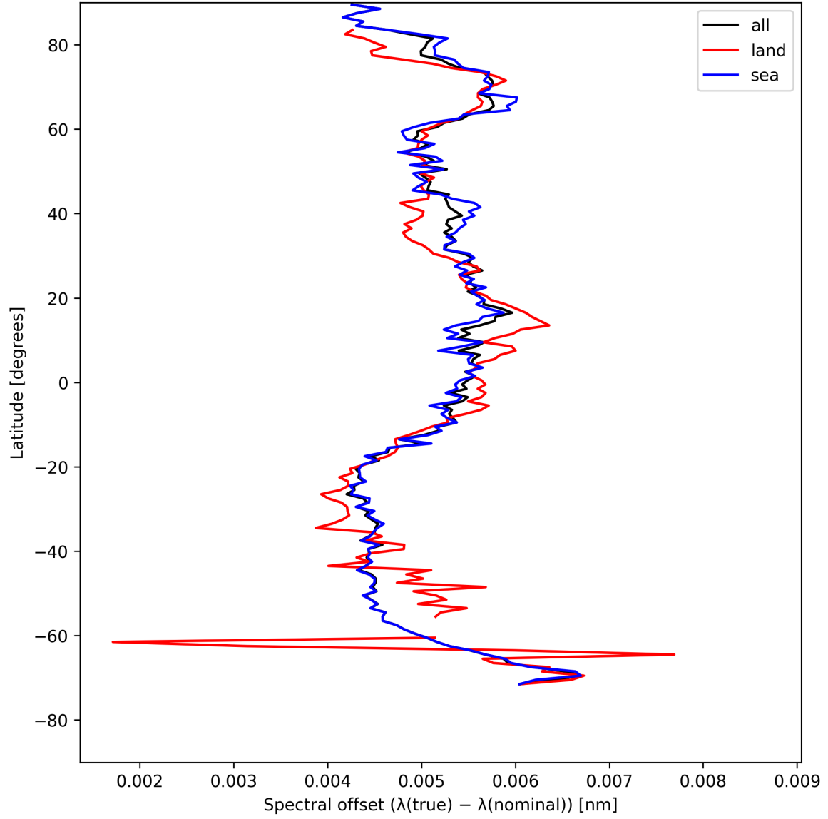
Figure 26: Zonal average of “Spectral offset ( \lambda_{\text{true}} - \lambda_{\text{nominal}} )” for 2025-08-06 to 2025-08-07.
