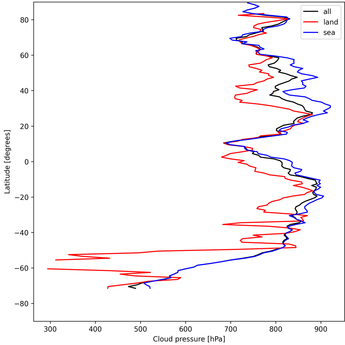
Figure 11: Zonal average of “Cloud pressure” for 2025-08-06 to 2025-08-07.
