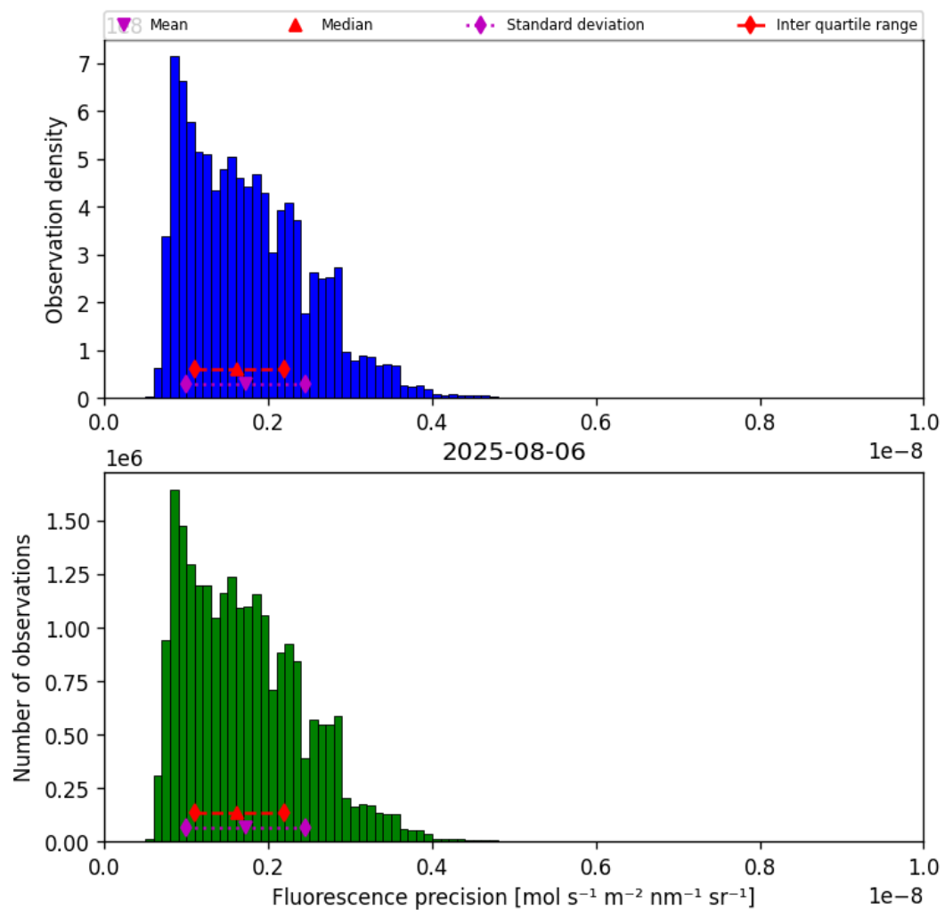
Figure 39: Histogram of “Fluorescence precision” for 2025-08-06 to 2025-08-07
