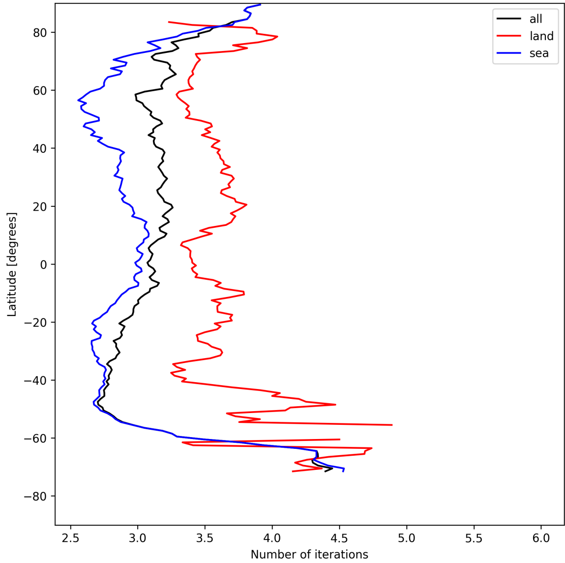
Figure 20: Zonal average of “Number of iterations” for 2025-08-06 to 2025-08-07.
