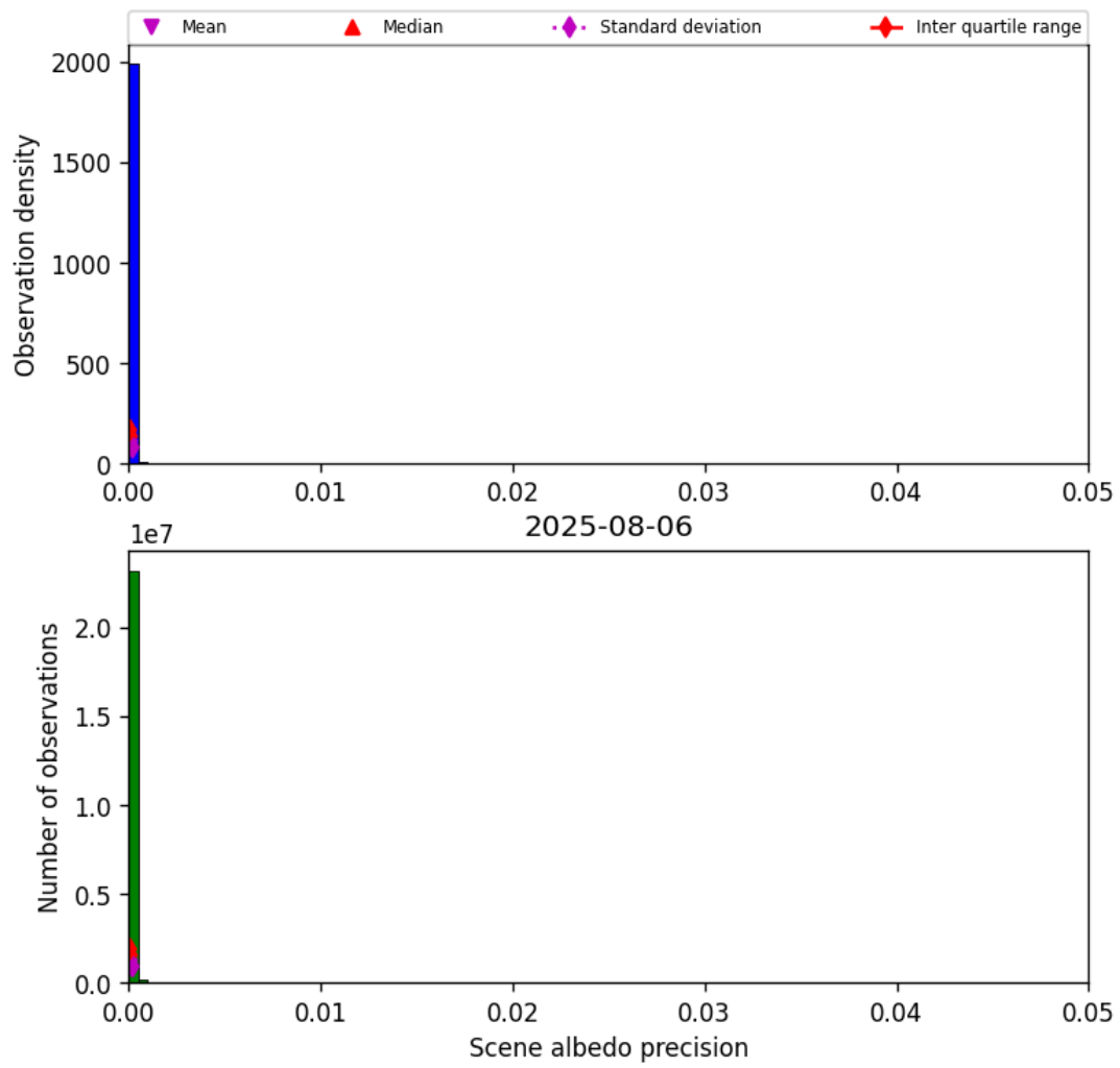
Figure 33: Histogram of “Scene albedo precision” for 2025-08-06 to 2025-08-07
