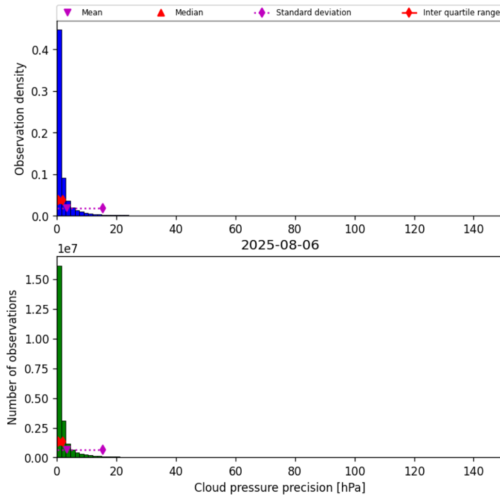
Figure 29: Histogram of “Cloud pressure precision” for 2025-08-06 to 2025-08-07
