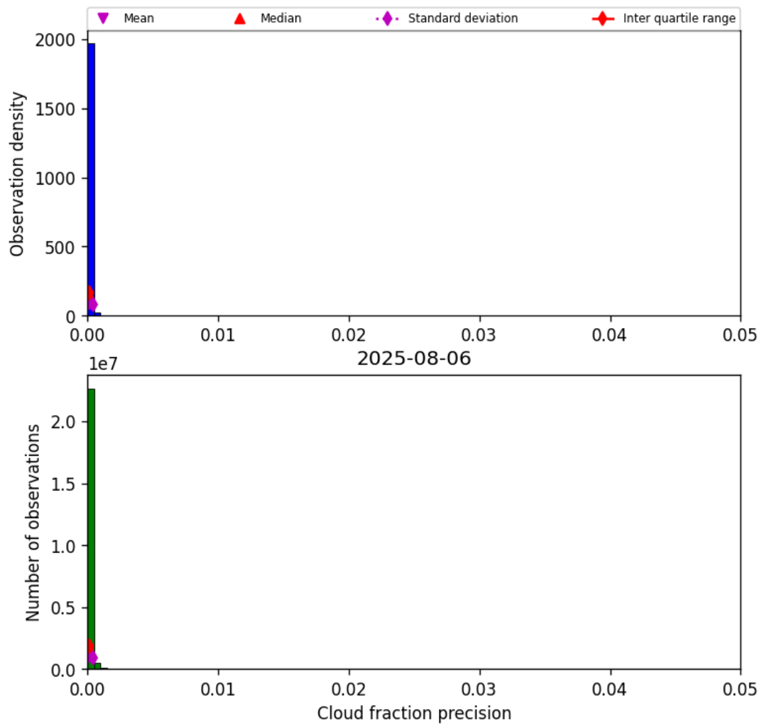
Figure 31: Histogram of “Cloud fraction precision” for 2025-08-06 to 2025-08-07
