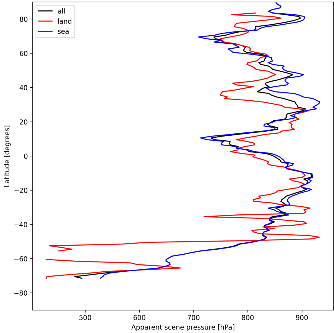
Figure 17: Zonal average of “Apparent scene pressure” for 2025-08-06 to 2025-08-07.
