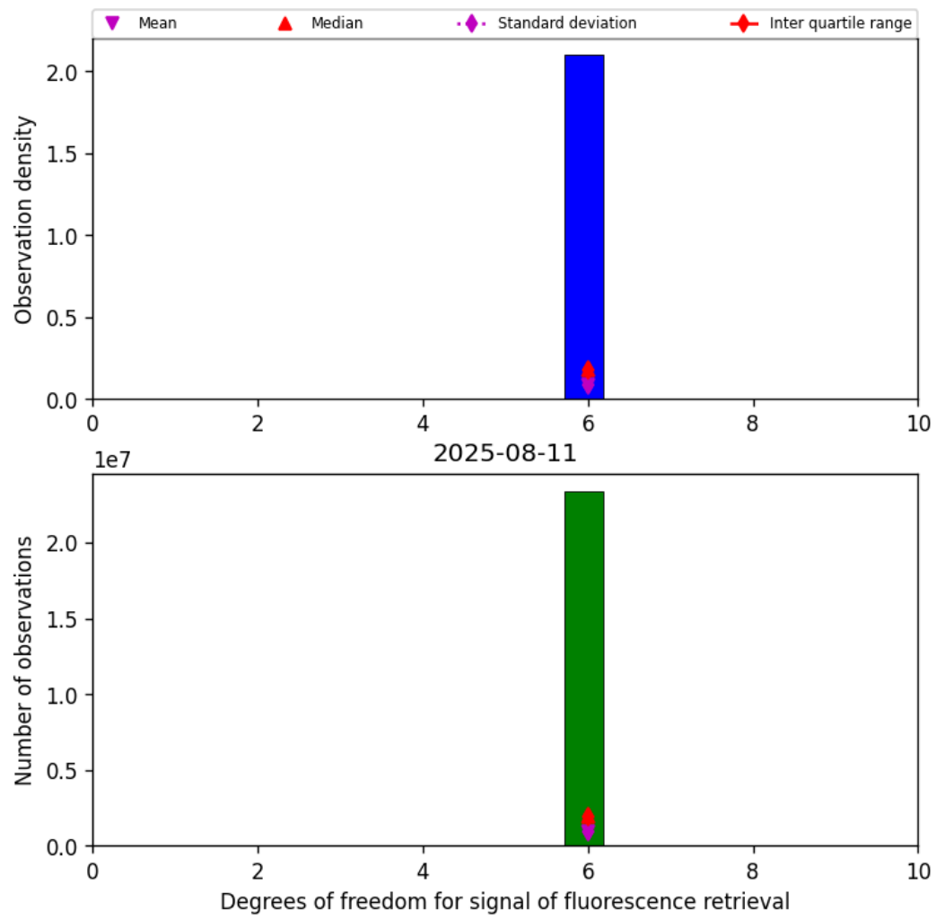
Figure 41: Histogram of “Degrees of freedom for signal of fluorescence retrieval” for 2025-08-11 to 2025-08-12
