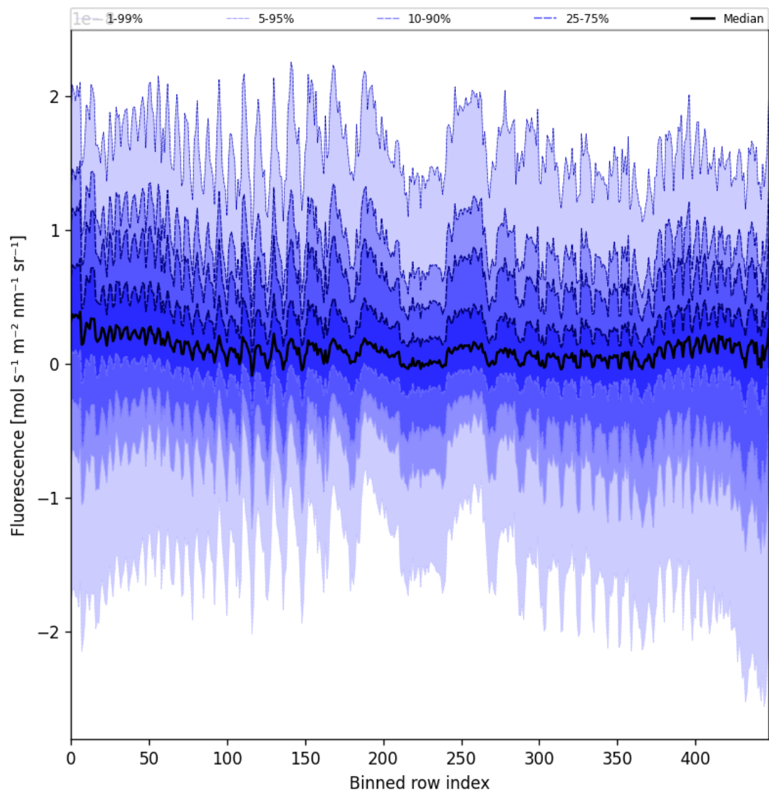
Figure 55: Along track statistics of “Fluorescence” for 2025-08-11 to 2025-08-12
