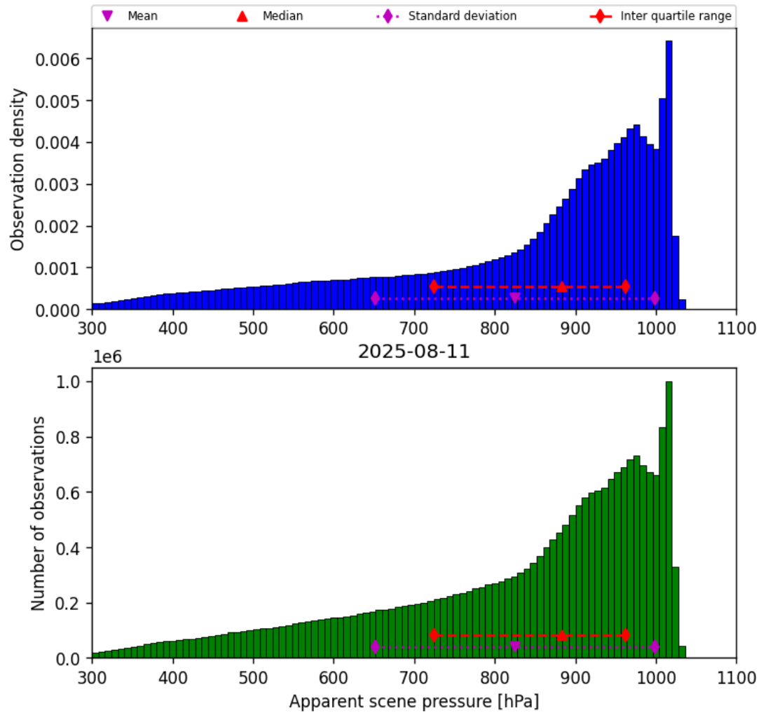
Figure 34: Histogram of “Apparent scene pressure” for 2025-08-11 to 2025-08-12
