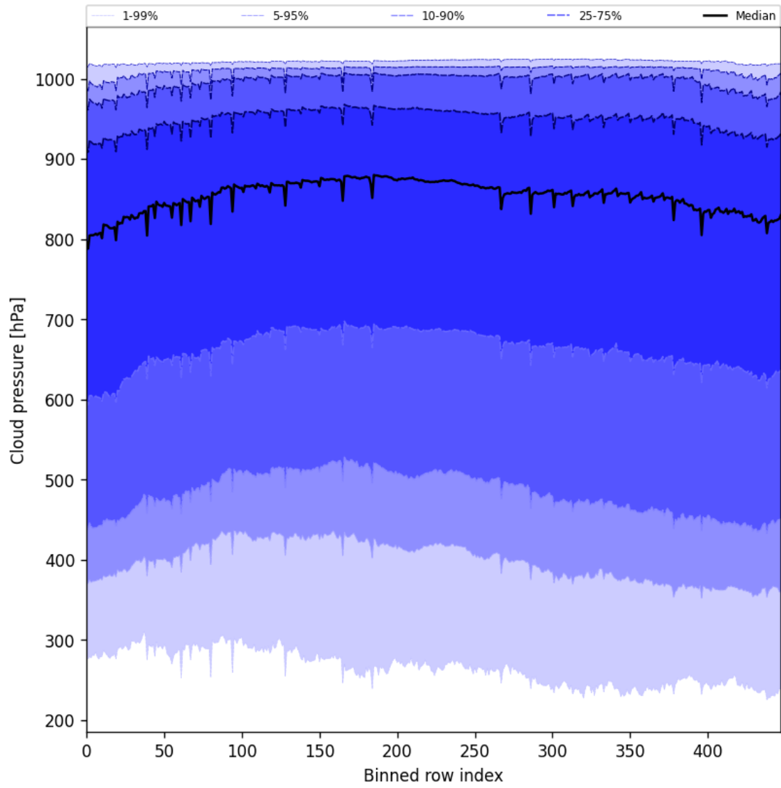
Figure 45: Along track statistics of “Cloud pressure” for 2025-08-11 to 2025-08-12
