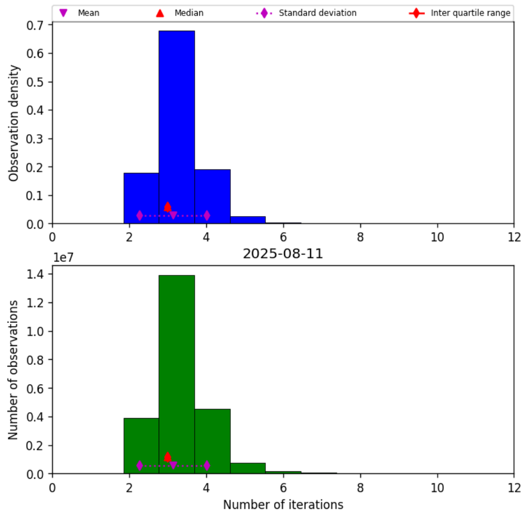
Figure 37: Histogram of “Number of iterations” for 2025-08-11 to 2025-08-12
