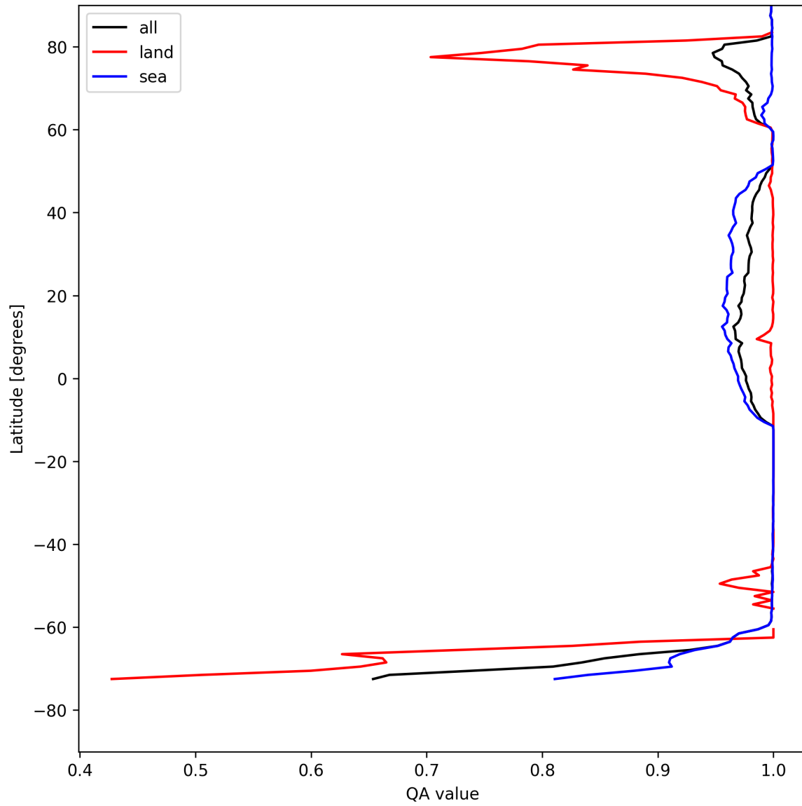
Figure 10: Zonal average of “QA value” for 2025-08-11 to 2025-08-12.
