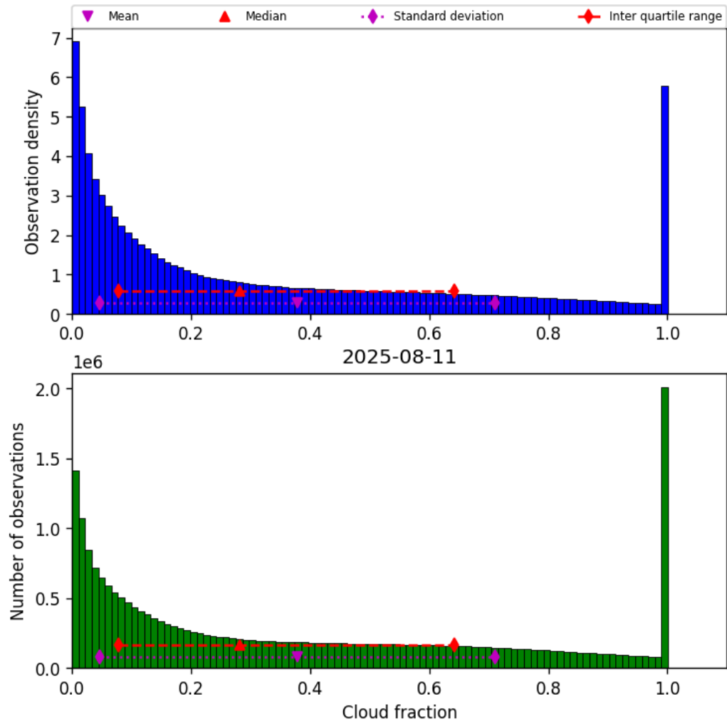
Figure 30: Histogram of “Cloud fraction” for 2025-08-11 to 2025-08-12
