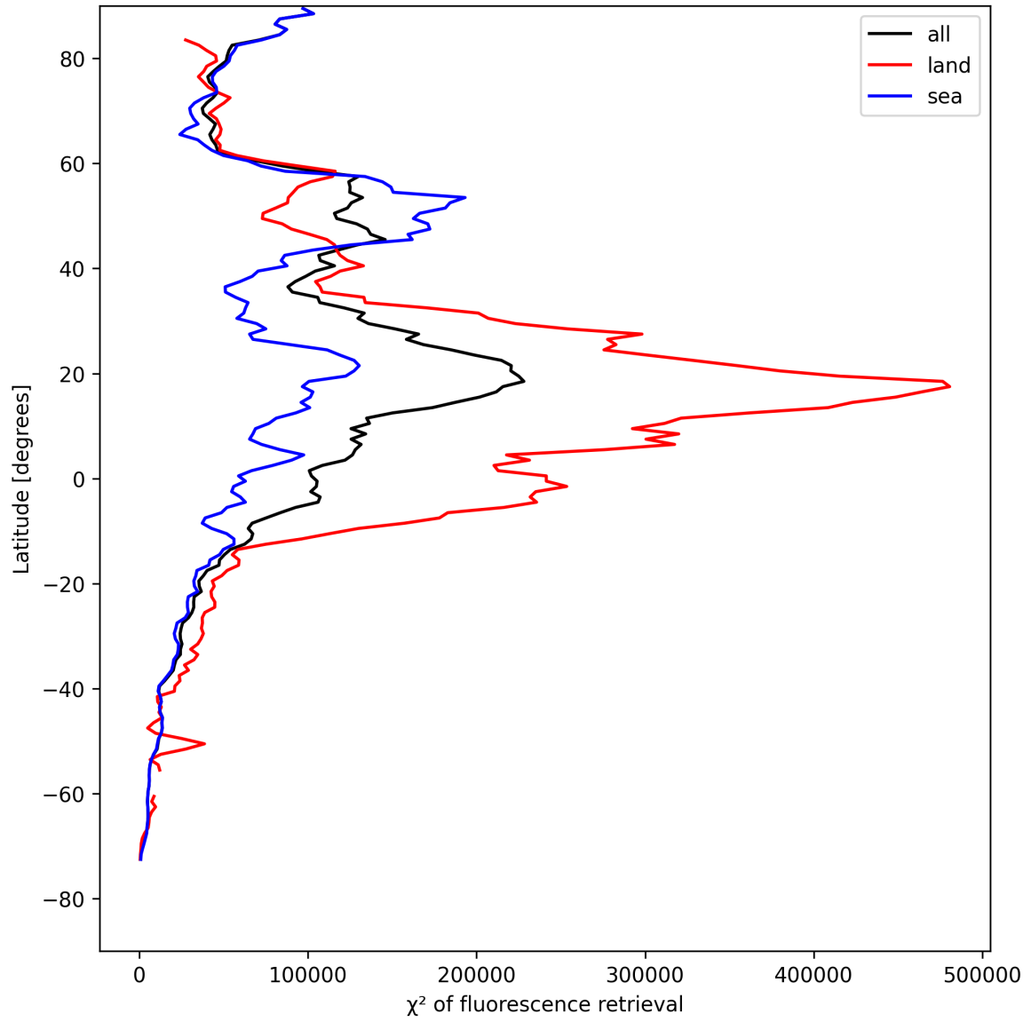
Figure 23: Zonal average of “ \chi^2 of fluorescence retrieval” for 2025-08-11 to 2025-08-12.
