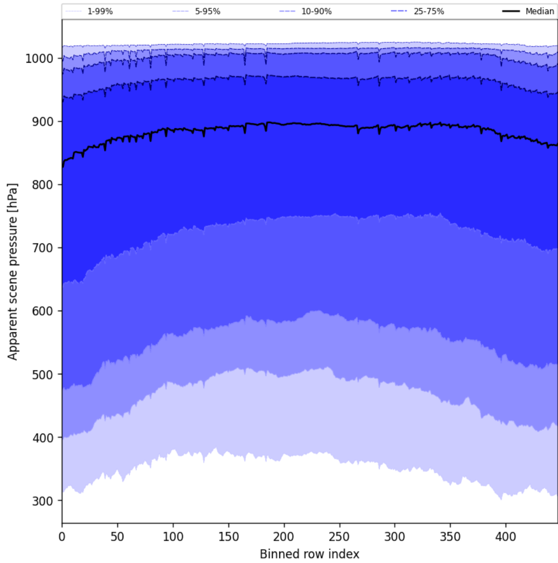
Figure 51: Along track statistics of “Apparent scene pressure” for 2025-08-11 to 2025-08-12
