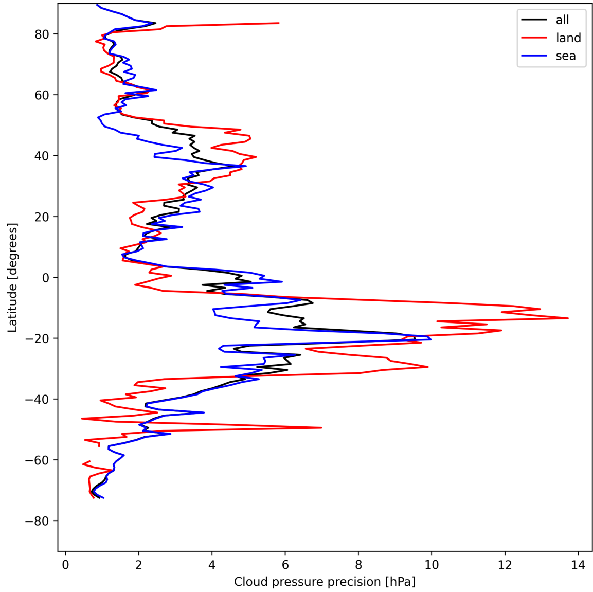
Figure 12: Zonal average of “Cloud pressure precision” for 2025-08-11 to 2025-08-12.
