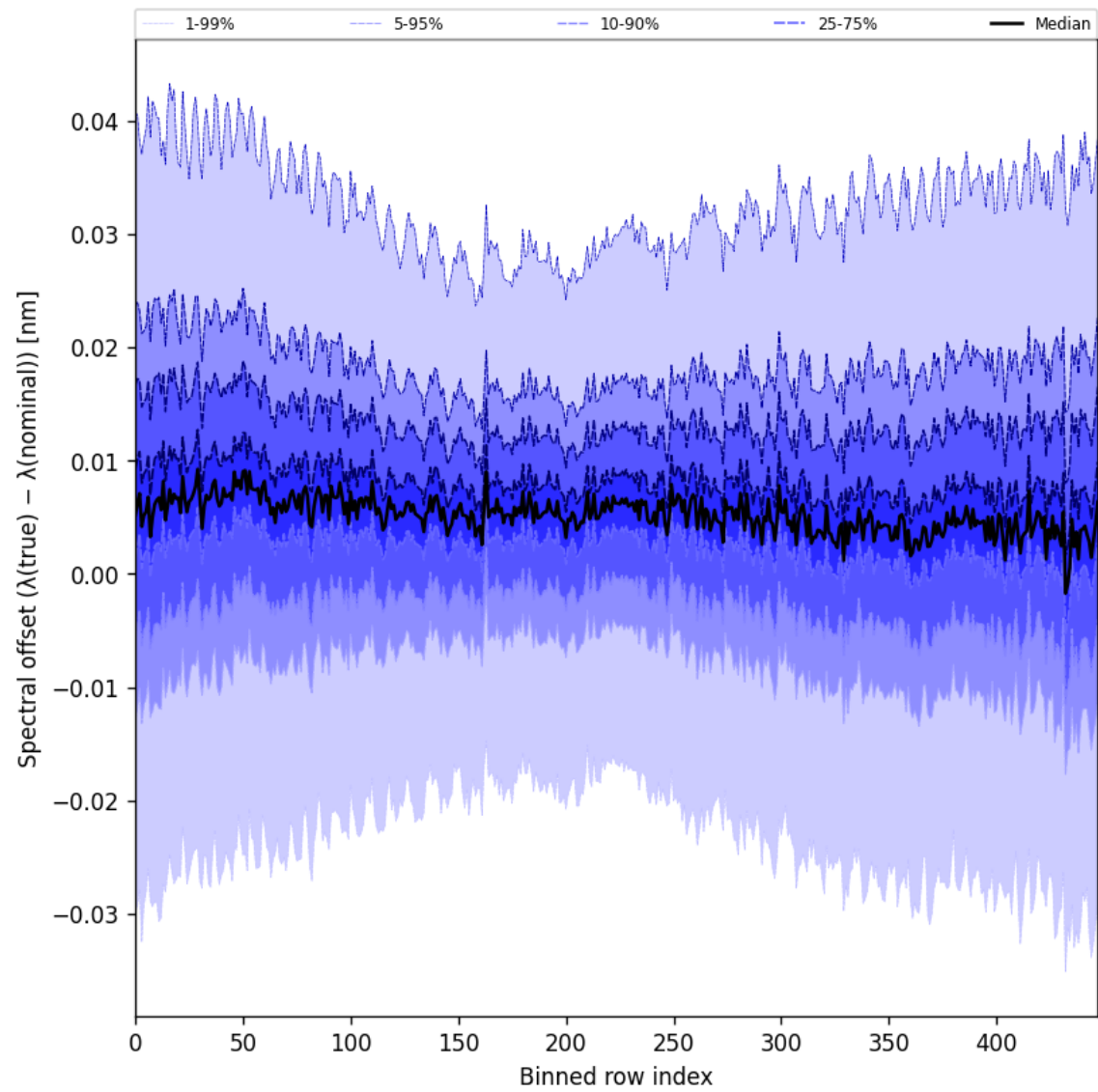
Figure 60: Along track statistics of “Spectral offset ( \lambda_{\text{true}} - \lambda_{\text{nominal}} )” for 2025-08-11 to 2025-08-12
