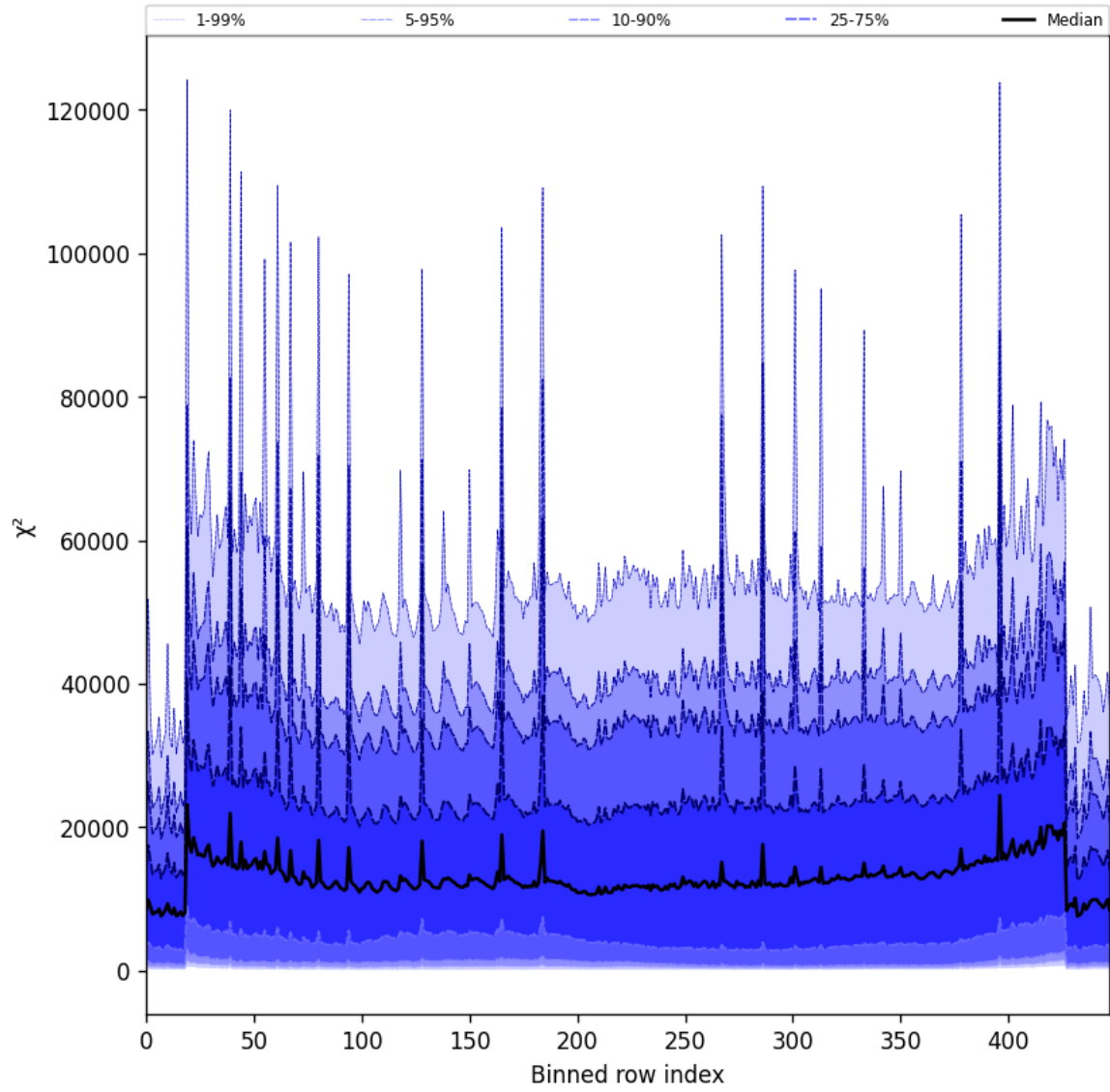
Figure 53: Along track statistics of “ \chi^2 ” for 2025-08-11 to 2025-08-12
