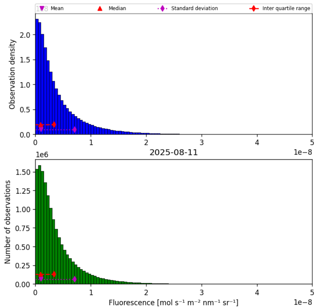
Figure 38: Histogram of “Fluorescence” for 2025-08-11 to 2025-08-12
