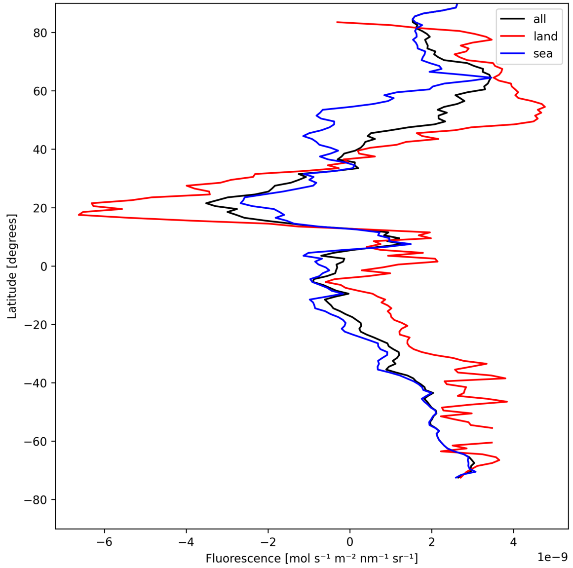
Figure 21: Zonal average of “Fluorescence” for 2025-08-11 to 2025-08-12.
