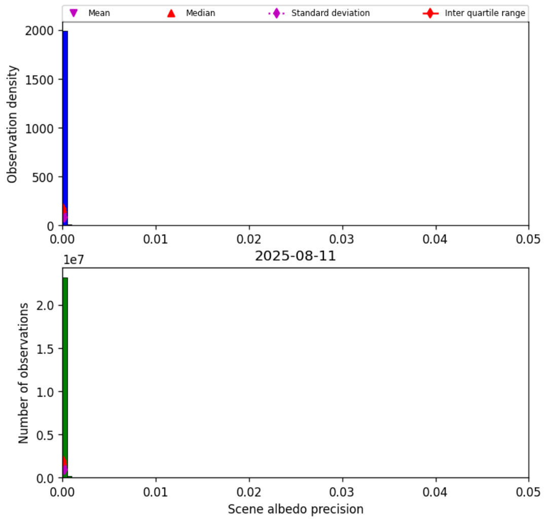
Figure 33: Histogram of “Scene albedo precision” for 2025-08-11 to 2025-08-12
