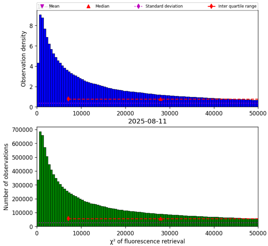
Figure 40: Histogram of “ \chi^2 of fluorescence retrieval” for 2025-08-11 to 2025-08-12
