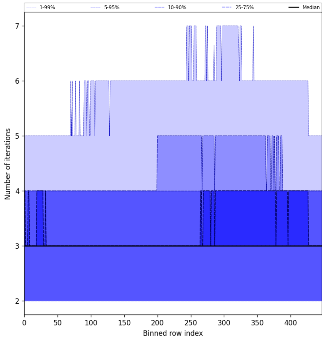
Figure 54: Along track statistics of “Number of iterations” for 2025-08-11 to 2025-08-12
