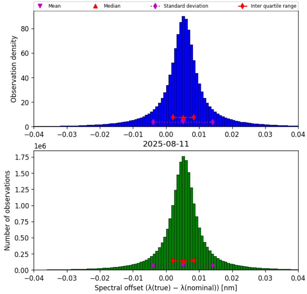
Figure 43: Histogram of “Spectral offset ( \lambda_{\text{true}} - \lambda_{\text{nominal}} )” for 2025-08-11 to 2025-08-12
