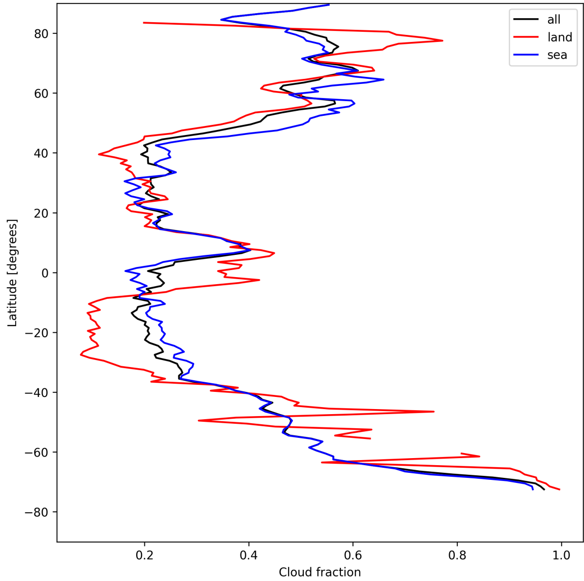
Figure 13: Zonal average of “Cloud fraction” for 2025-08-11 to 2025-08-12.
