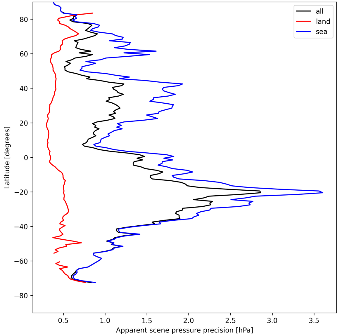
Figure 18: Zonal average of “Apparent scene pressure precision” for 2025-08-11 to 2025-08-12.
