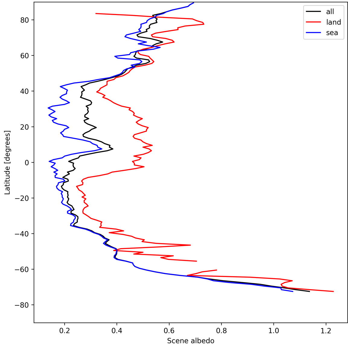
Figure 15: Zonal average of “Scene albedo” for 2025-08-11 to 2025-08-12.
