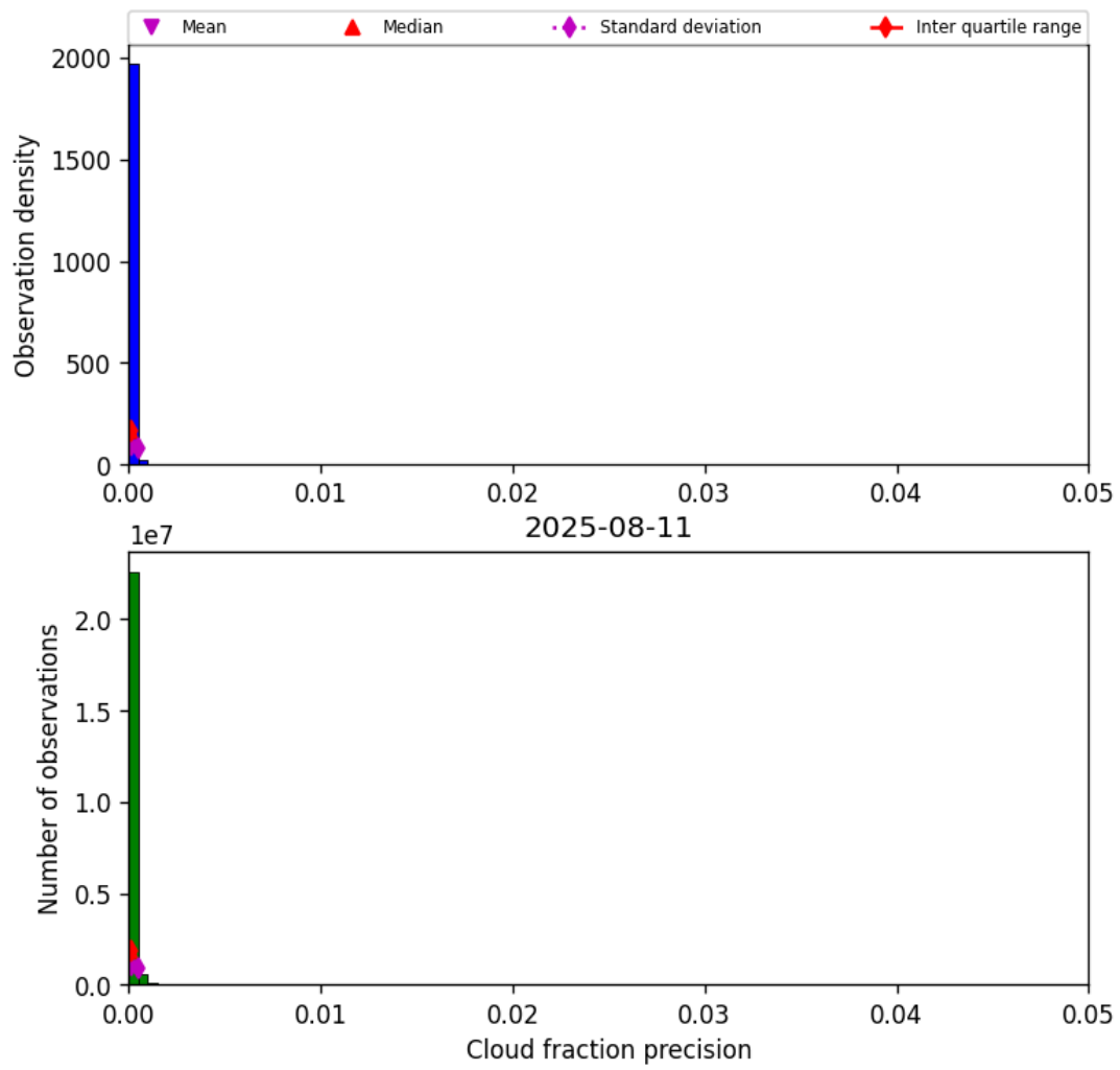
Figure 31: Histogram of “Cloud fraction precision” for 2025-08-11 to 2025-08-12
