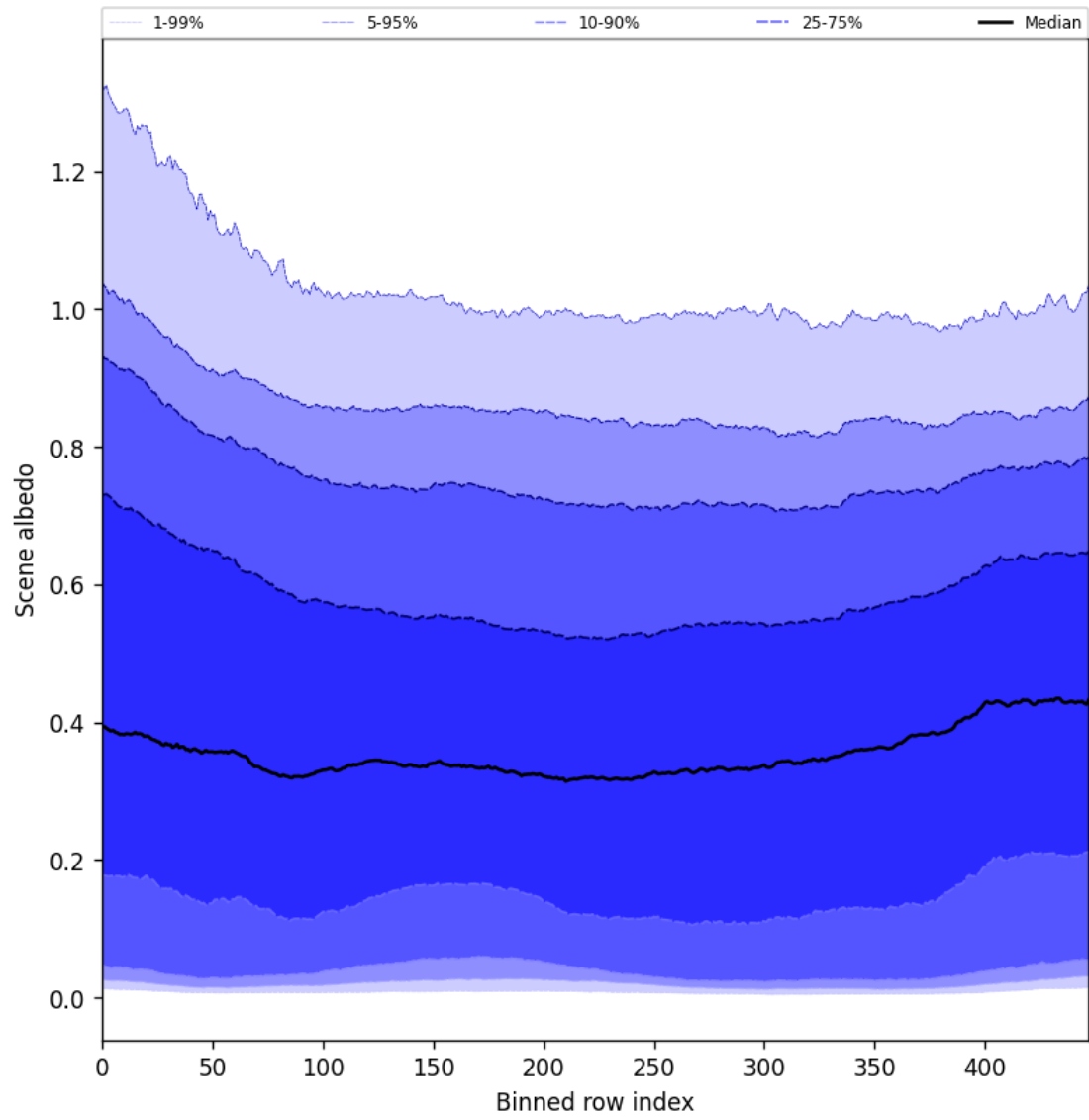
Figure 49: Along track statistics of "Scene albedo" for 2025-08-11 to 2025-08-12
