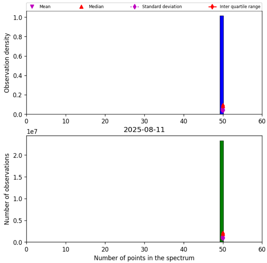
Figure 42: Histogram of “Number of points in the spectrum” for 2025-08-11 to 2025-08-12
