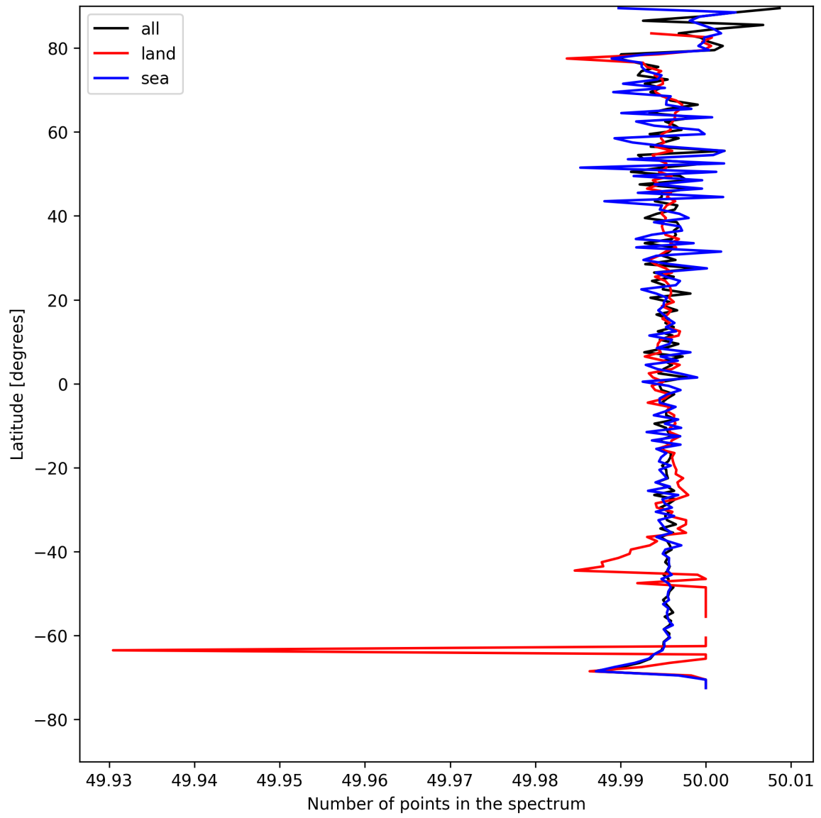
Figure 25: Zonal average of “Number of points in the spectrum” for 2025-08-11 to 2025-08-12.
