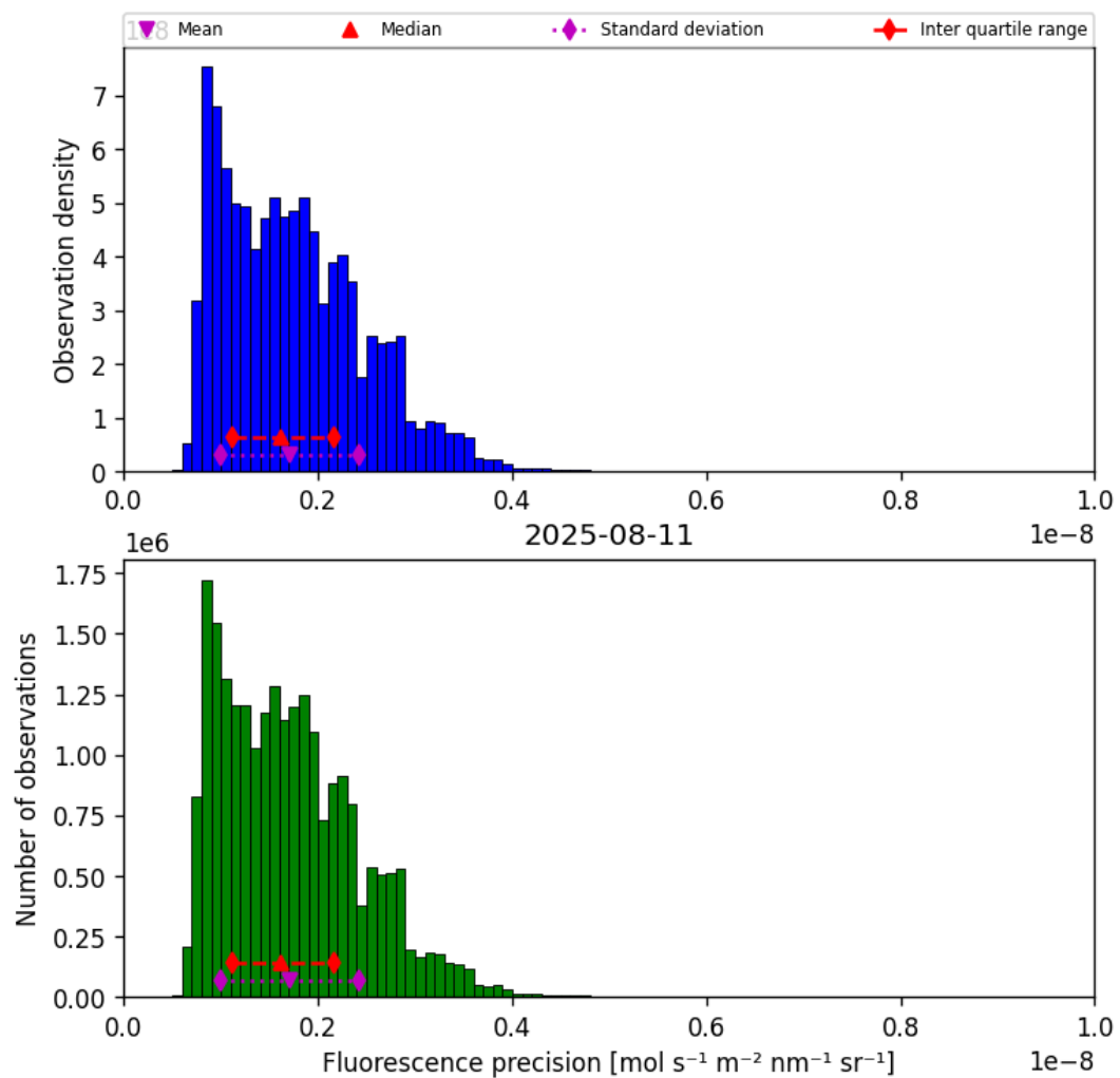
Figure 39: Histogram of “Fluorescence precision” for 2025-08-11 to 2025-08-12
