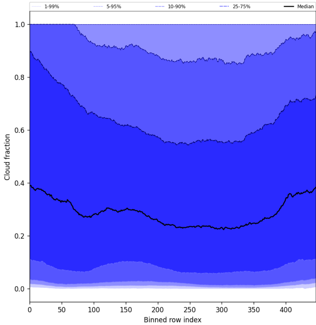
Figure 47: Along track statistics of “Cloud fraction” for 2025-08-11 to 2025-08-12
