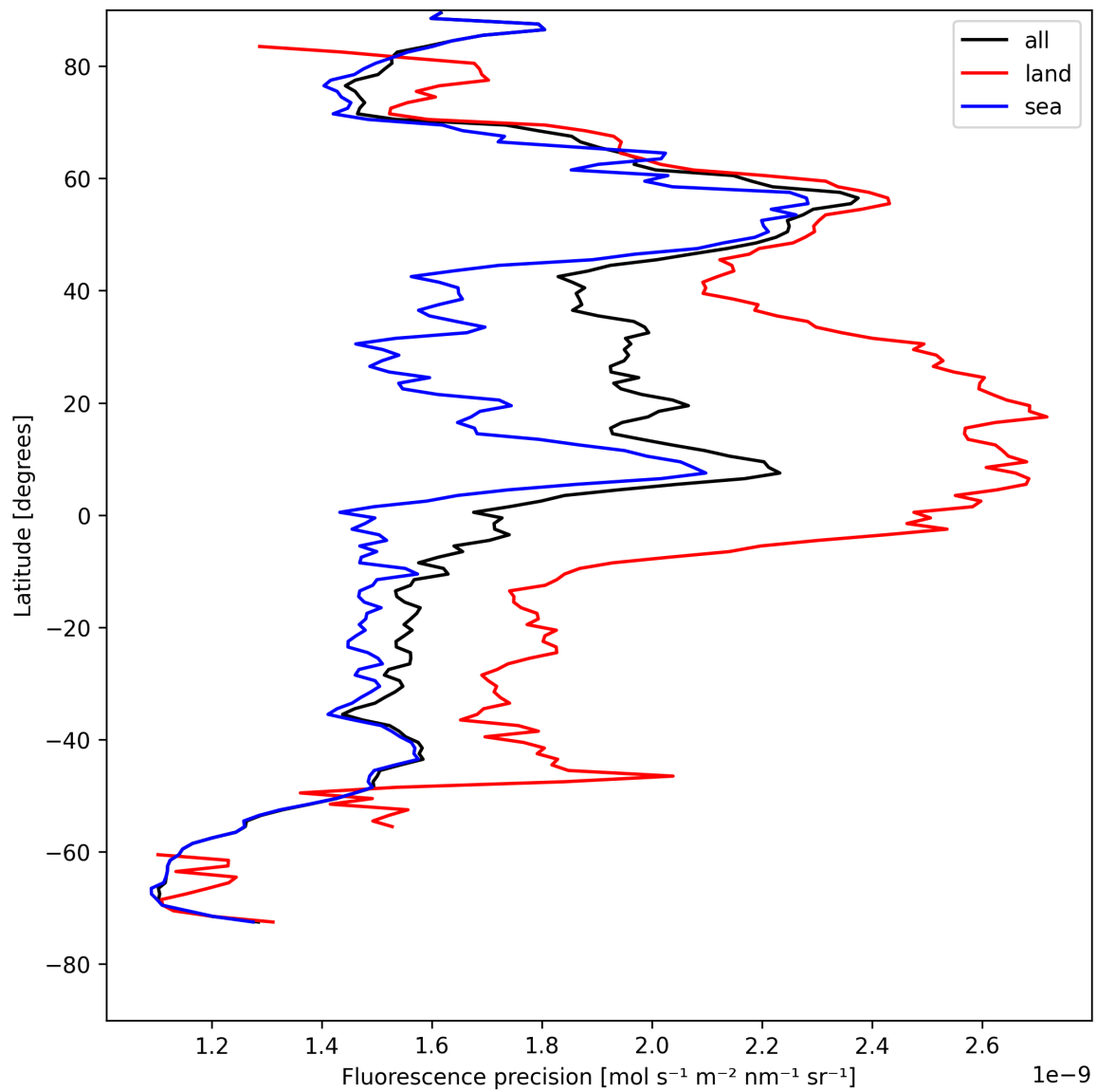
Figure 22: Zonal average of “Fluorescence precision” for 2025-08-11 to 2025-08-12.
