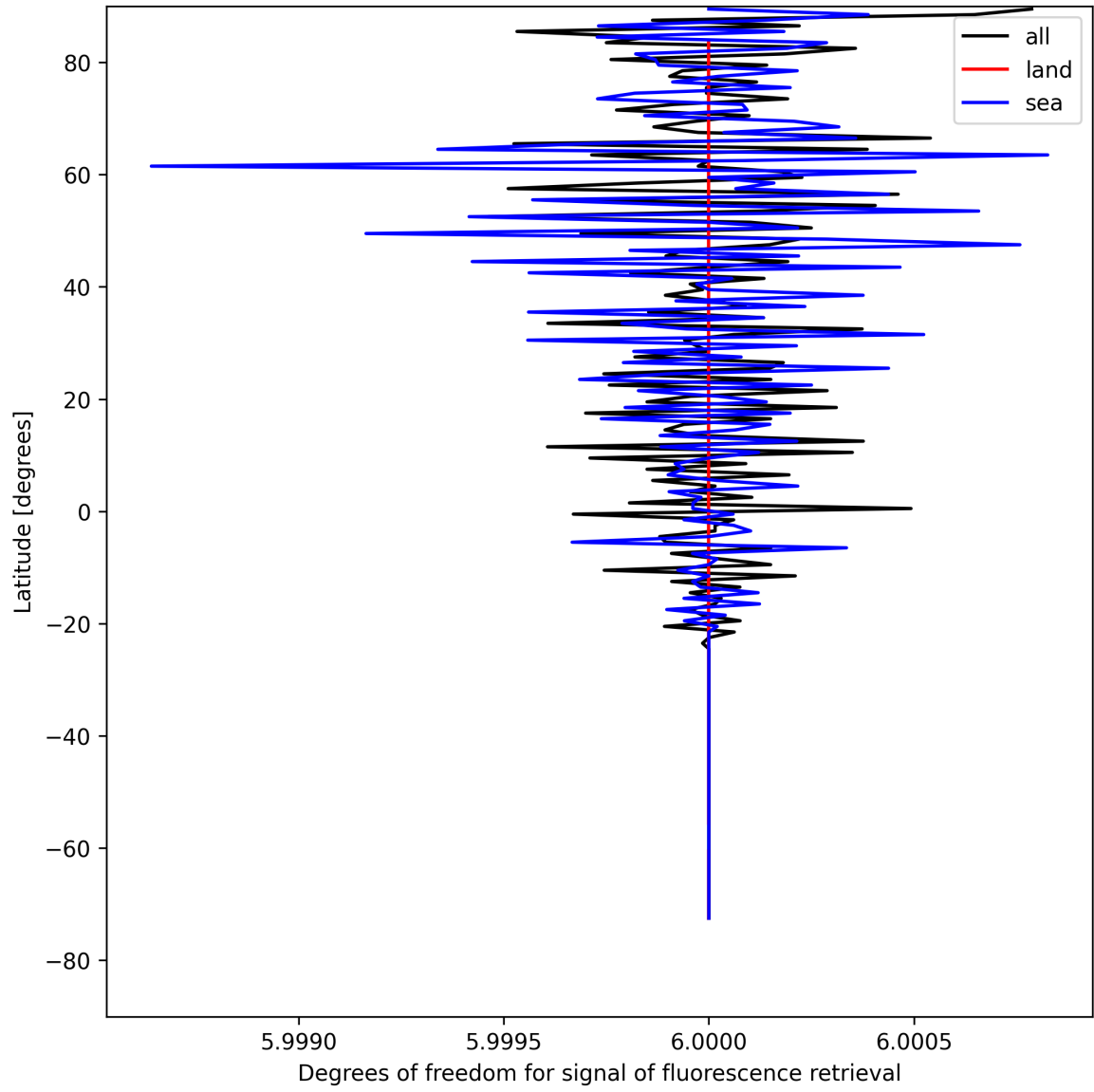
Figure 24: Zonal average of “Degrees of freedom for signal of fluorescence retrieval” for 2025-08-11 to 2025-08-12.
