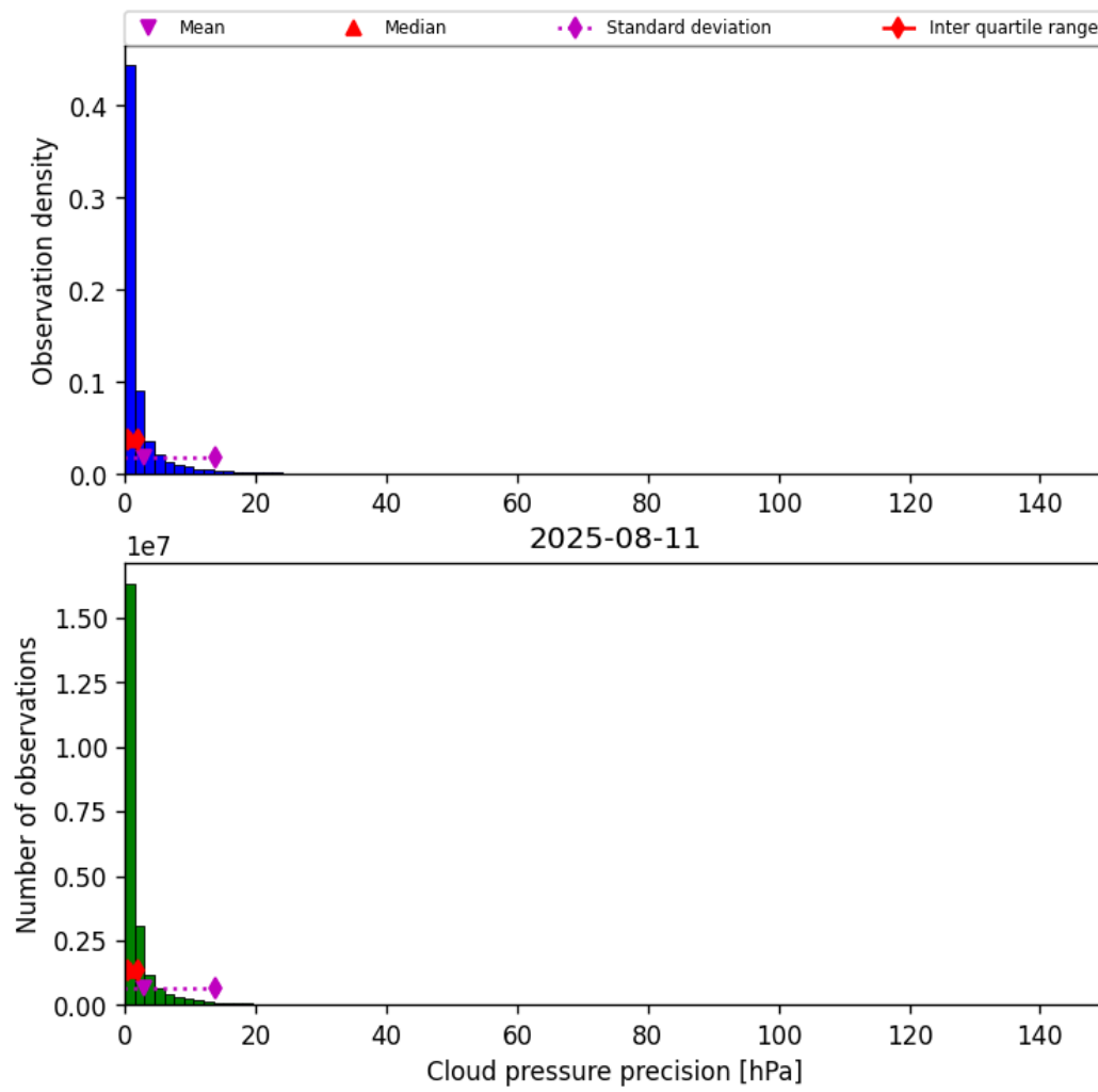
Figure 29: Histogram of “Cloud pressure precision” for 2025-08-11 to 2025-08-12
