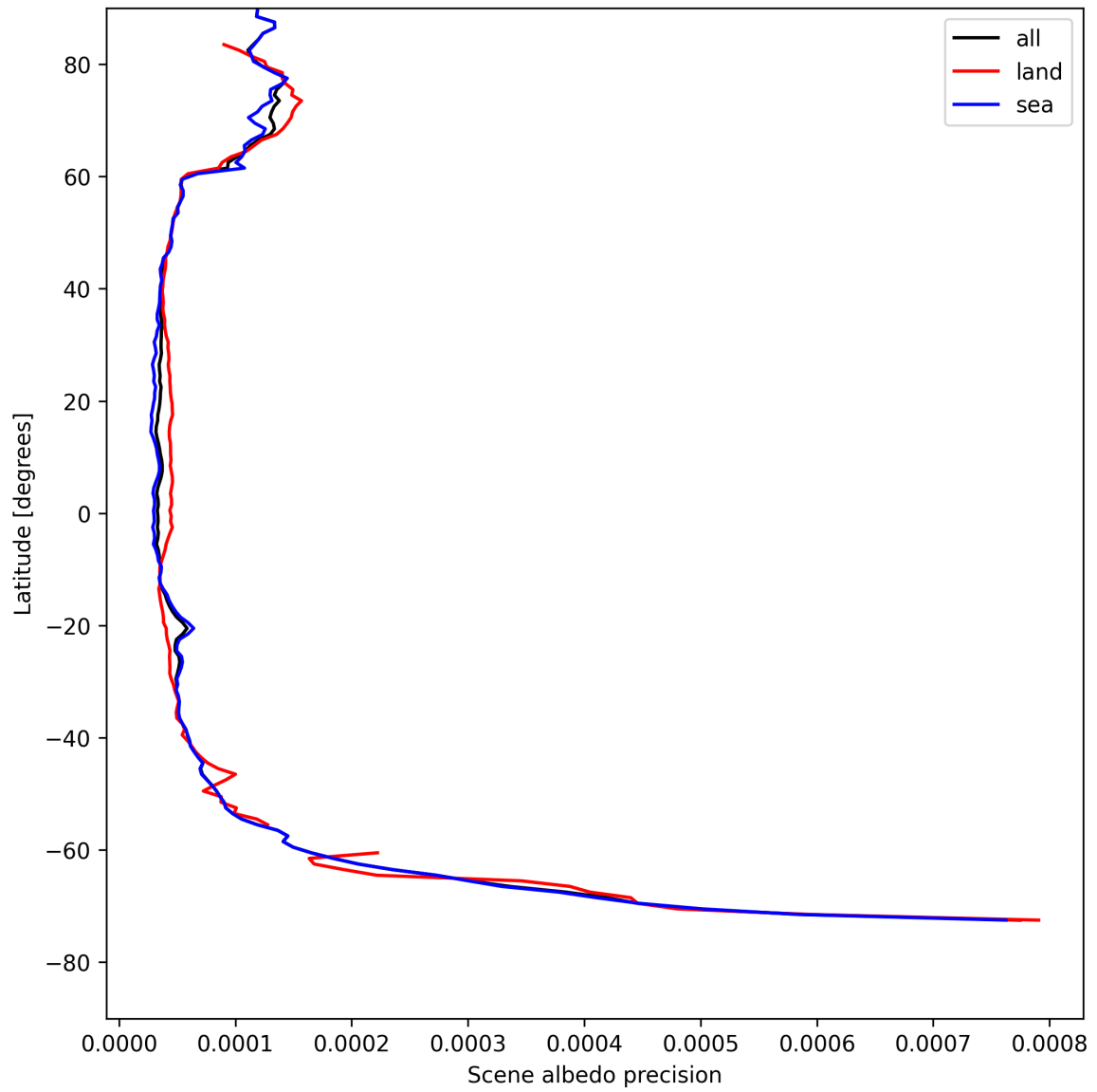
Figure 16: Zonal average of “Scene albedo precision” for 2025-08-11 to 2025-08-12.
