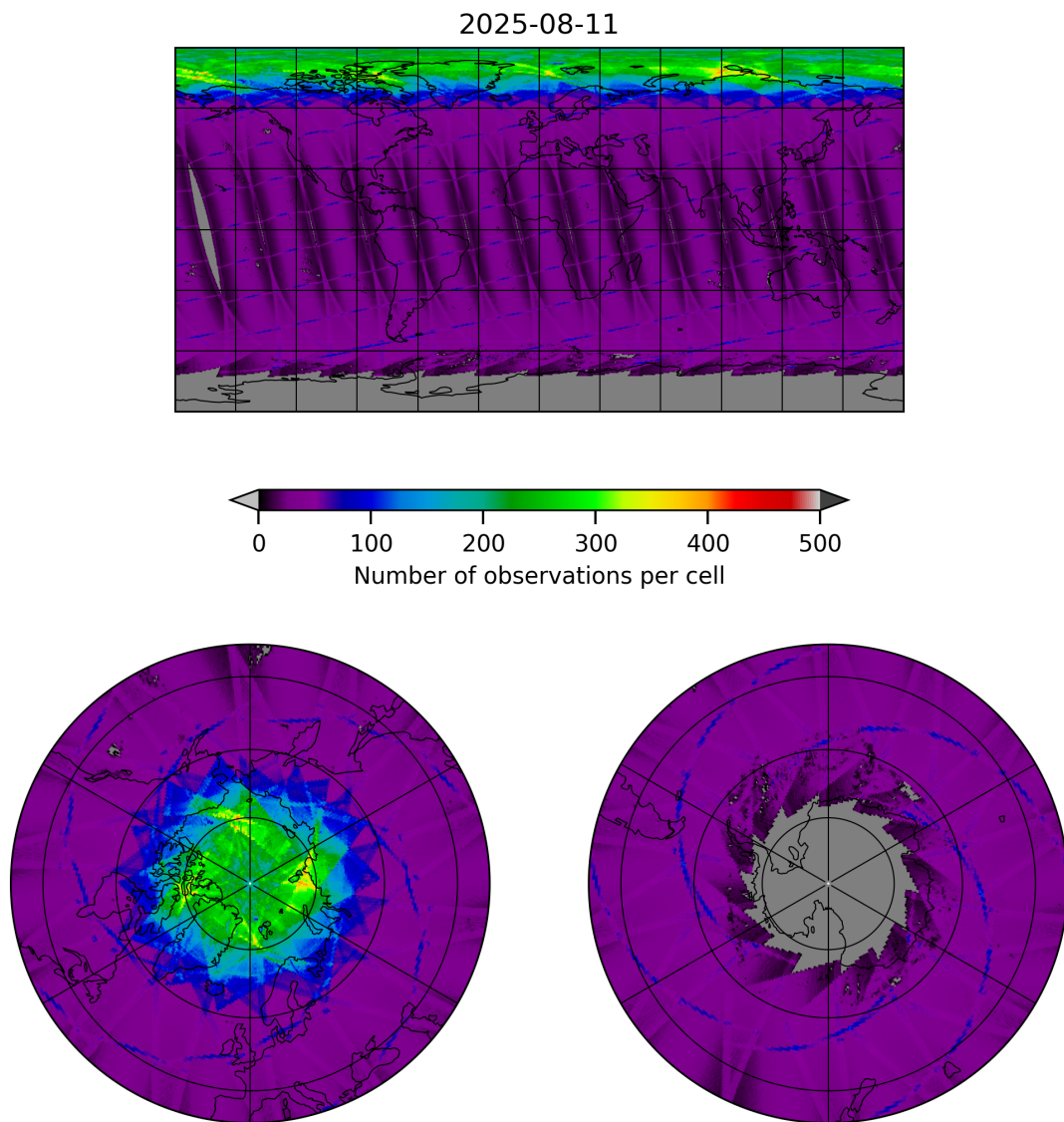
Figure 9: Map of the number of observations for 2025-08-11 to 2025-08-12
