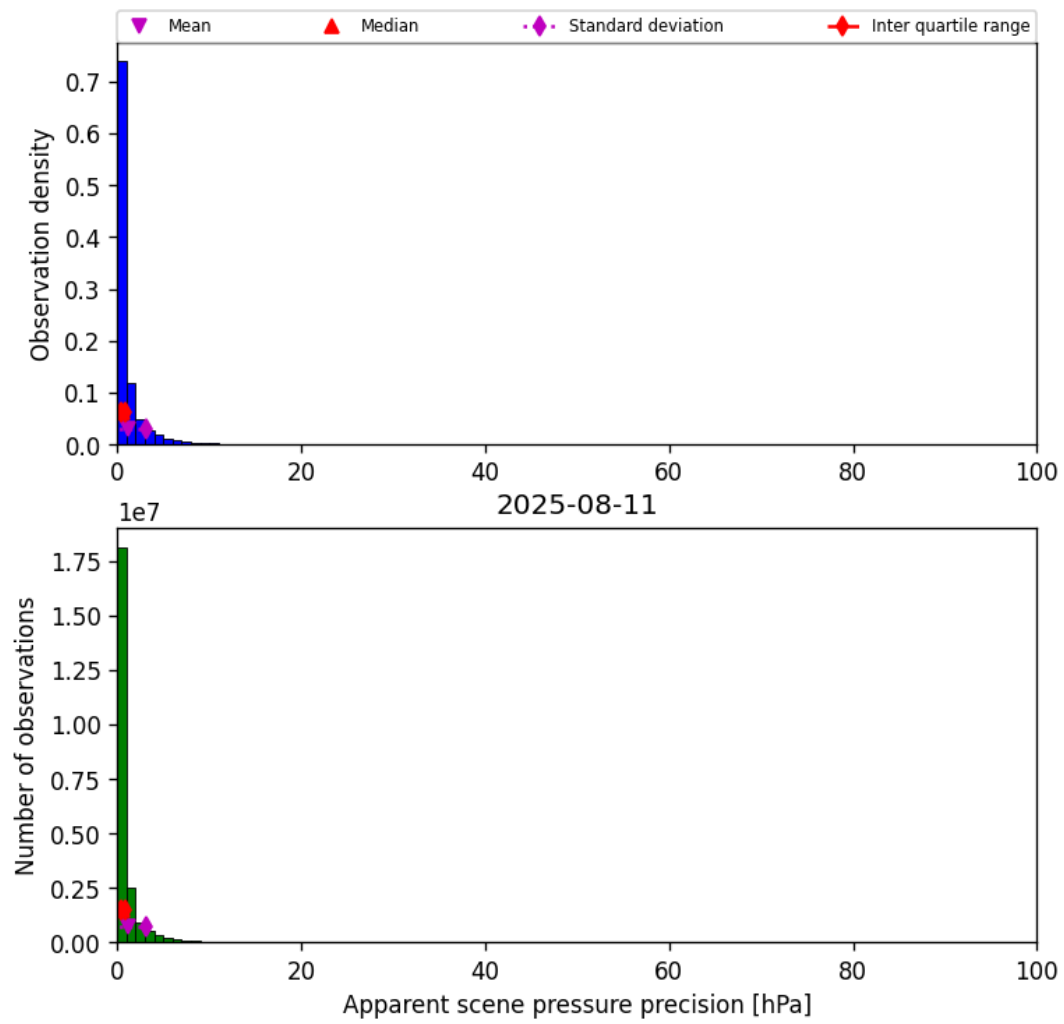
Figure 35: Histogram of “Apparent scene pressure precision” for 2025-08-11 to 2025-08-12
