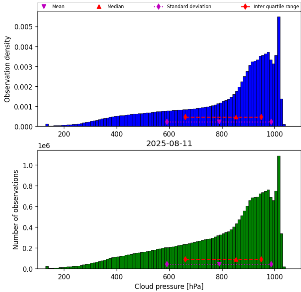
Figure 28: Histogram of “Cloud pressure” for 2025-08-11 to 2025-08-12
