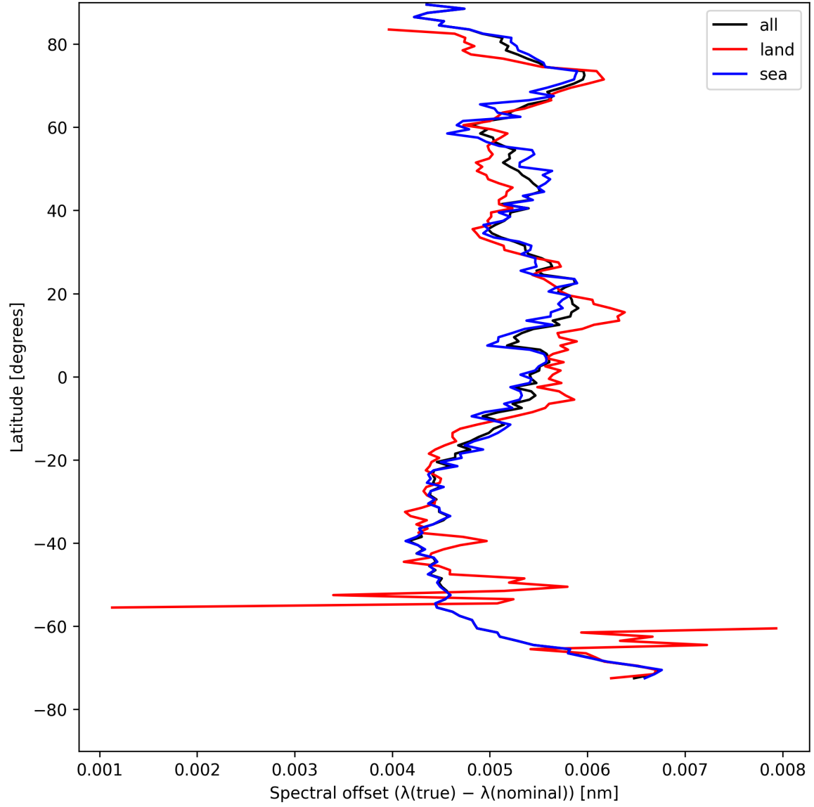
Figure 26: Zonal average of “Spectral offset ( \lambda_{\text{true}} - \lambda_{\text{nominal}} )” for 2025-08-11 to 2025-08-12.
