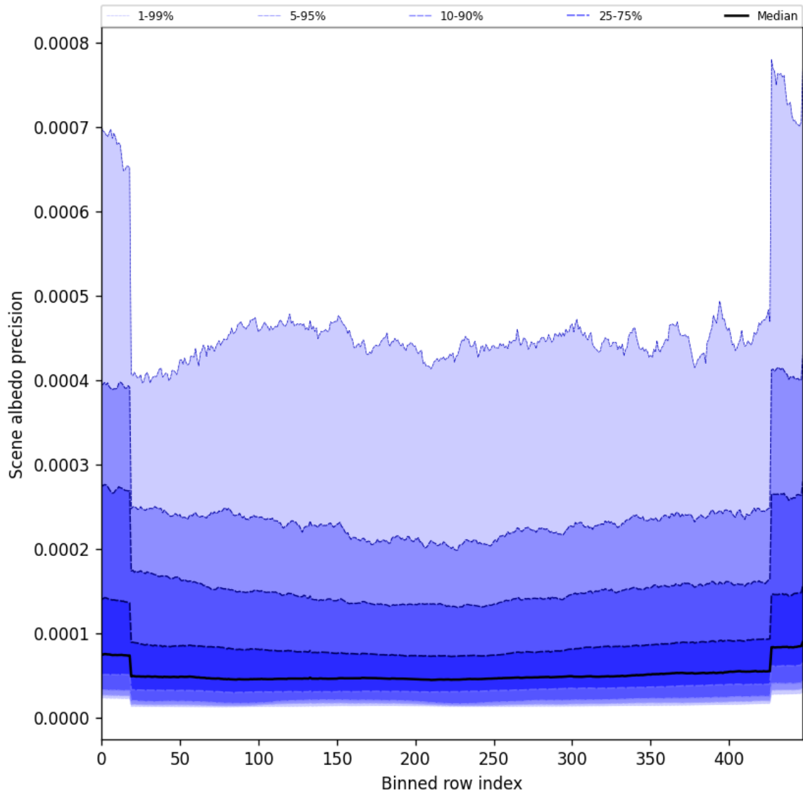
Figure 50: Along track statistics of “Scene albedo precision” for 2025-08-11 to 2025-08-12
