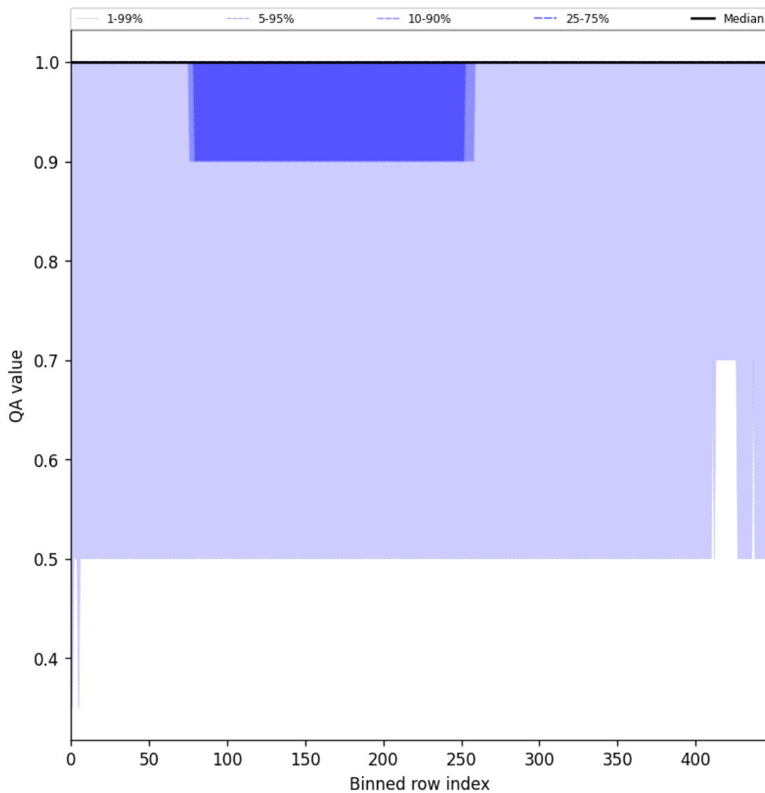
Figure 44: Along track statistics of “QA value” for 2025-08-11 to 2025-08-12
