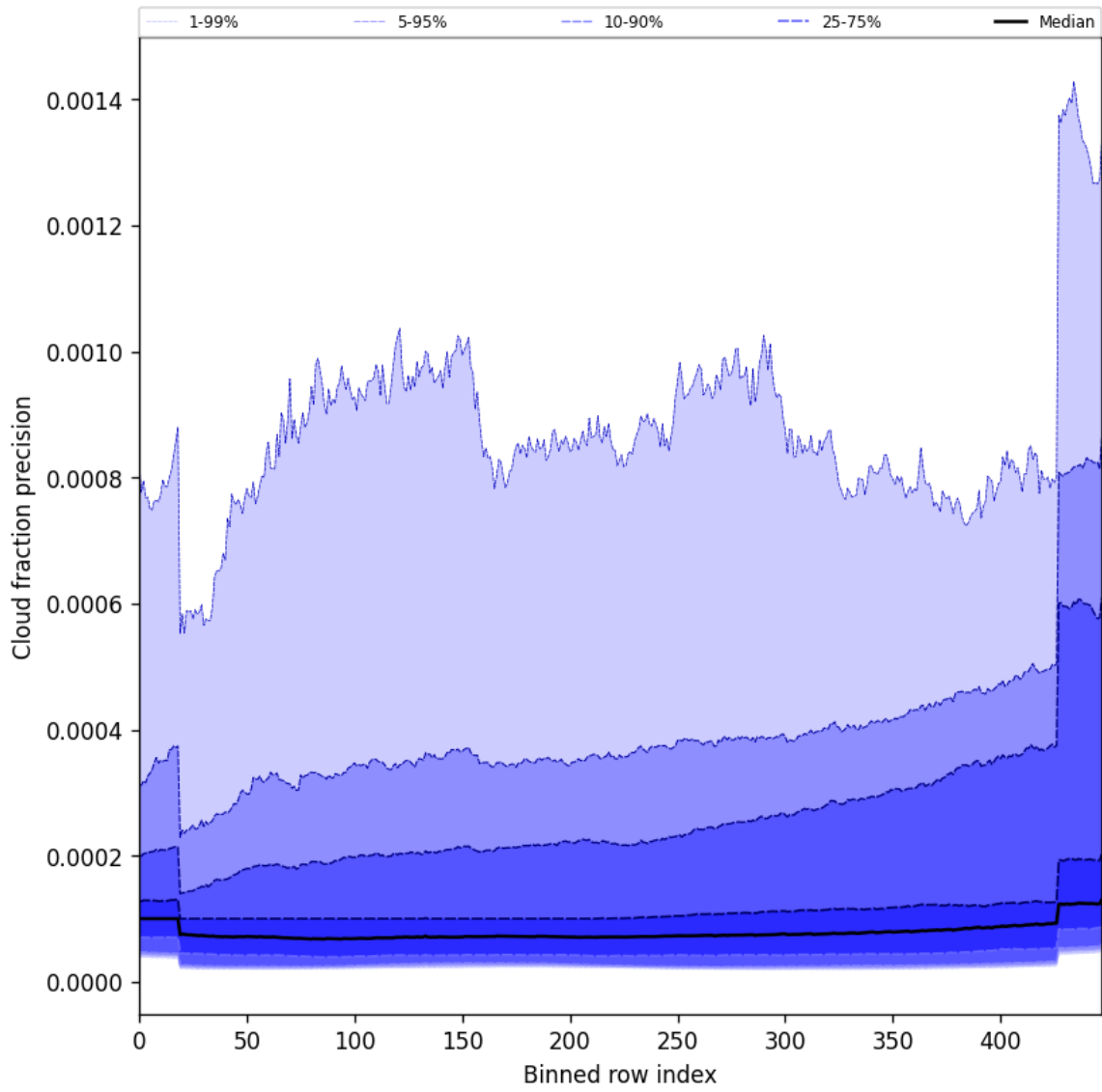
Figure 48: Along track statistics of “Cloud fraction precision” for 2025-08-11 to 2025-08-12
