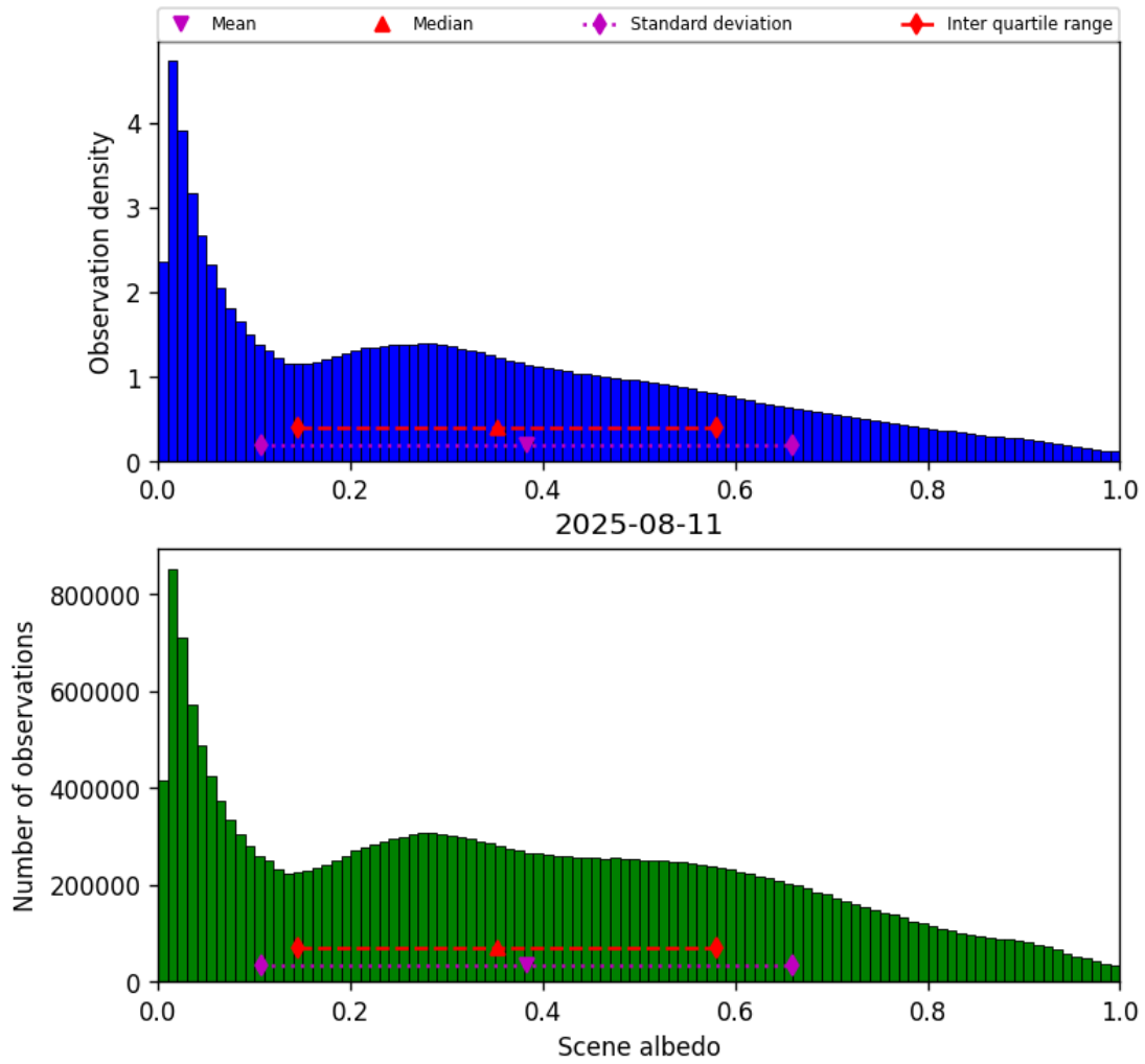
Figure 32: Histogram of “Scene albedo” for 2025-08-11 to 2025-08-12
