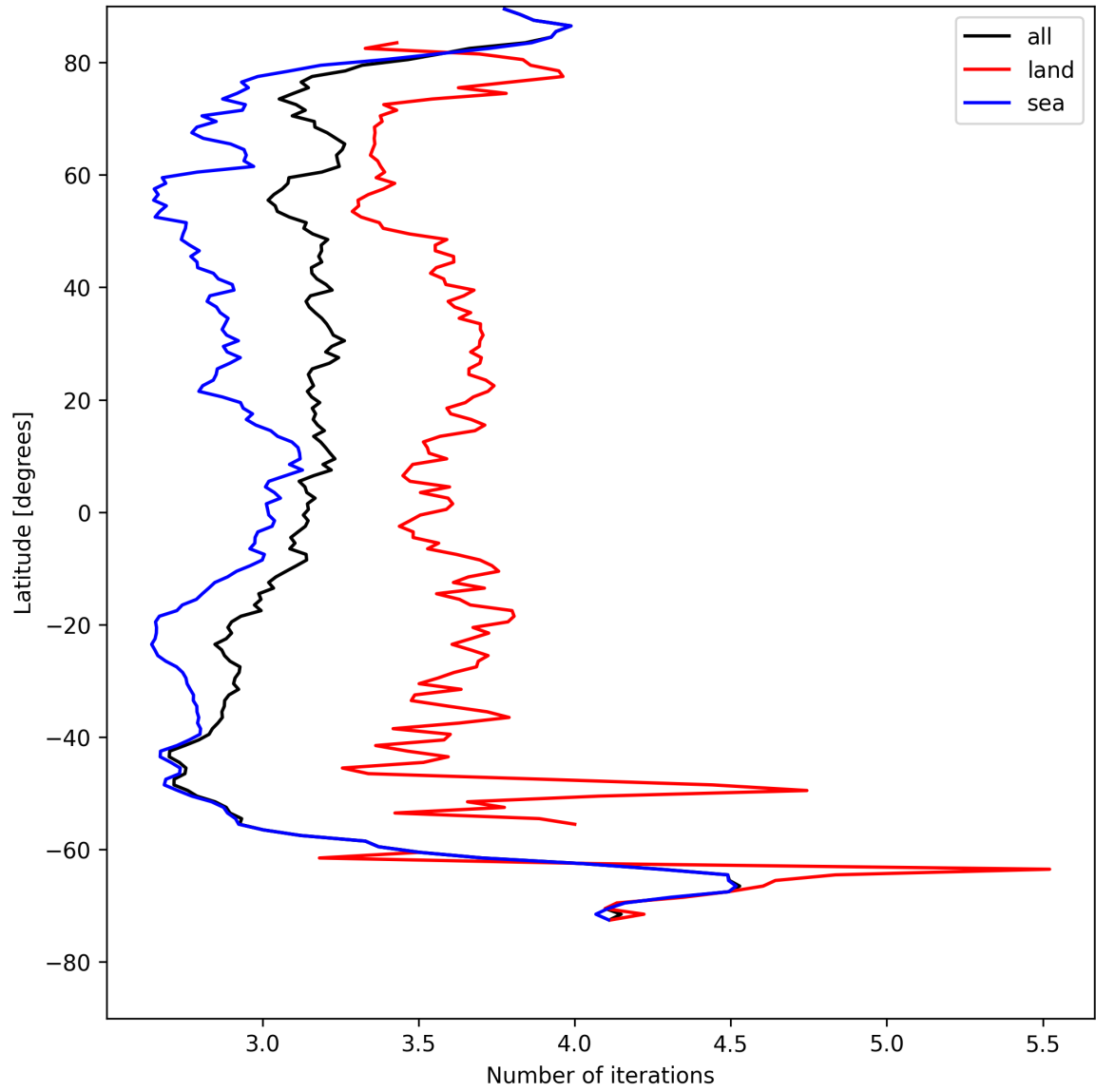
Figure 20: Zonal average of “Number of iterations” for 2025-08-11 to 2025-08-12.
