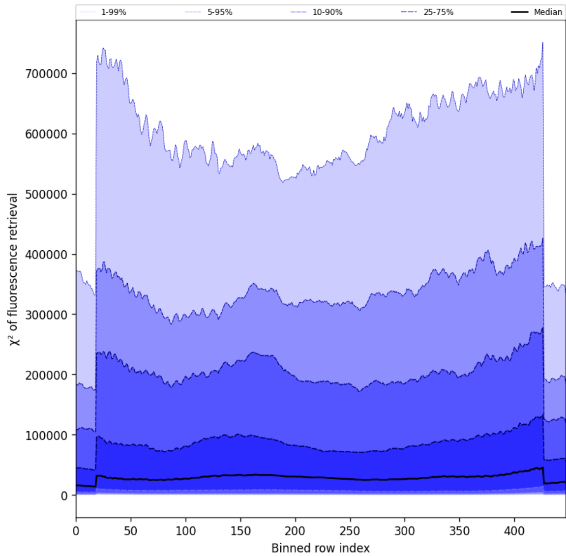
Figure 57: Along track statistics of “ \chi^2 of fluorescence retrieval” for 2025-08-11 to 2025-08-12
