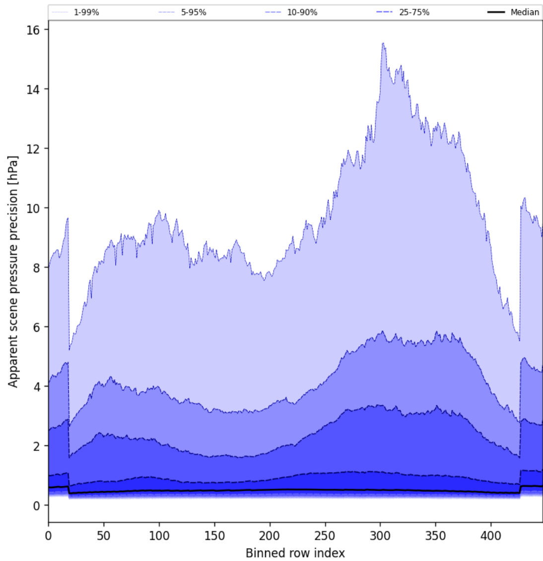
Figure 52: Along track statistics of “Apparent scene pressure precision” for 2025-08-11 to 2025-08-12
