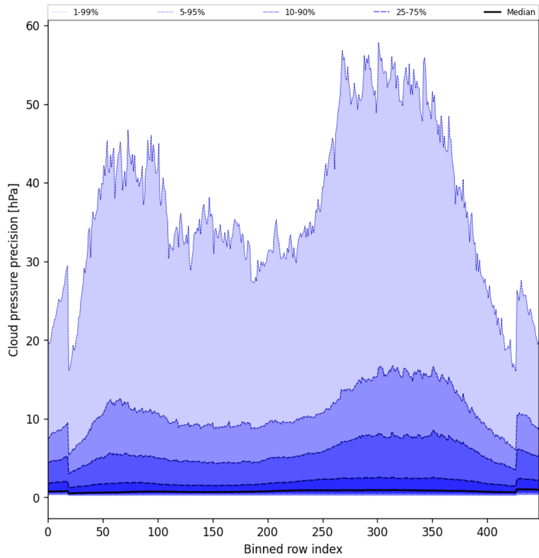
Figure 46: Along track statistics of “Cloud pressure precision” for 2025-08-11 to 2025-08-12
