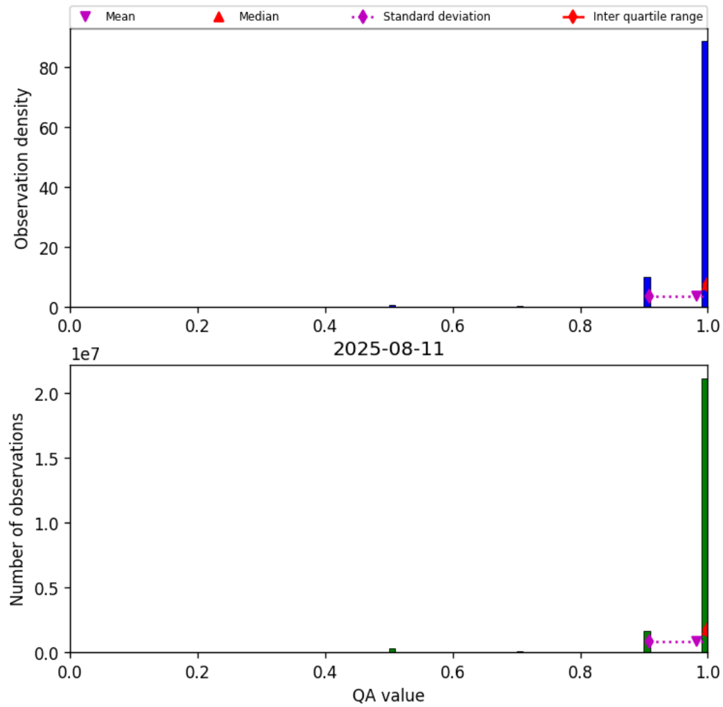
Figure 27: Histogram of “QA value” for 2025-08-11 to 2025-08-12
