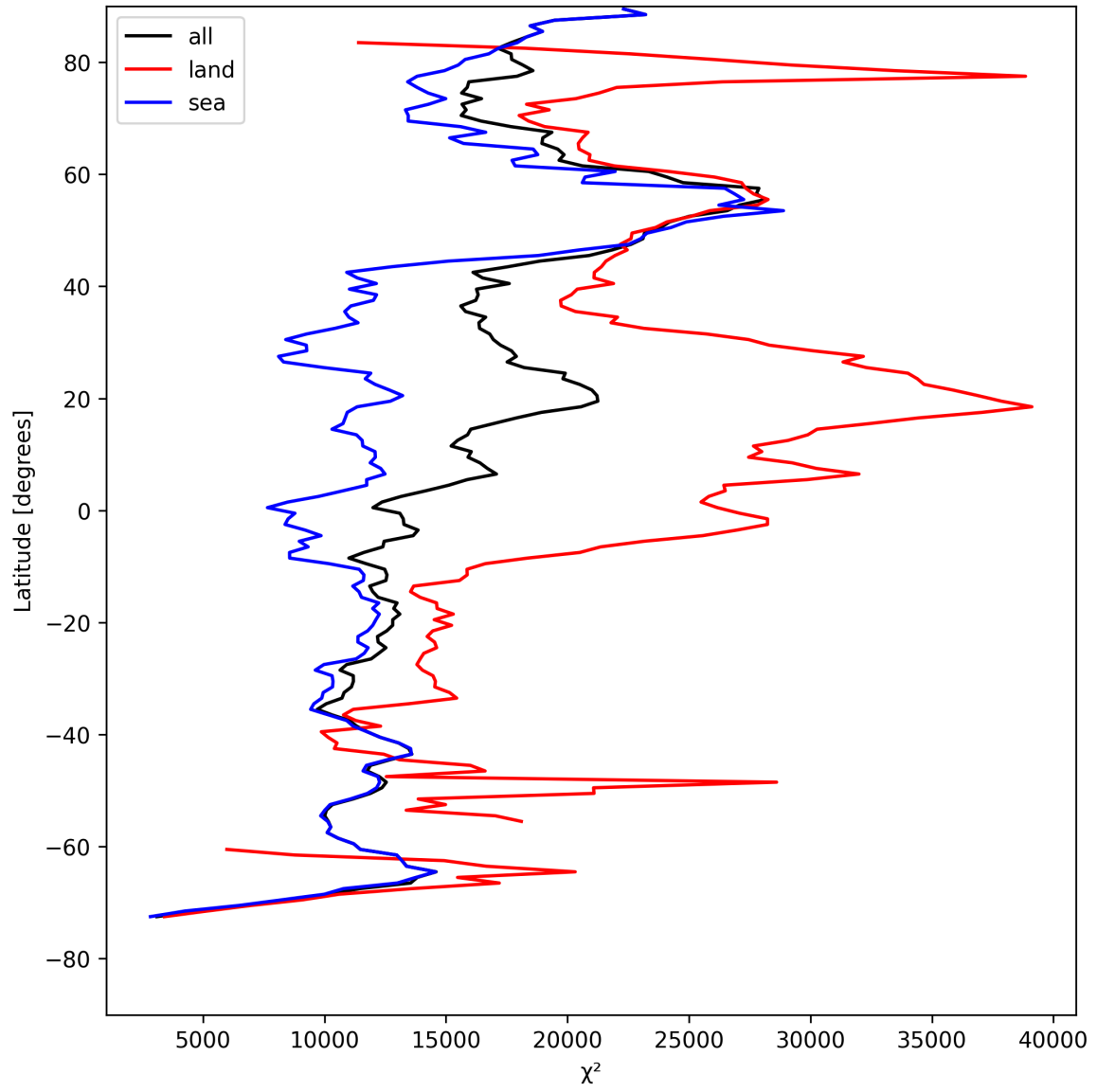
Figure 19: Zonal average of “ \chi^2 ” for 2025-08-11 to 2025-08-12.
