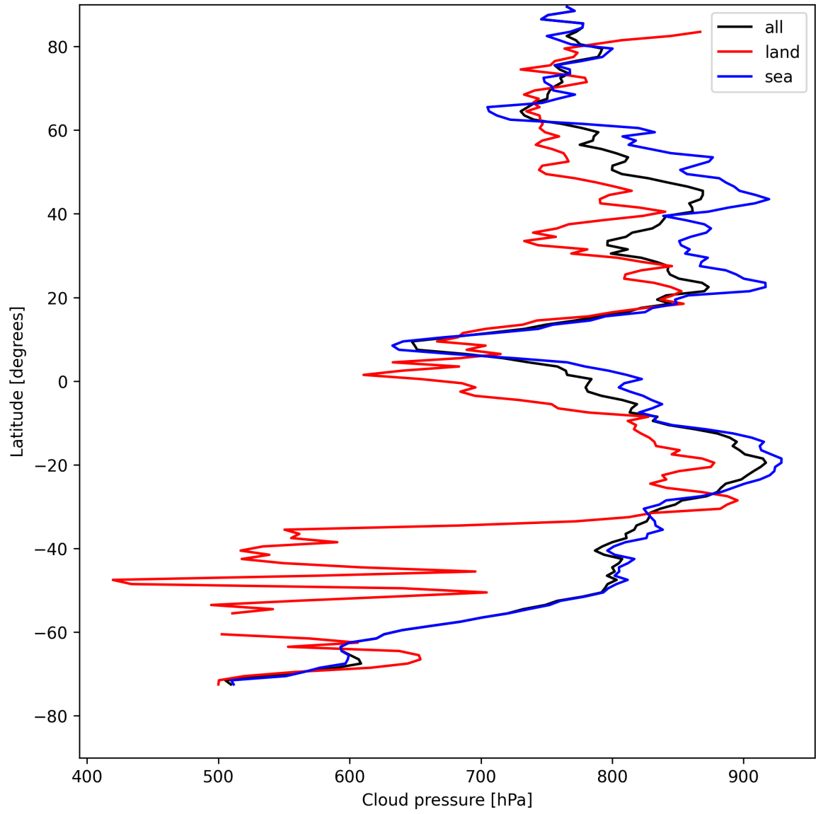
Figure 11: Zonal average of “Cloud pressure” for 2025-08-11 to 2025-08-12.
