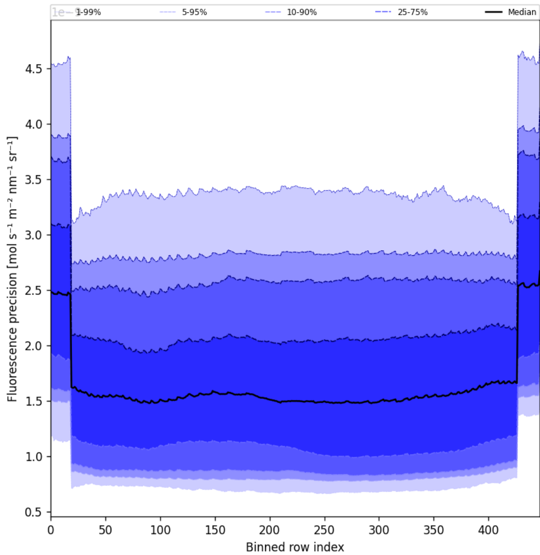
Figure 56: Along track statistics of “Fluorescence precision” for 2025-08-11 to 2025-08-12
