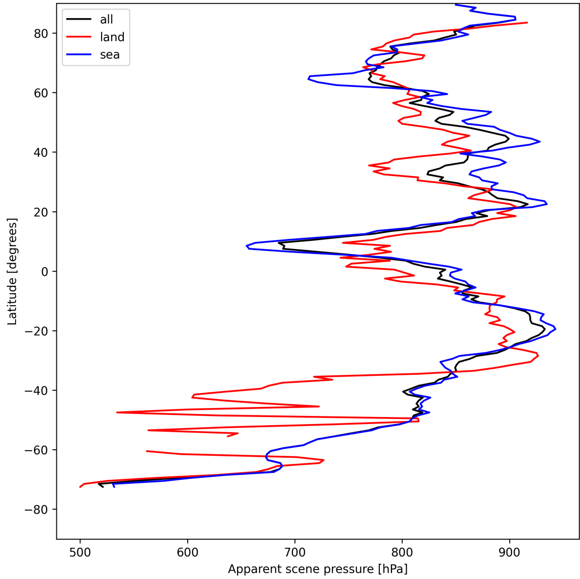
Figure 17: Zonal average of “Apparent scene pressure” for 2025-08-11 to 2025-08-12.
