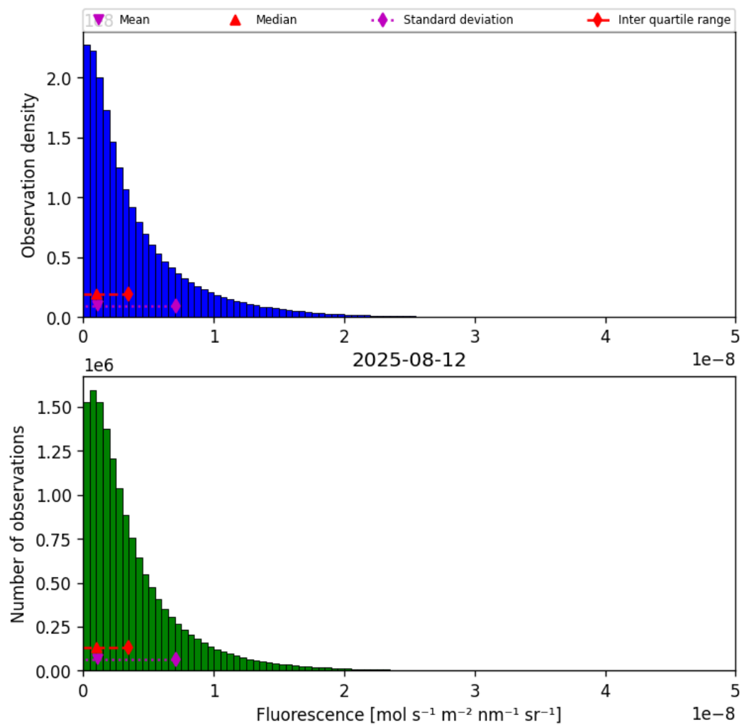
Figure 38: Histogram of “Fluorescence” for 2025-08-12 to 2025-08-12
