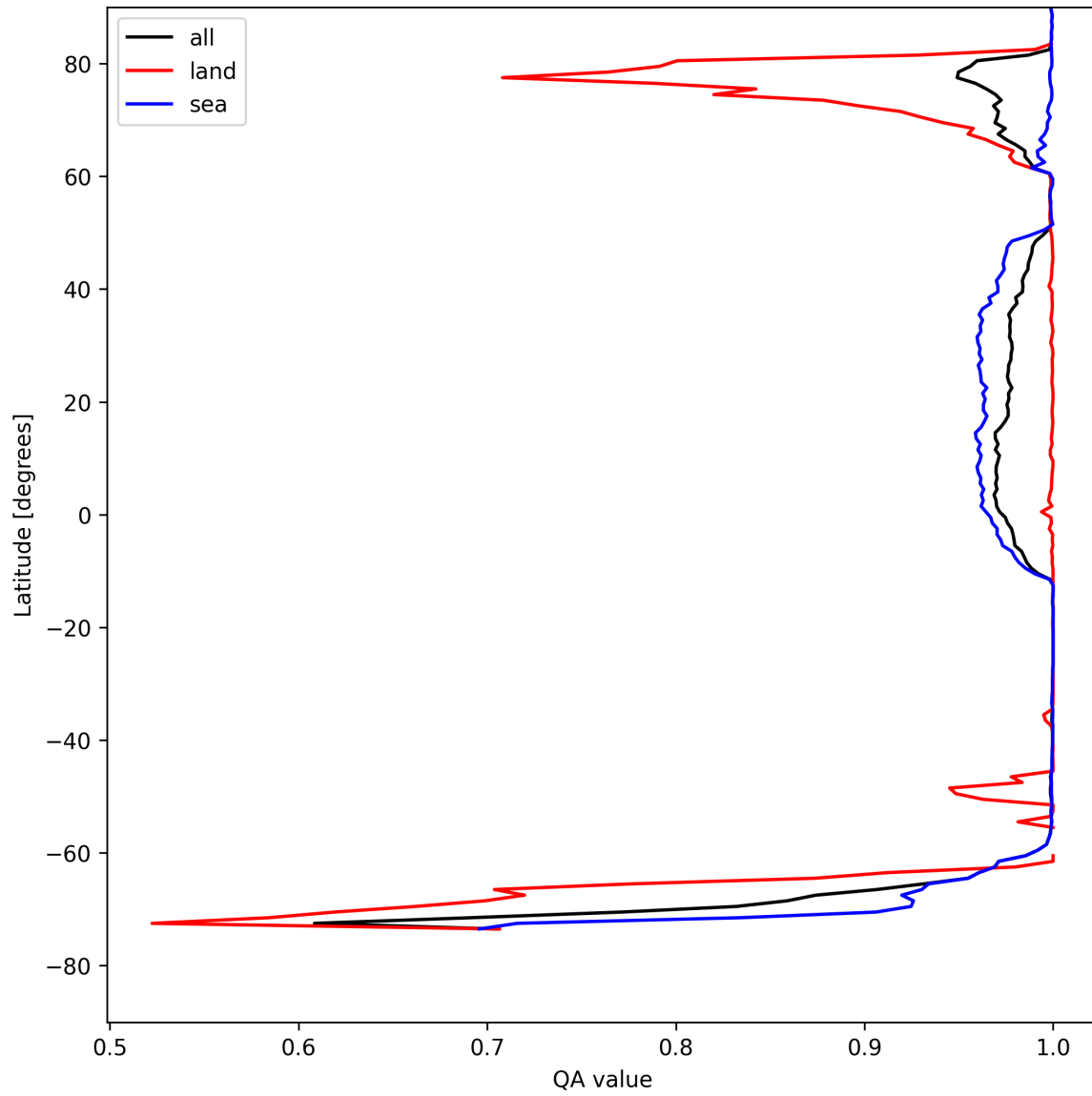
Figure 10: Zonal average of “QA value” for 2025-08-12 to 2025-08-12.
