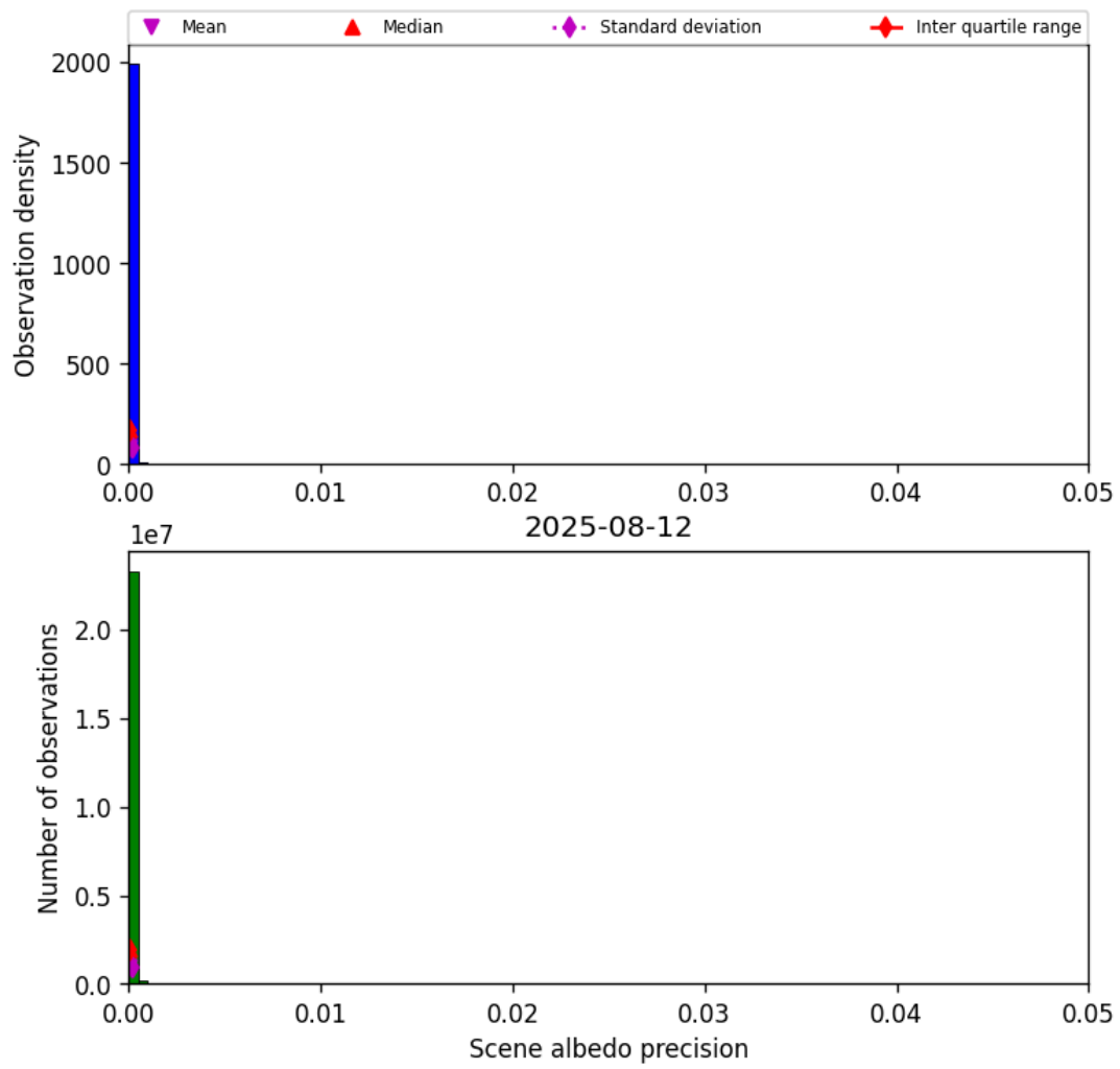
Figure 33: Histogram of “Scene albedo precision” for 2025-08-12 to 2025-08-12
