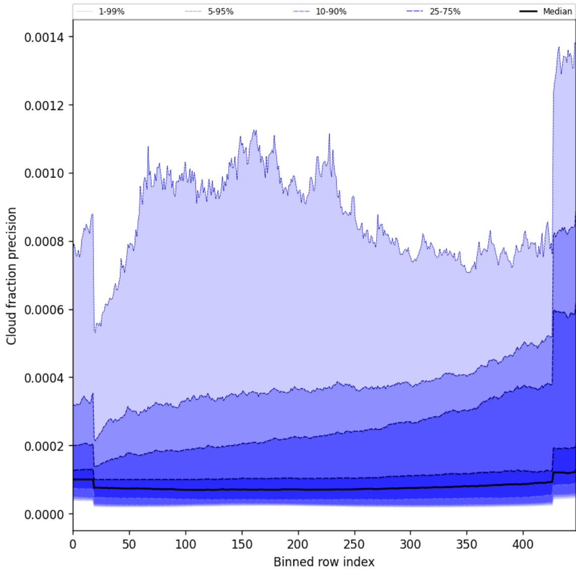
Figure 48: Along track statistics of “Cloud fraction precision” for 2025-08-12 to 2025-08-12
