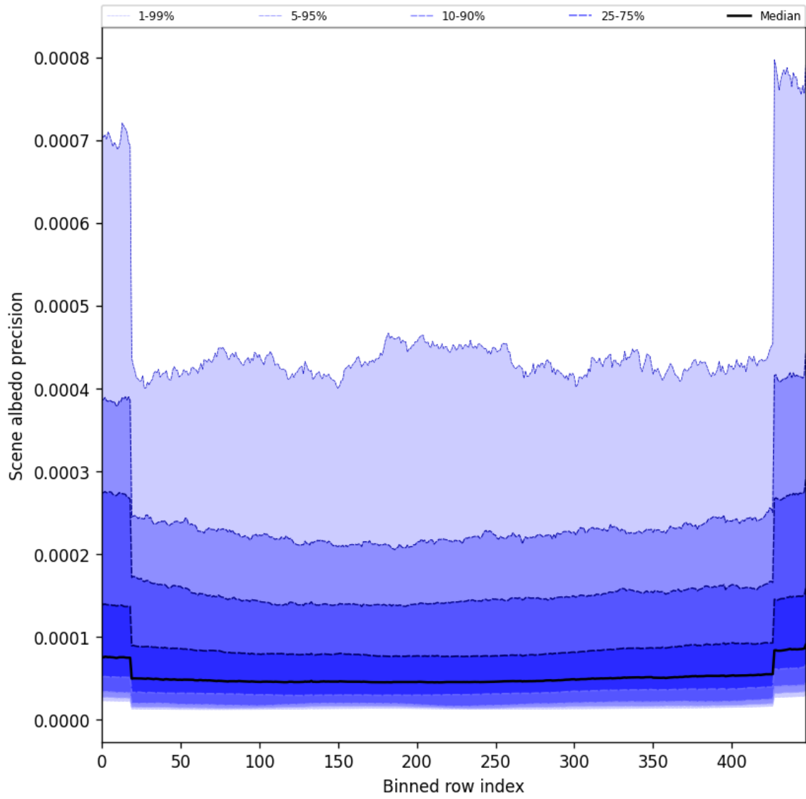
Figure 50: Along track statistics of “Scene albedo precision” for 2025-08-12 to 2025-08-12
