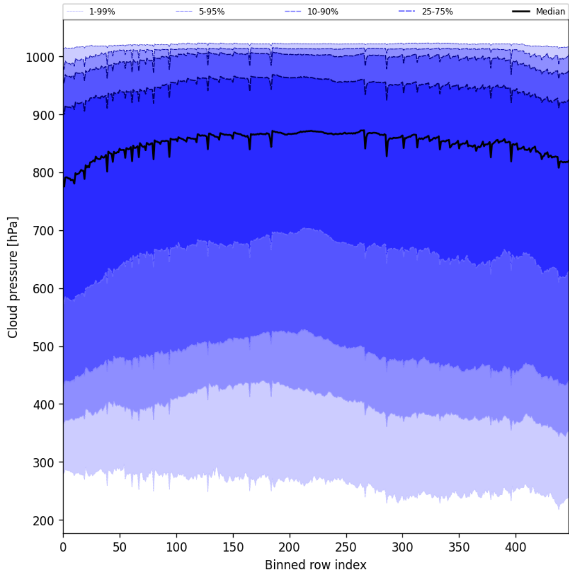
Figure 45: Along track statistics of “Cloud pressure” for 2025-08-12 to 2025-08-12
