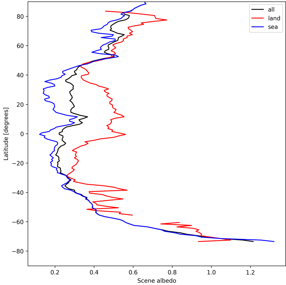
Figure 15: Zonal average of “Scene albedo” for 2025-08-12 to 2025-08-12.
