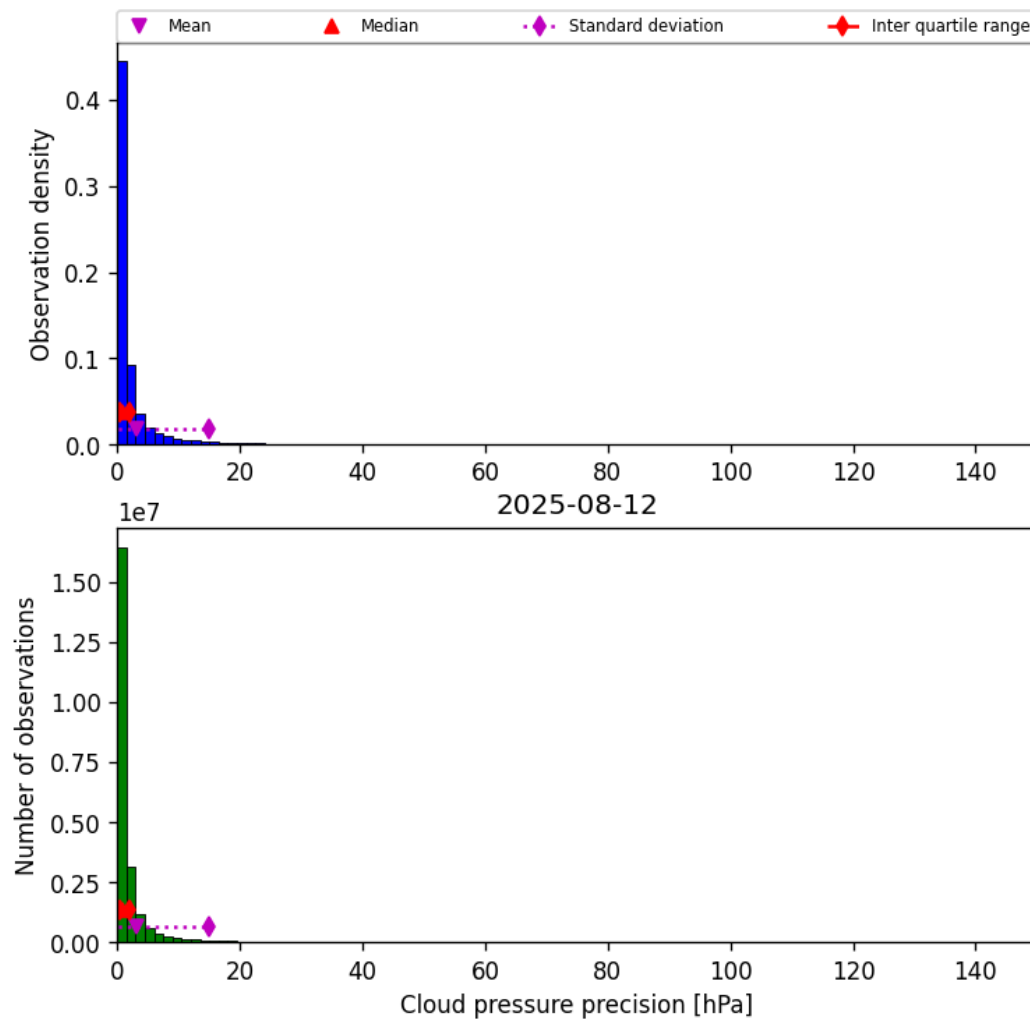
Figure 29: Histogram of “Cloud pressure precision” for 2025-08-12 to 2025-08-12
