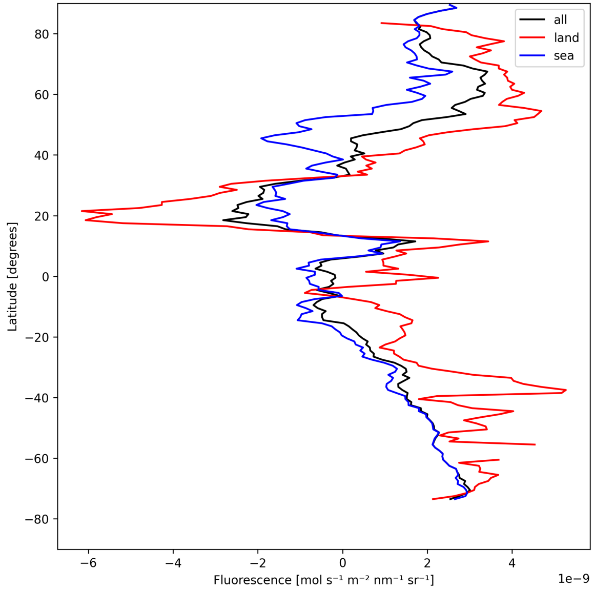
Figure 21: Zonal average of “Fluorescence” for 2025-08-12 to 2025-08-12.
