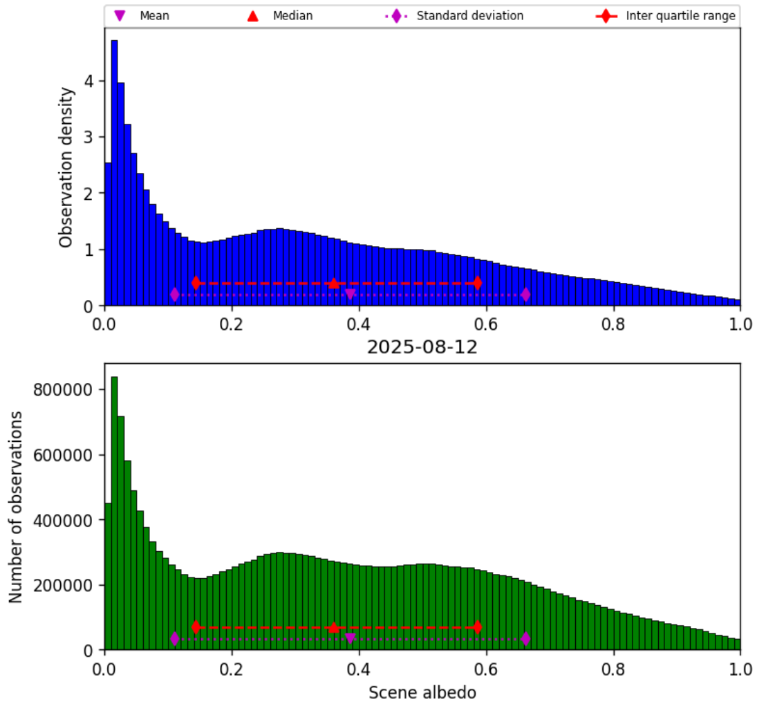
Figure 32: Histogram of “Scene albedo” for 2025-08-12 to 2025-08-12
