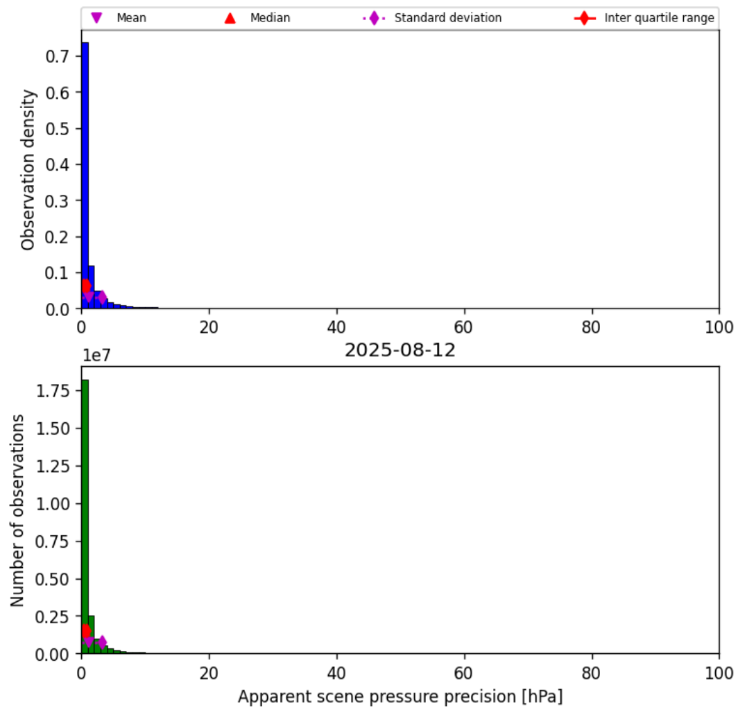
Figure 35: Histogram of “Apparent scene pressure precision” for 2025-08-12 to 2025-08-12
