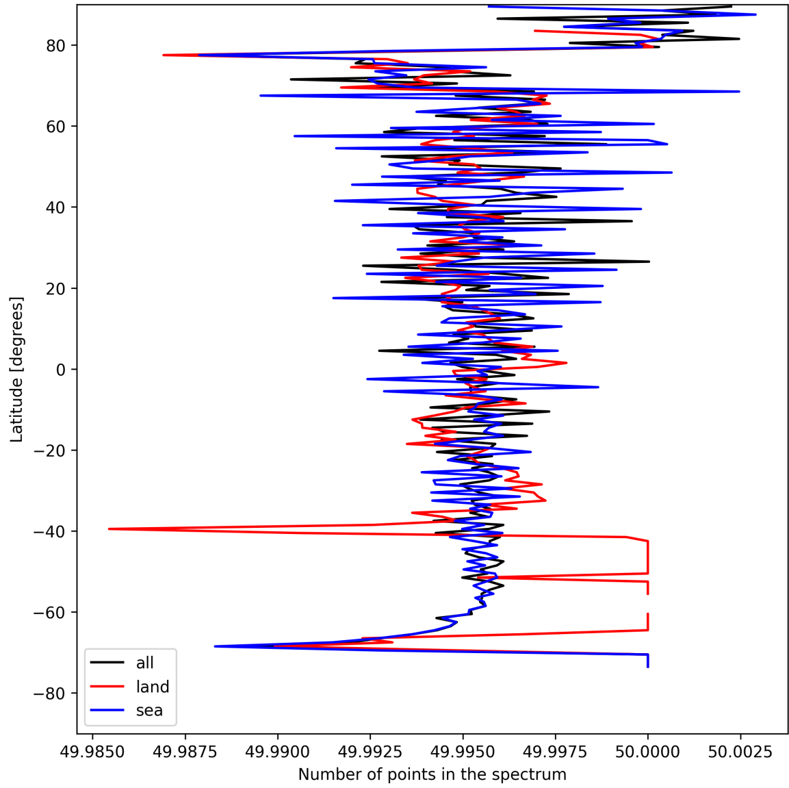
Figure 25: Zonal average of “Number of points in the spectrum” for 2025-08-12 to 2025-08-12.
