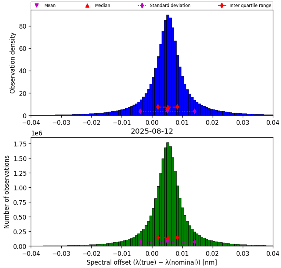
Figure 43: Histogram of “Spectral offset ( \lambda_{\text{true}} - \lambda_{\text{nominal}} )” for 2025-08-12 to 2025-08-12
