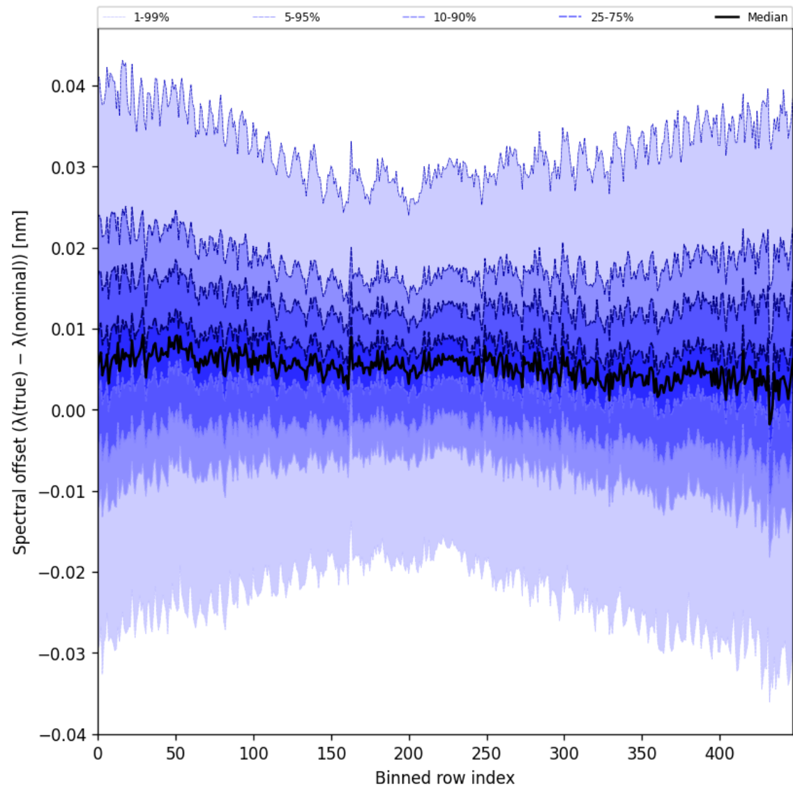
Figure 60: Along track statistics of “Spectral offset ( \lambda_{\text{true}} - \lambda_{\text{nominal}} )” for 2025-08-12 to 2025-08-12
