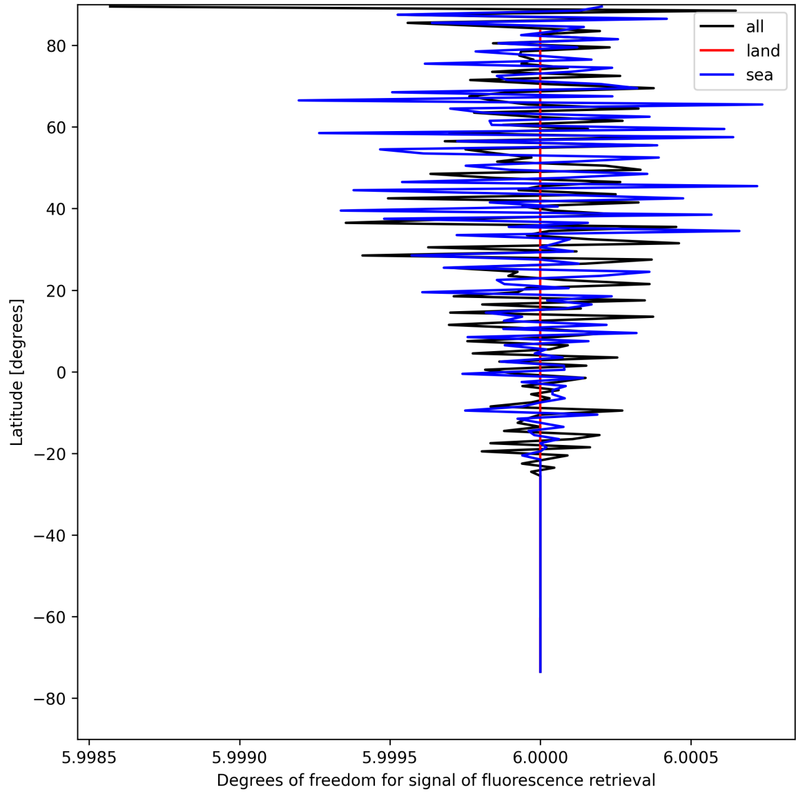
Figure 24: Zonal average of “Degrees of freedom for signal of fluorescence retrieval” for 2025-08-12 to 2025-08-12.
