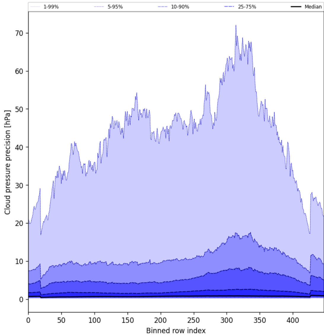
Figure 46: Along track statistics of “Cloud pressure precision” for 2025-08-12 to 2025-08-12
