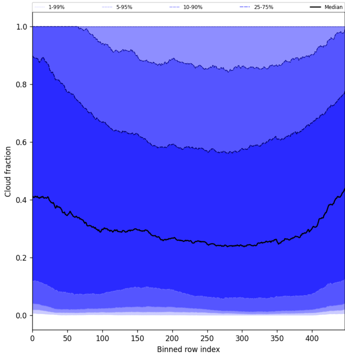
Figure 47: Along track statistics of “Cloud fraction” for 2025-08-12 to 2025-08-12
