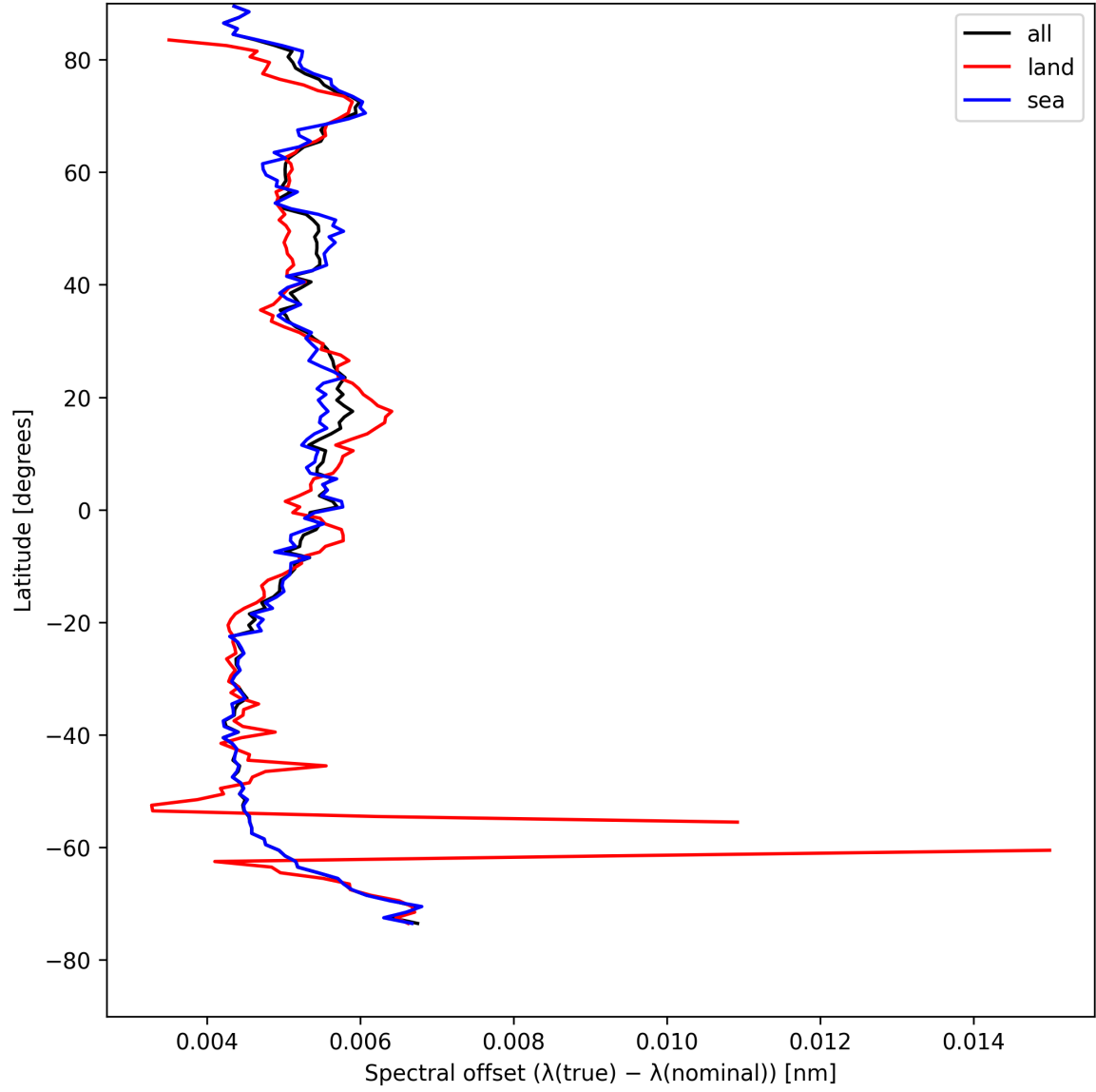
Figure 26: Zonal average of “Spectral offset ( \lambda_{\text{true}} - \lambda_{\text{nominal}} )” for 2025-08-12 to 2025-08-12.
