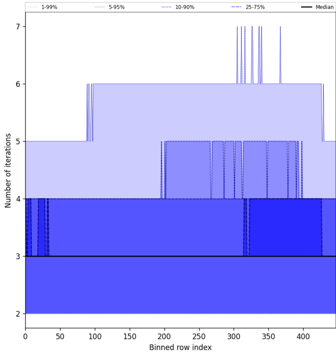
Figure 54: Along track statistics of “Number of iterations” for 2025-08-12 to 2025-08-12
