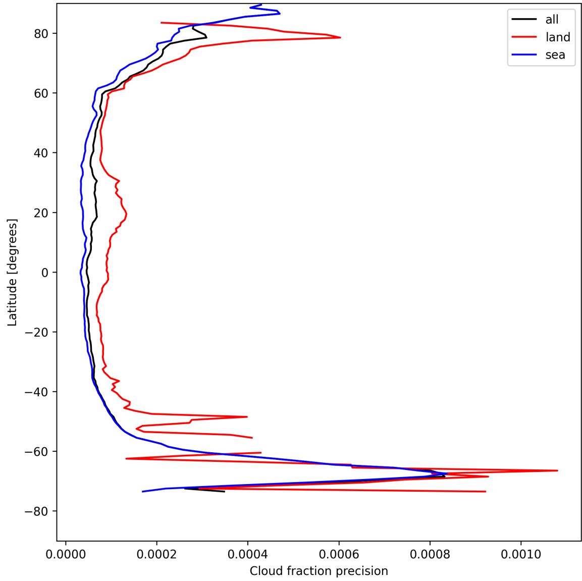
Figure 14: Zonal average of “Cloud fraction precision” for 2025-08-12 to 2025-08-12.
