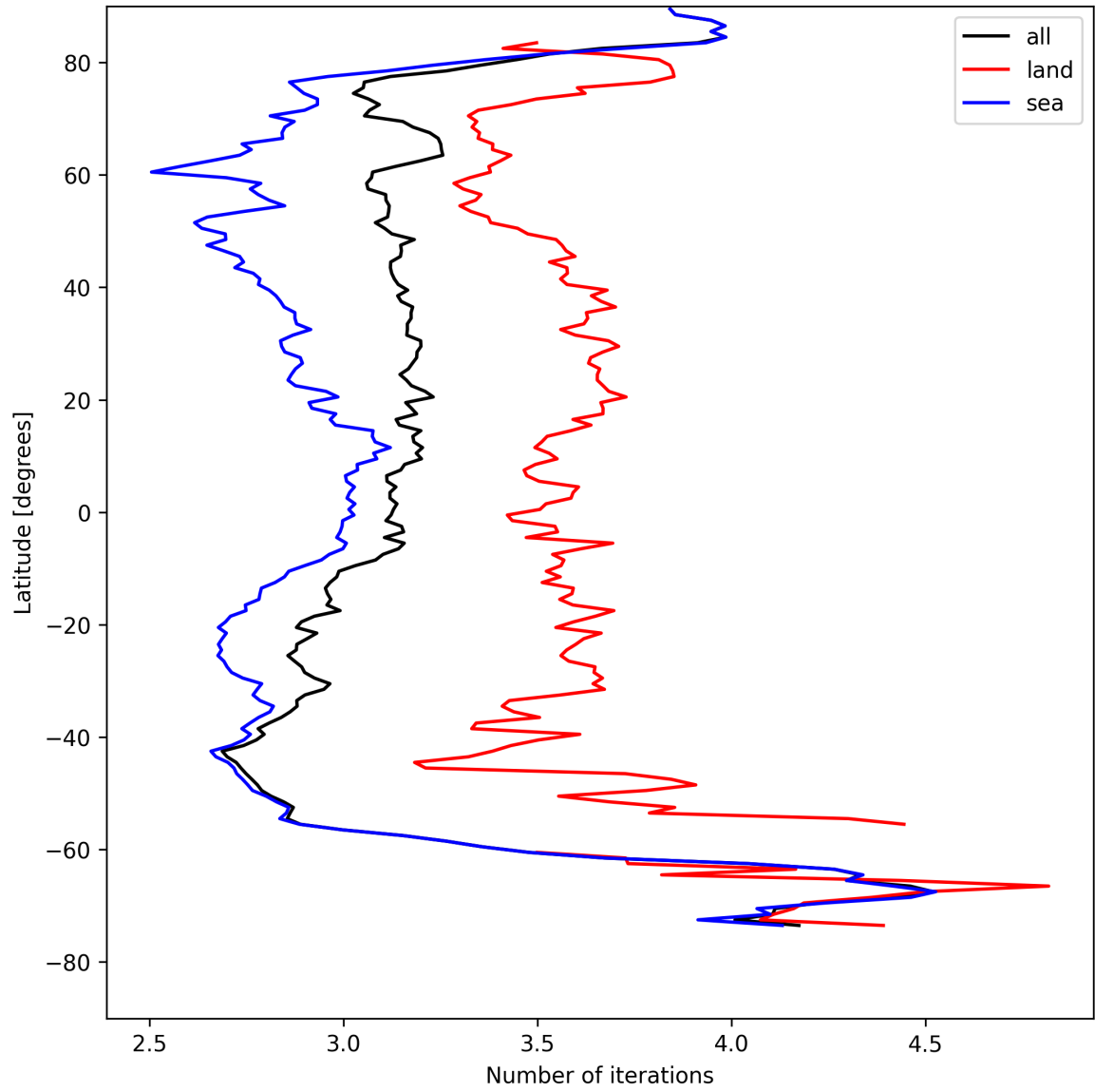
Figure 20: Zonal average of “Number of iterations” for 2025-08-12 to 2025-08-12.
