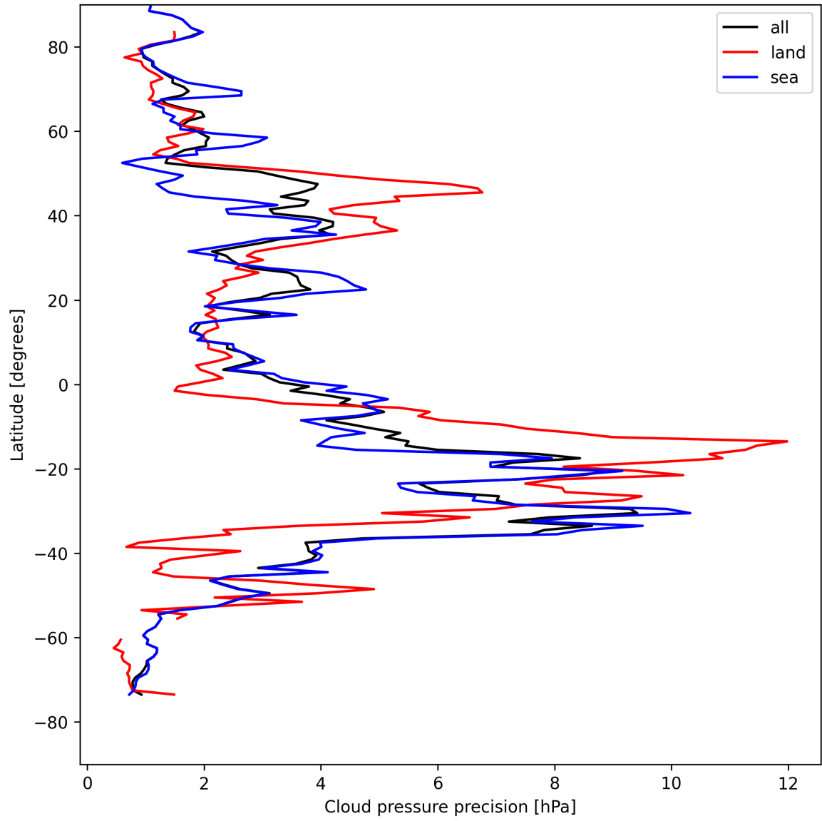
Figure 12: Zonal average of “Cloud pressure precision” for 2025-08-12 to 2025-08-12.
