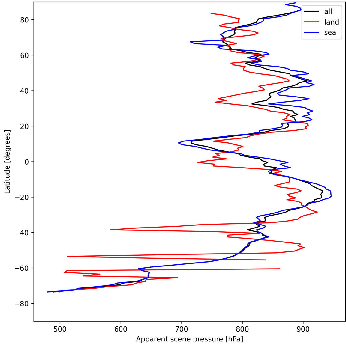
Figure 17: Zonal average of “Apparent scene pressure” for 2025-08-12 to 2025-08-12.
