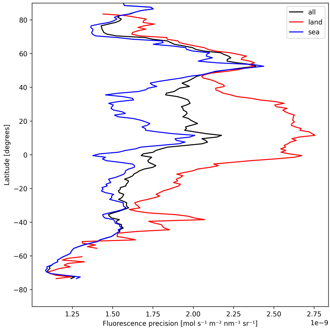
Figure 22: Zonal average of “Fluorescence precision” for 2025-08-12 to 2025-08-12.
