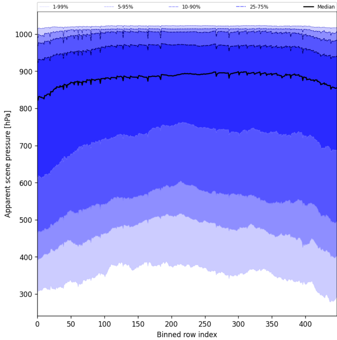
Figure 51: Along track statistics of “Apparent scene pressure” for 2025-08-12 to 2025-08-12
