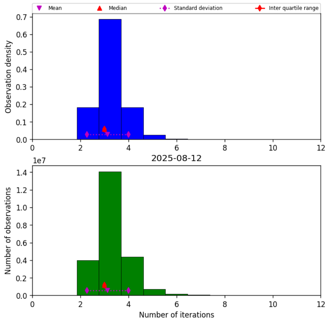
Figure 37: Histogram of “Number of iterations” for 2025-08-12 to 2025-08-12
