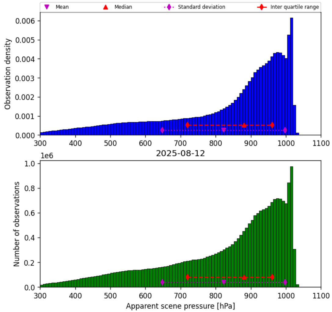
Figure 34: Histogram of “Apparent scene pressure” for 2025-08-12 to 2025-08-12
