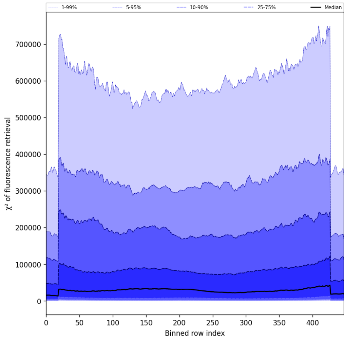
Figure 57: Along track statistics of “ \chi^2 of fluorescence retrieval” for 2025-08-12 to 2025-08-12
