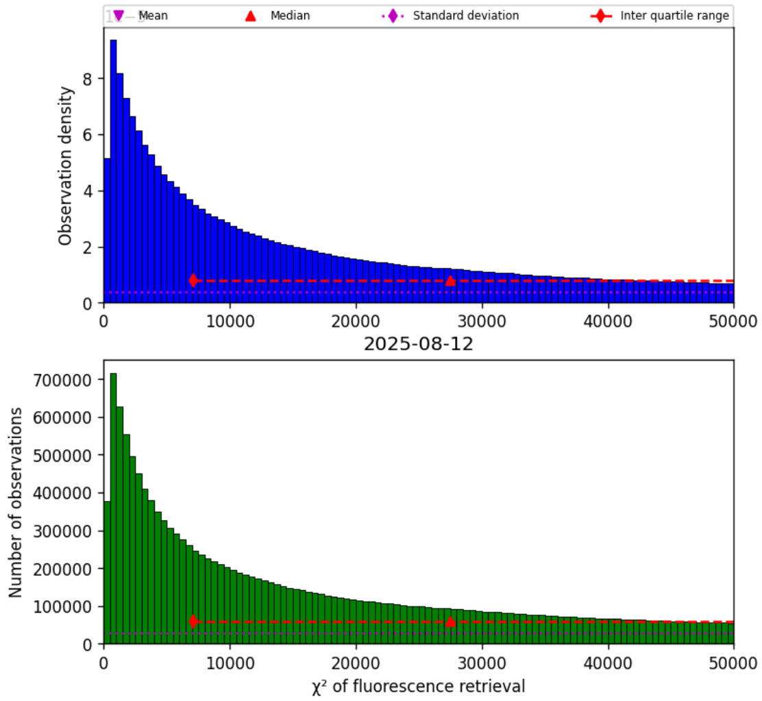
Figure 40: Histogram of “ \chi^2 of fluorescence retrieval” for 2025-08-12 to 2025-08-12
