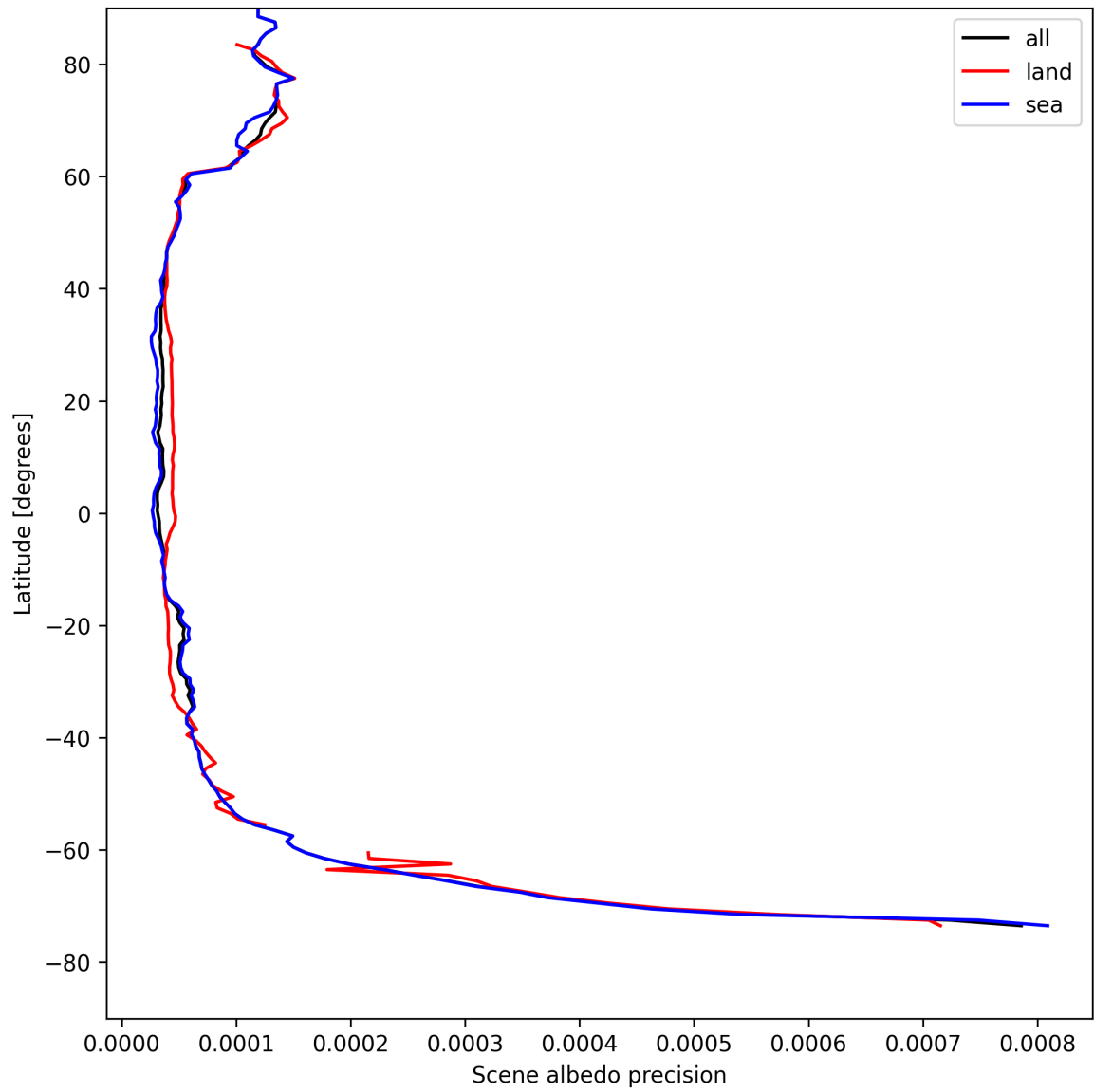
Figure 16: Zonal average of “Scene albedo precision” for 2025-08-12 to 2025-08-12.
