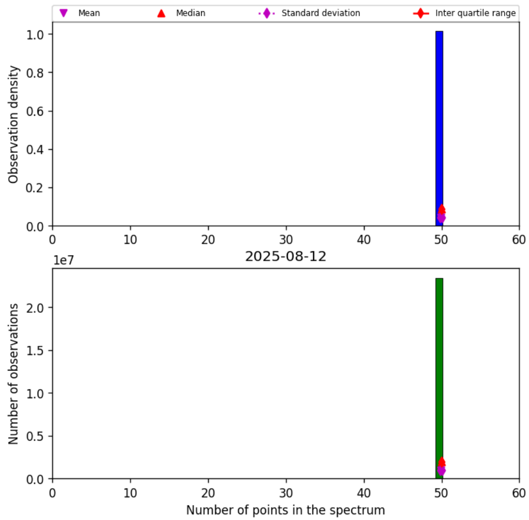
Figure 42: Histogram of “Number of points in the spectrum” for 2025-08-12 to 2025-08-12
