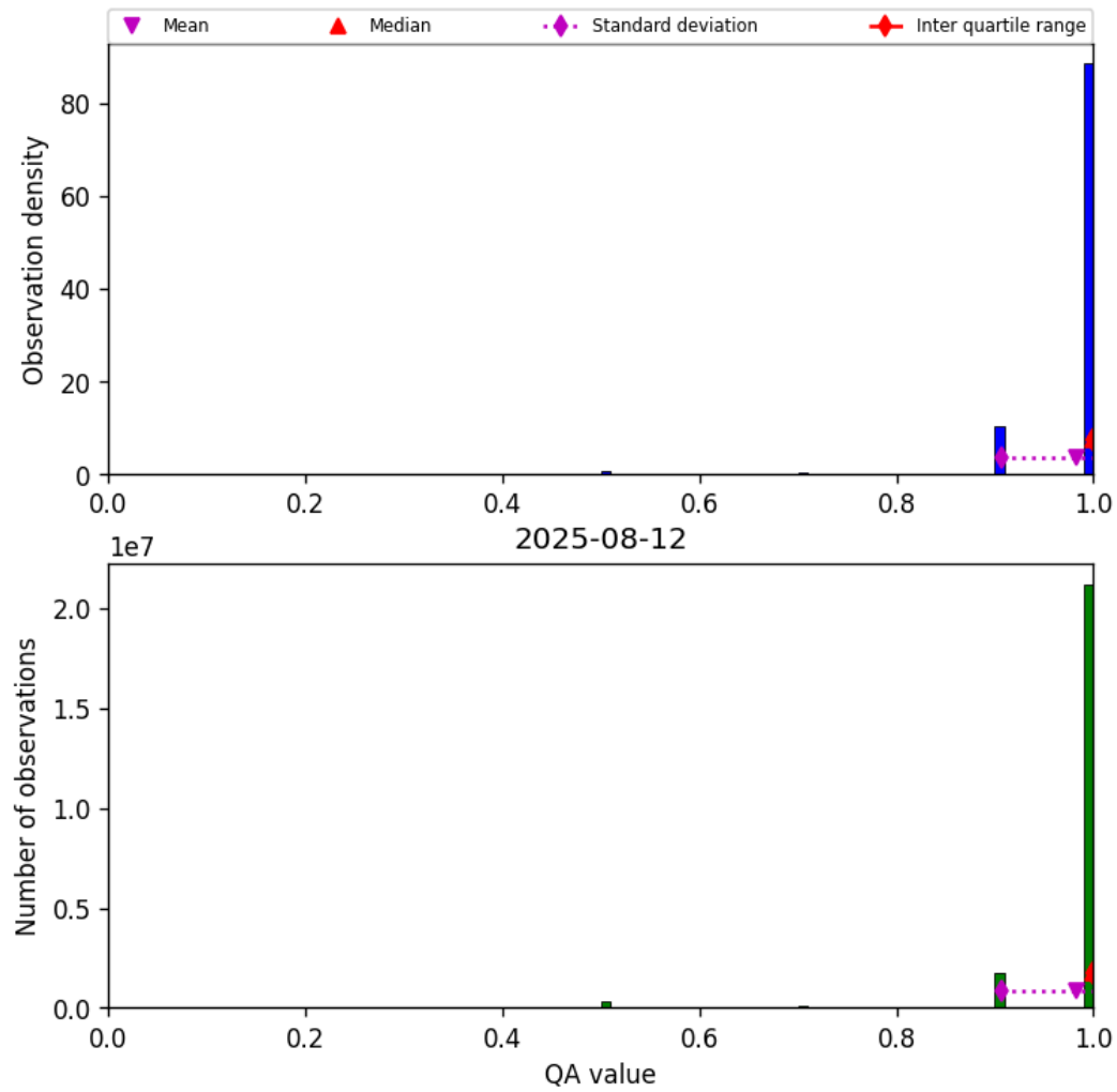
Figure 27: Histogram of “QA value” for 2025-08-12 to 2025-08-12
