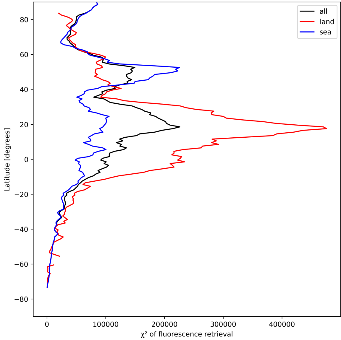
Figure 23: Zonal average of “ \chi^2 of fluorescence retrieval” for 2025-08-12 to 2025-08-12.
