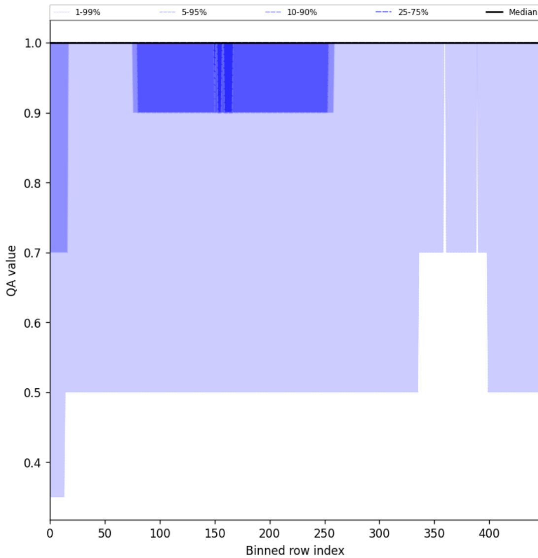
Figure 44: Along track statistics of “QA value” for 2025-08-12 to 2025-08-12
