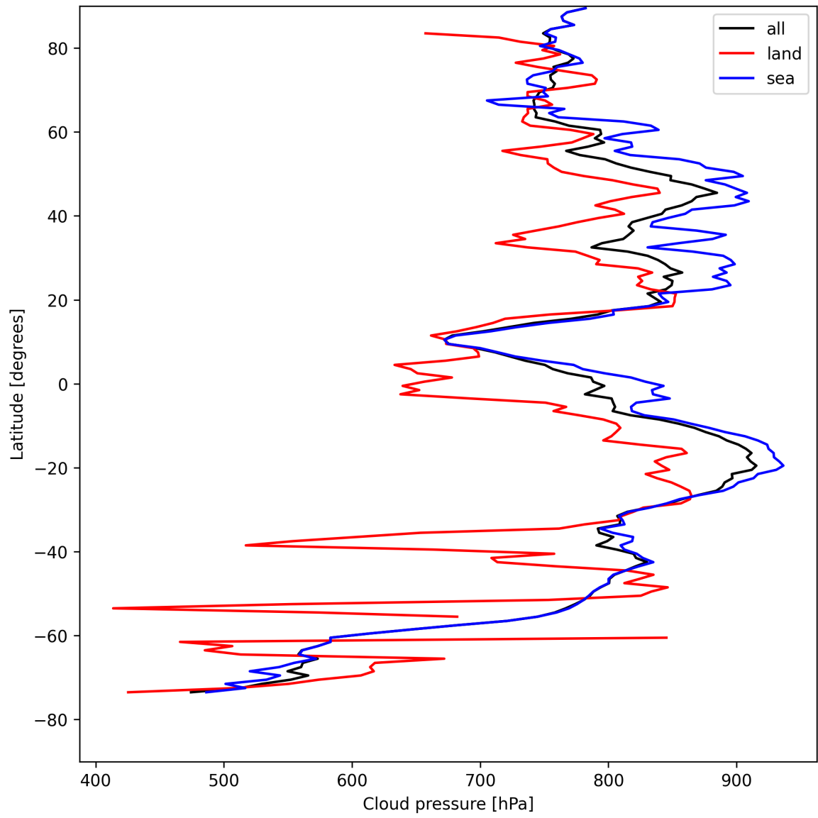
Figure 11: Zonal average of “Cloud pressure” for 2025-08-12 to 2025-08-12.
