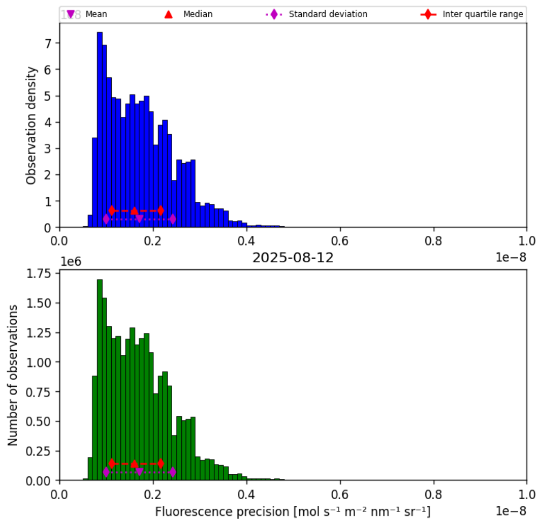
Figure 39: Histogram of “Fluorescence precision” for 2025-08-12 to 2025-08-12
