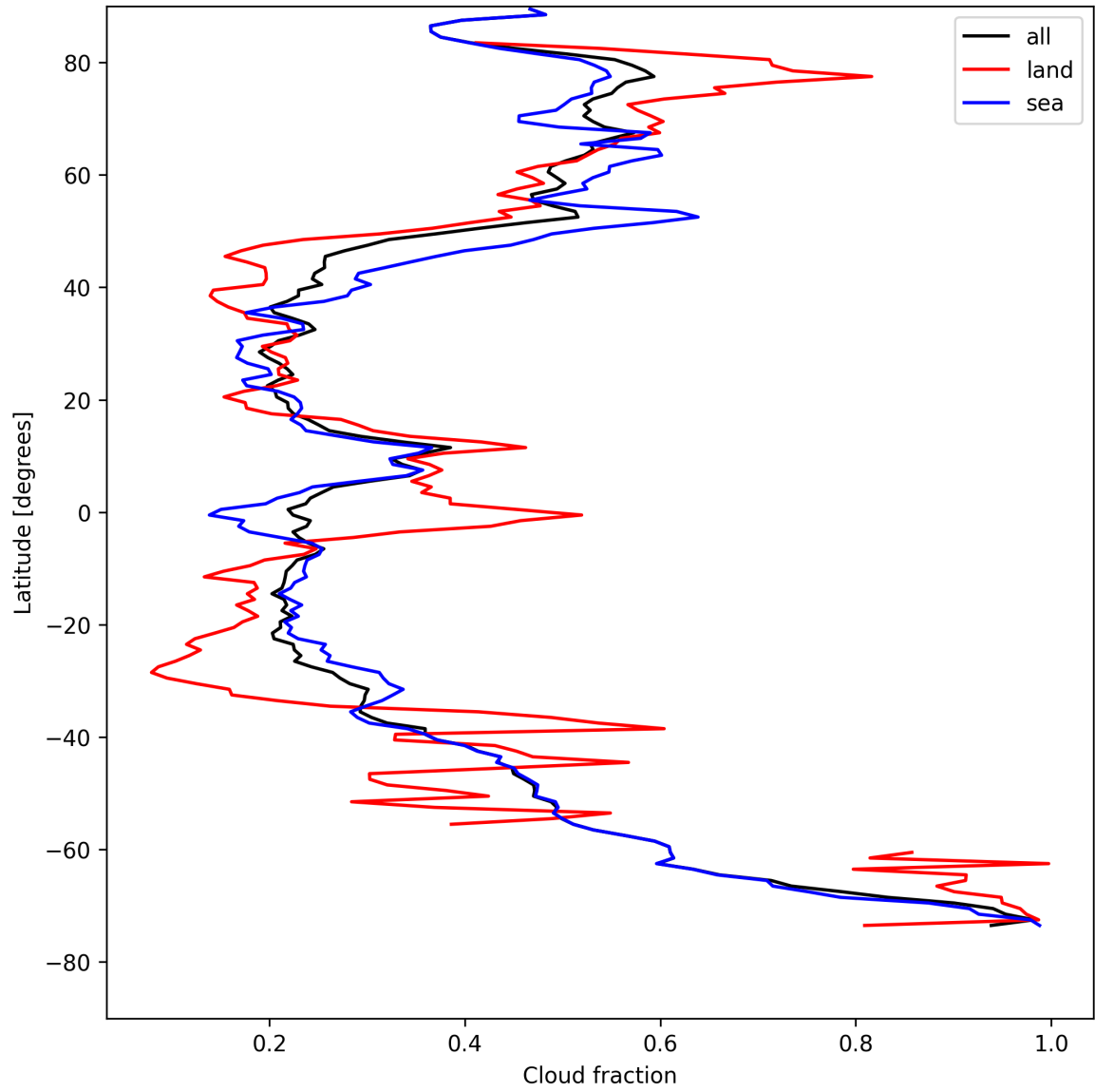
Figure 13: Zonal average of “Cloud fraction” for 2025-08-12 to 2025-08-12.
