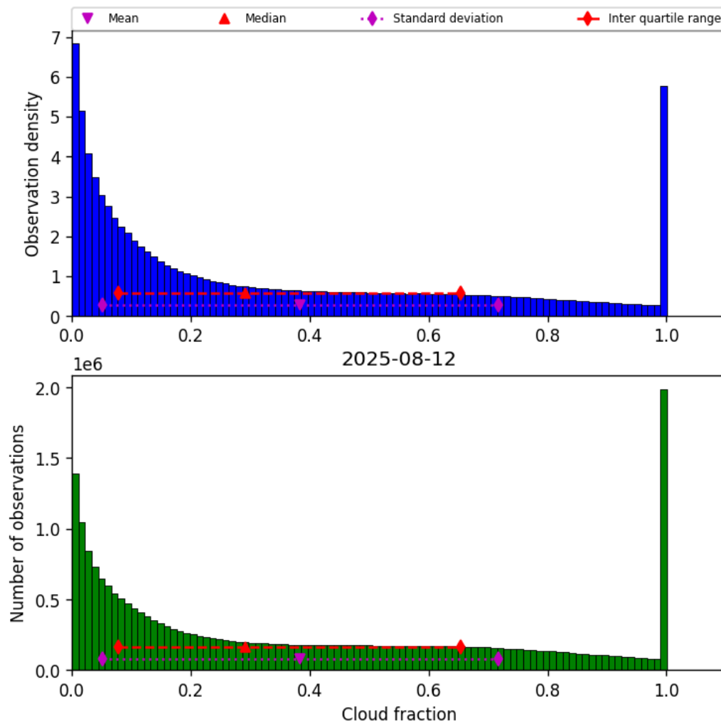
Figure 30: Histogram of “Cloud fraction” for 2025-08-12 to 2025-08-12
