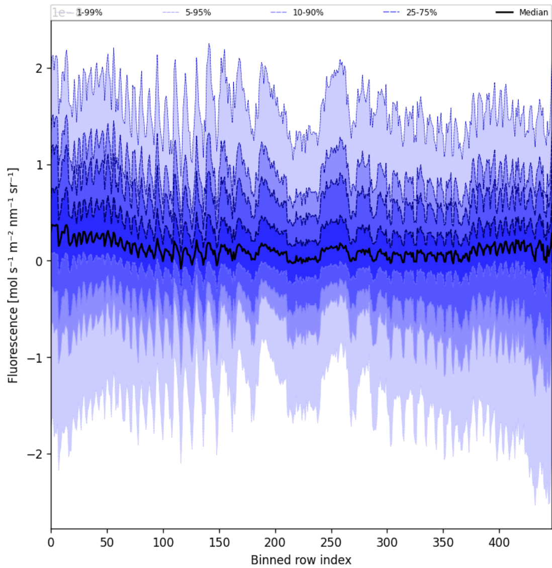
Figure 55: Along track statistics of “Fluorescence” for 2025-08-12 to 2025-08-12
