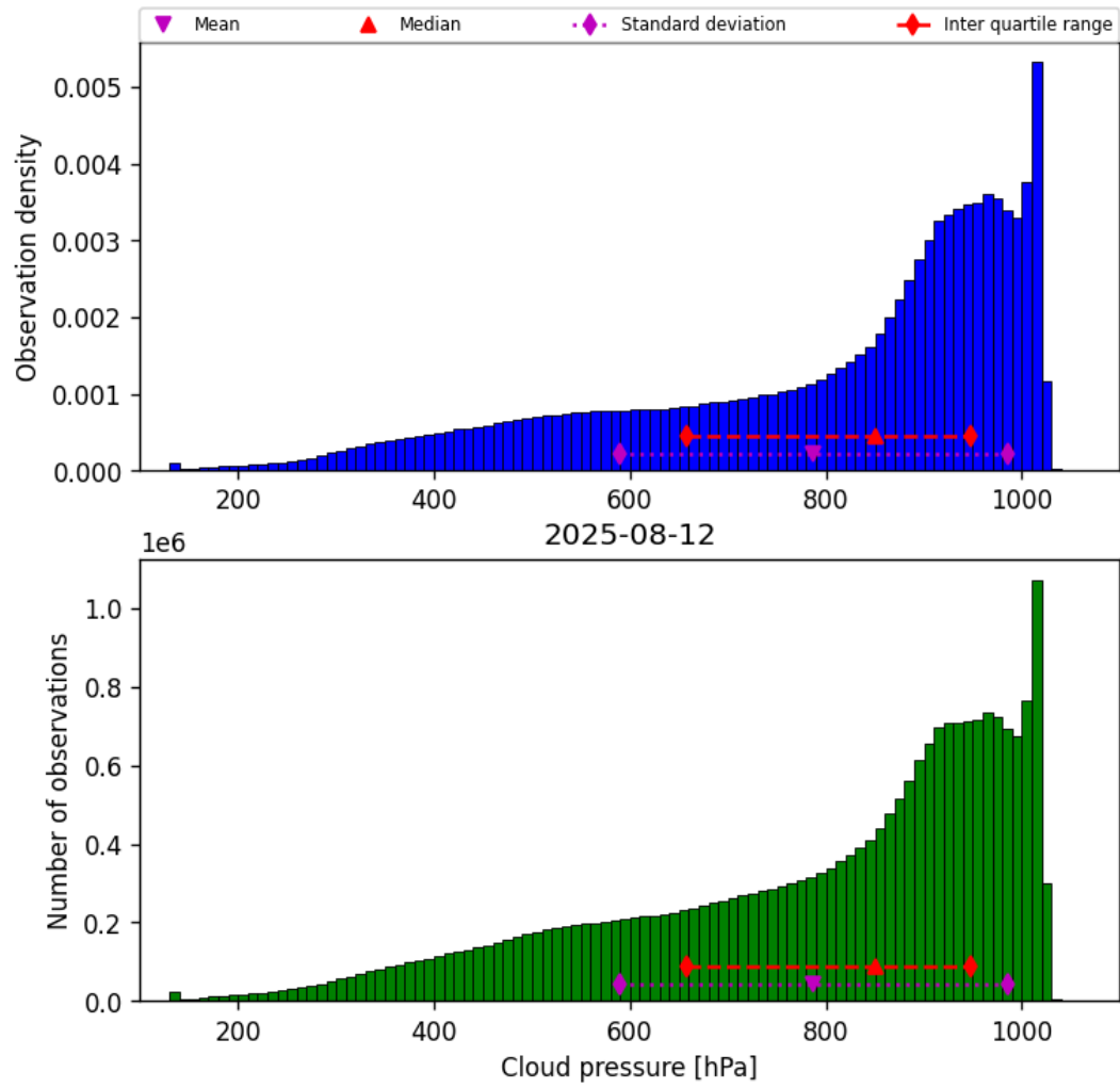
Figure 28: Histogram of “Cloud pressure” for 2025-08-12 to 2025-08-12
