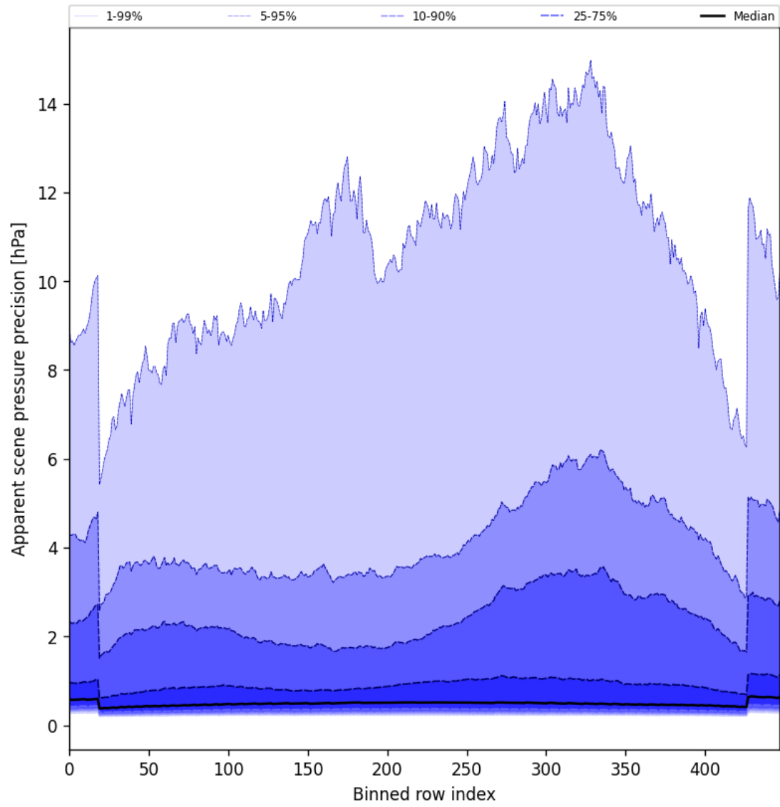
Figure 52: Along track statistics of “Apparent scene pressure precision” for 2025-08-12 to 2025-08-12
