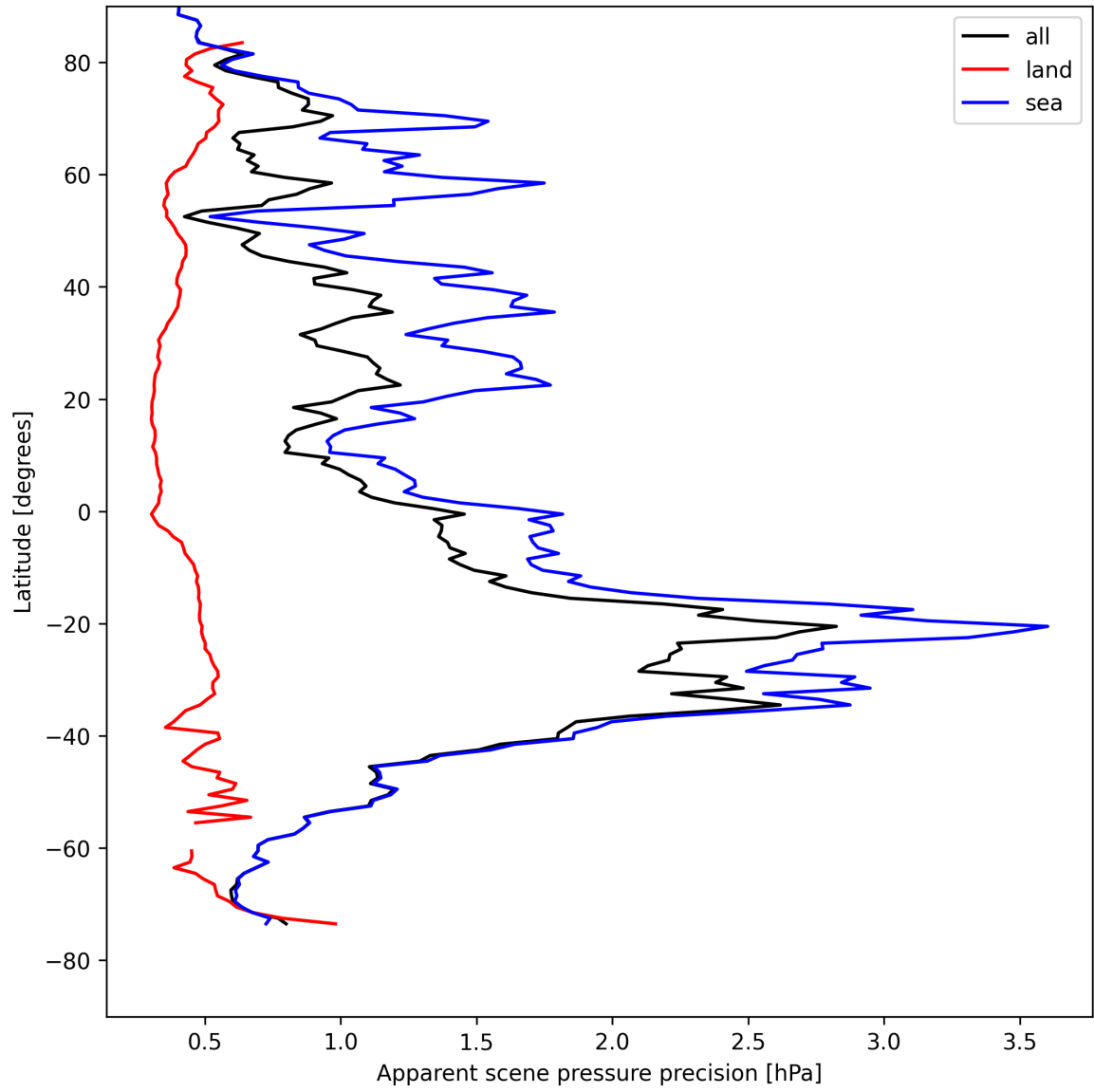
Figure 18: Zonal average of “Apparent scene pressure precision” for 2025-08-12 to 2025-08-12.
