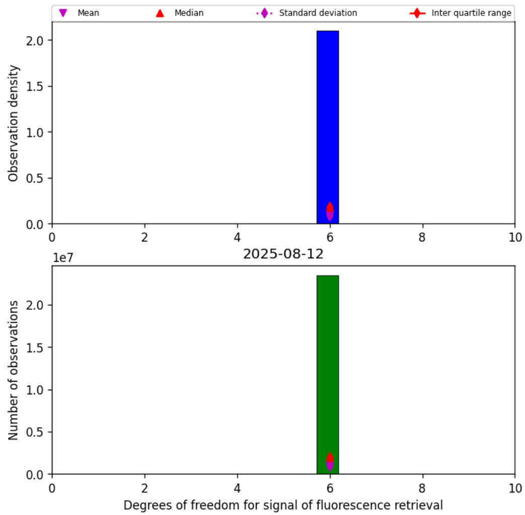
Figure 41: Histogram of “Degrees of freedom for signal of fluorescence retrieval” for 2025-08-12 to 2025-08-12
