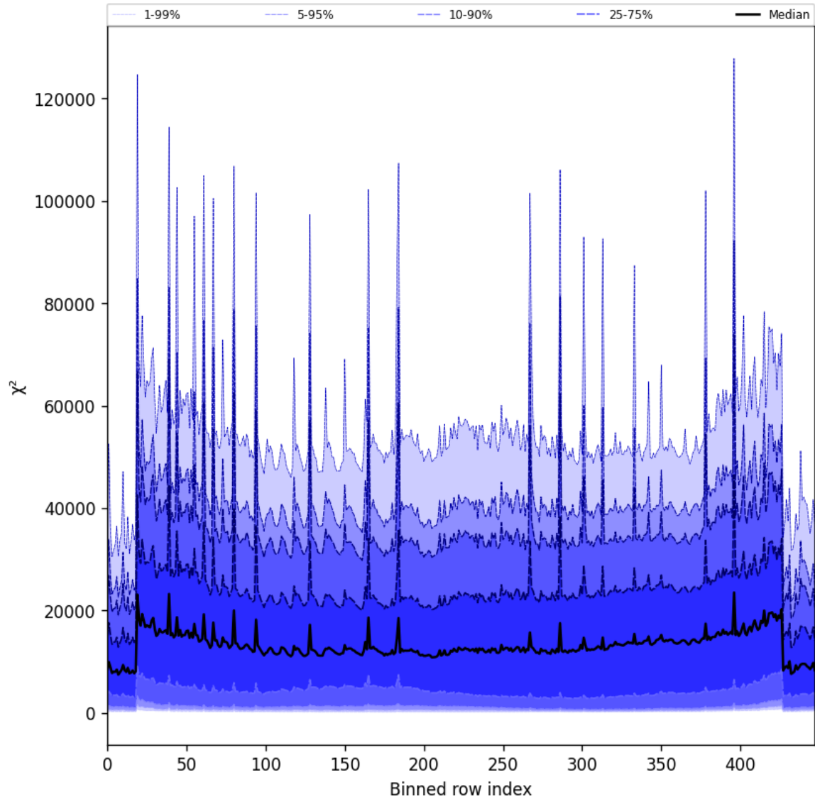
Figure 53: Along track statistics of “ \chi^2 ” for 2025-08-12 to 2025-08-12
