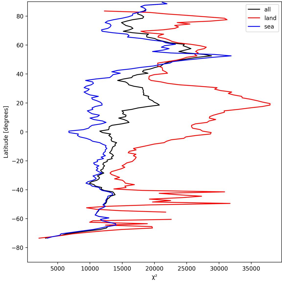
Figure 19: Zonal average of “ \chi^2 ” for 2025-08-12 to 2025-08-12.
