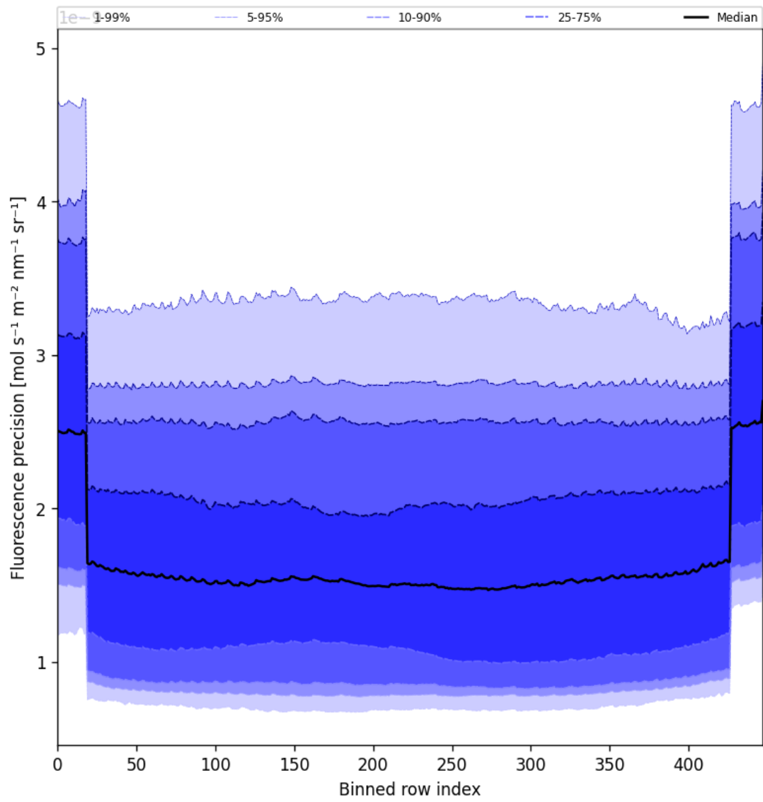
Figure 56: Along track statistics of “Fluorescence precision” for 2025-08-12 to 2025-08-12
