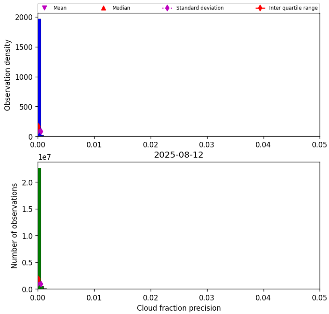
Figure 31: Histogram of “Cloud fraction precision” for 2025-08-12 to 2025-08-12
