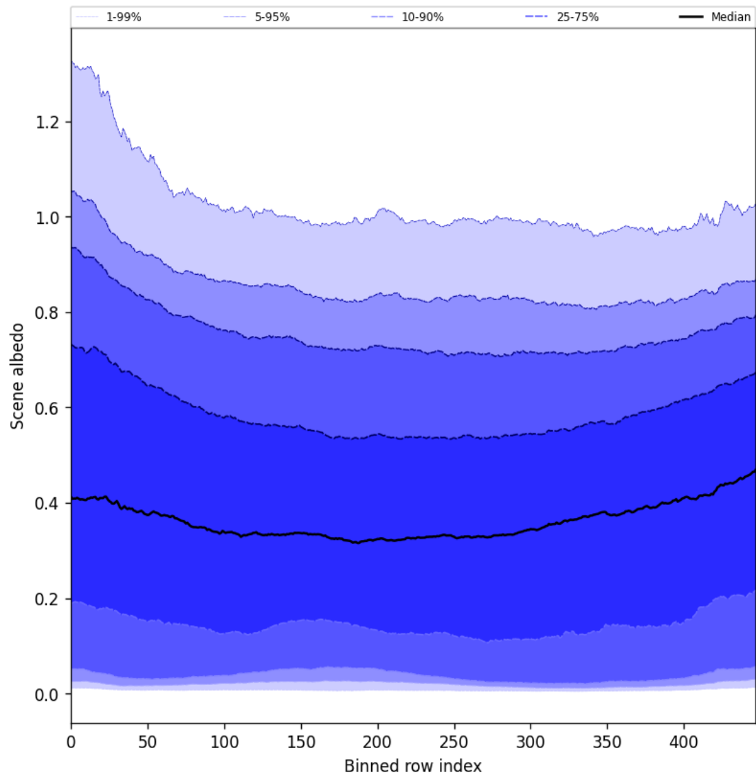
Figure 49: Along track statistics of “Scene albedo” for 2025-08-12 to 2025-08-12
