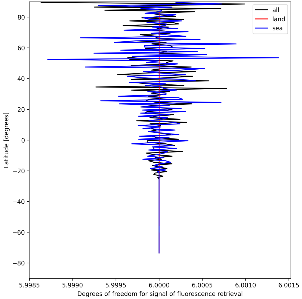
Figure 24: Zonal average of "Degrees of freedom for signal of fluorescence retrieval" for 2025-08-14 to 2025-08-15.
