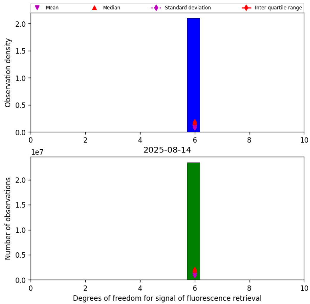
Figure 41: Histogram of “Degrees of freedom for signal of fluorescence retrieval” for 2025-08-14 to 2025-08-15
