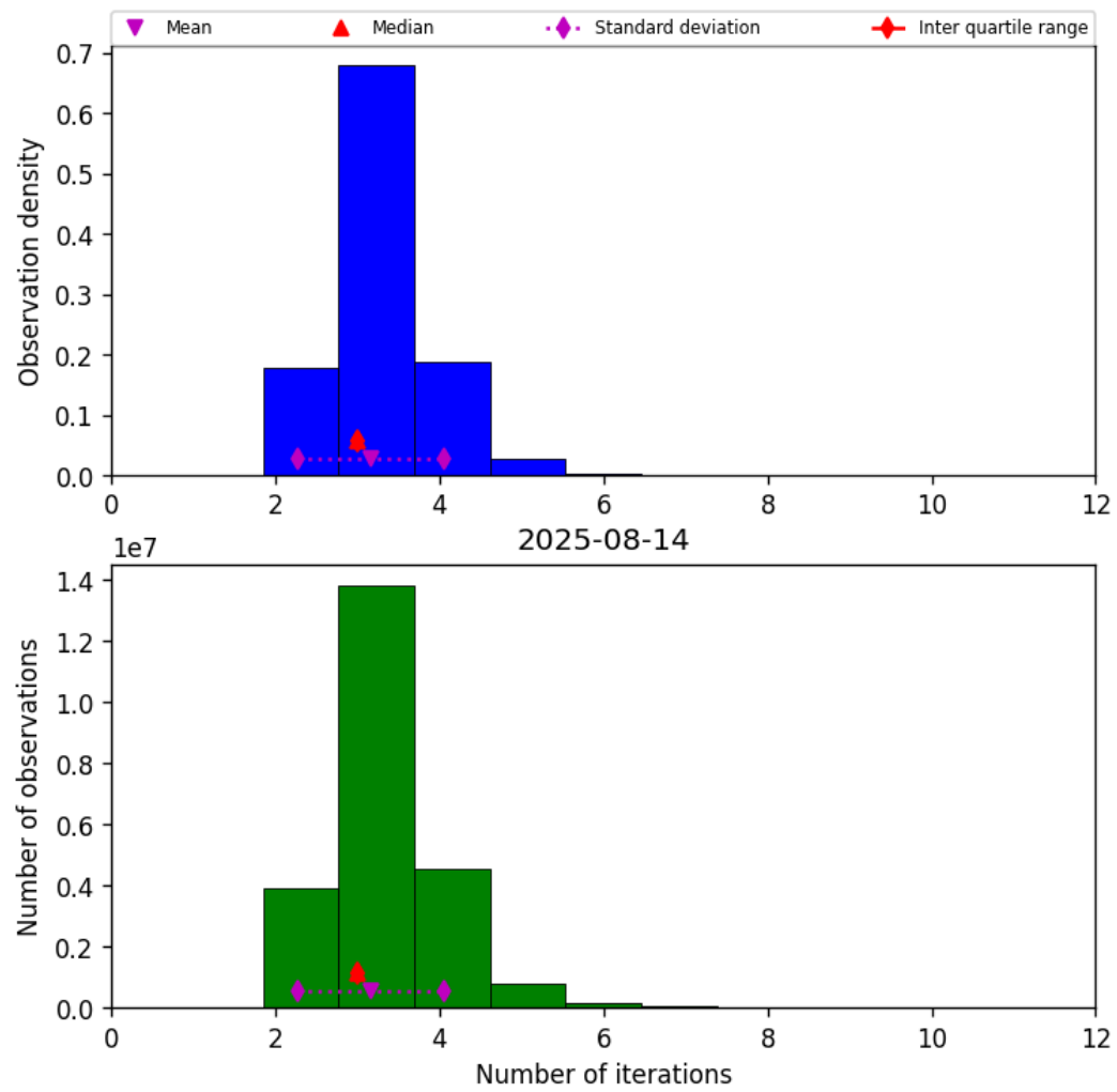
Figure 37: Histogram of “Number of iterations” for 2025-08-14 to 2025-08-15
