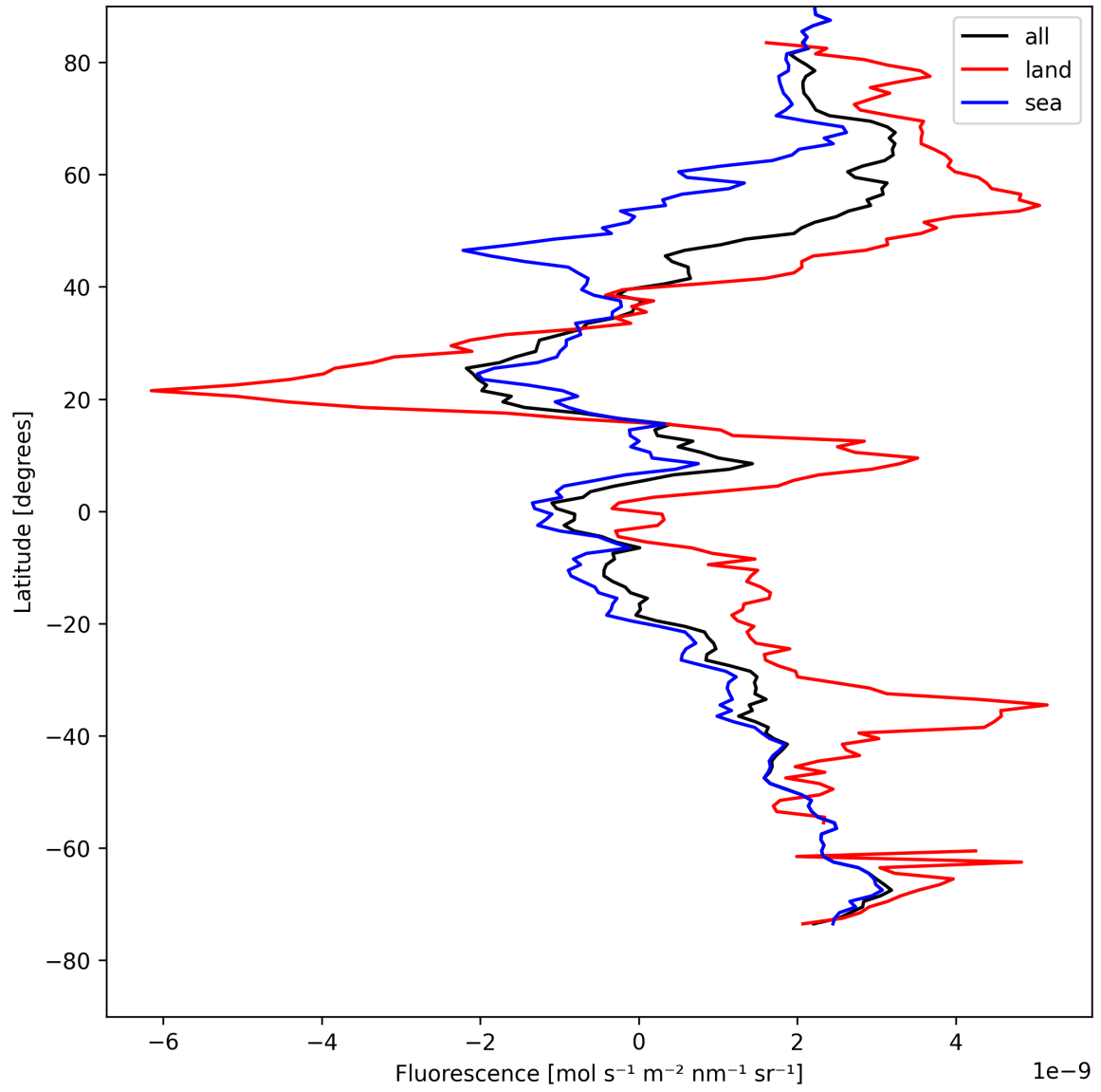
Figure 21: Zonal average of “Fluorescence” for 2025-08-14 to 2025-08-15.
