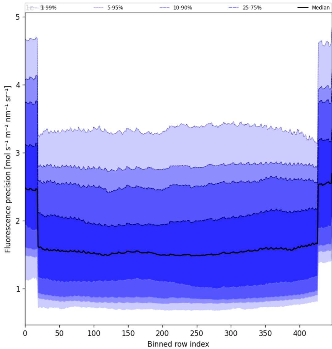
Figure 56: Along track statistics of “Fluorescence precision” for 2025-08-14 to 2025-08-15
