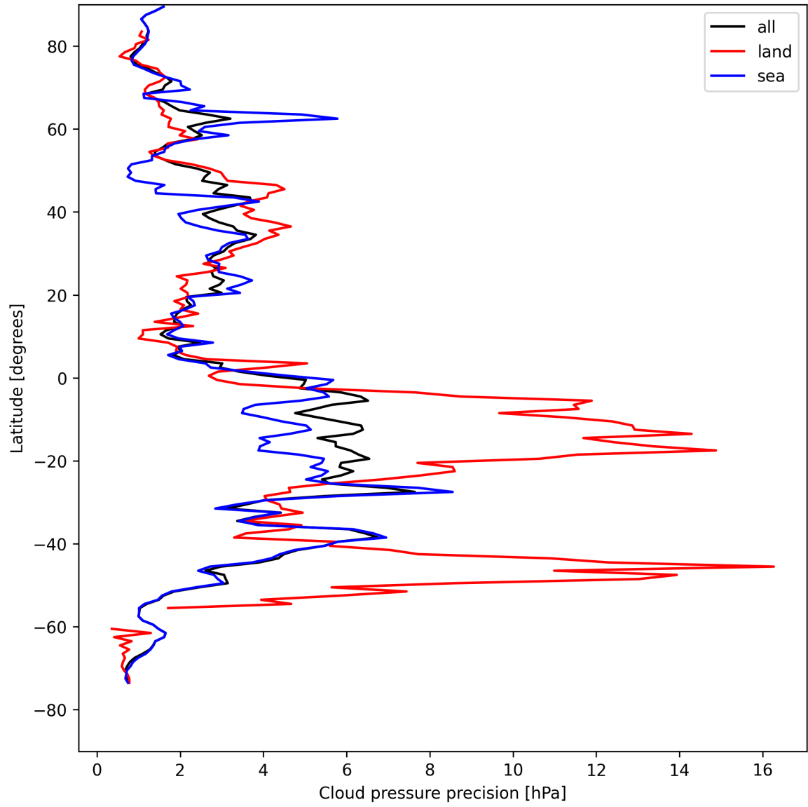
Figure 12: Zonal average of “Cloud pressure precision” for 2025-08-14 to 2025-08-15.
