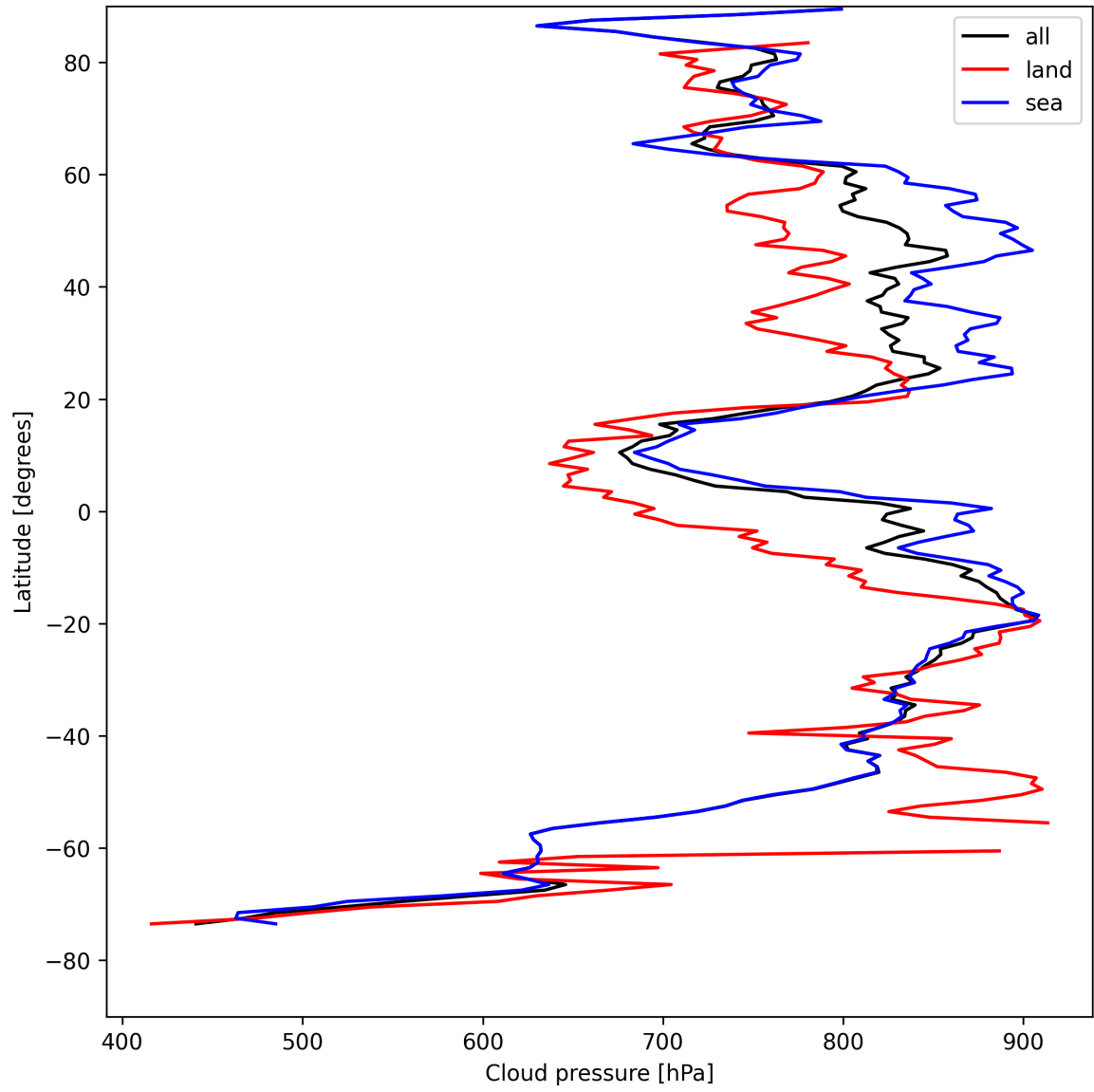
Figure 11: Zonal average of “Cloud pressure” for 2025-08-14 to 2025-08-15.
