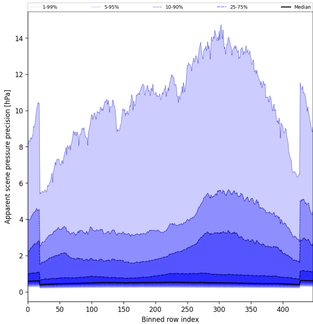
Figure 52: Along track statistics of “Apparent scene pressure precision” for 2025-08-14 to 2025-08-15
