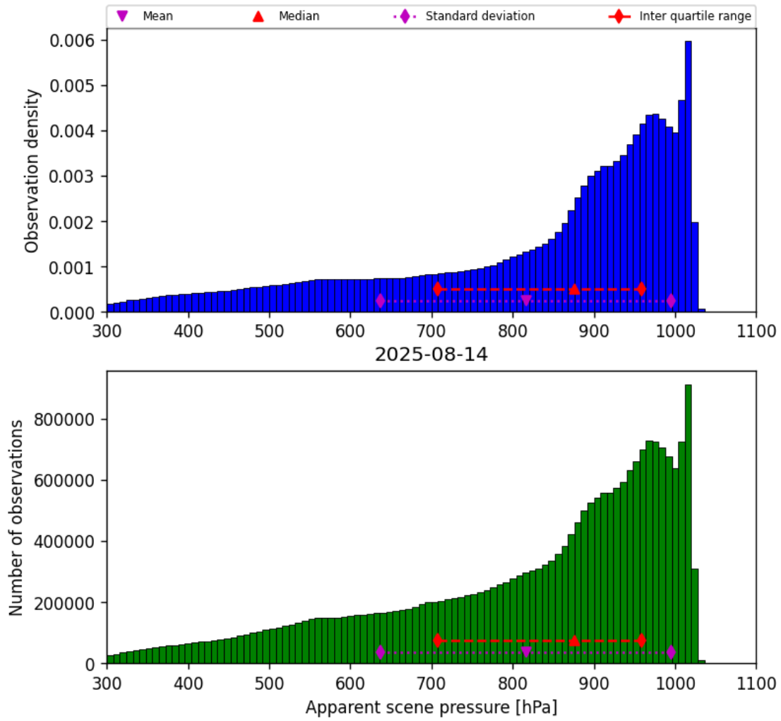
Figure 34: Histogram of “Apparent scene pressure” for 2025-08-14 to 2025-08-15
