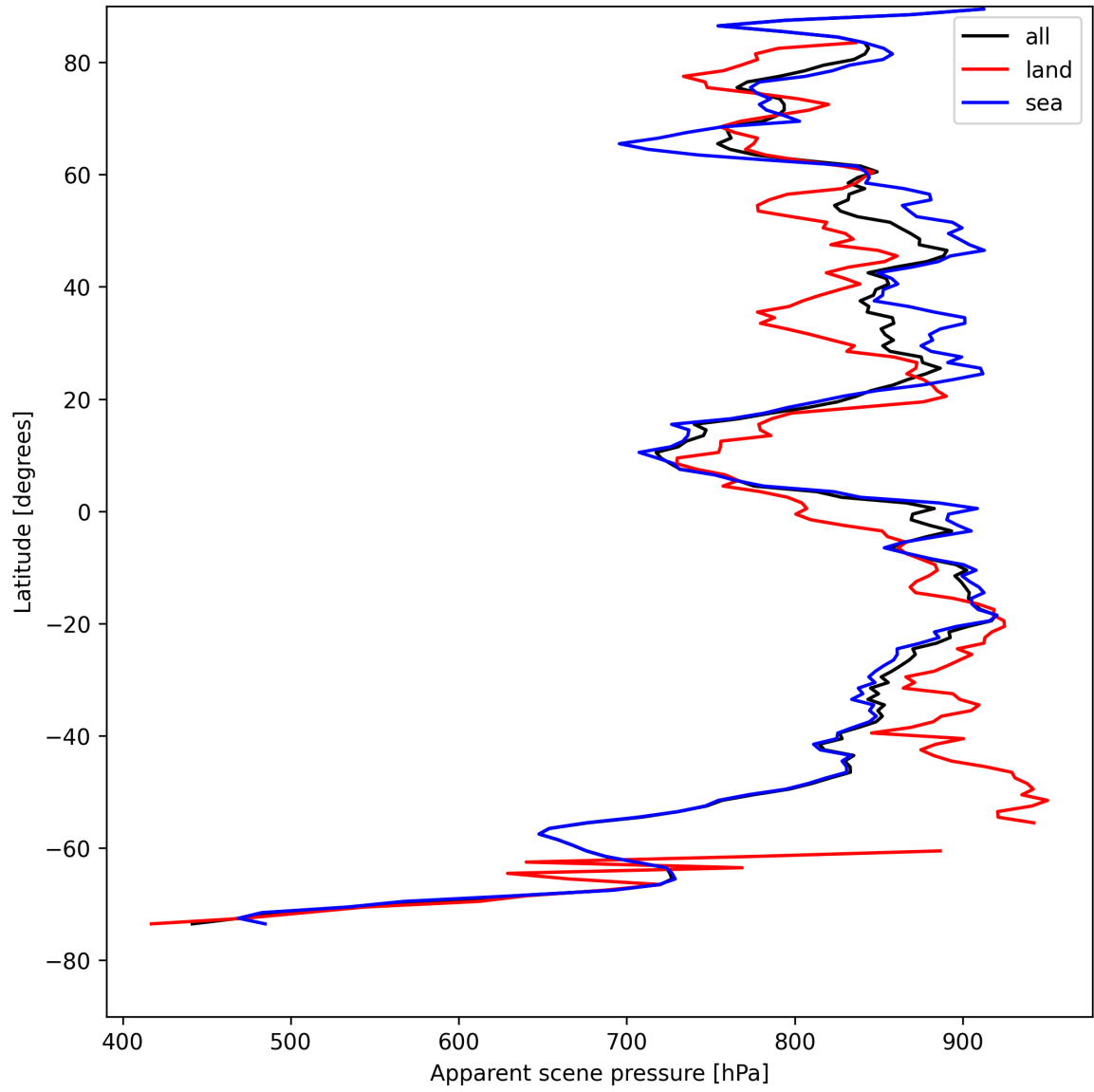
Figure 17: Zonal average of “Apparent scene pressure” for 2025-08-14 to 2025-08-15.
