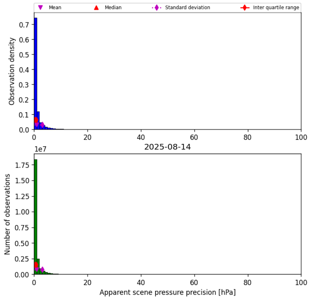
Figure 35: Histogram of “Apparent scene pressure precision” for 2025-08-14 to 2025-08-15
