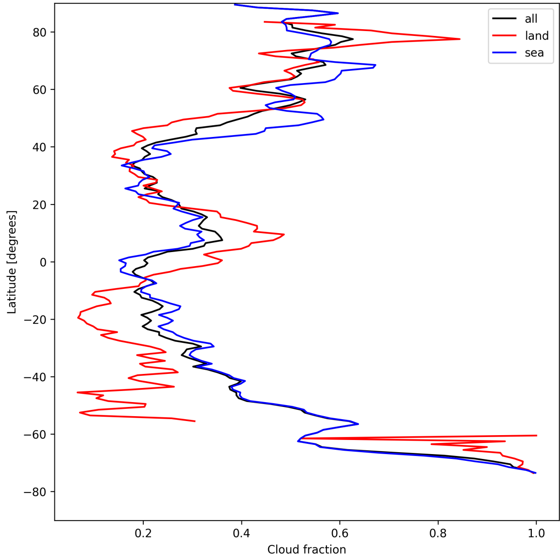
Figure 13: Zonal average of “Cloud fraction” for 2025-08-14 to 2025-08-15.
