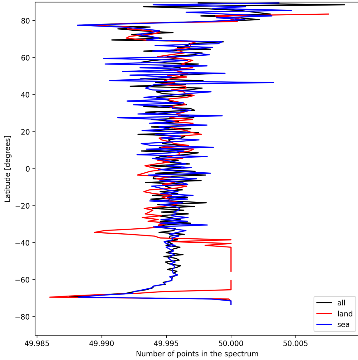
Figure 25: Zonal average of “Number of points in the spectrum” for 2025-08-14 to 2025-08-15.
