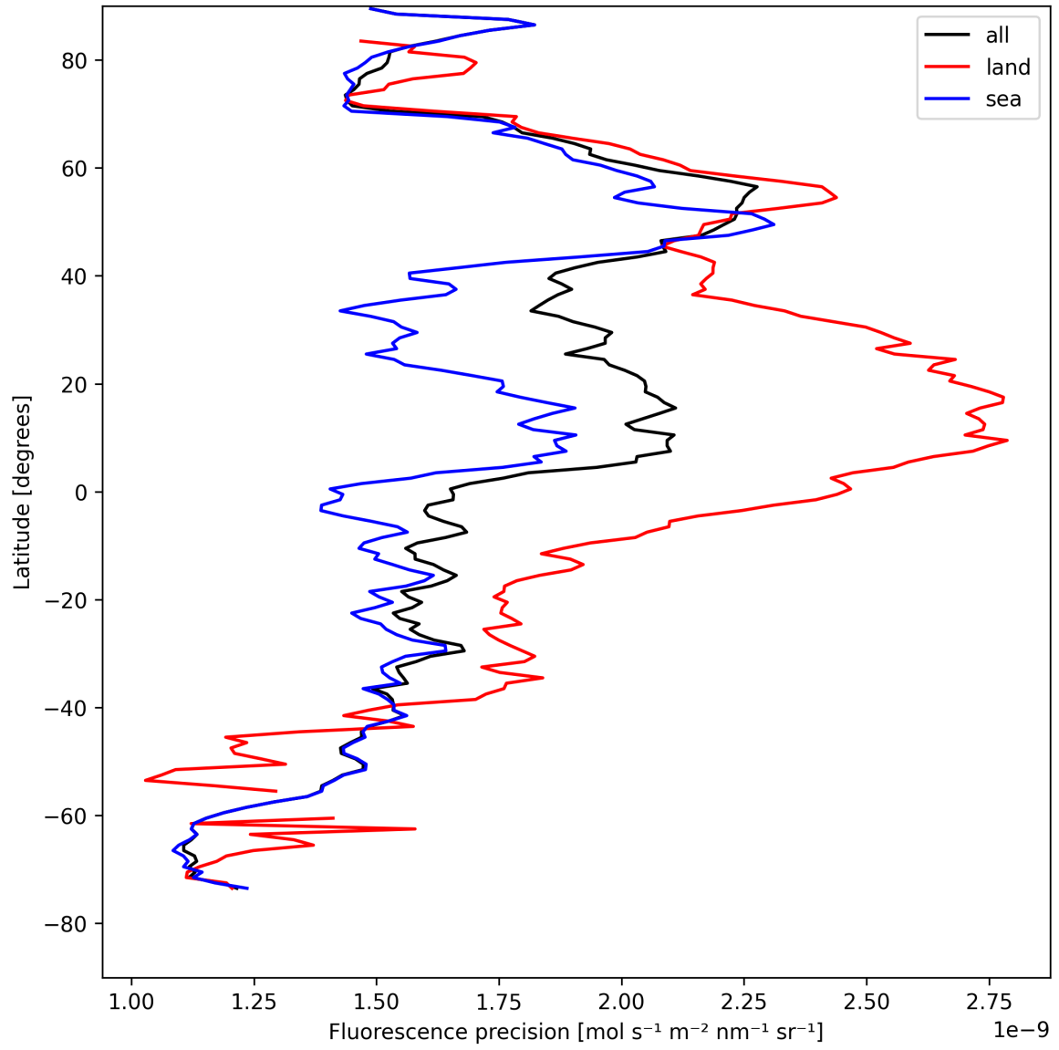
Figure 22: Zonal average of “Fluorescence precision” for 2025-08-14 to 2025-08-15.
