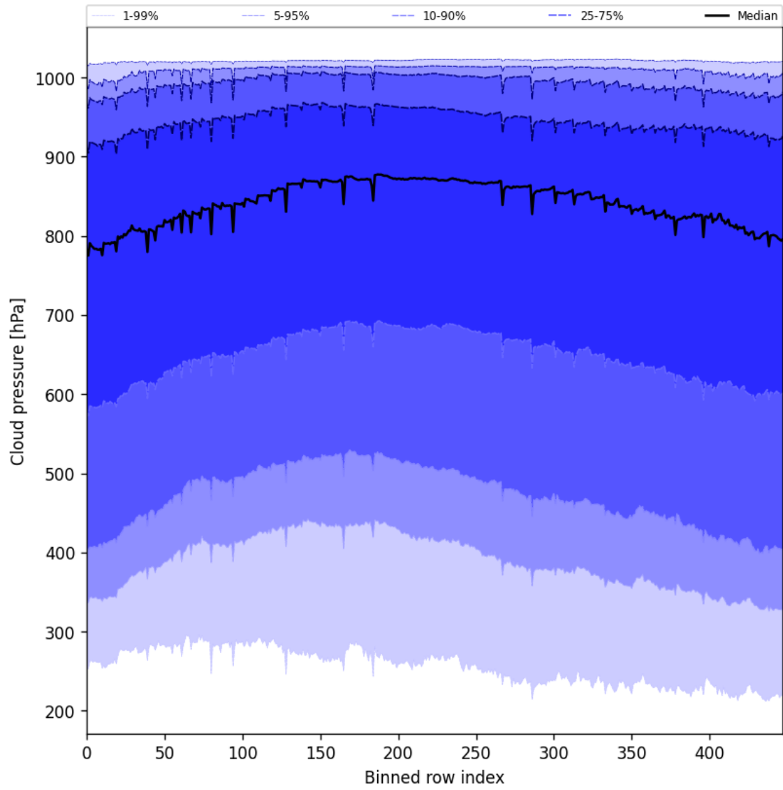
Figure 45: Along track statistics of “Cloud pressure” for 2025-08-14 to 2025-08-15
