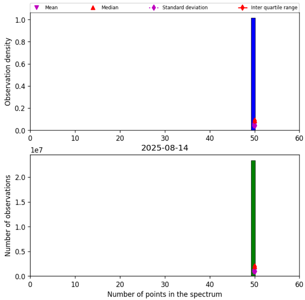
Figure 42: Histogram of “Number of points in the spectrum” for 2025-08-14 to 2025-08-15
