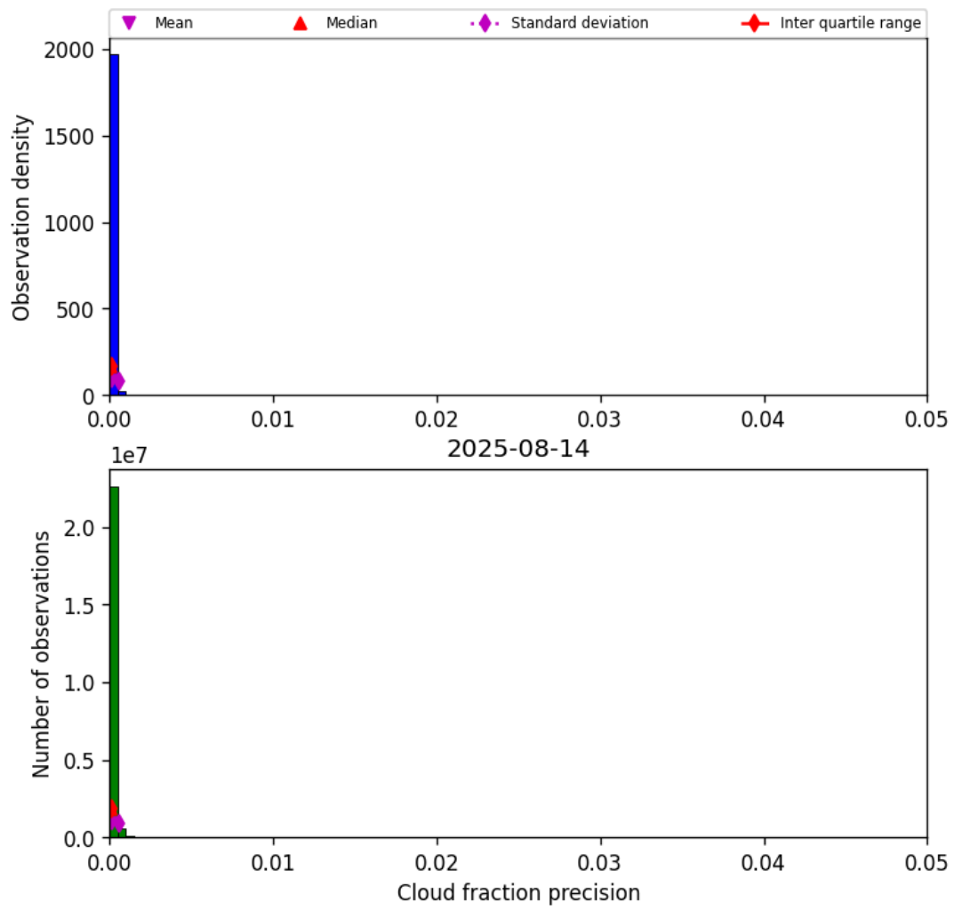
Figure 31: Histogram of “Cloud fraction precision” for 2025-08-14 to 2025-08-15
