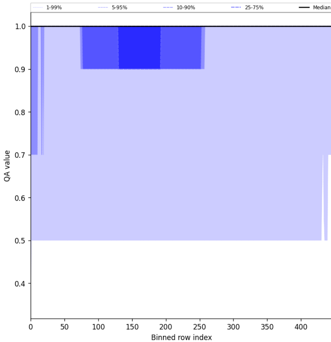
Figure 44: Along track statistics of “QA value” for 2025-08-15 to 2025-08-16
