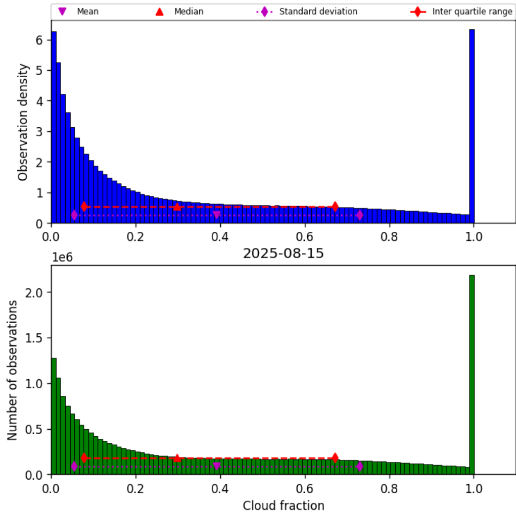
Figure 30: Histogram of “Cloud fraction” for 2025-08-15 to 2025-08-16
