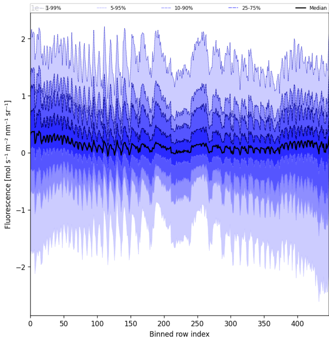
Figure 55: Along track statistics of “Fluorescence” for 2025-08-15 to 2025-08-16
