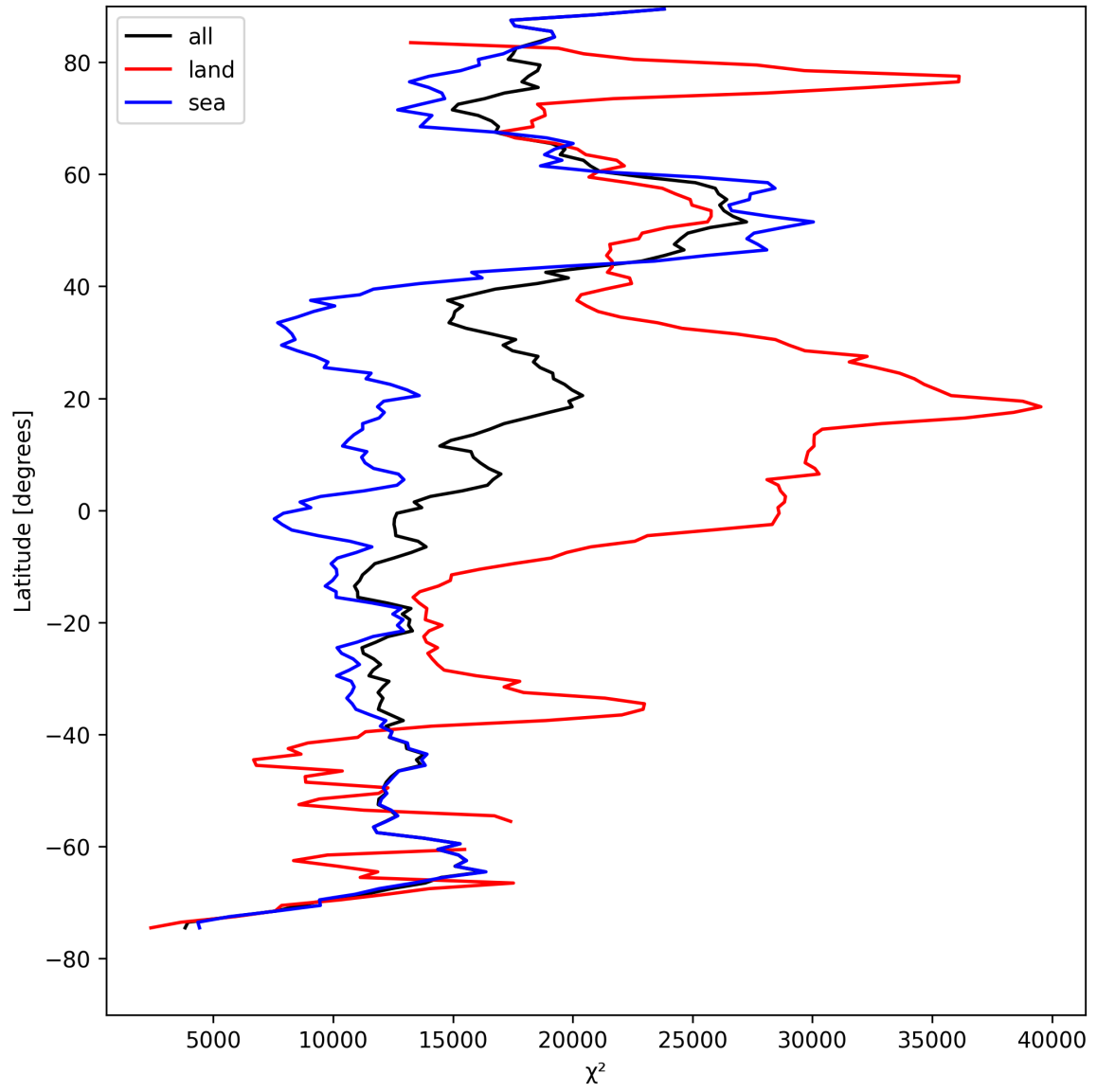
Figure 19: Zonal average of “ \chi^2 ” for 2025-08-15 to 2025-08-16.
