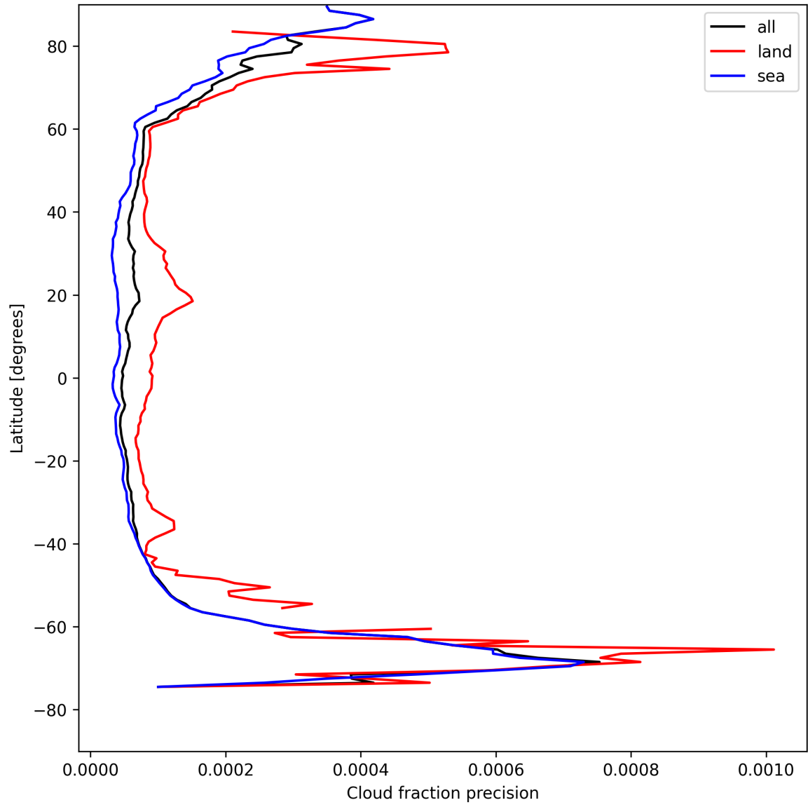
Figure 14: Zonal average of “Cloud fraction precision” for 2025-08-15 to 2025-08-16.
