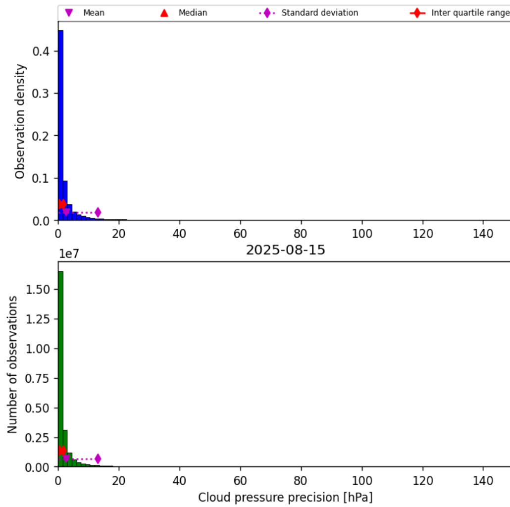
Figure 29: Histogram of “Cloud pressure precision” for 2025-08-15 to 2025-08-16
