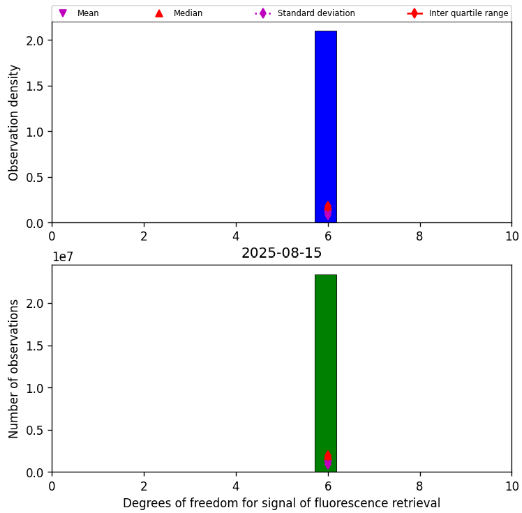
Figure 41: Histogram of “Degrees of freedom for signal of fluorescence retrieval” for 2025-08-15 to 2025-08-16
