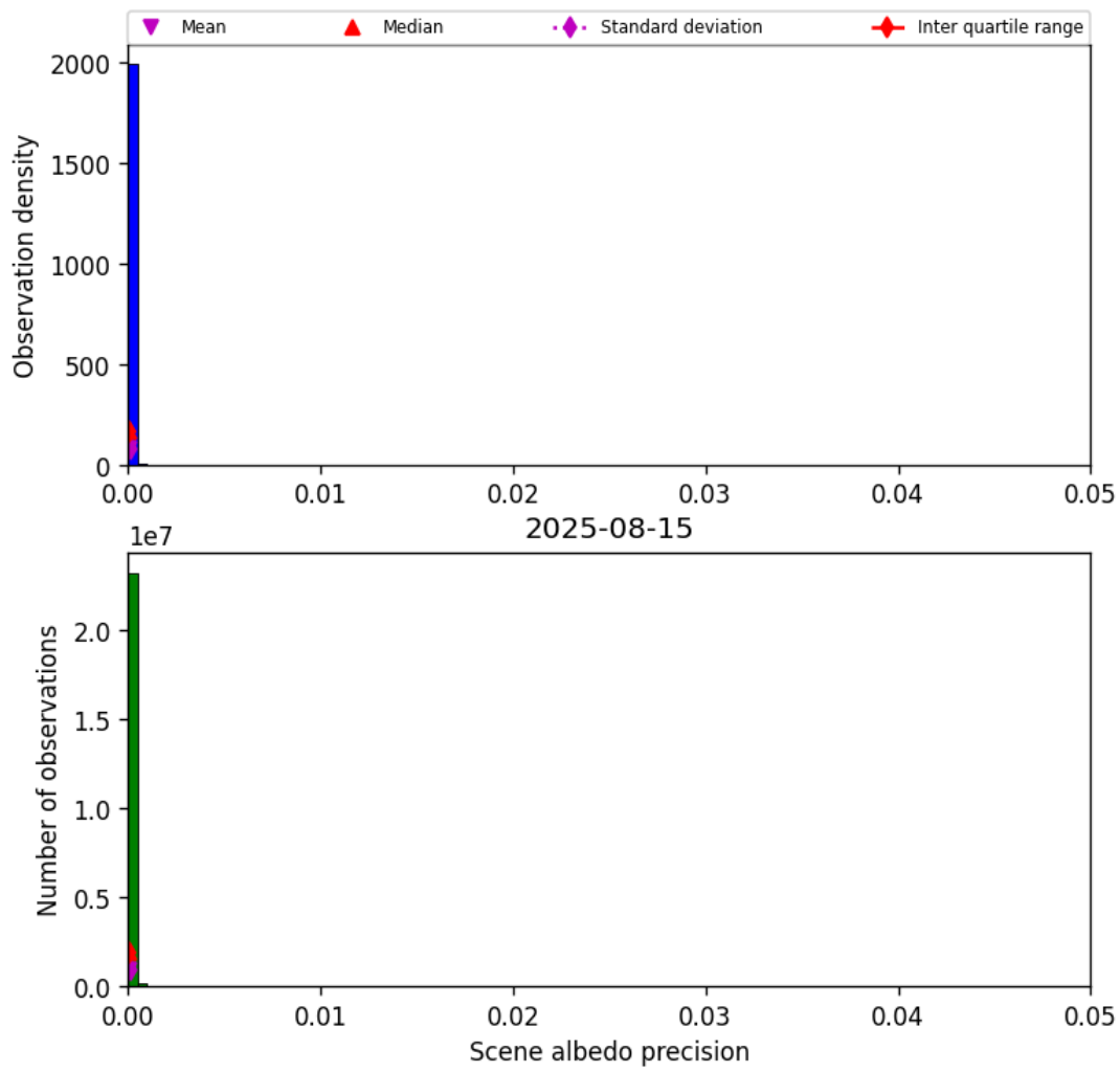
Figure 33: Histogram of “Scene albedo precision” for 2025-08-15 to 2025-08-16
