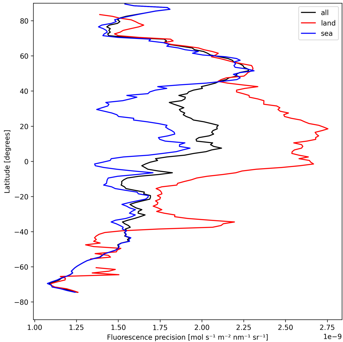
Figure 22: Zonal average of “Fluorescence precision” for 2025-08-15 to 2025-08-16.
