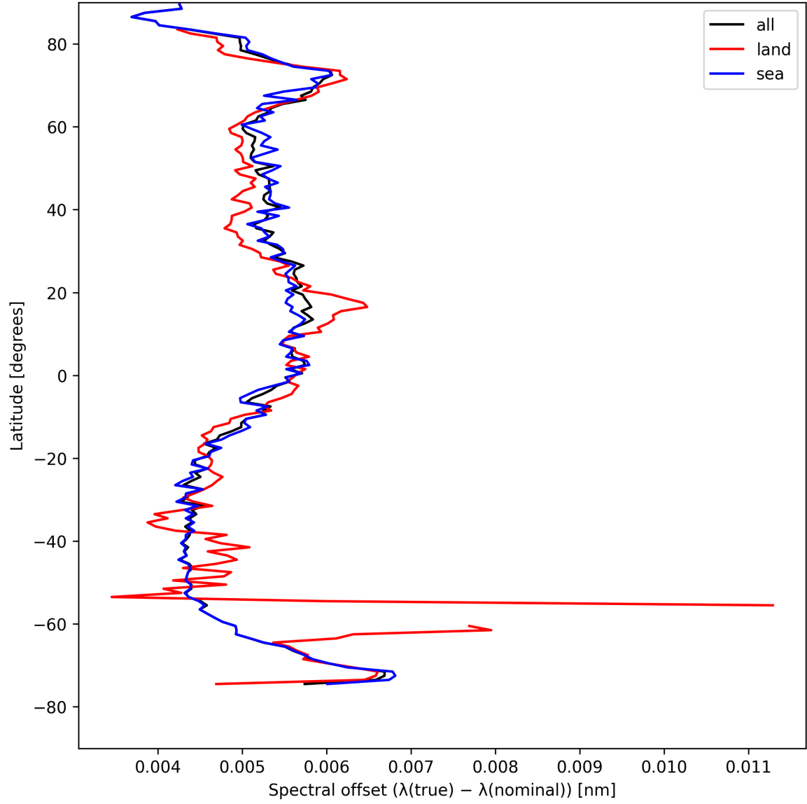
Figure 26: Zonal average of “Spectral offset ( \lambda_{\text{true}} - \lambda_{\text{nominal}} )” for 2025-08-15 to 2025-08-16.
