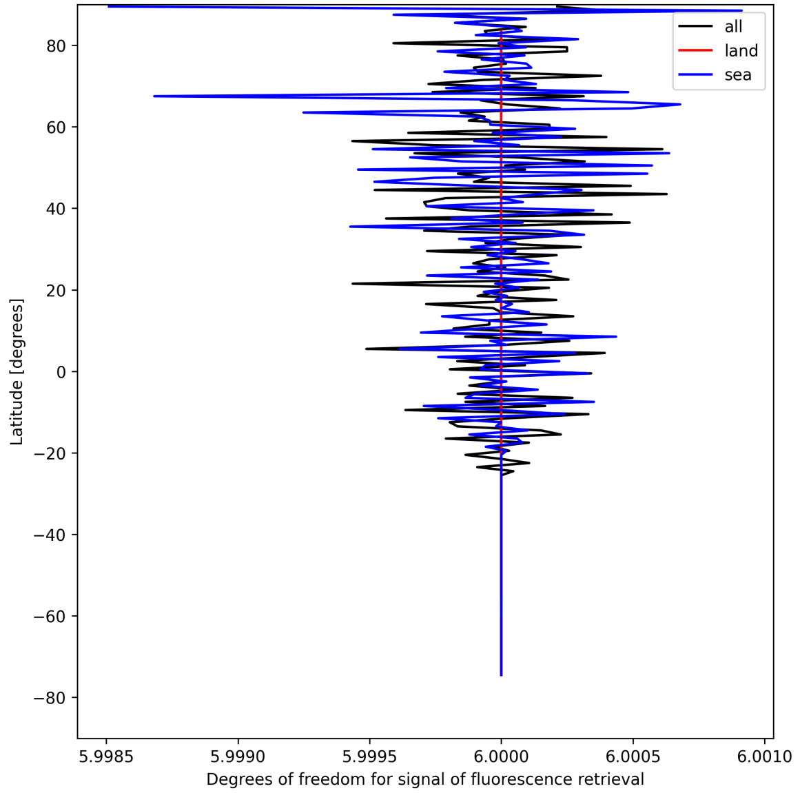
Figure 24: Zonal average of “Degrees of freedom for signal of fluorescence retrieval” for 2025-08-15 to 2025-08-16.
