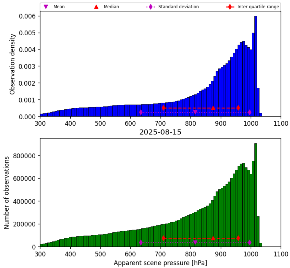
Figure 34: Histogram of “Apparent scene pressure” for 2025-08-15 to 2025-08-16
