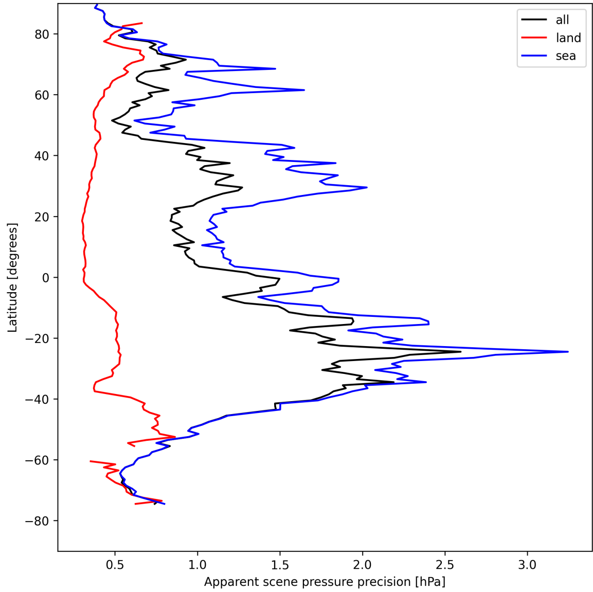
Figure 18: Zonal average of “Apparent scene pressure precision” for 2025-08-15 to 2025-08-16.
