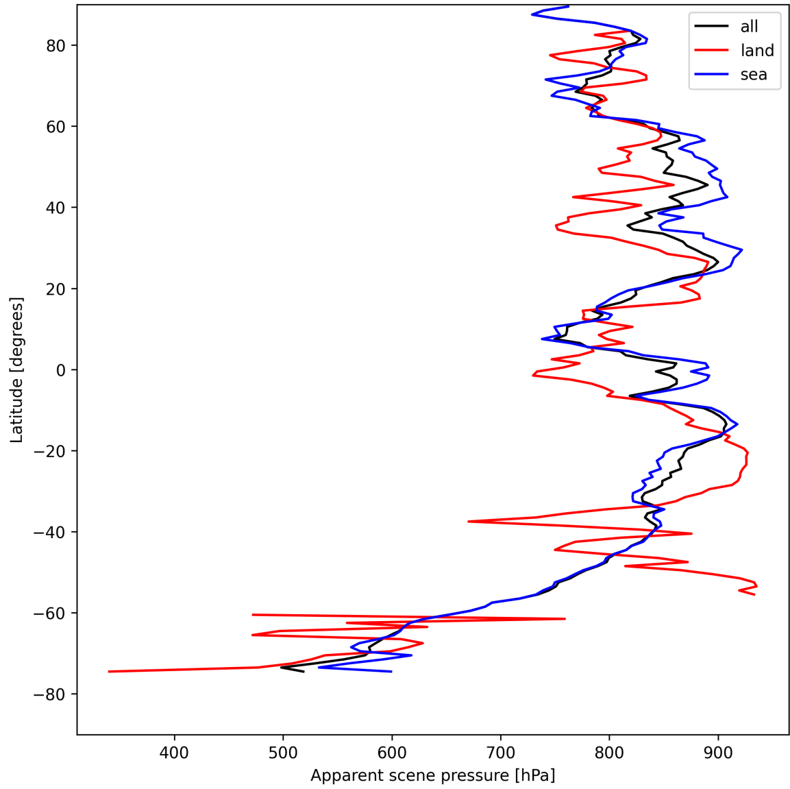
Figure 17: Zonal average of “Apparent scene pressure” for 2025-08-15 to 2025-08-16.
