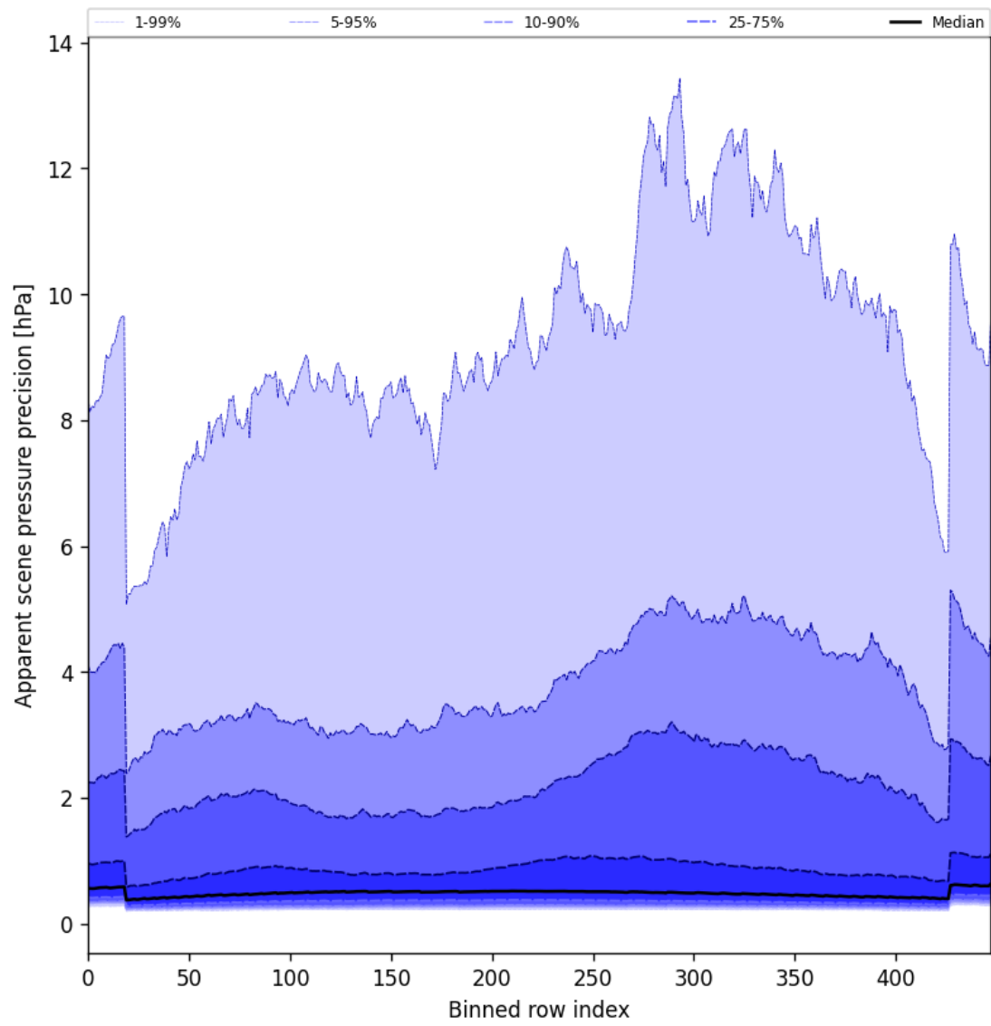
Figure 52: Along track statistics of “Apparent scene pressure precision” for 2025-08-15 to 2025-08-16
