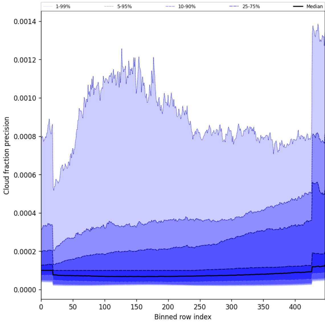
Figure 48: Along track statistics of “Cloud fraction precision” for 2025-08-15 to 2025-08-16
