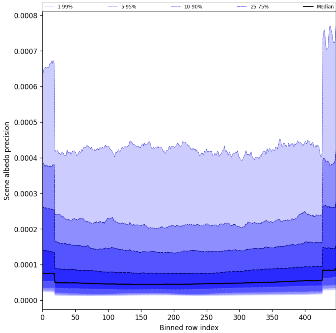
Figure 50: Along track statistics of “Scene albedo precision” for 2025-08-15 to 2025-08-16
