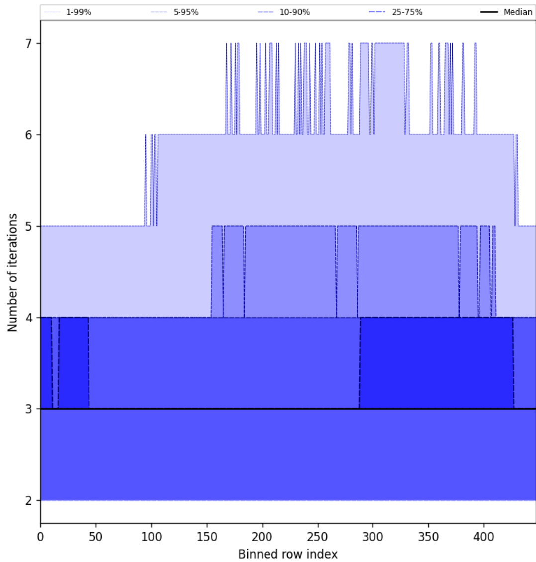
Figure 54: Along track statistics of “Number of iterations” for 2025-08-15 to 2025-08-16
