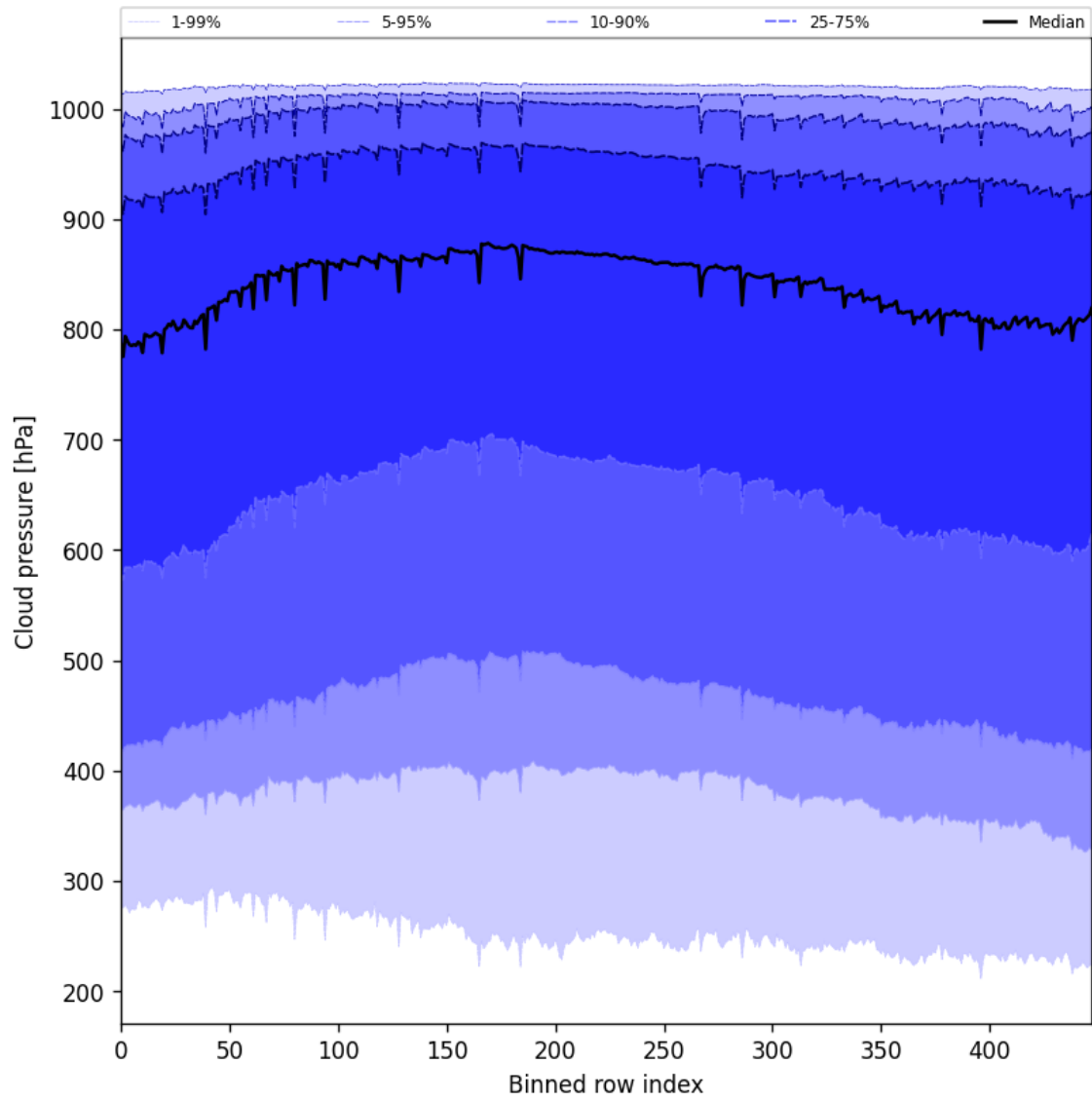
Figure 45: Along track statistics of “Cloud pressure” for 2025-08-15 to 2025-08-16
