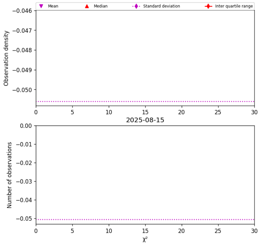
Figure 36: Histogram of " \chi^2 " for 2025-08-15 to 2025-08-16
