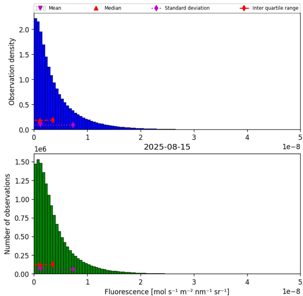
Figure 38: Histogram of “Fluorescence” for 2025-08-15 to 2025-08-16
