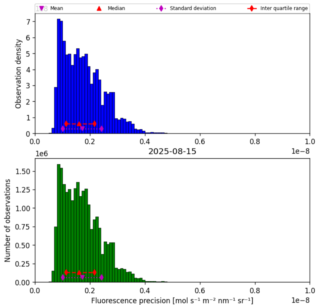
Figure 39: Histogram of “Fluorescence precision” for 2025-08-15 to 2025-08-16
