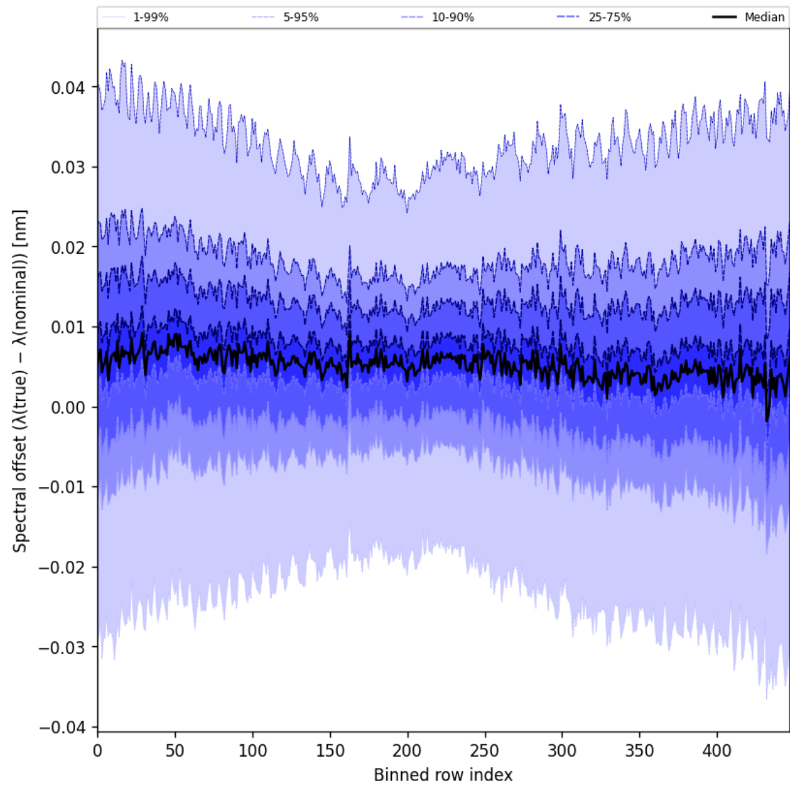
Figure 60: Along track statistics of “Spectral offset ( \lambda_{\text{true}} - \lambda_{\text{nominal}} )” for 2025-08-15 to 2025-08-16
