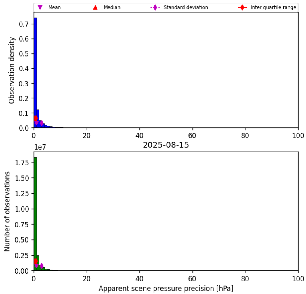
Figure 35: Histogram of “Apparent scene pressure precision” for 2025-08-15 to 2025-08-16
