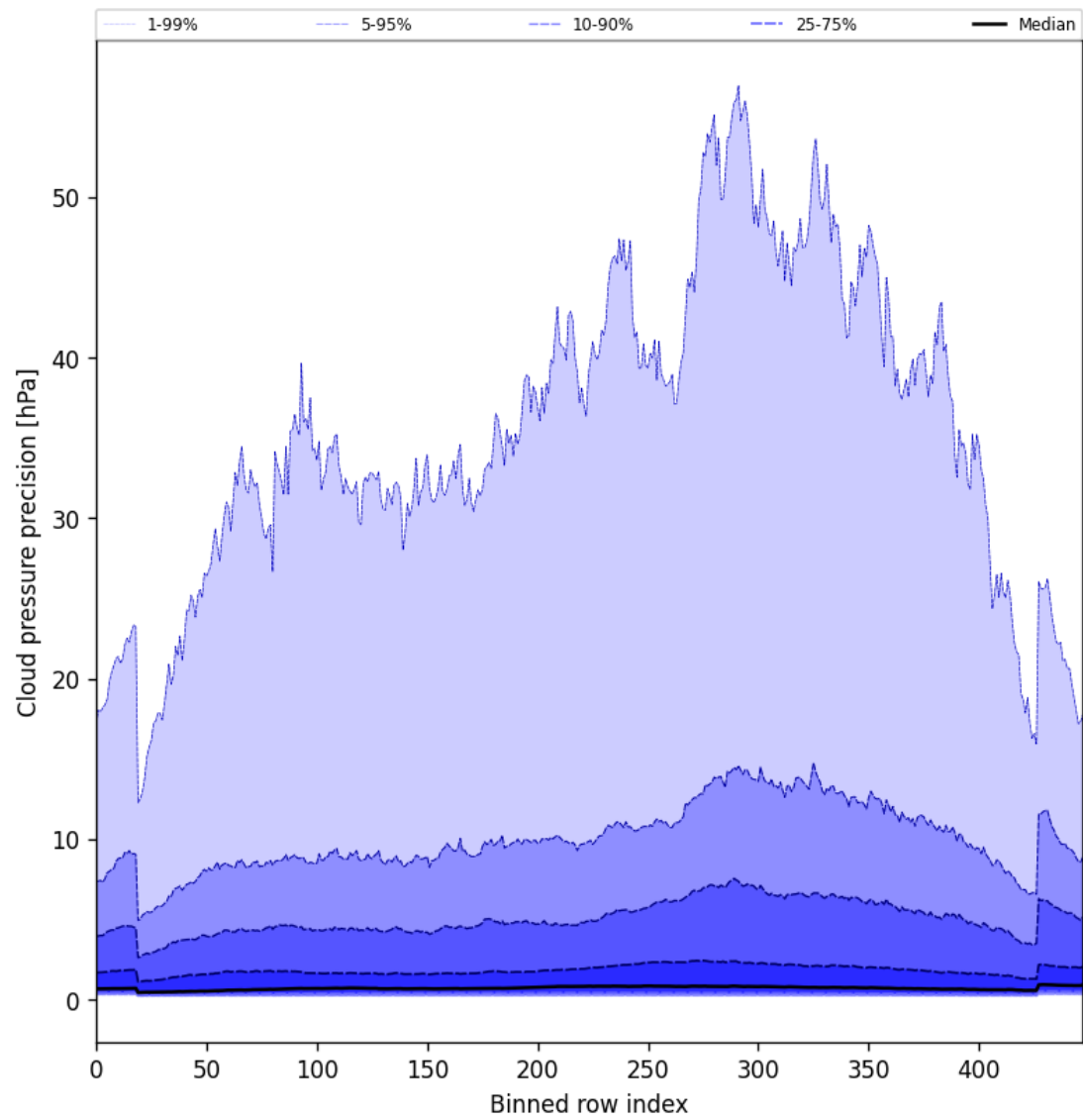
Figure 46: Along track statistics of “Cloud pressure precision” for 2025-08-15 to 2025-08-16
