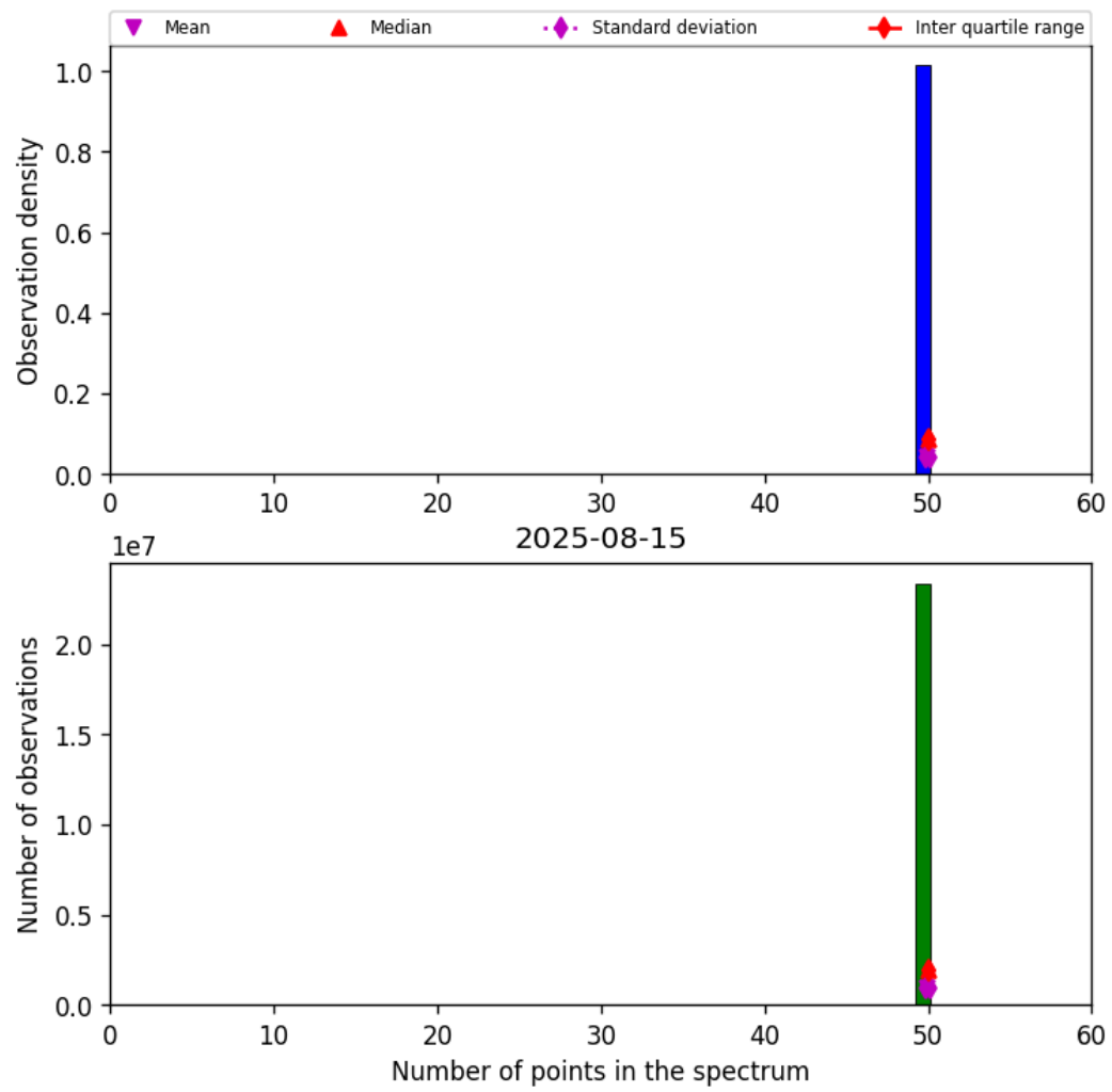
Figure 42: Histogram of “Number of points in the spectrum” for 2025-08-15 to 2025-08-16
