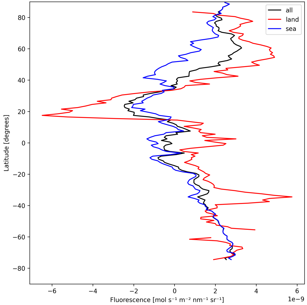
Figure 21: Zonal average of “Fluorescence” for 2025-08-15 to 2025-08-16.
