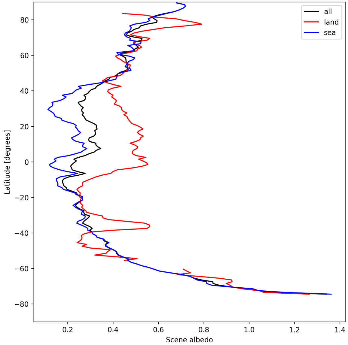
Figure 15: Zonal average of “Scene albedo” for 2025-08-15 to 2025-08-16.
