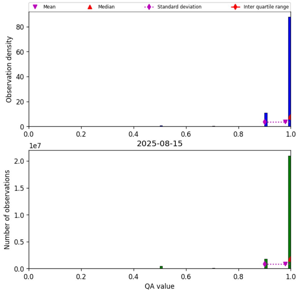
Figure 27: Histogram of “QA value” for 2025-08-15 to 2025-08-16
