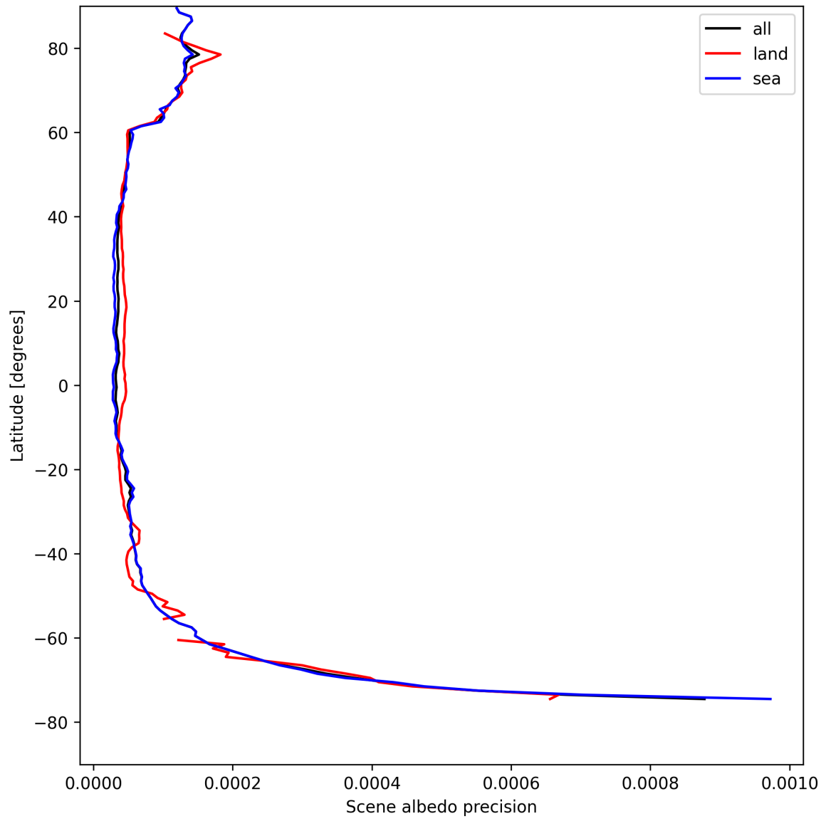
Figure 16: Zonal average of “Scene albedo precision” for 2025-08-15 to 2025-08-16.
