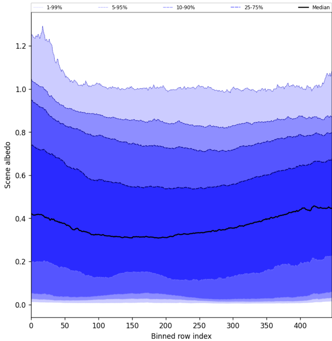
Figure 49: Along track statistics of “Scene albedo” for 2025-08-15 to 2025-08-16
