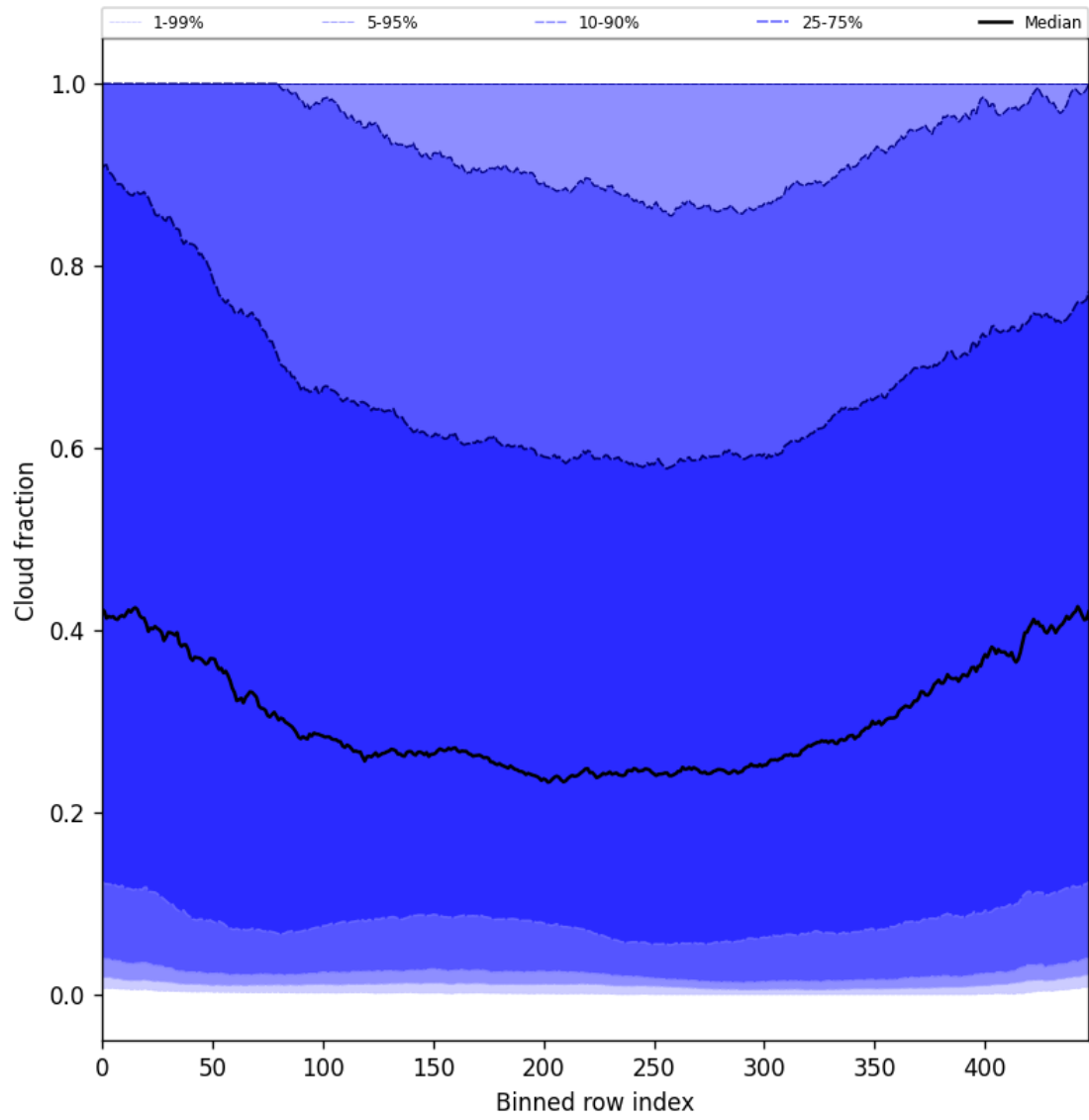
Figure 47: Along track statistics of “Cloud fraction” for 2025-08-15 to 2025-08-16
