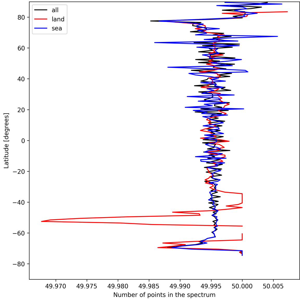
Figure 25: Zonal average of “Number of points in the spectrum” for 2025-08-15 to 2025-08-16.
