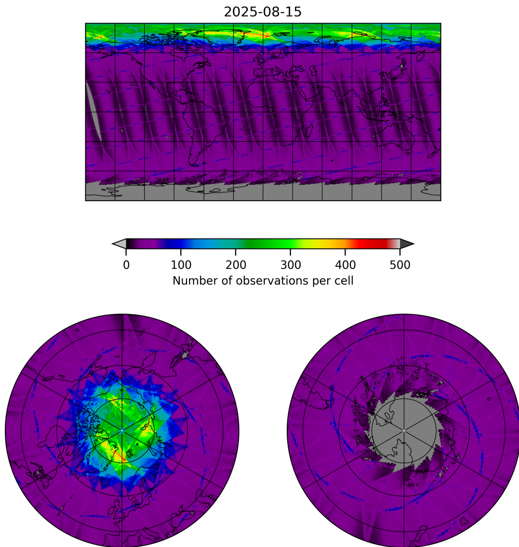
Figure 9: Map of the number of observations for 2025-08-15 to 2025-08-16
