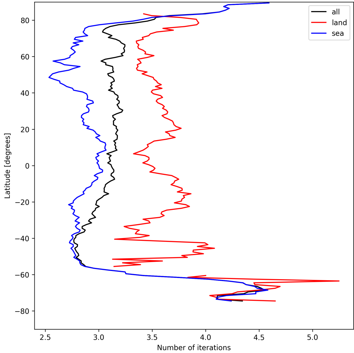
Figure 20: Zonal average of “Number of iterations” for 2025-08-15 to 2025-08-16.
