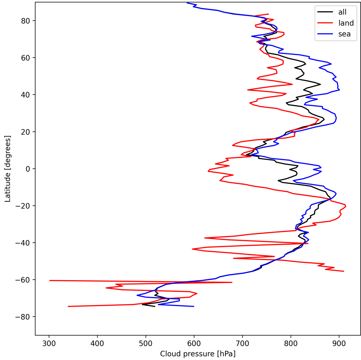
Figure 11: Zonal average of “Cloud pressure” for 2025-08-15 to 2025-08-16.
