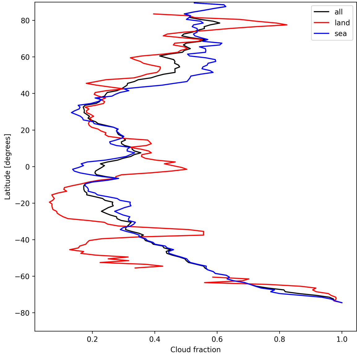
Figure 13: Zonal average of “Cloud fraction” for 2025-08-15 to 2025-08-16.
