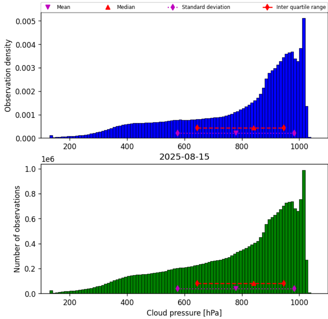
Figure 28: Histogram of “Cloud pressure” for 2025-08-15 to 2025-08-16
