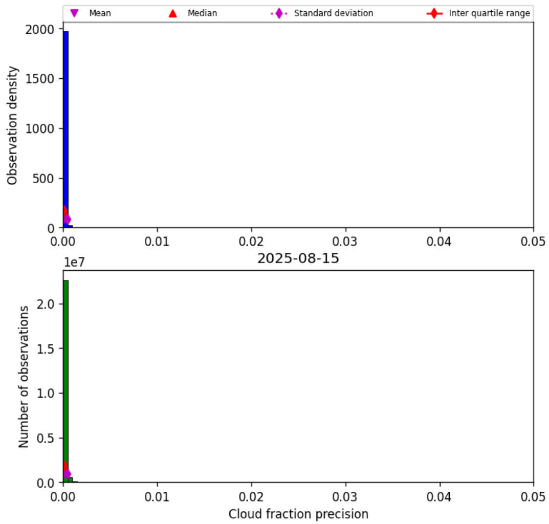
Figure 31: Histogram of “Cloud fraction precision” for 2025-08-15 to 2025-08-16
