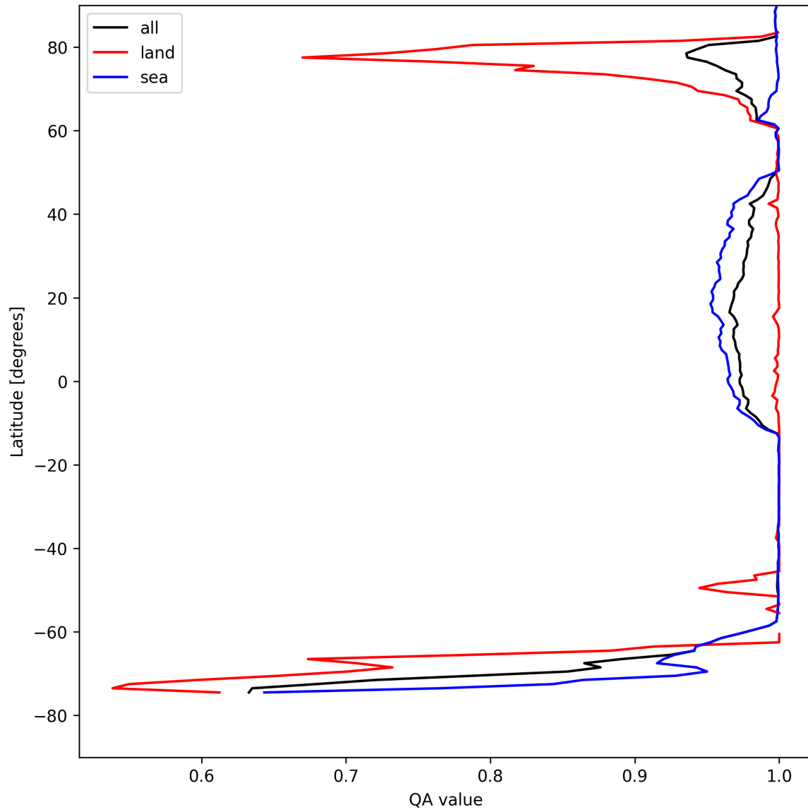
Figure 10: Zonal average of "QA value" for 2025-08-15 to 2025-08-16.
