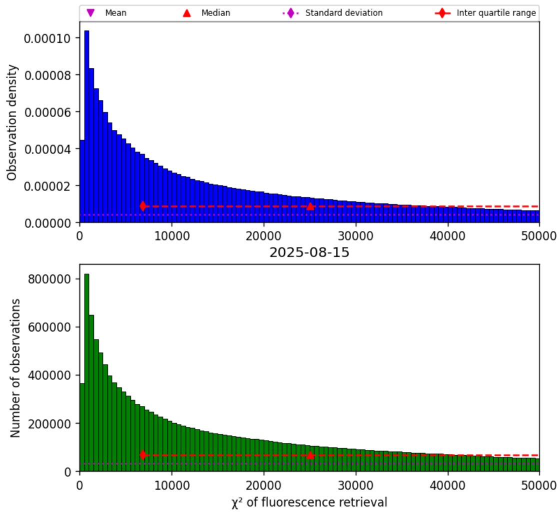
Figure 40: Histogram of “ \chi^2 of fluorescence retrieval” for 2025-08-15 to 2025-08-16
