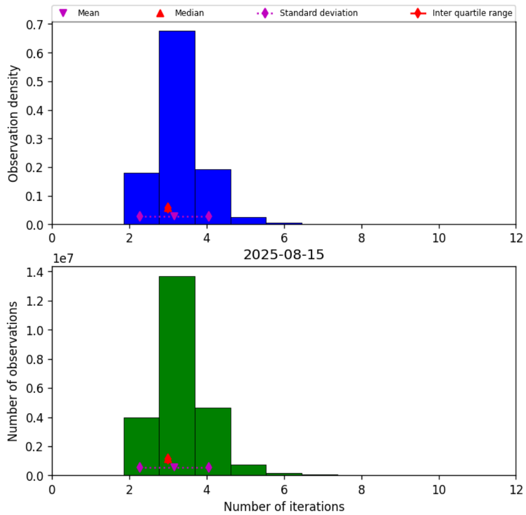
Figure 37: Histogram of “Number of iterations” for 2025-08-15 to 2025-08-16
