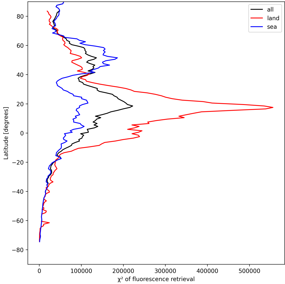
Figure 23: Zonal average of “ \chi^2 of fluorescence retrieval” for 2025-08-15 to 2025-08-16.
