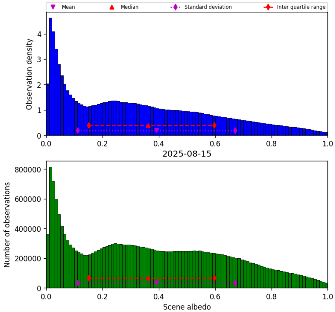
Figure 32: Histogram of “Scene albedo” for 2025-08-15 to 2025-08-16
