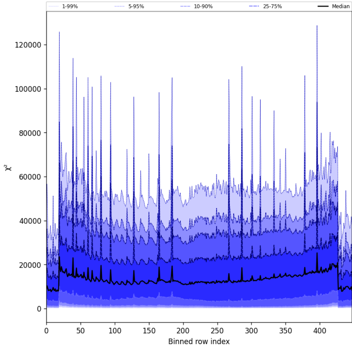
Figure 53: Along track statistics of “ \chi^2 ” for 2025-08-15 to 2025-08-16
