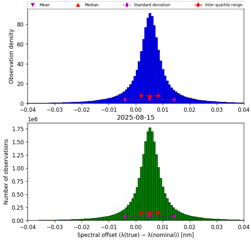
Figure 43: Histogram of “Spectral offset ( \lambda_{\text{true}} - \lambda_{\text{nominal}} )” for 2025-08-15 to 2025-08-16
