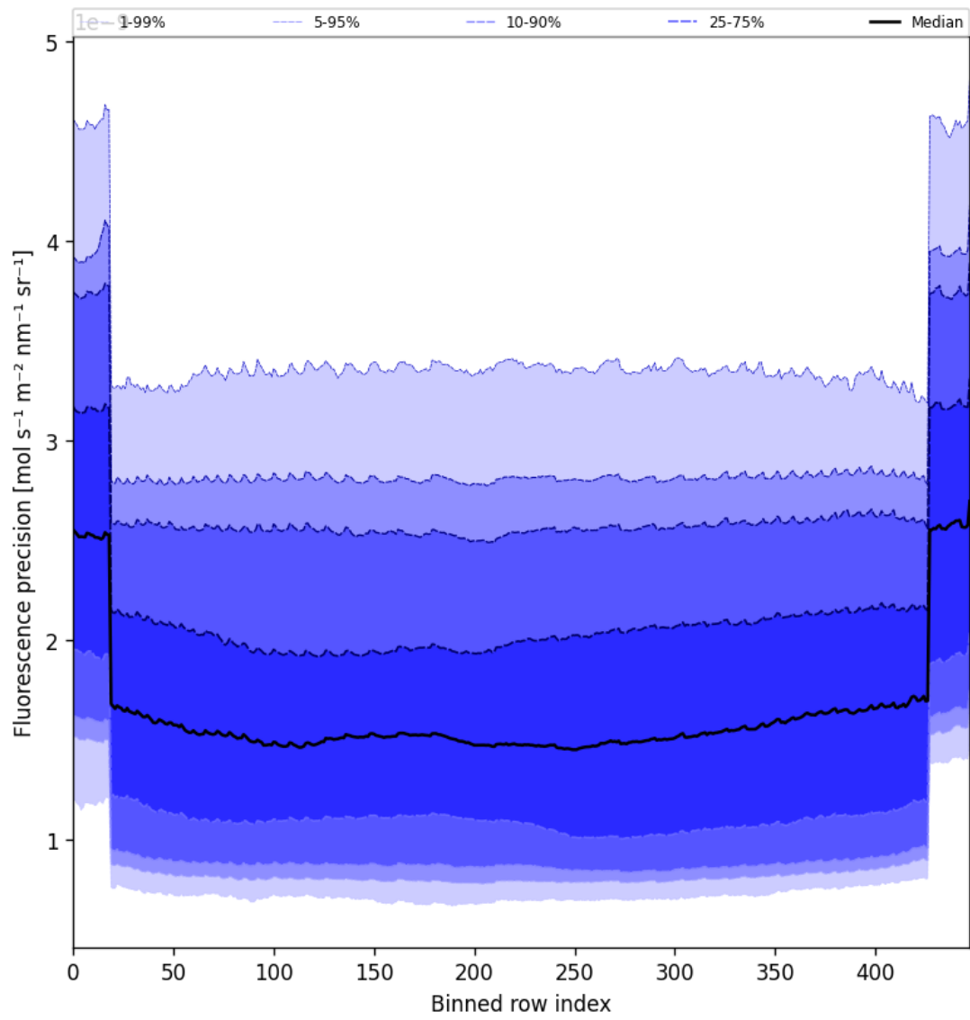
Figure 56: Along track statistics of “Fluorescence precision” for 2025-08-15 to 2025-08-16
