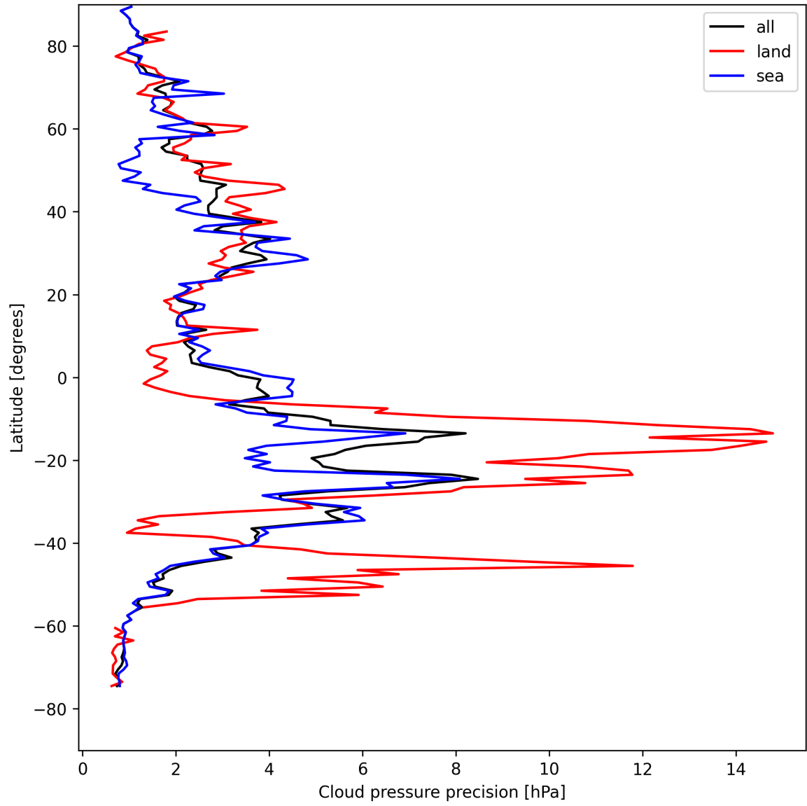
Figure 12: Zonal average of “Cloud pressure precision” for 2025-08-15 to 2025-08-16.
