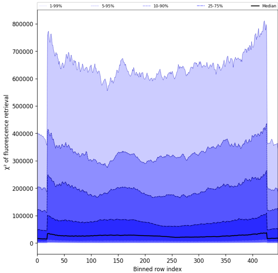
Figure 57: Along track statistics of “ \chi^2 of fluorescence retrieval” for 2025-08-15 to 2025-08-16
