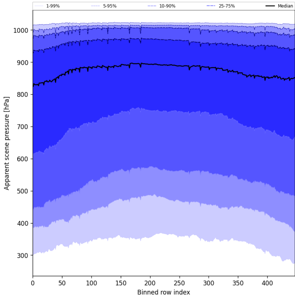
Figure 51: Along track statistics of “Apparent scene pressure” for 2025-08-15 to 2025-08-16
