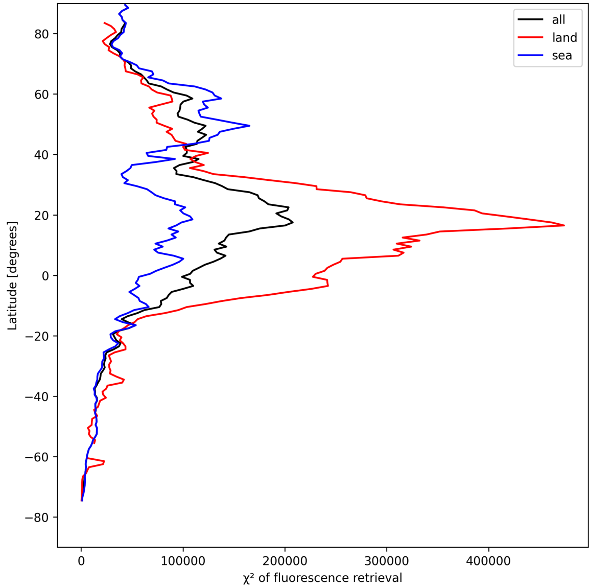
Figure 23: Zonal average of “ \chi^2 of fluorescence retrieval” for 2025-08-16 to 2025-08-17.
