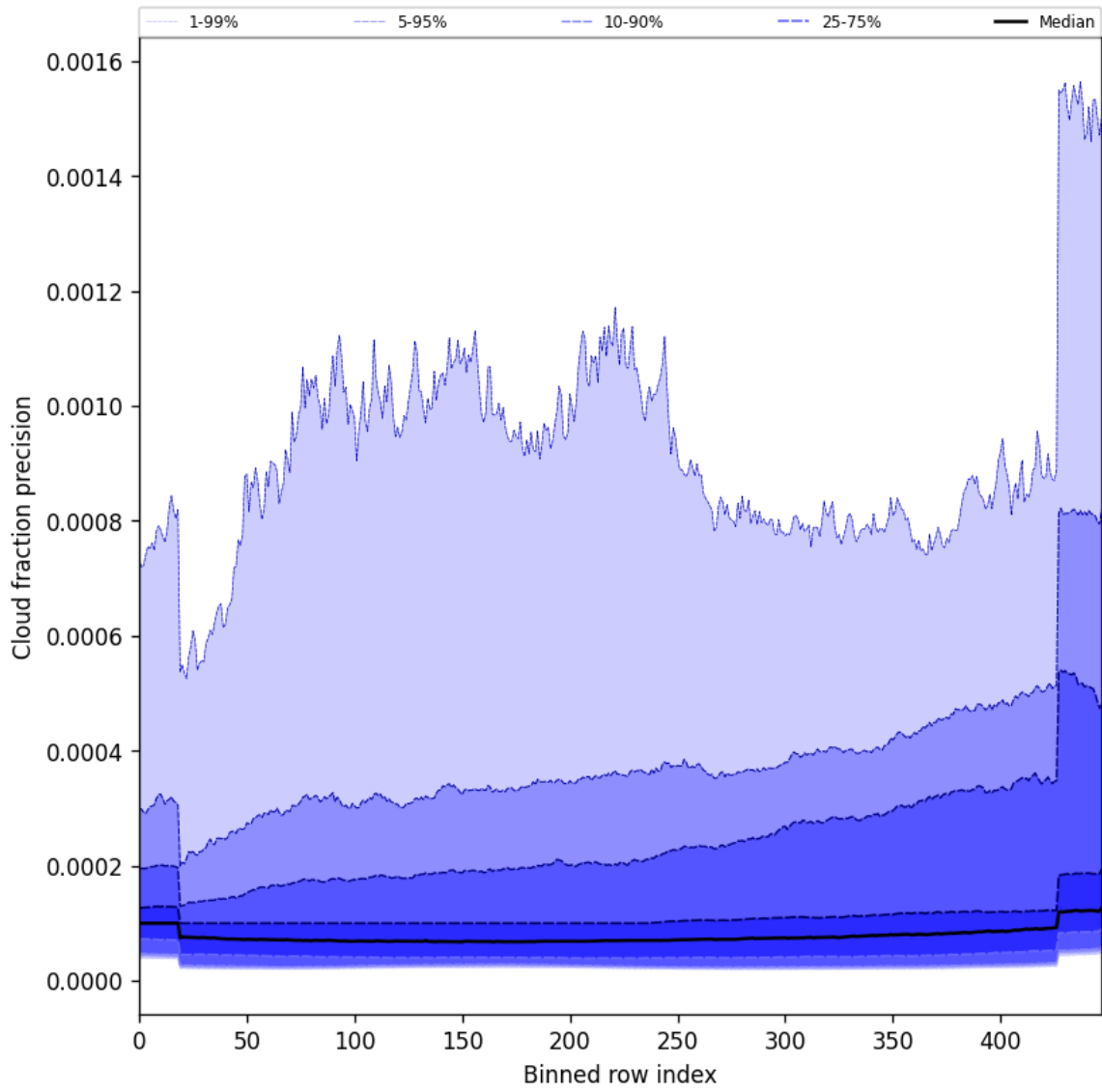
Figure 48: Along track statistics of “Cloud fraction precision” for 2025-08-16 to 2025-08-17
