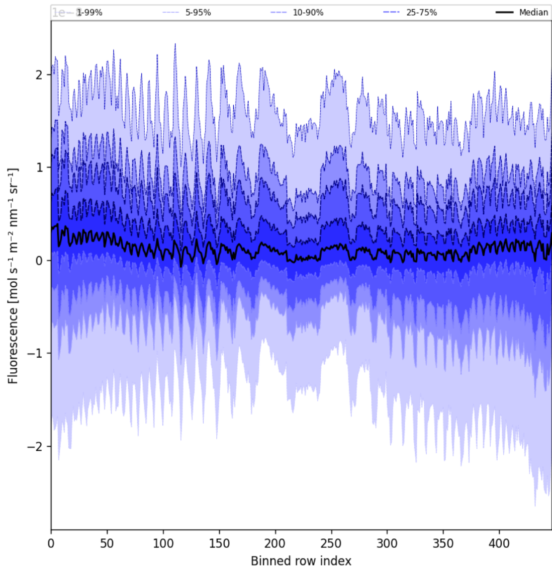
Figure 55: Along track statistics of “Fluorescence” for 2025-08-16 to 2025-08-17
