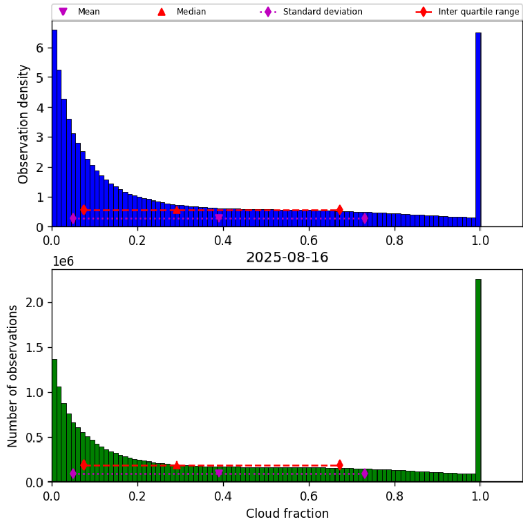
Figure 30: Histogram of “Cloud fraction” for 2025-08-16 to 2025-08-17
