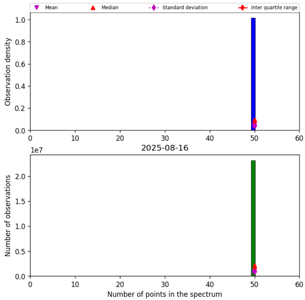
Figure 42: Histogram of “Number of points in the spectrum” for 2025-08-16 to 2025-08-17
