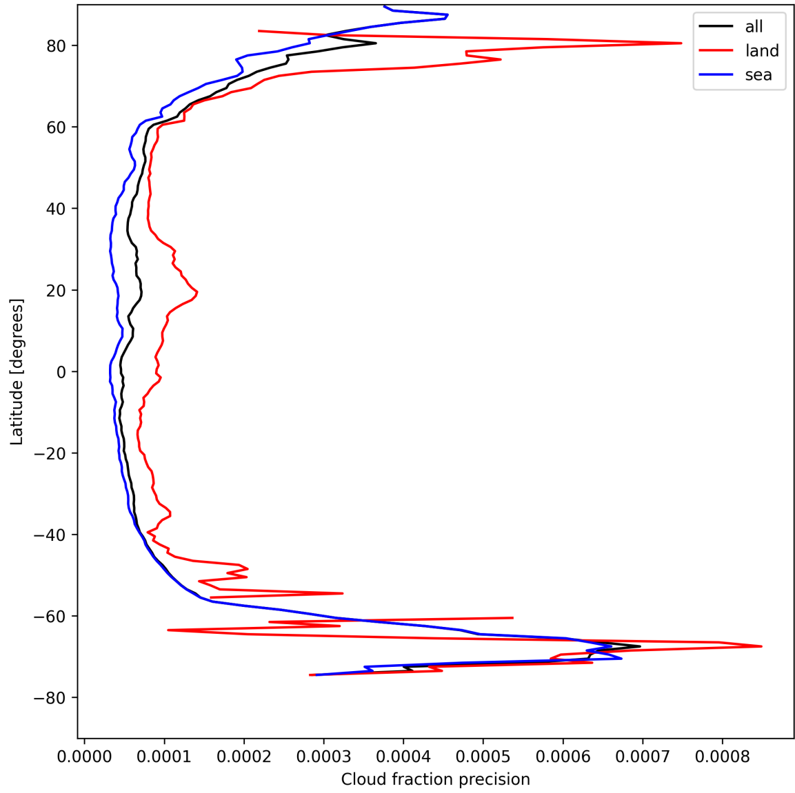
Figure 14: Zonal average of “Cloud fraction precision” for 2025-08-16 to 2025-08-17.
