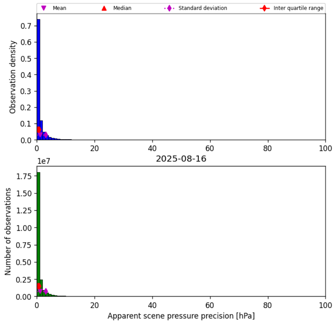
Figure 35: Histogram of “Apparent scene pressure precision” for 2025-08-16 to 2025-08-17
