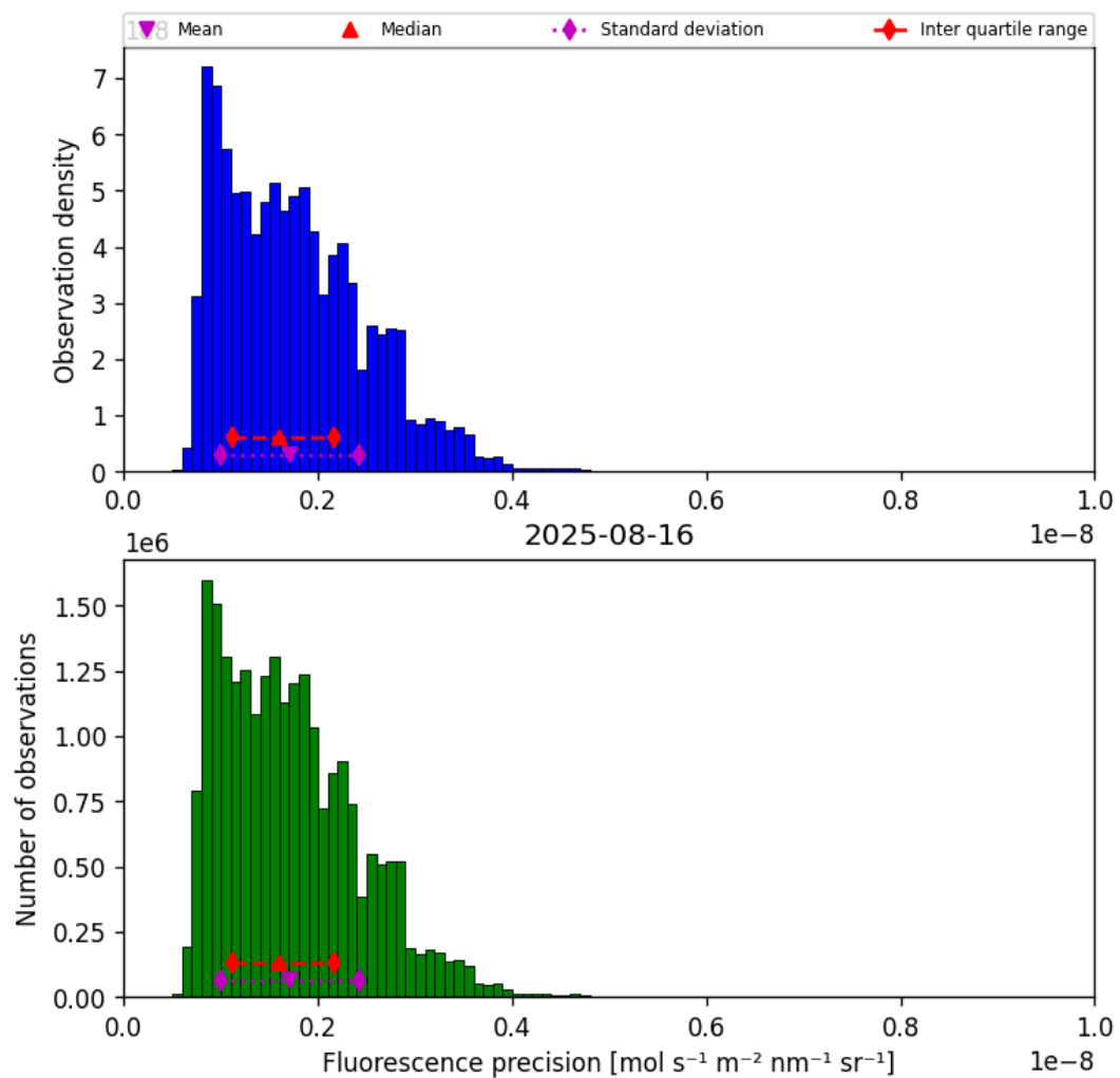
Figure 39: Histogram of “Fluorescence precision” for 2025-08-16 to 2025-08-17
