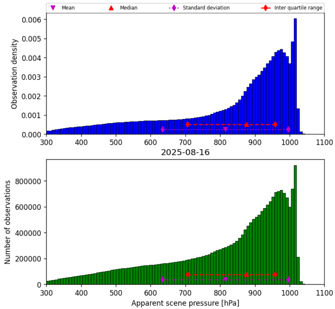
Figure 34: Histogram of “Apparent scene pressure” for 2025-08-16 to 2025-08-17
