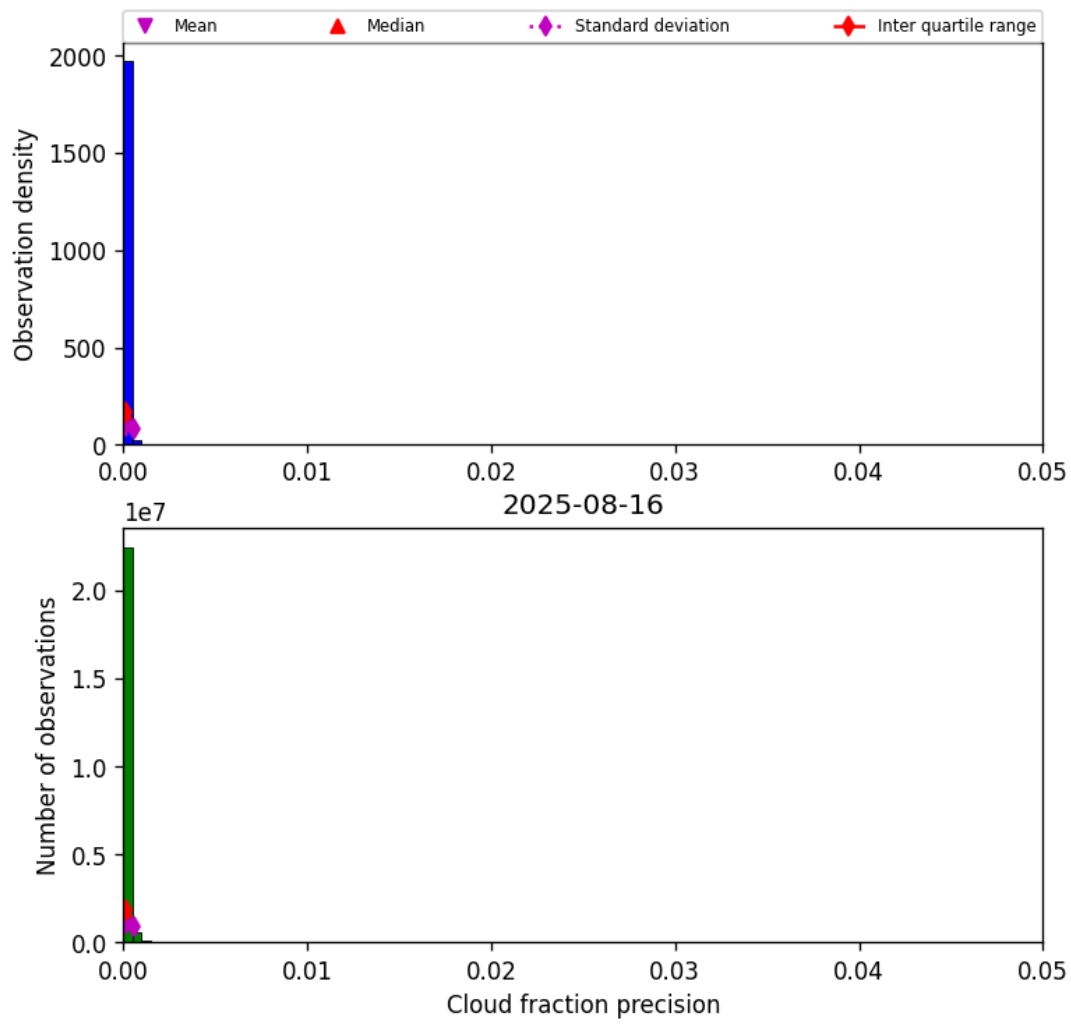
Figure 31: Histogram of “Cloud fraction precision” for 2025-08-16 to 2025-08-17
