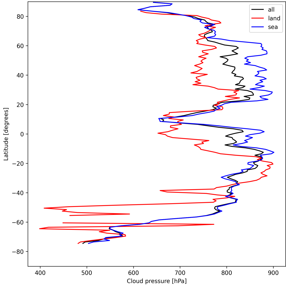
Figure 11: Zonal average of “Cloud pressure” for 2025-08-16 to 2025-08-17.
