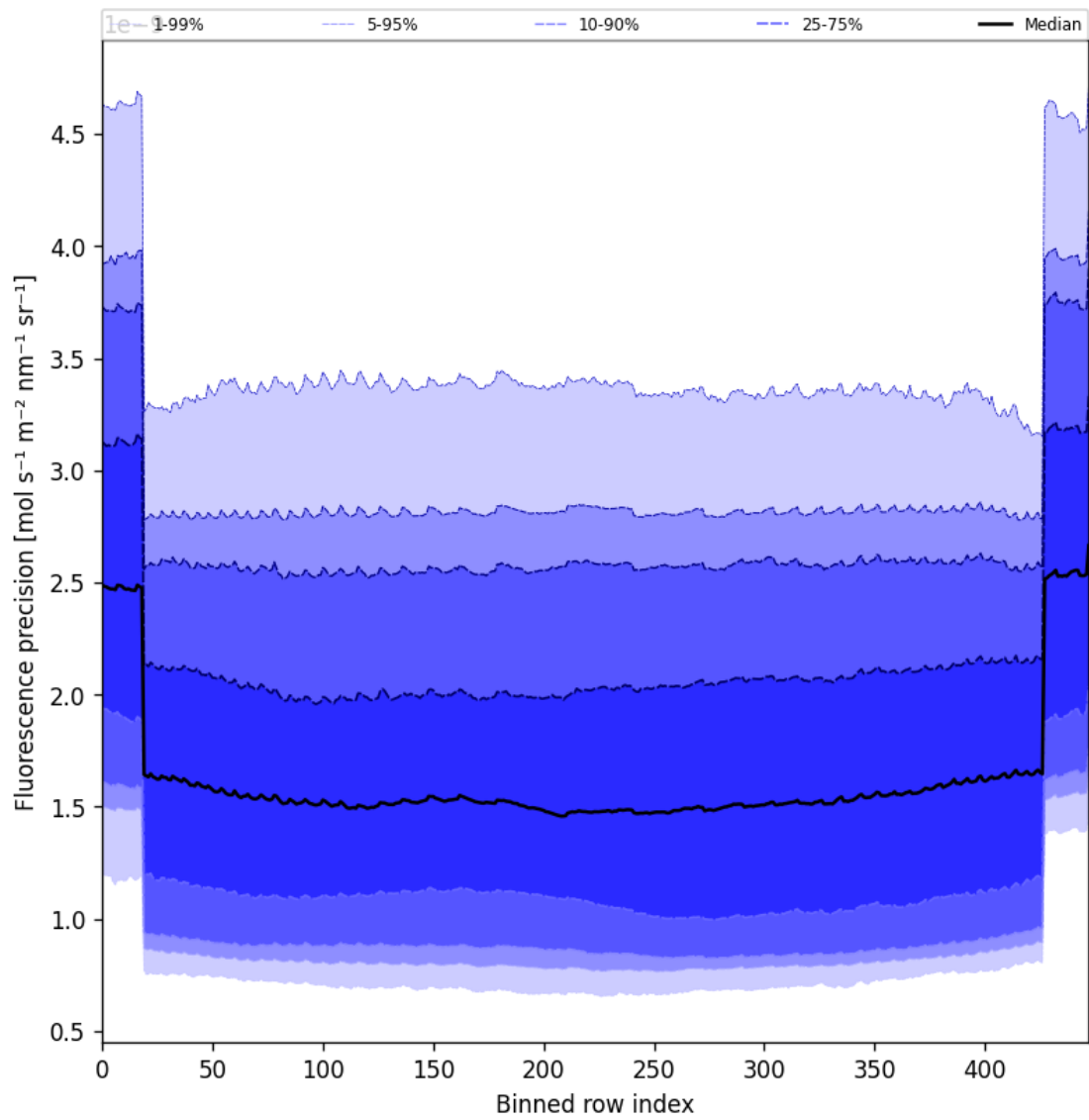
Figure 56: Along track statistics of “Fluorescence precision” for 2025-08-16 to 2025-08-17
