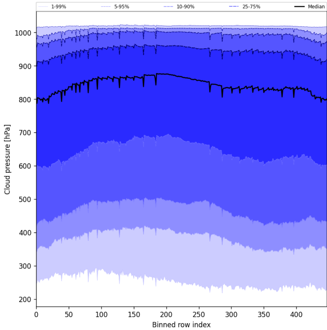
Figure 45: Along track statistics of “Cloud pressure” for 2025-08-16 to 2025-08-17
