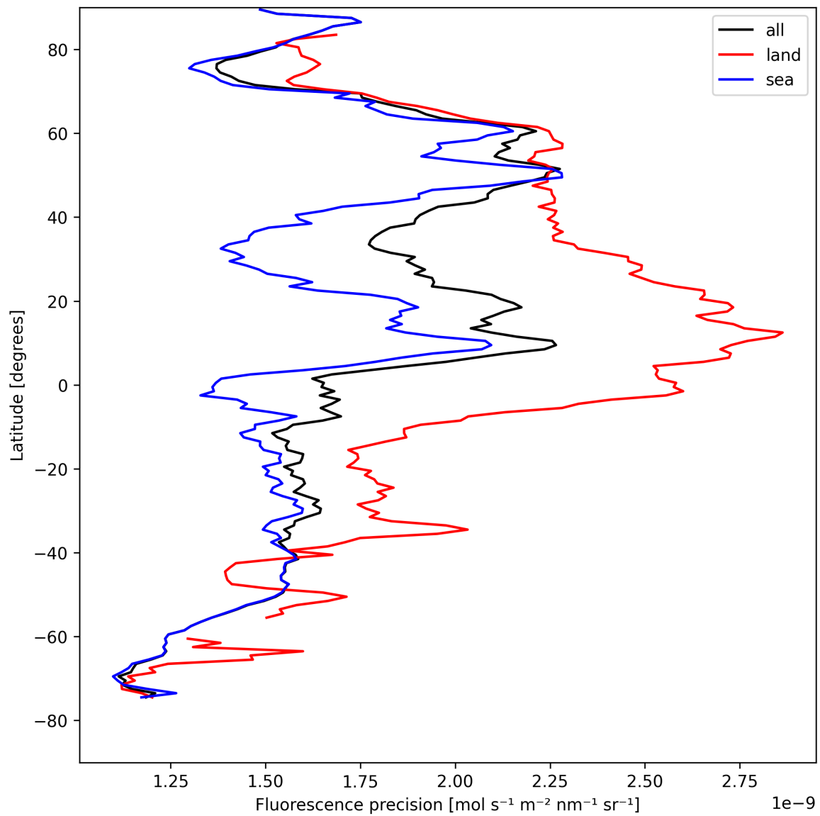
Figure 22: Zonal average of “Fluorescence precision” for 2025-08-16 to 2025-08-17.
