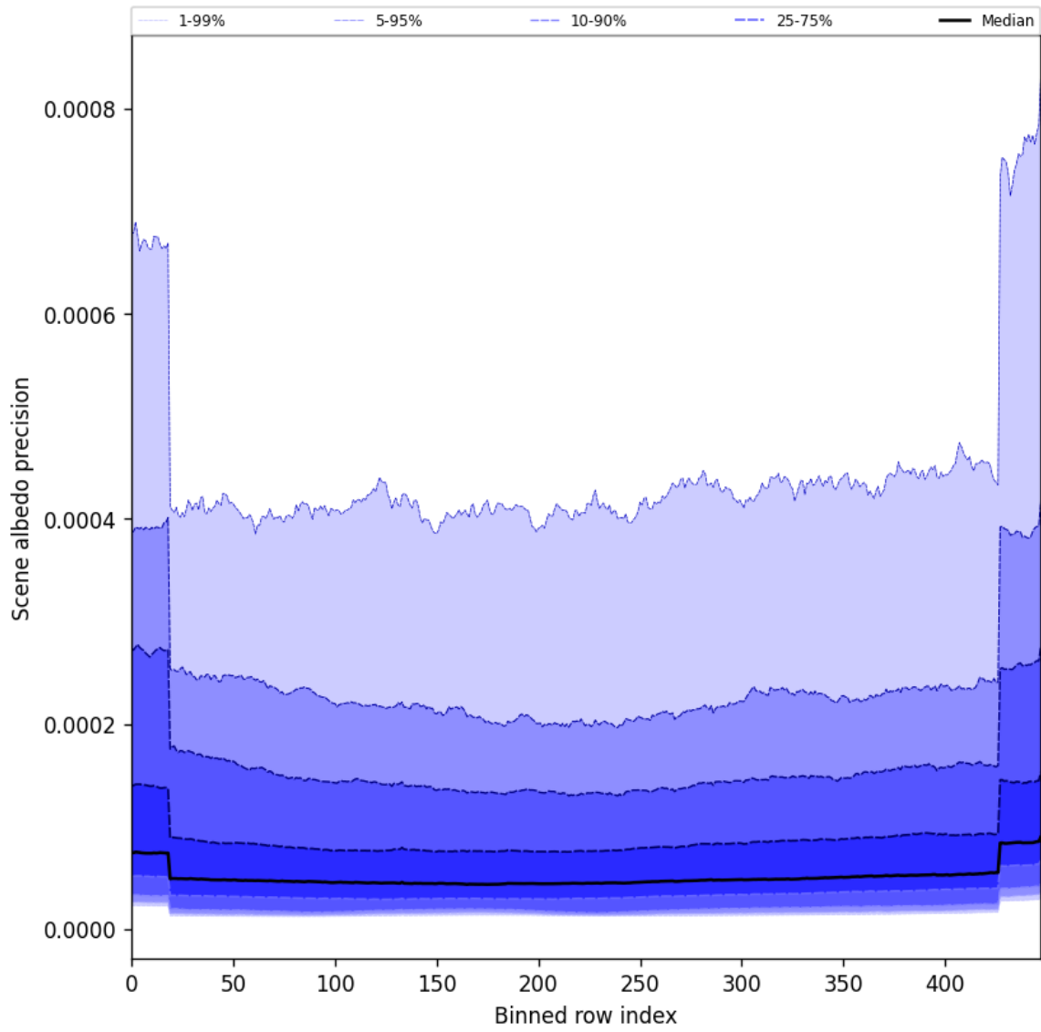
Figure 50: Along track statistics of “Scene albedo precision” for 2025-08-16 to 2025-08-17
