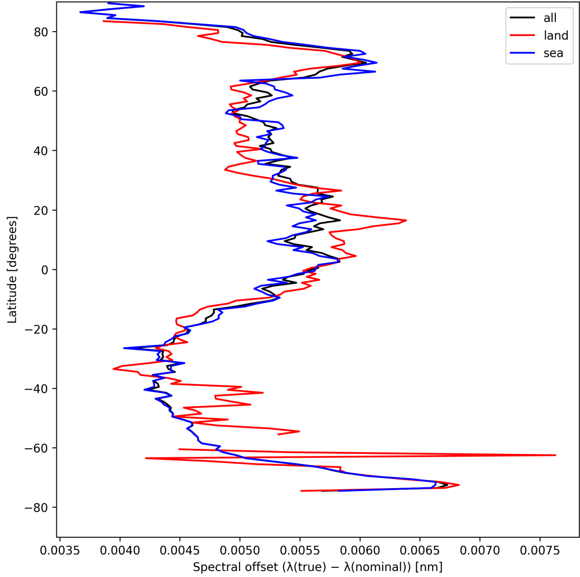
Figure 26: Zonal average of "Spectral offset ( \lambda_{\text{true}} - \lambda_{\text{nominal}} )" for 2025-08-16 to 2025-08-17.
