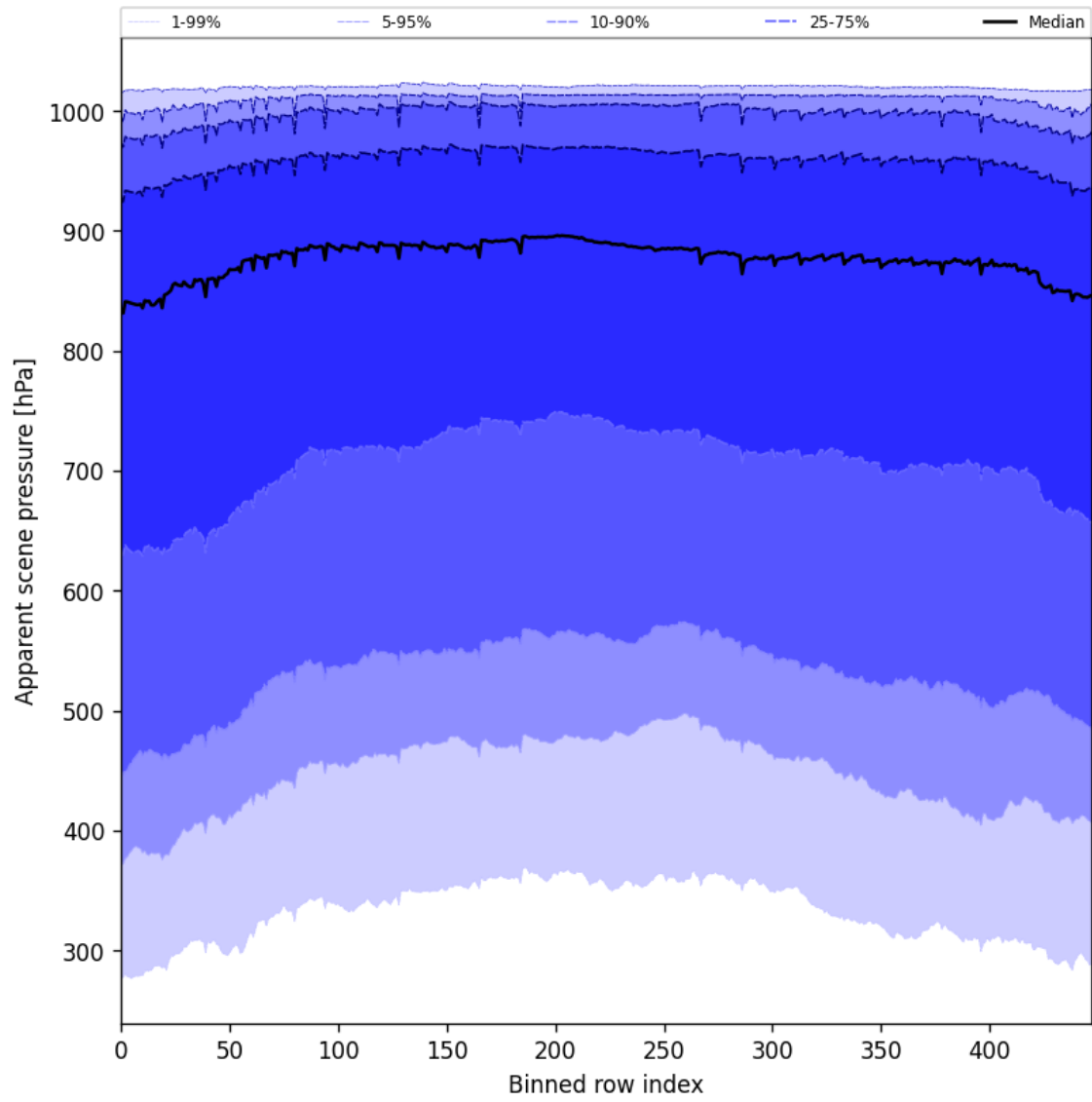
Figure 51: Along track statistics of “Apparent scene pressure” for 2025-08-16 to 2025-08-17
