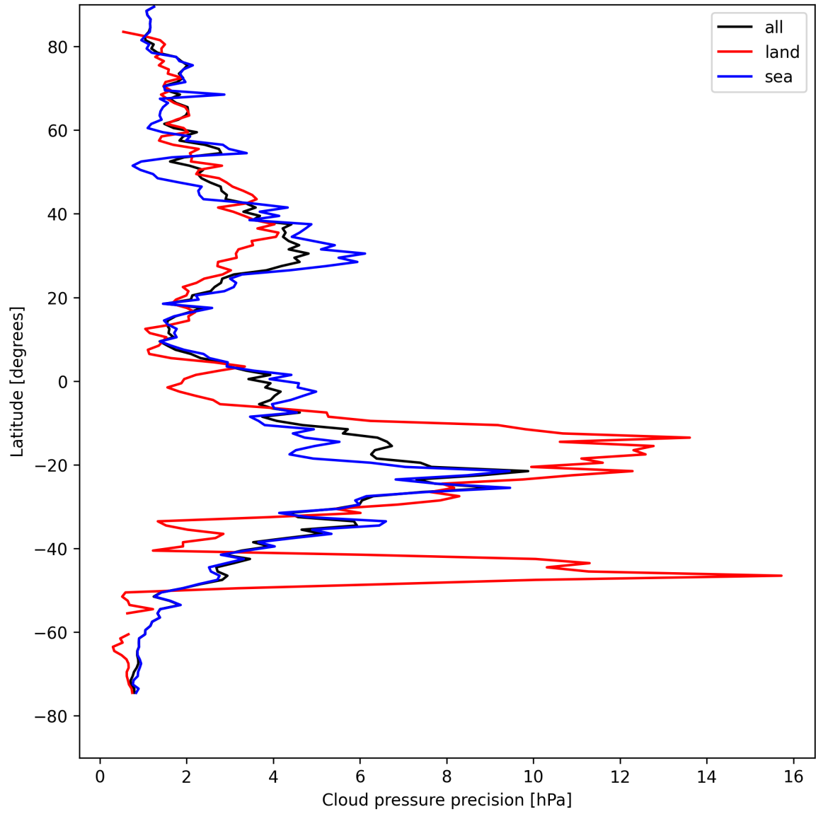
Figure 12: Zonal average of “Cloud pressure precision” for 2025-08-16 to 2025-08-17.
