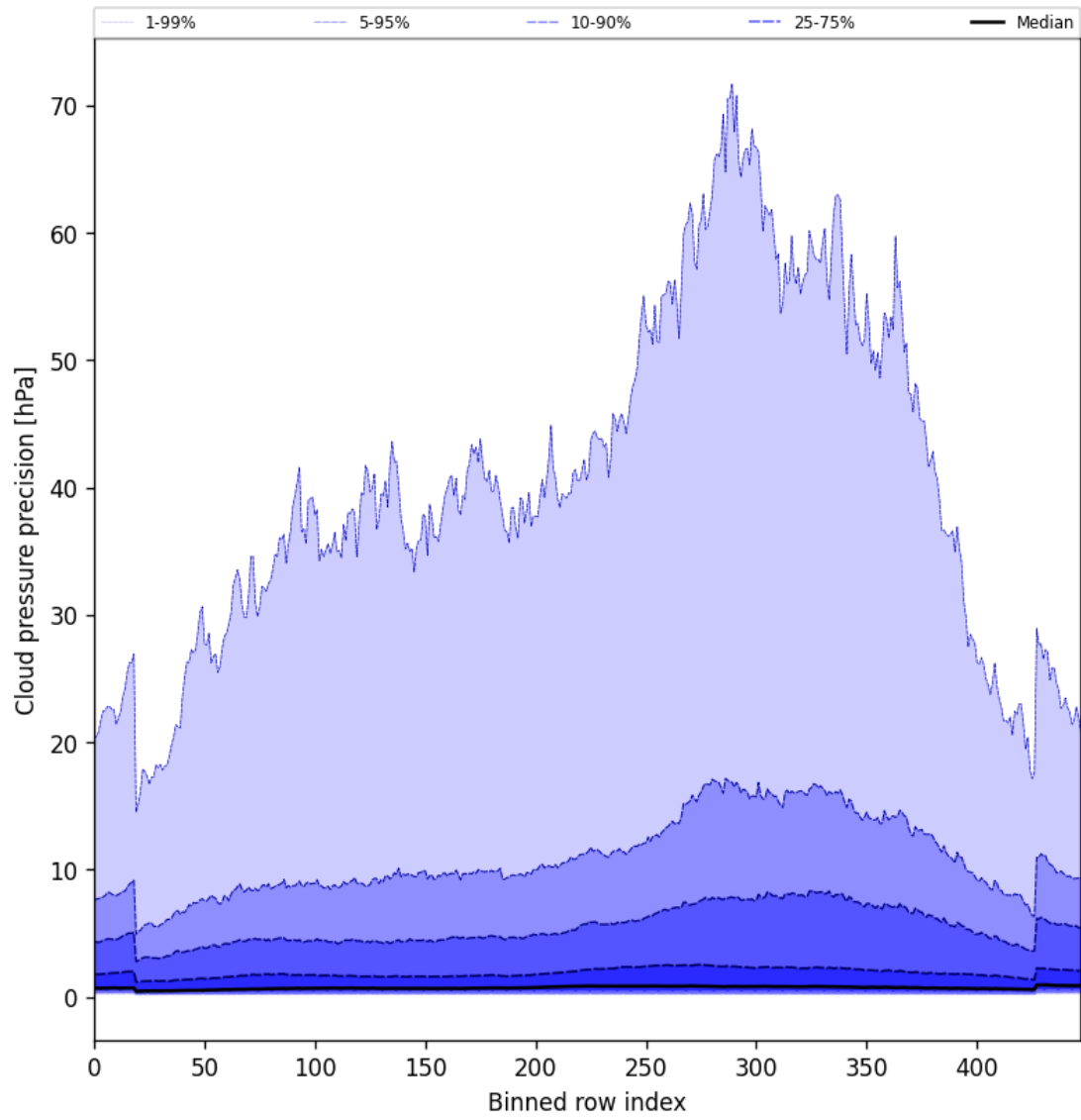
Figure 46: Along track statistics of “Cloud pressure precision” for 2025-08-16 to 2025-08-17
