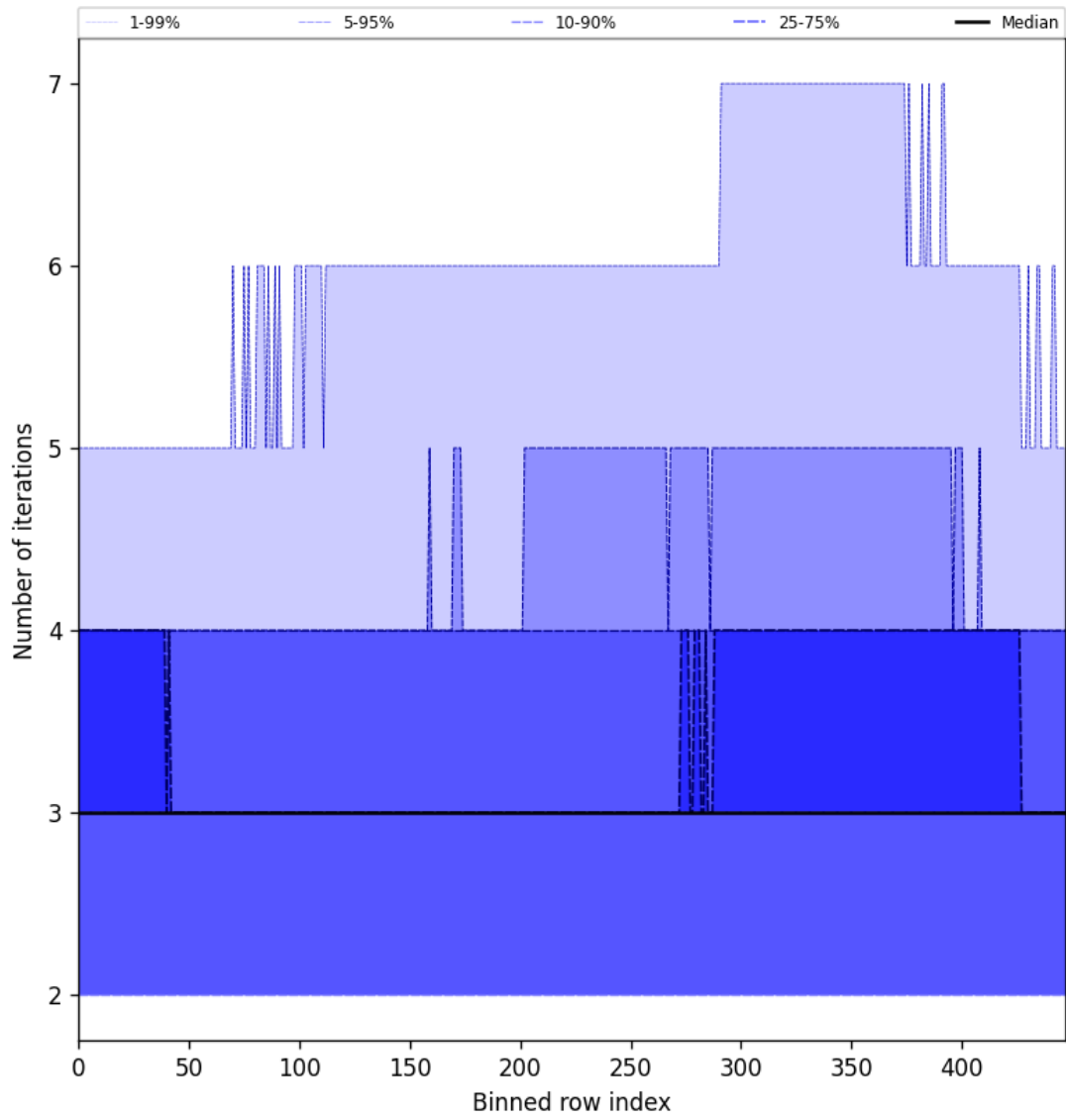
Figure 54: Along track statistics of “Number of iterations” for 2025-08-16 to 2025-08-17
