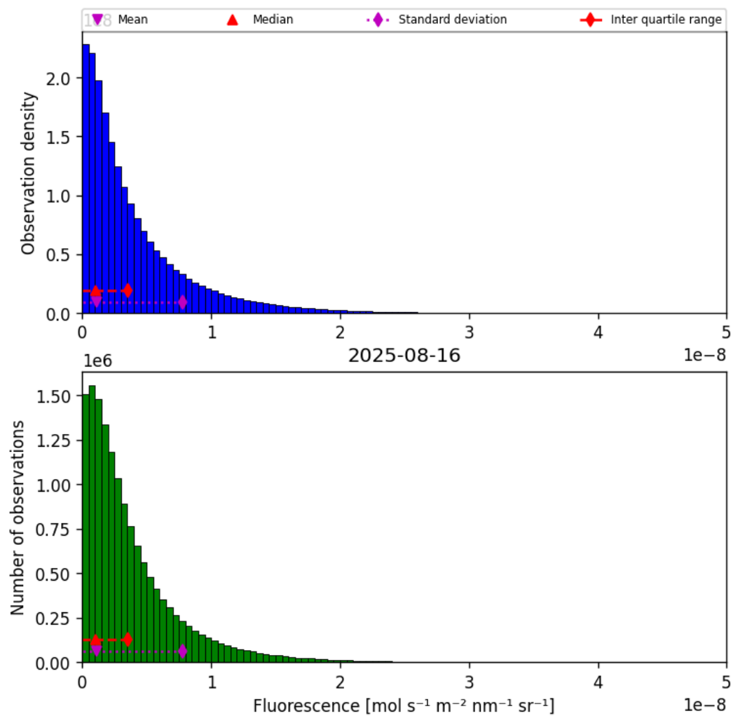
Figure 38: Histogram of “Fluorescence” for 2025-08-16 to 2025-08-17
