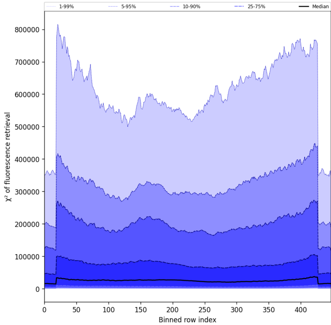
Figure 57: Along track statistics of “ \chi^2 of fluorescence retrieval” for 2025-08-16 to 2025-08-17
