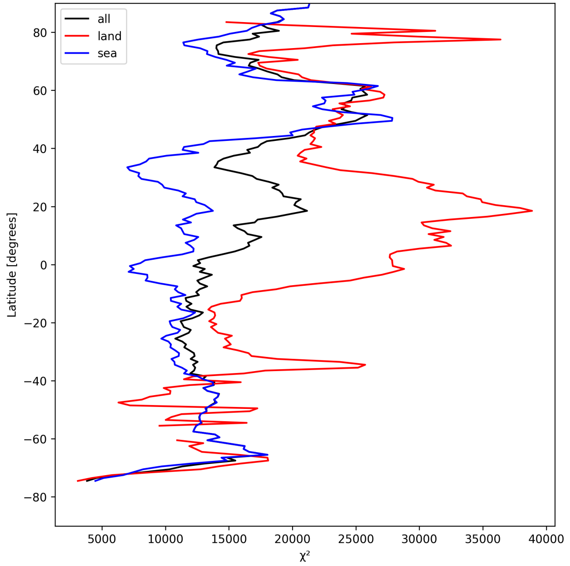
Figure 19: Zonal average of “ \chi^2 ” for 2025-08-16 to 2025-08-17.
