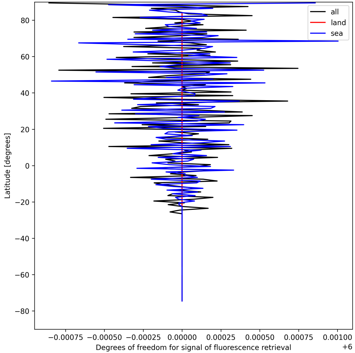
Figure 24: Zonal average of “Degrees of freedom for signal of fluorescence retrieval” for 2025-08-16 to 2025-08-17.
