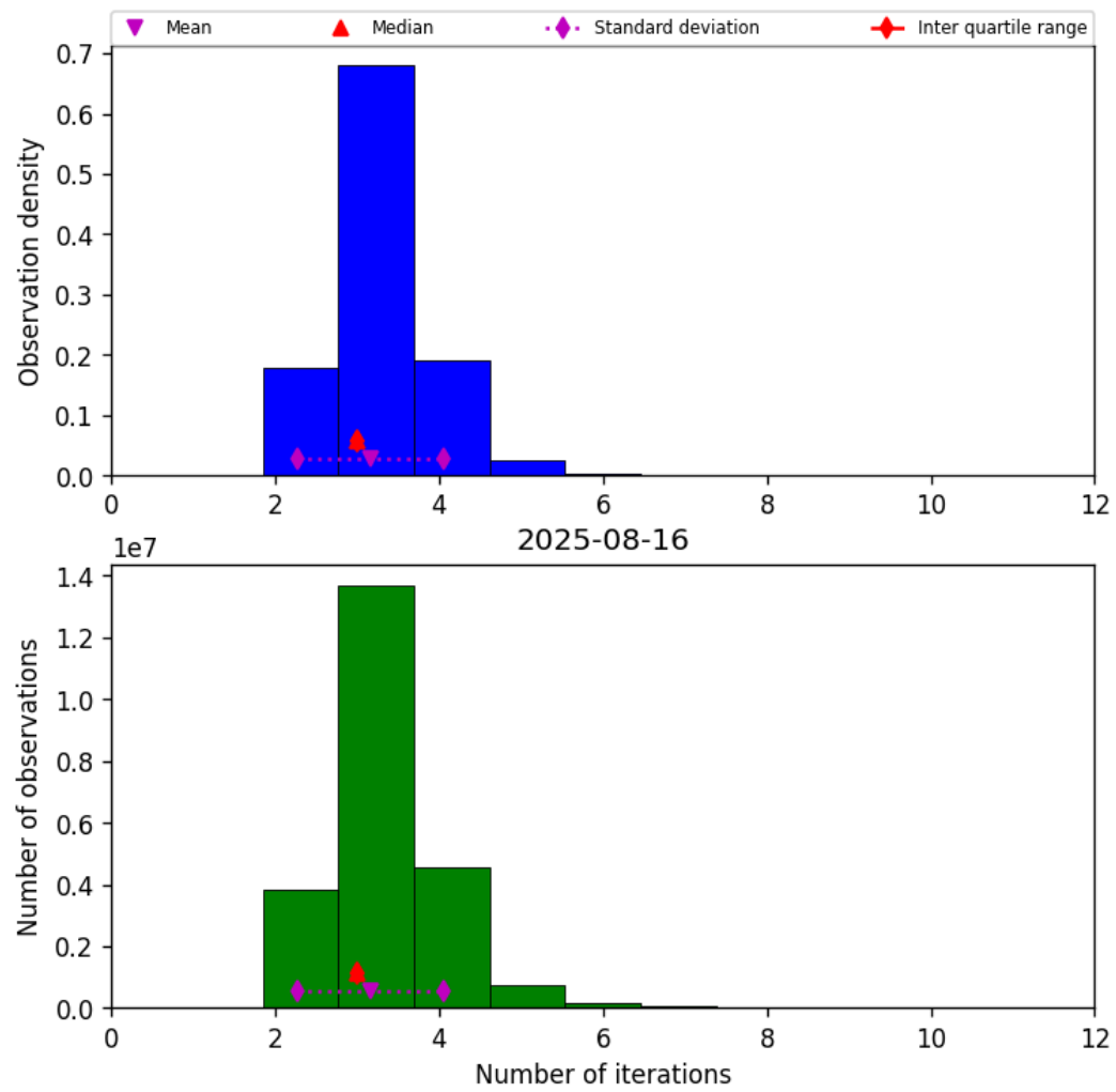
Figure 37: Histogram of “Number of iterations” for 2025-08-16 to 2025-08-17
