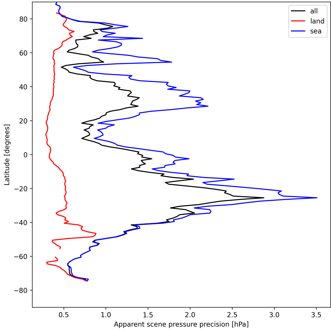
Figure 18: Zonal average of “Apparent scene pressure precision” for 2025-08-16 to 2025-08-17.
