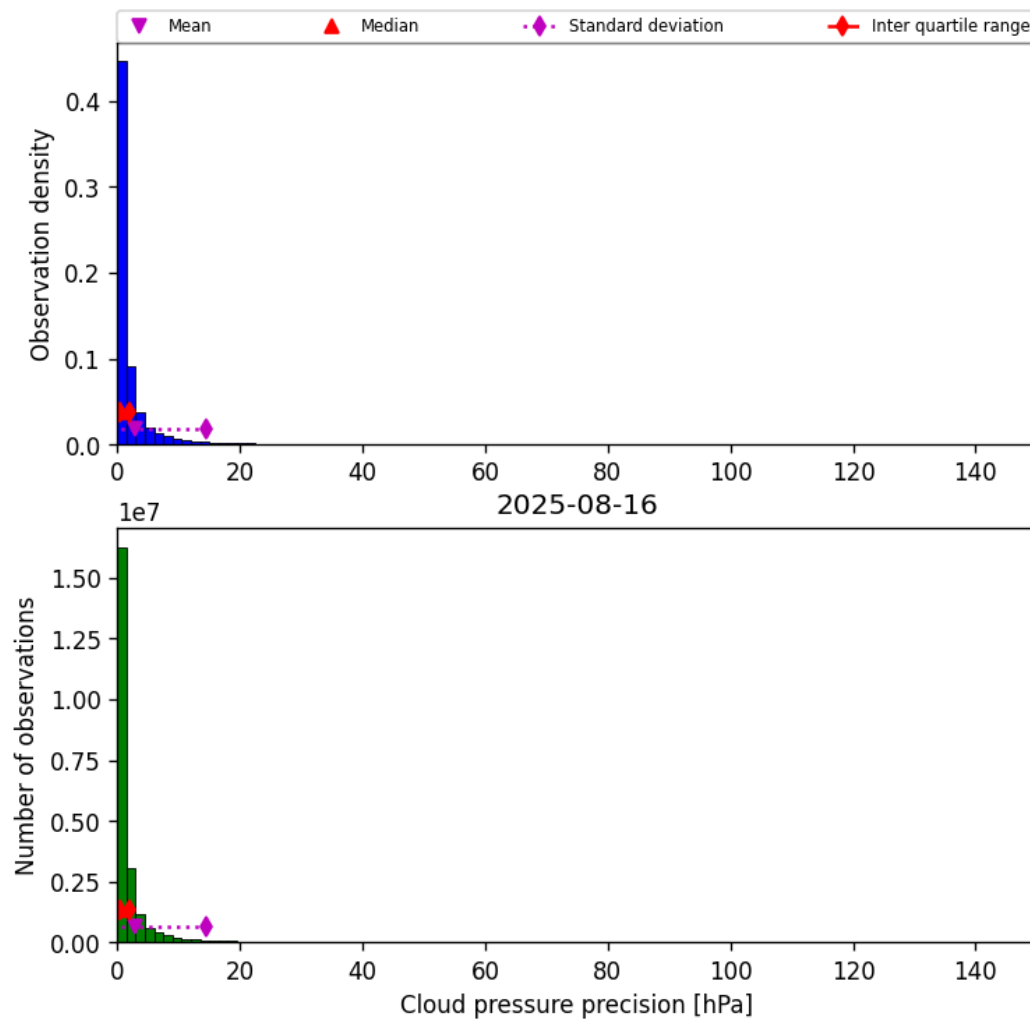
Figure 29: Histogram of “Cloud pressure precision” for 2025-08-16 to 2025-08-17
