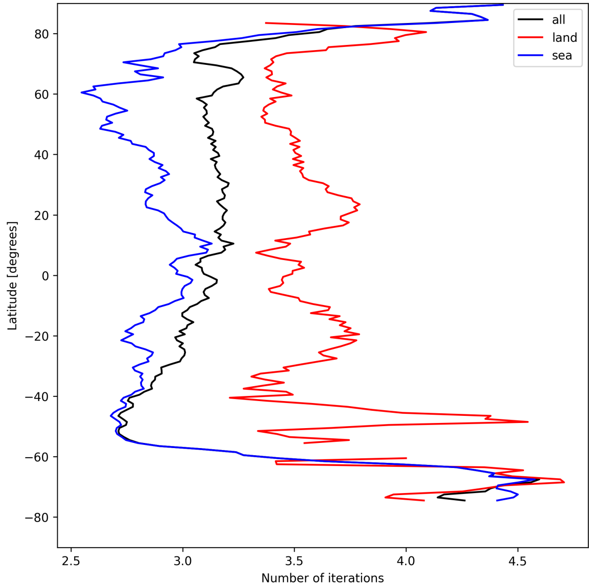
Figure 20: Zonal average of “Number of iterations” for 2025-08-16 to 2025-08-17.
