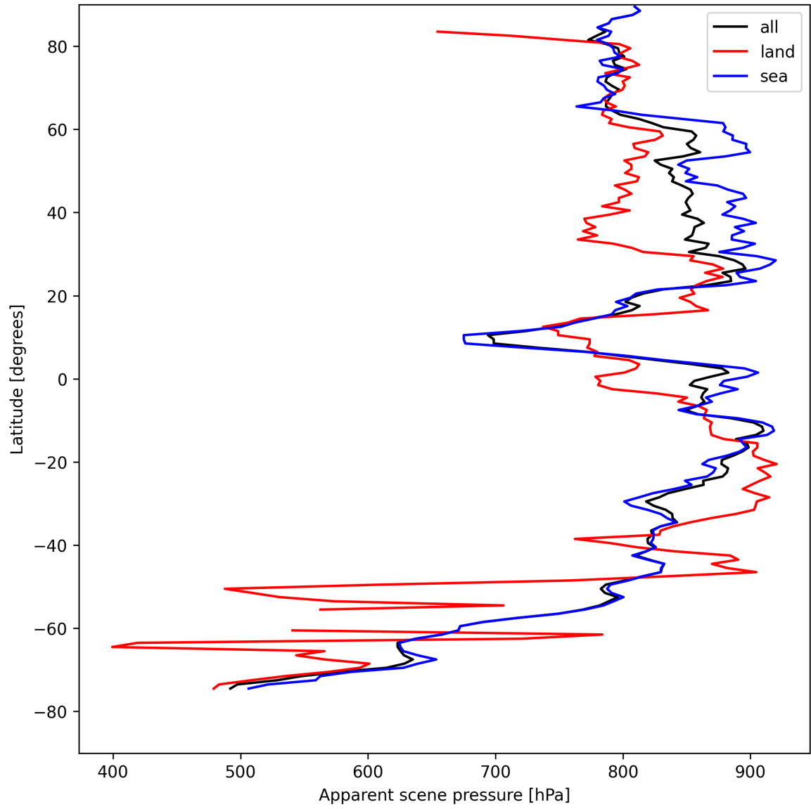
Figure 17: Zonal average of “Apparent scene pressure” for 2025-08-16 to 2025-08-17.
