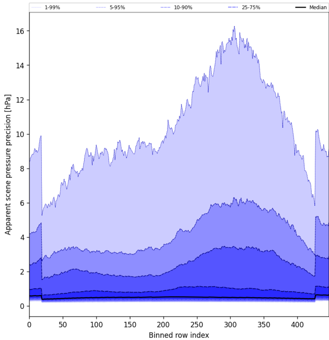
Figure 52: Along track statistics of “Apparent scene pressure precision” for 2025-08-16 to 2025-08-17
