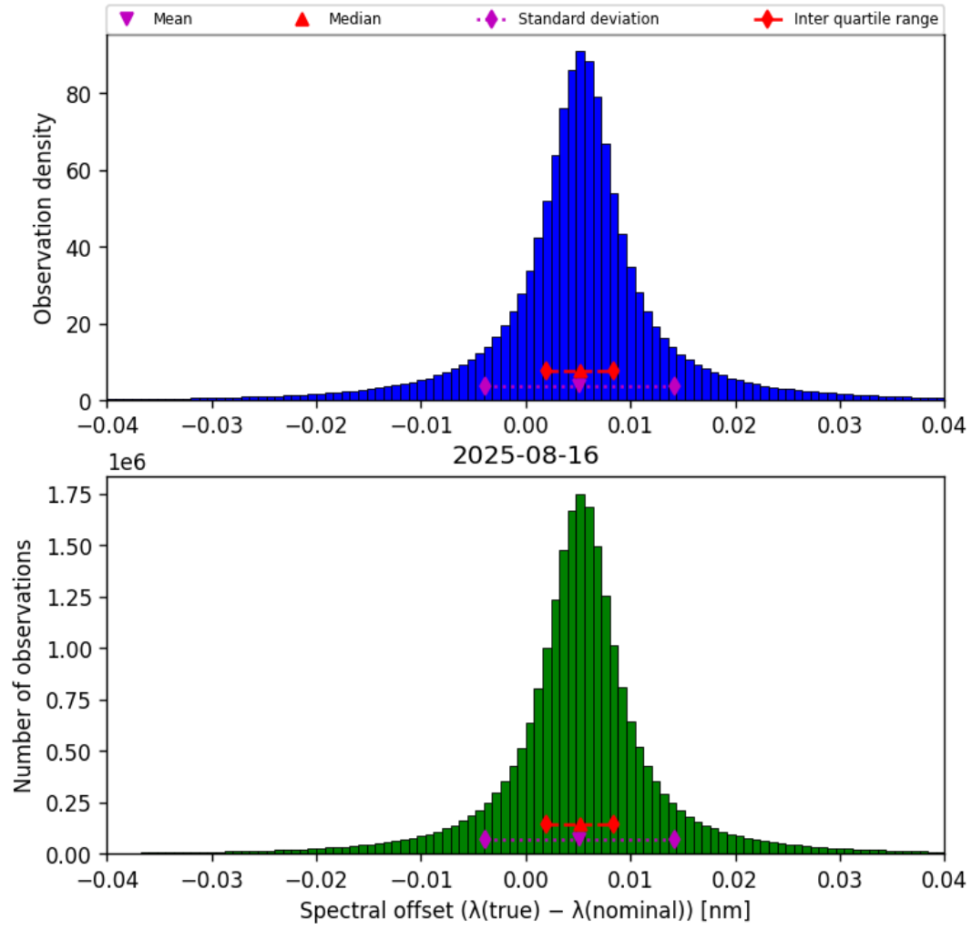
Figure 43: Histogram of “Spectral offset ( \lambda_{\text{true}} - \lambda_{\text{nominal}} )” for 2025-08-16 to 2025-08-17
