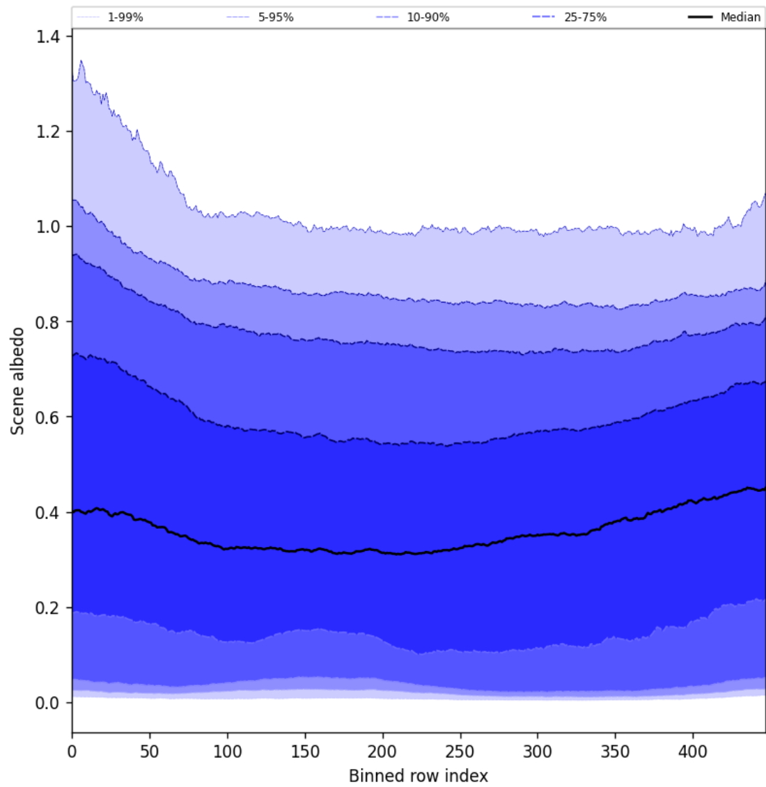
Figure 49: Along track statistics of “Scene albedo” for 2025-08-16 to 2025-08-17
