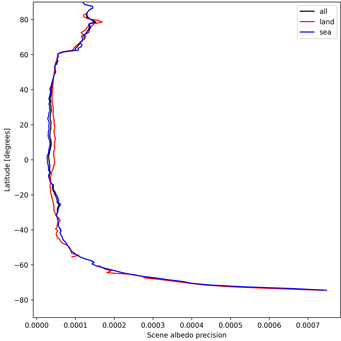
Figure 16: Zonal average of “Scene albedo precision” for 2025-08-16 to 2025-08-17.
