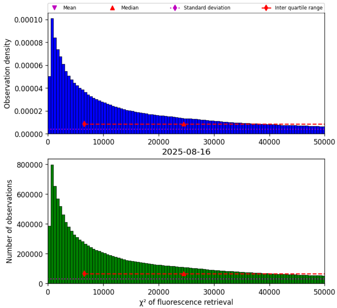
Figure 40: Histogram of “ \chi^2 of fluorescence retrieval” for 2025-08-16 to 2025-08-17
