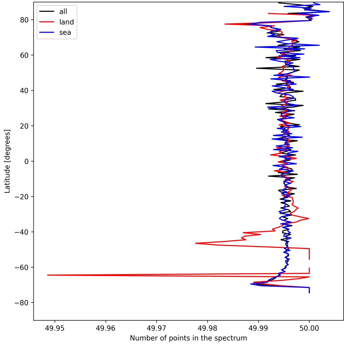
Figure 25: Zonal average of “Number of points in the spectrum” for 2025-08-16 to 2025-08-17.
