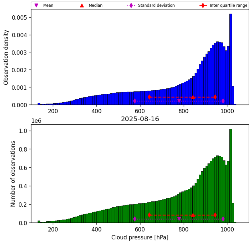
Figure 28: Histogram of “Cloud pressure” for 2025-08-16 to 2025-08-17
