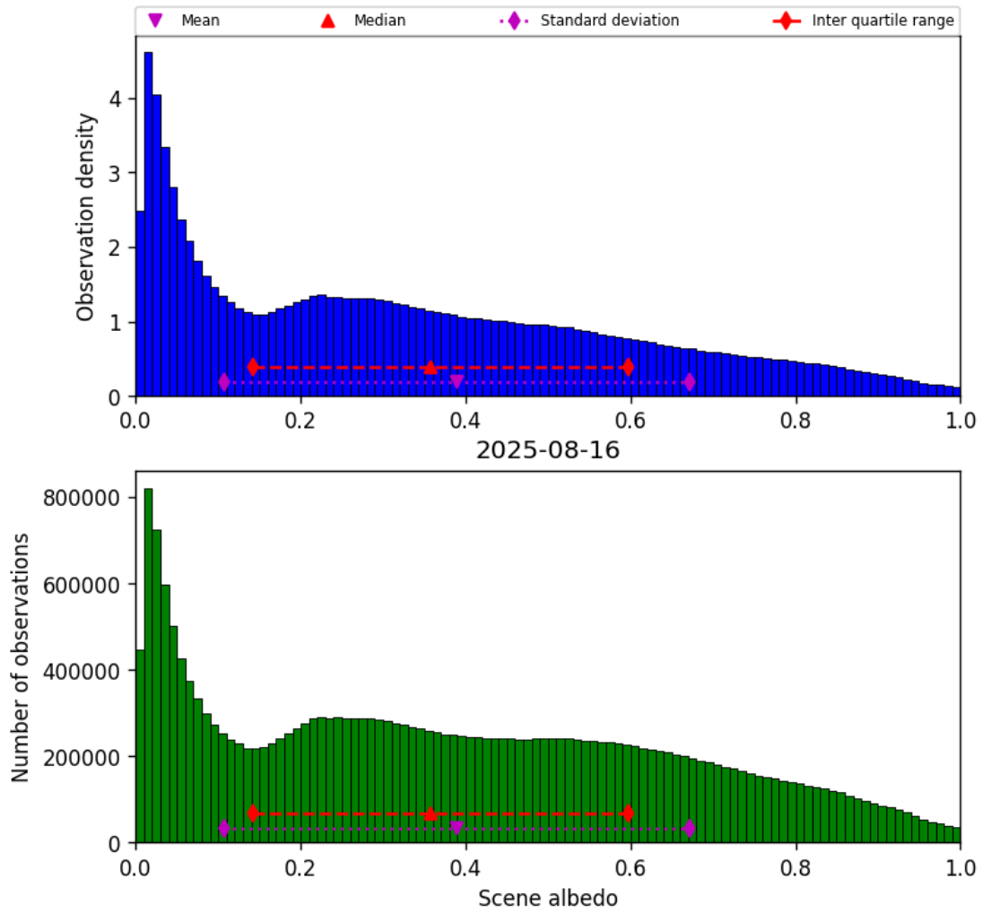
Figure 32: Histogram of “Scene albedo” for 2025-08-16 to 2025-08-17
