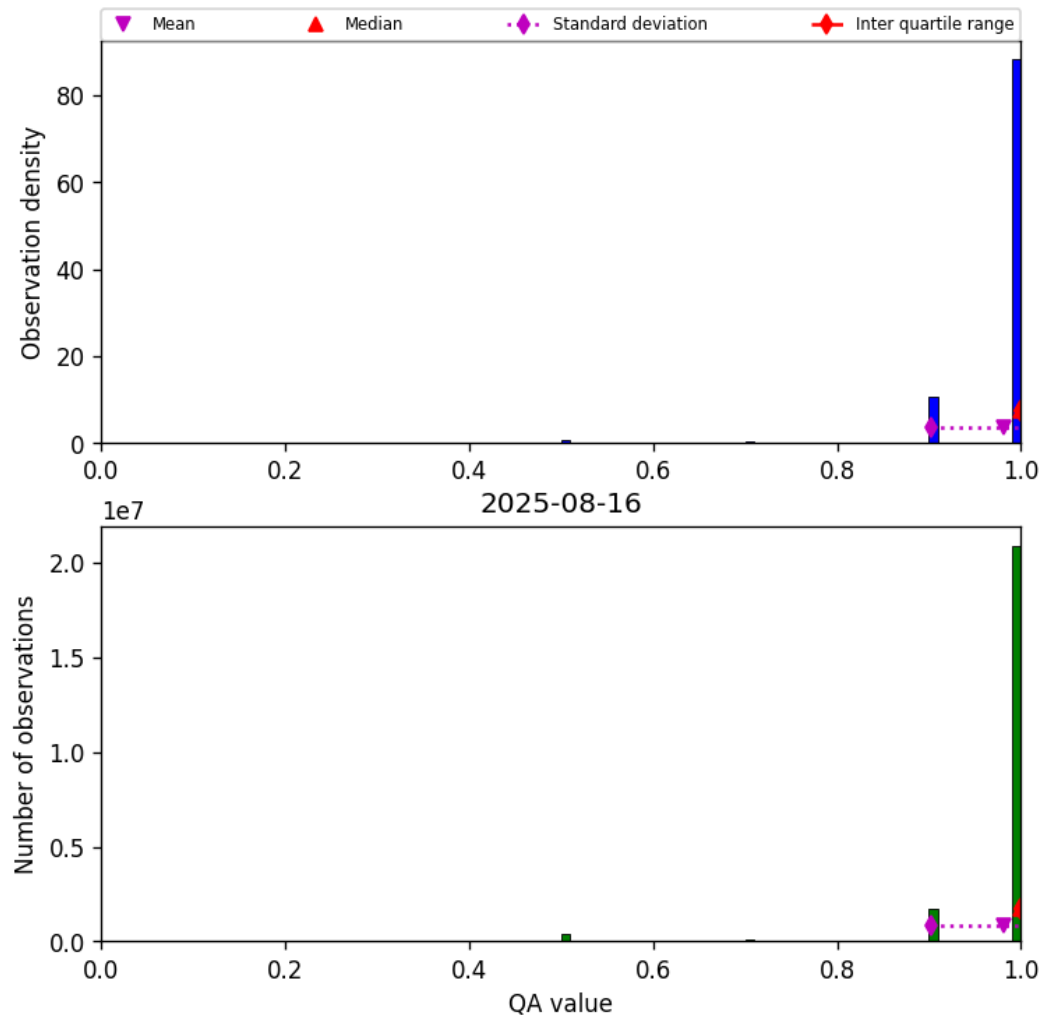
Figure 27: Histogram of “QA value” for 2025-08-16 to 2025-08-17
