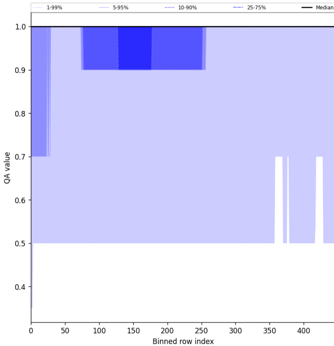
Figure 44: Along track statistics of “QA value” for 2025-08-16 to 2025-08-17
