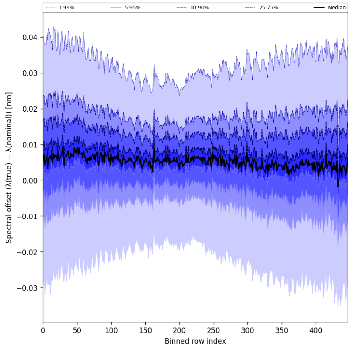
Figure 60: Along track statistics of “Spectral offset ( \lambda_{\text{true}} - \lambda_{\text{nominal}} )” for 2025-08-16 to 2025-08-17
