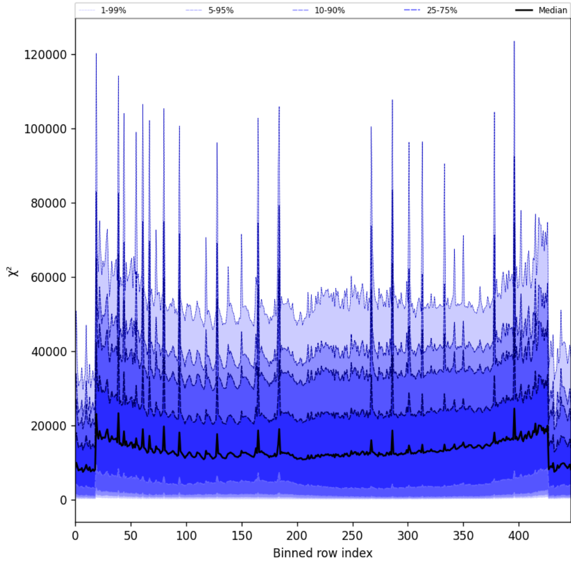
Figure 53: Along track statistics of “ \chi^2 ” for 2025-08-16 to 2025-08-17
