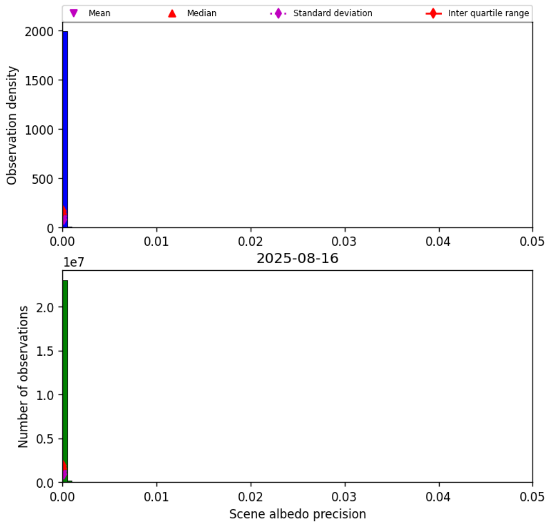
Figure 33: Histogram of “Scene albedo precision” for 2025-08-16 to 2025-08-17
