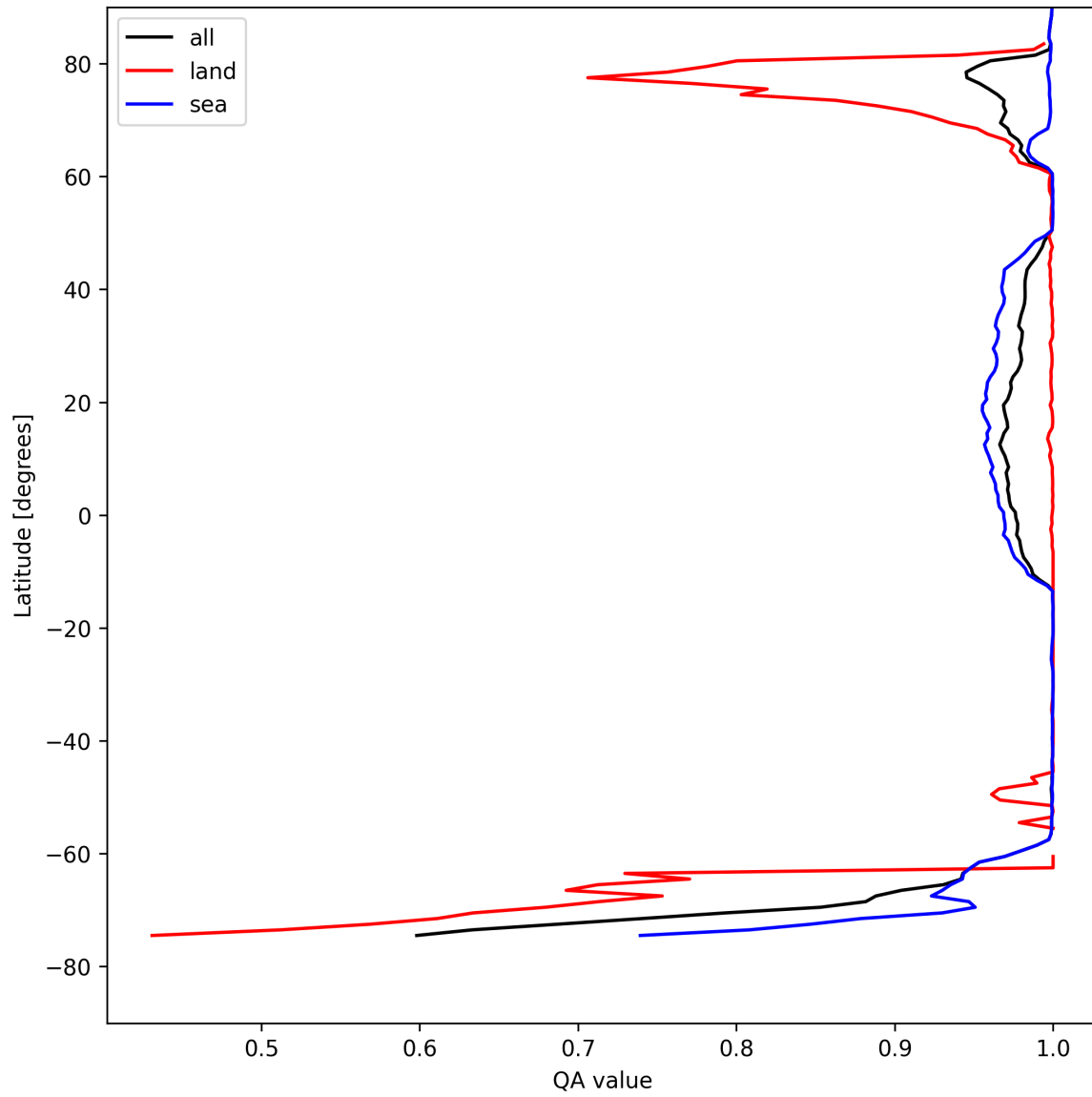
Figure 10: Zonal average of “QA value” for 2025-08-16 to 2025-08-17.
