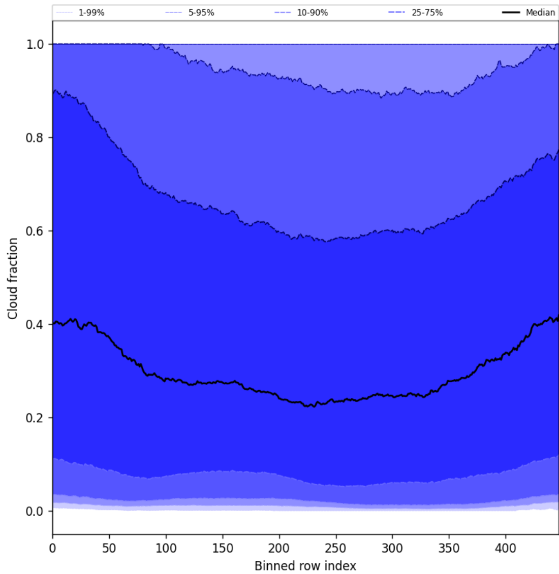
Figure 47: Along track statistics of “Cloud fraction” for 2025-08-16 to 2025-08-17
