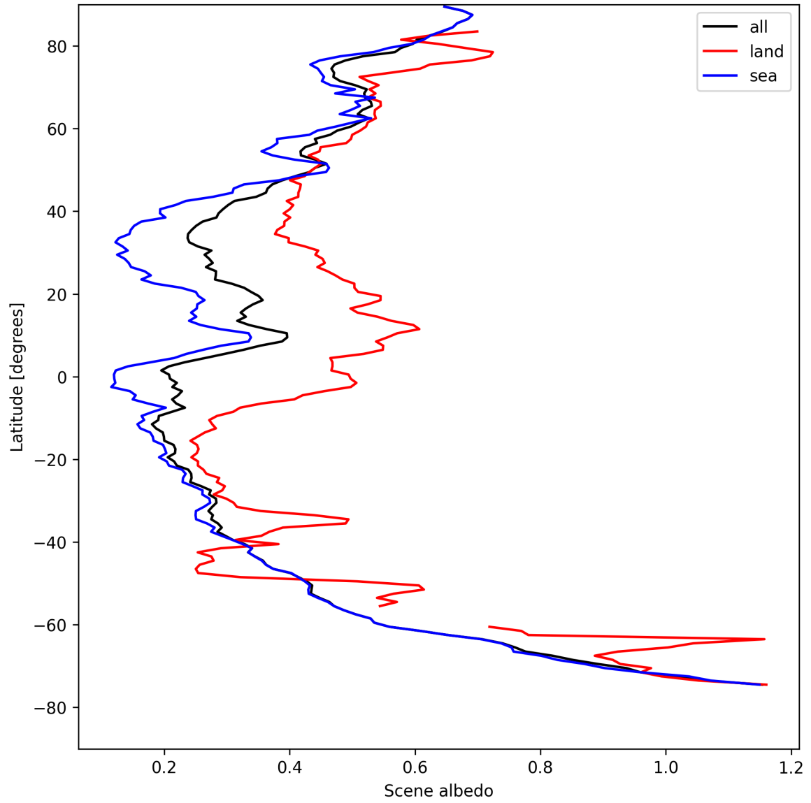
Figure 15: Zonal average of “Scene albedo” for 2025-08-16 to 2025-08-17.
