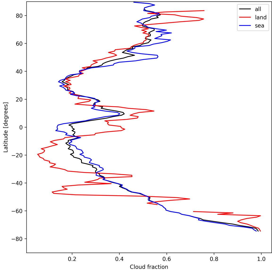
Figure 13: Zonal average of “Cloud fraction” for 2025-08-16 to 2025-08-17.
