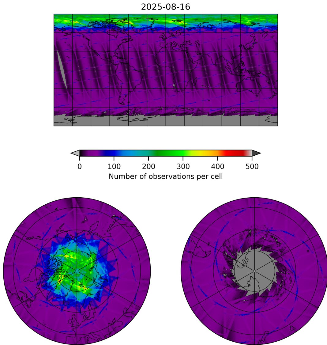
Figure 9: Map of the number of observations for 2025-08-16 to 2025-08-17
