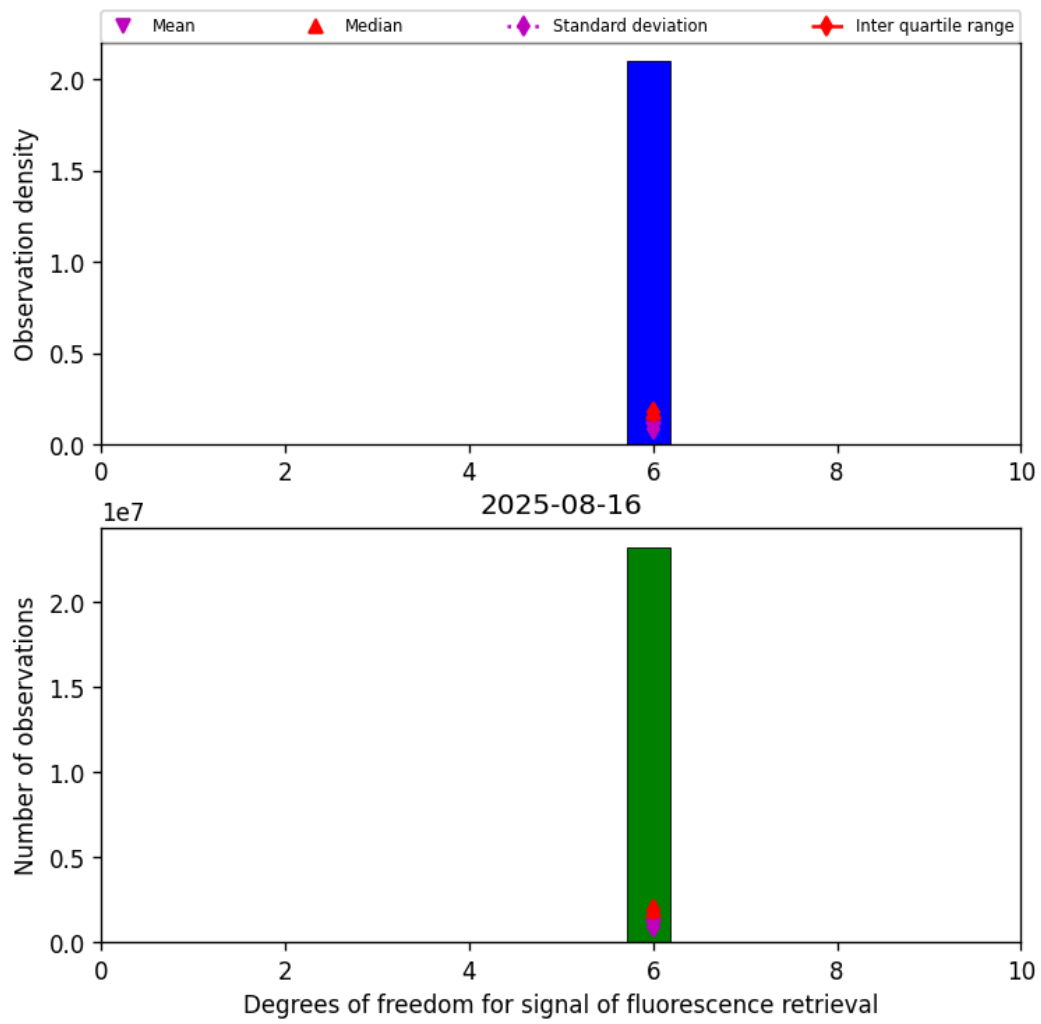
Figure 41: Histogram of “Degrees of freedom for signal of fluorescence retrieval” for 2025-08-16 to 2025-08-17
