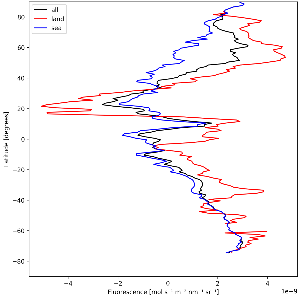
Figure 21: Zonal average of “Fluorescence” for 2025-08-16 to 2025-08-17.
