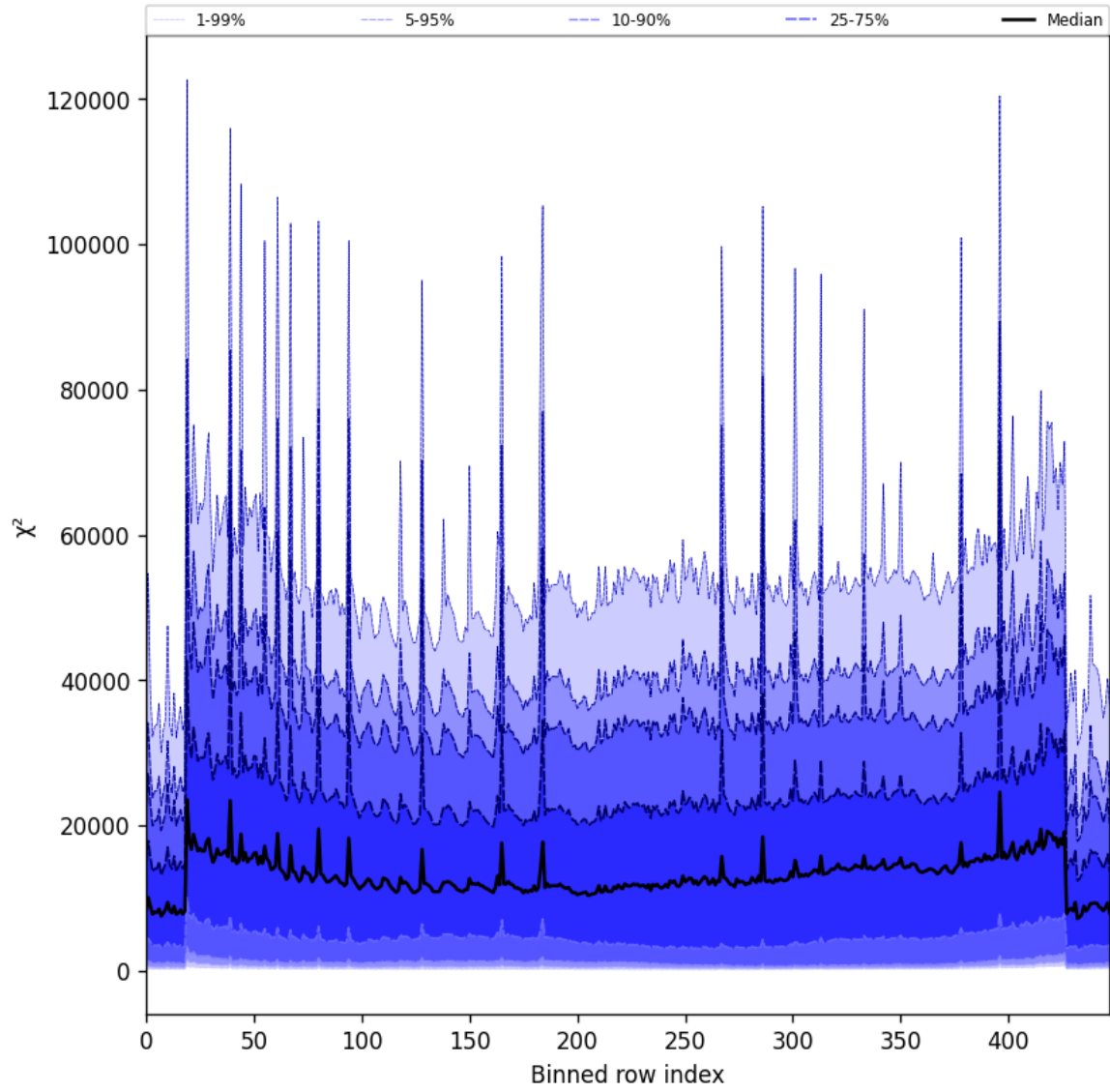
Figure 53: Along track statistics of “ \chi^2 ” for 2025-08-17 to 2025-08-17
