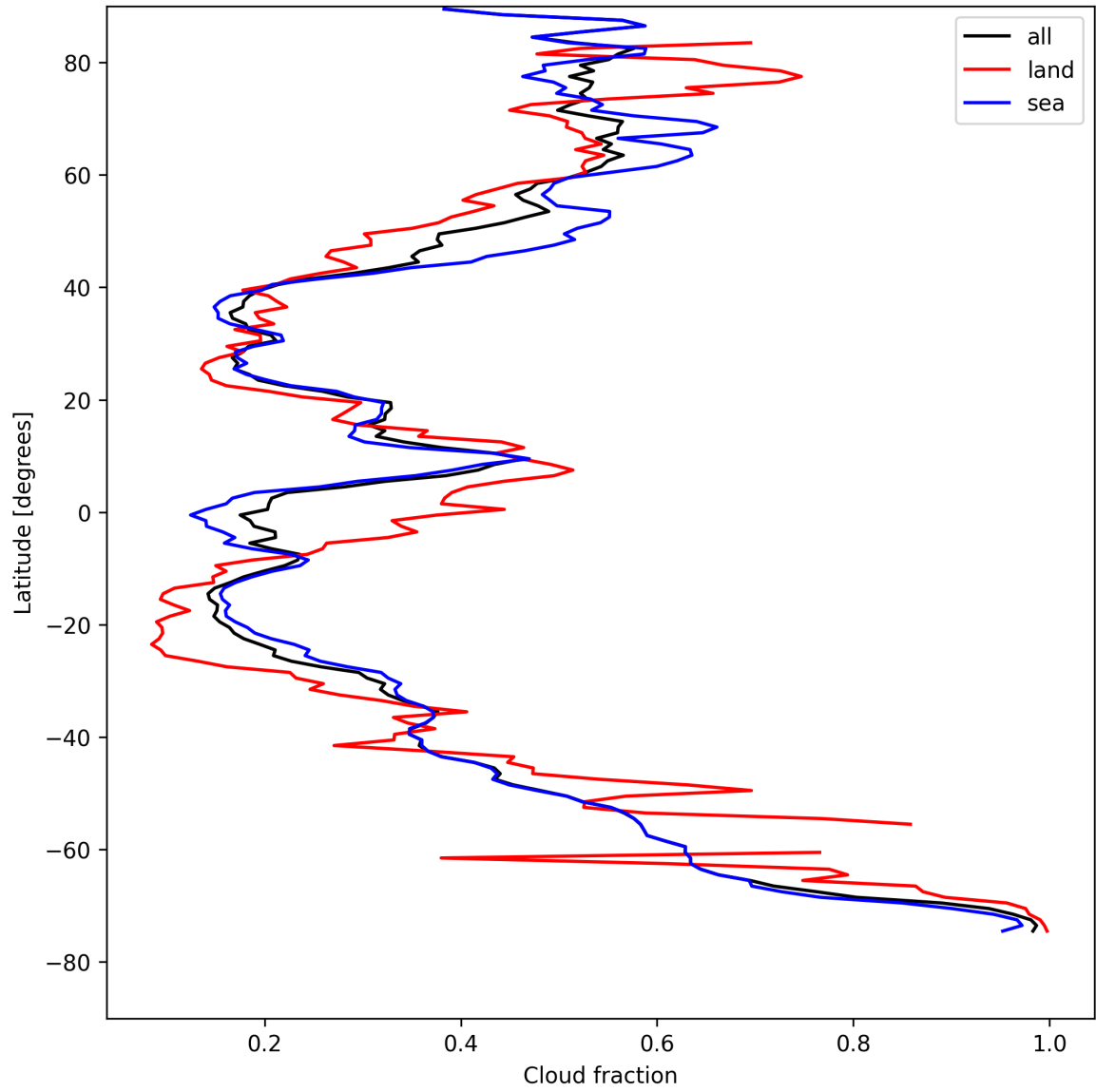
Figure 13: Zonal average of “Cloud fraction” for 2025-08-17 to 2025-08-17.
