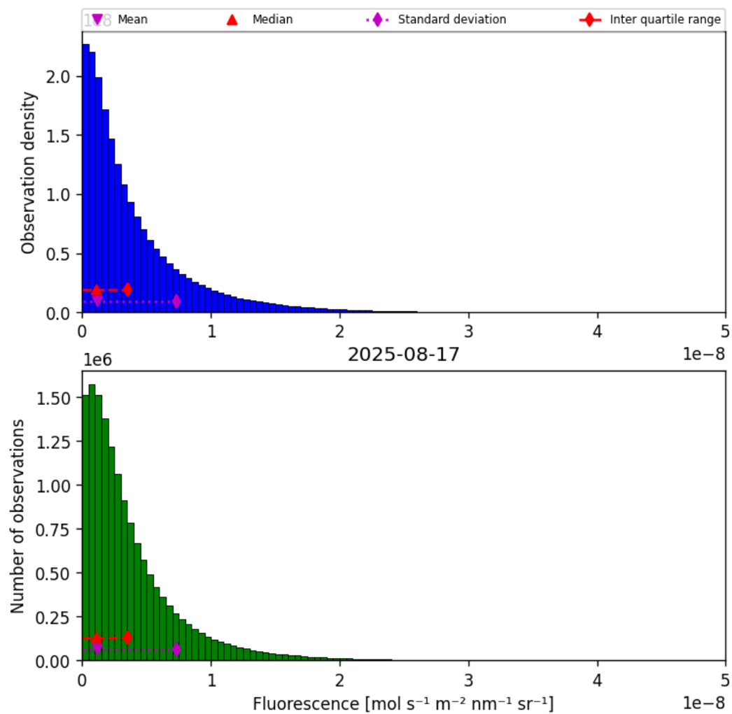
Figure 38: Histogram of “Fluorescence” for 2025-08-17 to 2025-08-17
