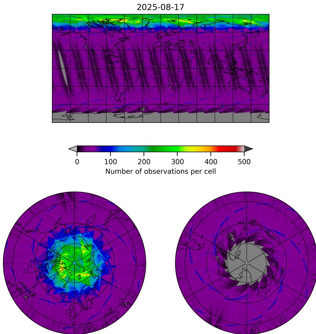
Figure 9: Map of the number of observations for 2025-08-17 to 2025-08-17
