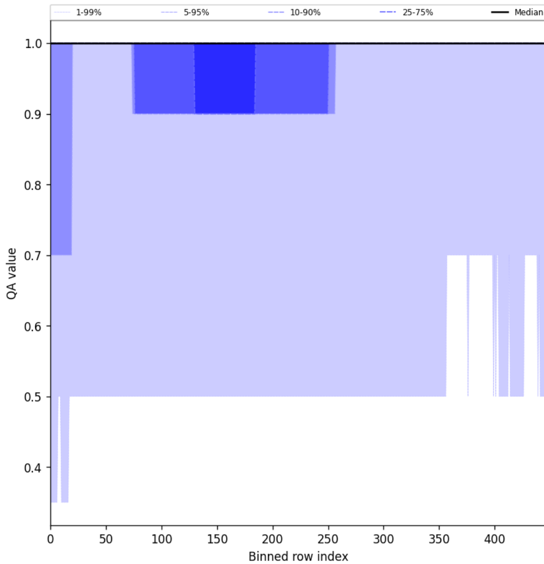
Figure 44: Along track statistics of “QA value” for 2025-08-17 to 2025-08-17
