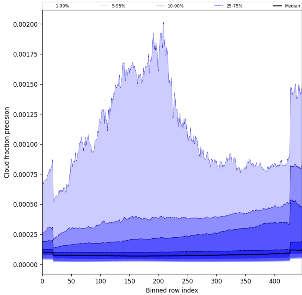
Figure 48: Along track statistics of “Cloud fraction precision” for 2025-08-17 to 2025-08-17
