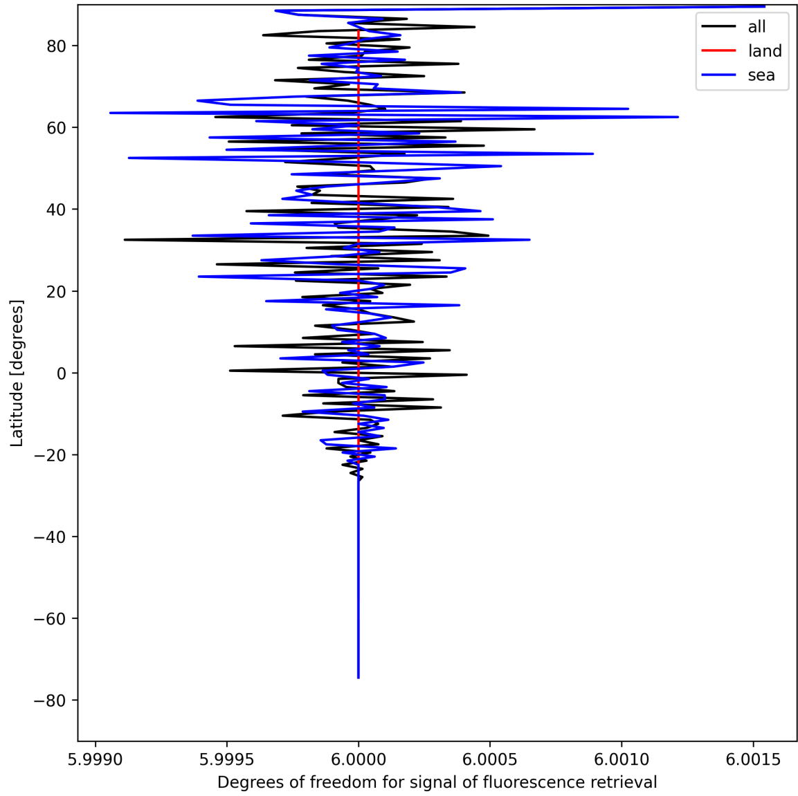
Figure 24: Zonal average of “Degrees of freedom for signal of fluorescence retrieval” for 2025-08-17 to 2025-08-17.
