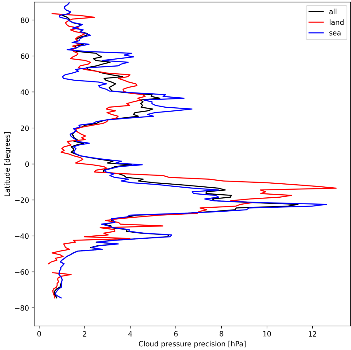
Figure 12: Zonal average of “Cloud pressure precision” for 2025-08-17 to 2025-08-17.
