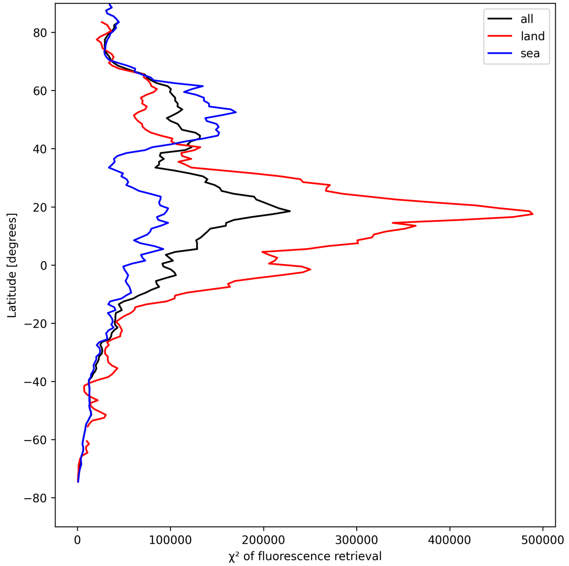
Figure 23: Zonal average of “ \chi^2 of fluorescence retrieval” for 2025-08-17 to 2025-08-17.
