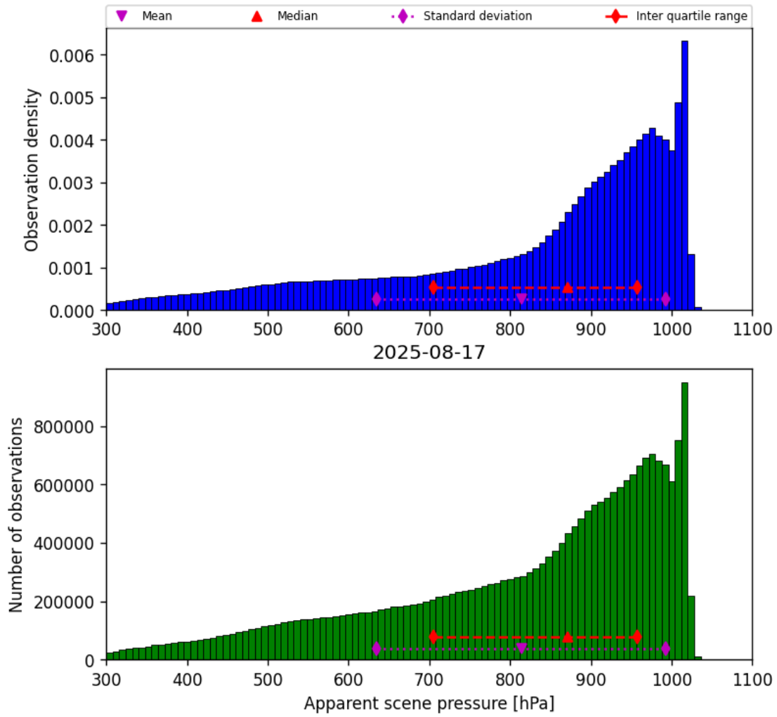
Figure 34: Histogram of “Apparent scene pressure” for 2025-08-17 to 2025-08-17
