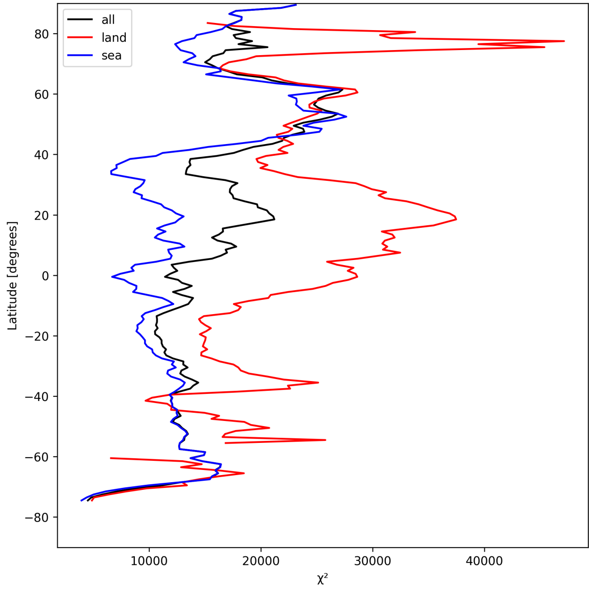
Figure 19: Zonal average of “ \chi^2 ” for 2025-08-17 to 2025-08-17.
