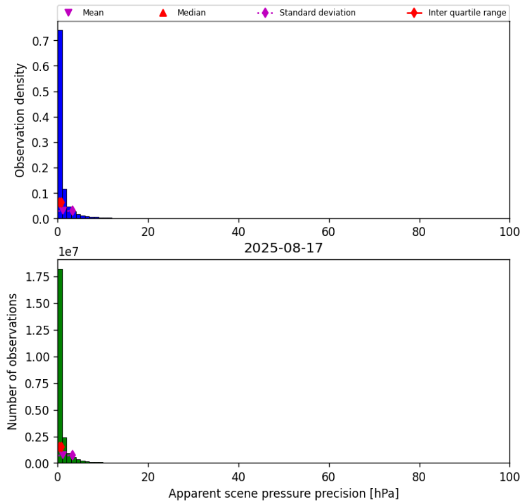
Figure 35: Histogram of “Apparent scene pressure precision” for 2025-08-17 to 2025-08-17
