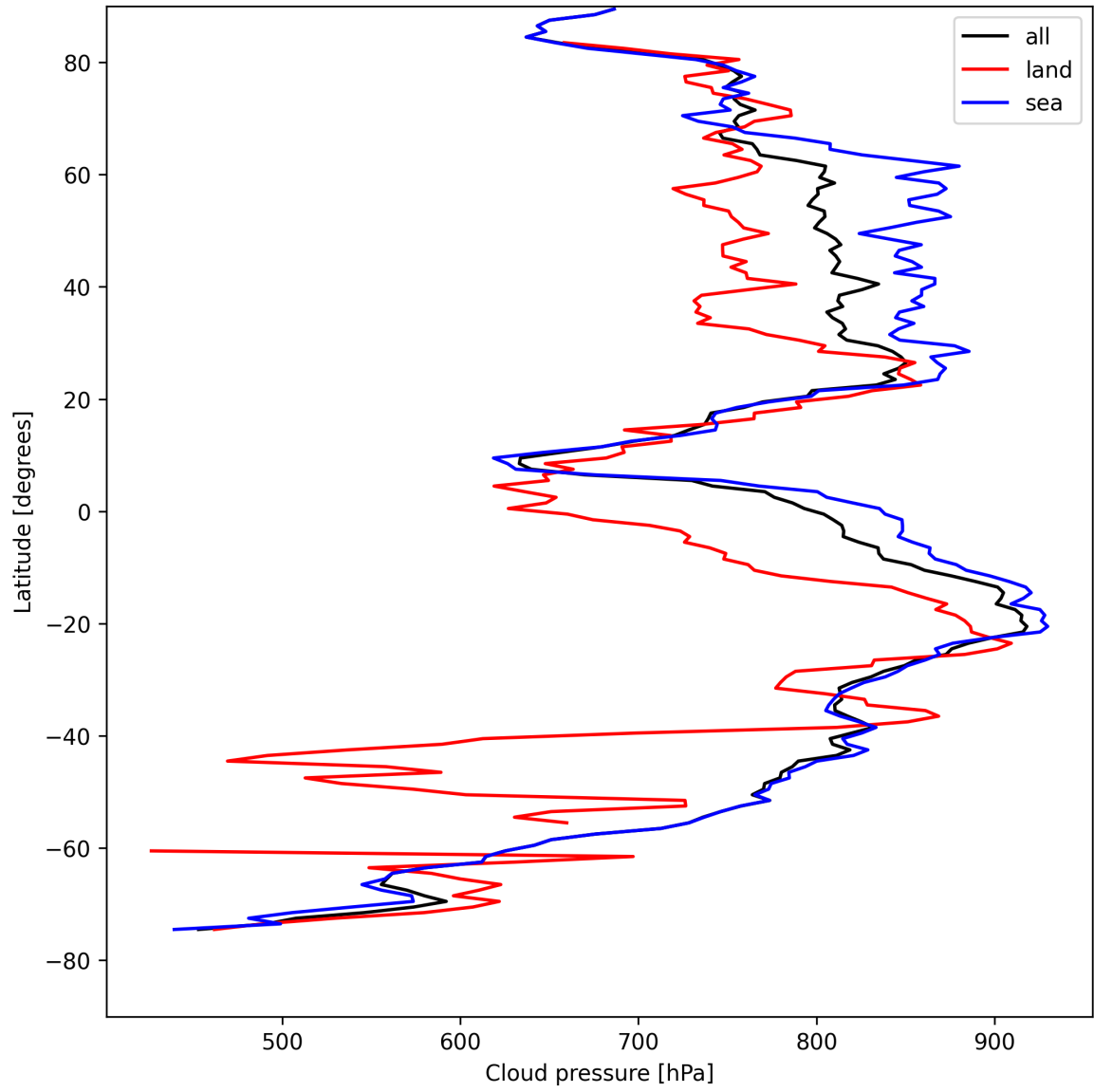
Figure 11: Zonal average of “Cloud pressure” for 2025-08-17 to 2025-08-17.
