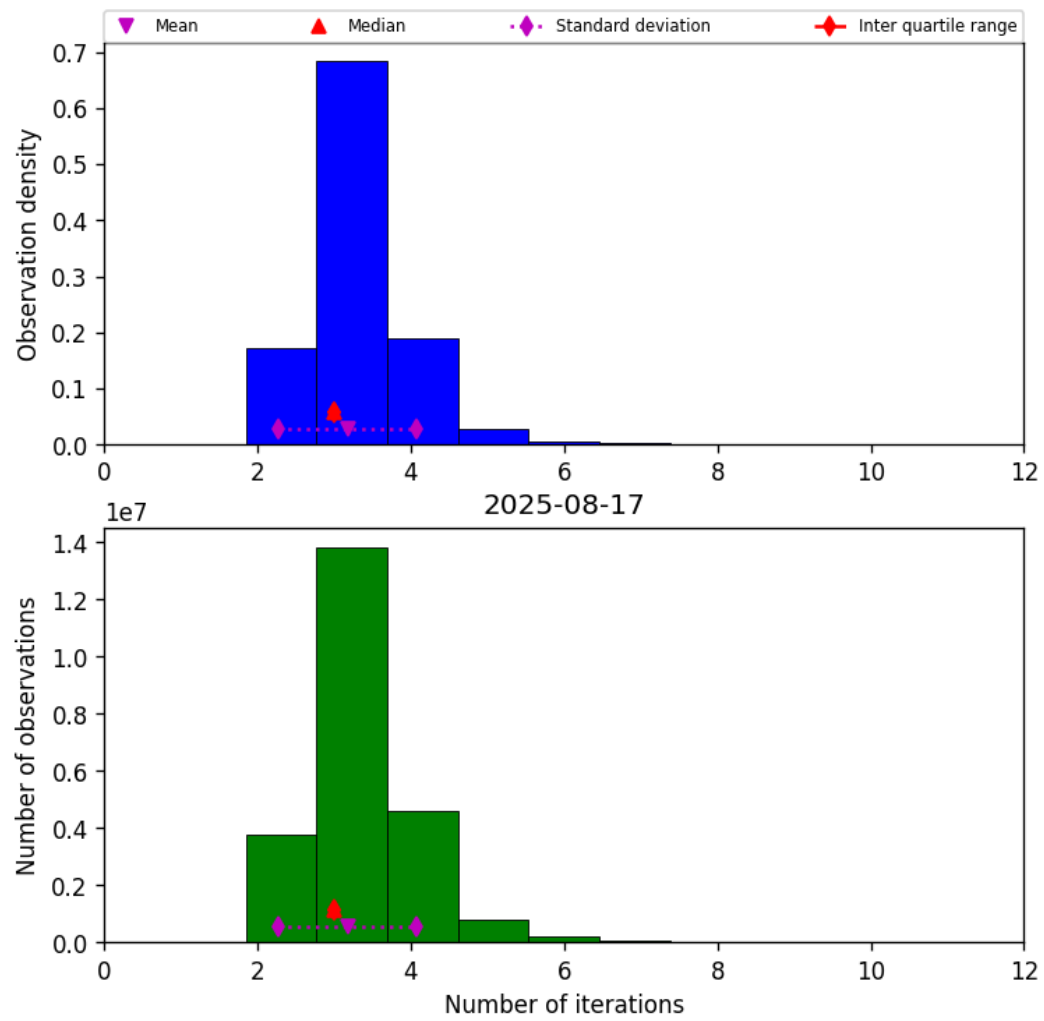
Figure 37: Histogram of “Number of iterations” for 2025-08-17 to 2025-08-17
