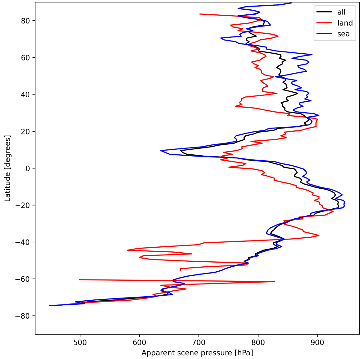
Figure 17: Zonal average of “Apparent scene pressure” for 2025-08-17 to 2025-08-17.
