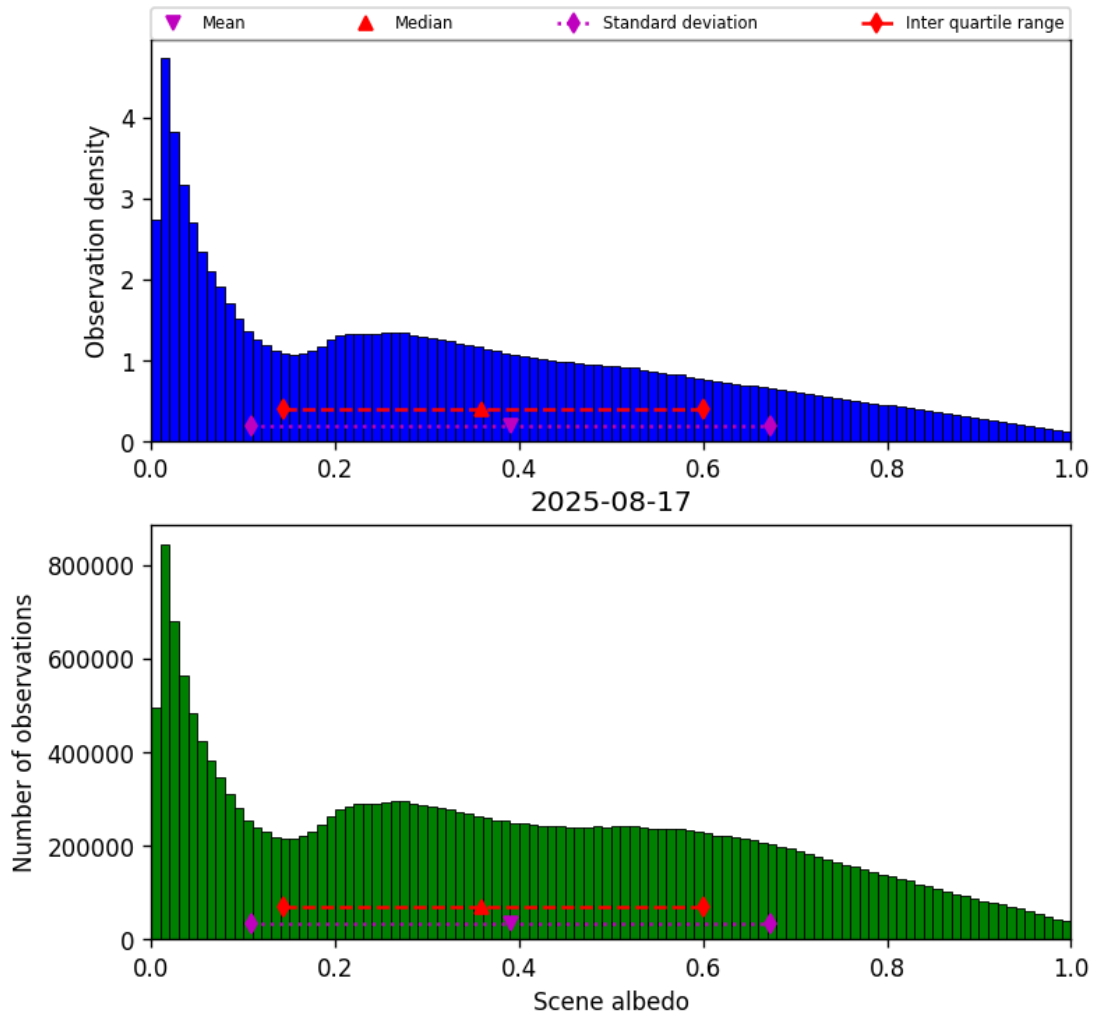
Figure 32: Histogram of “Scene albedo” for 2025-08-17 to 2025-08-17
