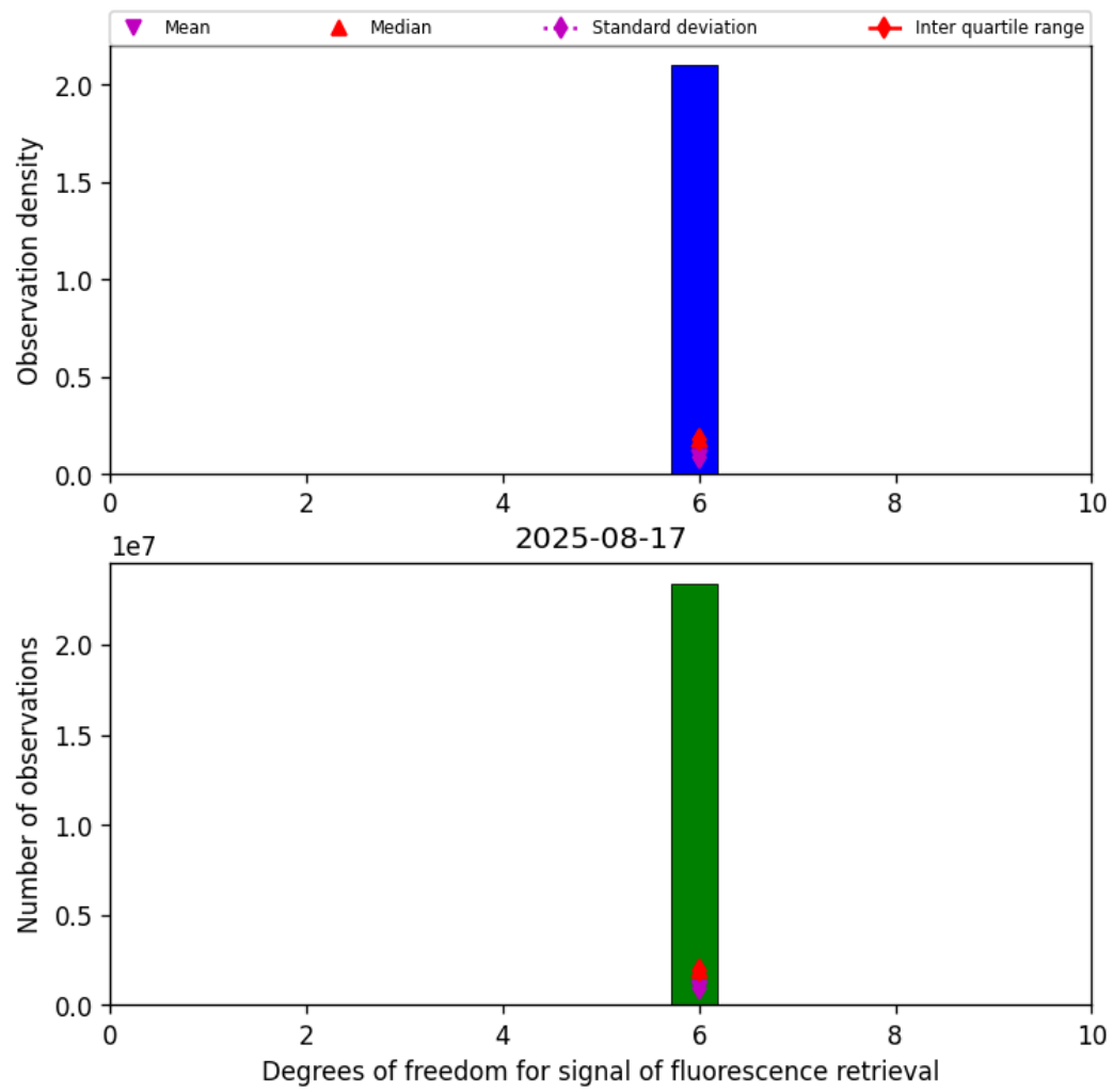
Figure 41: Histogram of “Degrees of freedom for signal of fluorescence retrieval” for 2025-08-17 to 2025-08-17
