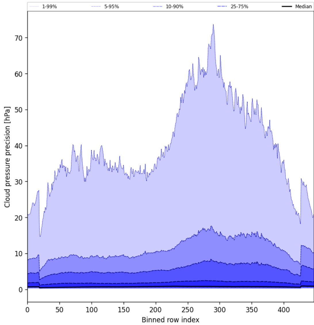
Figure 46: Along track statistics of “Cloud pressure precision” for 2025-08-17 to 2025-08-17
