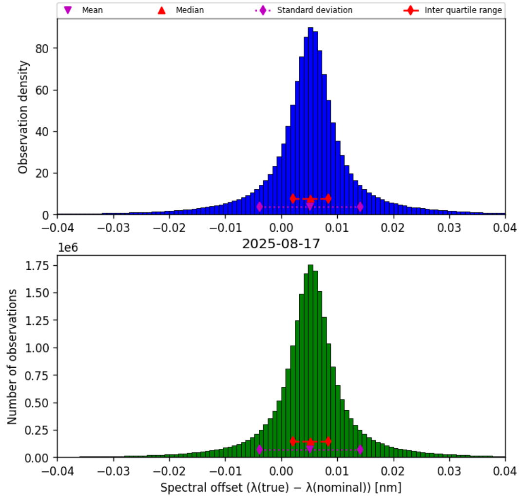
Figure 43: Histogram of “Spectral offset ( \lambda_{\text{true}} - \lambda_{\text{nominal}} )” for 2025-08-17 to 2025-08-17
