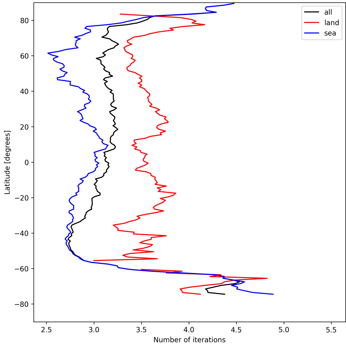
Figure 20: Zonal average of “Number of iterations” for 2025-08-17 to 2025-08-17.
