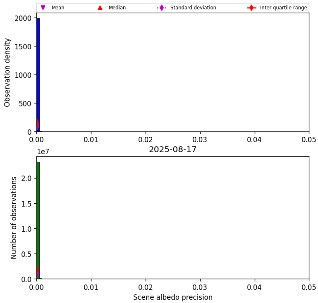
Figure 33: Histogram of “Scene albedo precision” for 2025-08-17 to 2025-08-17
