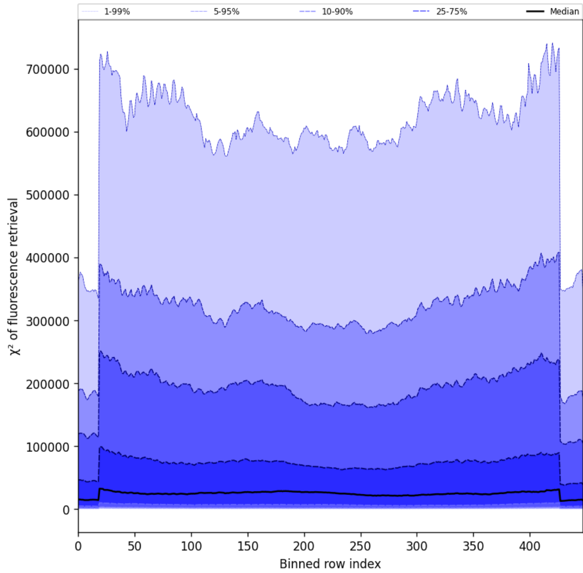
Figure 57: Along track statistics of “ \chi^2 of fluorescence retrieval” for 2025-08-17 to 2025-08-17
