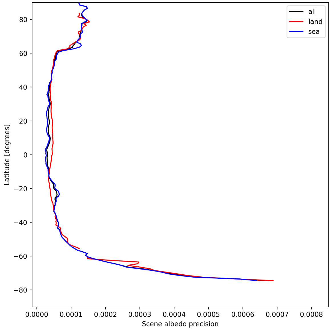
Figure 16: Zonal average of “Scene albedo precision” for 2025-08-17 to 2025-08-17.
