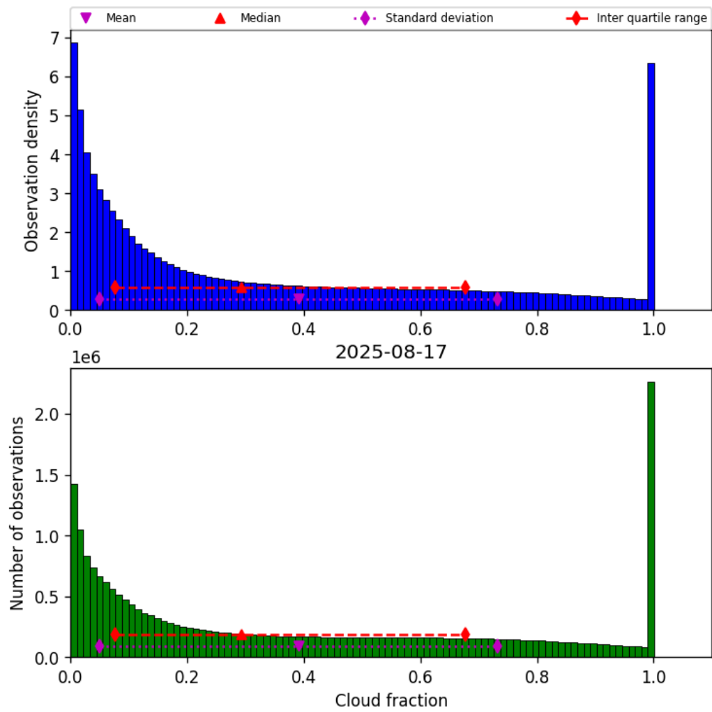
Figure 30: Histogram of “Cloud fraction” for 2025-08-17 to 2025-08-17
