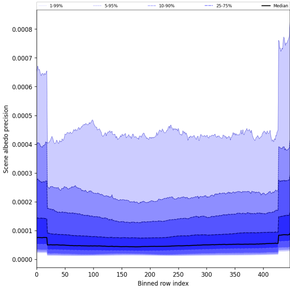
Figure 50: Along track statistics of “Scene albedo precision” for 2025-08-17 to 2025-08-17
