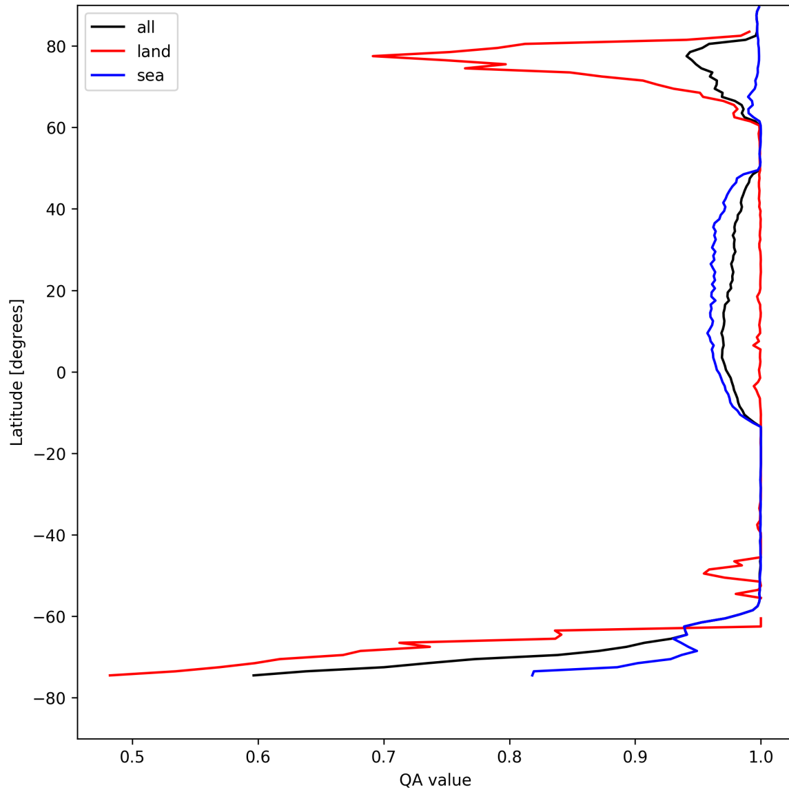
Figure 10: Zonal average of “QA value” for 2025-08-17 to 2025-08-17.
