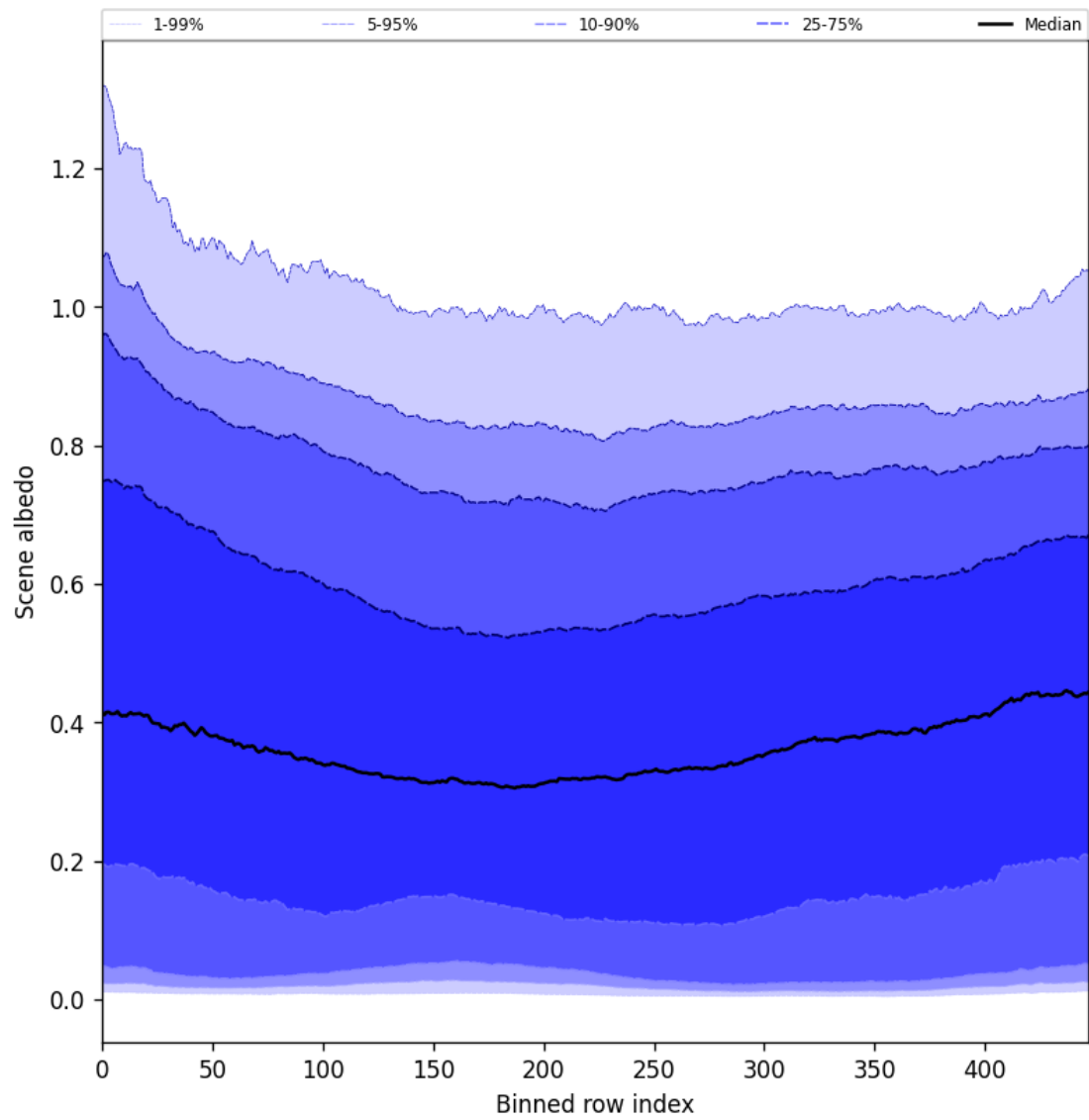
Figure 49: Along track statistics of “Scene albedo” for 2025-08-17 to 2025-08-17
