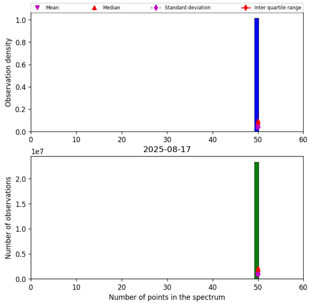
Figure 42: Histogram of “Number of points in the spectrum” for 2025-08-17 to 2025-08-17
