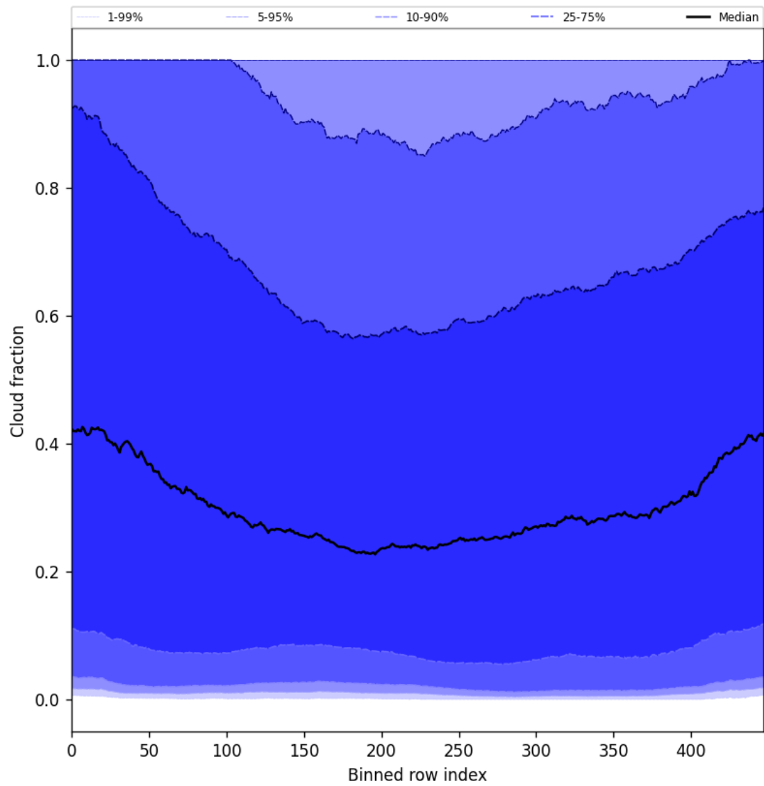
Figure 47: Along track statistics of “Cloud fraction” for 2025-08-17 to 2025-08-17
