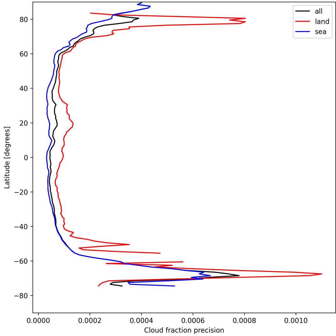
Figure 14: Zonal average of “Cloud fraction precision” for 2025-08-17 to 2025-08-17.
