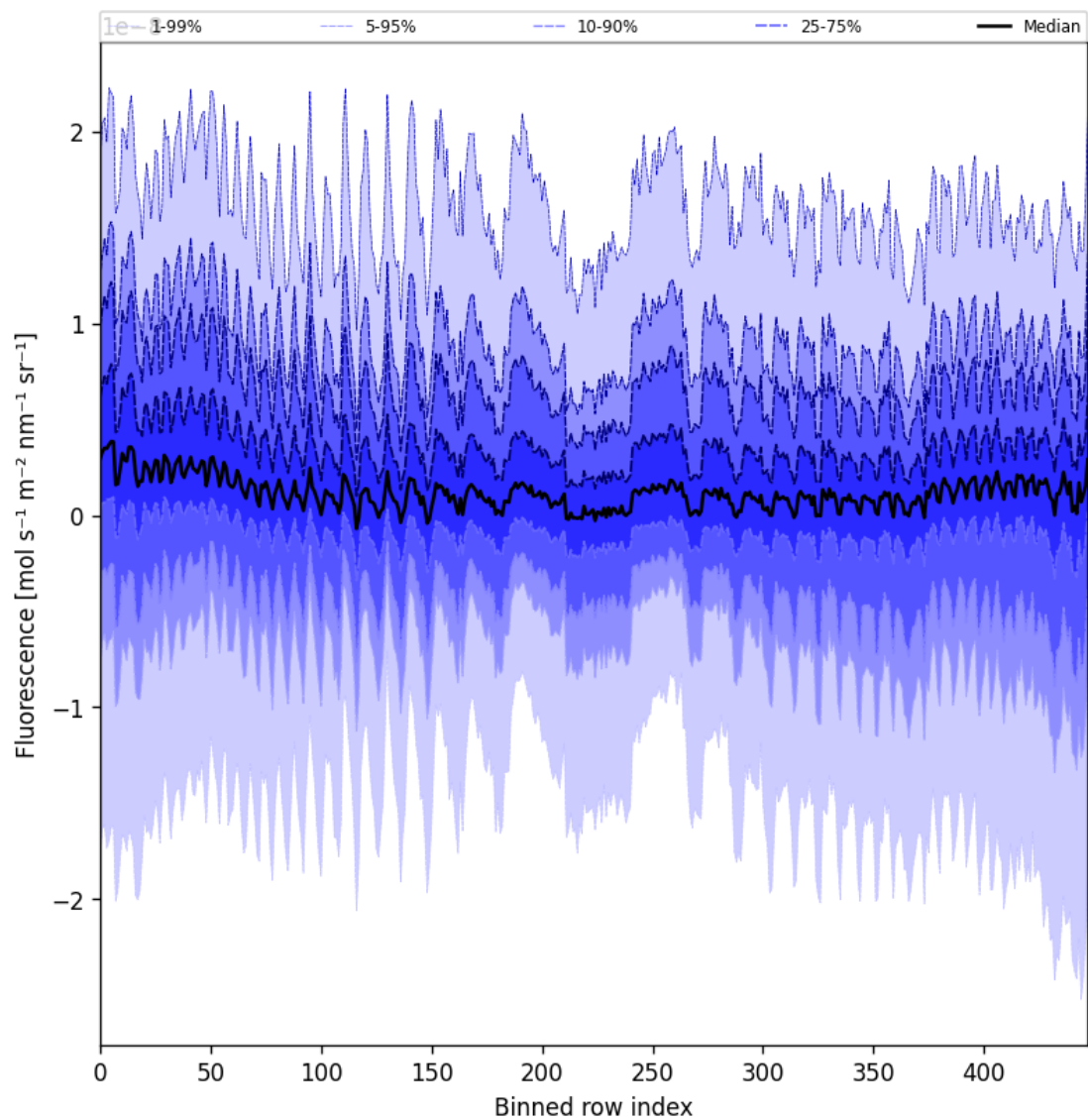
Figure 55: Along track statistics of “Fluorescence” for 2025-08-17 to 2025-08-17
