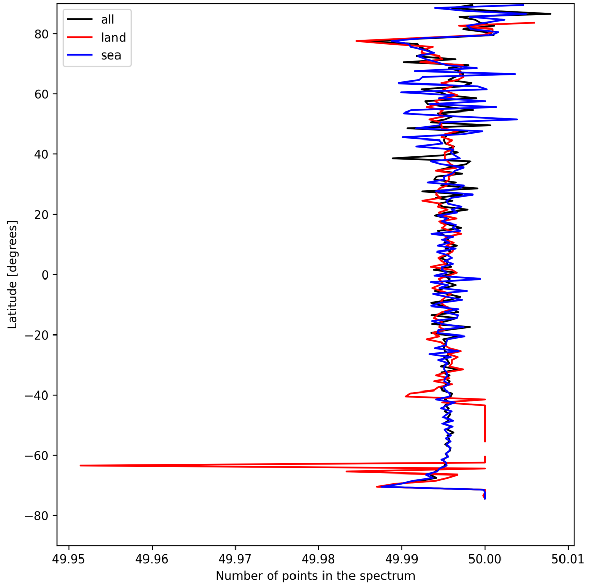
Figure 25: Zonal average of “Number of points in the spectrum” for 2025-08-17 to 2025-08-17.
