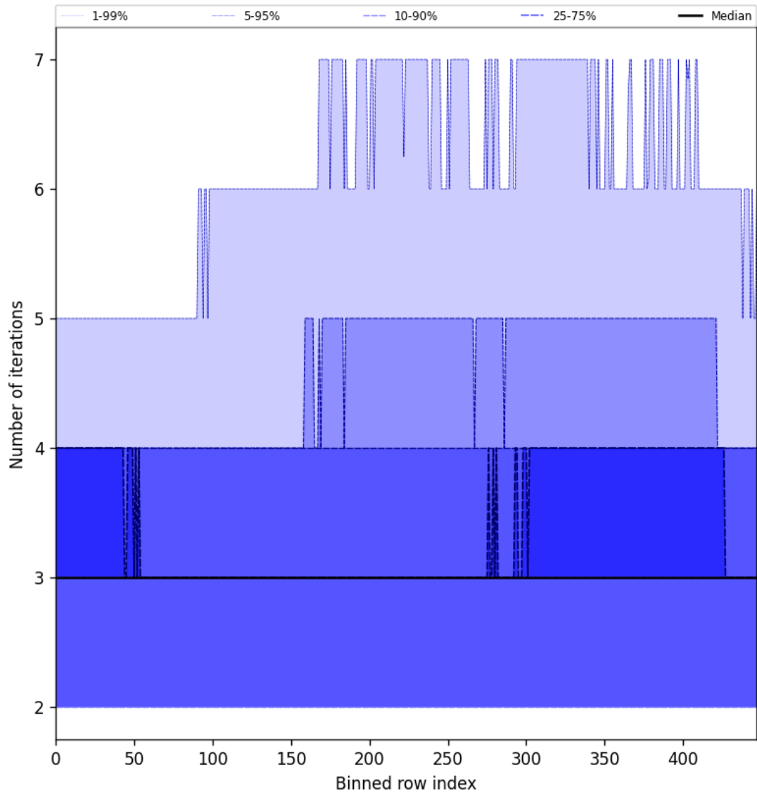
Figure 54: Along track statistics of “Number of iterations” for 2025-08-17 to 2025-08-17
