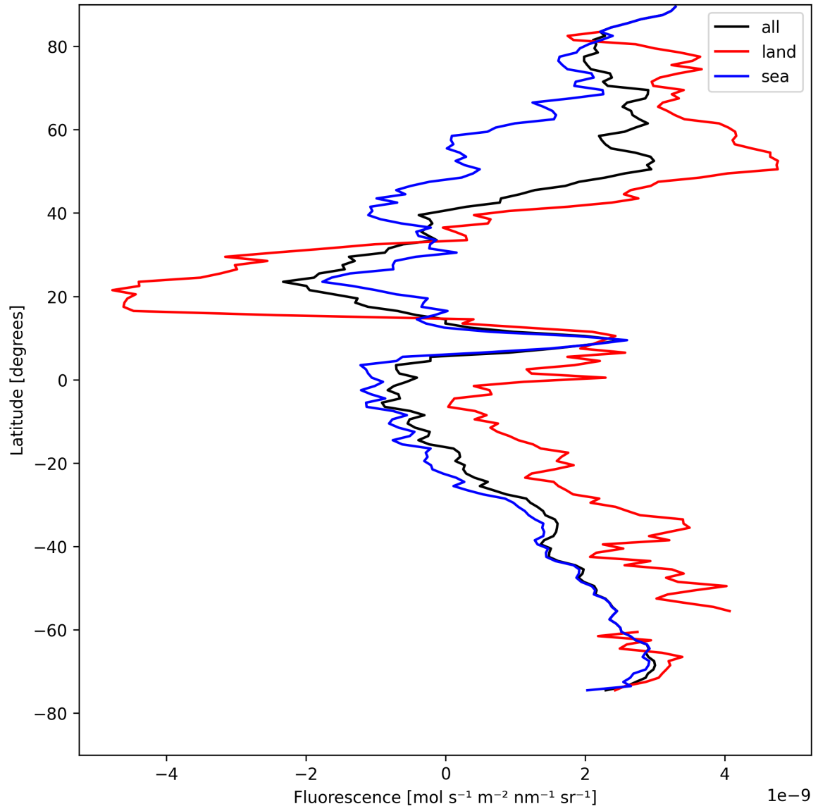
Figure 21: Zonal average of “Fluorescence” for 2025-08-17 to 2025-08-17.
