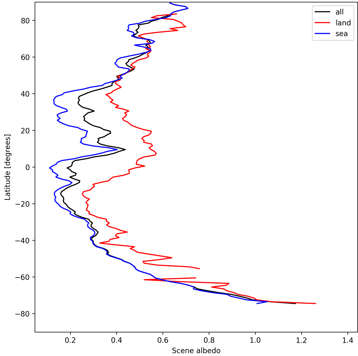
Figure 15: Zonal average of “Scene albedo” for 2025-08-17 to 2025-08-17.
