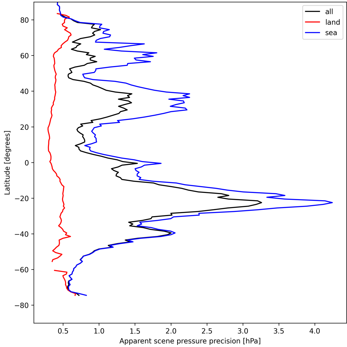
Figure 18: Zonal average of “Apparent scene pressure precision” for 2025-08-17 to 2025-08-17.
