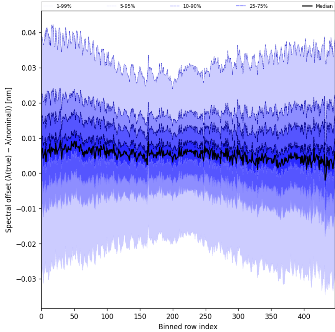
Figure 60: Along track statistics of “Spectral offset ( \lambda_{\text{true}} - \lambda_{\text{nominal}} )” for 2025-08-17 to 2025-08-17
