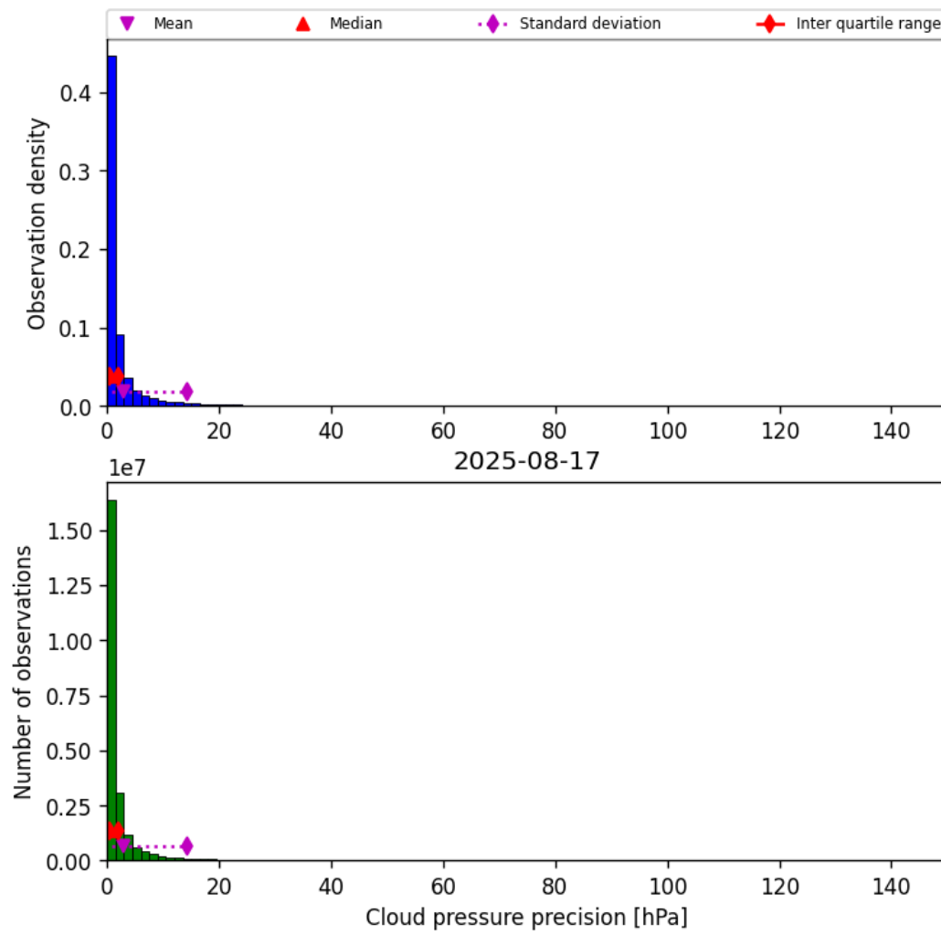
Figure 29: Histogram of “Cloud pressure precision” for 2025-08-17 to 2025-08-17
