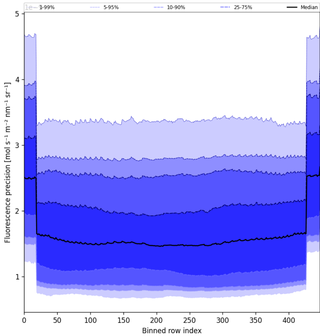
Figure 56: Along track statistics of “Fluorescence precision” for 2025-08-17 to 2025-08-17
