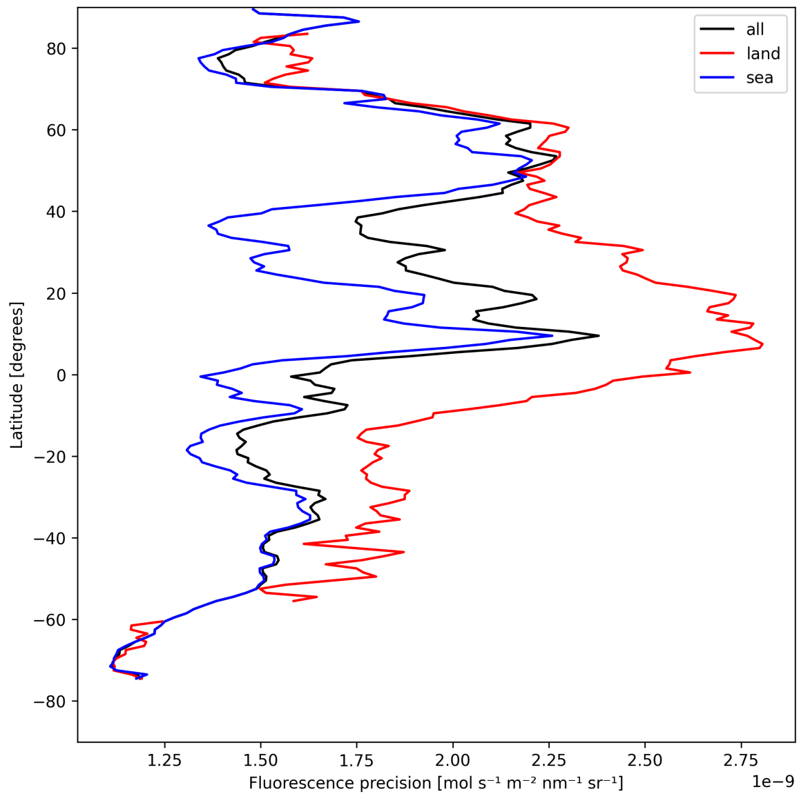
Figure 22: Zonal average of “Fluorescence precision” for 2025-08-17 to 2025-08-17.
