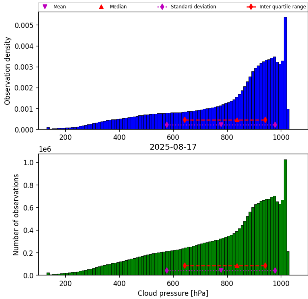
Figure 28: Histogram of “Cloud pressure” for 2025-08-17 to 2025-08-17
