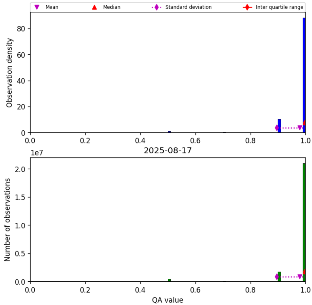
Figure 27: Histogram of “QA value” for 2025-08-17 to 2025-08-17
