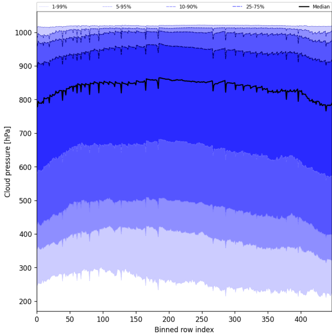
Figure 45: Along track statistics of “Cloud pressure” for 2025-08-17 to 2025-08-17
