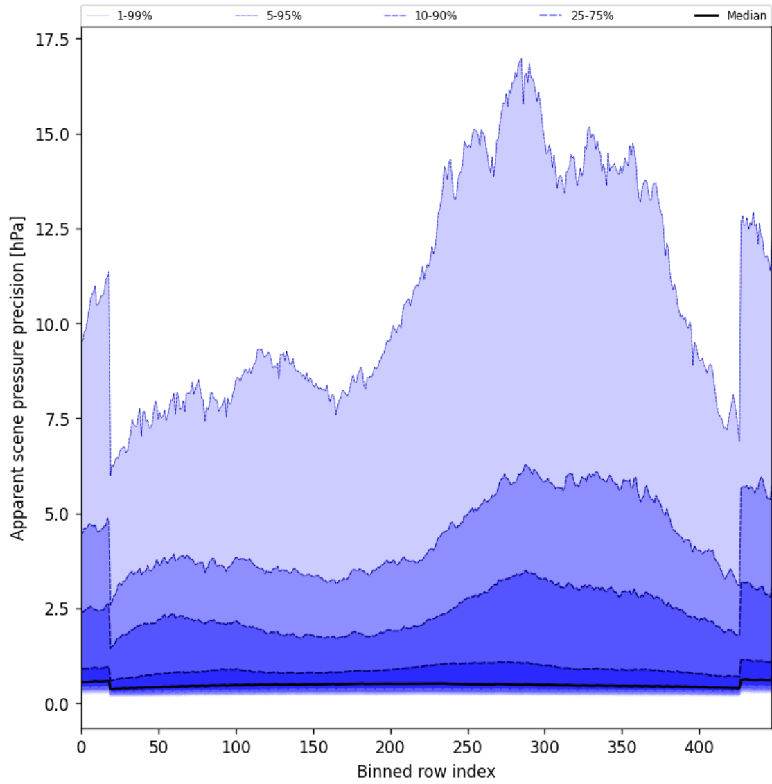
Figure 52: Along track statistics of “Apparent scene pressure precision” for 2025-08-17 to 2025-08-17
