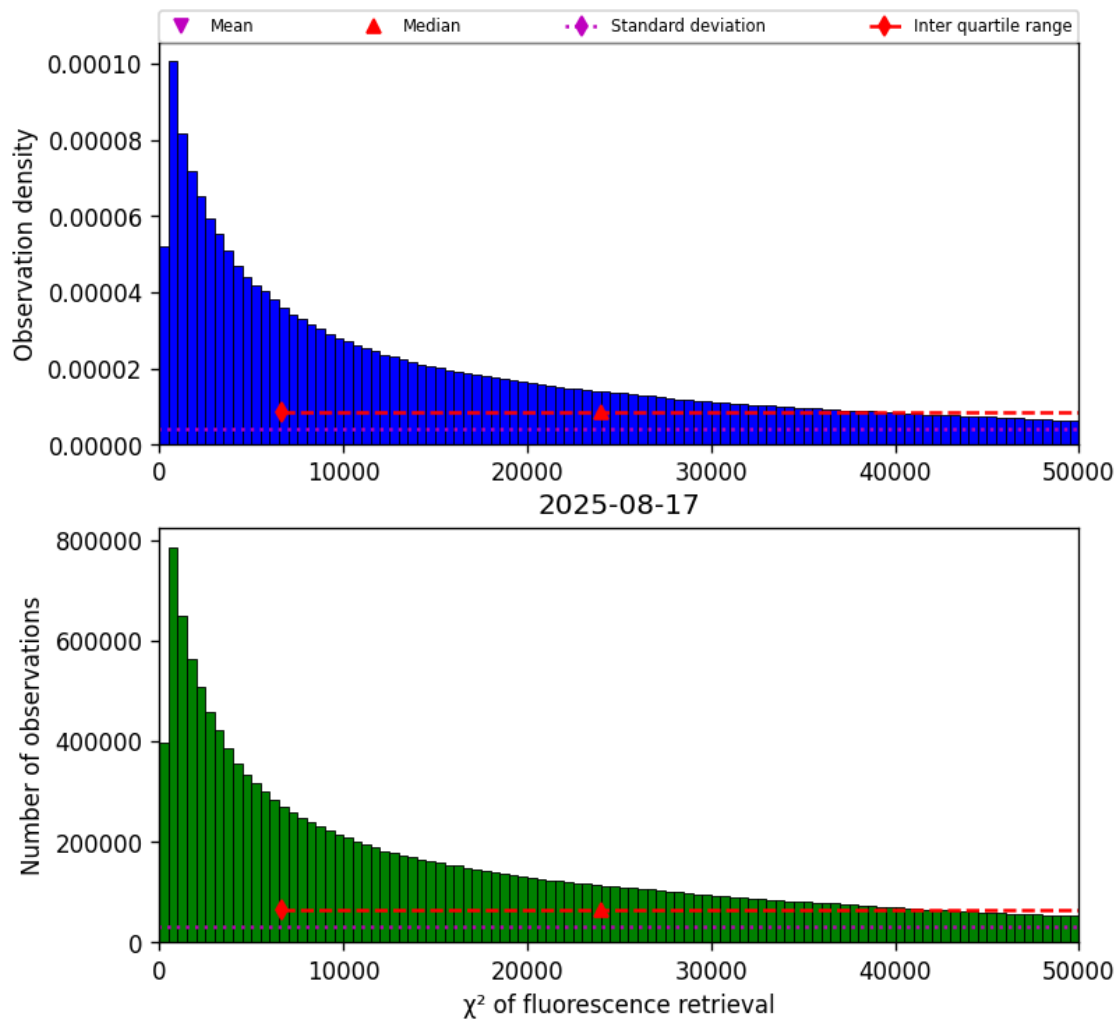
Figure 40: Histogram of “ \chi^2 of fluorescence retrieval” for 2025-08-17 to 2025-08-17
