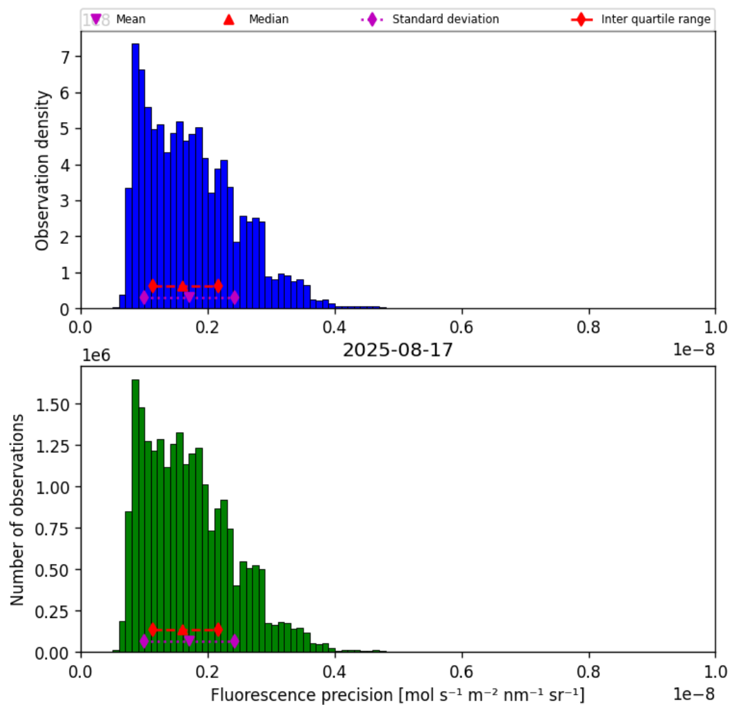
Figure 39: Histogram of “Fluorescence precision” for 2025-08-17 to 2025-08-17
