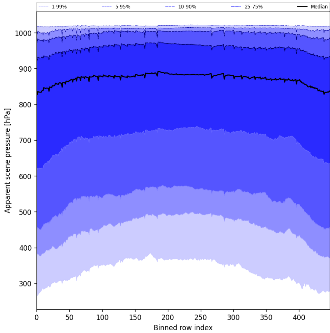
Figure 51: Along track statistics of “Apparent scene pressure” for 2025-08-17 to 2025-08-17
