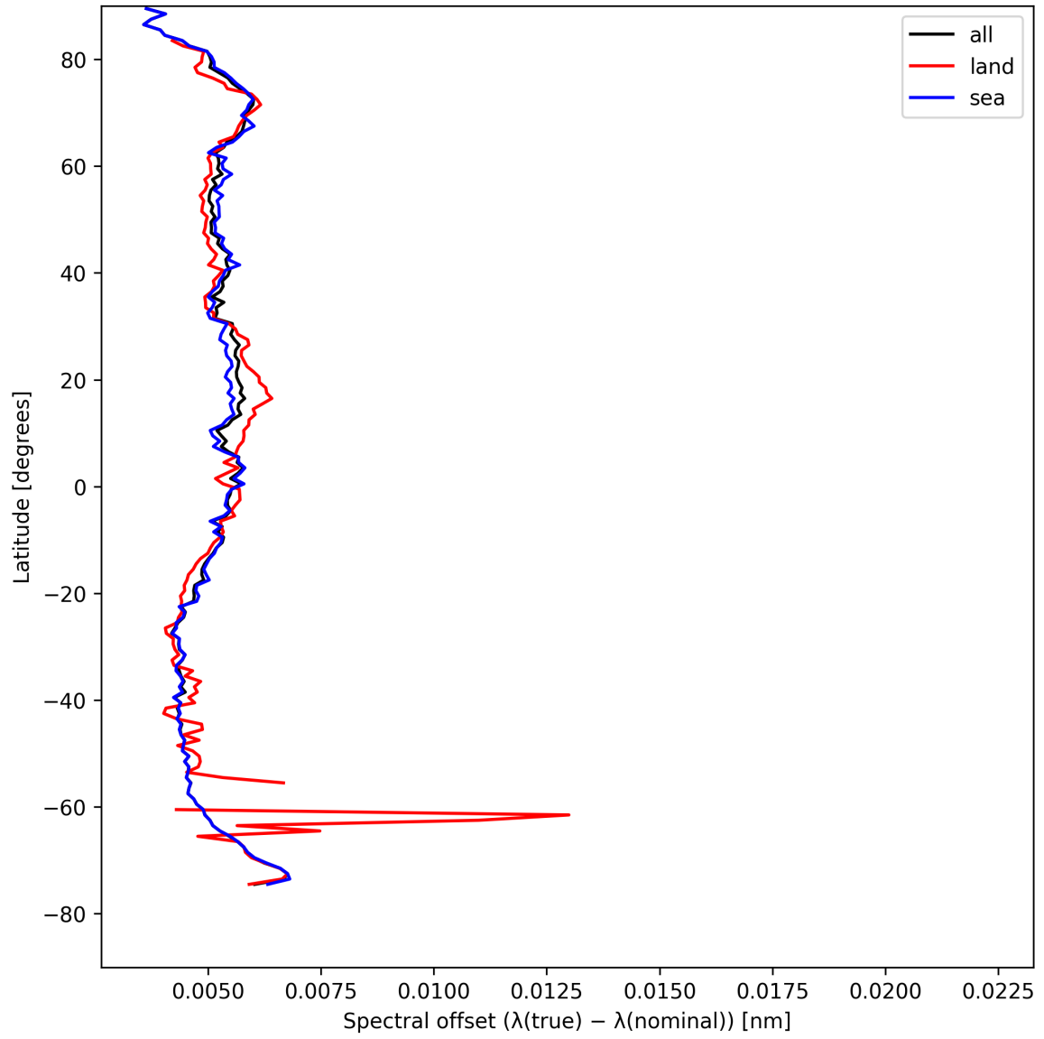
Figure 26: Zonal average of “Spectral offset ( \lambda_{\text{true}} - \lambda_{\text{nominal}} )” for 2025-08-17 to 2025-08-17.
