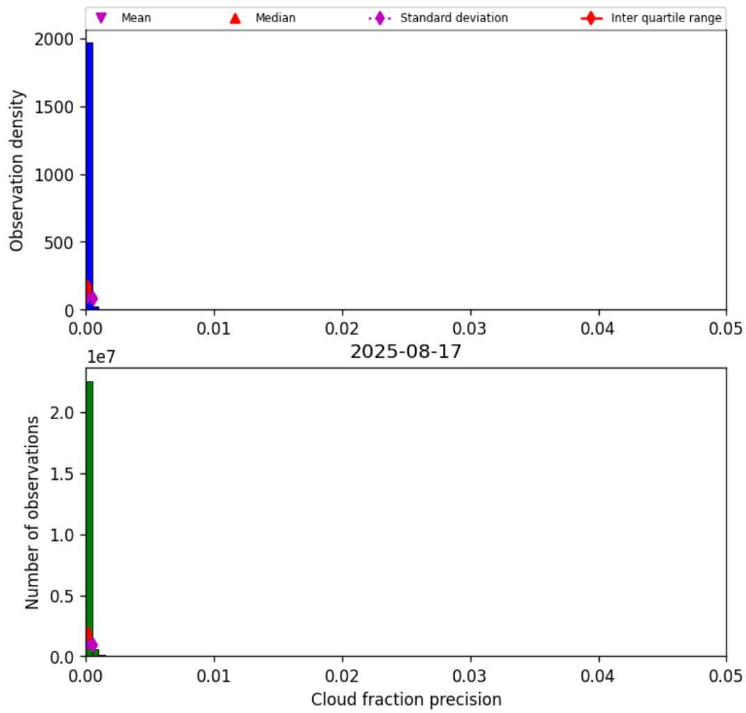
Figure 31: Histogram of “Cloud fraction precision” for 2025-08-17 to 2025-08-17
