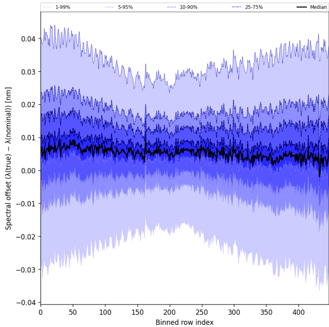
Figure 60: Along track statistics of “Spectral offset ( \lambda_{\text{true}} - \lambda_{\text{nominal}} )” for 2025-08-18 to 2025-08-19
