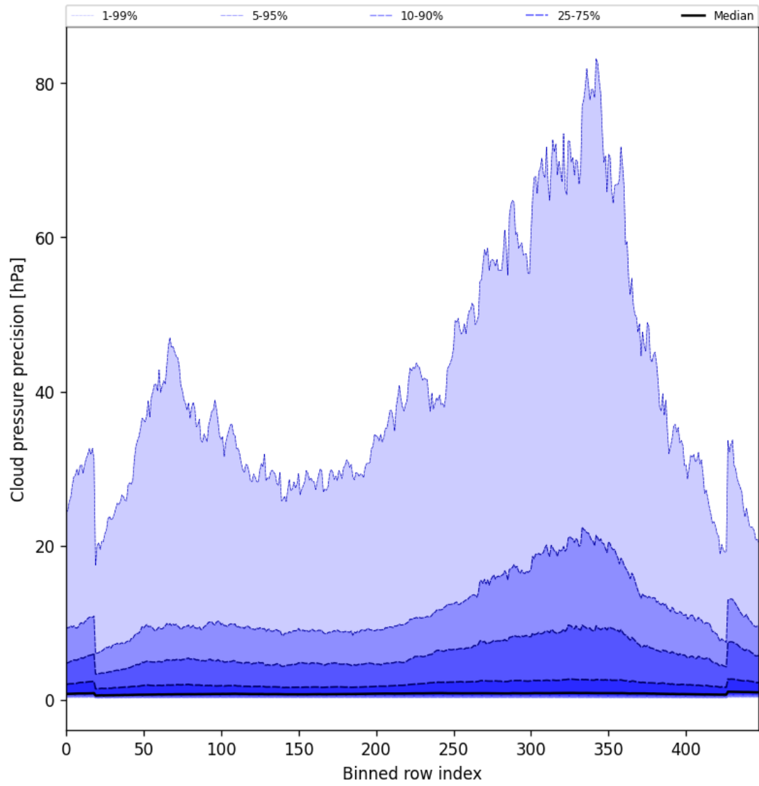
Figure 46: Along track statistics of “Cloud pressure precision” for 2025-08-18 to 2025-08-19
