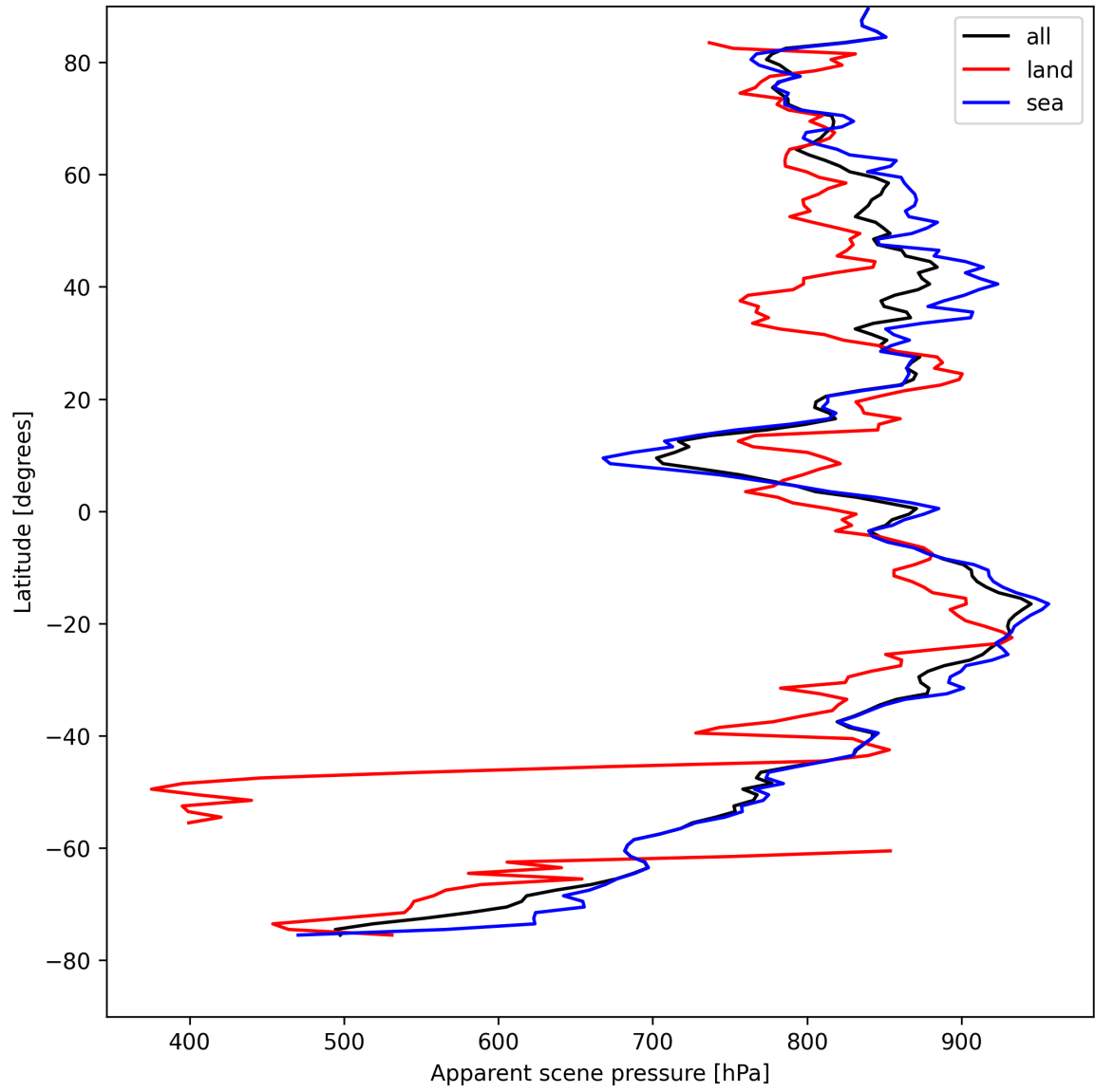
Figure 17: Zonal average of “Apparent scene pressure” for 2025-08-18 to 2025-08-19.
