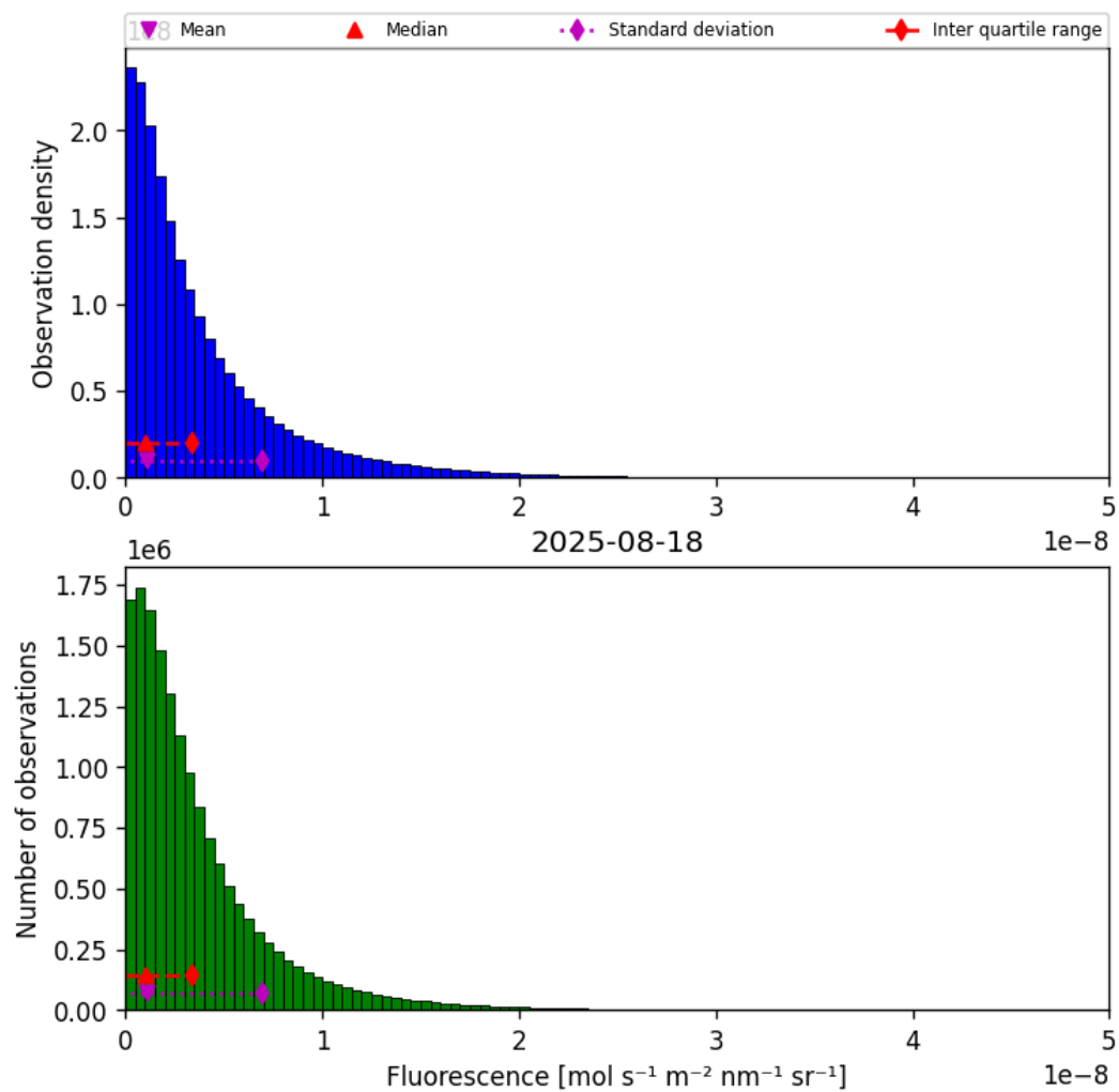
Figure 38: Histogram of “Fluorescence” for 2025-08-18 to 2025-08-19
