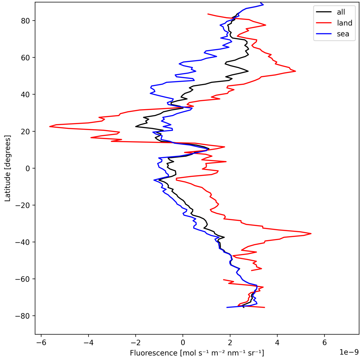
Figure 21: Zonal average of “Fluorescence” for 2025-08-18 to 2025-08-19.
