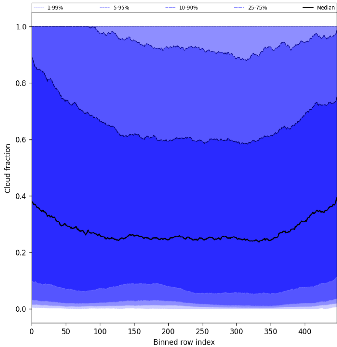
Figure 47: Along track statistics of “Cloud fraction” for 2025-08-18 to 2025-08-19
