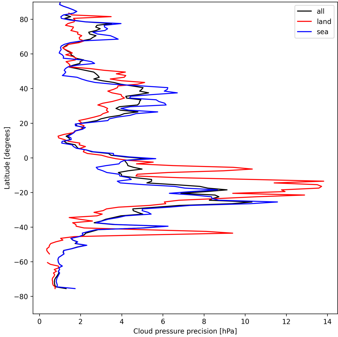
Figure 12: Zonal average of “Cloud pressure precision” for 2025-08-18 to 2025-08-19.
