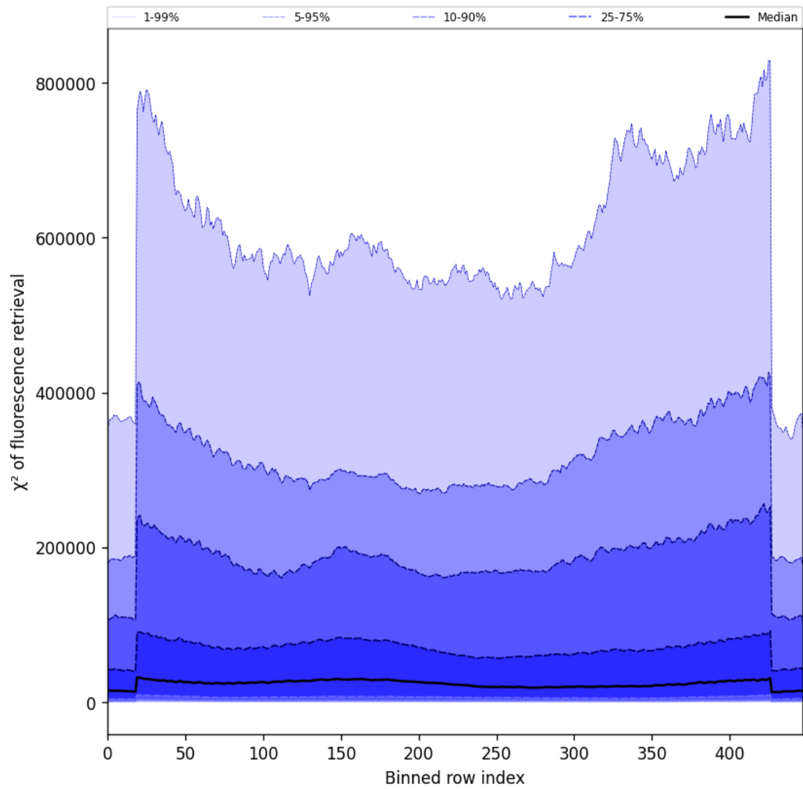
Figure 57: Along track statistics of “ \chi^2 of fluorescence retrieval” for 2025-08-18 to 2025-08-19
