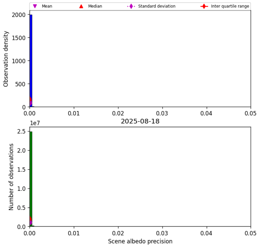
Figure 33: Histogram of “Scene albedo precision” for 2025-08-18 to 2025-08-19
