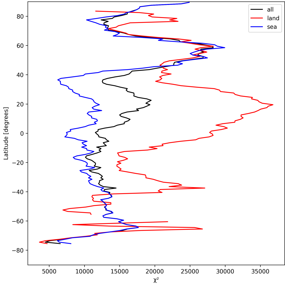
Figure 19: Zonal average of “ \chi^2 ” for 2025-08-18 to 2025-08-19.
