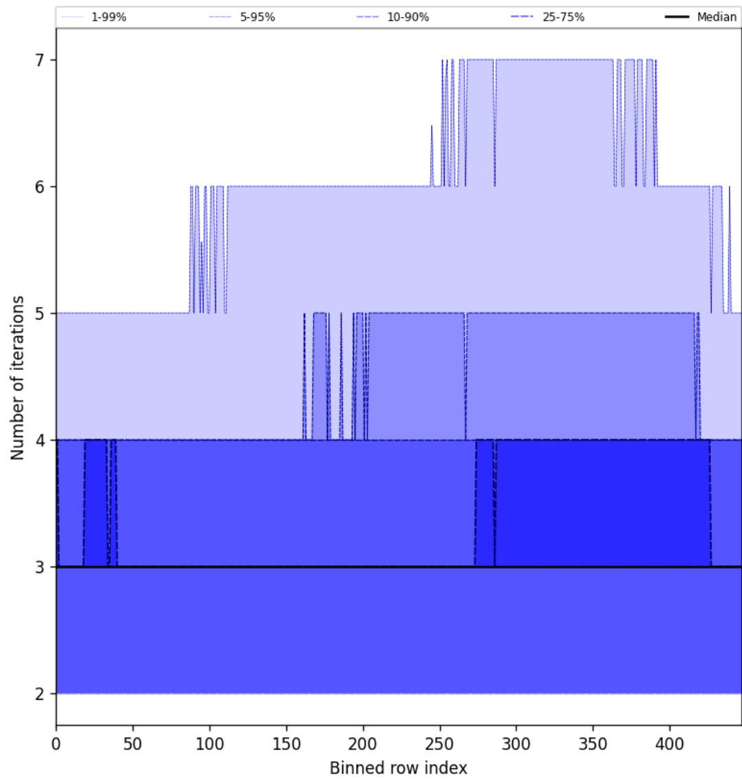
Figure 54: Along track statistics of “Number of iterations” for 2025-08-18 to 2025-08-19
