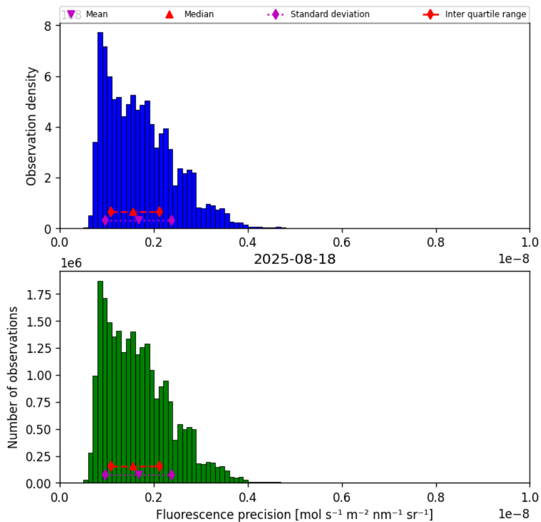
Figure 39: Histogram of “Fluorescence precision” for 2025-08-18 to 2025-08-19
