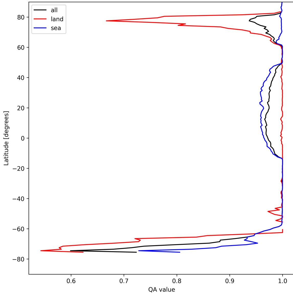
Figure 10: Zonal average of “QA value” for 2025-08-18 to 2025-08-19.
