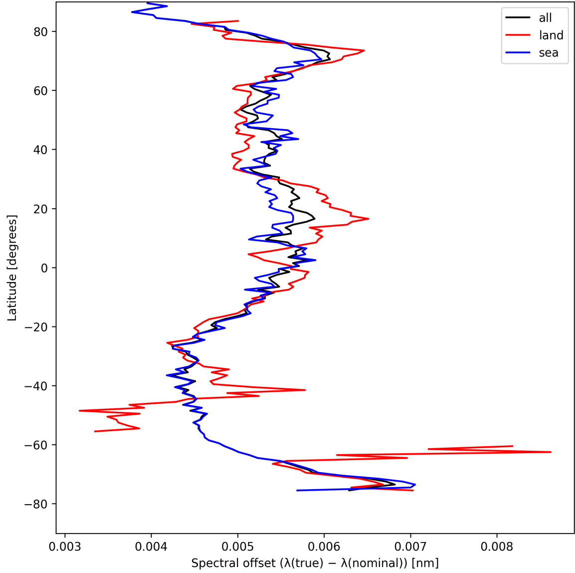
Figure 26: Zonal average of “Spectral offset ( \lambda_{\text{true}} - \lambda_{\text{nominal}} )” for 2025-08-18 to 2025-08-19.
