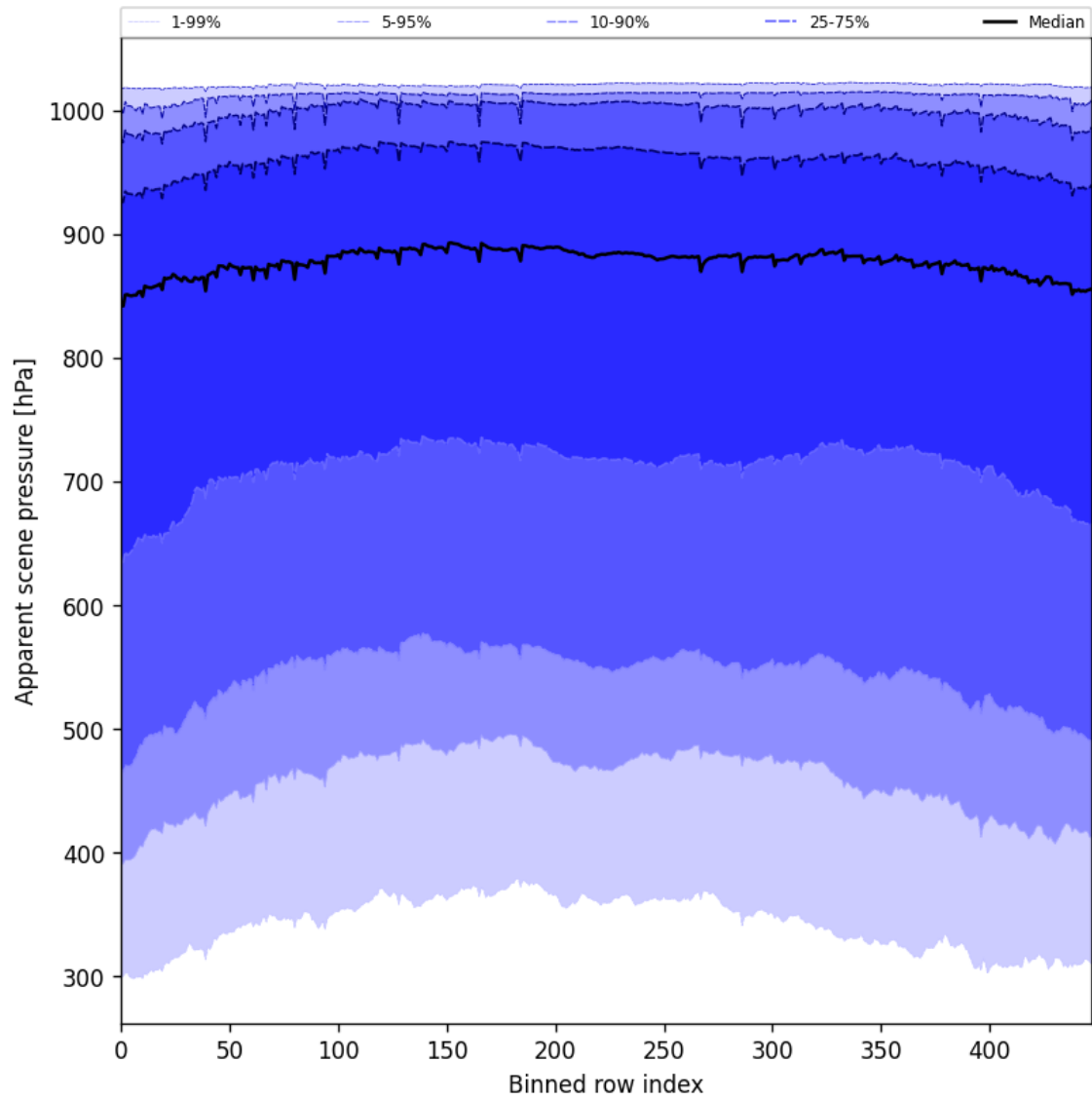
Figure 51: Along track statistics of “Apparent scene pressure” for 2025-08-18 to 2025-08-19
