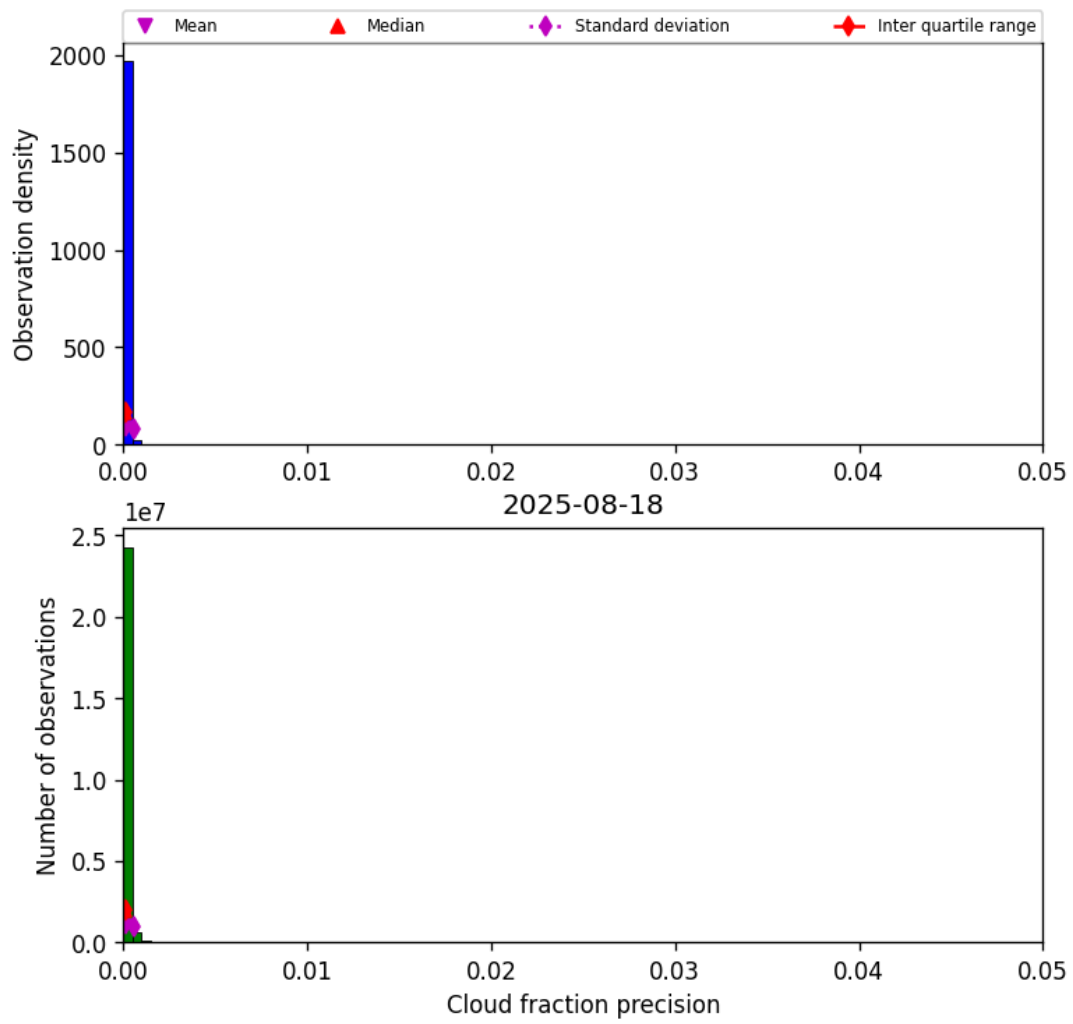
Figure 31: Histogram of “Cloud fraction precision” for 2025-08-18 to 2025-08-19
