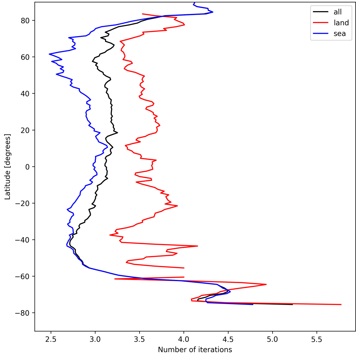
Figure 20: Zonal average of “Number of iterations” for 2025-08-18 to 2025-08-19.
