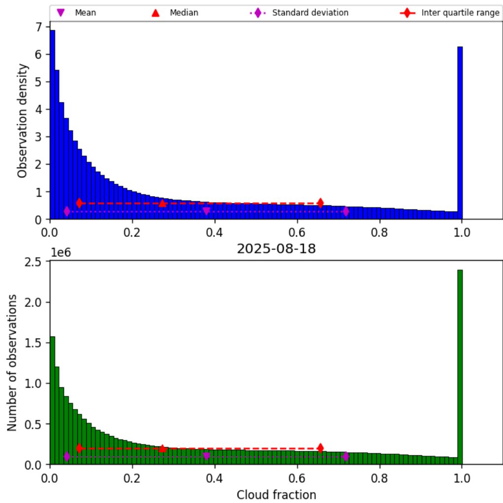
Figure 30: Histogram of “Cloud fraction” for 2025-08-18 to 2025-08-19
