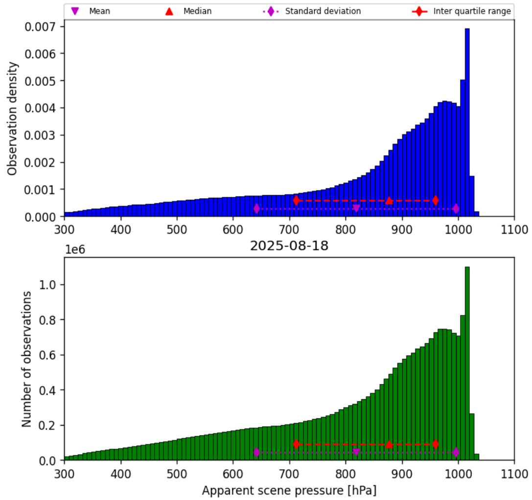
Figure 34: Histogram of “Apparent scene pressure” for 2025-08-18 to 2025-08-19
