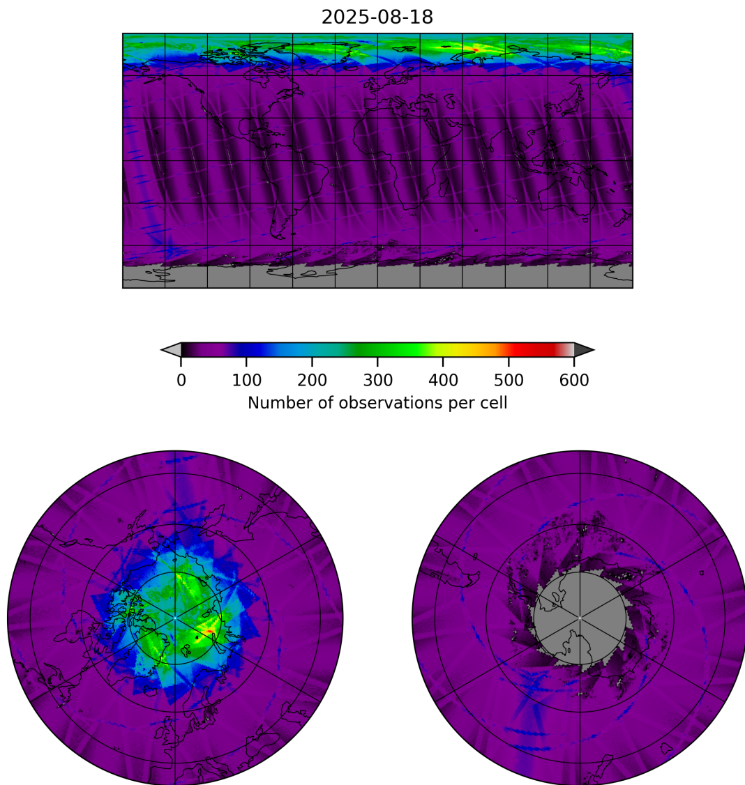
Figure 9: Map of the number of observations for 2025-08-18 to 2025-08-19
