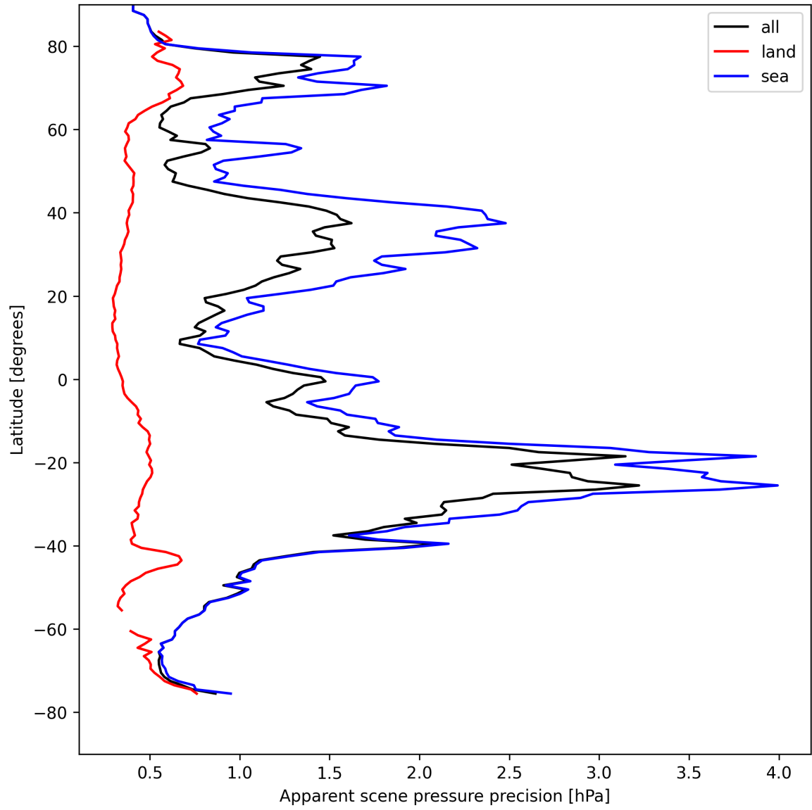
Figure 18: Zonal average of “Apparent scene pressure precision” for 2025-08-18 to 2025-08-19.
