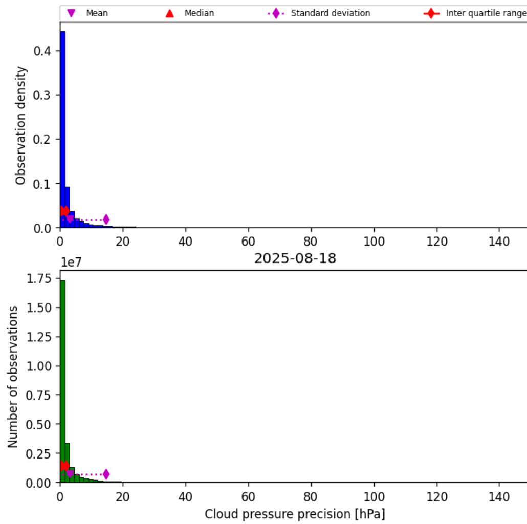
Figure 29: Histogram of “Cloud pressure precision” for 2025-08-18 to 2025-08-19
