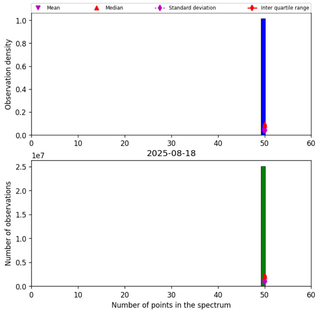
Figure 42: Histogram of “Number of points in the spectrum” for 2025-08-18 to 2025-08-19
