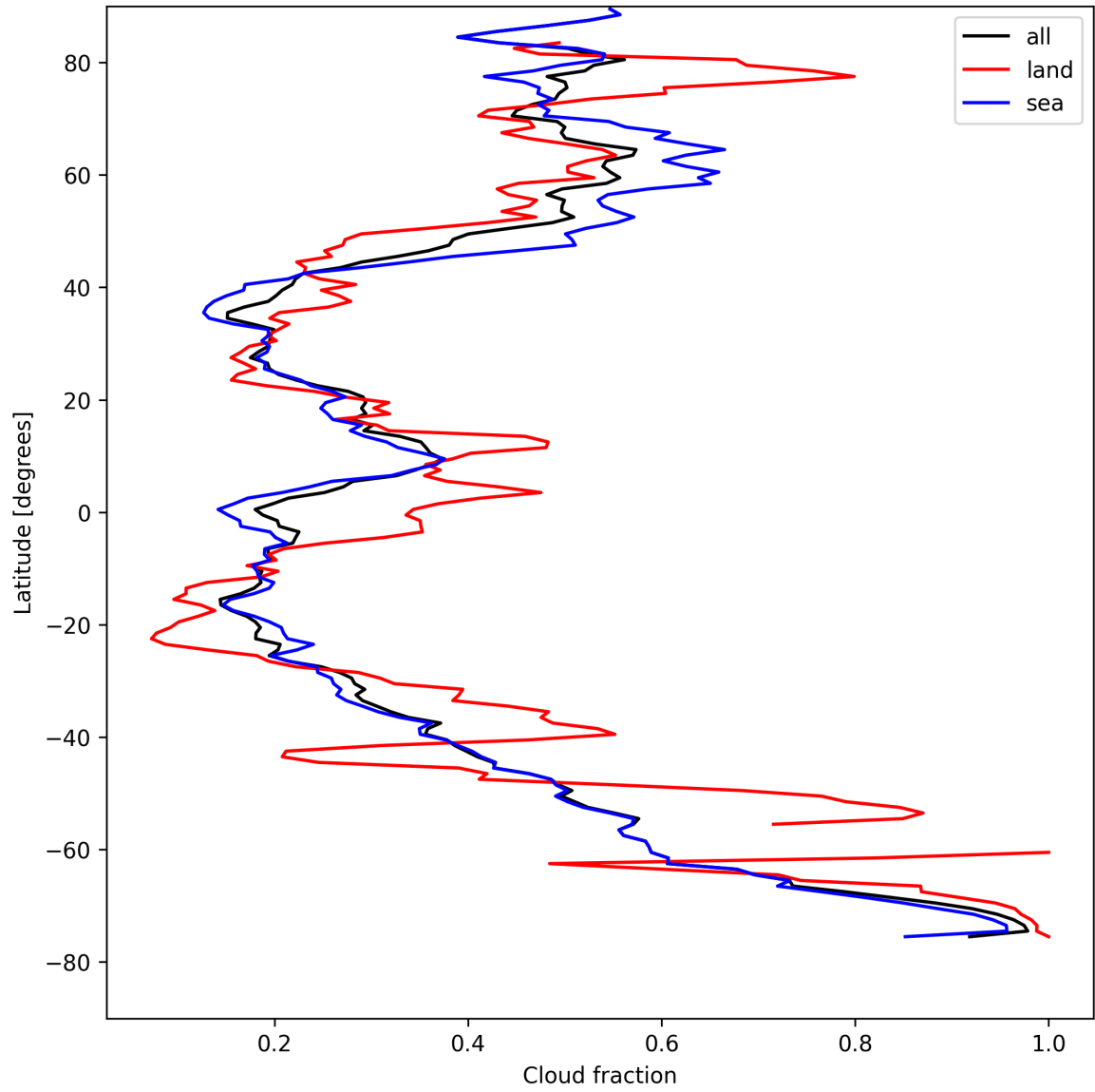
Figure 13: Zonal average of “Cloud fraction” for 2025-08-18 to 2025-08-19.
