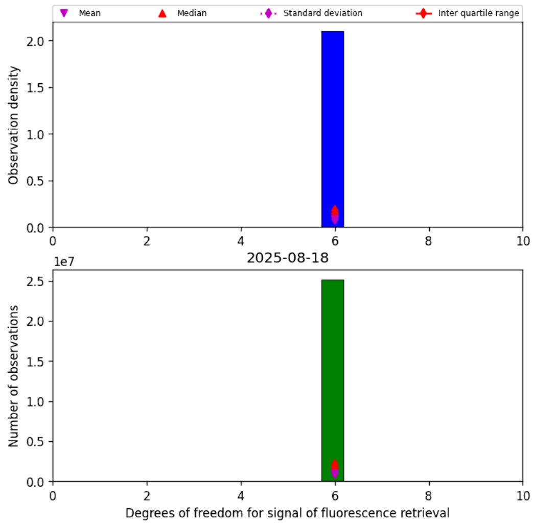
Figure 41: Histogram of “Degrees of freedom for signal of fluorescence retrieval” for 2025-08-18 to 2025-08-19
