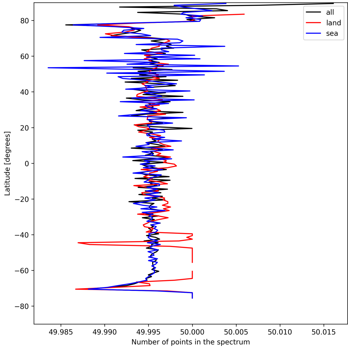
Figure 25: Zonal average of “Number of points in the spectrum” for 2025-08-18 to 2025-08-19.
