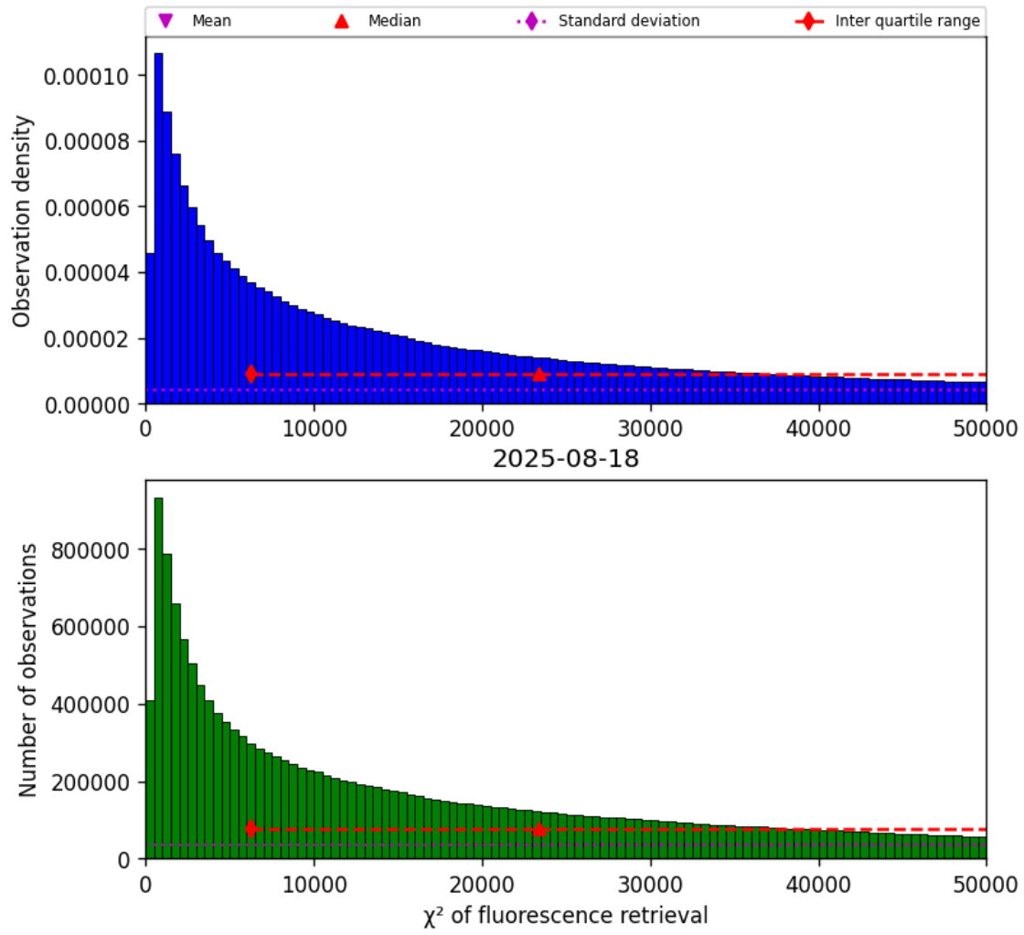
Figure 40: Histogram of “ \chi^2 of fluorescence retrieval” for 2025-08-18 to 2025-08-19
