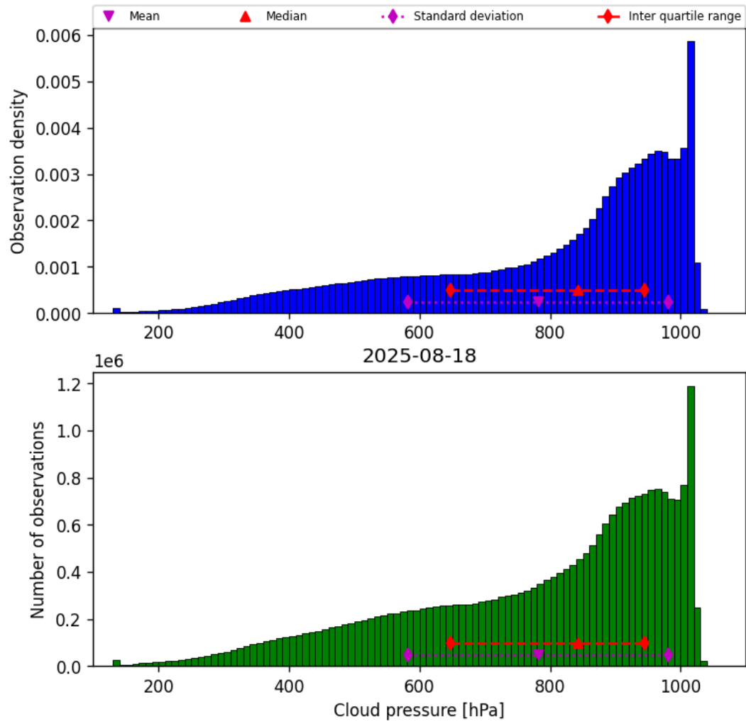
Figure 28: Histogram of “Cloud pressure” for 2025-08-18 to 2025-08-19
