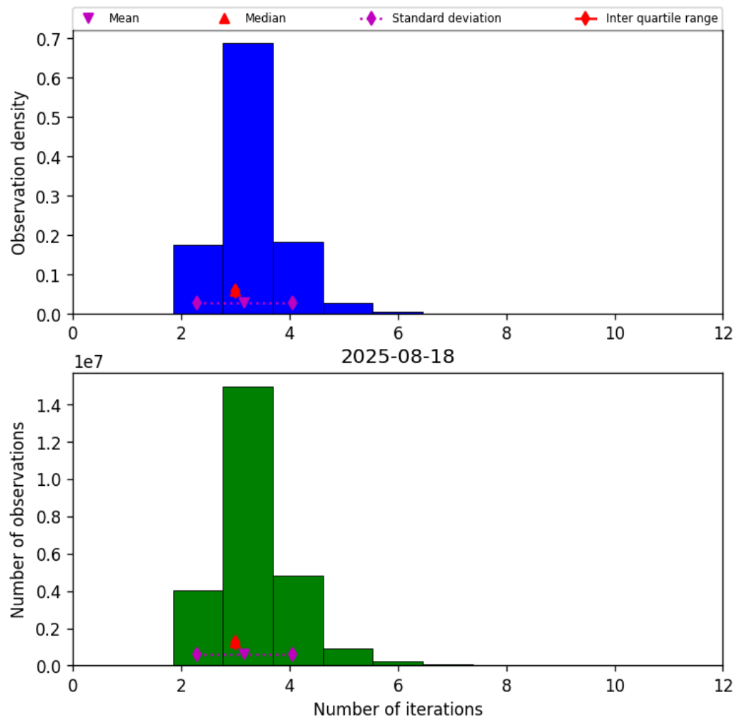
Figure 37: Histogram of “Number of iterations” for 2025-08-18 to 2025-08-19
