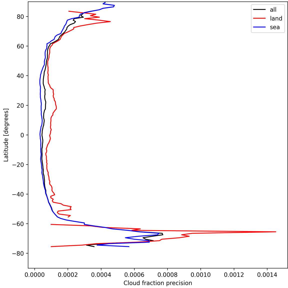
Figure 14: Zonal average of “Cloud fraction precision” for 2025-08-18 to 2025-08-19.
