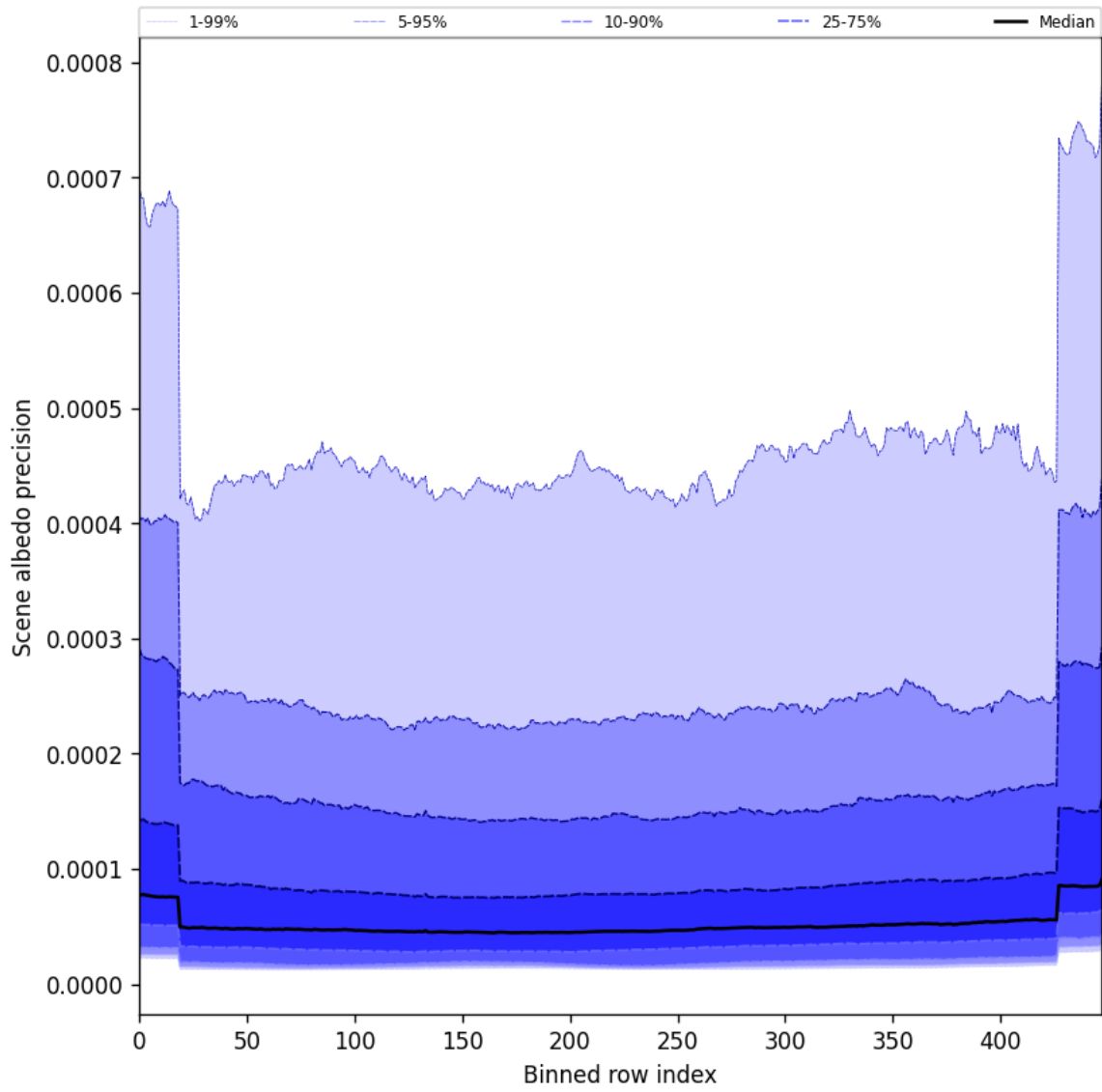
Figure 50: Along track statistics of “Scene albedo precision” for 2025-08-18 to 2025-08-19
