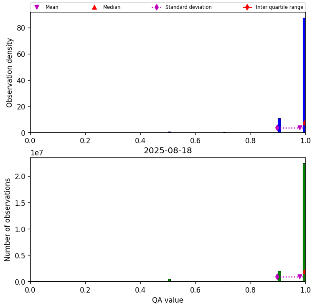
Figure 27: Histogram of “QA value” for 2025-08-18 to 2025-08-19
