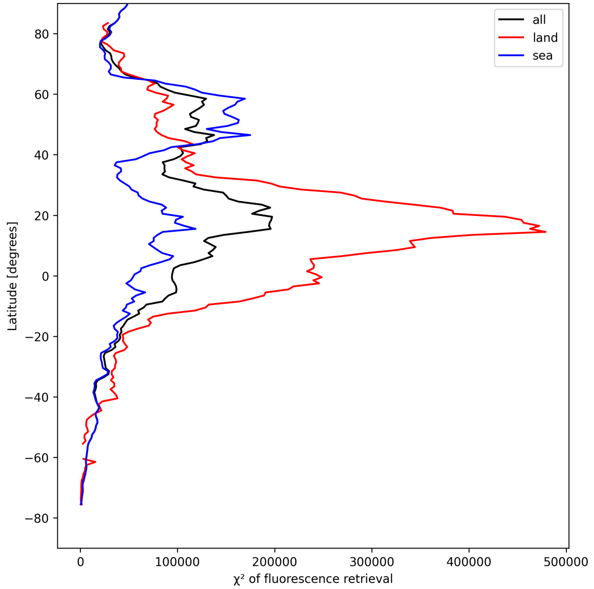
Figure 23: Zonal average of “ \chi^2 of fluorescence retrieval” for 2025-08-18 to 2025-08-19.
