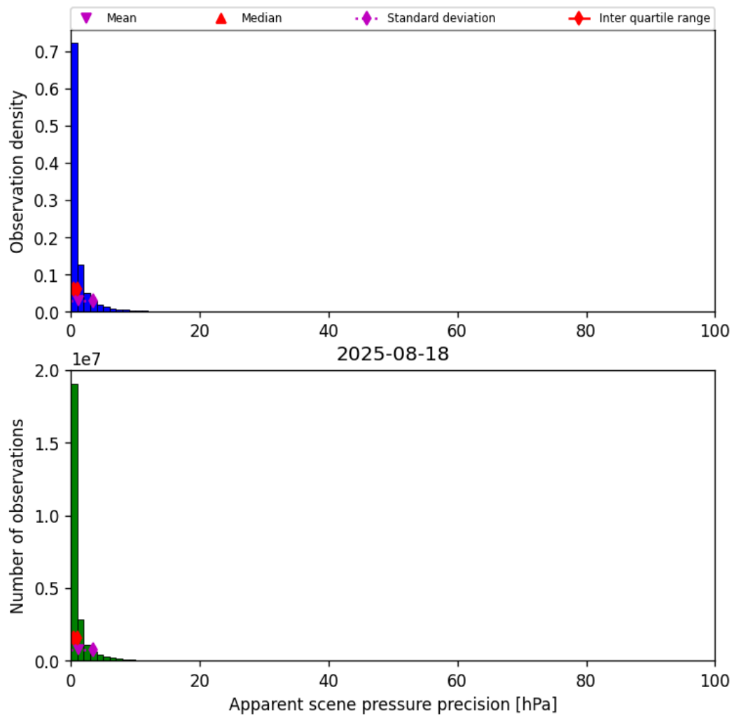
Figure 35: Histogram of “Apparent scene pressure precision” for 2025-08-18 to 2025-08-19
