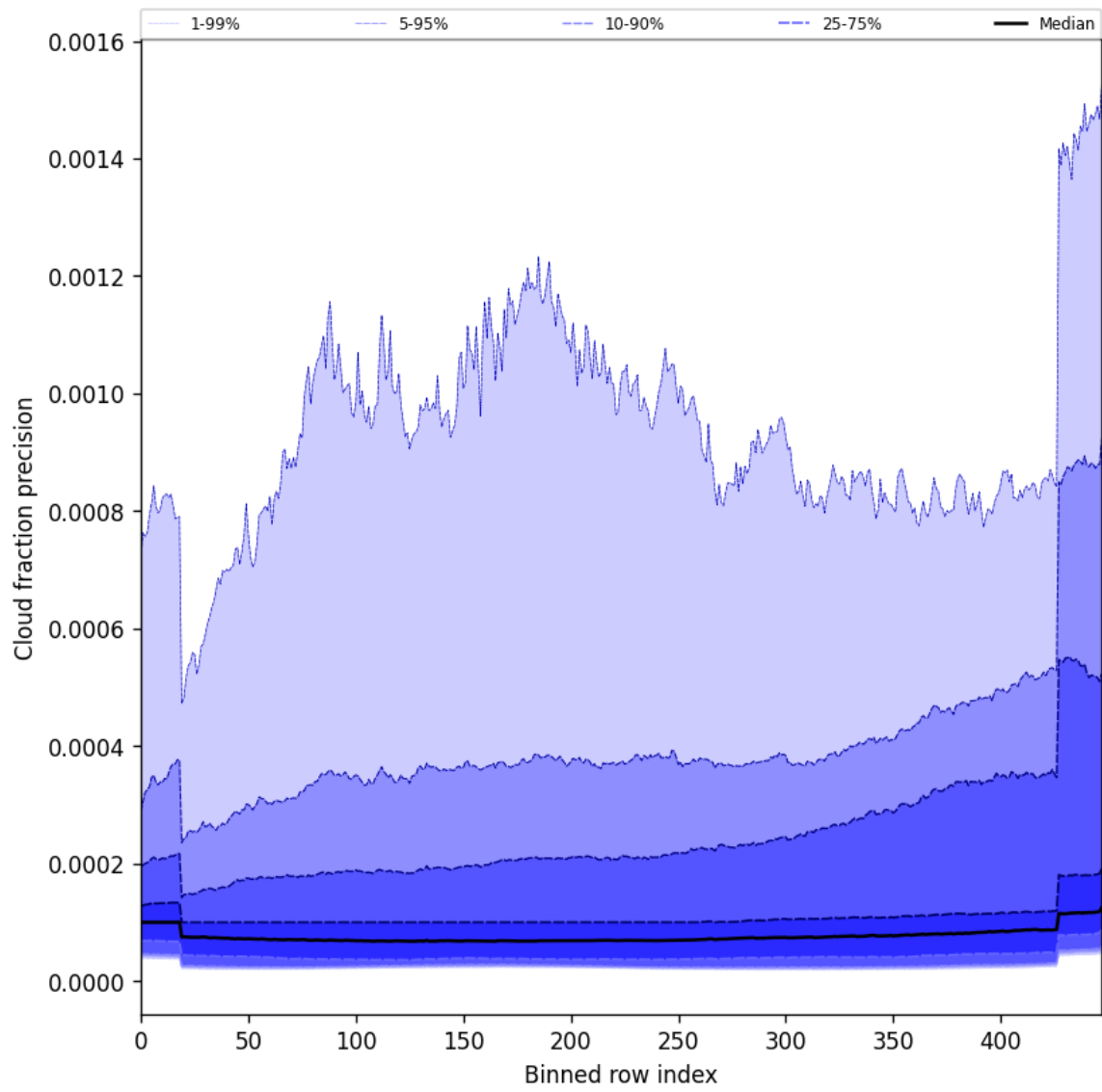
Figure 48: Along track statistics of “Cloud fraction precision” for 2025-08-18 to 2025-08-19
