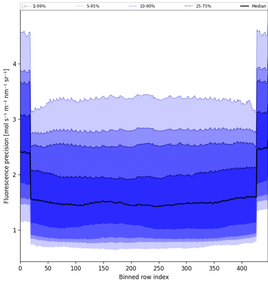
Figure 56: Along track statistics of “Fluorescence precision” for 2025-08-18 to 2025-08-19
