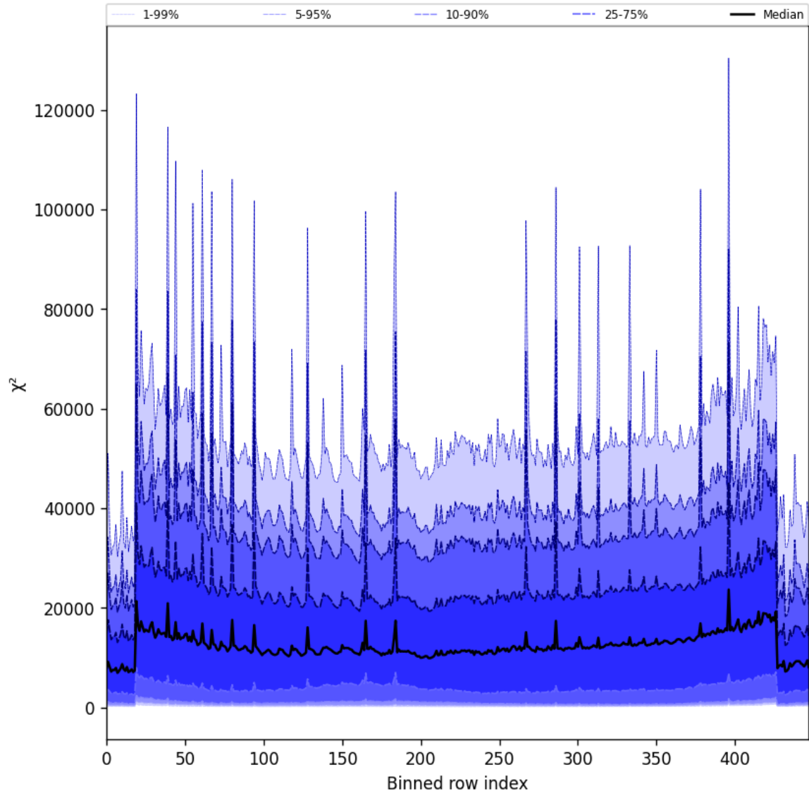
Figure 53: Along track statistics of “ \chi^2 ” for 2025-08-18 to 2025-08-19
