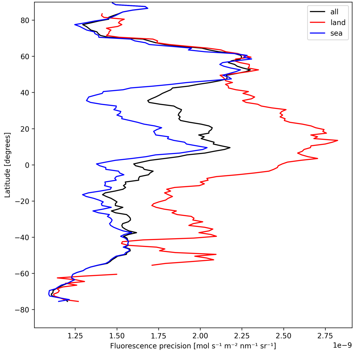
Figure 22: Zonal average of “Fluorescence precision” for 2025-08-18 to 2025-08-19.
