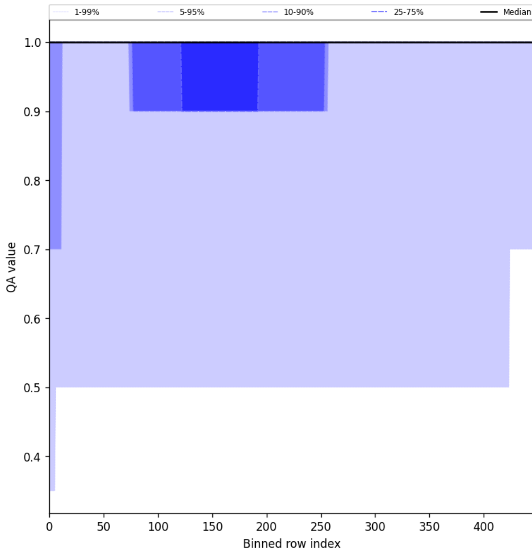
Figure 44: Along track statistics of “QA value” for 2025-08-18 to 2025-08-19
