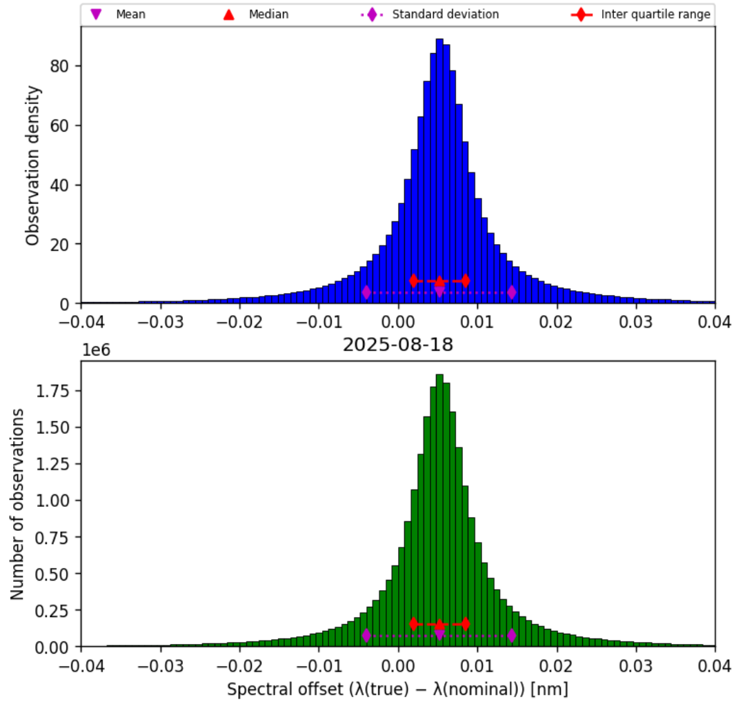
Figure 43: Histogram of “Spectral offset ( \lambda_{\text{true}} - \lambda_{\text{nominal}} )” for 2025-08-18 to 2025-08-19
