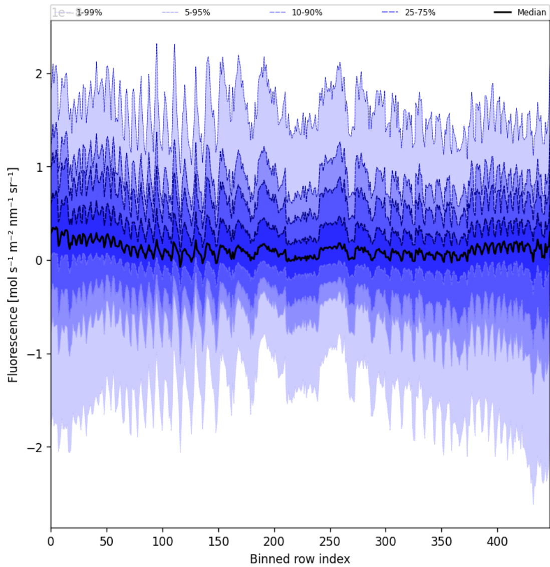
Figure 55: Along track statistics of “Fluorescence” for 2025-08-18 to 2025-08-19
