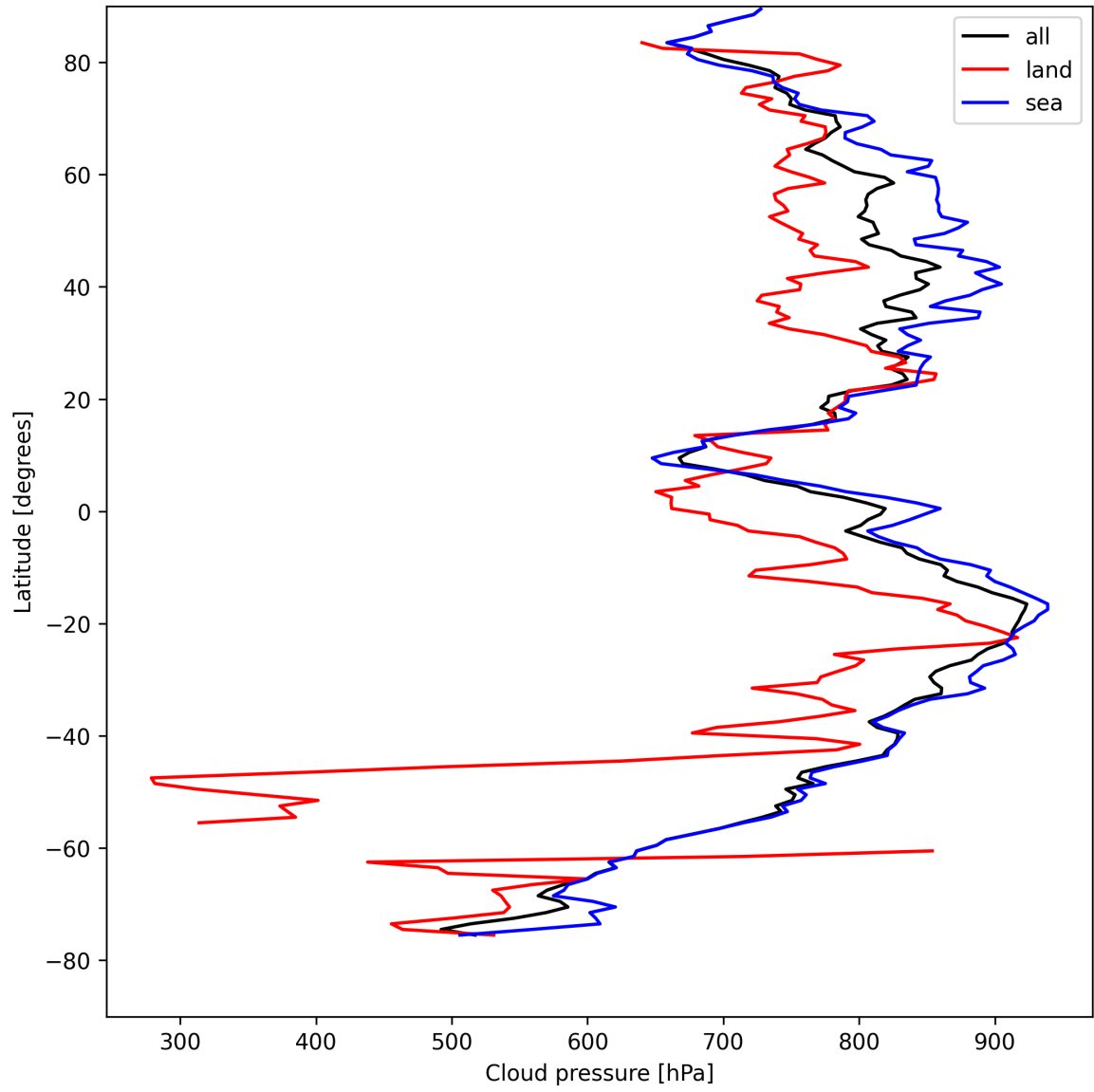
Figure 11: Zonal average of “Cloud pressure” for 2025-08-18 to 2025-08-19.
