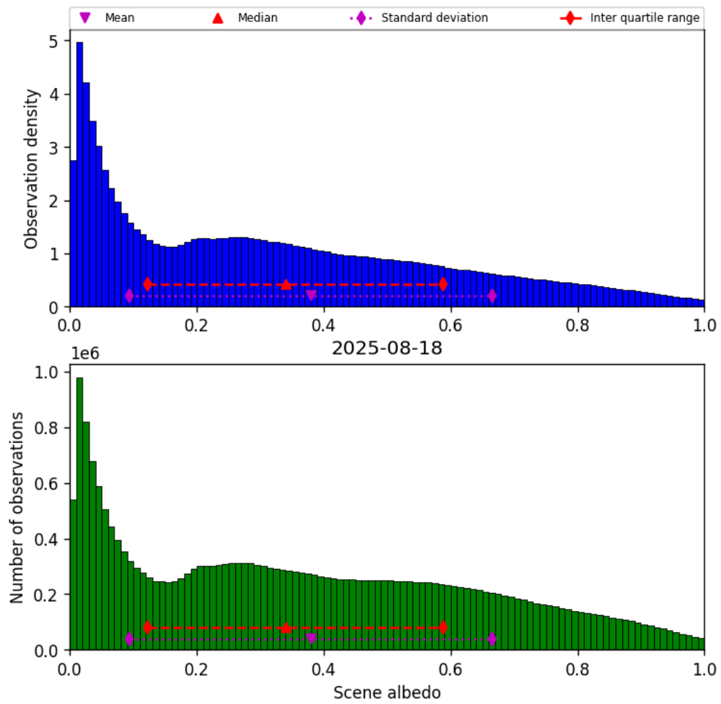
Figure 32: Histogram of “Scene albedo” for 2025-08-18 to 2025-08-19
