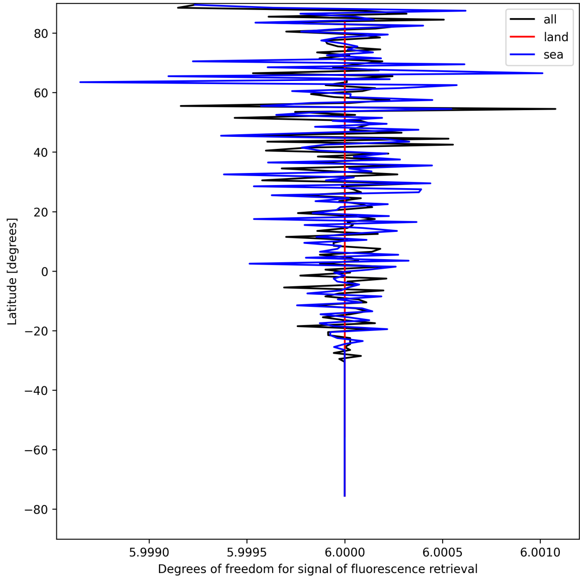
Figure 24: Zonal average of “Degrees of freedom for signal of fluorescence retrieval” for 2025-08-18 to 2025-08-19.
