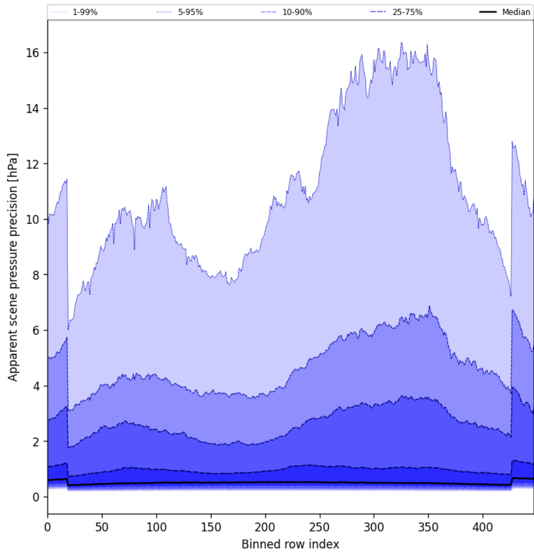
Figure 52: Along track statistics of “Apparent scene pressure precision” for 2025-08-18 to 2025-08-19
