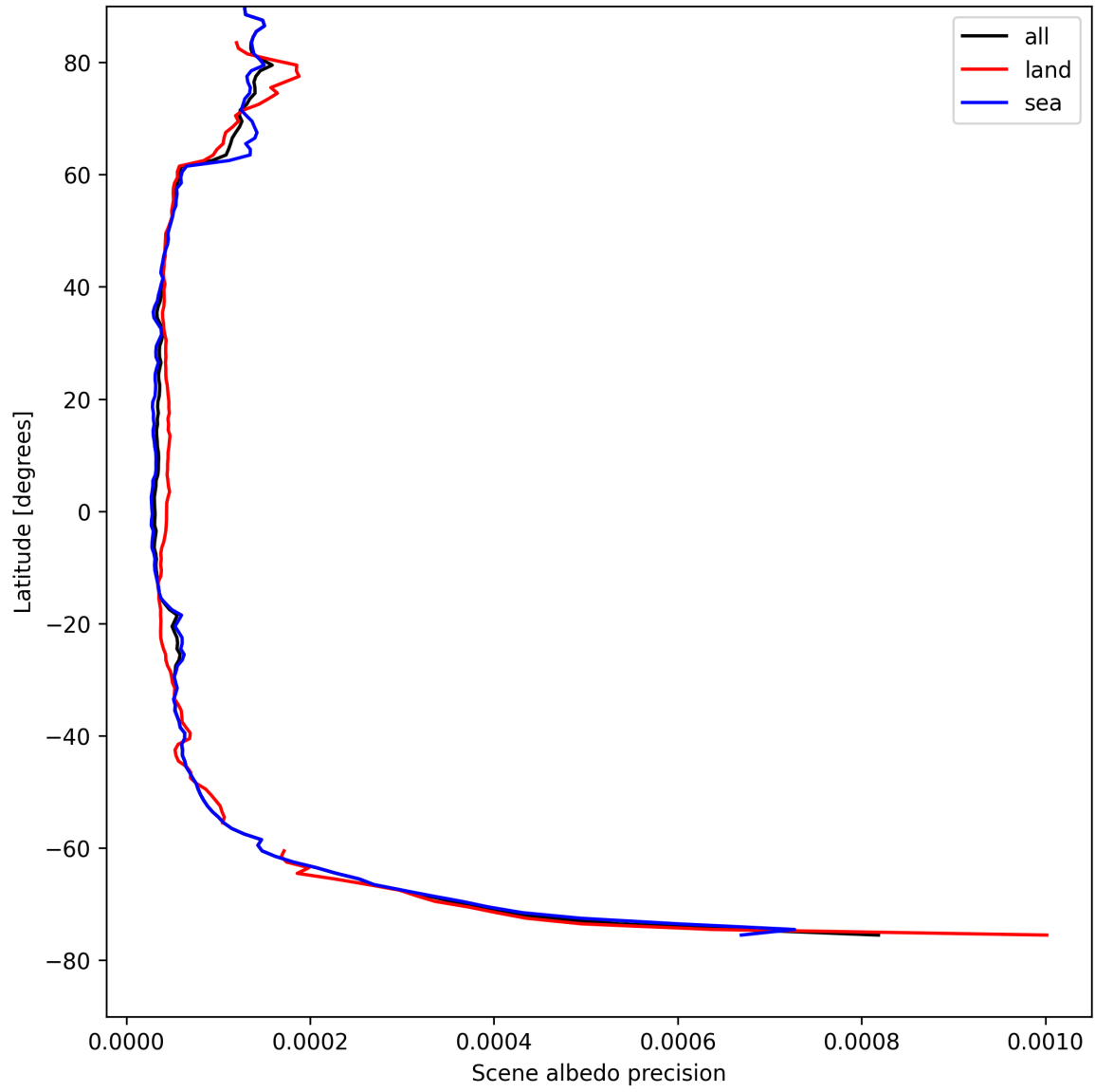
Figure 16: Zonal average of “Scene albedo precision” for 2025-08-18 to 2025-08-19.
