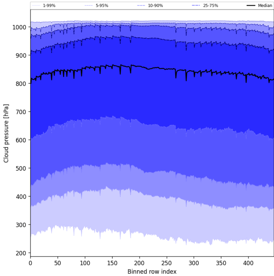
Figure 45: Along track statistics of “Cloud pressure” for 2025-08-18 to 2025-08-19
