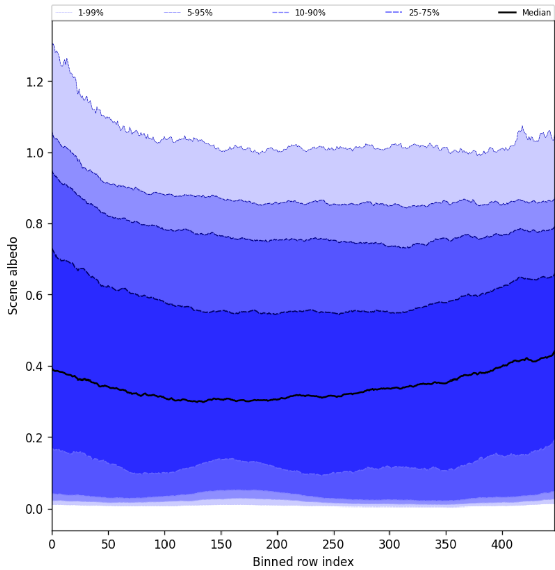
Figure 49: Along track statistics of “Scene albedo” for 2025-08-18 to 2025-08-19
