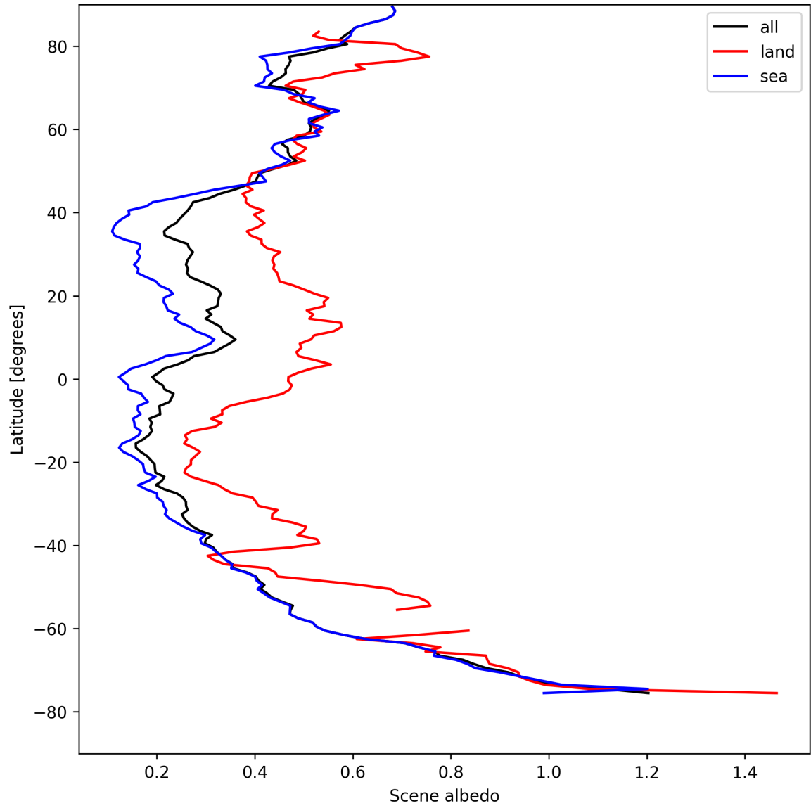
Figure 15: Zonal average of “Scene albedo” for 2025-08-18 to 2025-08-19.
