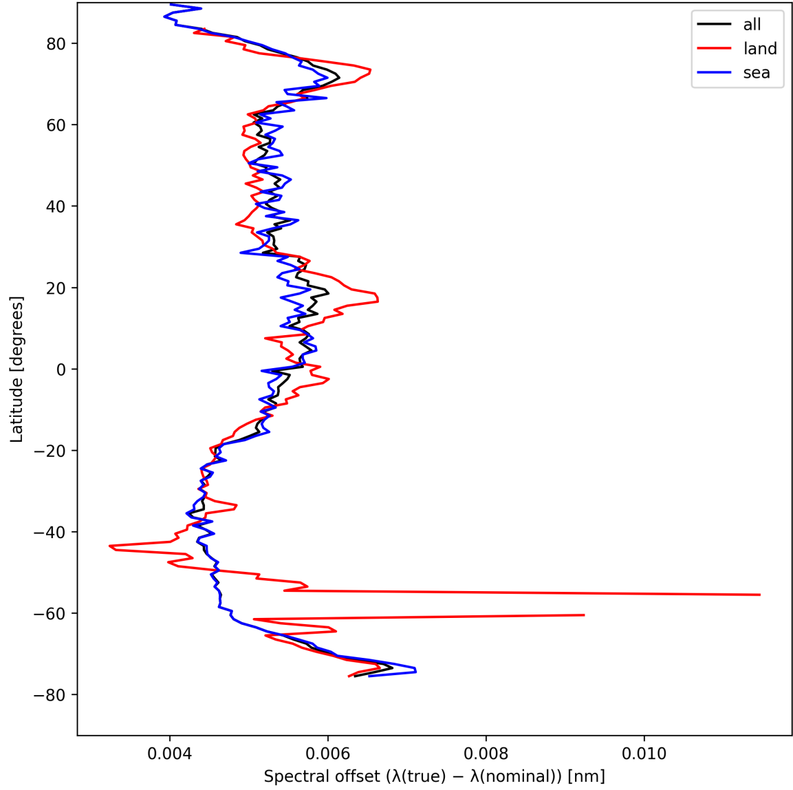
Figure 26: Zonal average of “Spectral offset ( \lambda_{\text{true}} - \lambda_{\text{nominal}} )” for 2025-08-19 to 2025-08-20.
