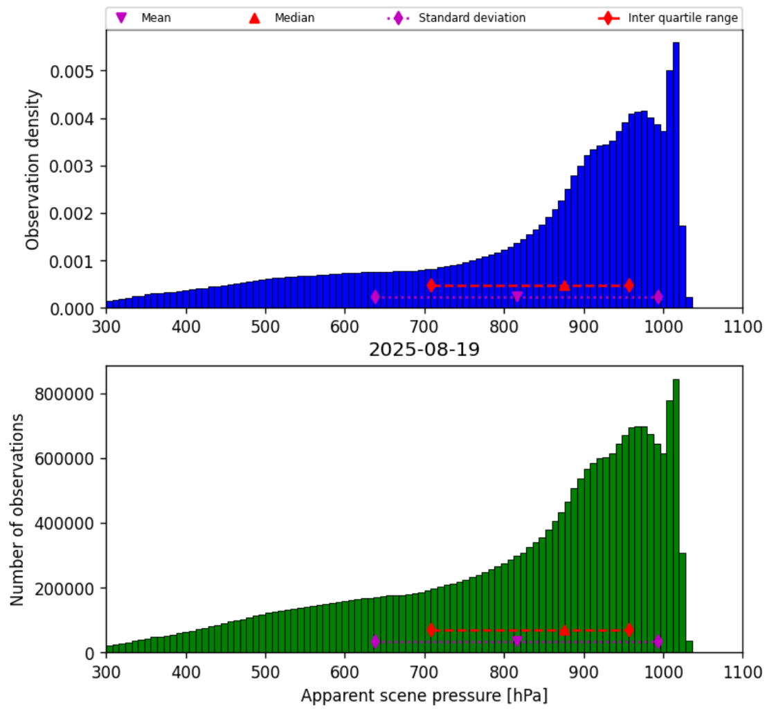
Figure 34: Histogram of “Apparent scene pressure” for 2025-08-19 to 2025-08-20
