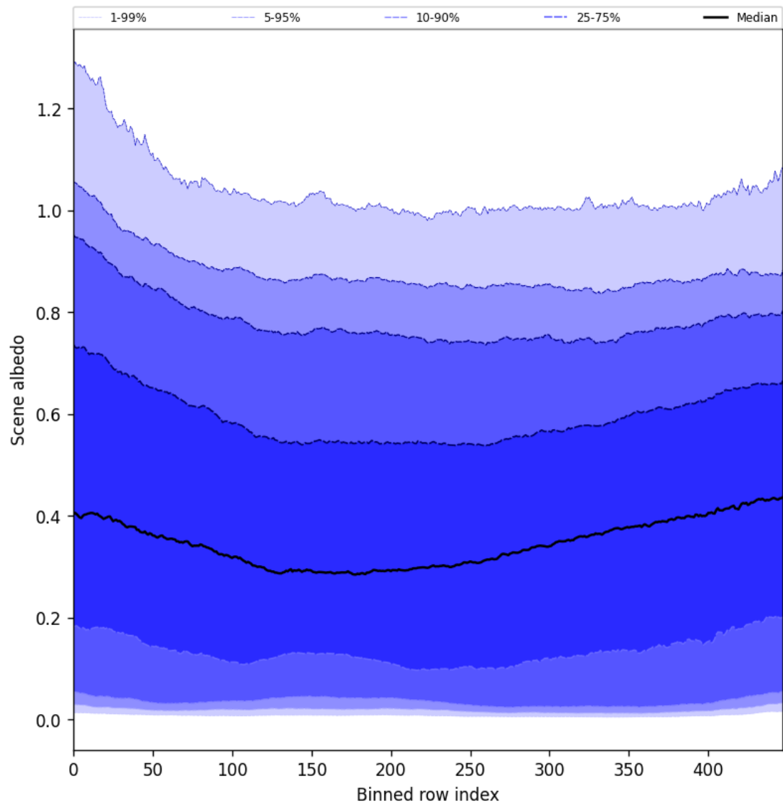
Figure 49: Along track statistics of “Scene albedo” for 2025-08-19 to 2025-08-20
