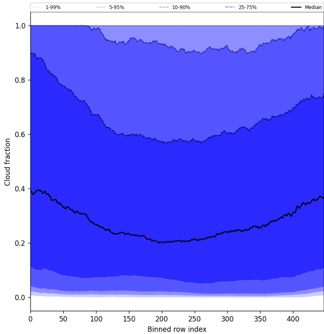
Figure 47: Along track statistics of “Cloud fraction” for 2025-08-19 to 2025-08-20
