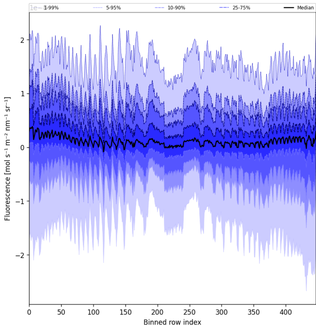
Figure 55: Along track statistics of “Fluorescence” for 2025-08-19 to 2025-08-20
