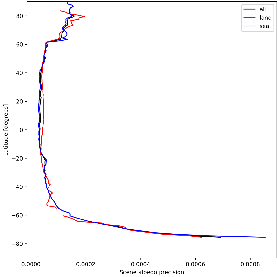
Figure 16: Zonal average of “Scene albedo precision” for 2025-08-19 to 2025-08-20.
