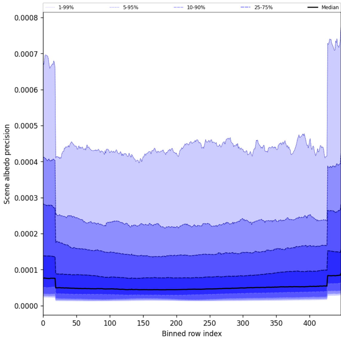
Figure 50: Along track statistics of “Scene albedo precision” for 2025-08-19 to 2025-08-20
