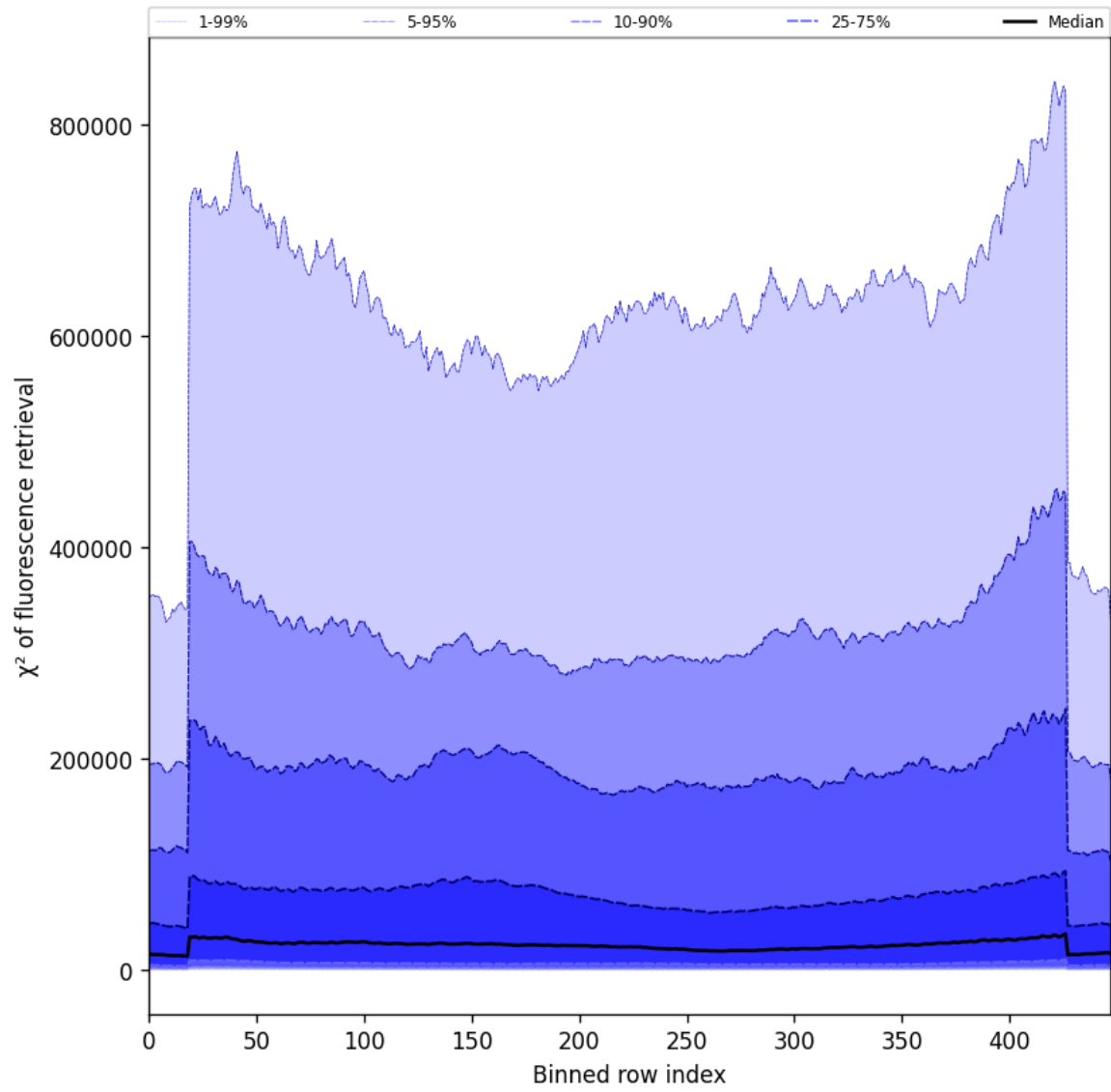
Figure 57: Along track statistics of “ \chi^2 of fluorescence retrieval” for 2025-08-19 to 2025-08-20
