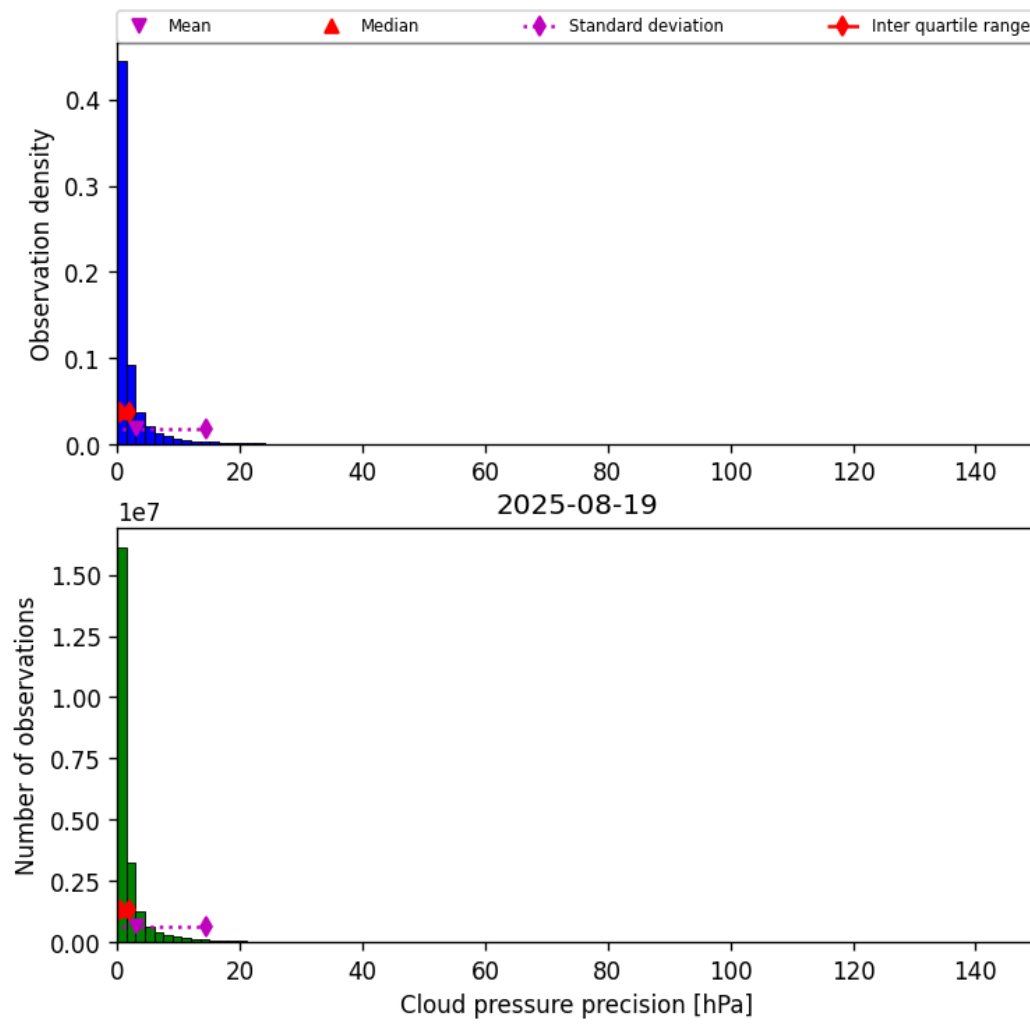
Figure 29: Histogram of “Cloud pressure precision” for 2025-08-19 to 2025-08-20
