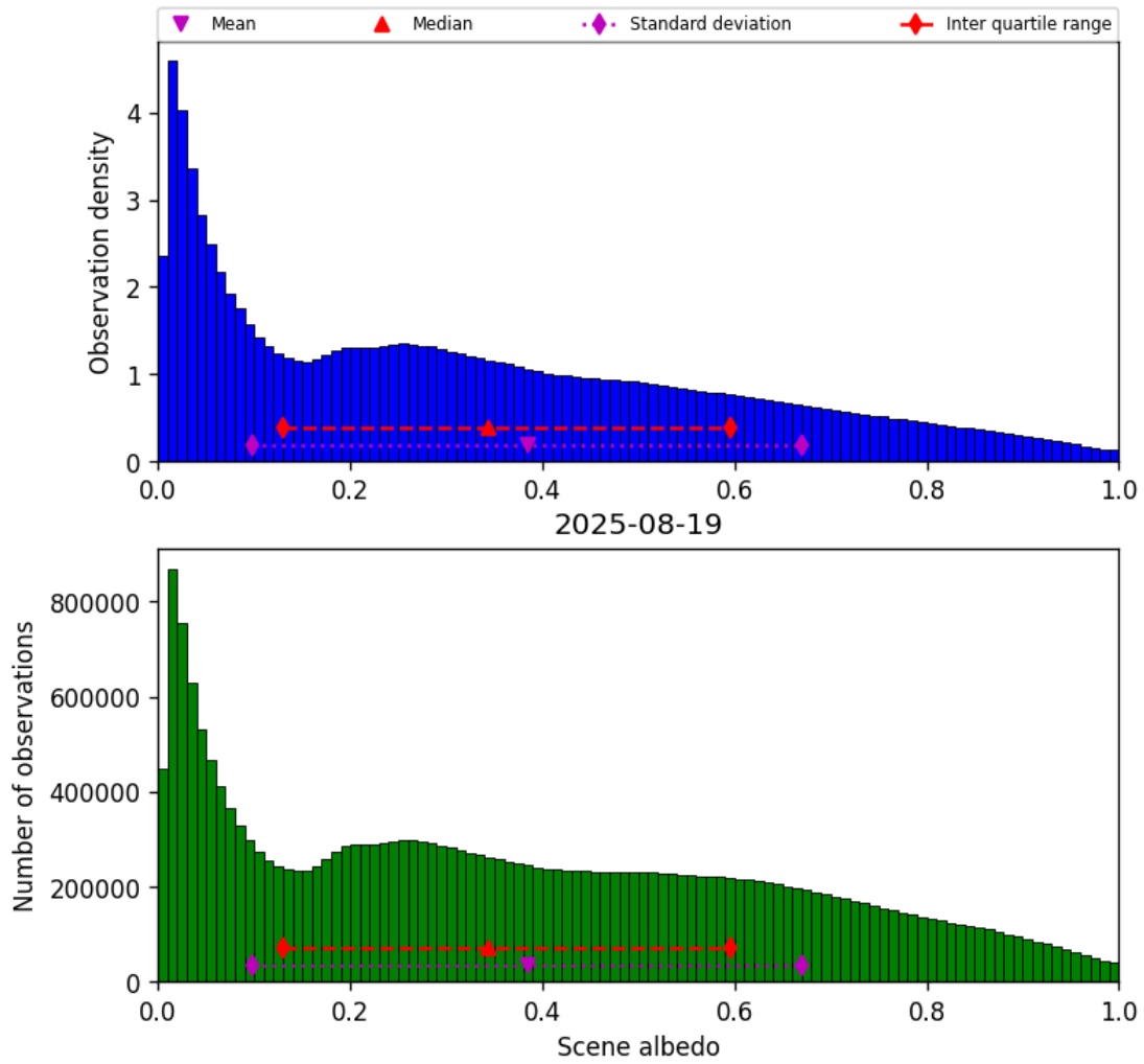
Figure 32: Histogram of “Scene albedo” for 2025-08-19 to 2025-08-20
