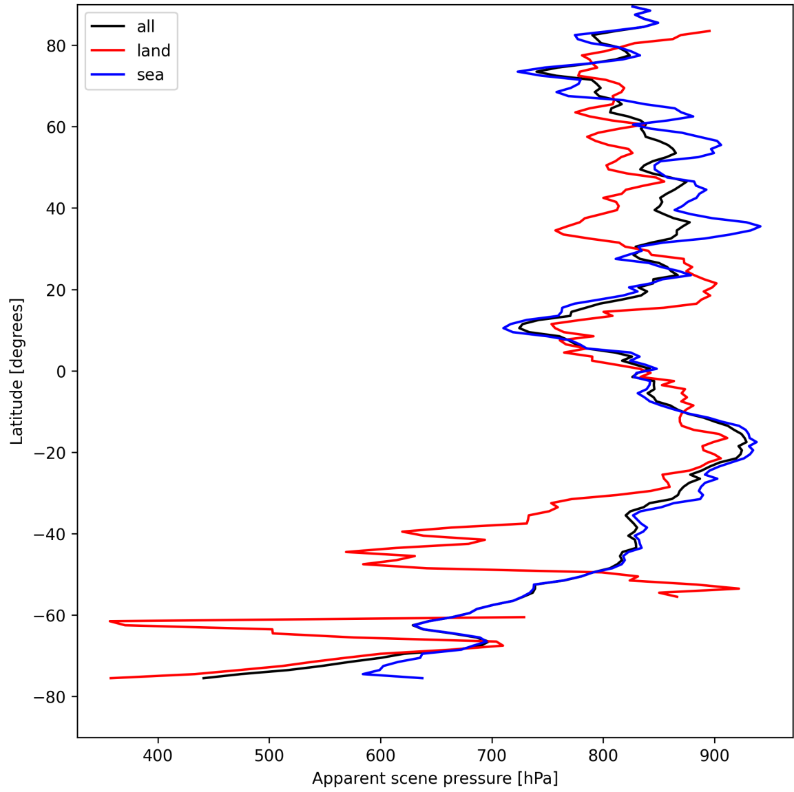
Figure 17: Zonal average of “Apparent scene pressure” for 2025-08-19 to 2025-08-20.
