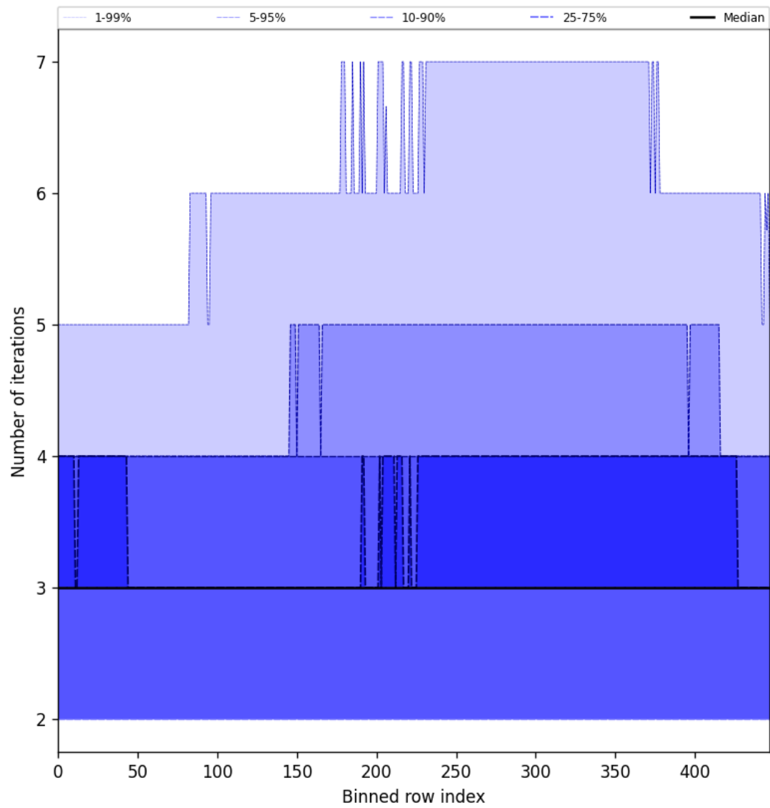
Figure 54: Along track statistics of “Number of iterations” for 2025-08-19 to 2025-08-20
