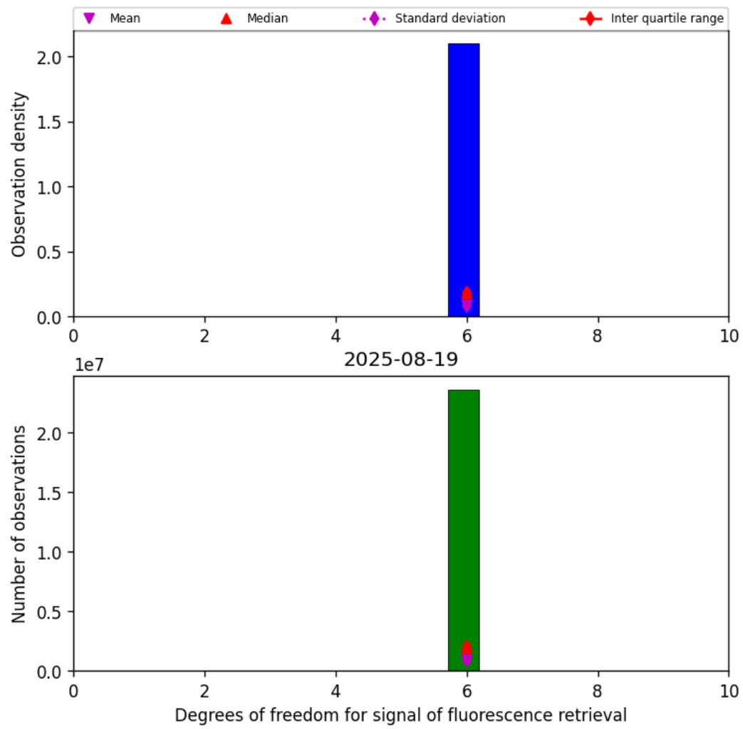
Figure 41: Histogram of “Degrees of freedom for signal of fluorescence retrieval” for 2025-08-19 to 2025-08-20
