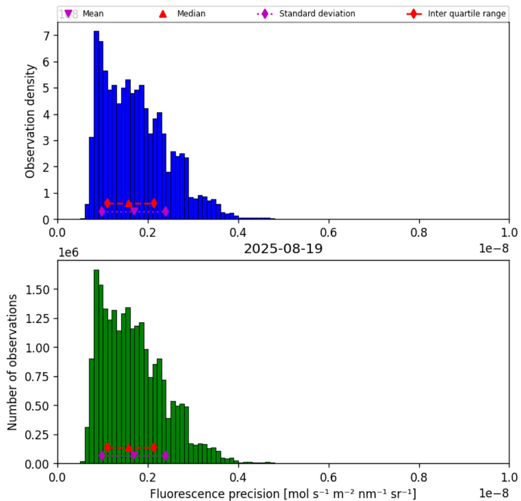
Figure 39: Histogram of “Fluorescence precision” for 2025-08-19 to 2025-08-20
