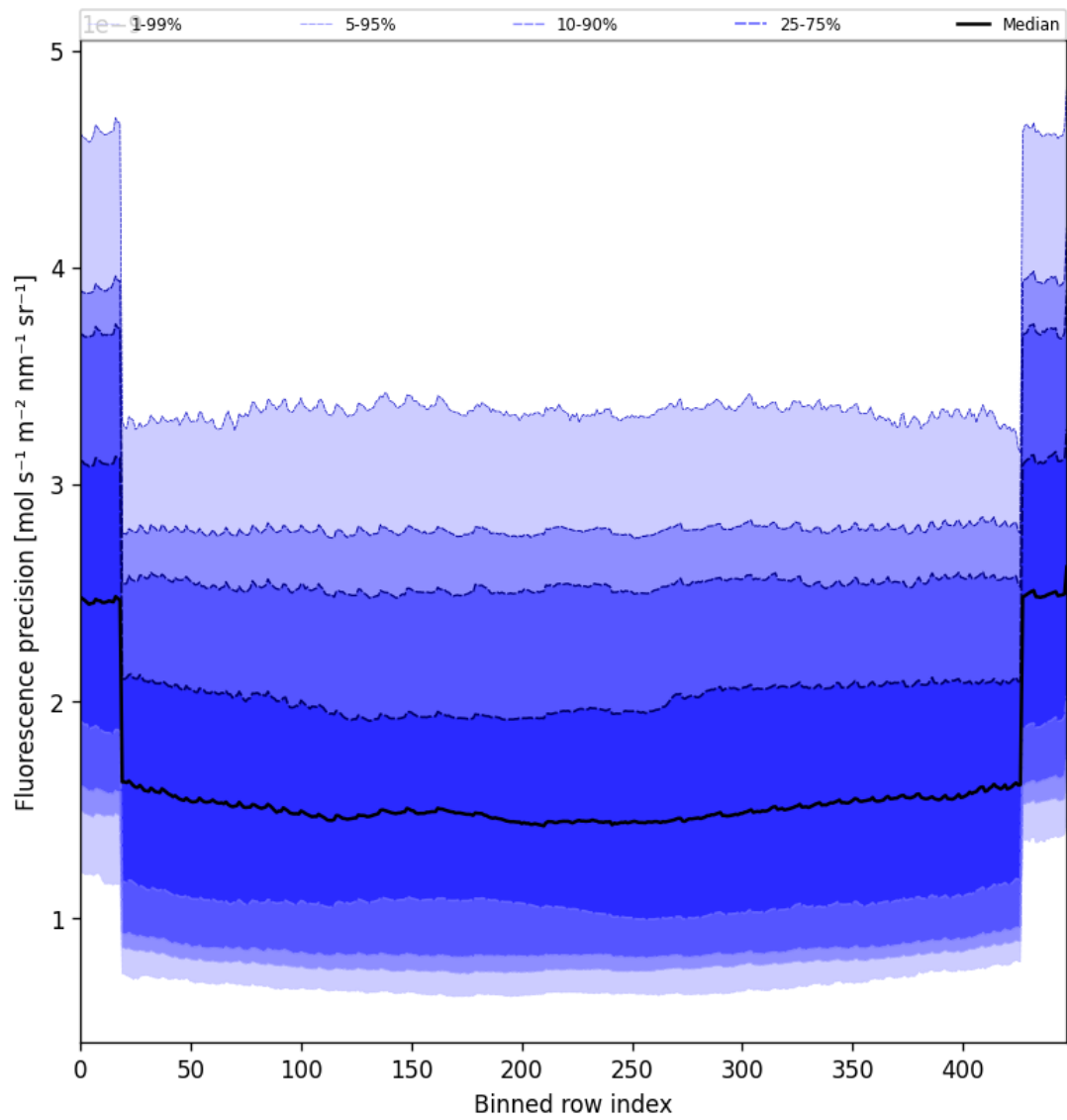
Figure 56: Along track statistics of “Fluorescence precision” for 2025-08-19 to 2025-08-20
