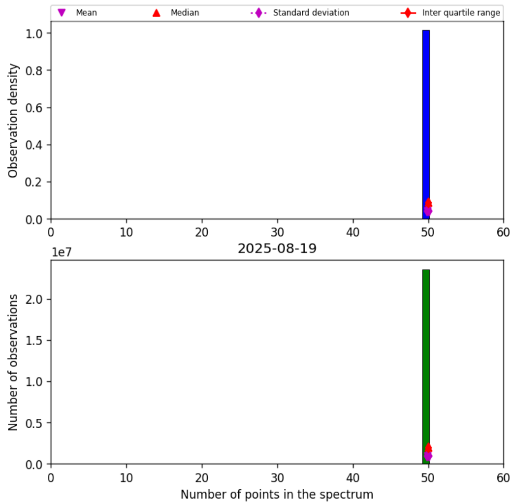
Figure 42: Histogram of “Number of points in the spectrum” for 2025-08-19 to 2025-08-20
