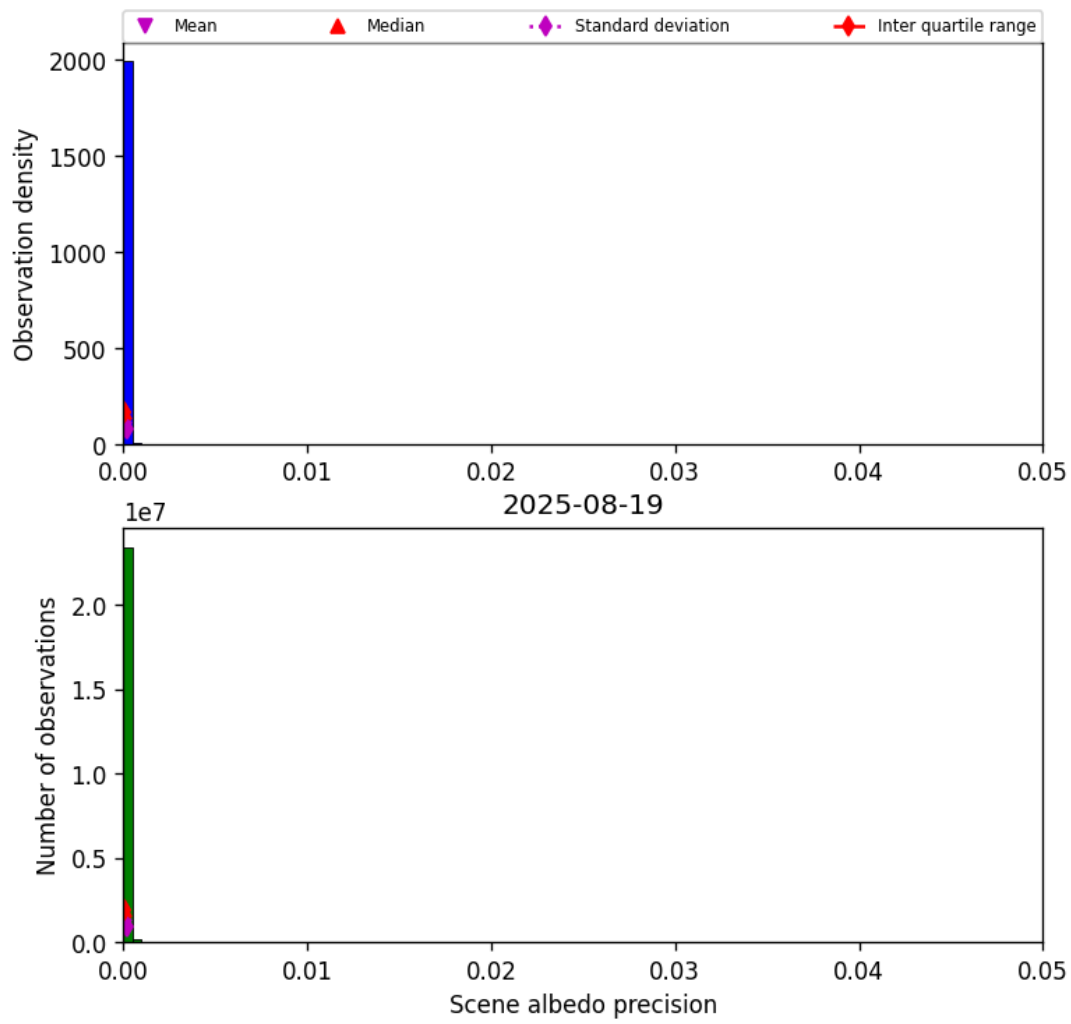
Figure 33: Histogram of “Scene albedo precision” for 2025-08-19 to 2025-08-20
