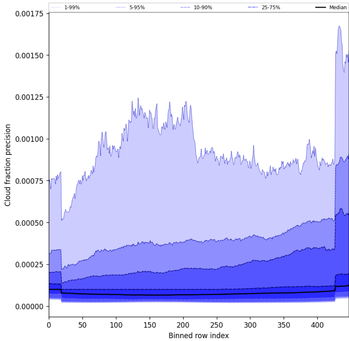
Figure 48: Along track statistics of “Cloud fraction precision” for 2025-08-19 to 2025-08-20
