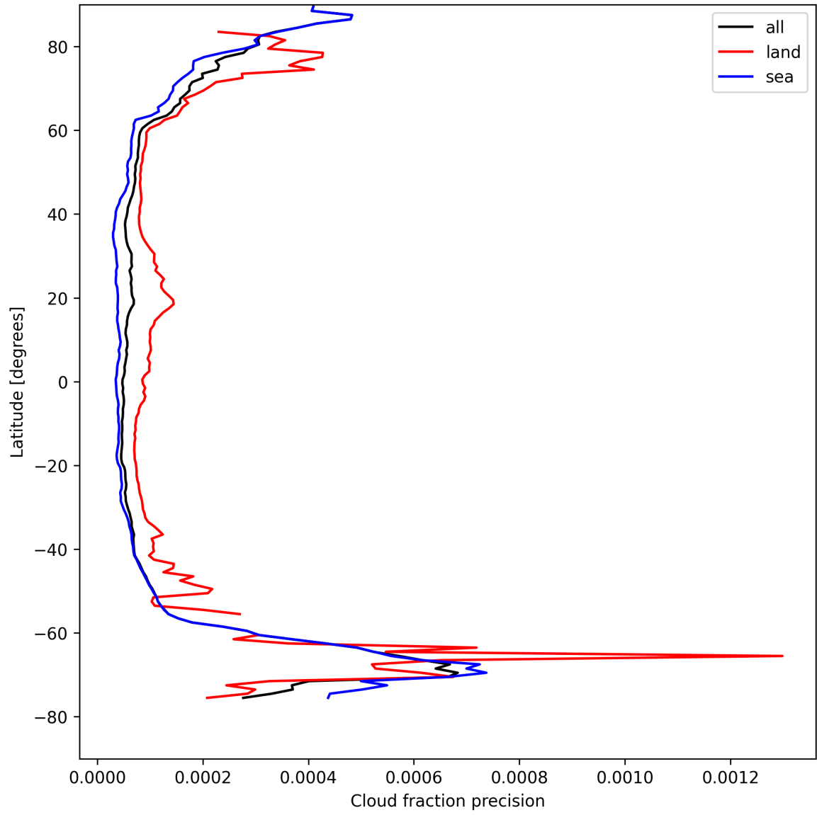
Figure 14: Zonal average of “Cloud fraction precision” for 2025-08-19 to 2025-08-20.
