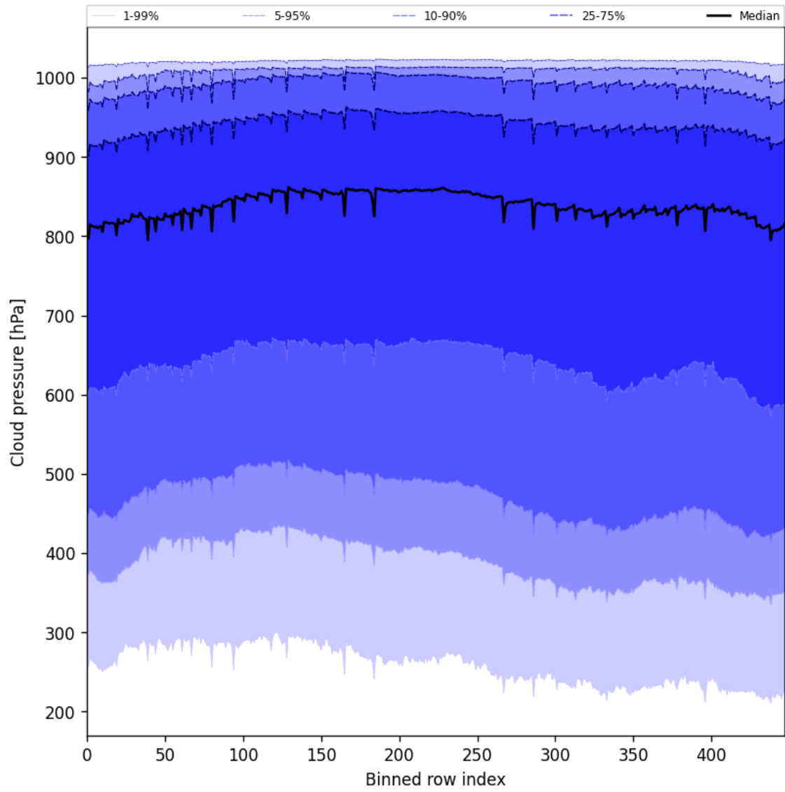
Figure 45: Along track statistics of “Cloud pressure” for 2025-08-19 to 2025-08-20
