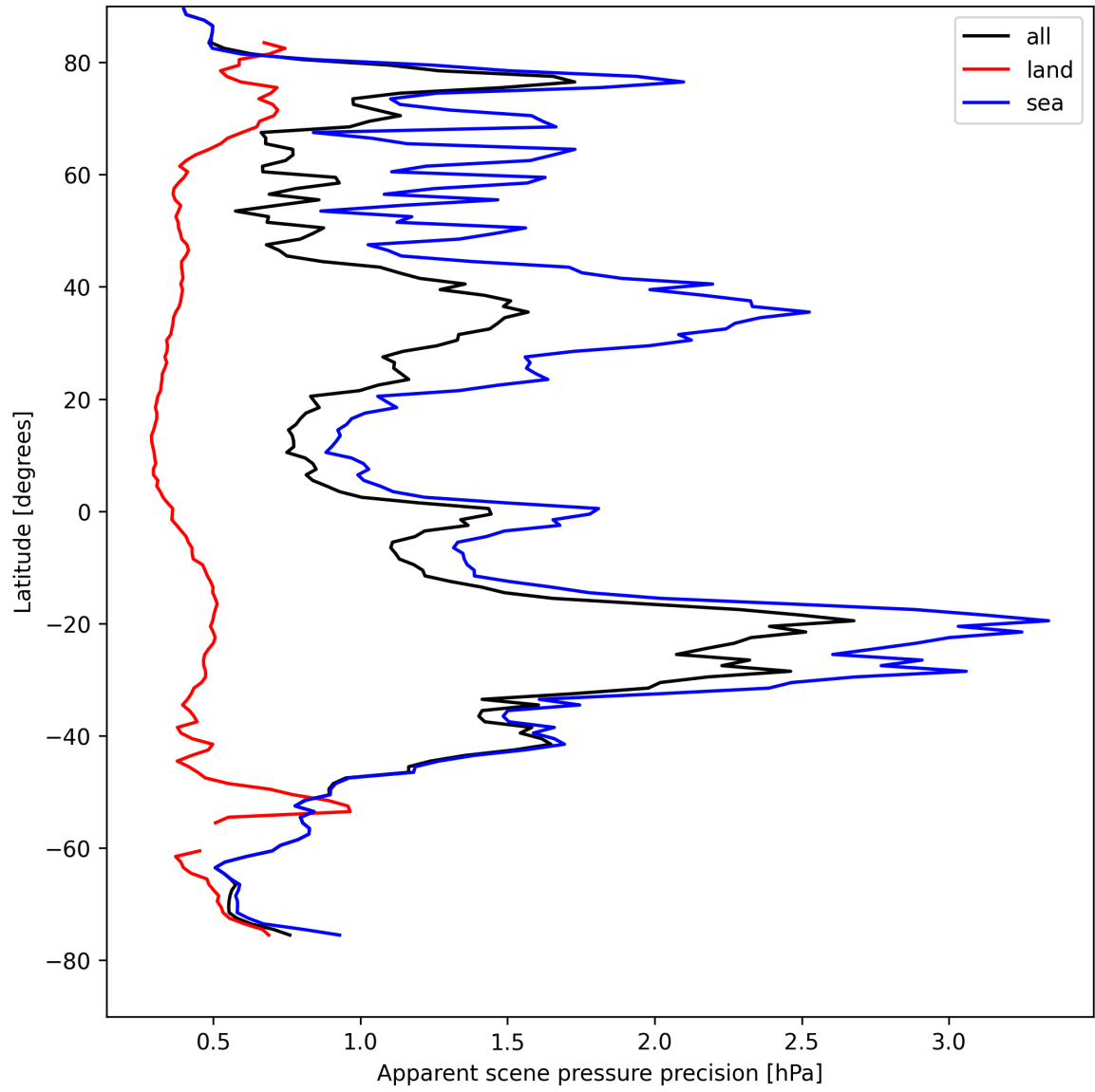
Figure 18: Zonal average of “Apparent scene pressure precision” for 2025-08-19 to 2025-08-20.
