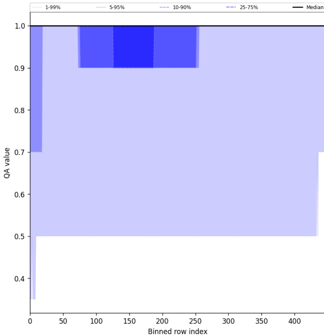
Figure 44: Along track statistics of “QA value” for 2025-08-19 to 2025-08-20
