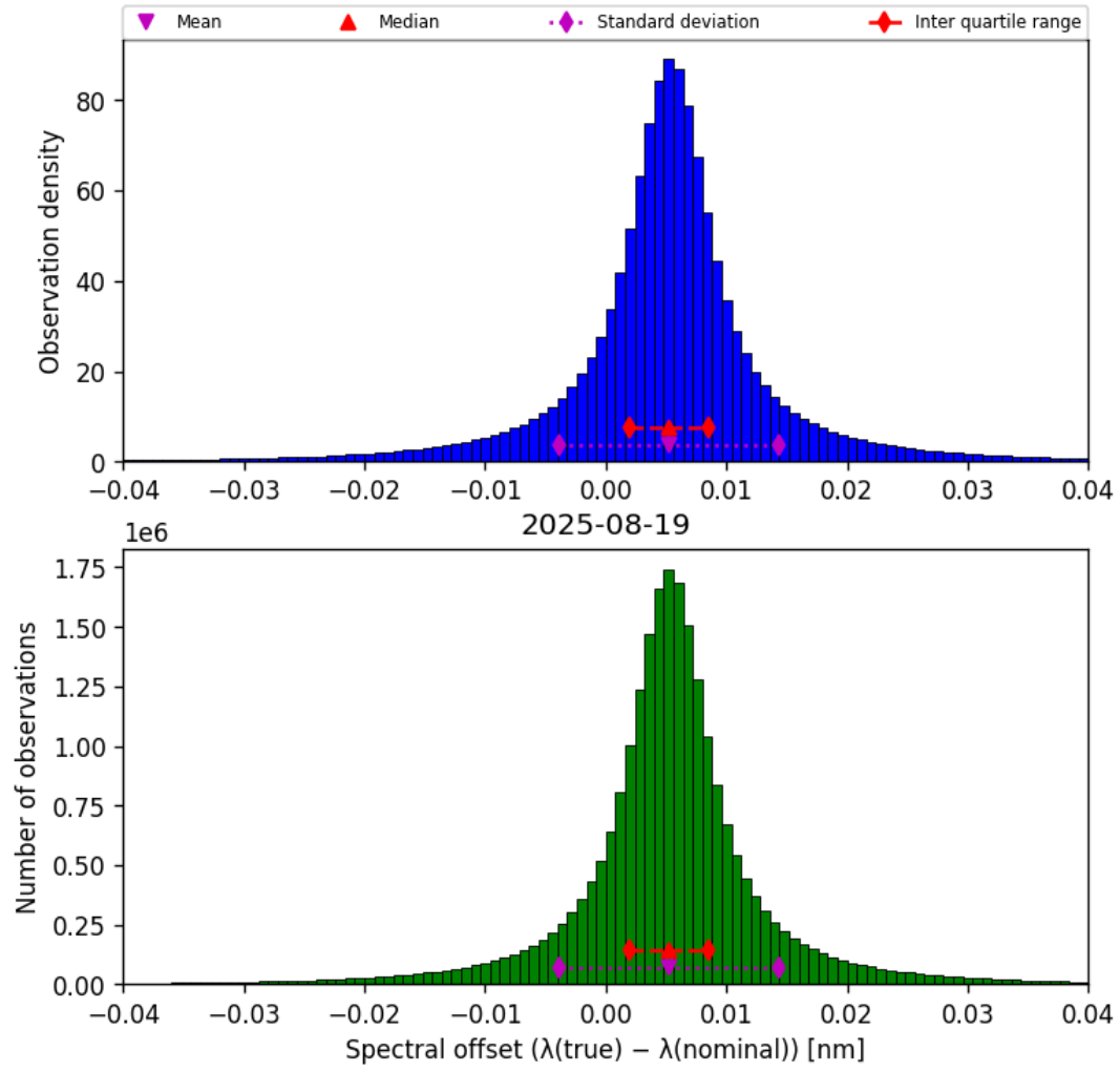
Figure 43: Histogram of “Spectral offset ( \lambda_{\text{true}} - \lambda_{\text{nominal}} )” for 2025-08-19 to 2025-08-20
