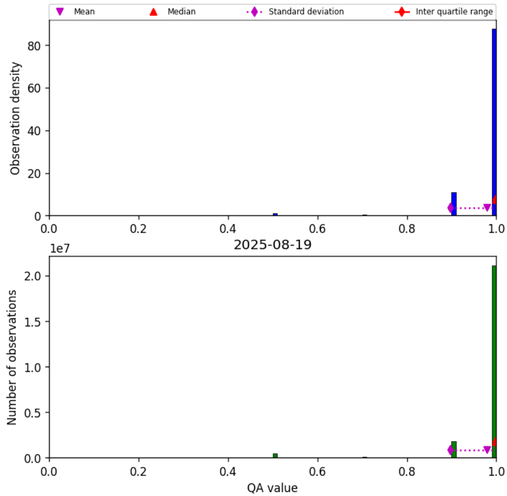
Figure 27: Histogram of “QA value” for 2025-08-19 to 2025-08-20
