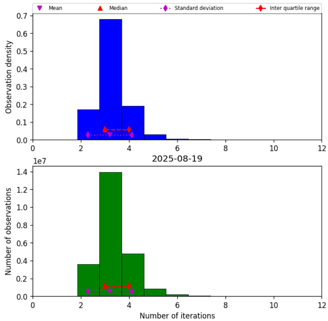
Figure 37: Histogram of “Number of iterations” for 2025-08-19 to 2025-08-20
