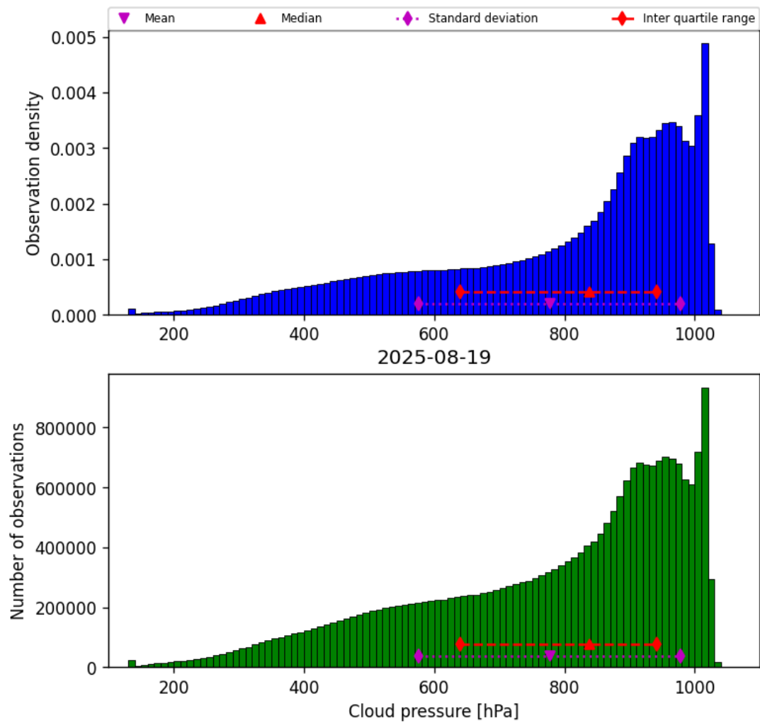
Figure 28: Histogram of “Cloud pressure” for 2025-08-19 to 2025-08-20
