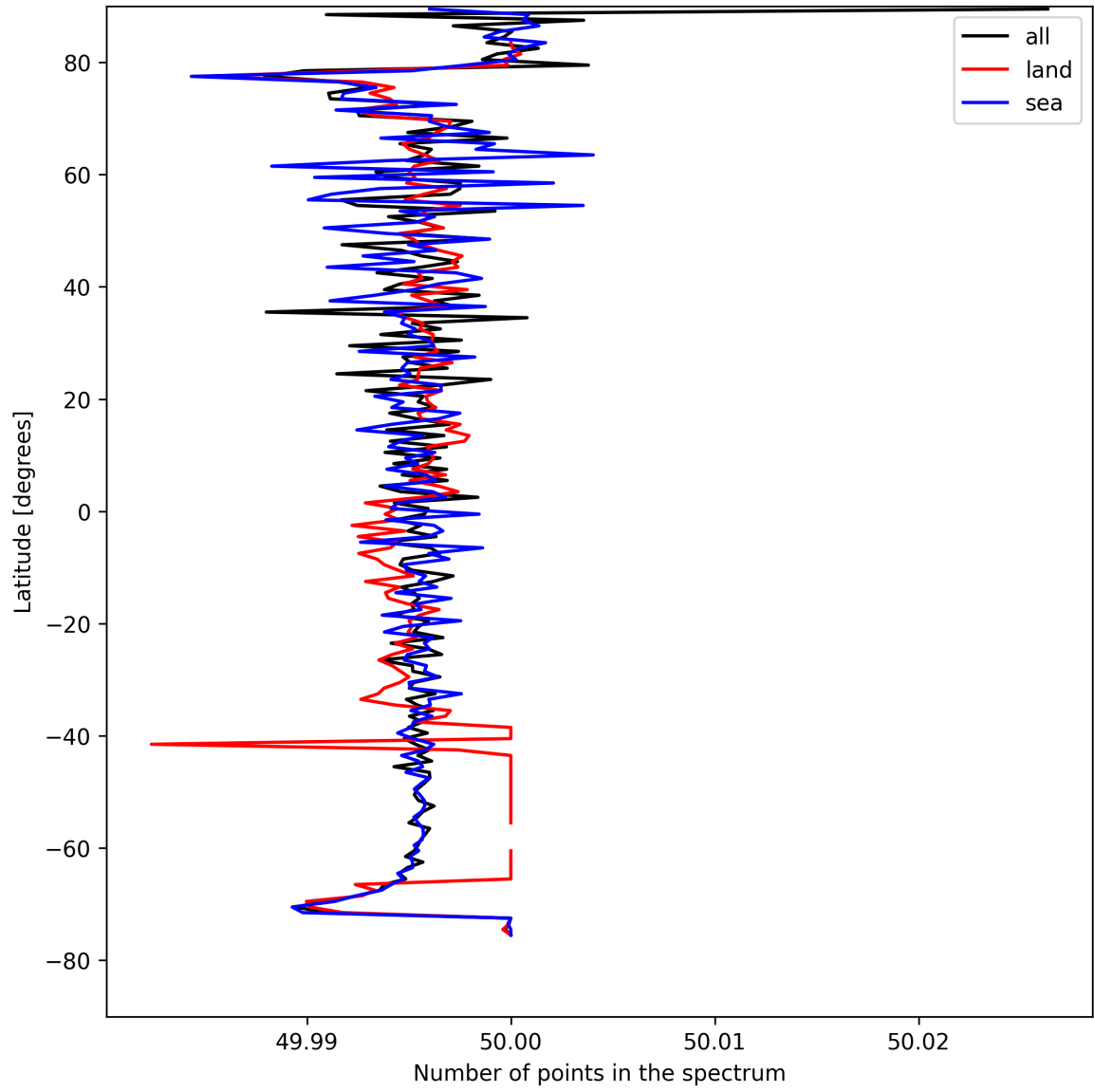
Figure 25: Zonal average of “Number of points in the spectrum” for 2025-08-19 to 2025-08-20.
