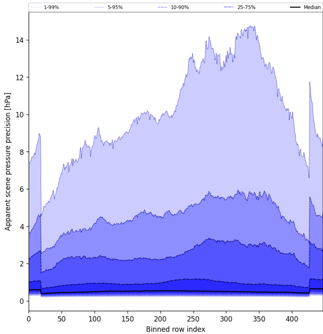
Figure 52: Along track statistics of “Apparent scene pressure precision” for 2025-08-19 to 2025-08-20
