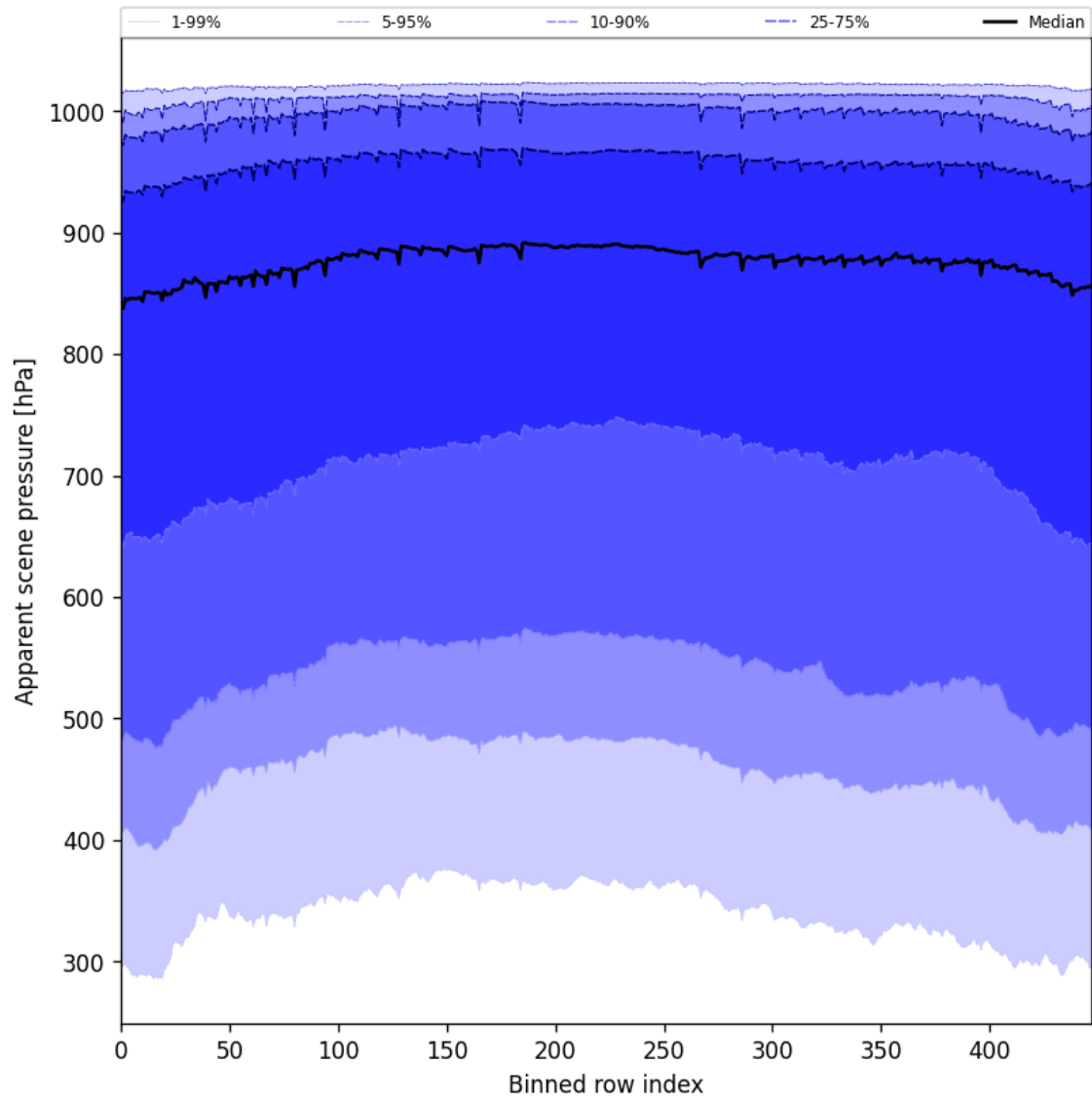
Figure 51: Along track statistics of “Apparent scene pressure” for 2025-08-19 to 2025-08-20
