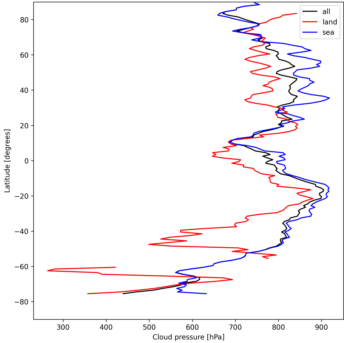
Figure 11: Zonal average of “Cloud pressure” for 2025-08-19 to 2025-08-20.
