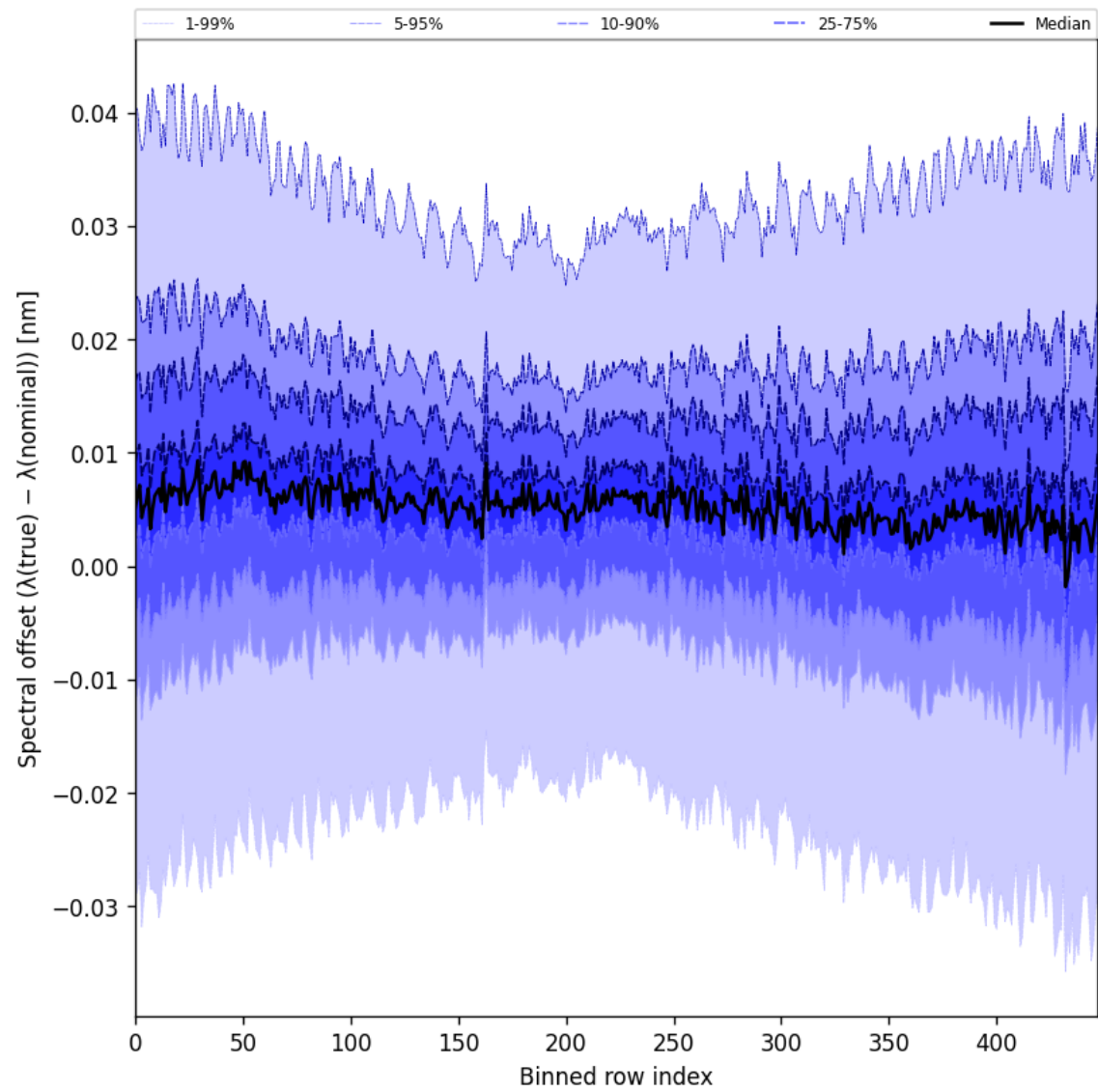
Figure 60: Along track statistics of “Spectral offset ( \lambda_{\text{true}} - \lambda_{\text{nominal}} )” for 2025-08-19 to 2025-08-20
