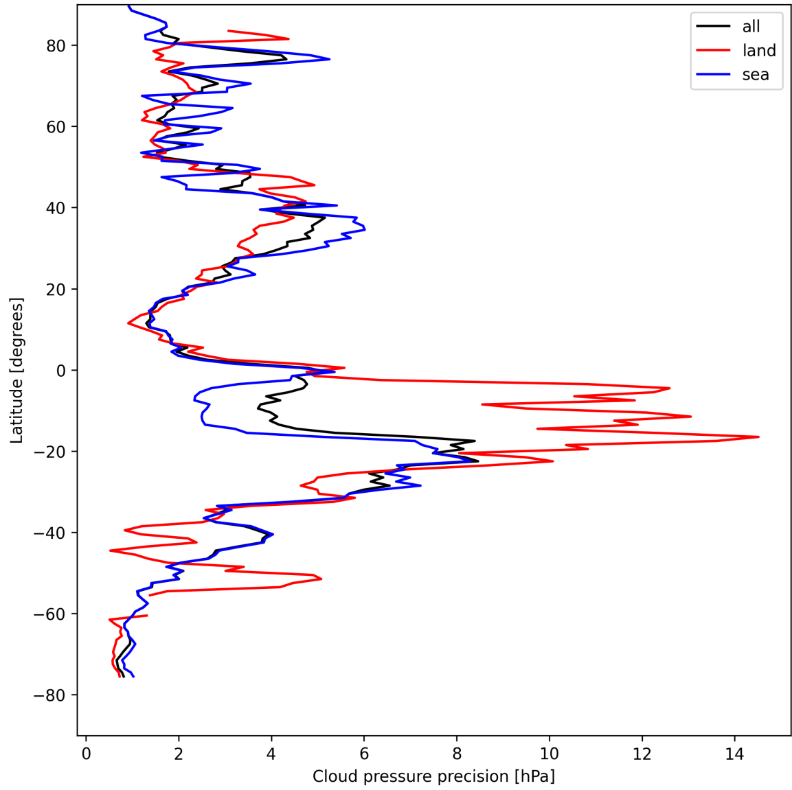
Figure 12: Zonal average of “Cloud pressure precision” for 2025-08-19 to 2025-08-20.
