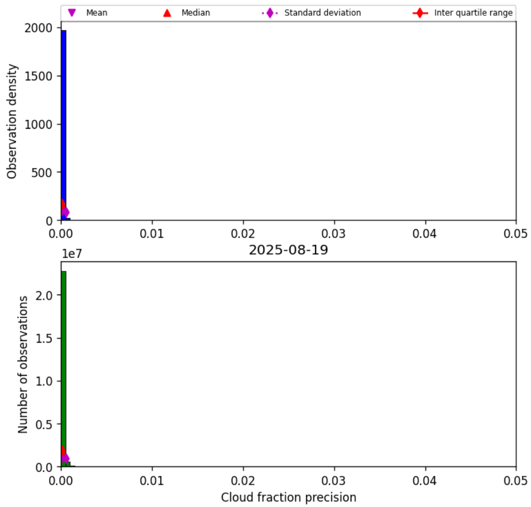
Figure 31: Histogram of “Cloud fraction precision” for 2025-08-19 to 2025-08-20
