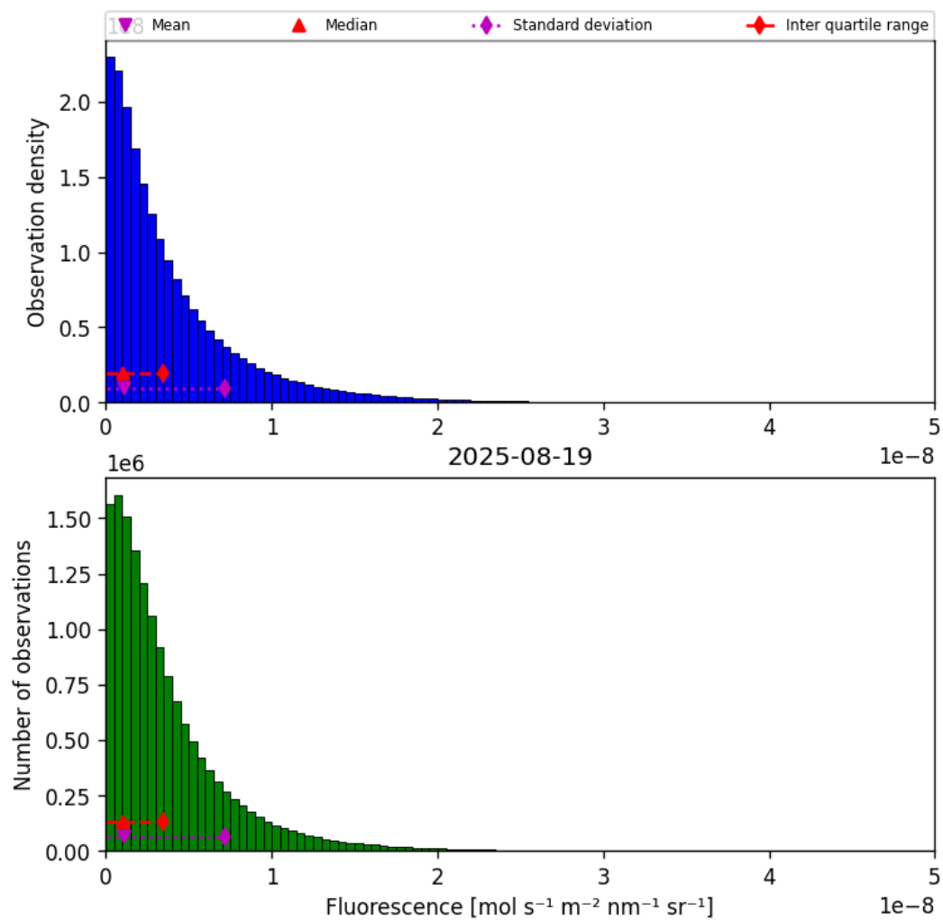
Figure 38: Histogram of “Fluorescence” for 2025-08-19 to 2025-08-20
