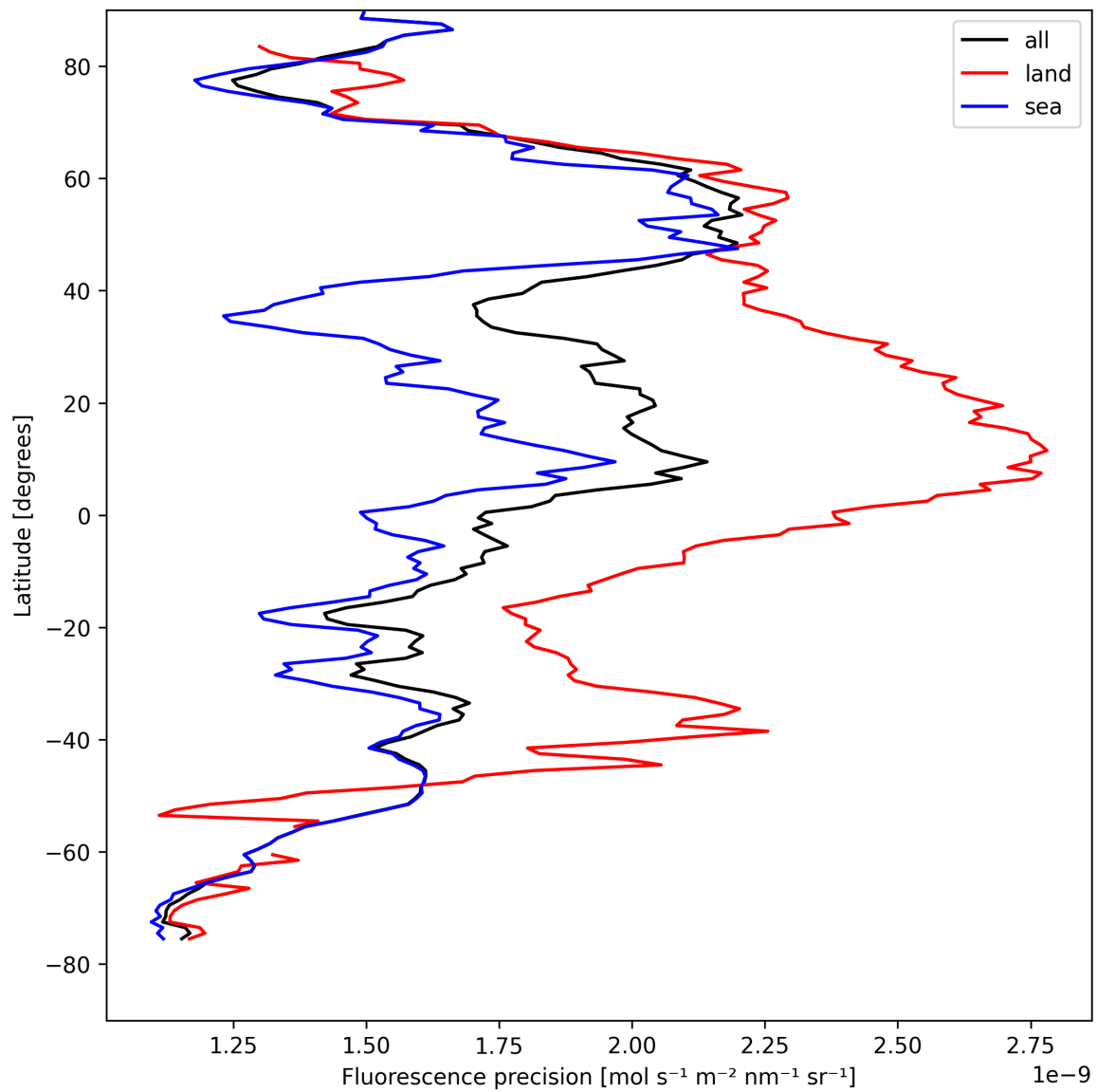
Figure 22: Zonal average of “Fluorescence precision” for 2025-08-19 to 2025-08-20.
