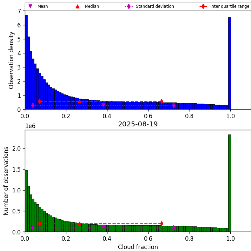
Figure 30: Histogram of “Cloud fraction” for 2025-08-19 to 2025-08-20
