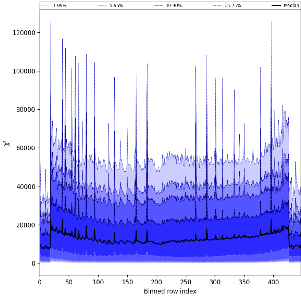
Figure 53: Along track statistics of “ \chi^2 ” for 2025-08-19 to 2025-08-20
