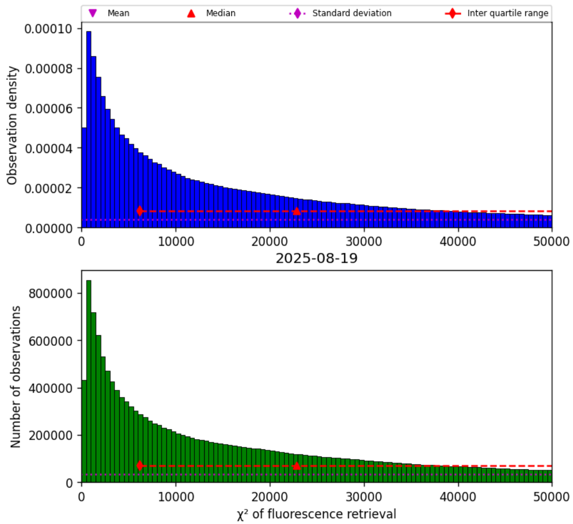
Figure 40: Histogram of “ \chi^2 of fluorescence retrieval” for 2025-08-19 to 2025-08-20
