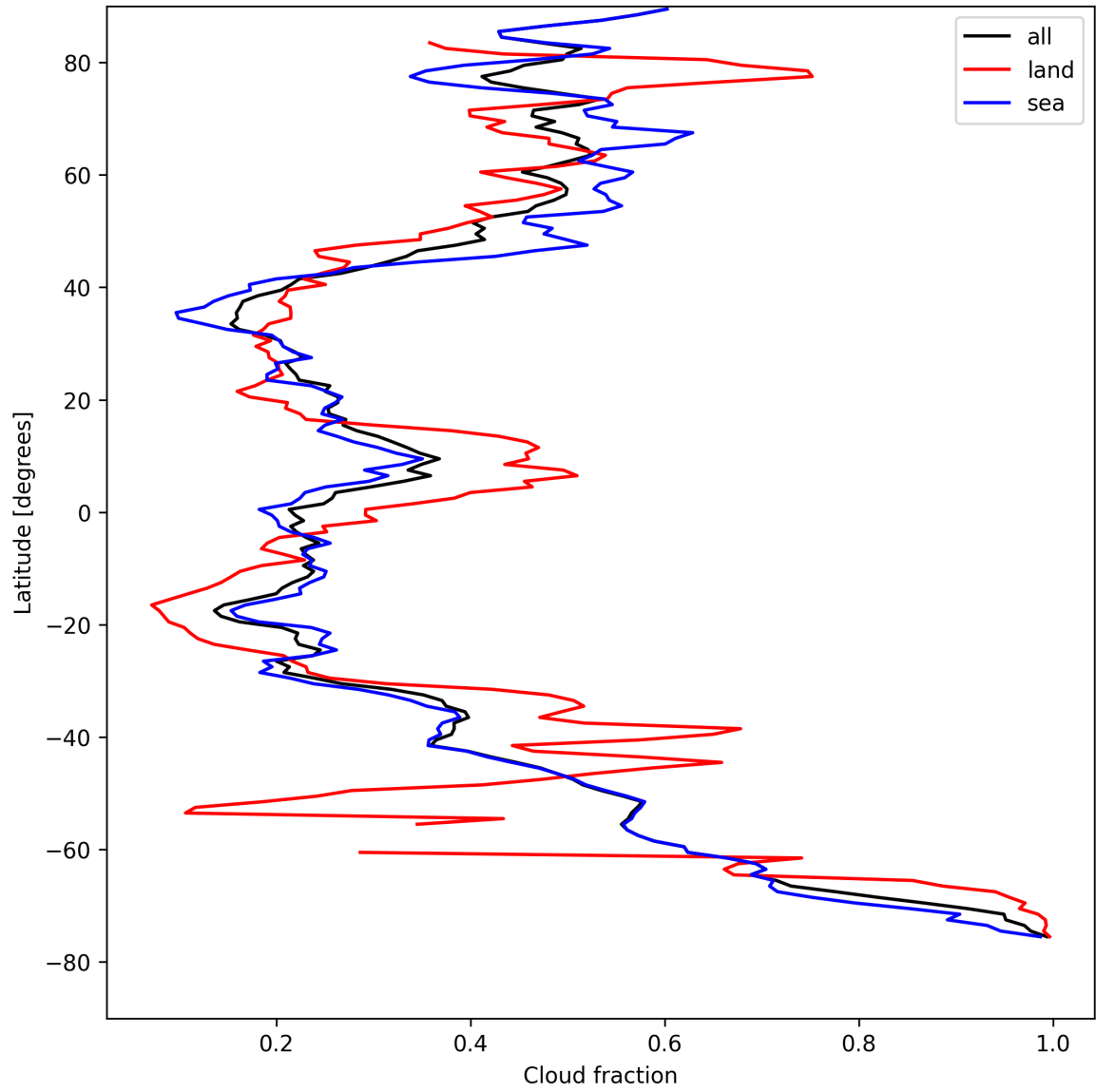
Figure 13: Zonal average of “Cloud fraction” for 2025-08-19 to 2025-08-20.
