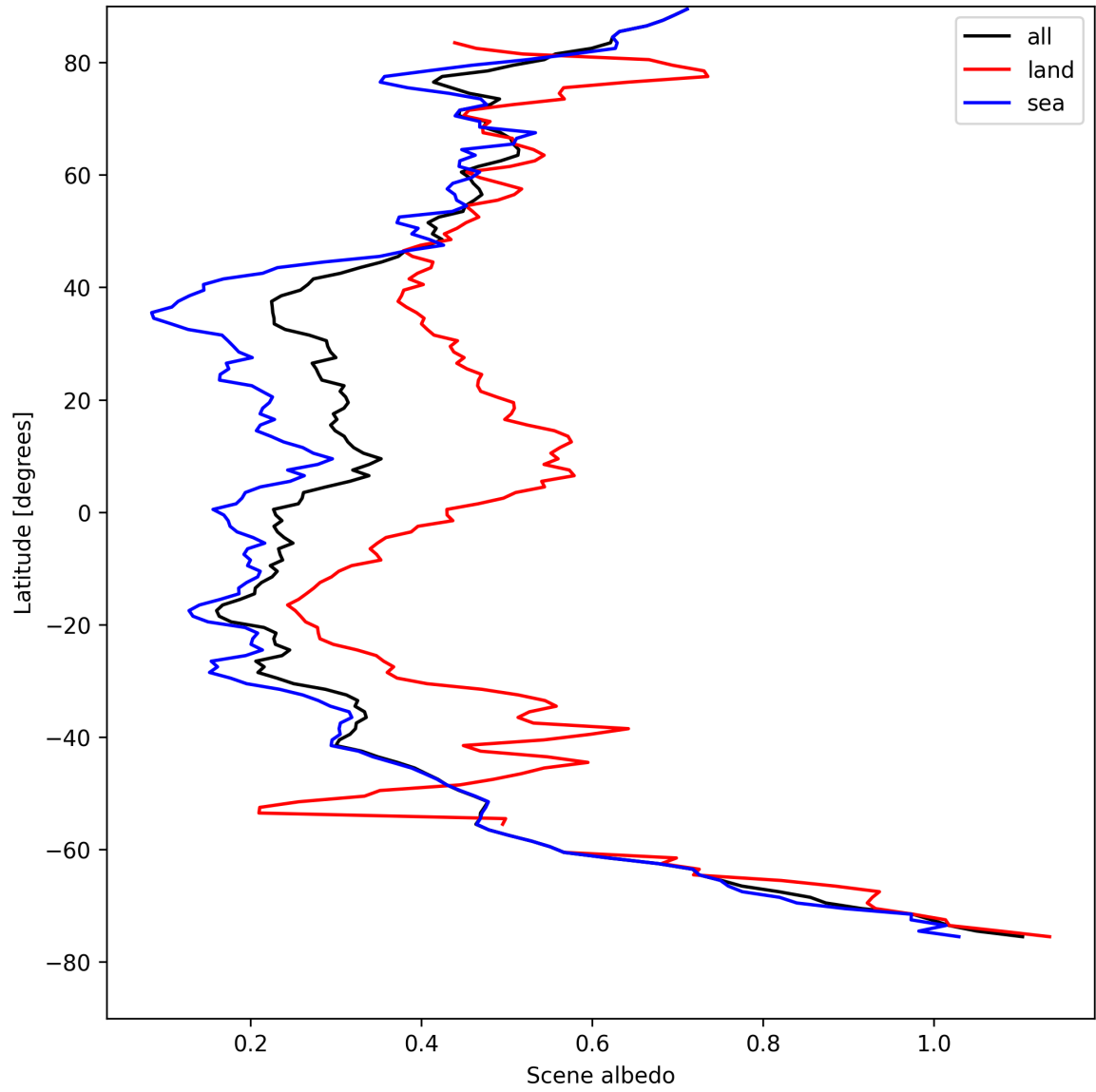
Figure 15: Zonal average of “Scene albedo” for 2025-08-19 to 2025-08-20.
