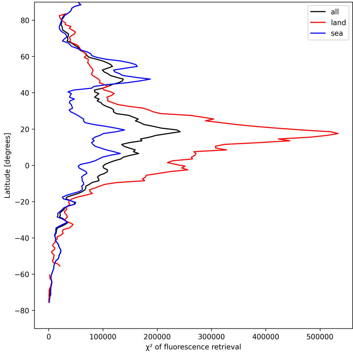
Figure 23: Zonal average of “ \chi^2 of fluorescence retrieval” for 2025-08-19 to 2025-08-20.
