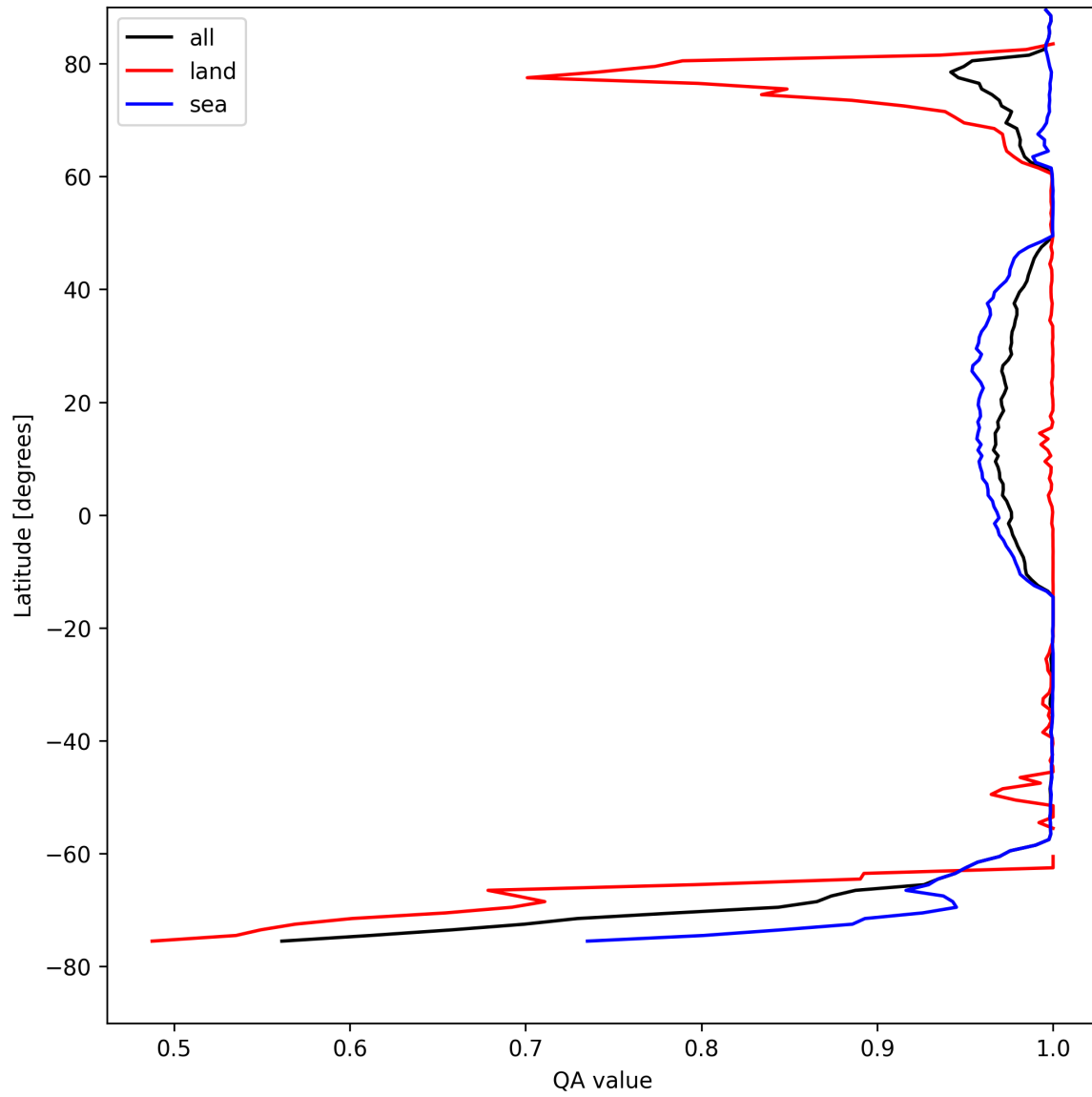
Figure 10: Zonal average of “QA value” for 2025-08-19 to 2025-08-20.
