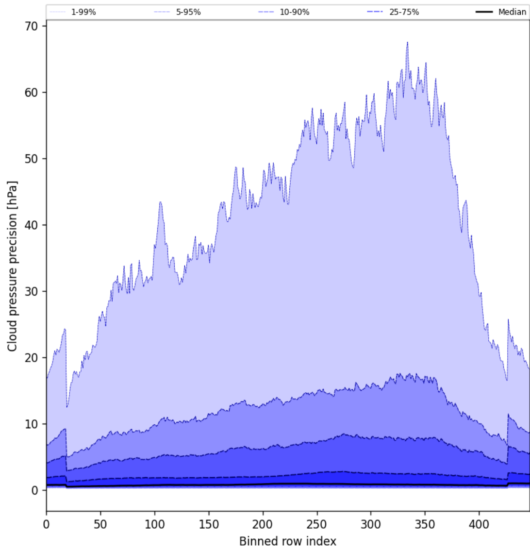
Figure 46: Along track statistics of “Cloud pressure precision” for 2025-08-19 to 2025-08-20
