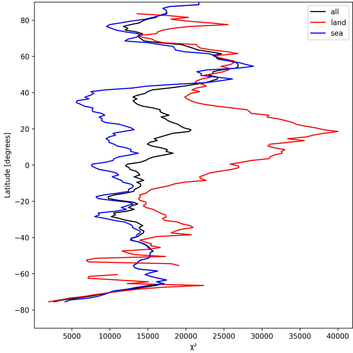
Figure 19: Zonal average of “ \chi^2 ” for 2025-08-19 to 2025-08-20.
