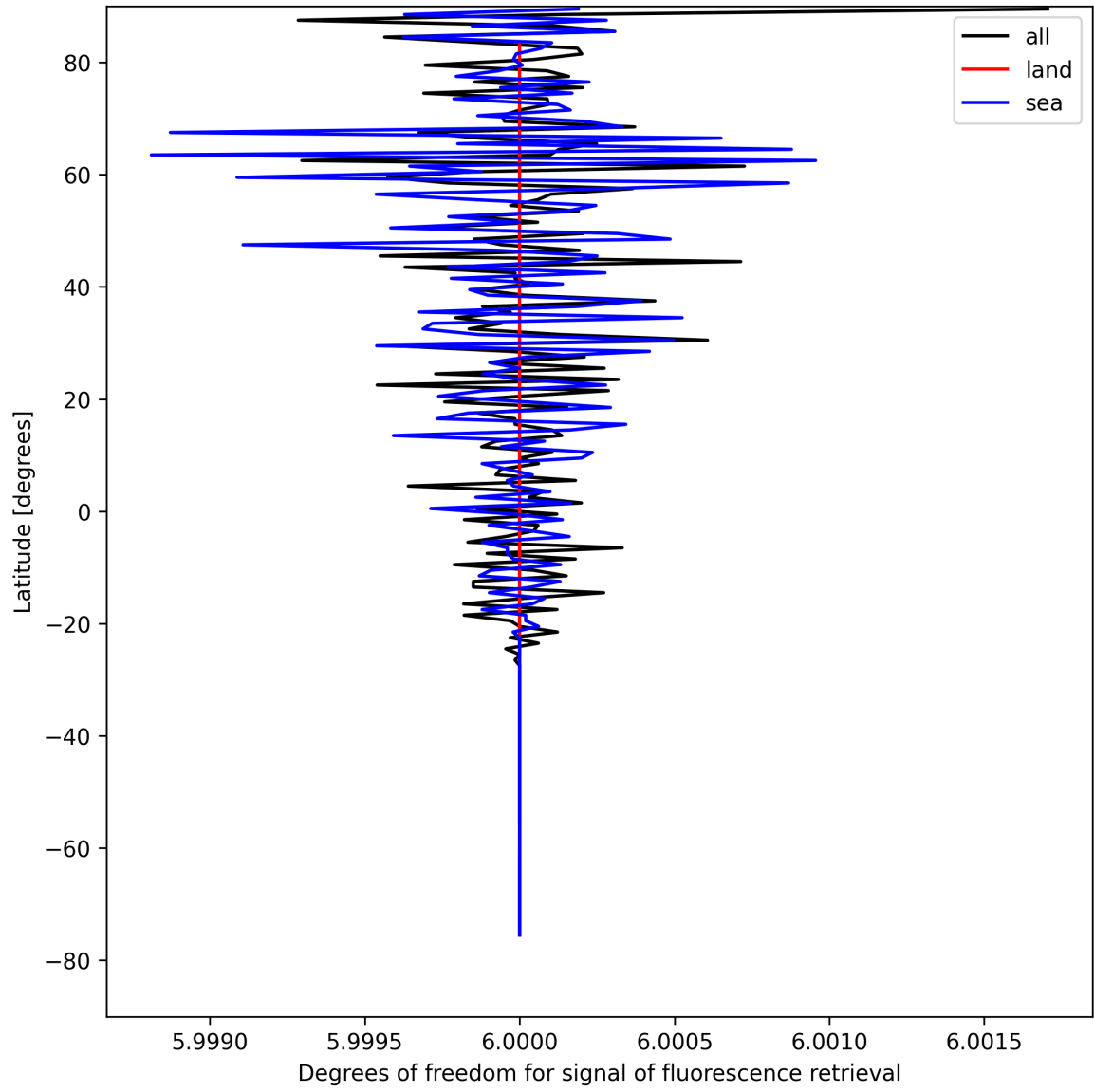
Figure 24: Zonal average of “Degrees of freedom for signal of fluorescence retrieval” for 2025-08-19 to 2025-08-20.
