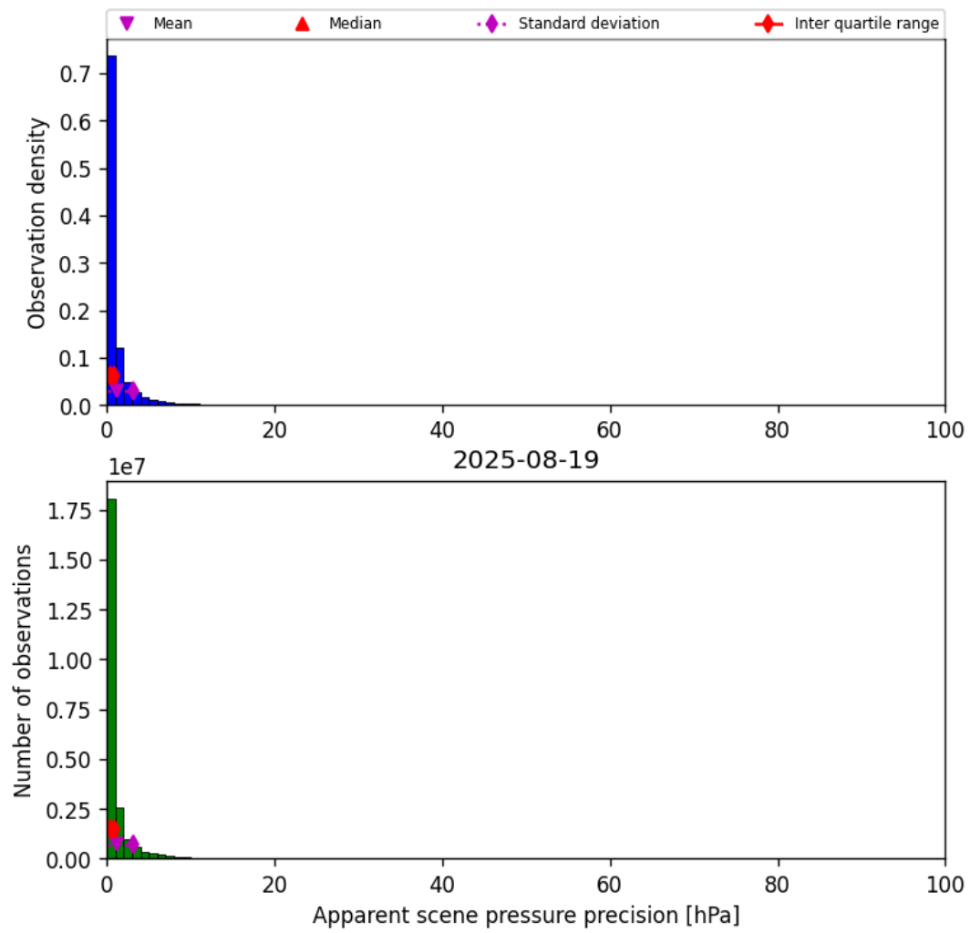
Figure 35: Histogram of “Apparent scene pressure precision” for 2025-08-19 to 2025-08-20
