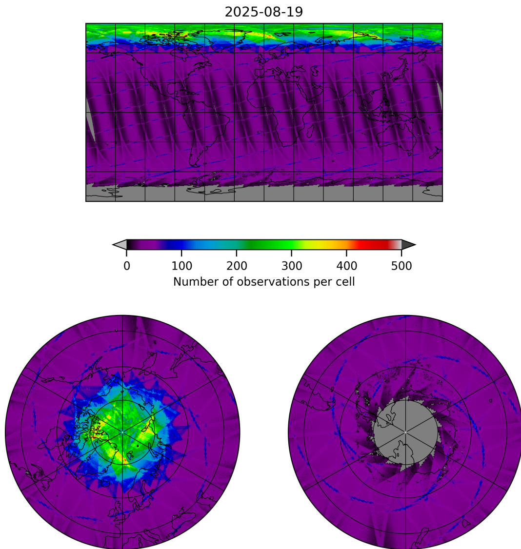
Figure 9: Map of the number of observations for 2025-08-19 to 2025-08-20
