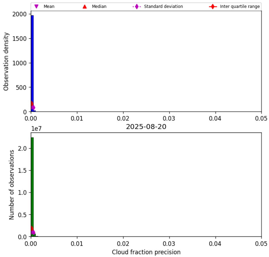
Figure 31: Histogram of “Cloud fraction precision” for 2025-08-20 to 2025-08-21
