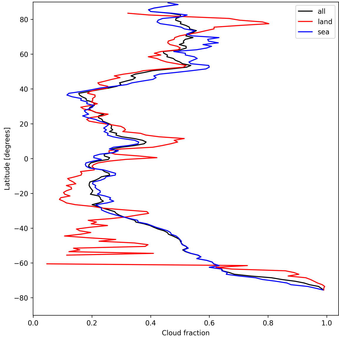
Figure 13: Zonal average of “Cloud fraction” for 2025-08-20 to 2025-08-21.
