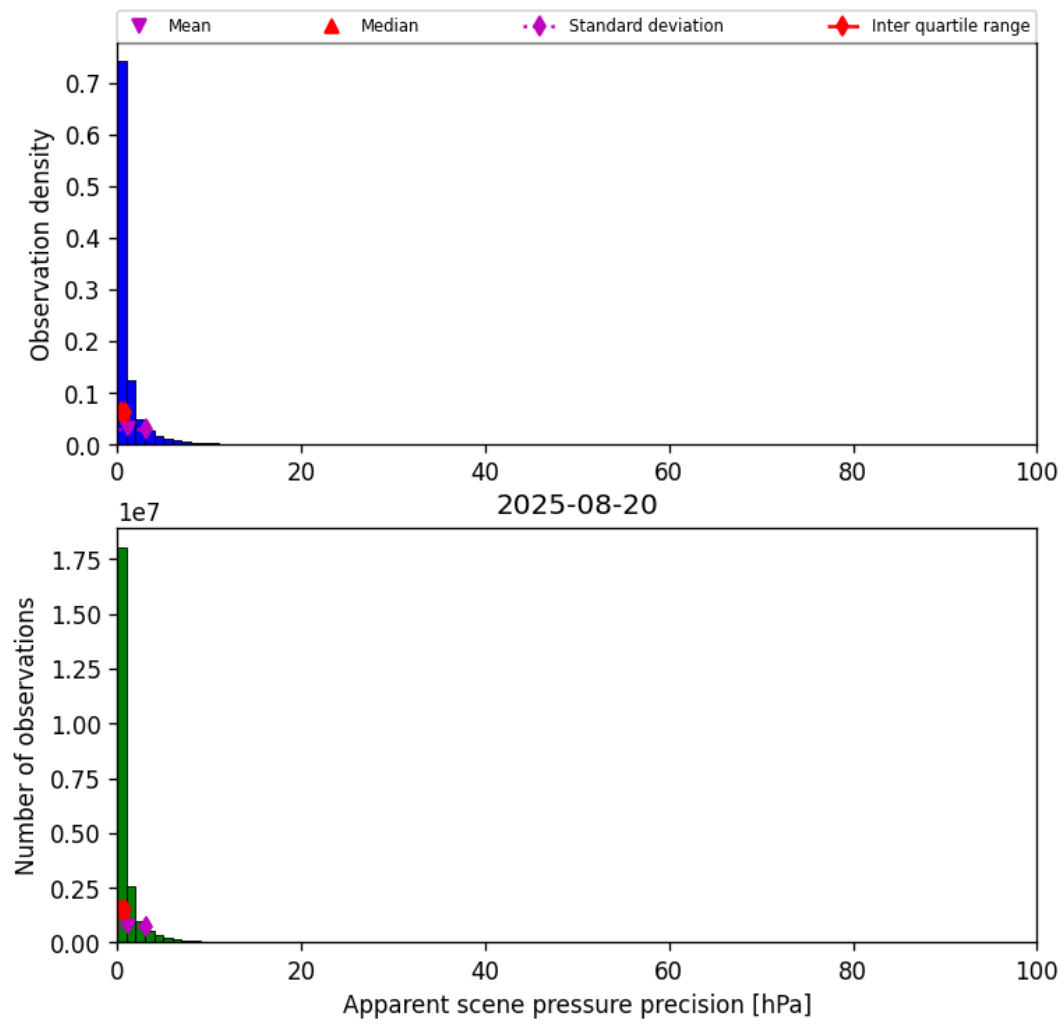
Figure 35: Histogram of “Apparent scene pressure precision” for 2025-08-20 to 2025-08-21
