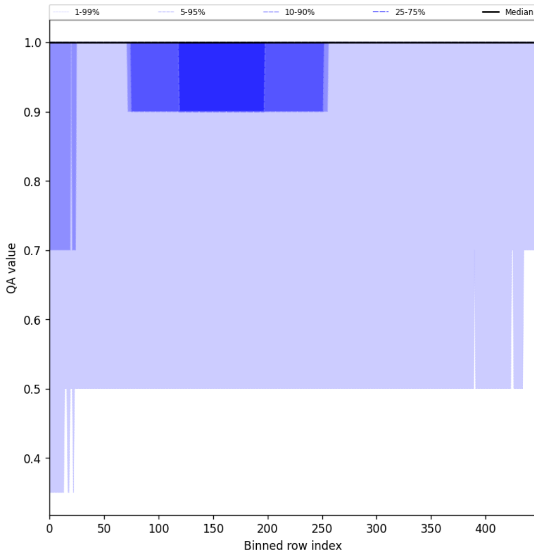
Figure 44: Along track statistics of “QA value” for 2025-08-20 to 2025-08-21
