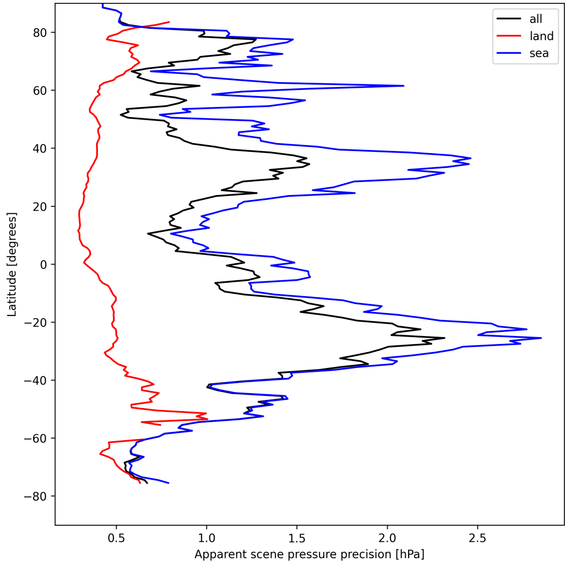
Figure 18: Zonal average of “Apparent scene pressure precision” for 2025-08-20 to 2025-08-21.
