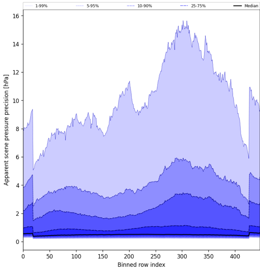
Figure 52: Along track statistics of “Apparent scene pressure precision” for 2025-08-20 to 2025-08-21
