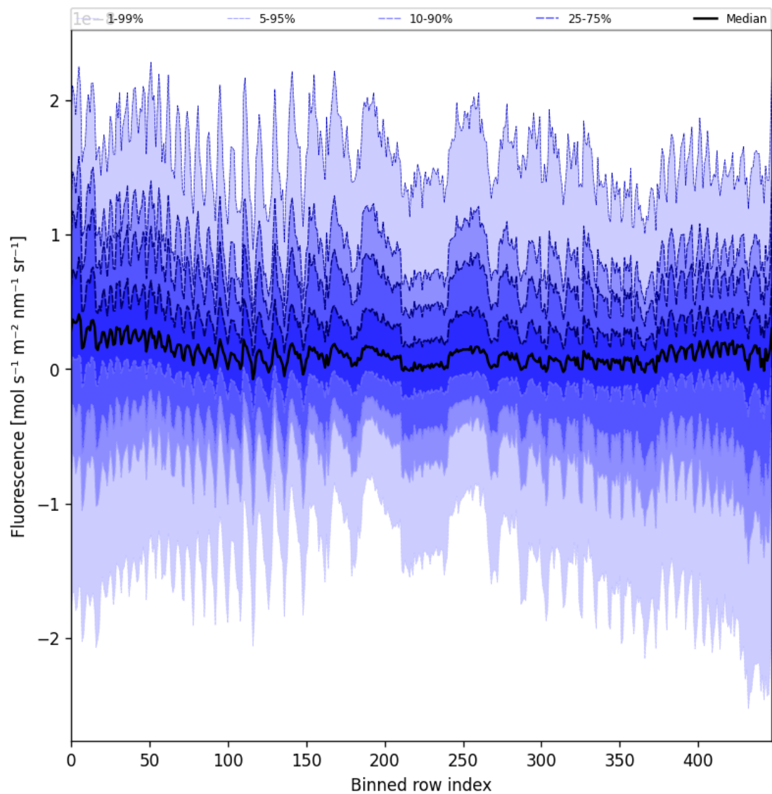
Figure 55: Along track statistics of “Fluorescence” for 2025-08-20 to 2025-08-21
