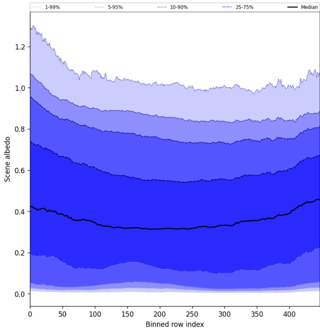
Figure 49: Along track statistics of “Scene albedo” for 2025-08-20 to 2025-08-21
