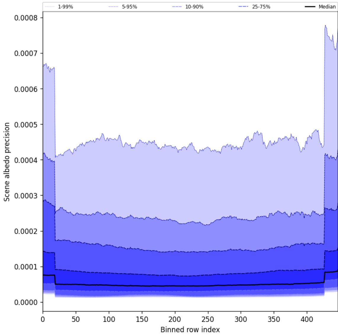
Figure 50: Along track statistics of “Scene albedo precision” for 2025-08-20 to 2025-08-21
