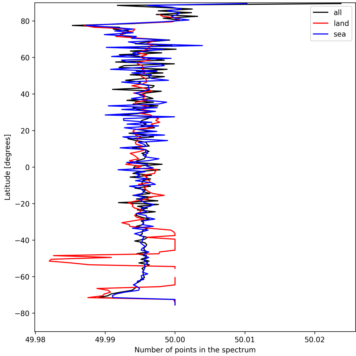
Figure 25: Zonal average of “Number of points in the spectrum” for 2025-08-20 to 2025-08-21.
