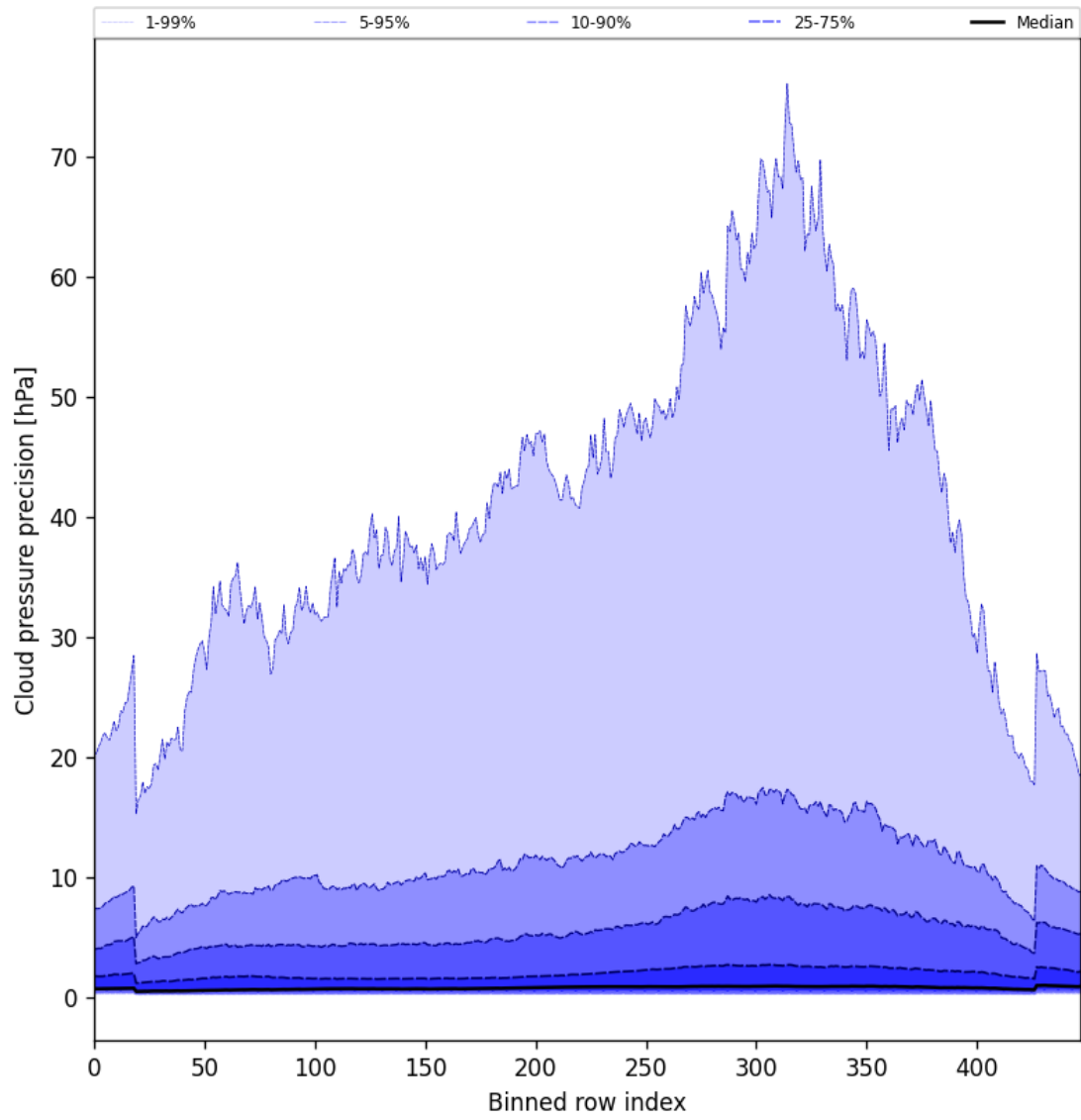
Figure 46: Along track statistics of “Cloud pressure precision” for 2025-08-20 to 2025-08-21
