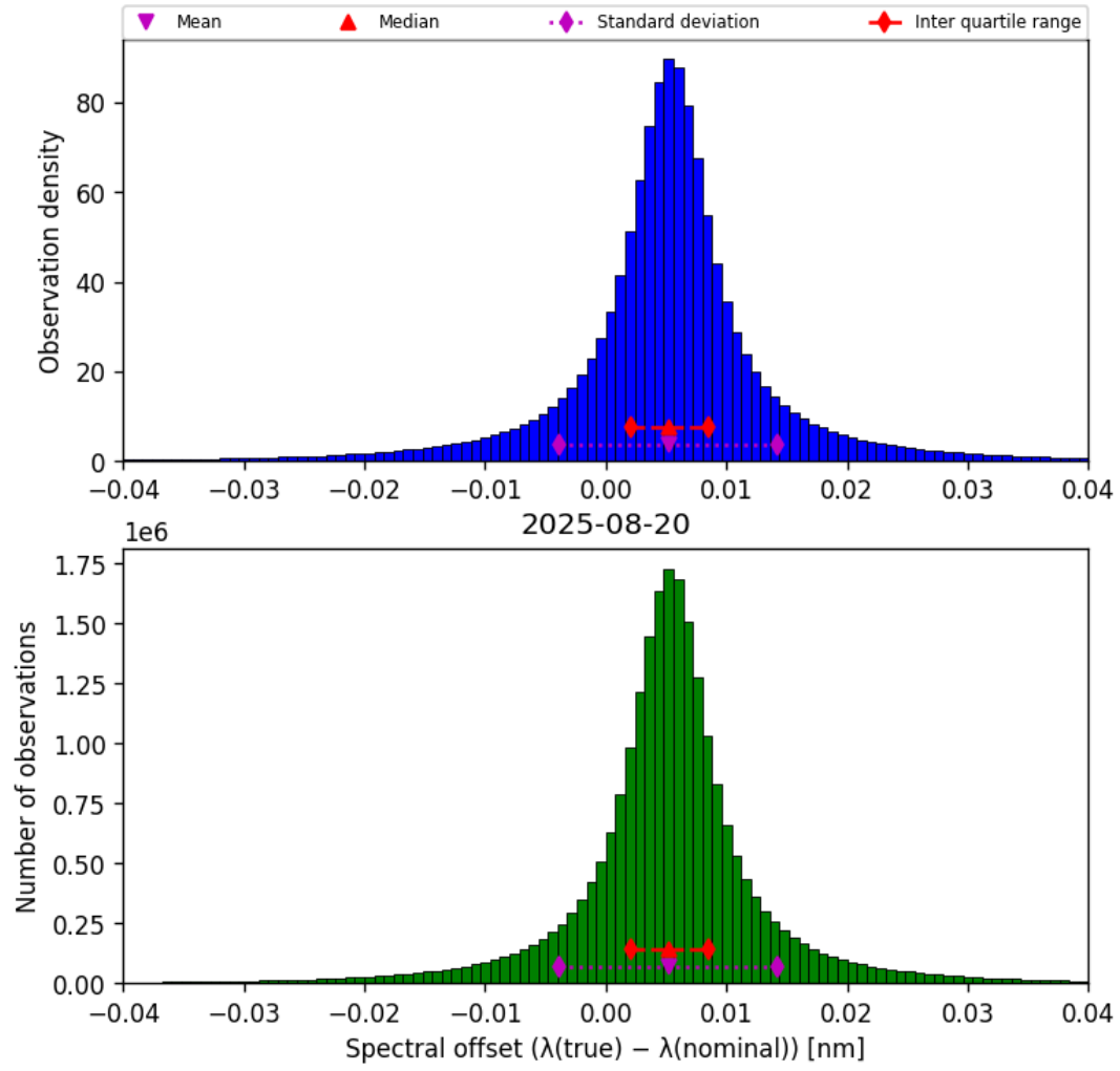
Figure 43: Histogram of “Spectral offset ( \lambda_{\text{true}} - \lambda_{\text{nominal}} )” for 2025-08-20 to 2025-08-21
