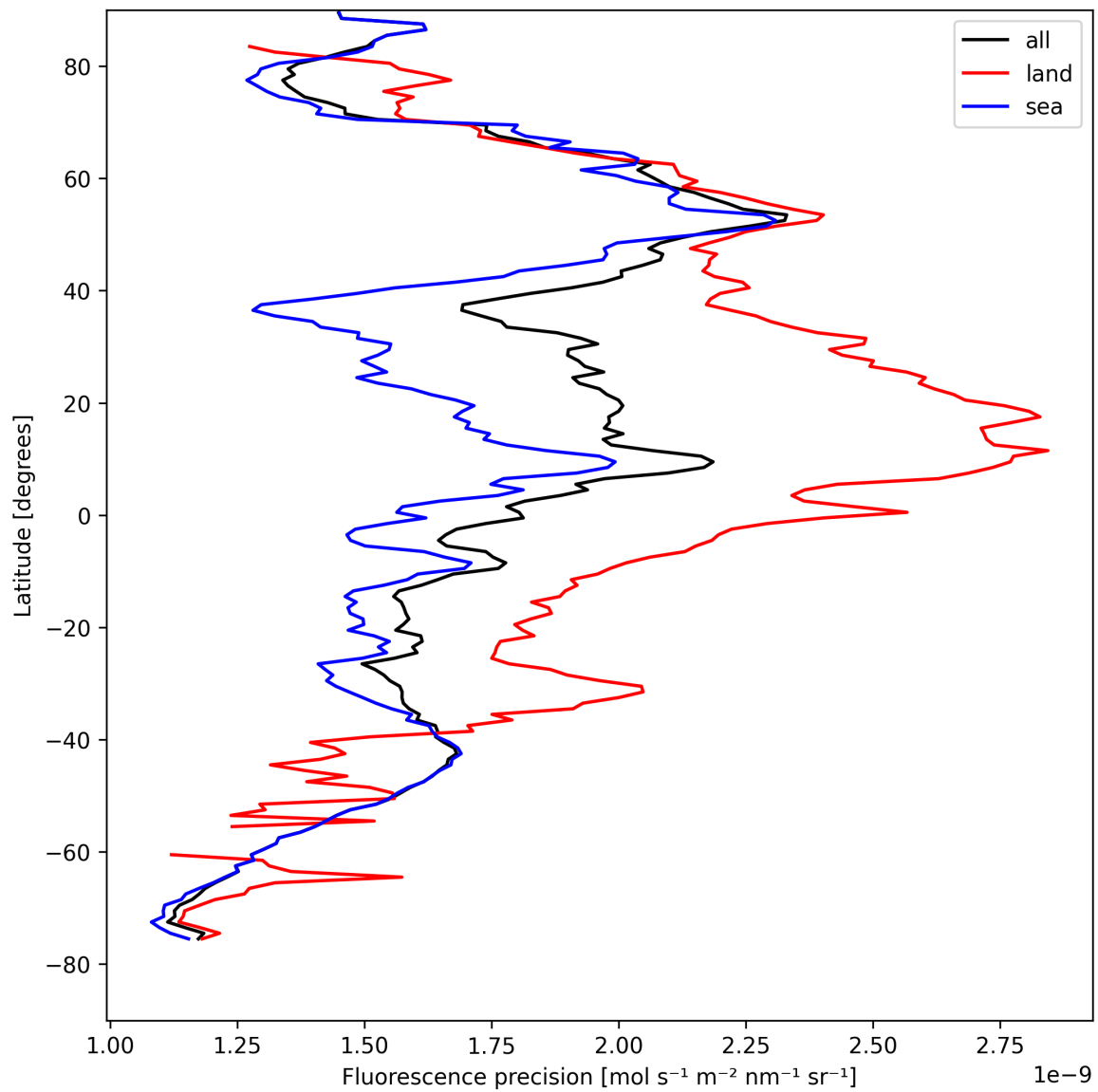
Figure 22: Zonal average of “Fluorescence precision” for 2025-08-20 to 2025-08-21.
