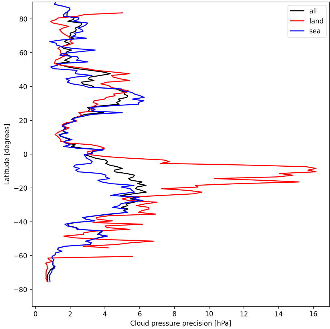
Figure 12: Zonal average of “Cloud pressure precision” for 2025-08-20 to 2025-08-21.
