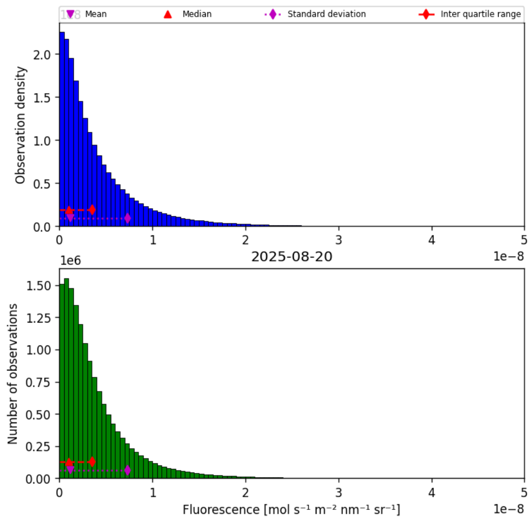
Figure 38: Histogram of “Fluorescence” for 2025-08-20 to 2025-08-21
