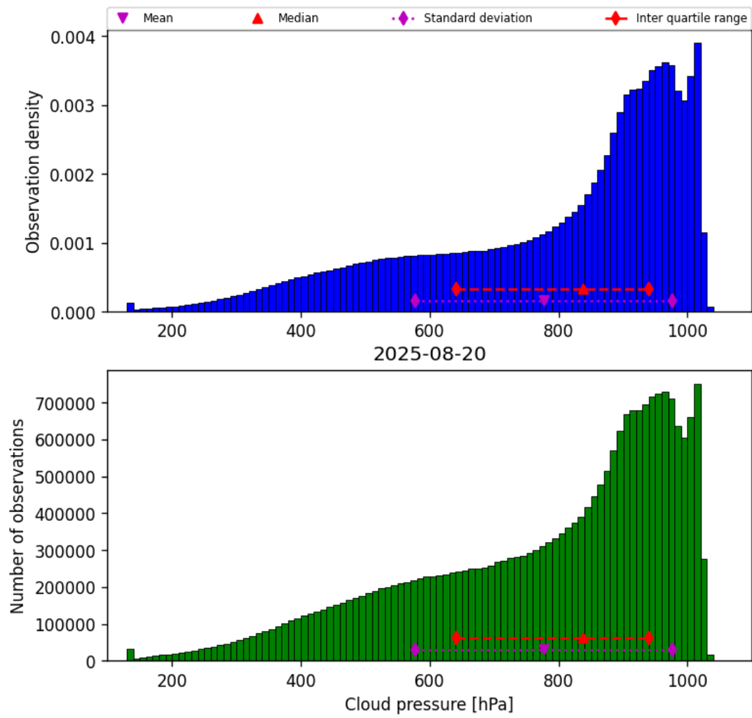
Figure 28: Histogram of “Cloud pressure” for 2025-08-20 to 2025-08-21
