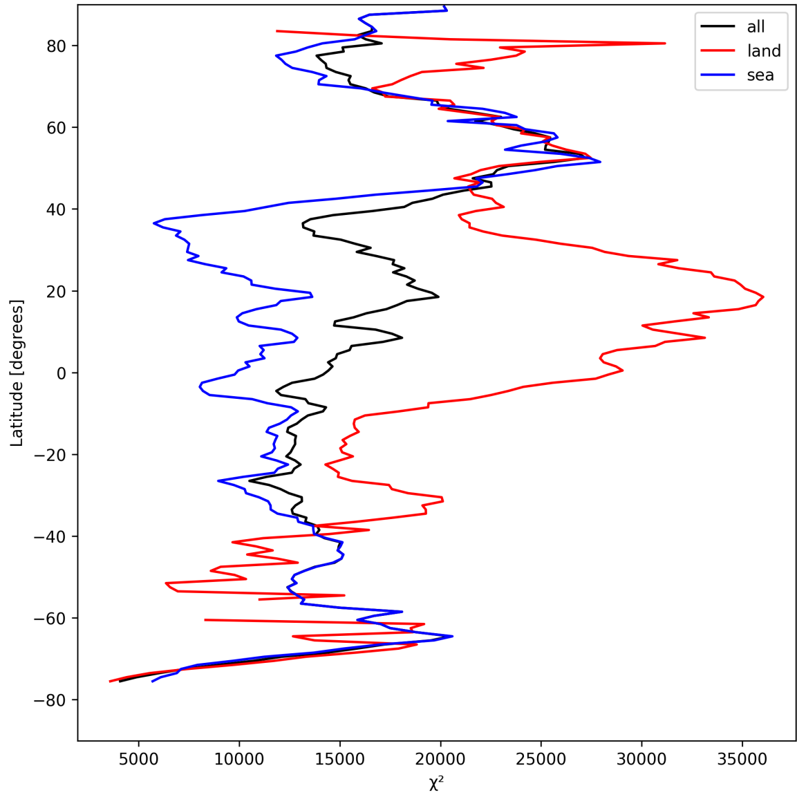
Figure 19: Zonal average of “ \chi^2 ” for 2025-08-20 to 2025-08-21.
