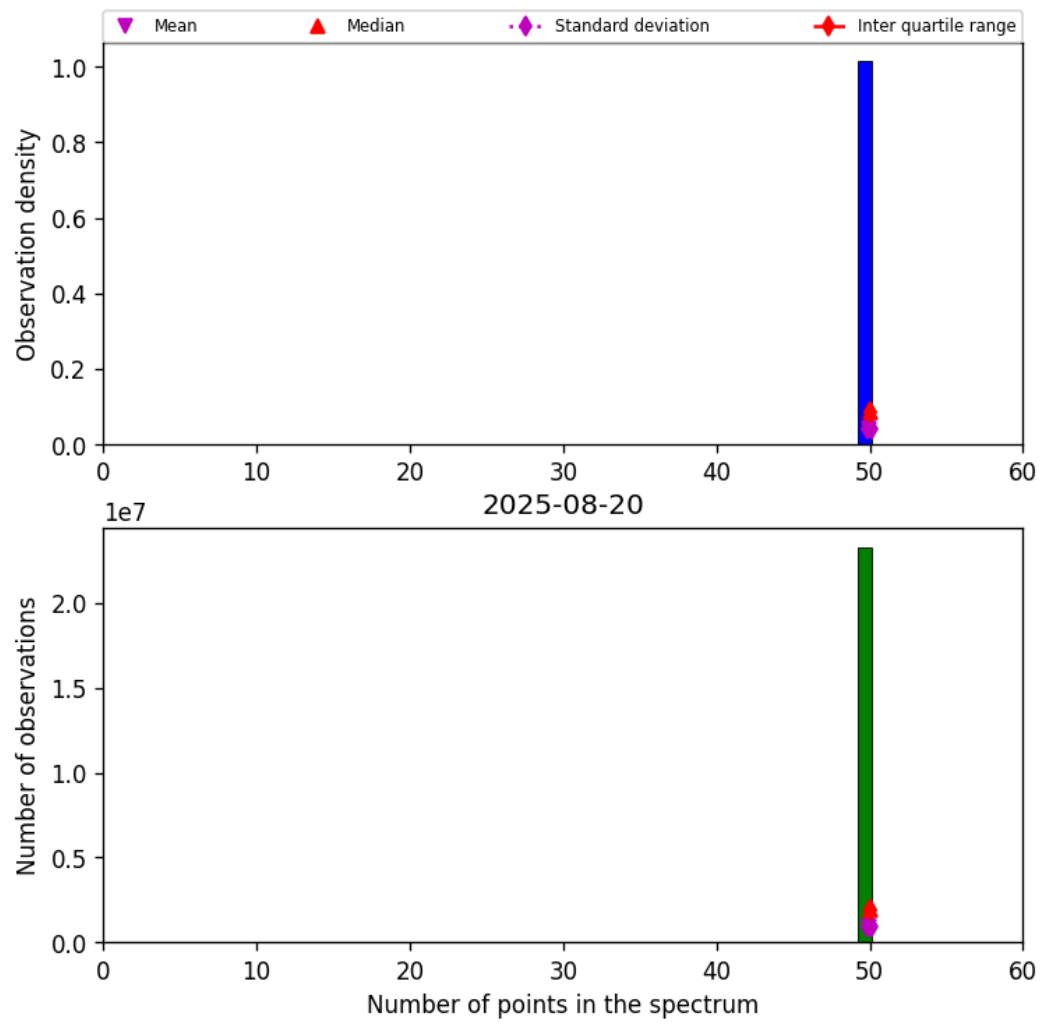
Figure 42: Histogram of “Number of points in the spectrum” for 2025-08-20 to 2025-08-21
