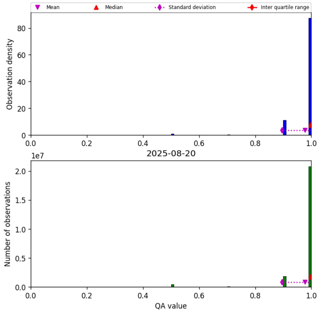
Figure 27: Histogram of “QA value” for 2025-08-20 to 2025-08-21
