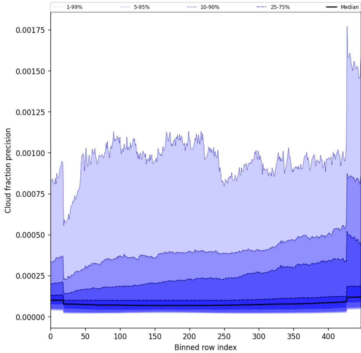
Figure 48: Along track statistics of “Cloud fraction precision” for 2025-08-20 to 2025-08-21
