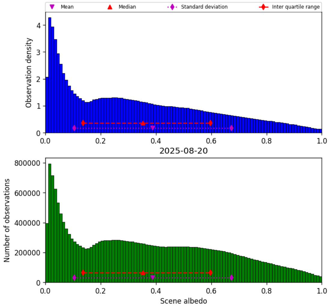
Figure 32: Histogram of “Scene albedo” for 2025-08-20 to 2025-08-21
