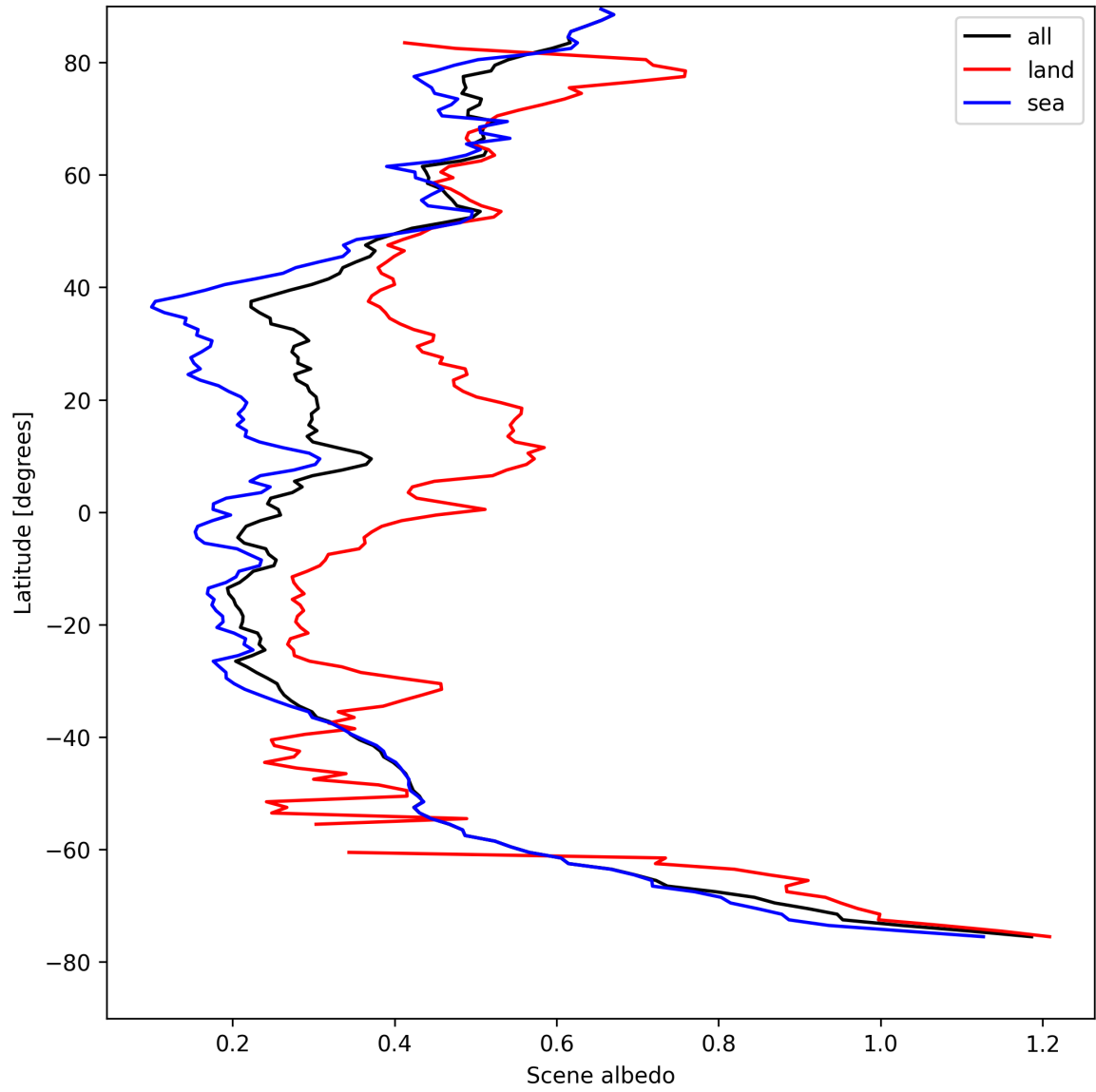
Figure 15: Zonal average of “Scene albedo” for 2025-08-20 to 2025-08-21.
