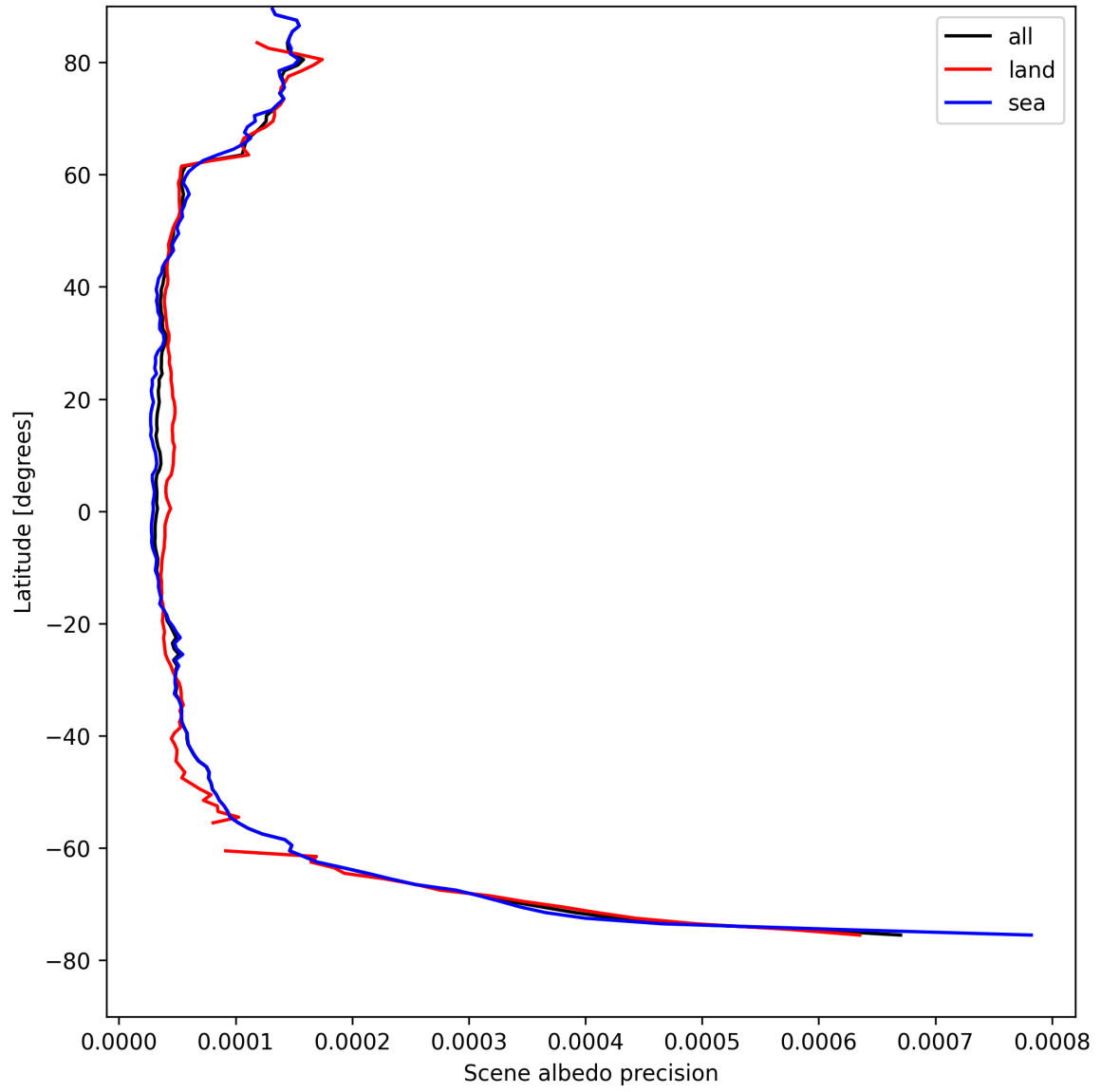
Figure 16: Zonal average of “Scene albedo precision” for 2025-08-20 to 2025-08-21.
