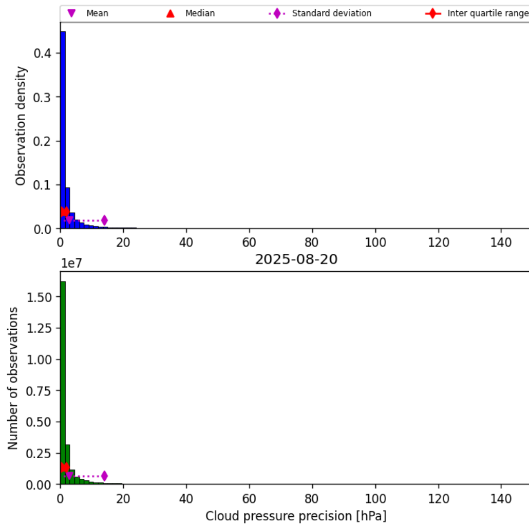
Figure 29: Histogram of "Cloud pressure precision" for 2025-08-20 to 2025-08-21
