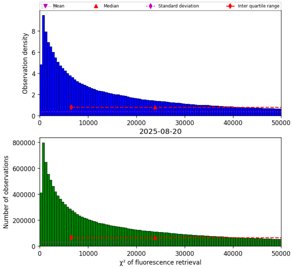
Figure 40: Histogram of “ \chi^2 of fluorescence retrieval” for 2025-08-20 to 2025-08-21
