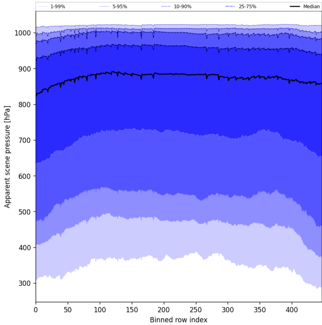
Figure 51: Along track statistics of “Apparent scene pressure” for 2025-08-20 to 2025-08-21
