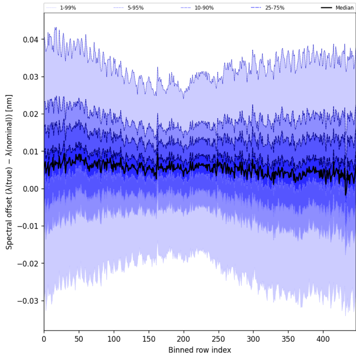
Figure 60: Along track statistics of “Spectral offset ( \lambda_{\text{true}} - \lambda_{\text{nominal}} )” for 2025-08-20 to 2025-08-21
