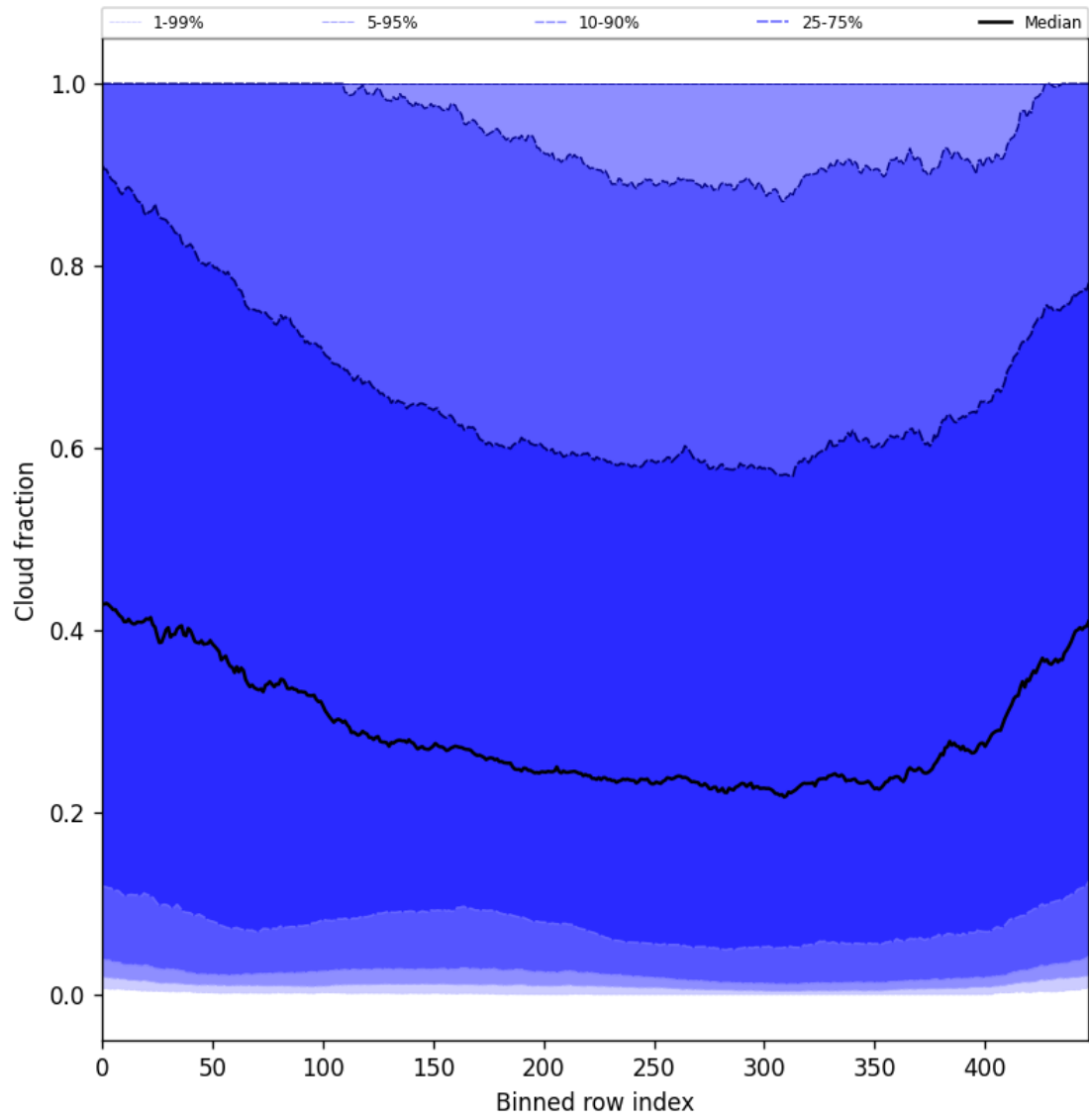
Figure 47: Along track statistics of “Cloud fraction” for 2025-08-20 to 2025-08-21
