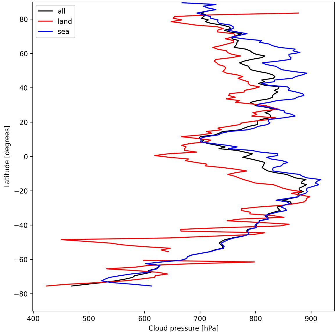
Figure 11: Zonal average of “Cloud pressure” for 2025-08-20 to 2025-08-21.
