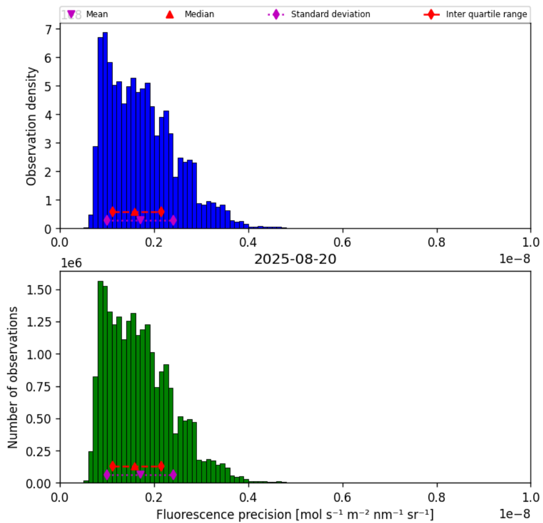
Figure 39: Histogram of “Fluorescence precision” for 2025-08-20 to 2025-08-21
