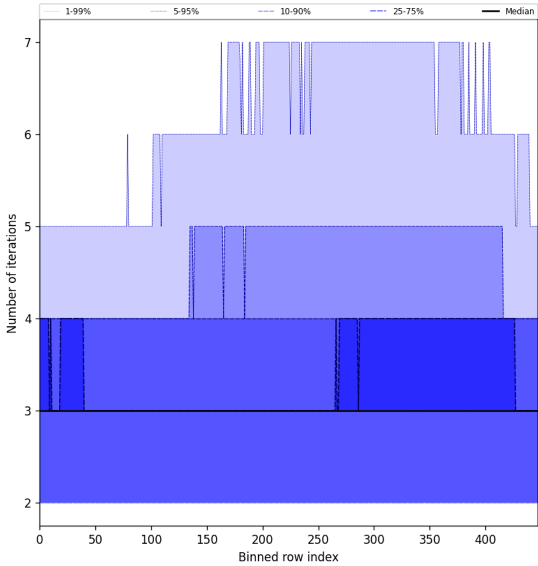
Figure 54: Along track statistics of “Number of iterations” for 2025-08-20 to 2025-08-21
