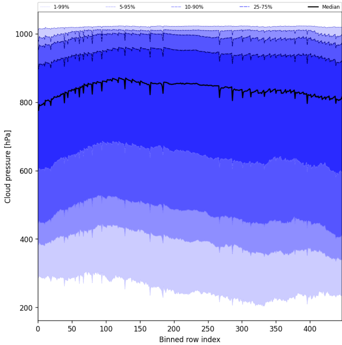
Figure 45: Along track statistics of “Cloud pressure” for 2025-08-20 to 2025-08-21
