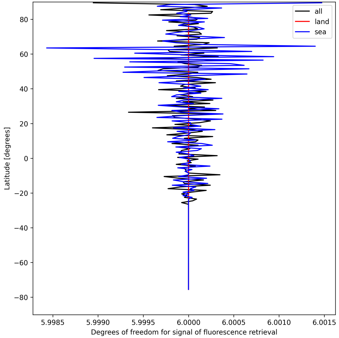
Figure 24: Zonal average of “Degrees of freedom for signal of fluorescence retrieval” for 2025-08-20 to 2025-08-21.
