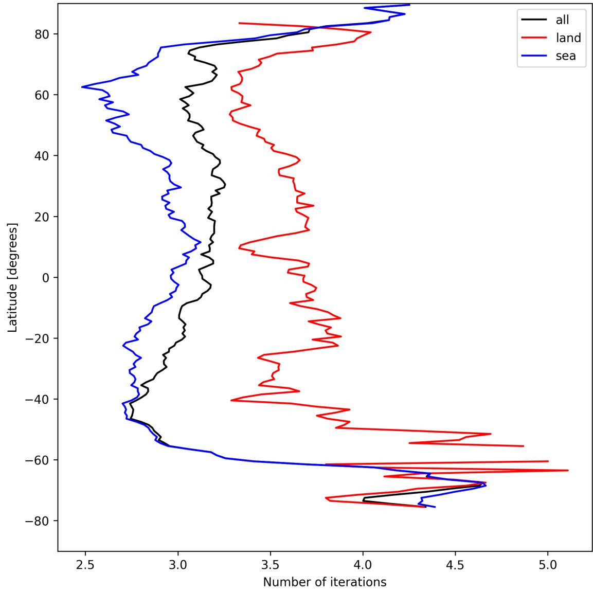
Figure 20: Zonal average of “Number of iterations” for 2025-08-20 to 2025-08-21.
