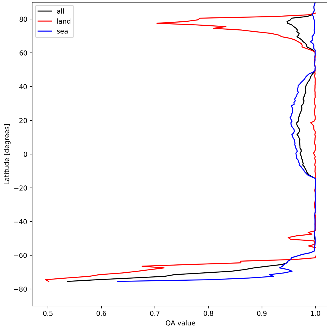
Figure 10: Zonal average of “QA value” for 2025-08-20 to 2025-08-21.
