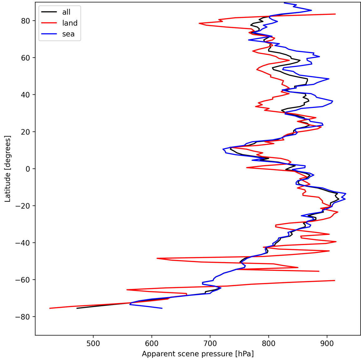
Figure 17: Zonal average of “Apparent scene pressure” for 2025-08-20 to 2025-08-21.
