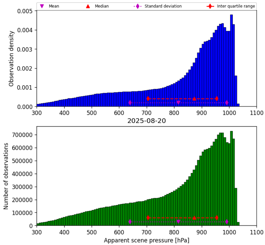
Figure 34: Histogram of “Apparent scene pressure” for 2025-08-20 to 2025-08-21
