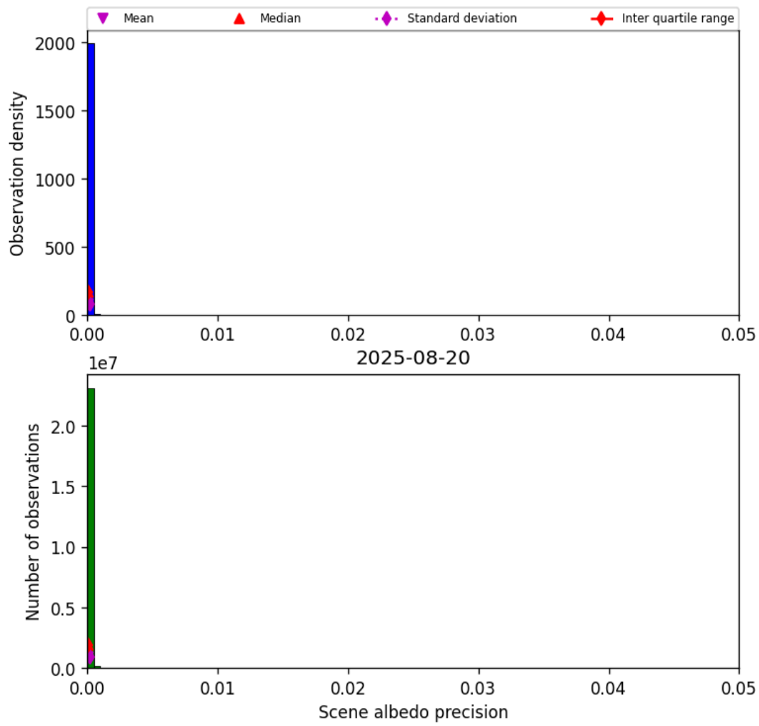
Figure 33: Histogram of “Scene albedo precision” for 2025-08-20 to 2025-08-21
