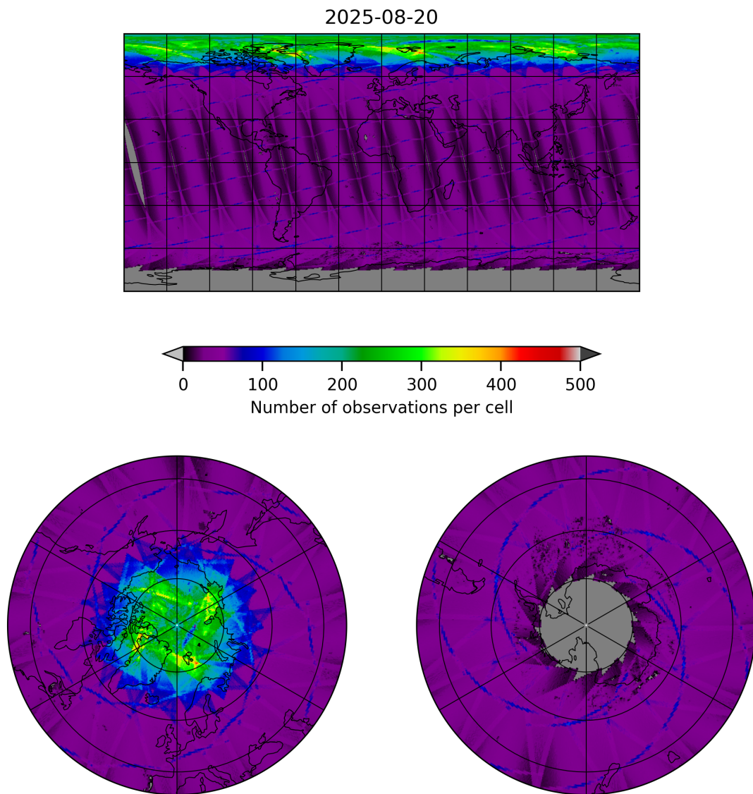
Figure 9: Map of the number of observations for 2025-08-20 to 2025-08-21
