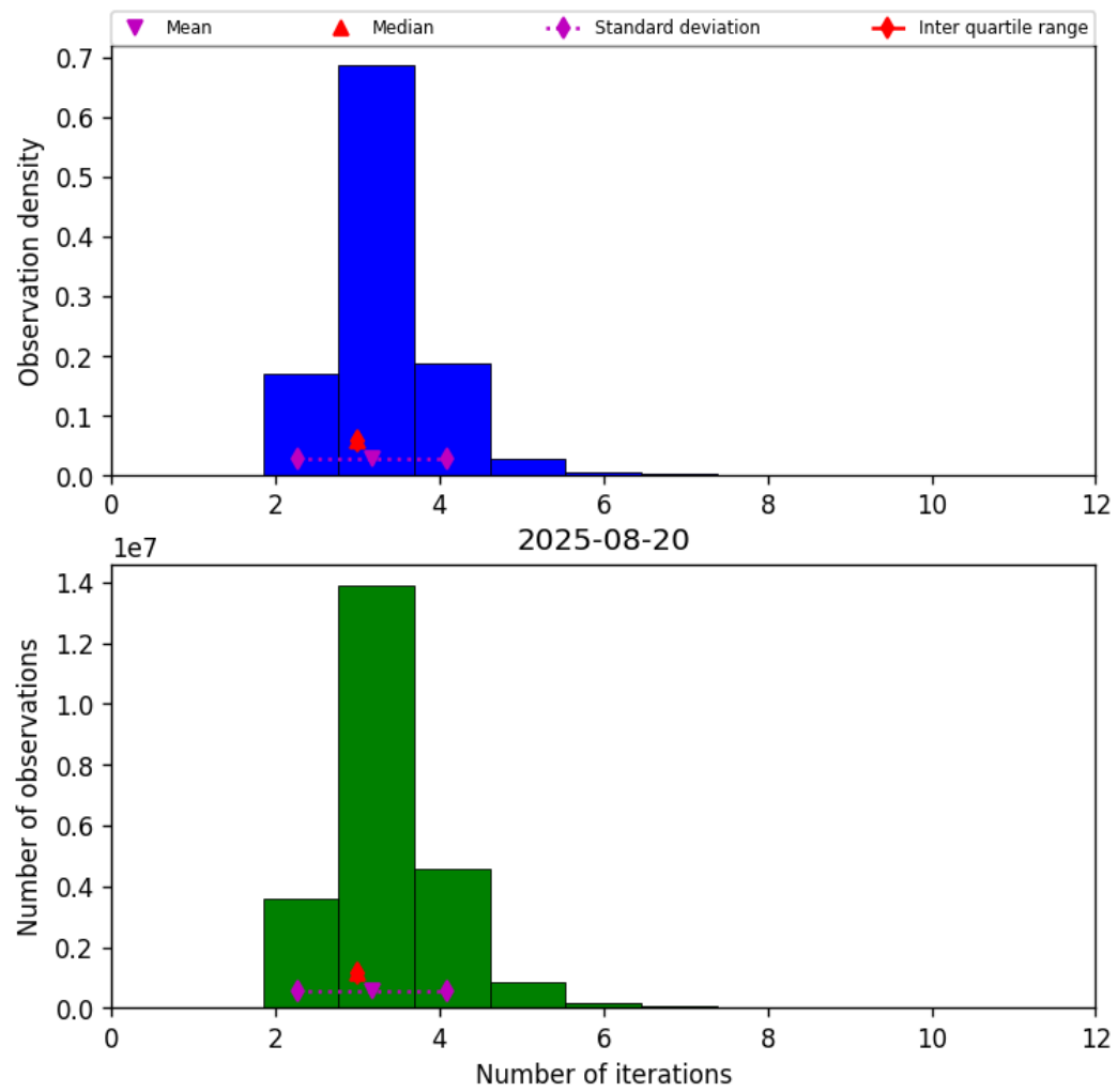
Figure 37: Histogram of “Number of iterations” for 2025-08-20 to 2025-08-21
