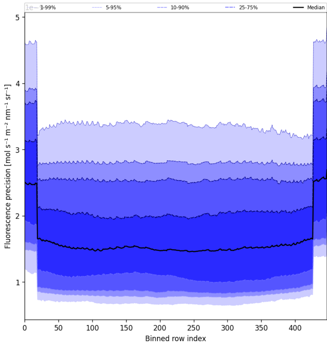
Figure 56: Along track statistics of “Fluorescence precision” for 2025-08-20 to 2025-08-21
