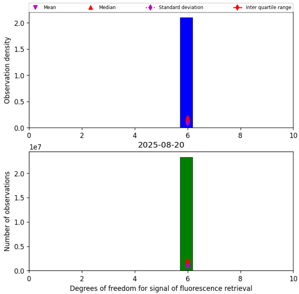
Figure 41: Histogram of “Degrees of freedom for signal of fluorescence retrieval” for 2025-08-20 to 2025-08-21
