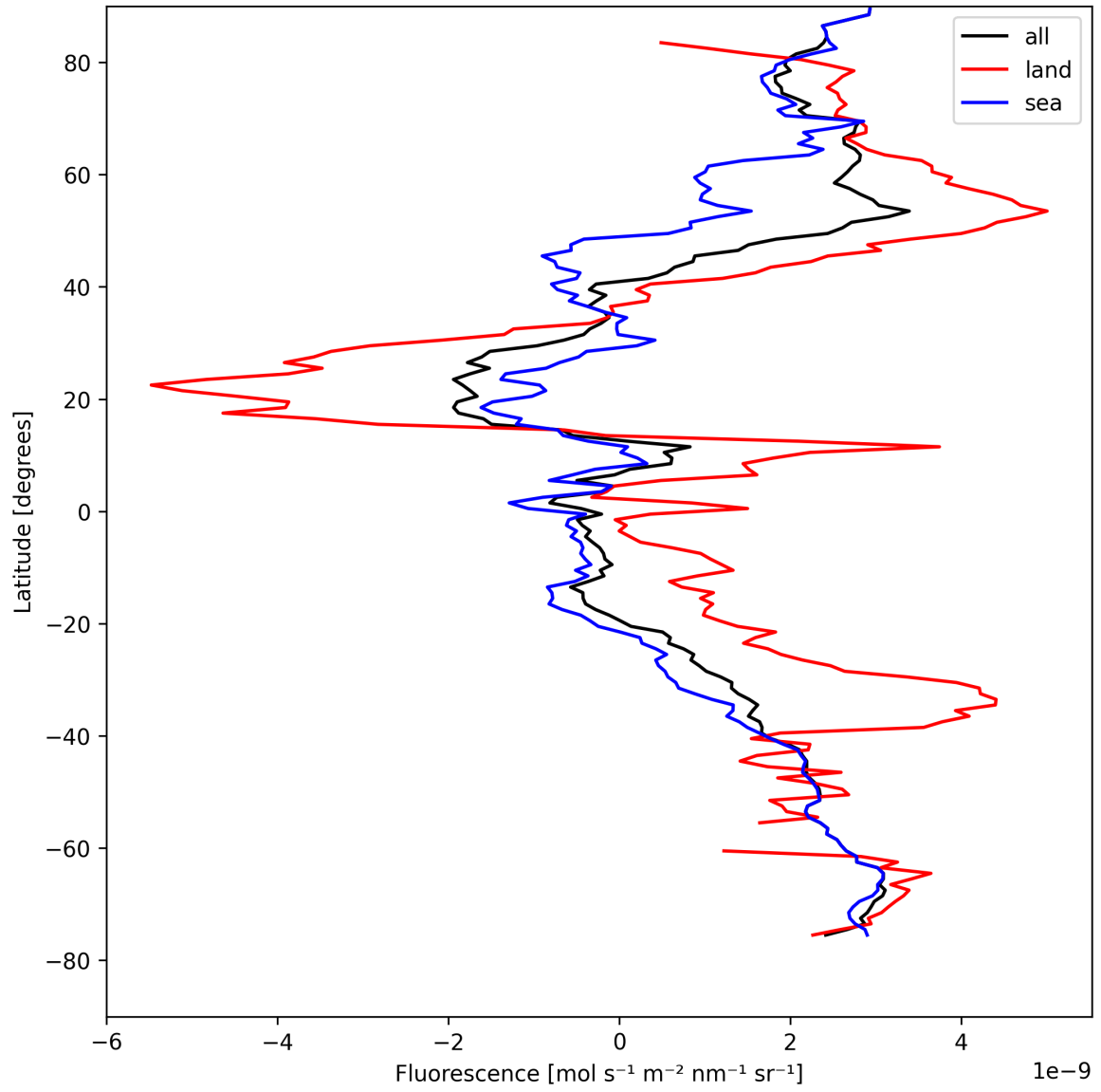
Figure 21: Zonal average of “Fluorescence” for 2025-08-20 to 2025-08-21.
