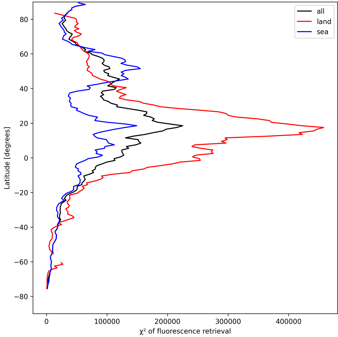
Figure 23: Zonal average of “ \chi^2 of fluorescence retrieval” for 2025-08-20 to 2025-08-21.
