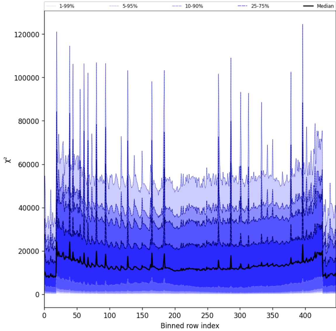
Figure 53: Along track statistics of “ \chi^2 ” for 2025-08-20 to 2025-08-21
