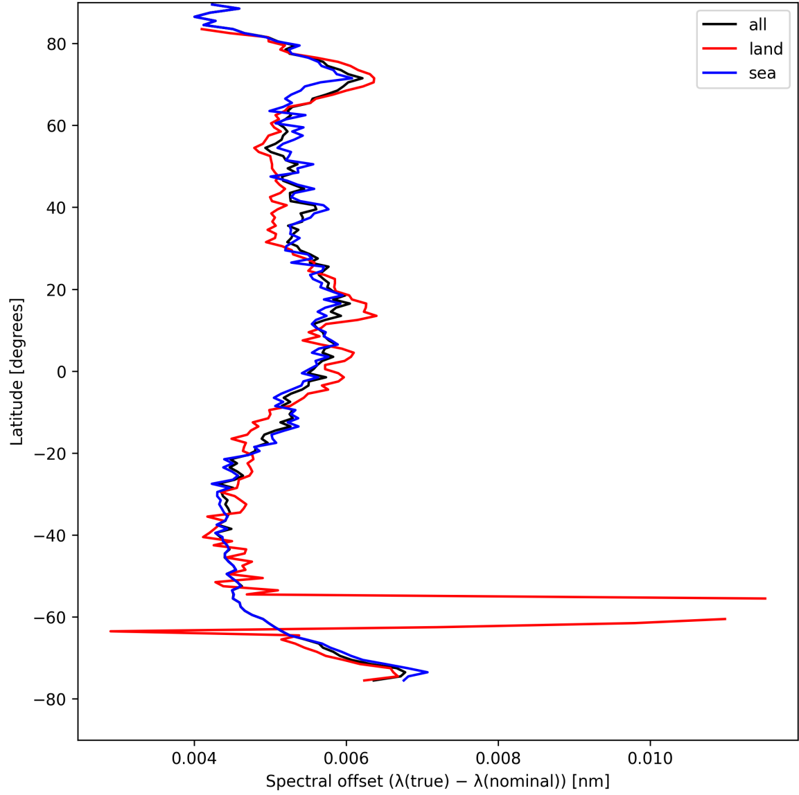
Figure 26: Zonal average of “Spectral offset ( \lambda_{\text{true}} - \lambda_{\text{nominal}} )” for 2025-08-20 to 2025-08-21.
