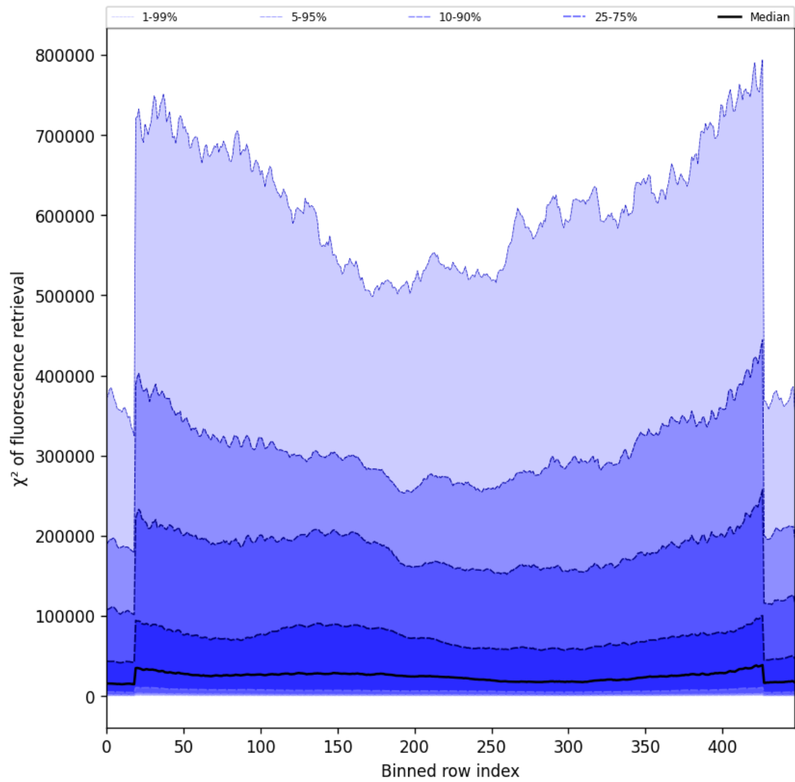
Figure 57: Along track statistics of “ \chi^2 of fluorescence retrieval” for 2025-08-20 to 2025-08-21
