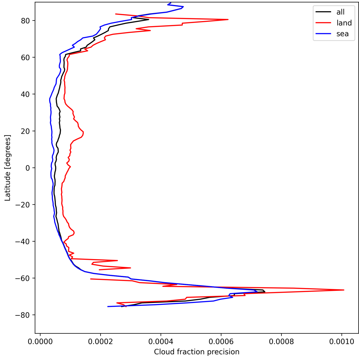
Figure 14: Zonal average of “Cloud fraction precision” for 2025-08-20 to 2025-08-21.
