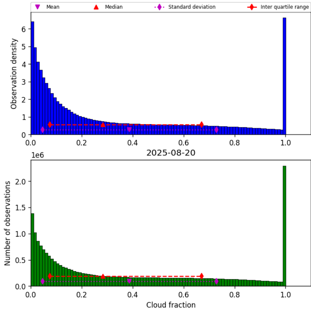
Figure 30: Histogram of “Cloud fraction” for 2025-08-20 to 2025-08-21
