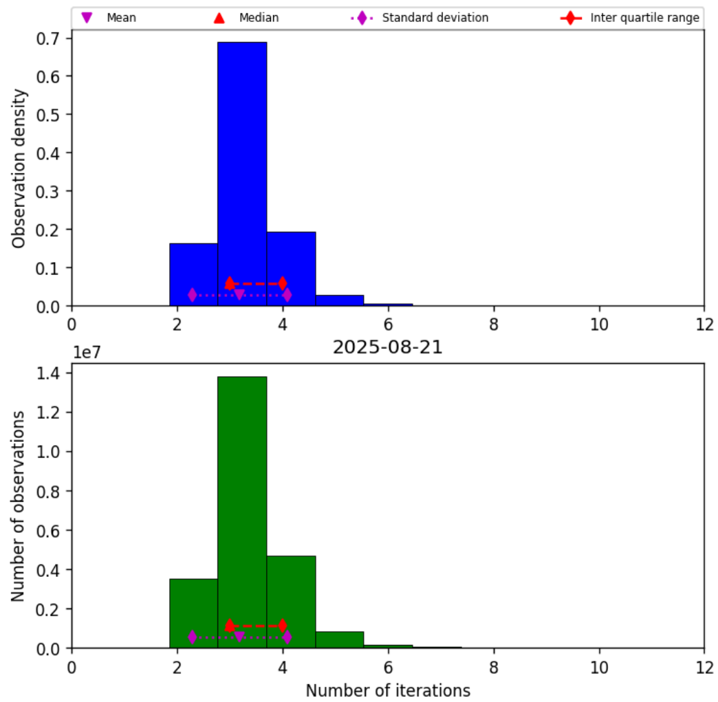
Figure 37: Histogram of “Number of iterations” for 2025-08-21 to 2025-08-22
