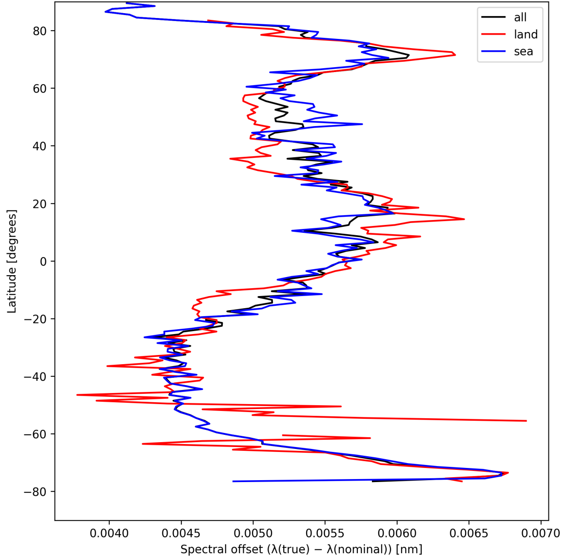
Figure 26: Zonal average of “Spectral offset ( \lambda_{\text{true}} - \lambda_{\text{nominal}} )” for 2025-08-21 to 2025-08-22.
