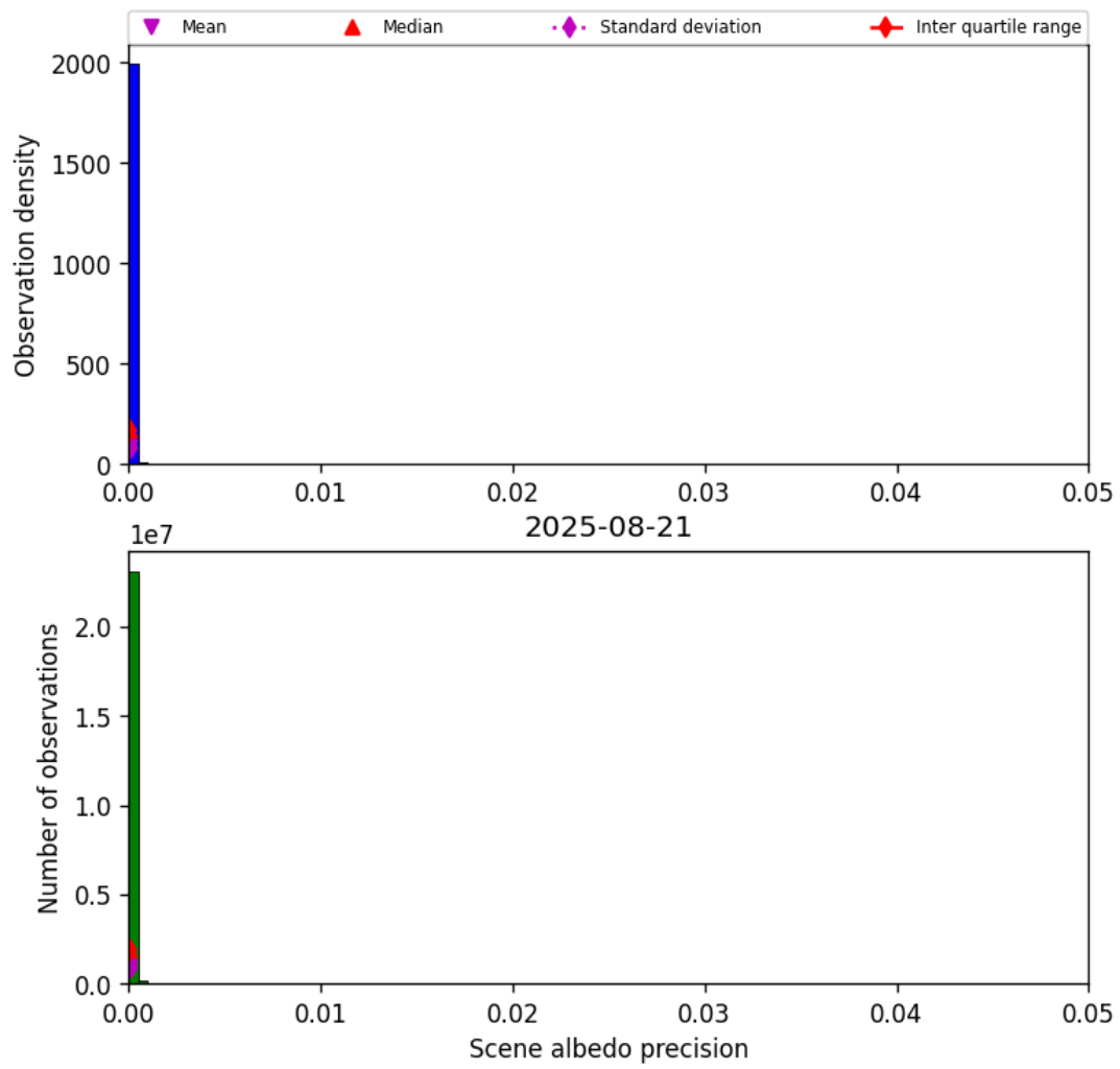
Figure 33: Histogram of “Scene albedo precision” for 2025-08-21 to 2025-08-22
