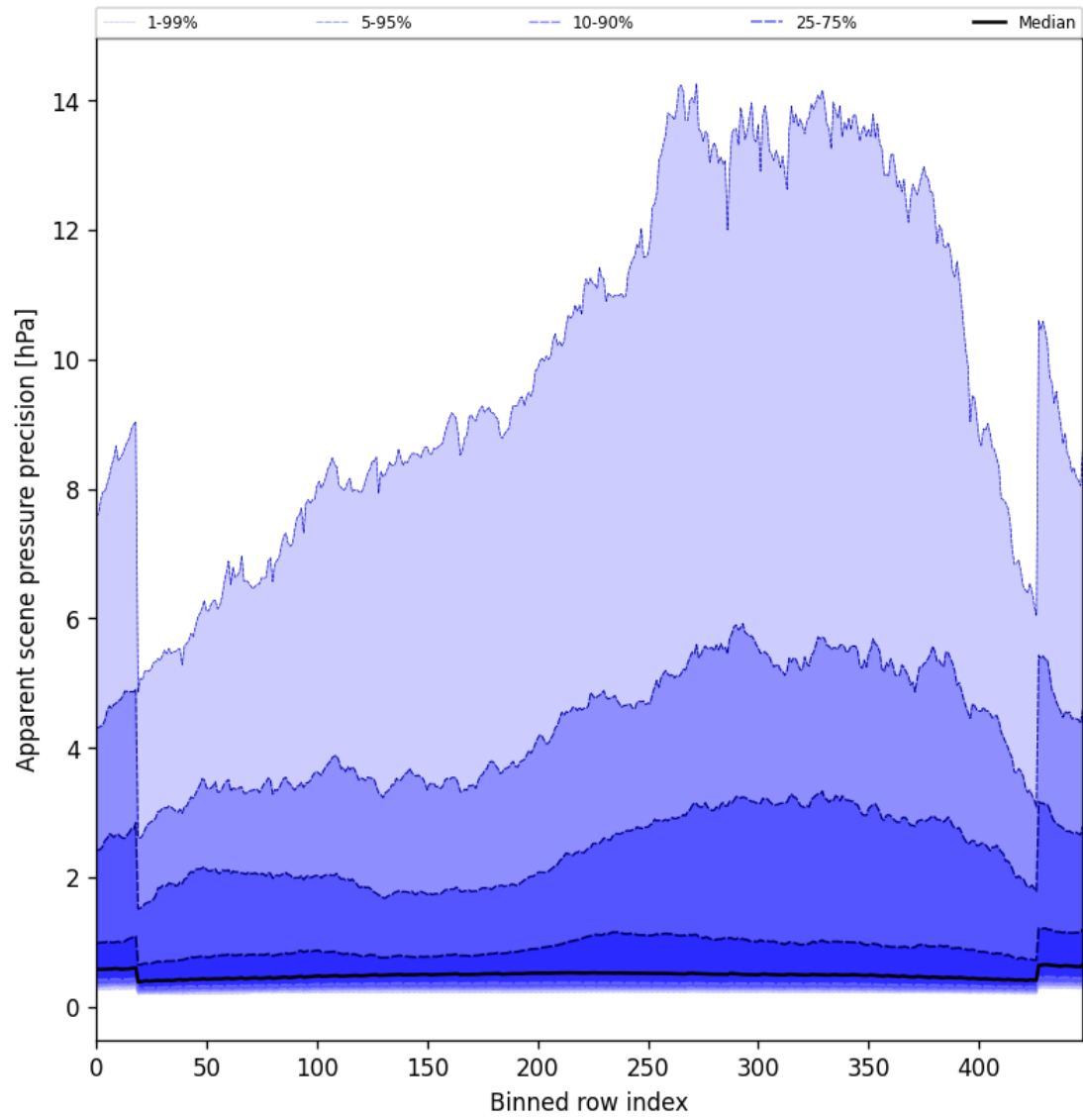
Figure 52: Along track statistics of “Apparent scene pressure precision” for 2025-08-21 to 2025-08-22
