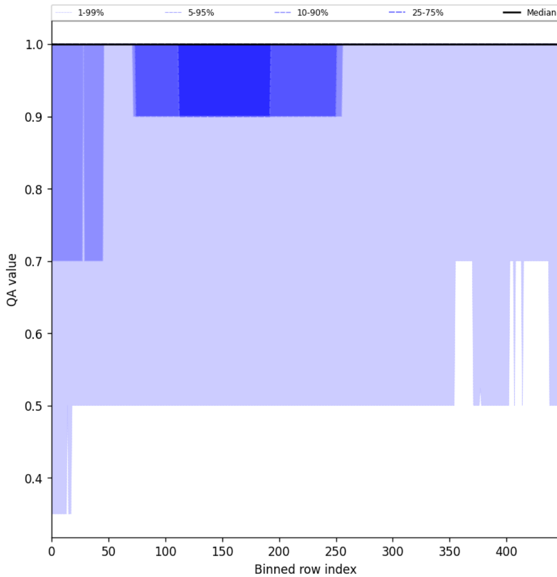
Figure 44: Along track statistics of “QA value” for 2025-08-21 to 2025-08-22
