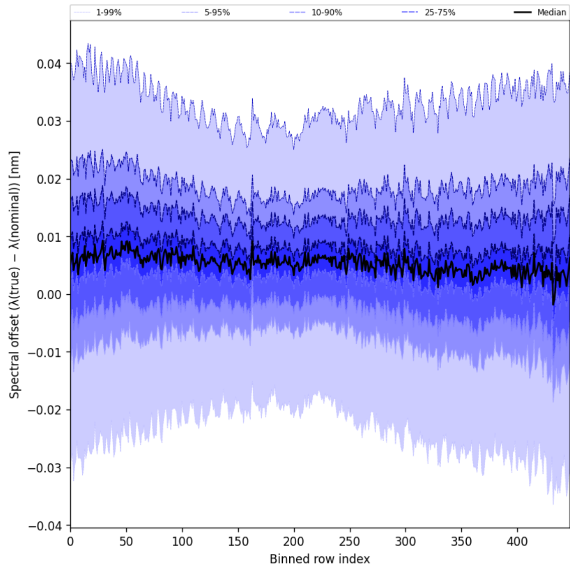
Figure 60: Along track statistics of “Spectral offset ( \lambda_{\text{true}} - \lambda_{\text{nominal}} )” for 2025-08-21 to 2025-08-22
