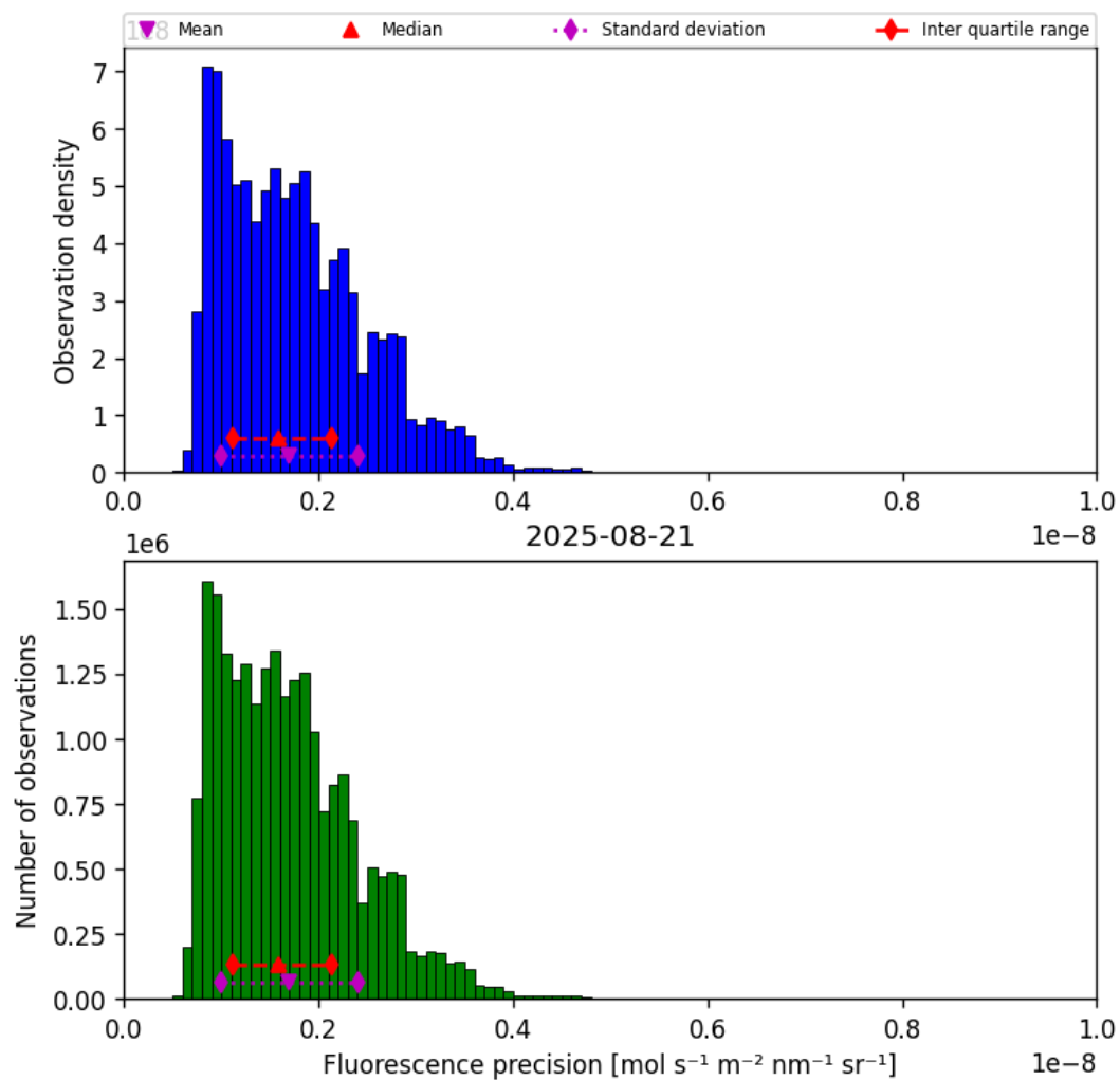
Figure 39: Histogram of “Fluorescence precision” for 2025-08-21 to 2025-08-22
