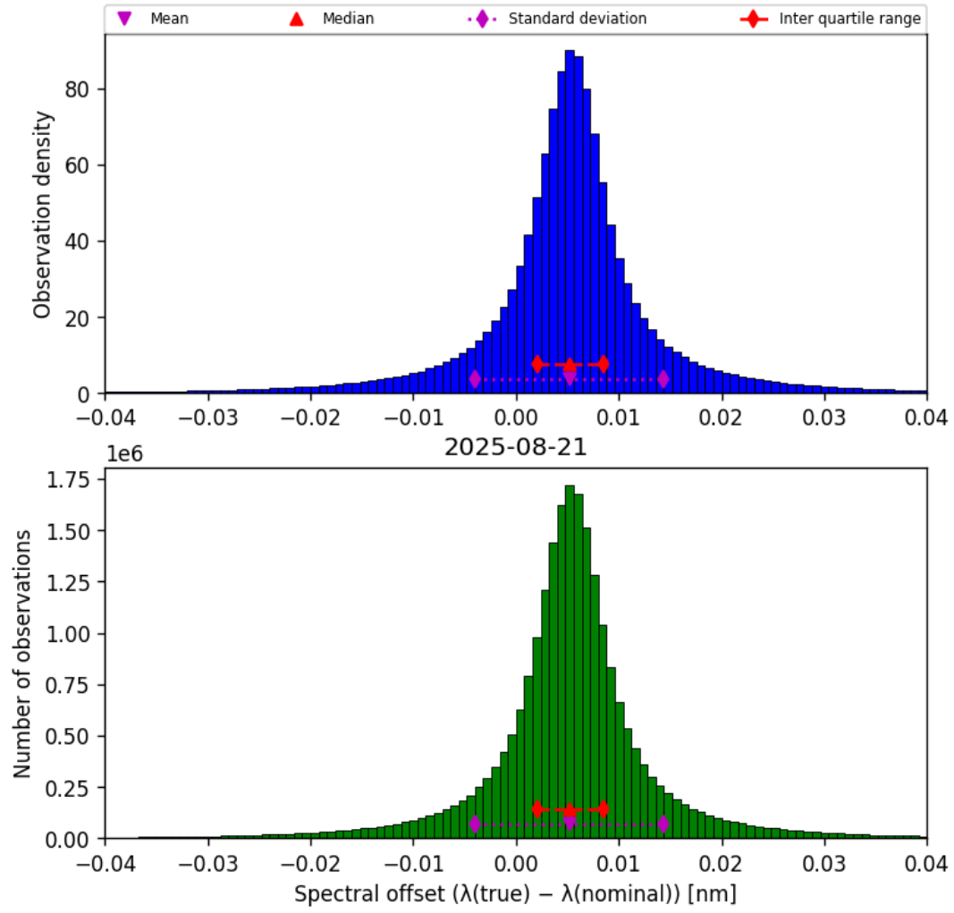
Figure 43: Histogram of “Spectral offset ( \lambda_{\text{true}} - \lambda_{\text{nominal}} )” for 2025-08-21 to 2025-08-22
