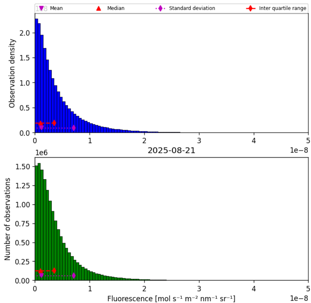
Figure 38: Histogram of “Fluorescence” for 2025-08-21 to 2025-08-22
