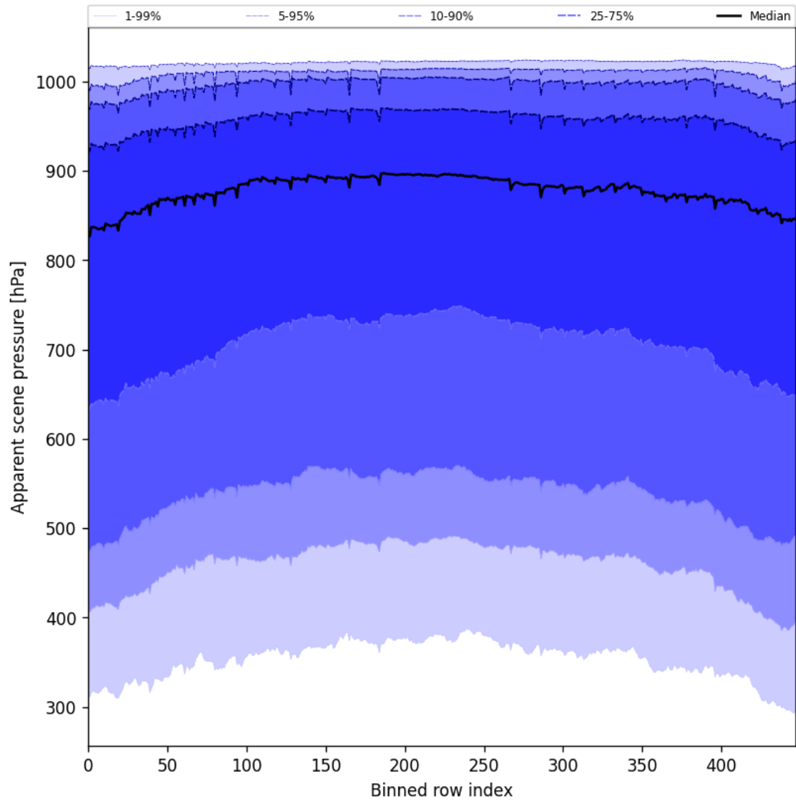
Figure 51: Along track statistics of “Apparent scene pressure” for 2025-08-21 to 2025-08-22
