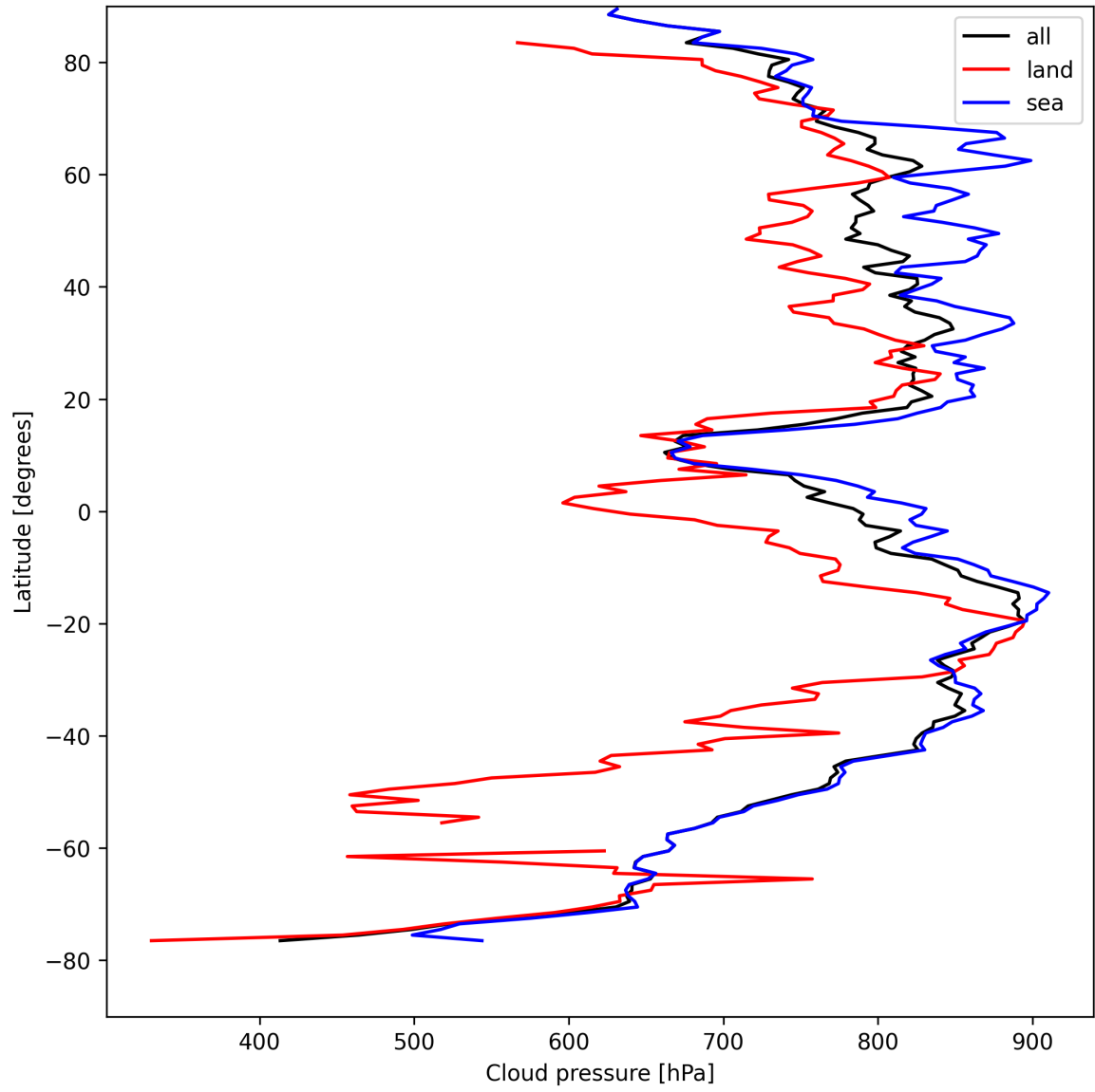
Figure 11: Zonal average of “Cloud pressure” for 2025-08-21 to 2025-08-22.
