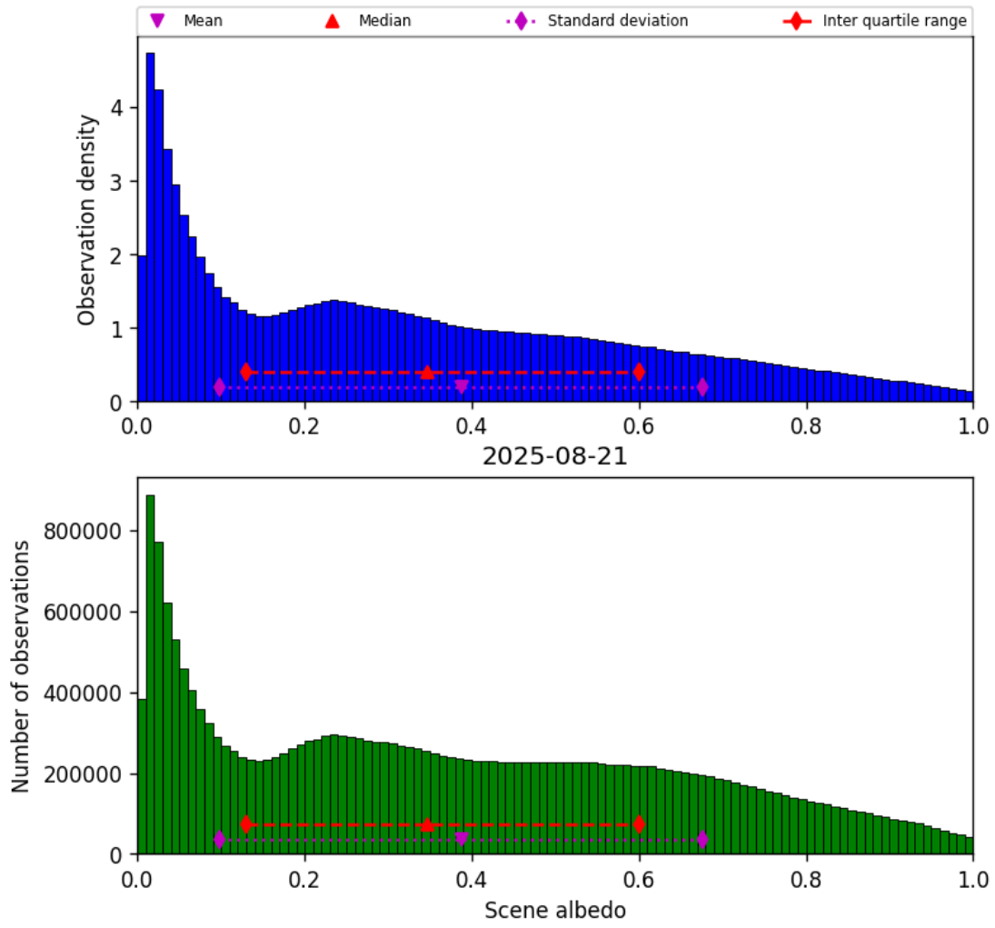
Figure 32: Histogram of “Scene albedo” for 2025-08-21 to 2025-08-22
