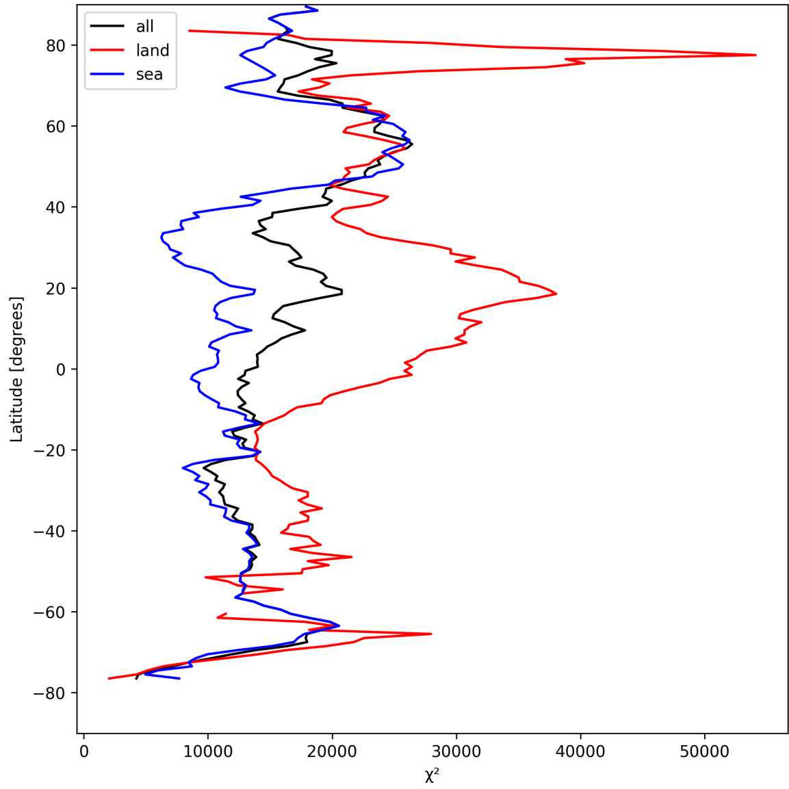
Figure 19: Zonal average of “ \chi^2 ” for 2025-08-21 to 2025-08-22.
