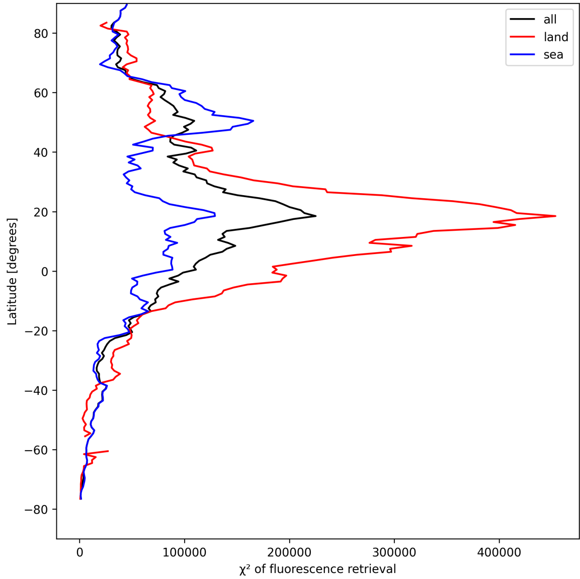
Figure 23: Zonal average of “ \chi^2 of fluorescence retrieval” for 2025-08-21 to 2025-08-22.
