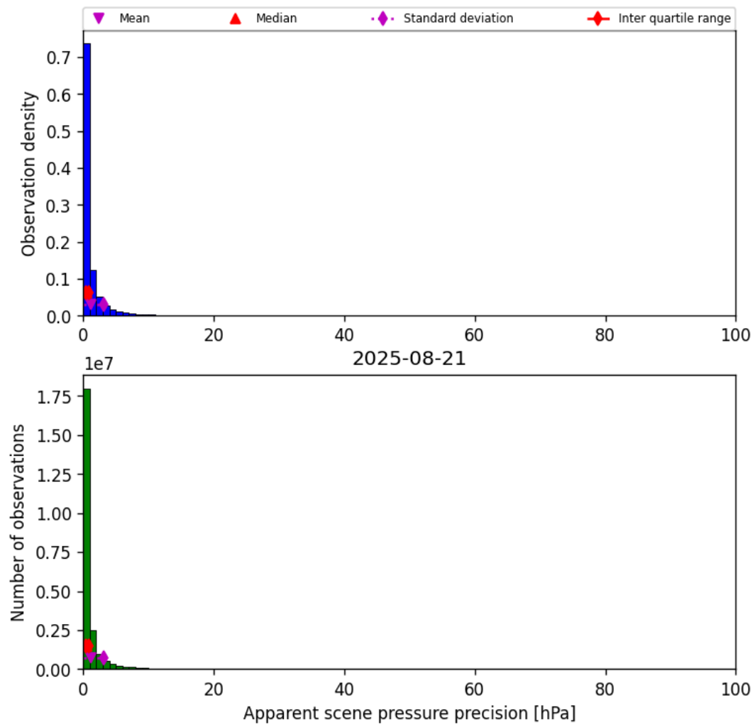
Figure 35: Histogram of “Apparent scene pressure precision” for 2025-08-21 to 2025-08-22
