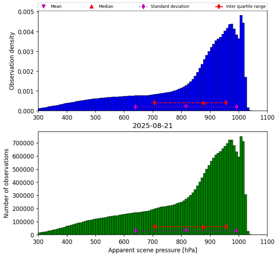
Figure 34: Histogram of “Apparent scene pressure” for 2025-08-21 to 2025-08-22
