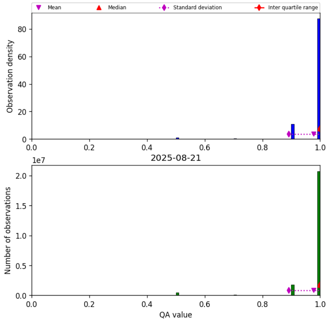
Figure 27: Histogram of “QA value” for 2025-08-21 to 2025-08-22
