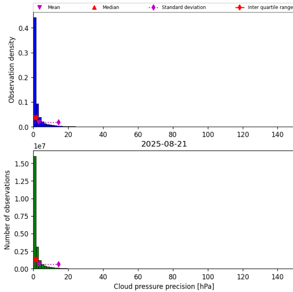
Figure 29: Histogram of “Cloud pressure precision” for 2025-08-21 to 2025-08-22
