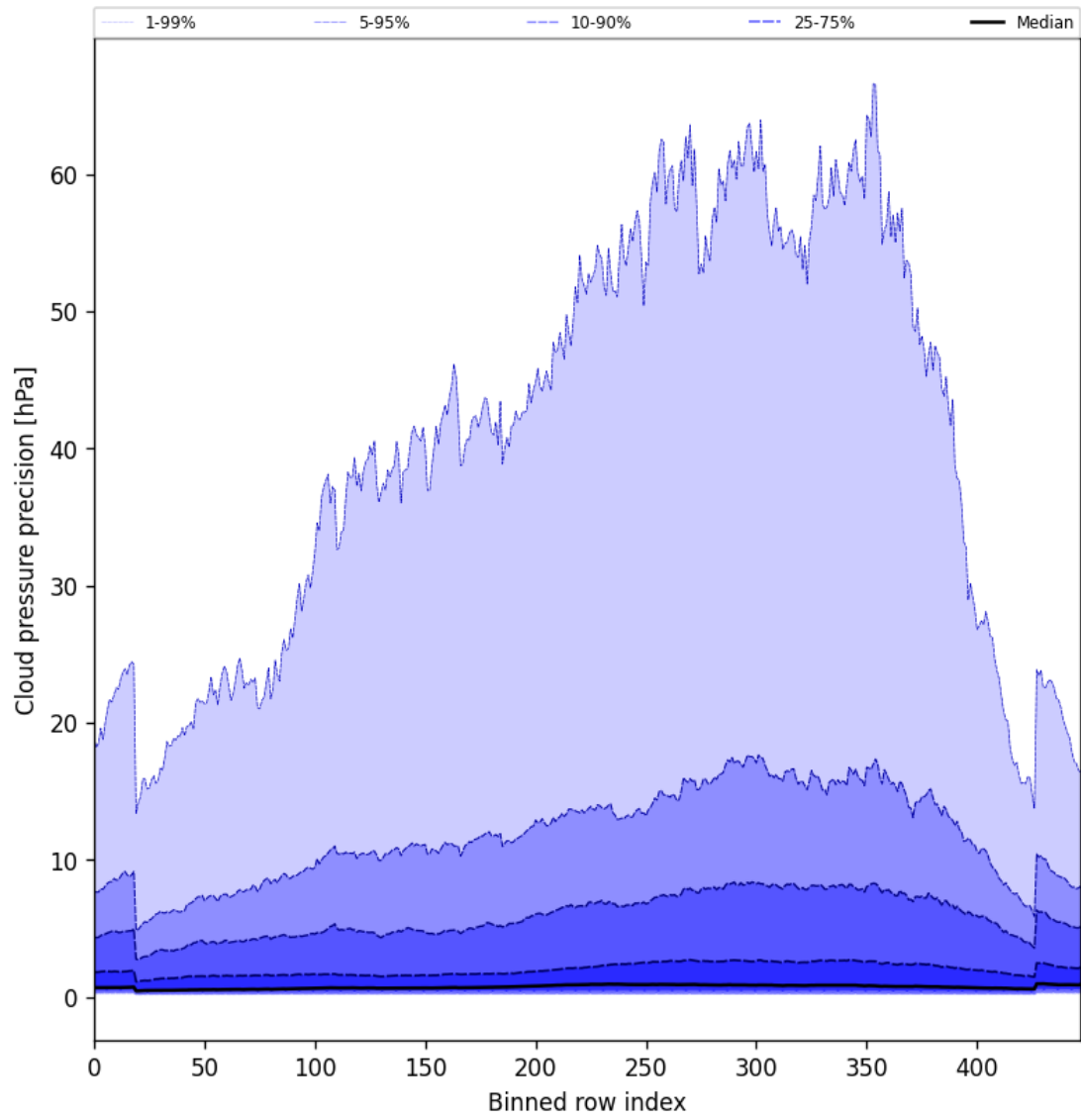
Figure 46: Along track statistics of “Cloud pressure precision” for 2025-08-21 to 2025-08-22
