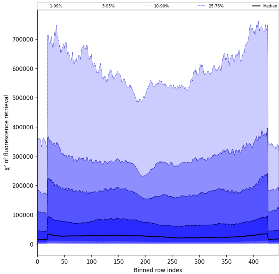
Figure 57: Along track statistics of “ \chi^2 of fluorescence retrieval” for 2025-08-21 to 2025-08-22
