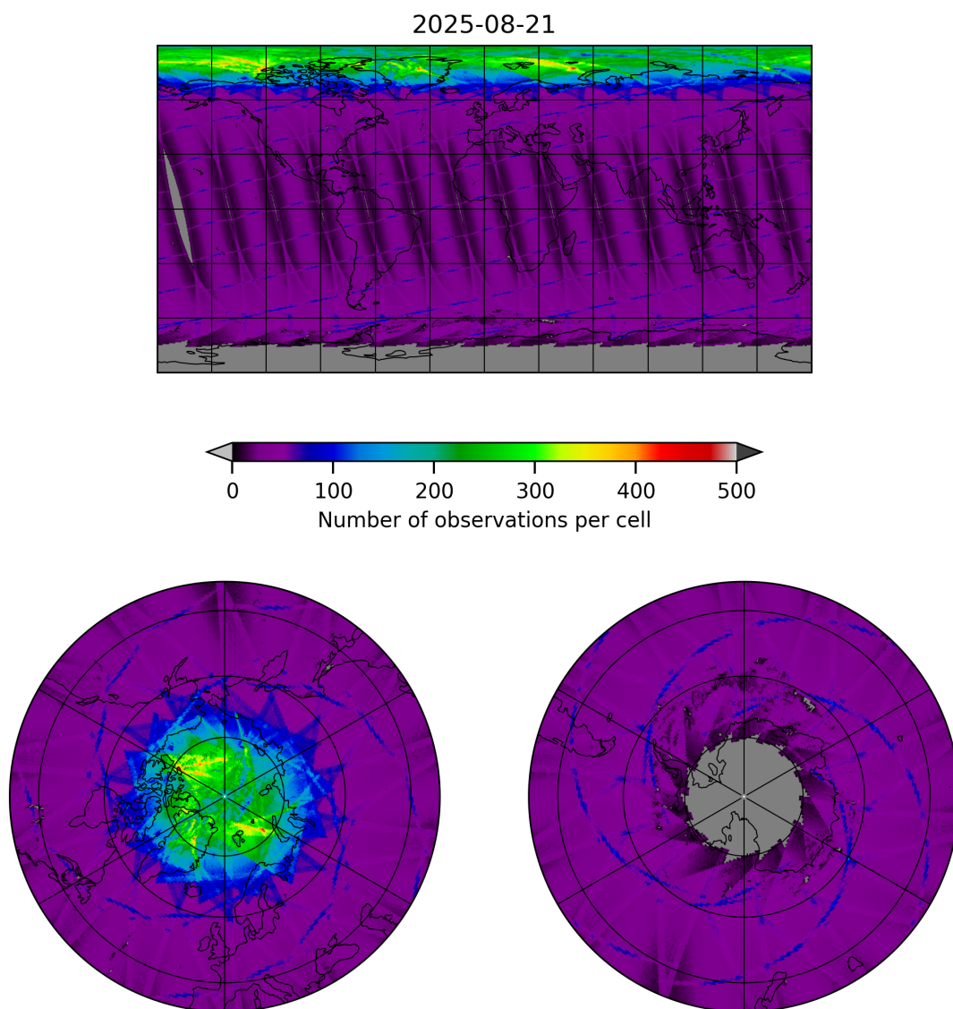
Figure 9: Map of the number of observations for 2025-08-21 to 2025-08-22
