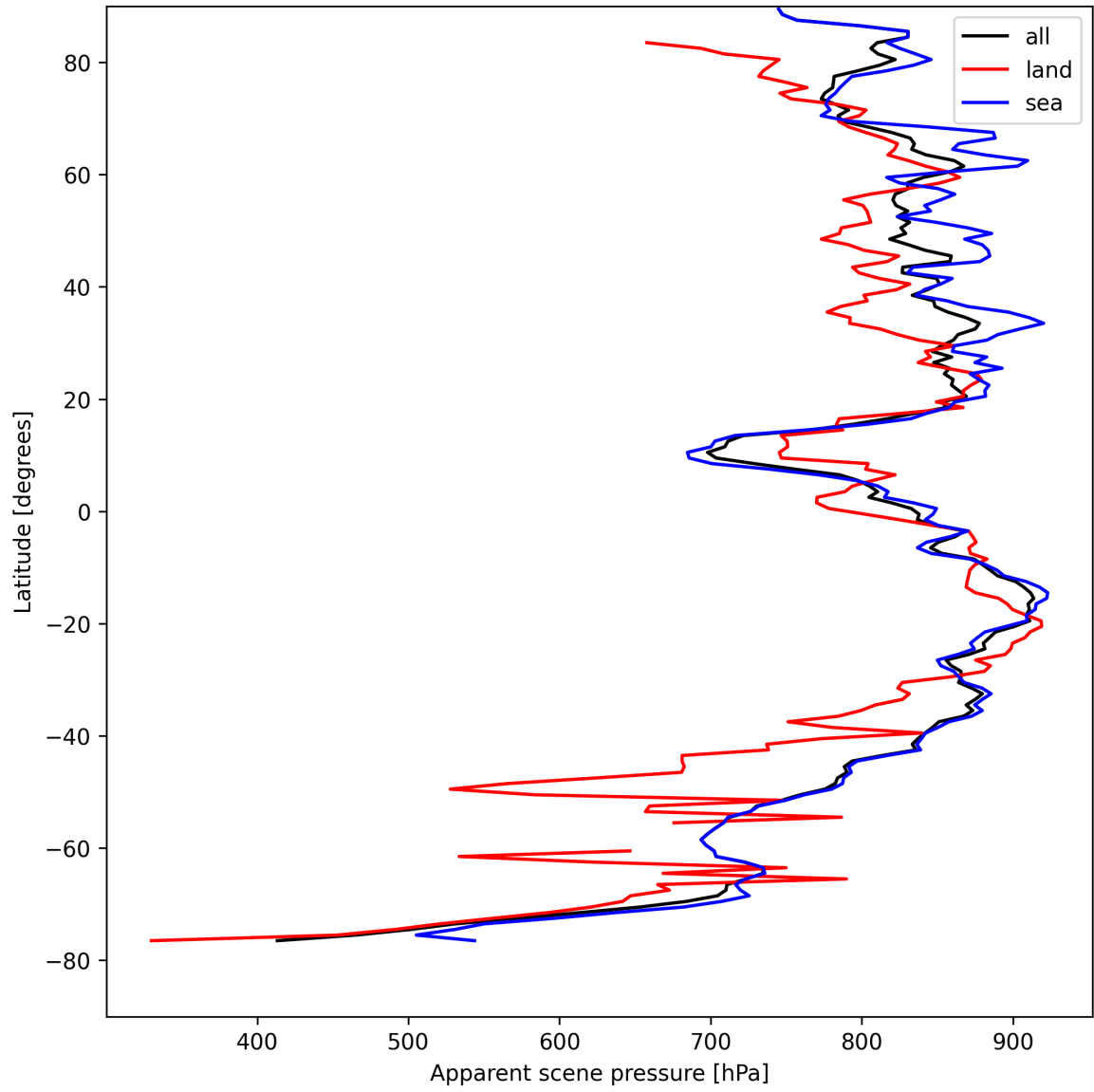
Figure 17: Zonal average of “Apparent scene pressure” for 2025-08-21 to 2025-08-22.
