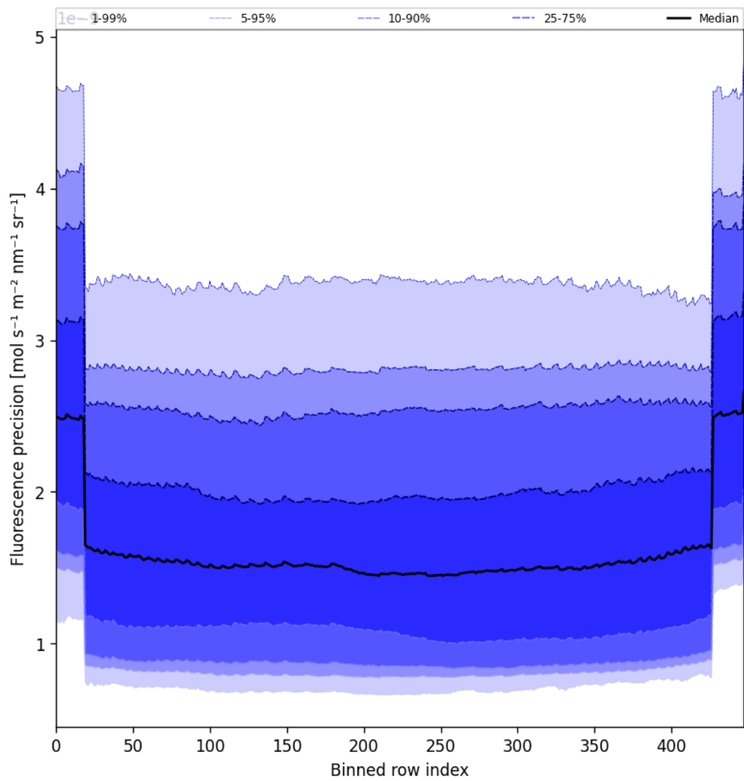
Figure 56: Along track statistics of “Fluorescence precision” for 2025-08-21 to 2025-08-22
