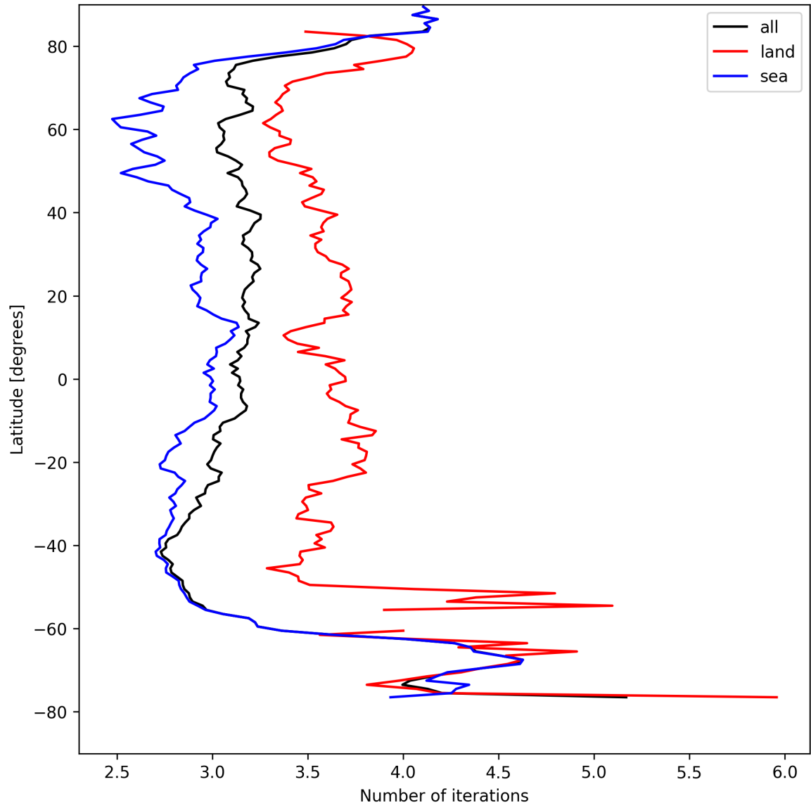
Figure 20: Zonal average of “Number of iterations” for 2025-08-21 to 2025-08-22.
