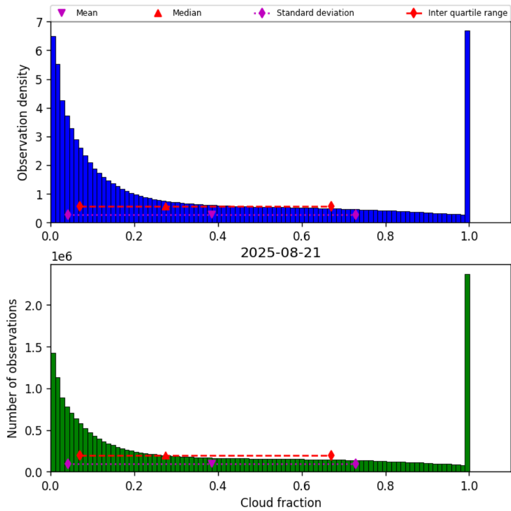
Figure 30: Histogram of “Cloud fraction” for 2025-08-21 to 2025-08-22
