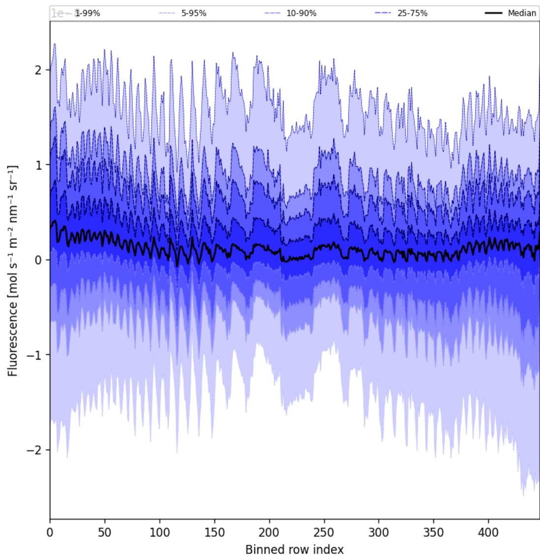
Figure 55: Along track statistics of “Fluorescence” for 2025-08-21 to 2025-08-22
