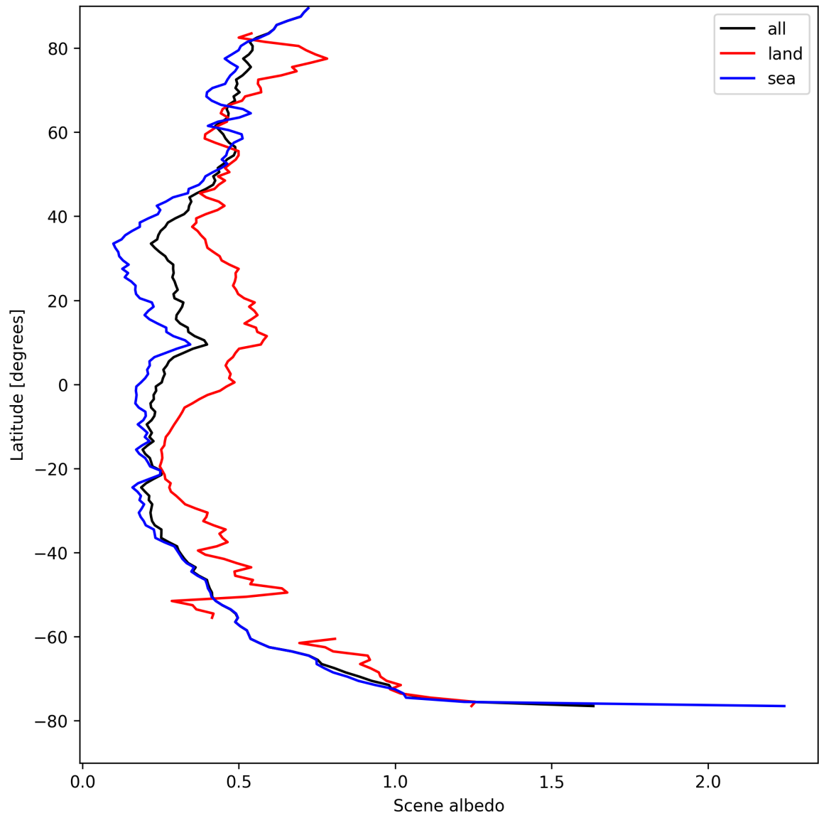
Figure 15: Zonal average of “Scene albedo” for 2025-08-21 to 2025-08-22.
