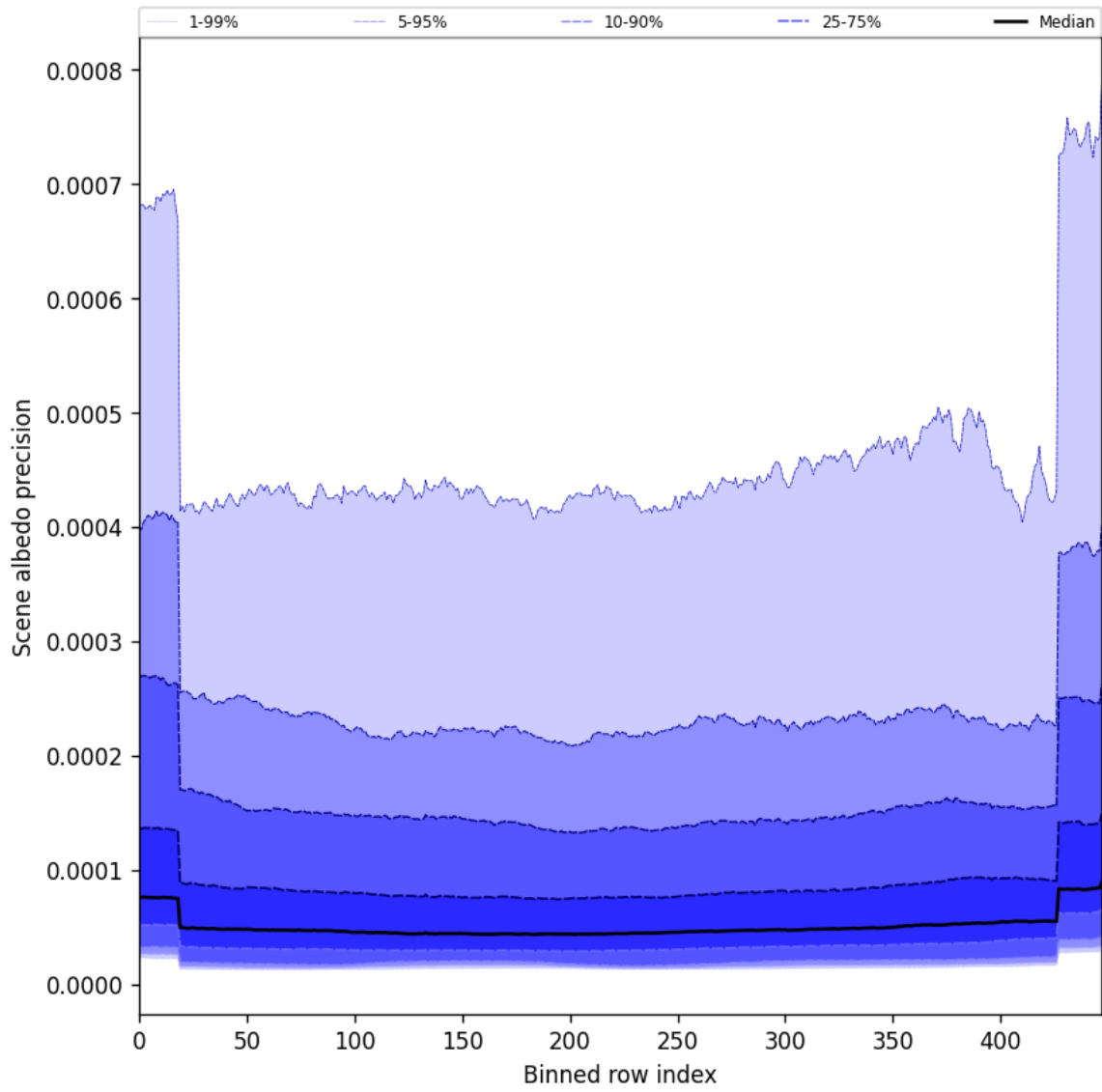
Figure 50: Along track statistics of “Scene albedo precision” for 2025-08-21 to 2025-08-22
