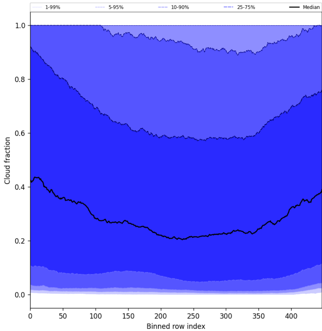
Figure 47: Along track statistics of “Cloud fraction” for 2025-08-21 to 2025-08-22
