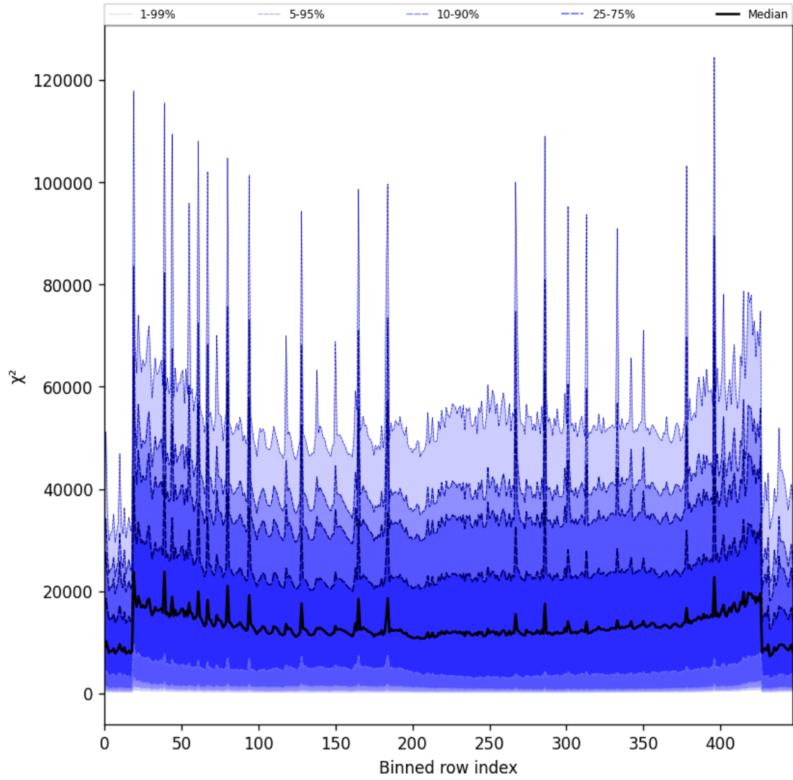
Figure 53: Along track statistics of “ \chi^2 ” for 2025-08-21 to 2025-08-22
