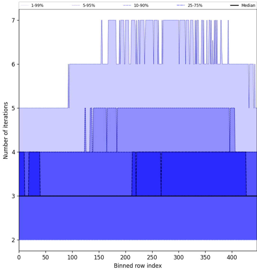
Figure 54: Along track statistics of “Number of iterations” for 2025-08-21 to 2025-08-22
