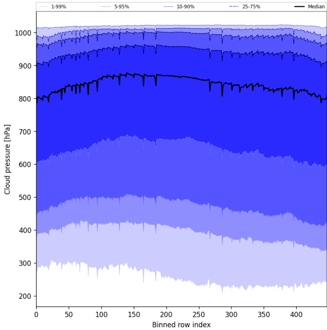
Figure 45: Along track statistics of “Cloud pressure” for 2025-08-21 to 2025-08-22
