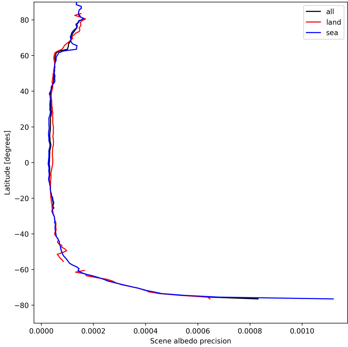
Figure 16: Zonal average of “Scene albedo precision” for 2025-08-21 to 2025-08-22.
