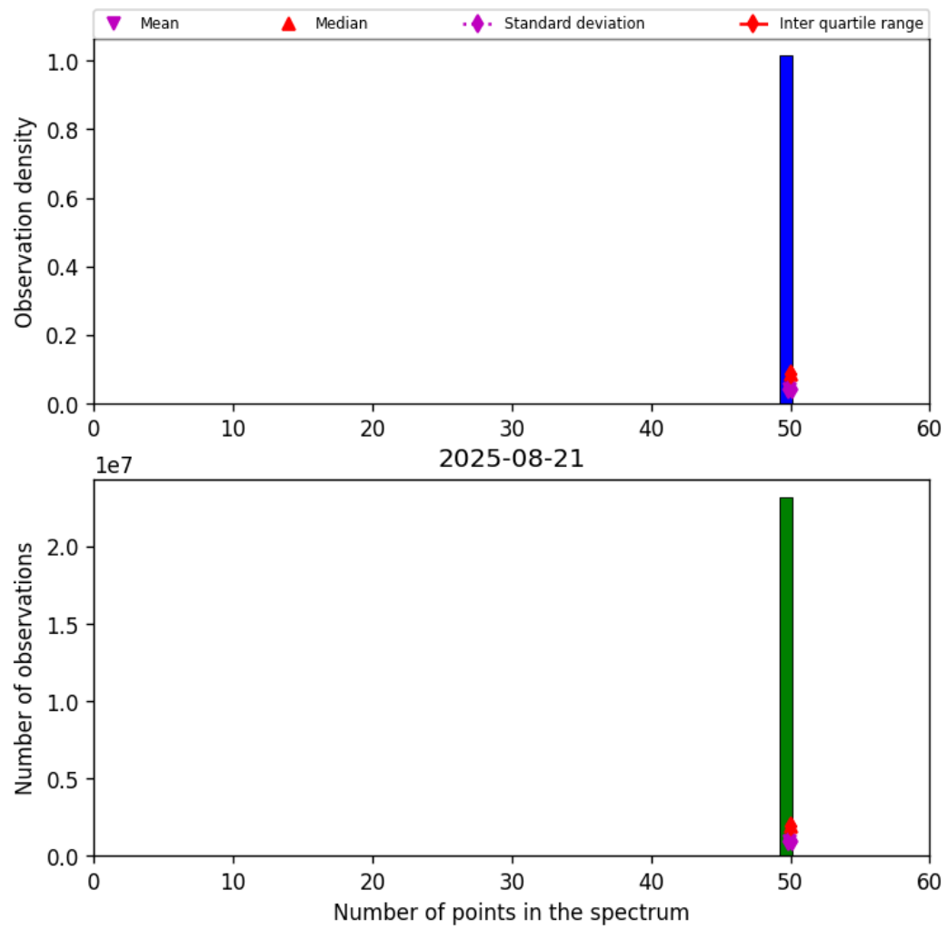
Figure 42: Histogram of “Number of points in the spectrum” for 2025-08-21 to 2025-08-22
