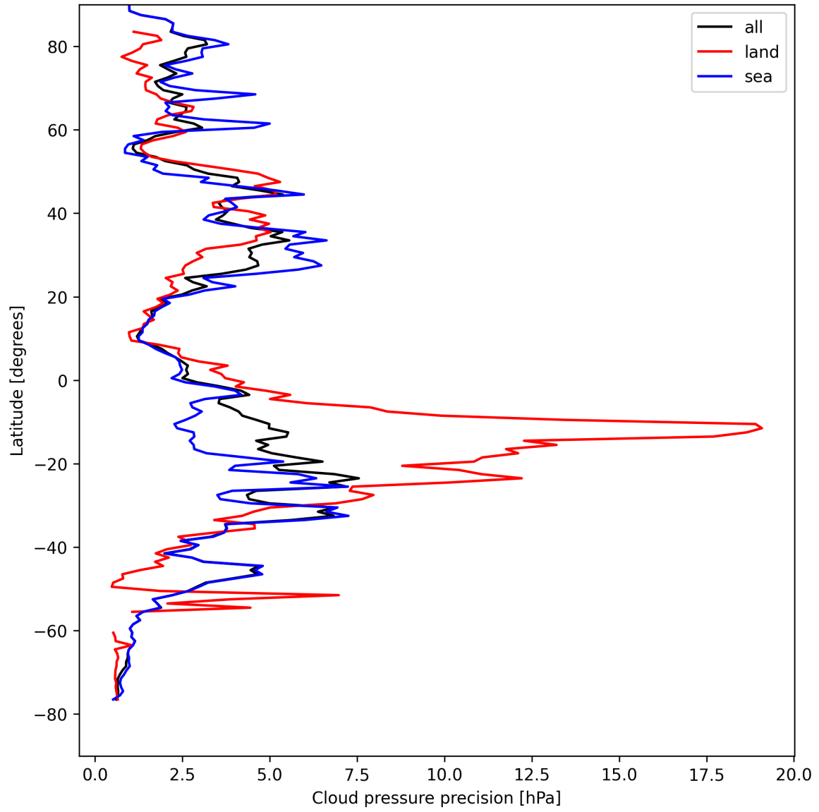
Figure 12: Zonal average of “Cloud pressure precision” for 2025-08-21 to 2025-08-22.
