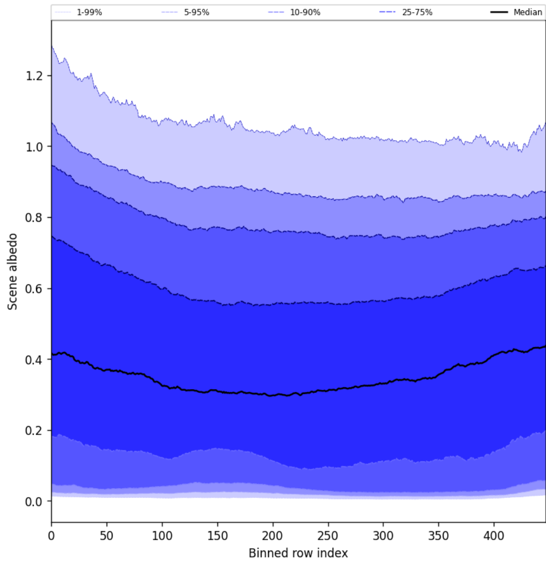
Figure 49: Along track statistics of “Scene albedo” for 2025-08-21 to 2025-08-22
