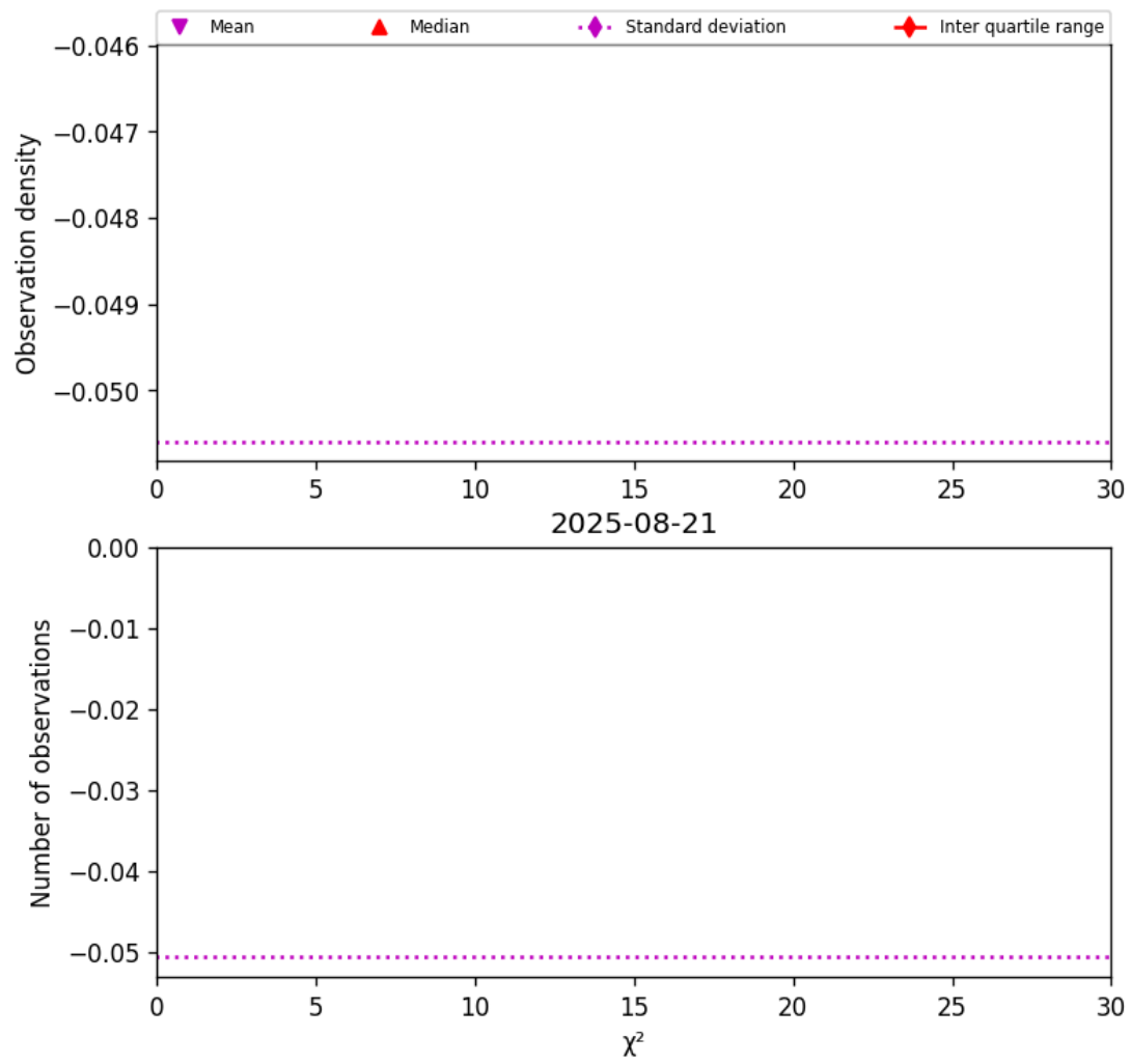
Figure 36: Histogram of “ \chi^2 ” for 2025-08-21 to 2025-08-22
