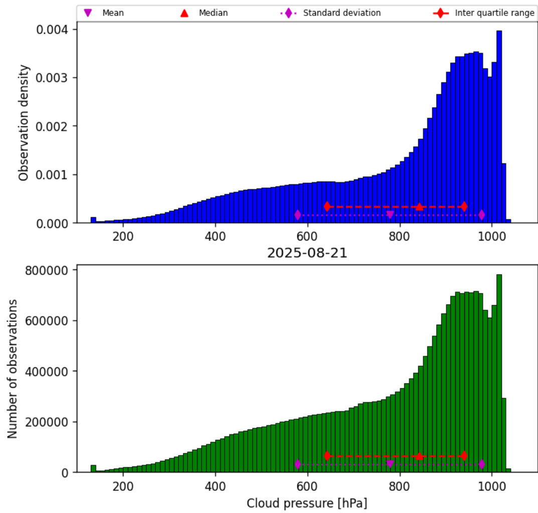
Figure 28: Histogram of “Cloud pressure” for 2025-08-21 to 2025-08-22
