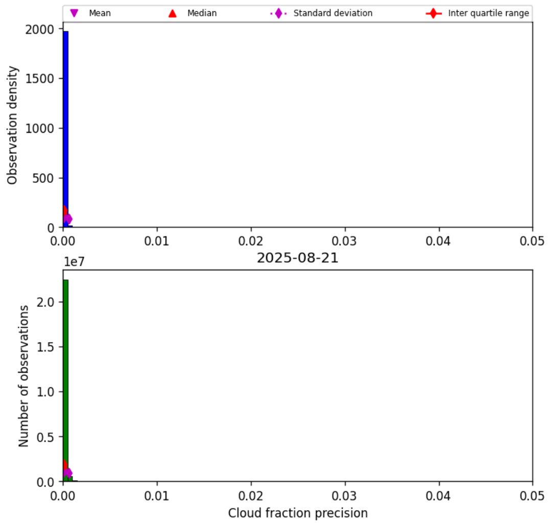
Figure 31: Histogram of “Cloud fraction precision” for 2025-08-21 to 2025-08-22
