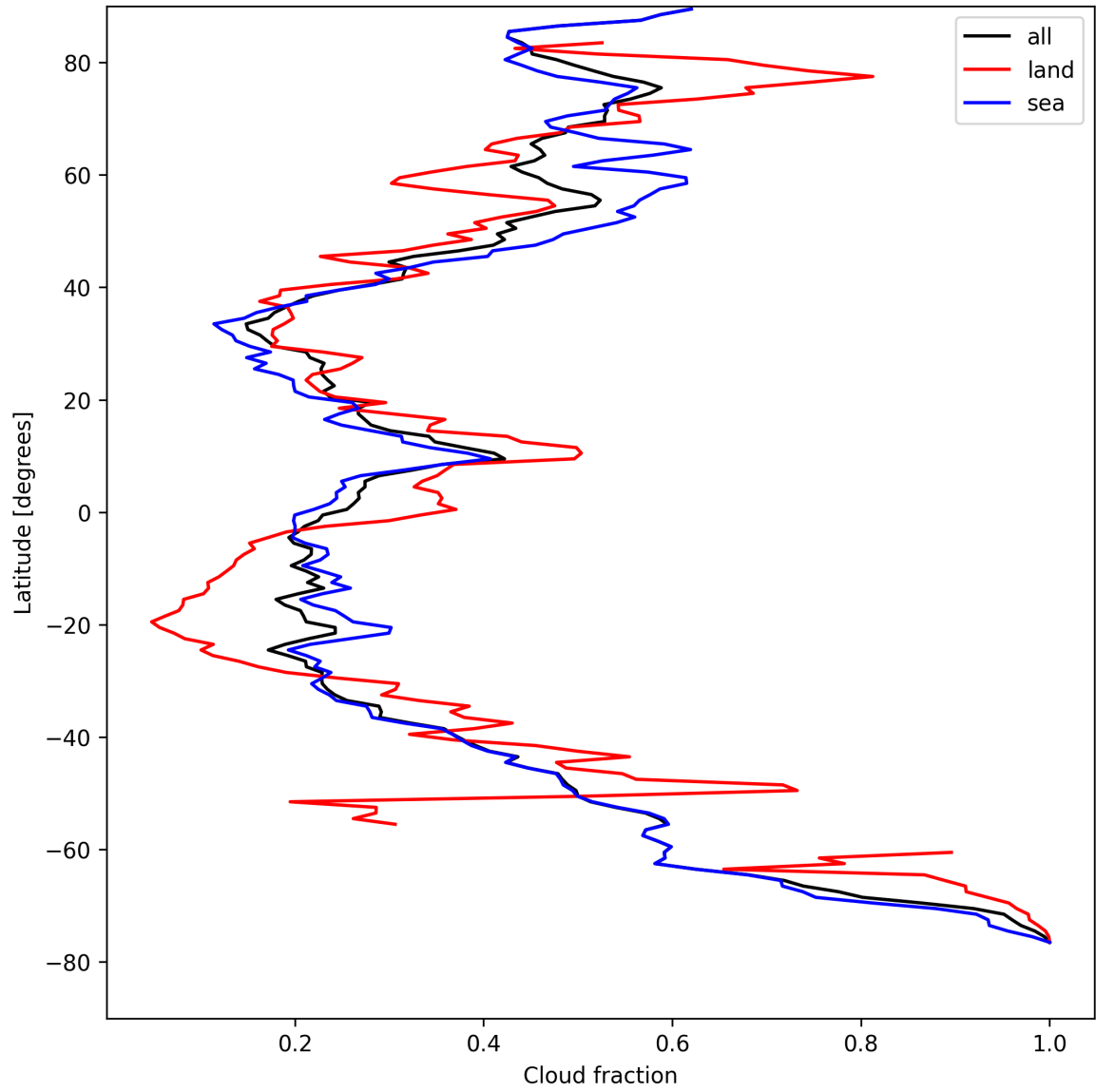
Figure 13: Zonal average of “Cloud fraction” for 2025-08-21 to 2025-08-22.
