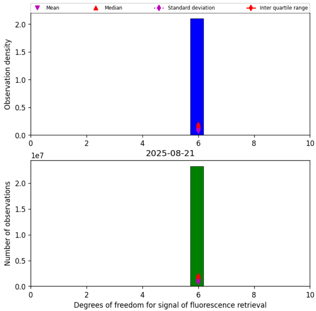
Figure 41: Histogram of “Degrees of freedom for signal of fluorescence retrieval” for 2025-08-21 to 2025-08-22
