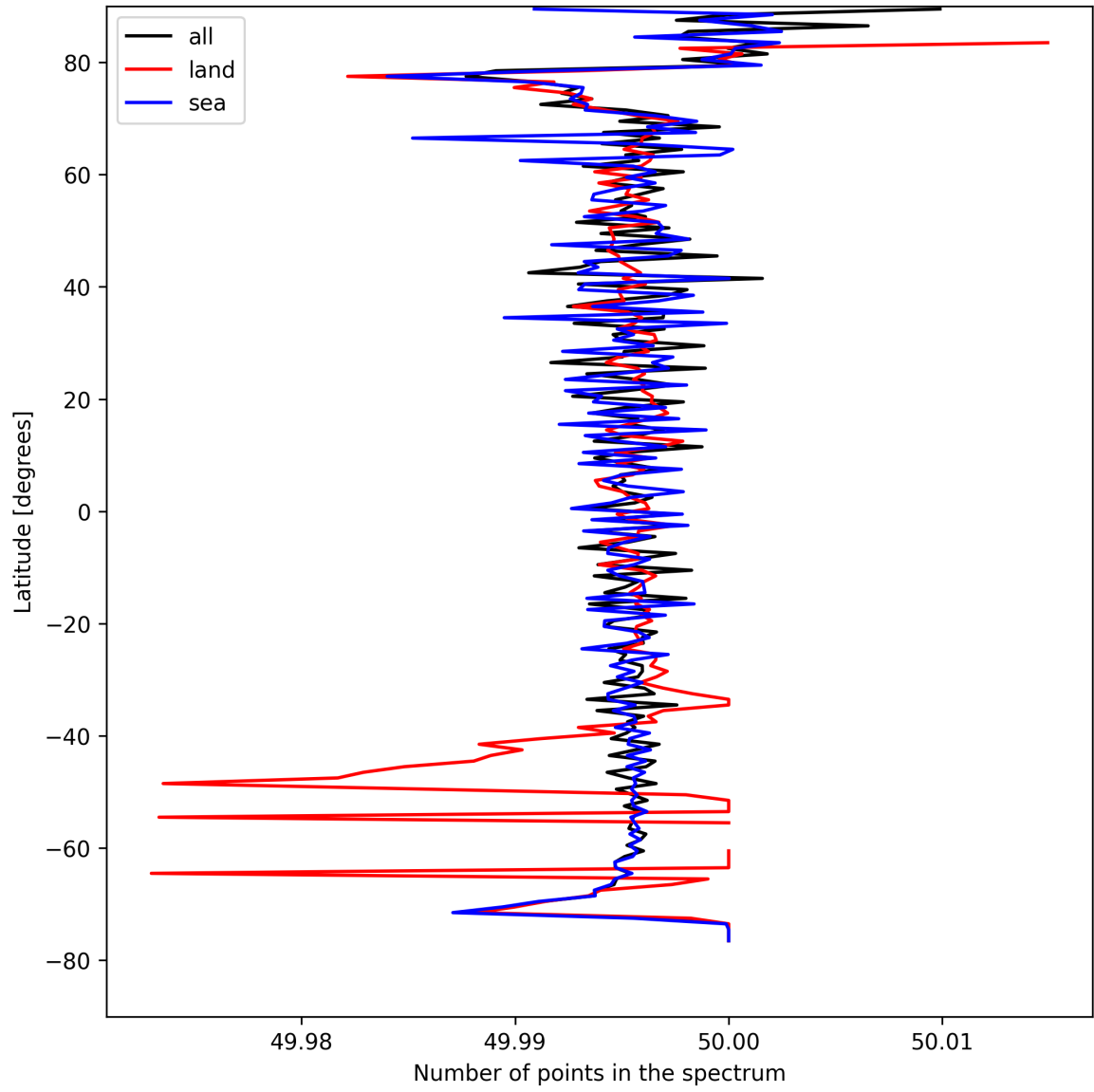
Figure 25: Zonal average of “Number of points in the spectrum” for 2025-08-21 to 2025-08-22.
