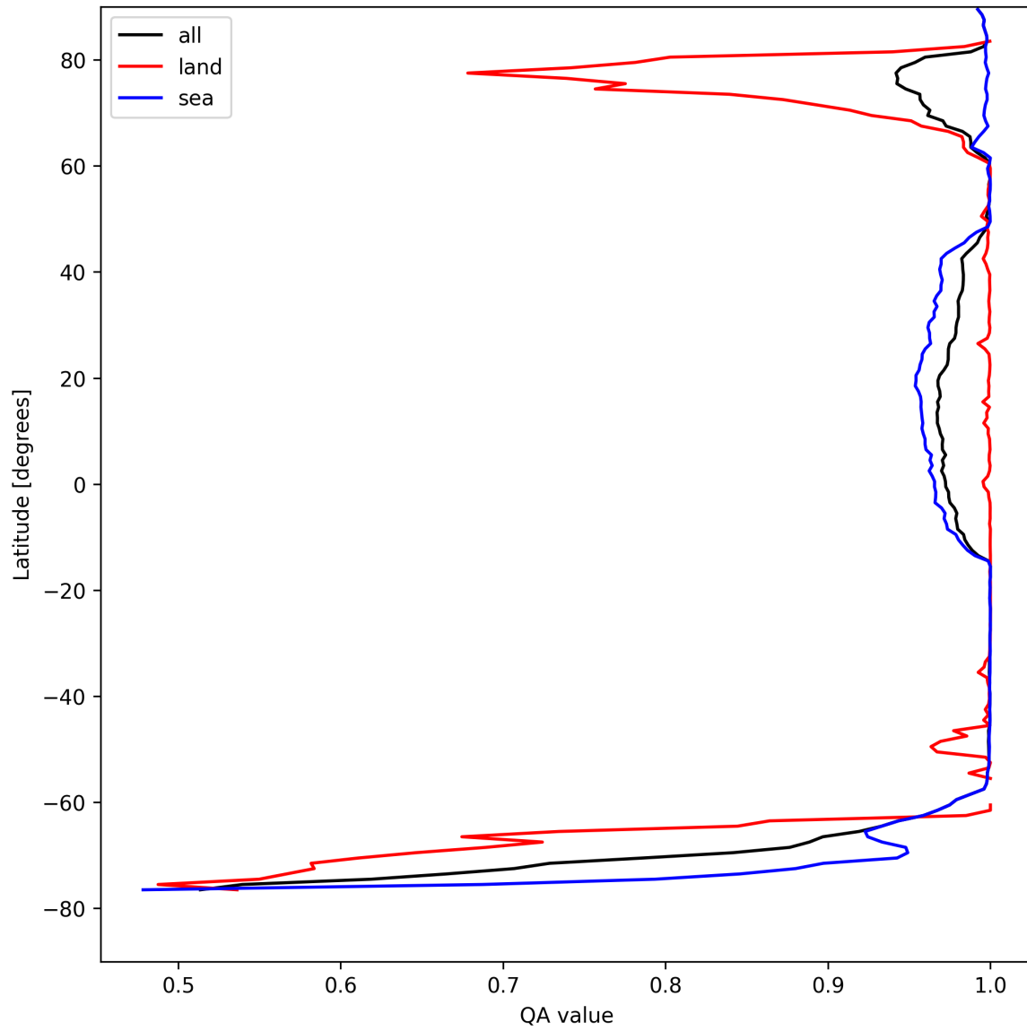
Figure 10: Zonal average of “QA value” for 2025-08-21 to 2025-08-22.
