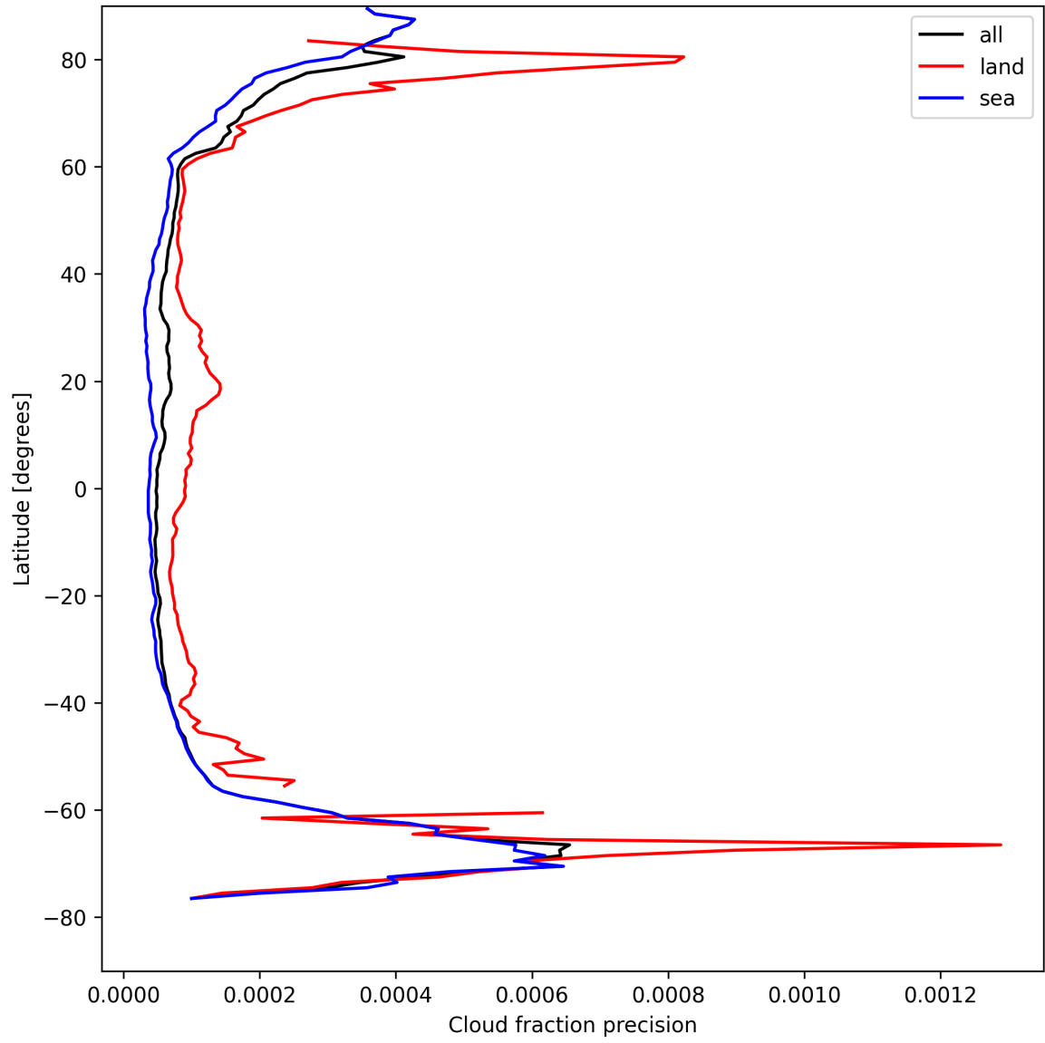
Figure 14: Zonal average of “Cloud fraction precision” for 2025-08-21 to 2025-08-22.
