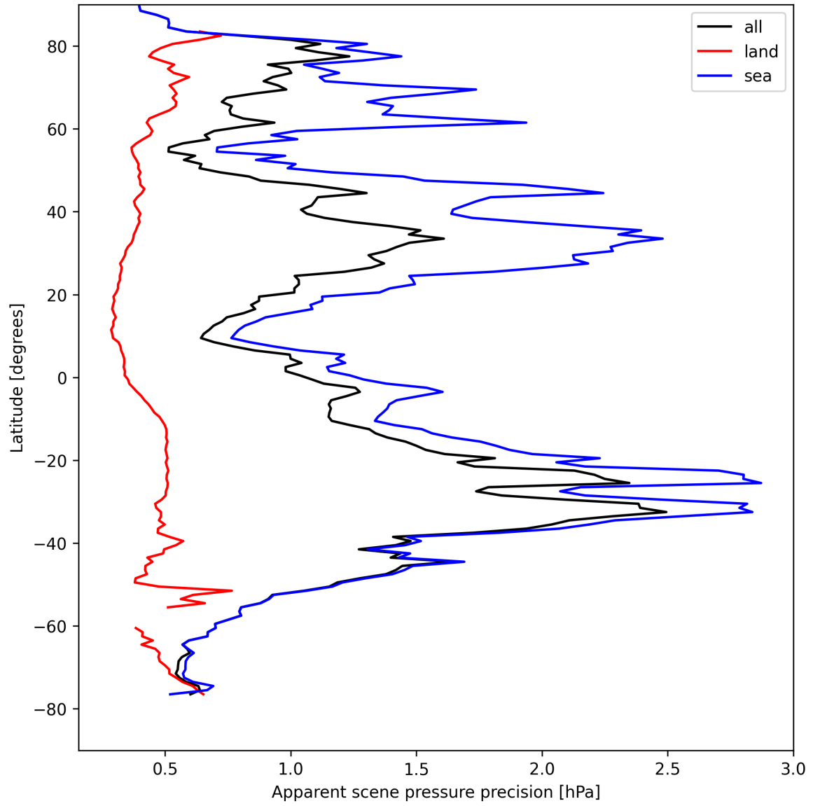
Figure 18: Zonal average of “Apparent scene pressure precision” for 2025-08-21 to 2025-08-22.
