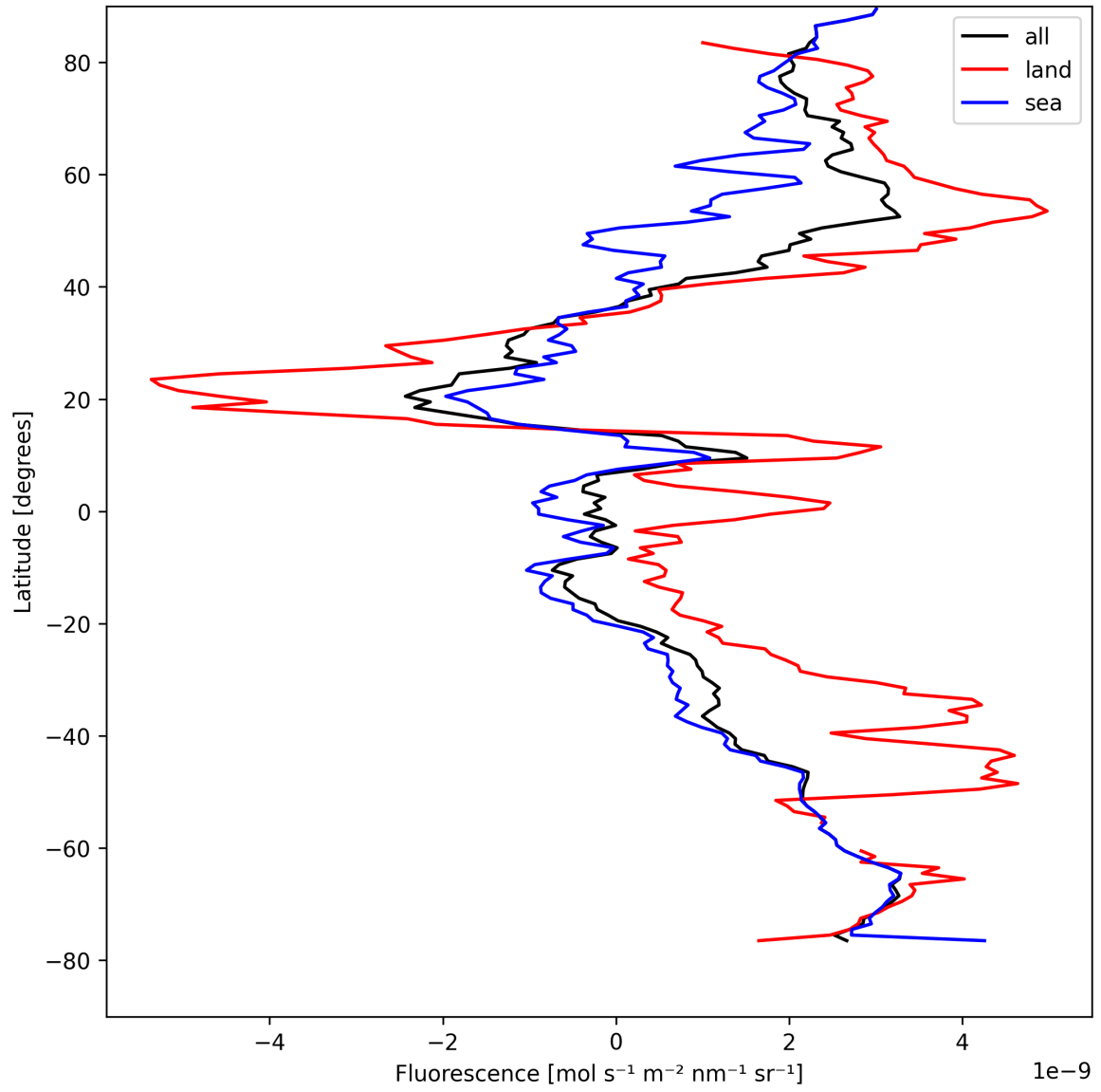
Figure 21: Zonal average of “Fluorescence” for 2025-08-21 to 2025-08-22.
