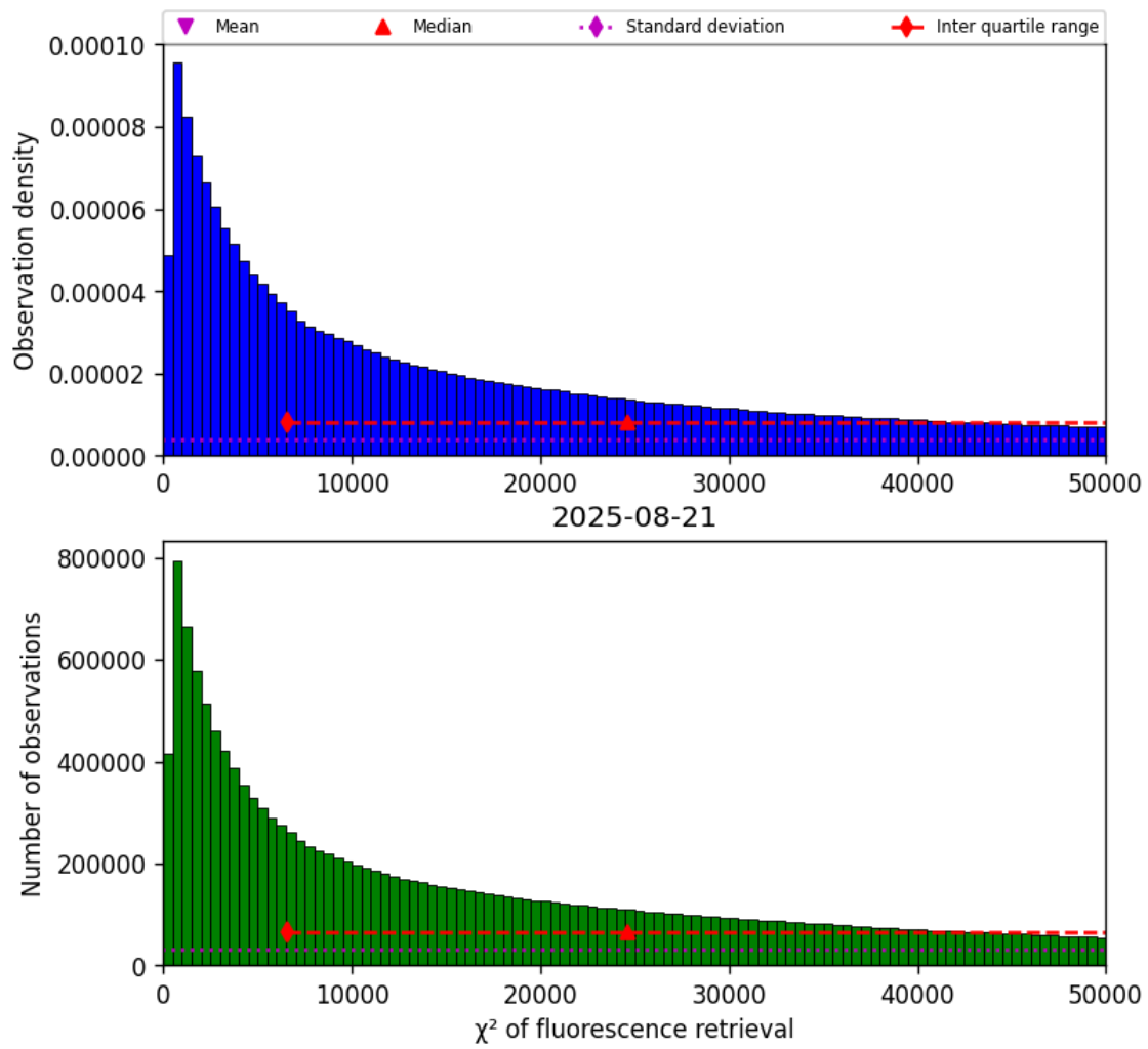
Figure 40: Histogram of “ \chi^2 of fluorescence retrieval” for 2025-08-21 to 2025-08-22
