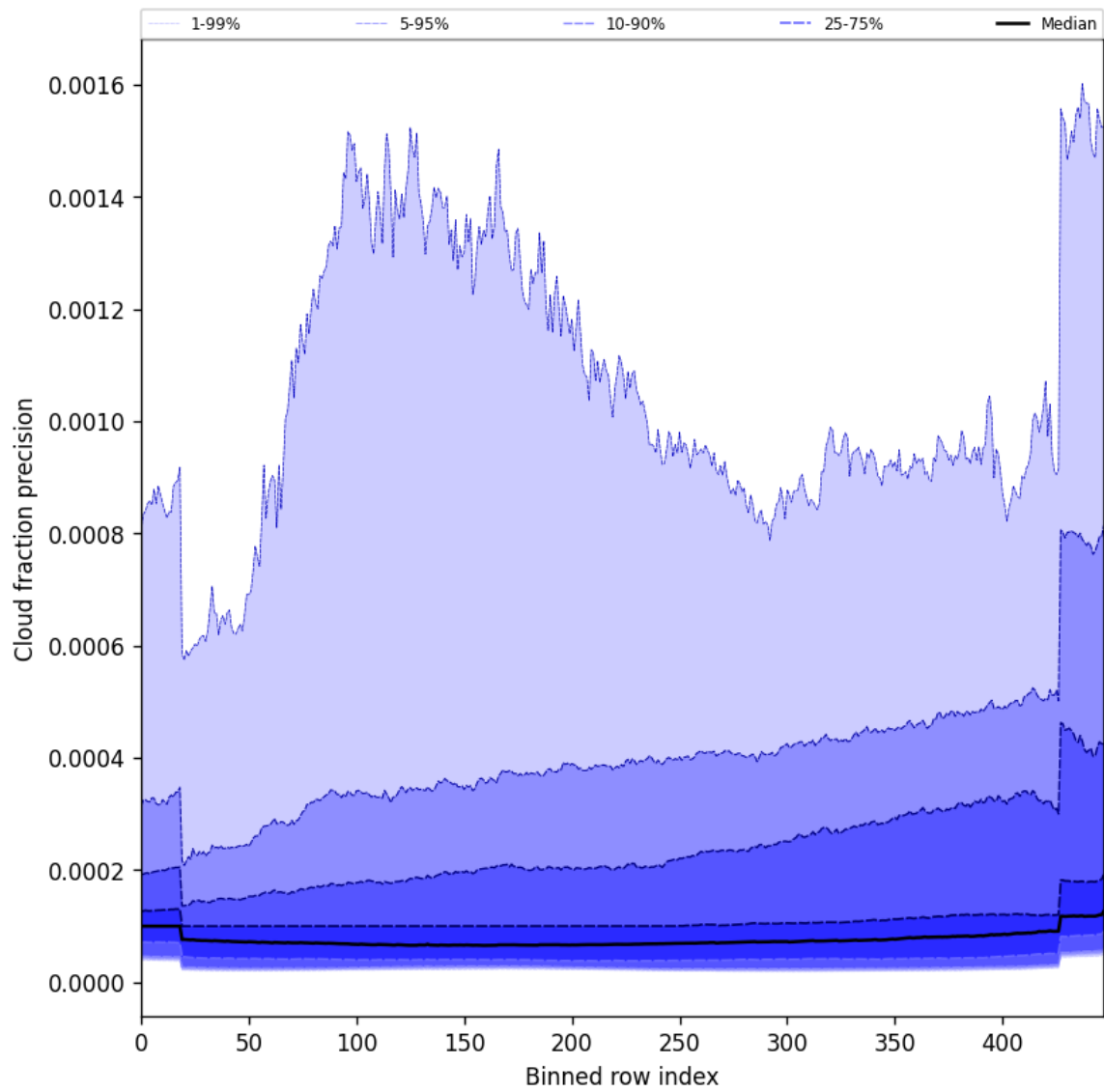
Figure 48: Along track statistics of “Cloud fraction precision” for 2025-08-21 to 2025-08-22
