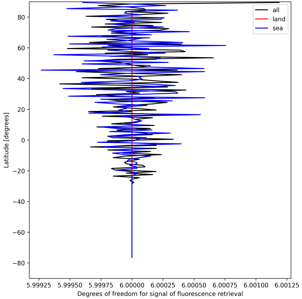
Figure 24: Zonal average of “Degrees of freedom for signal of fluorescence retrieval” for 2025-08-21 to 2025-08-22.
