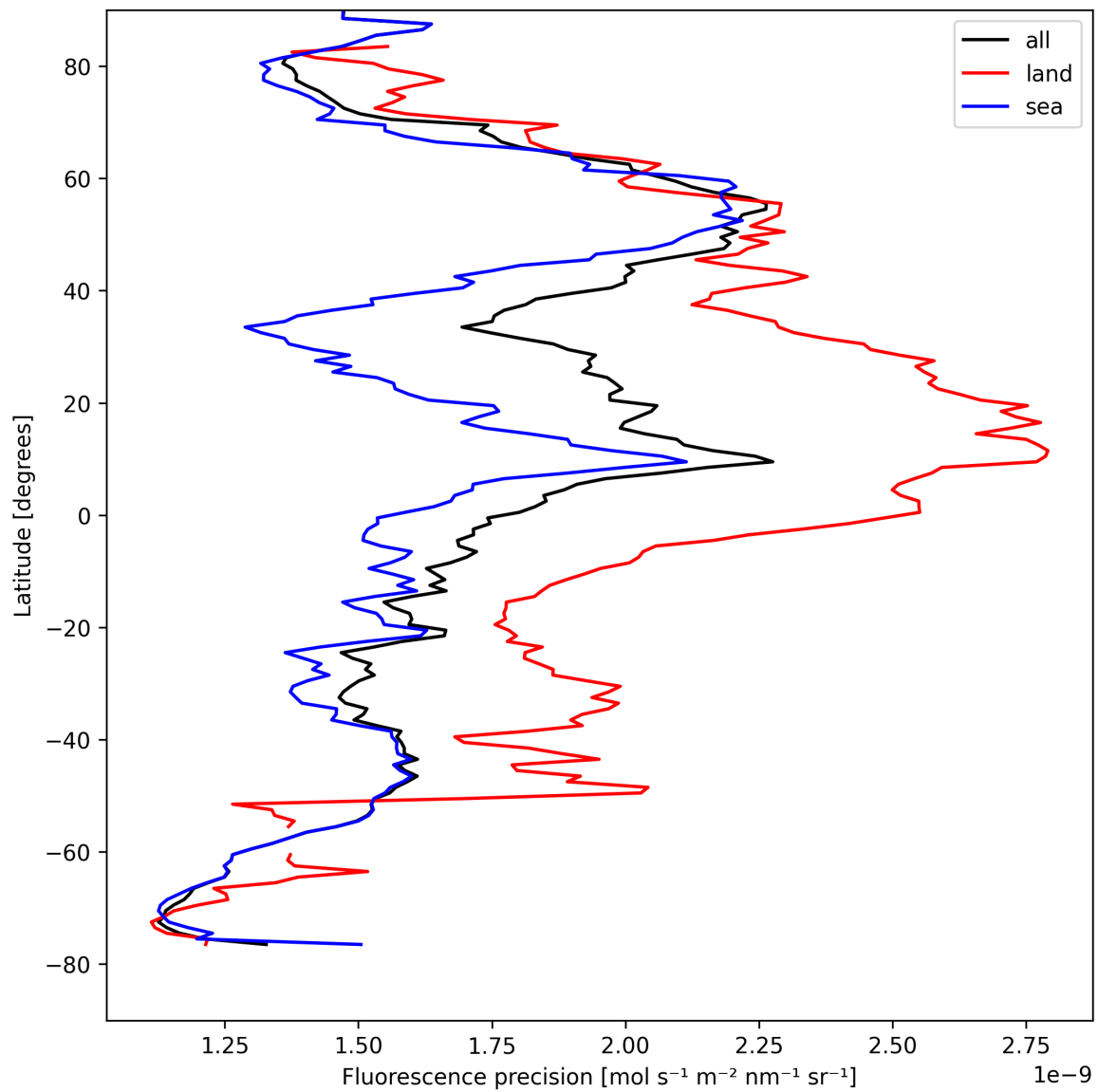
Figure 22: Zonal average of “Fluorescence precision” for 2025-08-21 to 2025-08-22.
