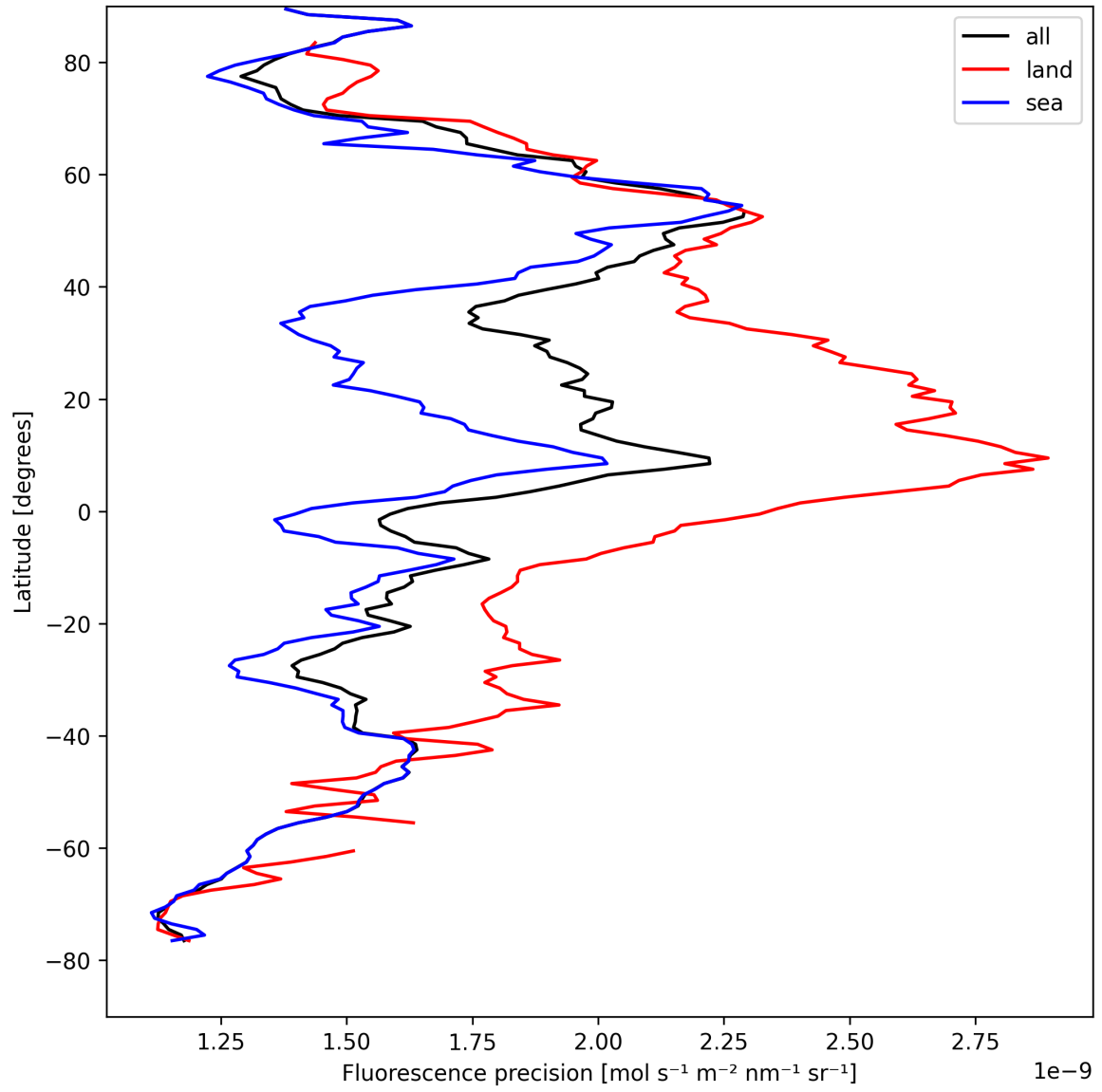
Figure 22: Zonal average of “Fluorescence precision” for 2025-08-22 to 2025-08-23.
