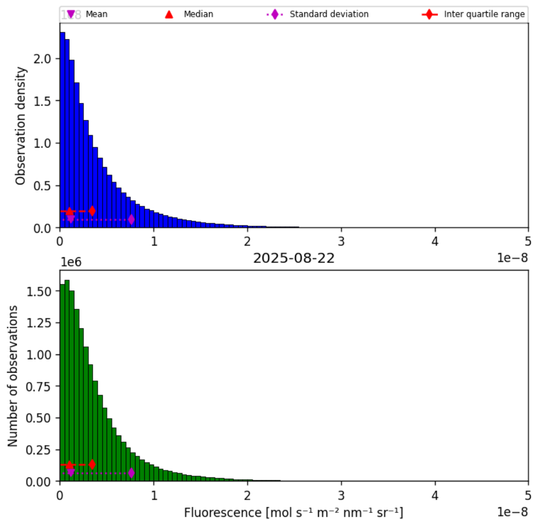
Figure 38: Histogram of “Fluorescence” for 2025-08-22 to 2025-08-23
