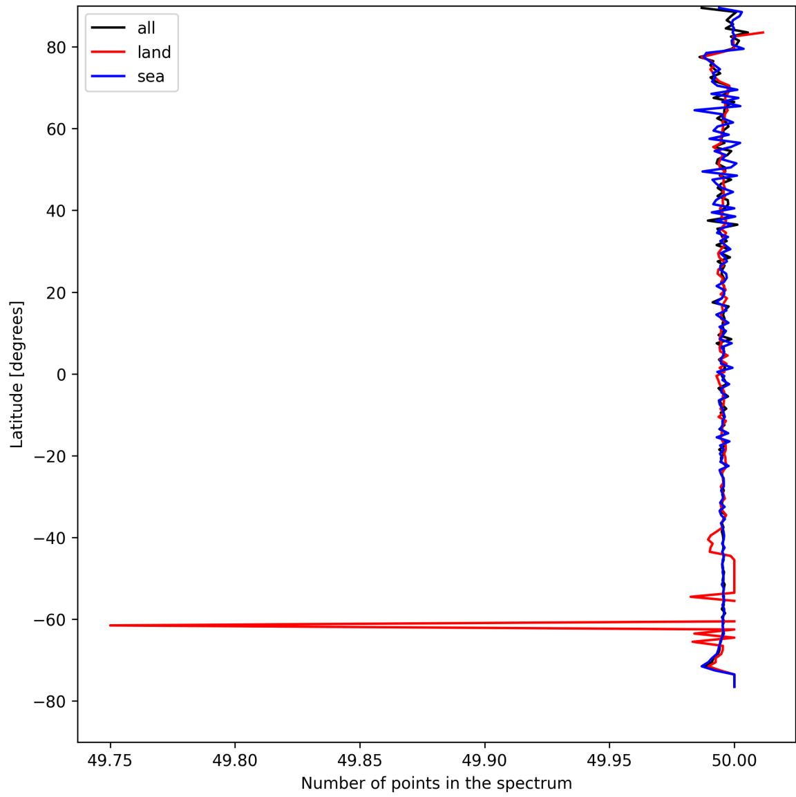
Figure 25: Zonal average of “Number of points in the spectrum” for 2025-08-22 to 2025-08-23.
