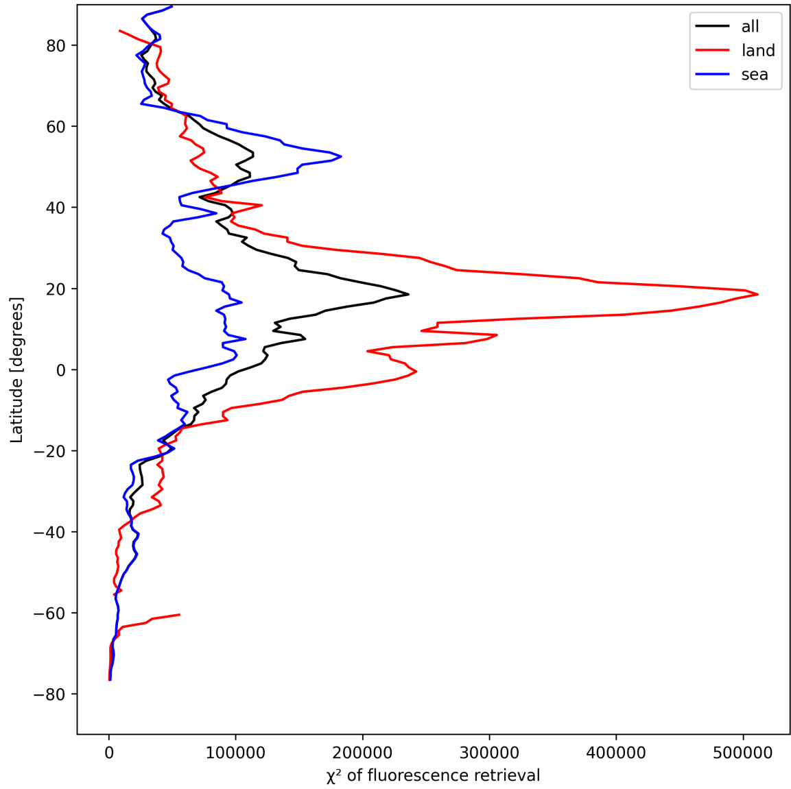
Figure 23: Zonal average of “ \chi^2 of fluorescence retrieval” for 2025-08-22 to 2025-08-23.
