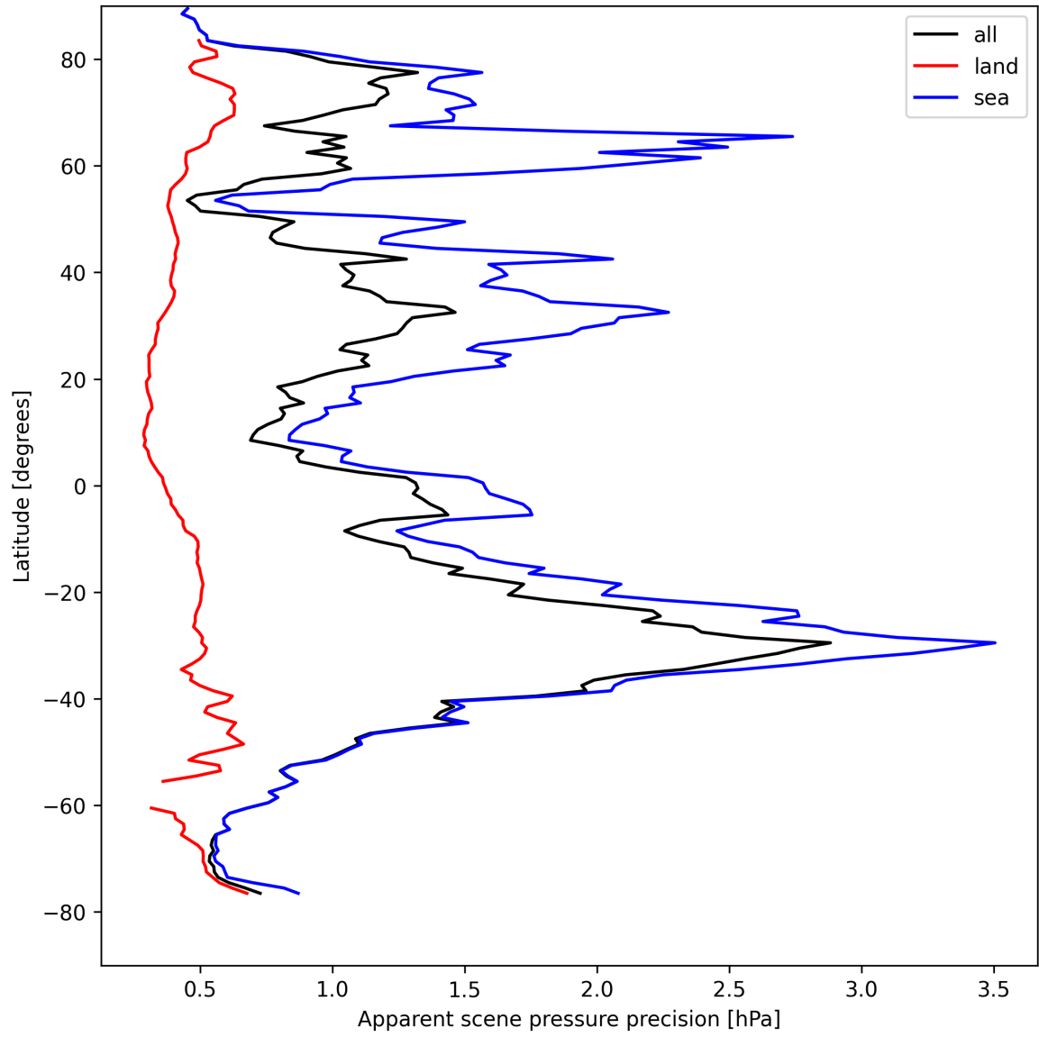
Figure 18: Zonal average of “Apparent scene pressure precision” for 2025-08-22 to 2025-08-23.
