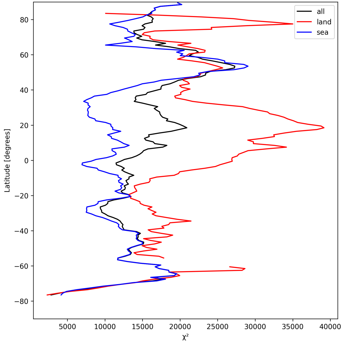
Figure 19: Zonal average of “ \chi^2 ” for 2025-08-22 to 2025-08-23.
