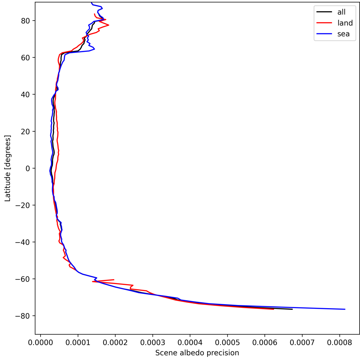
Figure 16: Zonal average of “Scene albedo precision” for 2025-08-22 to 2025-08-23.
