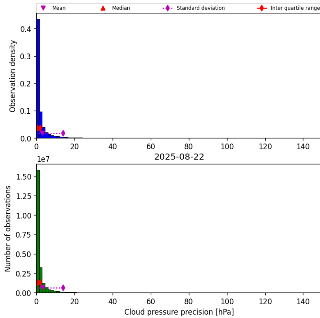
Figure 29: Histogram of “Cloud pressure precision” for 2025-08-22 to 2025-08-23
