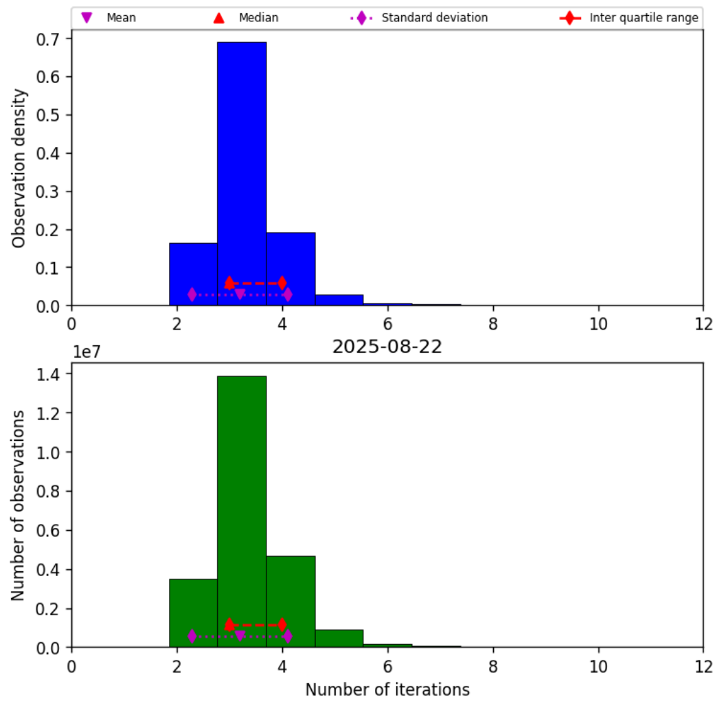
Figure 37: Histogram of “Number of iterations” for 2025-08-22 to 2025-08-23
