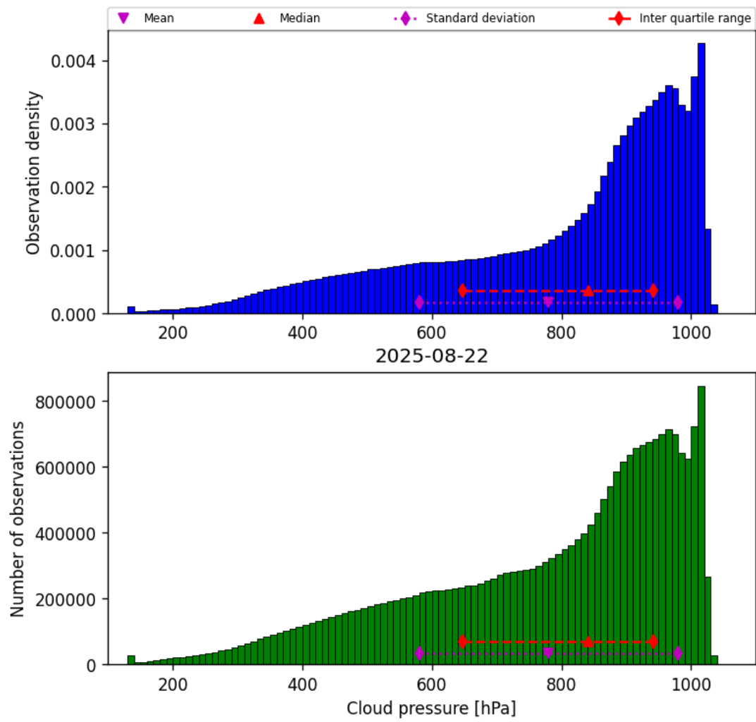
Figure 28: Histogram of “Cloud pressure” for 2025-08-22 to 2025-08-23
