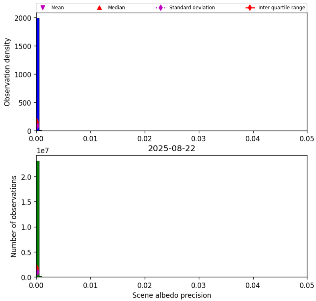
Figure 33: Histogram of “Scene albedo precision” for 2025-08-22 to 2025-08-23
