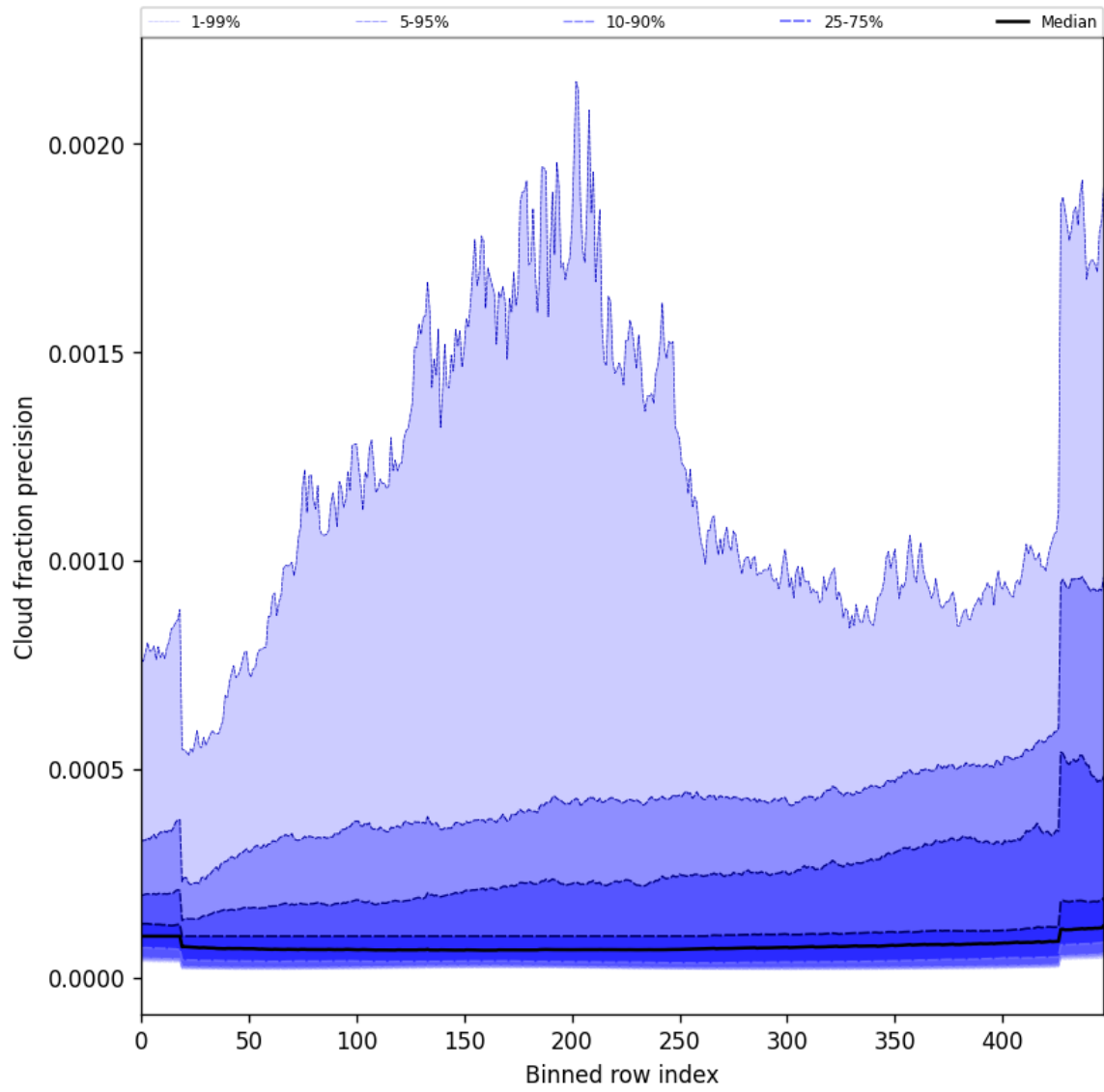
Figure 48: Along track statistics of “Cloud fraction precision” for 2025-08-22 to 2025-08-23
