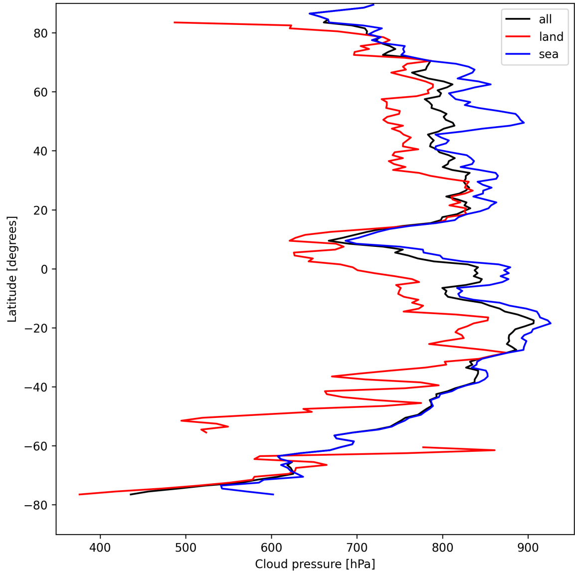
Figure 11: Zonal average of “Cloud pressure” for 2025-08-22 to 2025-08-23.
