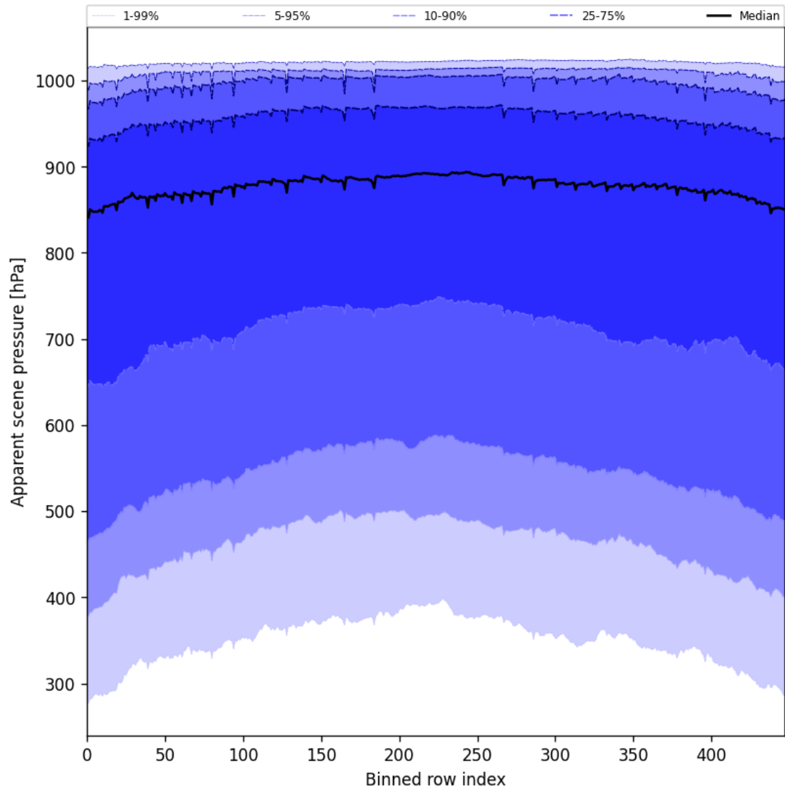
Figure 51: Along track statistics of “Apparent scene pressure” for 2025-08-22 to 2025-08-23
