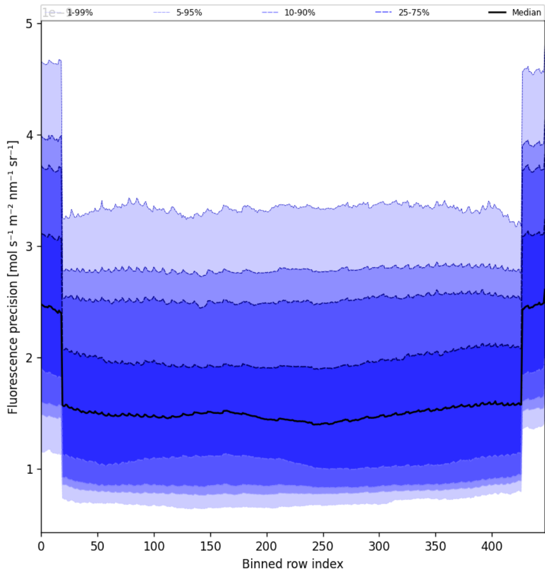
Figure 56: Along track statistics of “Fluorescence precision” for 2025-08-22 to 2025-08-23
