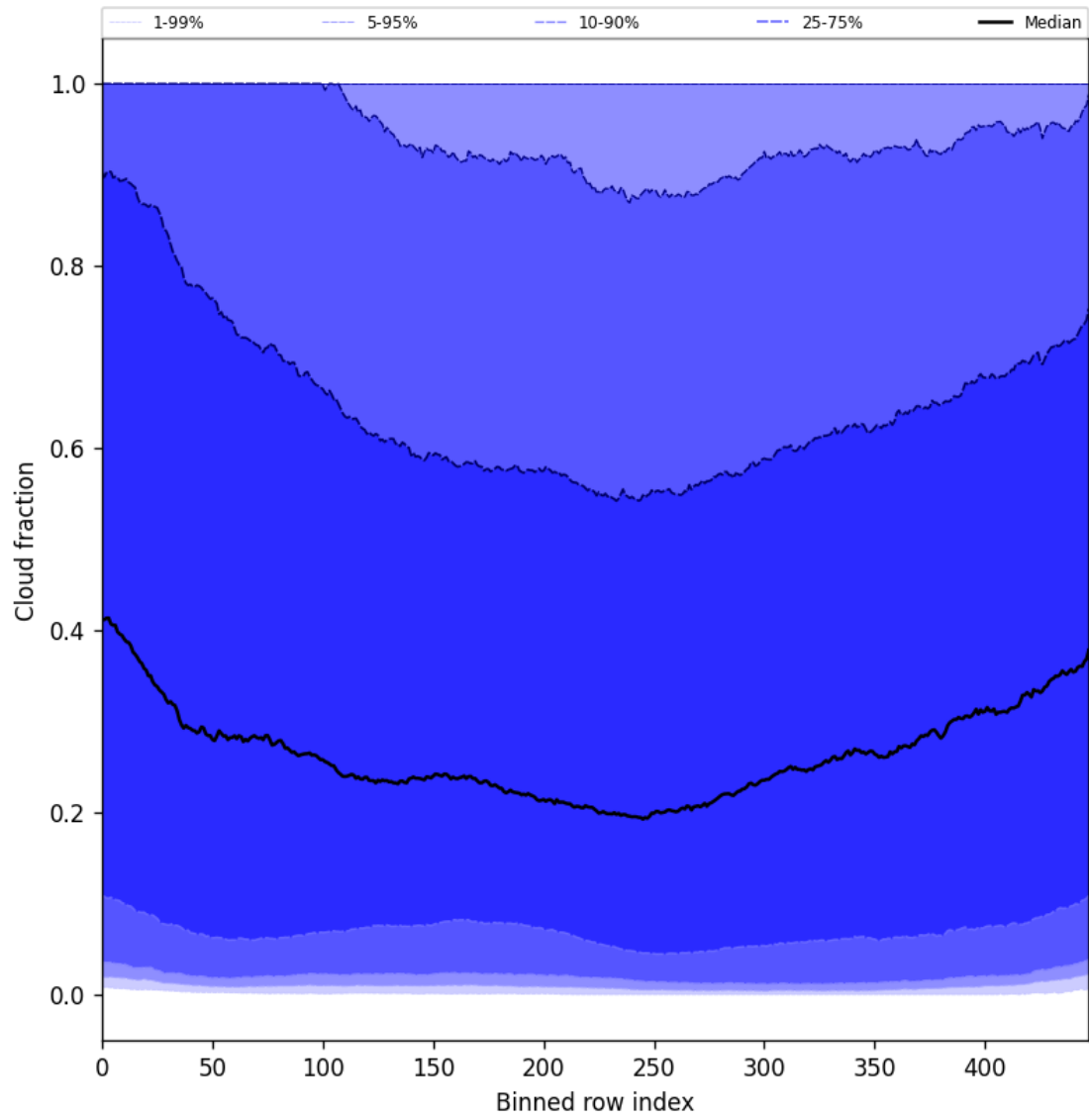
Figure 47: Along track statistics of “Cloud fraction” for 2025-08-22 to 2025-08-23
