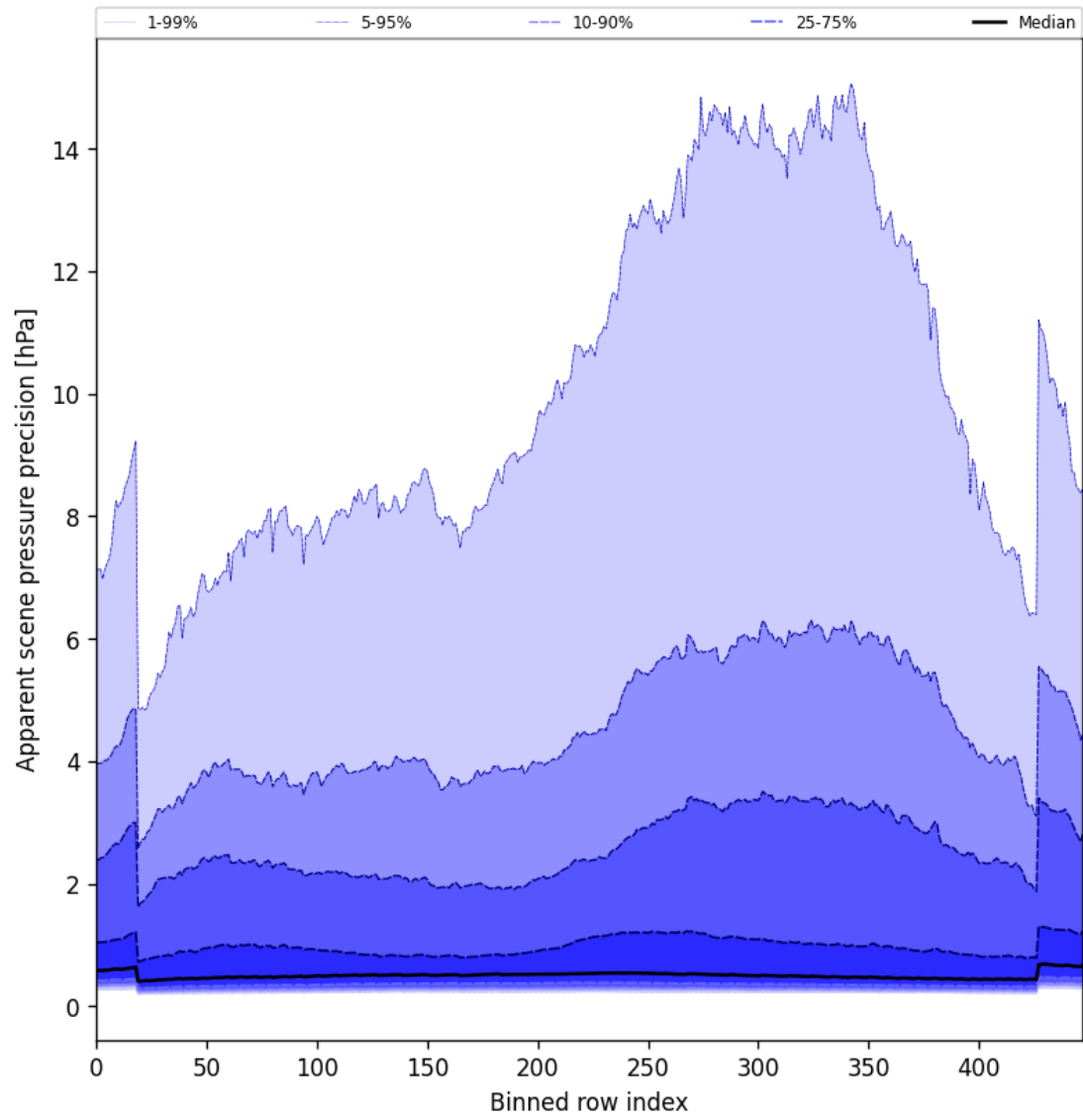
Figure 52: Along track statistics of “Apparent scene pressure precision” for 2025-08-22 to 2025-08-23
