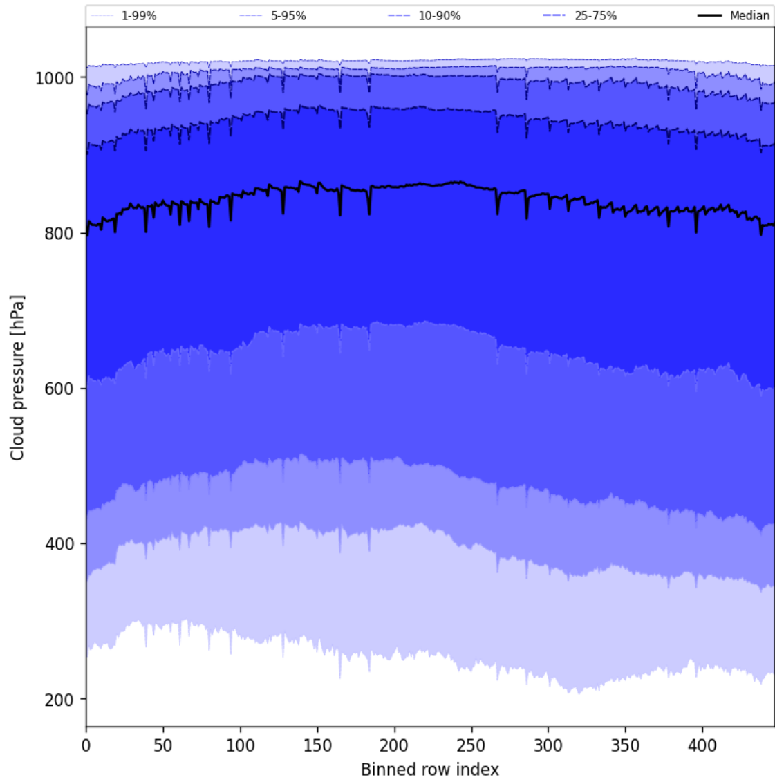
Figure 45: Along track statistics of “Cloud pressure” for 2025-08-22 to 2025-08-23
