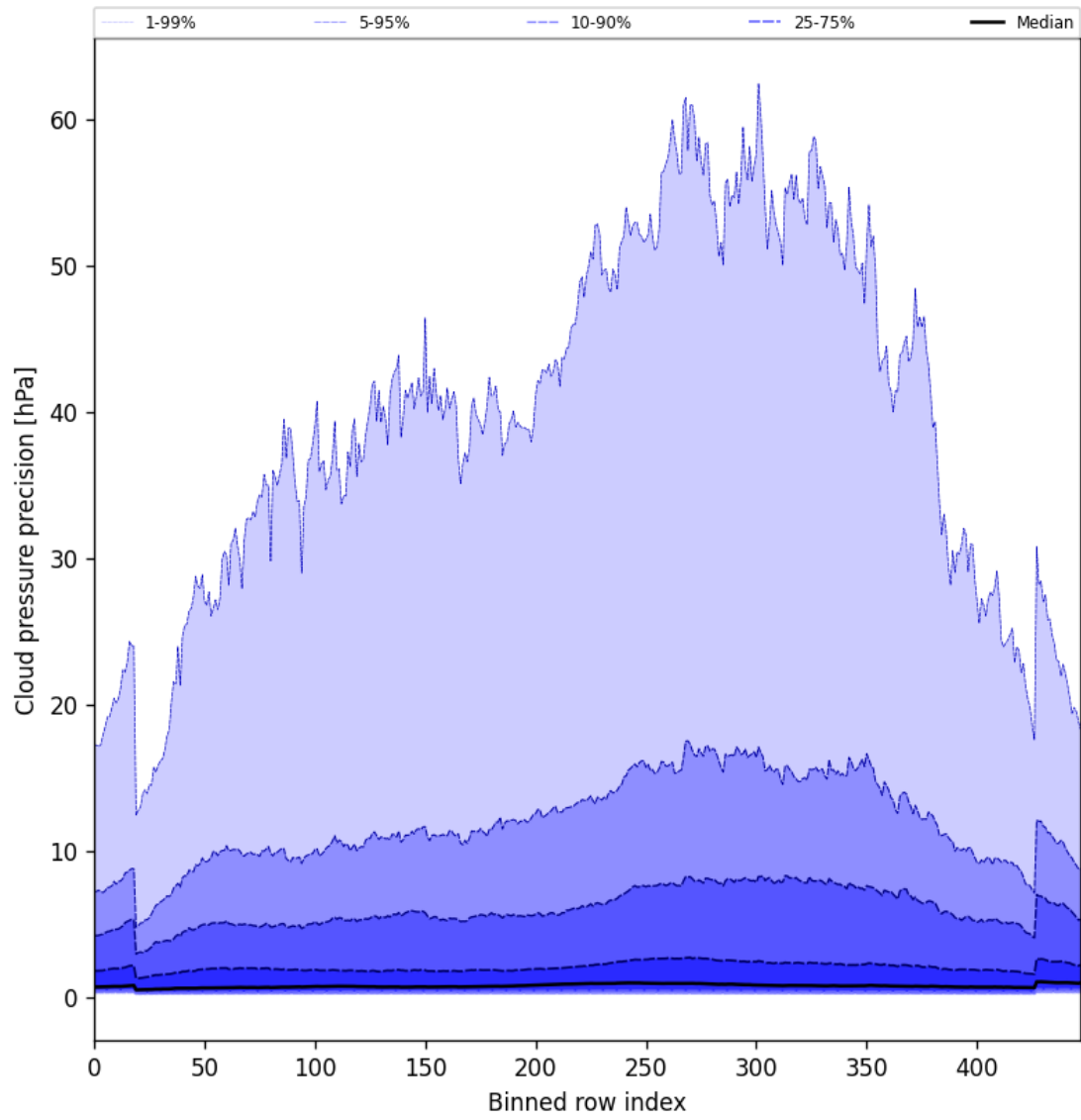
Figure 46: Along track statistics of “Cloud pressure precision” for 2025-08-22 to 2025-08-23
