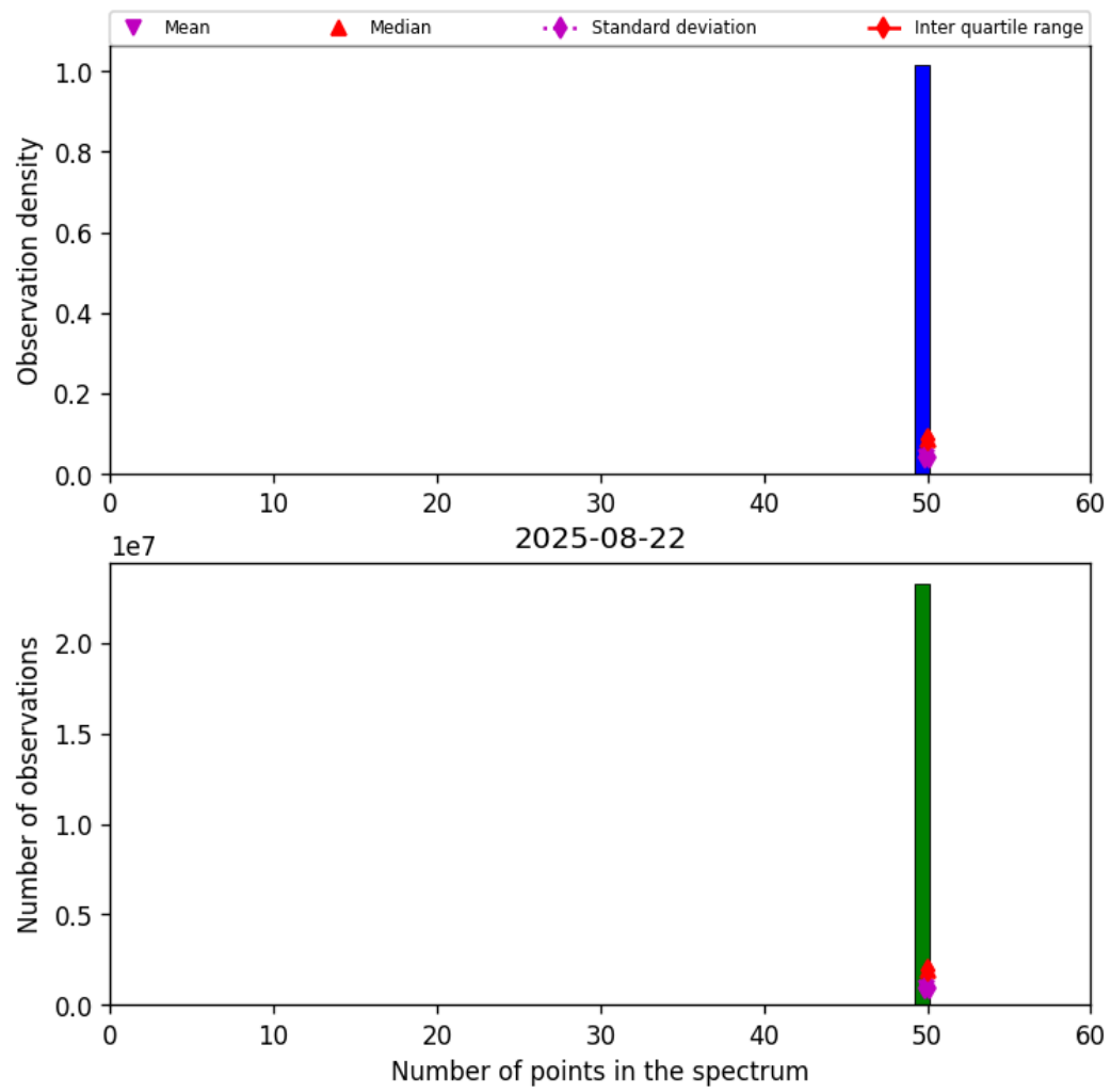
Figure 42: Histogram of “Number of points in the spectrum” for 2025-08-22 to 2025-08-23
