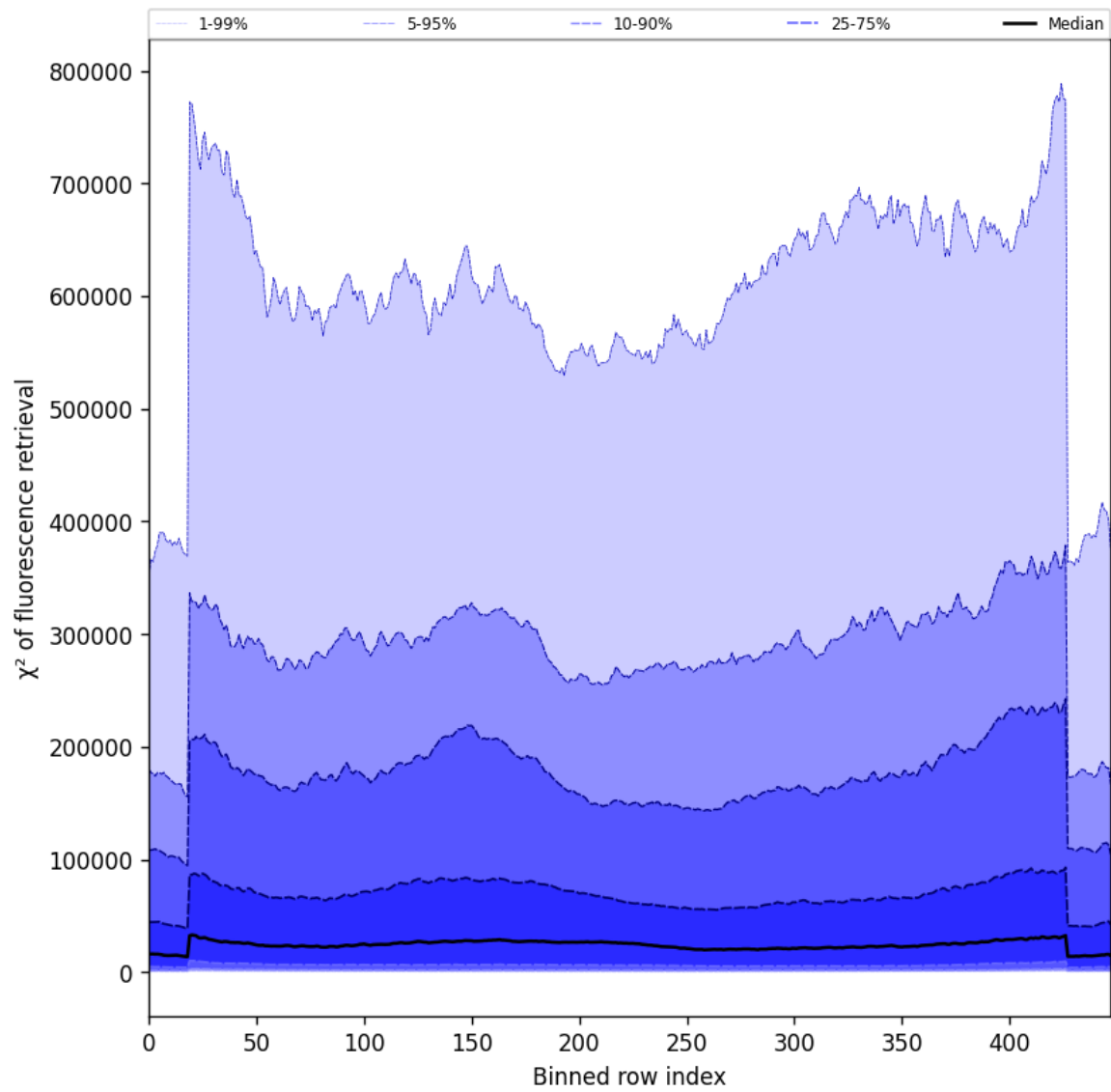
Figure 57: Along track statistics of “ \chi^2 of fluorescence retrieval” for 2025-08-22 to 2025-08-23
