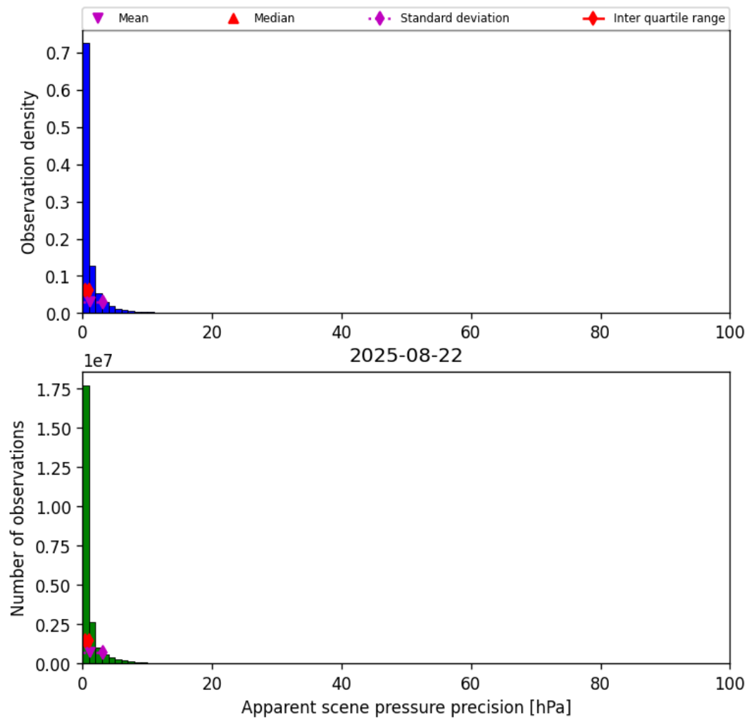
Figure 35: Histogram of “Apparent scene pressure precision” for 2025-08-22 to 2025-08-23
