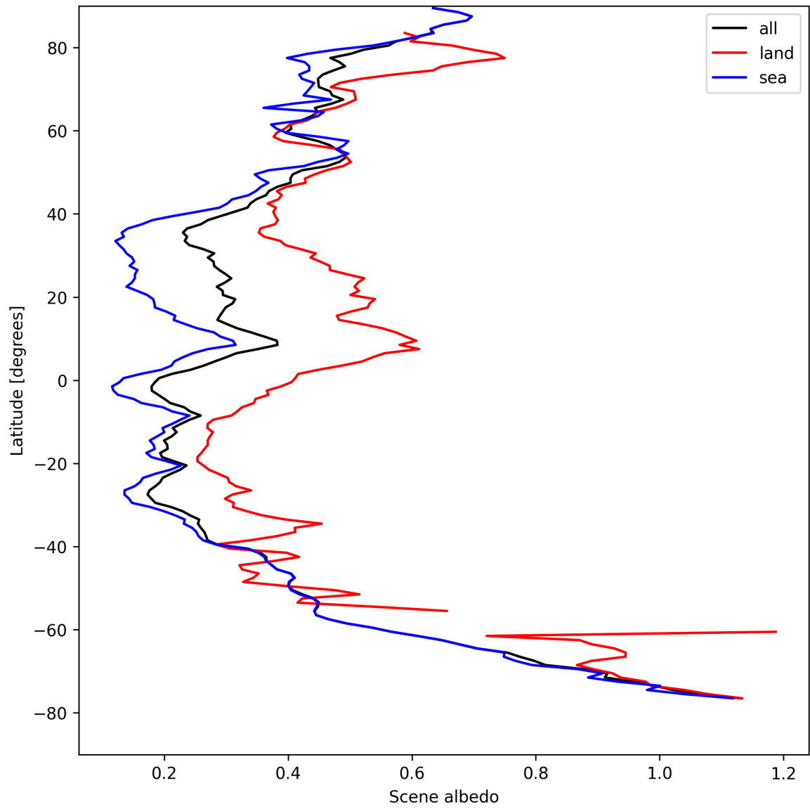
Figure 15: Zonal average of “Scene albedo” for 2025-08-22 to 2025-08-23.
