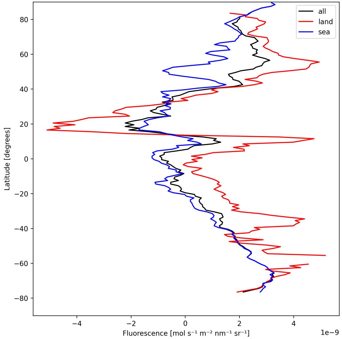
Figure 21: Zonal average of “Fluorescence” for 2025-08-22 to 2025-08-23.
