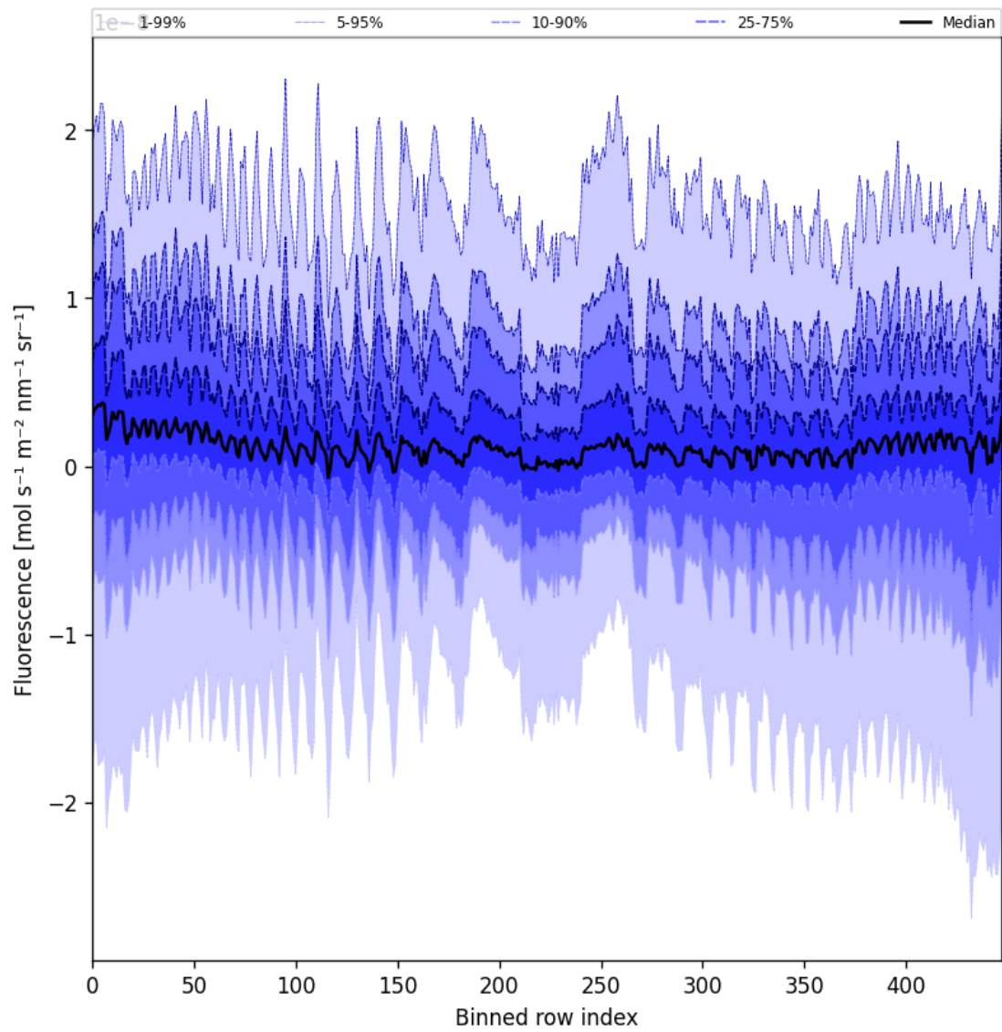
Figure 55: Along track statistics of “Fluorescence” for 2025-08-22 to 2025-08-23
