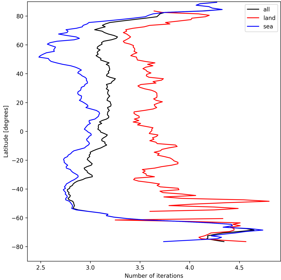
Figure 20: Zonal average of “Number of iterations” for 2025-08-22 to 2025-08-23.
