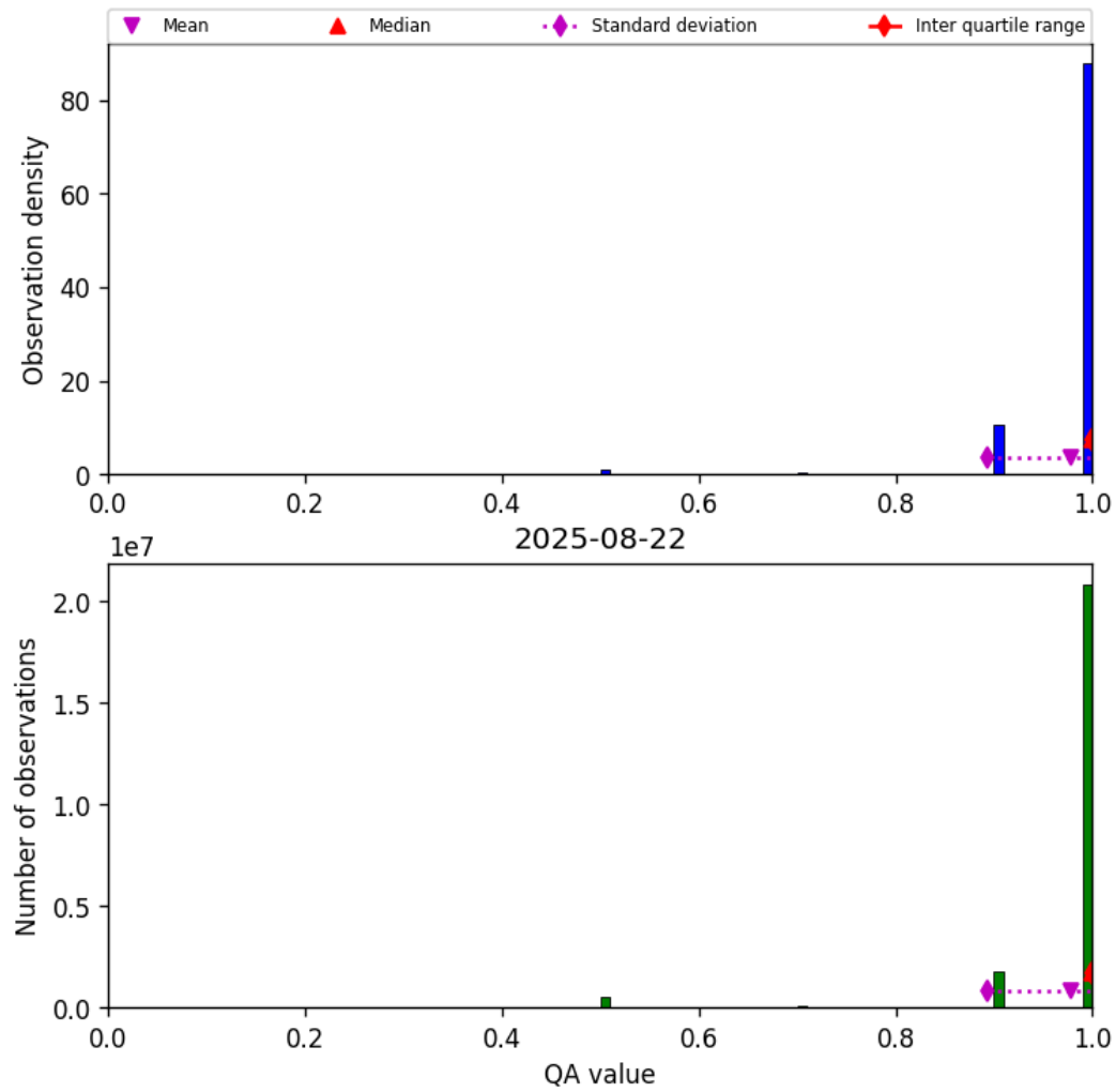
Figure 27: Histogram of “QA value” for 2025-08-22 to 2025-08-23
