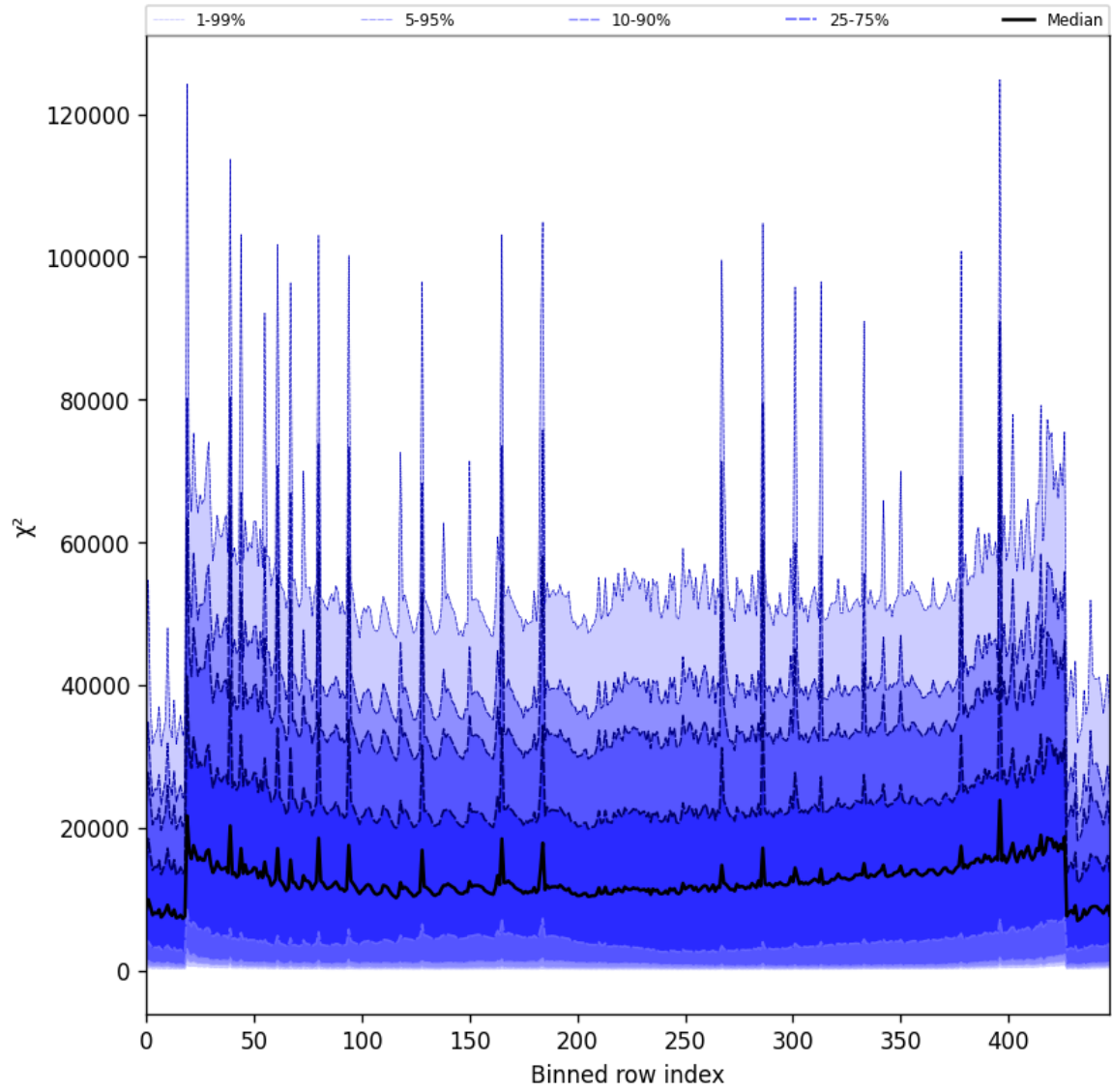
Figure 53: Along track statistics of “ \chi^2 ” for 2025-08-22 to 2025-08-23
