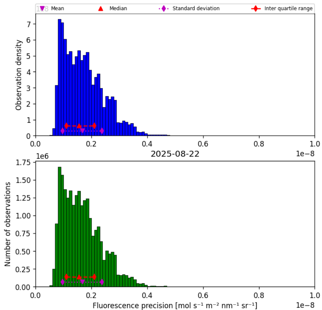
Figure 39: Histogram of “Fluorescence precision” for 2025-08-22 to 2025-08-23
