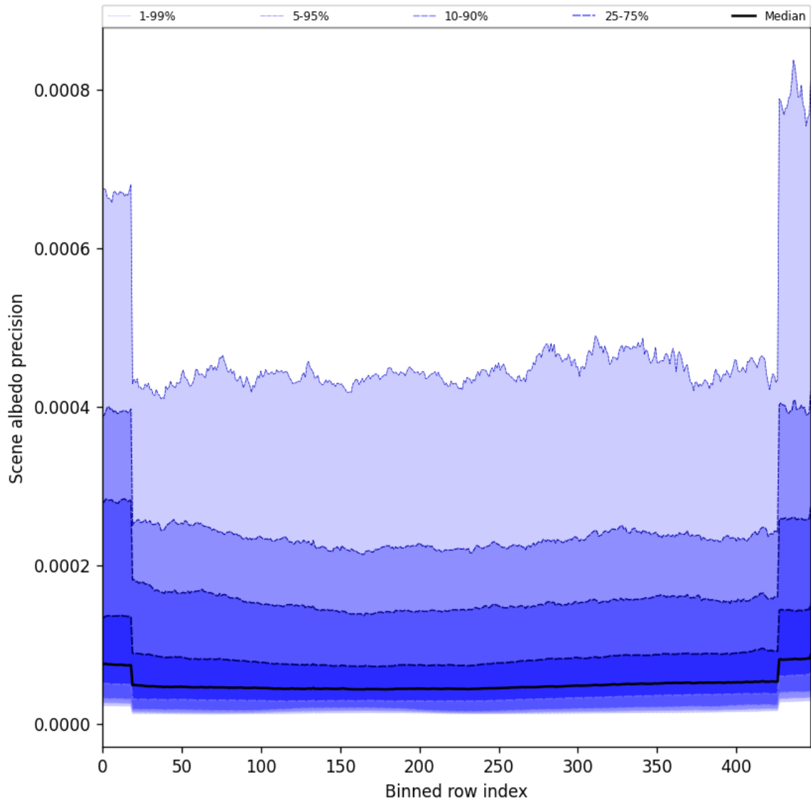
Figure 50: Along track statistics of “Scene albedo precision” for 2025-08-22 to 2025-08-23
