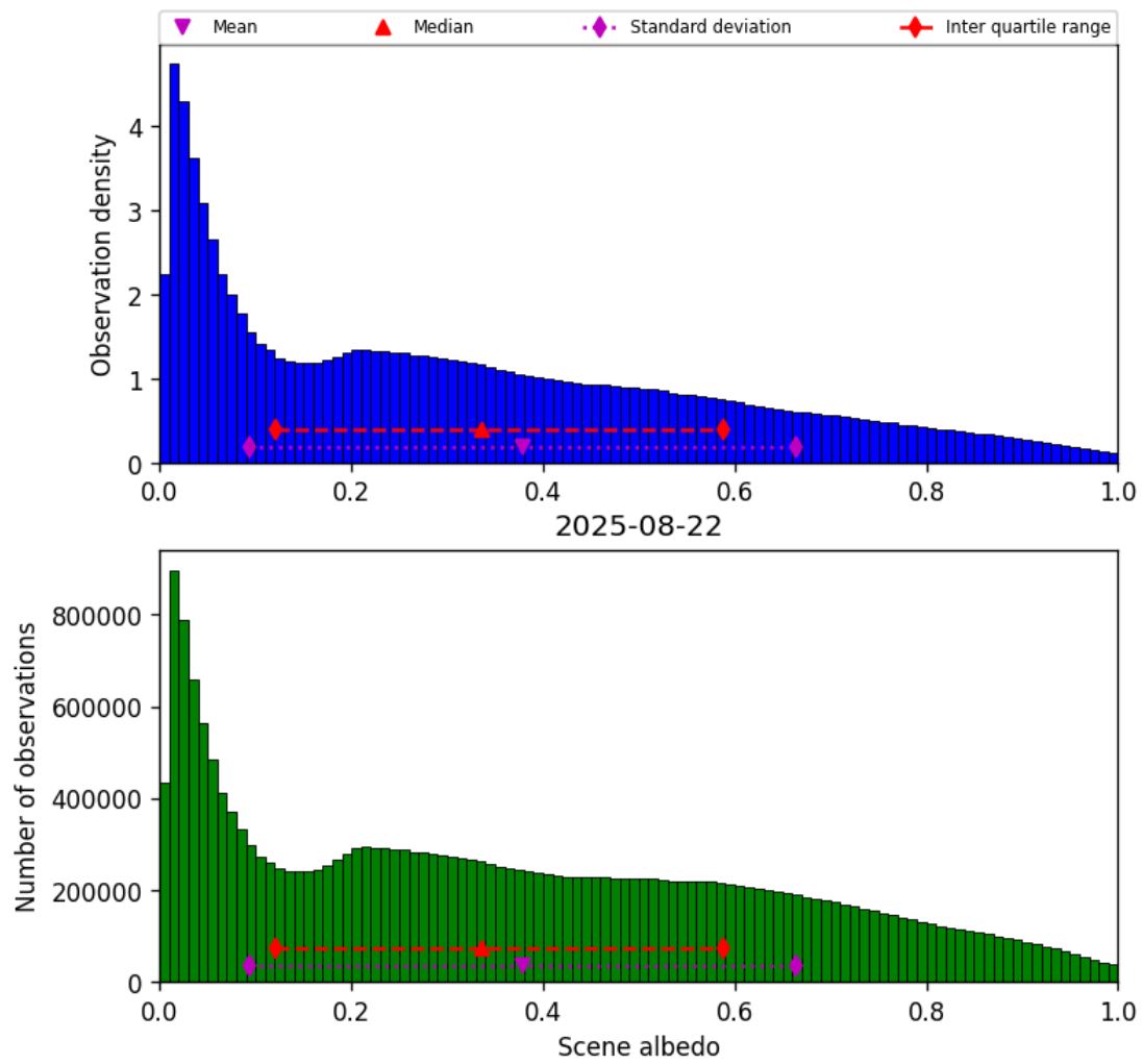
Figure 32: Histogram of “Scene albedo” for 2025-08-22 to 2025-08-23
