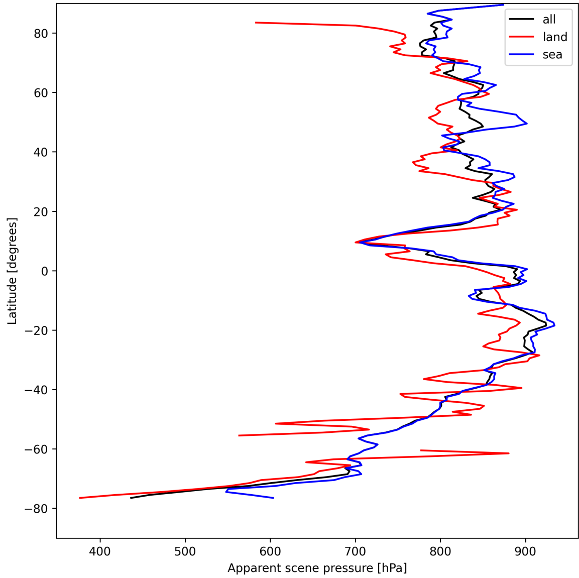
Figure 17: Zonal average of “Apparent scene pressure” for 2025-08-22 to 2025-08-23.
