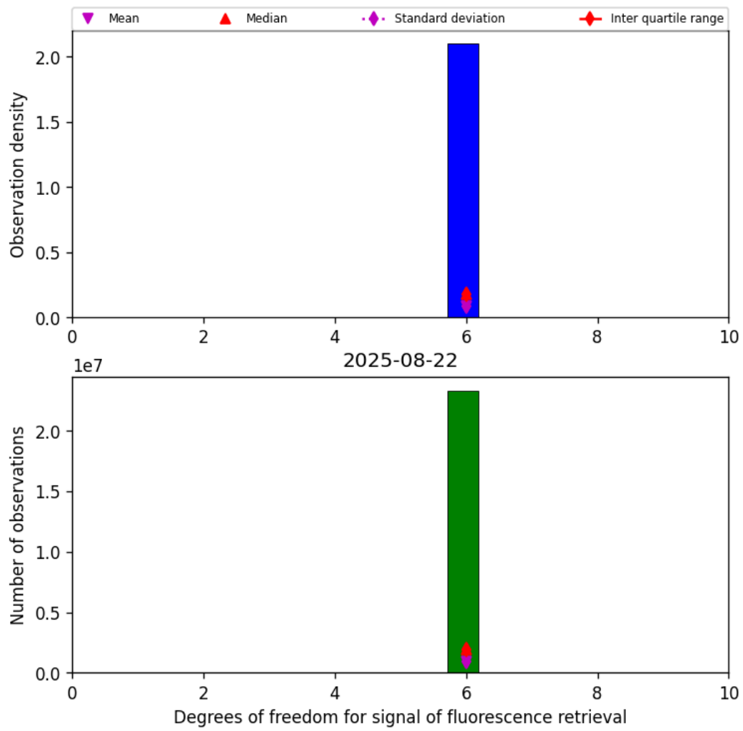
Figure 41: Histogram of “Degrees of freedom for signal of fluorescence retrieval” for 2025-08-22 to 2025-08-23
