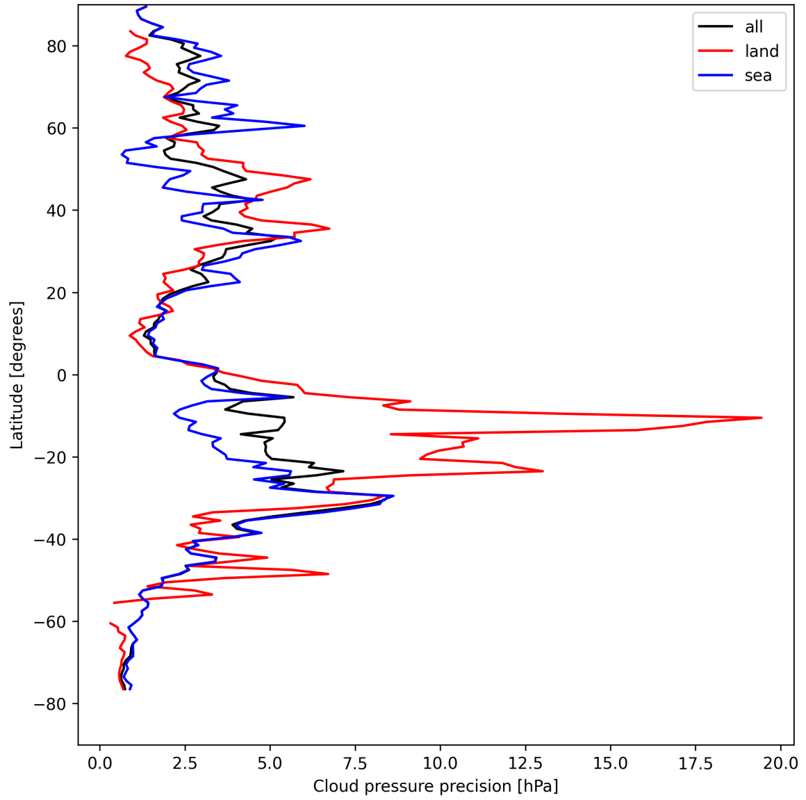
Figure 12: Zonal average of "Cloud pressure precision" for 2025-08-22 to 2025-08-23.
