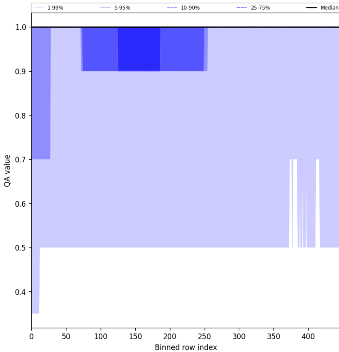
Figure 44: Along track statistics of “QA value” for 2025-08-22 to 2025-08-23
