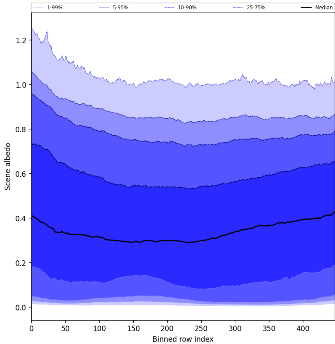
Figure 49: Along track statistics of “Scene albedo” for 2025-08-22 to 2025-08-23
