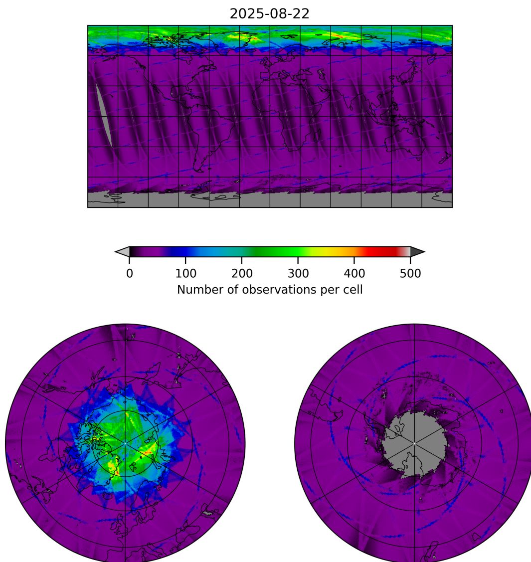
Figure 9: Map of the number of observations for 2025-08-22 to 2025-08-23
