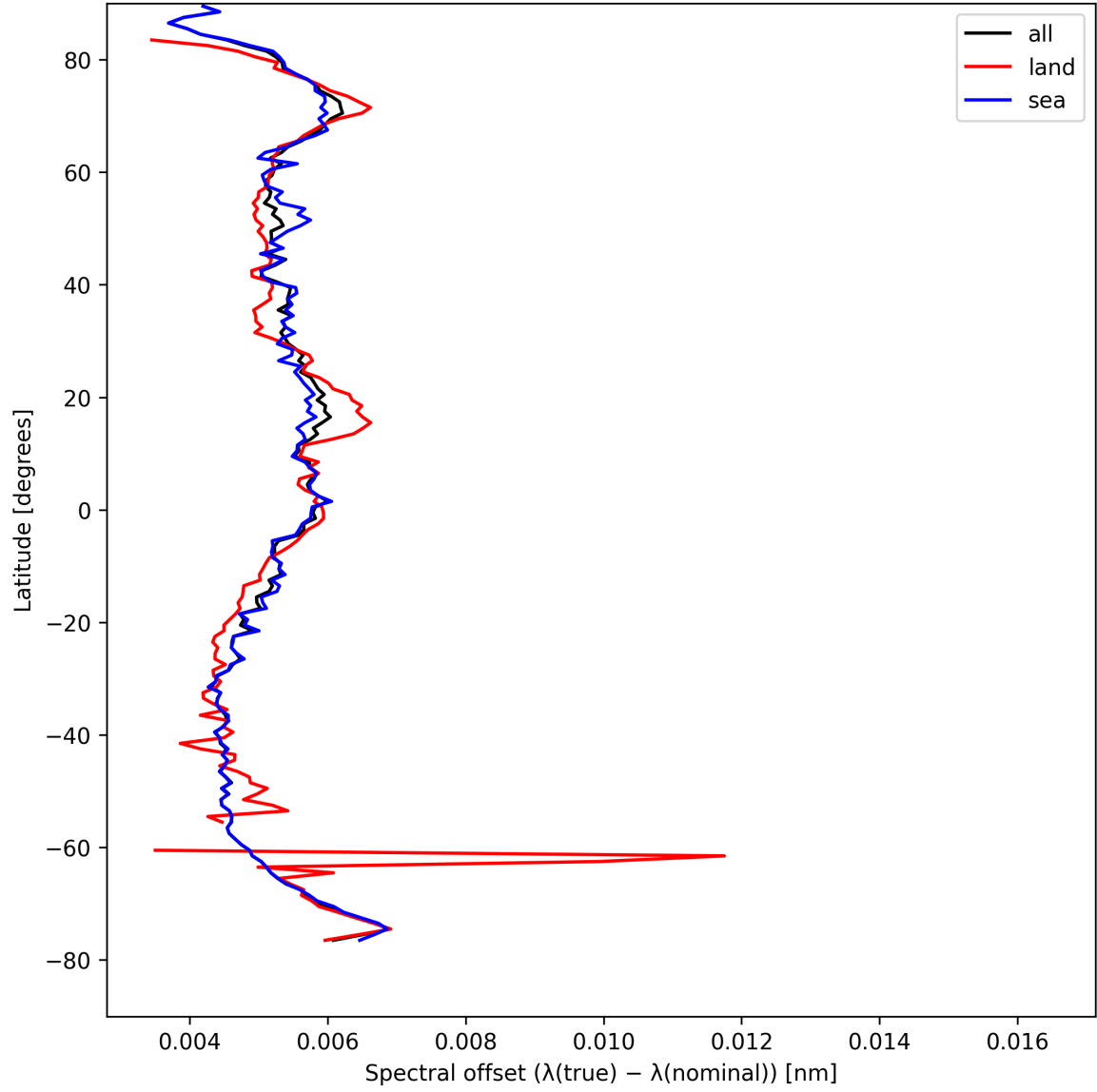
Figure 26: Zonal average of “Spectral offset ( \lambda_{\text{true}} - \lambda_{\text{nominal}} )” for 2025-08-22 to 2025-08-23.
