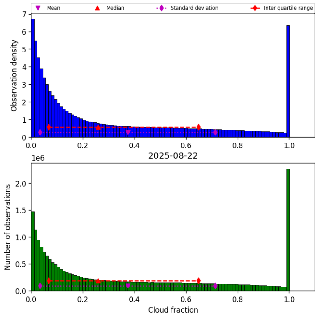
Figure 30: Histogram of “Cloud fraction” for 2025-08-22 to 2025-08-23
