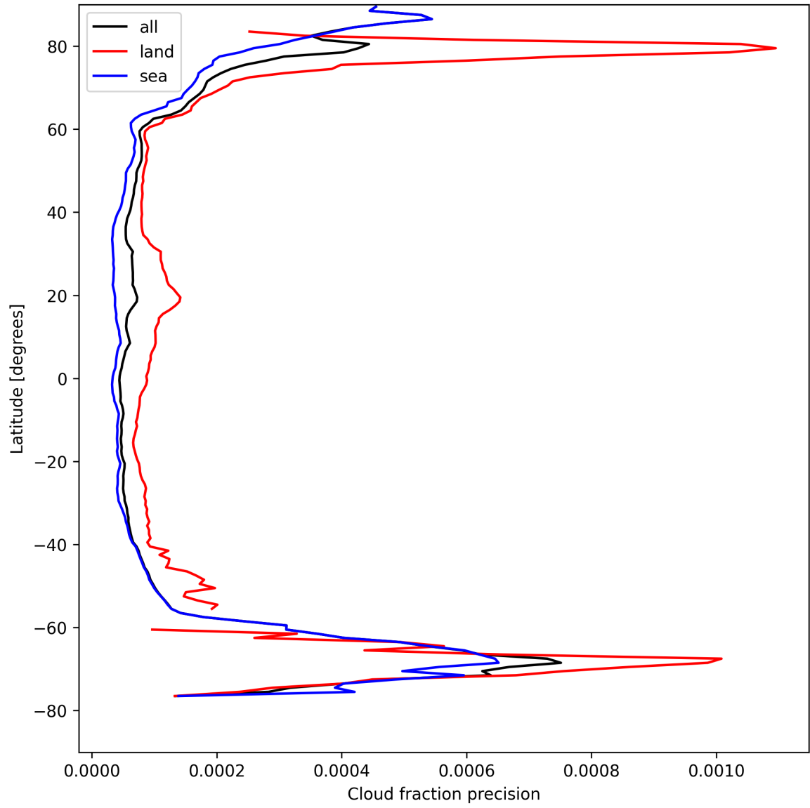
Figure 14: Zonal average of “Cloud fraction precision” for 2025-08-22 to 2025-08-23.
