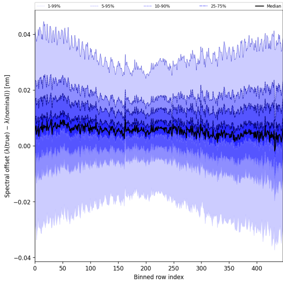
Figure 60: Along track statistics of “Spectral offset ( \lambda_{\text{true}} - \lambda_{\text{nominal}} )” for 2025-08-22 to 2025-08-23
