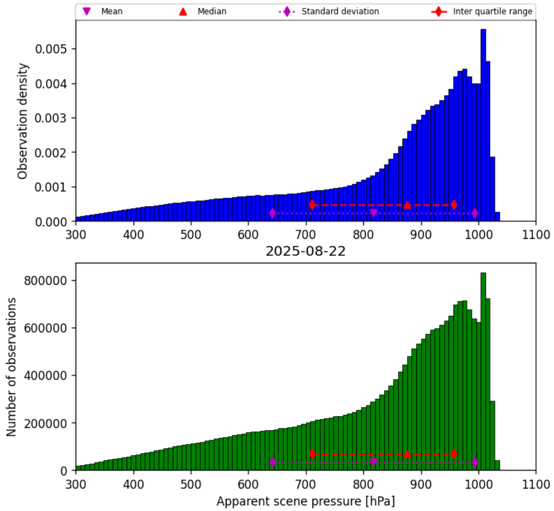
Figure 34: Histogram of “Apparent scene pressure” for 2025-08-22 to 2025-08-23
