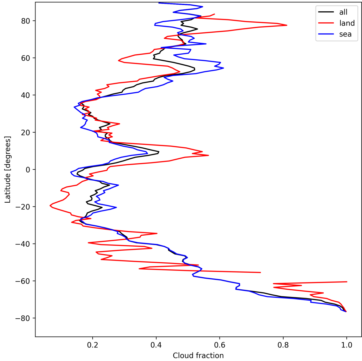
Figure 13: Zonal average of “Cloud fraction” for 2025-08-22 to 2025-08-23.
