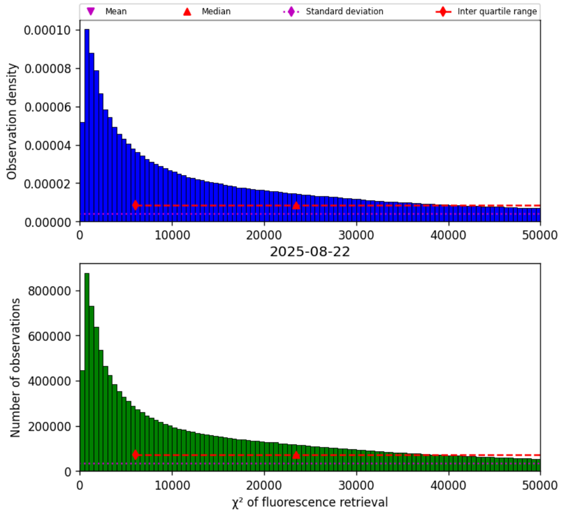
Figure 40: Histogram of “ \chi^2 of fluorescence retrieval” for 2025-08-22 to 2025-08-23
