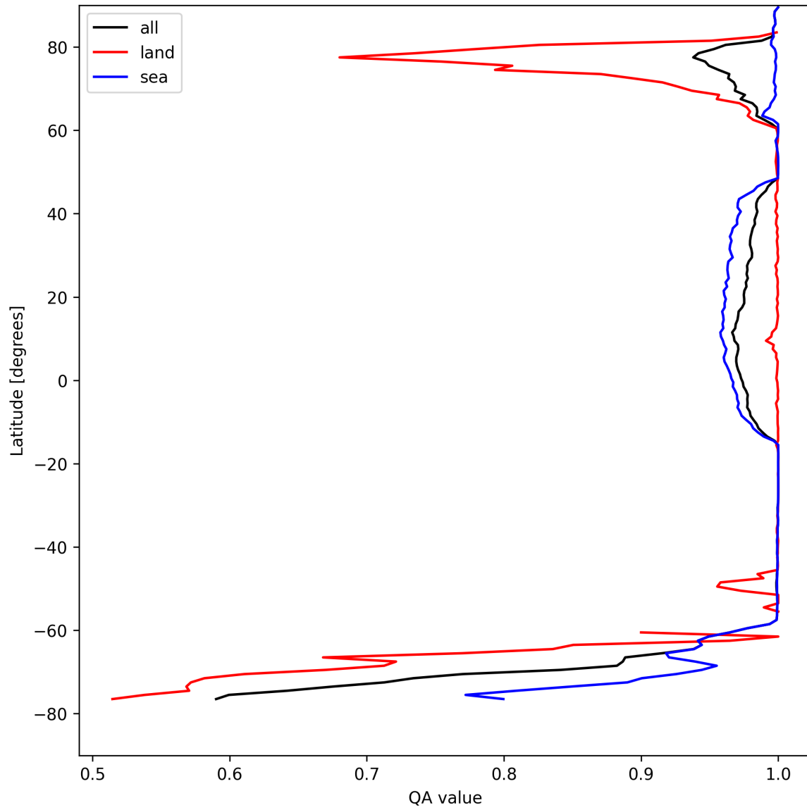
Figure 10: Zonal average of “QA value” for 2025-08-22 to 2025-08-23.
