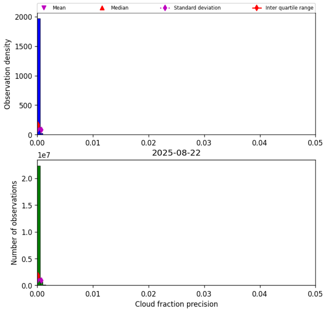
Figure 31: Histogram of “Cloud fraction precision” for 2025-08-22 to 2025-08-23
