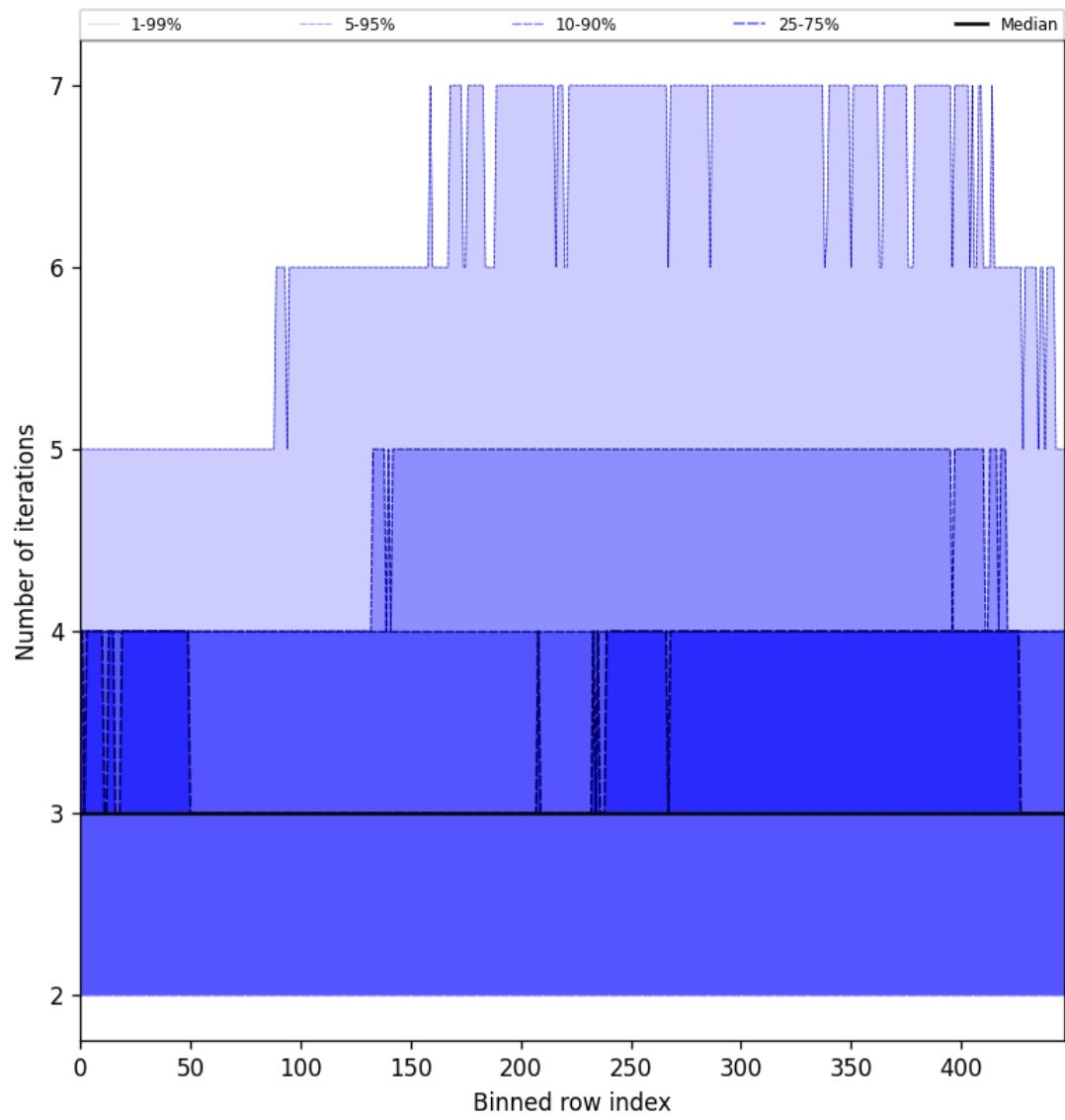
Figure 54: Along track statistics of “Number of iterations” for 2025-08-22 to 2025-08-23
