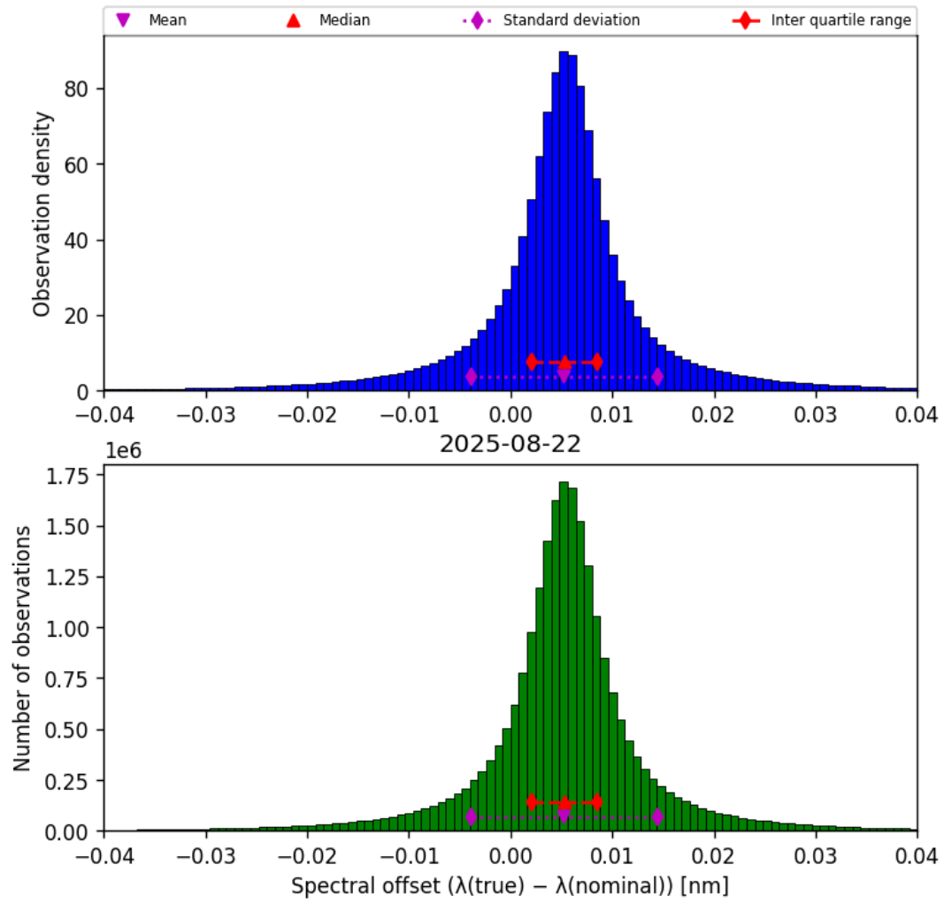
Figure 43: Histogram of “Spectral offset ( \lambda_{\text{true}} - \lambda_{\text{nominal}} )” for 2025-08-22 to 2025-08-23
