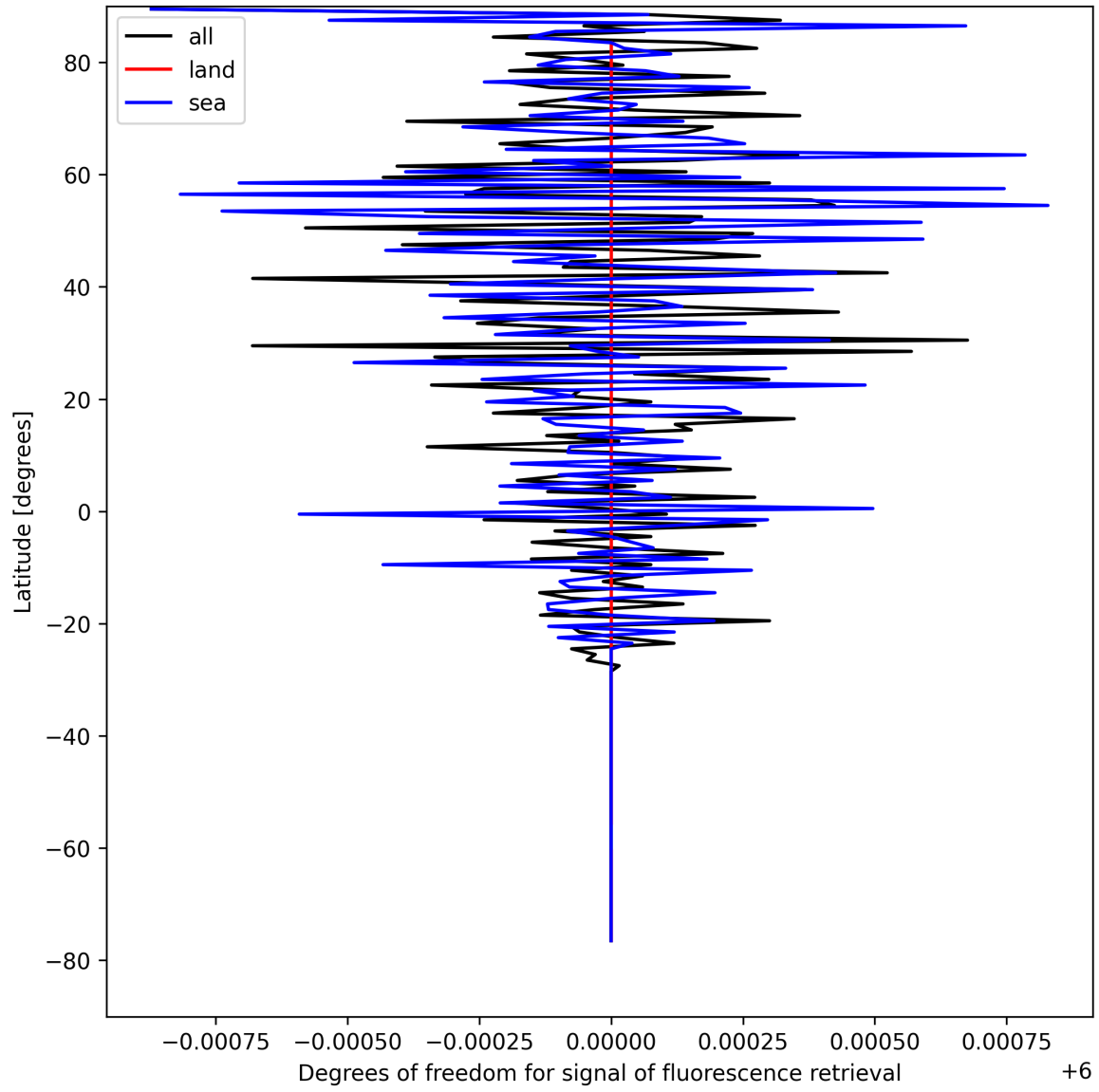
Figure 24: Zonal average of “Degrees of freedom for signal of fluorescence retrieval” for 2025-08-22 to 2025-08-23.
