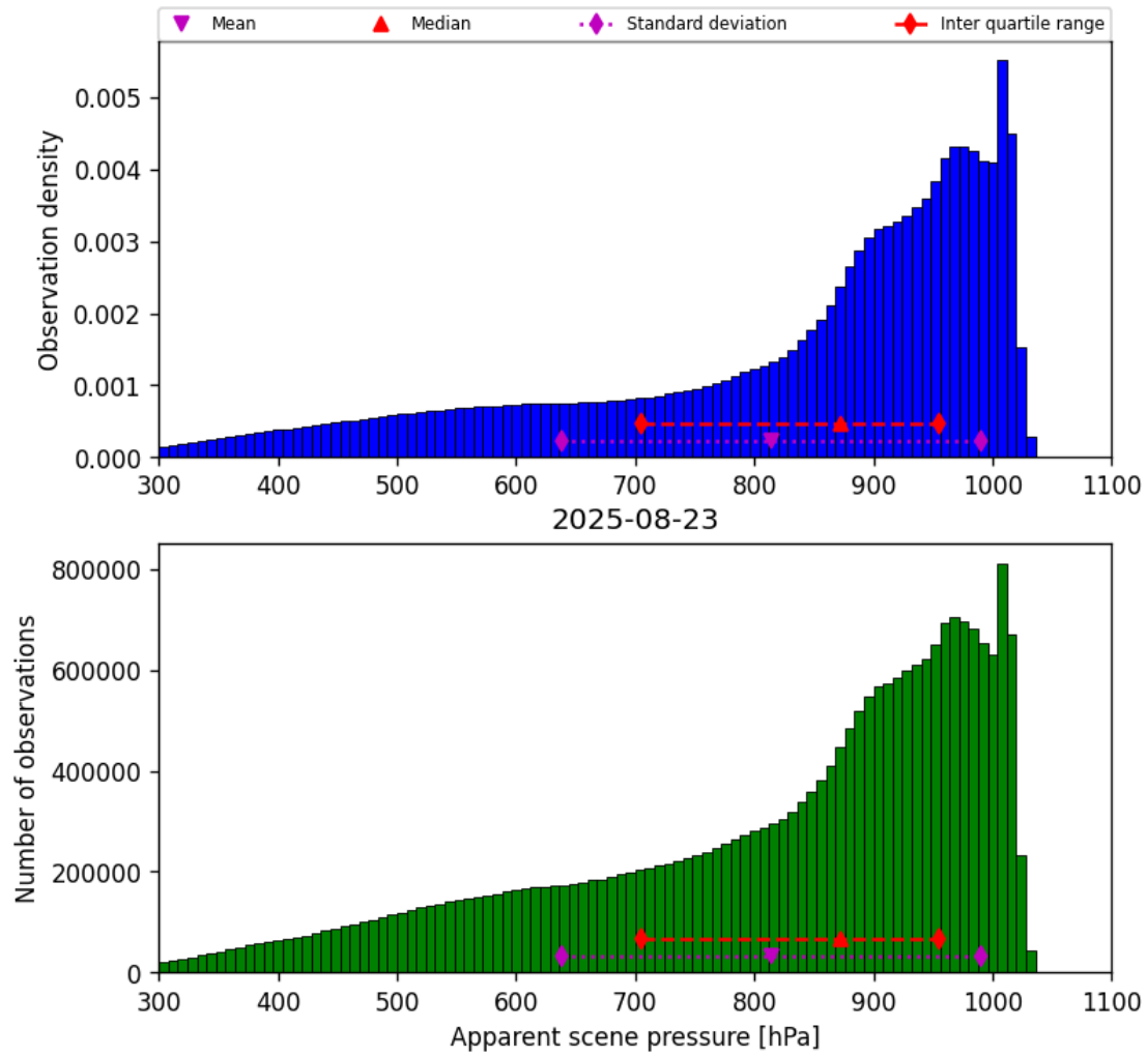
Figure 34: Histogram of “Apparent scene pressure” for 2025-08-23 to 2025-08-23
