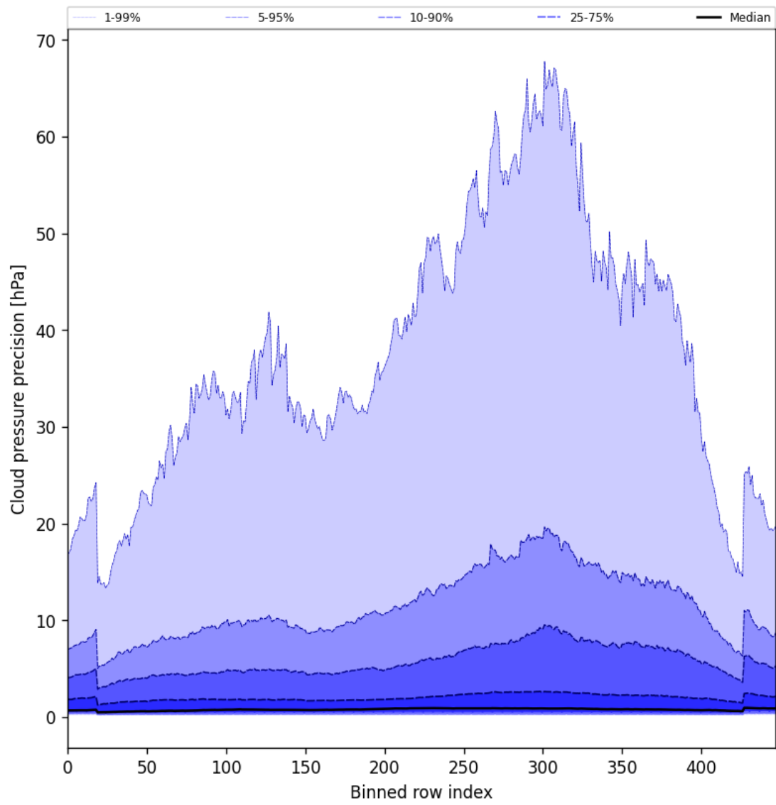
Figure 46: Along track statistics of “Cloud pressure precision” for 2025-08-23 to 2025-08-23
