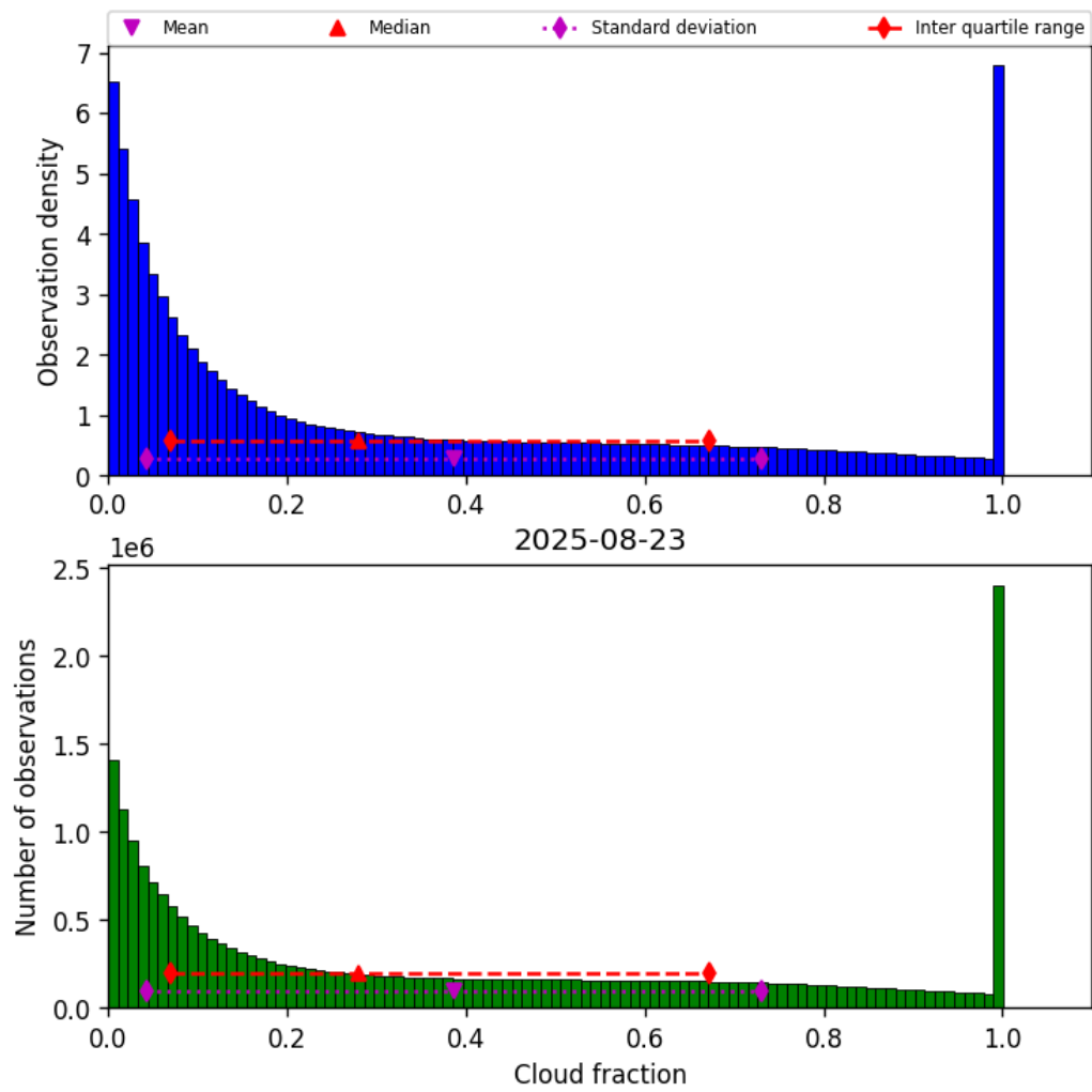
Figure 30: Histogram of “Cloud fraction” for 2025-08-23 to 2025-08-23
