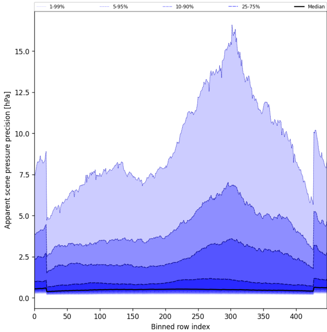
Figure 52: Along track statistics of “Apparent scene pressure precision” for 2025-08-23 to 2025-08-23
