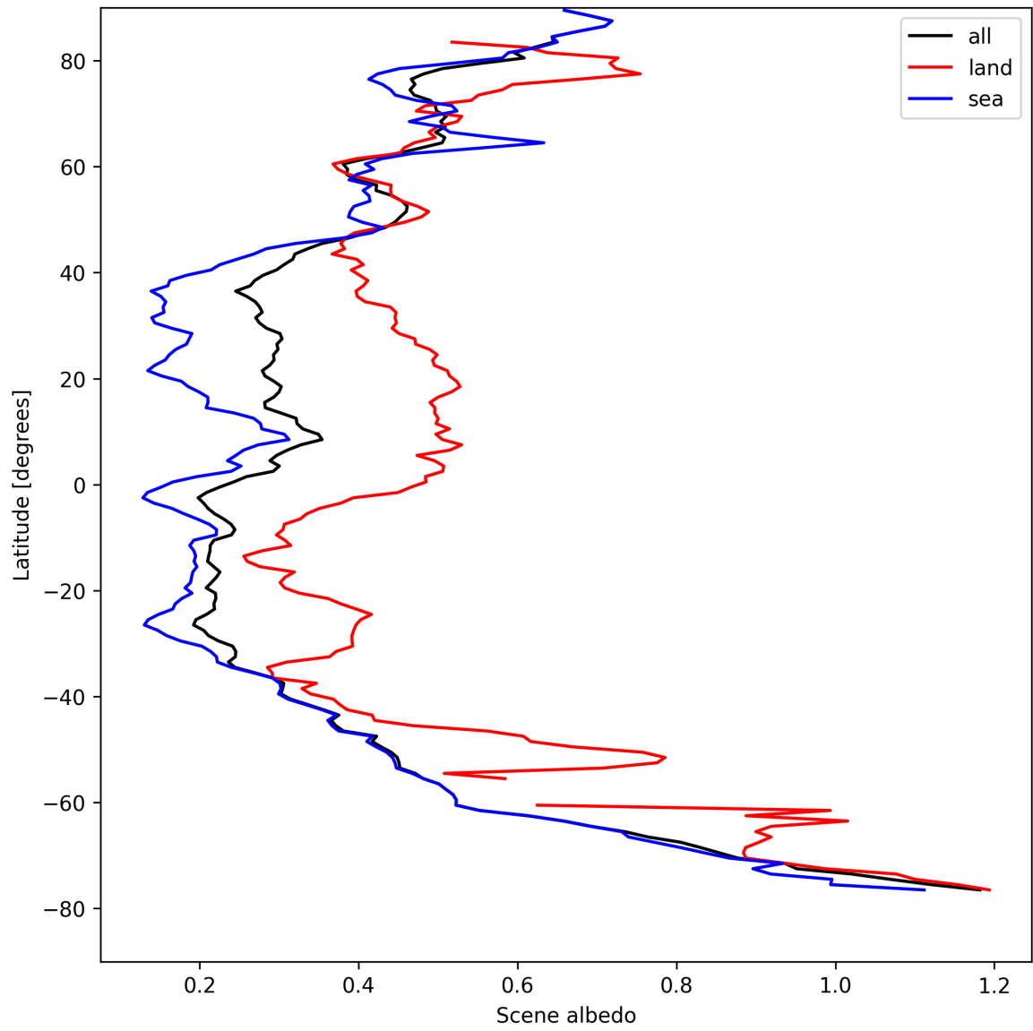
Figure 15: Zonal average of “Scene albedo” for 2025-08-23 to 2025-08-23.
