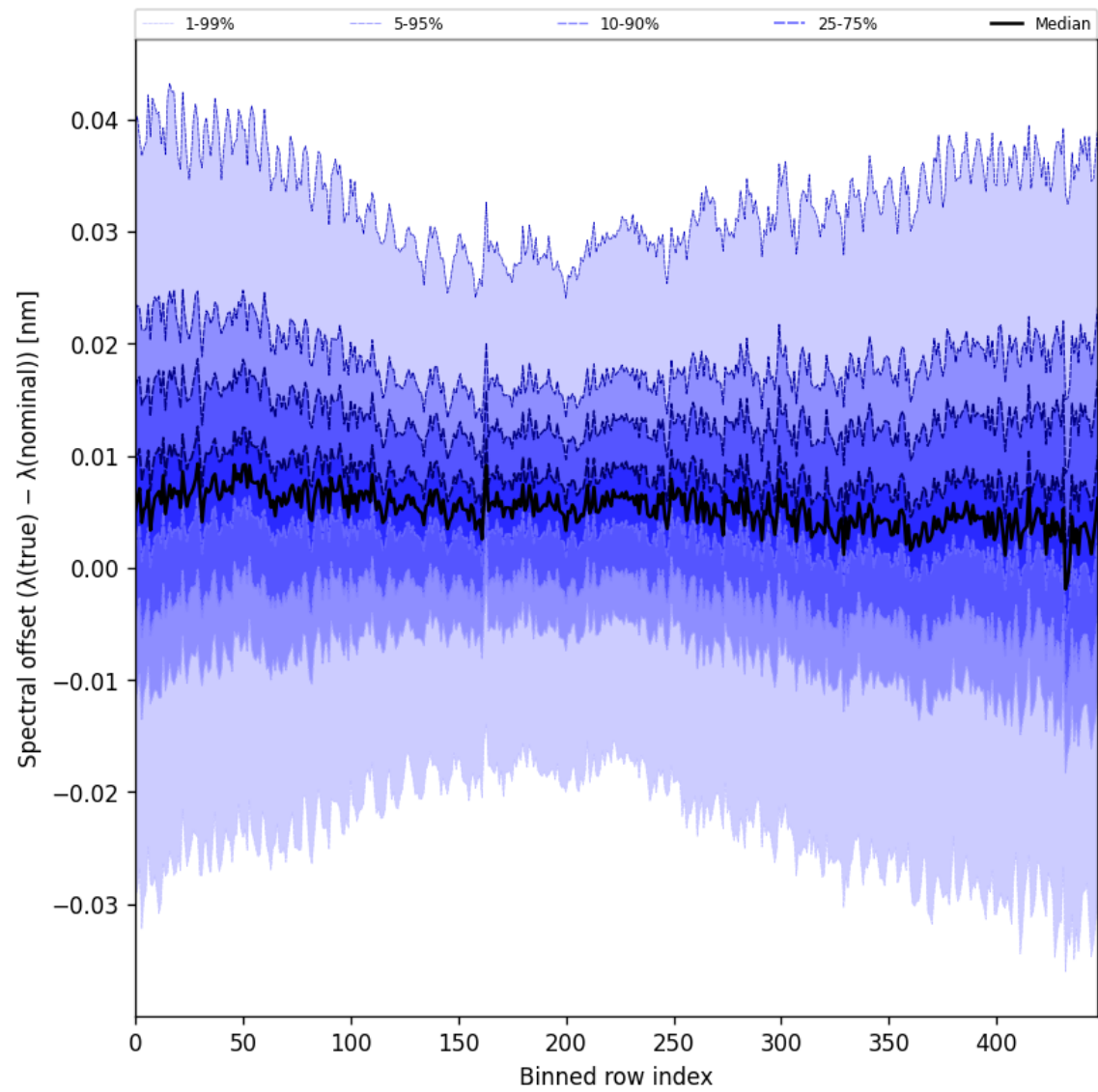
Figure 60: Along track statistics of “Spectral offset ( \lambda_{\text{true}} - \lambda_{\text{nominal}} )” for 2025-08-23 to 2025-08-23
