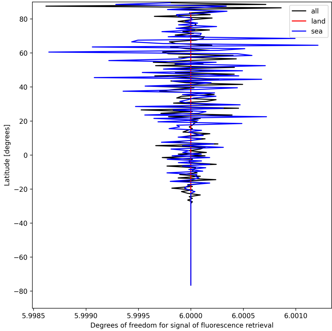
Figure 24: Zonal average of “Degrees of freedom for signal of fluorescence retrieval” for 2025-08-23 to 2025-08-23.
