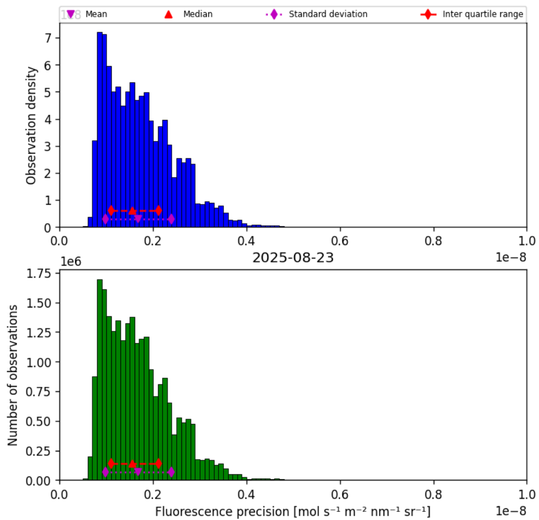
Figure 39: Histogram of “Fluorescence precision” for 2025-08-23 to 2025-08-23
