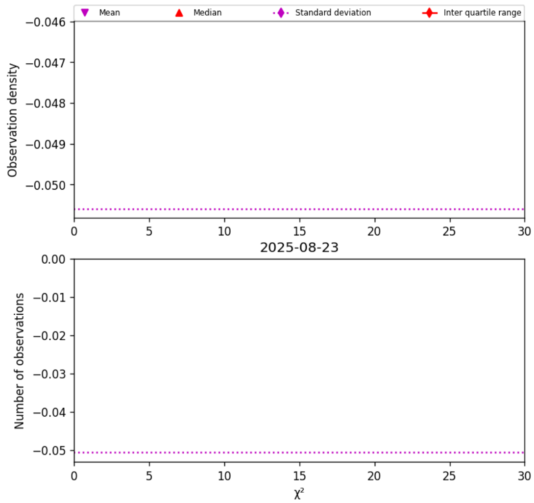
Figure 36: Histogram of " \chi^2 " for 2025-08-23 to 2025-08-23
