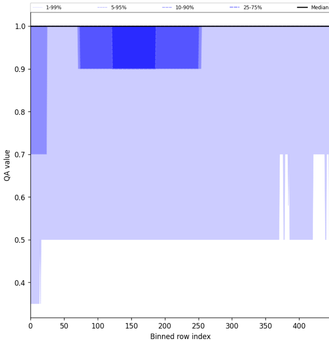
Figure 44: Along track statistics of “QA value” for 2025-08-23 to 2025-08-23
