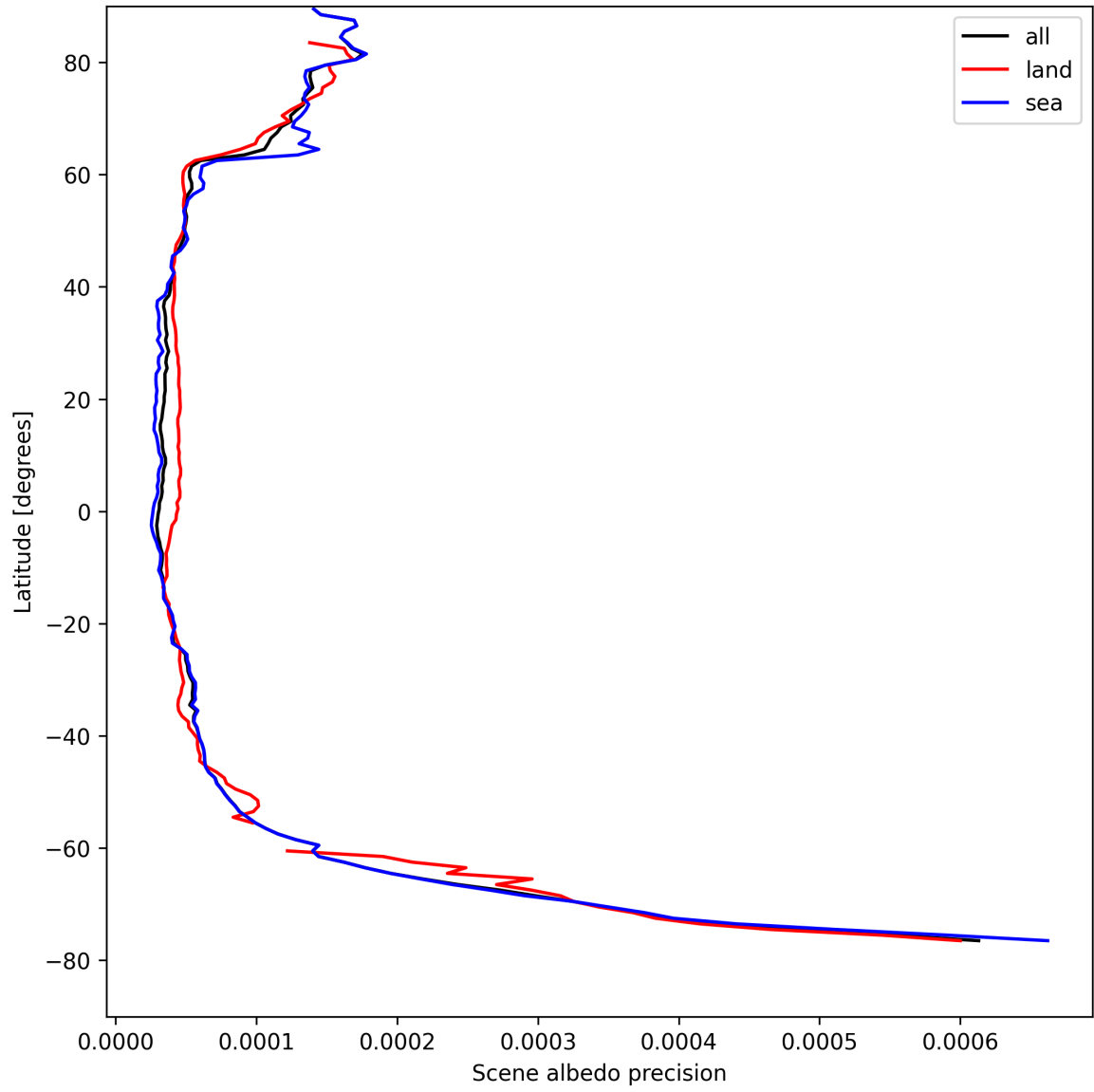
Figure 16: Zonal average of “Scene albedo precision” for 2025-08-23 to 2025-08-23.
