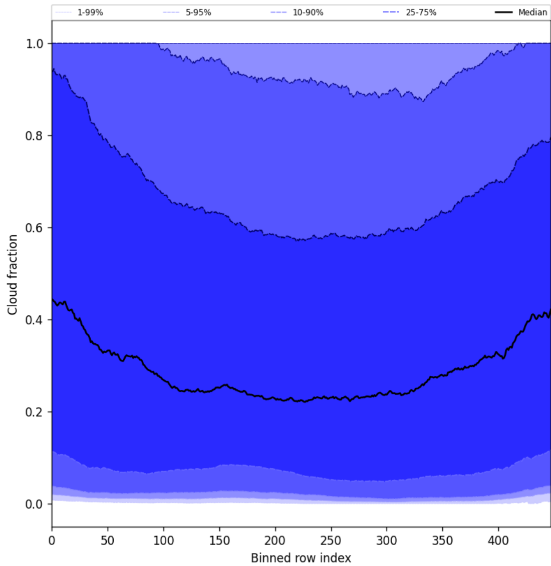
Figure 47: Along track statistics of “Cloud fraction” for 2025-08-23 to 2025-08-23
