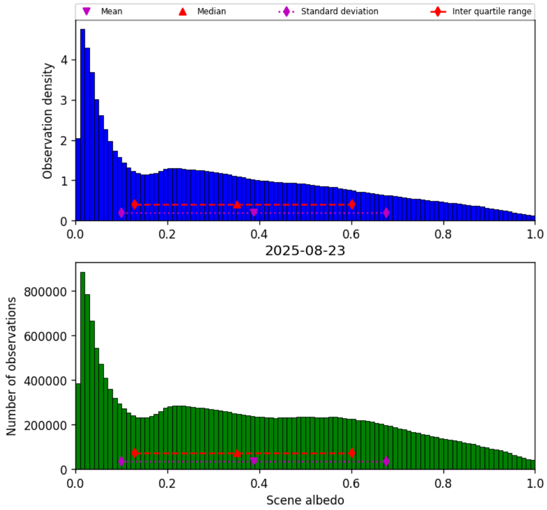
Figure 32: Histogram of “Scene albedo” for 2025-08-23 to 2025-08-23
