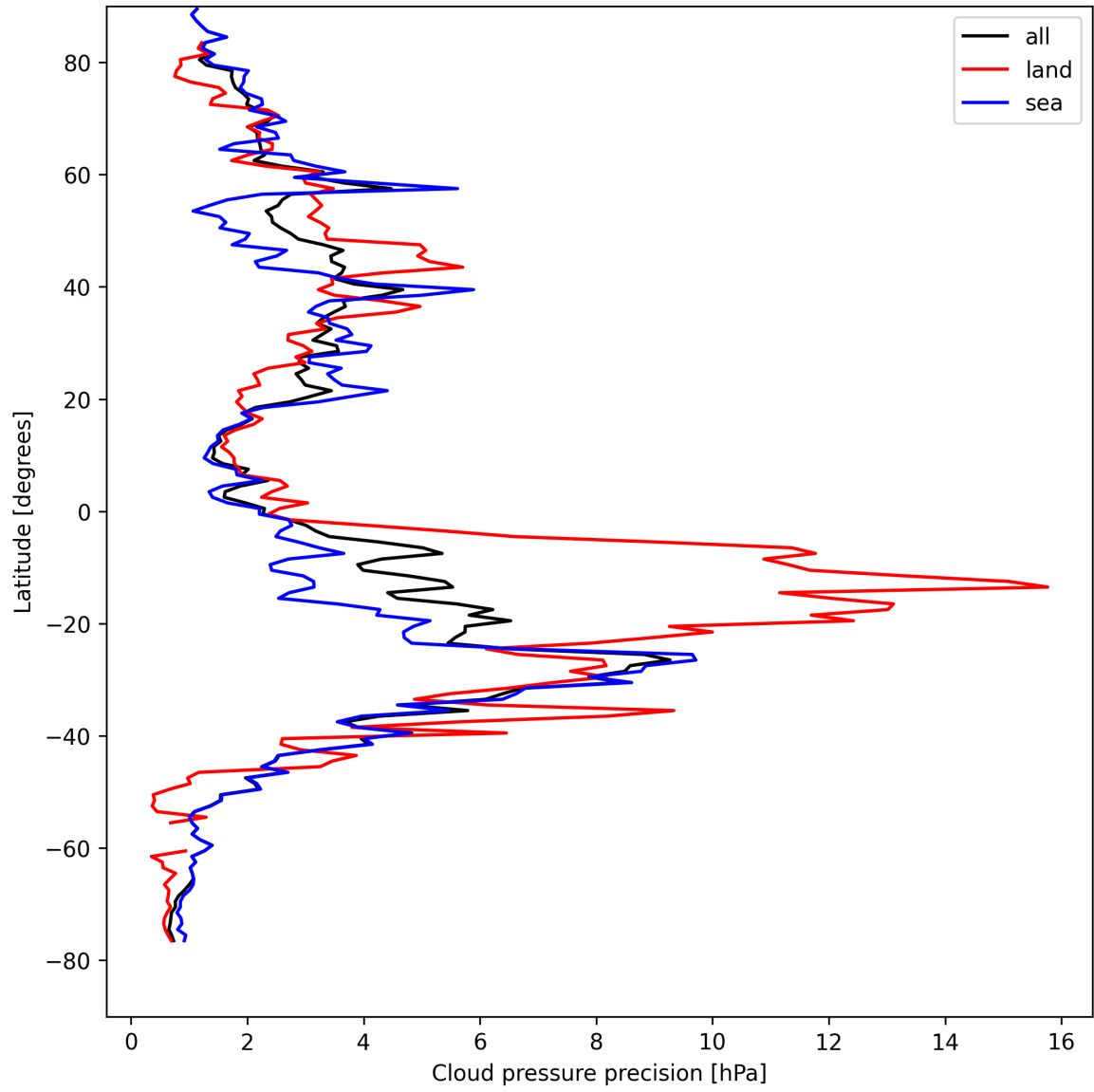
Figure 12: Zonal average of “Cloud pressure precision” for 2025-08-23 to 2025-08-23.
