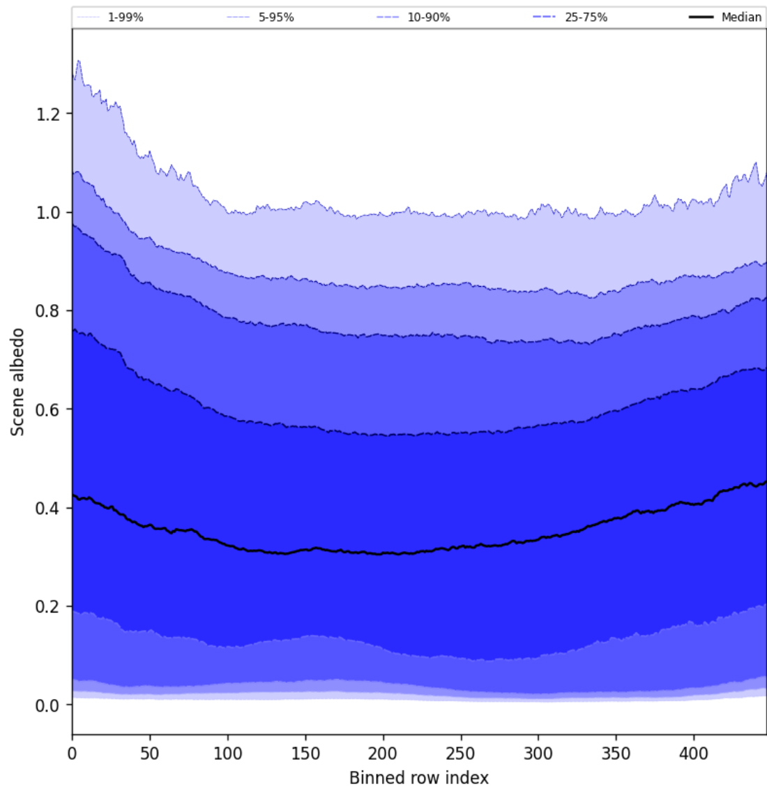
Figure 49: Along track statistics of “Scene albedo” for 2025-08-23 to 2025-08-23
