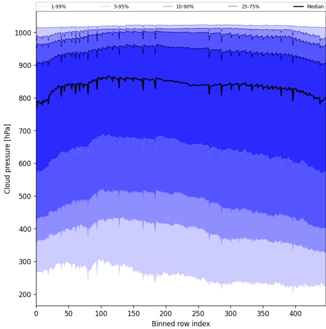
Figure 45: Along track statistics of “Cloud pressure” for 2025-08-23 to 2025-08-23
