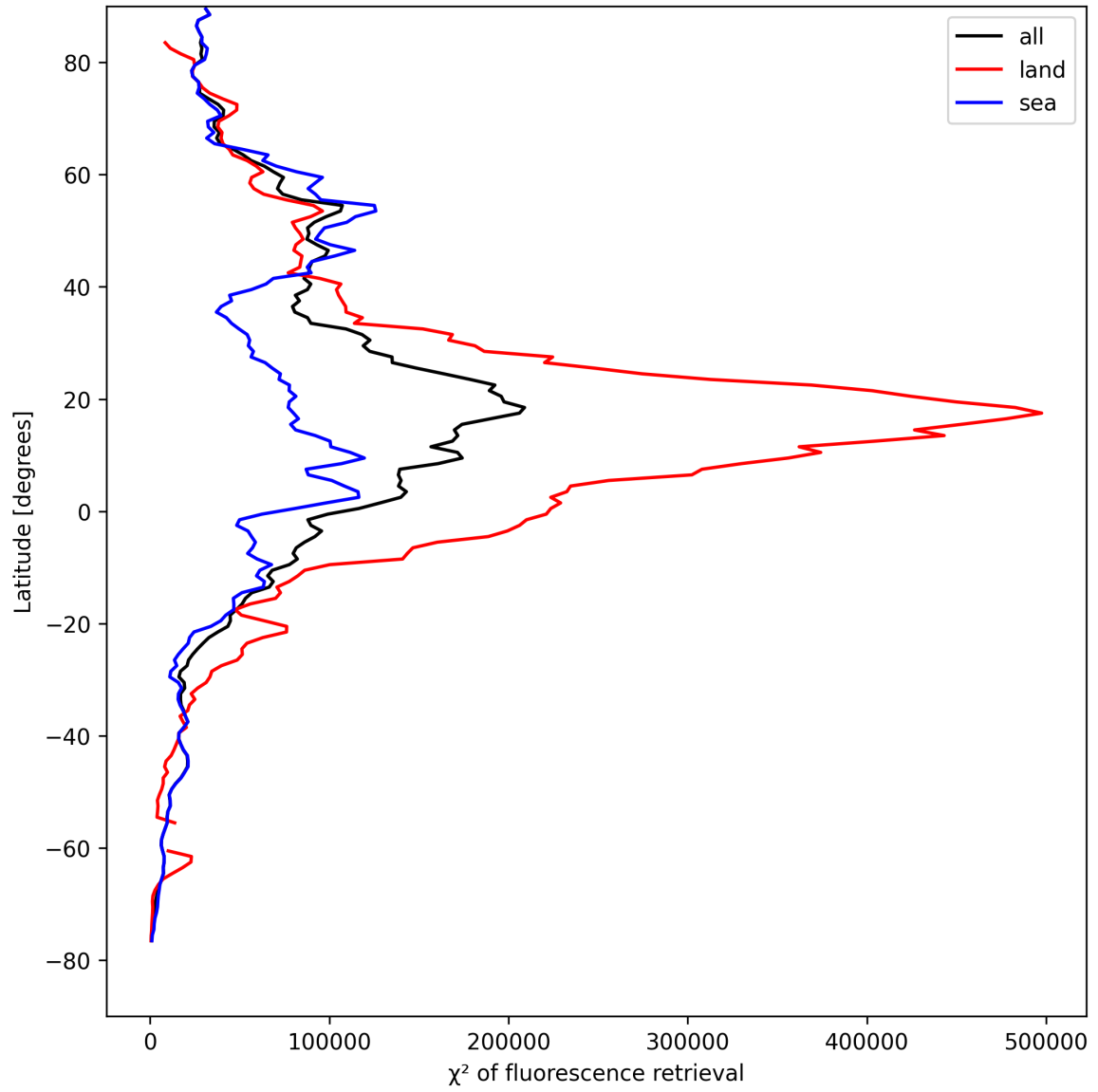
Figure 23: Zonal average of “ \chi^2 of fluorescence retrieval” for 2025-08-23 to 2025-08-23.
