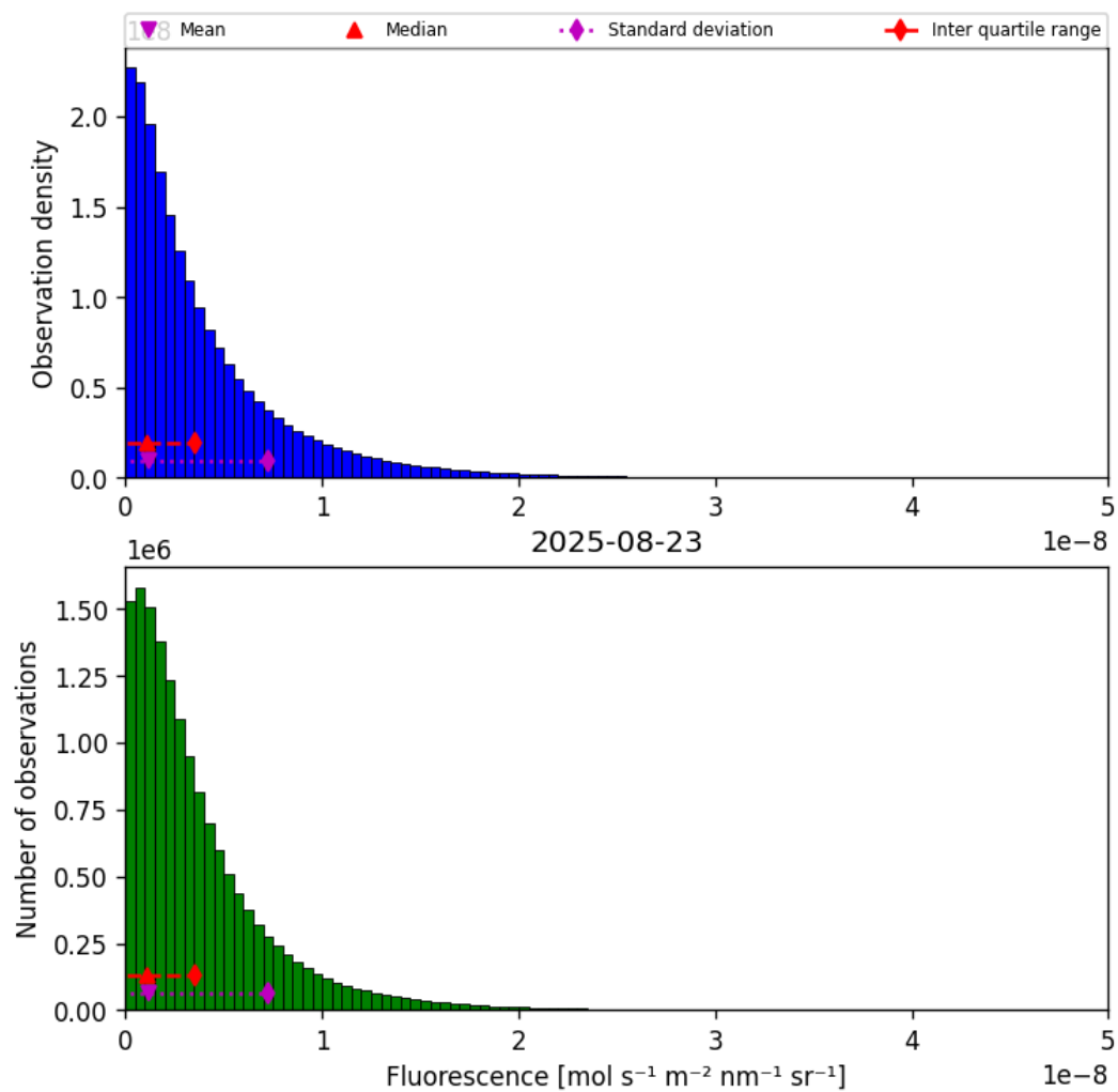
Figure 38: Histogram of “Fluorescence” for 2025-08-23 to 2025-08-23
