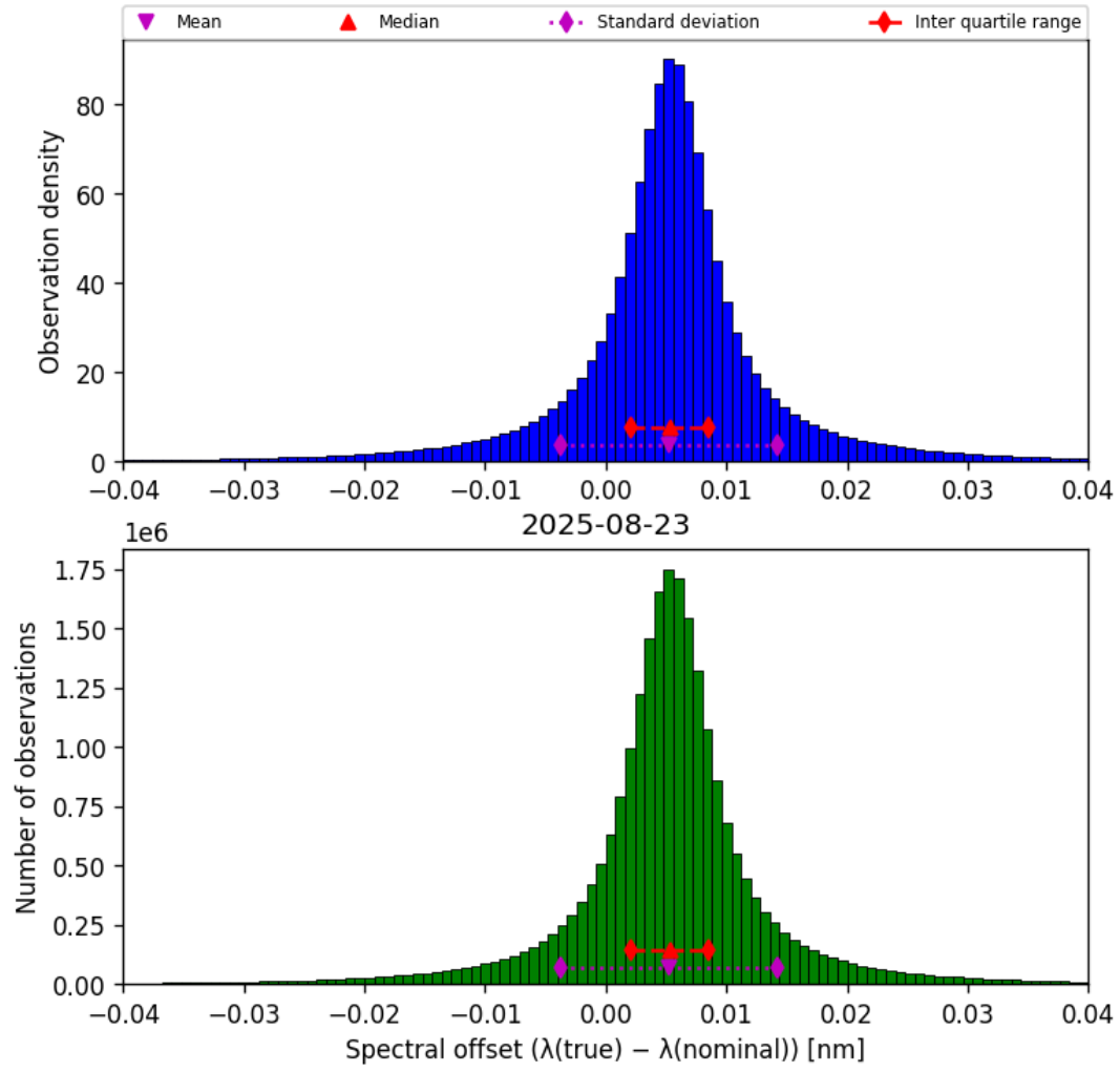
Figure 43: Histogram of “Spectral offset ( \lambda_{\text{true}} - \lambda_{\text{nominal}} )” for 2025-08-23 to 2025-08-23
