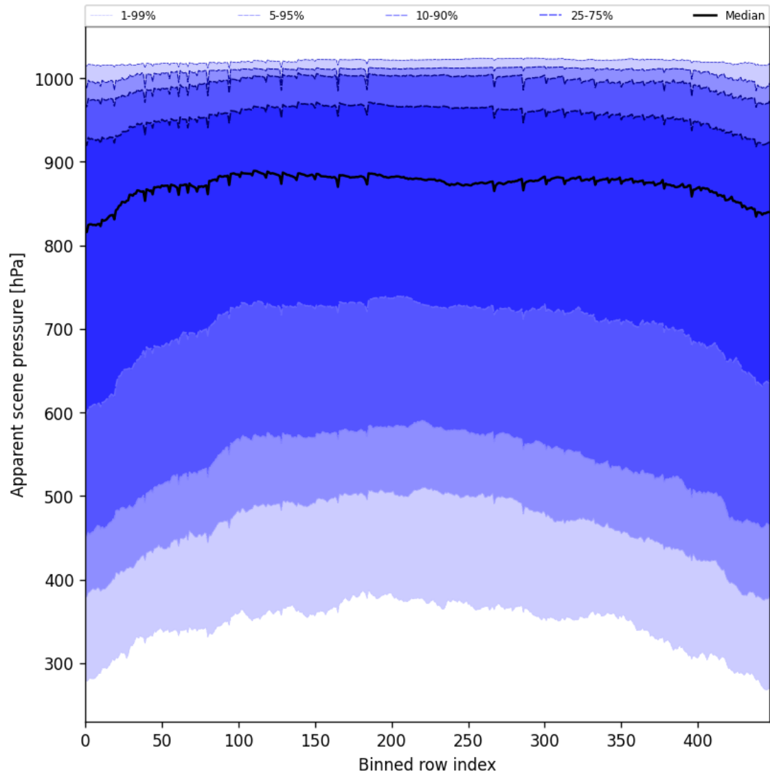
Figure 51: Along track statistics of “Apparent scene pressure” for 2025-08-23 to 2025-08-23
