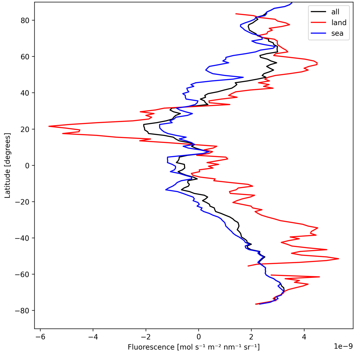
Figure 21: Zonal average of “Fluorescence” for 2025-08-23 to 2025-08-23.
