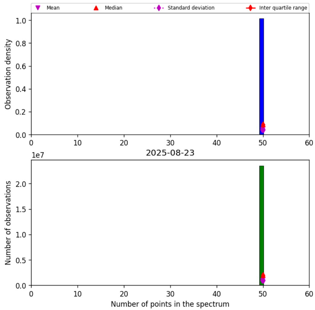
Figure 42: Histogram of "Number of points in the spectrum" for 2025-08-23 to 2025-08-23
