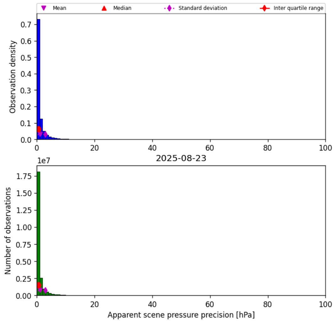
Figure 35: Histogram of “Apparent scene pressure precision” for 2025-08-23 to 2025-08-23
