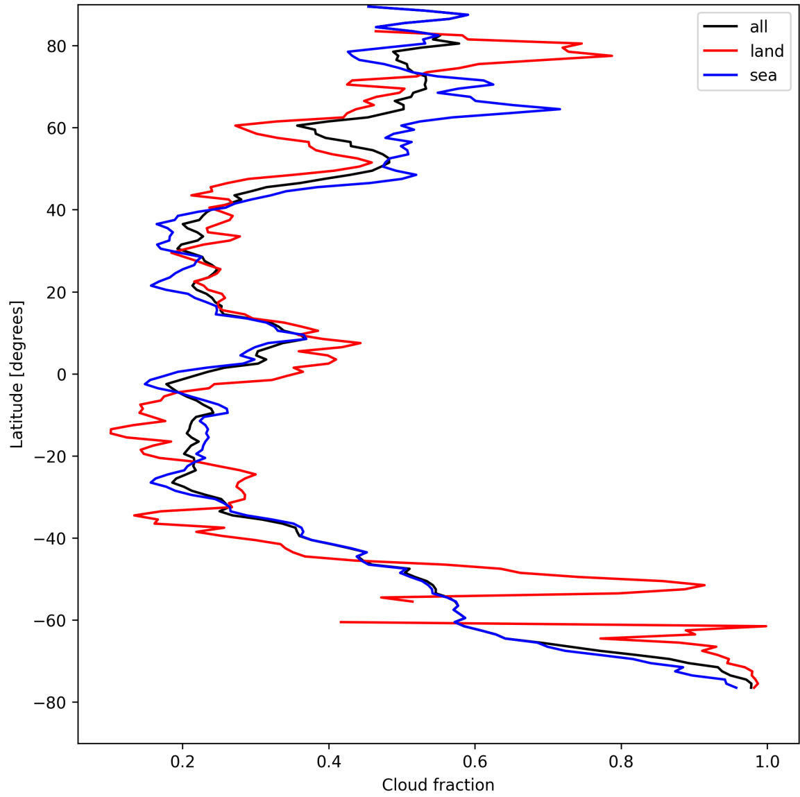
Figure 13: Zonal average of “Cloud fraction” for 2025-08-23 to 2025-08-23.
