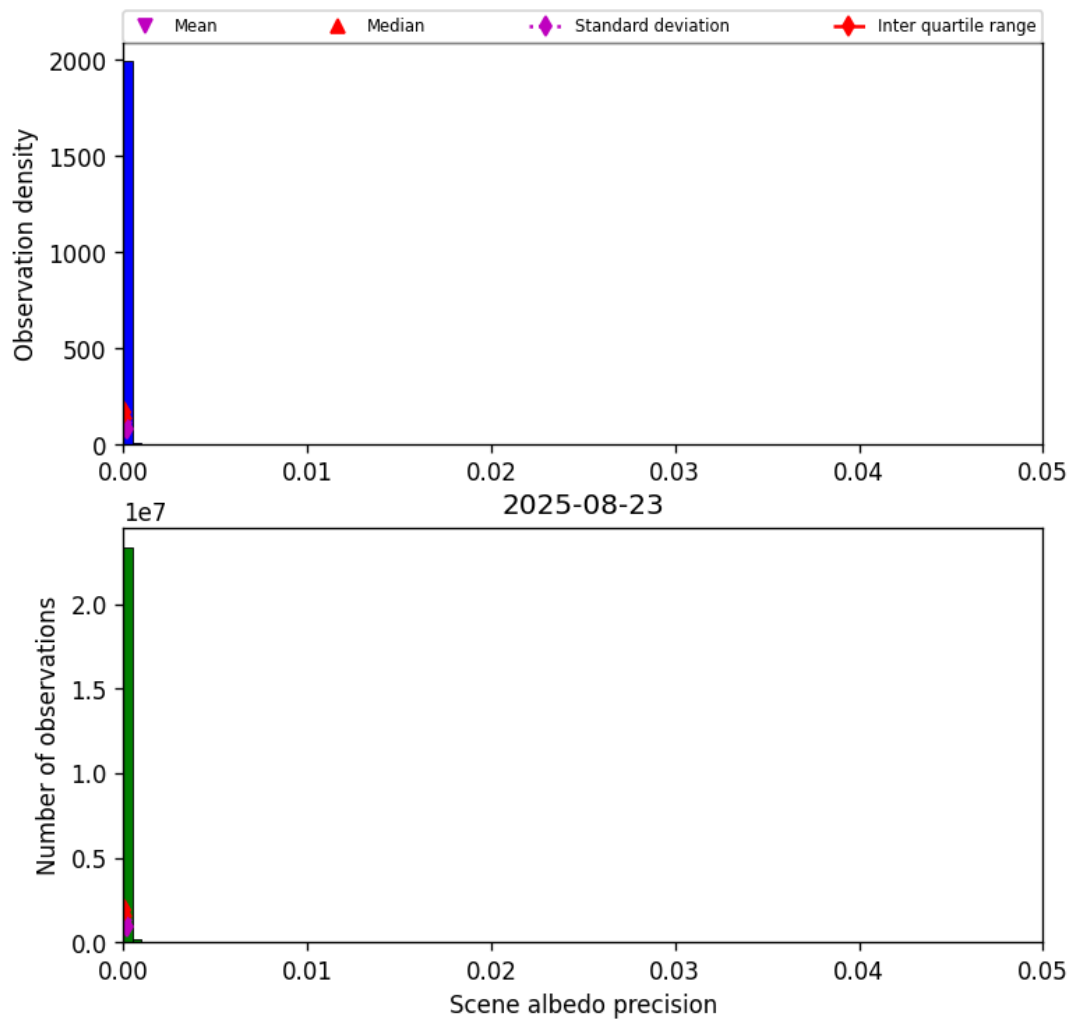
Figure 33: Histogram of “Scene albedo precision” for 2025-08-23 to 2025-08-23
