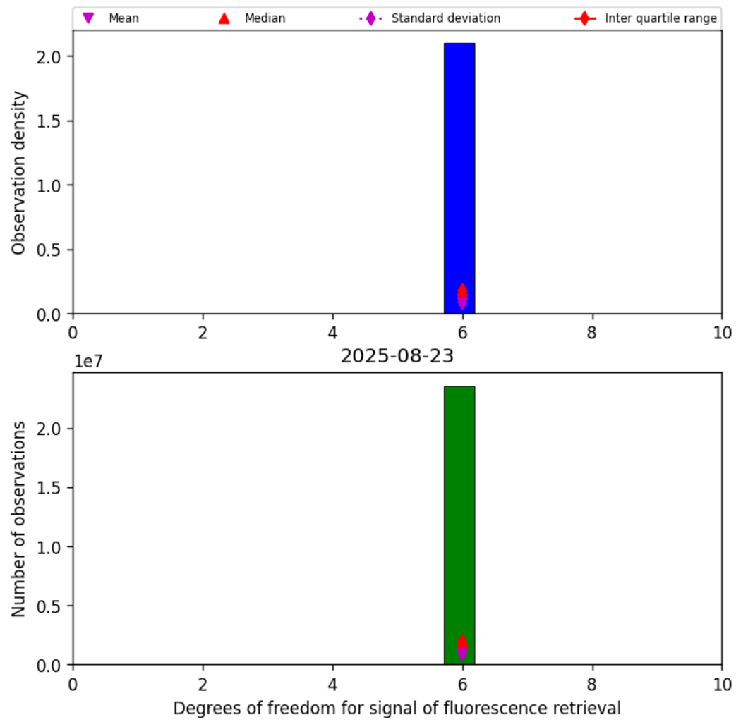
Figure 41: Histogram of “Degrees of freedom for signal of fluorescence retrieval” for 2025-08-23 to 2025-08-23
