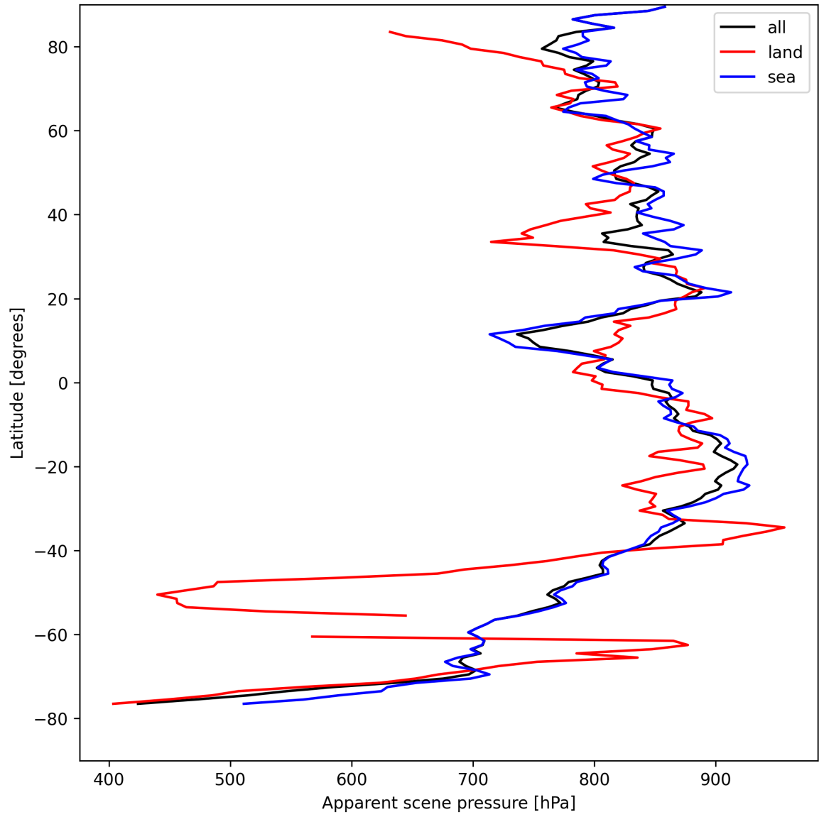
Figure 17: Zonal average of “Apparent scene pressure” for 2025-08-23 to 2025-08-23.
