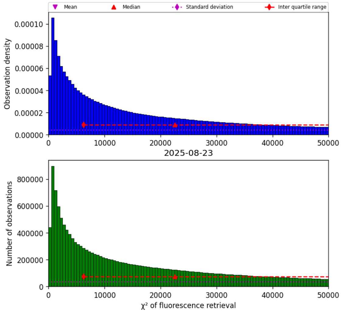
Figure 40: Histogram of “ \chi^2 of fluorescence retrieval” for 2025-08-23 to 2025-08-23
