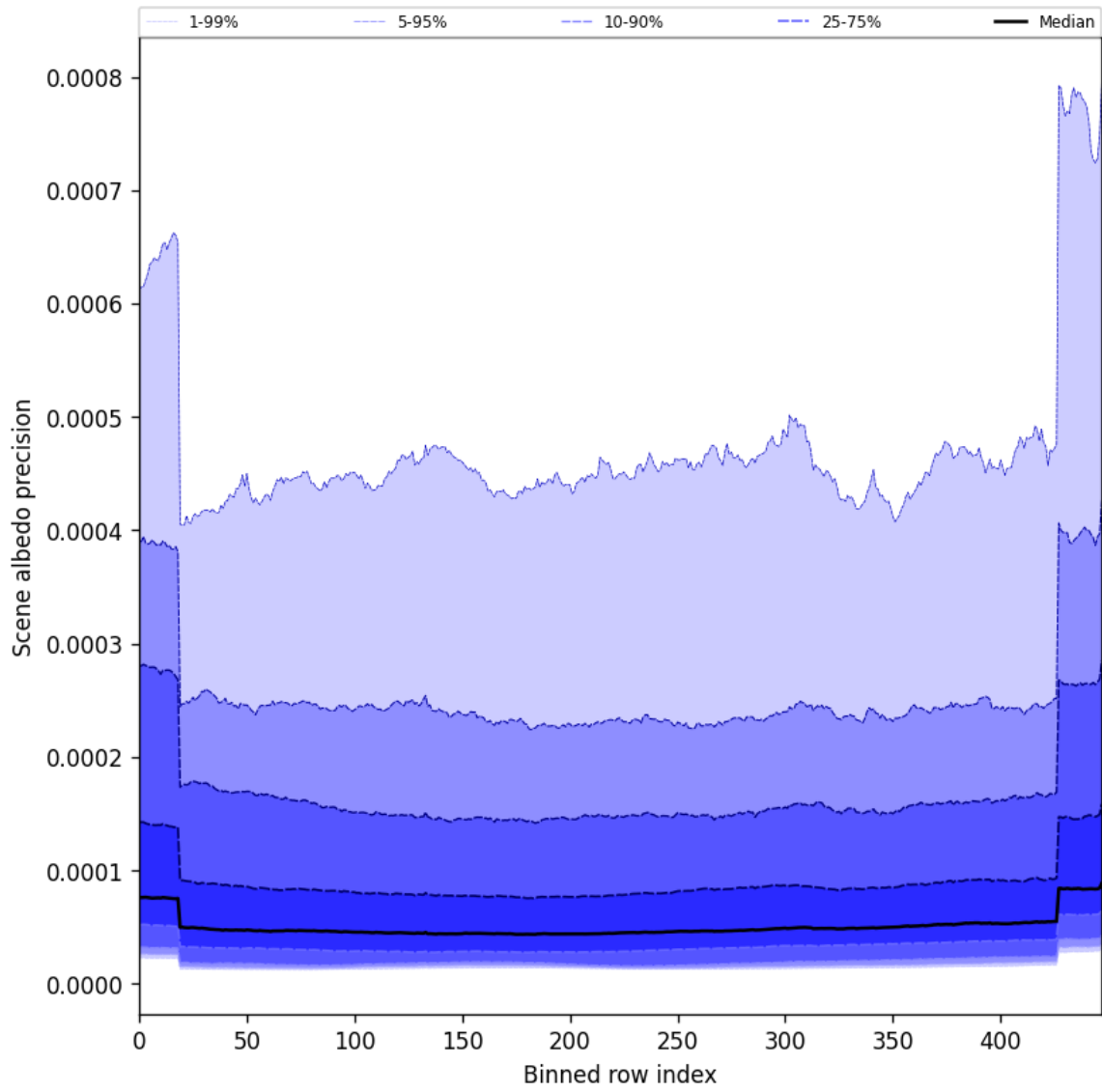
Figure 50: Along track statistics of “Scene albedo precision” for 2025-08-23 to 2025-08-23
