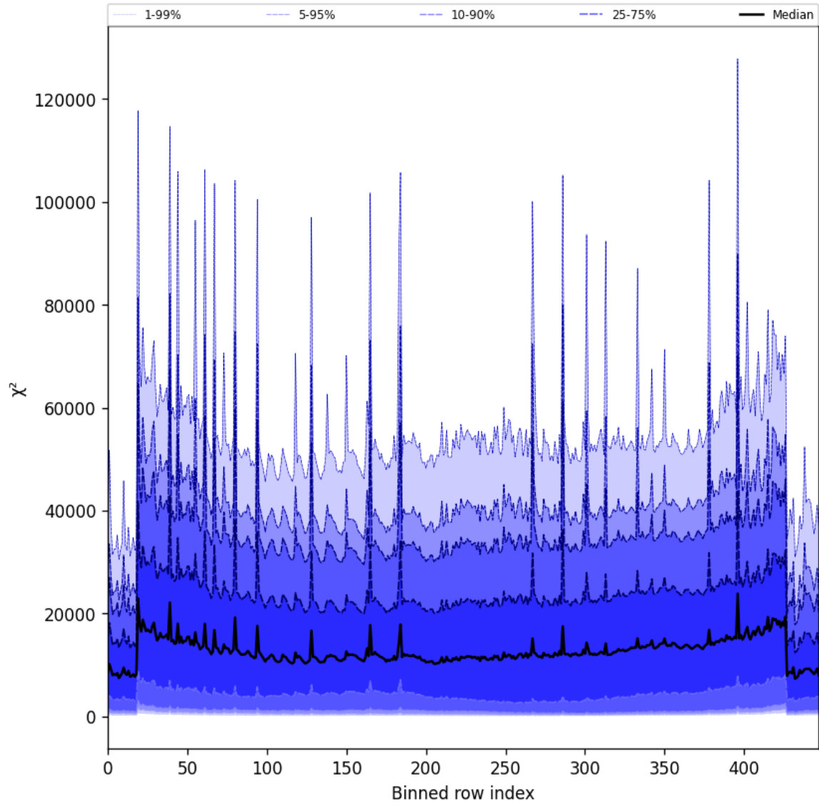
Figure 53: Along track statistics of “ \chi^2 ” for 2025-08-23 to 2025-08-23
