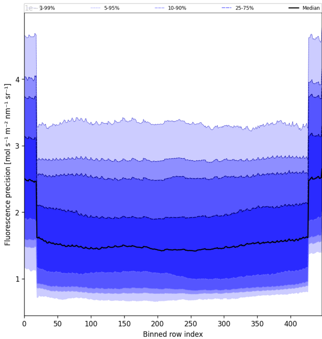
Figure 56: Along track statistics of “Fluorescence precision” for 2025-08-23 to 2025-08-23
