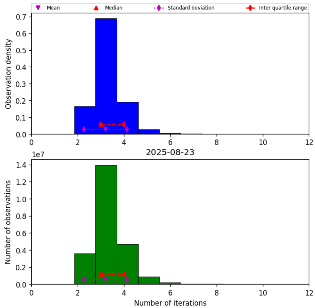
Figure 37: Histogram of “Number of iterations” for 2025-08-23 to 2025-08-23
