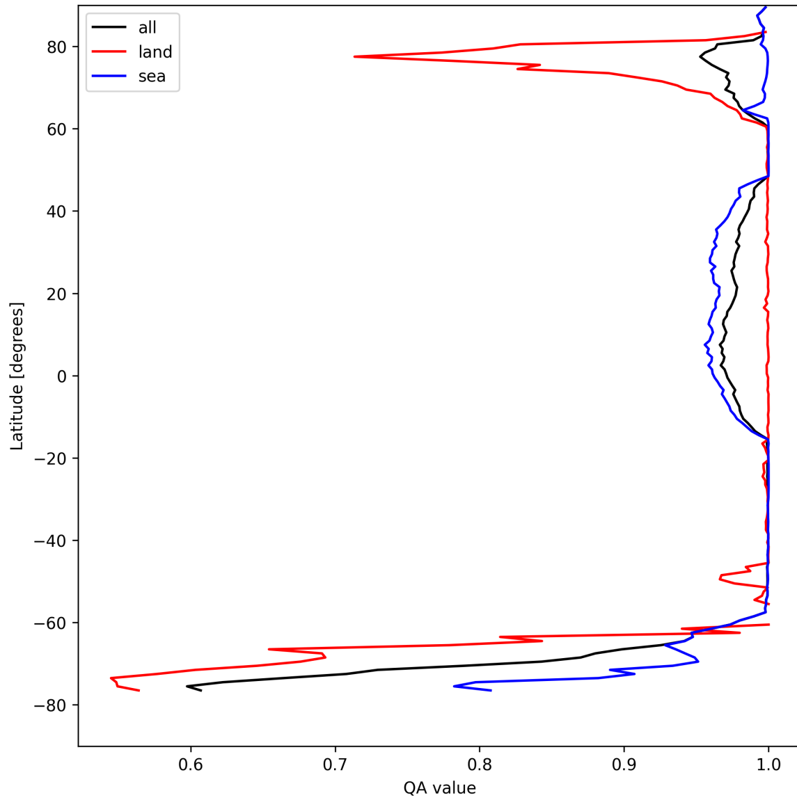
Figure 10: Zonal average of “QA value” for 2025-08-23 to 2025-08-23.
