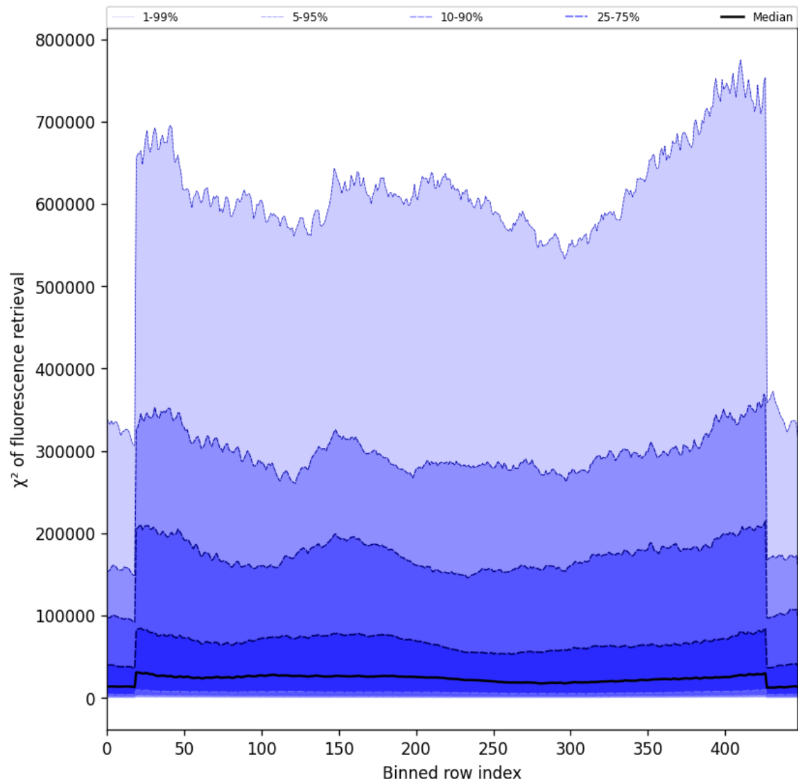
Figure 57: Along track statistics of “ \chi^2 of fluorescence retrieval” for 2025-08-23 to 2025-08-23
