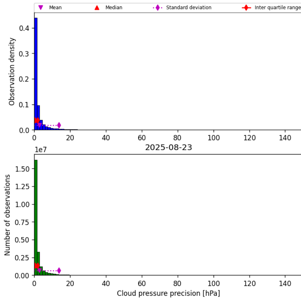
Figure 29: Histogram of “Cloud pressure precision” for 2025-08-23 to 2025-08-23
