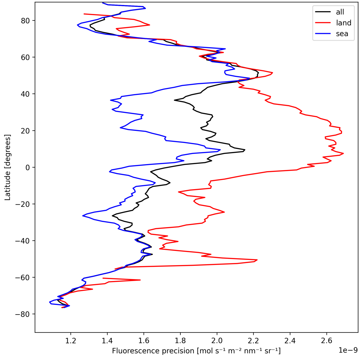
Figure 22: Zonal average of “Fluorescence precision” for 2025-08-23 to 2025-08-23.
