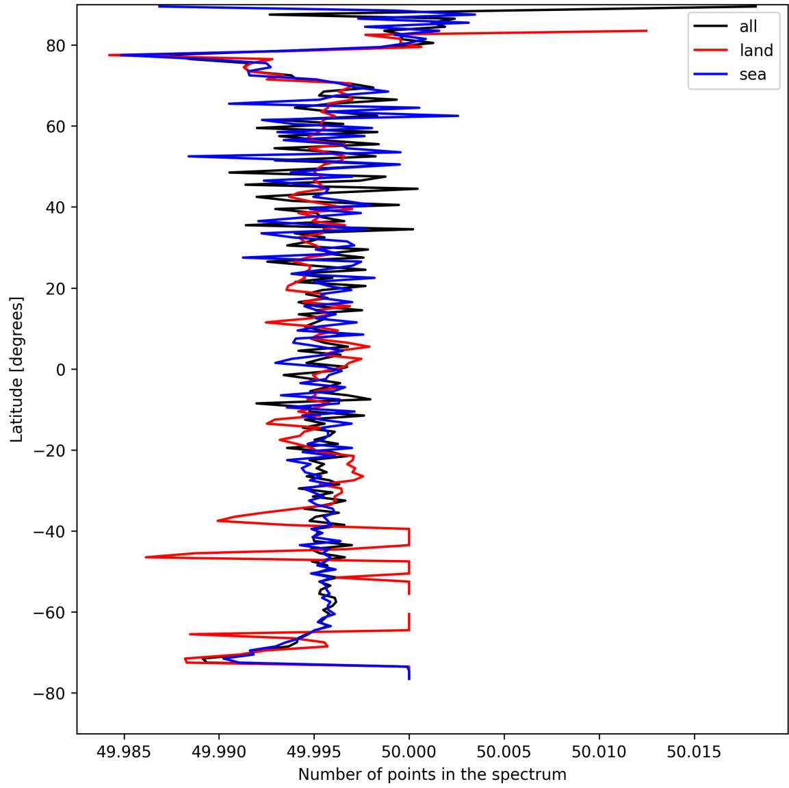
Figure 25: Zonal average of “Number of points in the spectrum” for 2025-08-23 to 2025-08-23.
