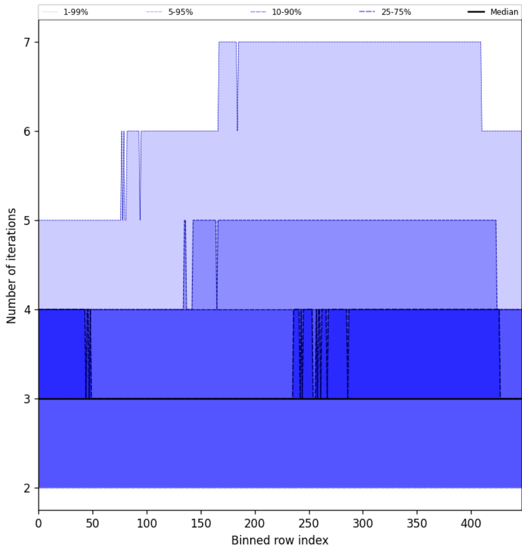
Figure 54: Along track statistics of “Number of iterations” for 2025-08-23 to 2025-08-23
