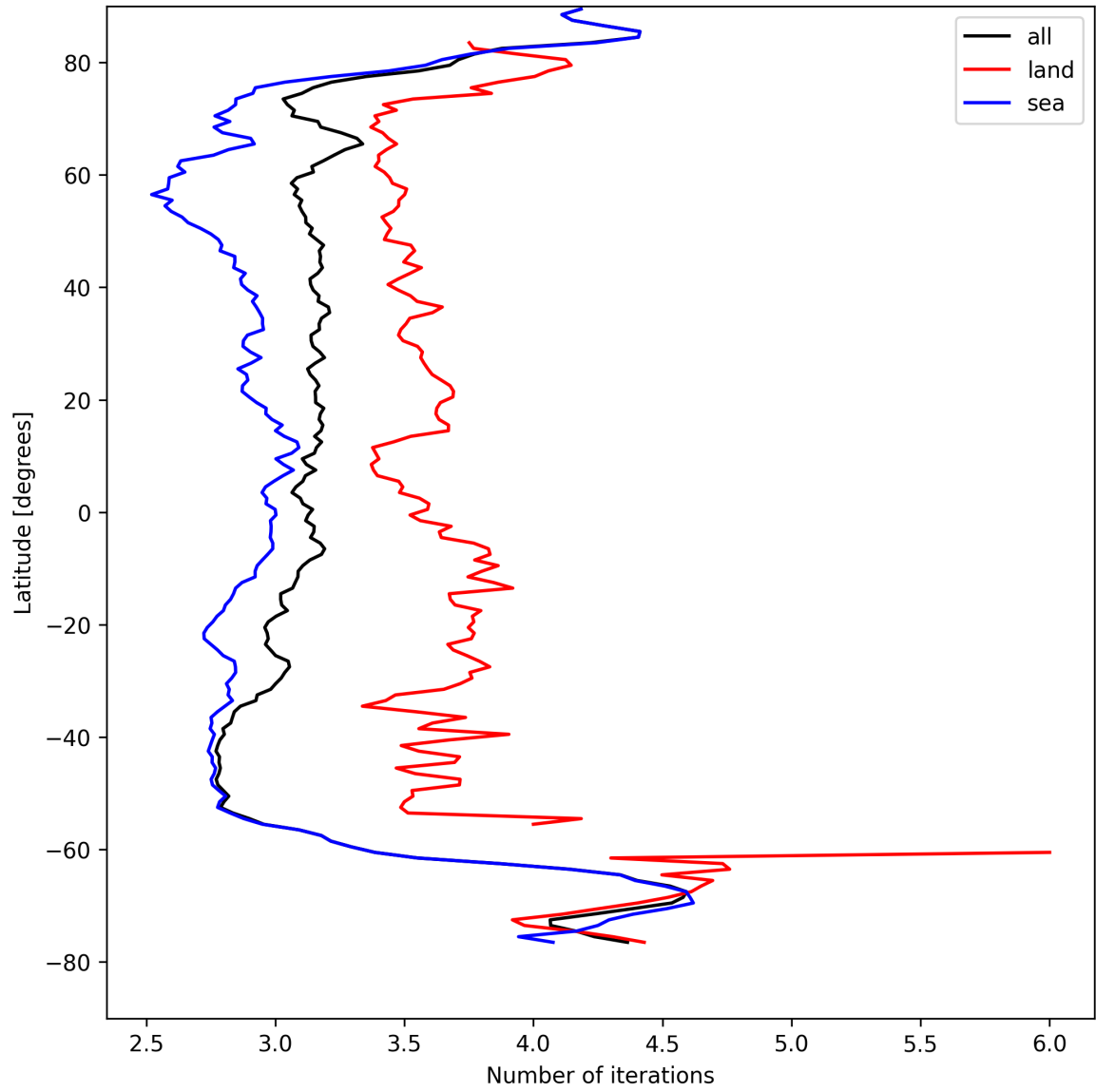
Figure 20: Zonal average of “Number of iterations” for 2025-08-23 to 2025-08-23.
