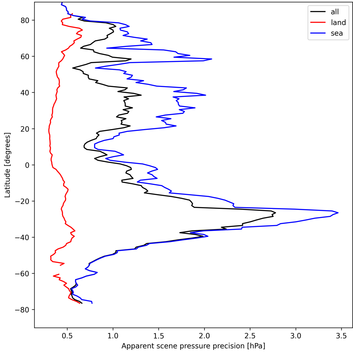
Figure 18: Zonal average of “Apparent scene pressure precision” for 2025-08-23 to 2025-08-23.
