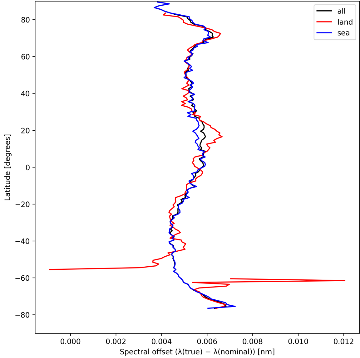
Figure 26: Zonal average of “Spectral offset ( \lambda_{\text{true}} - \lambda_{\text{nominal}} )” for 2025-08-23 to 2025-08-23.
