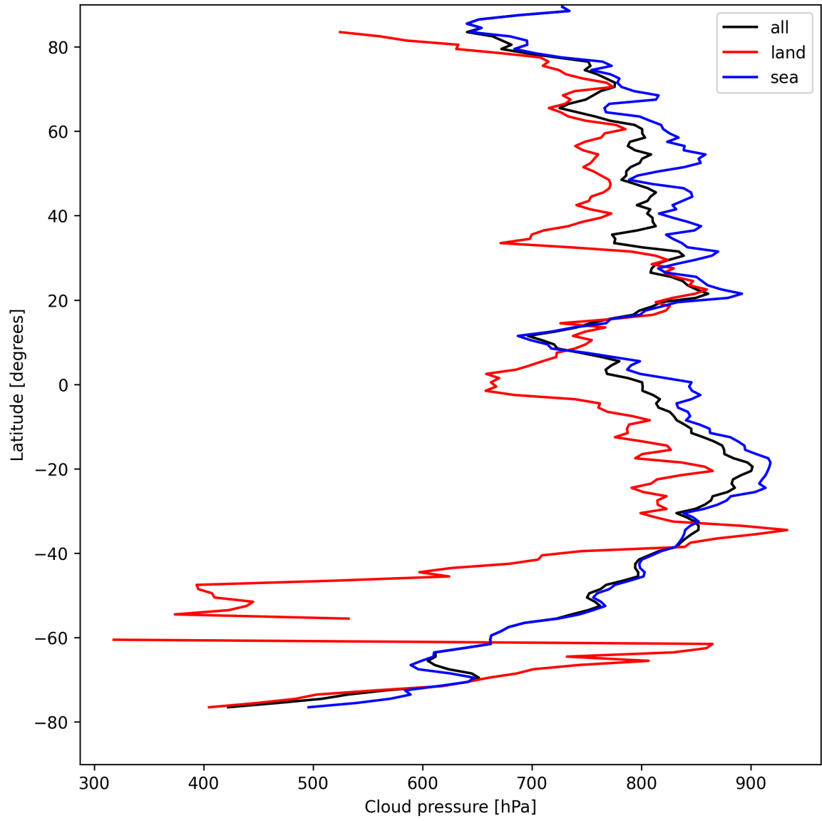
Figure 11: Zonal average of “Cloud pressure” for 2025-08-23 to 2025-08-23.
