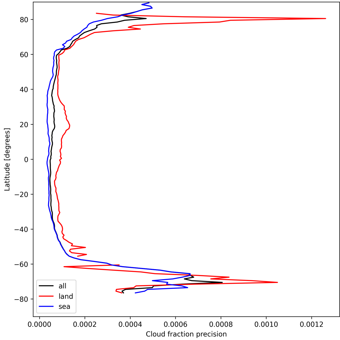
Figure 14: Zonal average of “Cloud fraction precision” for 2025-08-23 to 2025-08-23.
