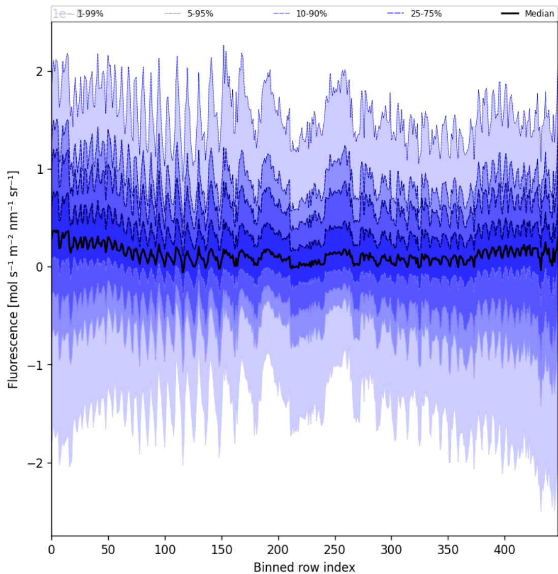
Figure 55: Along track statistics of “Fluorescence” for 2025-08-23 to 2025-08-23
