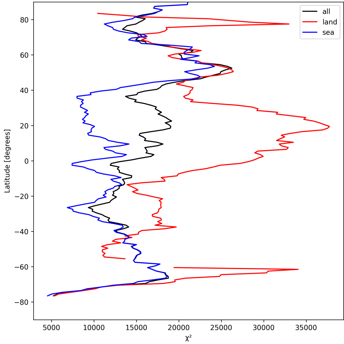
Figure 19: Zonal average of “ \chi^2 ” for 2025-08-23 to 2025-08-23.
