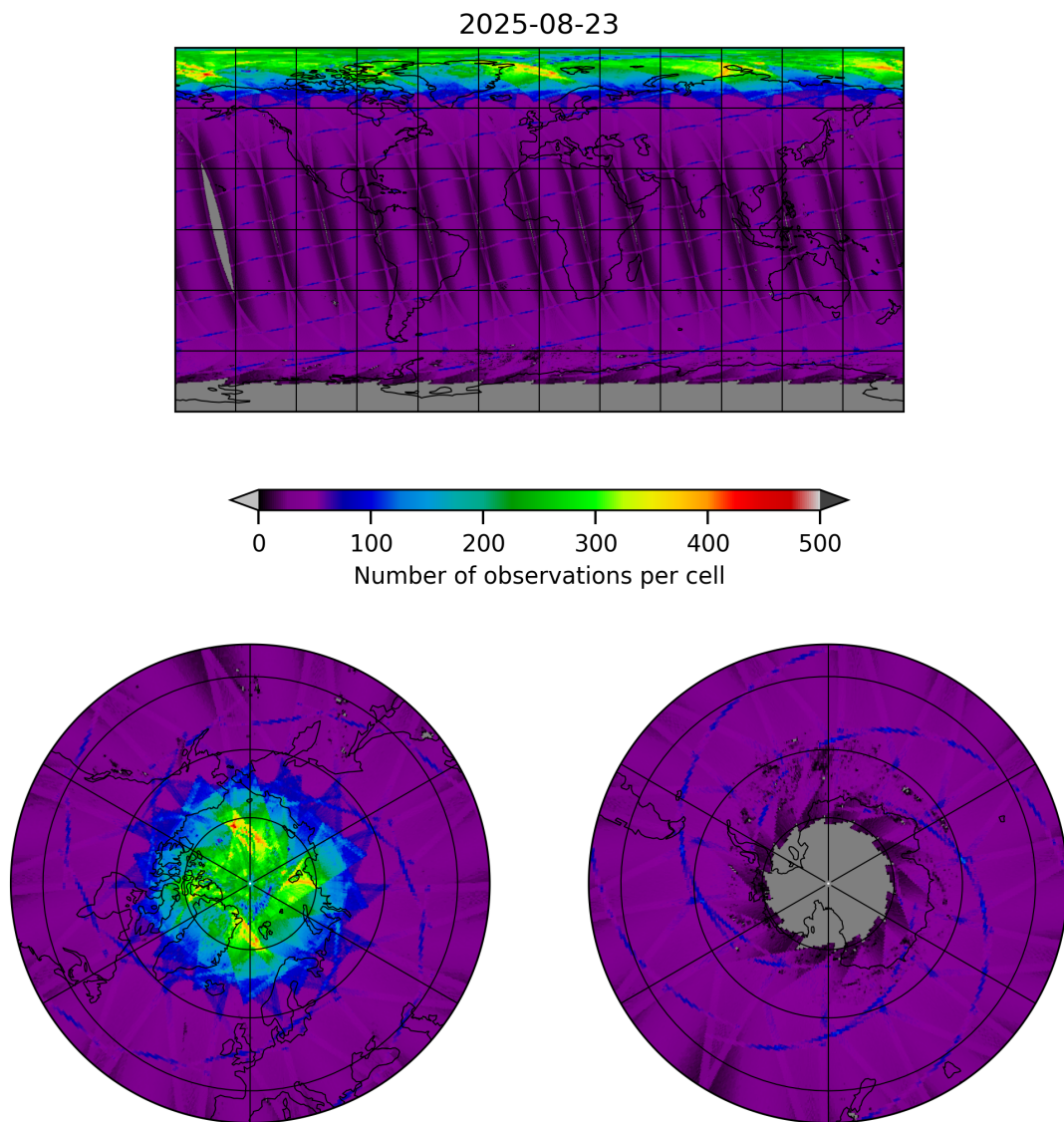
Figure 9: Map of the number of observations for 2025-08-23 to 2025-08-23
