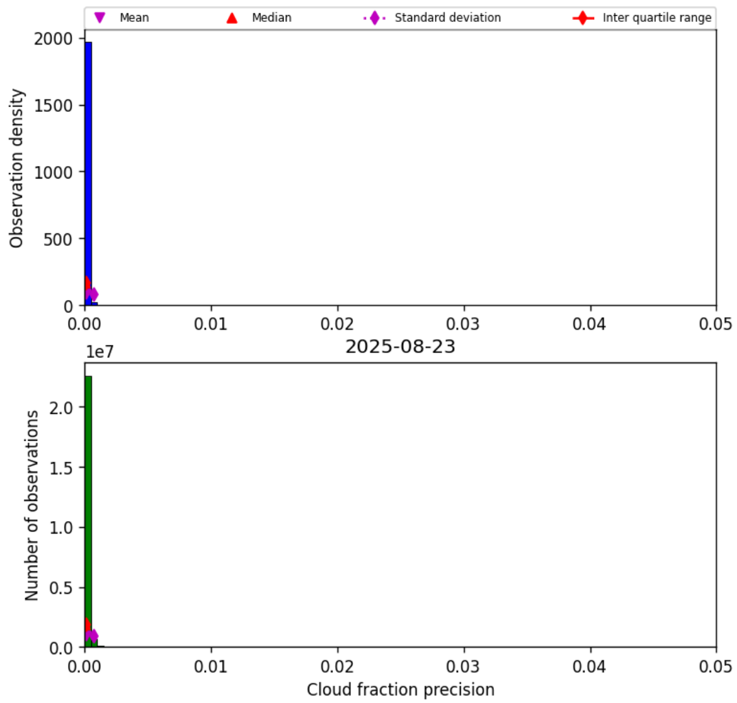
Figure 31: Histogram of “Cloud fraction precision” for 2025-08-23 to 2025-08-23
