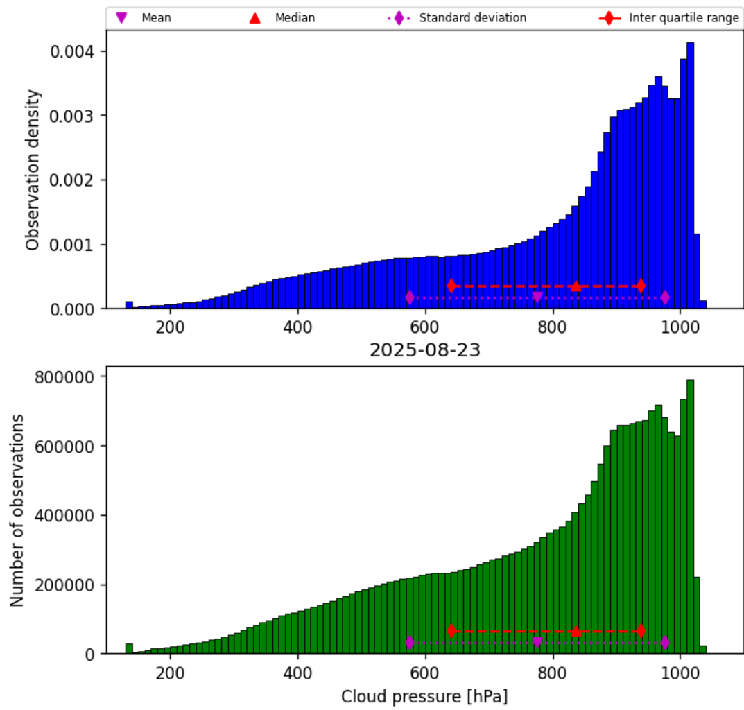
Figure 28: Histogram of “Cloud pressure” for 2025-08-23 to 2025-08-23
