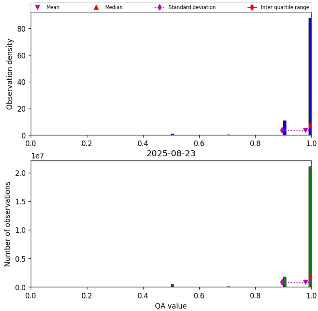
Figure 27: Histogram of “QA value” for 2025-08-23 to 2025-08-23
