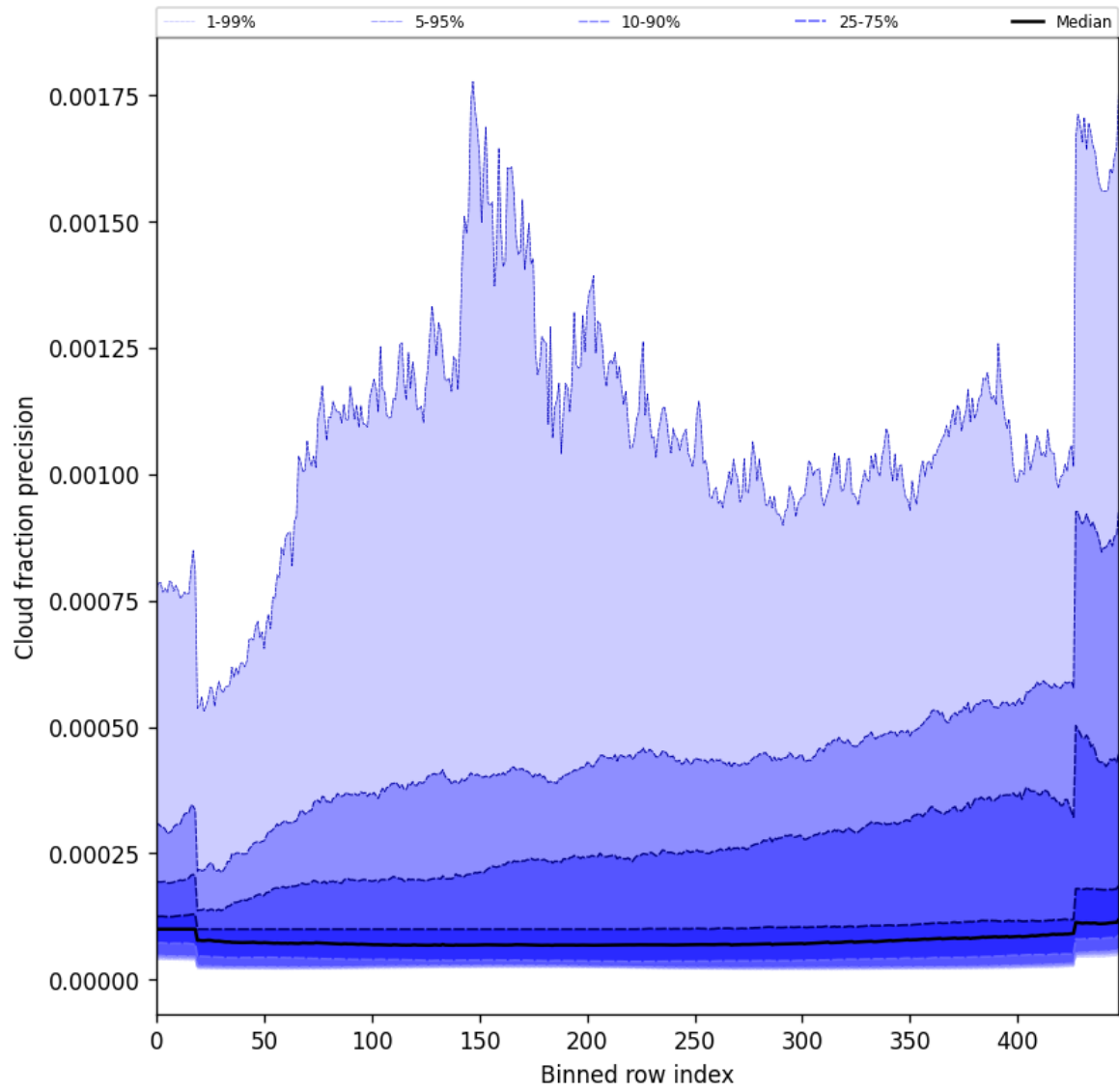
Figure 48: Along track statistics of “Cloud fraction precision” for 2025-08-23 to 2025-08-23
