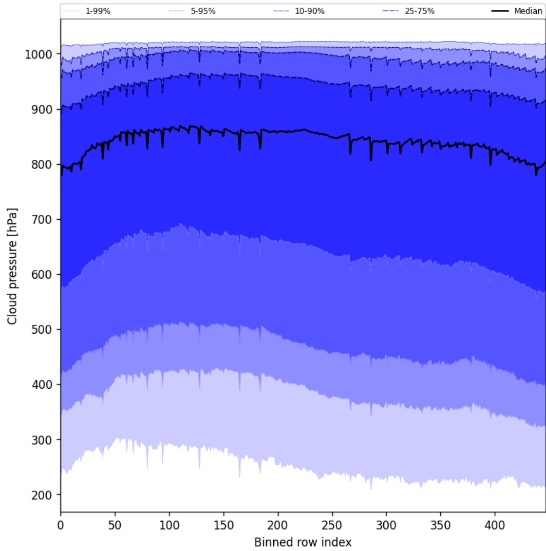
Figure 45: Along track statistics of “Cloud pressure” for 2025-08-25 to 2025-08-26
