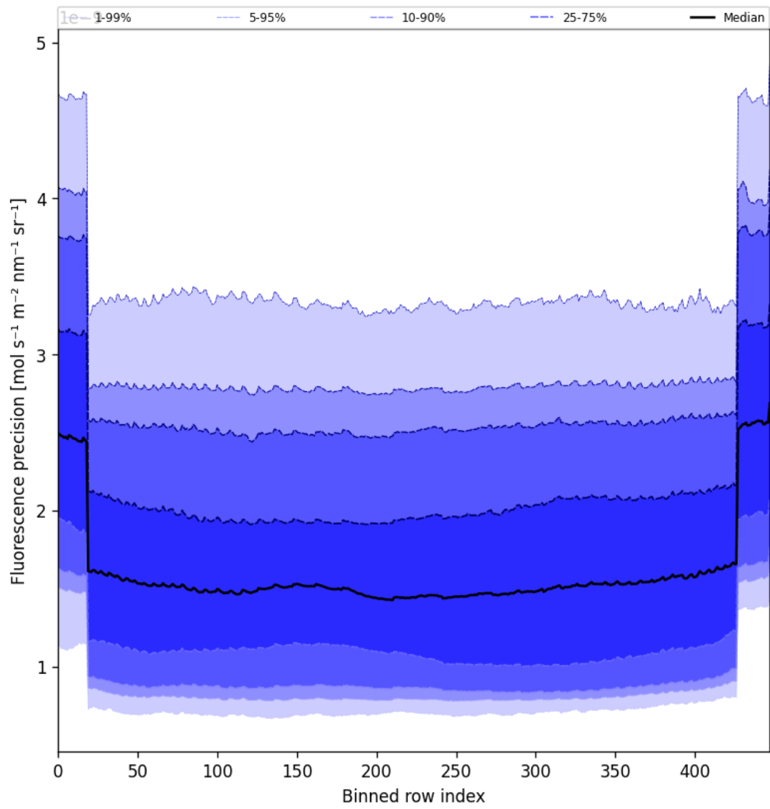
Figure 56: Along track statistics of “Fluorescence precision” for 2025-08-25 to 2025-08-26
