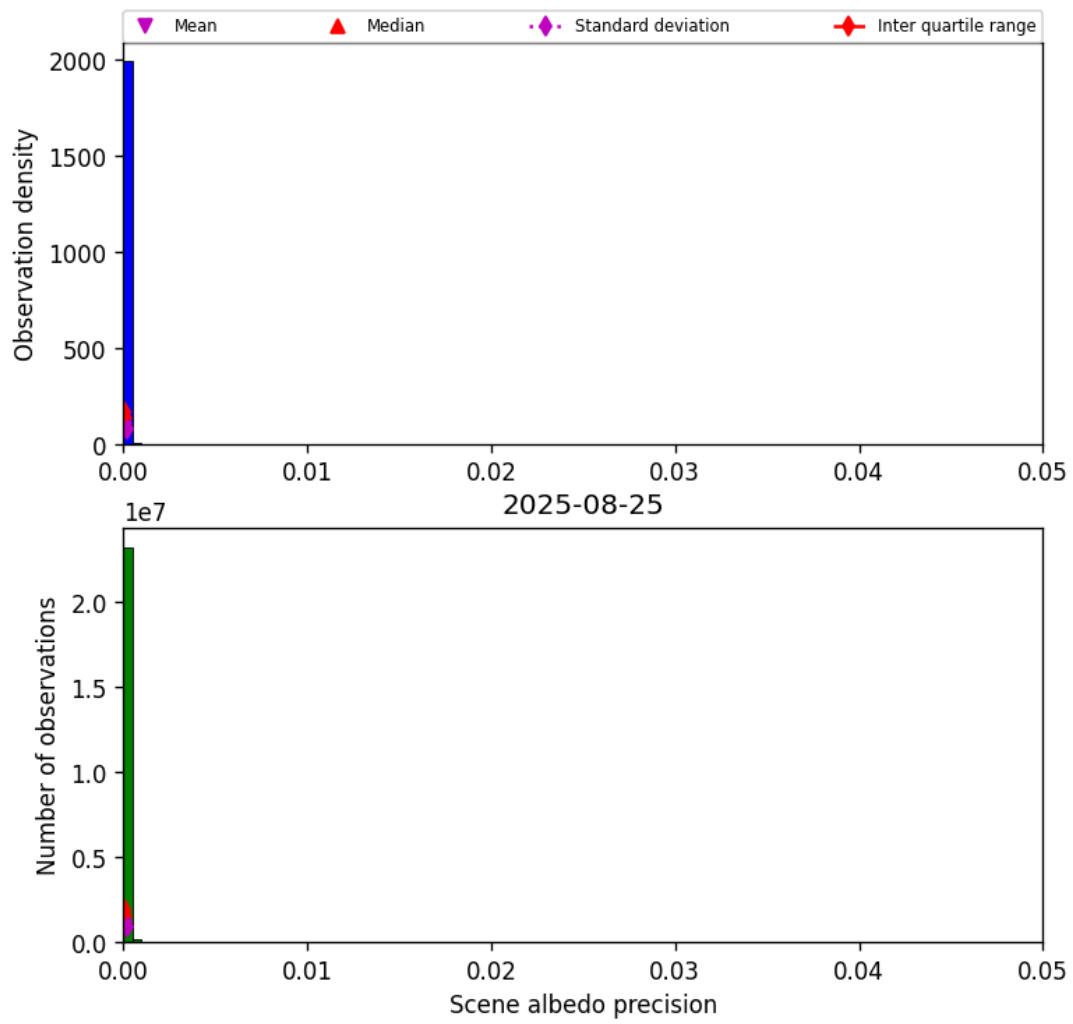
Figure 33: Histogram of “Scene albedo precision” for 2025-08-25 to 2025-08-26
