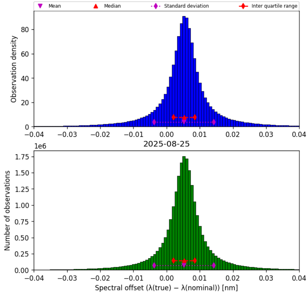
Figure 43: Histogram of “Spectral offset ( \lambda_{\text{true}} - \lambda_{\text{nominal}} )” for 2025-08-25 to 2025-08-26
