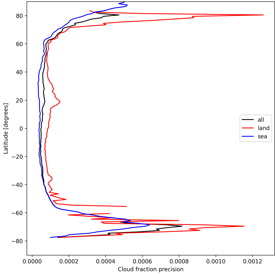
Figure 14: Zonal average of “Cloud fraction precision” for 2025-08-25 to 2025-08-26.
