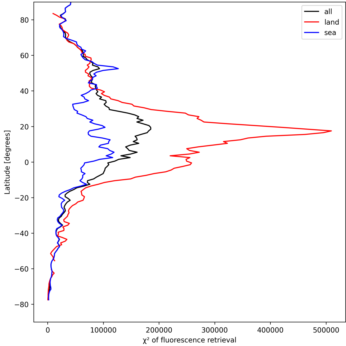
Figure 23: Zonal average of “ \chi^2 of fluorescence retrieval” for 2025-08-25 to 2025-08-26.
