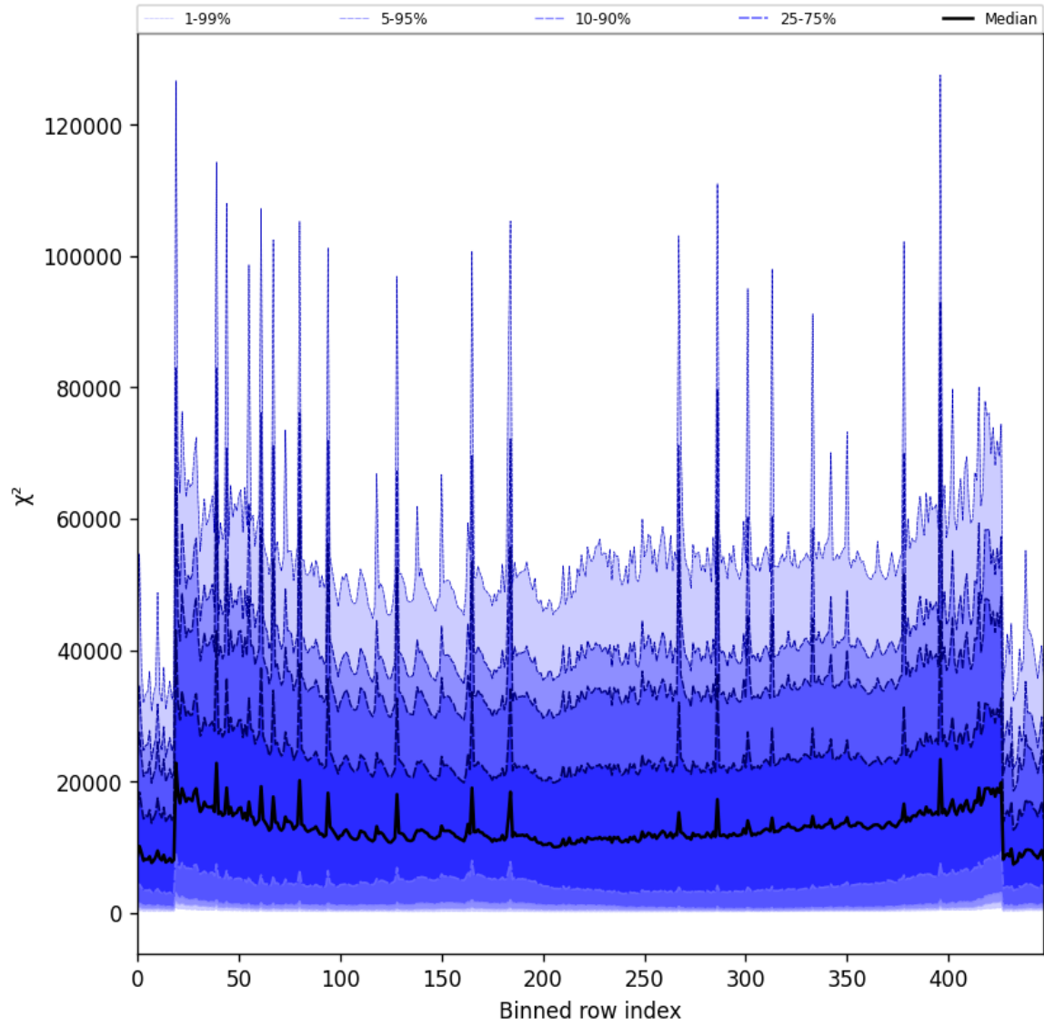
Figure 53: Along track statistics of “ \chi^2 ” for 2025-08-25 to 2025-08-26
