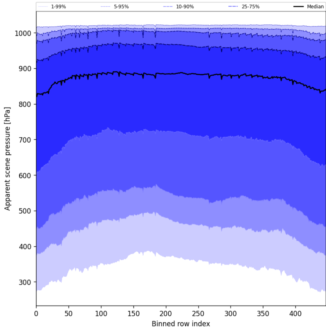
Figure 51: Along track statistics of “Apparent scene pressure” for 2025-08-25 to 2025-08-26
