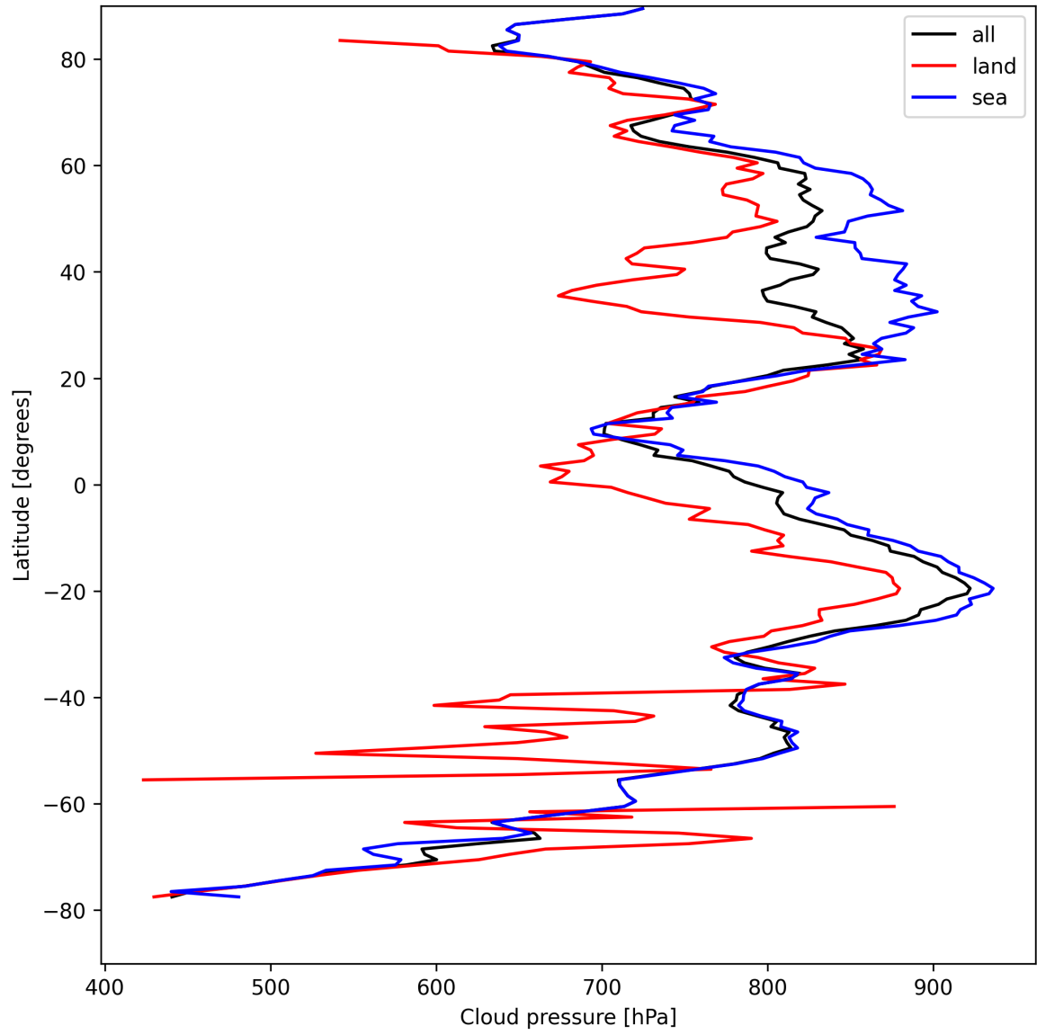
Figure 11: Zonal average of “Cloud pressure” for 2025-08-25 to 2025-08-26.
