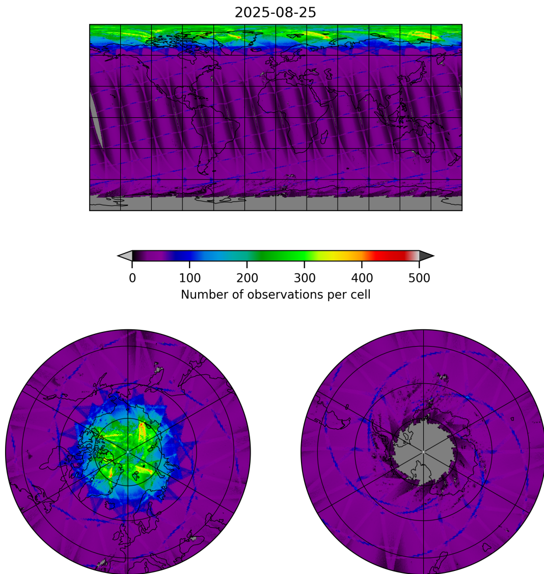
Figure 9: Map of the number of observations for 2025-08-25 to 2025-08-26
