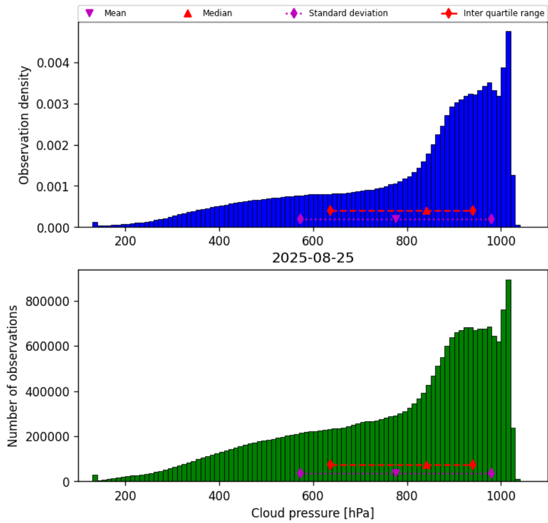
Figure 28: Histogram of “Cloud pressure” for 2025-08-25 to 2025-08-26
