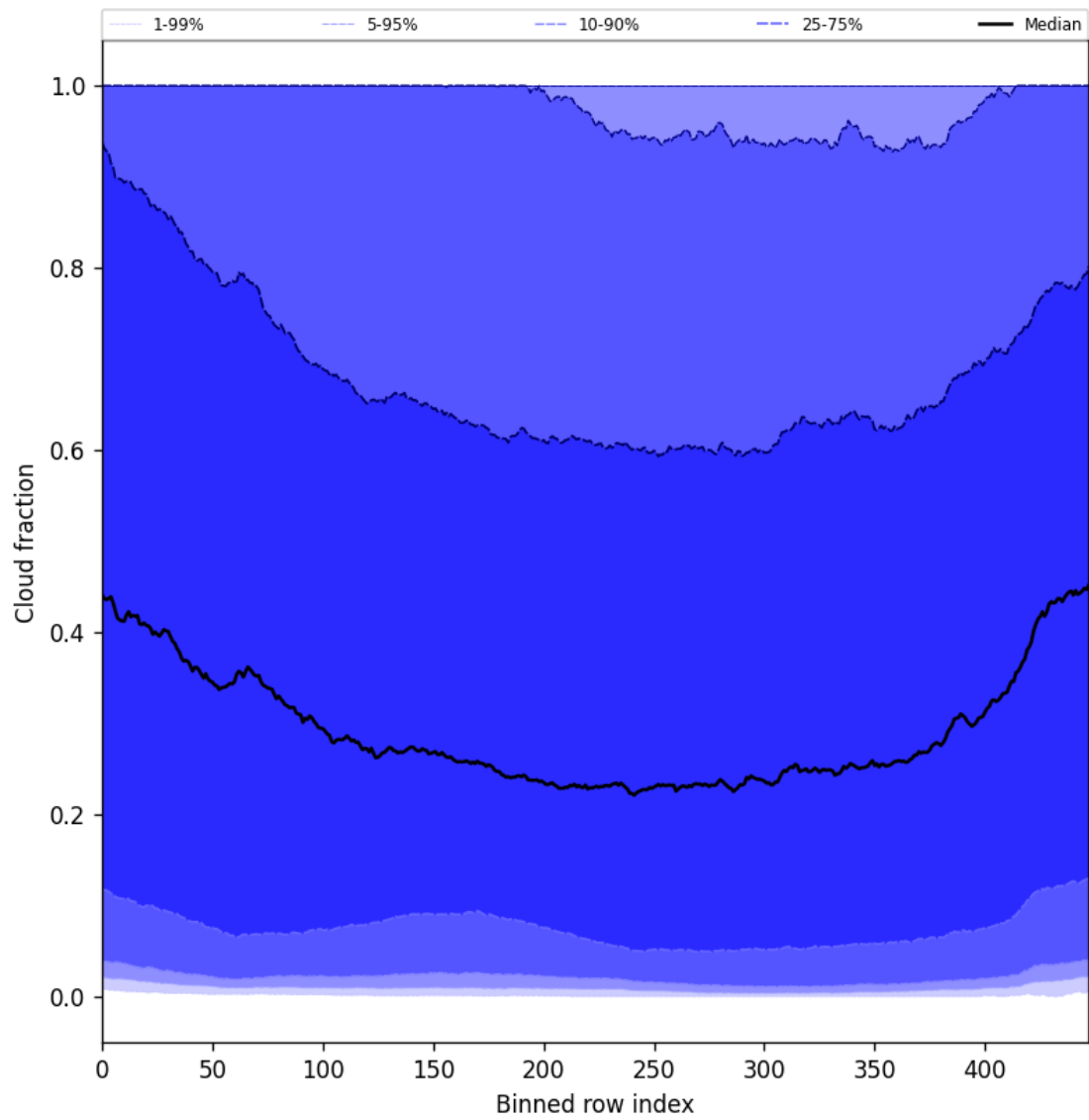
Figure 47: Along track statistics of “Cloud fraction” for 2025-08-25 to 2025-08-26
