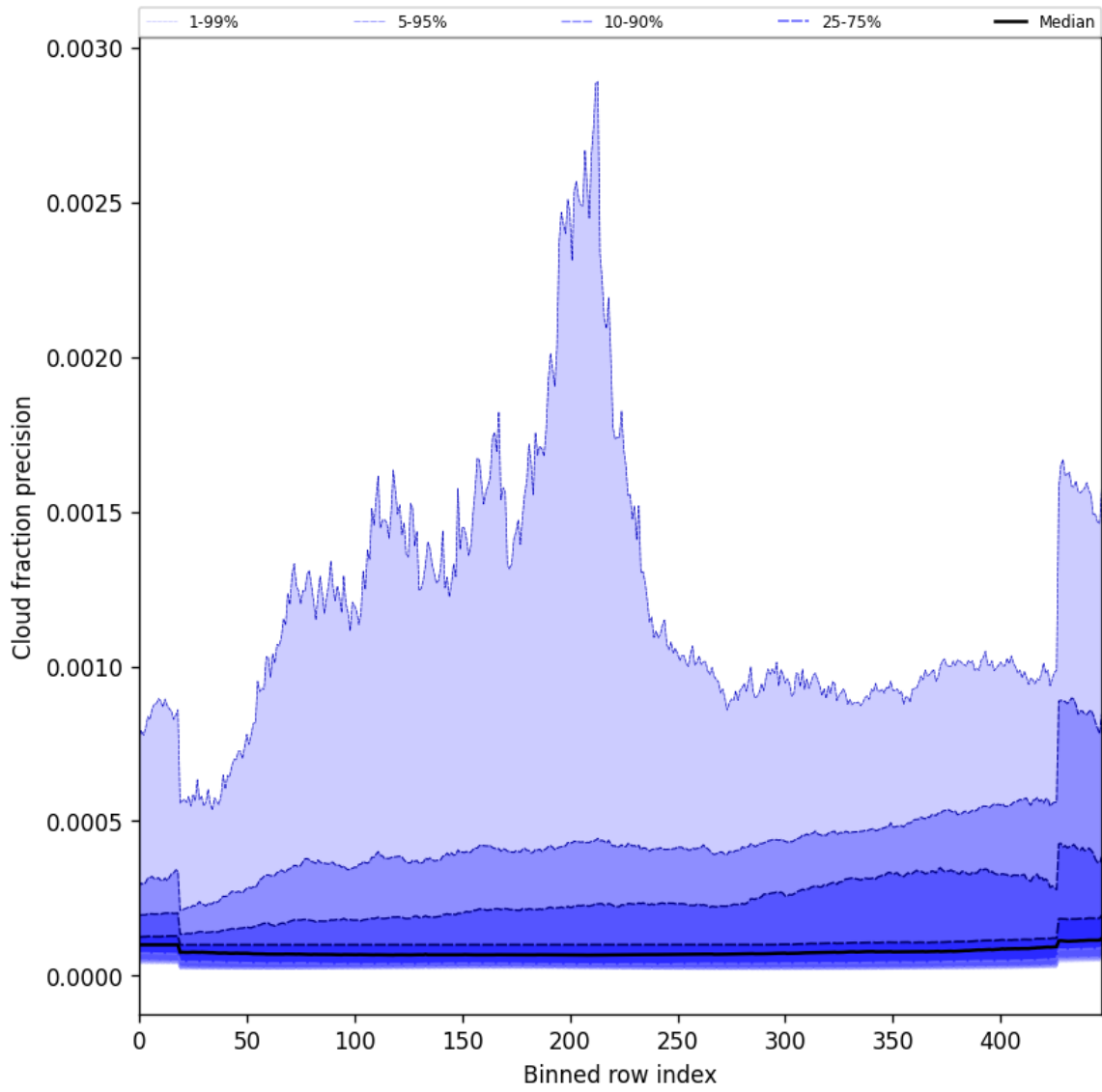
Figure 48: Along track statistics of “Cloud fraction precision” for 2025-08-25 to 2025-08-26
