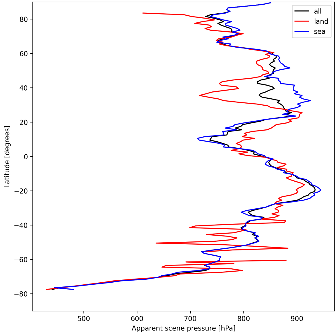
Figure 17: Zonal average of “Apparent scene pressure” for 2025-08-25 to 2025-08-26.
