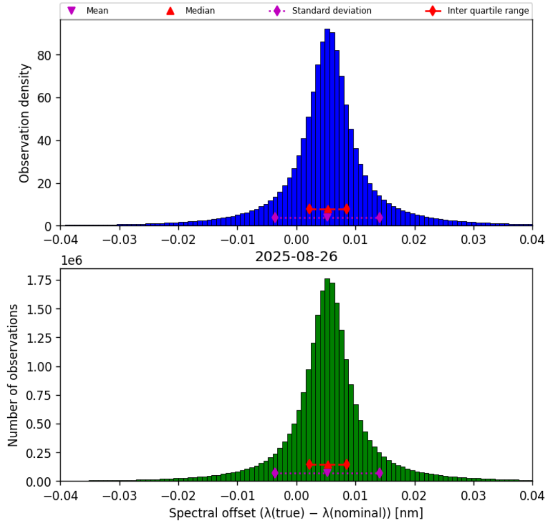
Figure 43: Histogram of “Spectral offset ( \lambda_{\text{true}} - \lambda_{\text{nominal}} )” for 2025-08-26 to 2025-08-27
