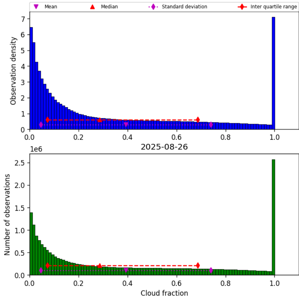
Figure 30: Histogram of “Cloud fraction” for 2025-08-26 to 2025-08-27
