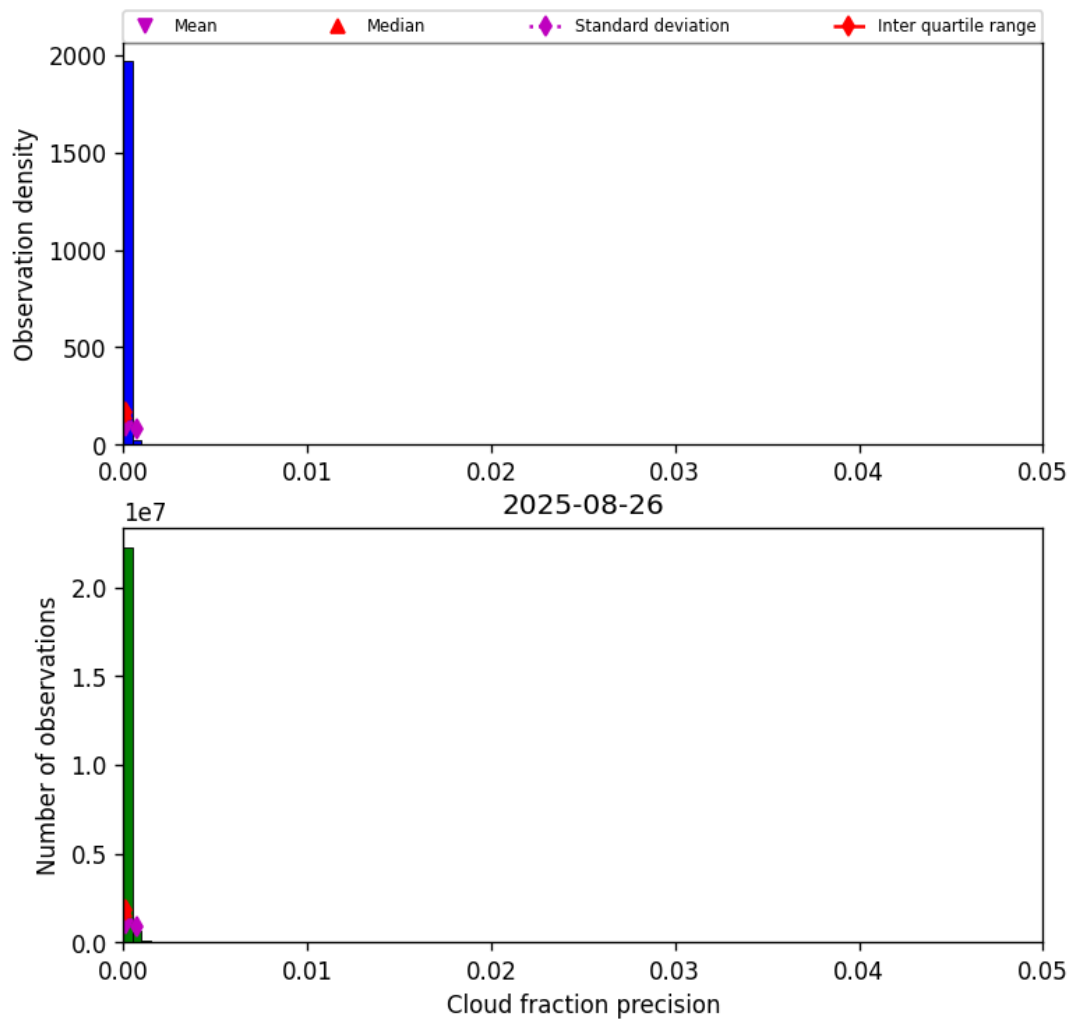
Figure 31: Histogram of “Cloud fraction precision” for 2025-08-26 to 2025-08-27
