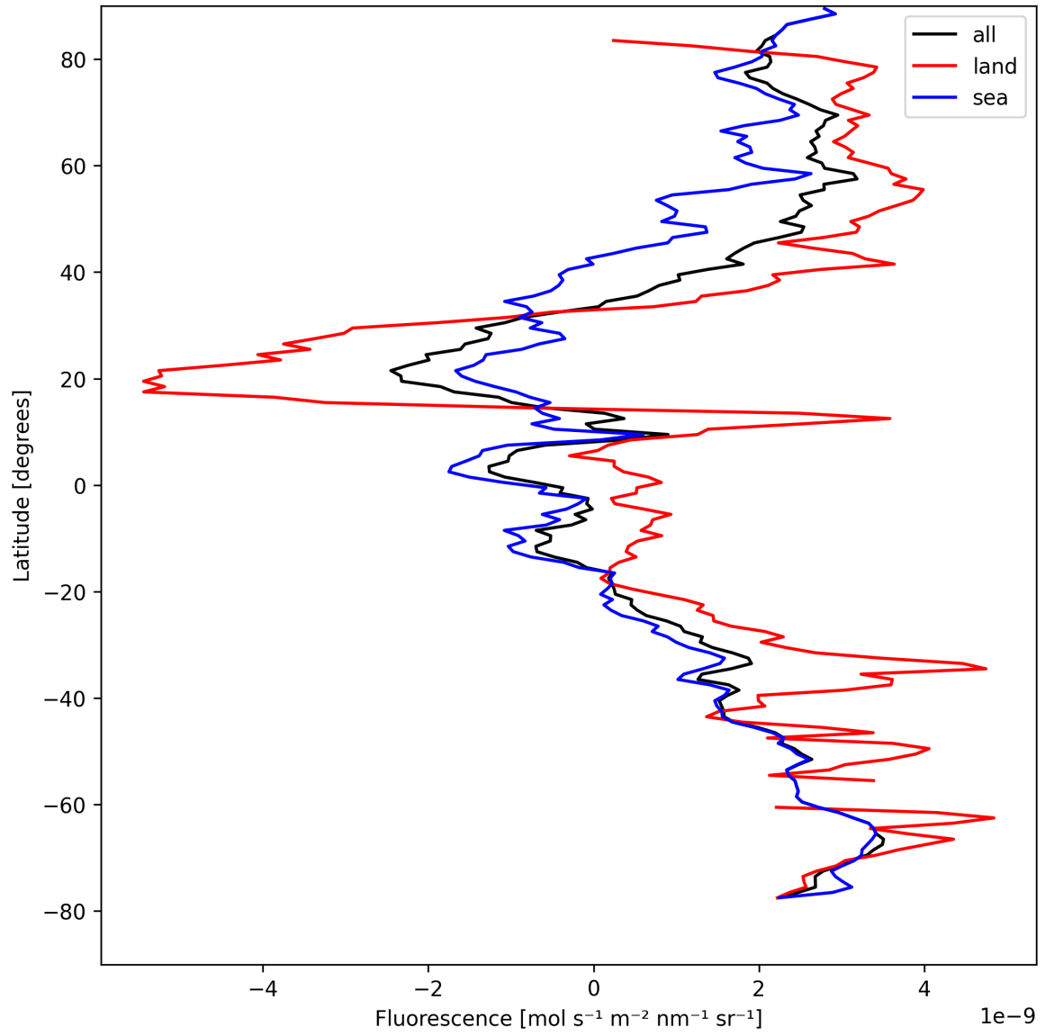
Figure 21: Zonal average of “Fluorescence” for 2025-08-26 to 2025-08-27.
