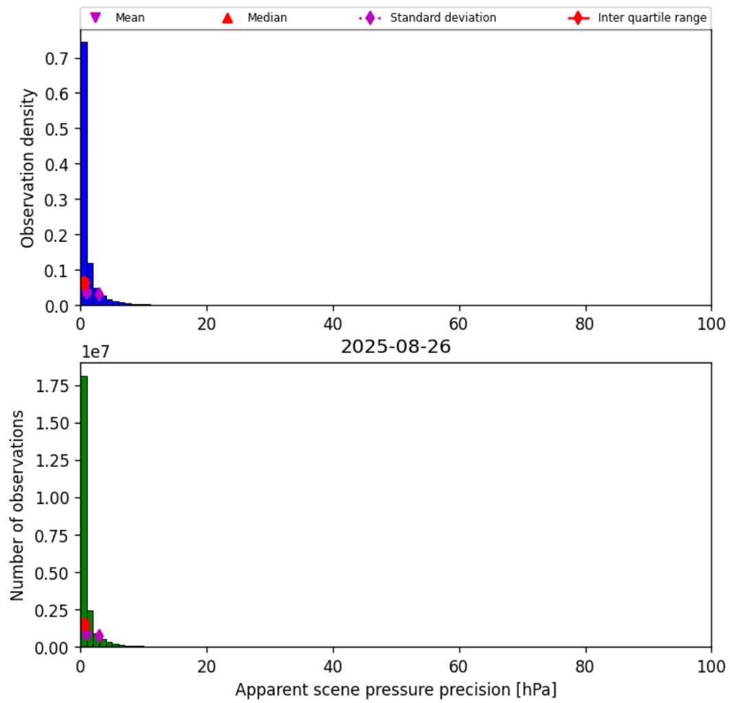
Figure 35: Histogram of “Apparent scene pressure precision” for 2025-08-26 to 2025-08-27
