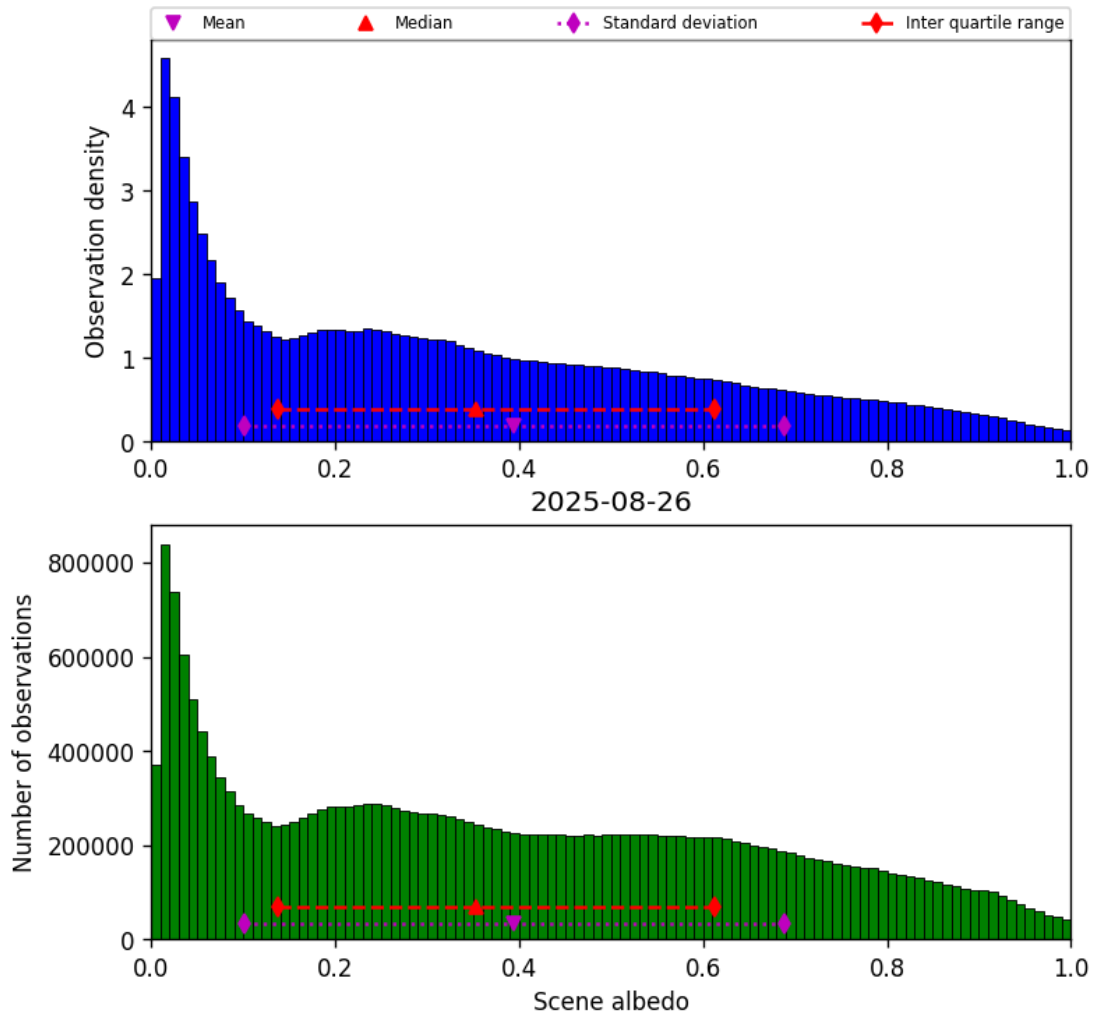
Figure 32: Histogram of “Scene albedo” for 2025-08-26 to 2025-08-27
