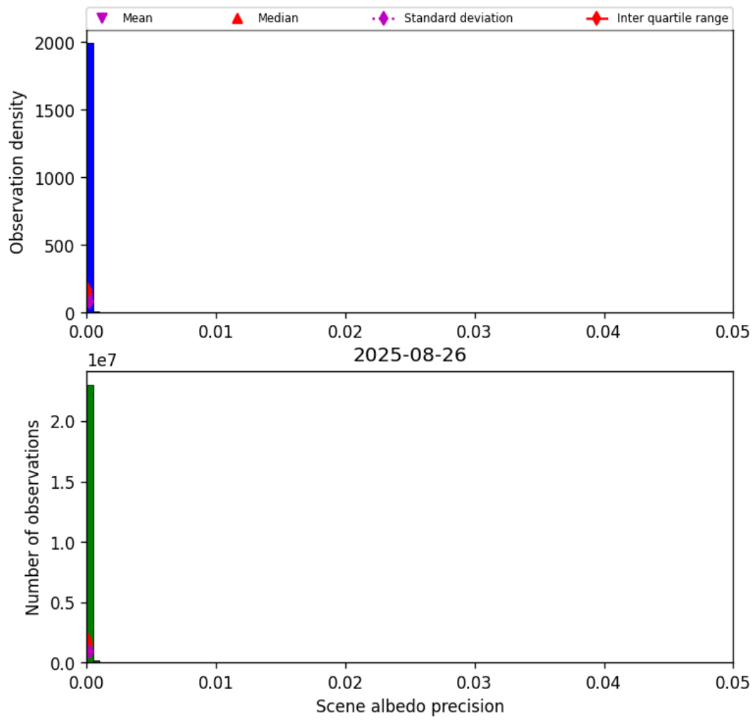
Figure 33: Histogram of “Scene albedo precision” for 2025-08-26 to 2025-08-27
