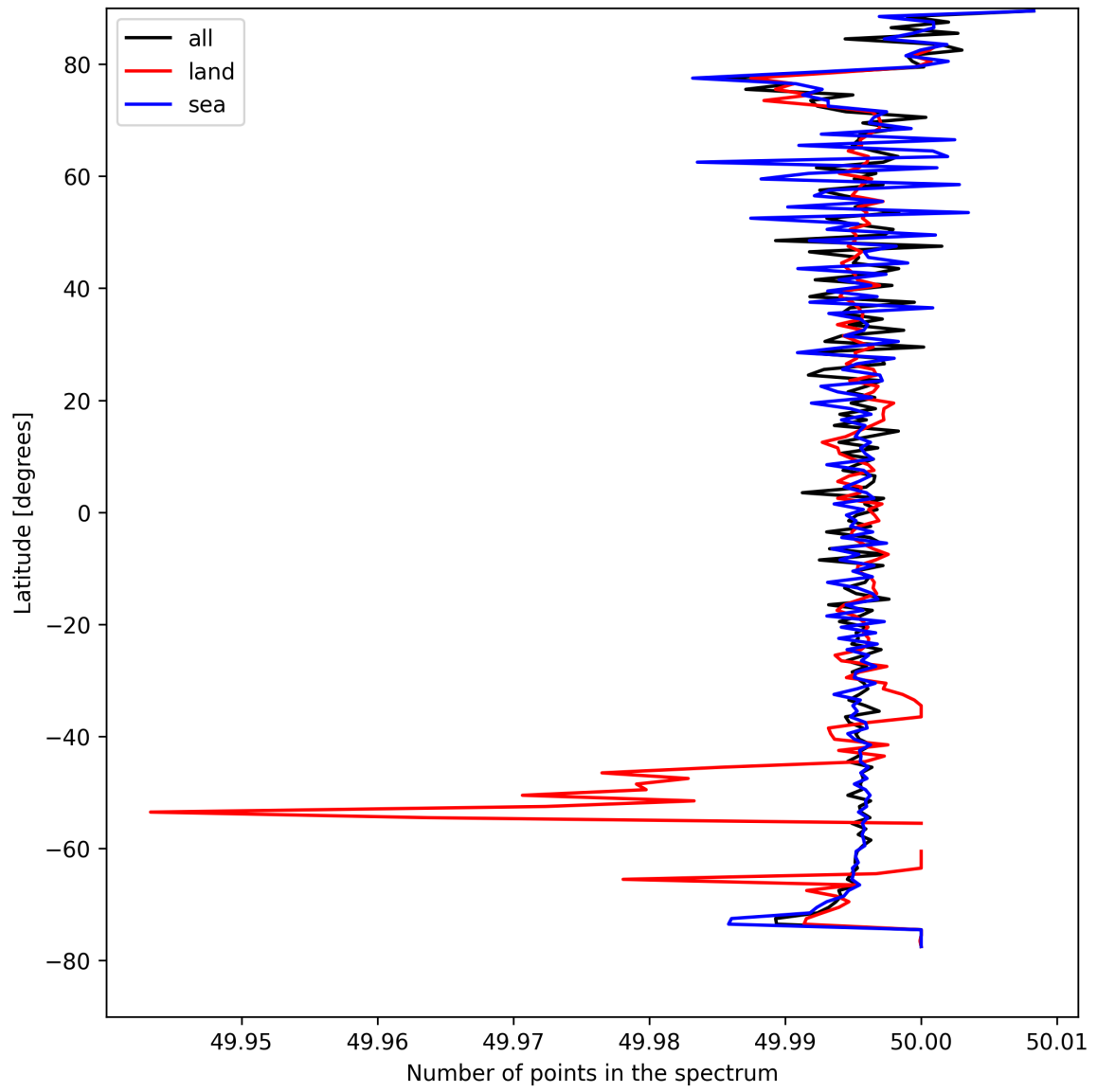
Figure 25: Zonal average of “Number of points in the spectrum” for 2025-08-26 to 2025-08-27.
