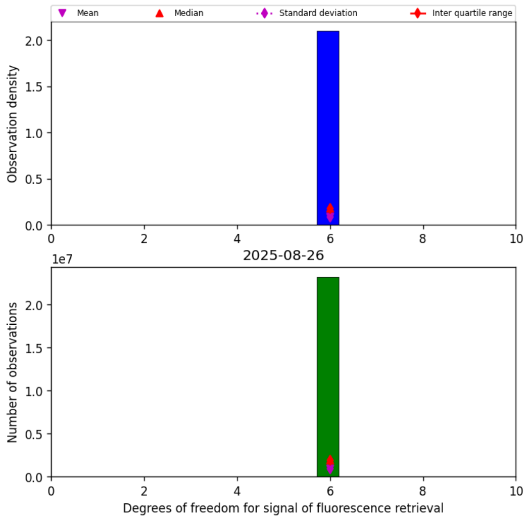
Figure 41: Histogram of “Degrees of freedom for signal of fluorescence retrieval” for 2025-08-26 to 2025-08-27
