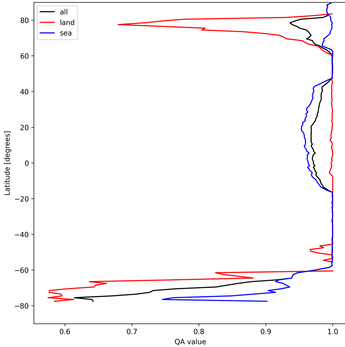
Figure 10: Zonal average of “QA value” for 2025-08-26 to 2025-08-27.
