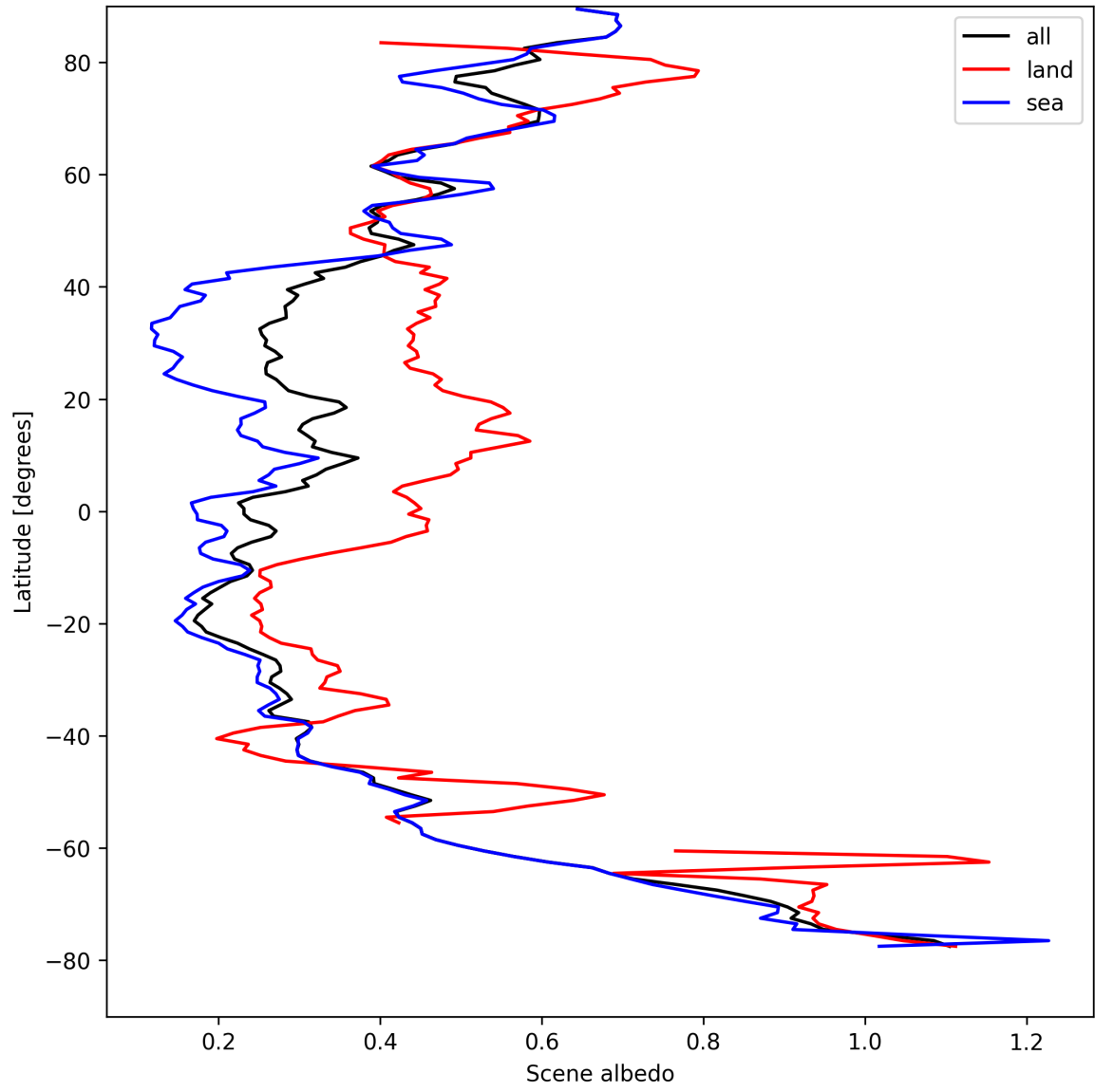
Figure 15: Zonal average of “Scene albedo” for 2025-08-26 to 2025-08-27.
