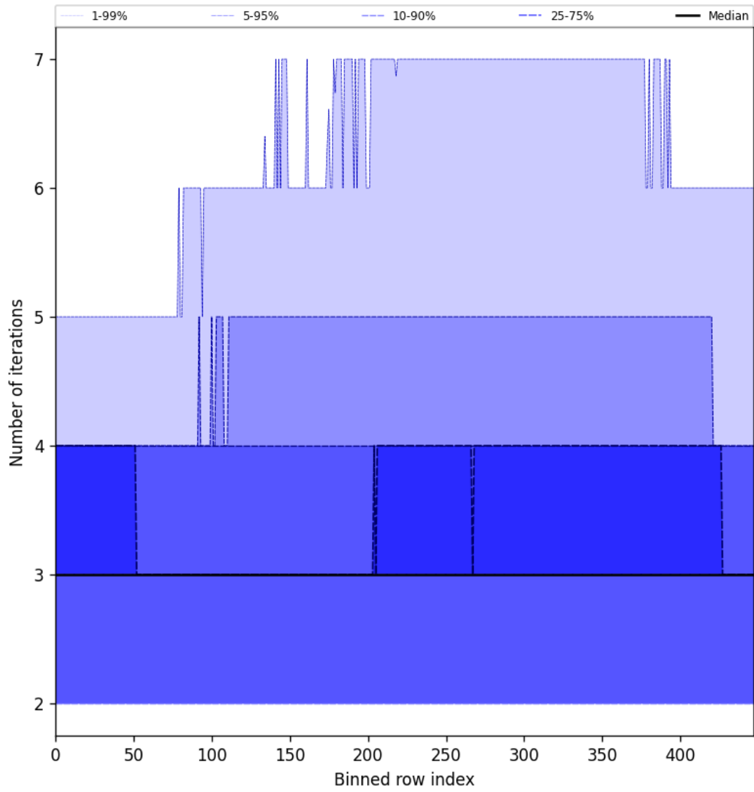
Figure 54: Along track statistics of “Number of iterations” for 2025-08-26 to 2025-08-27
