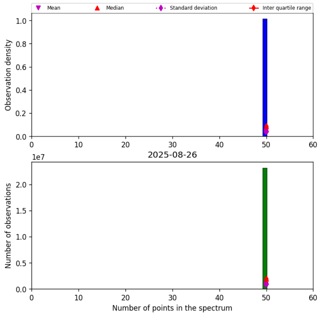
Figure 42: Histogram of “Number of points in the spectrum” for 2025-08-26 to 2025-08-27
