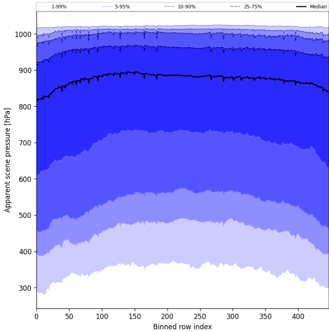
Figure 51: Along track statistics of “Apparent scene pressure” for 2025-08-26 to 2025-08-27
