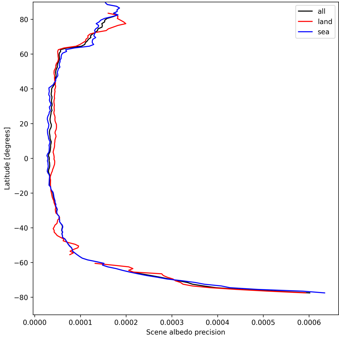
Figure 16: Zonal average of “Scene albedo precision” for 2025-08-26 to 2025-08-27.
