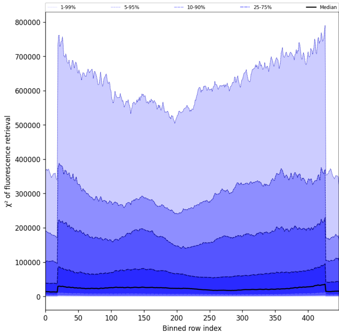
Figure 57: Along track statistics of “ \chi^2 of fluorescence retrieval” for 2025-08-26 to 2025-08-27
