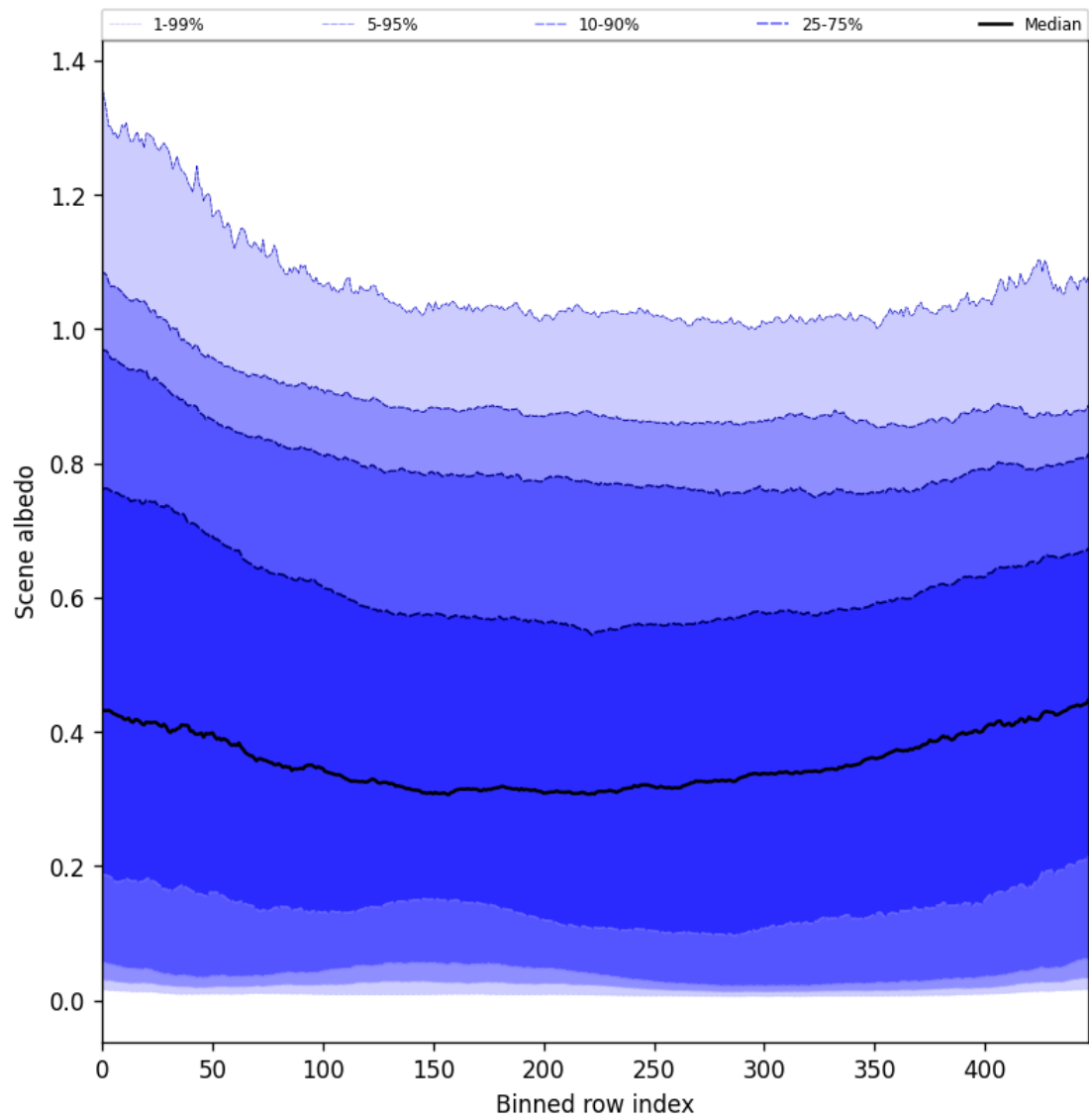
Figure 49: Along track statistics of “Scene albedo” for 2025-08-26 to 2025-08-27
