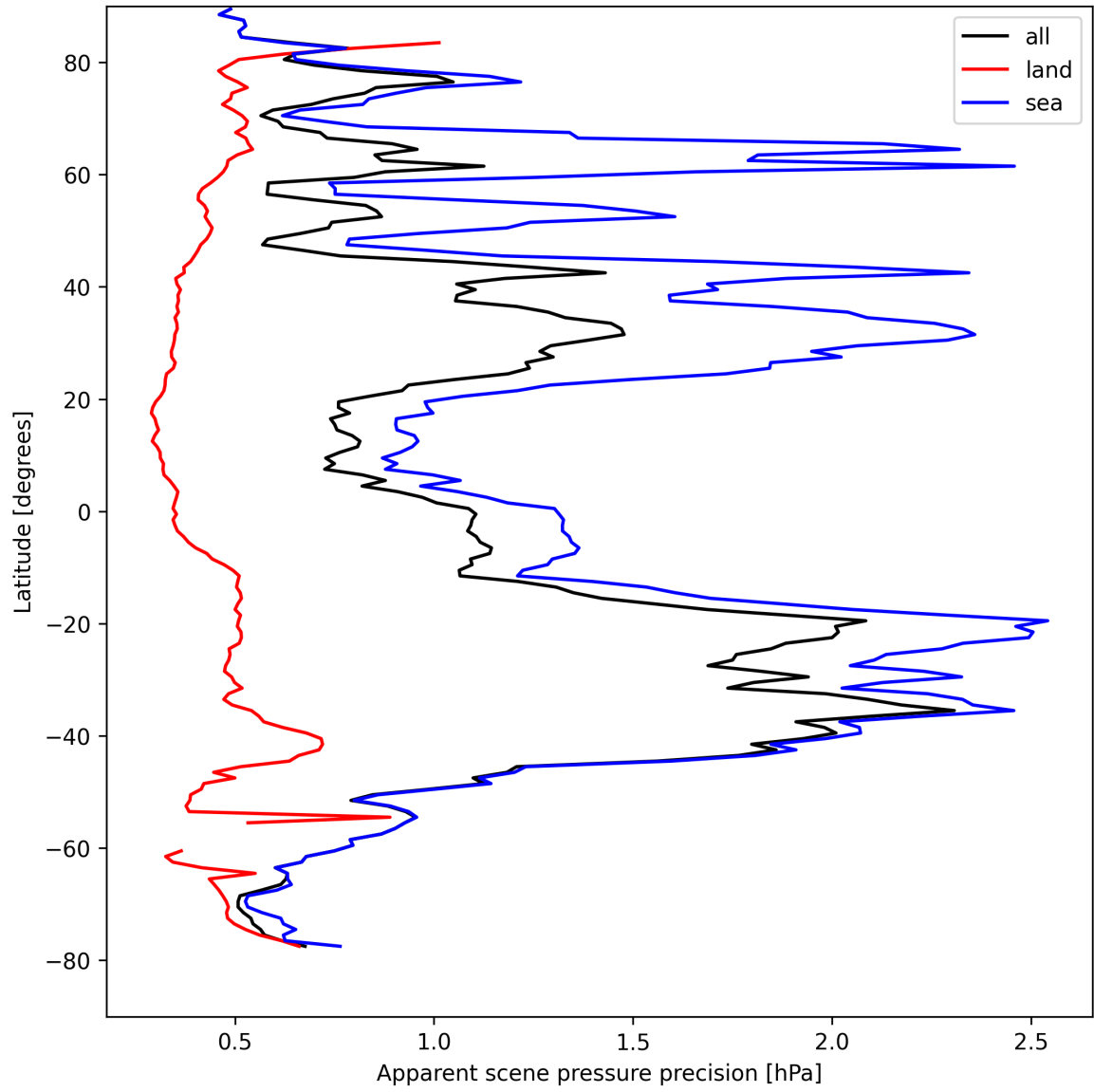
Figure 18: Zonal average of “Apparent scene pressure precision” for 2025-08-26 to 2025-08-27.
