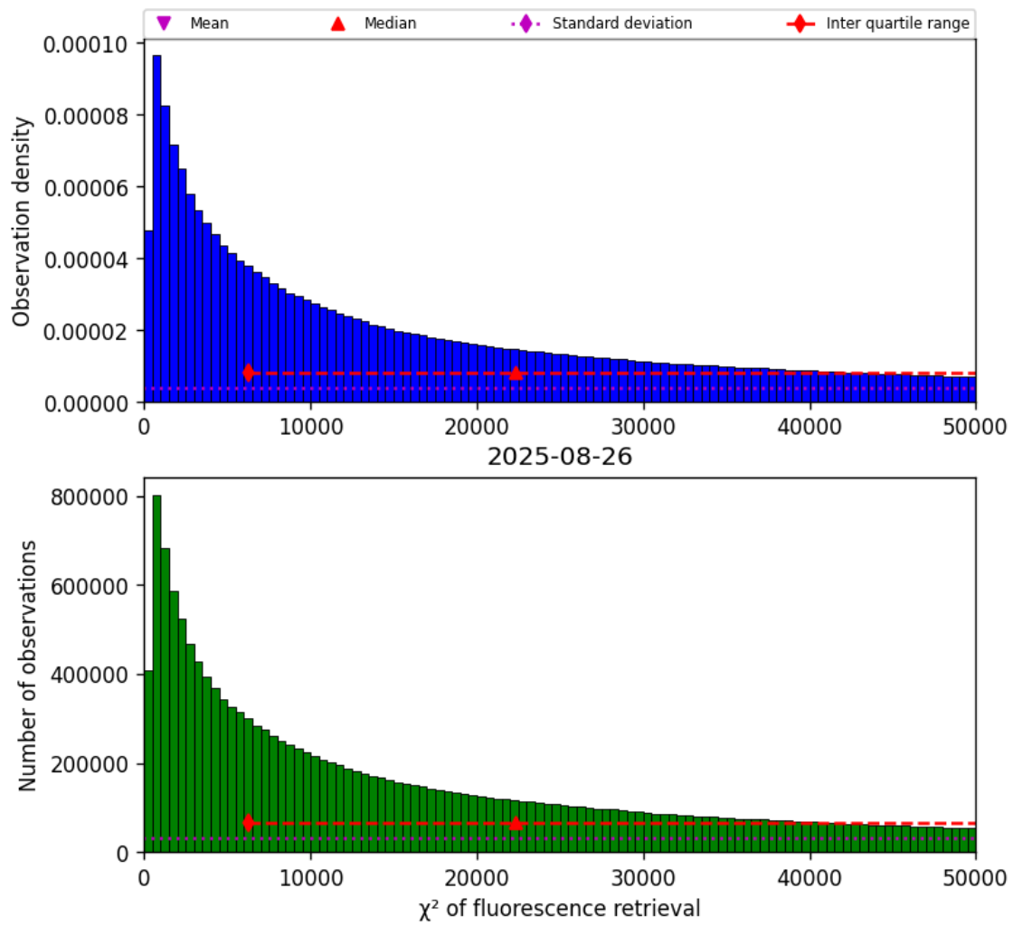
Figure 40: Histogram of “ \chi^2 of fluorescence retrieval” for 2025-08-26 to 2025-08-27
