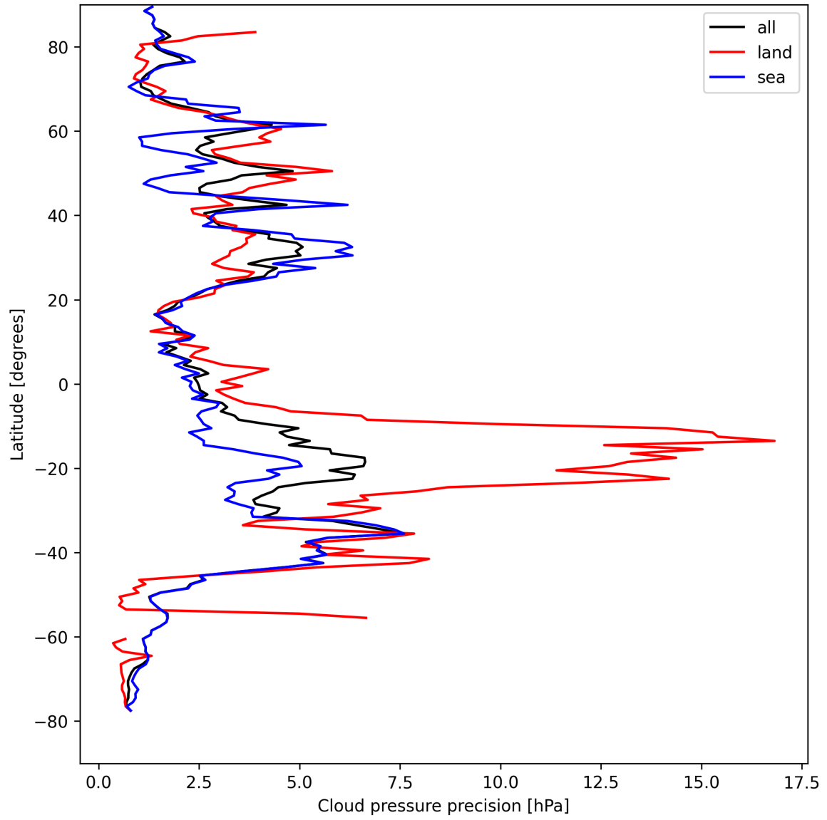
Figure 12: Zonal average of “Cloud pressure precision” for 2025-08-26 to 2025-08-27.
