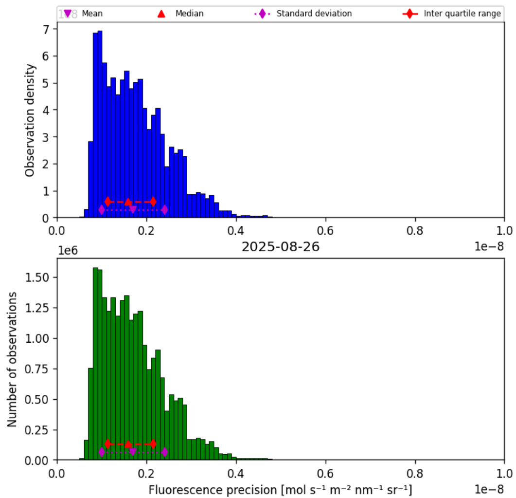
Figure 39: Histogram of “Fluorescence precision” for 2025-08-26 to 2025-08-27
