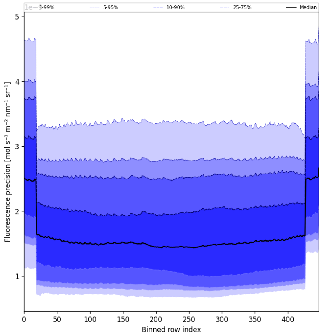
Figure 56: Along track statistics of “Fluorescence precision” for 2025-08-26 to 2025-08-27
