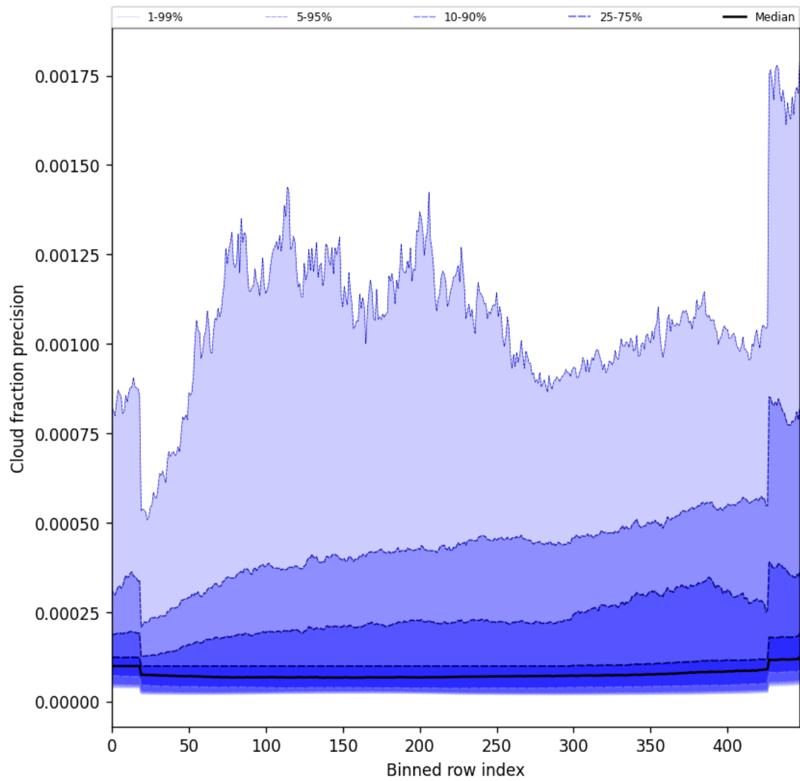
Figure 48: Along track statistics of “Cloud fraction precision” for 2025-08-26 to 2025-08-27
