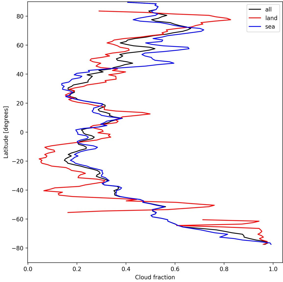
Figure 13: Zonal average of “Cloud fraction” for 2025-08-26 to 2025-08-27.
