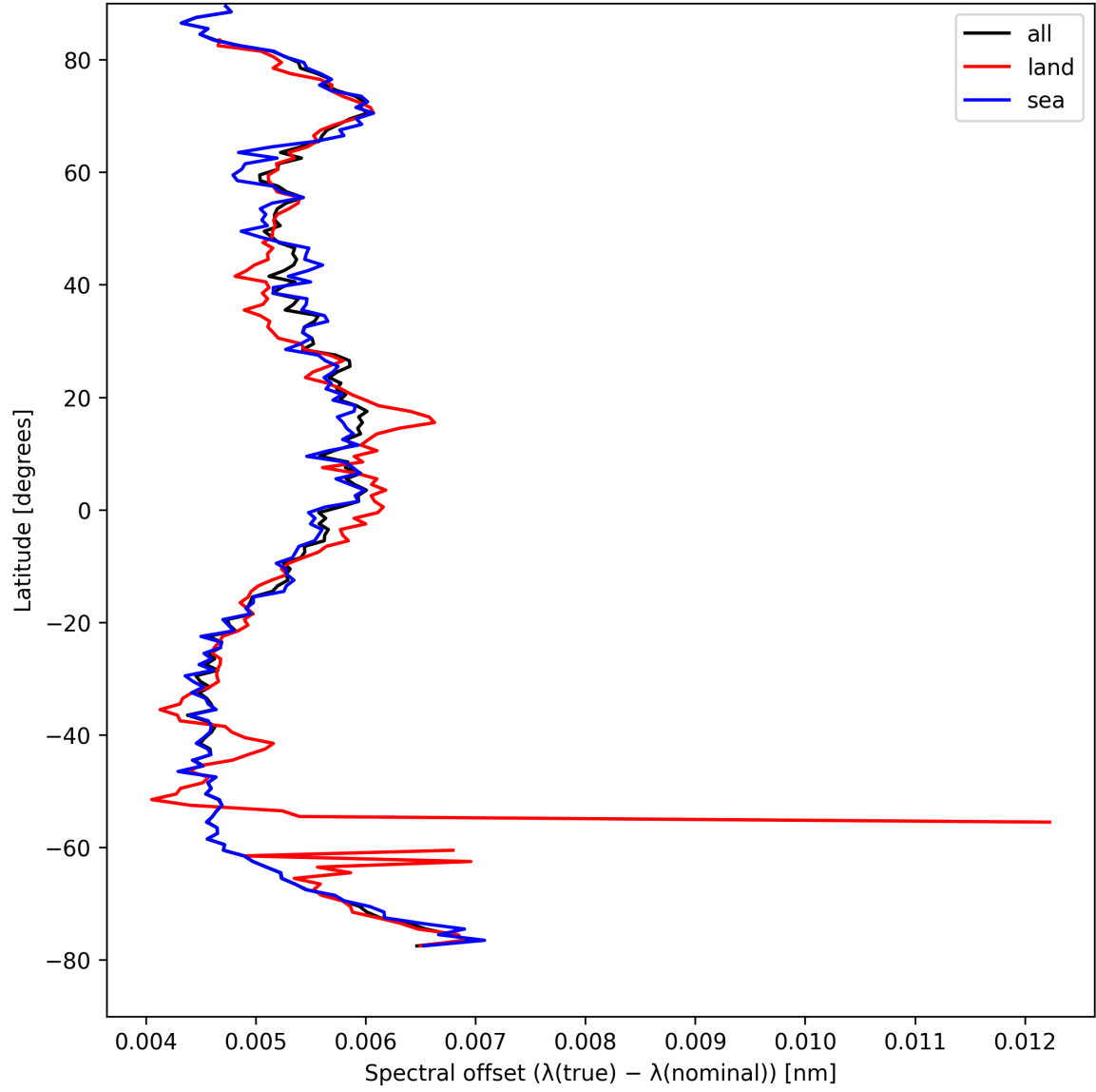
Figure 26: Zonal average of “Spectral offset ( \lambda_{\text{true}} - \lambda_{\text{nominal}} )” for 2025-08-26 to 2025-08-27.
