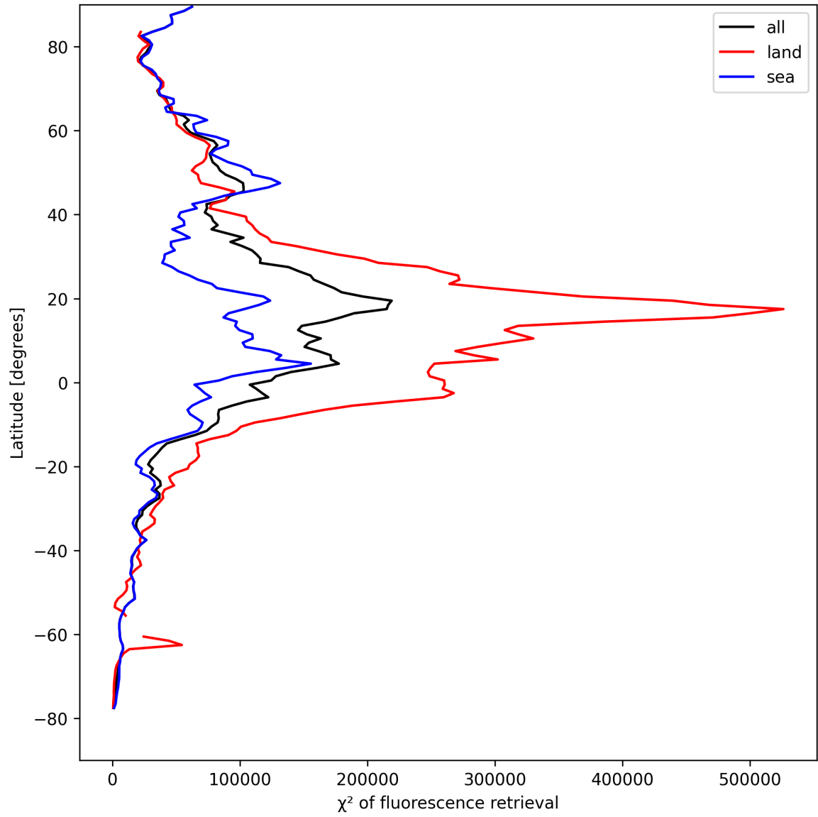
Figure 23: Zonal average of “ \chi^2 of fluorescence retrieval” for 2025-08-26 to 2025-08-27.
