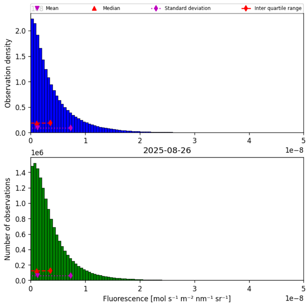
Figure 38: Histogram of “Fluorescence” for 2025-08-26 to 2025-08-27
