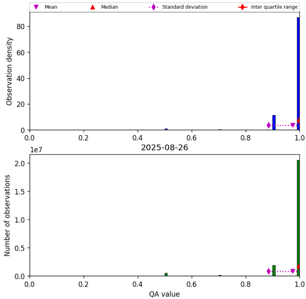
Figure 27: Histogram of “QA value” for 2025-08-26 to 2025-08-27
