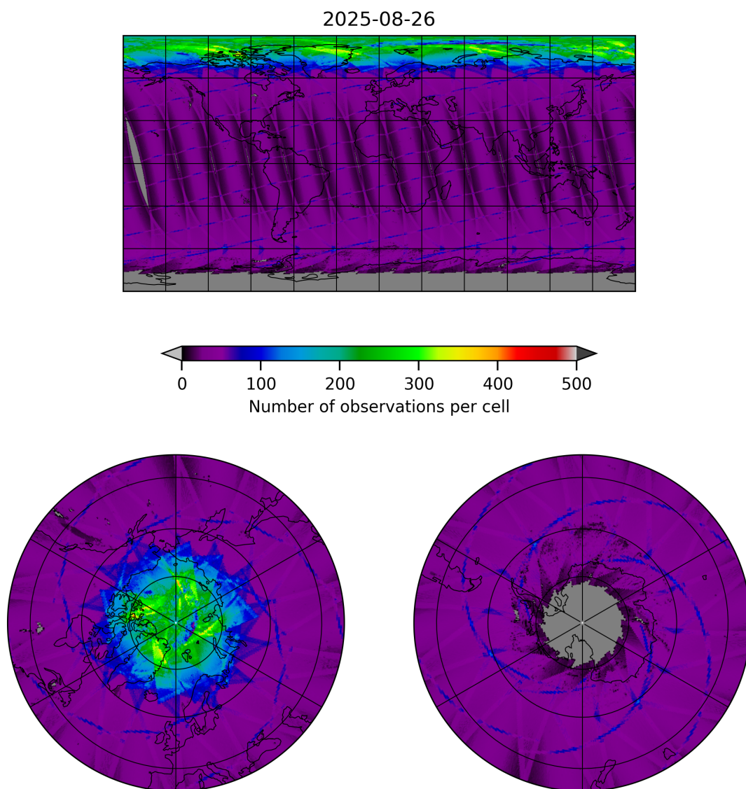
Figure 9: Map of the number of observations for 2025-08-26 to 2025-08-27
