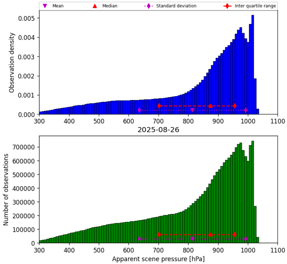
Figure 34: Histogram of “Apparent scene pressure” for 2025-08-26 to 2025-08-27
