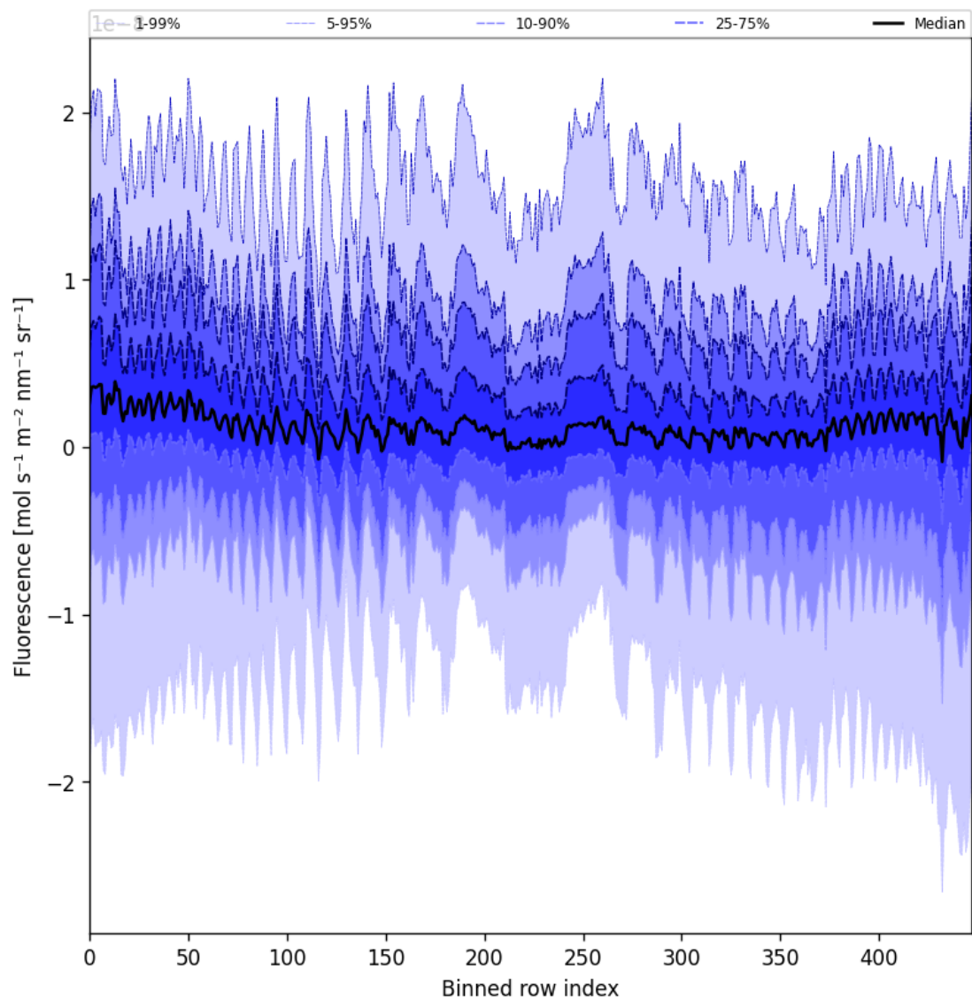
Figure 55: Along track statistics of “Fluorescence” for 2025-08-26 to 2025-08-27
