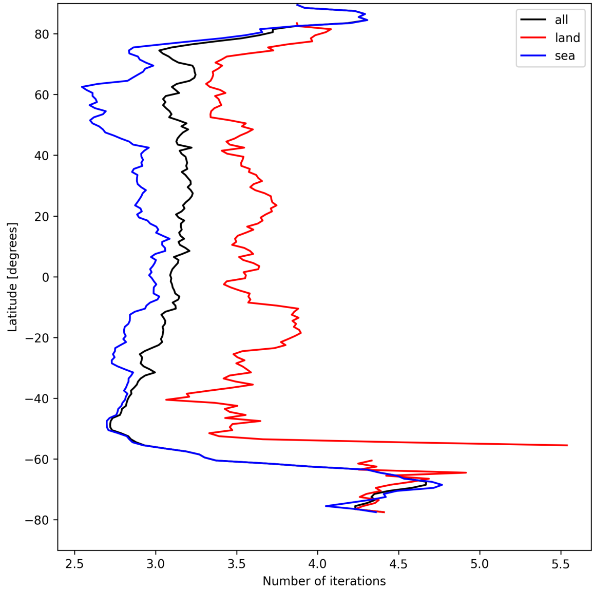
Figure 20: Zonal average of “Number of iterations” for 2025-08-26 to 2025-08-27.
