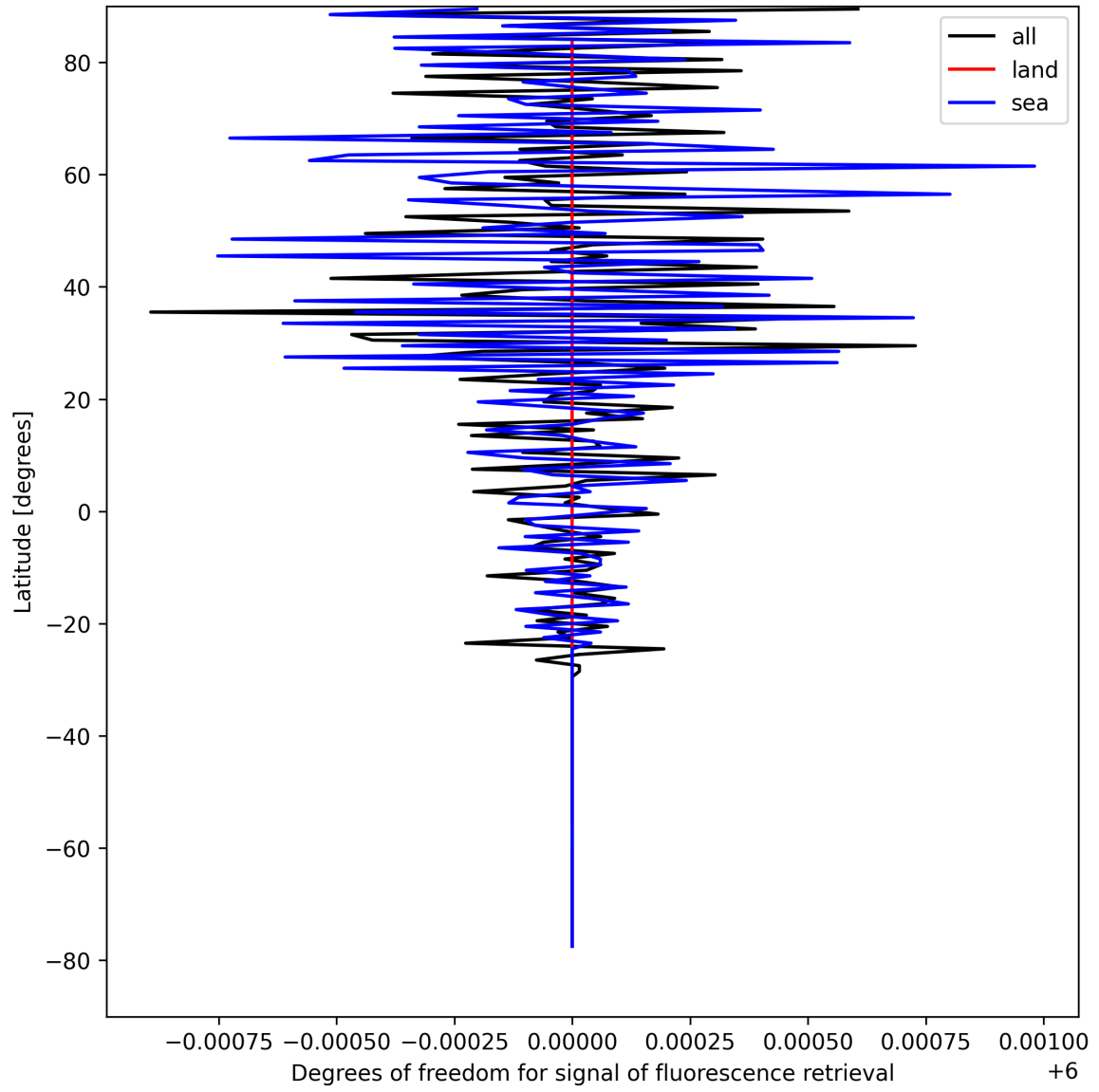
Figure 24: Zonal average of “Degrees of freedom for signal of fluorescence retrieval” for 2025-08-26 to 2025-08-27.
