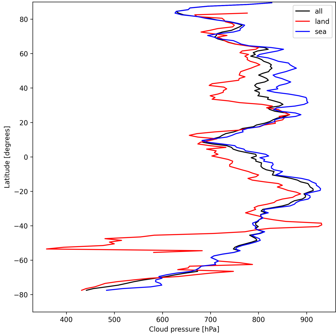
Figure 11: Zonal average of “Cloud pressure” for 2025-08-26 to 2025-08-27.
