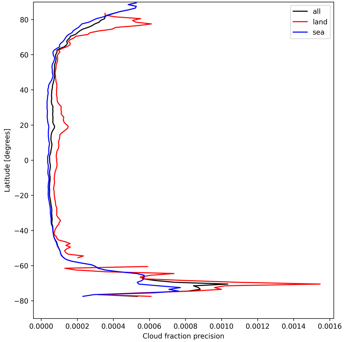
Figure 14: Zonal average of “Cloud fraction precision” for 2025-08-26 to 2025-08-27.
