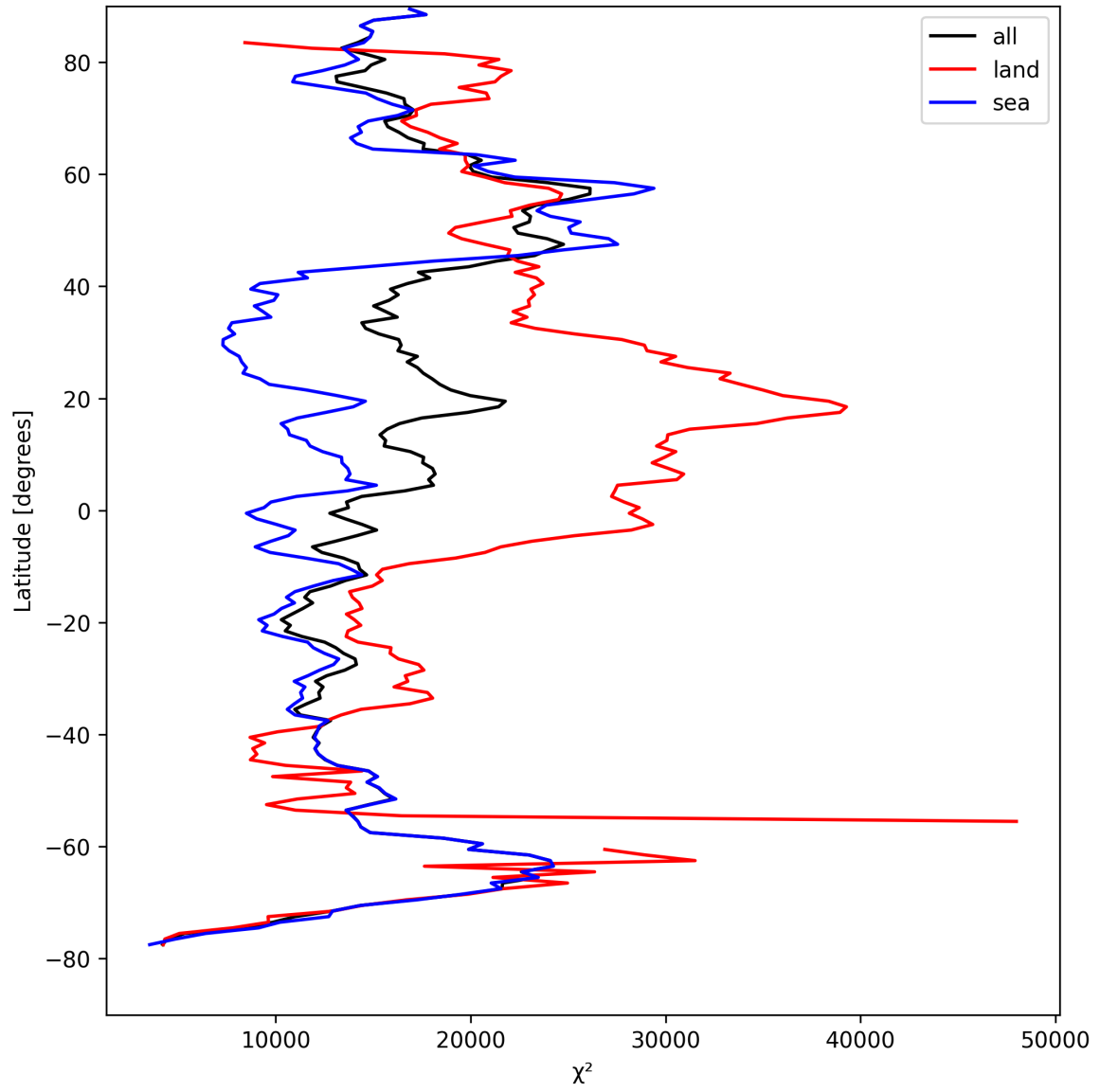
Figure 19: Zonal average of “ \chi^2 ” for 2025-08-26 to 2025-08-27.
