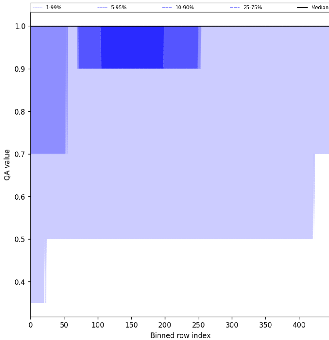
Figure 44: Along track statistics of “QA value” for 2025-08-26 to 2025-08-27
