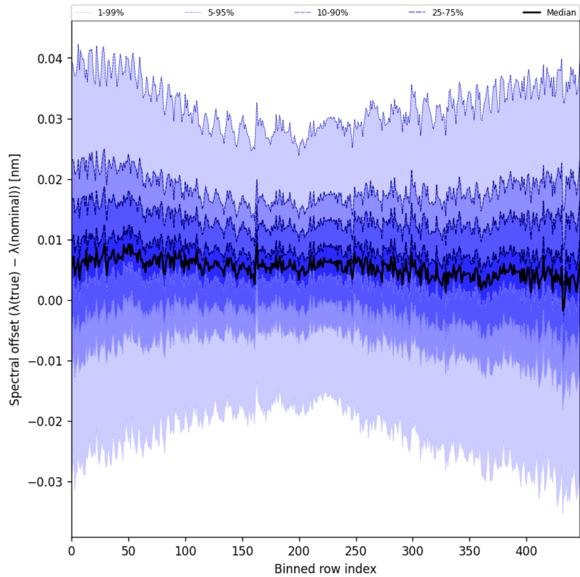
Figure 60: Along track statistics of “Spectral offset ( \lambda_{\text{true}} - \lambda_{\text{nominal}} )” for 2025-08-26 to 2025-08-27
