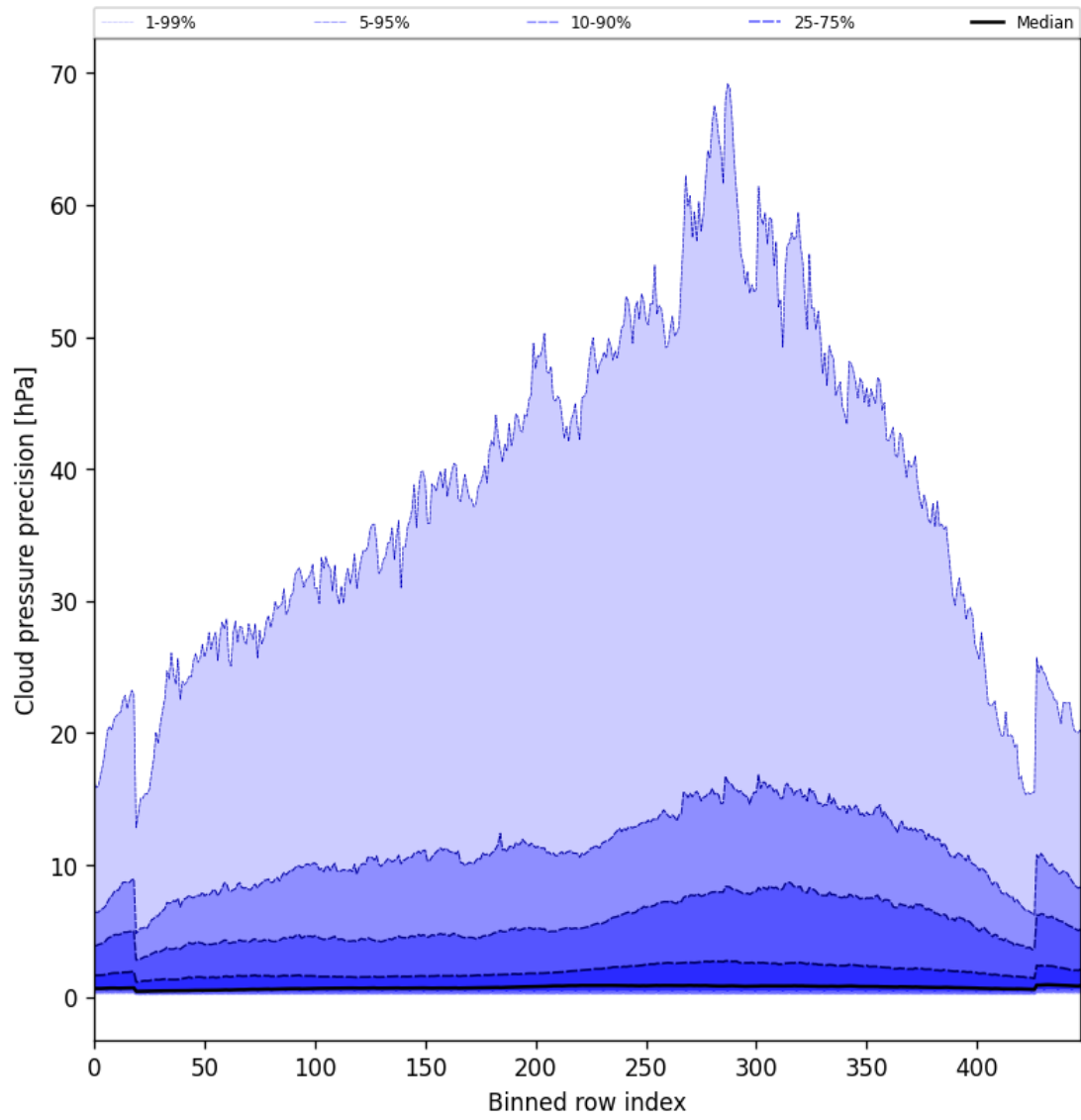
Figure 46: Along track statistics of “Cloud pressure precision” for 2025-08-26 to 2025-08-27
