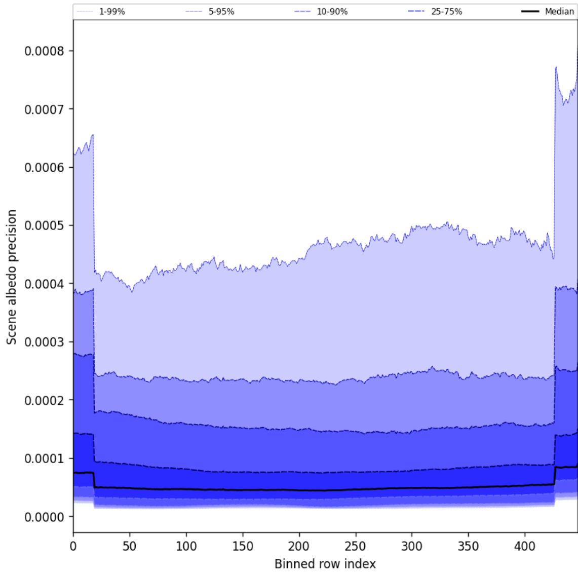
Figure 50: Along track statistics of “Scene albedo precision” for 2025-08-26 to 2025-08-27
