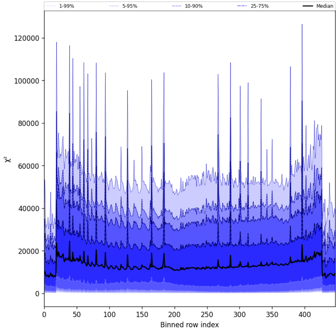
Figure 53: Along track statistics of “ \chi^2 ” for 2025-08-26 to 2025-08-27
