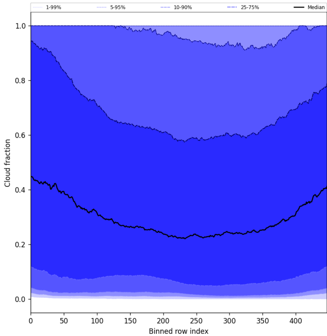
Figure 47: Along track statistics of “Cloud fraction” for 2025-08-26 to 2025-08-27
