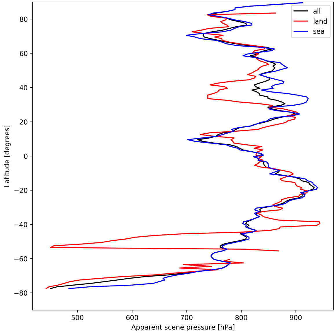
Figure 17: Zonal average of “Apparent scene pressure” for 2025-08-26 to 2025-08-27.
