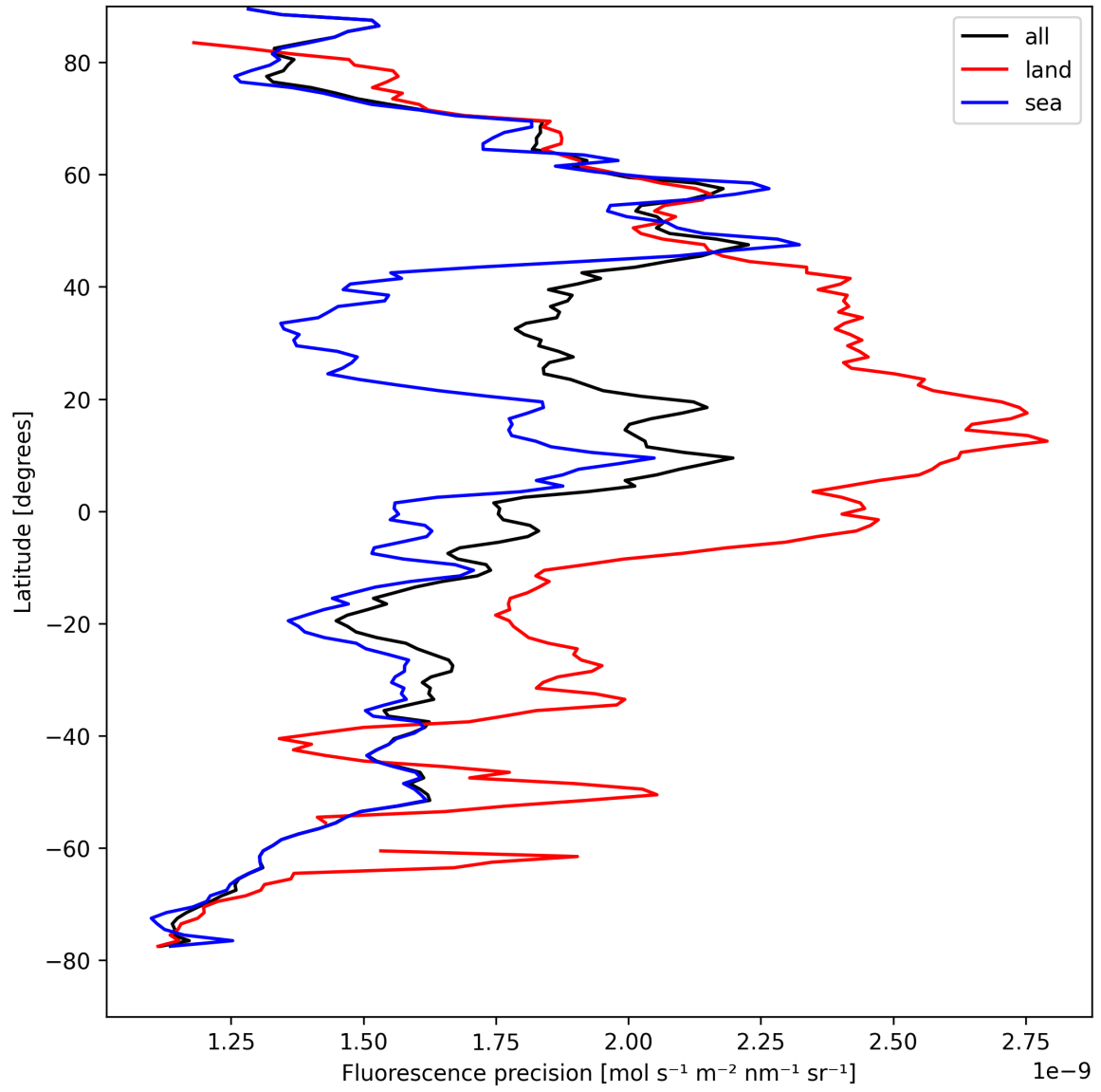
Figure 22: Zonal average of “Fluorescence precision” for 2025-08-26 to 2025-08-27.
