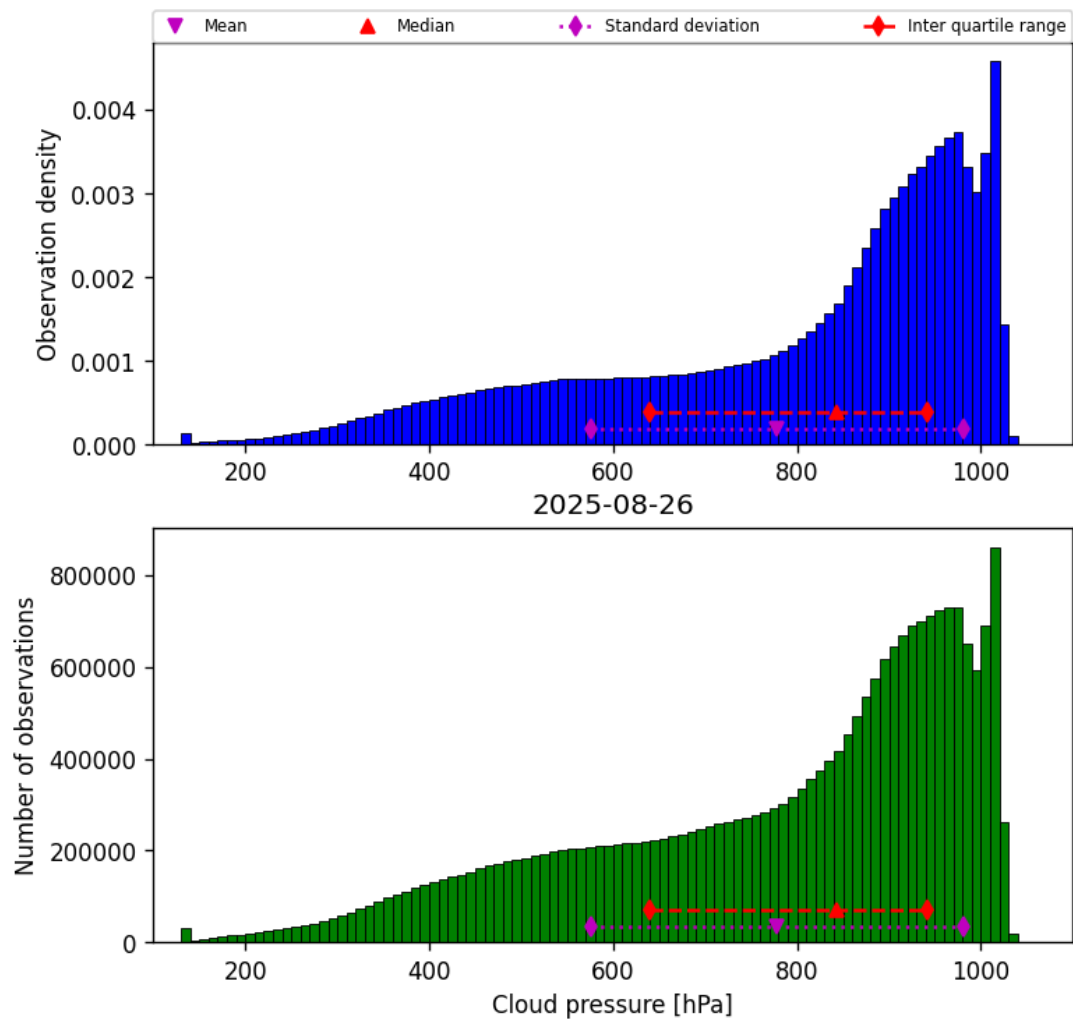
Figure 28: Histogram of “Cloud pressure” for 2025-08-26 to 2025-08-27
