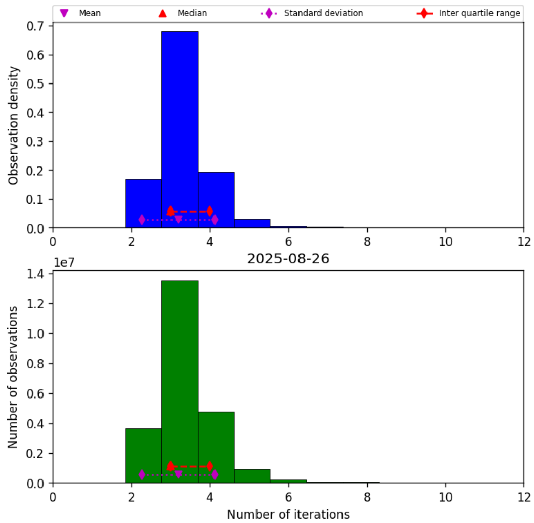
Figure 37: Histogram of “Number of iterations” for 2025-08-26 to 2025-08-27
