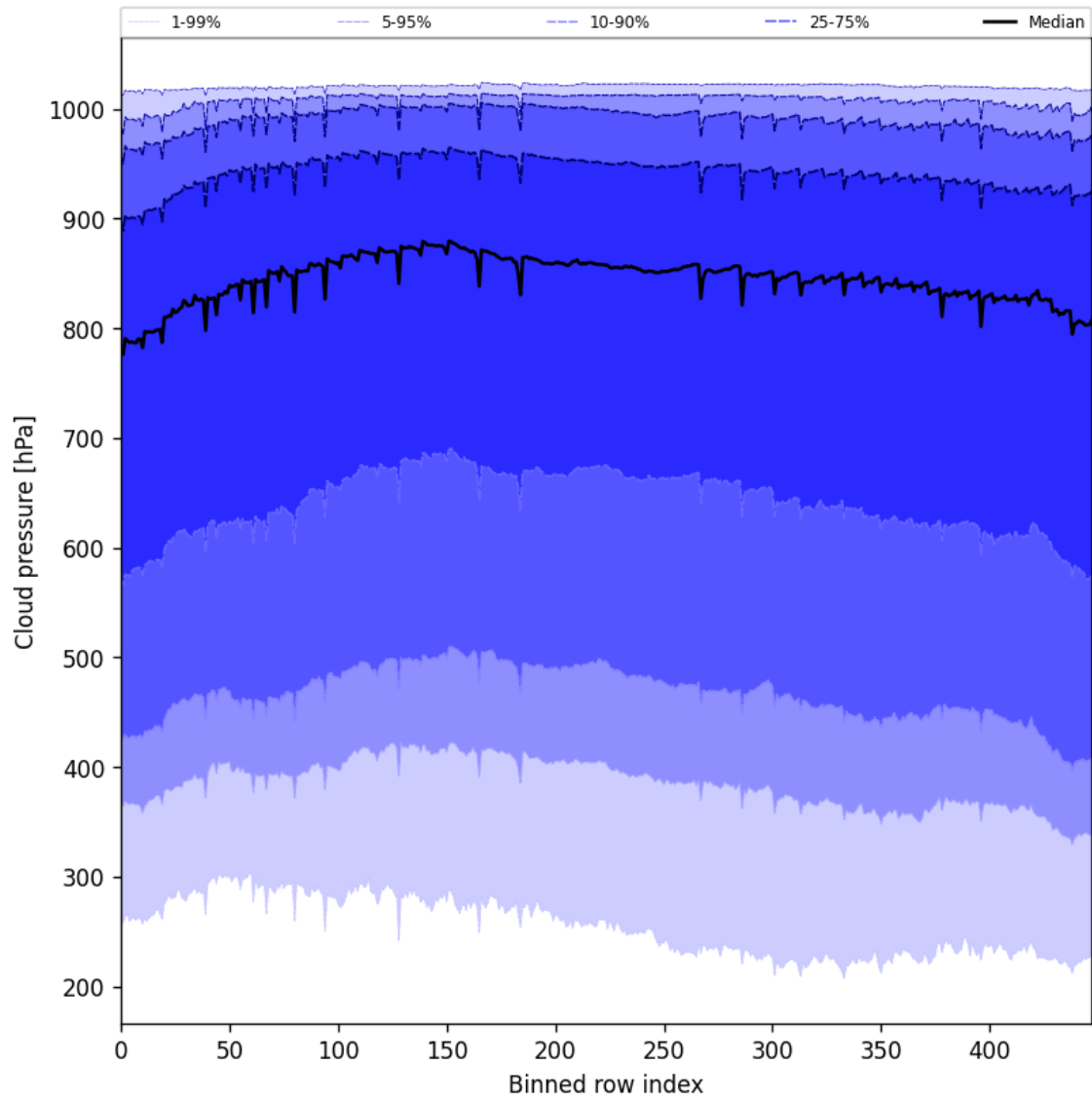
Figure 45: Along track statistics of “Cloud pressure” for 2025-08-26 to 2025-08-27
