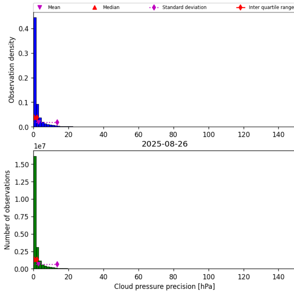
Figure 29: Histogram of “Cloud pressure precision” for 2025-08-26 to 2025-08-27
