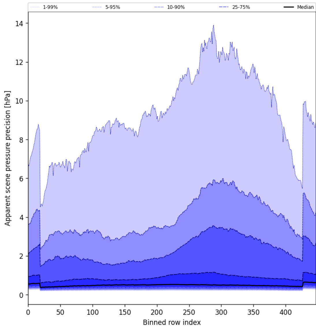
Figure 52: Along track statistics of “Apparent scene pressure precision” for 2025-08-26 to 2025-08-27
