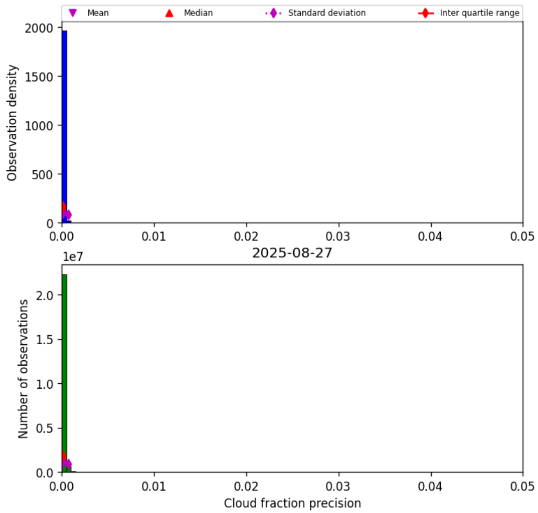
Figure 31: Histogram of “Cloud fraction precision” for 2025-08-27 to 2025-08-28
