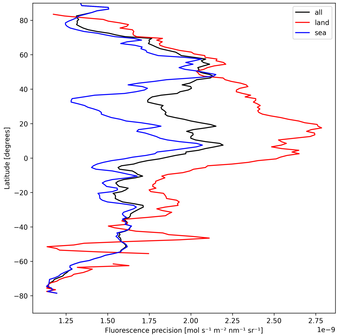
Figure 22: Zonal average of "Fluorescence precision" for 2025-08-27 to 2025-08-28.
