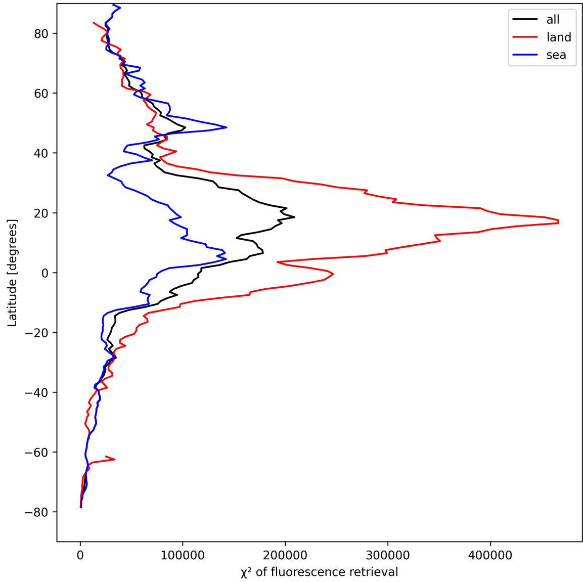
Figure 23: Zonal average of “ \chi^2 of fluorescence retrieval” for 2025-08-27 to 2025-08-28.
