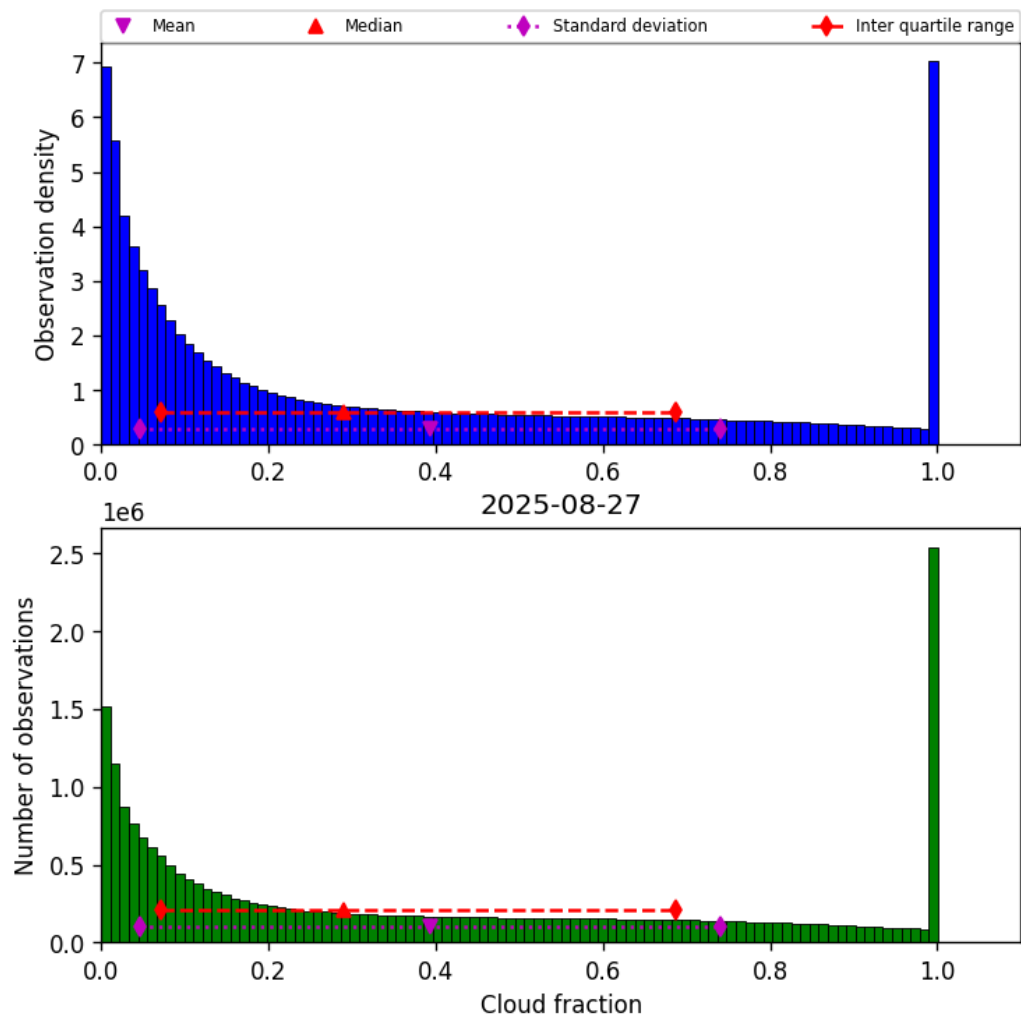
Figure 30: Histogram of “Cloud fraction” for 2025-08-27 to 2025-08-28
