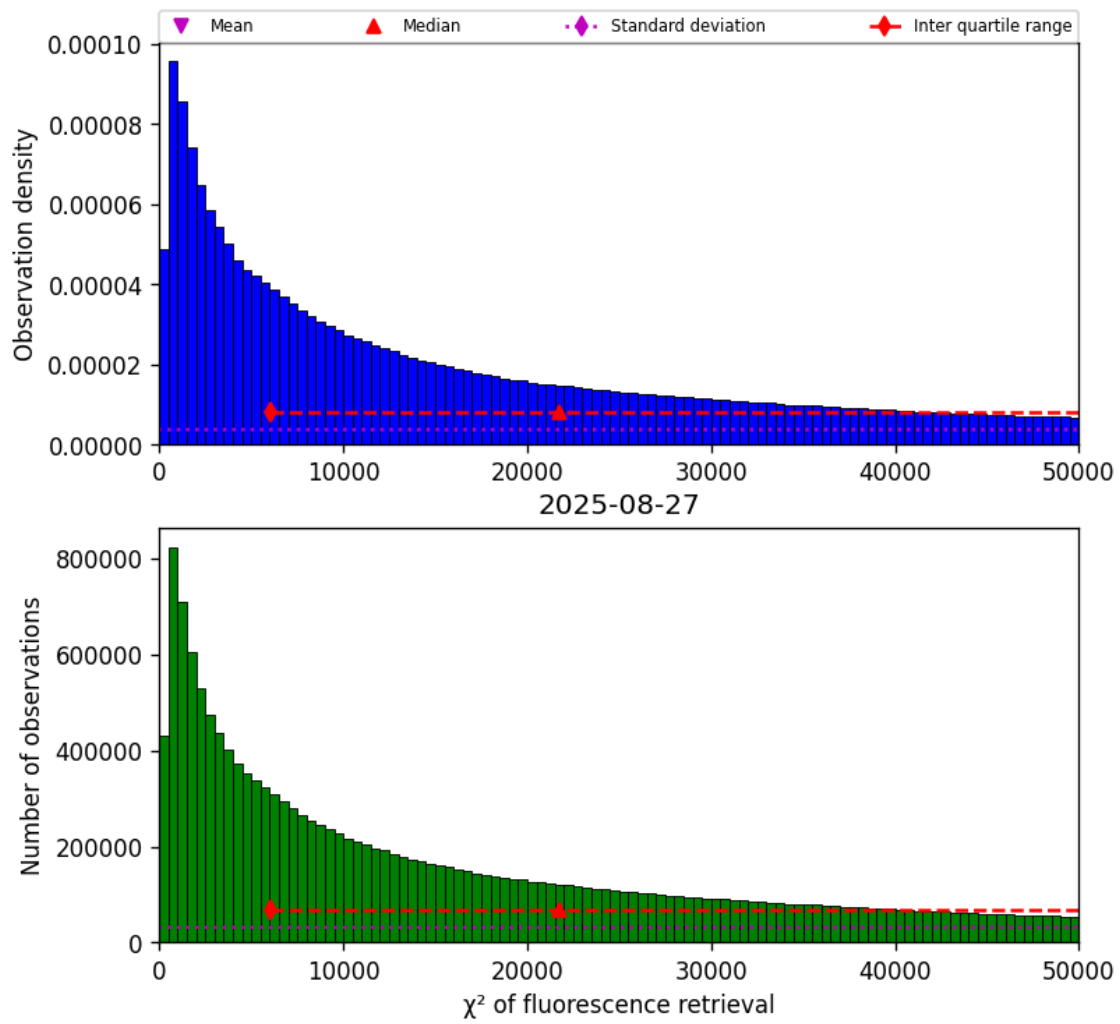
Figure 40: Histogram of “ \chi^2 of fluorescence retrieval” for 2025-08-27 to 2025-08-28
