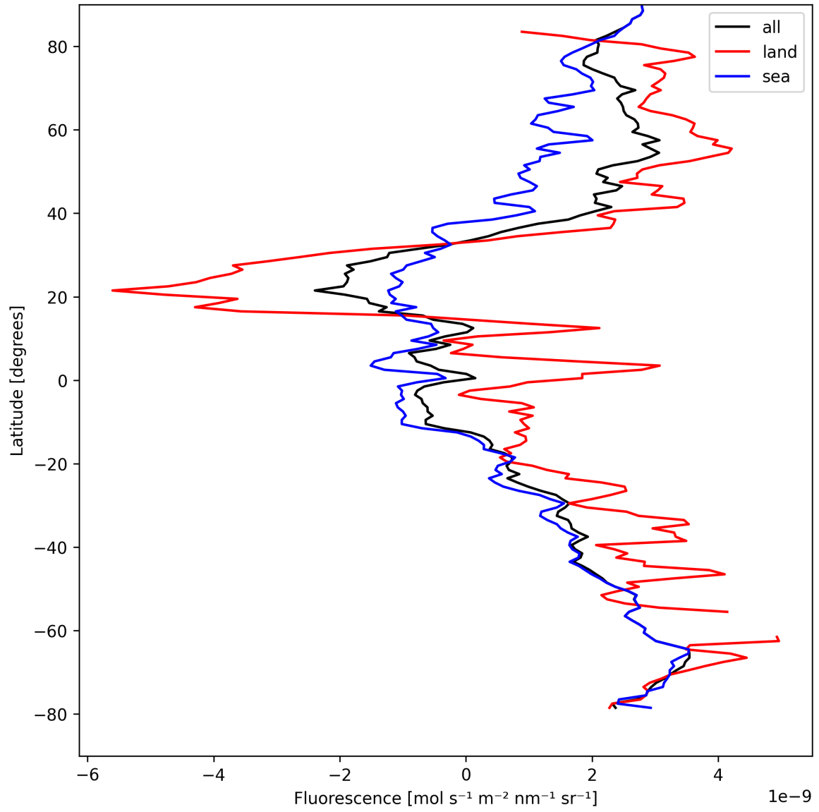
Figure 21: Zonal average of “Fluorescence” for 2025-08-27 to 2025-08-28.
