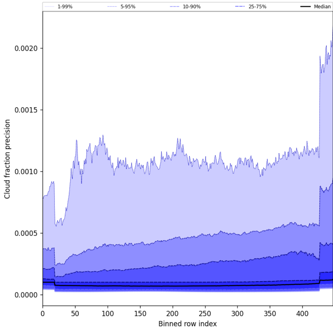
Figure 48: Along track statistics of “Cloud fraction precision” for 2025-08-27 to 2025-08-28
