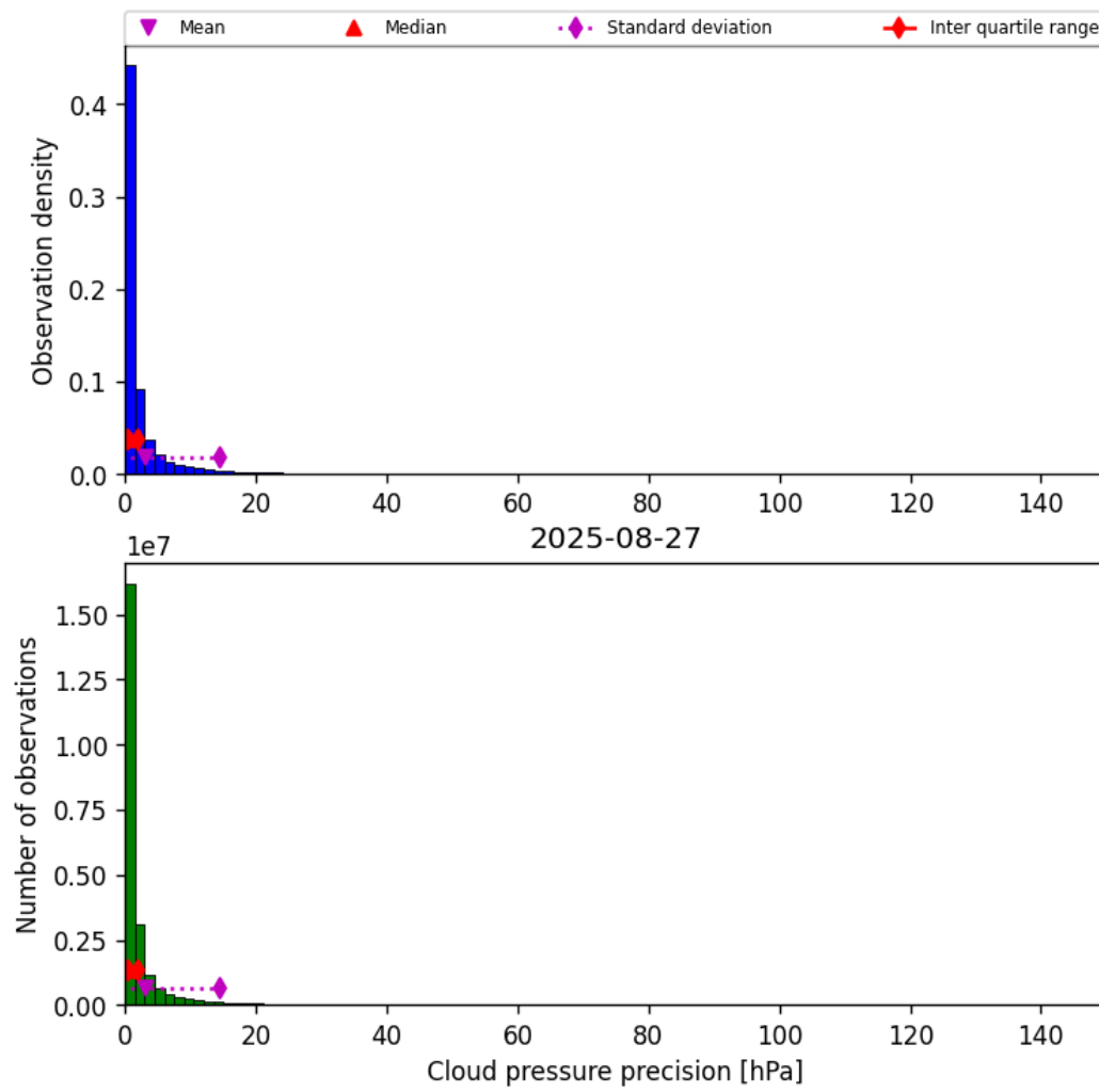
Figure 29: Histogram of “Cloud pressure precision” for 2025-08-27 to 2025-08-28
