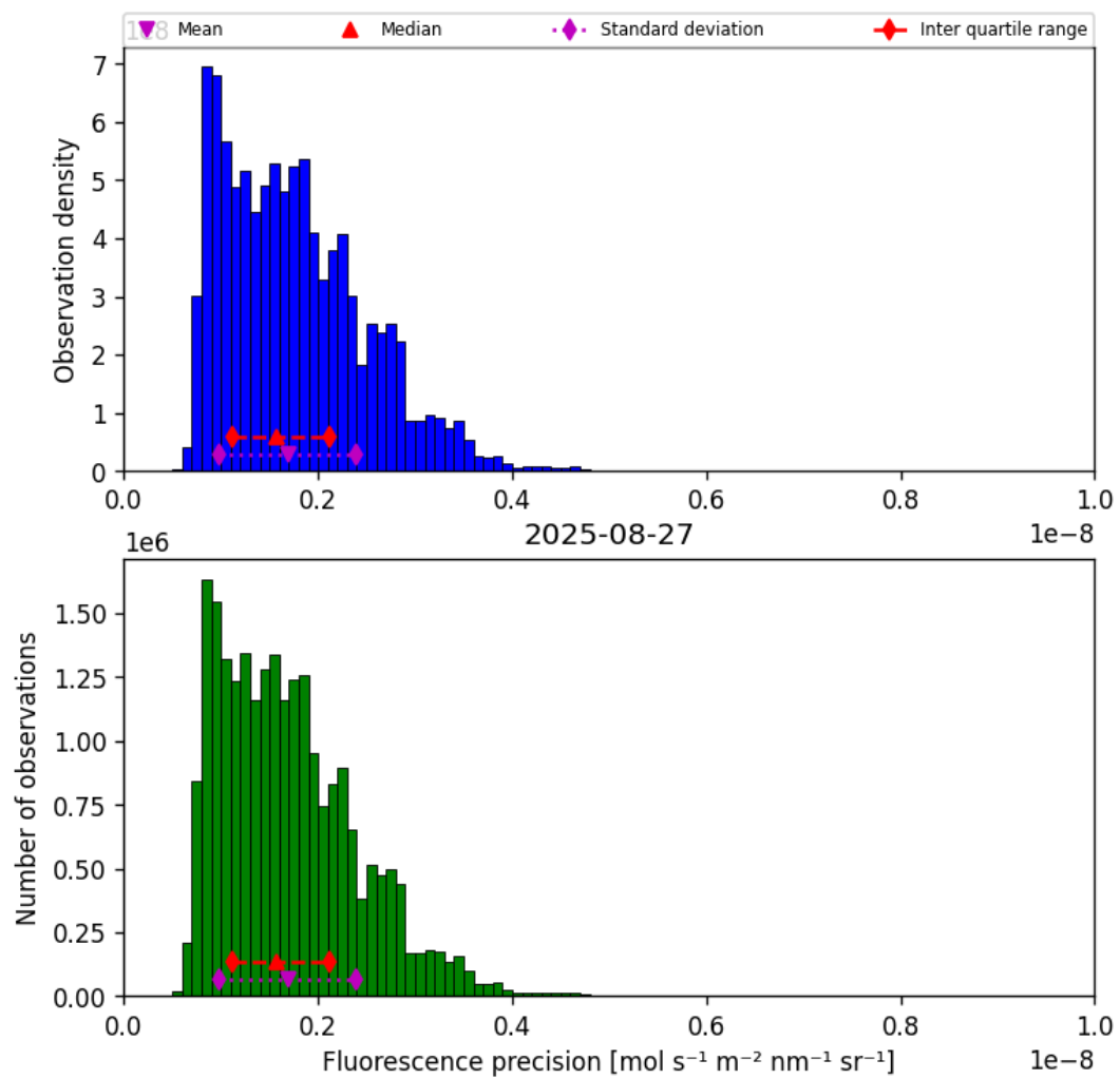
Figure 39: Histogram of “Fluorescence precision” for 2025-08-27 to 2025-08-28
