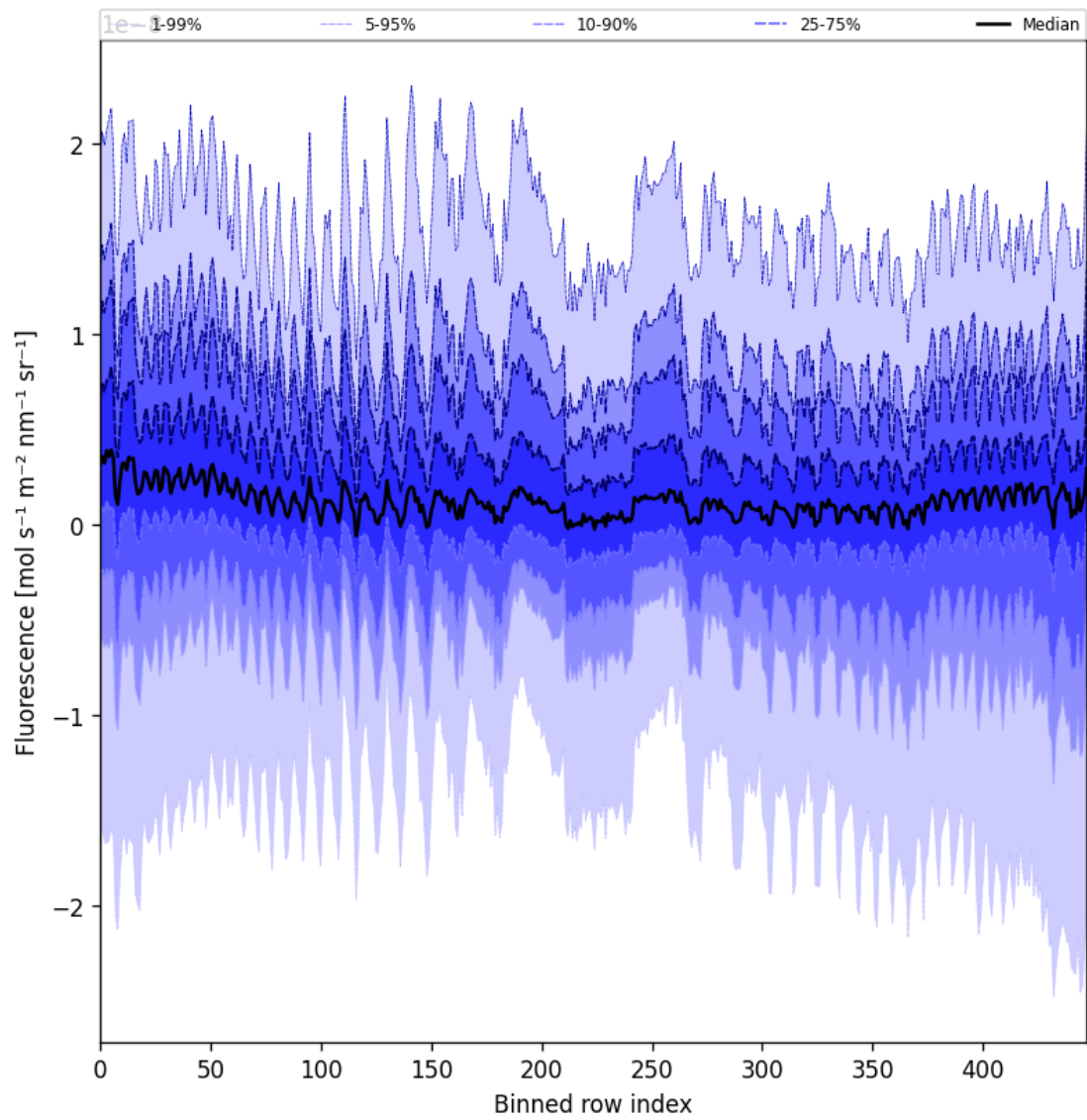
Figure 55: Along track statistics of "Fluorescence" for 2025-08-27 to 2025-08-28
