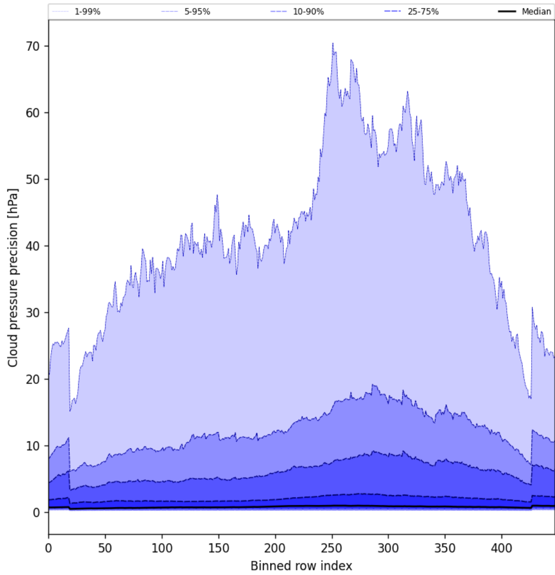
Figure 46: Along track statistics of “Cloud pressure precision” for 2025-08-27 to 2025-08-28
