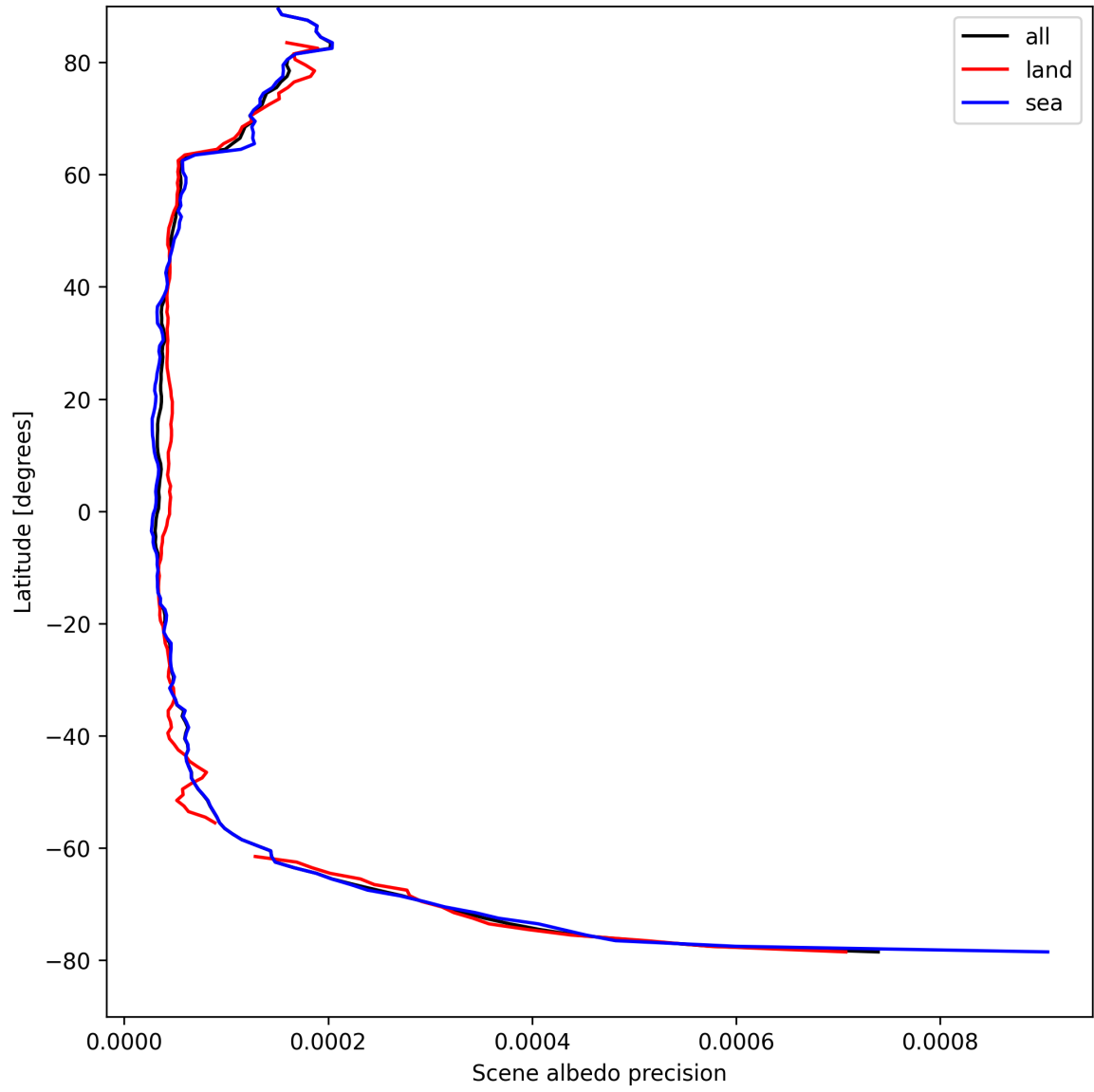
Figure 16: Zonal average of “Scene albedo precision” for 2025-08-27 to 2025-08-28.
