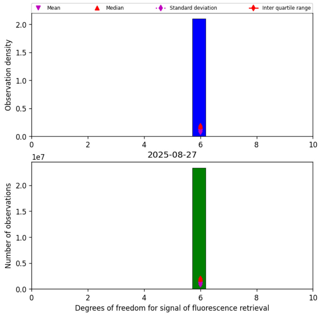
Figure 41: Histogram of “Degrees of freedom for signal of fluorescence retrieval” for 2025-08-27 to 2025-08-28
