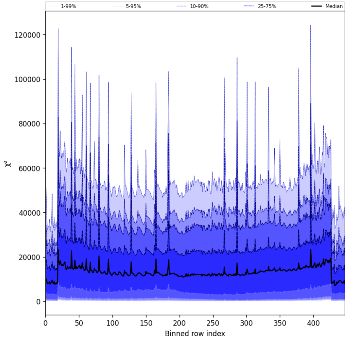
Figure 53: Along track statistics of “ \chi^2 ” for 2025-08-27 to 2025-08-28
