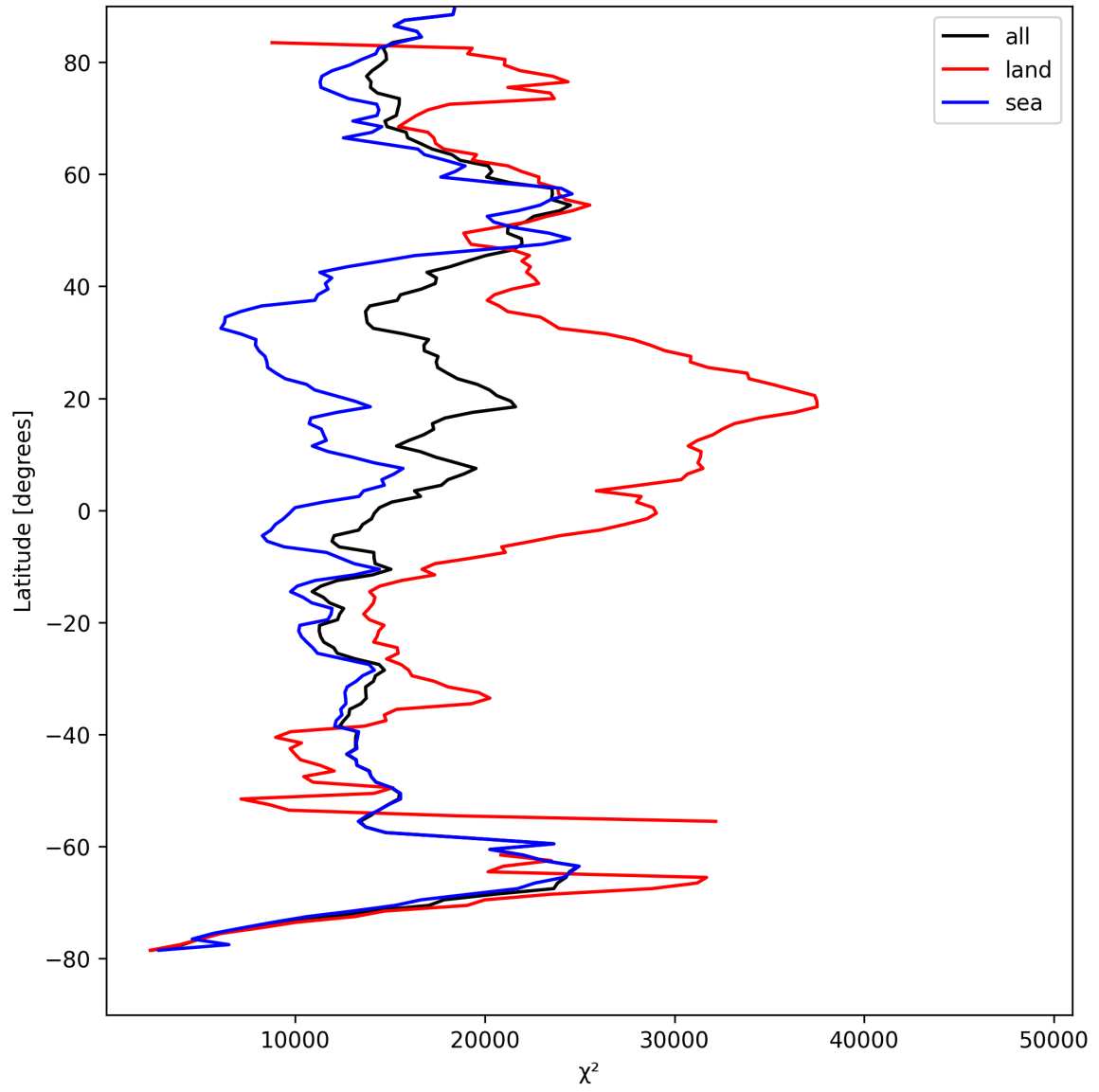
Figure 19: Zonal average of “ \chi^2 ” for 2025-08-27 to 2025-08-28.
