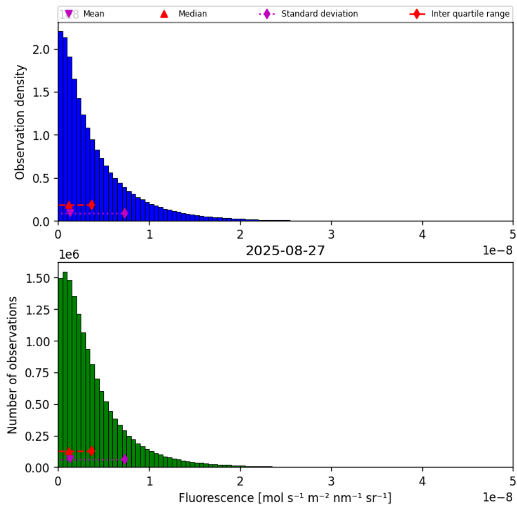
Figure 38: Histogram of “Fluorescence” for 2025-08-27 to 2025-08-28
