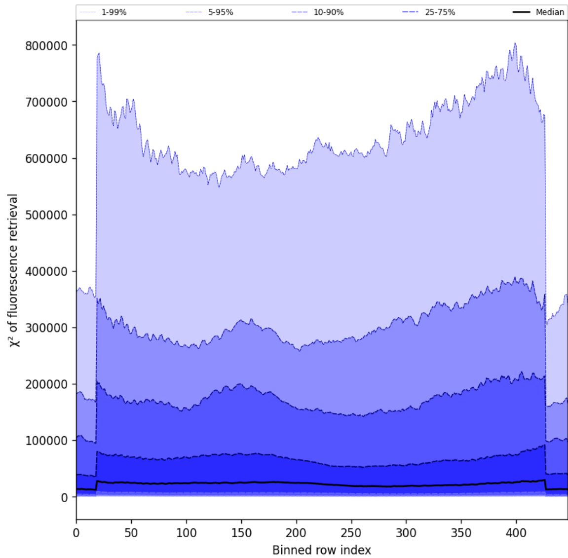
Figure 57: Along track statistics of “ \chi^2 of fluorescence retrieval” for 2025-08-27 to 2025-08-28
