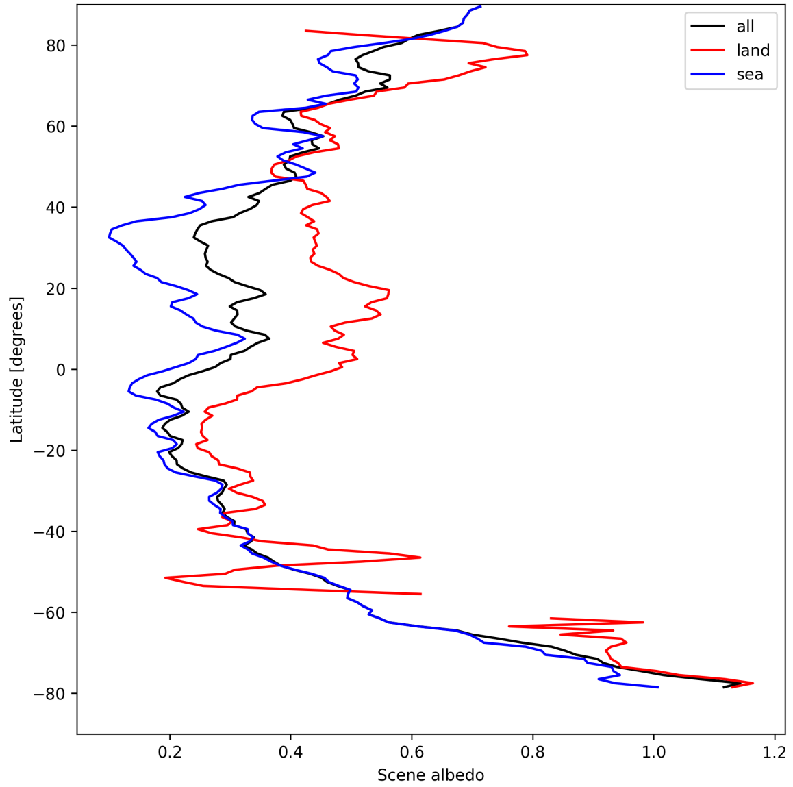
Figure 15: Zonal average of “Scene albedo” for 2025-08-27 to 2025-08-28.
