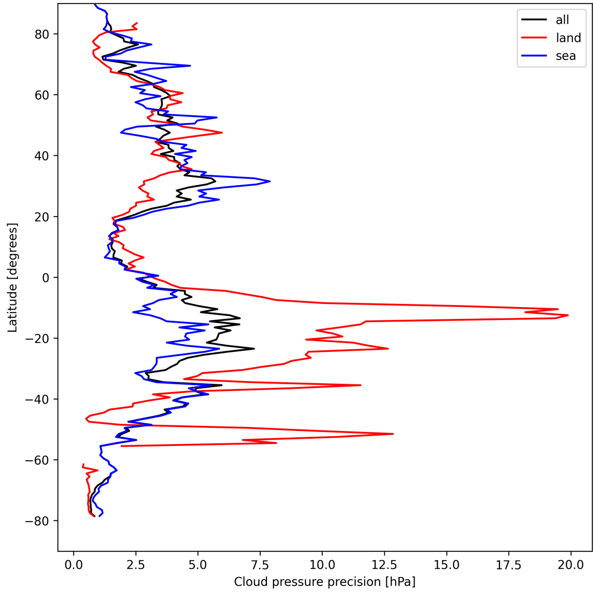
Figure 12: Zonal average of “Cloud pressure precision” for 2025-08-27 to 2025-08-28.
