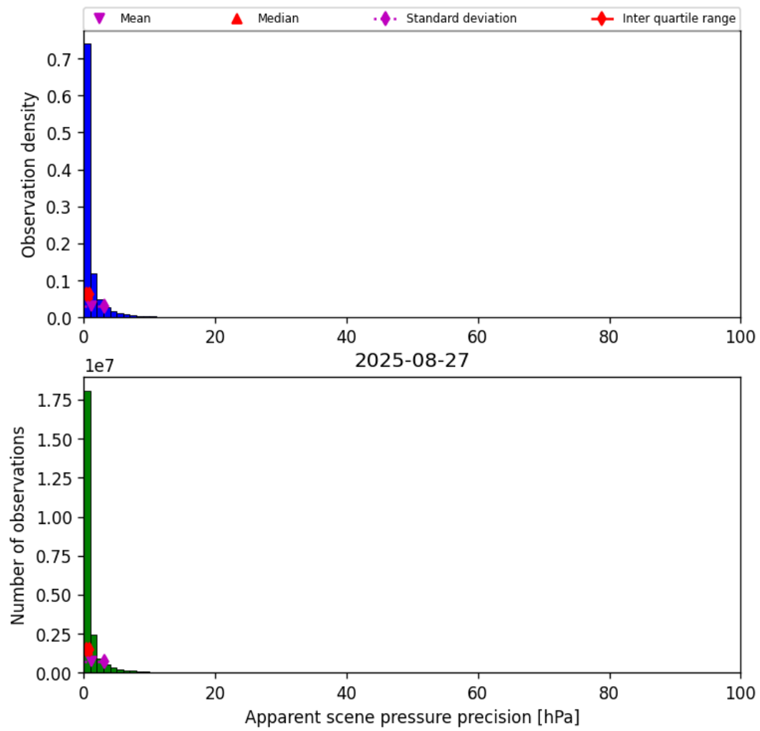
Figure 35: Histogram of “Apparent scene pressure precision” for 2025-08-27 to 2025-08-28
