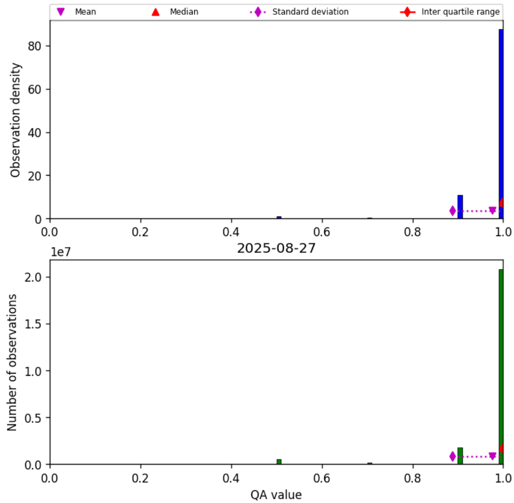
Figure 27: Histogram of “QA value” for 2025-08-27 to 2025-08-28
