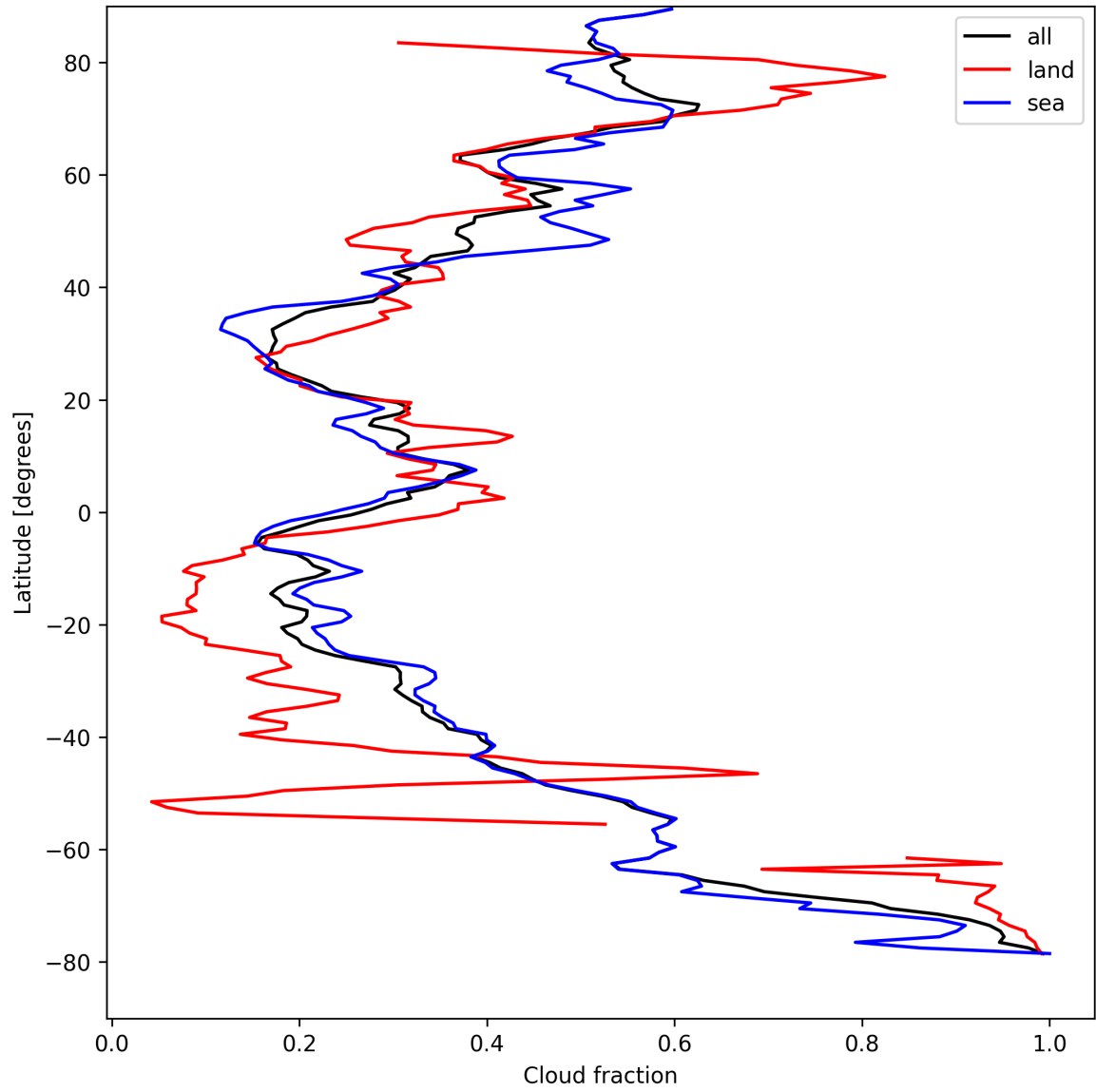
Figure 13: Zonal average of “Cloud fraction” for 2025-08-27 to 2025-08-28.
