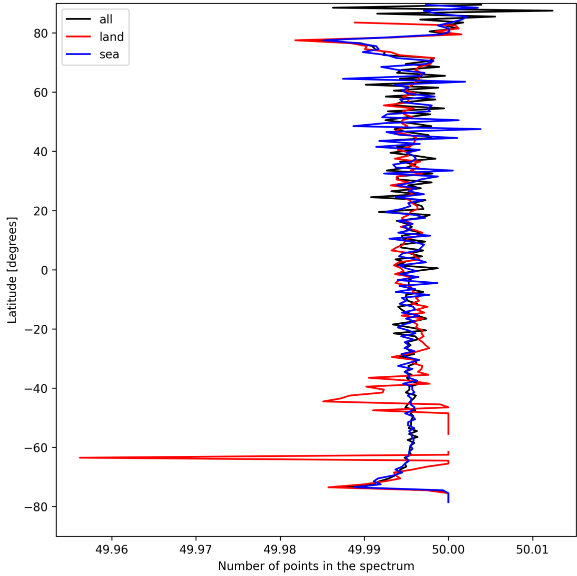
Figure 25: Zonal average of “Number of points in the spectrum” for 2025-08-27 to 2025-08-28.
