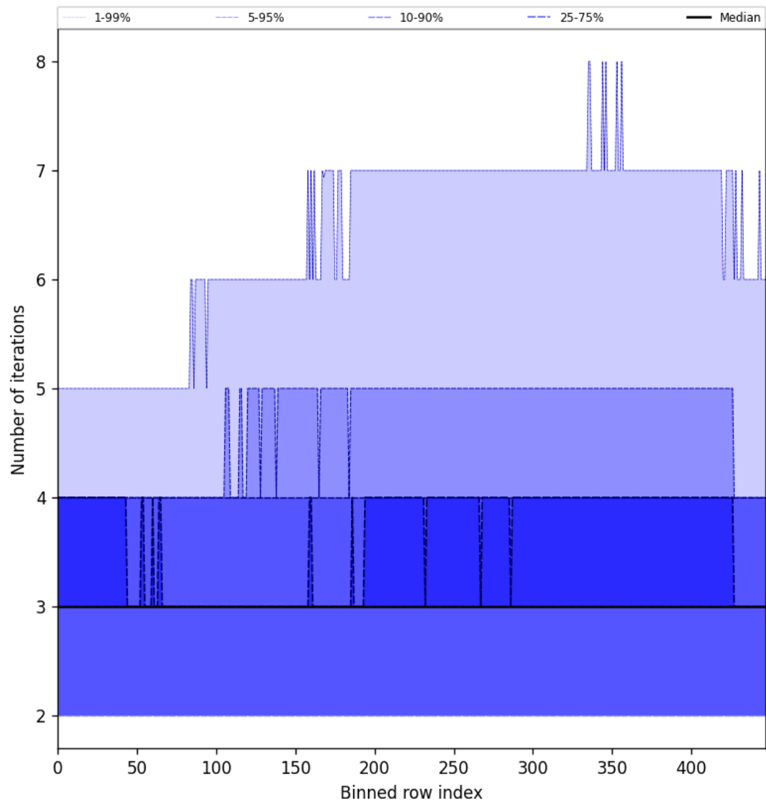
Figure 54: Along track statistics of “Number of iterations” for 2025-08-27 to 2025-08-28
