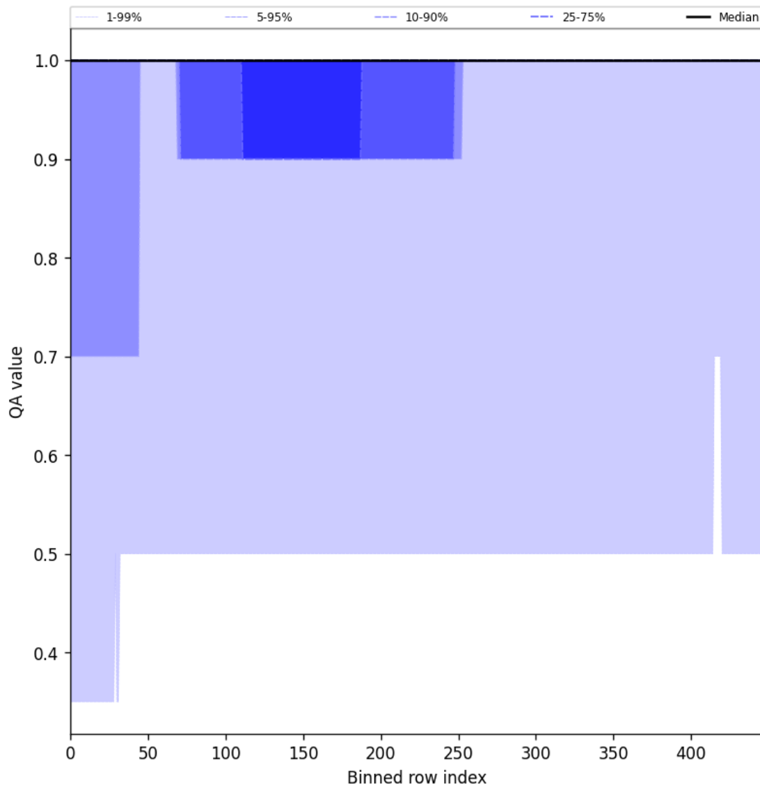
Figure 44: Along track statistics of “QA value” for 2025-08-27 to 2025-08-28
