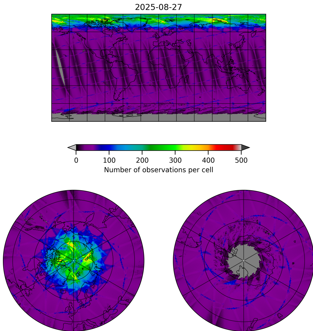
Figure 9: Map of the number of observations for 2025-08-27 to 2025-08-28
