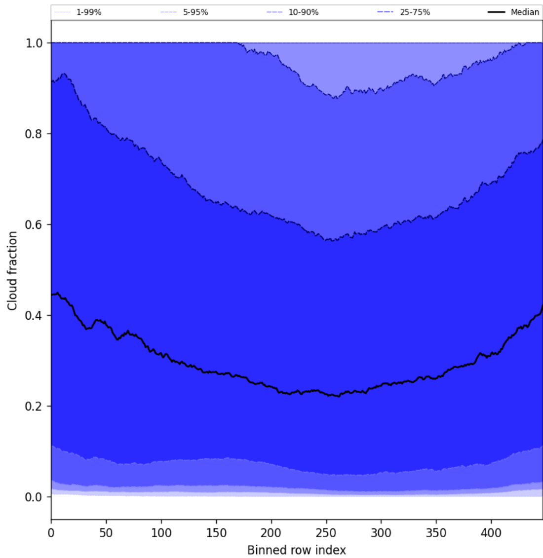
Figure 47: Along track statistics of “Cloud fraction” for 2025-08-27 to 2025-08-28
