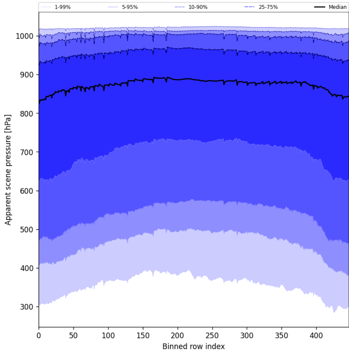
Figure 51: Along track statistics of “Apparent scene pressure” for 2025-08-27 to 2025-08-28
