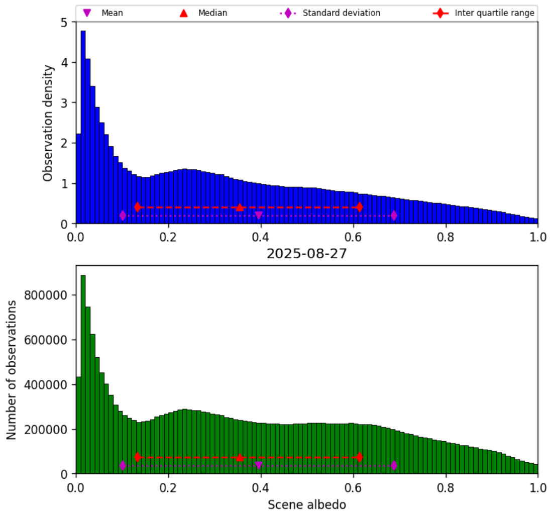
Figure 32: Histogram of “Scene albedo” for 2025-08-27 to 2025-08-28
