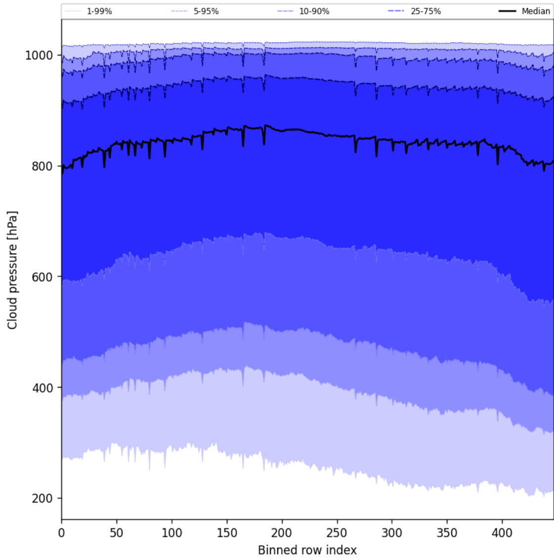
Figure 45: Along track statistics of “Cloud pressure” for 2025-08-27 to 2025-08-28
