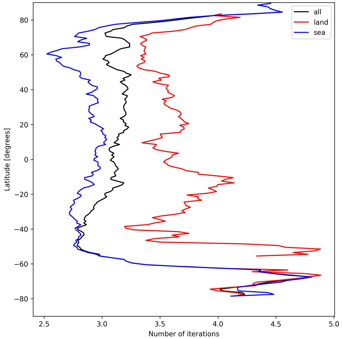
Figure 20: Zonal average of “Number of iterations” for 2025-08-27 to 2025-08-28.
