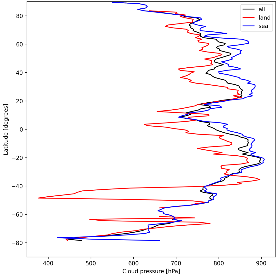
Figure 11: Zonal average of “Cloud pressure” for 2025-08-27 to 2025-08-28.
