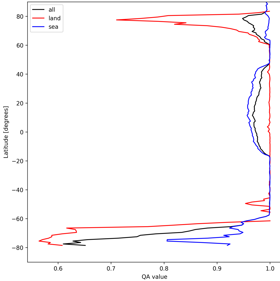
Figure 10: Zonal average of "QA value" for 2025-08-27 to 2025-08-28.
