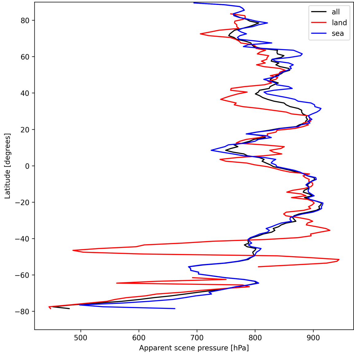
Figure 17: Zonal average of “Apparent scene pressure” for 2025-08-27 to 2025-08-28.
