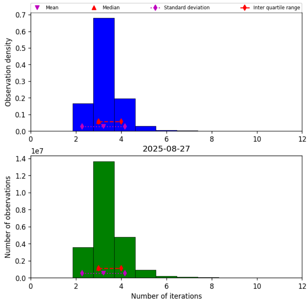
Figure 37: Histogram of “Number of iterations” for 2025-08-27 to 2025-08-28
