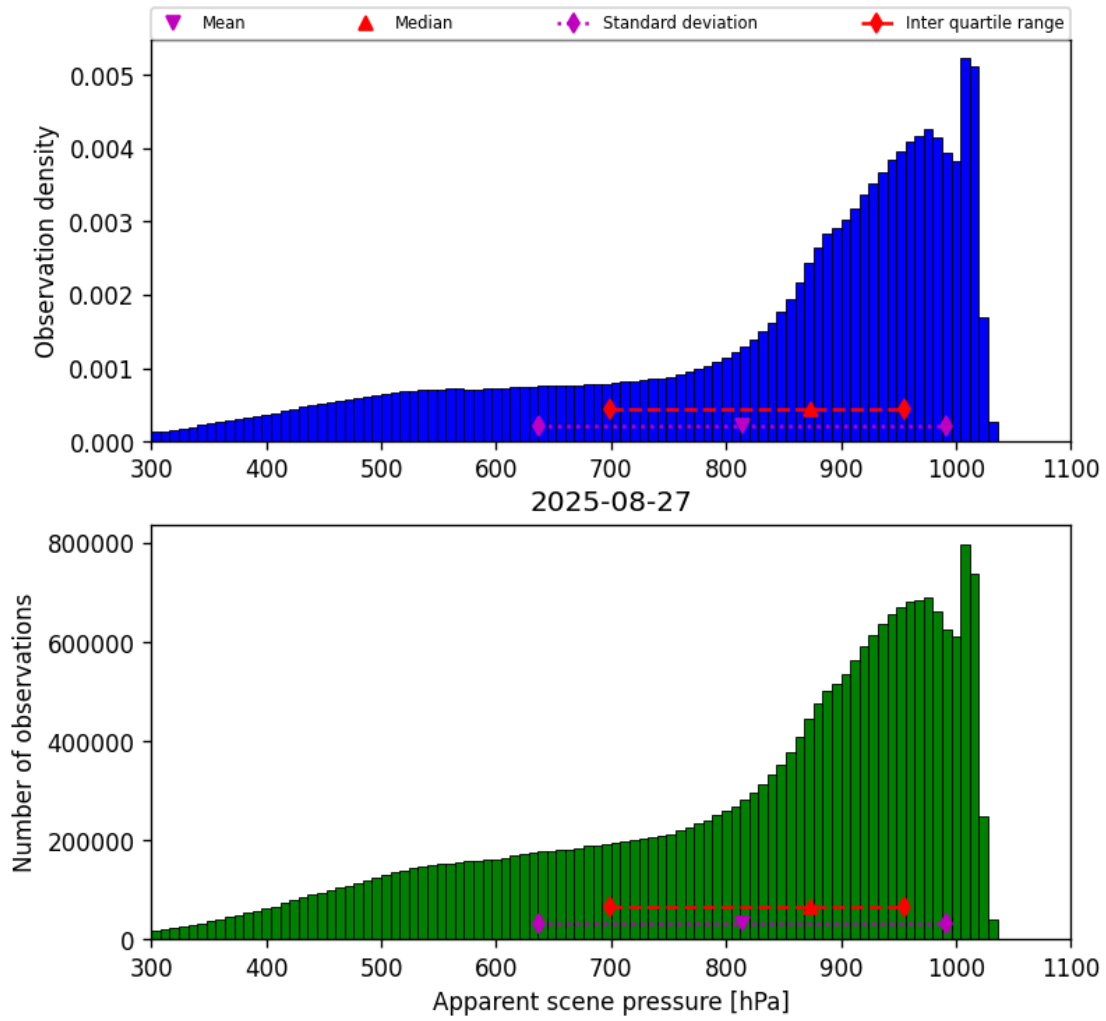
Figure 34: Histogram of “Apparent scene pressure” for 2025-08-27 to 2025-08-28
