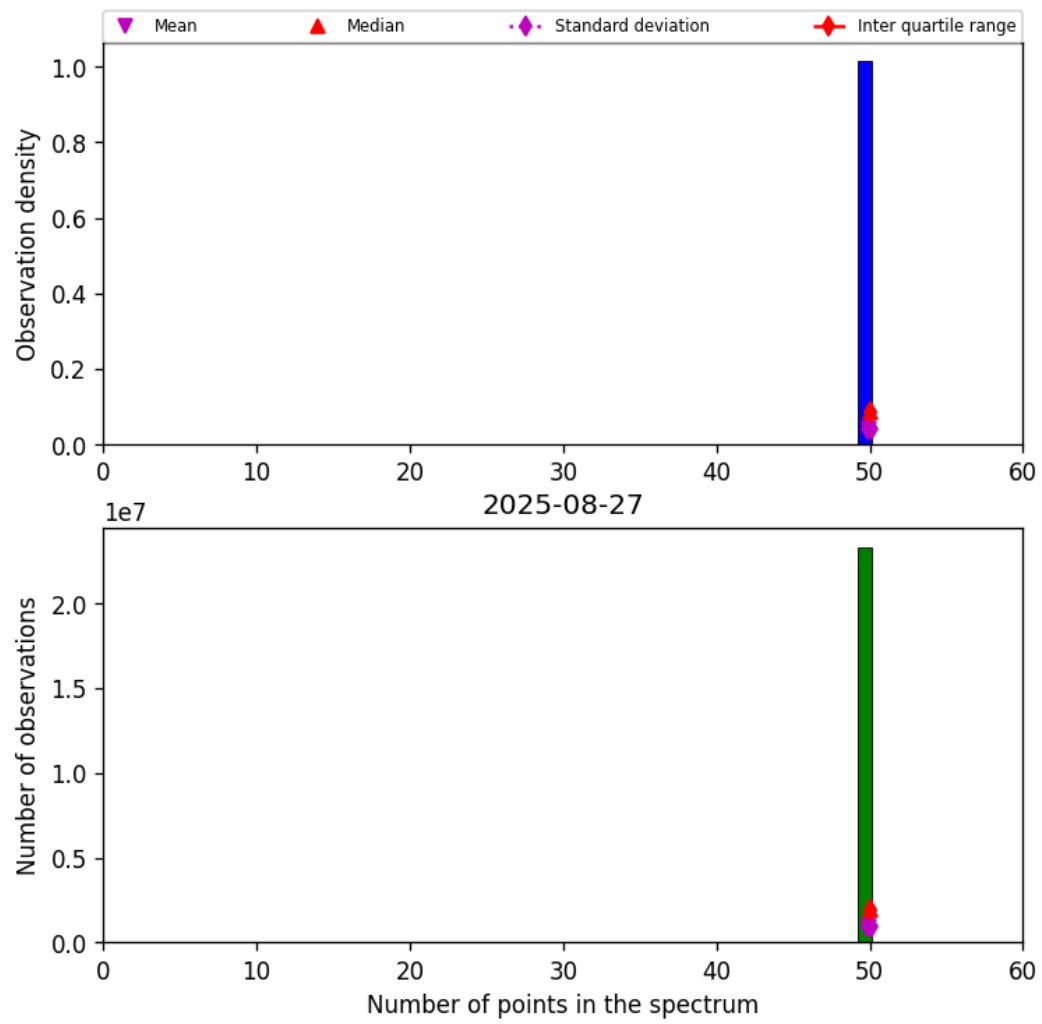
Figure 42: Histogram of “Number of points in the spectrum” for 2025-08-27 to 2025-08-28
