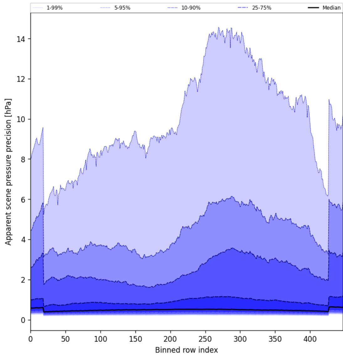
Figure 52: Along track statistics of “Apparent scene pressure precision” for 2025-08-27 to 2025-08-28
