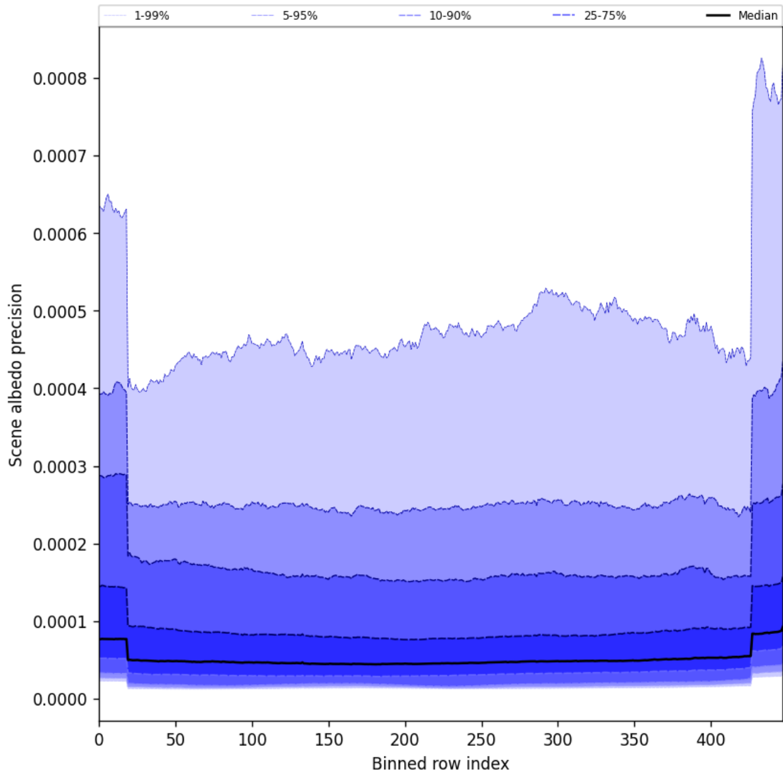
Figure 50: Along track statistics of “Scene albedo precision” for 2025-08-27 to 2025-08-28
