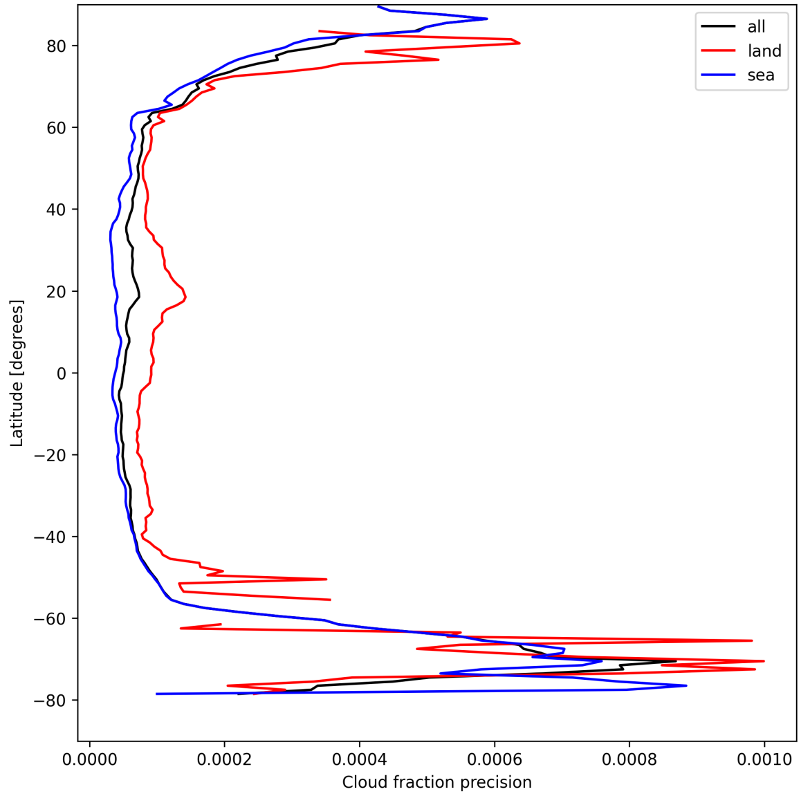
Figure 14: Zonal average of “Cloud fraction precision” for 2025-08-27 to 2025-08-28.
