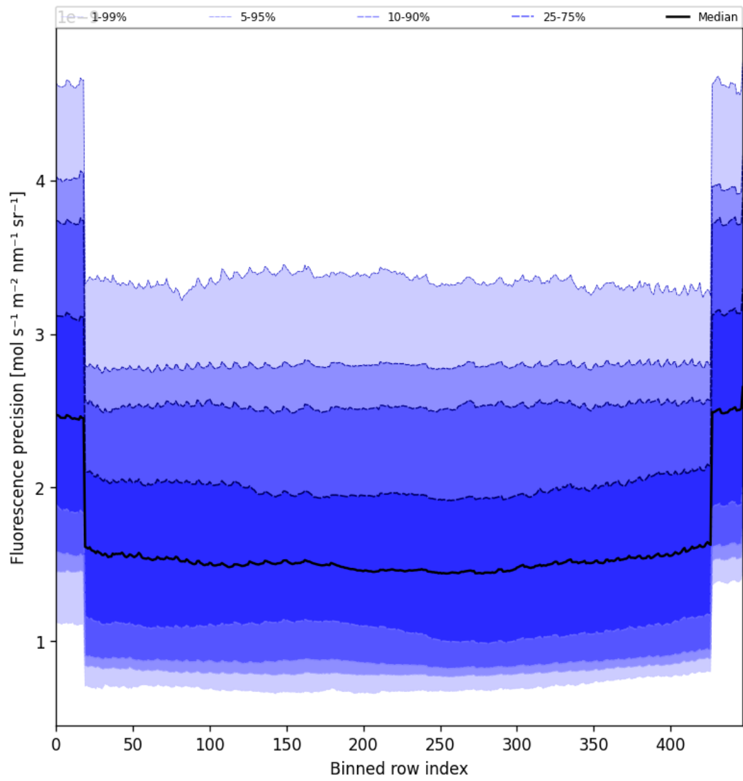
Figure 56: Along track statistics of “Fluorescence precision” for 2025-08-27 to 2025-08-28
