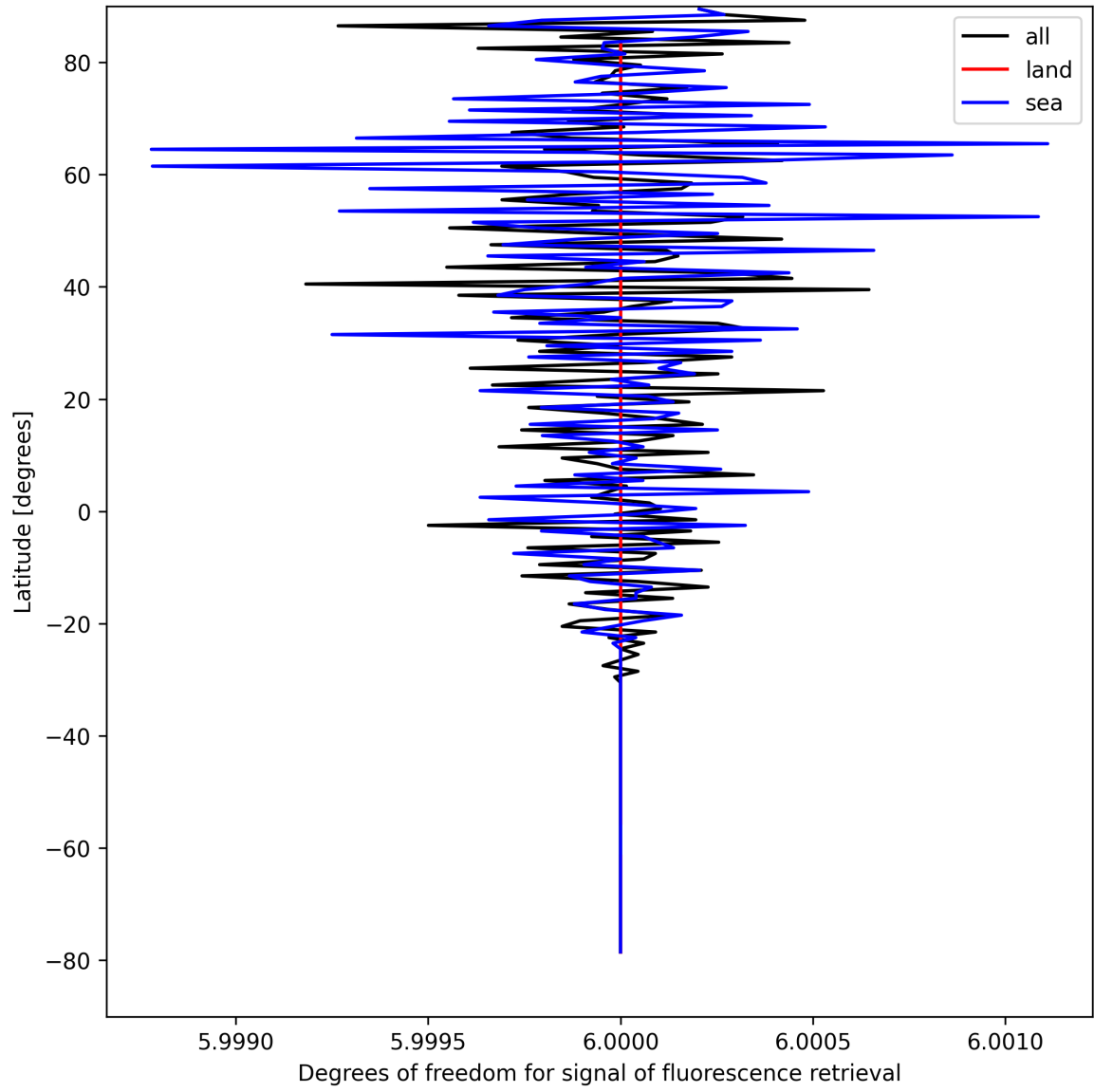
Figure 24: Zonal average of “Degrees of freedom for signal of fluorescence retrieval” for 2025-08-27 to 2025-08-28.
