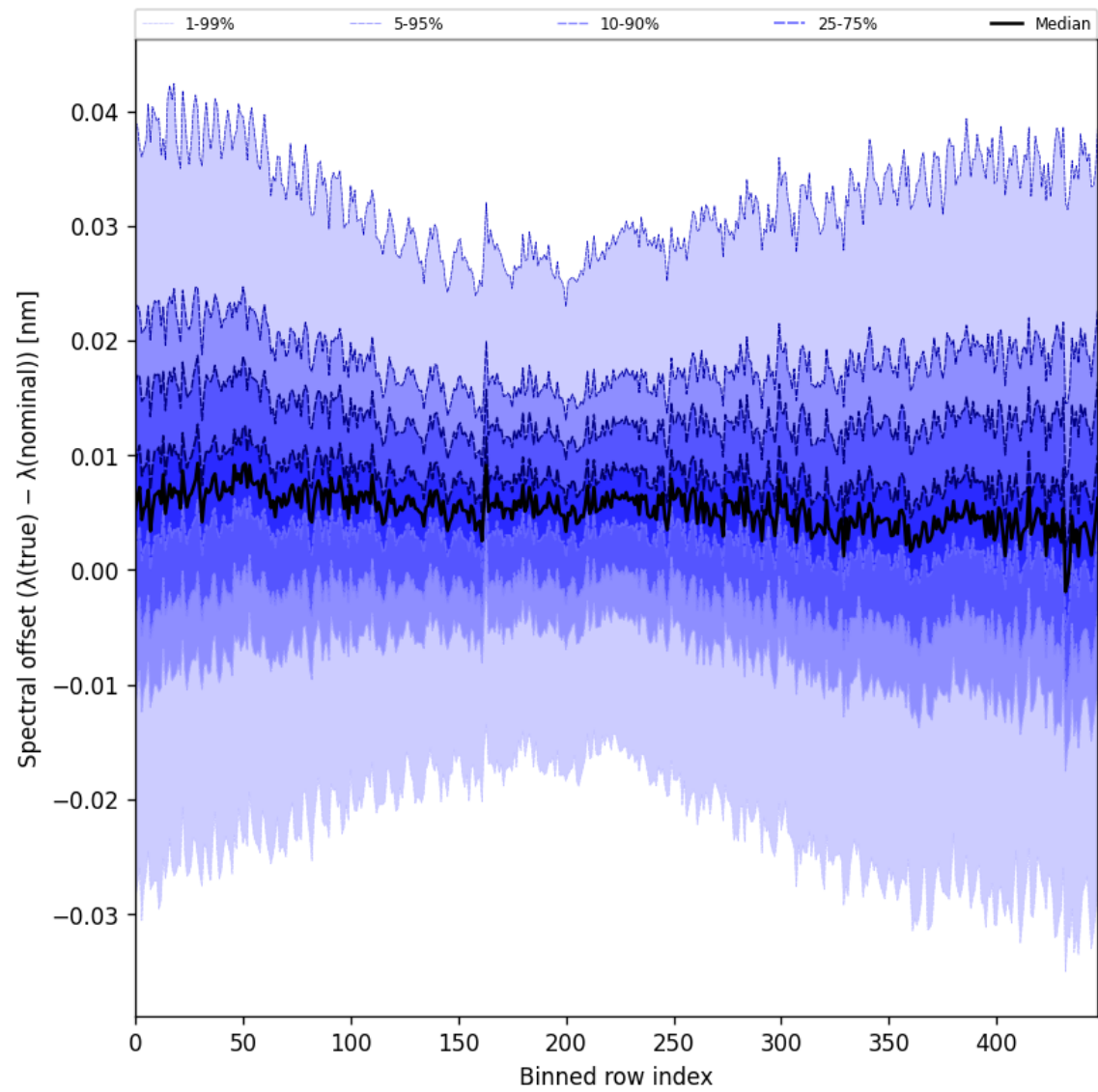
Figure 60: Along track statistics of “Spectral offset ( \lambda_{\text{true}} - \lambda_{\text{nominal}} )” for 2025-08-27 to 2025-08-28
