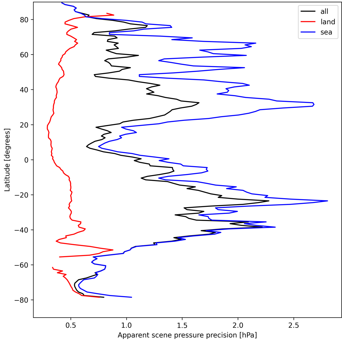
Figure 18: Zonal average of “Apparent scene pressure precision” for 2025-08-27 to 2025-08-28.
