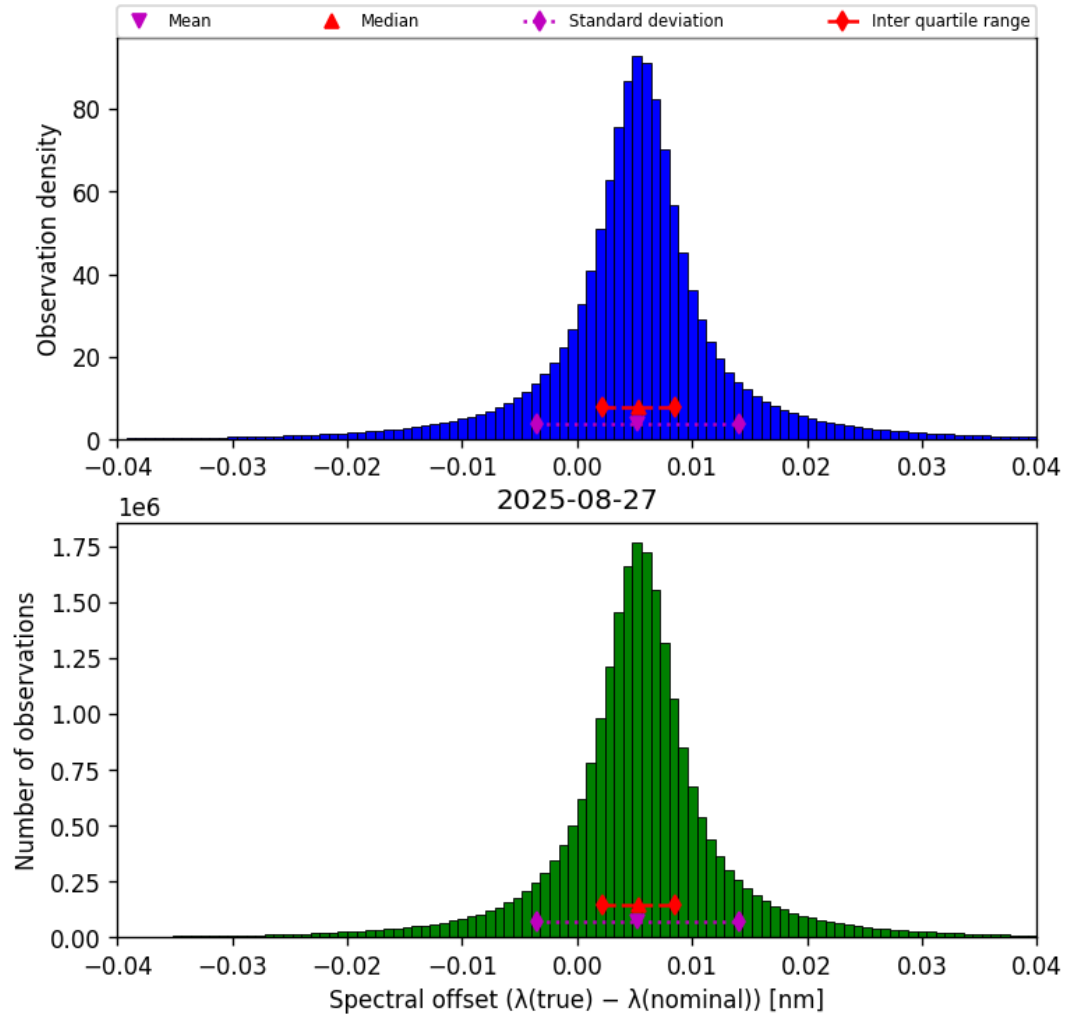
Figure 43: Histogram of “Spectral offset ( \lambda_{\text{true}} - \lambda_{\text{nominal}} )” for 2025-08-27 to 2025-08-28
