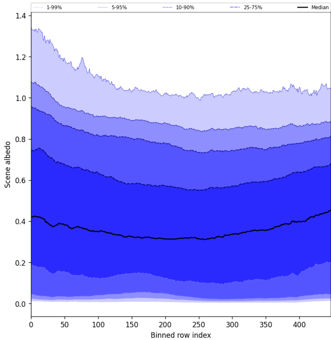
Figure 49: Along track statistics of “Scene albedo” for 2025-08-27 to 2025-08-28
