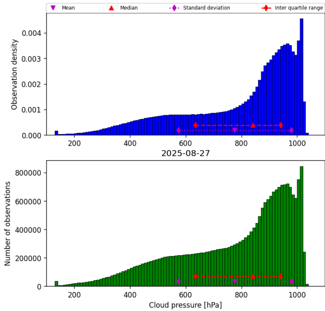
Figure 28: Histogram of “Cloud pressure” for 2025-08-27 to 2025-08-28
