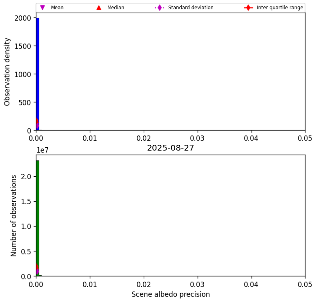
Figure 33: Histogram of “Scene albedo precision” for 2025-08-27 to 2025-08-28
