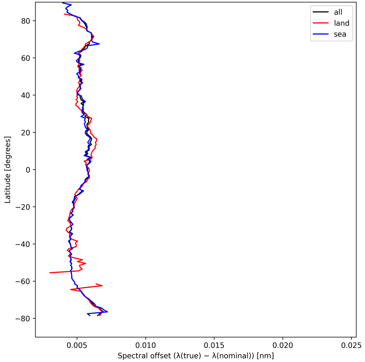
Figure 26: Zonal average of “Spectral offset ( \lambda_{\text{true}} - \lambda_{\text{nominal}} )” for 2025-08-27 to 2025-08-28.
