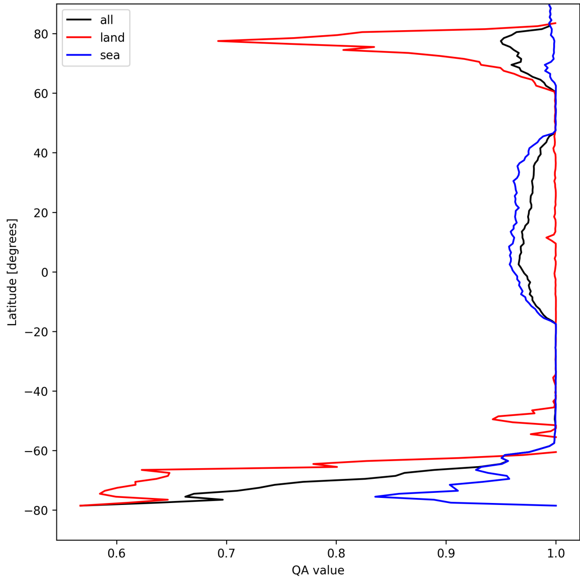
Figure 10: Zonal average of “QA value” for 2025-08-28 to 2025-08-28.
