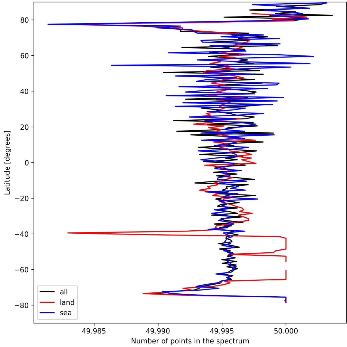
Figure 25: Zonal average of “Number of points in the spectrum” for 2025-08-28 to 2025-08-28.
