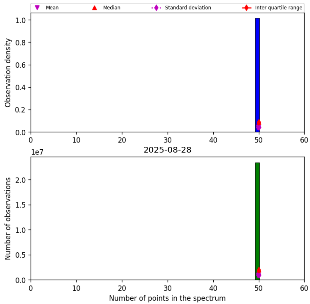
Figure 42: Histogram of “Number of points in the spectrum” for 2025-08-28 to 2025-08-28
