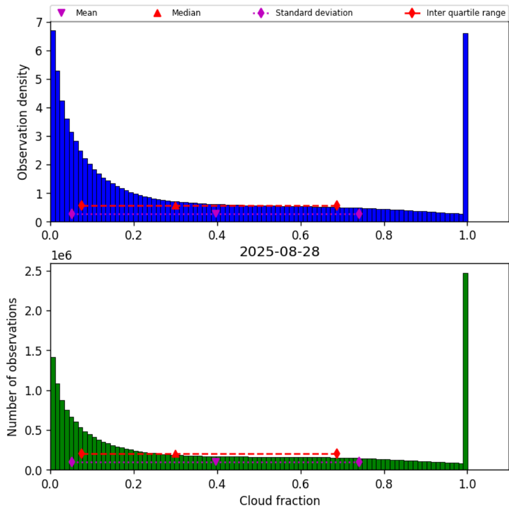
Figure 30: Histogram of “Cloud fraction” for 2025-08-28 to 2025-08-28
