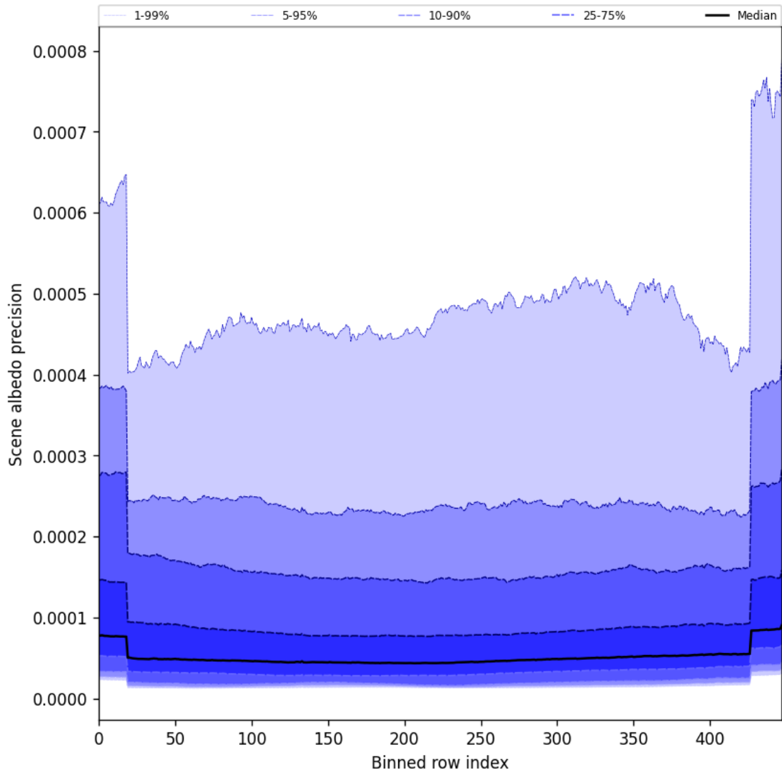
Figure 50: Along track statistics of “Scene albedo precision” for 2025-08-28 to 2025-08-28
