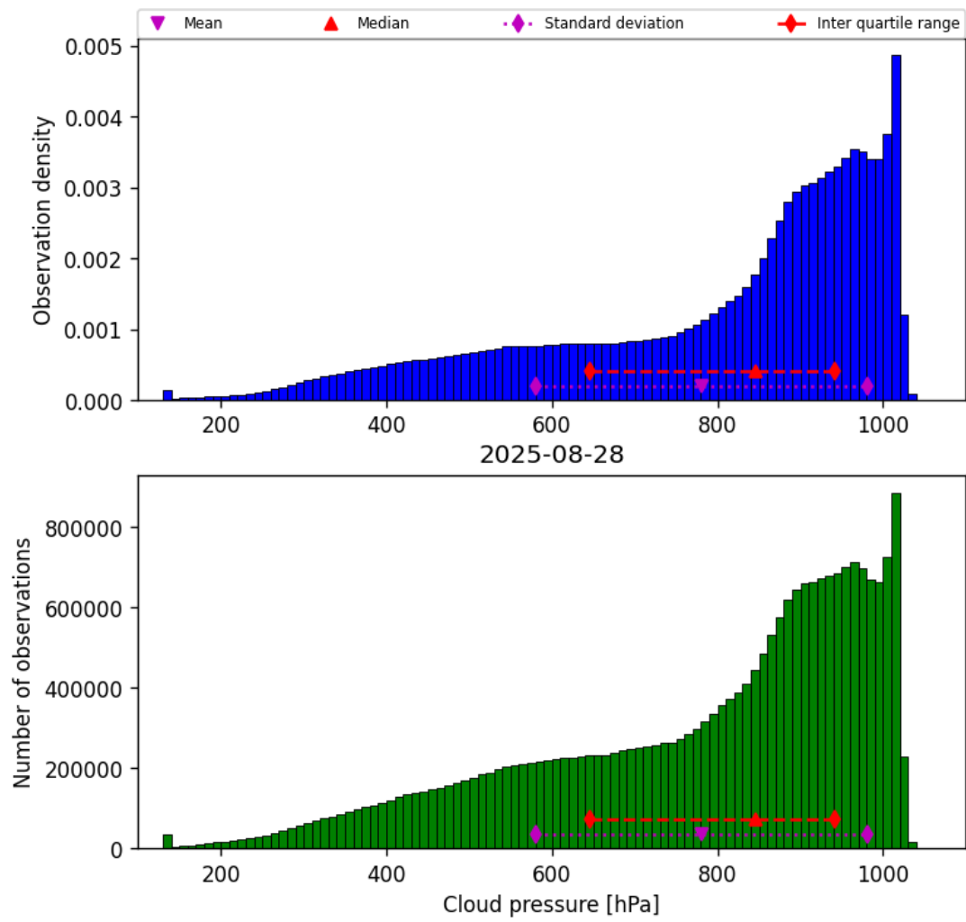
Figure 28: Histogram of “Cloud pressure” for 2025-08-28 to 2025-08-28
