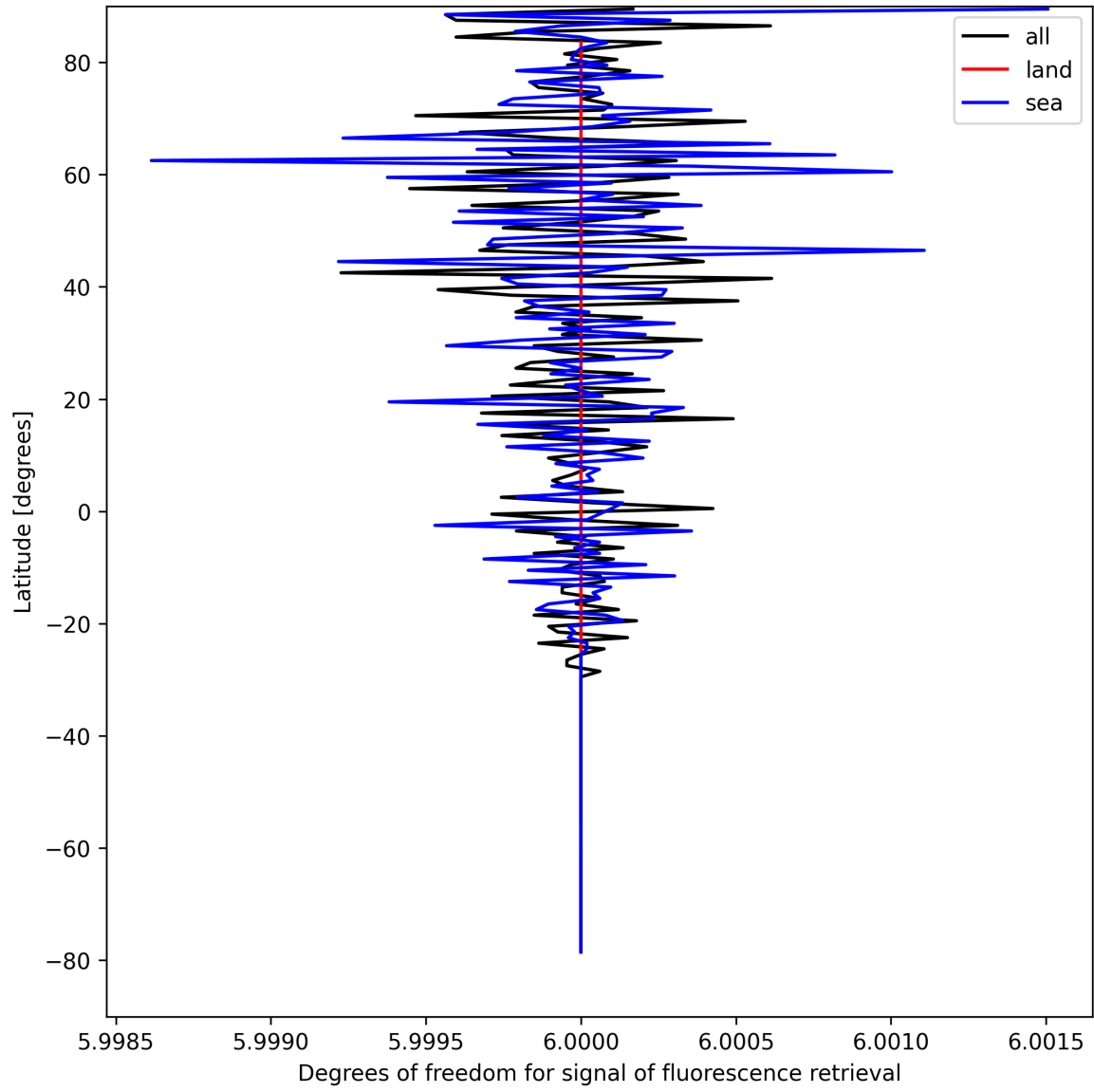
Figure 24: Zonal average of “Degrees of freedom for signal of fluorescence retrieval” for 2025-08-28 to 2025-08-28.
