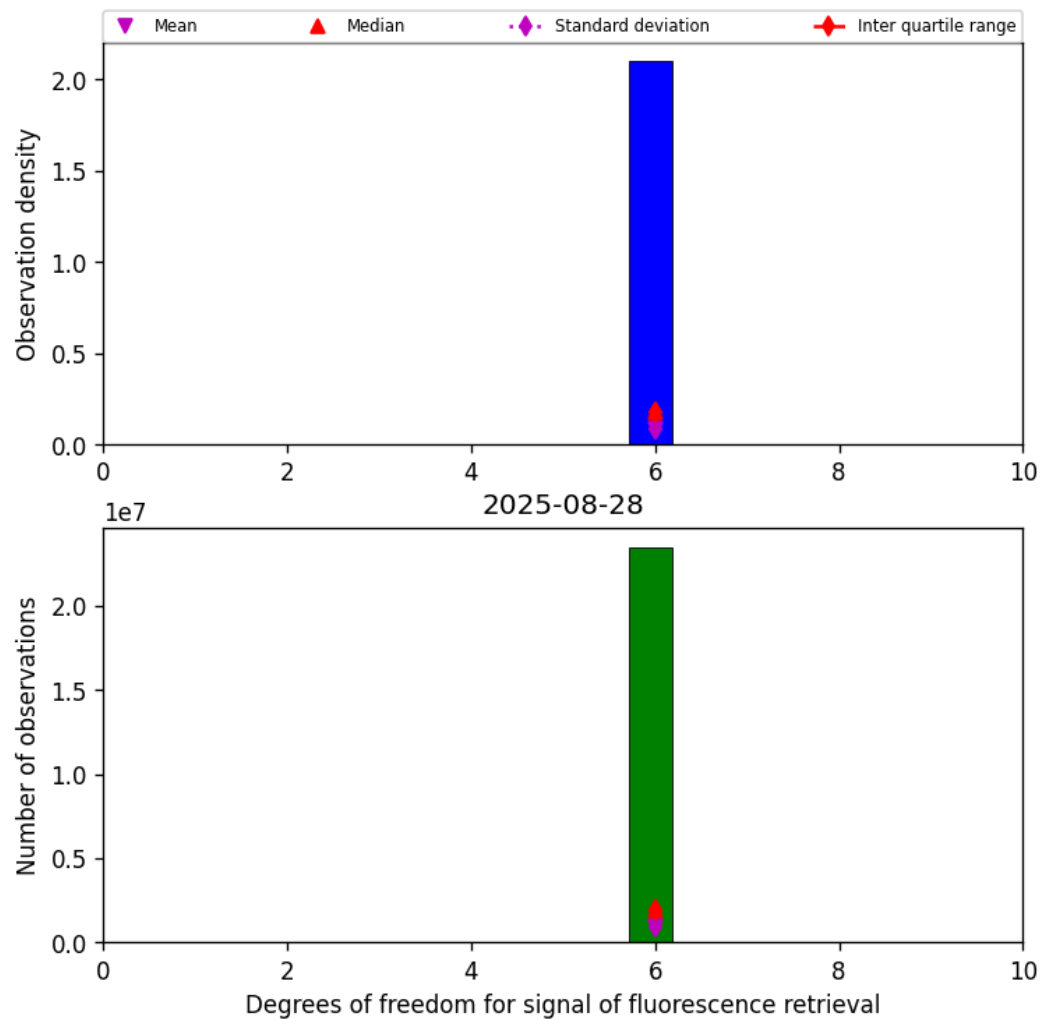
Figure 41: Histogram of “Degrees of freedom for signal of fluorescence retrieval” for 2025-08-28 to 2025-08-28
