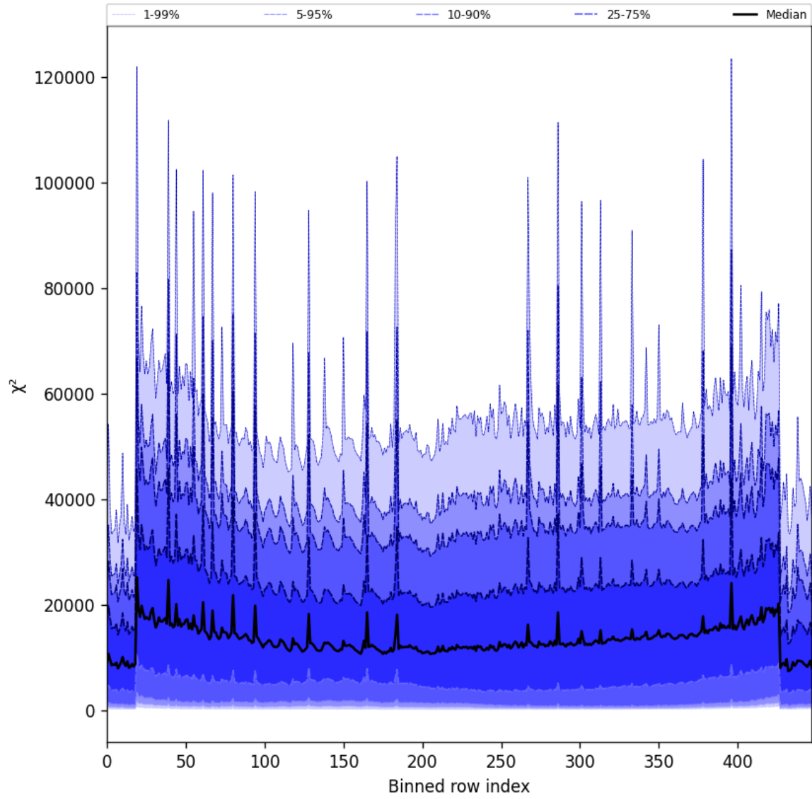
Figure 53: Along track statistics of " \chi^2 " for 2025-08-28 to 2025-08-28
