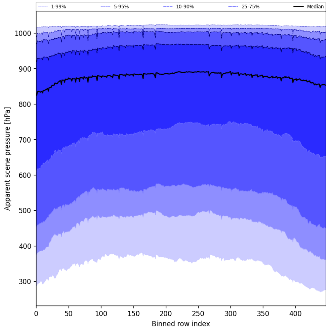
Figure 51: Along track statistics of “Apparent scene pressure” for 2025-08-28 to 2025-08-28
