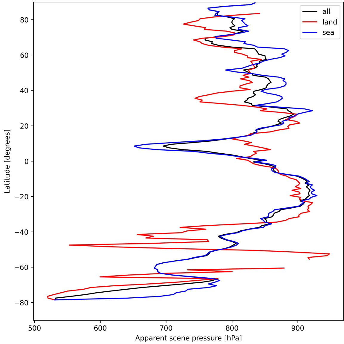
Figure 17: Zonal average of “Apparent scene pressure” for 2025-08-28 to 2025-08-28.
