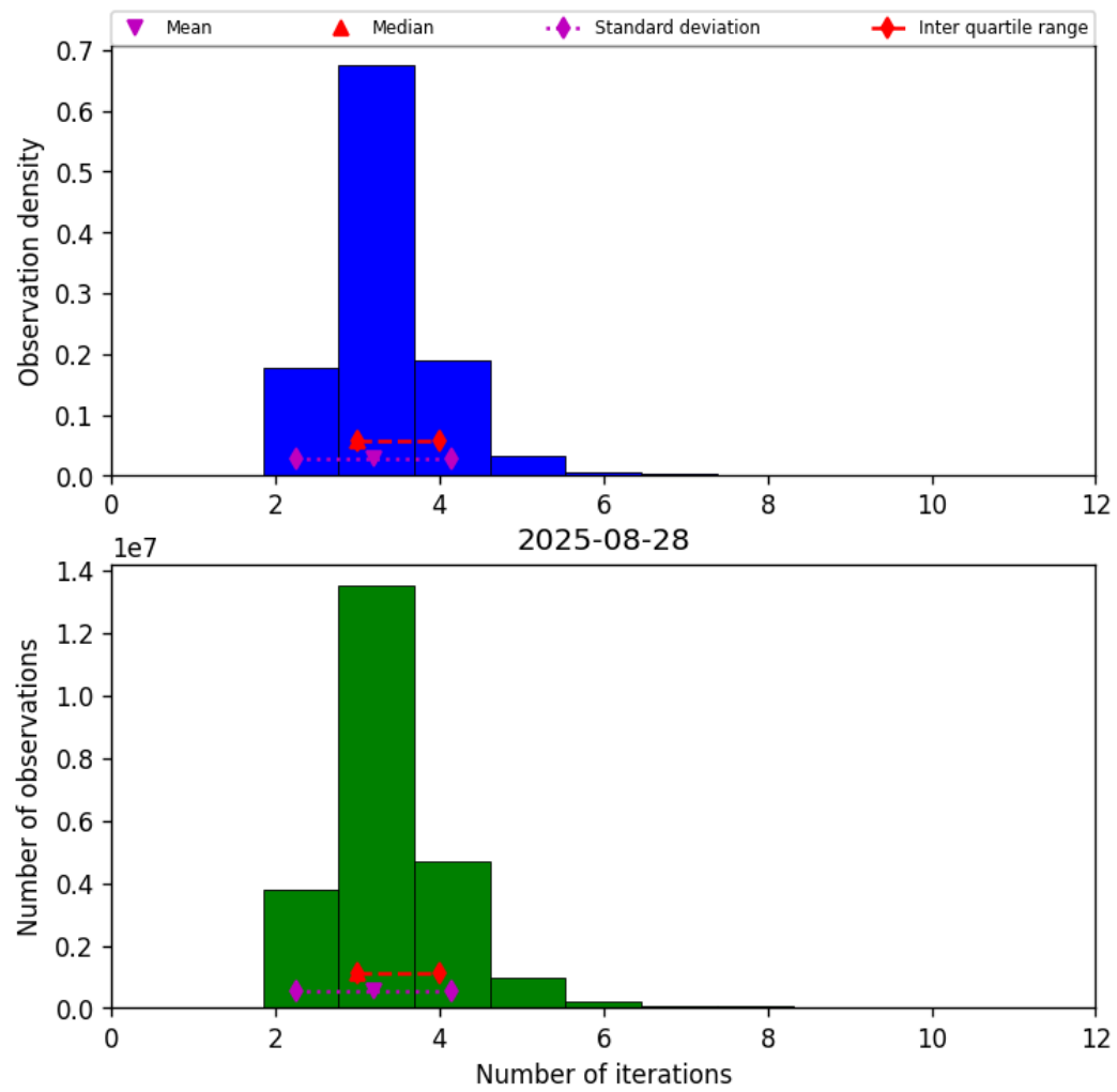
Figure 37: Histogram of “Number of iterations” for 2025-08-28 to 2025-08-28
