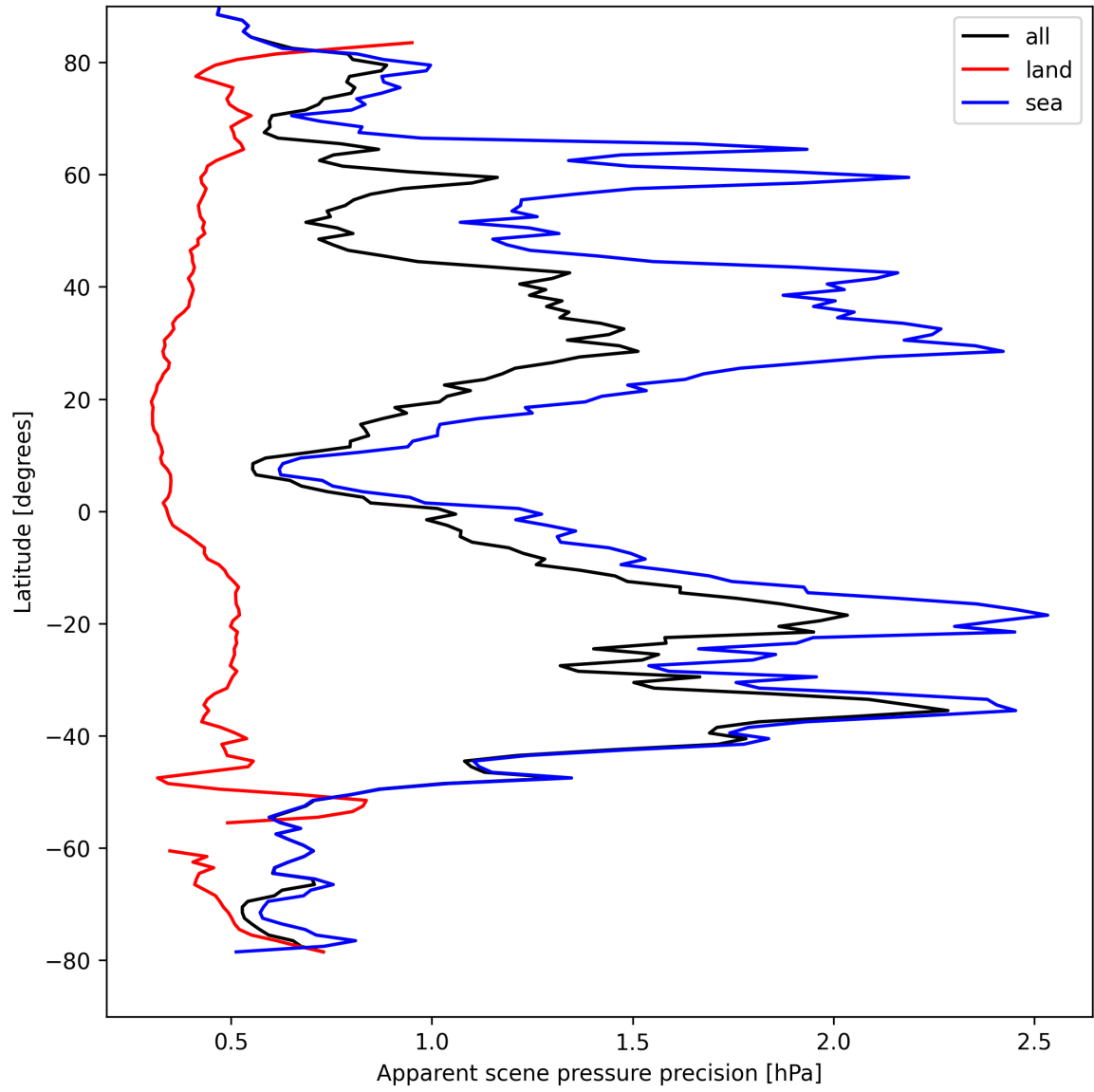
Figure 18: Zonal average of “Apparent scene pressure precision” for 2025-08-28 to 2025-08-28.
