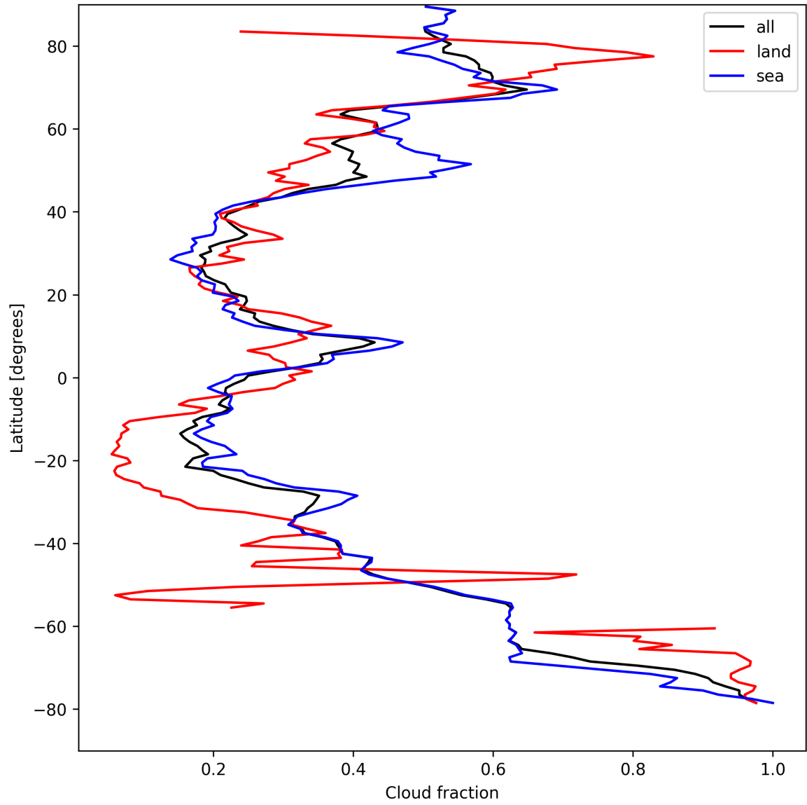
Figure 13: Zonal average of “Cloud fraction” for 2025-08-28 to 2025-08-28.
