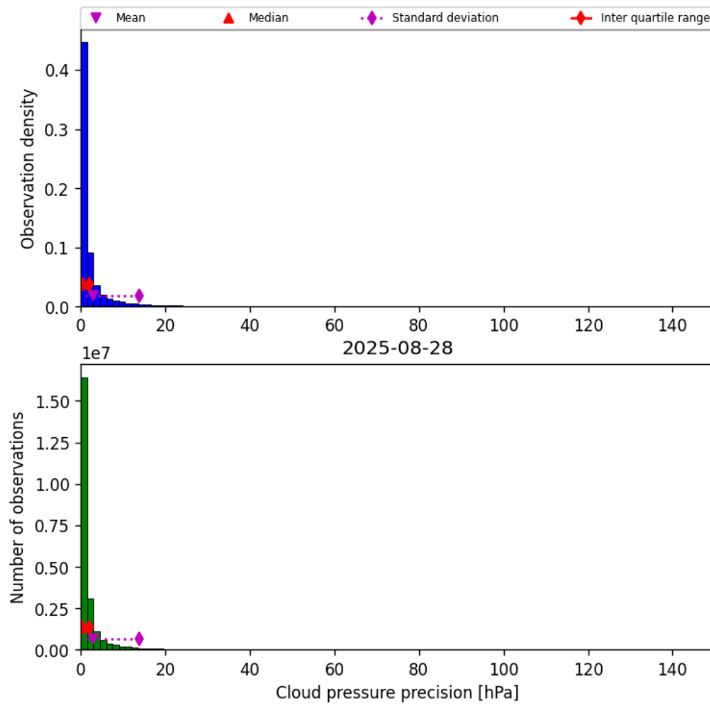
Figure 29: Histogram of “Cloud pressure precision” for 2025-08-28 to 2025-08-28
