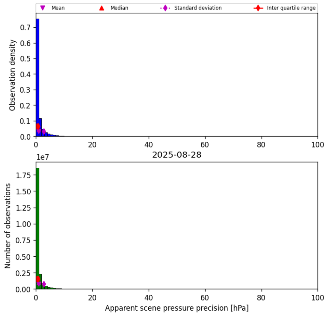
Figure 35: Histogram of “Apparent scene pressure precision” for 2025-08-28 to 2025-08-28
