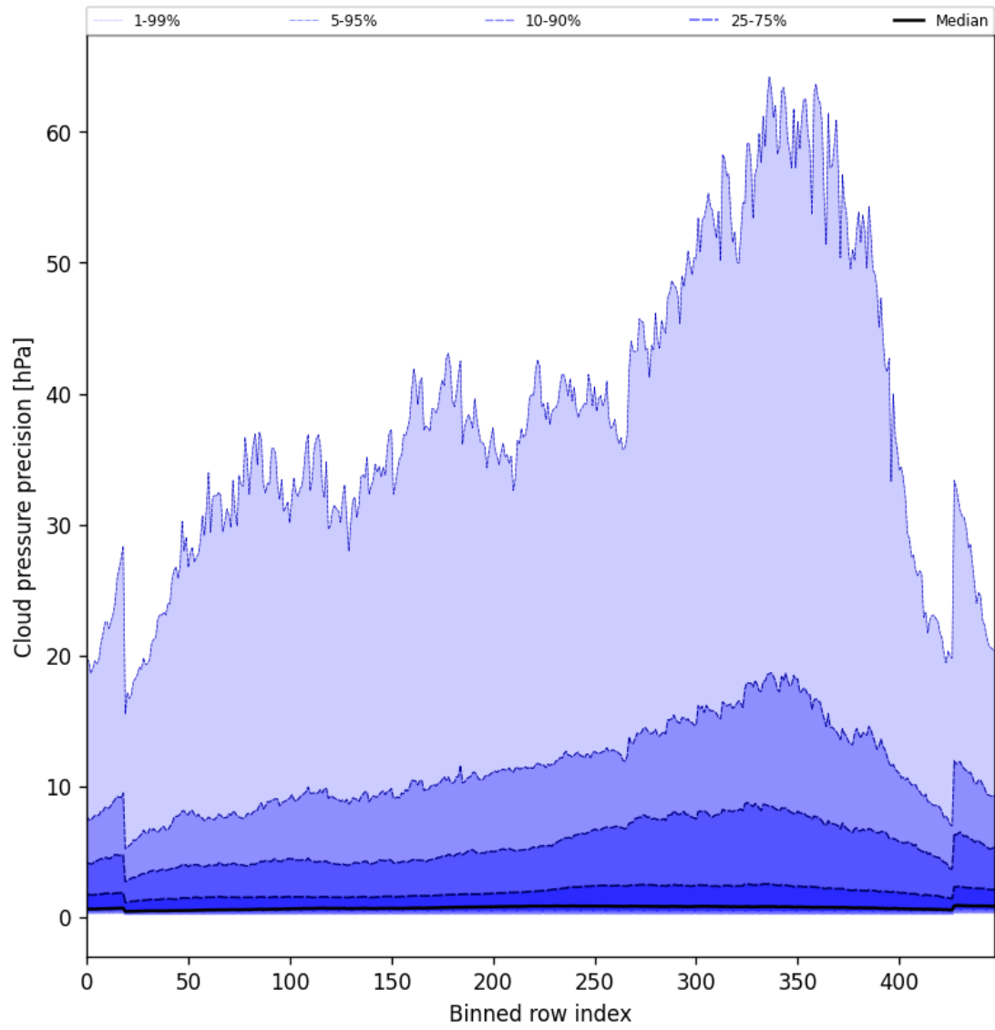
Figure 46: Along track statistics of “Cloud pressure precision” for 2025-08-28 to 2025-08-28
