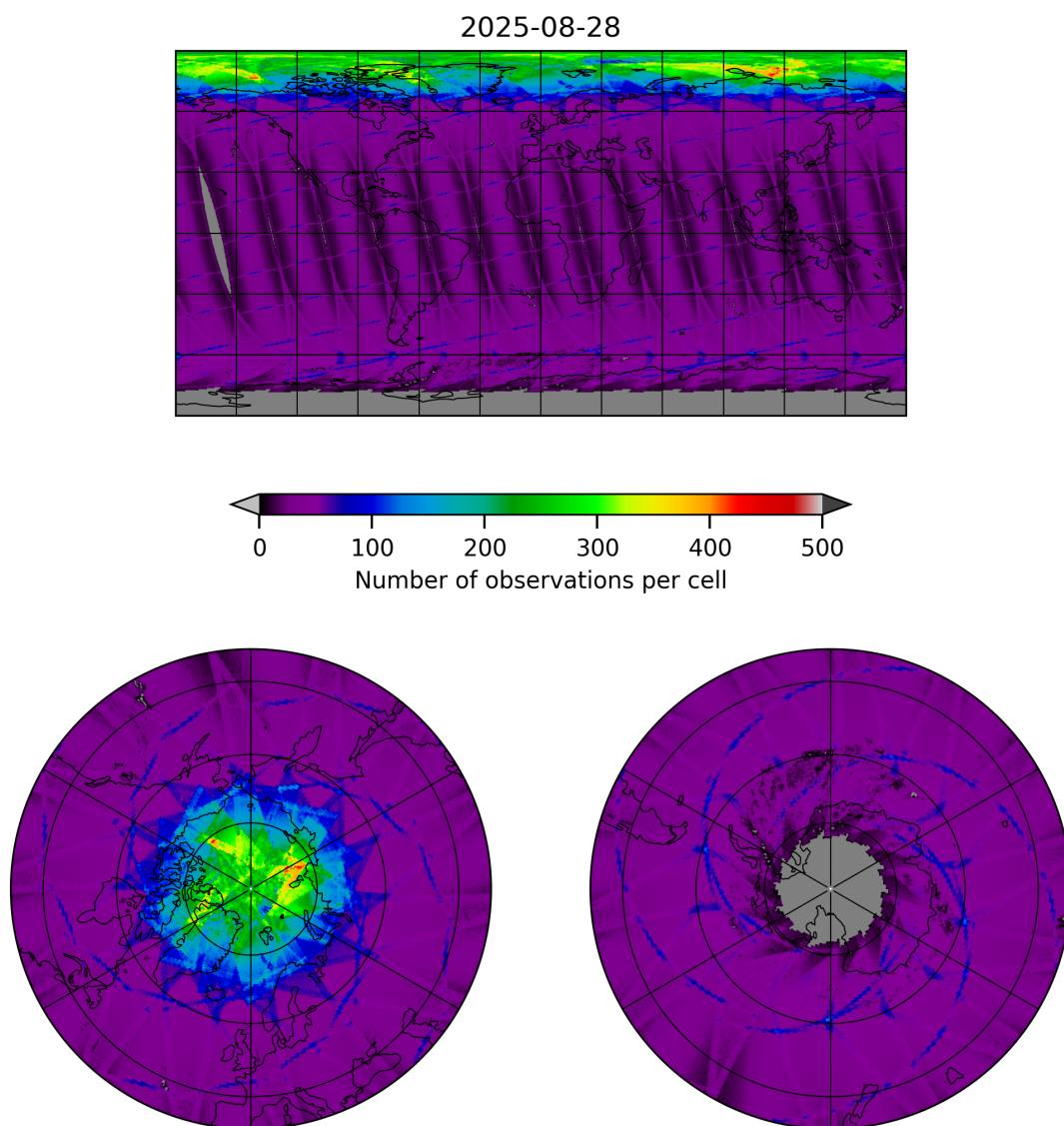
Figure 9: Map of the number of observations for 2025-08-28 to 2025-08-28
