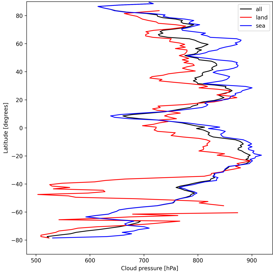
Figure 11: Zonal average of “Cloud pressure” for 2025-08-28 to 2025-08-28.
