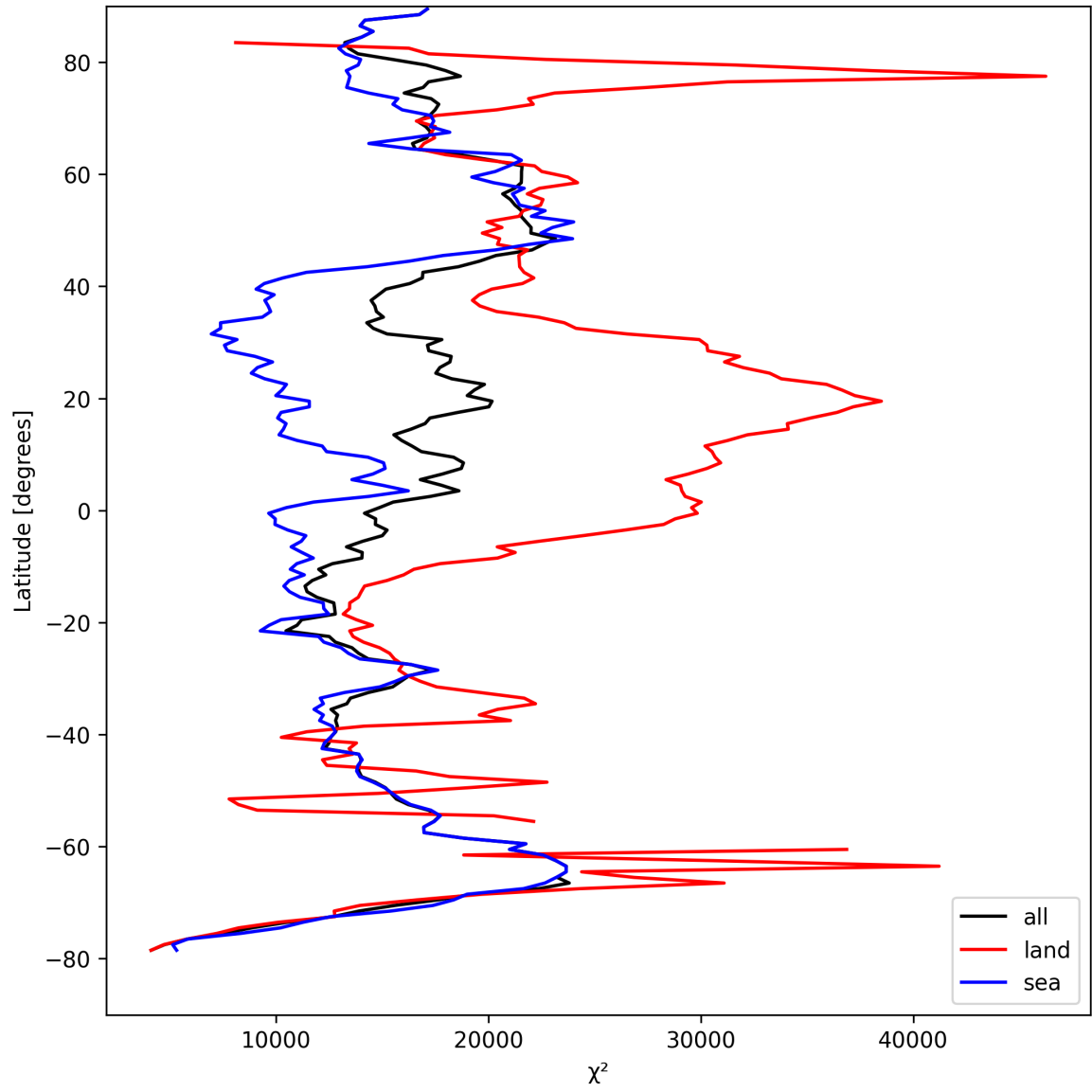
Figure 19: Zonal average of “ \chi^2 ” for 2025-08-28 to 2025-08-28.
