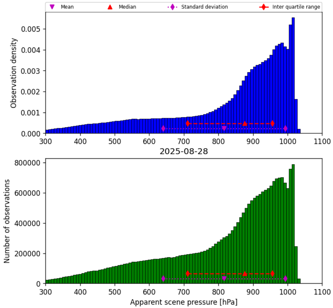
Figure 34: Histogram of “Apparent scene pressure” for 2025-08-28 to 2025-08-28
