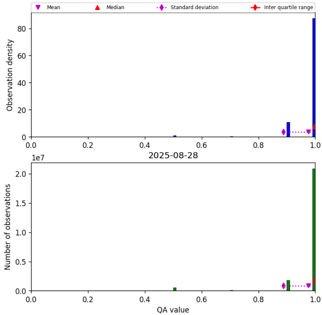
Figure 27: Histogram of “QA value” for 2025-08-28 to 2025-08-28
