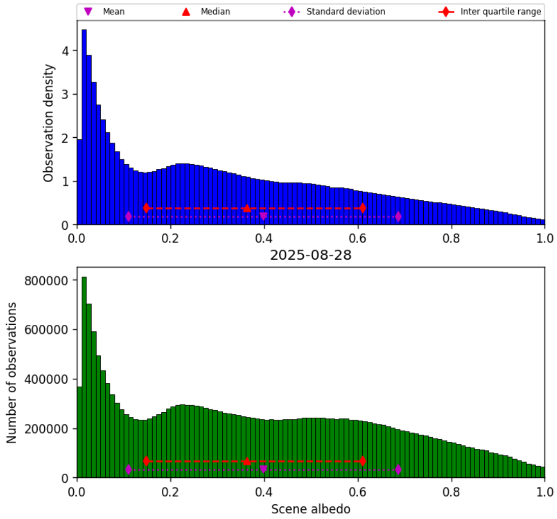
Figure 32: Histogram of “Scene albedo” for 2025-08-28 to 2025-08-28
