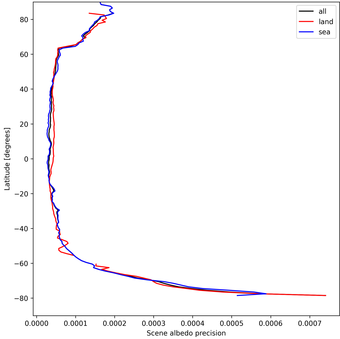
Figure 16: Zonal average of “Scene albedo precision” for 2025-08-28 to 2025-08-28.
