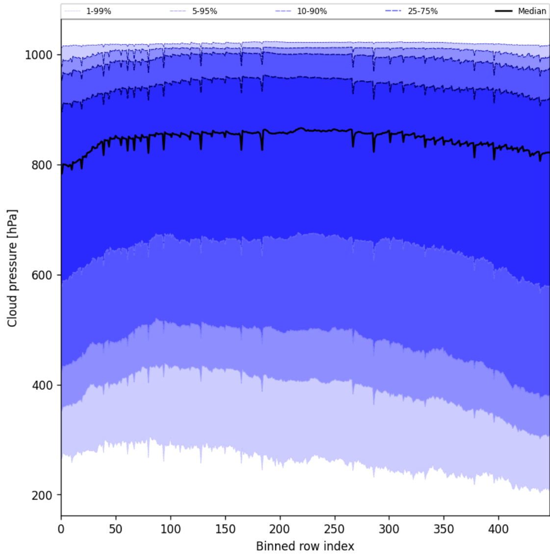
Figure 45: Along track statistics of “Cloud pressure” for 2025-08-28 to 2025-08-28
