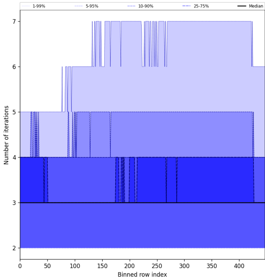
Figure 54: Along track statistics of “Number of iterations” for 2025-08-28 to 2025-08-28
