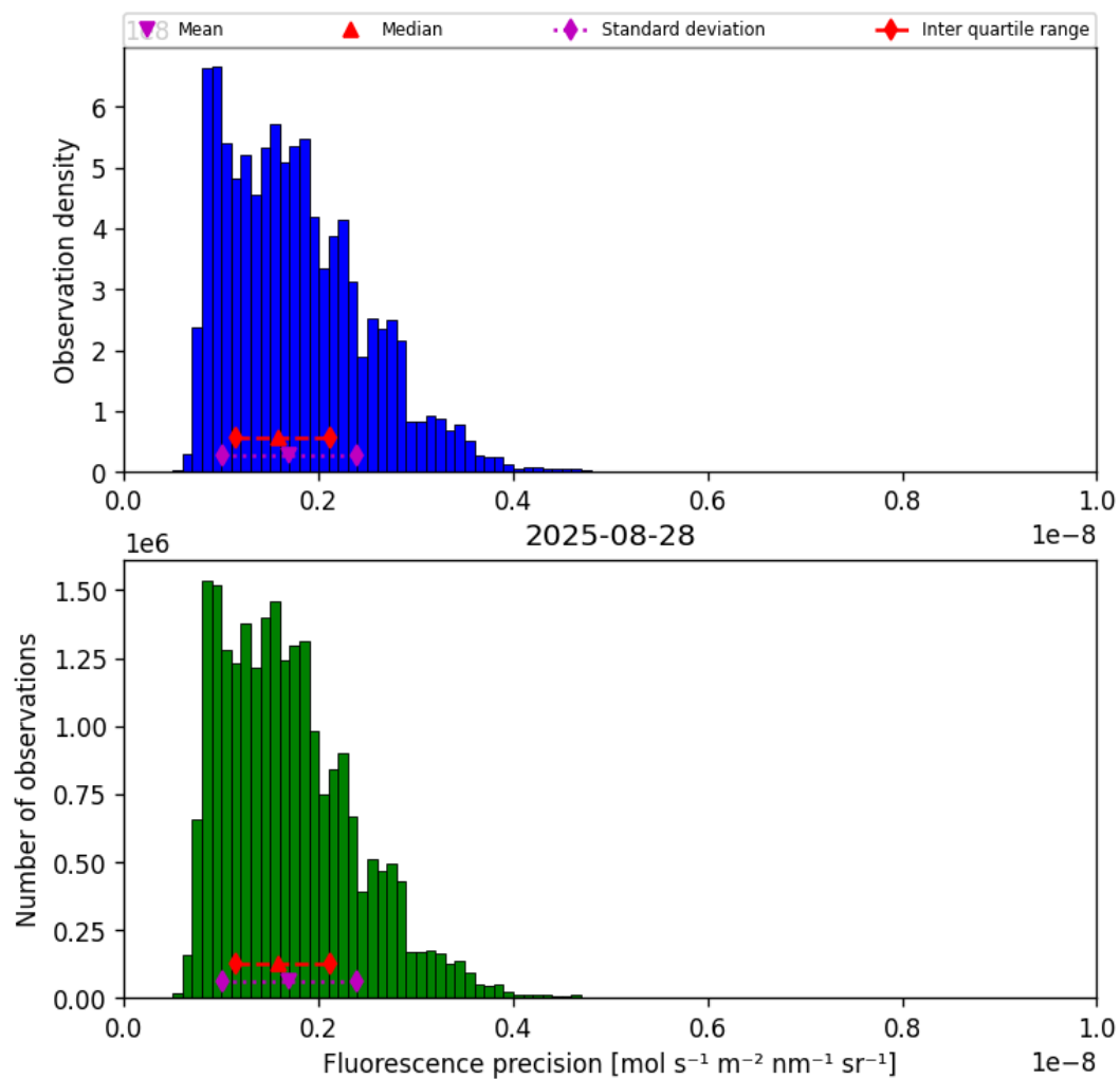
Figure 39: Histogram of “Fluorescence precision” for 2025-08-28 to 2025-08-28
