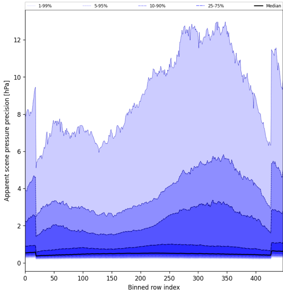
Figure 52: Along track statistics of “Apparent scene pressure precision” for 2025-08-28 to 2025-08-28
