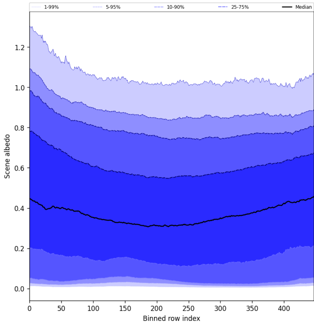
Figure 49: Along track statistics of “Scene albedo” for 2025-08-28 to 2025-08-28
