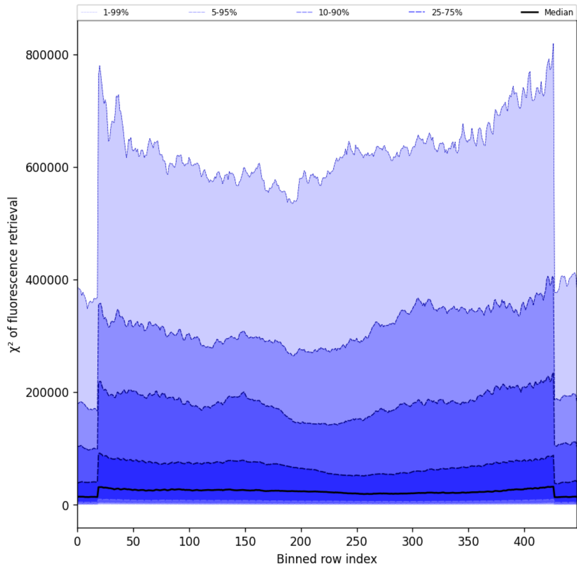
Figure 57: Along track statistics of “ \chi^2 of fluorescence retrieval” for 2025-08-28 to 2025-08-28
