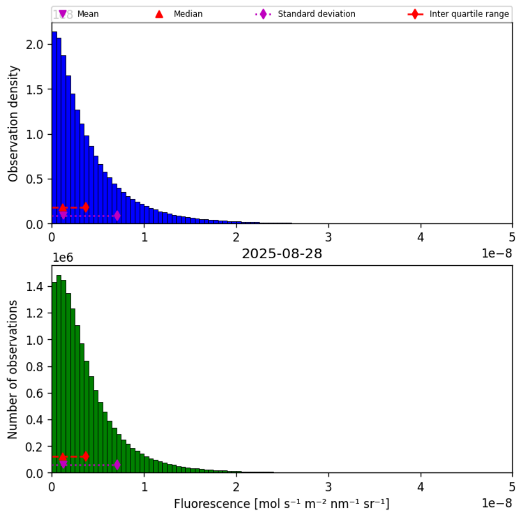
Figure 38: Histogram of “Fluorescence” for 2025-08-28 to 2025-08-28
