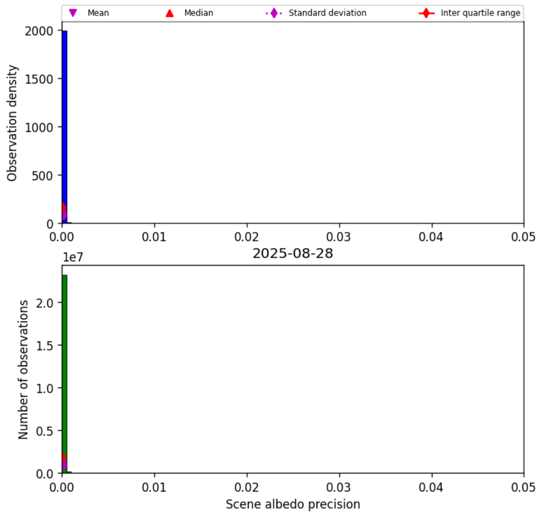
Figure 33: Histogram of “Scene albedo precision” for 2025-08-28 to 2025-08-28
