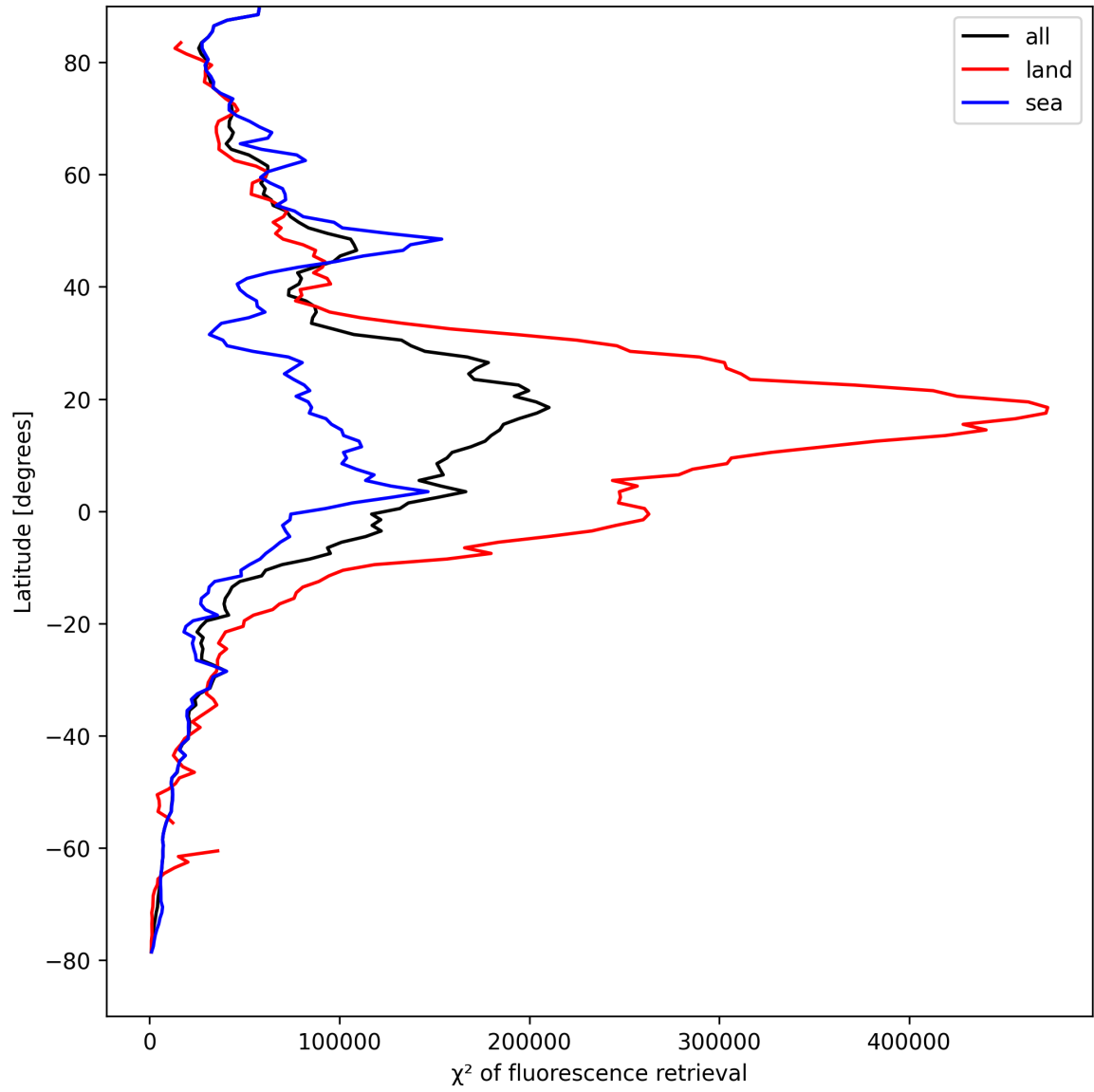
Figure 23: Zonal average of “ \chi^2 of fluorescence retrieval” for 2025-08-28 to 2025-08-28.
