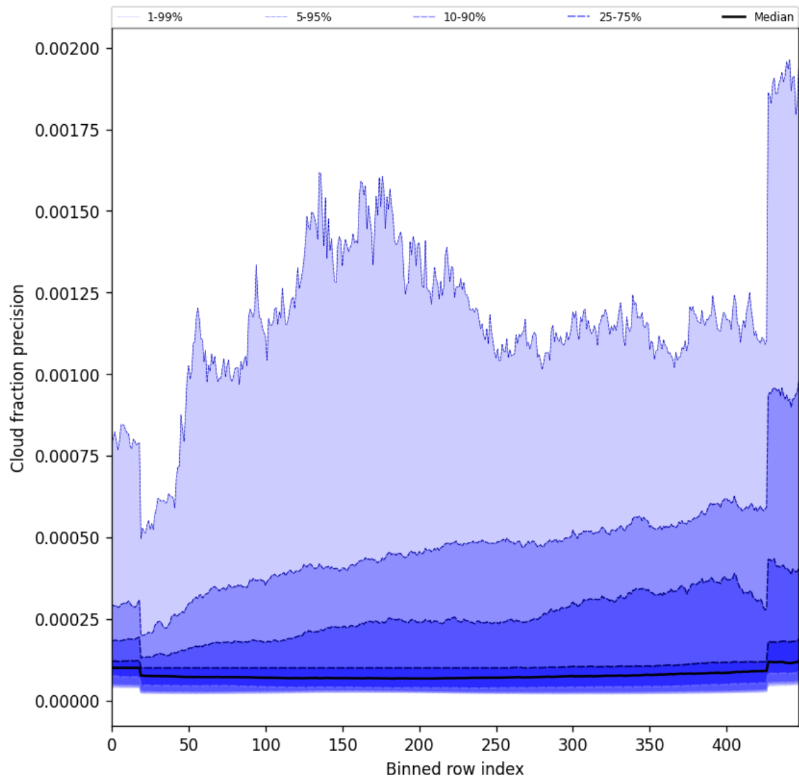
Figure 48: Along track statistics of “Cloud fraction precision” for 2025-08-28 to 2025-08-28
