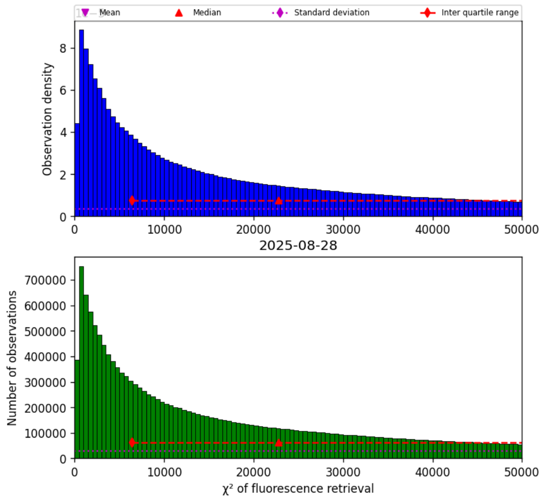
Figure 40: Histogram of “ \chi^2 of fluorescence retrieval” for 2025-08-28 to 2025-08-28
