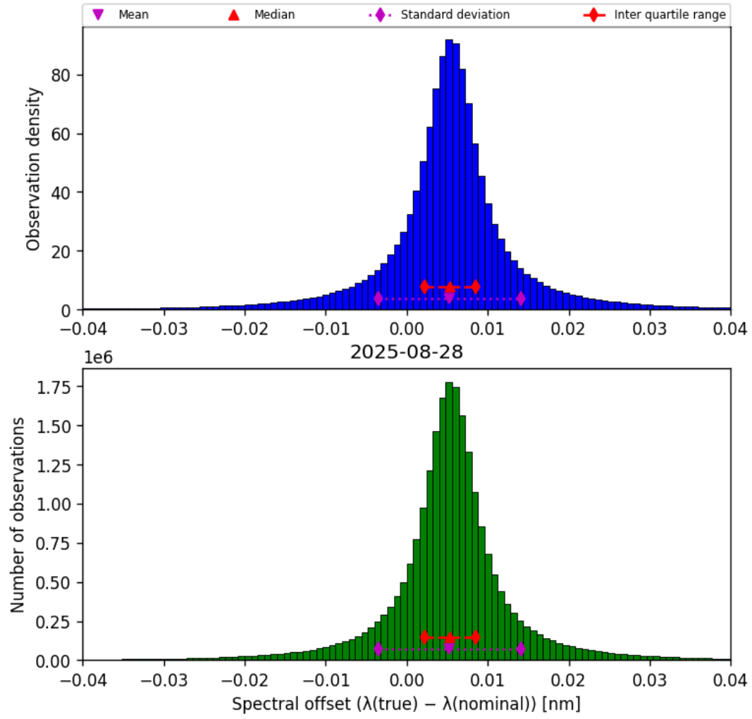
Figure 43: Histogram of “Spectral offset ( \lambda_{\text{true}} - \lambda_{\text{nominal}} )” for 2025-08-28 to 2025-08-28
