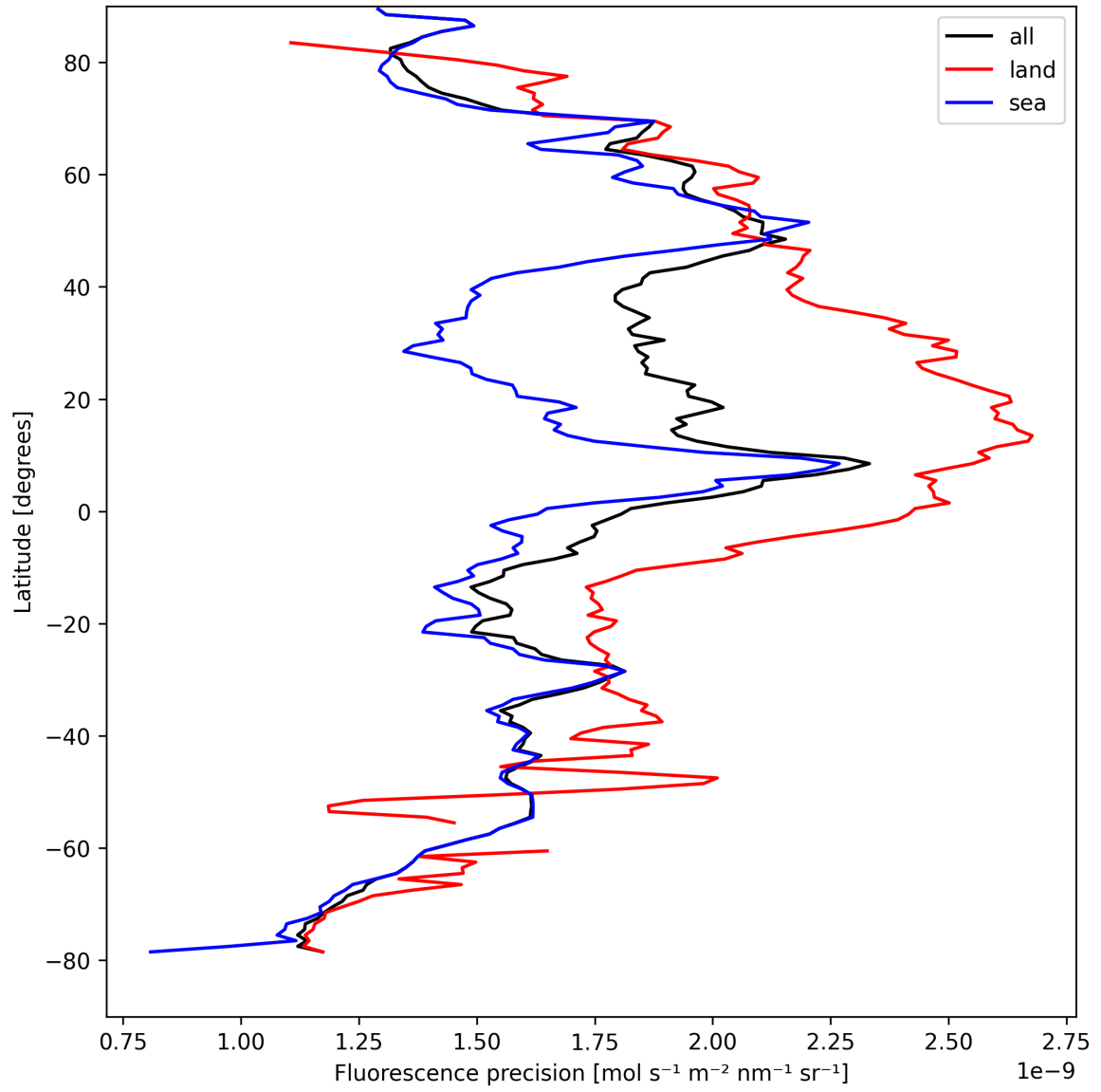
Figure 22: Zonal average of “Fluorescence precision” for 2025-08-28 to 2025-08-28.
