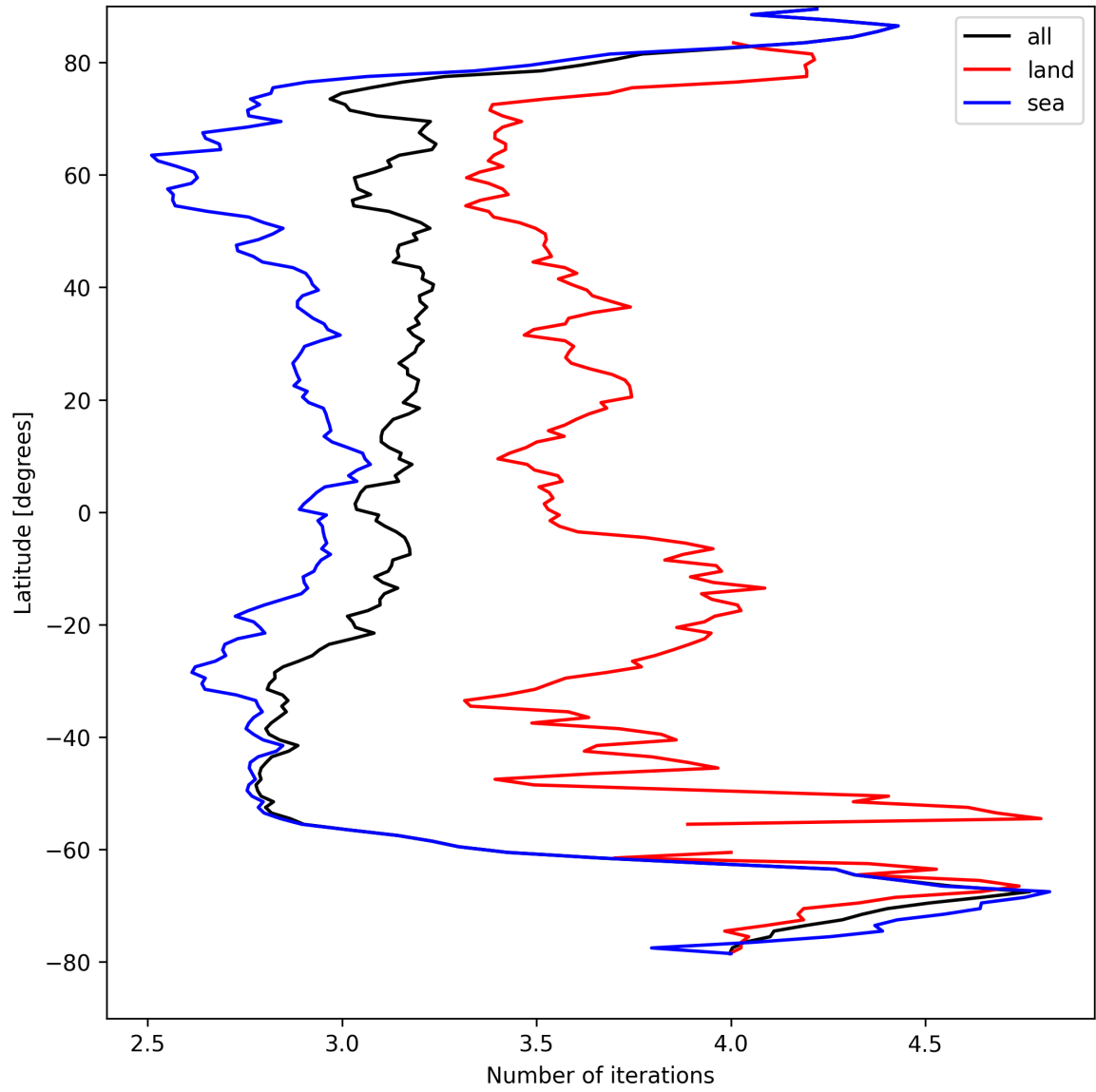
Figure 20: Zonal average of “Number of iterations” for 2025-08-28 to 2025-08-28.
