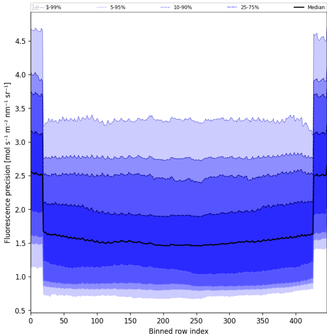
Figure 56: Along track statistics of “Fluorescence precision” for 2025-08-28 to 2025-08-28
