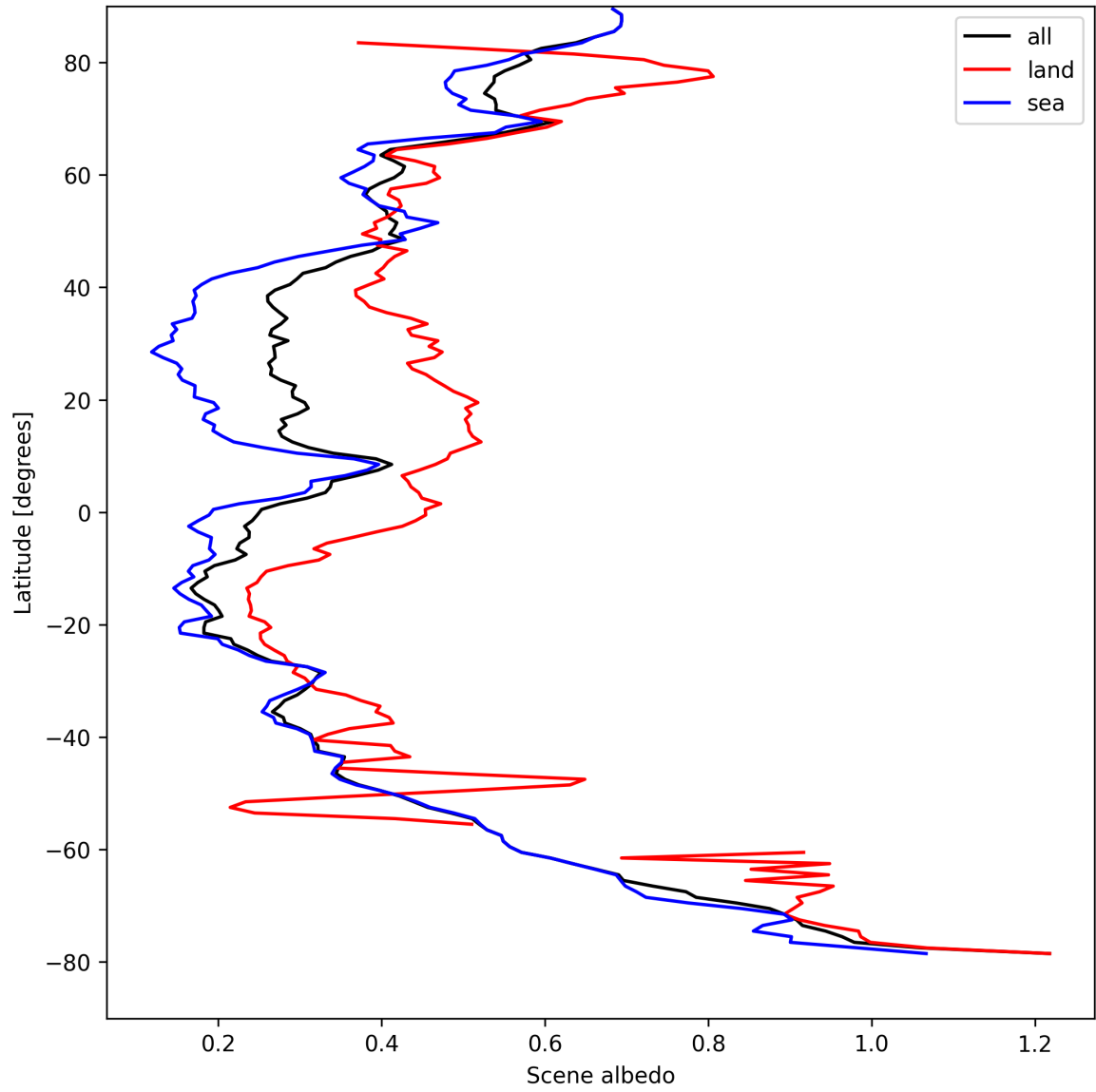
Figure 15: Zonal average of “Scene albedo” for 2025-08-28 to 2025-08-28.
