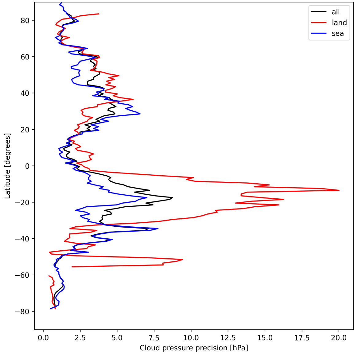
Figure 12: Zonal average of “Cloud pressure precision” for 2025-08-28 to 2025-08-28.
