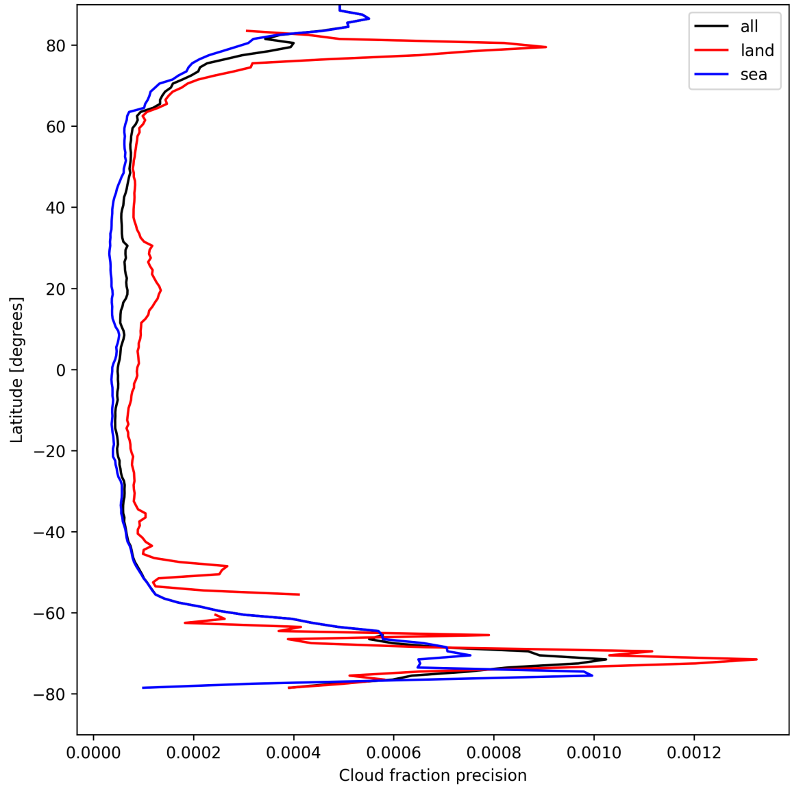
Figure 14: Zonal average of “Cloud fraction precision” for 2025-08-28 to 2025-08-28.
