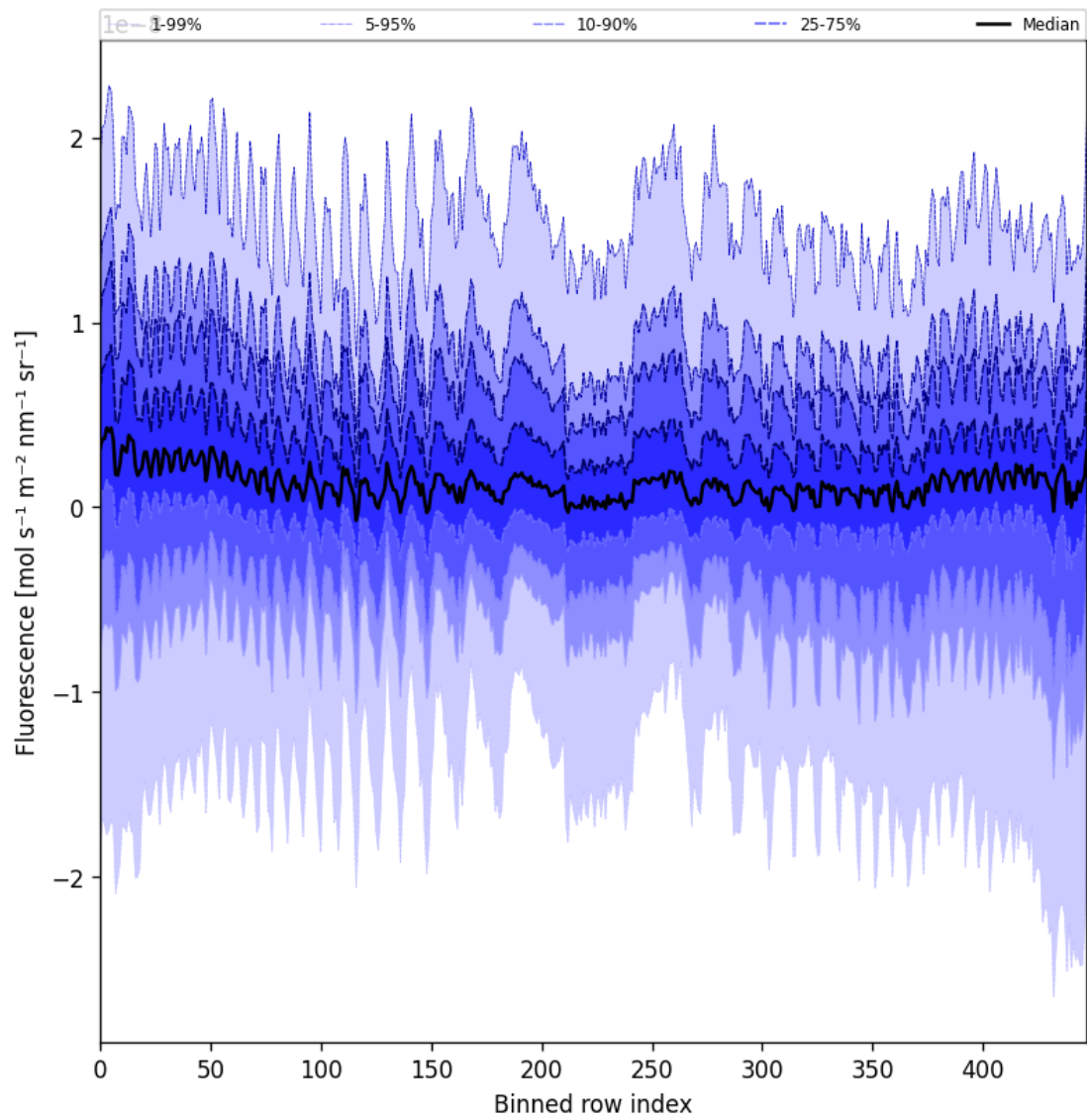
Figure 55: Along track statistics of “Fluorescence” for 2025-08-28 to 2025-08-28
