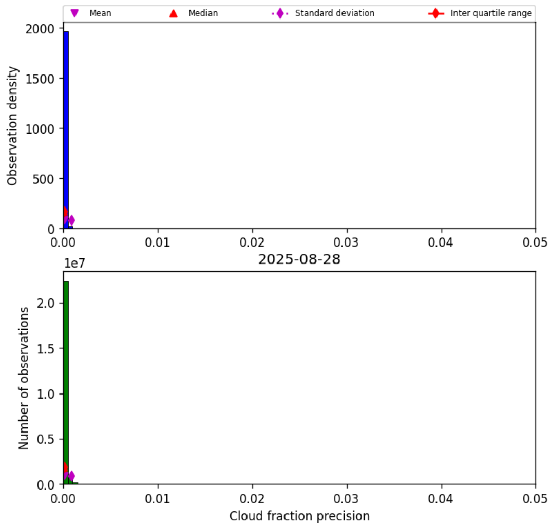
Figure 31: Histogram of “Cloud fraction precision” for 2025-08-28 to 2025-08-28
