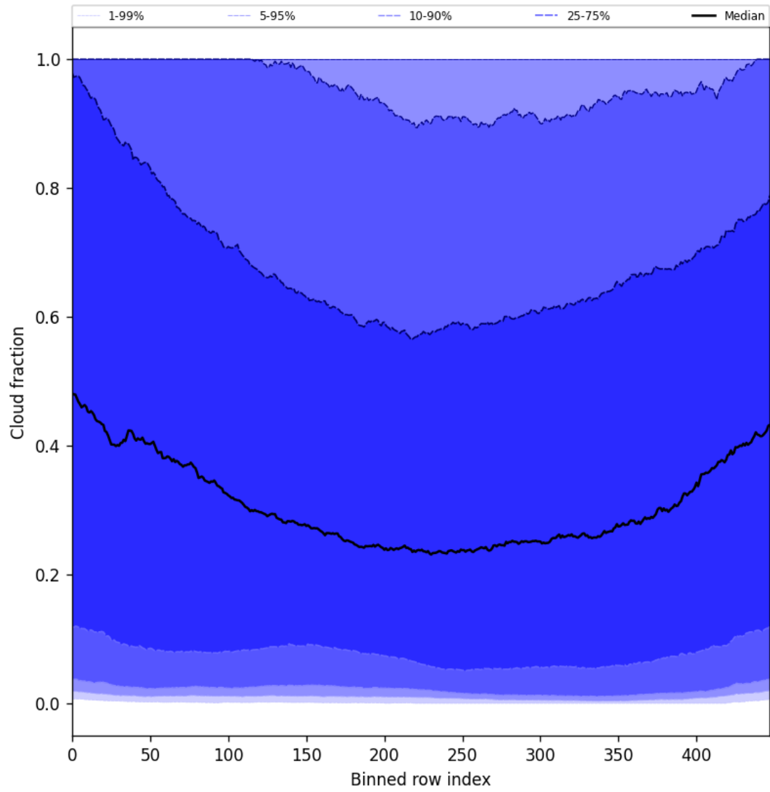
Figure 47: Along track statistics of “Cloud fraction” for 2025-08-28 to 2025-08-28
