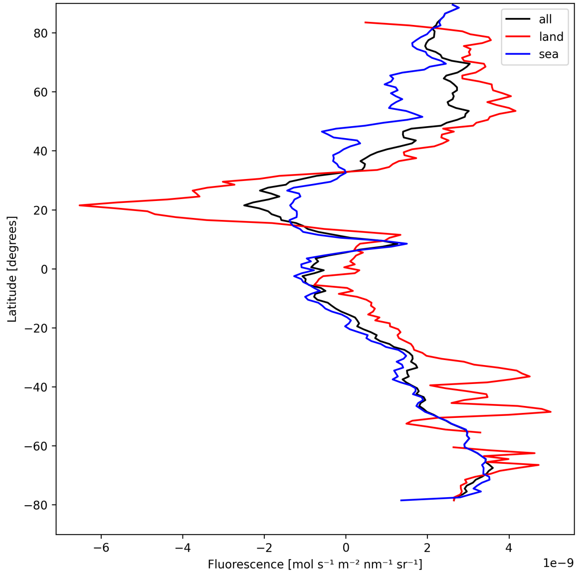
Figure 21: Zonal average of “Fluorescence” for 2025-08-28 to 2025-08-28.
