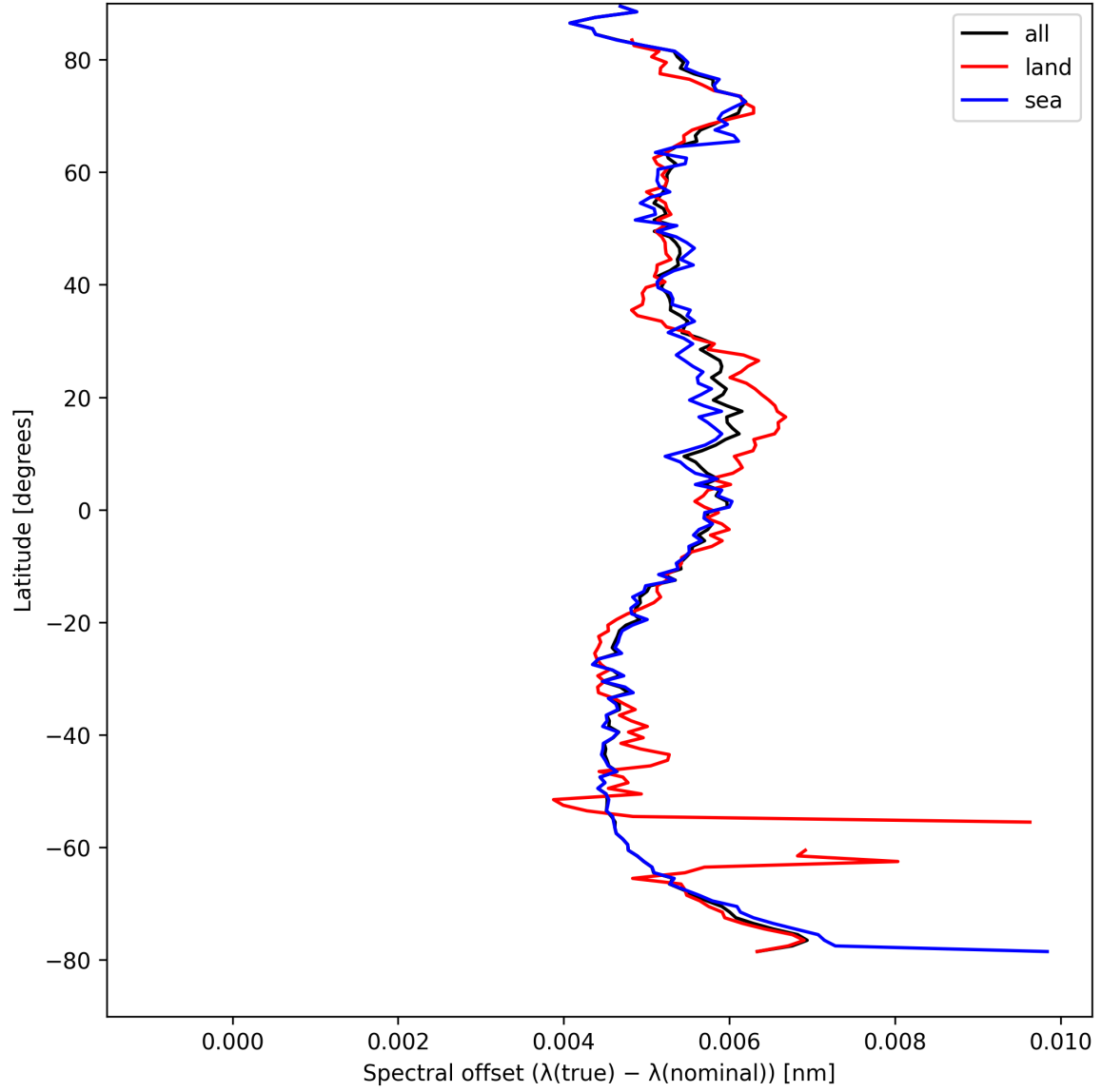
Figure 26: Zonal average of “Spectral offset ( \lambda_{\text{true}} - \lambda_{\text{nominal}} )” for 2025-08-28 to 2025-08-28.
