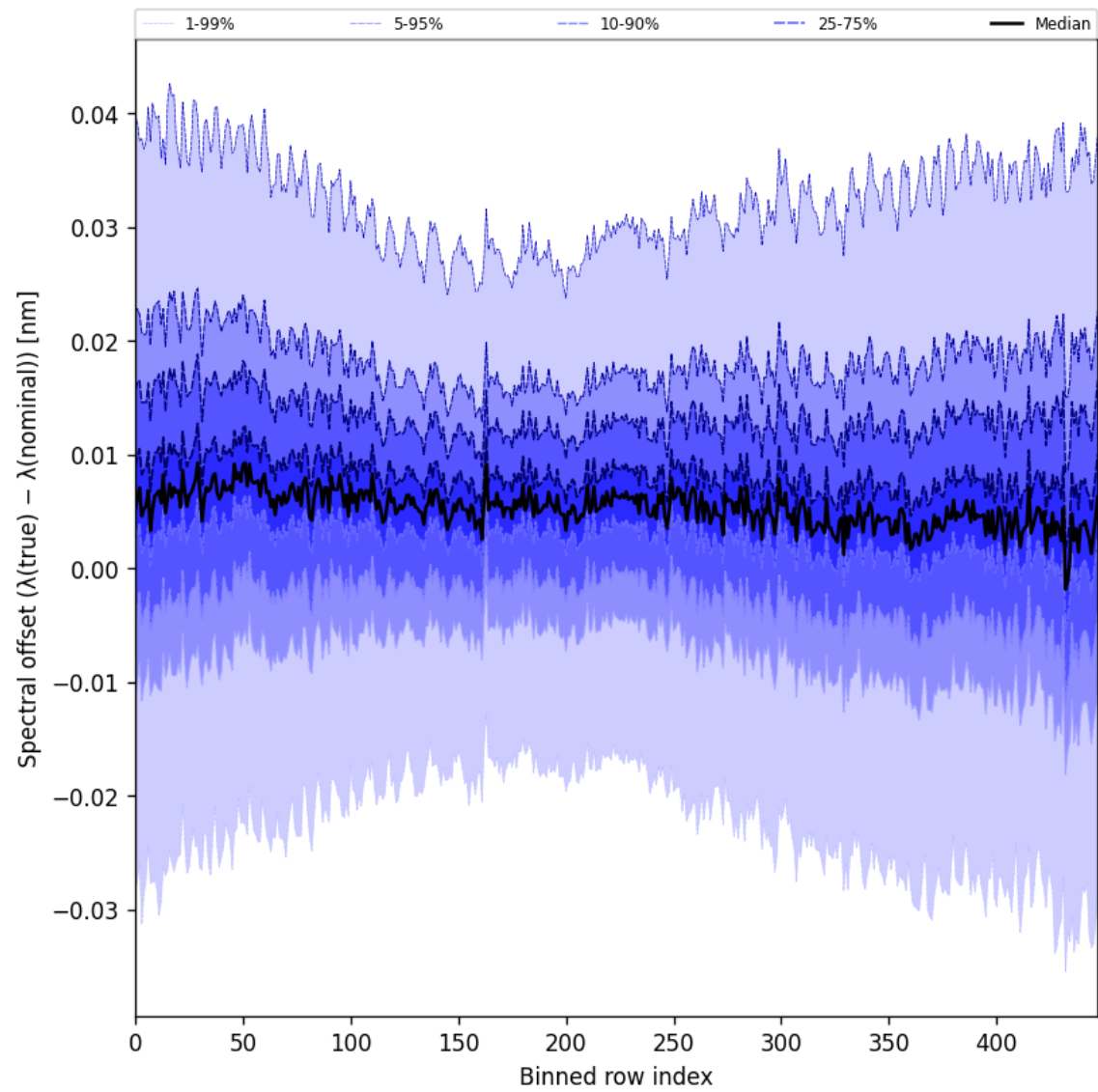
Figure 60: Along track statistics of “Spectral offset ( \lambda_{\text{true}} - \lambda_{\text{nominal}} )” for 2025-08-28 to 2025-08-28
