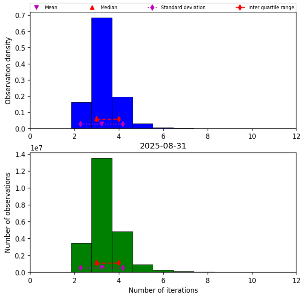
Figure 37: Histogram of “Number of iterations” for 2025-08-31 to 2025-09-01
