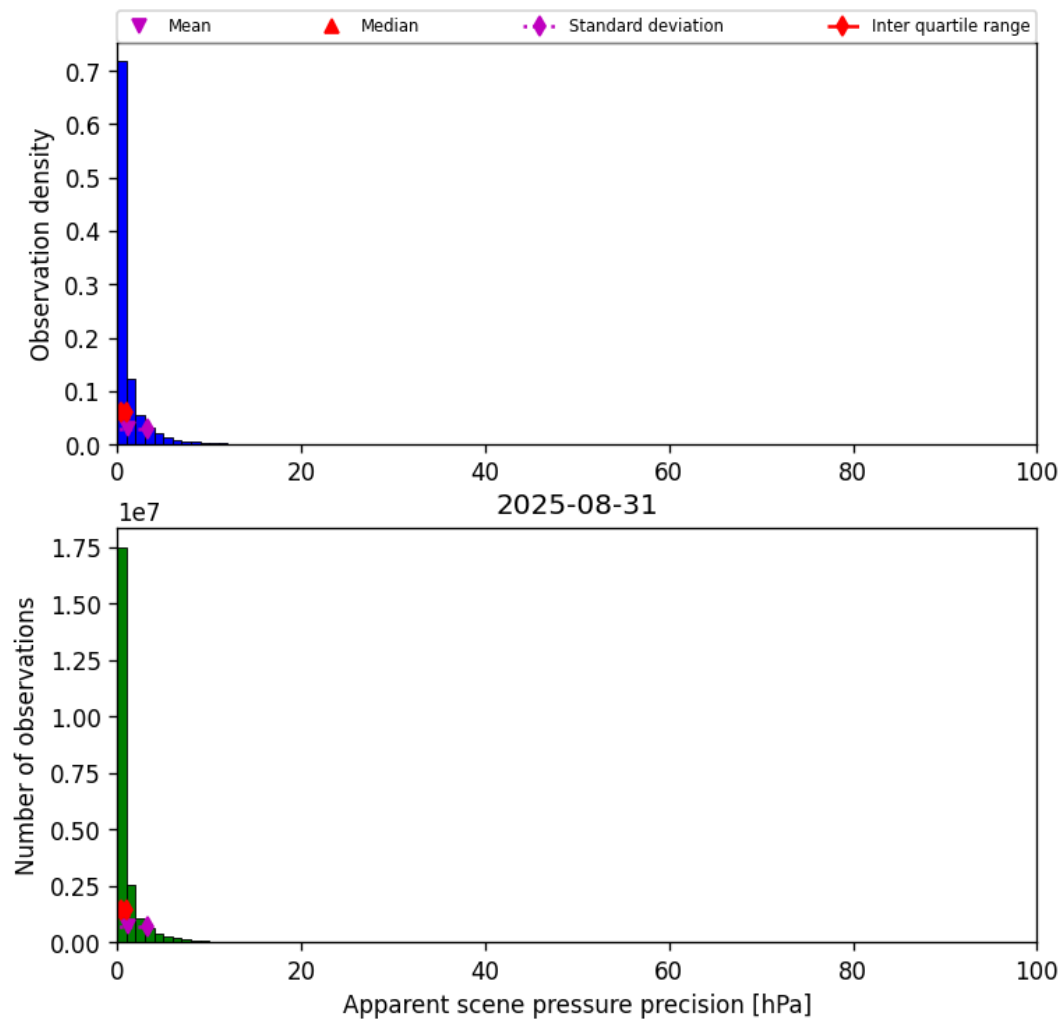
Figure 35: Histogram of “Apparent scene pressure precision” for 2025-08-31 to 2025-09-01
