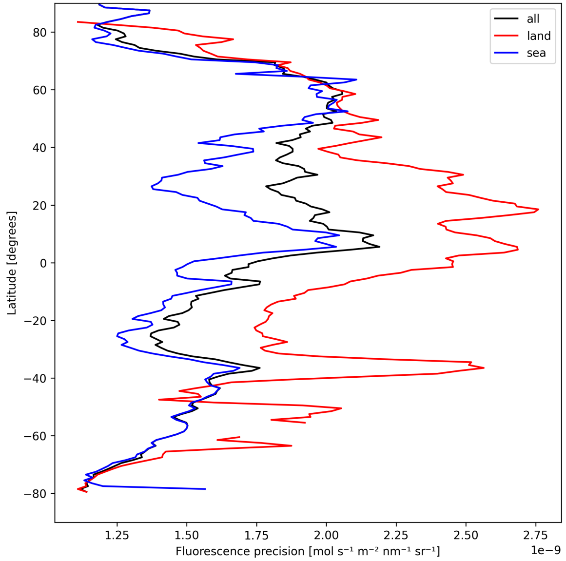
Figure 22: Zonal average of “Fluorescence precision” for 2025-08-31 to 2025-09-01.
