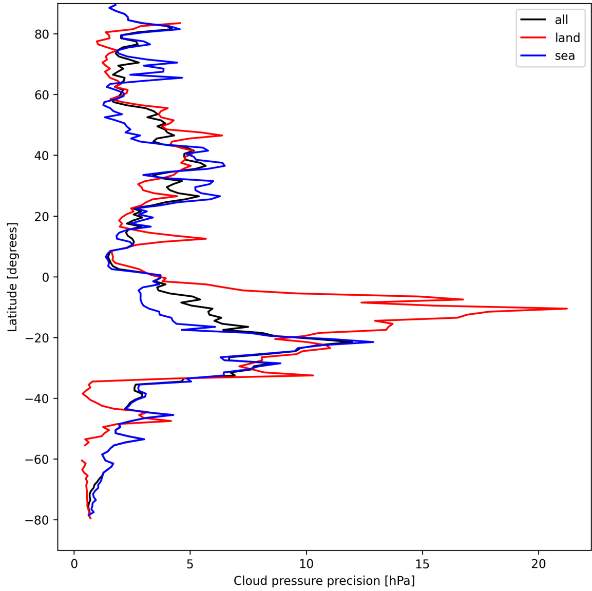
Figure 12: Zonal average of “Cloud pressure precision” for 2025-08-31 to 2025-09-01.
