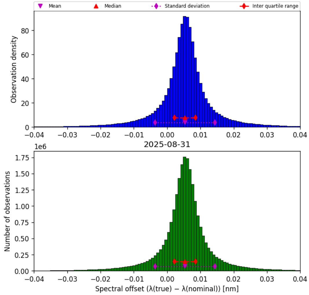
Figure 43: Histogram of “Spectral offset ( \lambda_{\text{true}} - \lambda_{\text{nominal}} )” for 2025-08-31 to 2025-09-01
