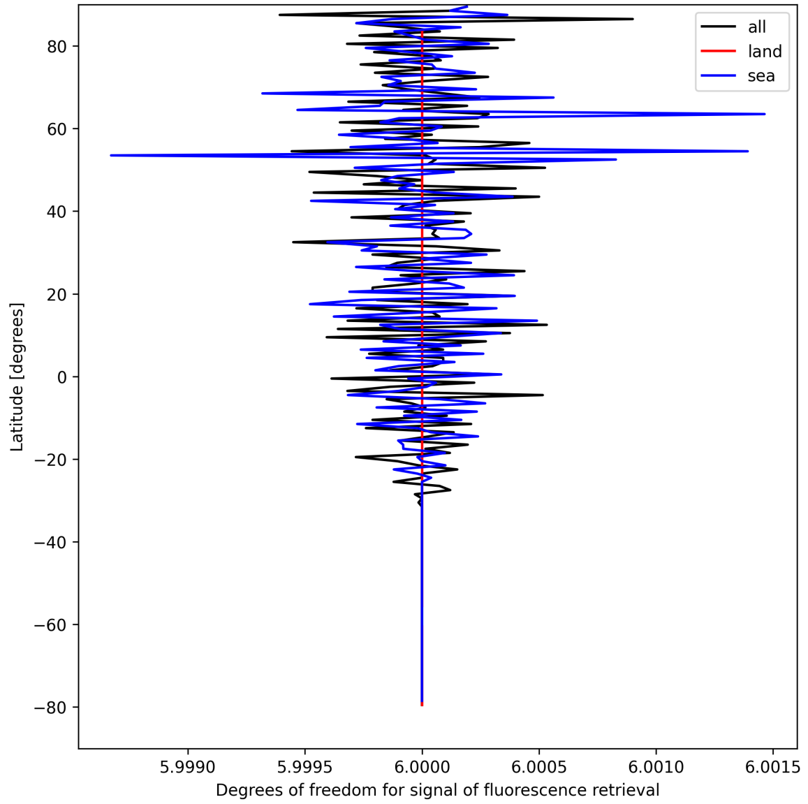
Figure 24: Zonal average of “Degrees of freedom for signal of fluorescence retrieval” for 2025-08-31 to 2025-09-01.
