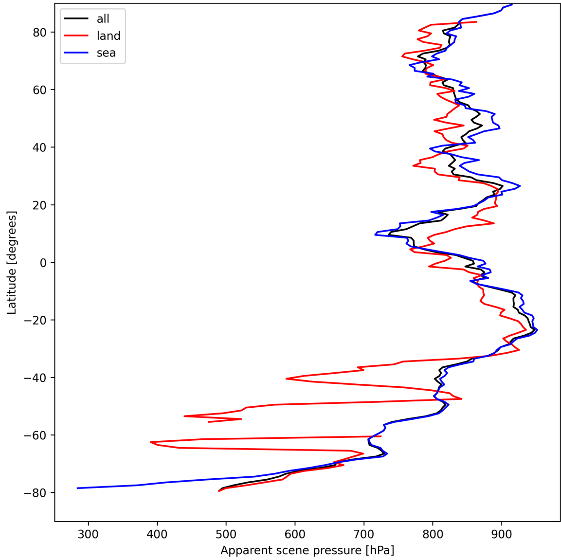
Figure 17: Zonal average of “Apparent scene pressure” for 2025-08-31 to 2025-09-01.
