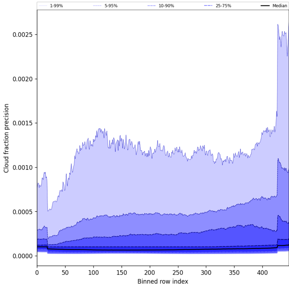
Figure 48: Along track statistics of “Cloud fraction precision” for 2025-08-31 to 2025-09-01
