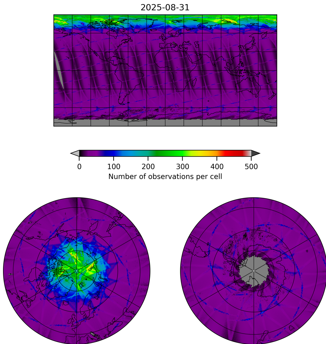
Figure 9: Map of the number of observations for 2025-08-31 to 2025-09-01
