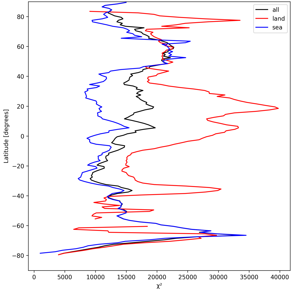
Figure 19: Zonal average of “ \chi^2 ” for 2025-08-31 to 2025-09-01.
