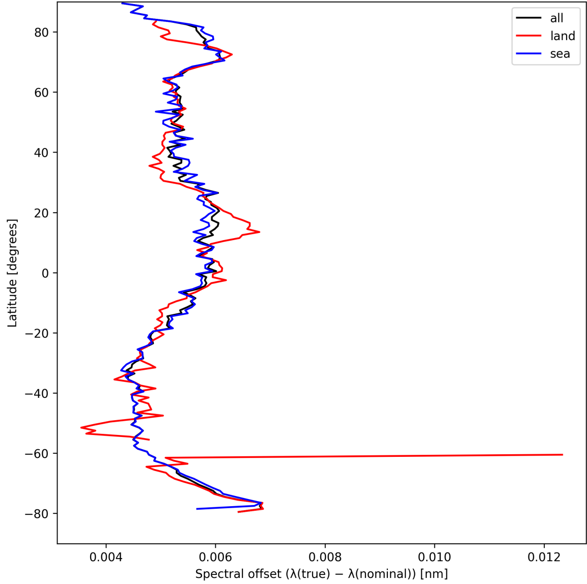
Figure 26: Zonal average of “Spectral offset ( \lambda_{\text{true}} - \lambda_{\text{nominal}} )” for 2025-08-31 to 2025-09-01.
