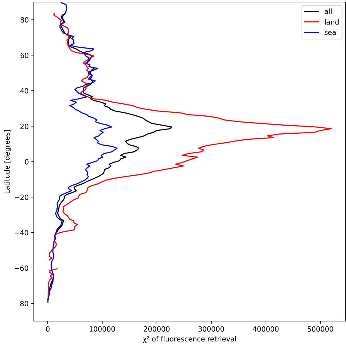
Figure 23: Zonal average of “ \chi^2 of fluorescence retrieval” for 2025-08-31 to 2025-09-01.
