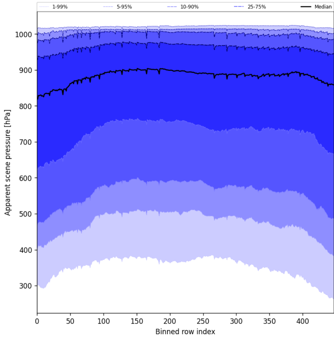
Figure 51: Along track statistics of “Apparent scene pressure” for 2025-08-31 to 2025-09-01
