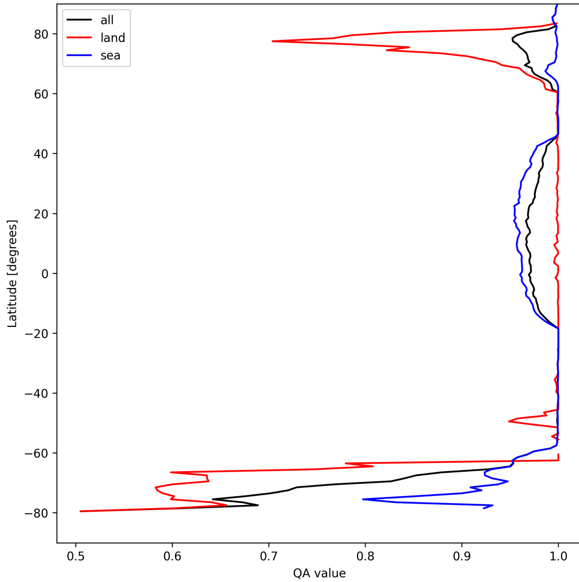
Figure 10: Zonal average of “QA value” for 2025-08-31 to 2025-09-01.
