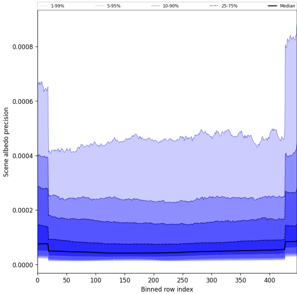
Figure 50: Along track statistics of “Scene albedo precision” for 2025-08-31 to 2025-09-01
