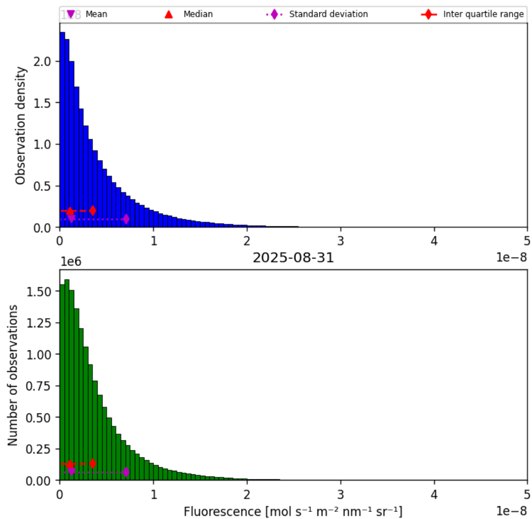
Figure 38: Histogram of “Fluorescence” for 2025-08-31 to 2025-09-01
