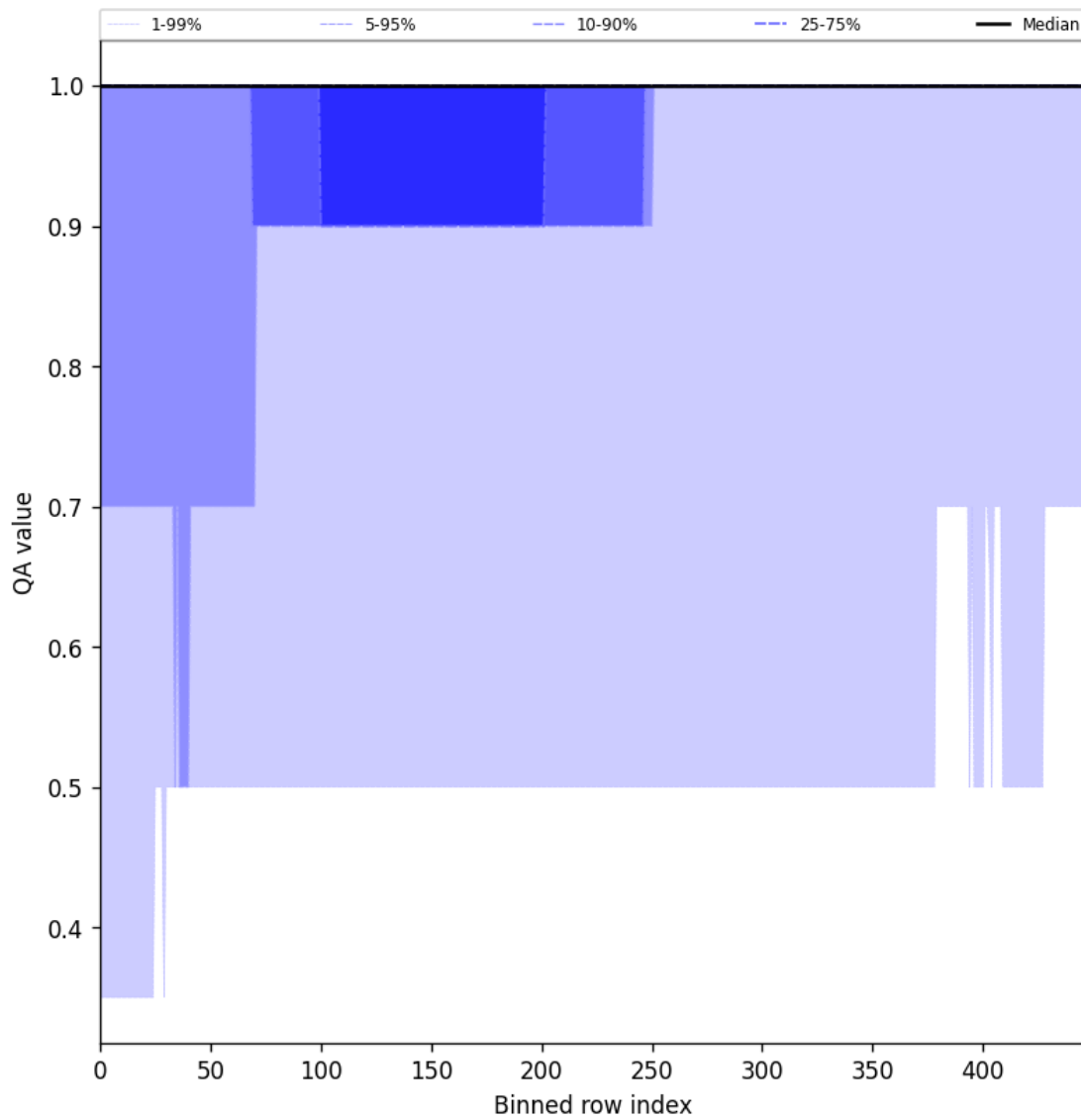
Figure 44: Along track statistics of “QA value” for 2025-08-31 to 2025-09-01
