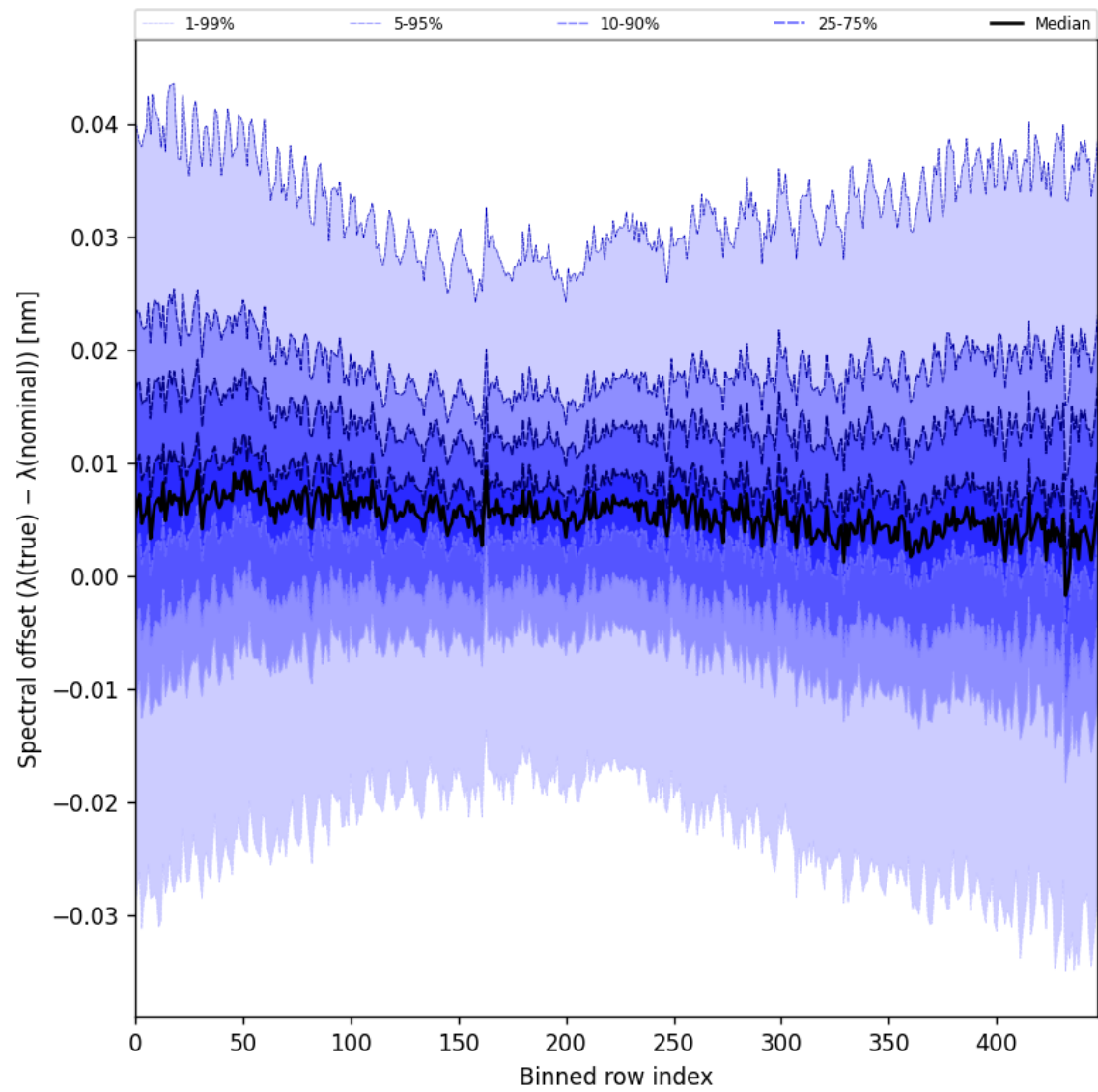
Figure 60: Along track statistics of “Spectral offset ( \lambda_{\text{true}} - \lambda_{\text{nominal}} )” for 2025-08-31 to 2025-09-01
