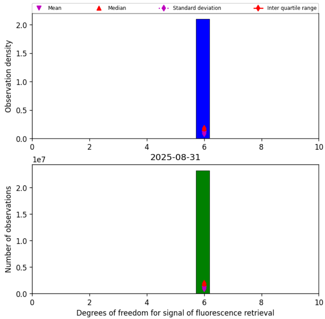
Figure 41: Histogram of “Degrees of freedom for signal of fluorescence retrieval” for 2025-08-31 to 2025-09-01
