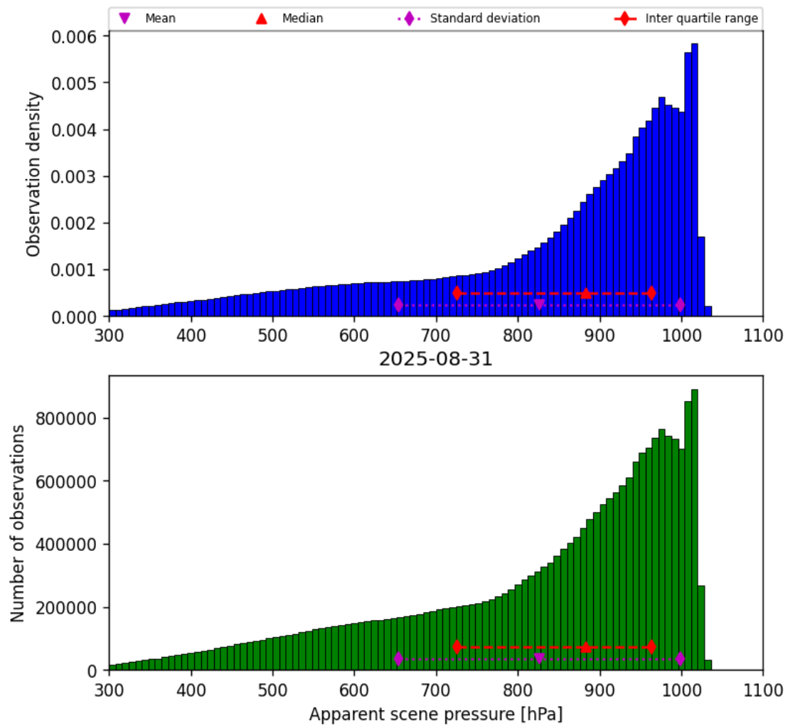
Figure 34: Histogram of “Apparent scene pressure” for 2025-08-31 to 2025-09-01
