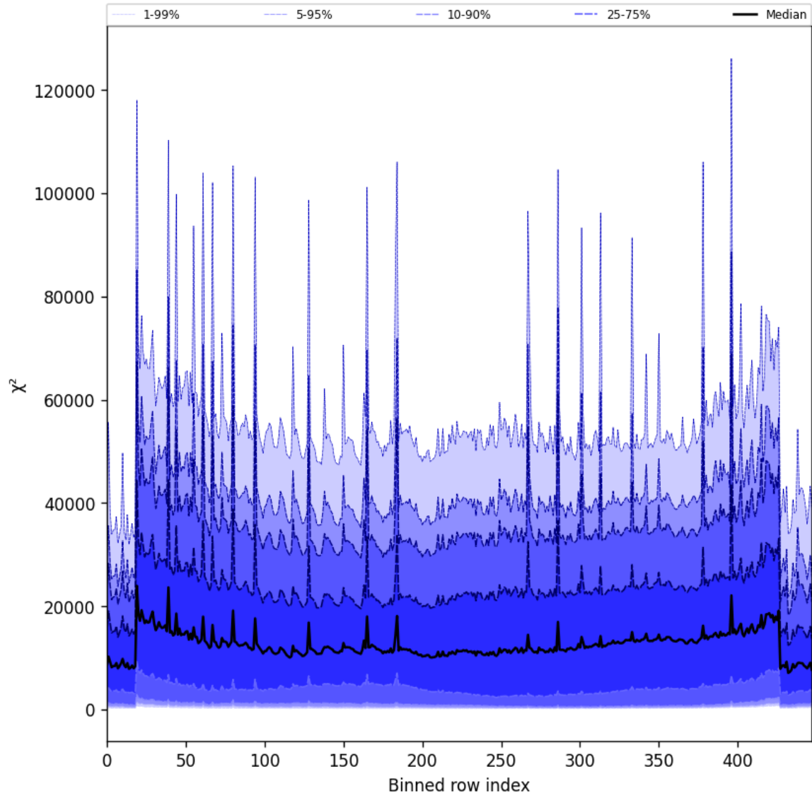
Figure 53: Along track statistics of “ \chi^2 ” for 2025-08-31 to 2025-09-01
