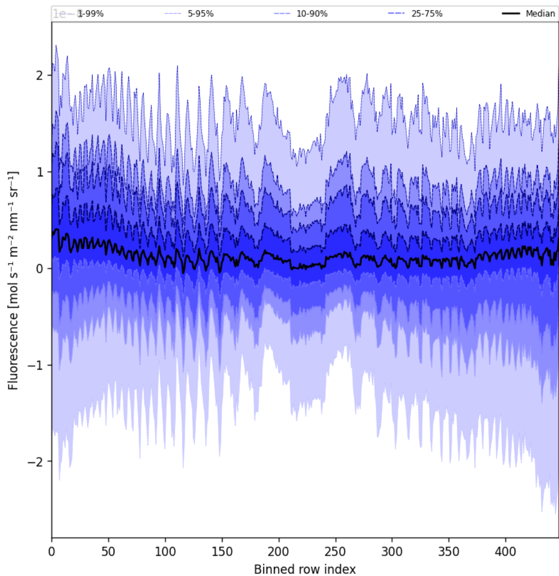
Figure 55: Along track statistics of “Fluorescence” for 2025-08-31 to 2025-09-01
