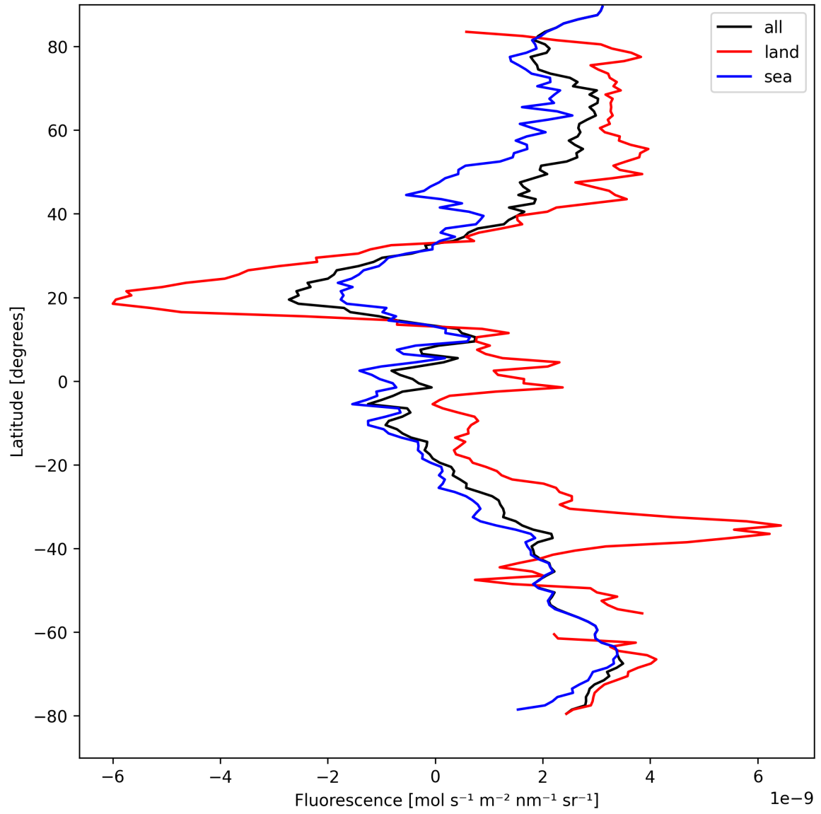
Figure 21: Zonal average of “Fluorescence” for 2025-08-31 to 2025-09-01.
