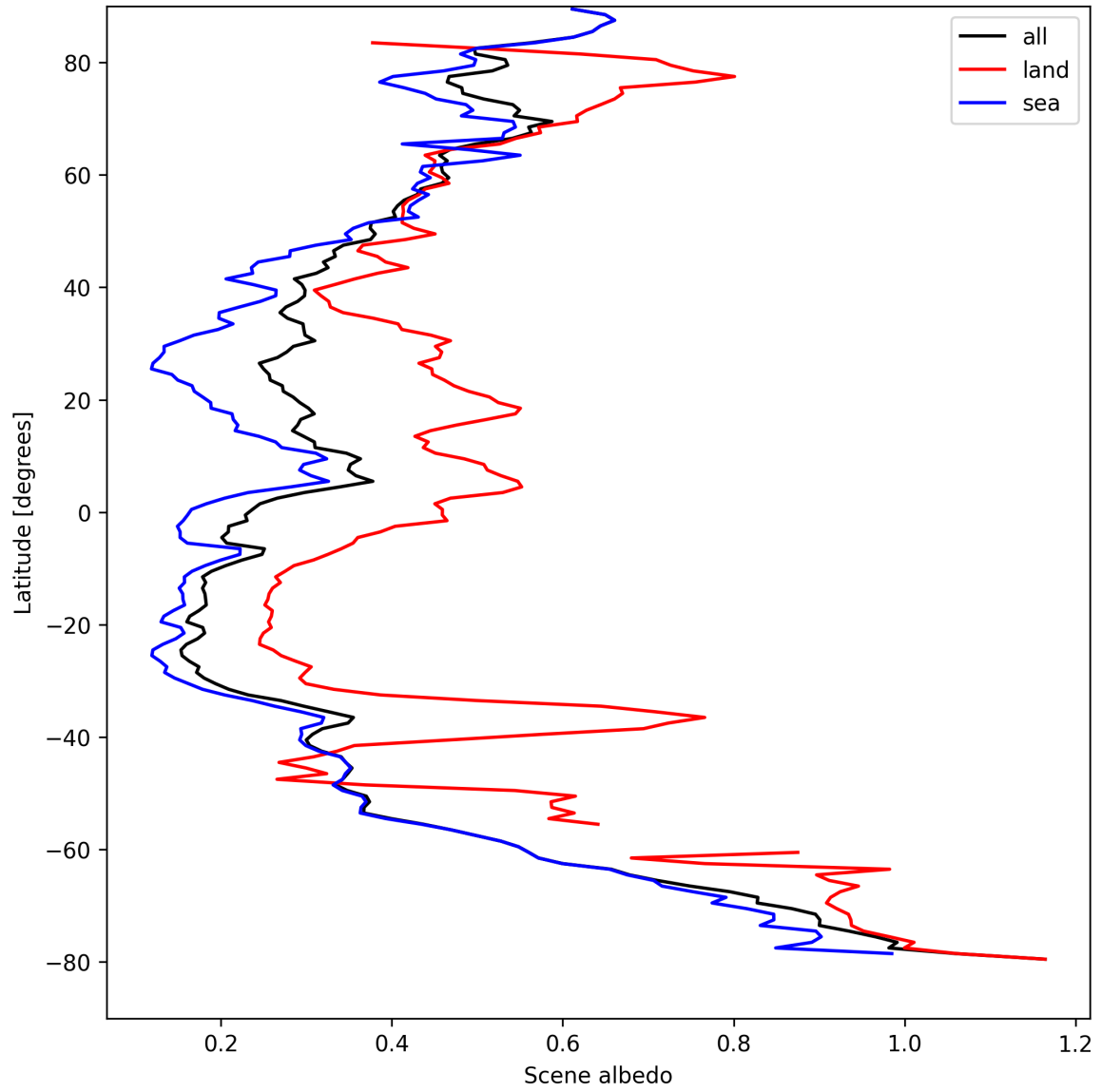
Figure 15: Zonal average of “Scene albedo” for 2025-08-31 to 2025-09-01.
