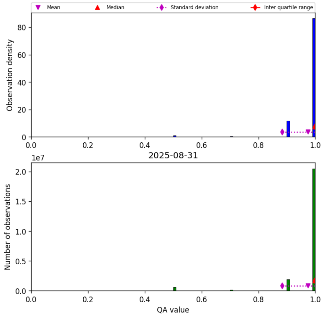
Figure 27: Histogram of “QA value” for 2025-08-31 to 2025-09-01
