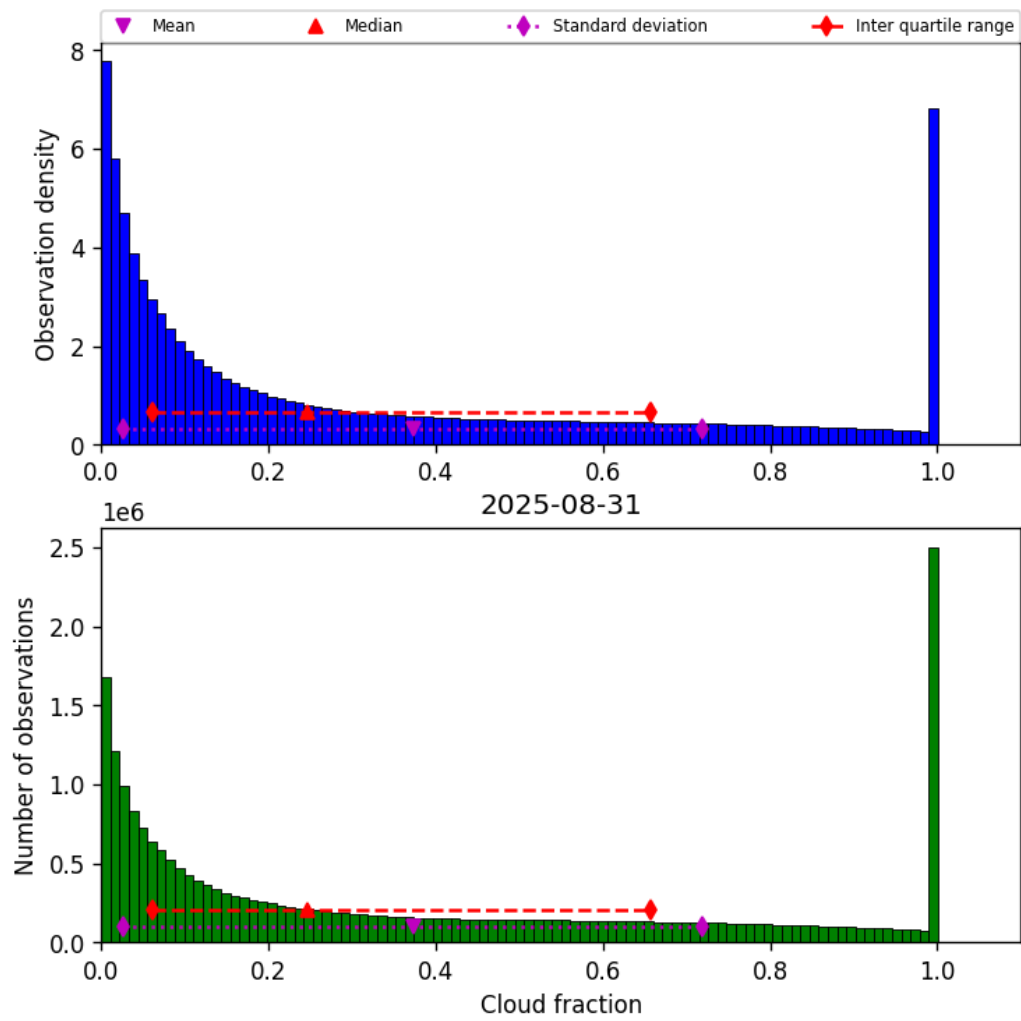
Figure 30: Histogram of “Cloud fraction” for 2025-08-31 to 2025-09-01
