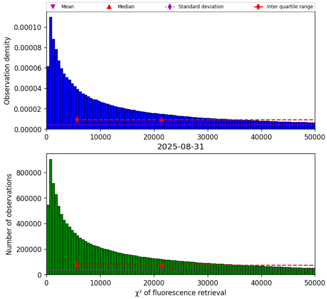
Figure 40: Histogram of “ \chi^2 of fluorescence retrieval” for 2025-08-31 to 2025-09-01
