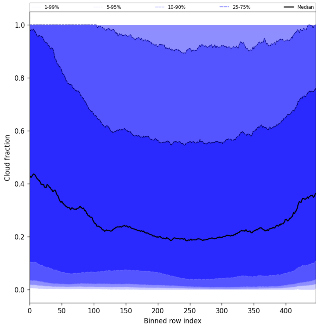
Figure 47: Along track statistics of “Cloud fraction” for 2025-08-31 to 2025-09-01
