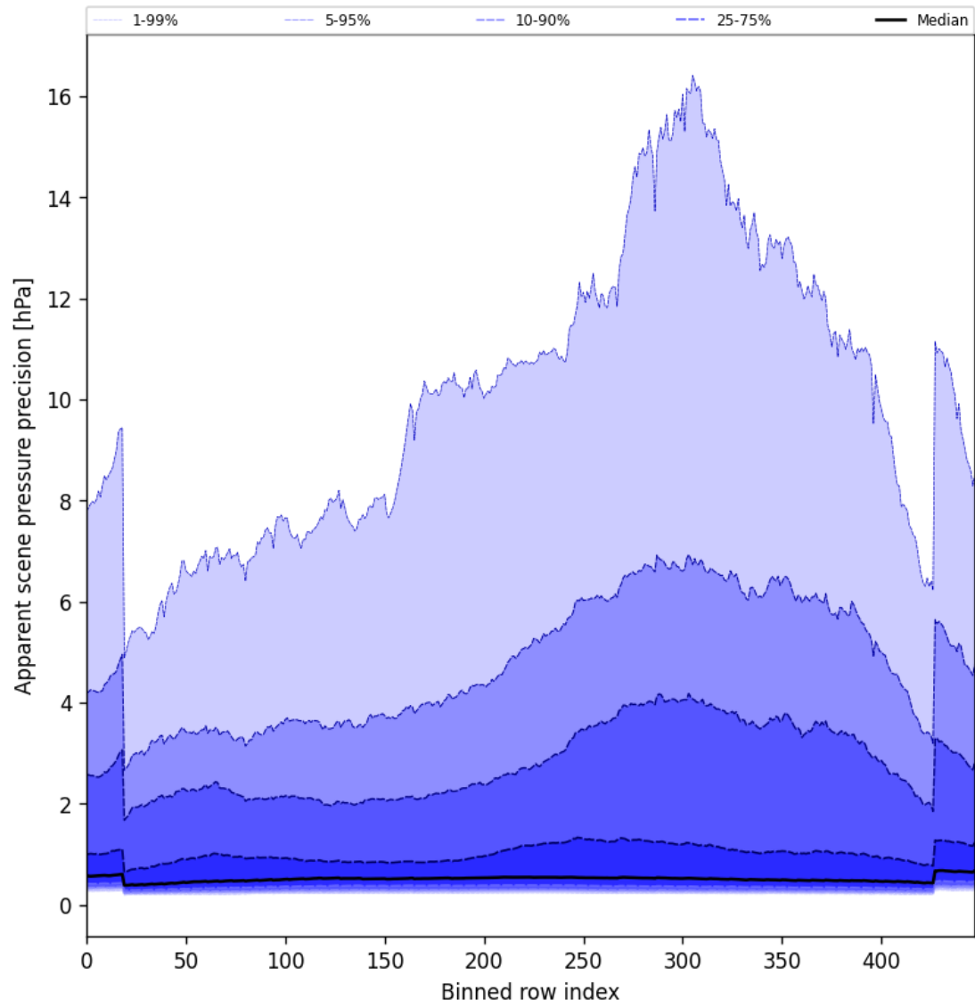
Figure 52: Along track statistics of “Apparent scene pressure precision” for 2025-08-31 to 2025-09-01
