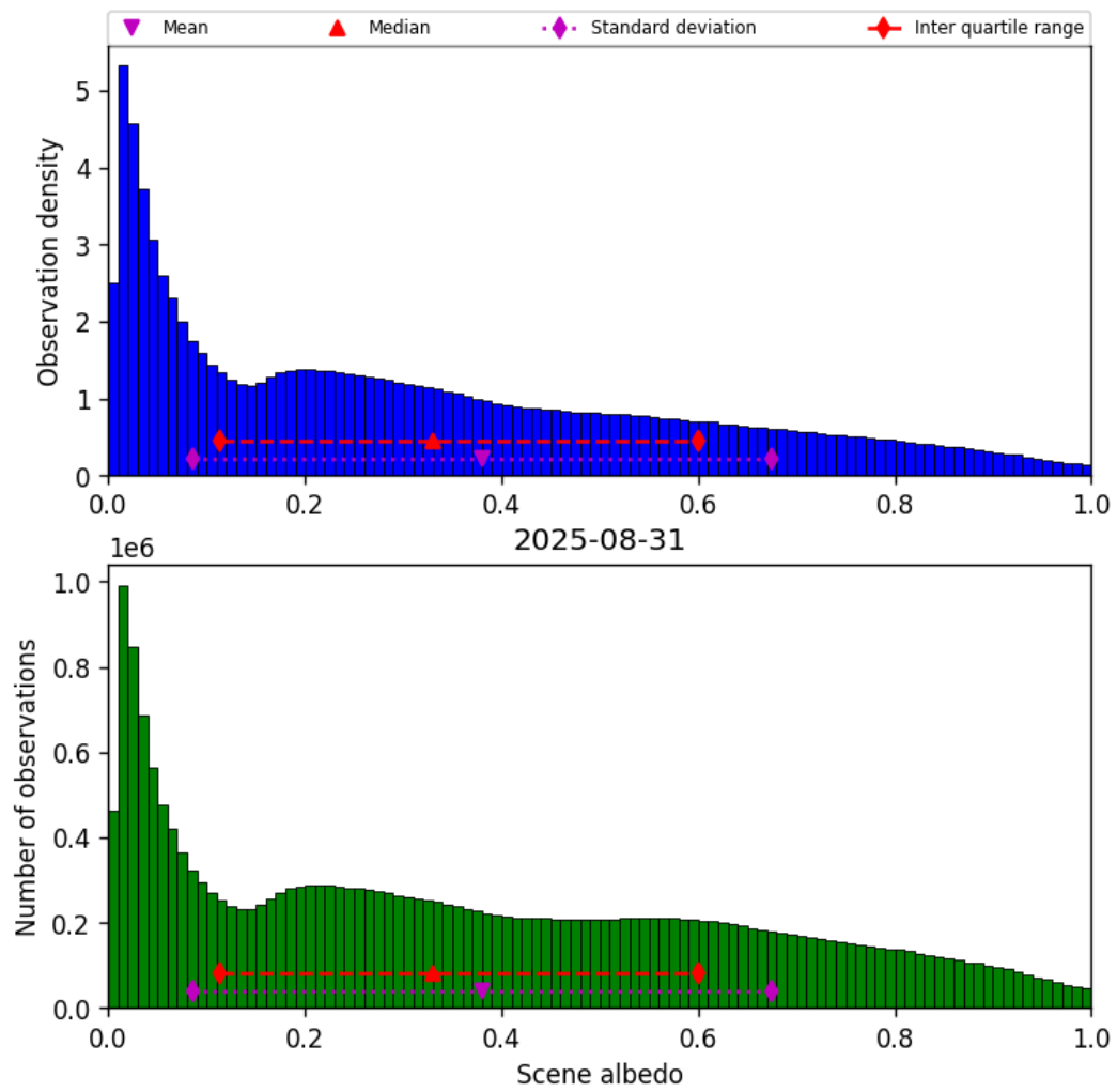
Figure 32: Histogram of “Scene albedo” for 2025-08-31 to 2025-09-01
