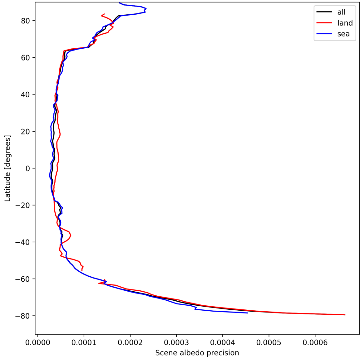
Figure 16: Zonal average of “Scene albedo precision” for 2025-08-31 to 2025-09-01.
