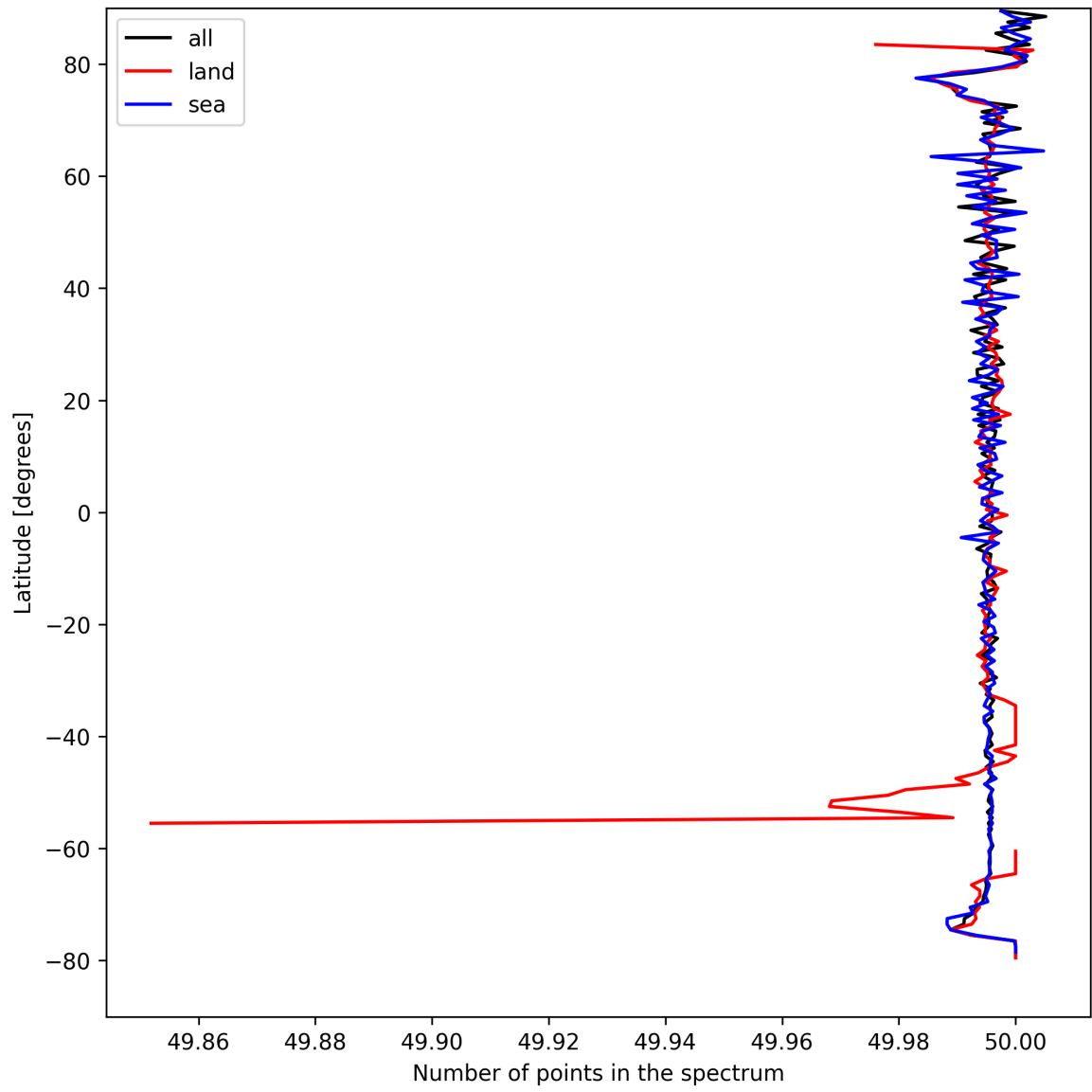
Figure 25: Zonal average of “Number of points in the spectrum” for 2025-08-31 to 2025-09-01.
