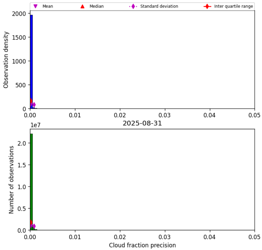
Figure 31: Histogram of “Cloud fraction precision” for 2025-08-31 to 2025-09-01
