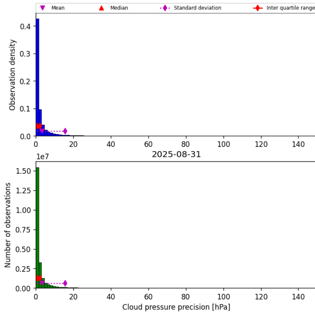
Figure 29: Histogram of “Cloud pressure precision” for 2025-08-31 to 2025-09-01
