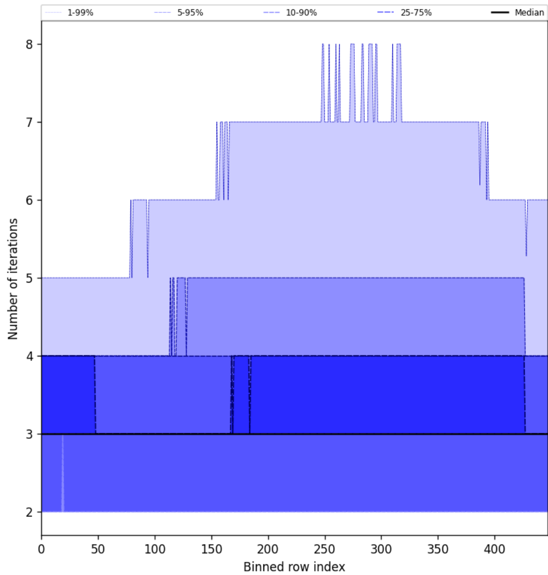
Figure 54: Along track statistics of “Number of iterations” for 2025-08-31 to 2025-09-01
