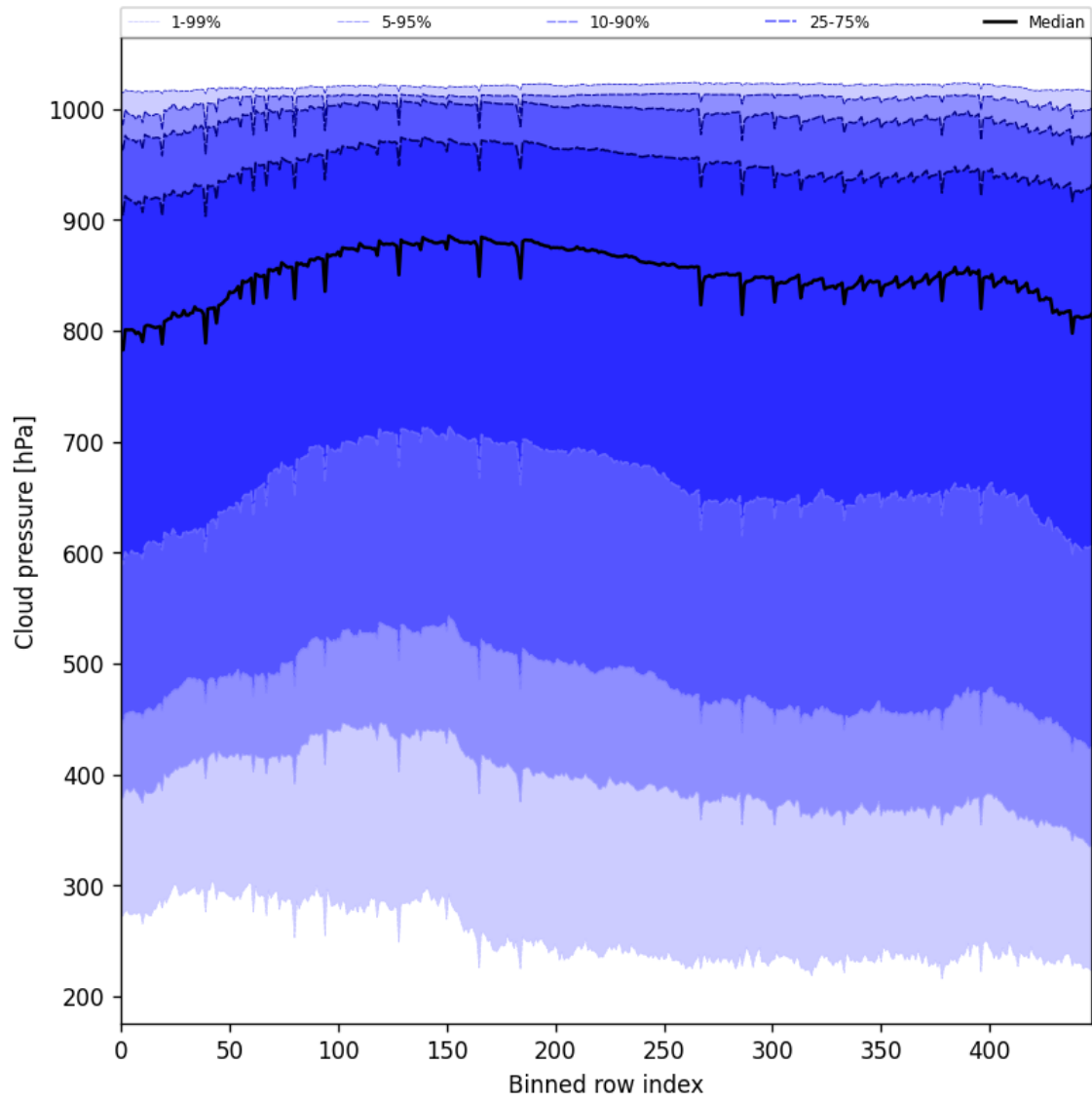
Figure 45: Along track statistics of “Cloud pressure” for 2025-08-31 to 2025-09-01
