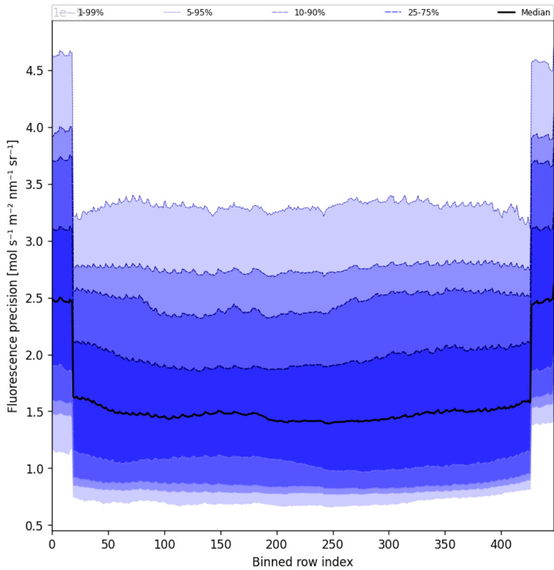
Figure 56: Along track statistics of “Fluorescence precision” for 2025-08-31 to 2025-09-01
