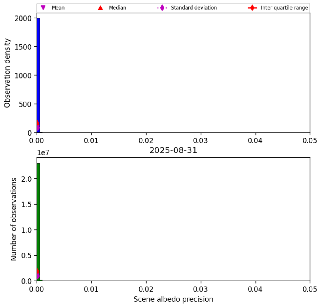
Figure 33: Histogram of “Scene albedo precision” for 2025-08-31 to 2025-09-01
