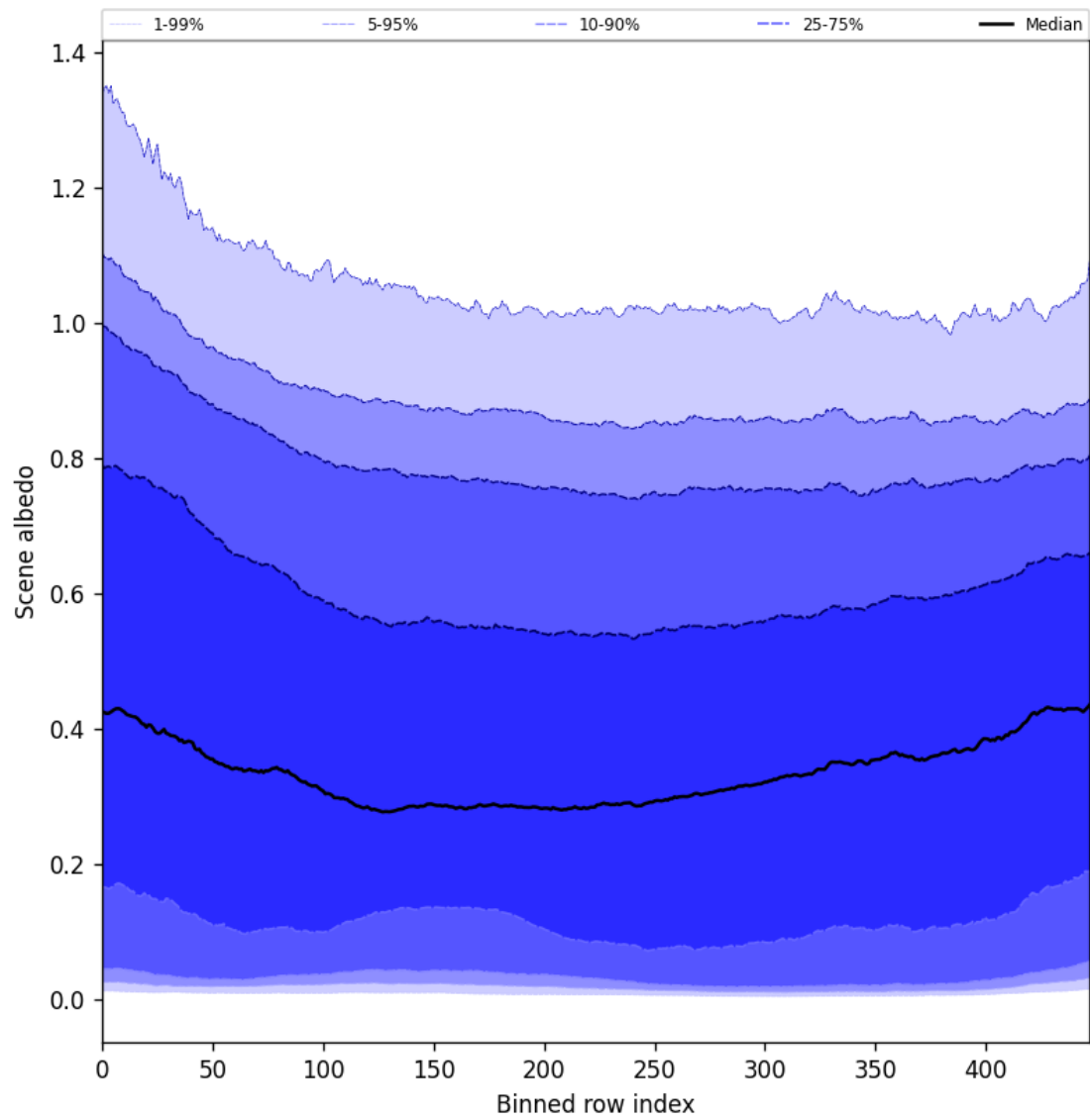
Figure 49: Along track statistics of “Scene albedo” for 2025-08-31 to 2025-09-01
