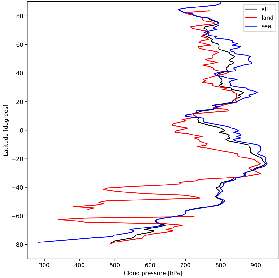
Figure 11: Zonal average of “Cloud pressure” for 2025-08-31 to 2025-09-01.
