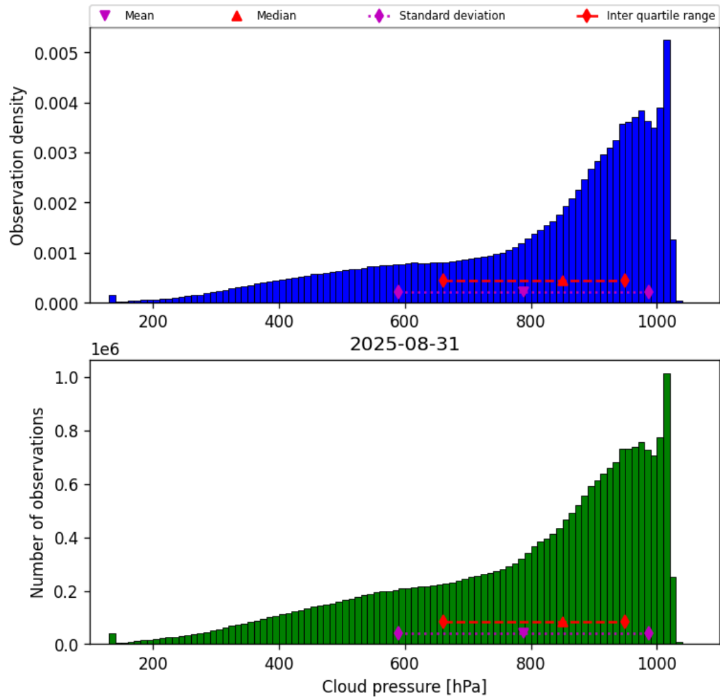
Figure 28: Histogram of “Cloud pressure” for 2025-08-31 to 2025-09-01
