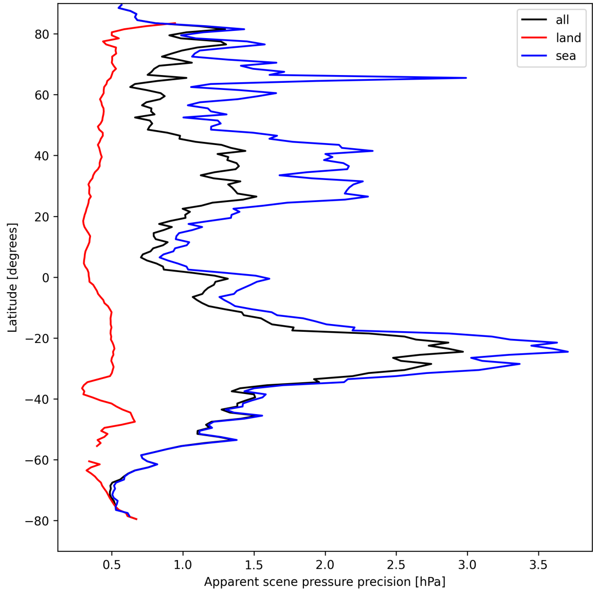
Figure 18: Zonal average of “Apparent scene pressure precision” for 2025-08-31 to 2025-09-01.
