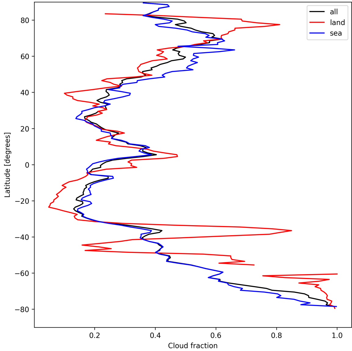
Figure 13: Zonal average of “Cloud fraction” for 2025-08-31 to 2025-09-01.
