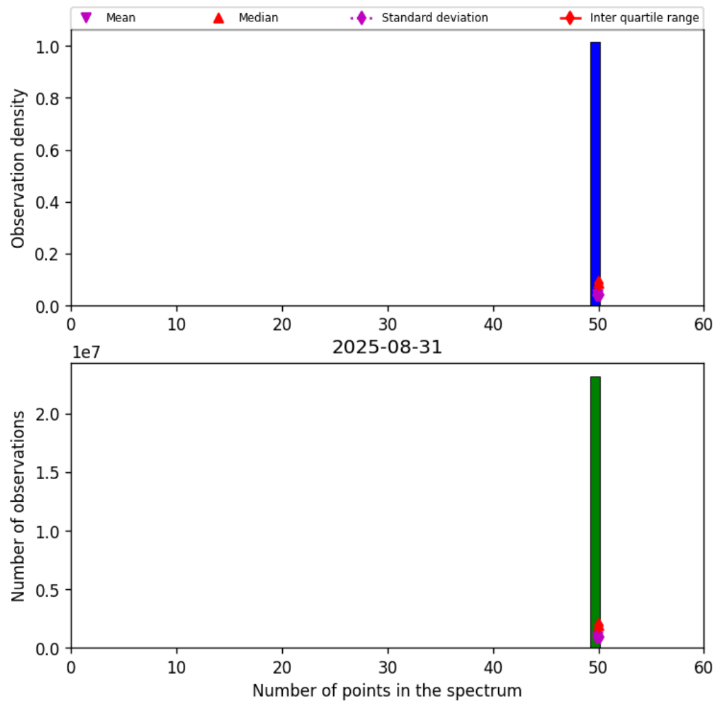
Figure 42: Histogram of “Number of points in the spectrum” for 2025-08-31 to 2025-09-01
