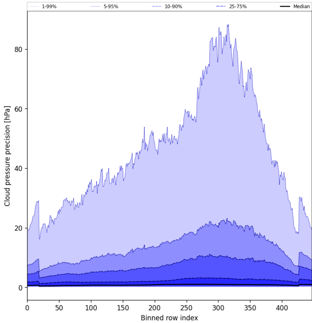
Figure 46: Along track statistics of “Cloud pressure precision” for 2025-08-31 to 2025-09-01
