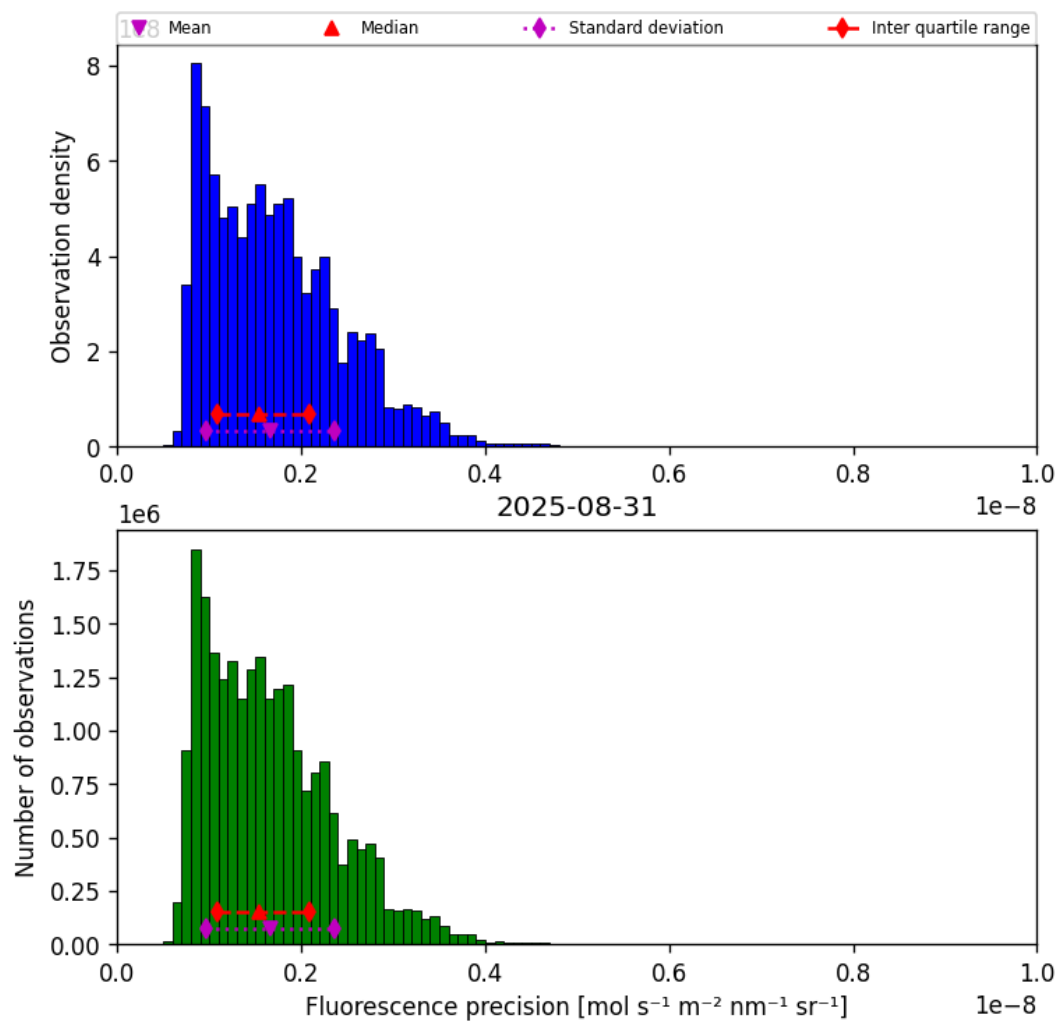
Figure 39: Histogram of “Fluorescence precision” for 2025-08-31 to 2025-09-01
