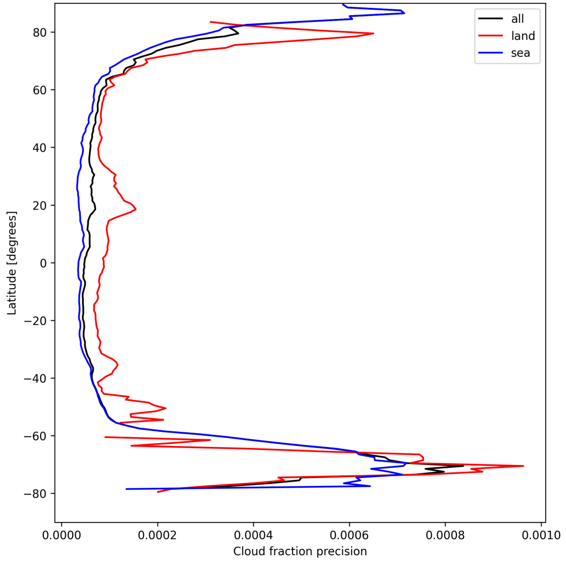
Figure 14: Zonal average of “Cloud fraction precision” for 2025-08-31 to 2025-09-01.
