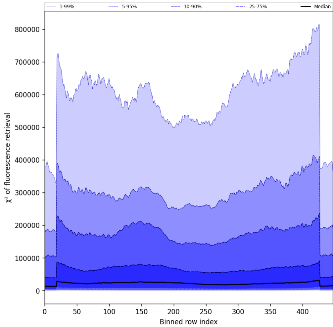
Figure 57: Along track statistics of “ \chi^2 of fluorescence retrieval” for 2025-08-31 to 2025-09-01
