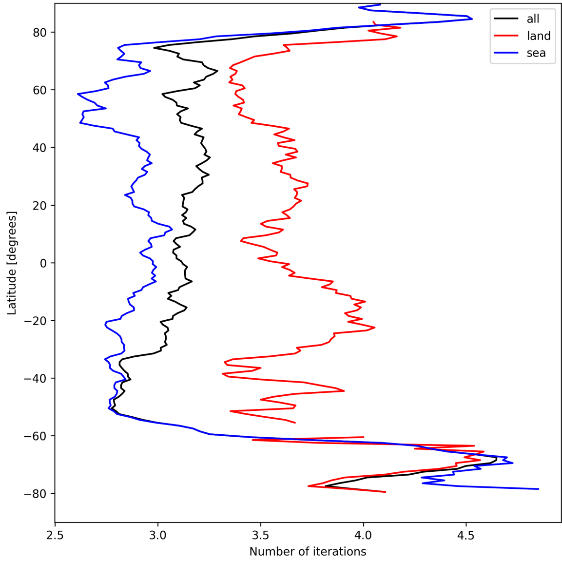
Figure 20: Zonal average of “Number of iterations” for 2025-08-31 to 2025-09-01.
