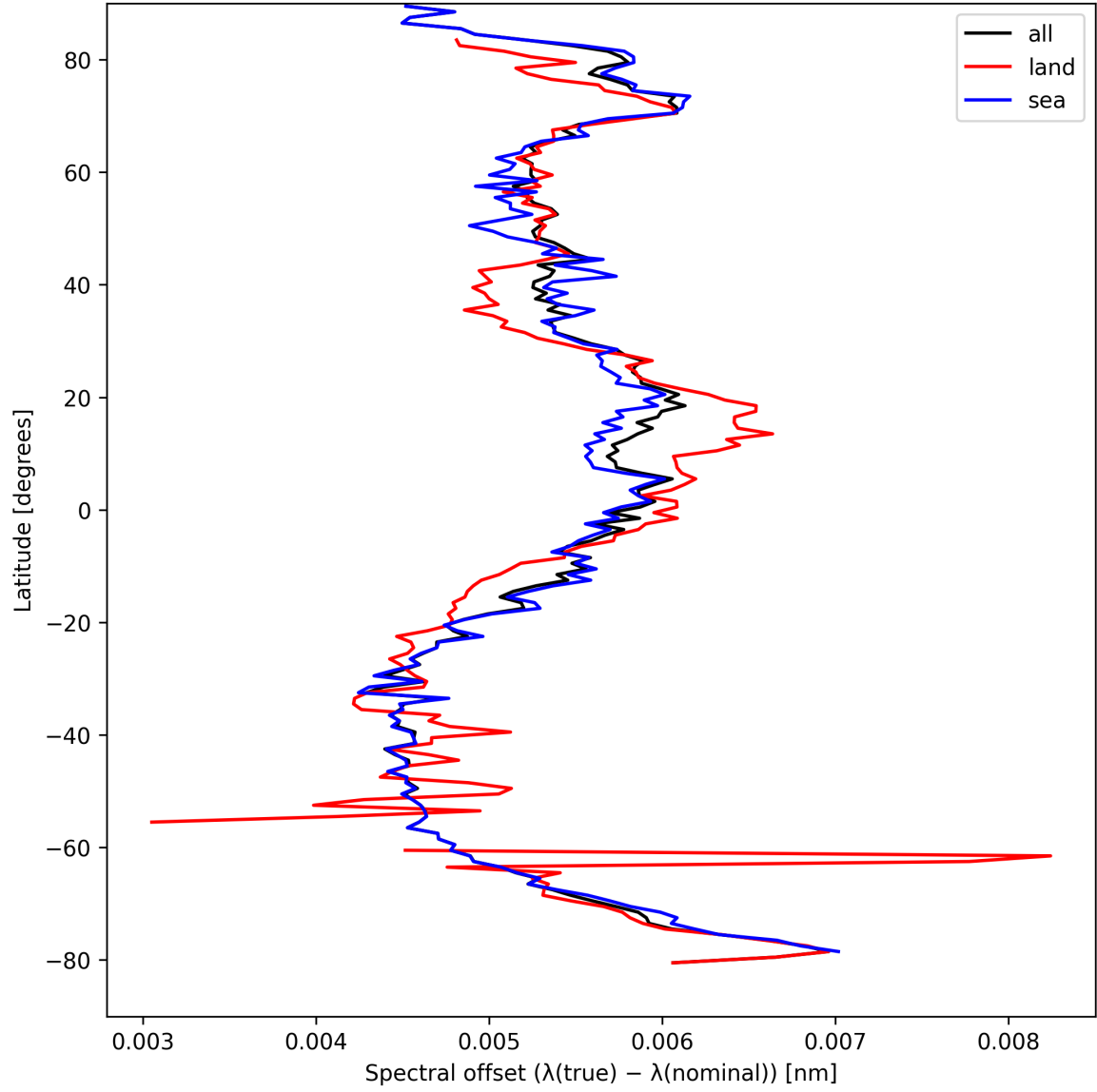
Figure 26: Zonal average of “Spectral offset ( \lambda_{\text{true}} - \lambda_{\text{nominal}} )” for 2025-09-01 to 2025-09-02.
