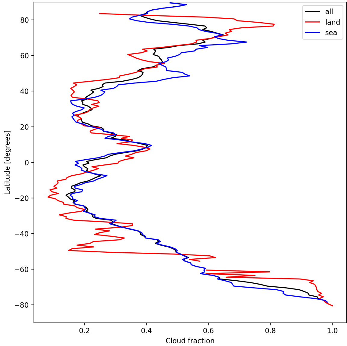
Figure 13: Zonal average of “Cloud fraction” for 2025-09-01 to 2025-09-02.
