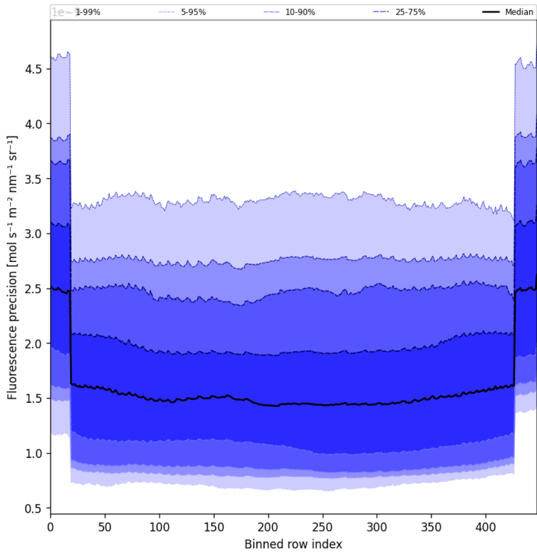
Figure 56: Along track statistics of “Fluorescence precision” for 2025-09-01 to 2025-09-02
