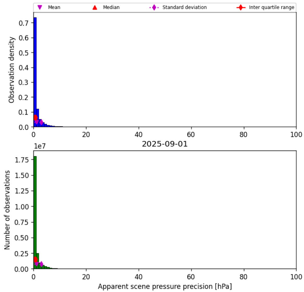
Figure 35: Histogram of “Apparent scene pressure precision” for 2025-09-01 to 2025-09-02
