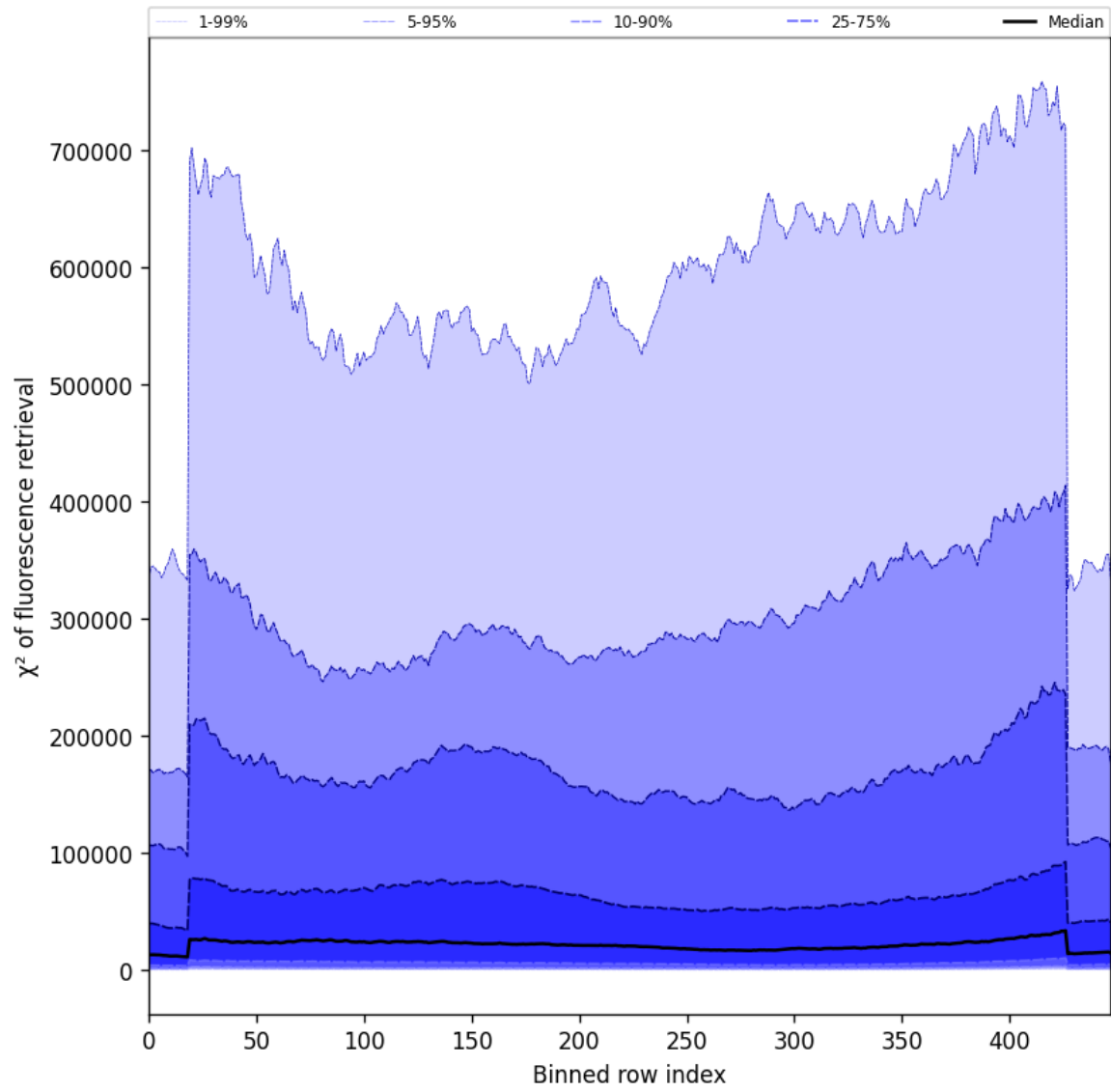
Figure 57: Along track statistics of “ \chi^2 of fluorescence retrieval” for 2025-09-01 to 2025-09-02
