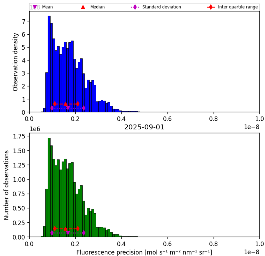
Figure 39: Histogram of “Fluorescence precision” for 2025-09-01 to 2025-09-02
