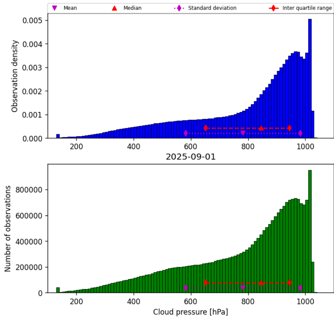
Figure 28: Histogram of “Cloud pressure” for 2025-09-01 to 2025-09-02
