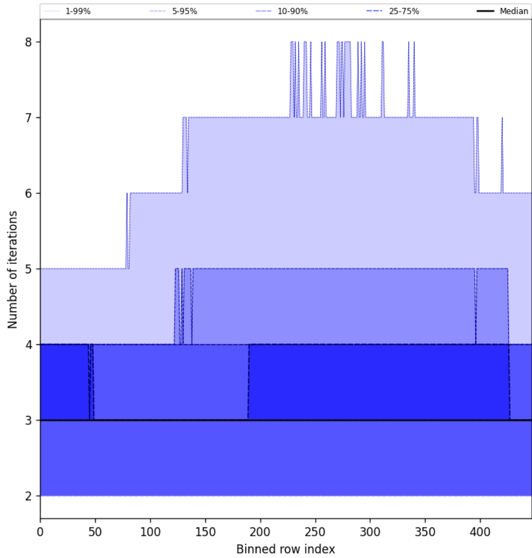
Figure 54: Along track statistics of “Number of iterations” for 2025-09-01 to 2025-09-02
