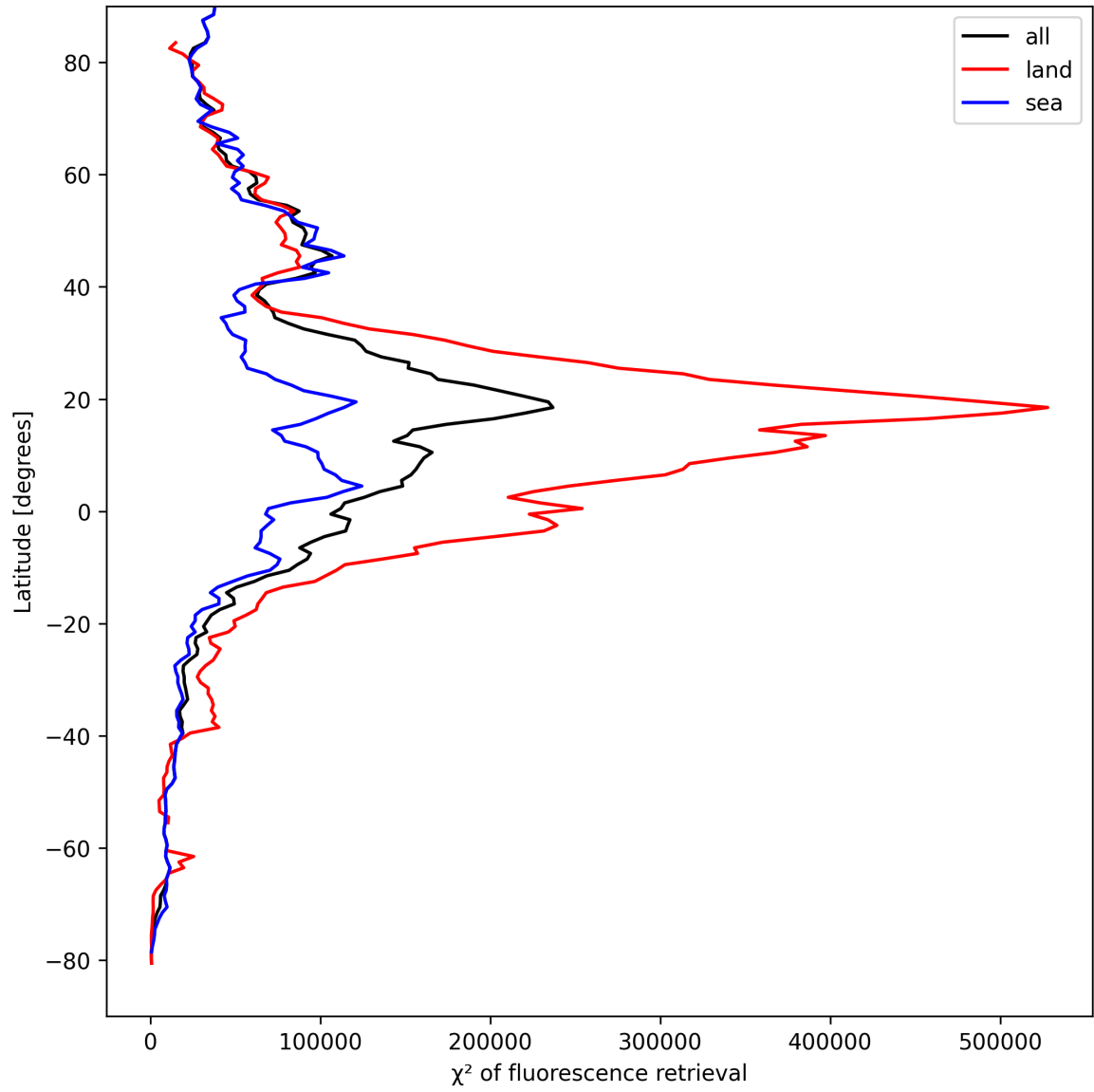
Figure 23: Zonal average of “ \chi^2 of fluorescence retrieval” for 2025-09-01 to 2025-09-02.
