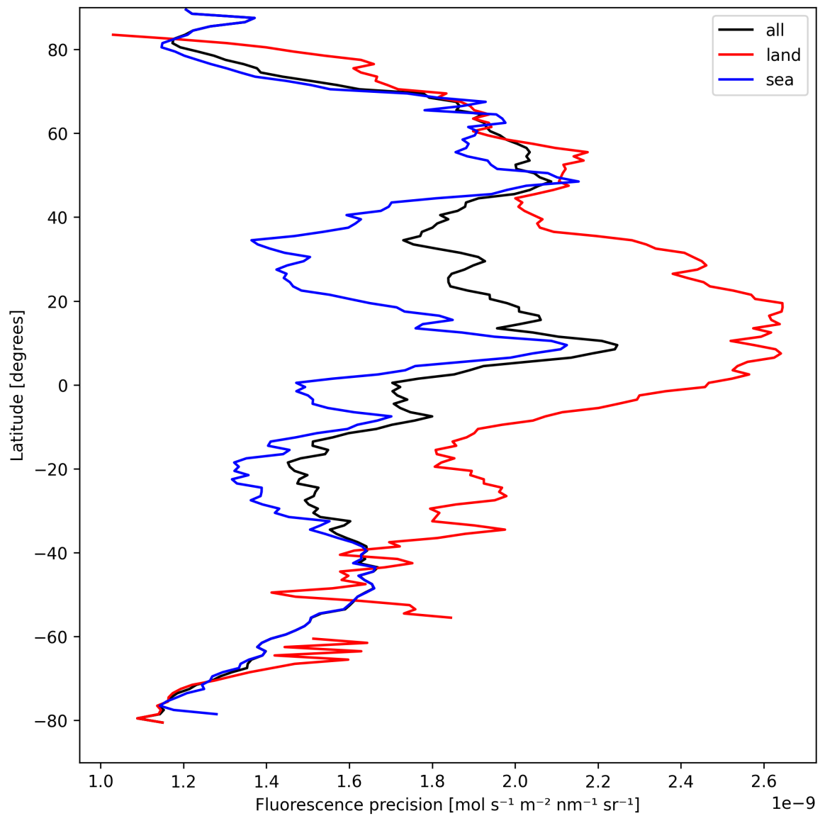
Figure 22: Zonal average of “Fluorescence precision” for 2025-09-01 to 2025-09-02.
