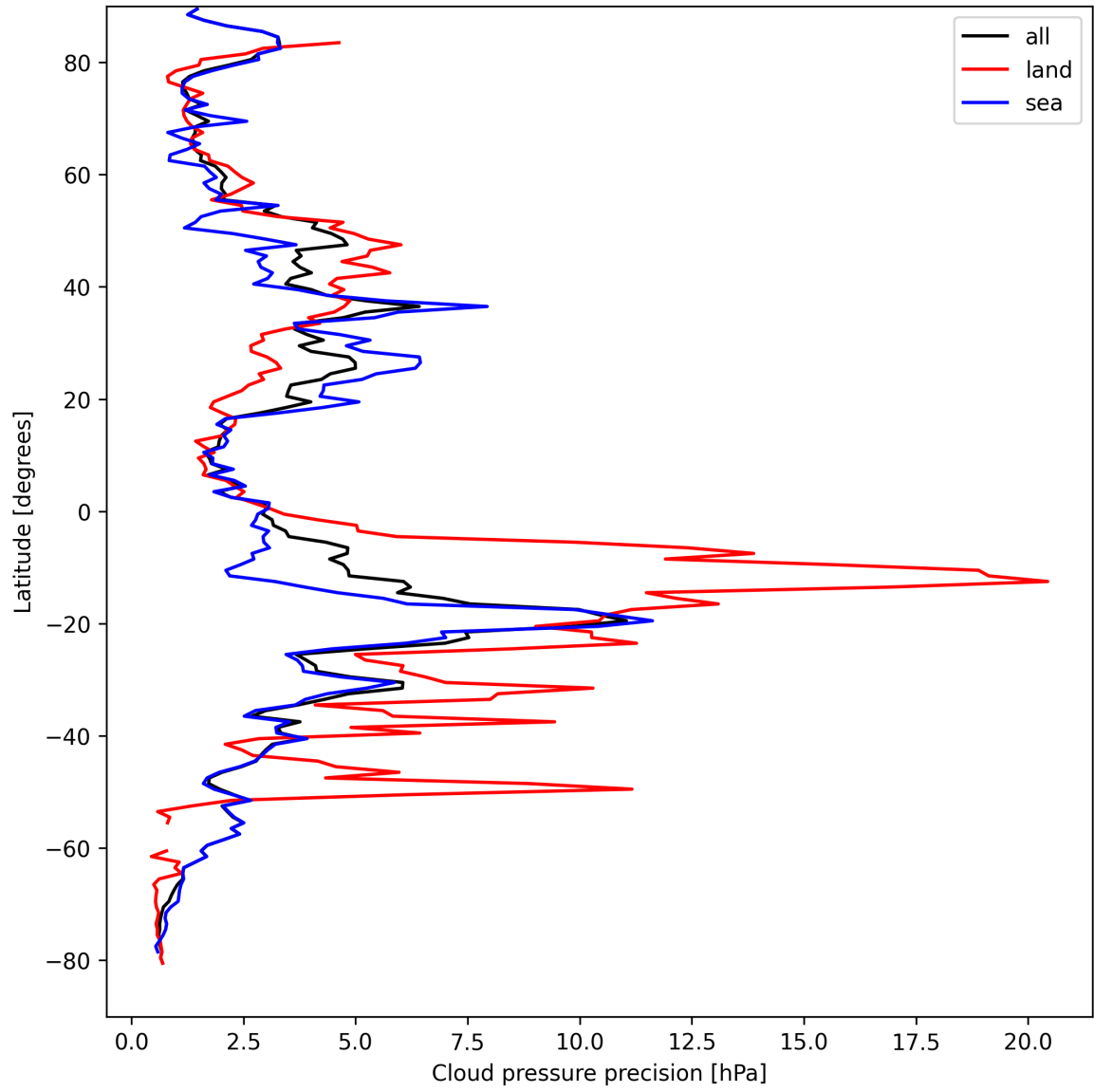
Figure 12: Zonal average of “Cloud pressure precision” for 2025-09-01 to 2025-09-02.
