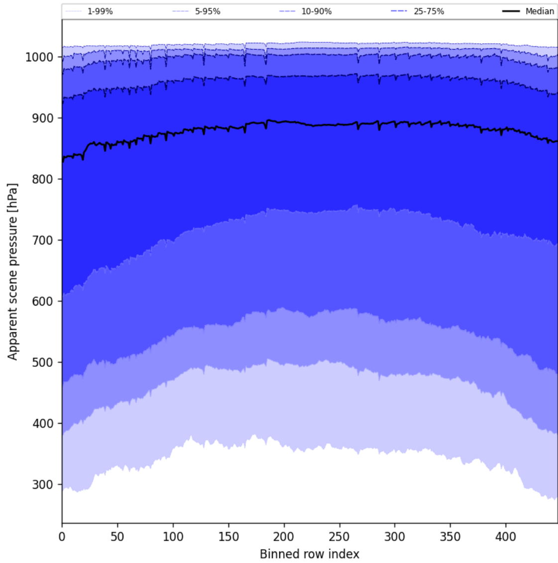
Figure 51: Along track statistics of “Apparent scene pressure” for 2025-09-01 to 2025-09-02
