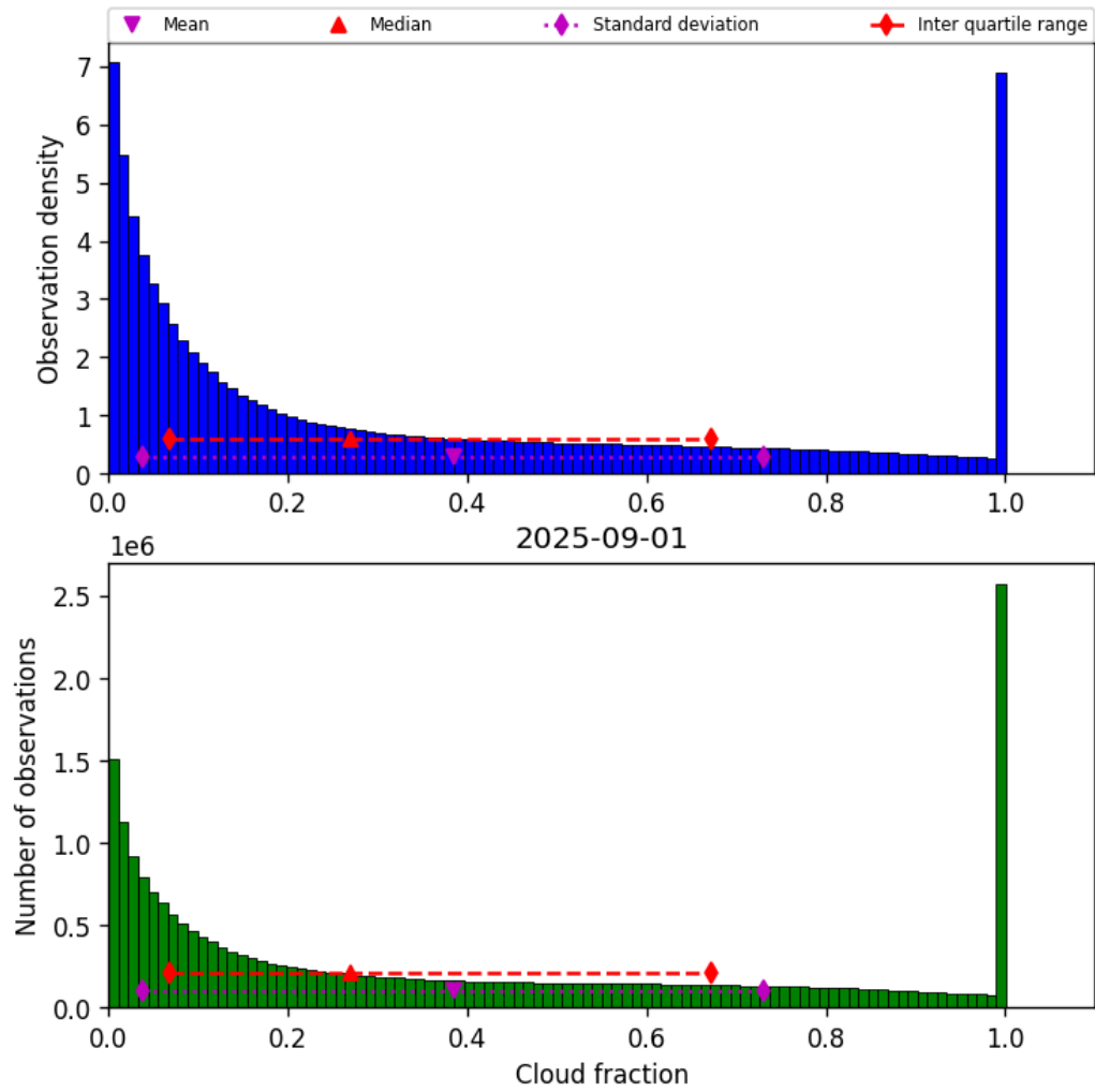
Figure 30: Histogram of “Cloud fraction” for 2025-09-01 to 2025-09-02
