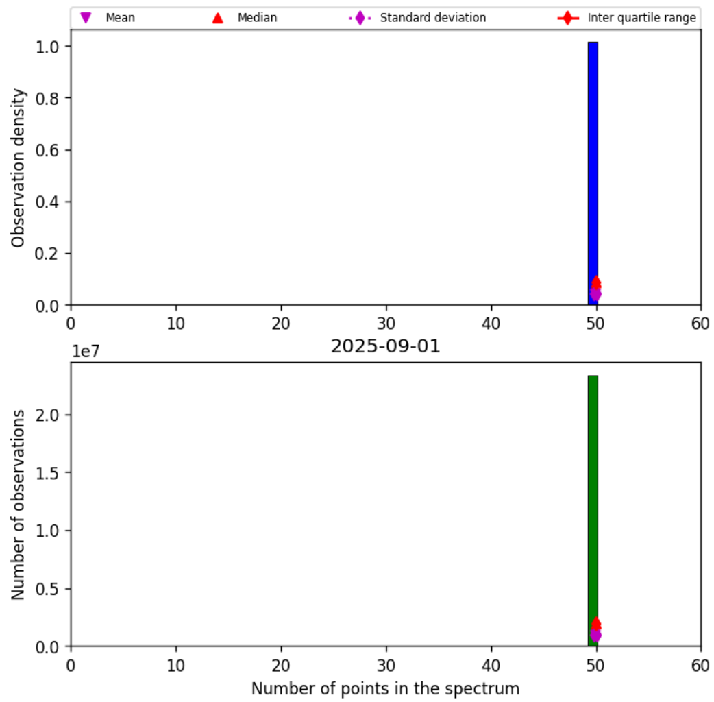
Figure 42: Histogram of “Number of points in the spectrum” for 2025-09-01 to 2025-09-02
