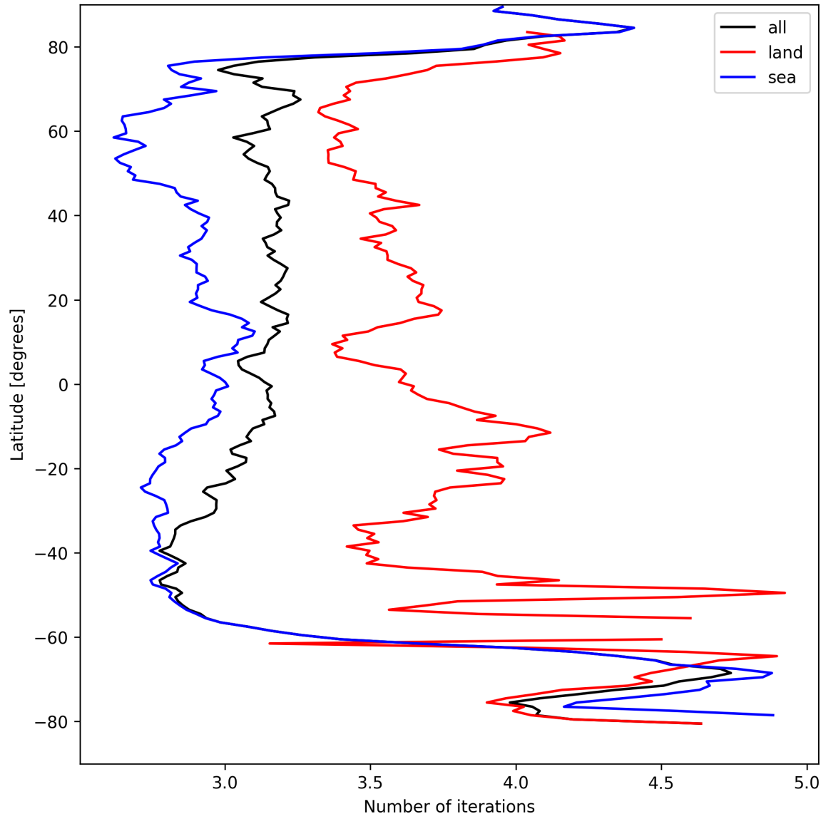
Figure 20: Zonal average of “Number of iterations” for 2025-09-01 to 2025-09-02.
