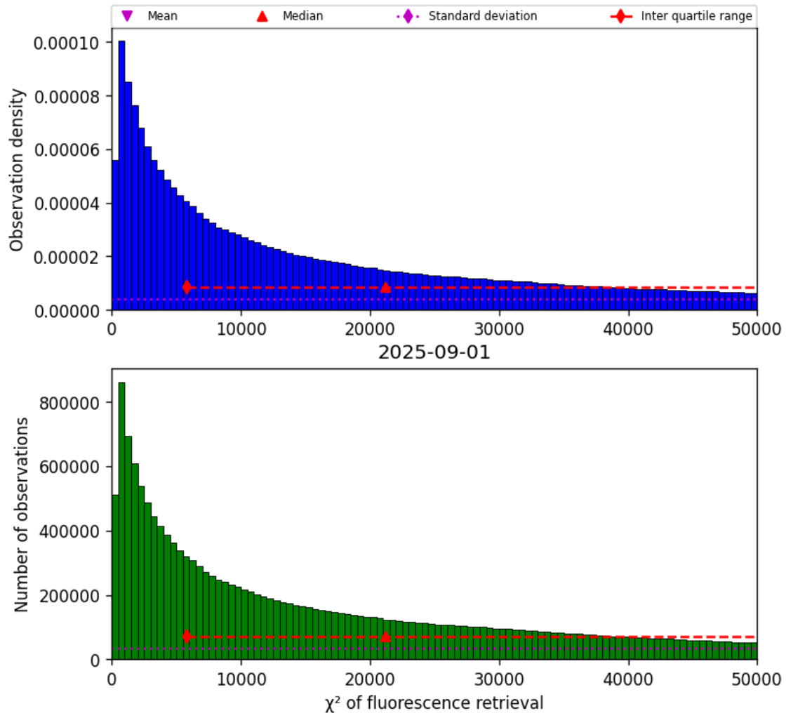
Figure 40: Histogram of “ \chi^2 of fluorescence retrieval” for 2025-09-01 to 2025-09-02
