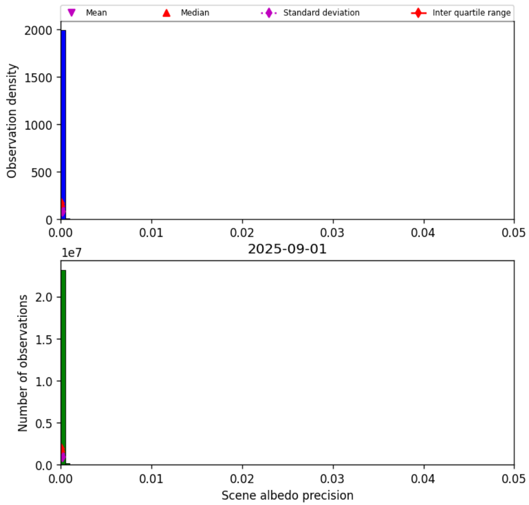
Figure 33: Histogram of “Scene albedo precision” for 2025-09-01 to 2025-09-02
