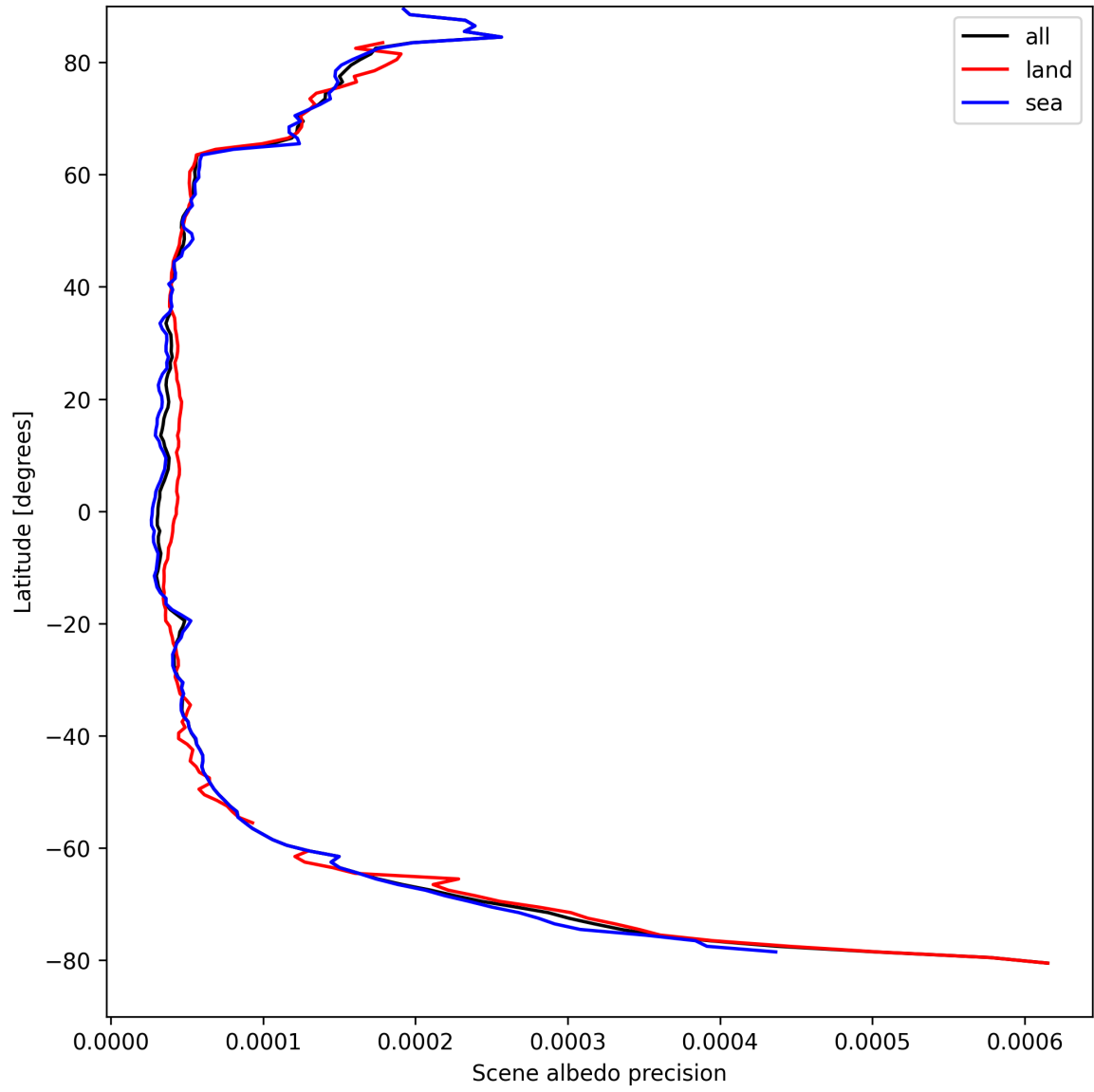
Figure 16: Zonal average of “Scene albedo precision” for 2025-09-01 to 2025-09-02.
