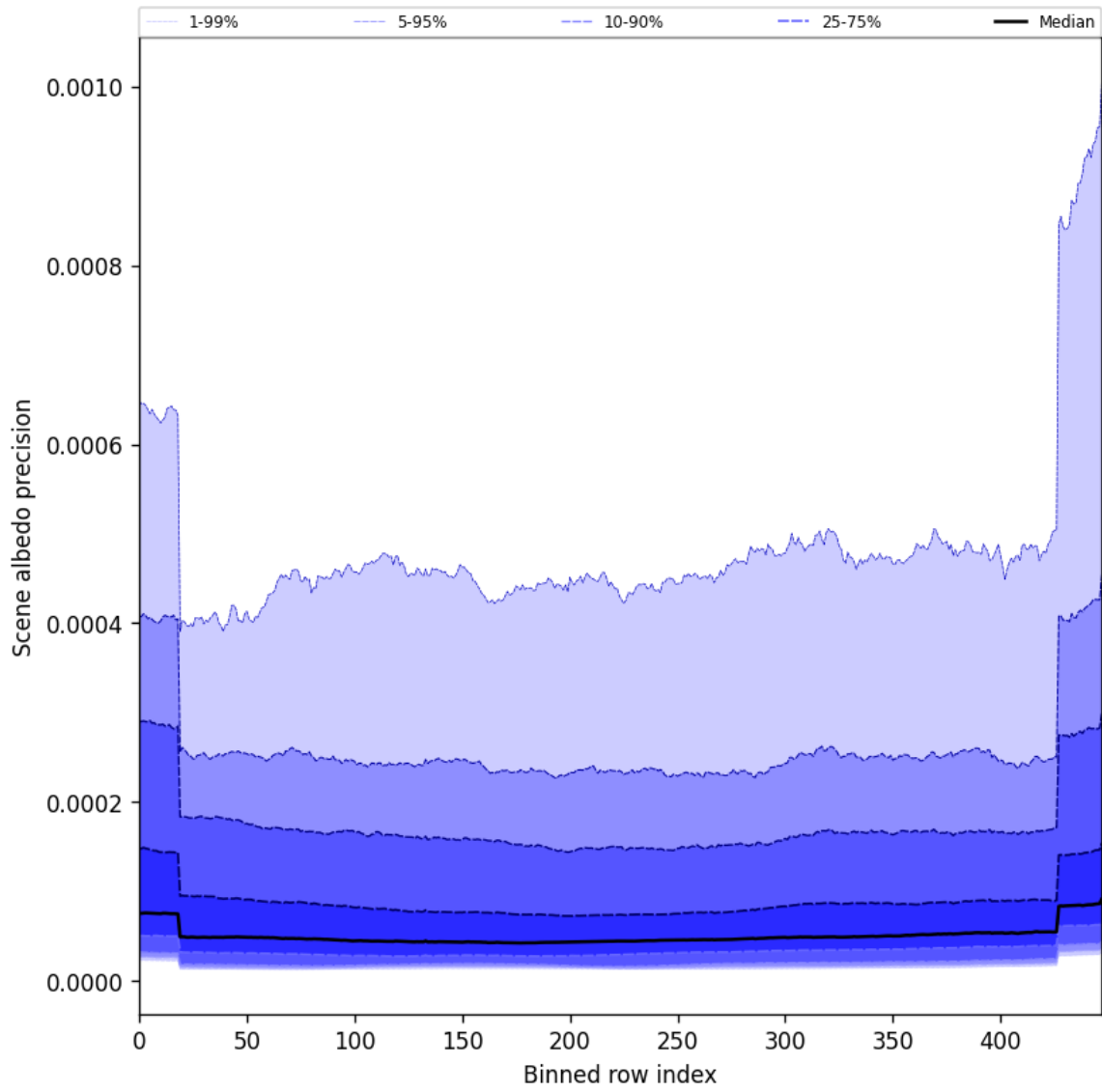
Figure 50: Along track statistics of “Scene albedo precision” for 2025-09-01 to 2025-09-02
