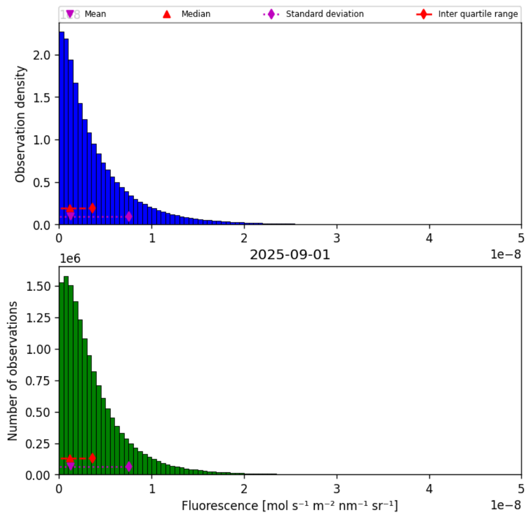
Figure 38: Histogram of “Fluorescence” for 2025-09-01 to 2025-09-02
