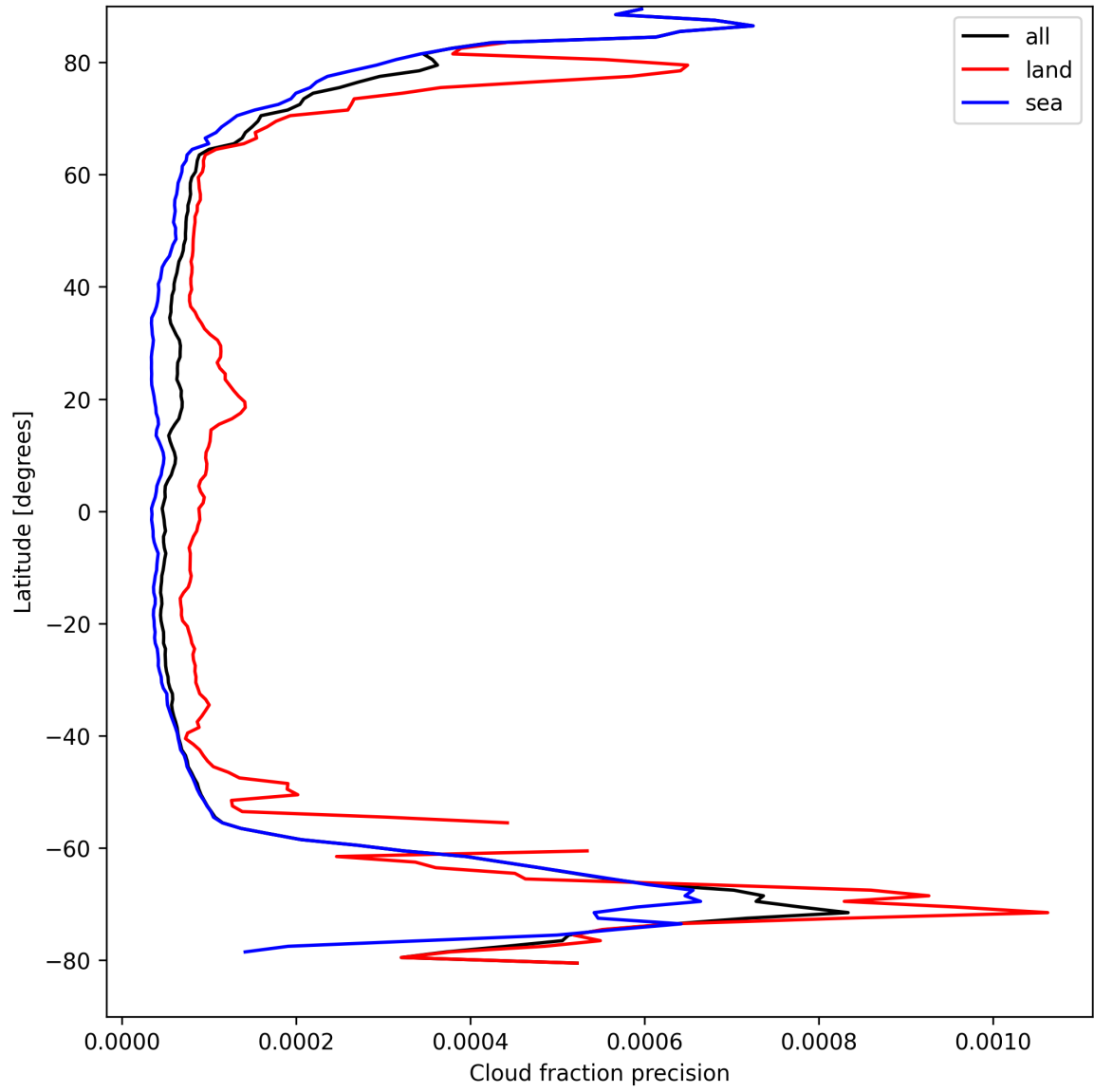
Figure 14: Zonal average of “Cloud fraction precision” for 2025-09-01 to 2025-09-02.
