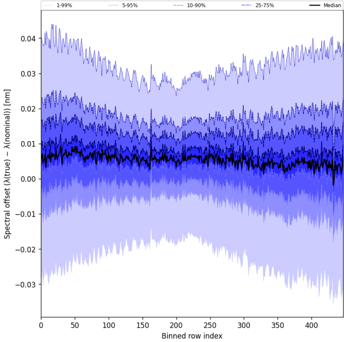
Figure 60: Along track statistics of “Spectral offset ( \lambda_{\text{true}} - \lambda_{\text{nominal}} )” for 2025-09-01 to 2025-09-02
