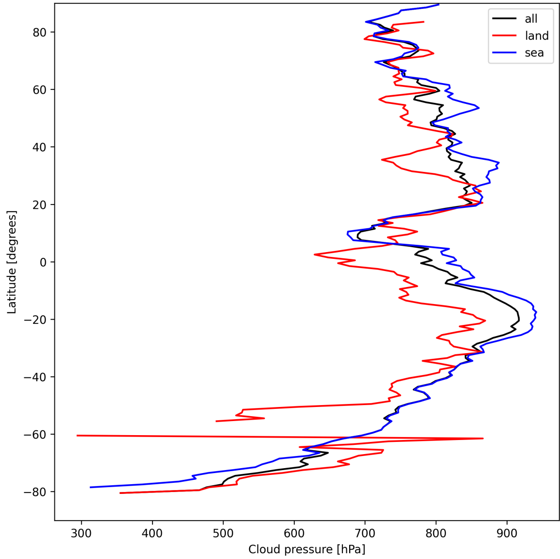
Figure 11: Zonal average of “Cloud pressure” for 2025-09-01 to 2025-09-02.
