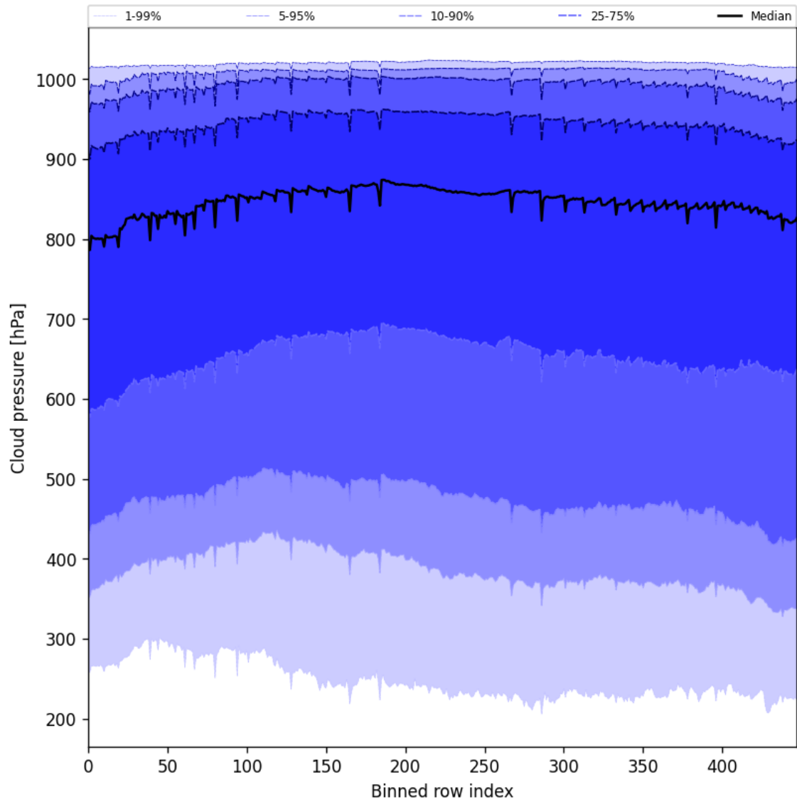
Figure 45: Along track statistics of “Cloud pressure” for 2025-09-01 to 2025-09-02
