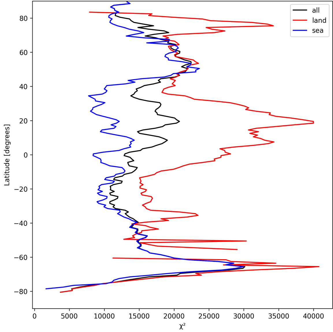
Figure 19: Zonal average of “ \chi^2 ” for 2025-09-01 to 2025-09-02.
