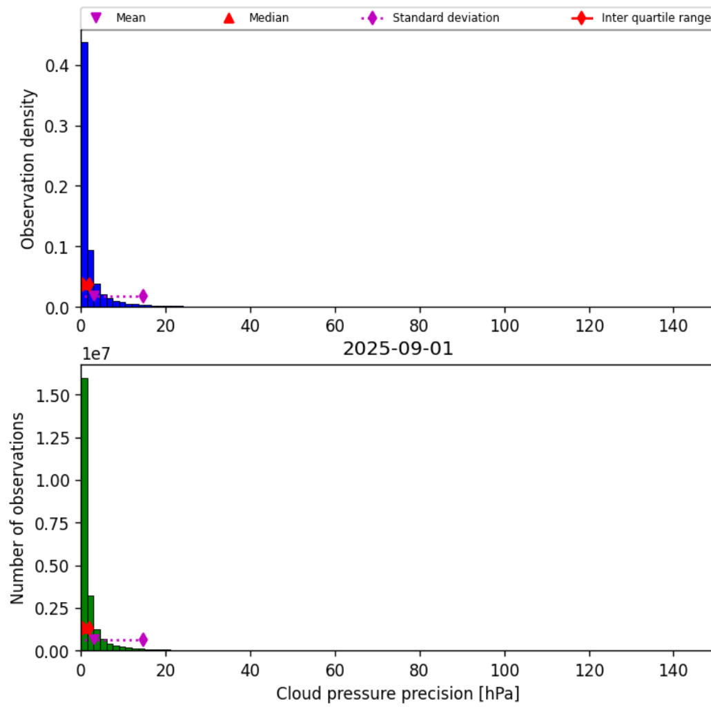
Figure 29: Histogram of “Cloud pressure precision” for 2025-09-01 to 2025-09-02
