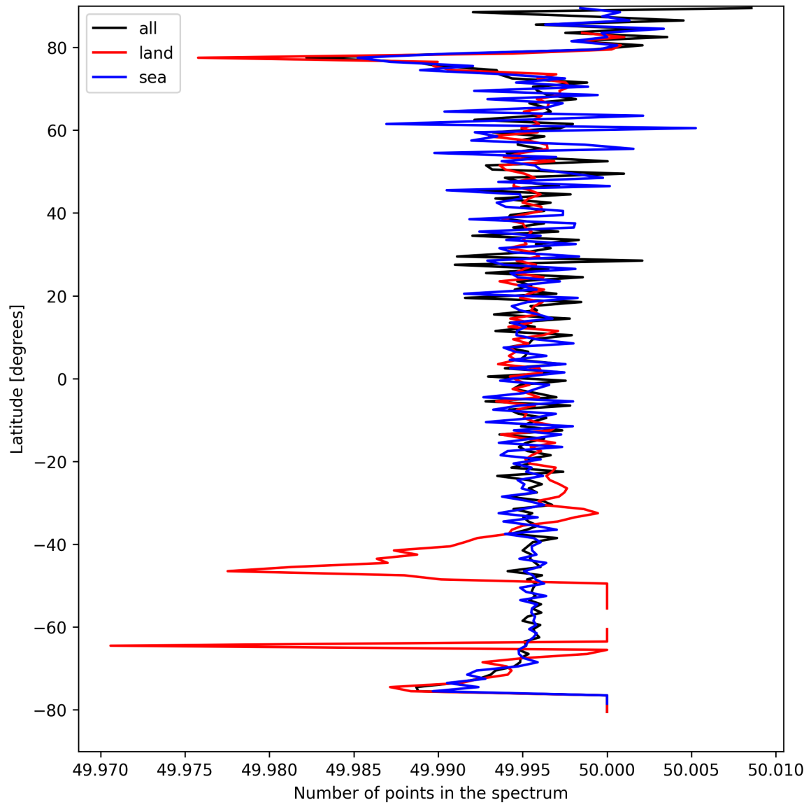
Figure 25: Zonal average of “Number of points in the spectrum” for 2025-09-01 to 2025-09-02.
