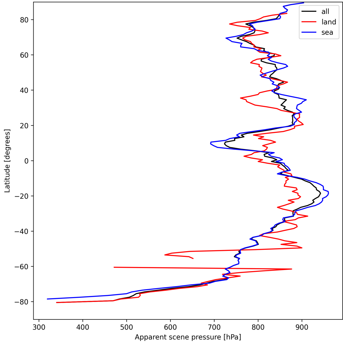
Figure 17: Zonal average of “Apparent scene pressure” for 2025-09-01 to 2025-09-02.
