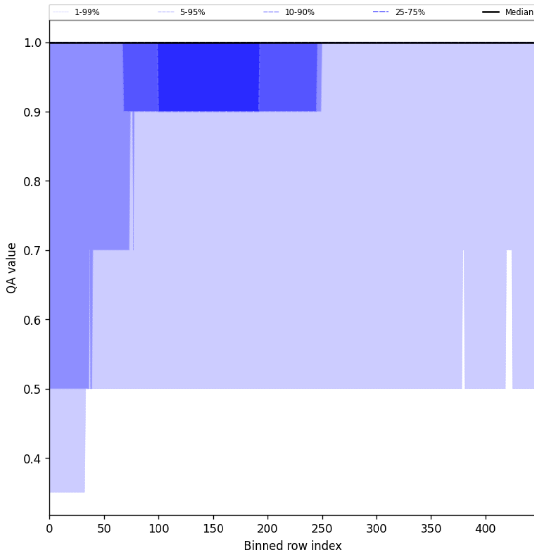
Figure 44: Along track statistics of “QA value” for 2025-09-01 to 2025-09-02
