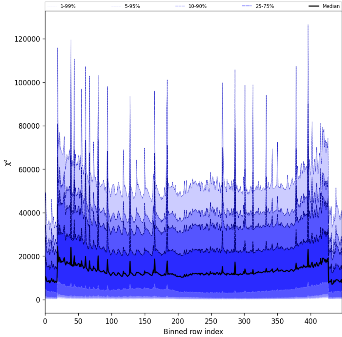
Figure 53: Along track statistics of “ \chi^2 ” for 2025-09-01 to 2025-09-02
