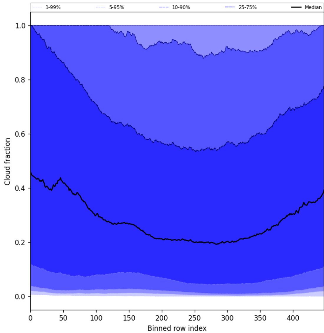
Figure 47: Along track statistics of “Cloud fraction” for 2025-09-01 to 2025-09-02
