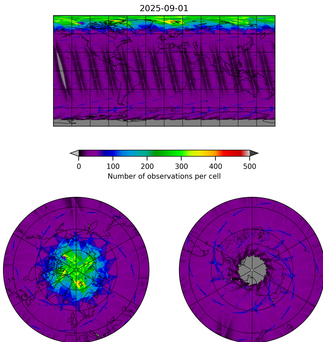
Figure 9: Map of the number of observations for 2025-09-01 to 2025-09-02
