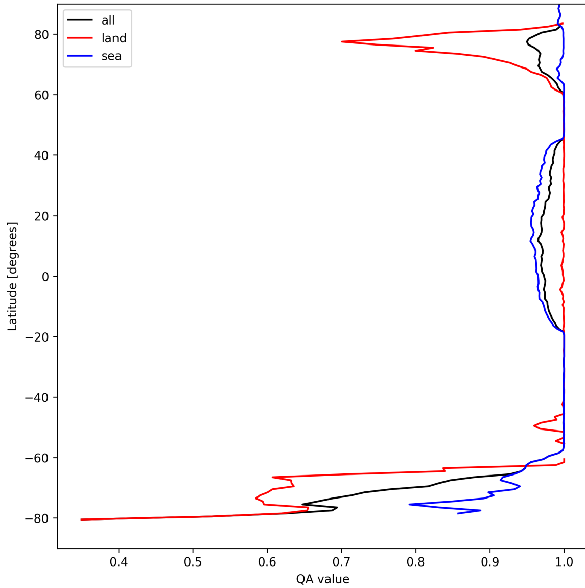
Figure 10: Zonal average of "QA value" for 2025-09-01 to 2025-09-02.
