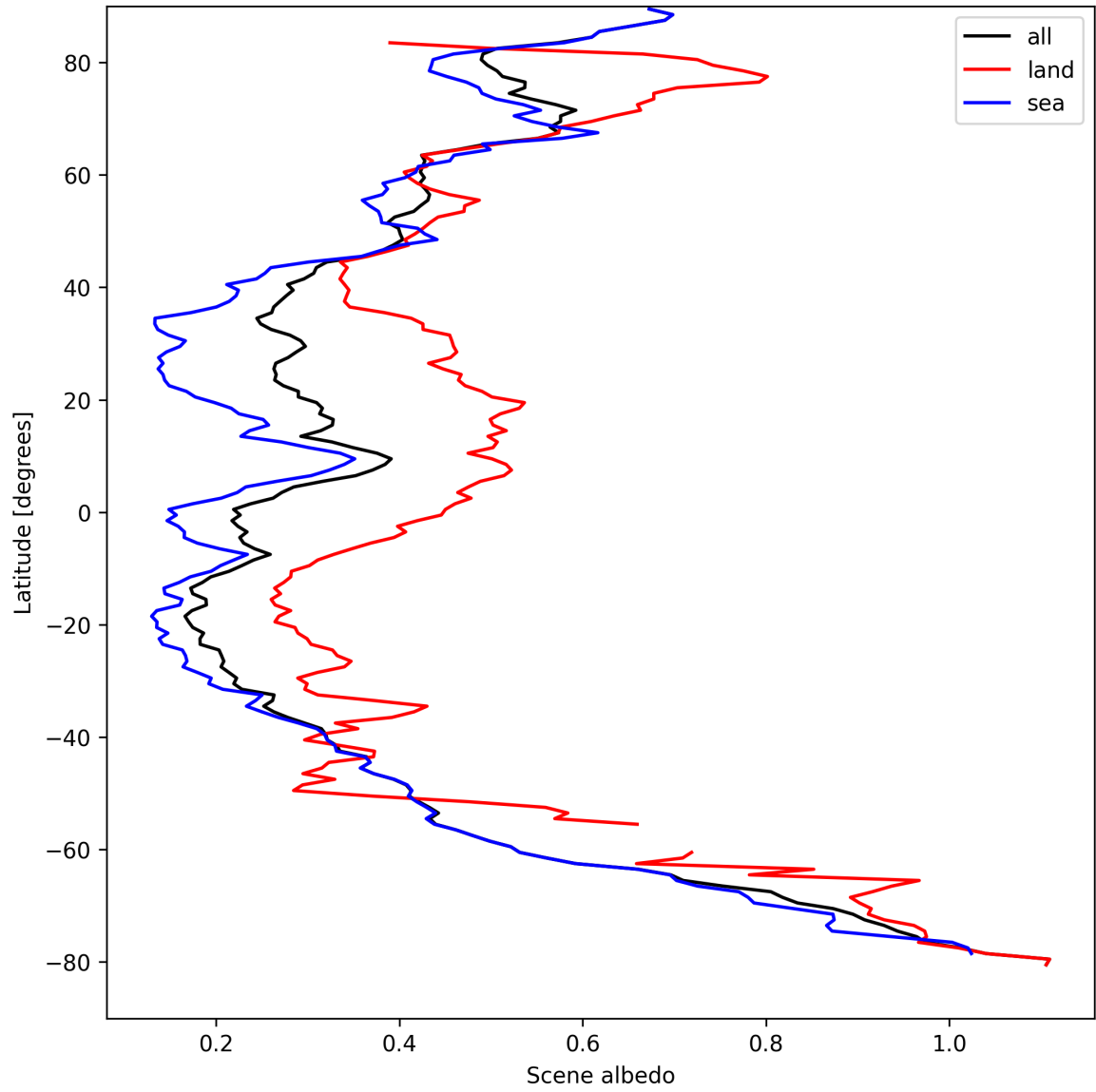
Figure 15: Zonal average of “Scene albedo” for 2025-09-01 to 2025-09-02.
