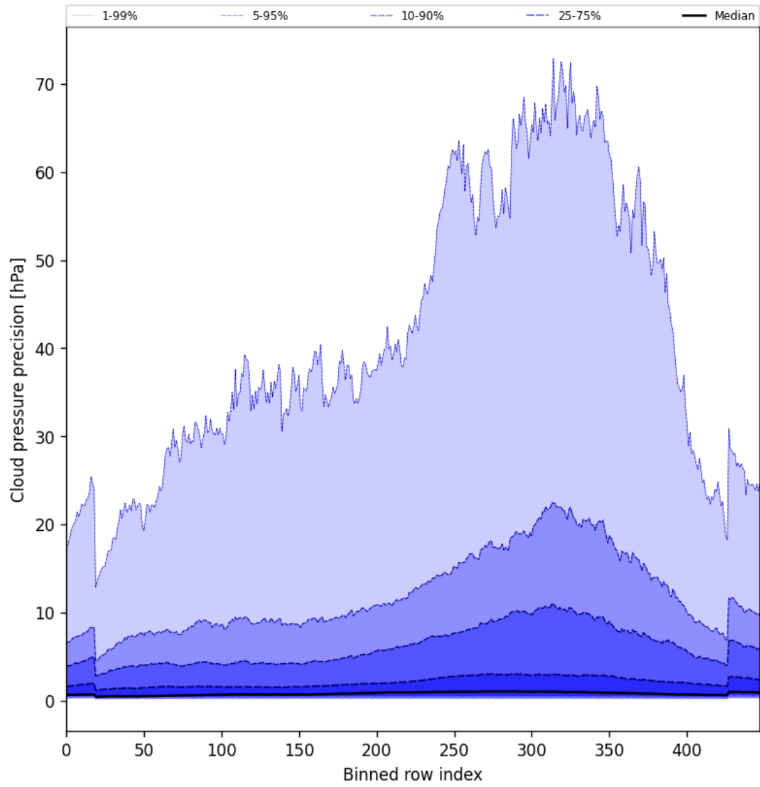
Figure 46: Along track statistics of “Cloud pressure precision” for 2025-09-01 to 2025-09-02
