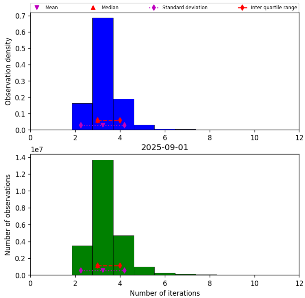
Figure 37: Histogram of “Number of iterations” for 2025-09-01 to 2025-09-02
