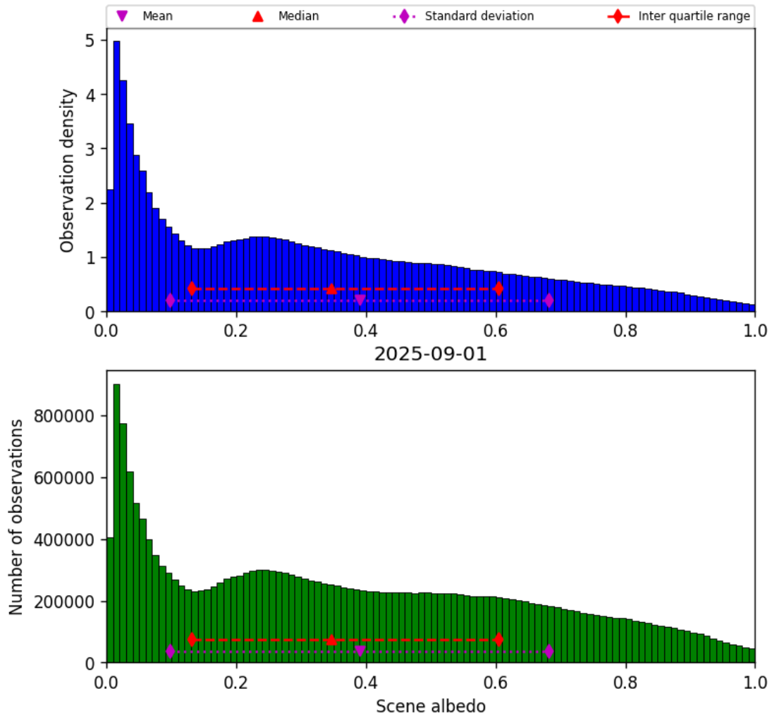
Figure 32: Histogram of “Scene albedo” for 2025-09-01 to 2025-09-02
