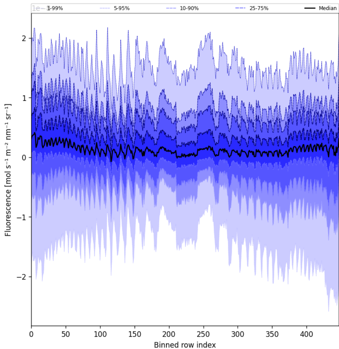
Figure 55: Along track statistics of “Fluorescence” for 2025-09-01 to 2025-09-02
