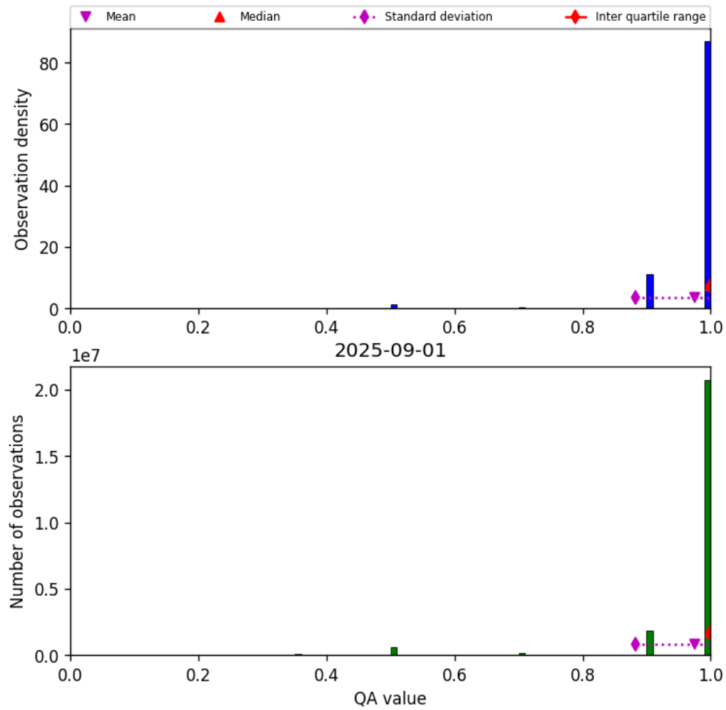
Figure 27: Histogram of “QA value” for 2025-09-01 to 2025-09-02
