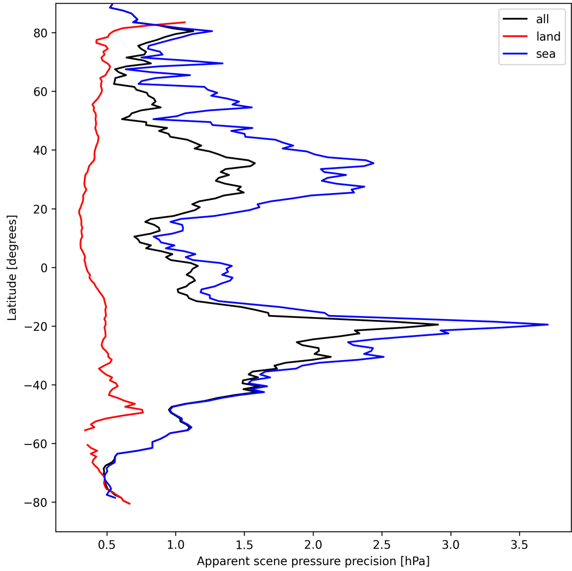
Figure 18: Zonal average of “Apparent scene pressure precision” for 2025-09-01 to 2025-09-02.
