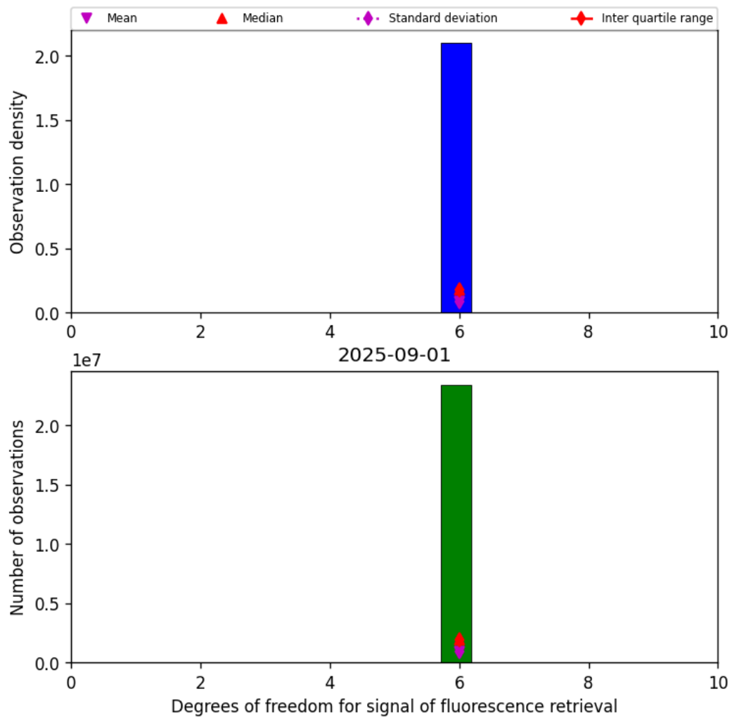
Figure 41: Histogram of “Degrees of freedom for signal of fluorescence retrieval” for 2025-09-01 to 2025-09-02
