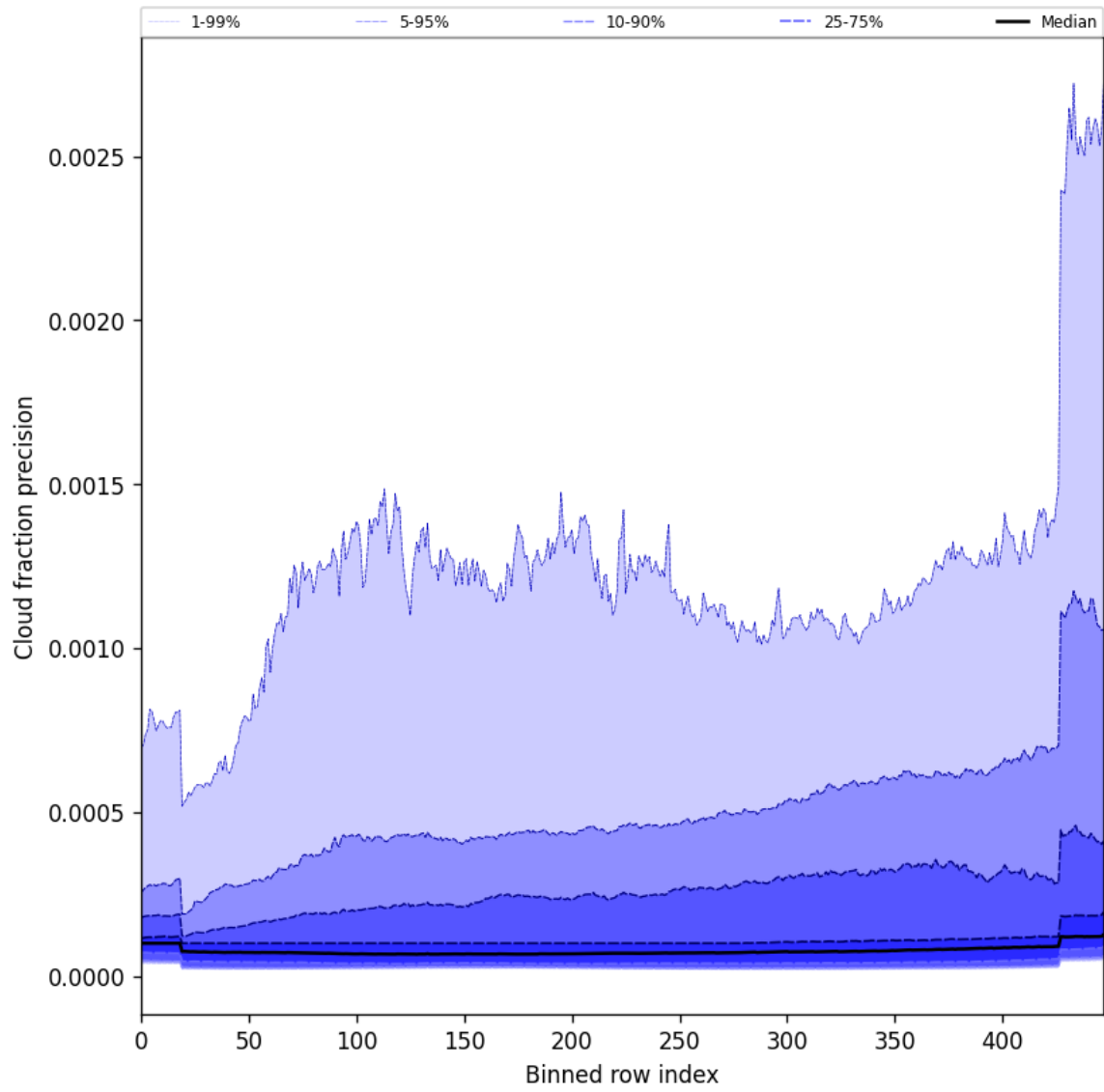
Figure 48: Along track statistics of “Cloud fraction precision” for 2025-09-01 to 2025-09-02
