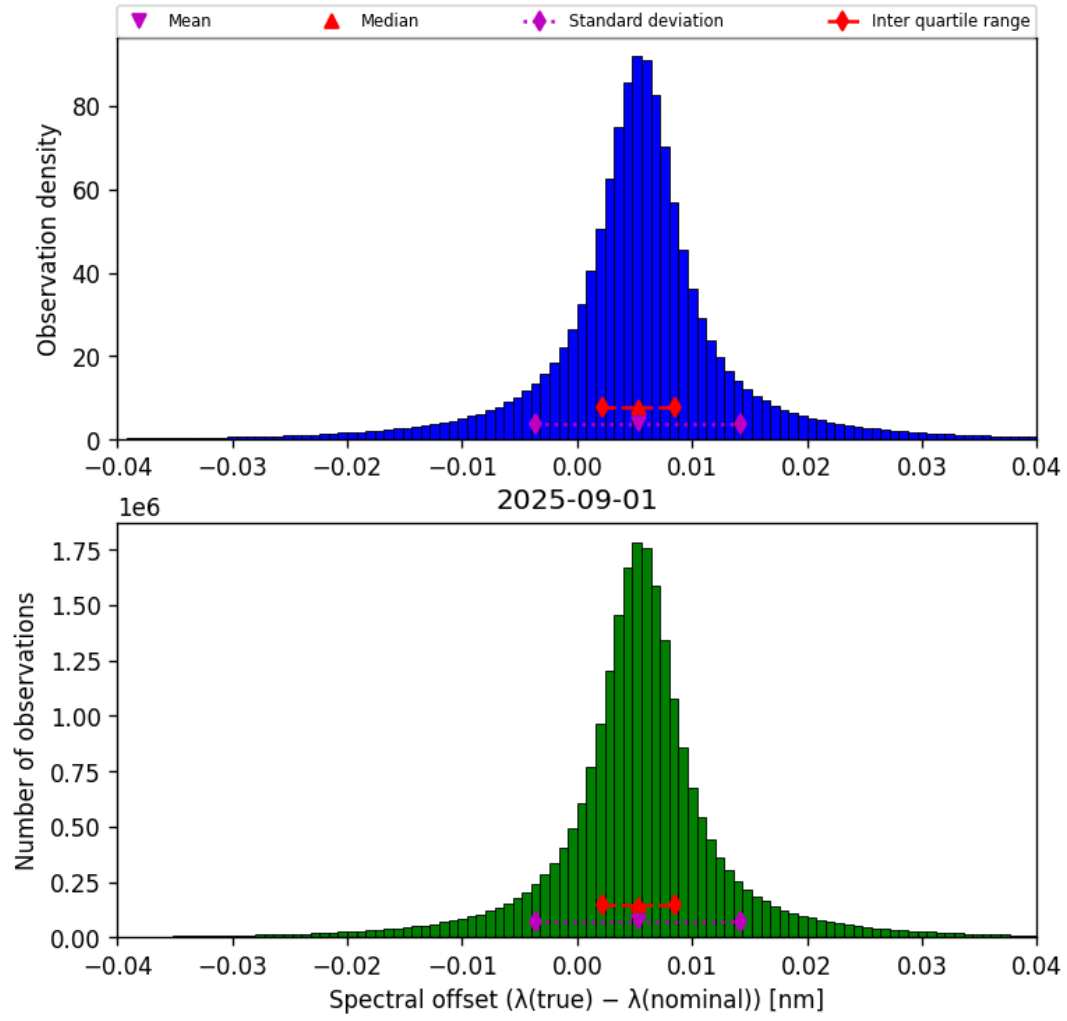
Figure 43: Histogram of “Spectral offset ( \lambda_{\text{true}} - \lambda_{\text{nominal}} )” for 2025-09-01 to 2025-09-02
