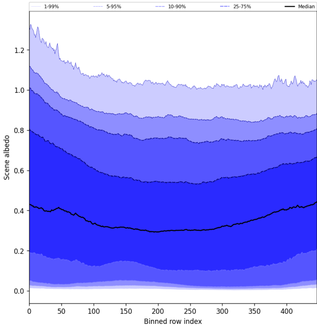
Figure 49: Along track statistics of “Scene albedo” for 2025-09-01 to 2025-09-02
