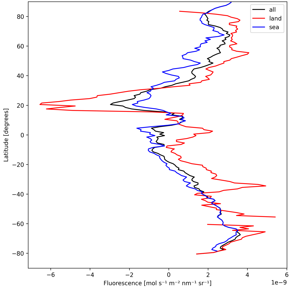
Figure 21: Zonal average of “Fluorescence” for 2025-09-01 to 2025-09-02.
