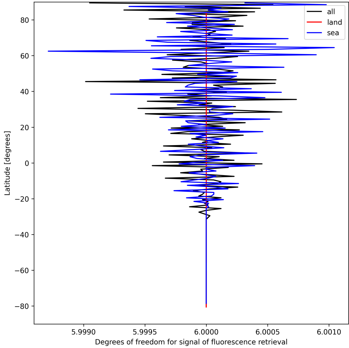
Figure 24: Zonal average of “Degrees of freedom for signal of fluorescence retrieval” for 2025-09-01 to 2025-09-02.
