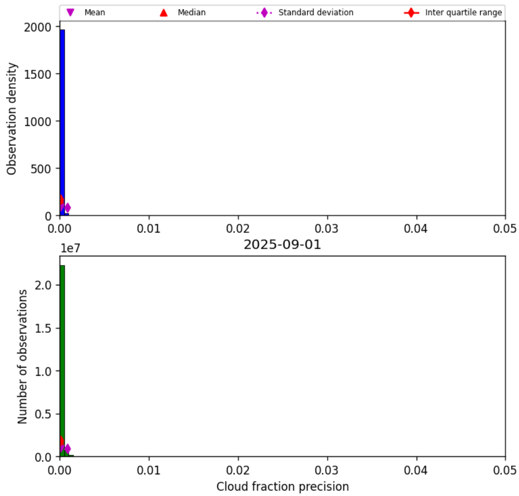
Figure 31: Histogram of “Cloud fraction precision” for 2025-09-01 to 2025-09-02
