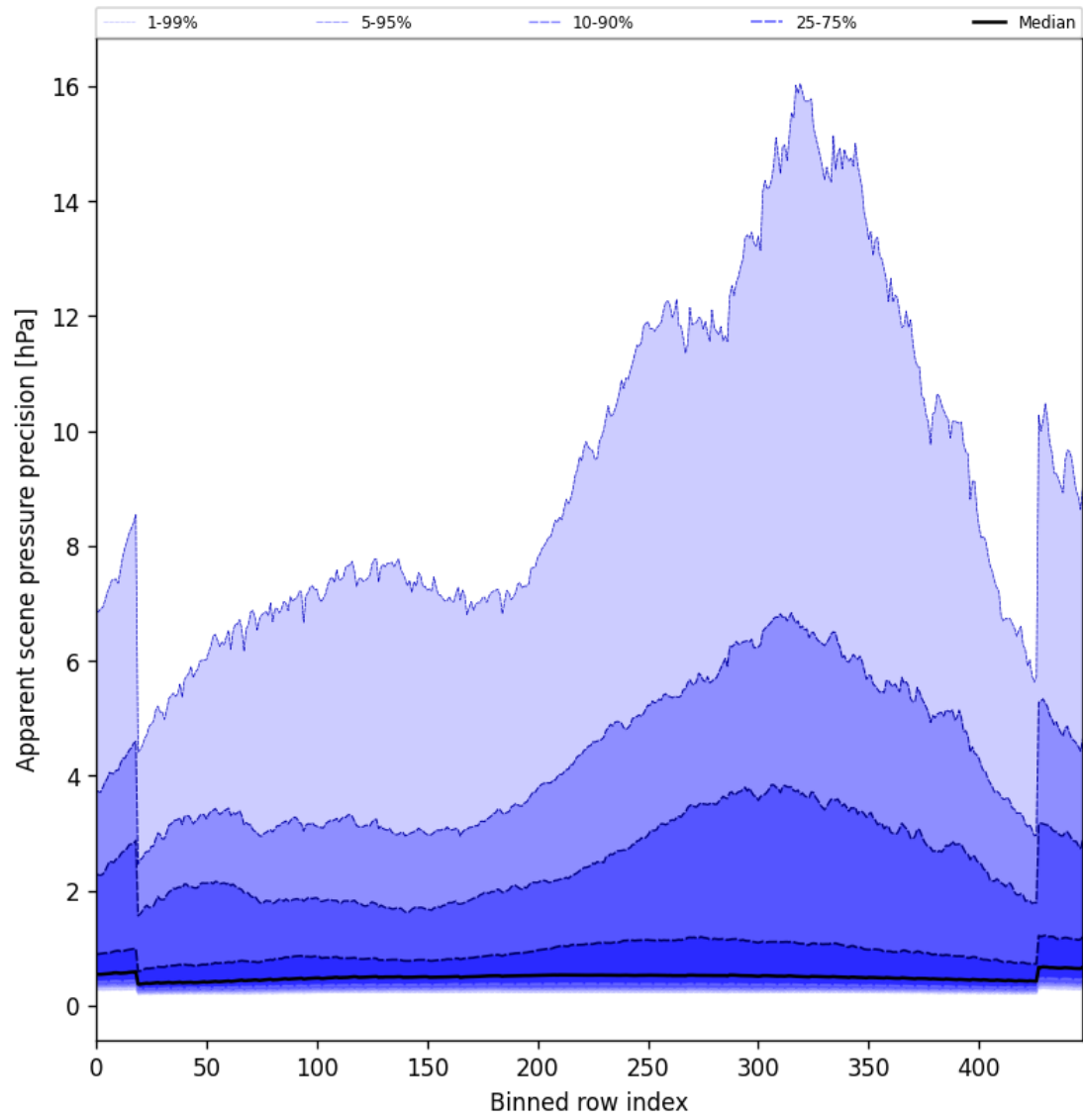
Figure 52: Along track statistics of “Apparent scene pressure precision” for 2025-09-01 to 2025-09-02
