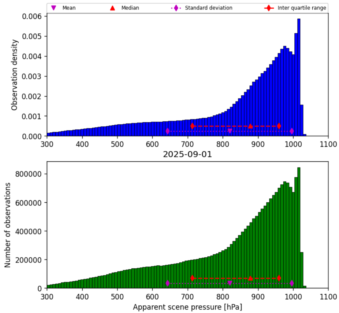
Figure 34: Histogram of “Apparent scene pressure” for 2025-09-01 to 2025-09-02
