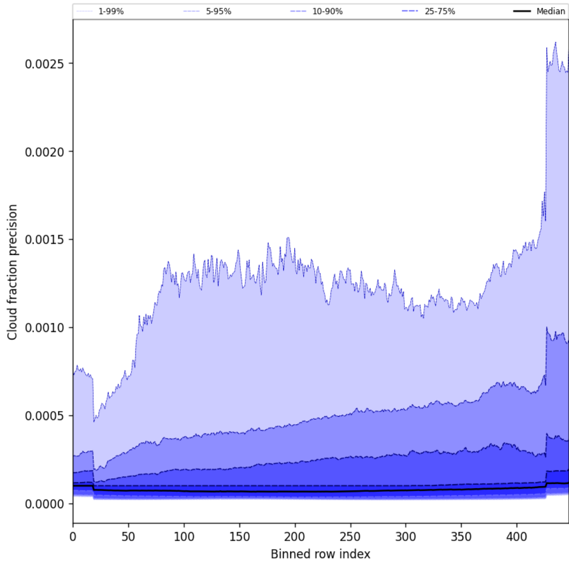
Figure 48: Along track statistics of “Cloud fraction precision” for 2025-09-02 to 2025-09-02
