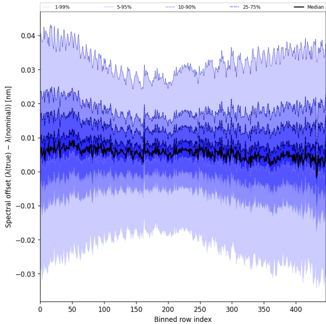
Figure 60: Along track statistics of “Spectral offset ( \lambda_{\text{true}} - \lambda_{\text{nominal}} )” for 2025-09-02 to 2025-09-02
