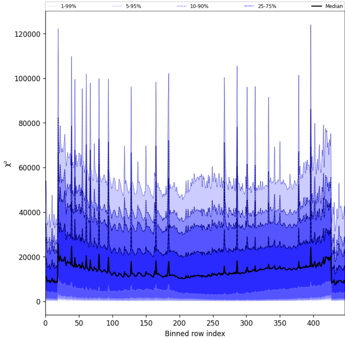
Figure 53: Along track statistics of “ \chi^2 ” for 2025-09-02 to 2025-09-02
