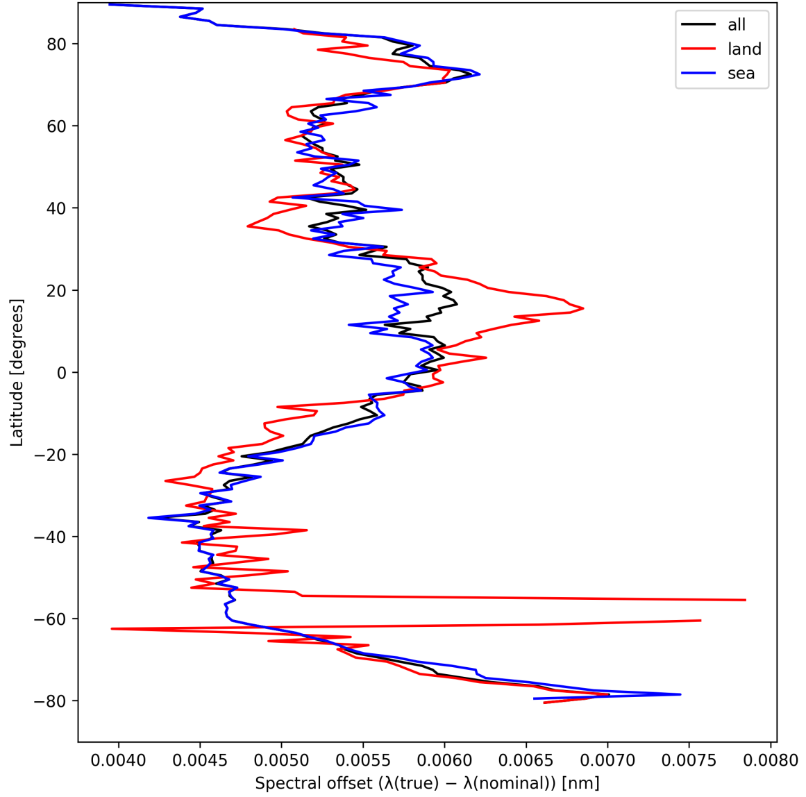
Figure 26: Zonal average of “Spectral offset ( \lambda_{\text{true}} - \lambda_{\text{nominal}} )” for 2025-09-02 to 2025-09-02.
