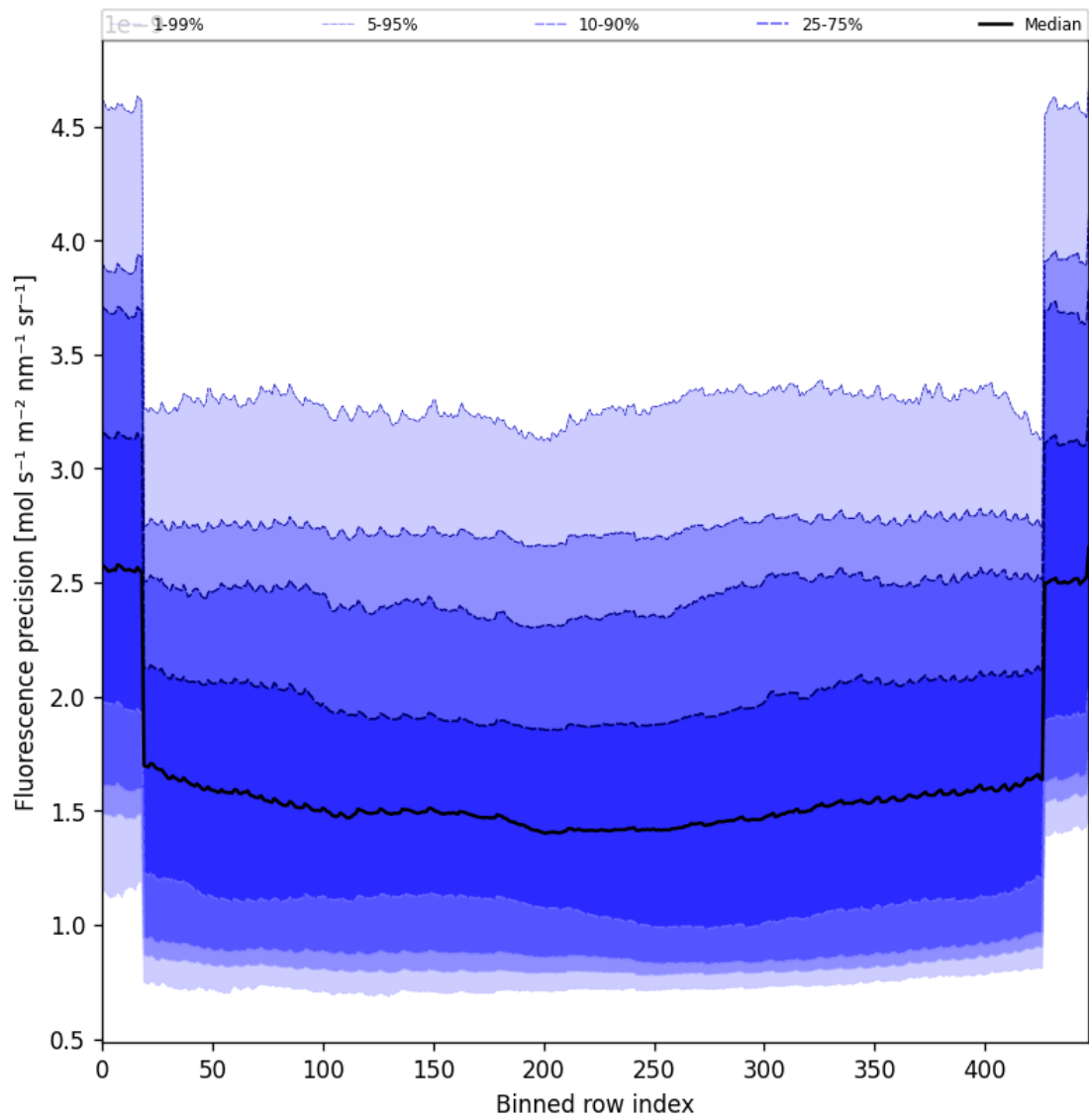
Figure 56: Along track statistics of “Fluorescence precision” for 2025-09-02 to 2025-09-02
