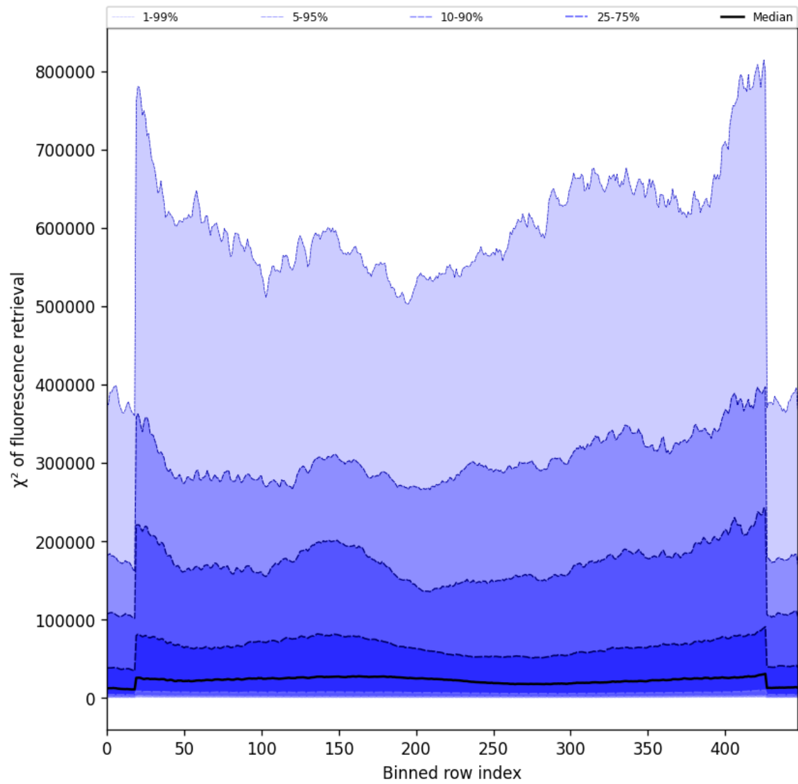
Figure 57: Along track statistics of “ \chi^2 of fluorescence retrieval” for 2025-09-02 to 2025-09-02
