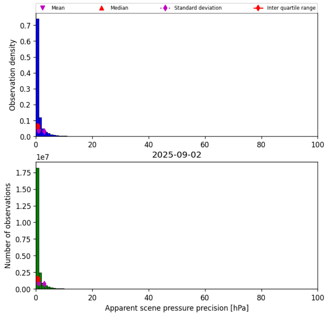
Figure 35: Histogram of “Apparent scene pressure precision” for 2025-09-02 to 2025-09-02
