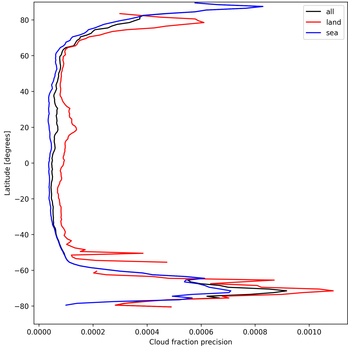
Figure 14: Zonal average of “Cloud fraction precision” for 2025-09-02 to 2025-09-02.
