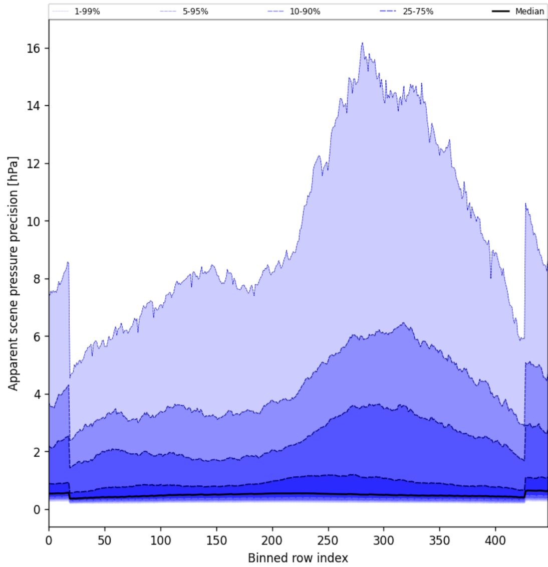
Figure 52: Along track statistics of “Apparent scene pressure precision” for 2025-09-02 to 2025-09-02
