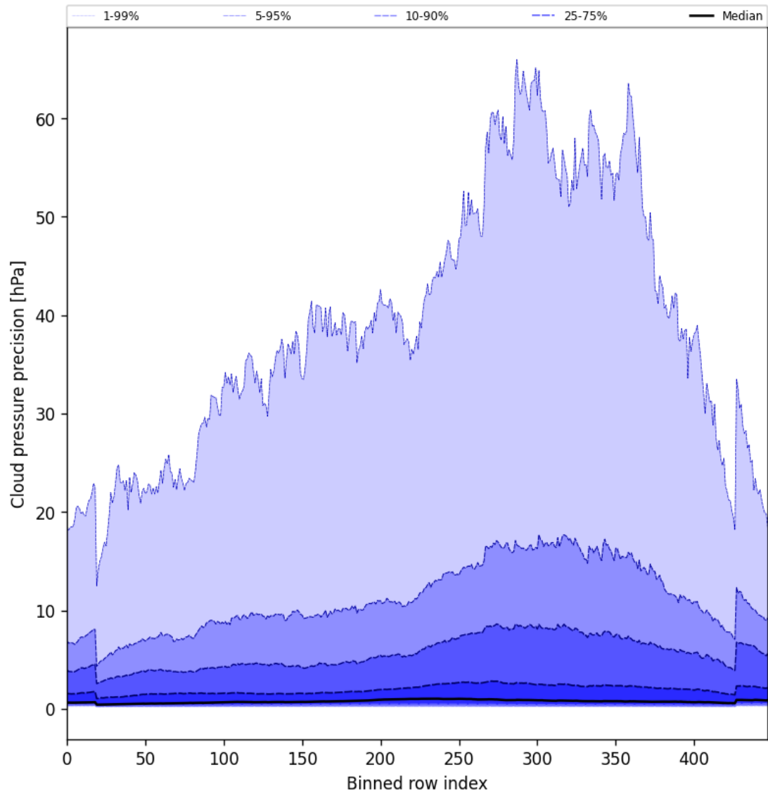
Figure 46: Along track statistics of “Cloud pressure precision” for 2025-09-02 to 2025-09-02
