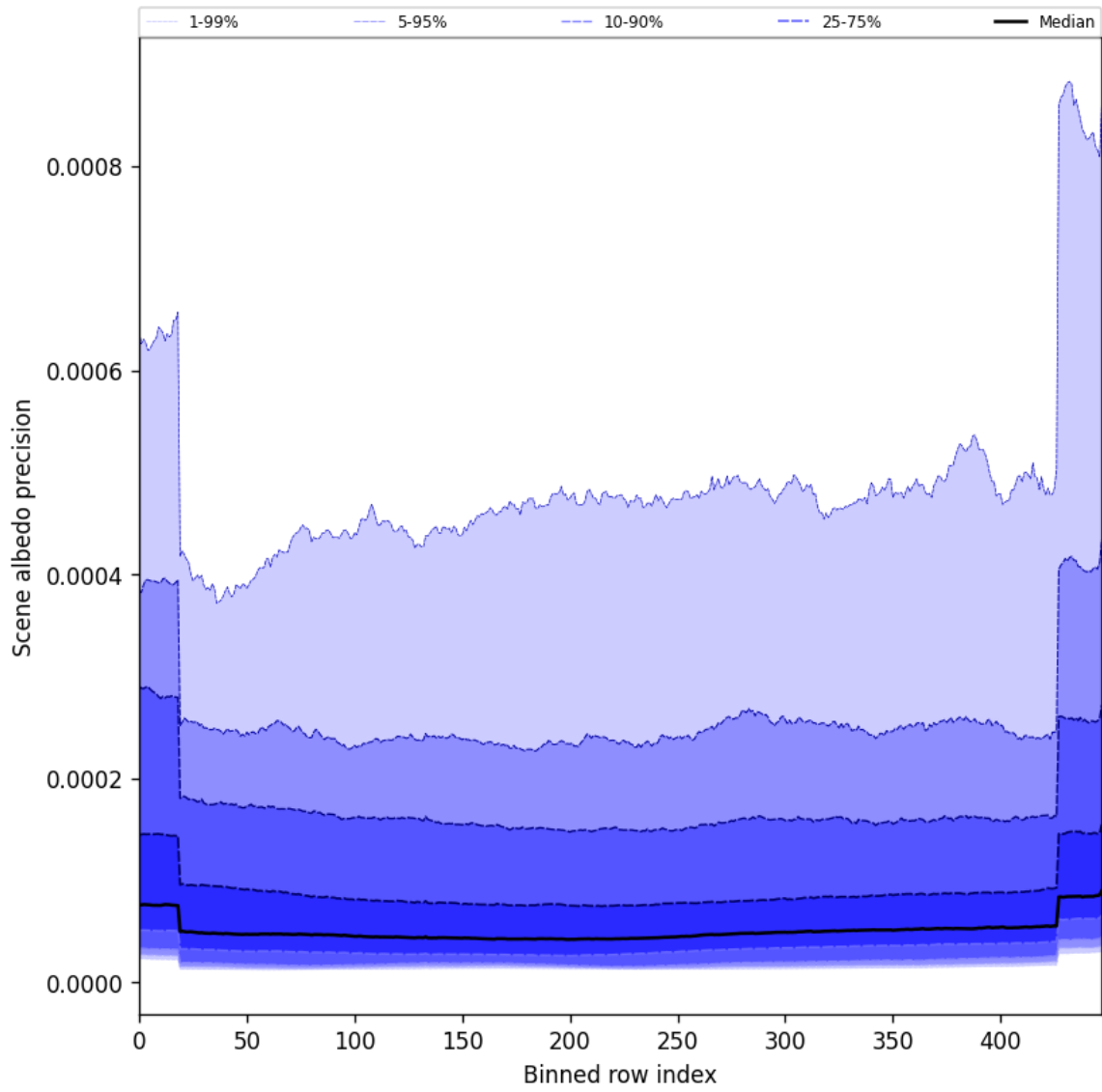
Figure 50: Along track statistics of “Scene albedo precision” for 2025-09-02 to 2025-09-02
