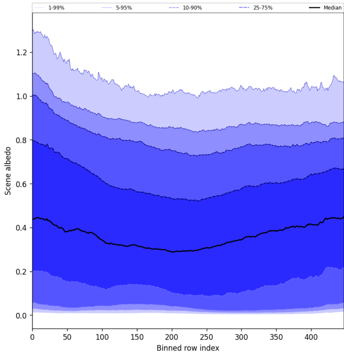
Figure 49: Along track statistics of "Scene albedo" for 2025-09-02 to 2025-09-02
