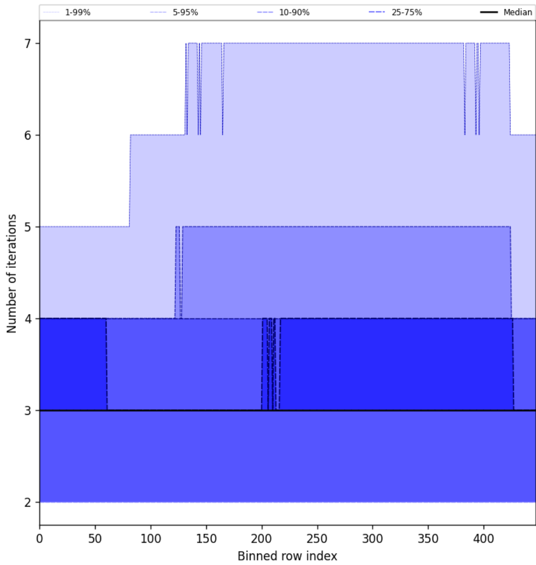
Figure 54: Along track statistics of “Number of iterations” for 2025-09-02 to 2025-09-02
