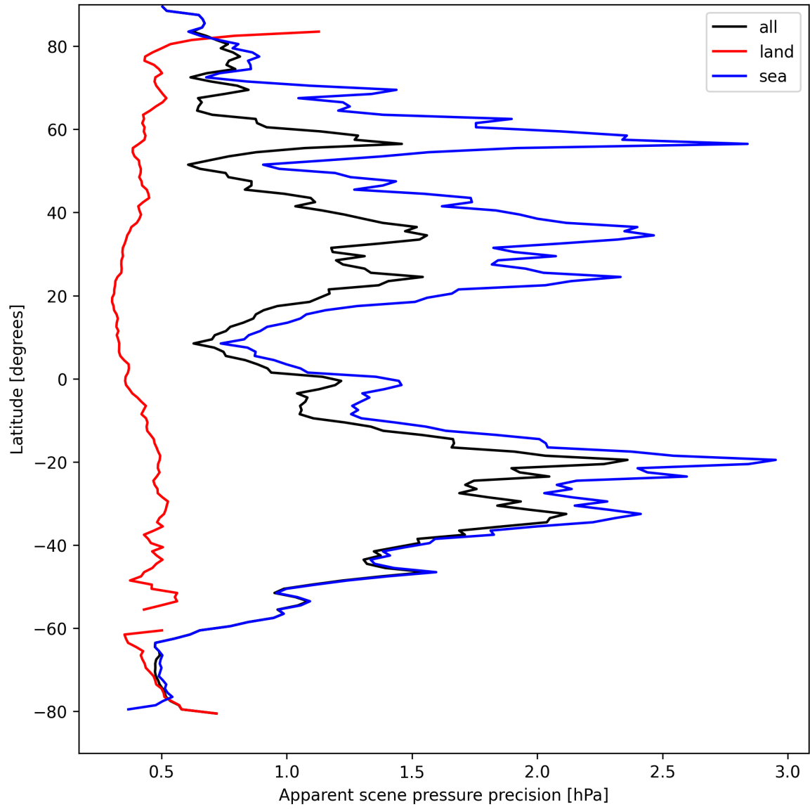
Figure 18: Zonal average of “Apparent scene pressure precision” for 2025-09-02 to 2025-09-02.
