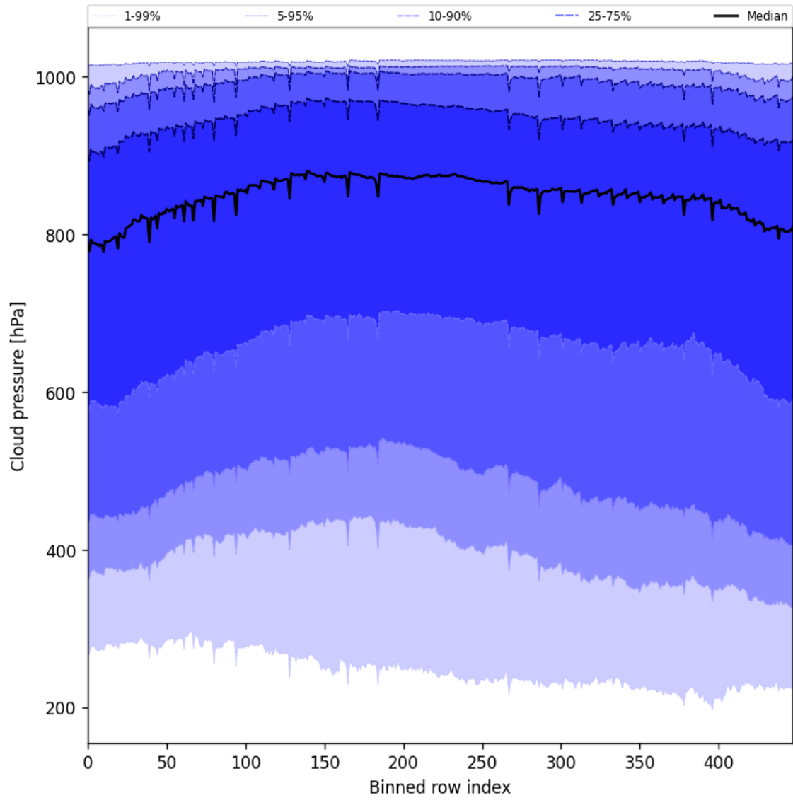
Figure 45: Along track statistics of “Cloud pressure” for 2025-09-02 to 2025-09-02
