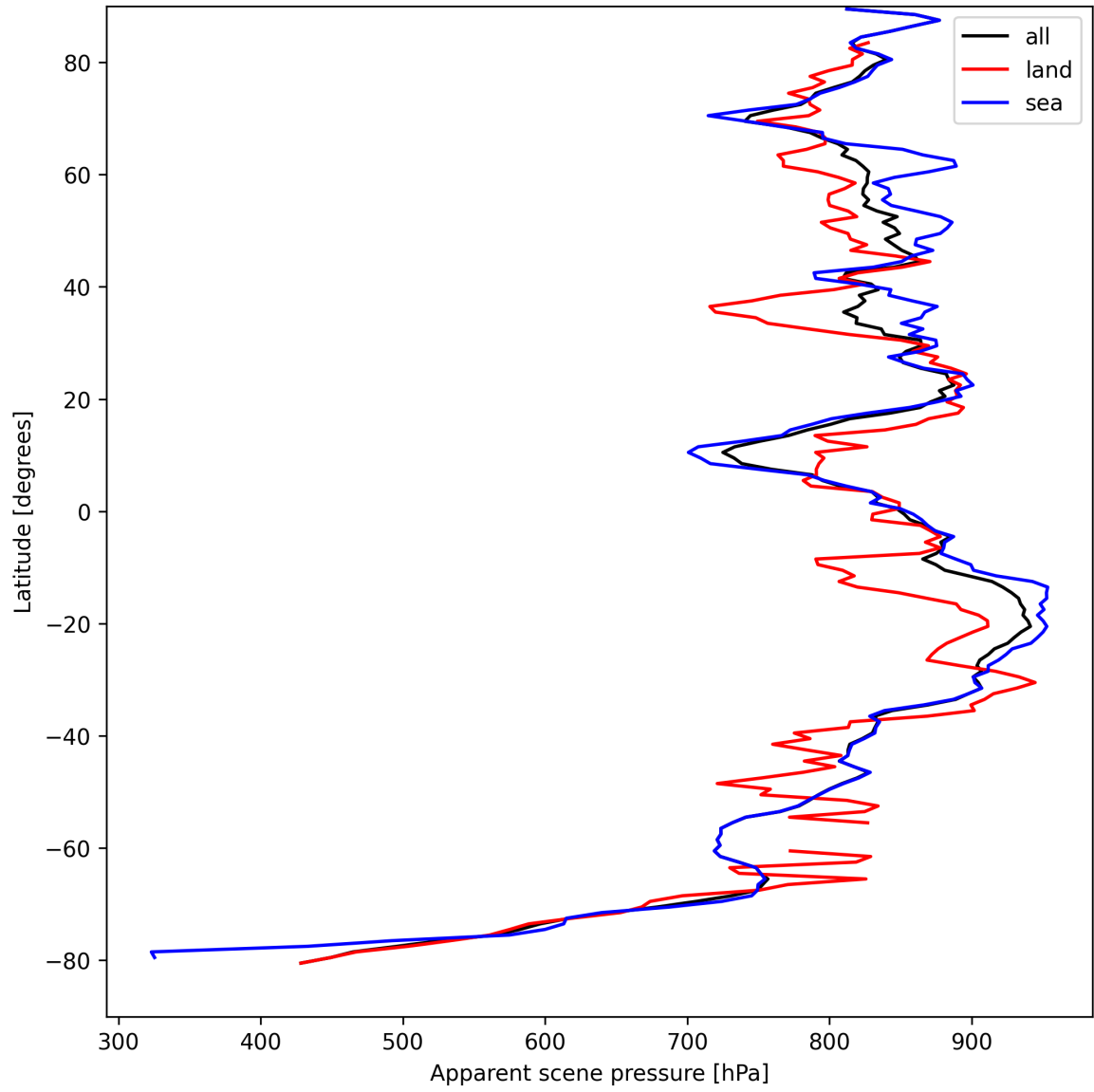
Figure 17: Zonal average of “Apparent scene pressure” for 2025-09-02 to 2025-09-02.
