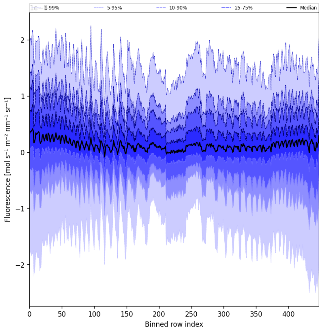
Figure 55: Along track statistics of “Fluorescence” for 2025-09-02 to 2025-09-02
